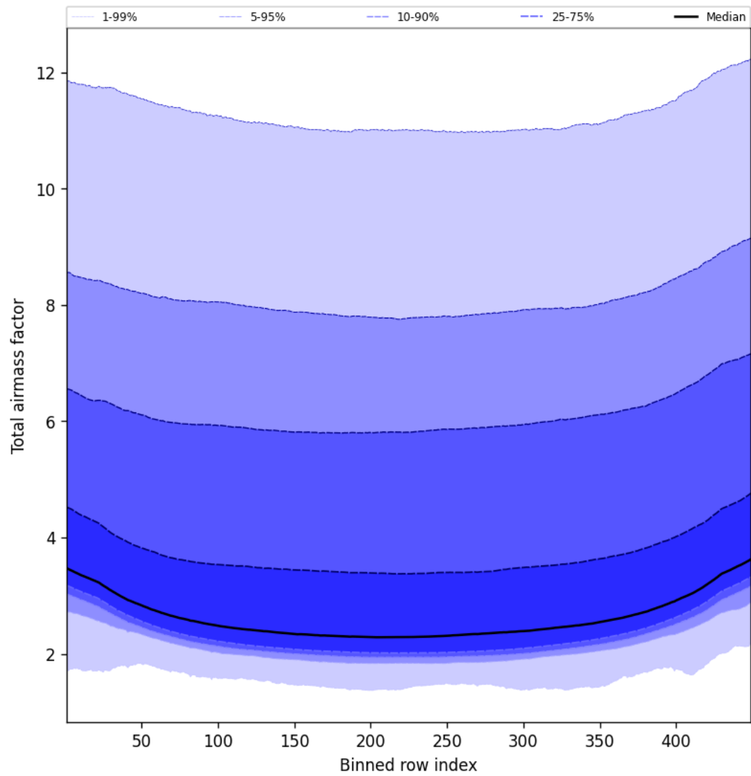
Figure 49: Along track statistics of “Total airmass factor” for 2025-03-01 to 2025-03-02
