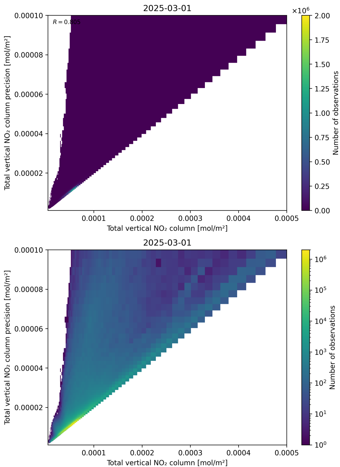
Figure 114: Scatter density plot of “Total vertical NO 2 column” against “Total vertical NO 2 column precision” for 2025-03-01 to 2025-03-02.
