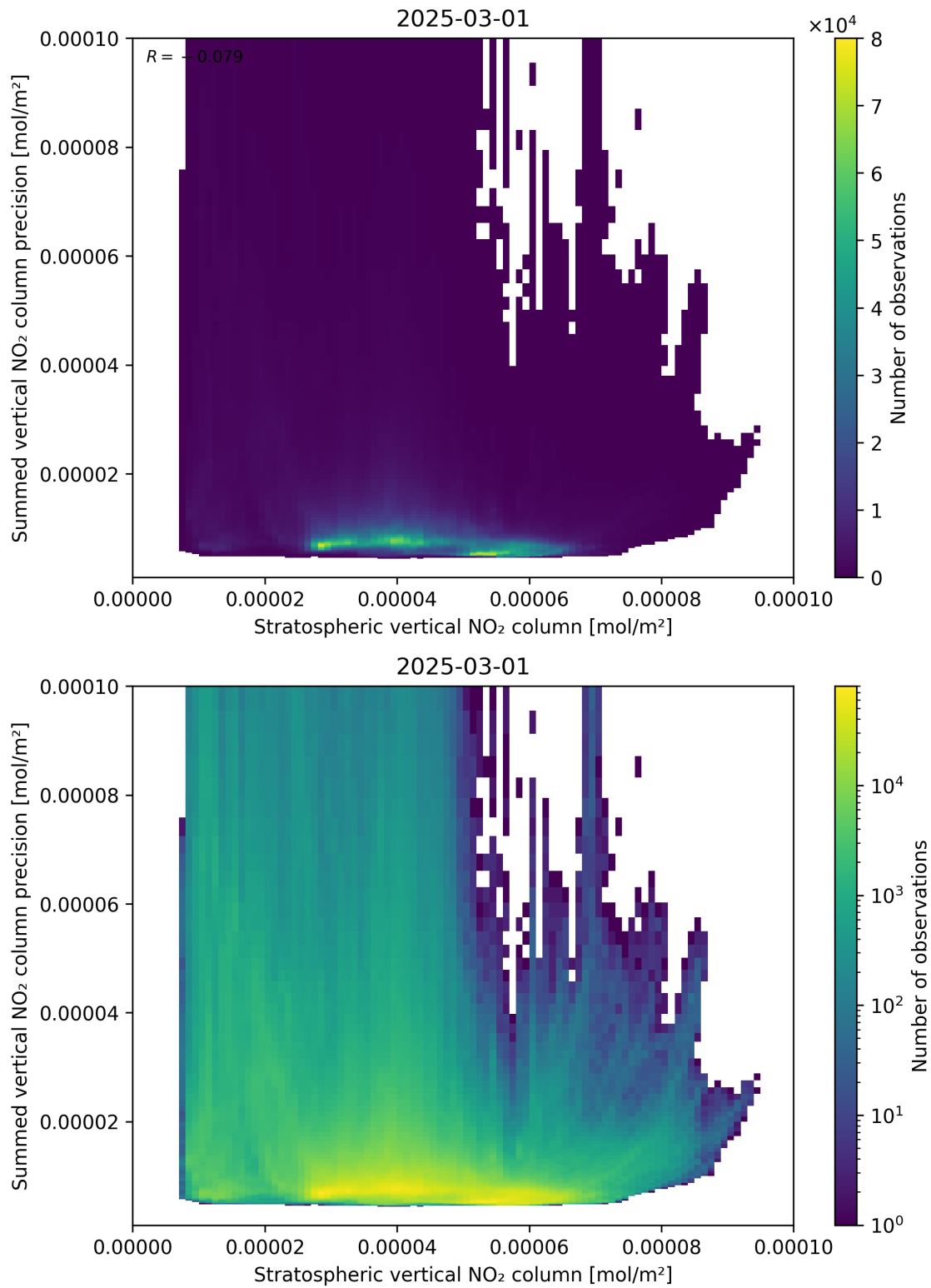
Figure 99: Scatter density plot of “Stratospheric vertical NO 2 column” against “Summed vertical NO 2 column precision” for 2025-03-01 to 2025-03-02.
