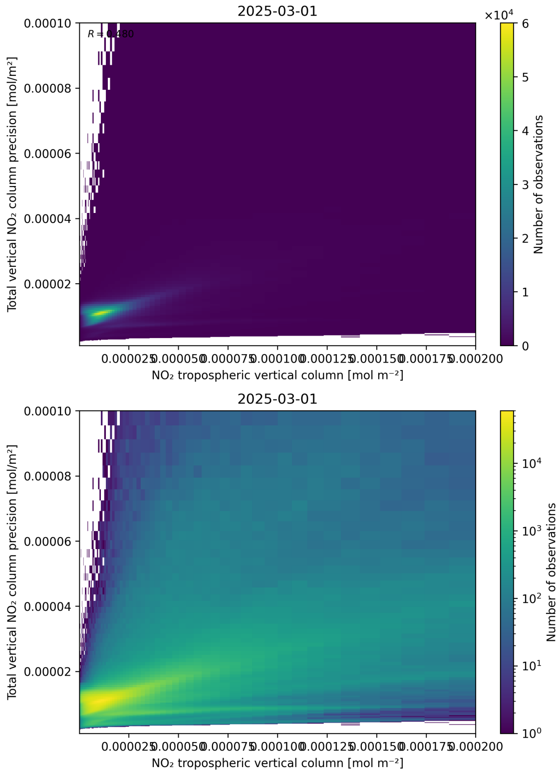
Figure 129: Scatter density plot of “NO 2 tropospheric vertical column” against “Total vertical NO 2 column precision” for 2025-03-01 to 2025-03-02.
