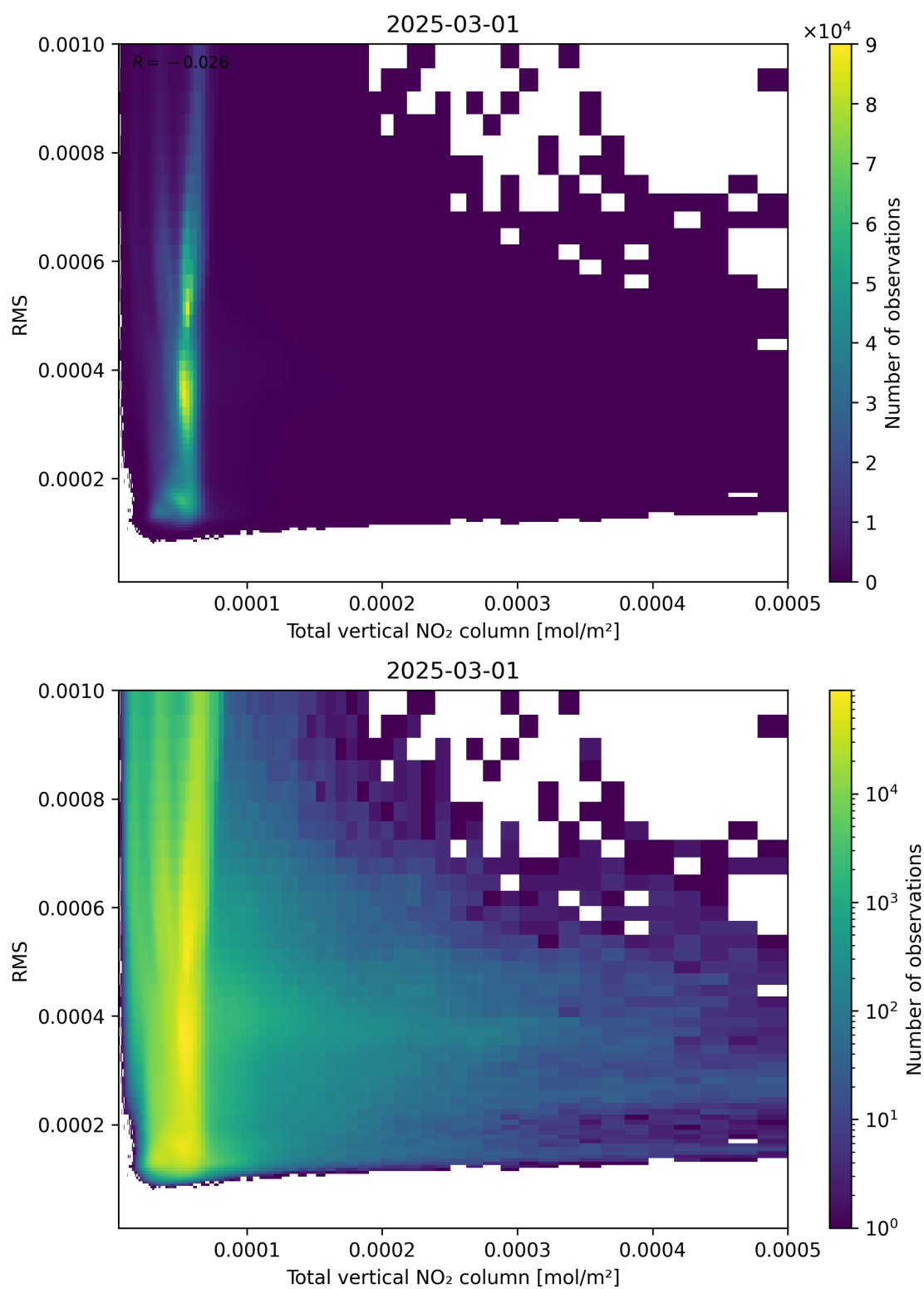
Figure 120: Scatter density plot of “Total vertical NO 2 column” against “RMS” for 2025-03-01 to 2025-03-02.
