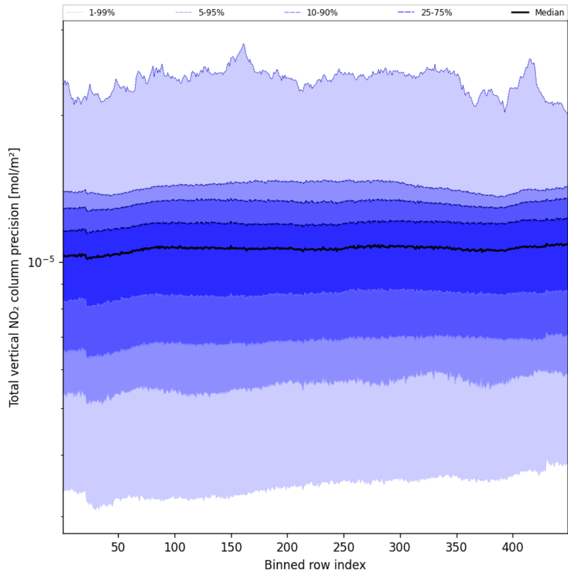
Figure 56: Along track statistics of “Total vertical NO 2 column precision” for 2025-03-01 to 2025-03-02
