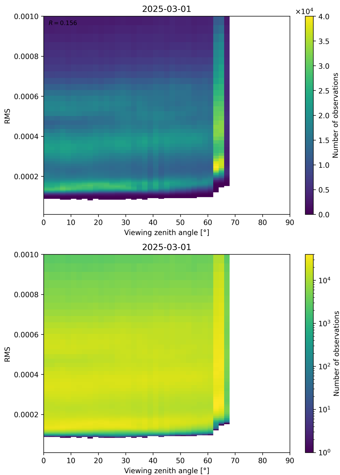
Figure 171: Scatter density plot of “Viewing zenith angle” against “RMS” for 2025-03-01 to 2025-03-02.
