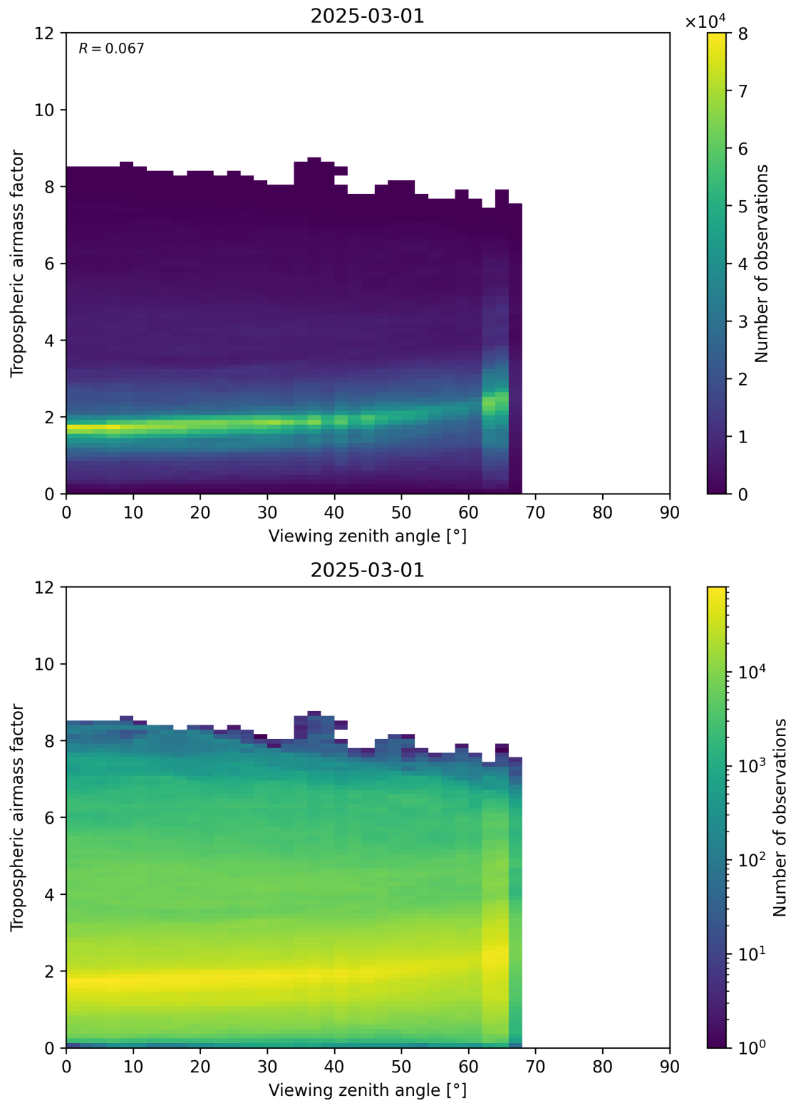
Figure 161: Scatter density plot of “Viewing zenith angle” against “Tropospheric airmass factor” for 2025-03-01 to 2025-03-02.
