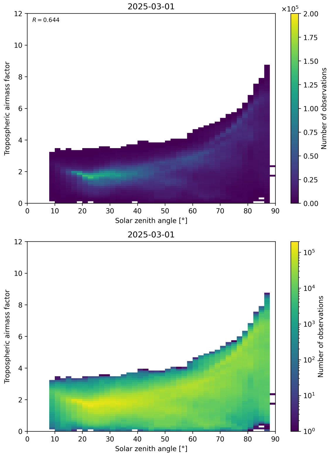
Figure 147: Scatter density plot of “Solar zenith angle” against “Tropospheric airmass factor” for 2025-03-01 to 2025-03-02.
