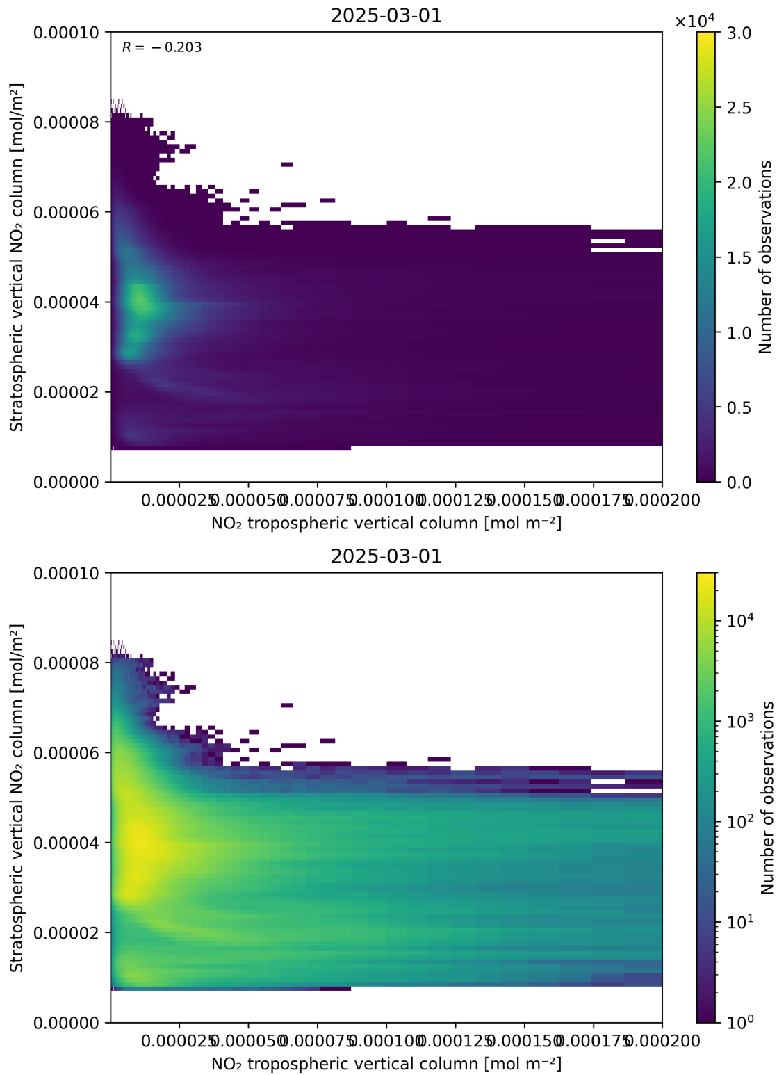
Figure 125: Scatter density plot of “NO 2 tropospheric vertical column” against “Stratospheric vertical NO 2 column” for 2025-03-01 to 2025-03-02.
