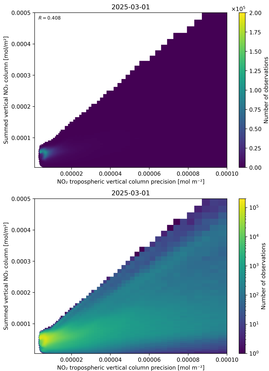
Figure 136: Scatter density plot of “NO 2 tropospheric vertical column precision” against “Summed vertical NO 2 column” for 2025-03-01 to 2025-03-02.
