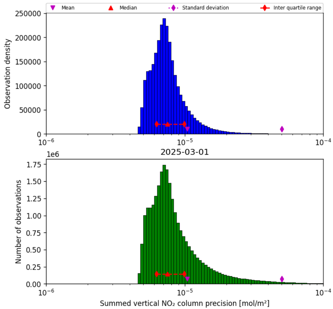
Figure 41: Histogram of “Summed vertical NO 2 column precision” for 2025-03-01 to 2025-03-02
