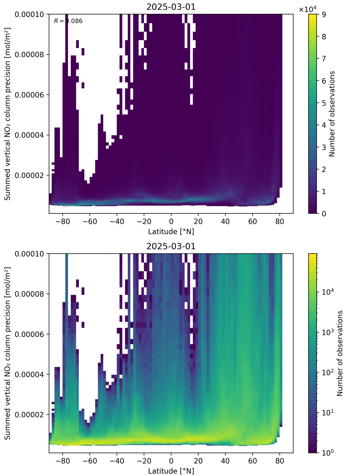
Figure 89: Scatter density plot of “Latitude” against “Summed vertical NO 2 column precision” for 2025-03-01 to 2025-03-02.
