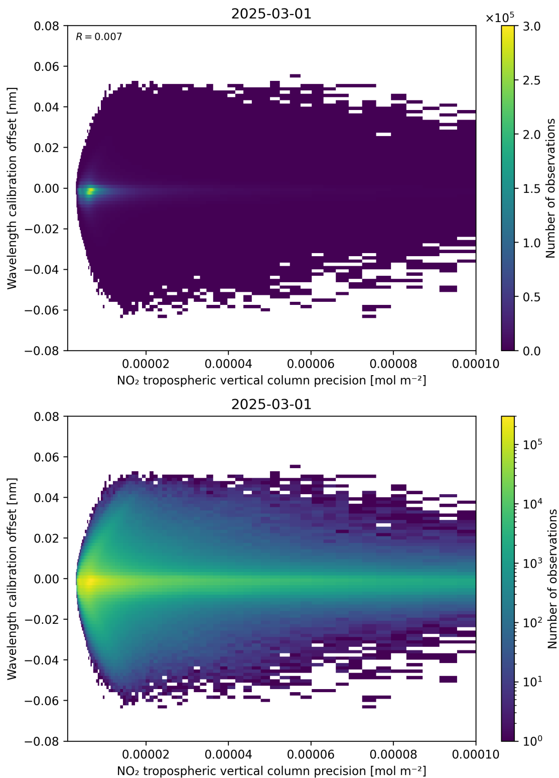
Figure 141: Scatter density plot of “NO 2 tropospheric vertical column precision” against “Wavelength calibration offset” for 2025-03-01 to 2025-03-02.
