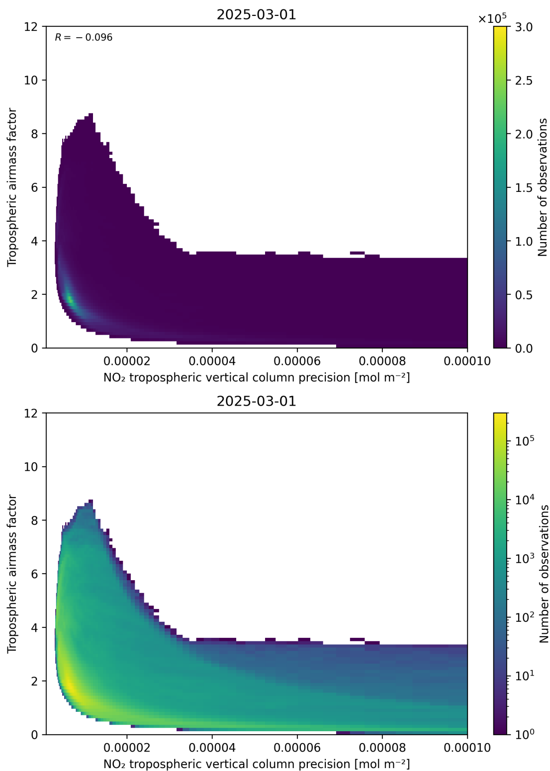
Figure 133: Scatter density plot of “NO 2 tropospheric vertical column precision” against “Tropospheric airmass factor” for 2025-03-01 to 2025-03-02.
