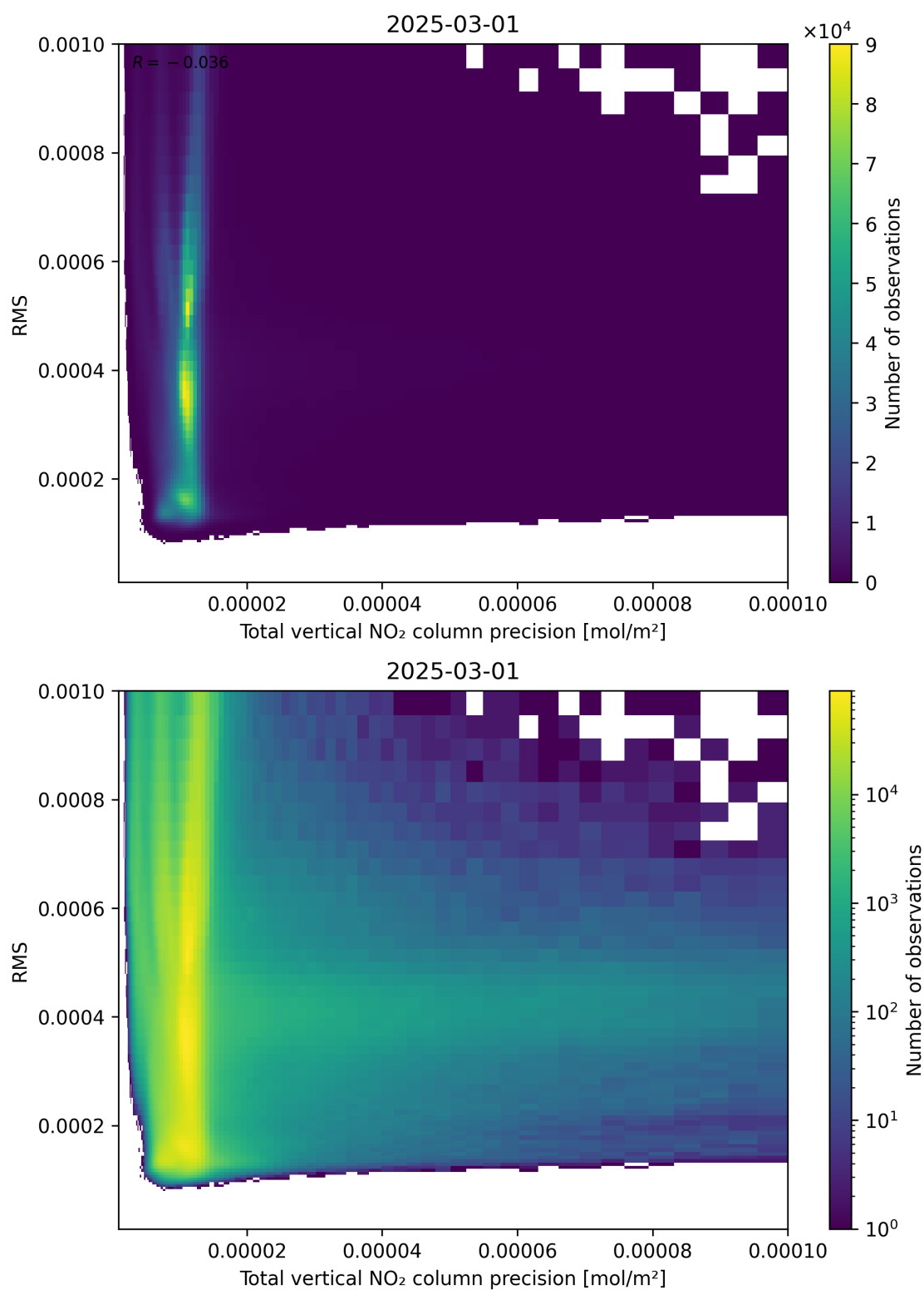
Figure 119: Scatter density plot of “Total vertical NO 2 column precision” against “RMS” for 2025-03-01 to 2025-03-02.
