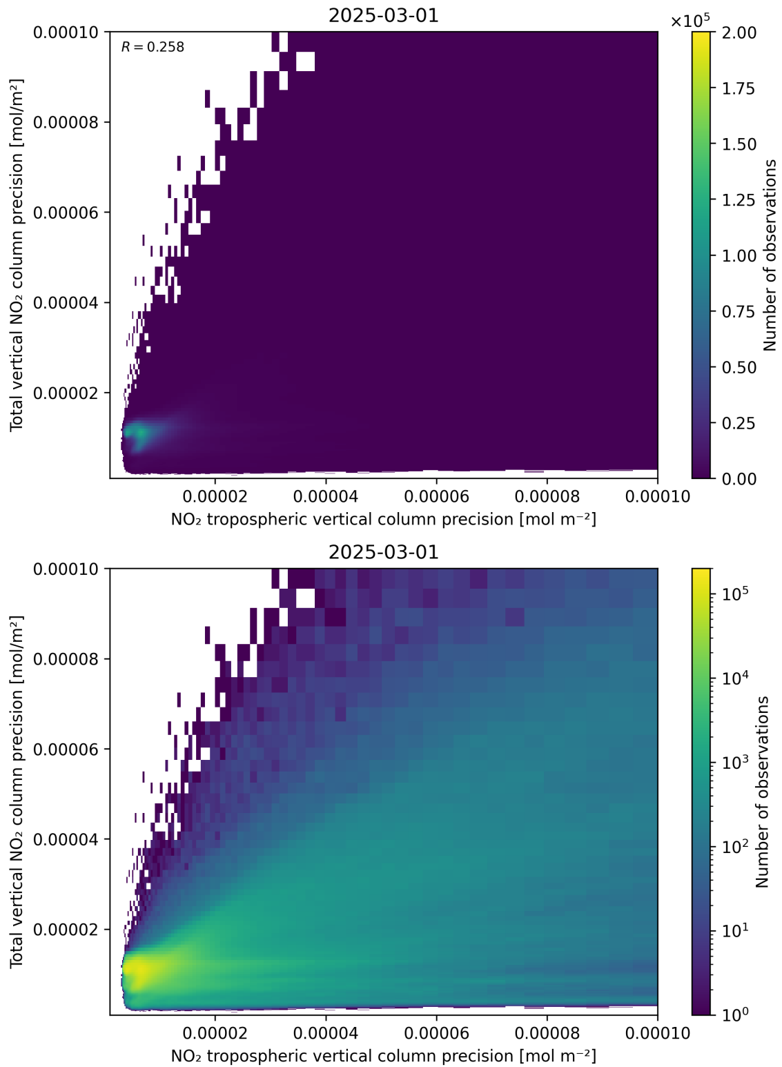
Figure 139: Scatter density plot of “NO 2 tropospheric vertical column precision” against “Total vertical NO 2 column precision” for 2025-03-01 to 2025-03-02.
