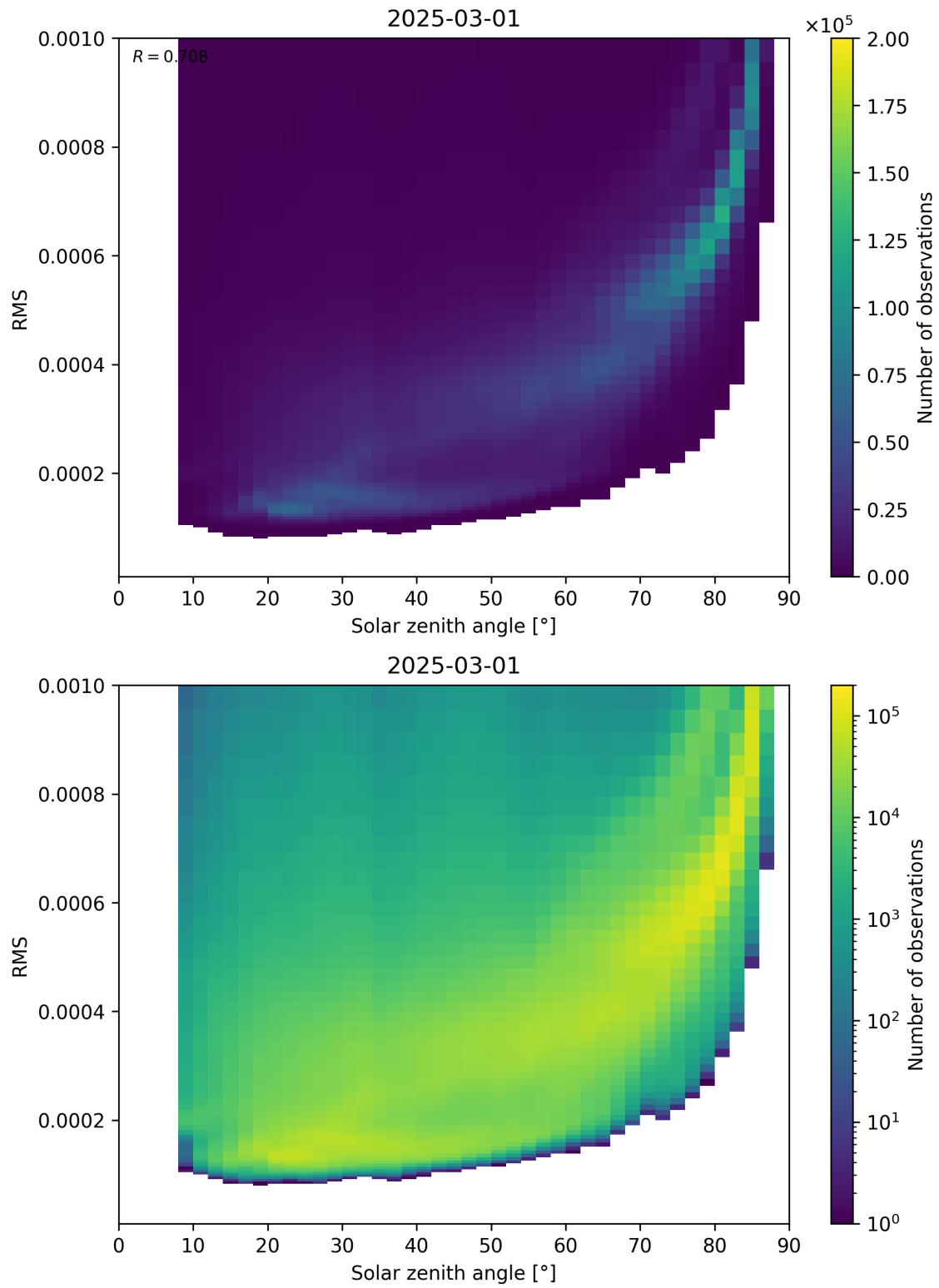
Figure 157: Scatter density plot of “Solar zenith angle” against “RMS” for 2025-03-01 to 2025-03-02.
