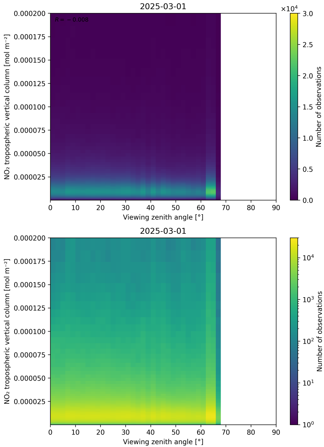
Figure 169: Scatter density plot of “Viewing zenith angle” against “NO 2 tropospheric vertical column” for 2025-03-01 to 2025-03-02.
