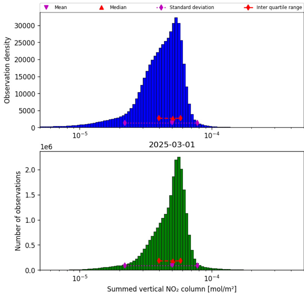
Figure 40: Histogram of “Summed vertical NO 2 column” for 2025-03-01 to 2025-03-02
