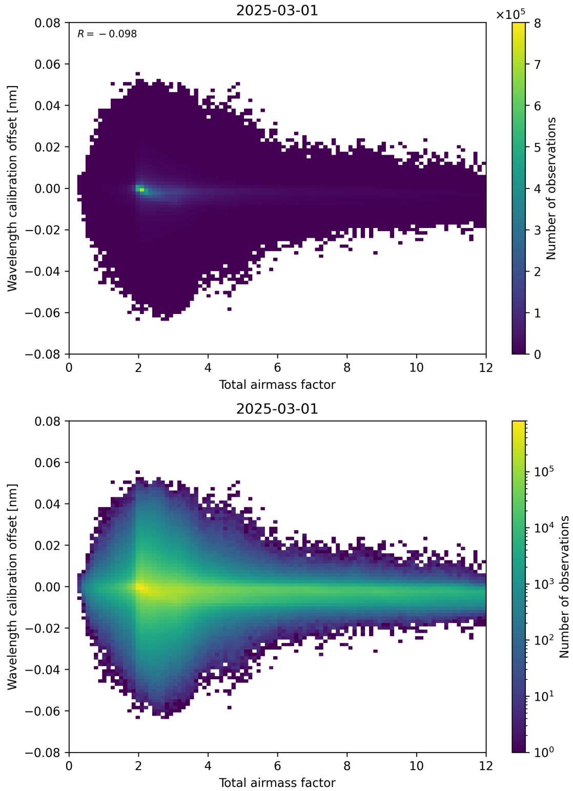
Figure 70: Scatter density plot of “Total airmass factor” against “Wavelength calibration offset” for 2025-03-01 to 2025-03-02.
