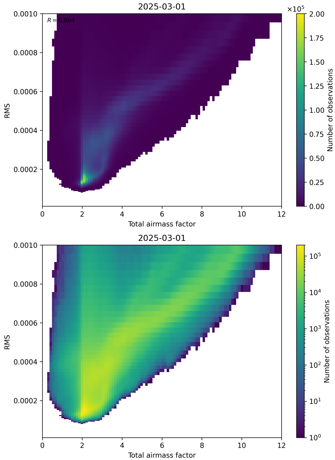
Figure 69: Scatter density plot of “Total airmass factor” against “RMS” for 2025-03-01 to 2025-03-02.
