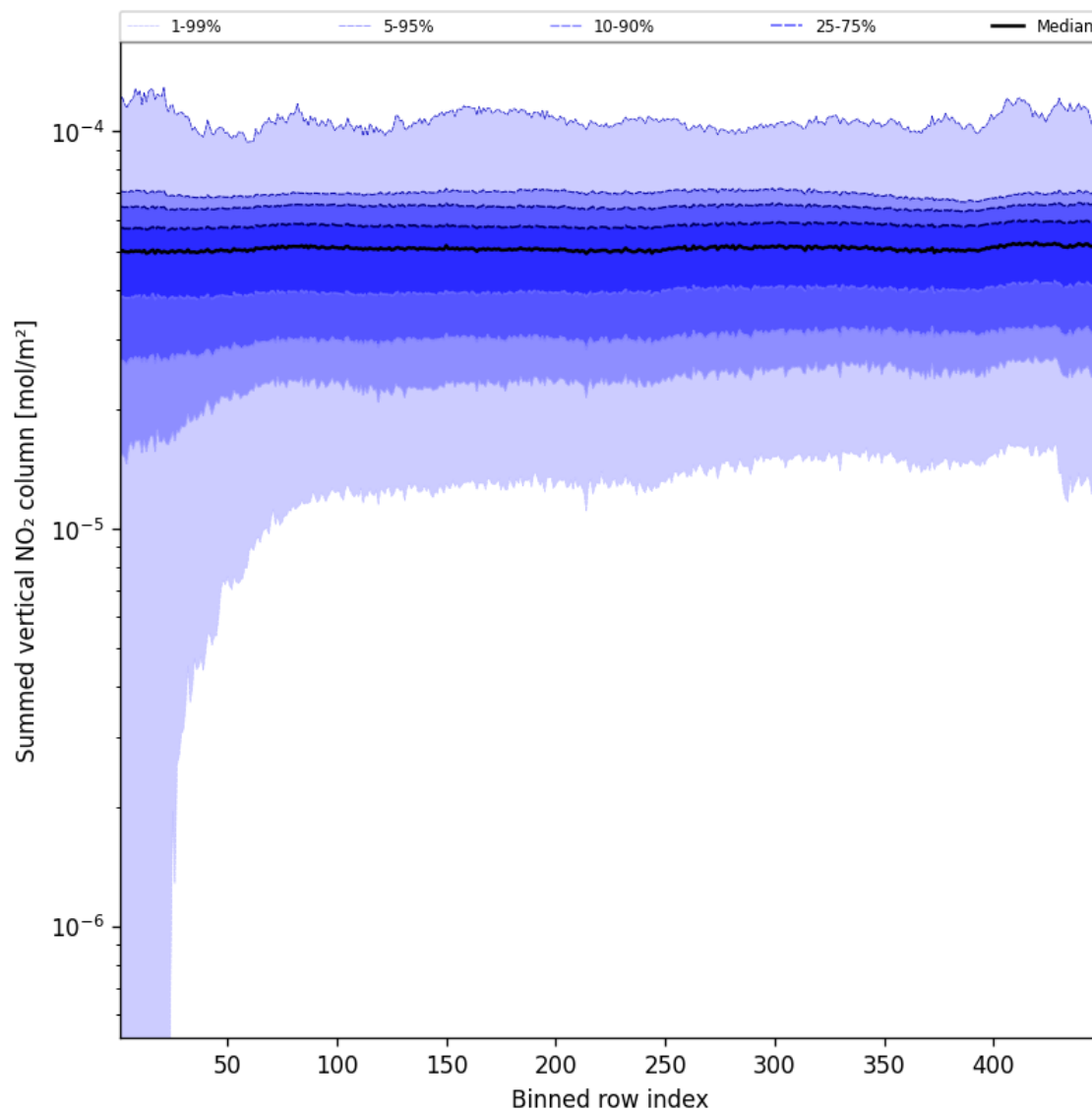
Figure 57: Along track statistics of “Summed vertical NO 2 column” for 2025-03-01 to 2025-03-02
