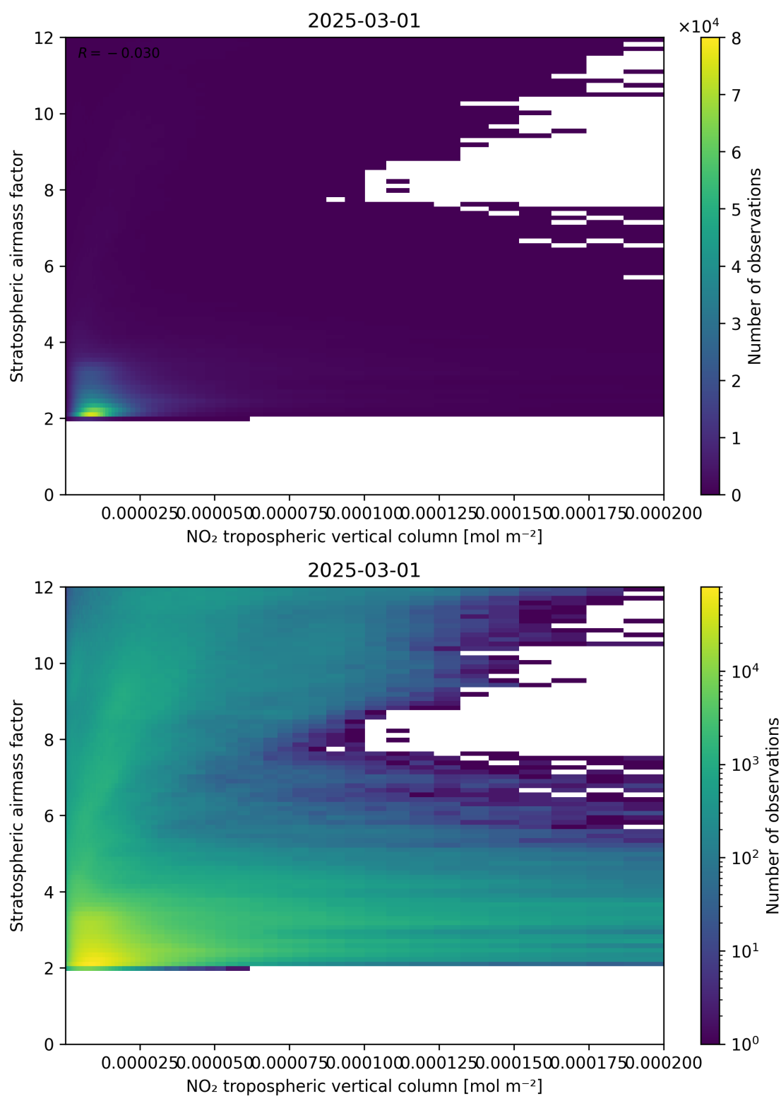
Figure 121: Scatter density plot of “NO 2 tropospheric vertical column” against “Stratospheric air mass factor” for 2025-03-01 to 2025-03-02.
