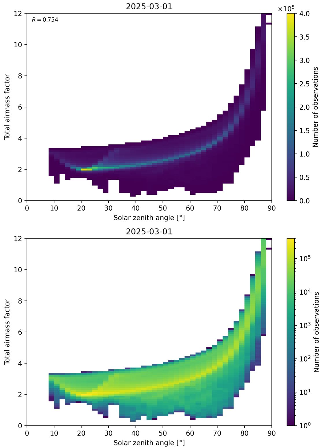
Figure 146: Scatter density plot of “Solar zenith angle” against “Total air mass factor” for 2025-03-01 to 2025-03-02.
