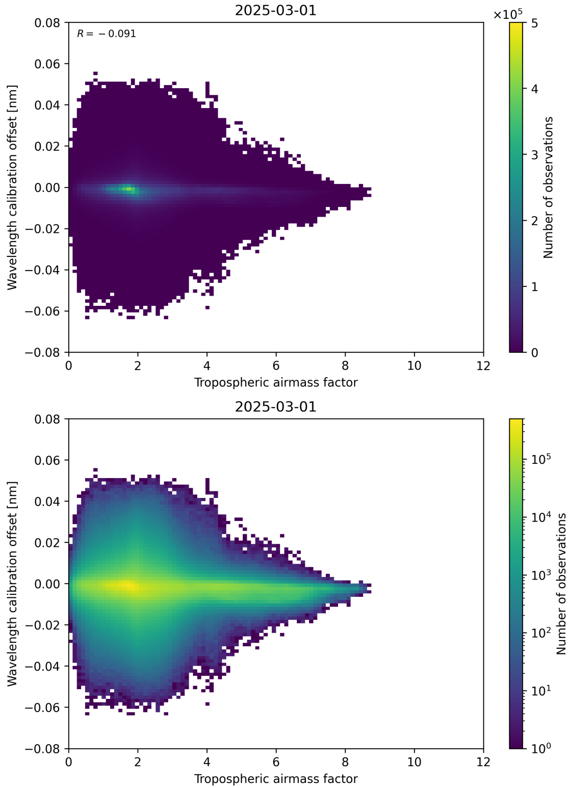
Figure 80: Scatter density plot of “Tropospheric airmass factor” against “Wavelength calibration offset” for 2025-03-01 to 2025-03-02.
