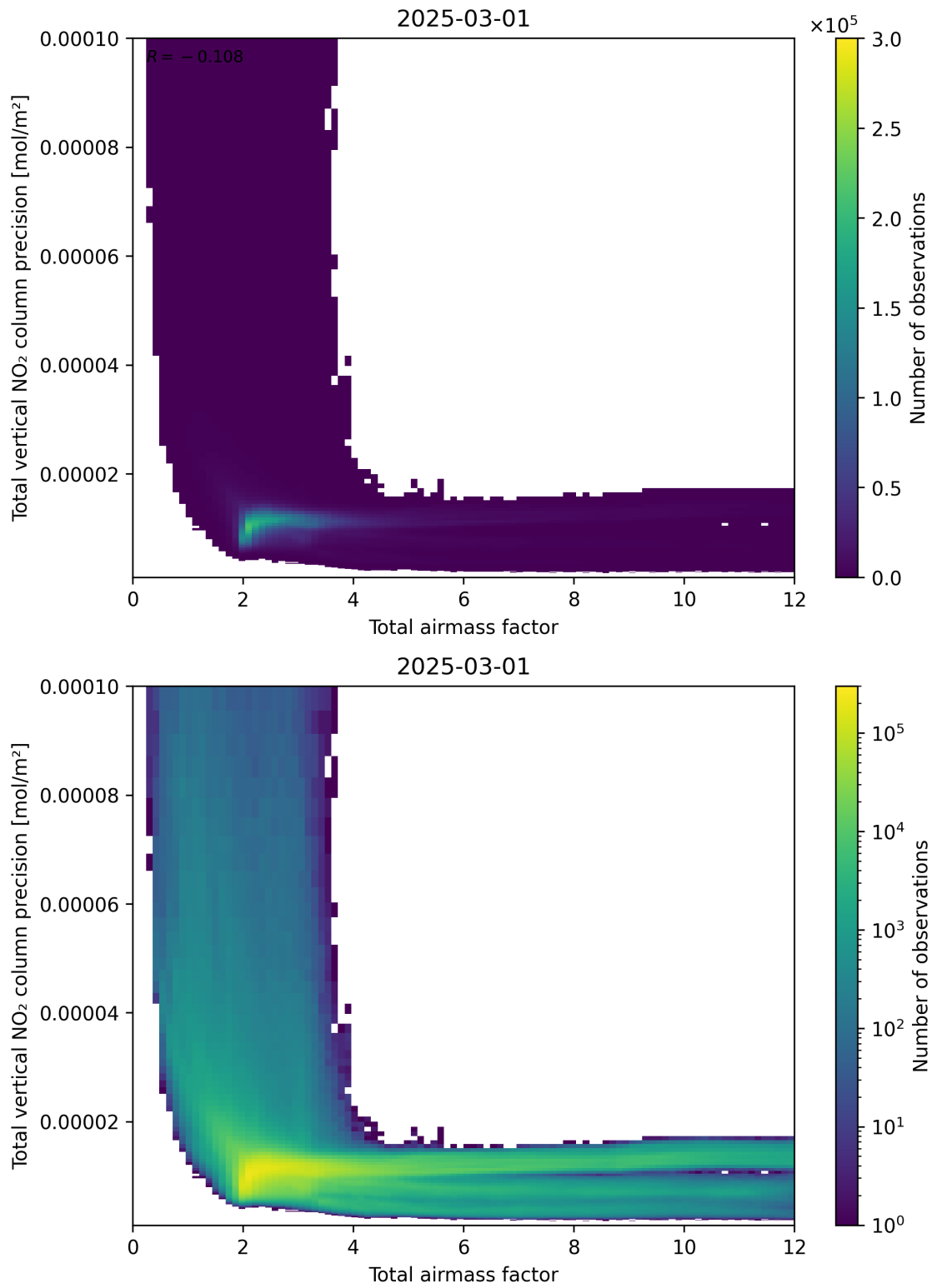
Figure 68: Scatter density plot of “Total airmass factor” against “Total vertical NO 2 column precision” for 2025-03-01 to 2025-03-02.
