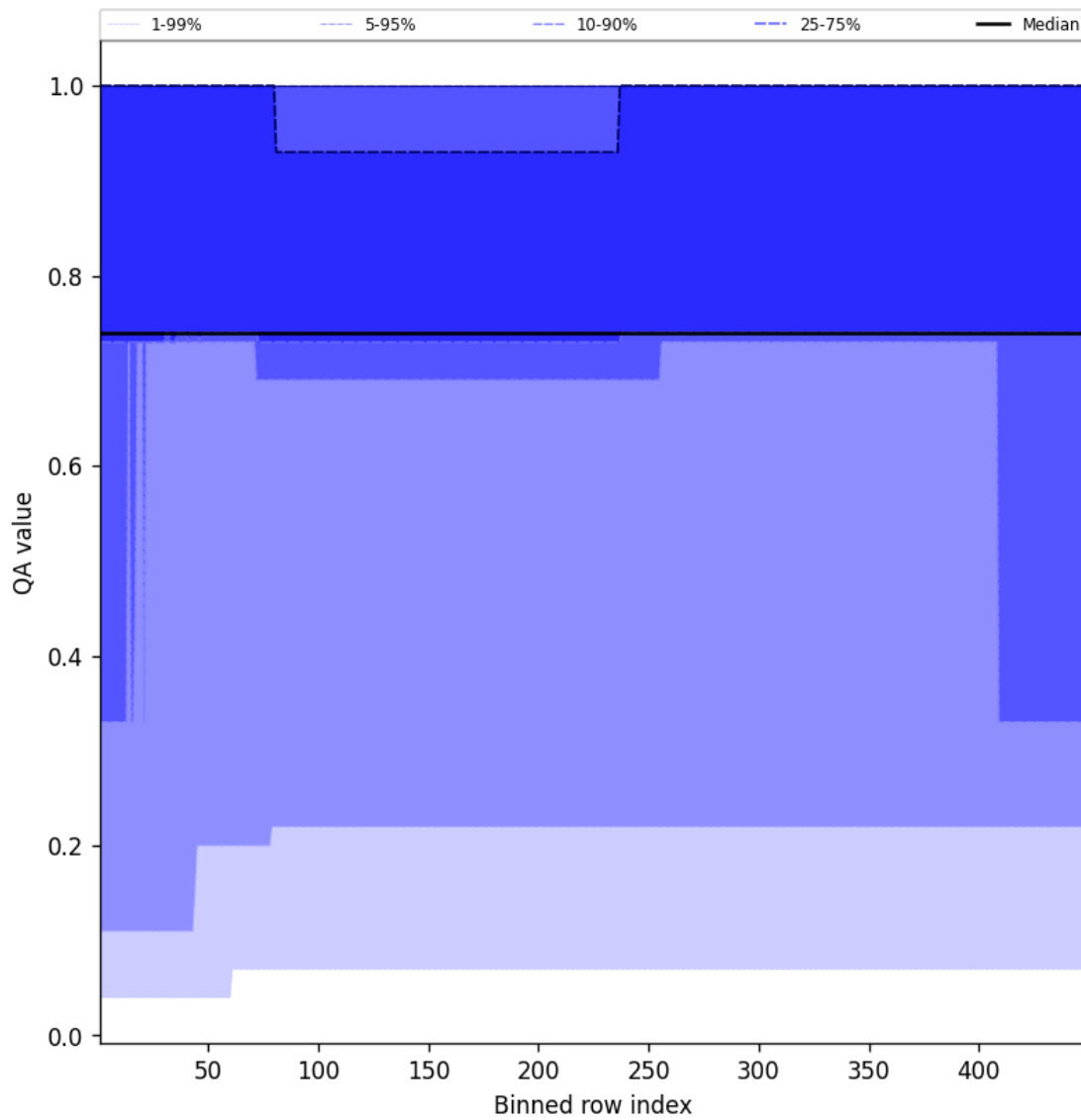
Figure 45: Along track statistics of “QA value” for 2025-03-01 to 2025-03-02
