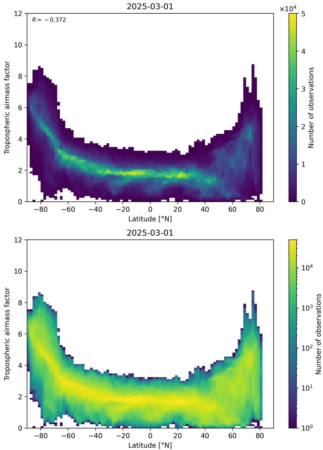
Figure 85: Scatter density plot of “Latitude” against “Tropospheric airmass factor” for 2025-03-01 to 2025-03-02.
