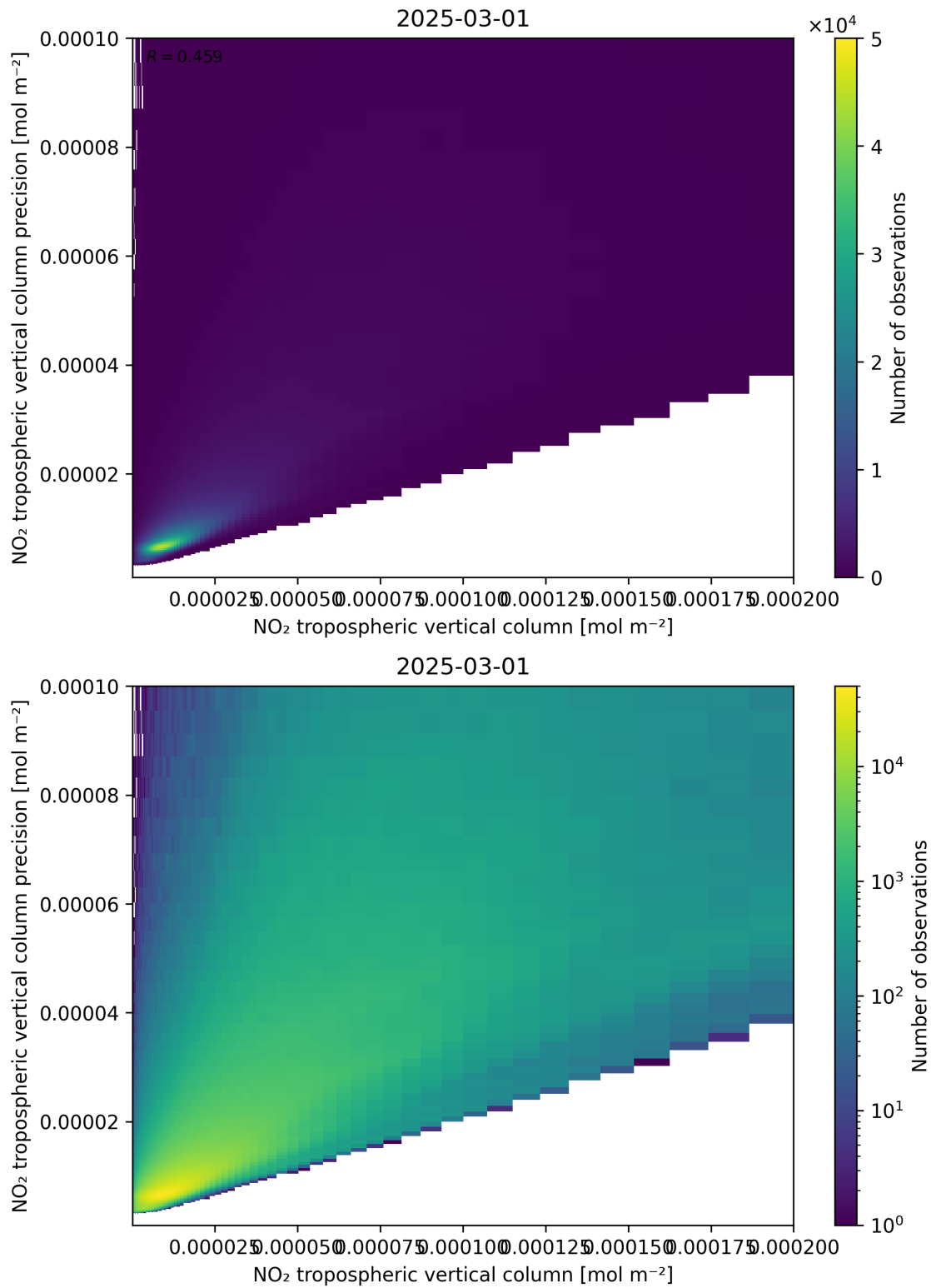
Figure 130: Scatter density plot of “NO 2 tropospheric vertical column” against “NO 2 tropospheric vertical column precision” for 2025-03-01 to 2025-03-02.
