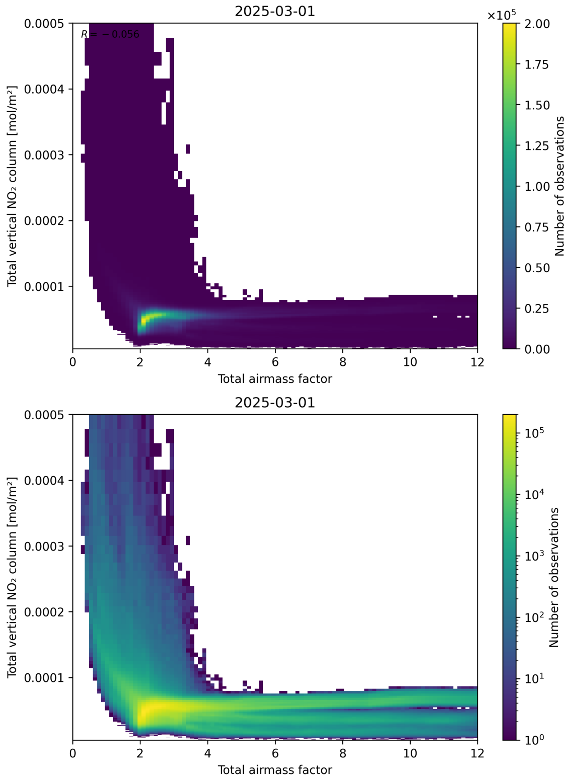
Figure 67: Scatter density plot of “Total airmass factor” against “Total vertical NO 2 column” for 2025-03-01 to 2025-03-02.
