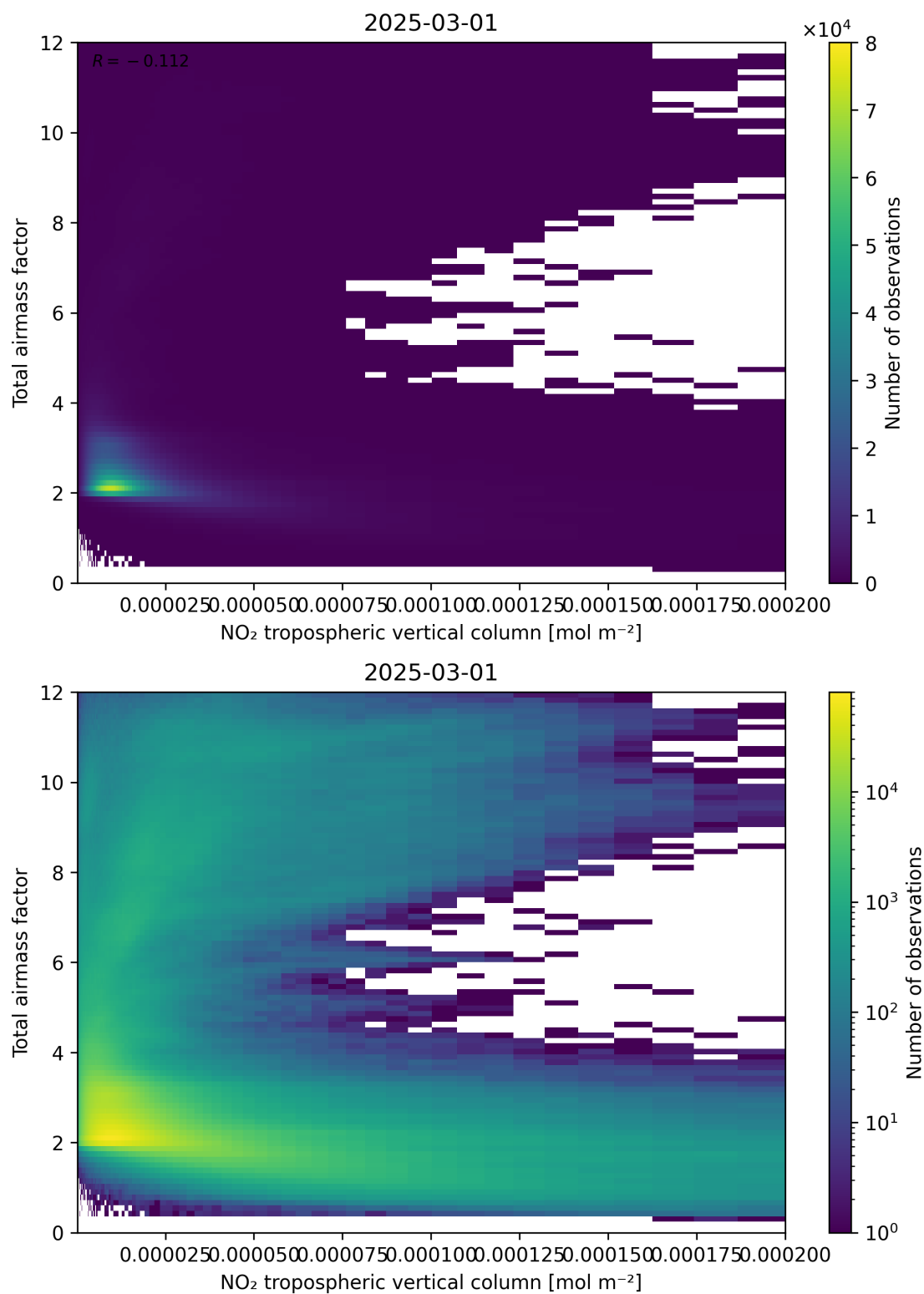
Figure 122: Scatter density plot of “NO 2 tropospheric vertical column” against “Total air mass factor” for 2025-03-01 to 2025-03-02.
