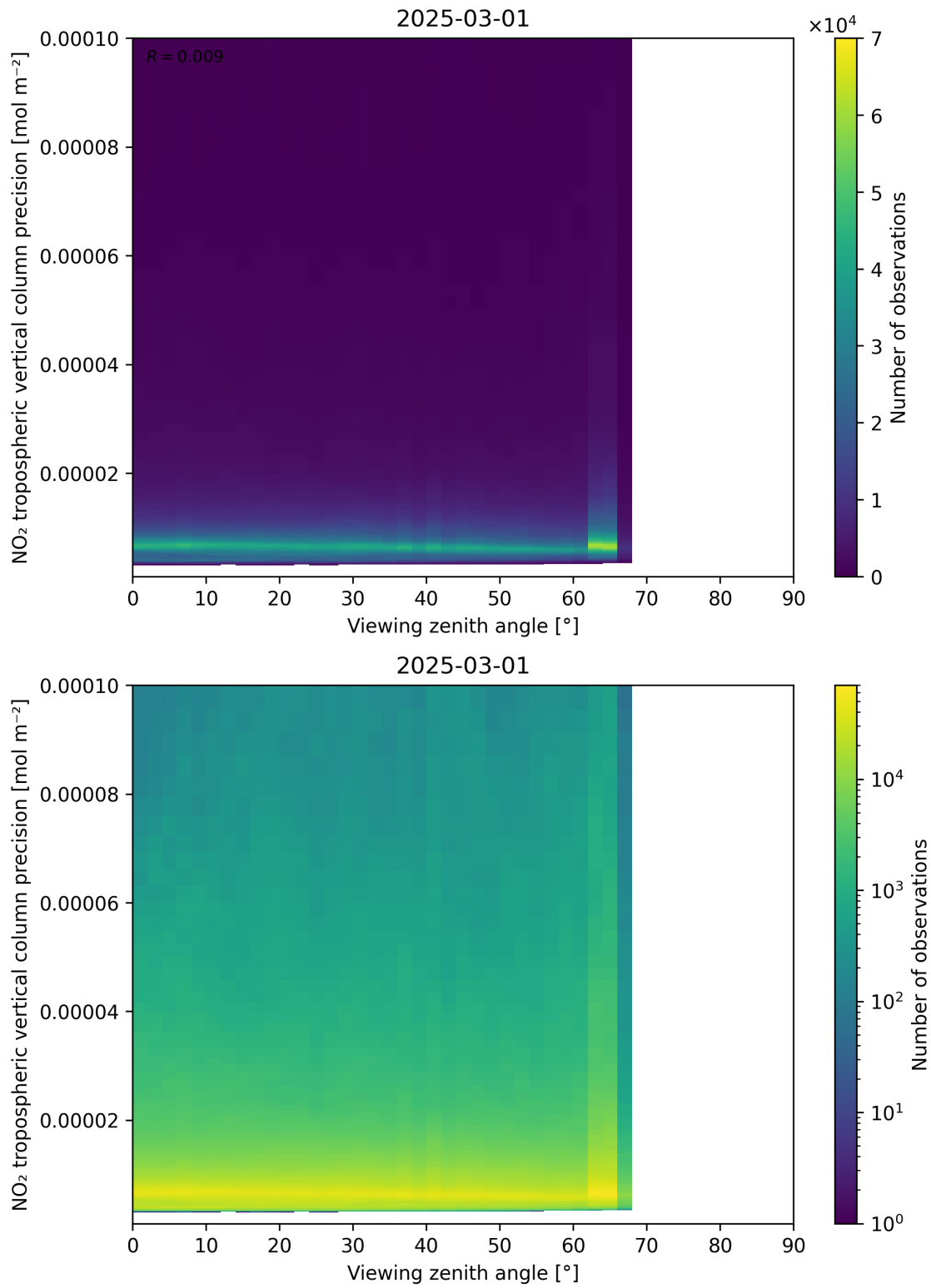
Figure 170: Scatter density plot of “Viewing zenith angle” against “NO 2 tropospheric vertical column precision” for 2025-03-01 to 2025-03-02.
