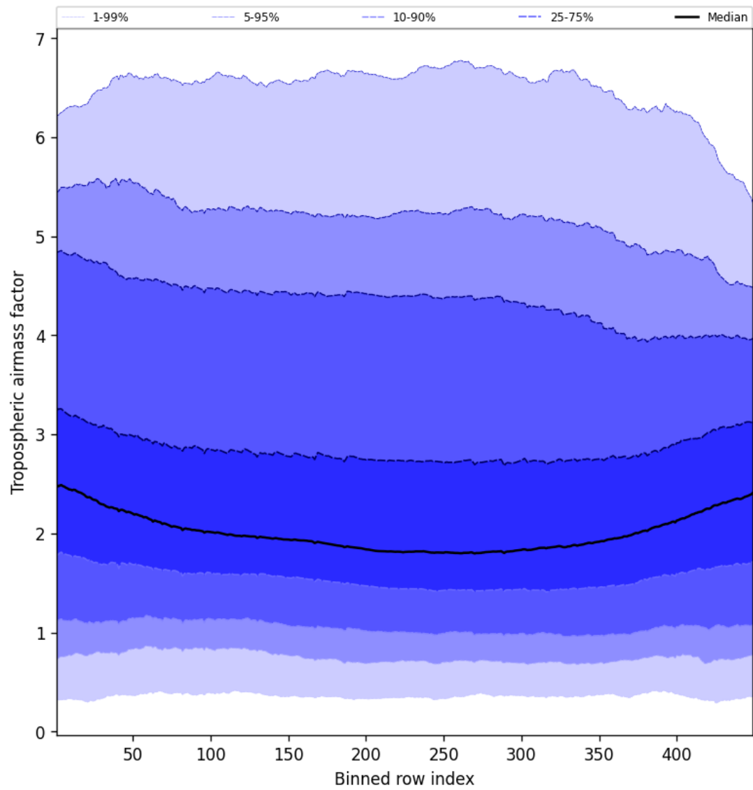
Figure 48: Along track statistics of "Tropospheric air mass factor" for 2025-03-01 to 2025-03-02
