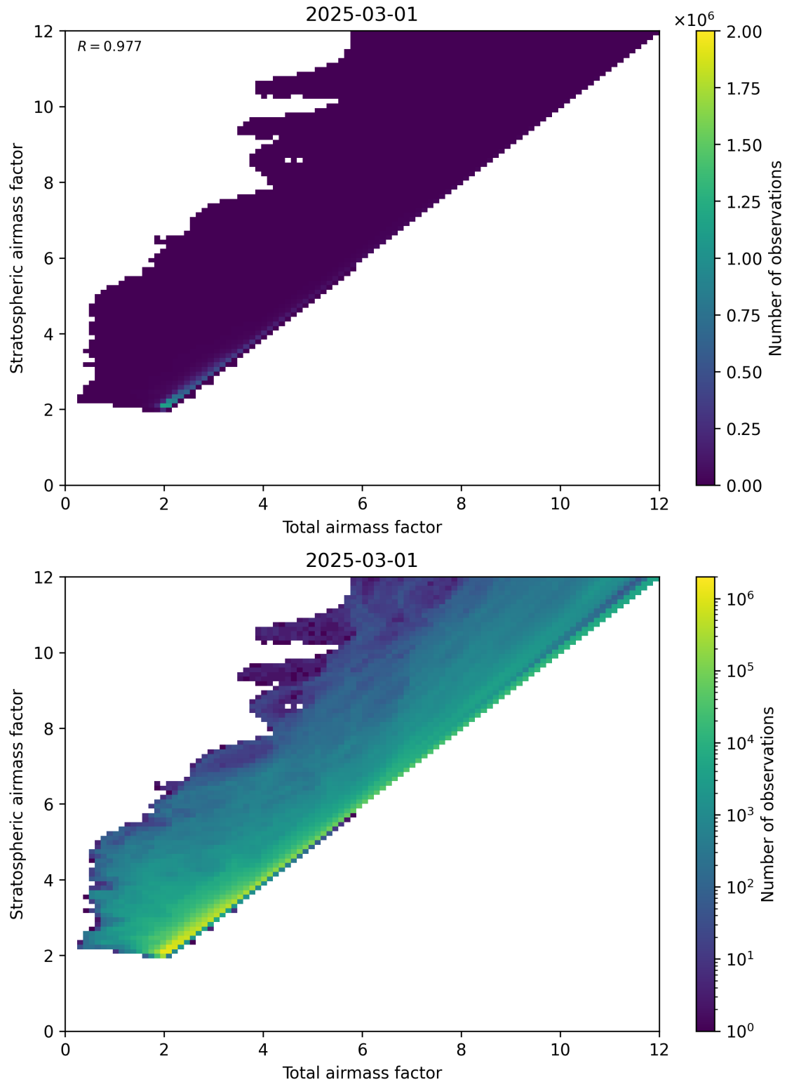
Figure 62: Scatter density plot of “Total airmass factor” against “Stratospheric airmass factor” for 2025-03-01 to 2025-03-02.
