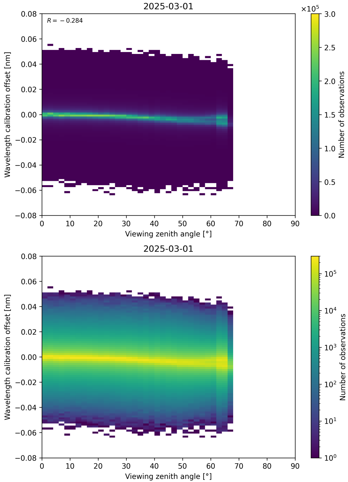
Figure 173: Scatter density plot of “Viewing zenith angle” against “Wavelength calibration offset” for 2025-03-01 to 2025-03-02.
