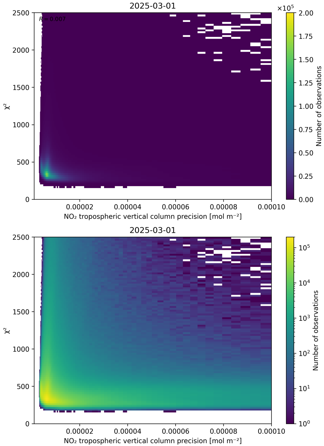
Figure 134: Scatter density plot of “NO 2 tropospheric vertical column precision” against “ \chi^2 ” for 2025-03-01 to 2025-03-02.
