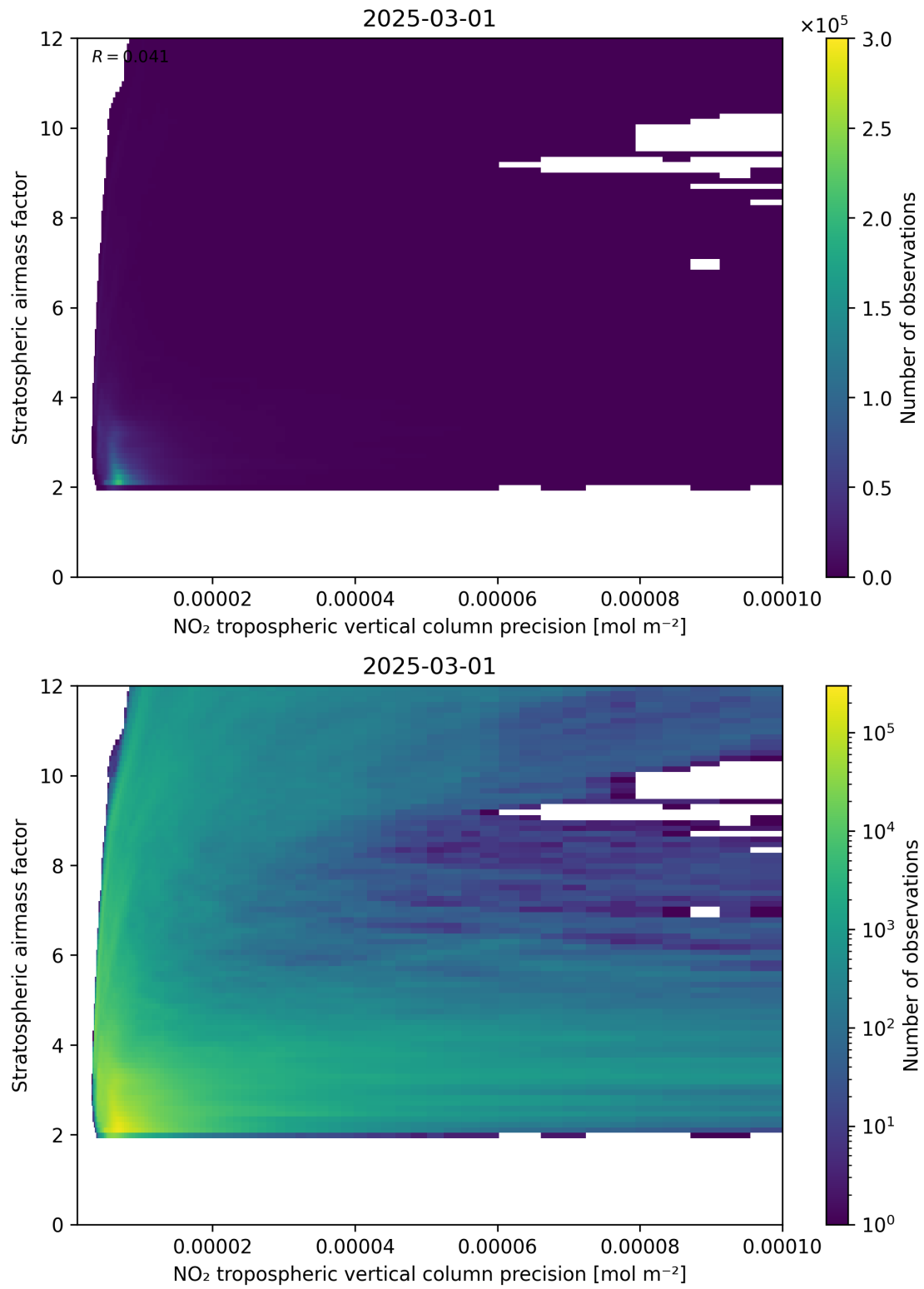
Figure 131: Scatter density plot of “NO 2 tropospheric vertical column precision” against “Stratospheric airmass factor” for 2025-03-01 to 2025-03-02.
