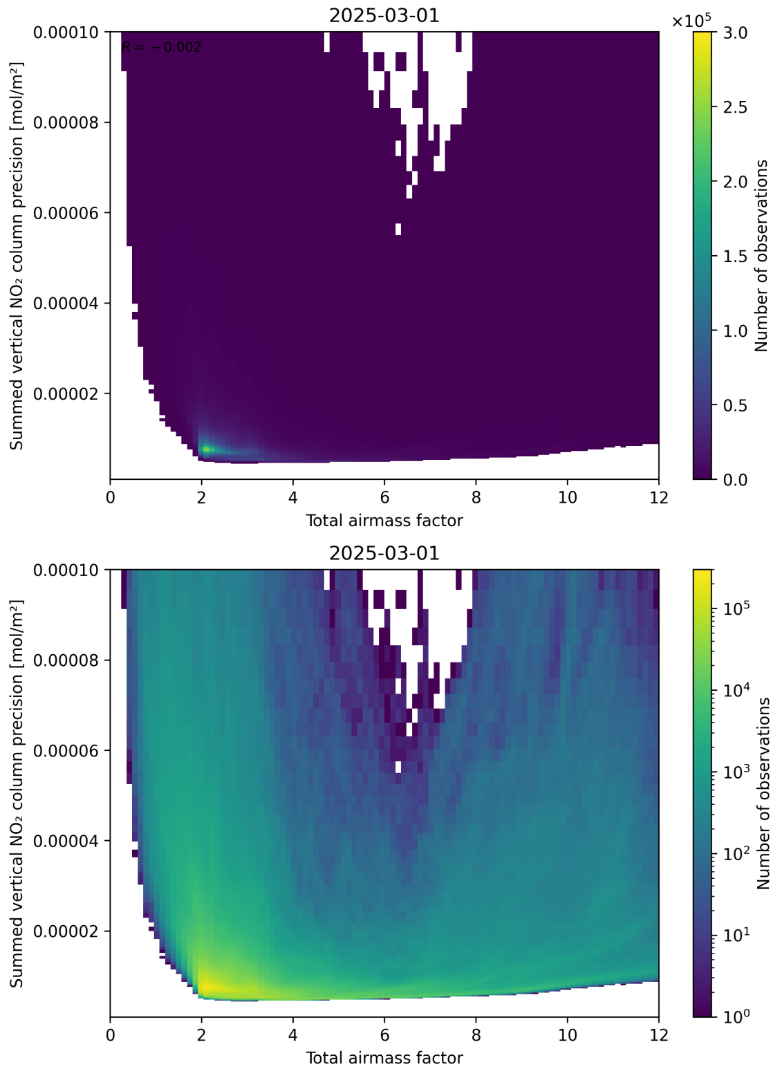
Figure 66: Scatter density plot of “Total airmass factor” against “Summed vertical NO 2 column precision” for 2025-03-01 to 2025-03-02.
