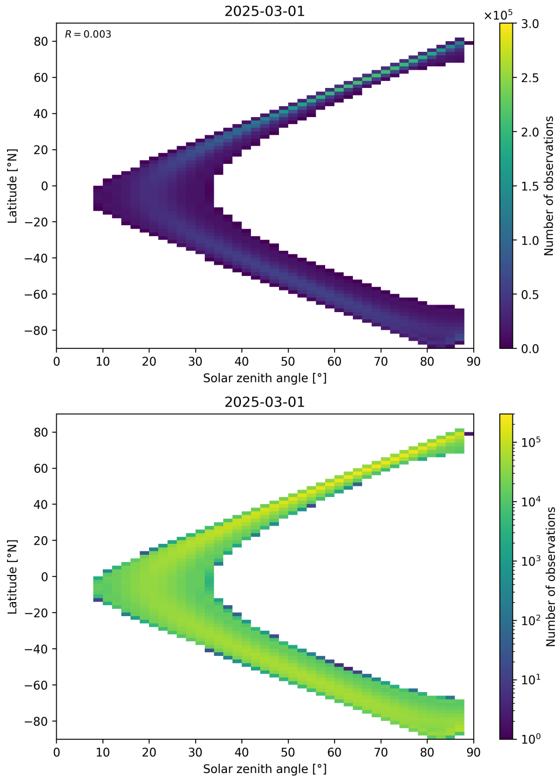
Figure 149: Scatter density plot of “Solar zenith angle” against “Latitude” for 2025-03-01 to 2025-03-02.
