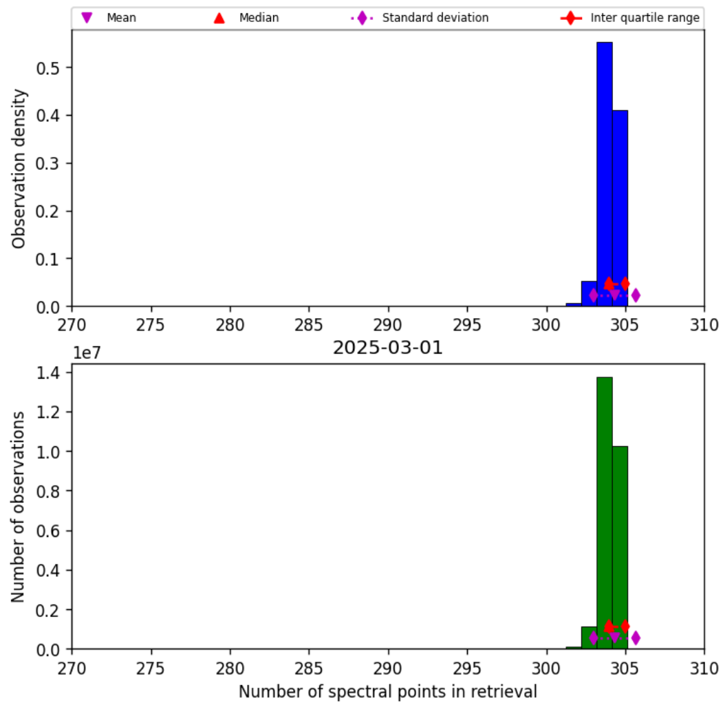
Figure 33: Histogram of “Number of spectral points in retrieval” for 2025-03-01 to 2025-03-02
