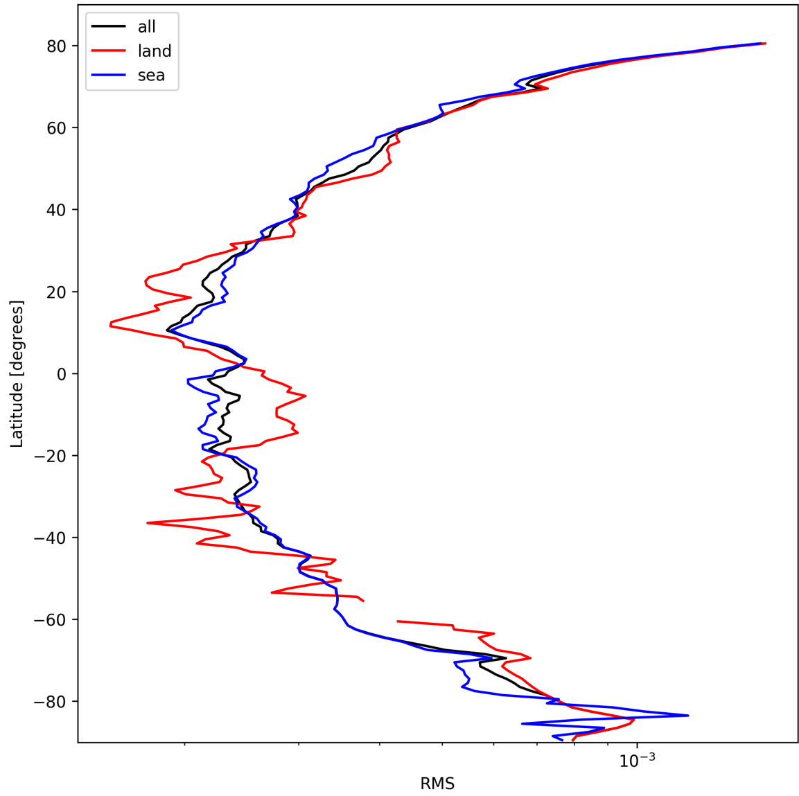
Figure 26: Zonal average of “RMS” for 2025-03-01 to 2025-03-02.
