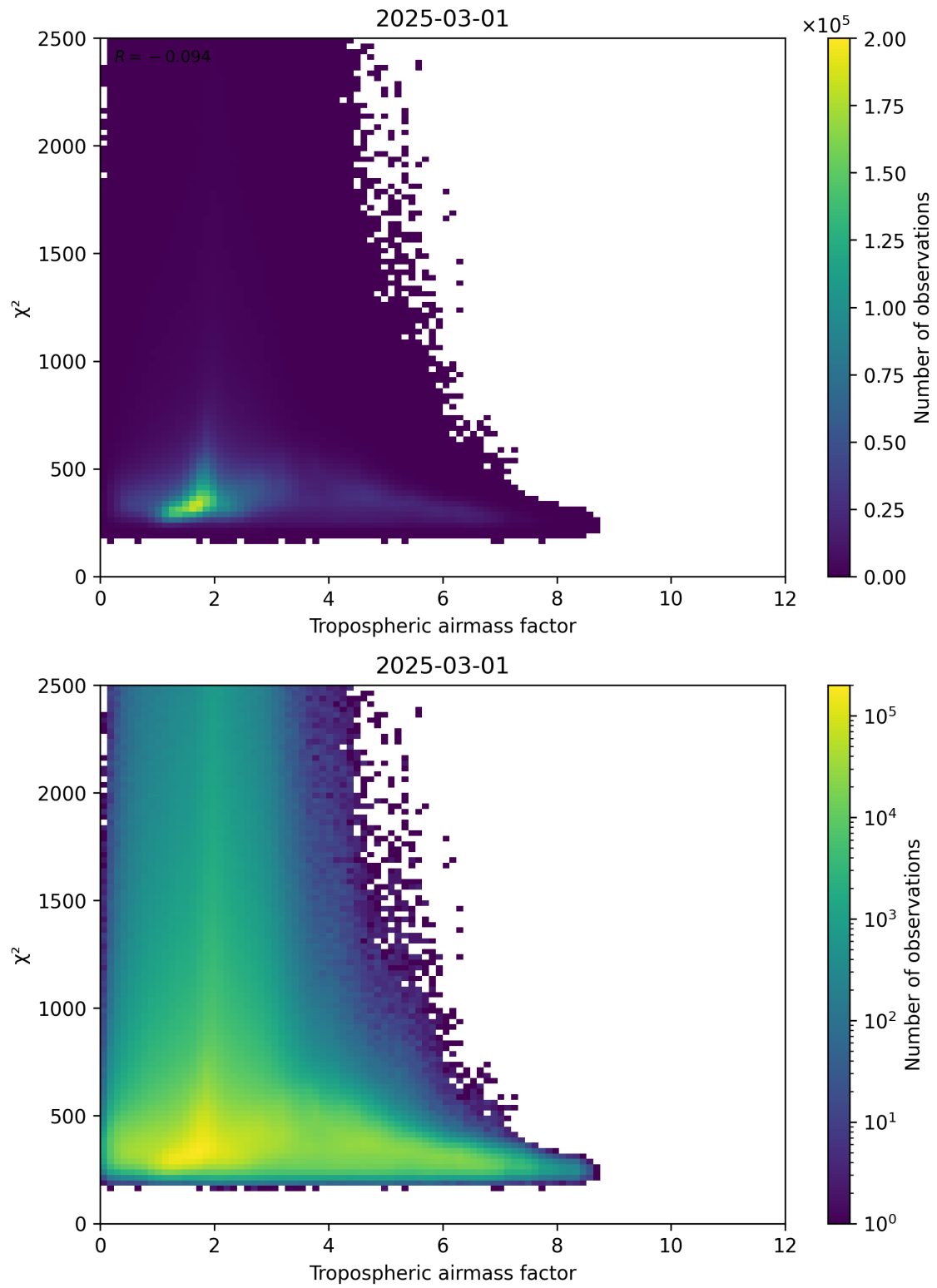
Figure 73: Scatter density plot of “Tropospheric airmass factor” against “ \chi^2 ” for 2025-03-01 to 2025-03-02.
