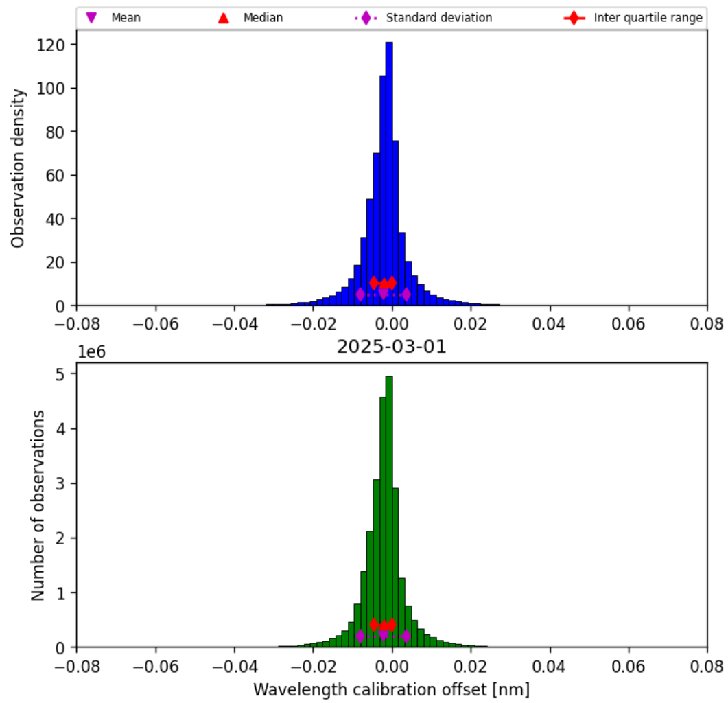
Figure 35: Histogram of “Wavelength calibration offset” for 2025-03-01 to 2025-03-02
