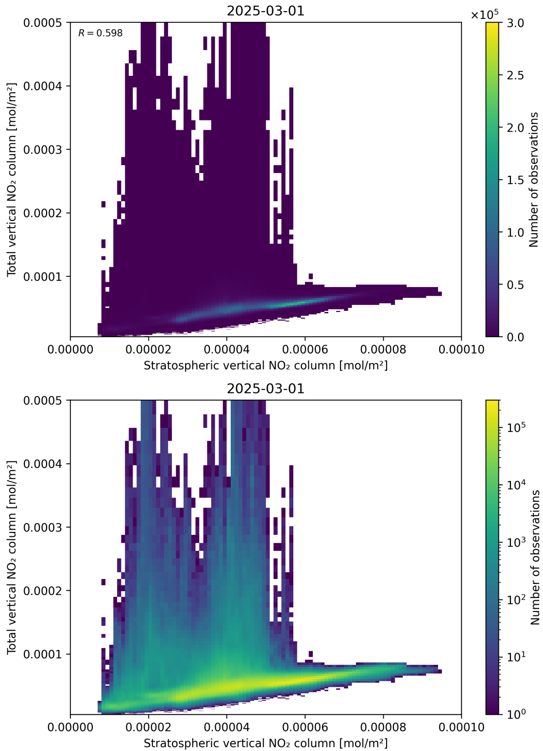
Figure 100: Scatter density plot of “Stratospheric vertical NO 2 column” against “Total vertical NO 2 column” for 2025-03-01 to 2025-03-02.
