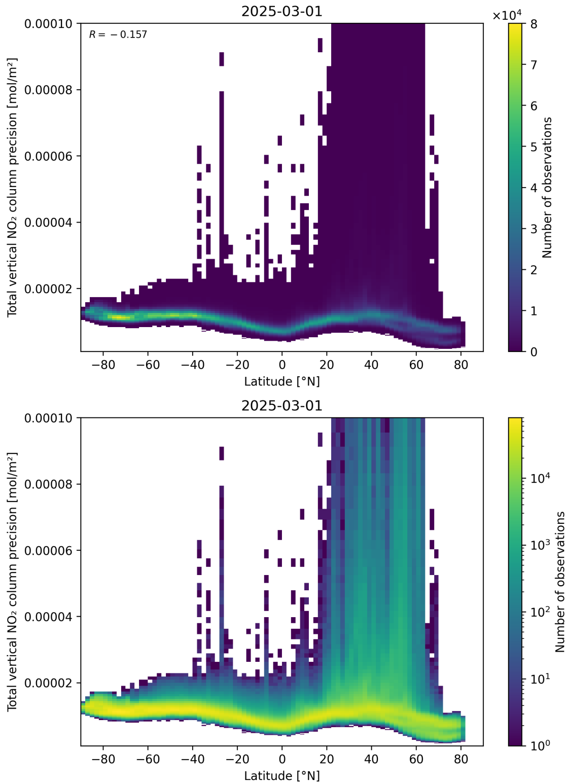
Figure 91: Scatter density plot of “Latitude” against “Total vertical NO 2 column precision” for 2025-03-01 to 2025-03-02.
