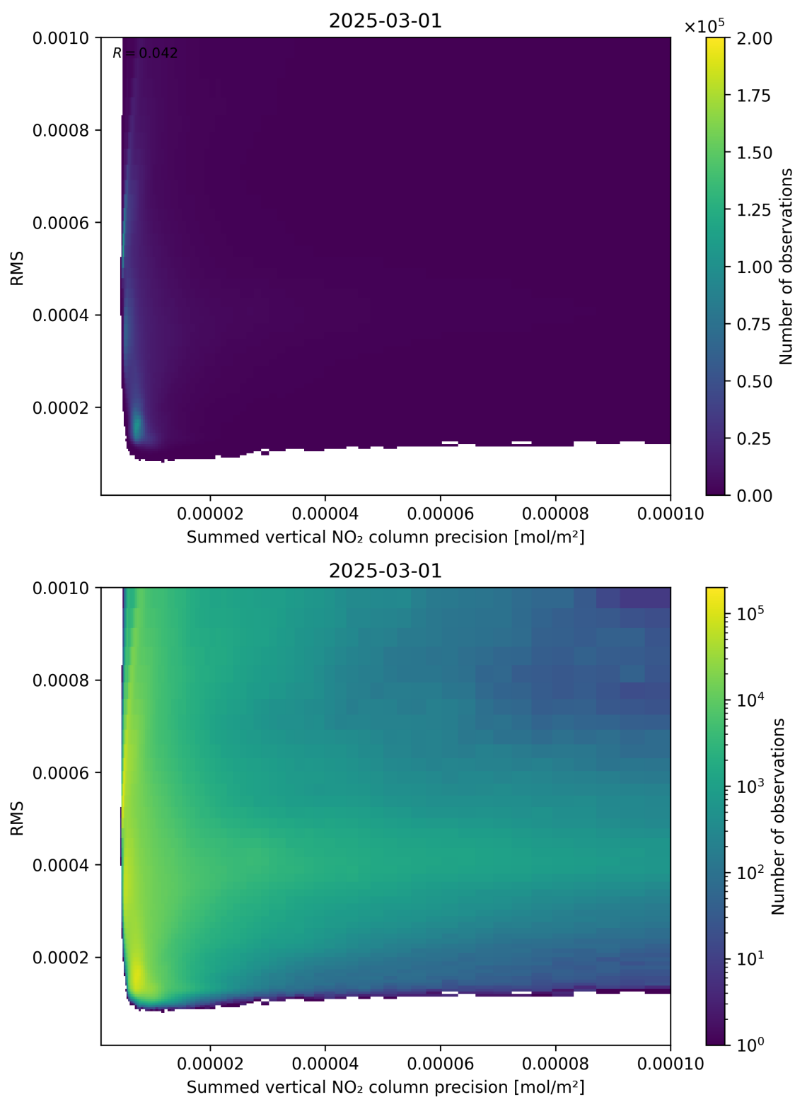
Figure 108: Scatter density plot of “Summed vertical NO 2 column precision” against “RMS” for 2025-03-01 to 2025-03-02.
