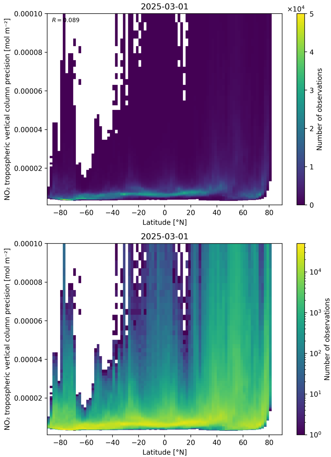
Figure 93: Scatter density plot of “Latitude” against “NO 2 tropospheric vertical column precision” for 2025-03-01 to 2025-03-02.
