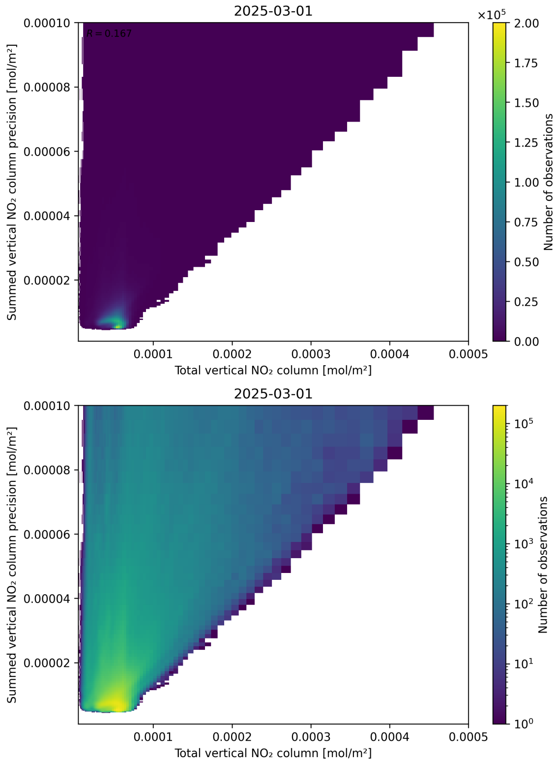
Figure 113: Scatter density plot of “Total vertical NO 2 column” against “Summed vertical NO 2 column precision” for 2025-03-01 to 2025-03-02.
