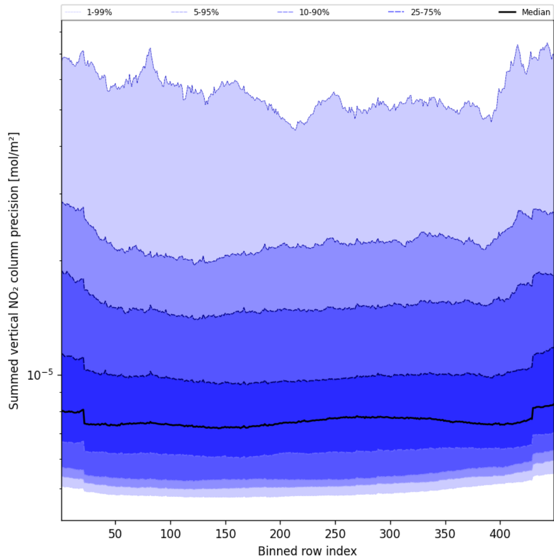
Figure 58: Along track statistics of “Summed vertical NO 2 column precision” for 2025-03-01 to 2025-03-02
