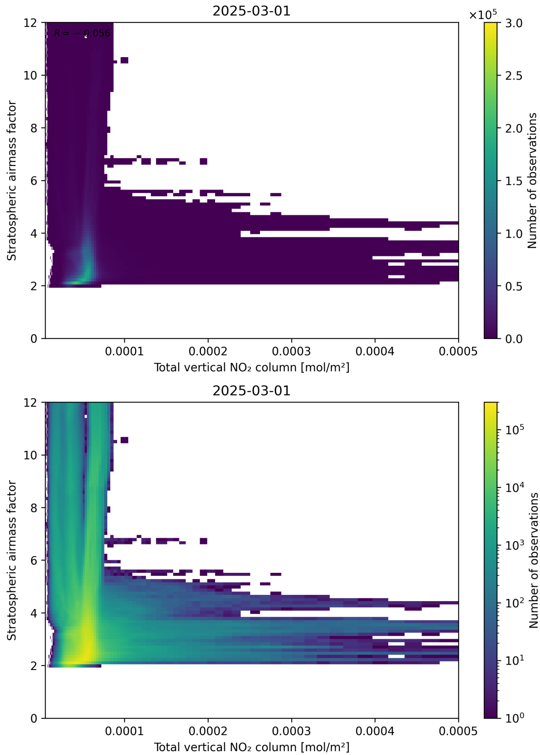
Figure 110: Scatter density plot of “Total vertical NO 2 column” against “Stratospheric airmass factor” for 2025-03-01 to 2025-03-02.
