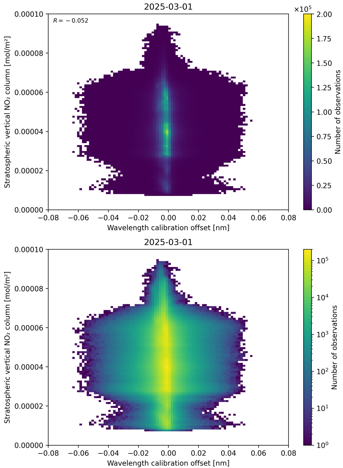
Figure 176: Scatter density plot of “Wavelength calibration offset” against “Stratospheric vertical NO 2 column” for 2025-03-01 to 2025-03-02.
