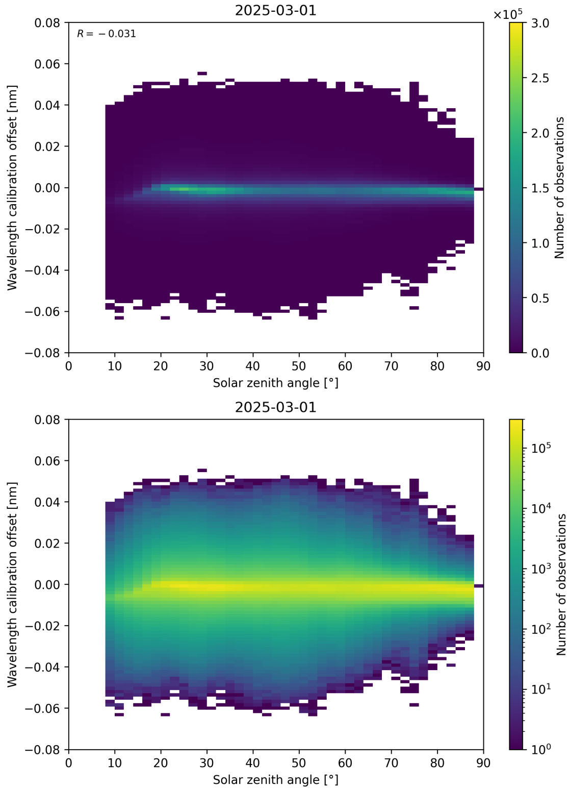
Figure 158: Scatter density plot of “Solar zenith angle” against “Wavelength calibration offset” for 2025-03-01 to 2025-03-02.
