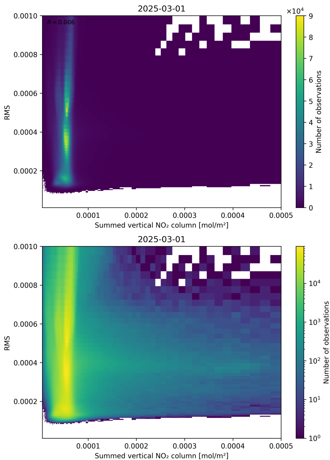
Figure 109: Scatter density plot of “Summed vertical NO 2 column” against “RMS” for 2025-03-01 to 2025-03-02.
