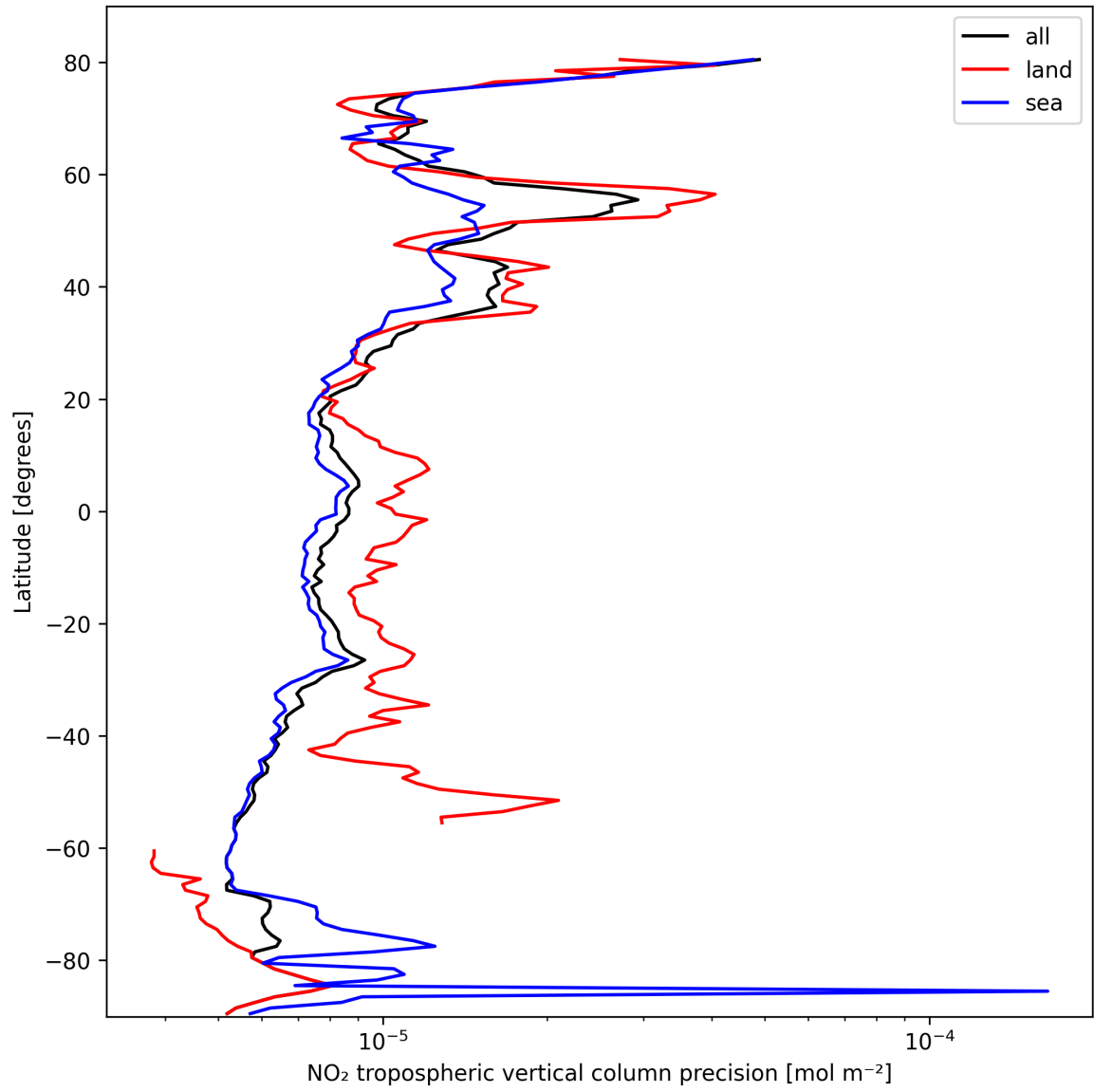
Figure 13: Zonal average of “NO 2 tropospheric vertical column precision” for 2025-03-01 to 2025-03-02.
