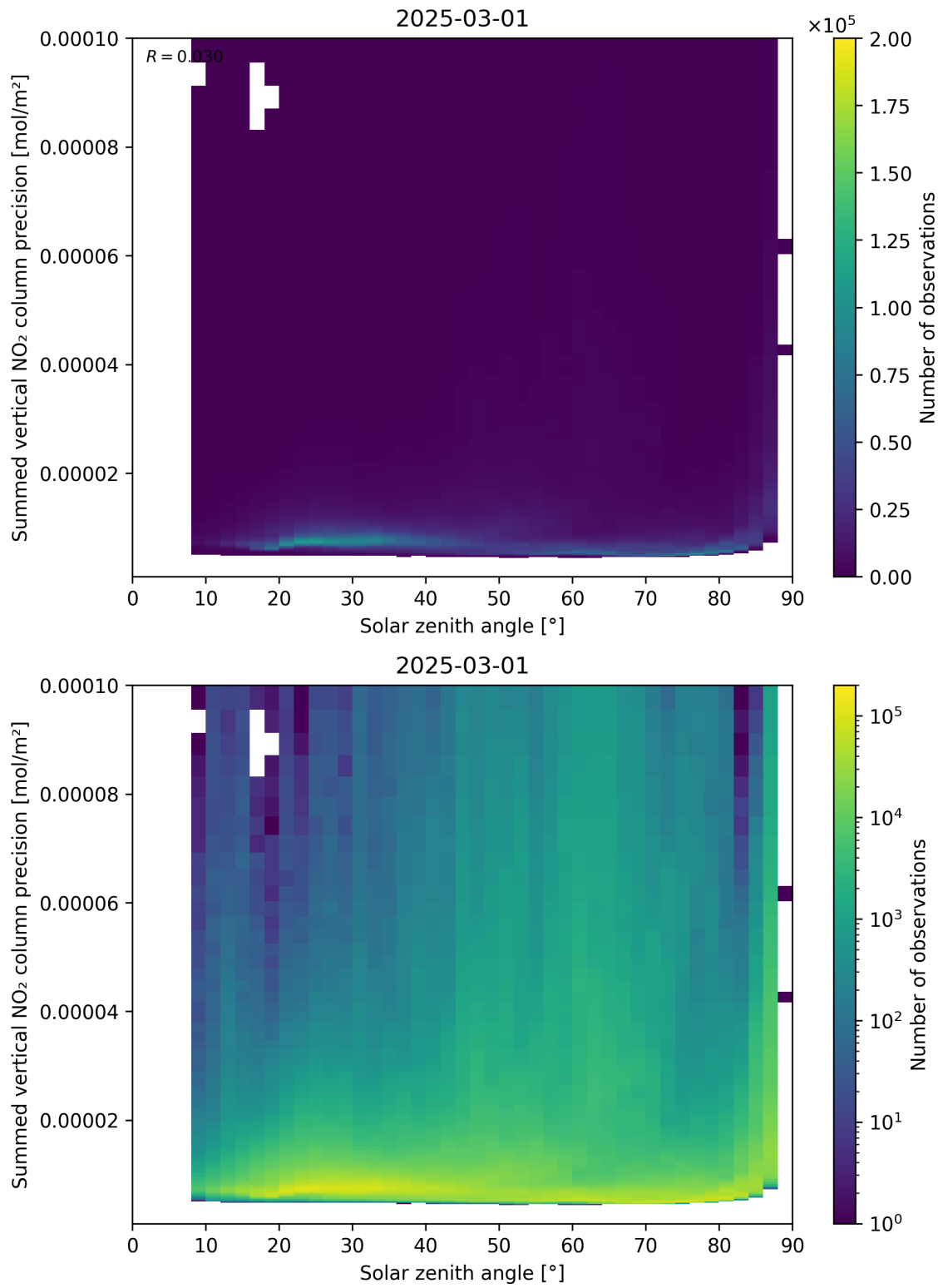
Figure 152: Scatter density plot of “Solar zenith angle” against “Summed vertical NO 2 column precision” for 2025-03-01 to 2025-03-02.
