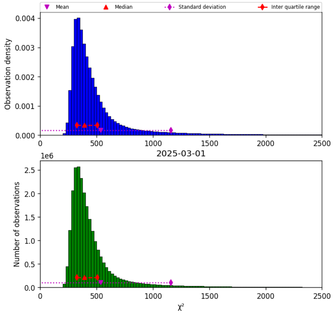
Figure 42: Histogram of “ \chi^2 ” for 2025-03-01 to 2025-03-02
