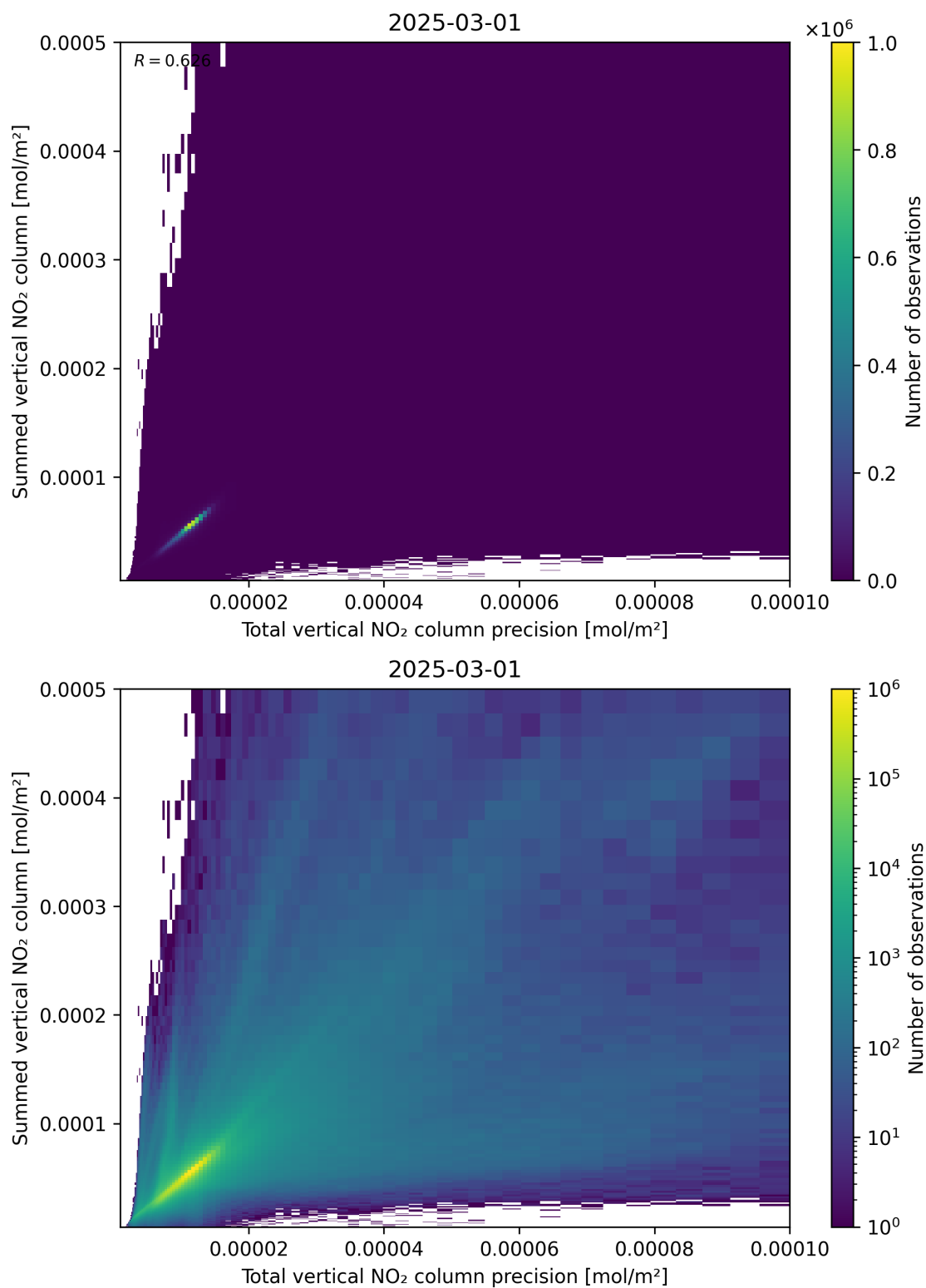
Figure 117: Scatter density plot of “Total vertical NO 2 column precision” against “Summed vertical NO 2 column” for 2025-03-01 to 2025-03-02.
