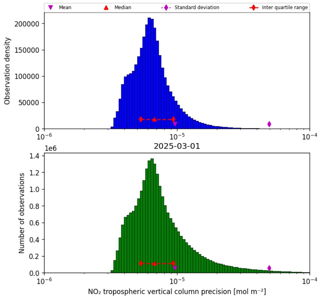
Figure 30: Histogram of “NO 2 tropospheric vertical column precision” for 2025-03-01 to 2025-03-02
