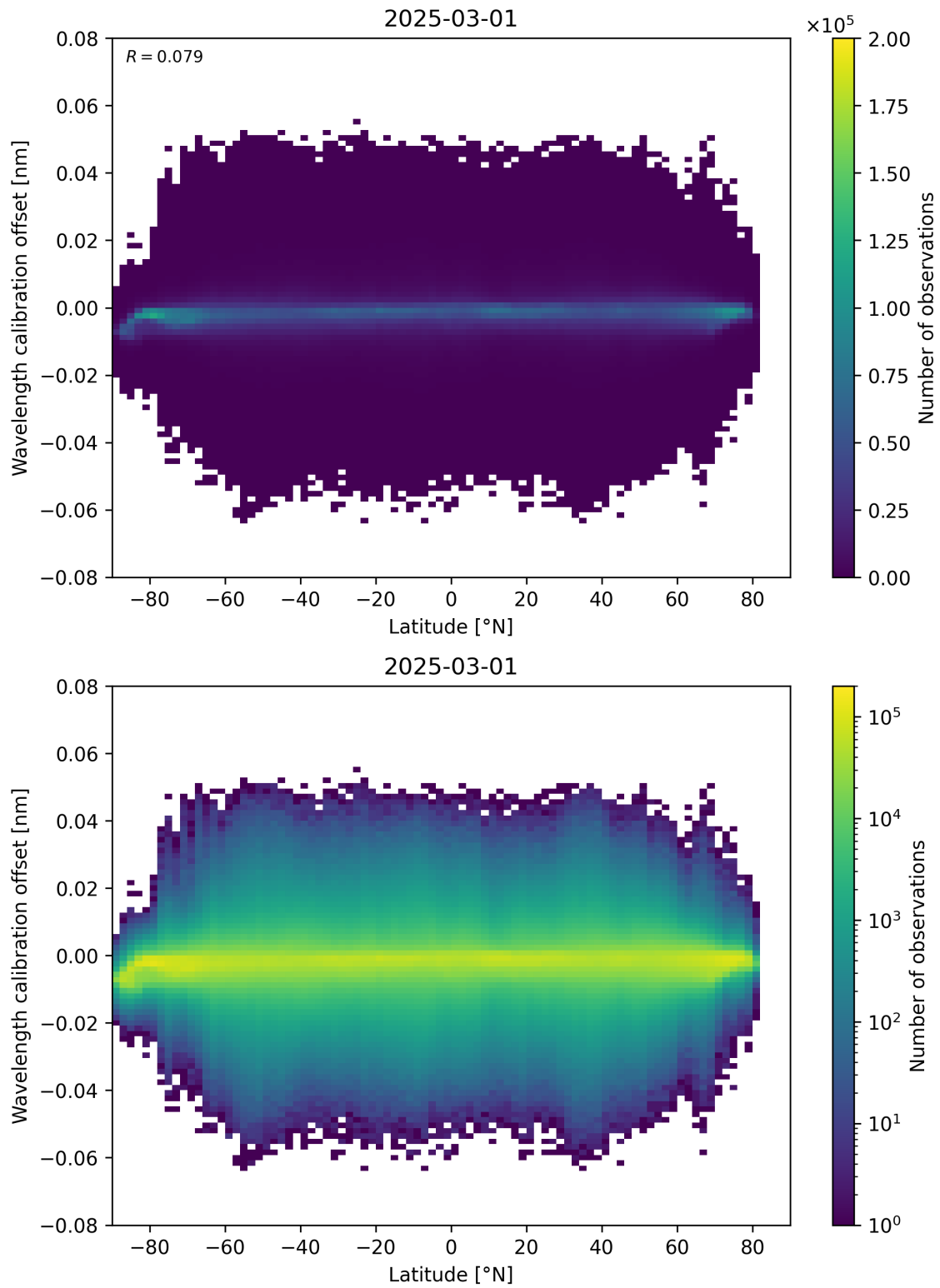
Figure 95: Scatter density plot of “Latitude” against “Wavelength calibration offset” for 2025-03-01 to 2025-03-02.
