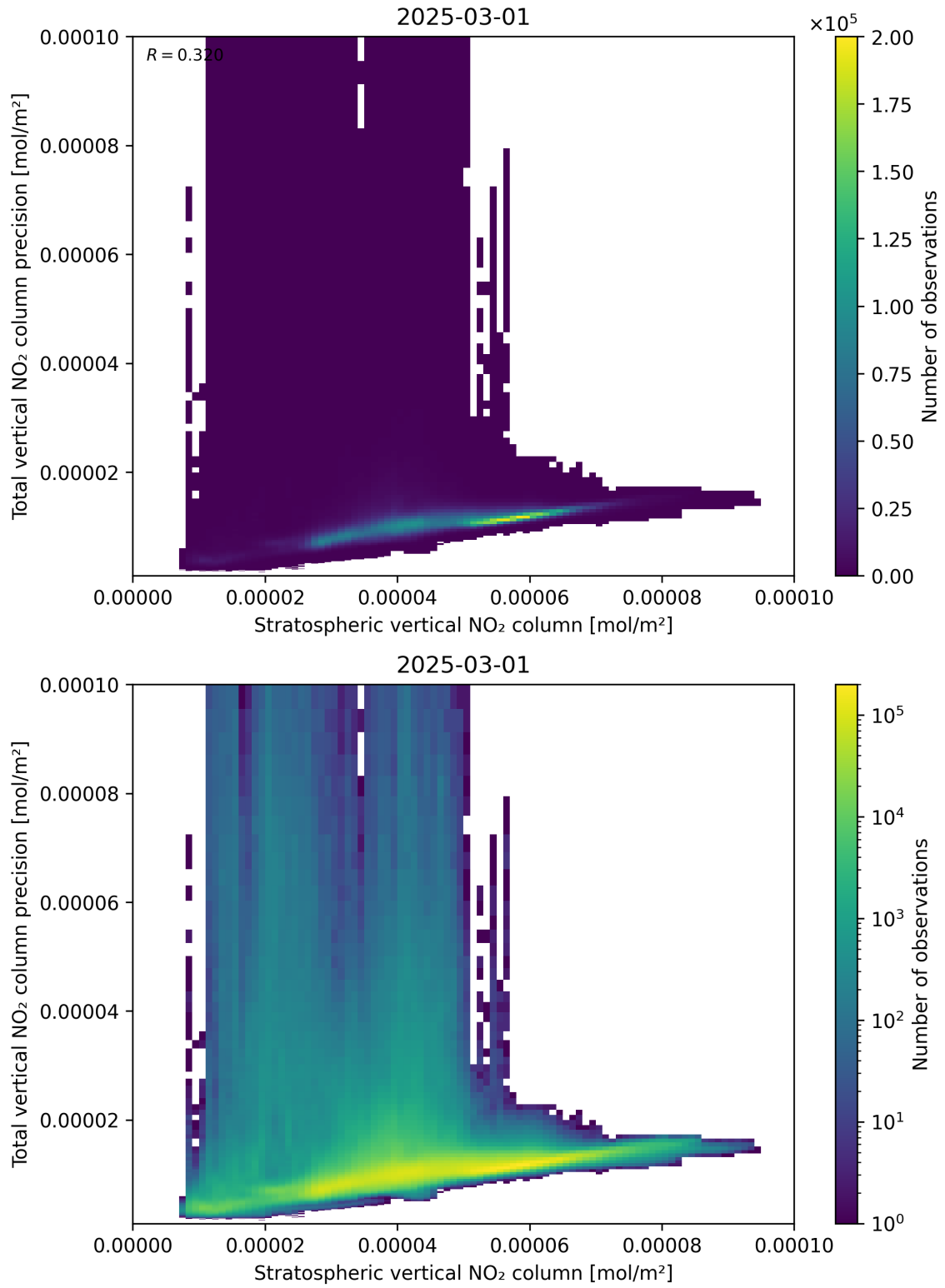
Figure 101: Scatter density plot of “Stratospheric vertical NO 2 column” against “Total vertical NO 2 column precision” for 2025-03-01 to 2025-03-02.
