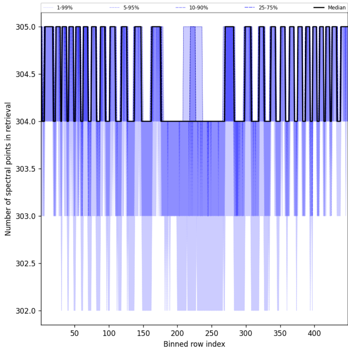
Figure 50: Along track statistics of “Number of spectral points in retrieval” for 2025-03-01 to 2025-03-02
