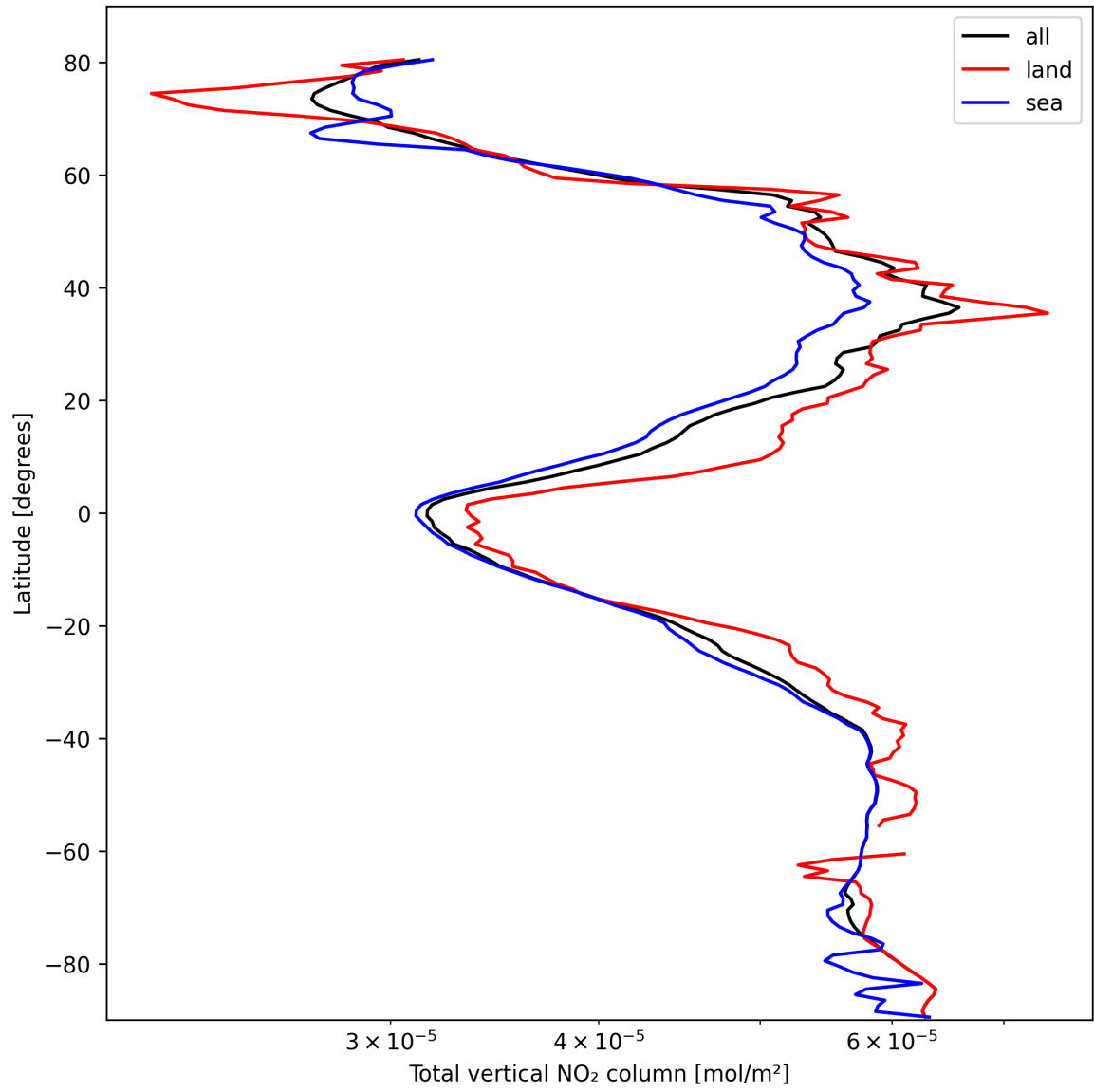
Figure 21: Zonal average of “Total vertical NO 2 column” for 2025-03-01 to 2025-03-02.
