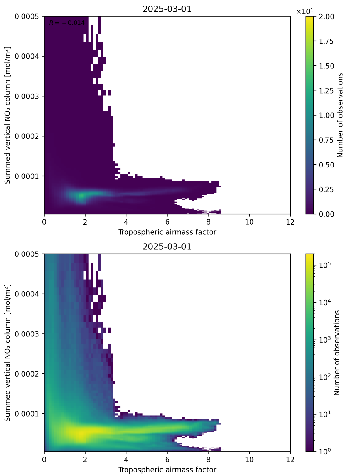
Figure 75: Scatter density plot of “Tropospheric air mass factor” against “Summed vertical NO 2 column” for 2025-03-01 to 2025-03-02.
