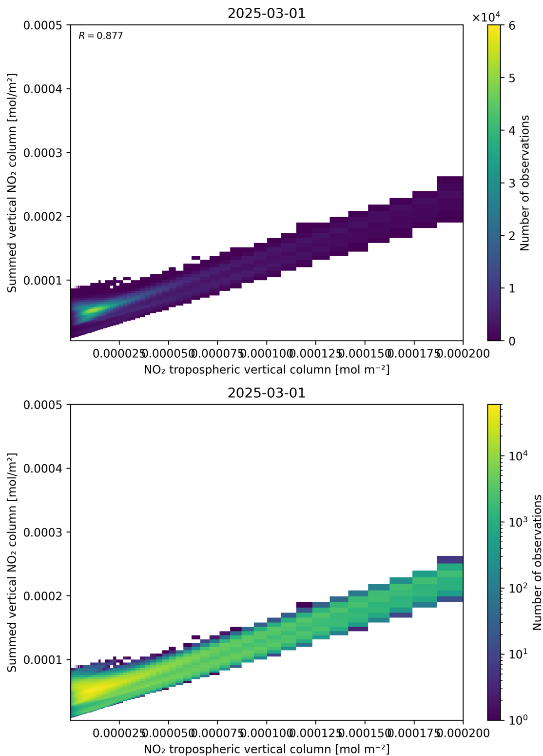
Figure 126: Scatter density plot of “NO 2 tropospheric vertical column” against “Summed vertical NO 2 column” for 2025-03-01 to 2025-03-02.
