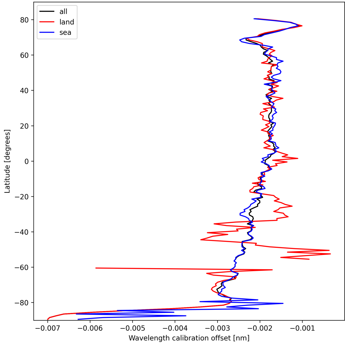
Figure 18: Zonal average of “Wavelength calibration offset” for 2025-03-01 to 2025-03-02.
