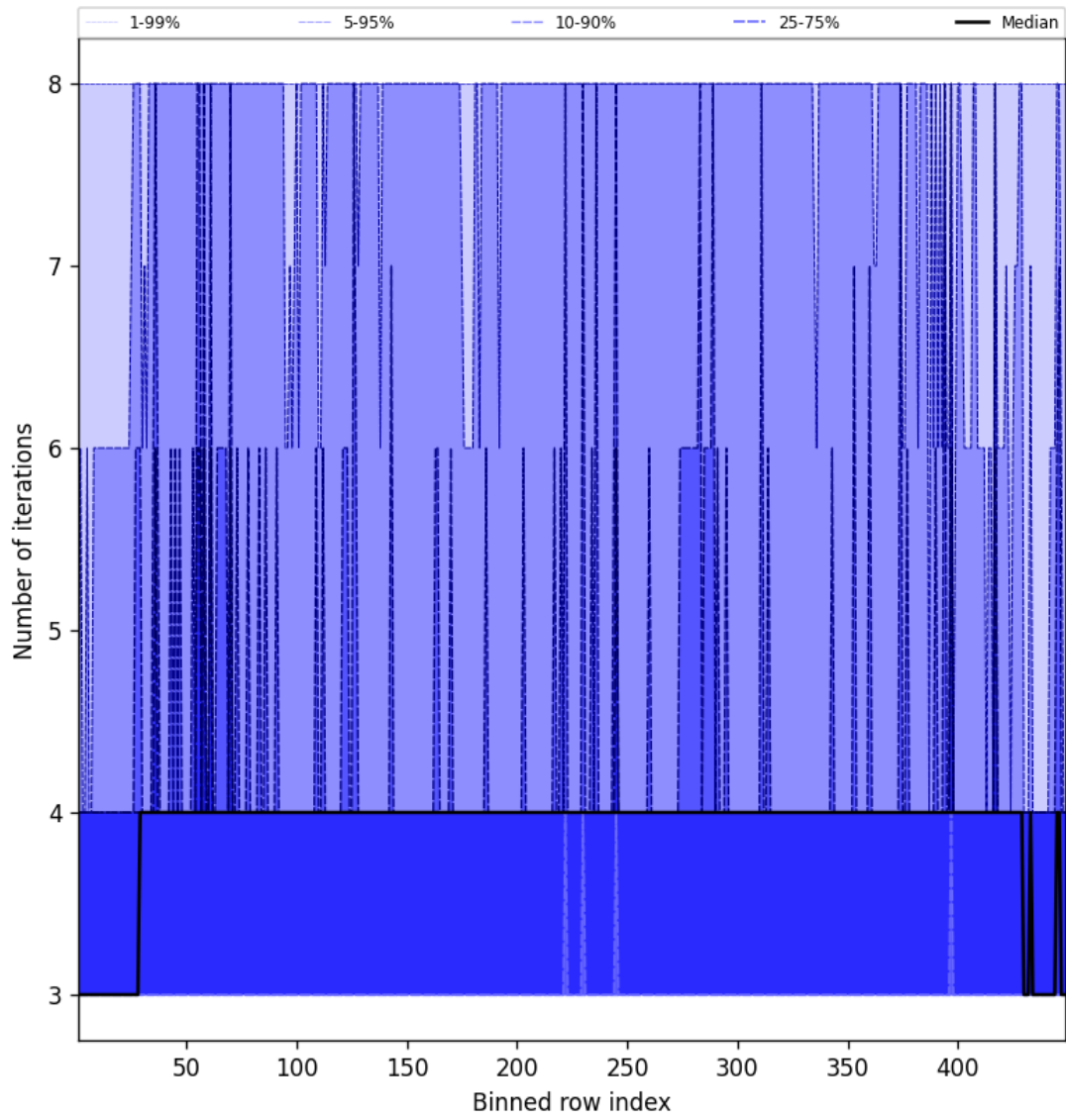
Figure 51: Along track statistics of “Number of iterations” for 2025-03-01 to 2025-03-02
