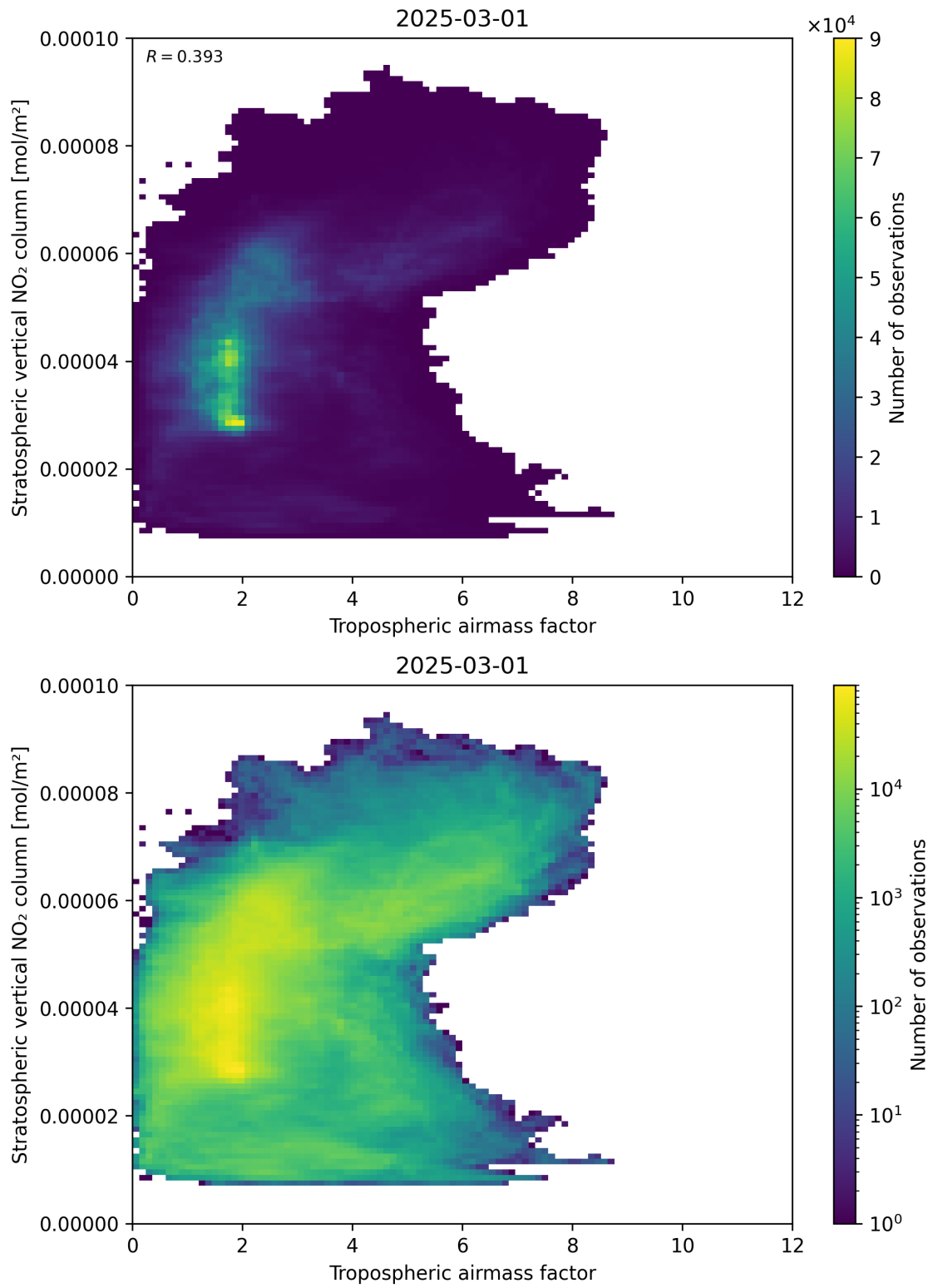
Figure 74: Scatter density plot of “Tropospheric air mass factor” against “Stratospheric vertical NO 2 column” for 2025-03-01 to 2025-03-02.
