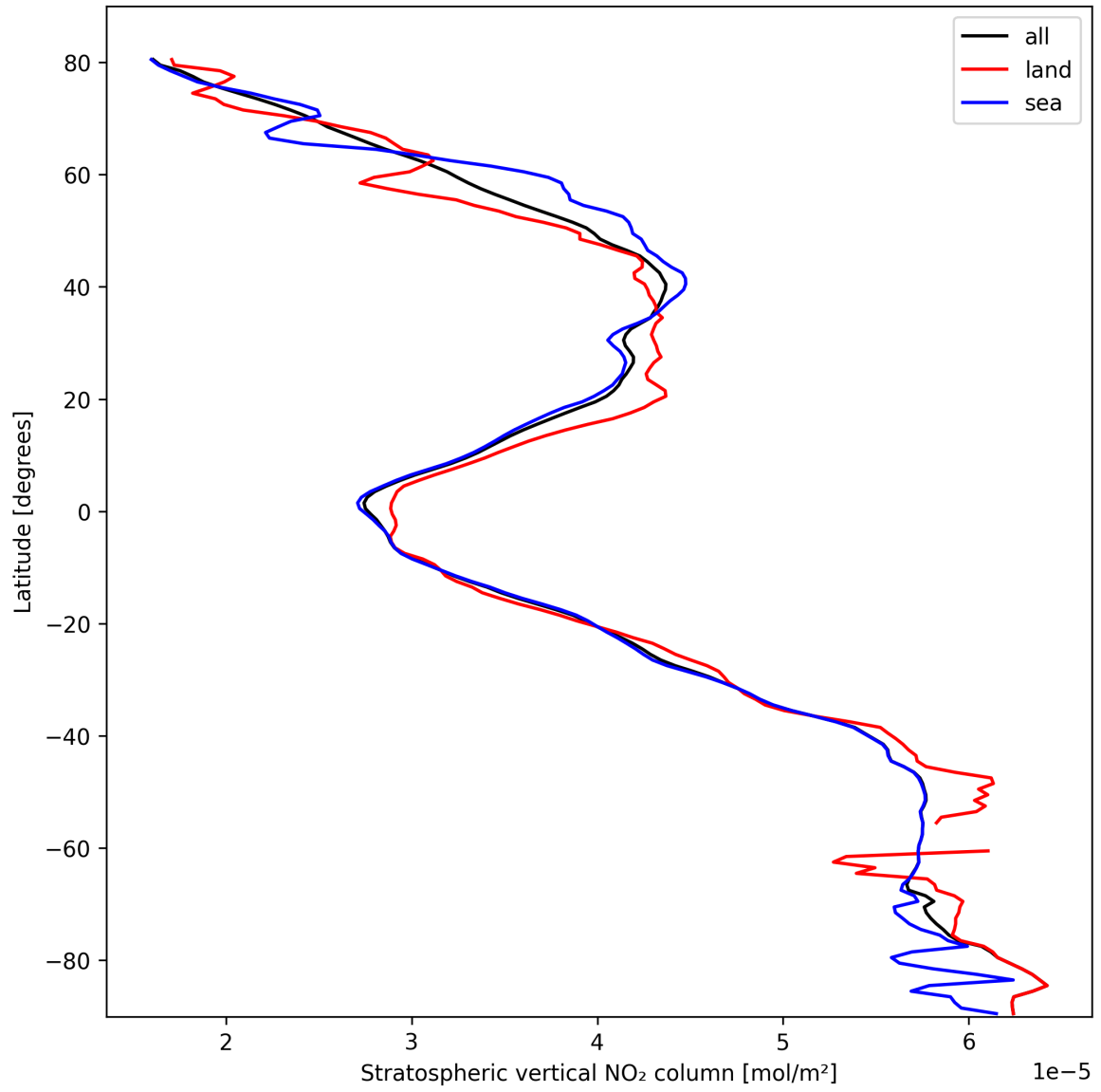
Figure 19: Zonal average of “Stratospheric vertical NO 2 column” for 2025-03-01 to 2025-03-02.
