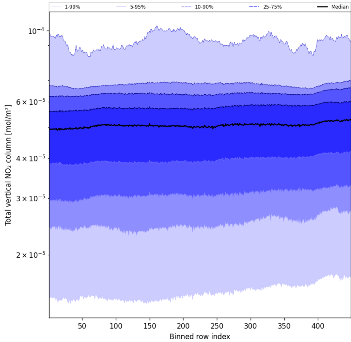
Figure 55: Along track statistics of “Total vertical NO 2 column” for 2025-03-01 to 2025-03-02
