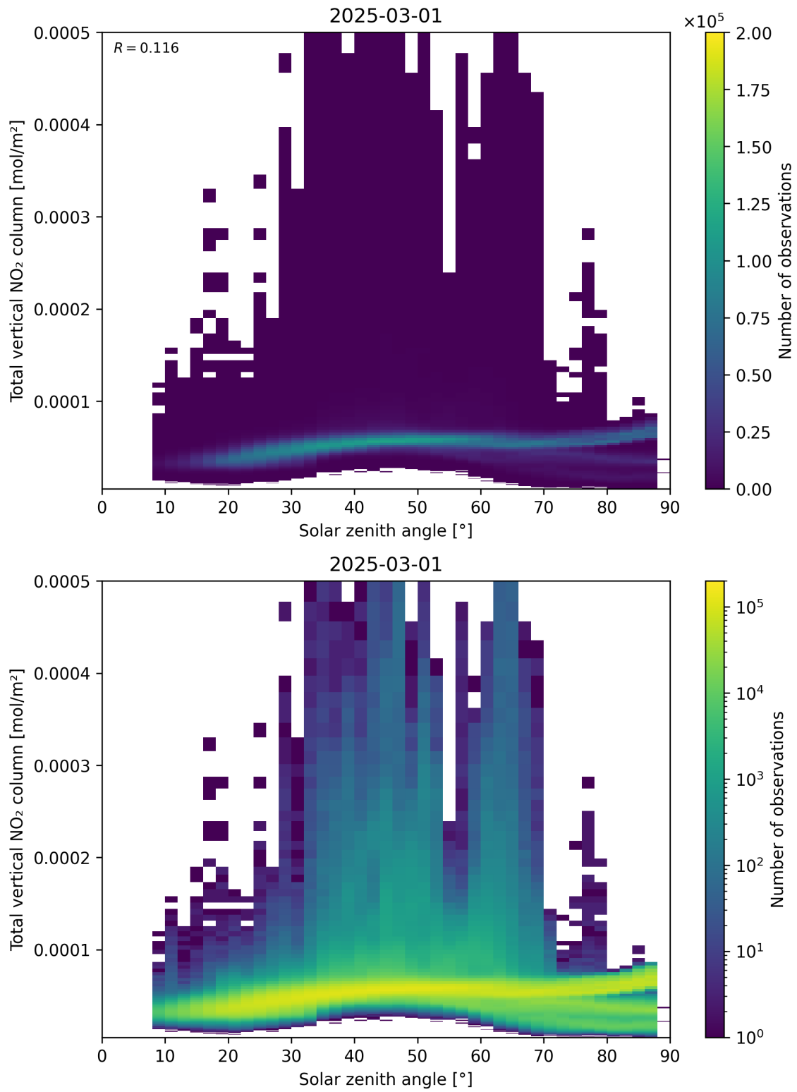
Figure 153: Scatter density plot of “Solar zenith angle” against “Total vertical NO 2 column” for 2025-03-01 to 2025-03-02.
