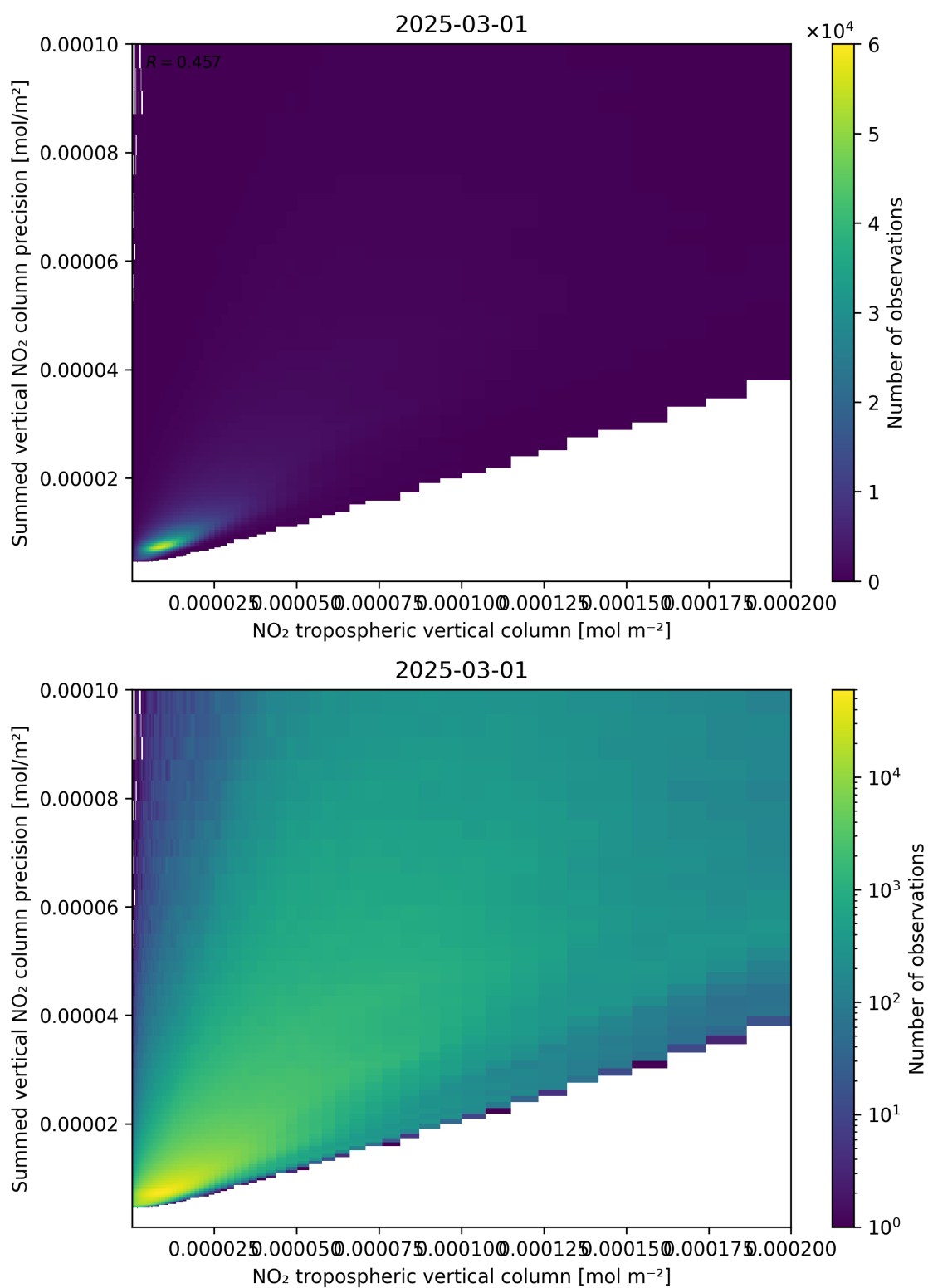
Figure 127: Scatter density plot of “NO 2 tropospheric vertical column” against “Summed vertical NO 2 column precision” for 2025-03-01 to 2025-03-02.
