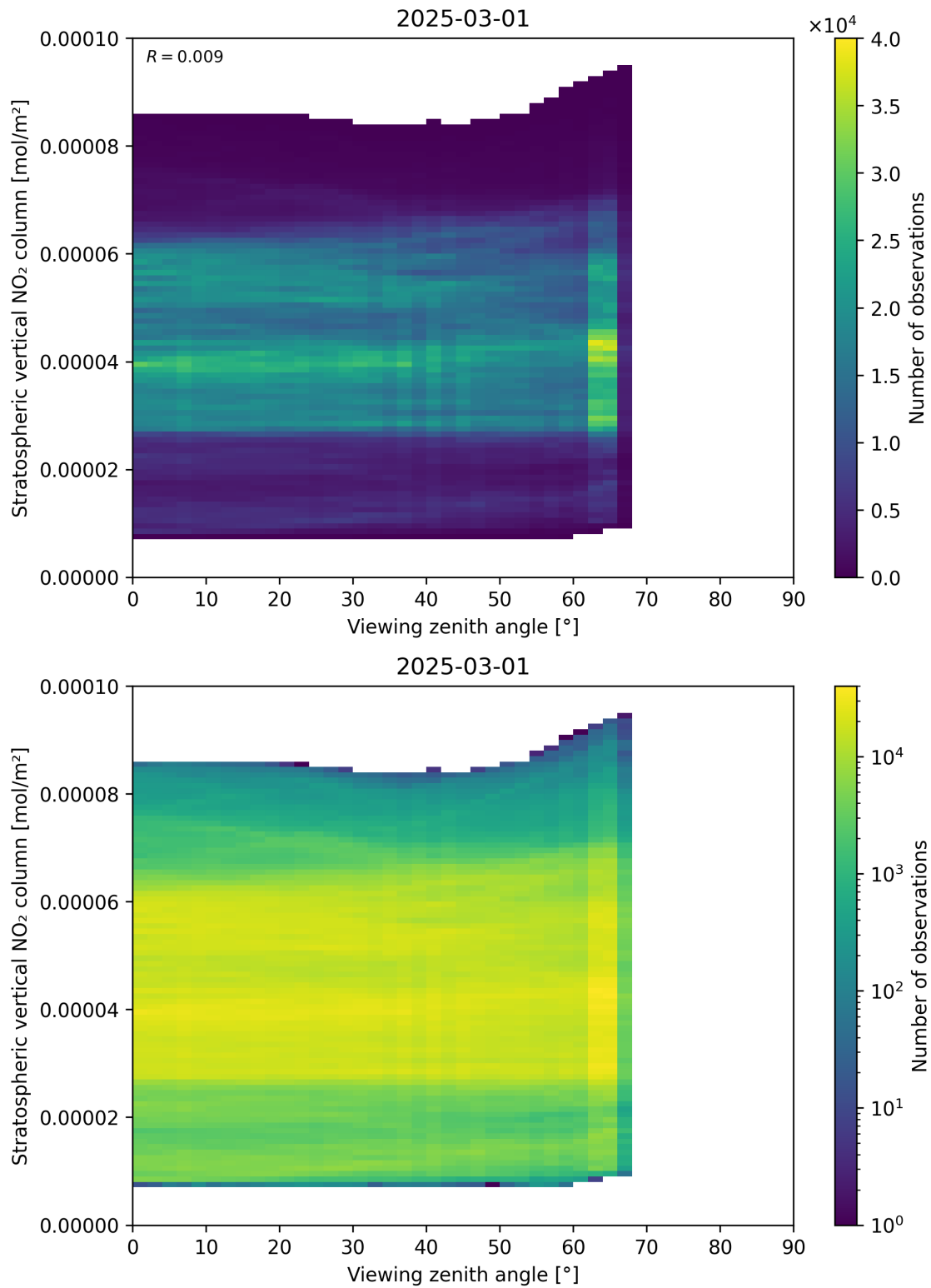
Figure 164: Scatter density plot of “Viewing zenith angle” against “Stratospheric vertical NO 2 column” for 2025-03-01 to 2025-03-02.
