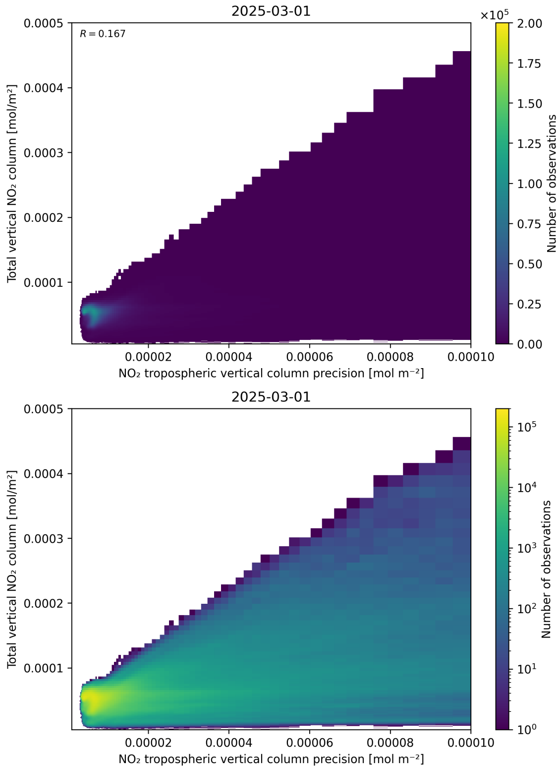
Figure 138: Scatter density plot of “NO 2 tropospheric vertical column precision” against “Total vertical NO 2 column” for 2025-03-01 to 2025-03-02.
