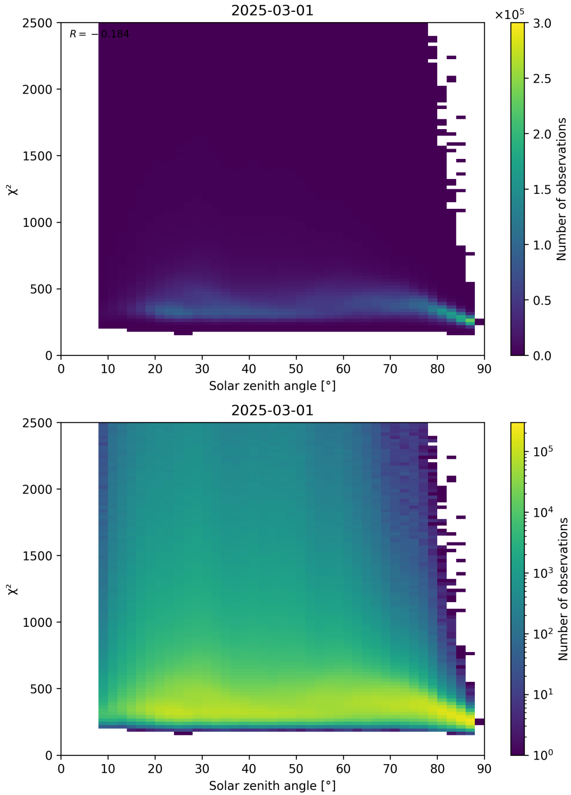
Figure 148: Scatter density plot of “Solar zenith angle” against “ \chi^2 ” for 2025-03-01 to 2025-03-02.
