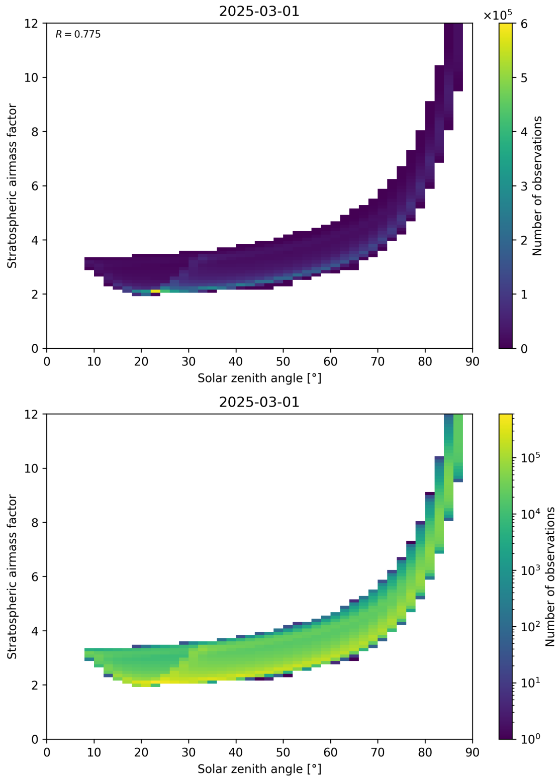
Figure 145: Scatter density plot of “Solar zenith angle” against “Stratospheric airmass factor” for 2025-03-01 to 2025-03-02.
