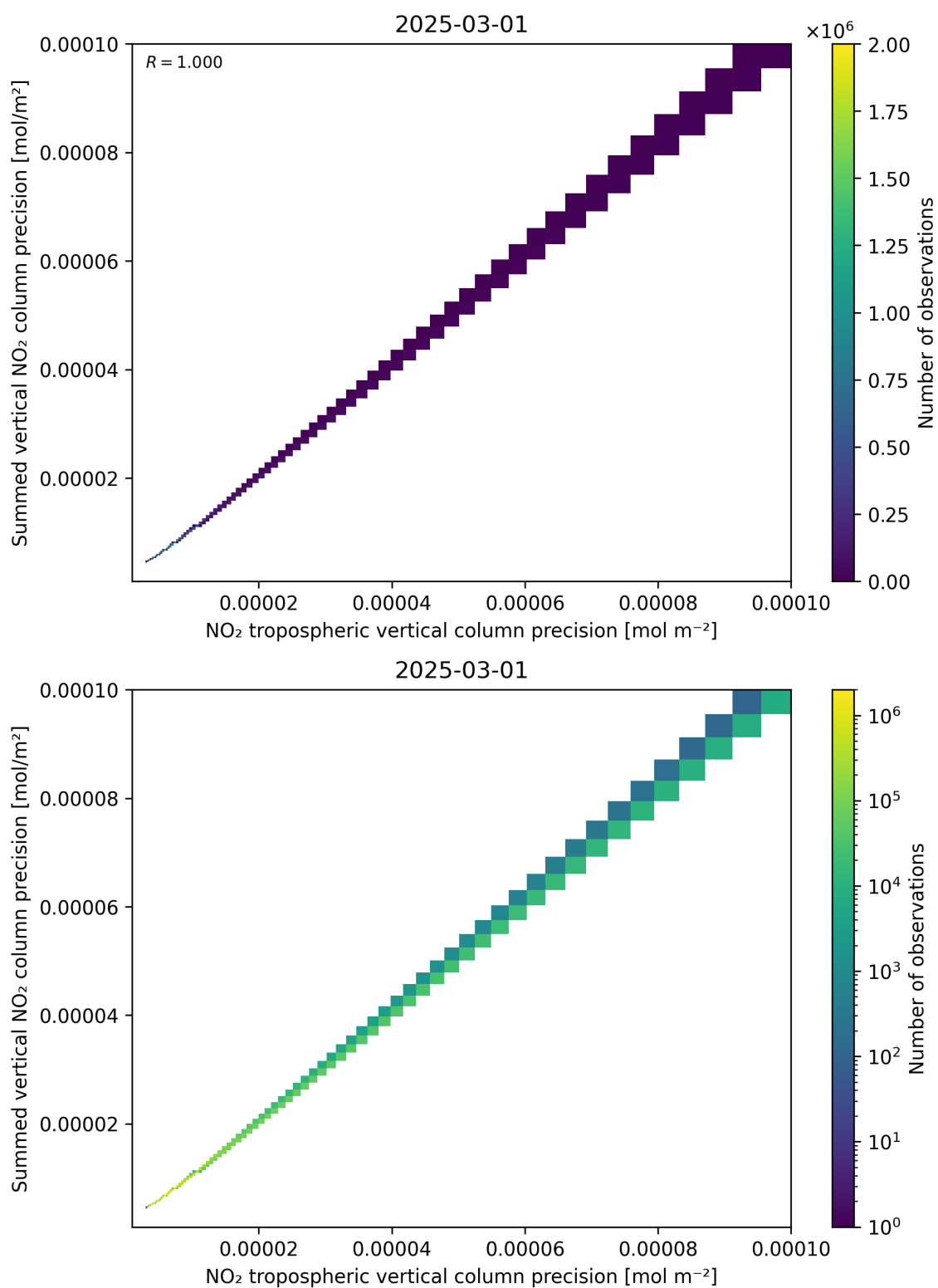
Figure 137: Scatter density plot of “NO 2 tropospheric vertical column precision” against “Summed vertical NO 2 column precision” for 2025-03-01 to 2025-03-02.
