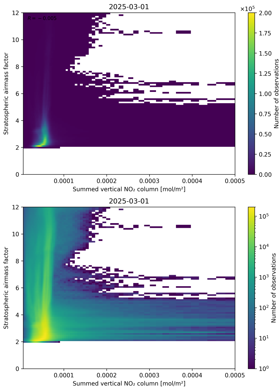
Figure 103: Scatter density plot of “Summed vertical NO 2 column” against “Stratospheric air mass factor” for 2025-03-01 to 2025-03-02.
