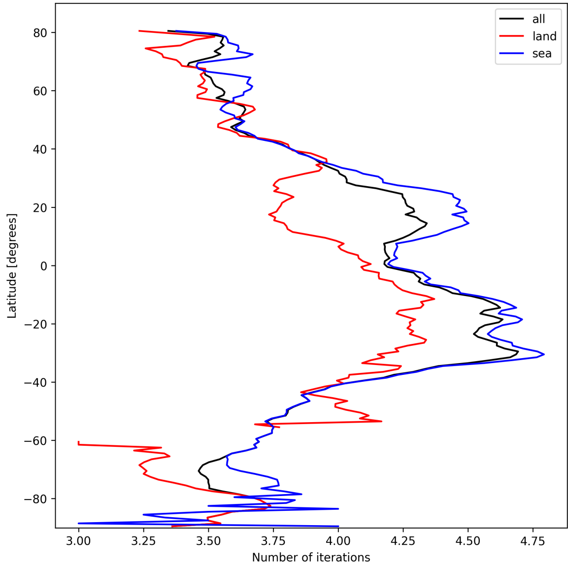
Figure 17: Zonal average of “Number of iterations” for 2025-03-01 to 2025-03-02.
