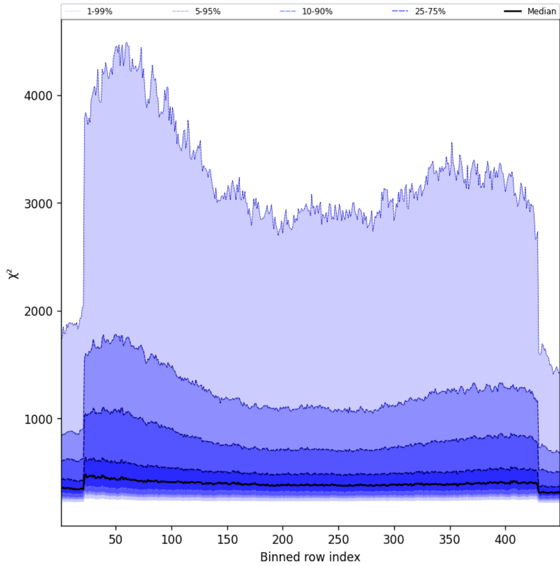
Figure 59: Along track statistics of “ \chi^2 ” for 2025-03-01 to 2025-03-02
