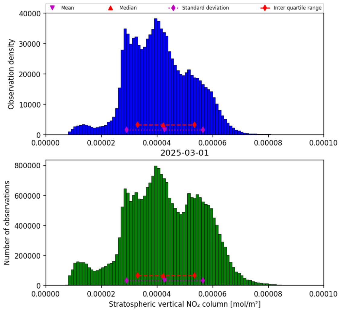
Figure 36: Histogram of “Stratospheric vertical NO 2 column” for 2025-03-01 to 2025-03-02
