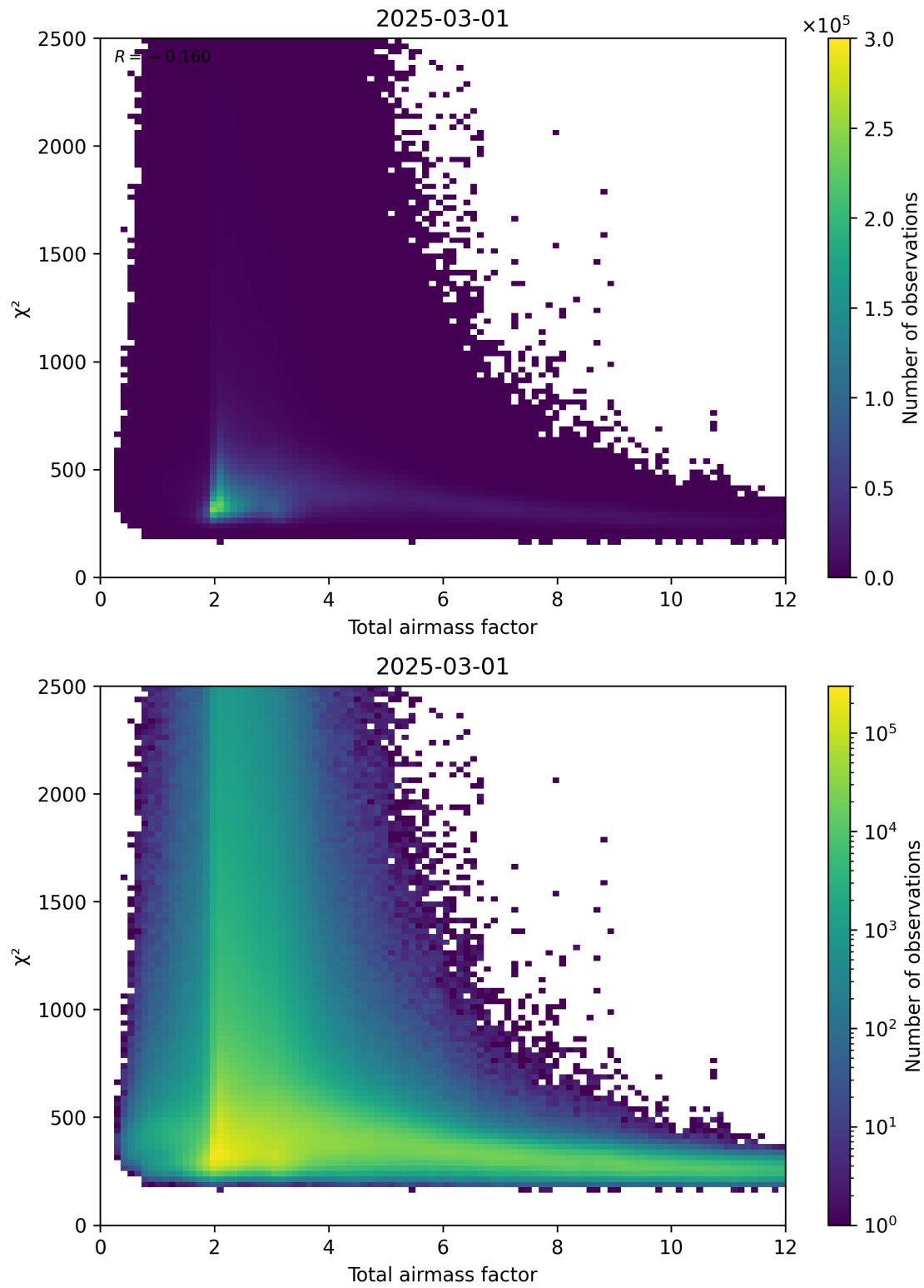
Figure 63: Scatter density plot of “Total airmass factor” against “ \chi^2 ” for 2025-03-01 to 2025-03-02.
