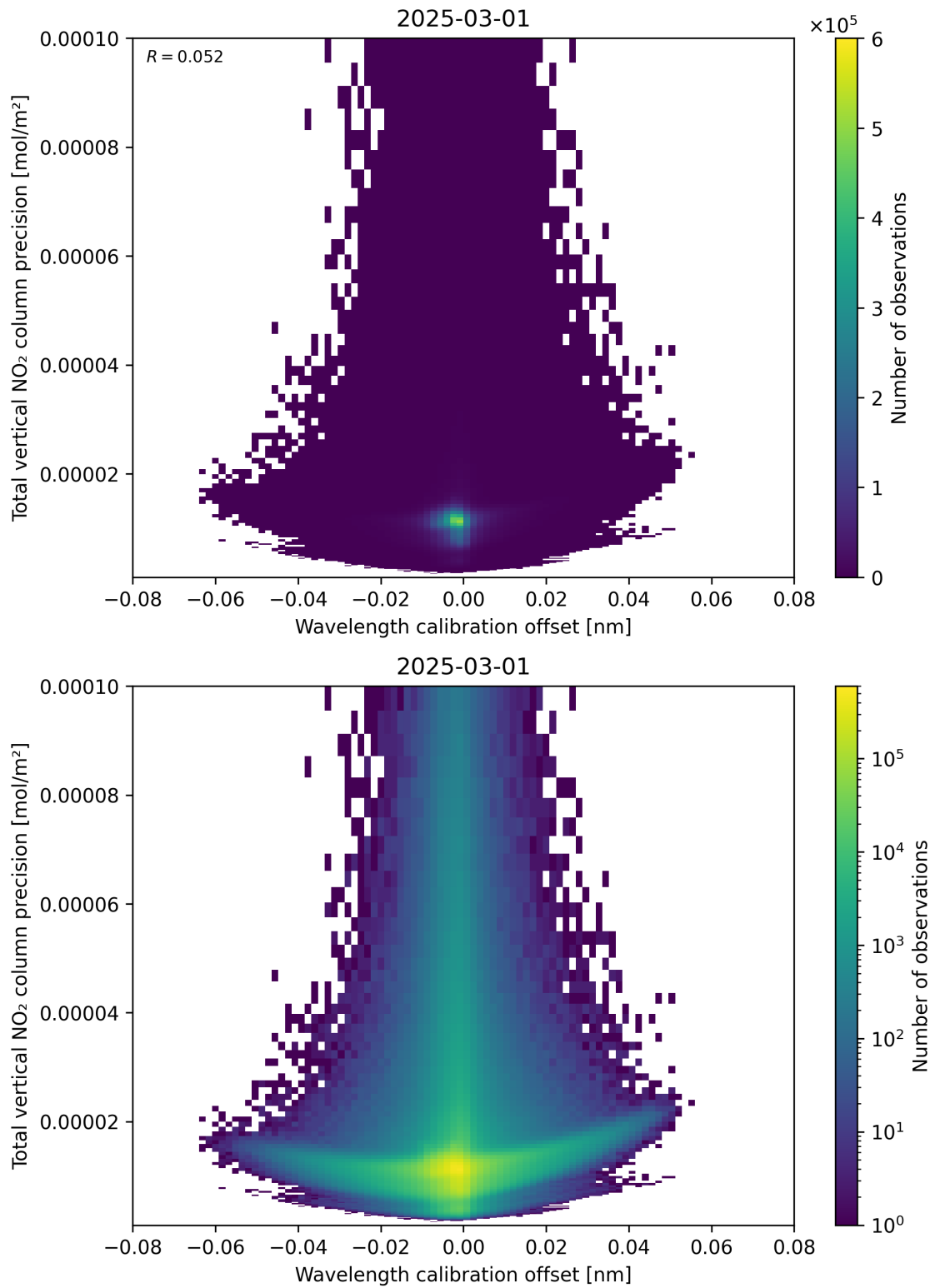
Figure 180: Scatter density plot of “Wavelength calibration offset” against “Total vertical NO 2 column precision” for 2025-03-01 to 2025-03-02.
