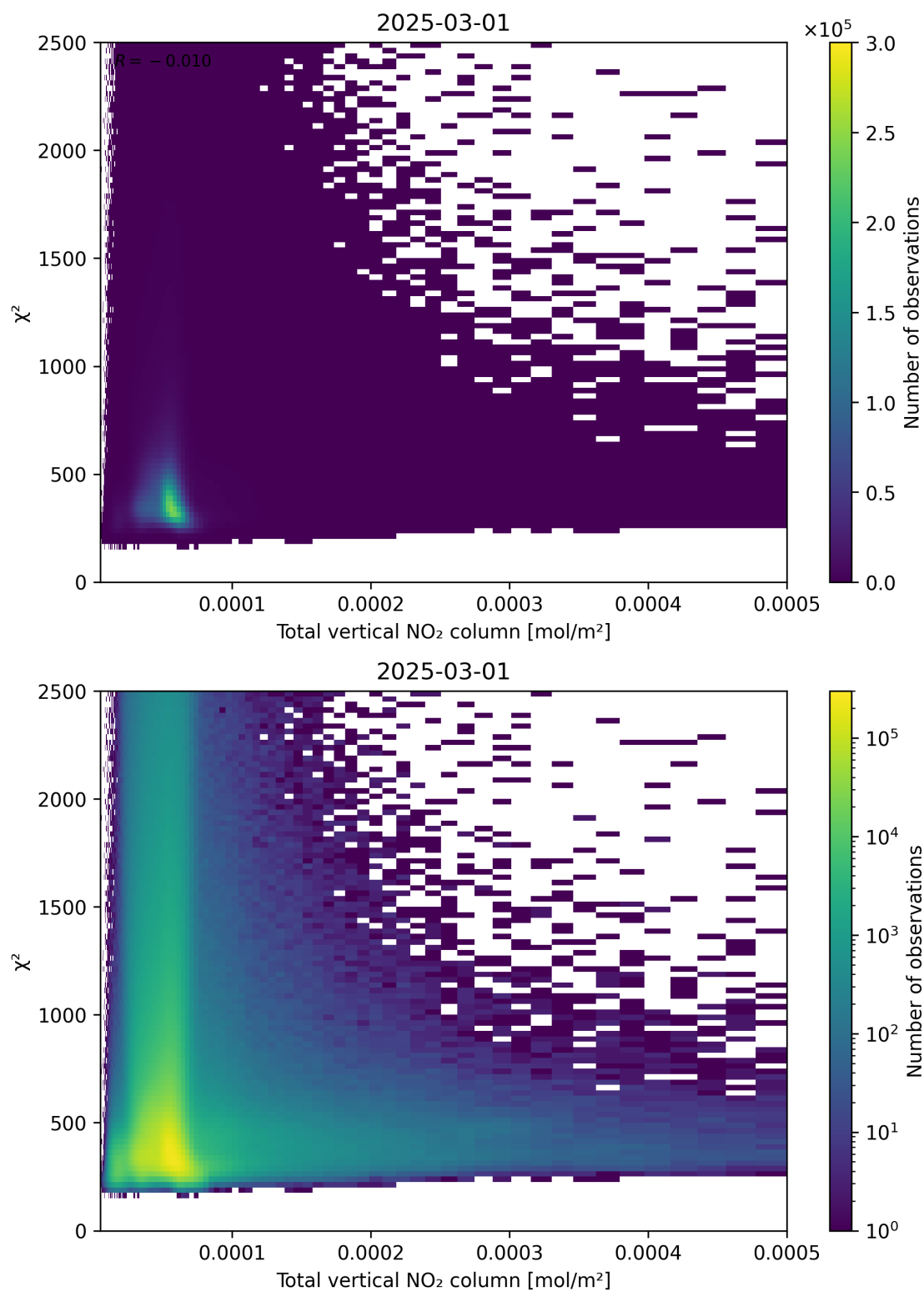
Figure 111: Scatter density plot of “Total vertical NO 2 column” against “ \chi^2 ” for 2025-03-01 to 2025-03-02.
