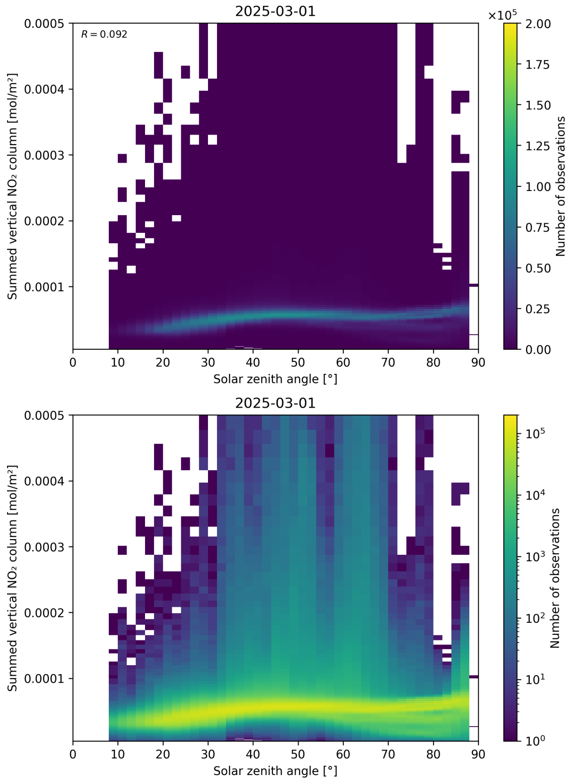
Figure 151: Scatter density plot of “Solar zenith angle” against “Summed vertical NO 2 column” for 2025-03-01 to 2025-03-02.
