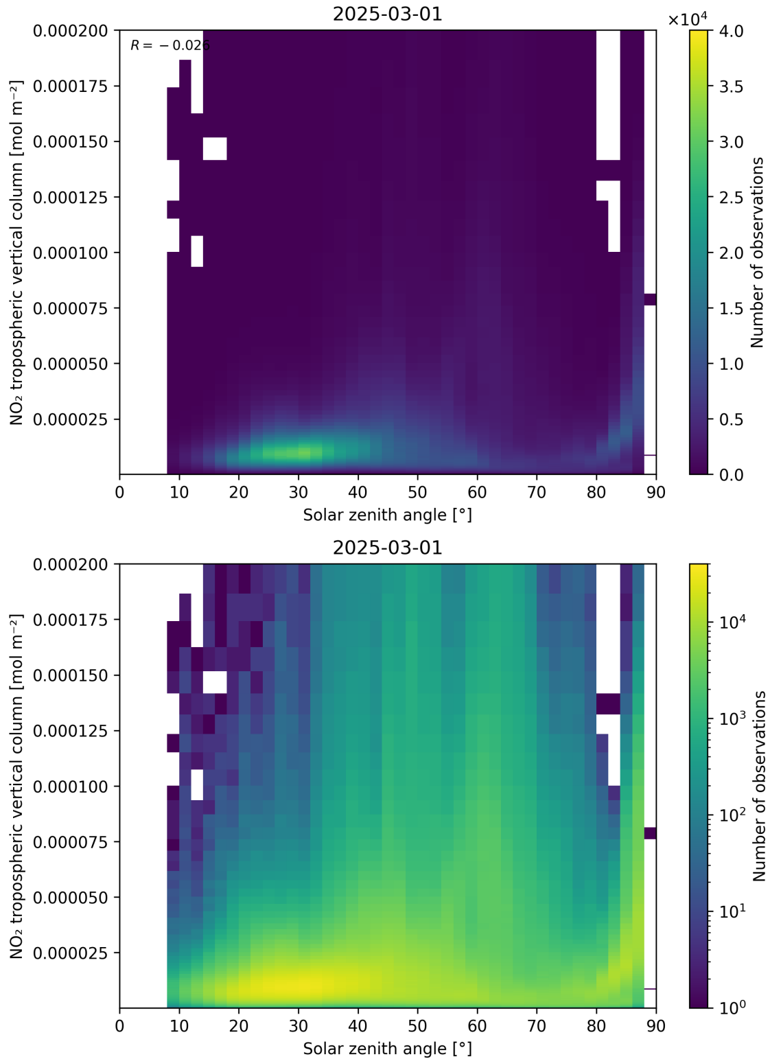
Figure 155: Scatter density plot of “Solar zenith angle” against “NO 2 tropospheric vertical column” for 2025-03-01 to 2025-03-02.
