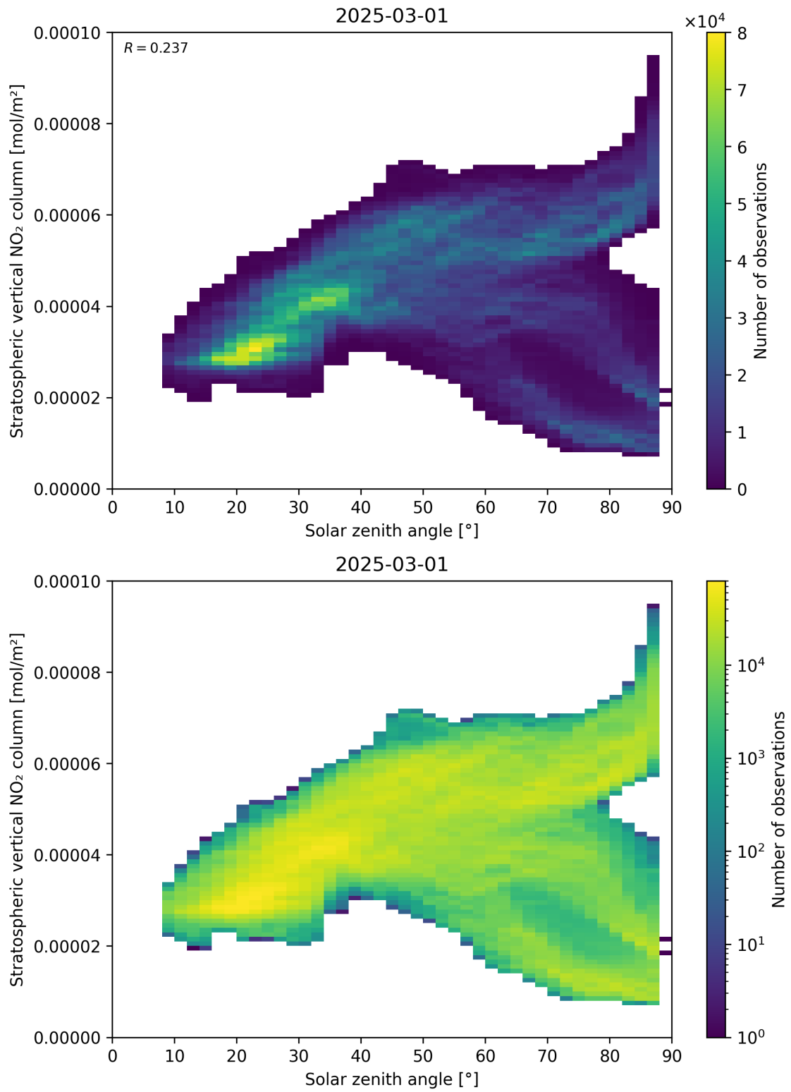
Figure 150: Scatter density plot of “Solar zenith angle” against “Stratospheric vertical NO 2 column” for 2025-03-01 to 2025-03-02.
