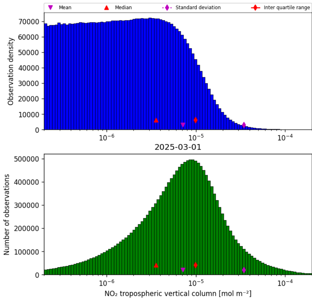
Figure 29: Histogram of “NO 2 tropospheric vertical column” for 2025-03-01 to 2025-03-02
