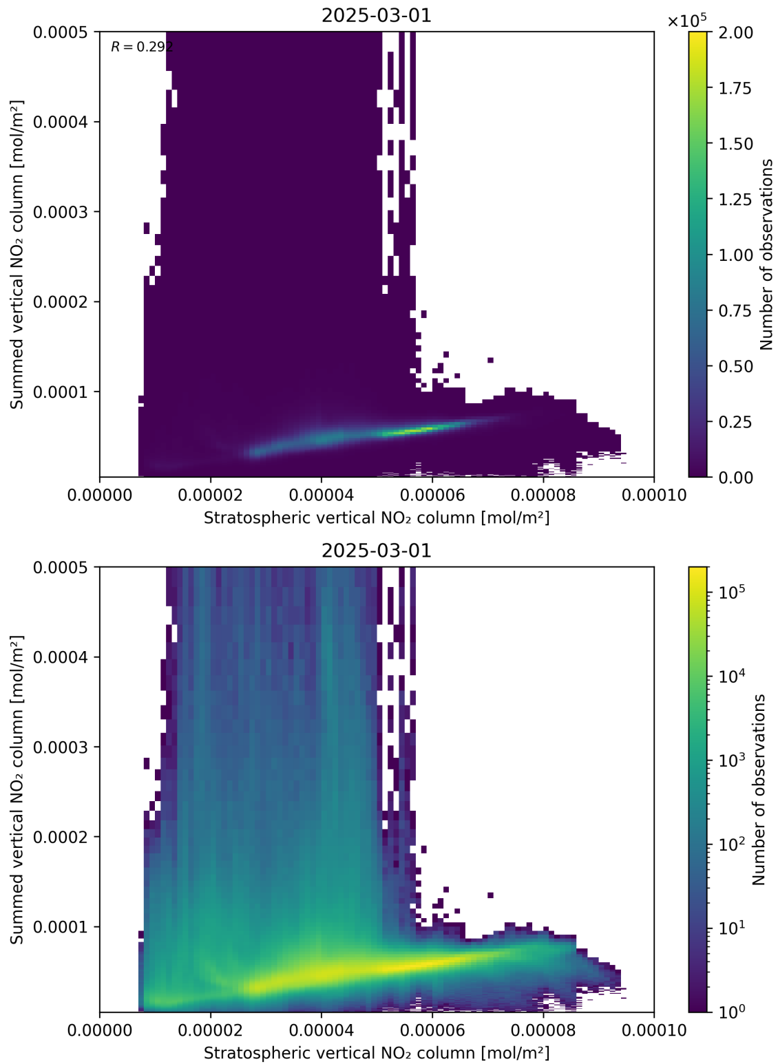
Figure 98: Scatter density plot of “Stratospheric vertical NO 2 column” against “Summed vertical NO 2 column” for 2025-03-01 to 2025-03-02.
