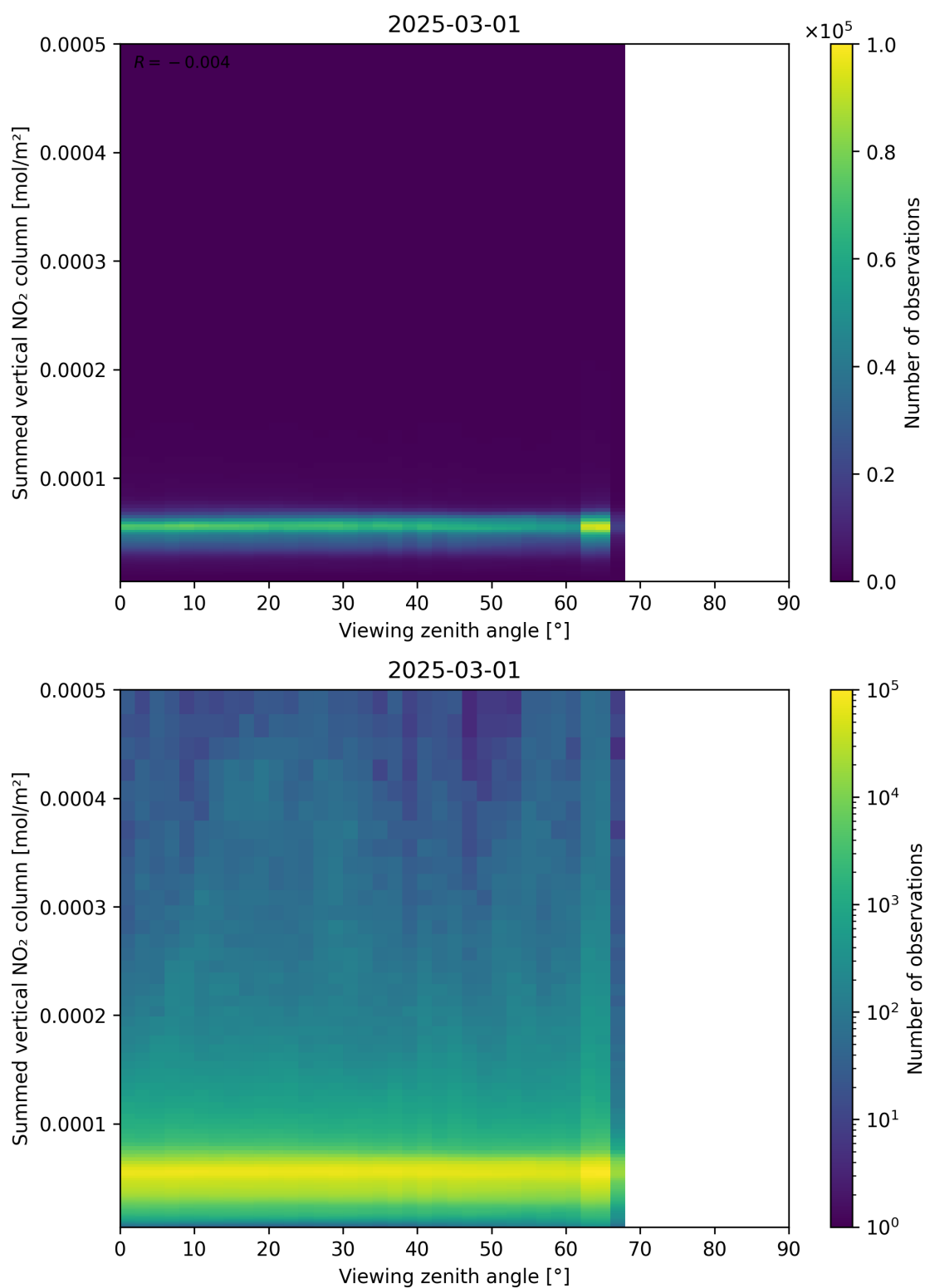
Figure 165: Scatter density plot of “Viewing zenith angle” against “Summed vertical NO 2 column” for 2025-03-01 to 2025-03-02.
