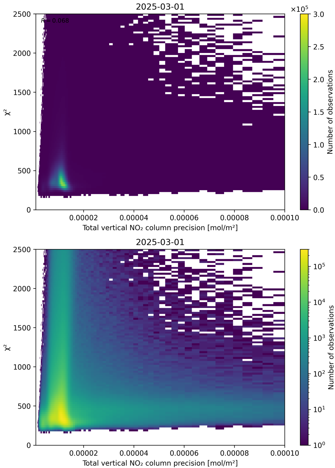
Figure 116: Scatter density plot of “Total vertical NO 2 column precision” against “ \chi^2 ” for 2025-03-01 to 2025-03-02.
