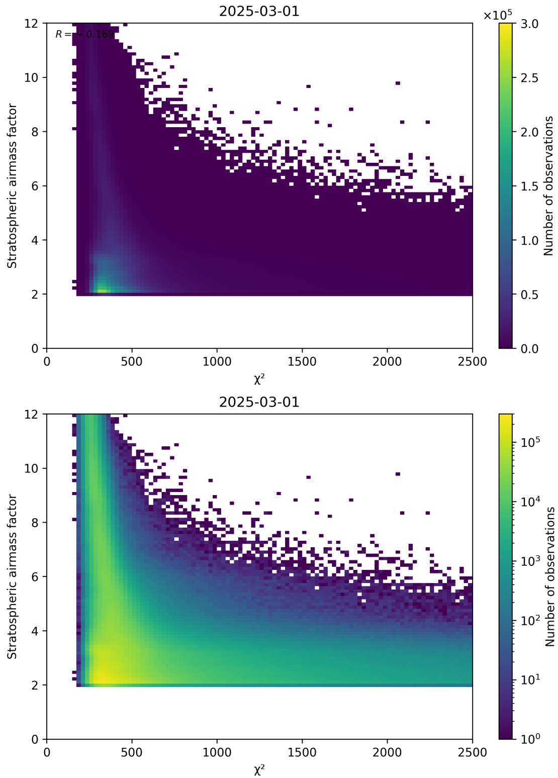
Figure 81: Scatter density plot of “ \chi^2 ” against “Stratospheric airmass factor” for 2025-03-01 to 2025-03-02.
