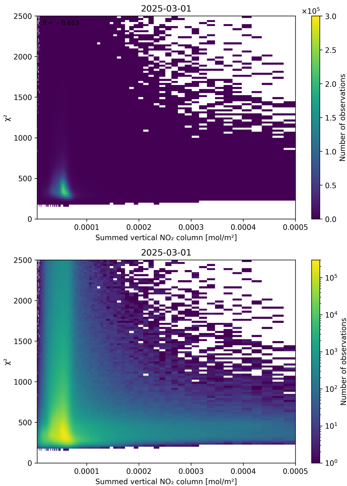
Figure 104: Scatter density plot of “Summed vertical NO 2 column” against “ \chi^2 ” for 2025-03-01 to 2025-03-02.
