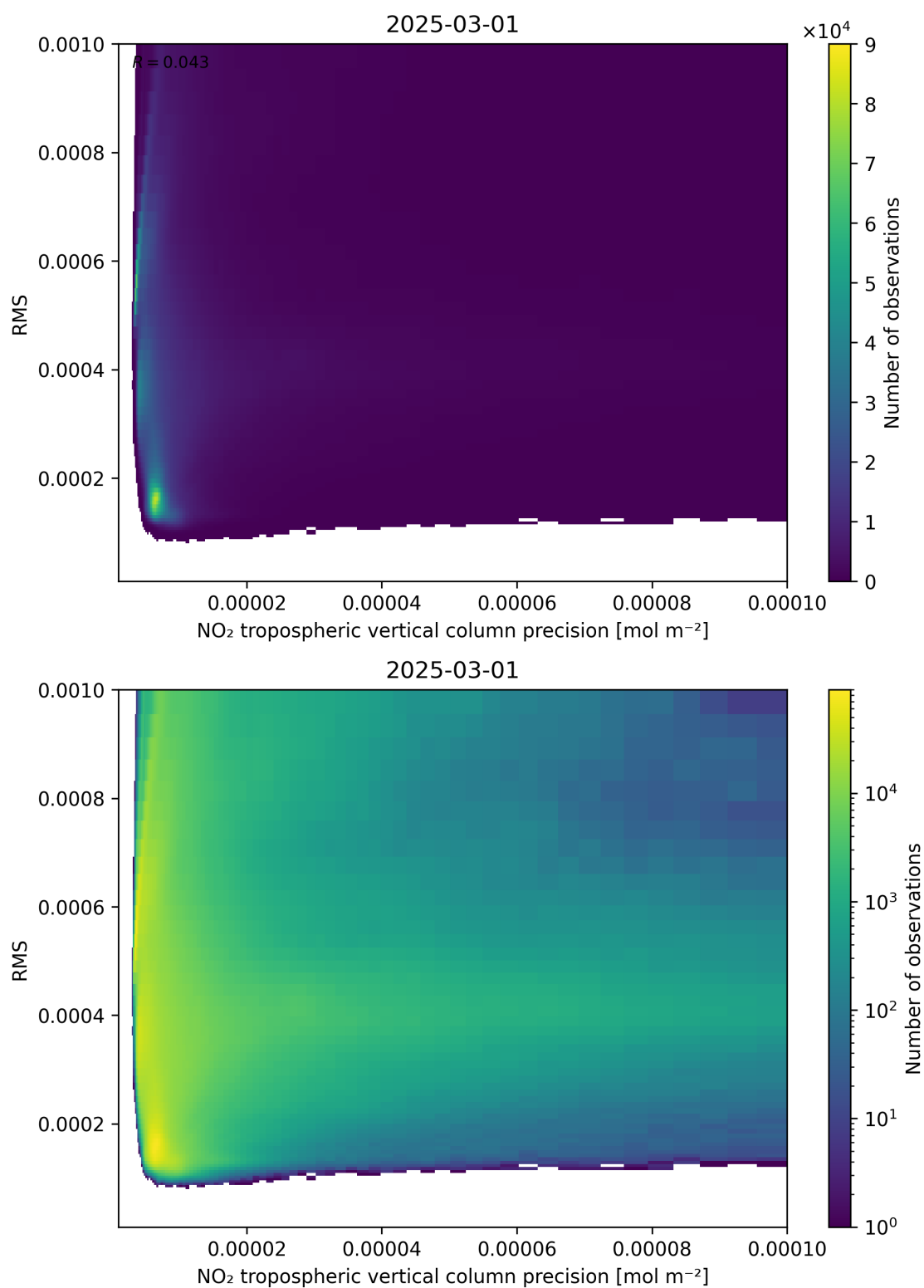
Figure 140: Scatter density plot of “NO 2 tropospheric vertical column precision” against “RMS” for 2025-03-01 to 2025-03-02.
