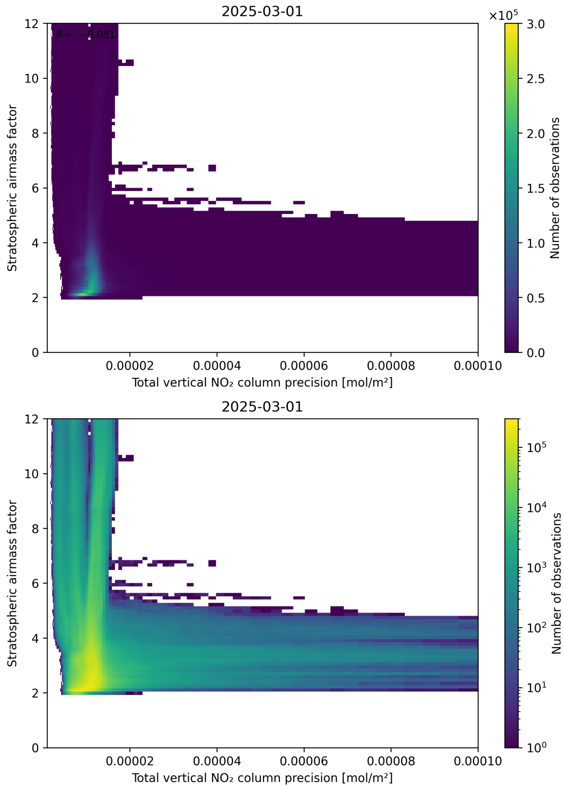
Figure 115: Scatter density plot of “Total vertical NO 2 column precision” against “Stratospheric air mass factor” for 2025-03-01 to 2025-03-02.
