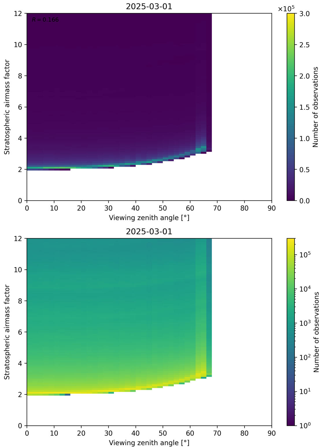
Figure 159: Scatter density plot of “Viewing zenith angle” against “Stratospheric airmass factor” for 2025-03-01 to 2025-03-02.
