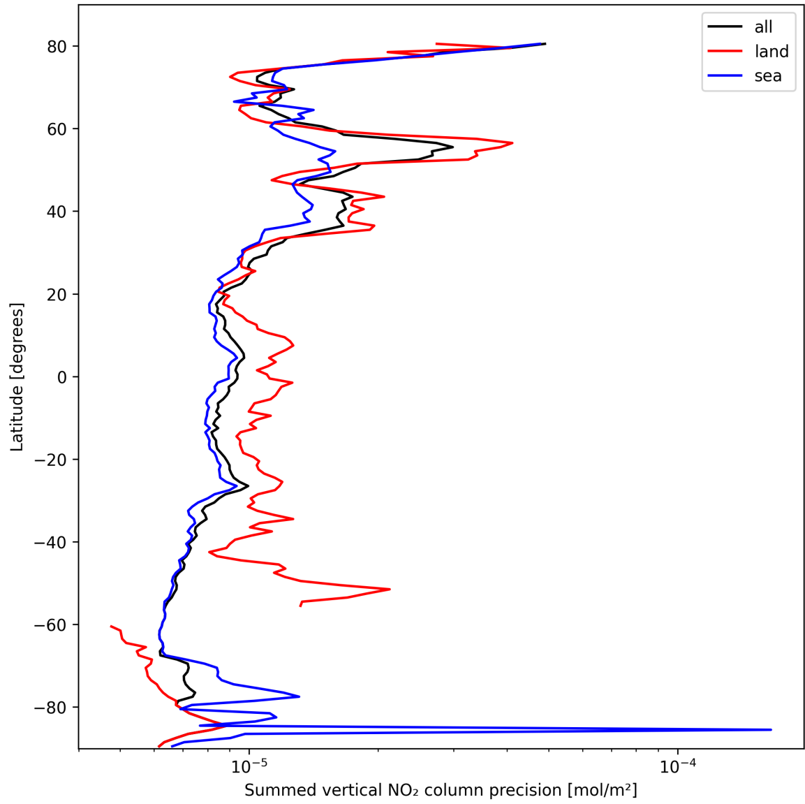
Figure 24: Zonal average of “Summed vertical NO 2 column precision” for 2025-03-01 to 2025-03-02.
