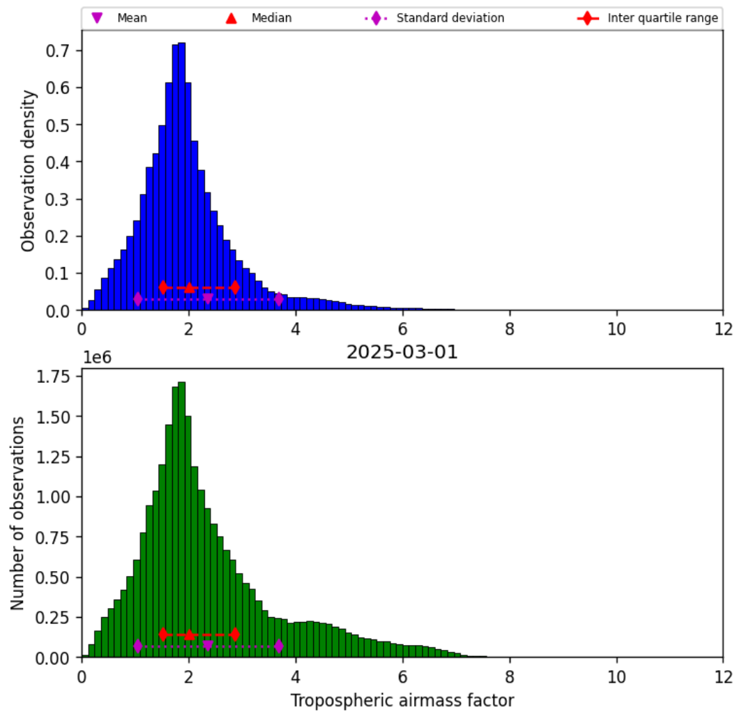
Figure 31: Histogram of “Tropospheric airmass factor” for 2025-03-01 to 2025-03-02
