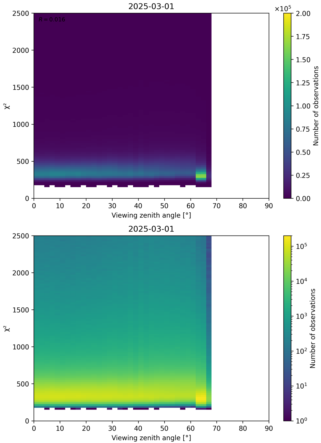
Figure 162: Scatter density plot of “Viewing zenith angle” against “ \chi^2 ” for 2025-03-01 to 2025-03-02.
