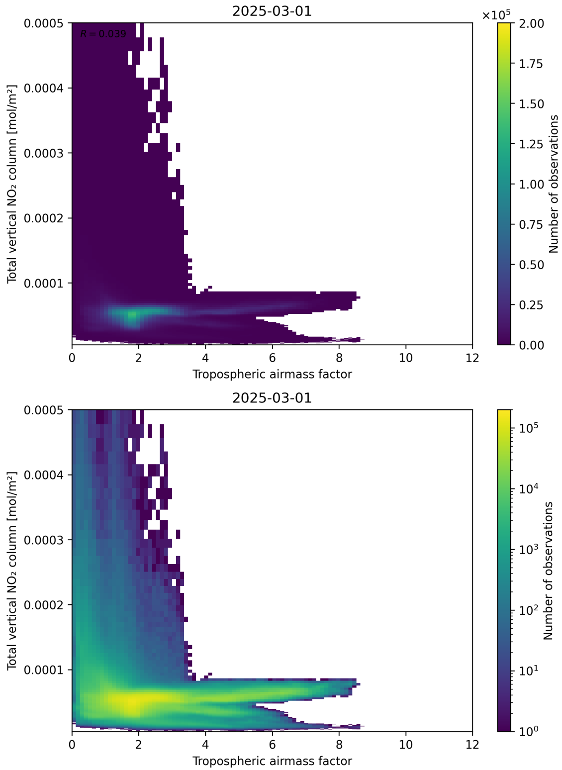
Figure 77: Scatter density plot of “Tropospheric airmass factor” against “Total vertical \text{NO}_2 column” for 2025-03-01 to 2025-03-02.
