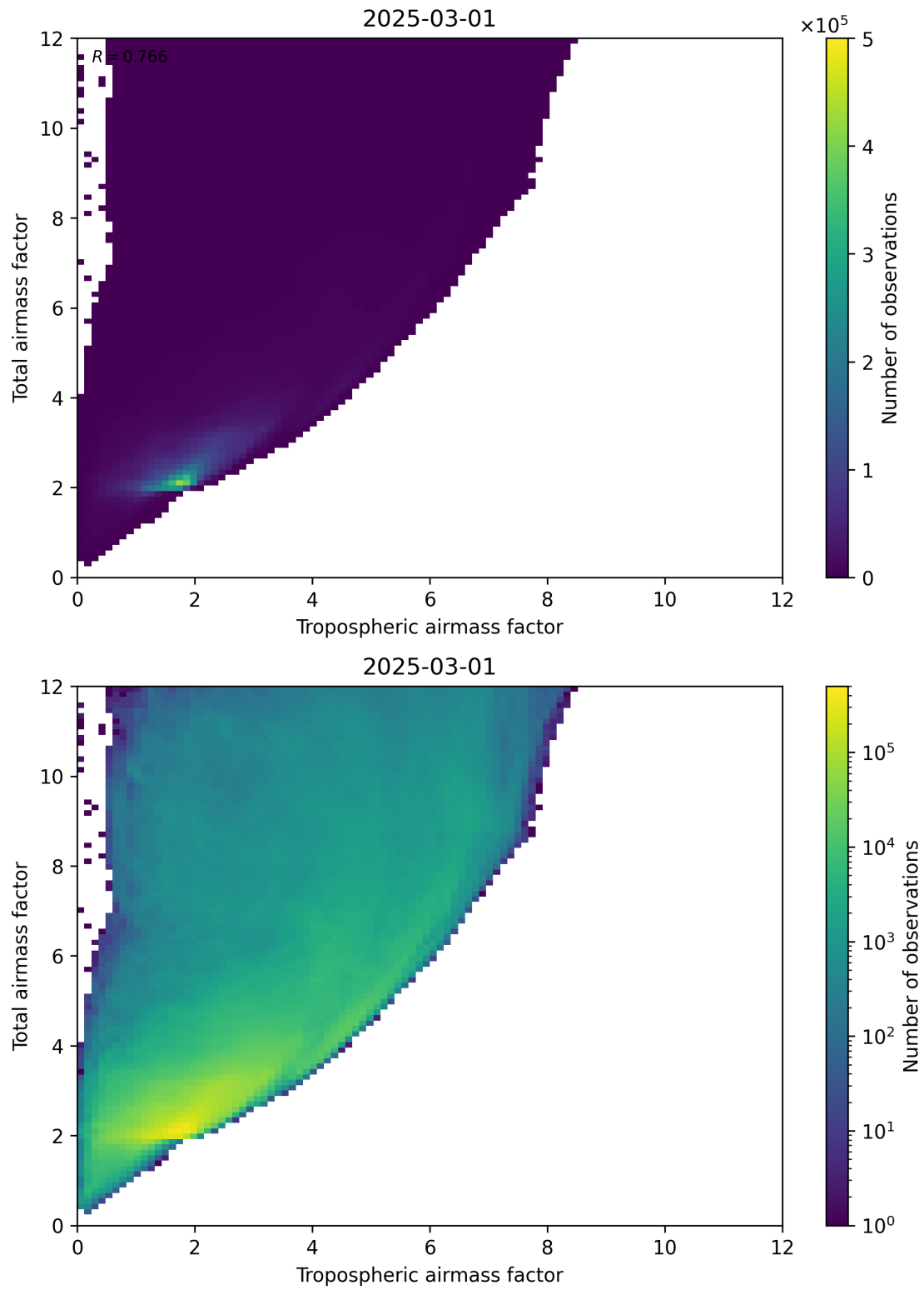
Figure 72: Scatter density plot of “Tropospheric airmass factor” against “Total airmass factor” for 2025-03-01 to 2025-03-02.
