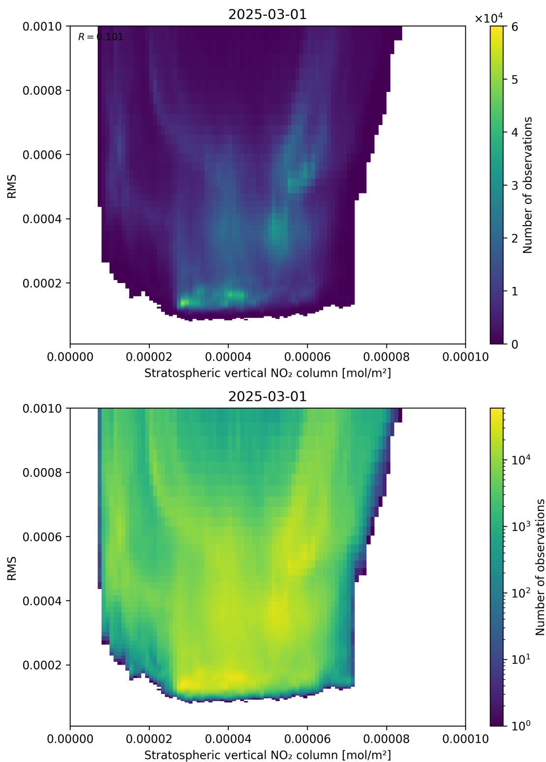
Figure 102: Scatter density plot of “Stratospheric vertical NO 2 column” against “RMS” for 2025-03-01 to 2025-03-02.
