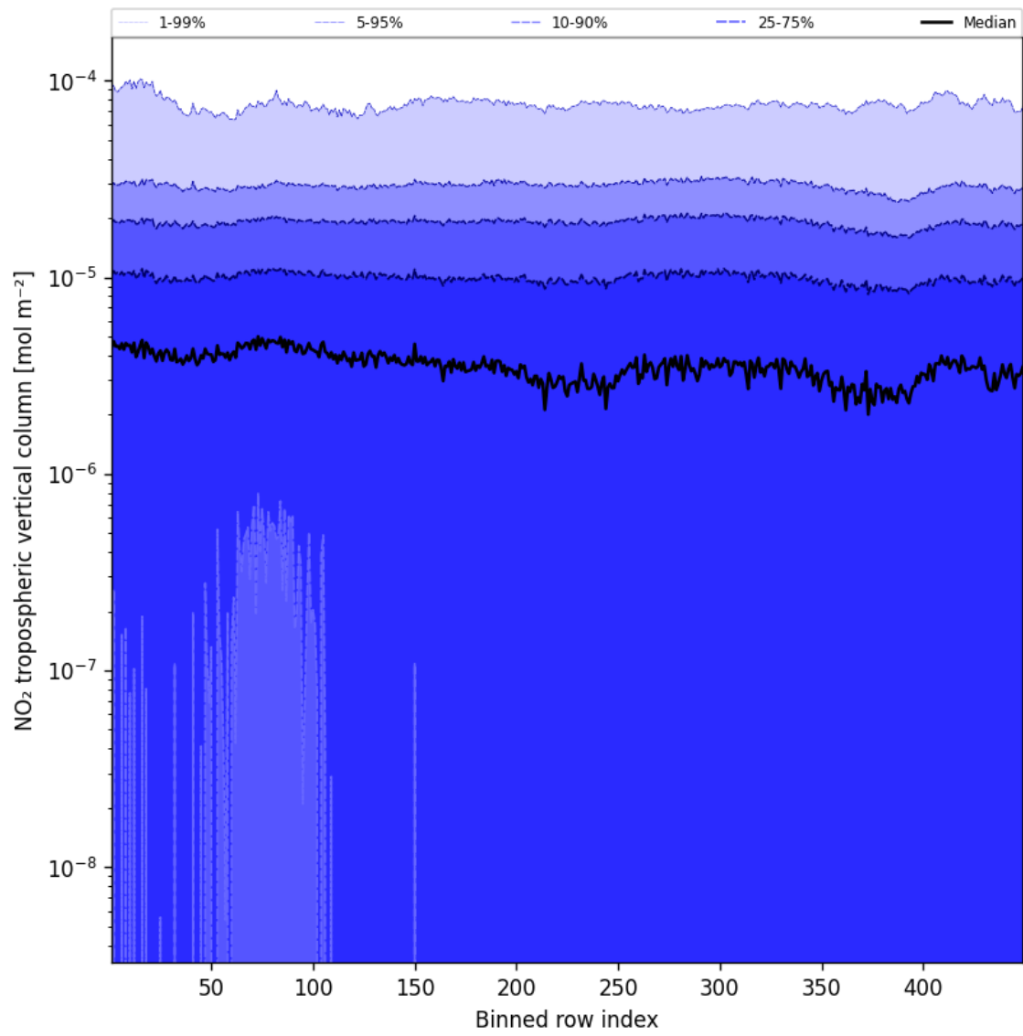
Figure 46: Along track statistics of “NO 2 tropospheric vertical column” for 2025-03-01 to 2025-03-02
