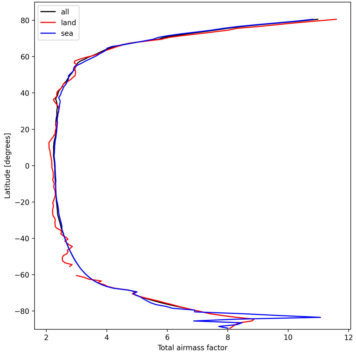
Figure 15: Zonal average of “Total airmass factor” for 2025-03-01 to 2025-03-02.
