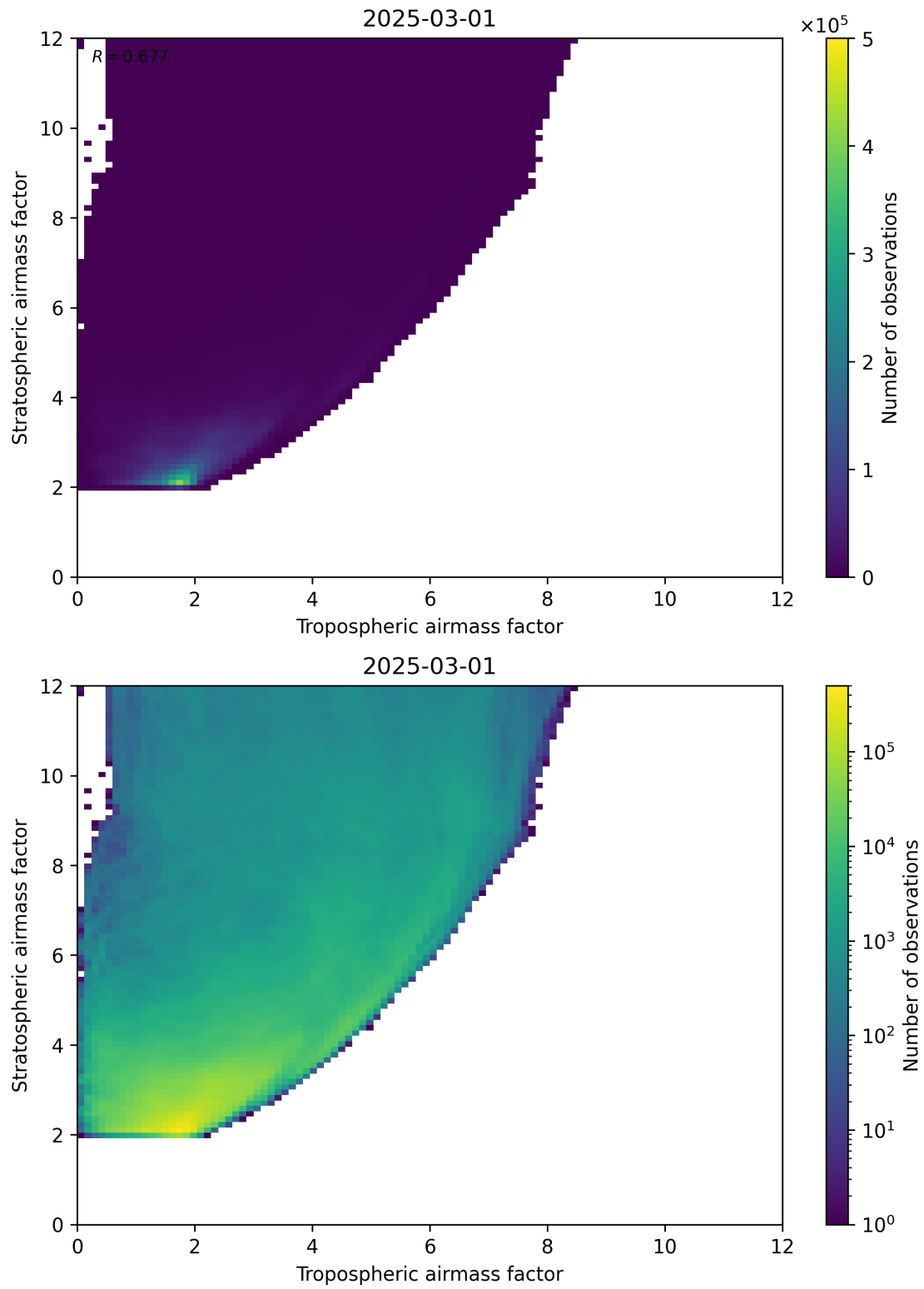
Figure 71: Scatter density plot of “Tropospheric airmass factor” against “Stratospheric airmass factor” for 2025-03-01 to 2025-03-02.
