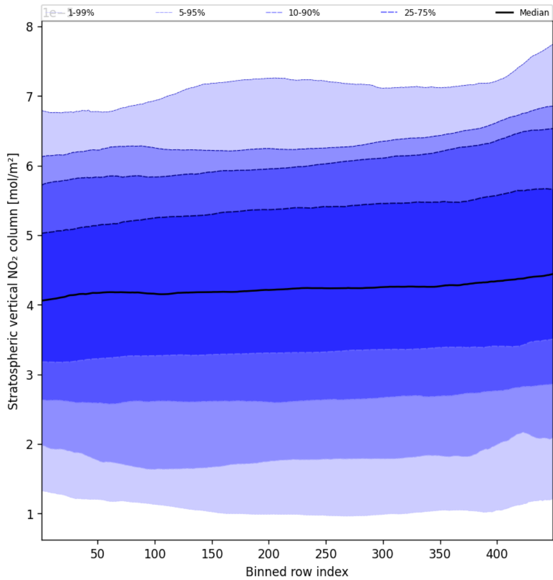
Figure 53: Along track statistics of “Stratospheric vertical NO 2 column” for 2025-03-01 to 2025-03-02
