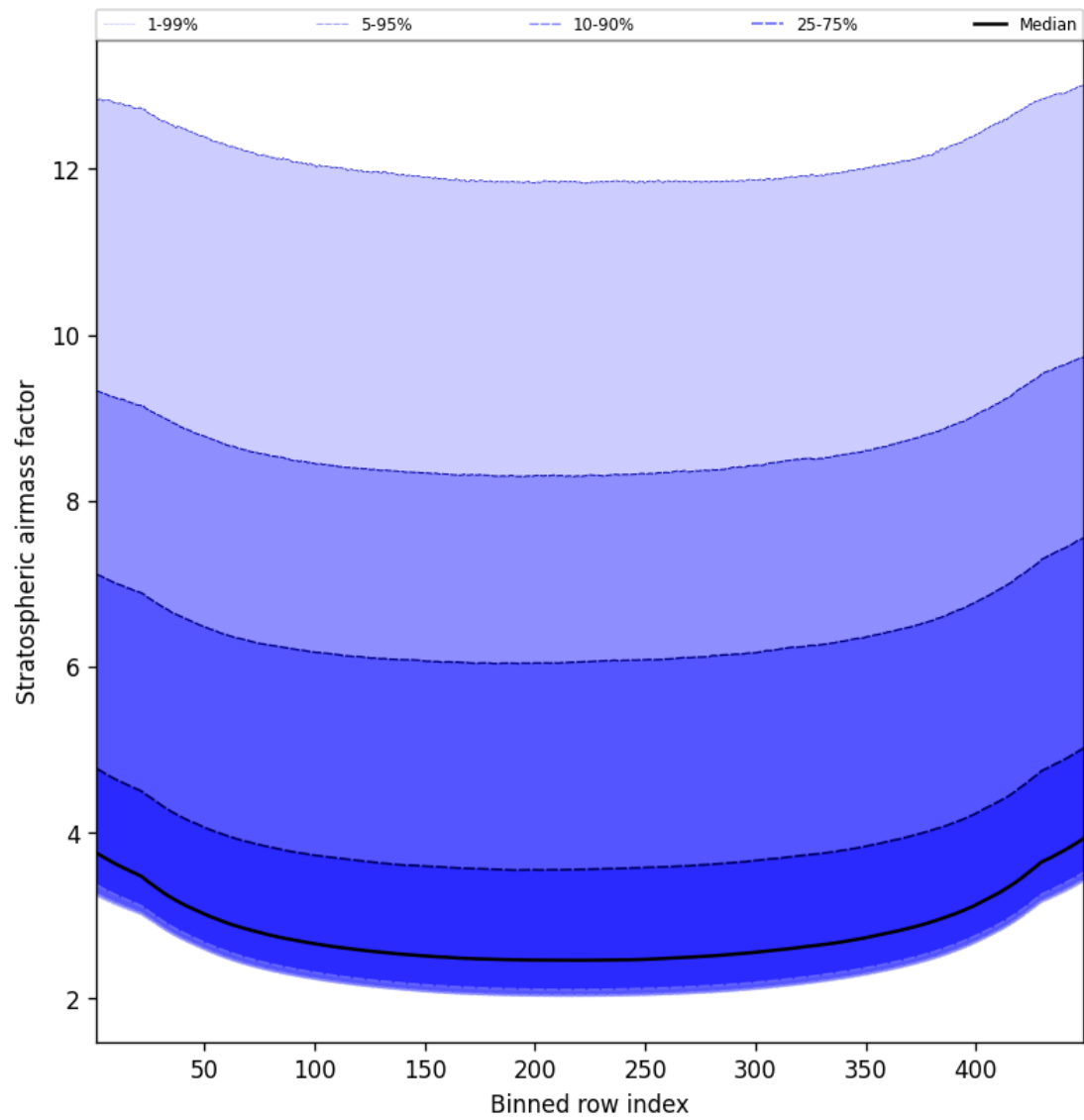
Figure 61: Along track statistics of “Stratospheric airmass factor” for 2025-03-01 to 2025-03-02
