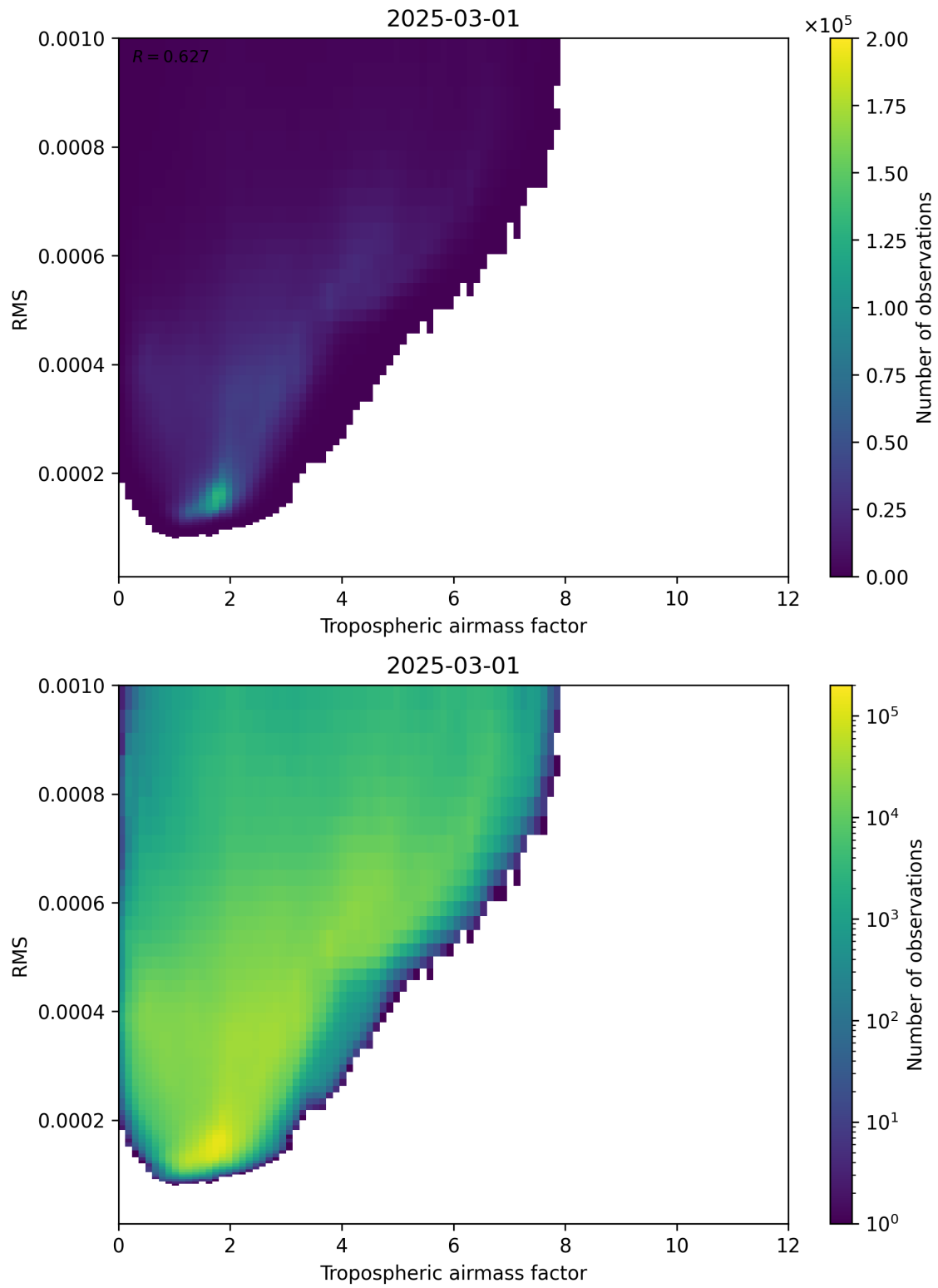
Figure 79: Scatter density plot of “Tropospheric airmass factor” against “RMS” for 2025-03-01 to 2025-03-02.
