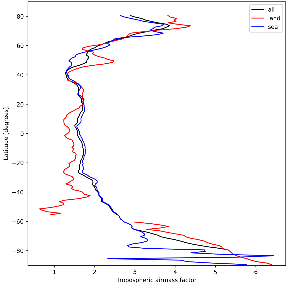
Figure 14: Zonal average of “Tropospheric airmass factor” for 2025-03-01 to 2025-03-02.
