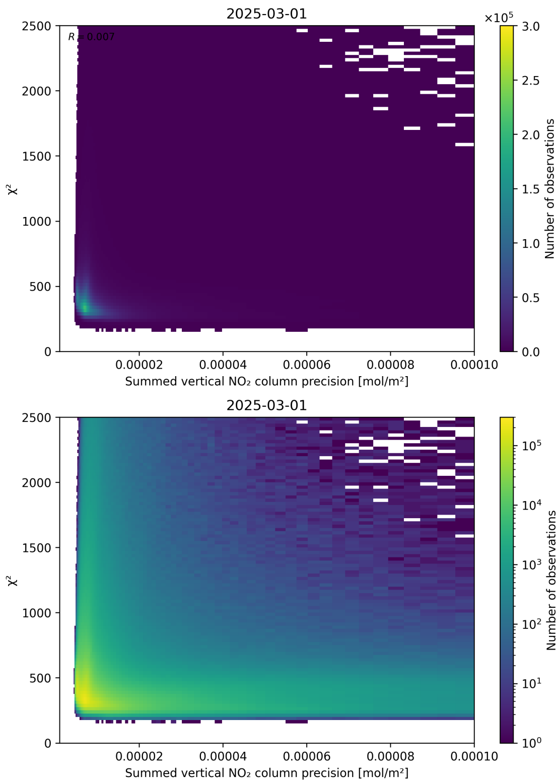
Figure 107: Scatter density plot of “Summed vertical NO 2 column precision” against “ \chi^2 ” for 2025-03-01 to 2025-03-02.
