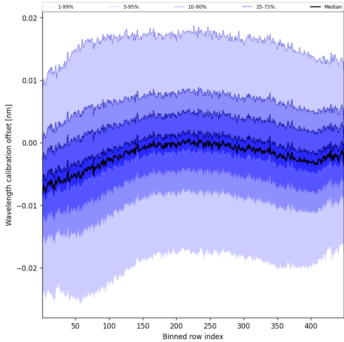
Figure 52: Along track statistics of “Wavelength calibration offset” for 2025-03-01 to 2025-03-02
