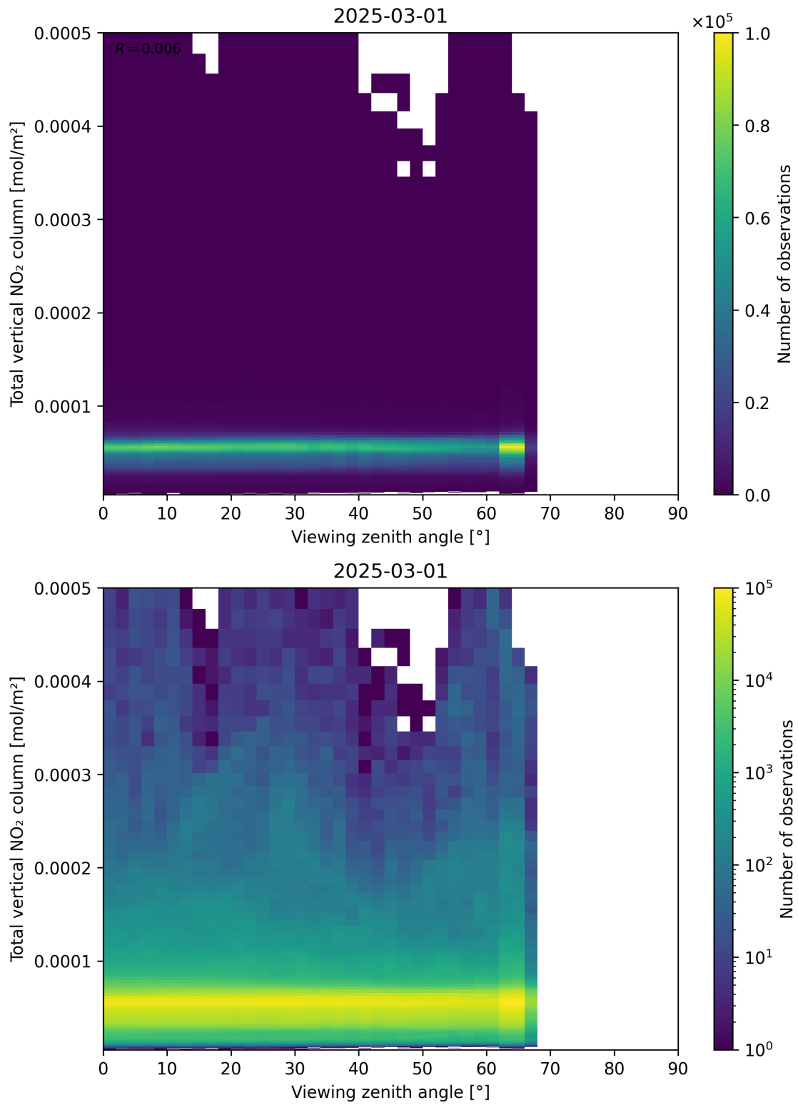
Figure 167: Scatter density plot of “Viewing zenith angle” against “Total vertical NO 2 column” for 2025-03-01 to 2025-03-02.
