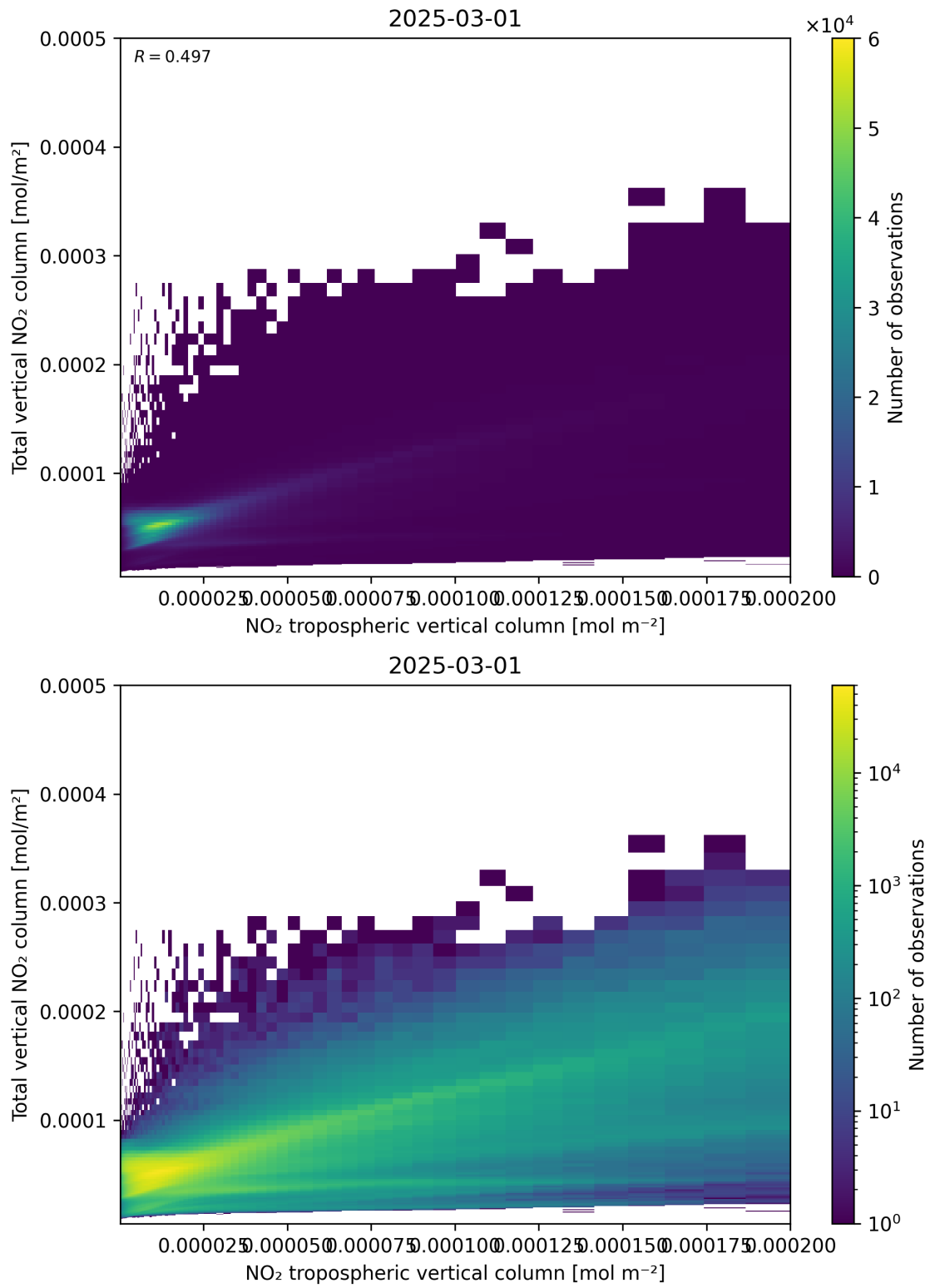
Figure 128: Scatter density plot of “NO 2 tropospheric vertical column” against “Total vertical NO 2 column” for 2025-03-01 to 2025-03-02.
