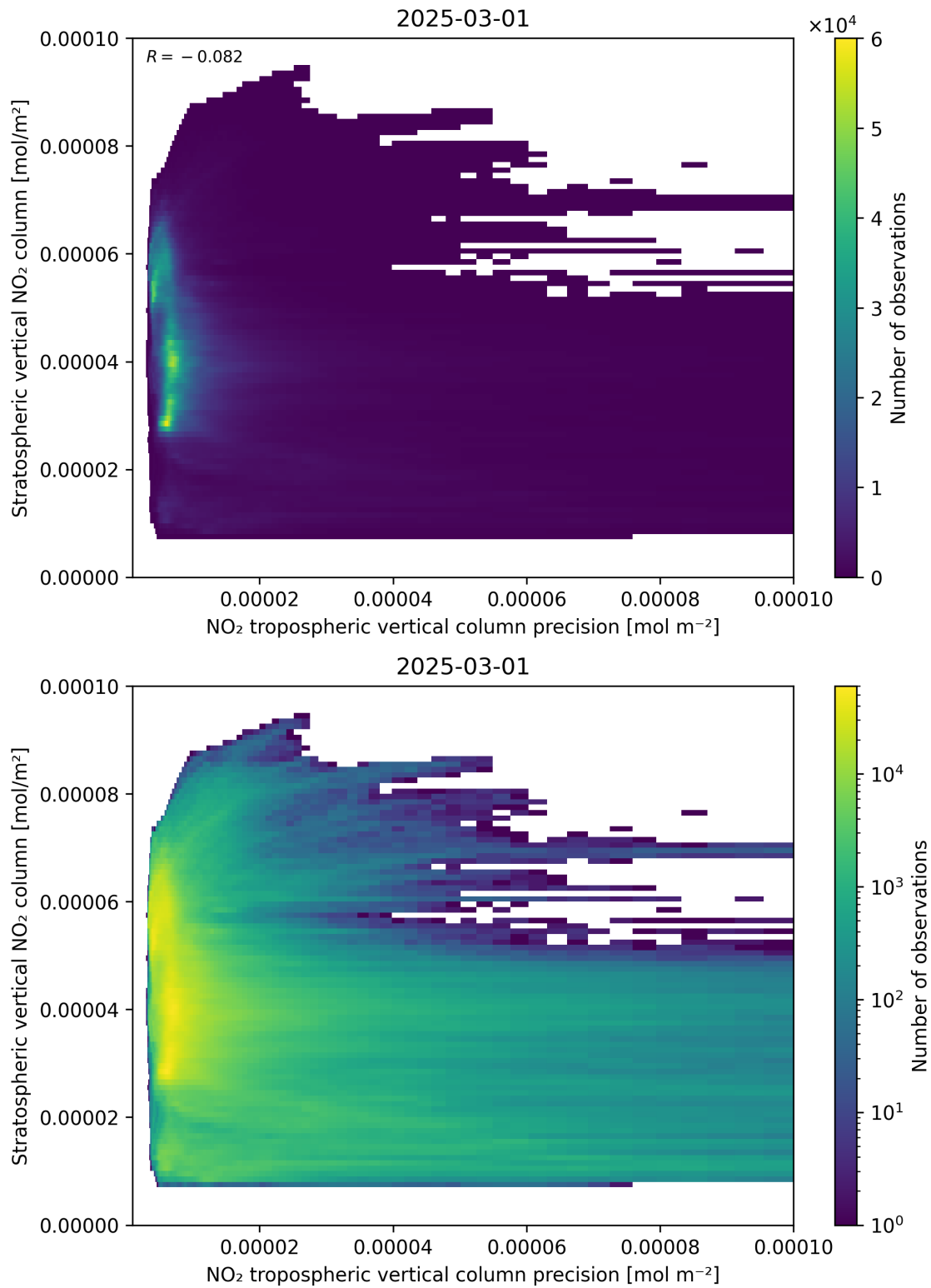
Figure 135: Scatter density plot of “NO 2 tropospheric vertical column precision” against “Stratospheric vertical NO 2 column” for 2025-03-01 to 2025-03-02.
