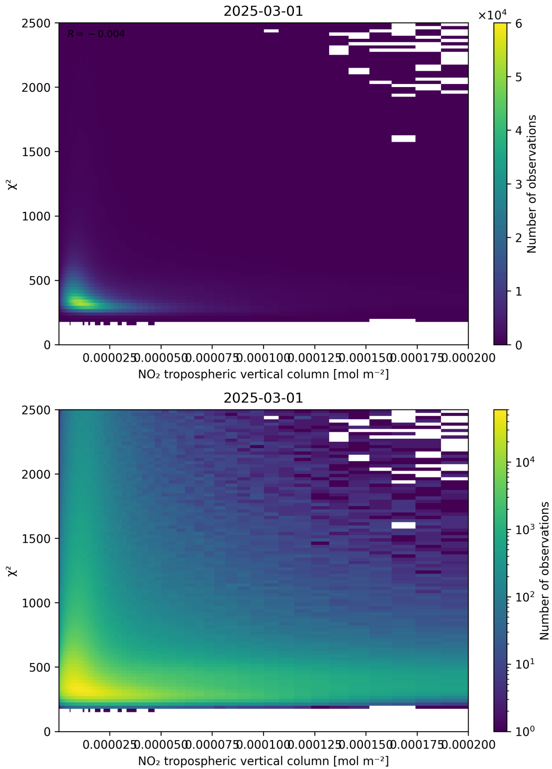
Figure 124: Scatter density plot of “NO 2 tropospheric vertical column” against “ \chi^2 ” for 2025-03-01 to 2025-03-02.
