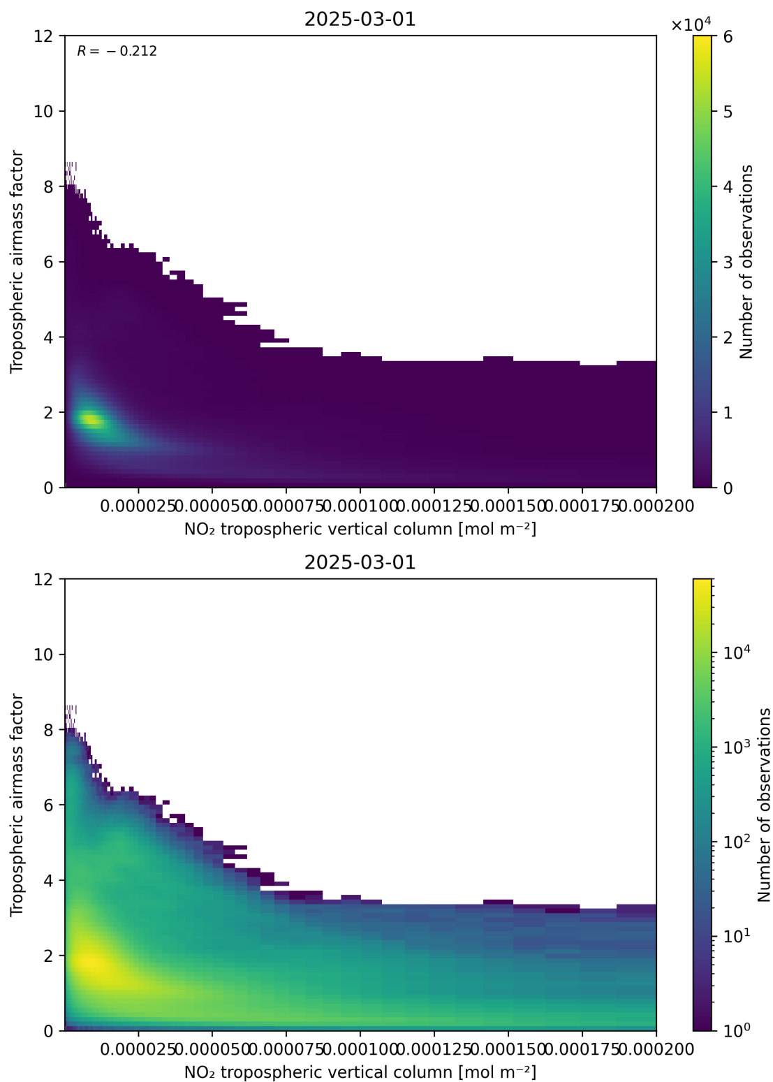
Figure 123: Scatter density plot of “NO 2 tropospheric vertical column” against “Tropospheric air mass factor” for 2025-03-01 to 2025-03-02.
