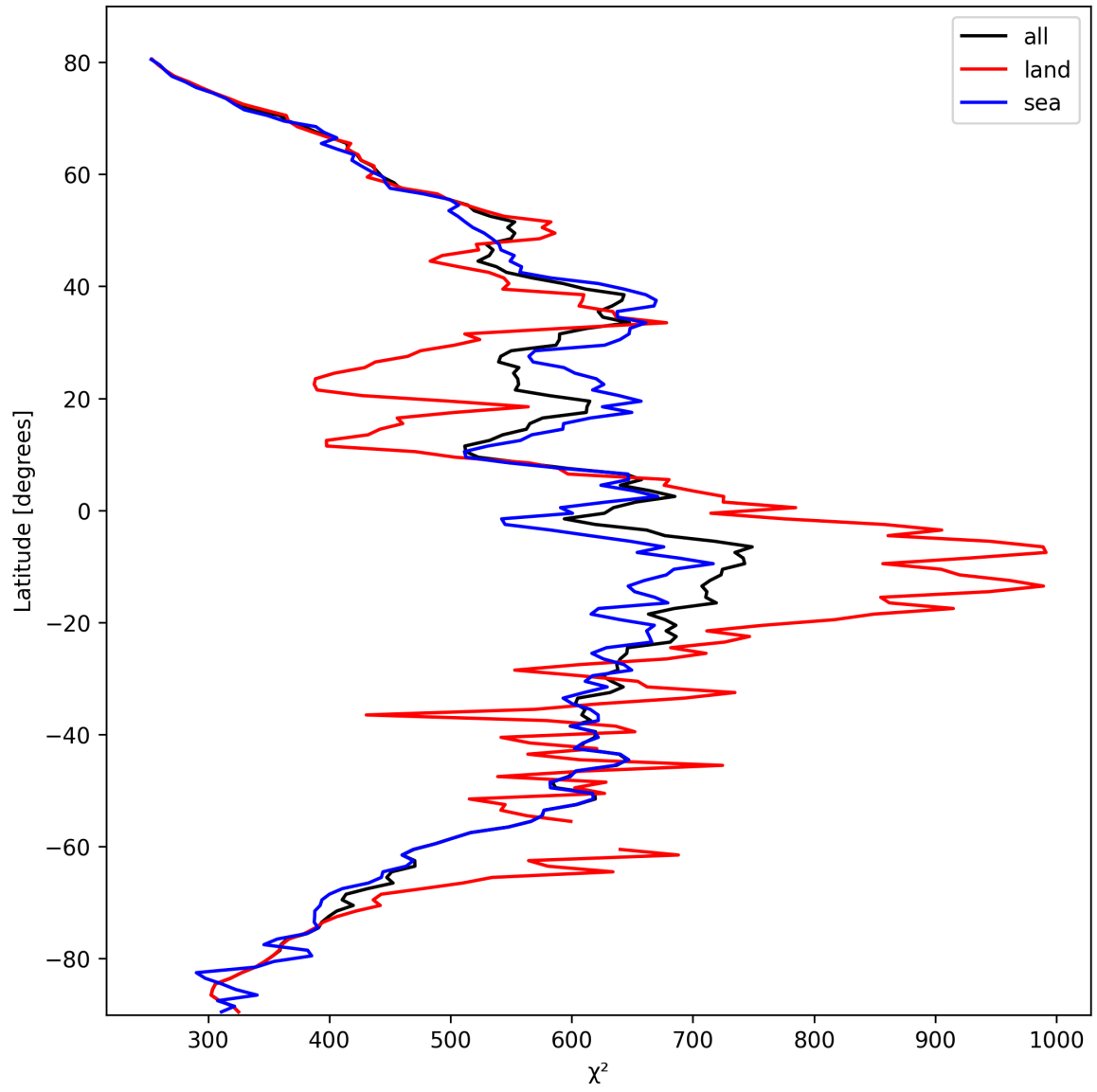
Figure 25: Zonal average of “ \chi^2 ” for 2025-03-01 to 2025-03-02.
