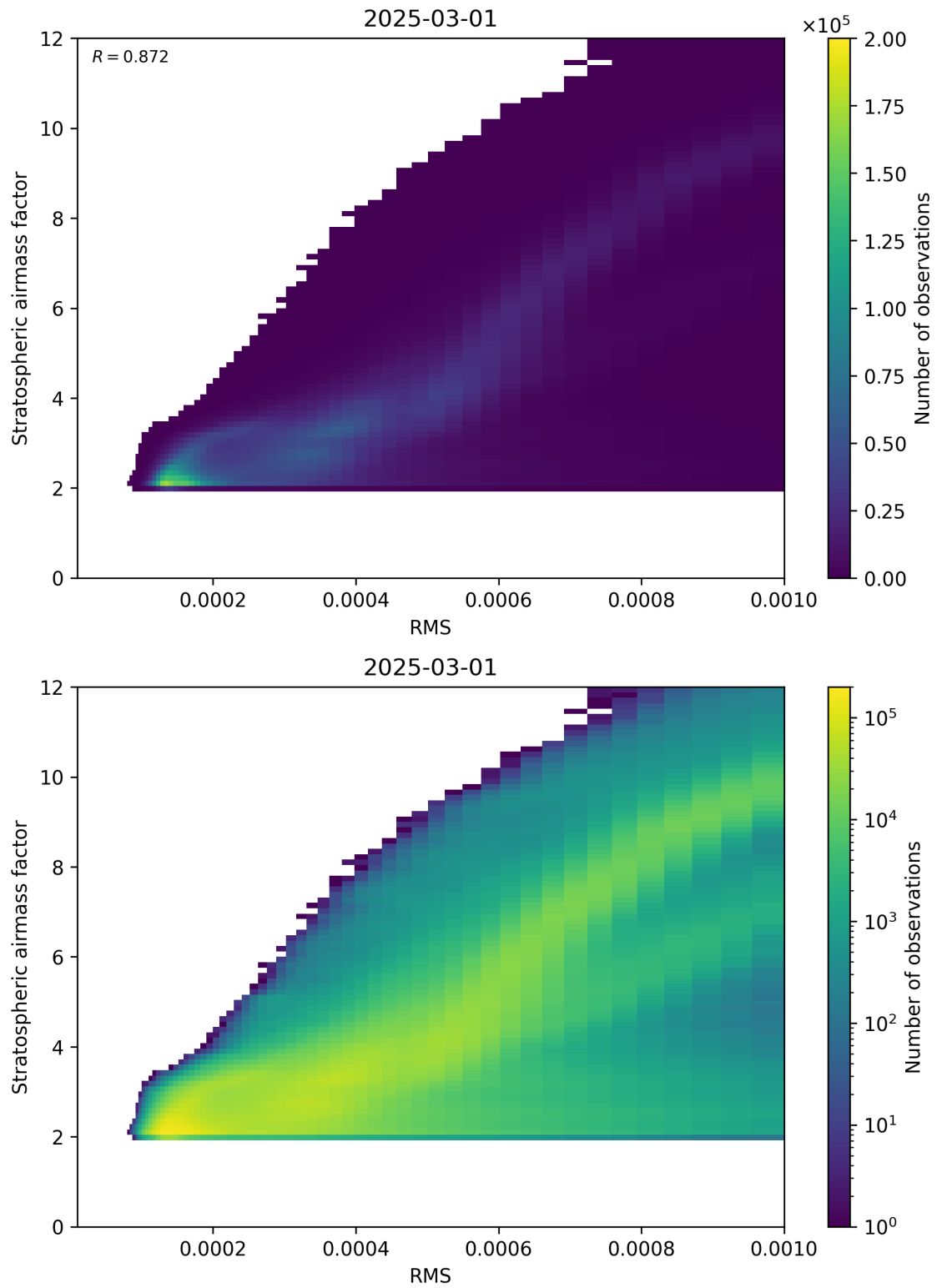
Figure 144: Scatter density plot of “RMS” against “Stratospheric airmass factor” for 2025-03-01 to 2025-03-02.
