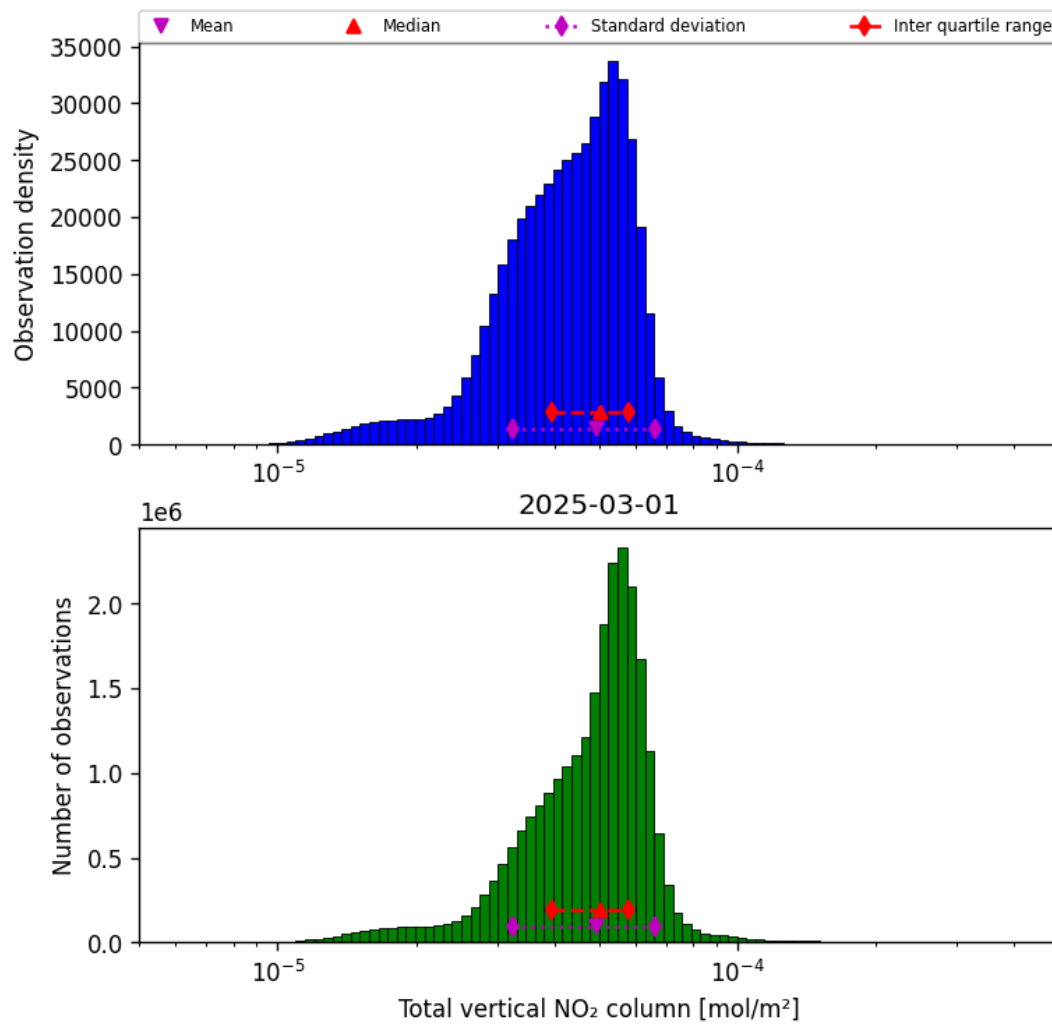
Figure 38: Histogram of “Total vertical NO 2 column” for 2025-03-01 to 2025-03-02
