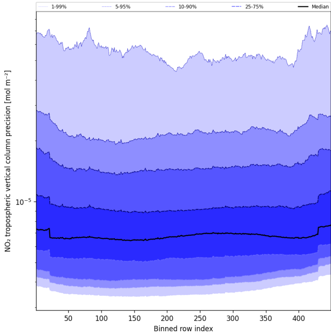
Figure 47: Along track statistics of “NO 2 tropospheric vertical column precision” for 2025-03-01 to 2025-03-02
