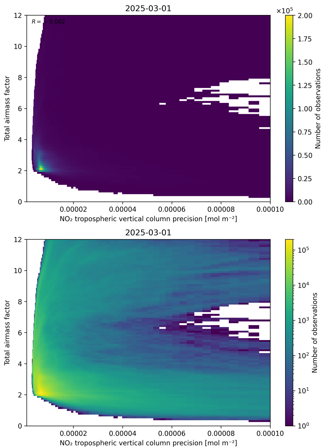
Figure 132: Scatter density plot of “NO 2 tropospheric vertical column precision” against “Total air mass factor” for 2025-03-01 to 2025-03-02.
