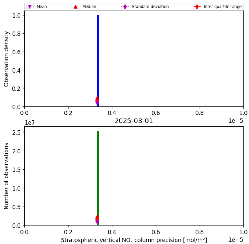
Figure 37: Histogram of "Stratospheric vertical NO 2 column precision" for 2025-03-01 to 2025-03-02
