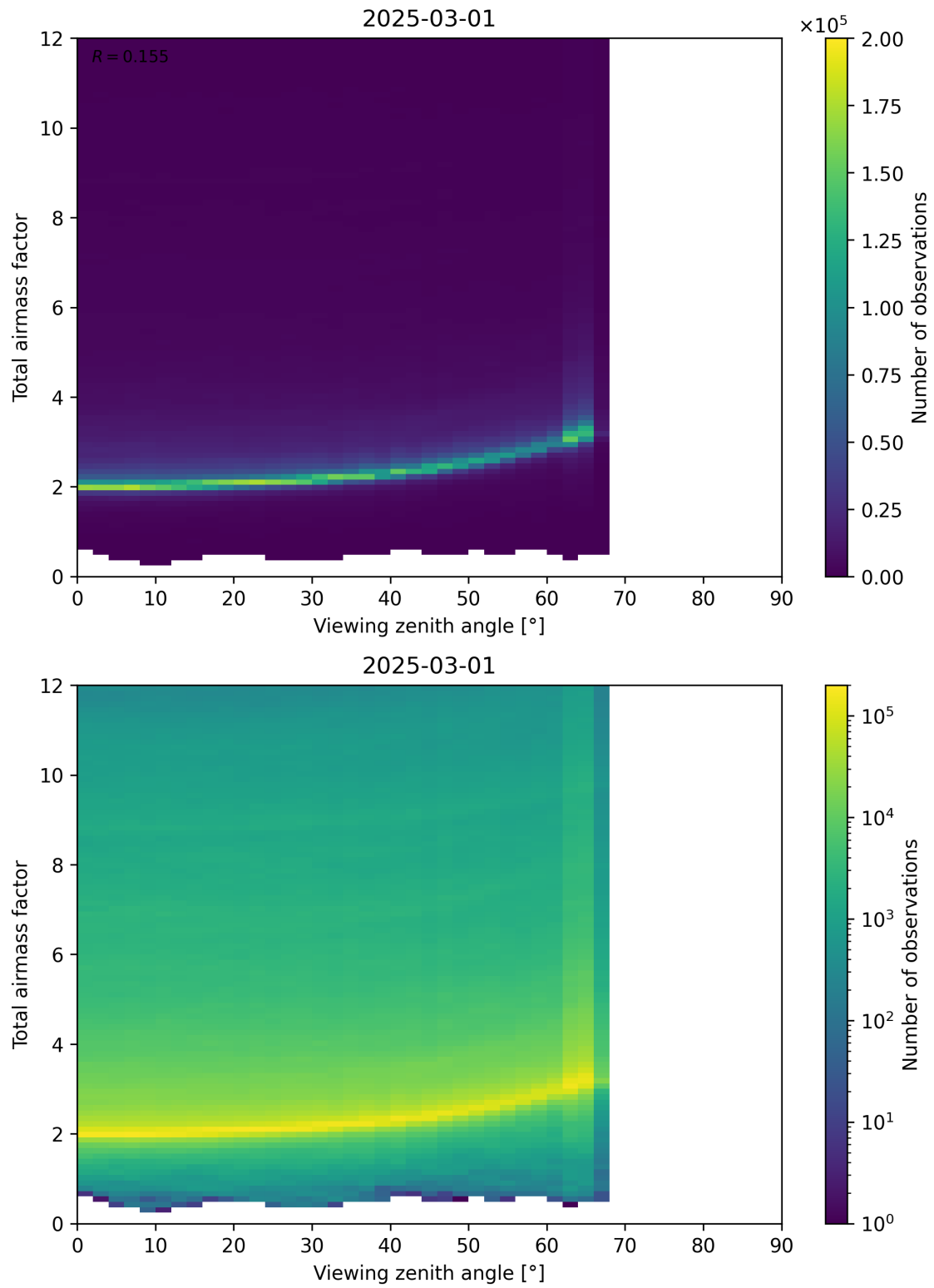
Figure 160: Scatter density plot of “Viewing zenith angle” against “Total airmass factor” for 2025-03-01 to 2025-03-02.
