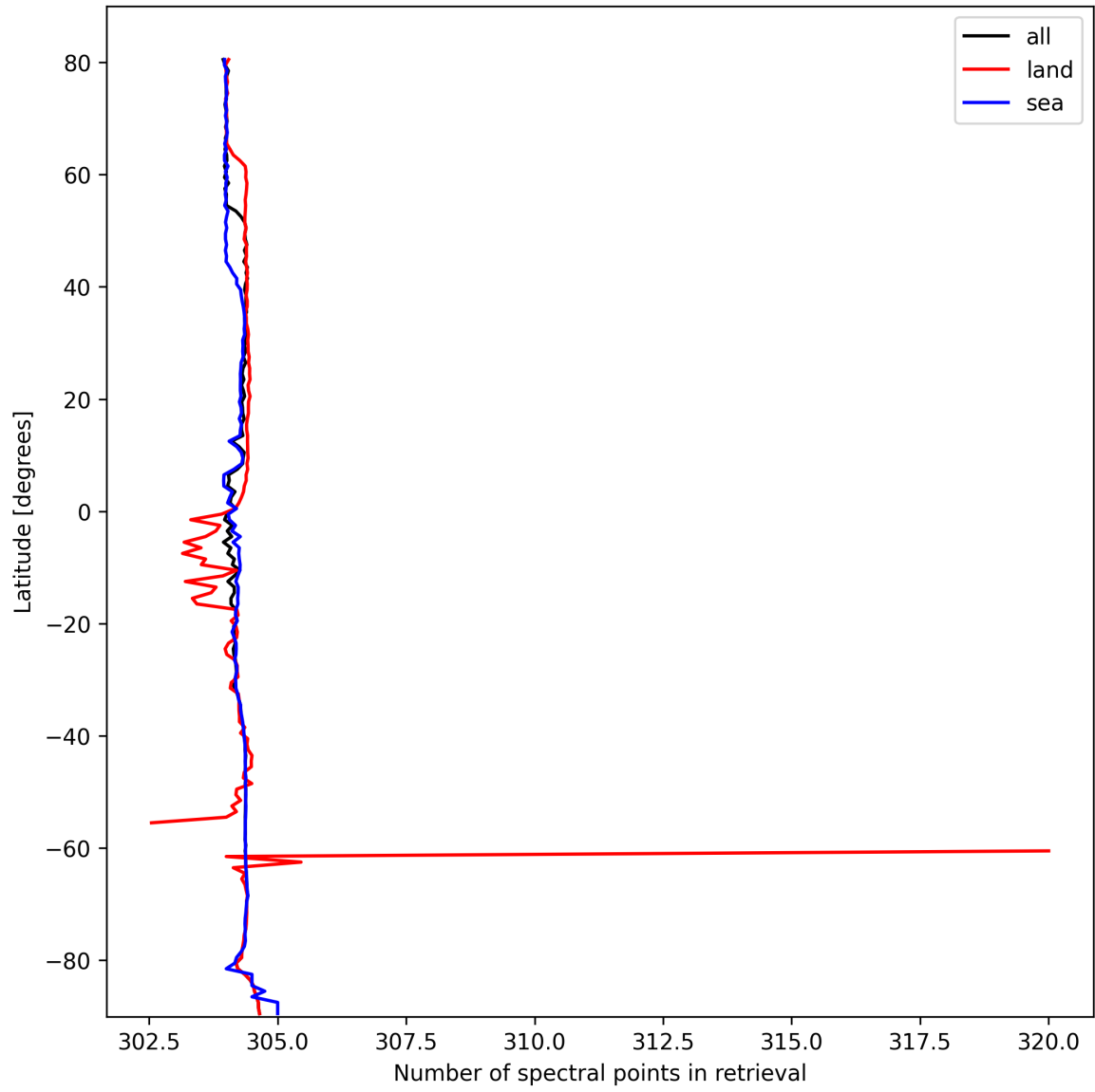
Figure 16: Zonal average of “Number of spectral points in retrieval” for 2025-03-01 to 2025-03-02.
