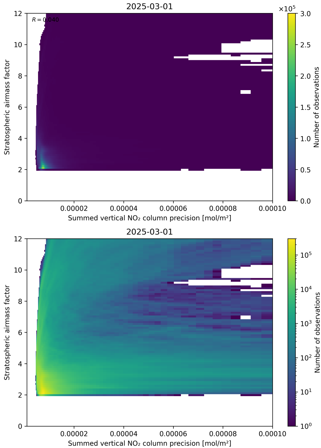
Figure 106: Scatter density plot of “Summed vertical NO 2 column precision” against “Stratospheric airmass factor” for 2025-03-01 to 2025-03-02.
