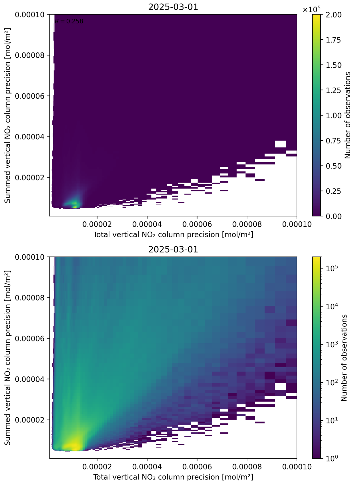
Figure 118: Scatter density plot of “Total vertical NO 2 column precision” against “Summed vertical NO 2 column precision” for 2025-03-01 to 2025-03-02.
