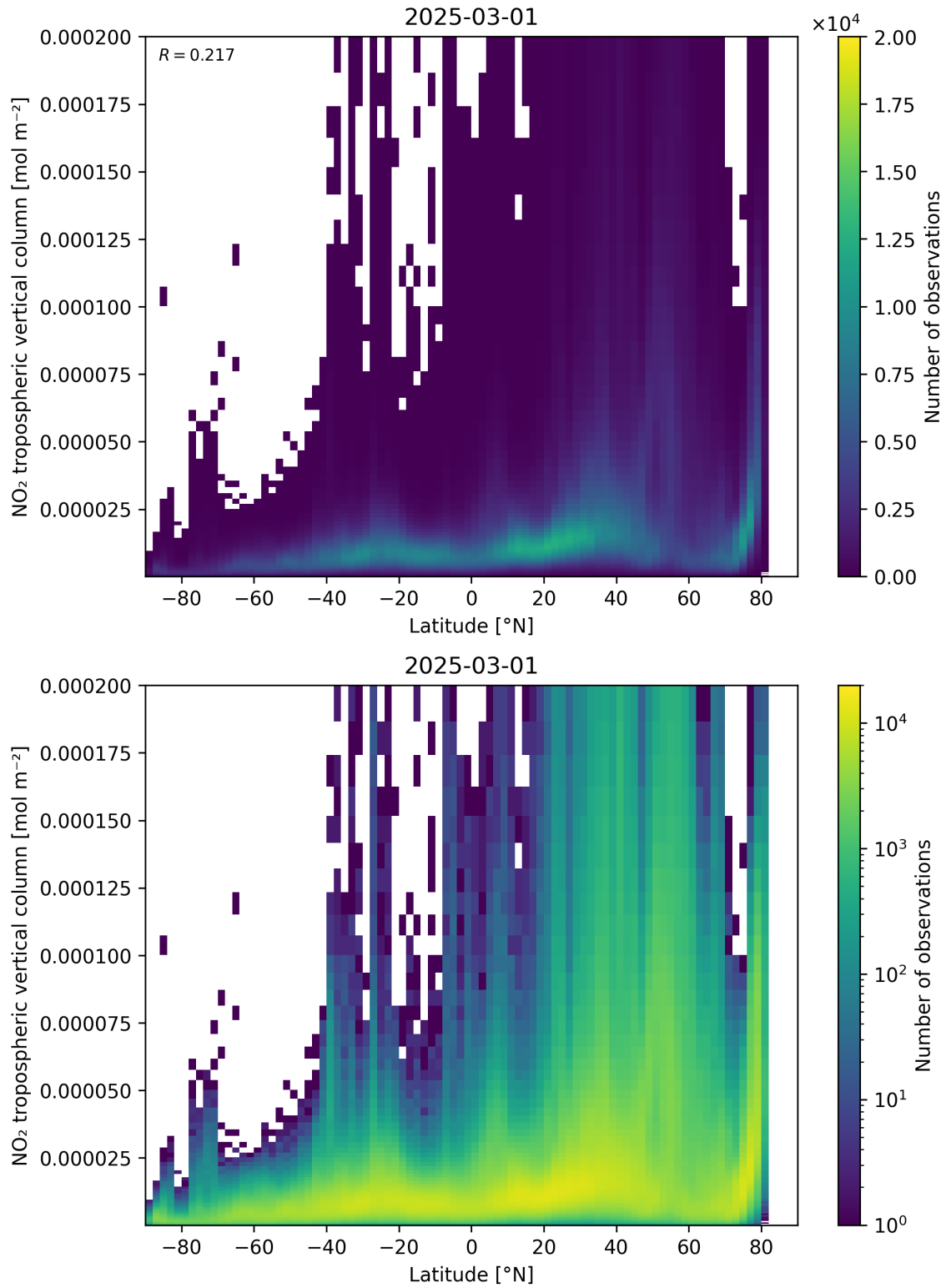
Figure 92: Scatter density plot of “Latitude” against “NO 2 tropospheric vertical column” for 2025-03-01 to 2025-03-02.
