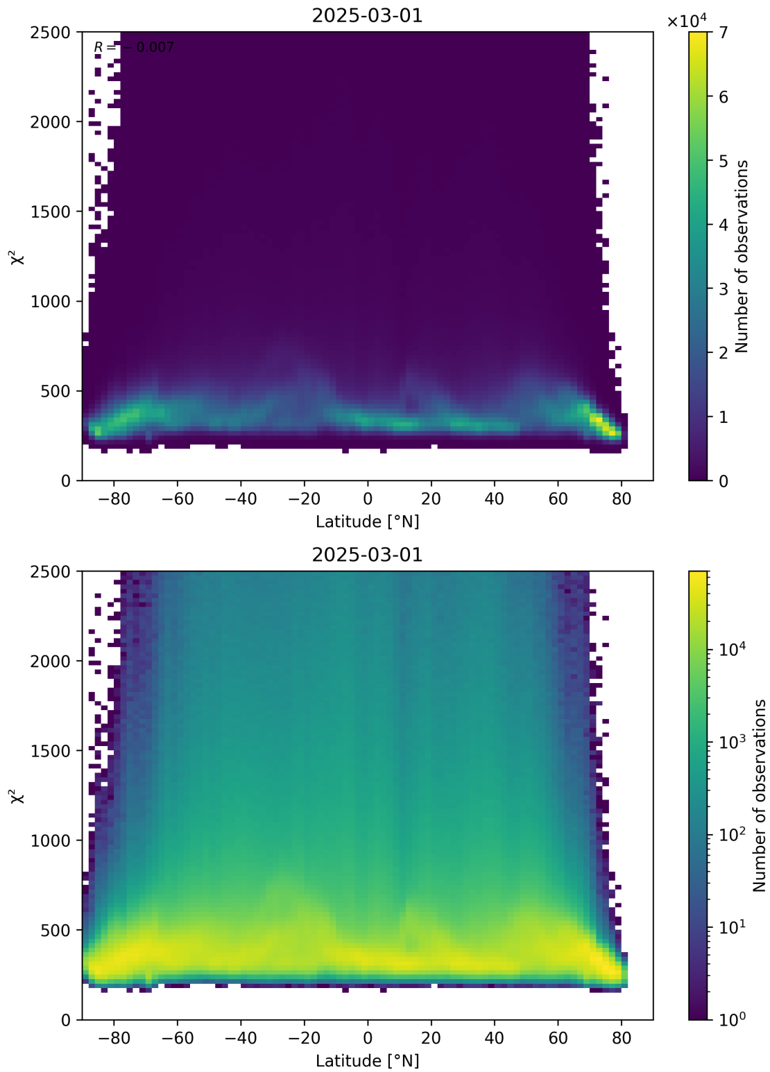
Figure 86: Scatter density plot of “Latitude” against “ \chi^2 ” for 2025-03-01 to 2025-03-02.
