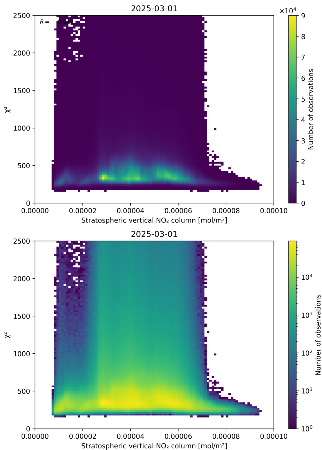
Figure 97: Scatter density plot of “Stratospheric vertical NO 2 column” against “ \chi^2 ” for 2025-03-01 to 2025-03-02.
