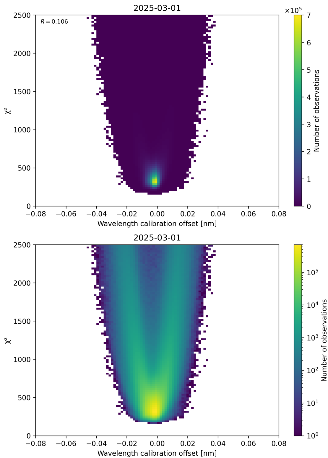
Figure 175: Scatter density plot of “Wavelength calibration offset” against “ \chi^2 ” for 2025-03-01 to 2025-03-02.
