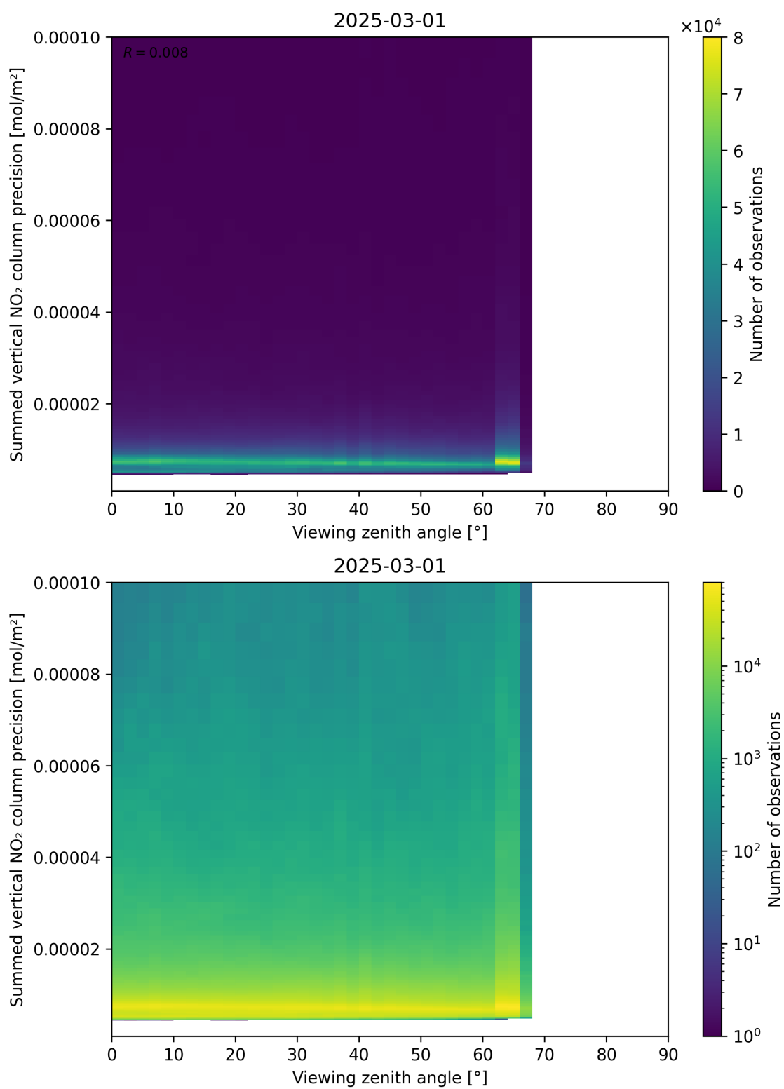
Figure 166: Scatter density plot of “Viewing zenith angle” against “Summed vertical NO 2 column precision” for 2025-03-01 to 2025-03-02.
