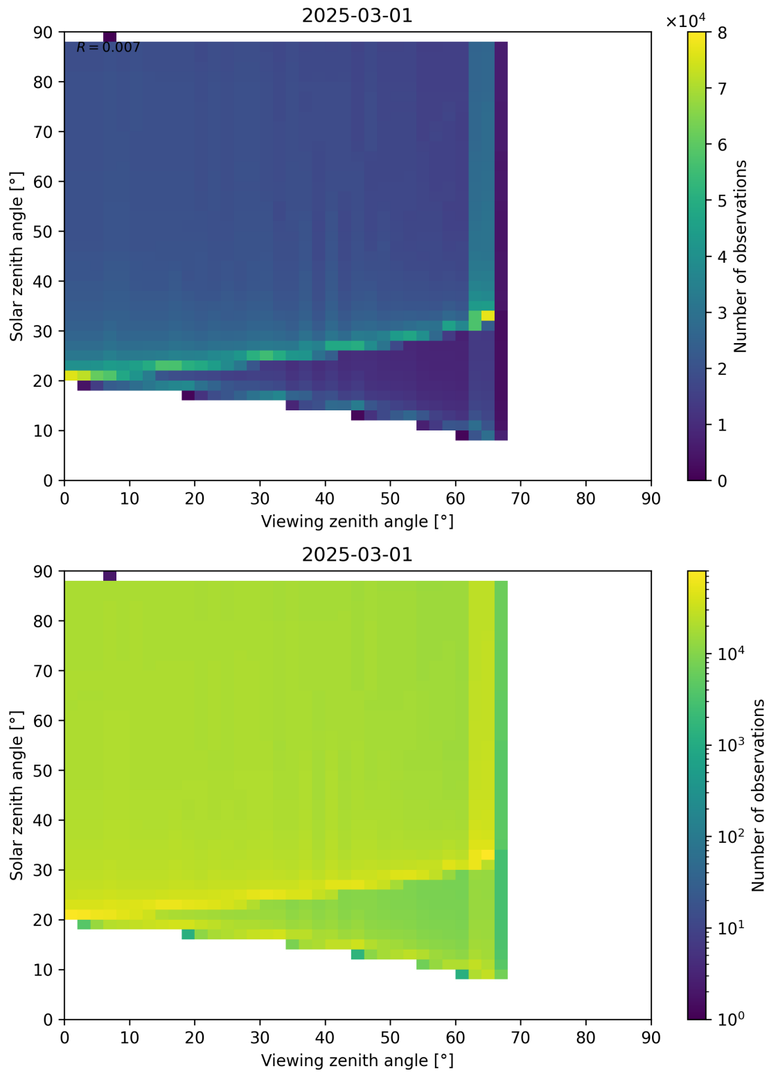
Figure 172: Scatter density plot of “Viewing zenith angle” against “Solar zenith angle” for 2025-03-01 to 2025-03-02.
