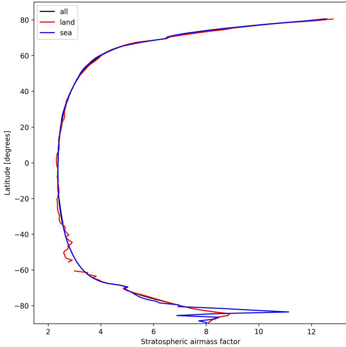
Figure 27: Zonal average of “Stratospheric airmass factor” for 2025-03-01 to 2025-03-02.
