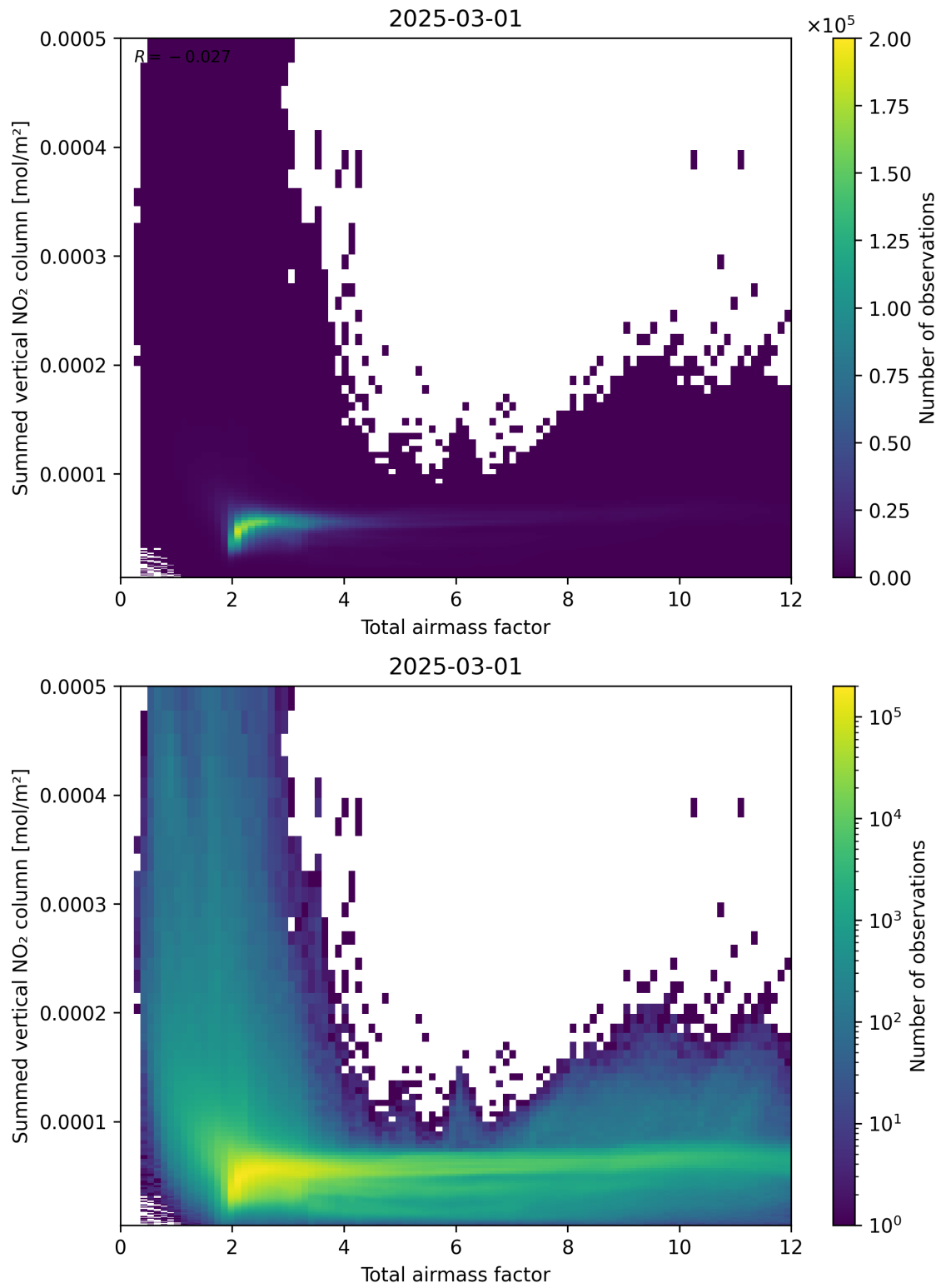
Figure 65: Scatter density plot of “Total airmass factor” against “Summed vertical NO 2 column” for 2025-03-01 to 2025-03-02.
