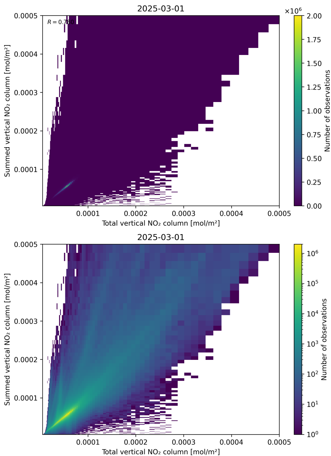
Figure 112: Scatter density plot of “Total vertical NO 2 column” against “Summed vertical NO 2 column” for 2025-03-01 to 2025-03-02.
