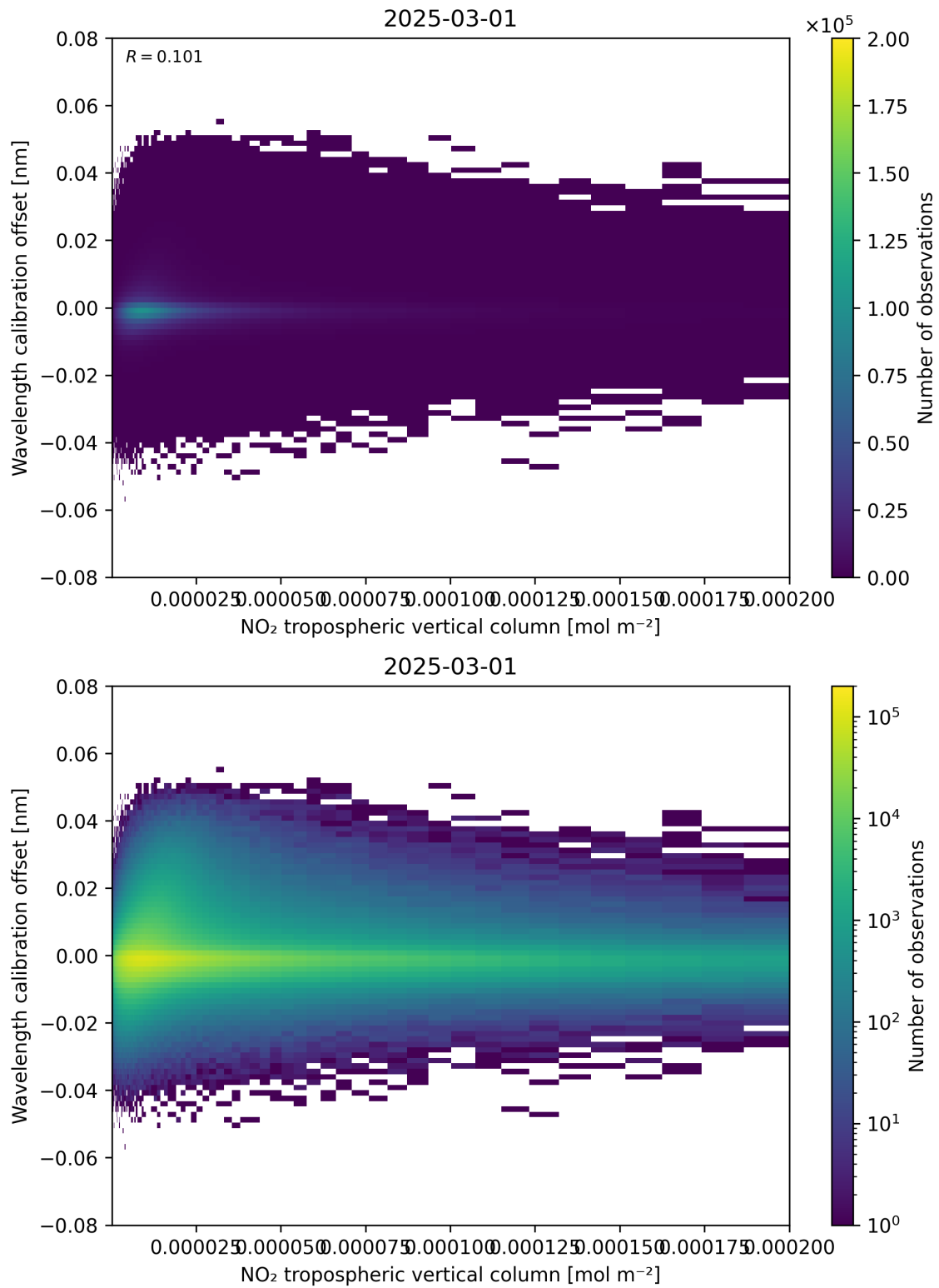
Figure 143: Scatter density plot of “NO 2 tropospheric vertical column” against “Wavelength calibration offset” for 2025-03-01 to 2025-03-02.
