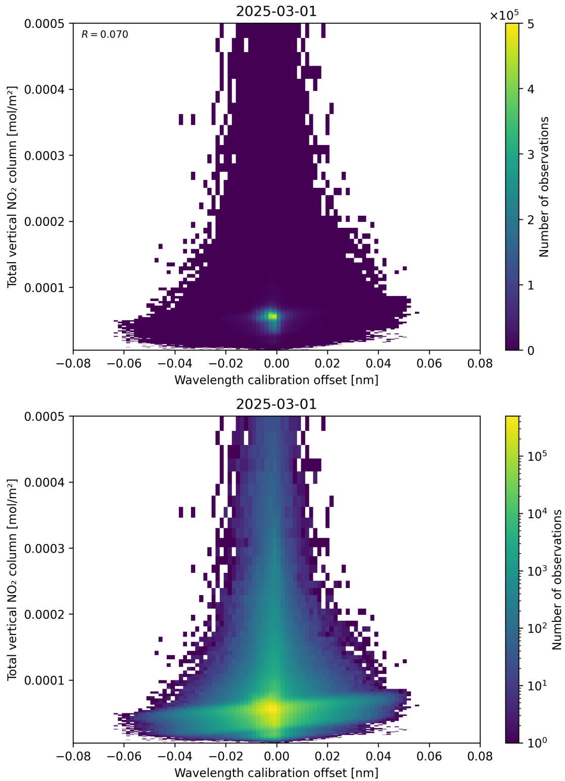
Figure 179: Scatter density plot of “Wavelength calibration offset” against “Total vertical NO 2 column” for 2025-03-01 to 2025-03-02.
