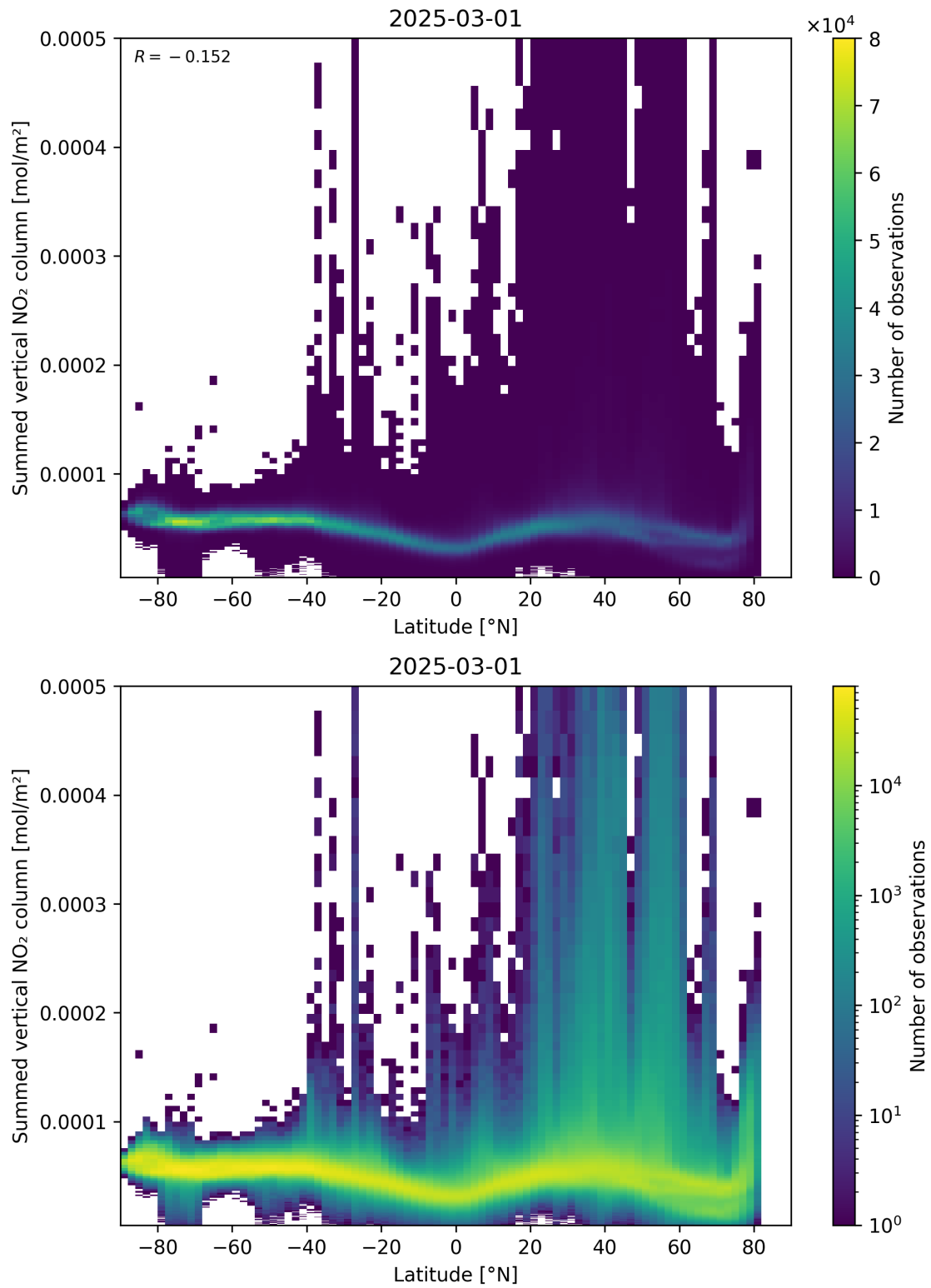
Figure 88: Scatter density plot of “Latitude” against “Summed vertical NO 2 column” for 2025-03-01 to 2025-03-02.
