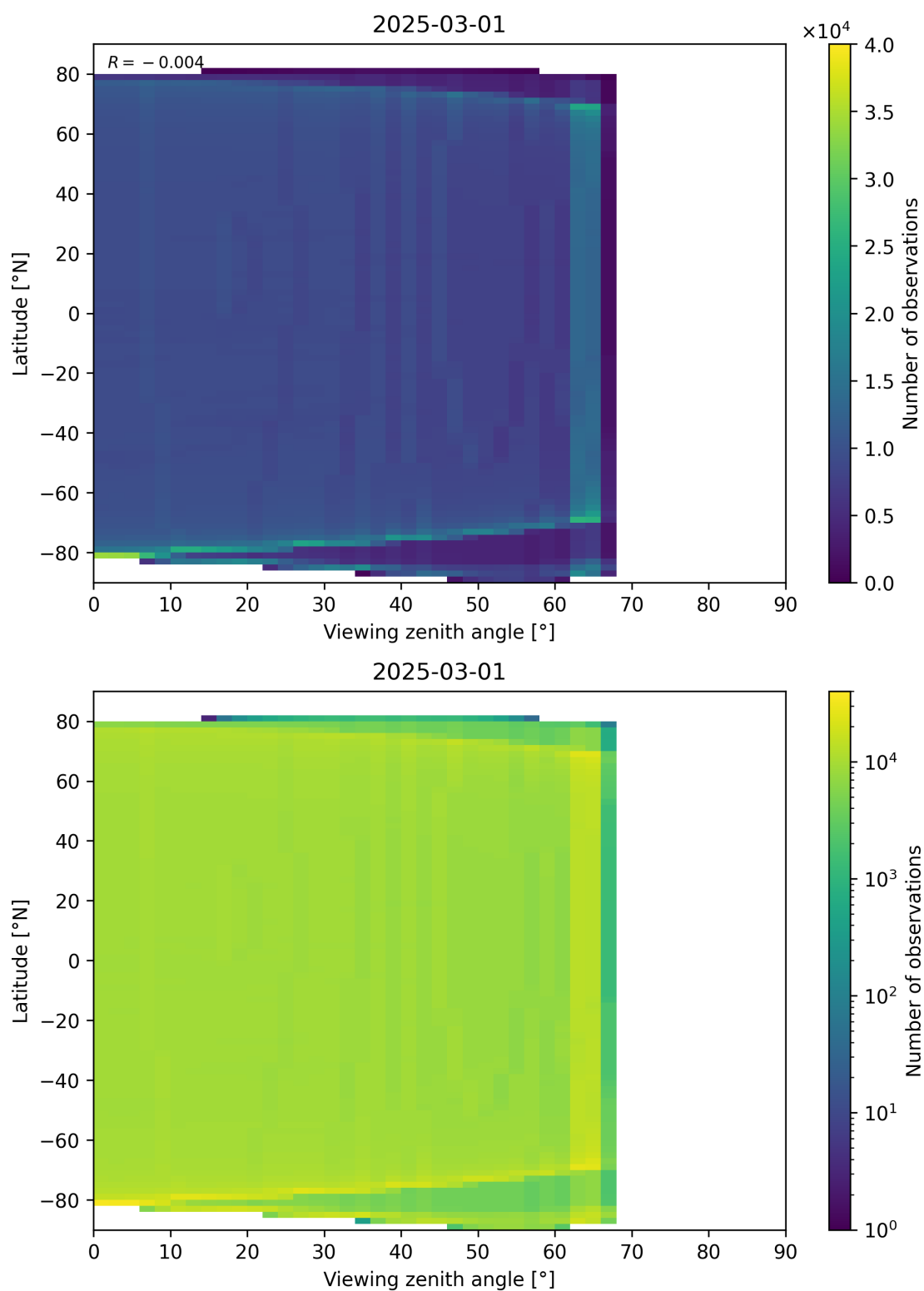
Figure 163: Scatter density plot of “Viewing zenith angle” against “Latitude” for 2025-03-01 to 2025-03-02.
