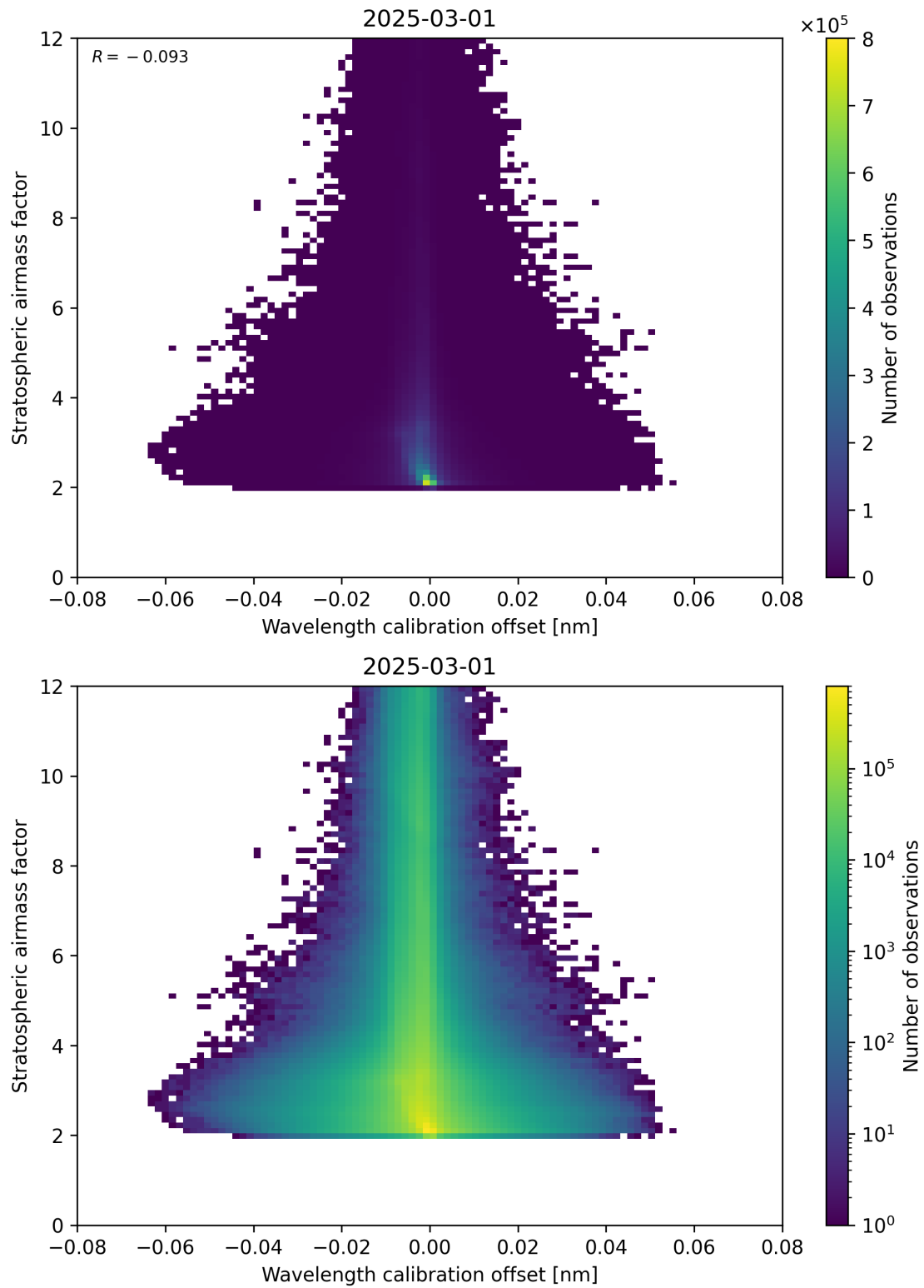
Figure 174: Scatter density plot of “Wavelength calibration offset” against “Stratospheric airmass factor” for 2025-03-01 to 2025-03-02.
