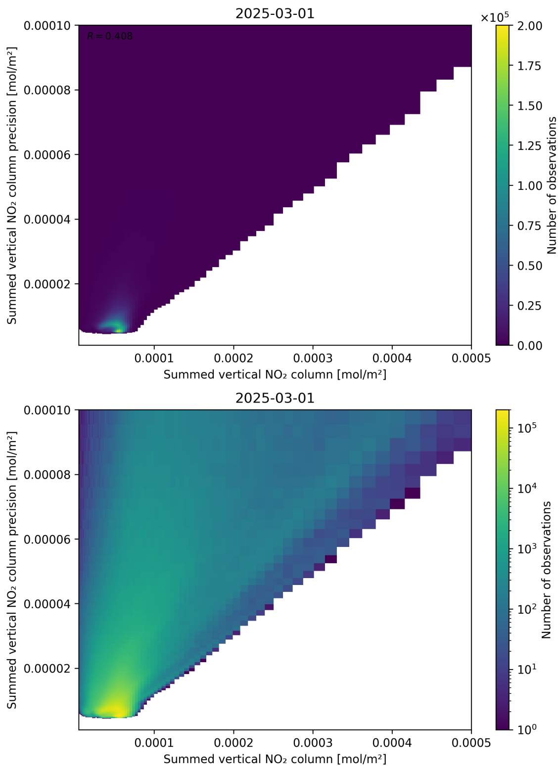
Figure 105: Scatter density plot of “Summed vertical NO 2 column” against “Summed vertical NO 2 column precision” for 2025-03-01 to 2025-03-02.
