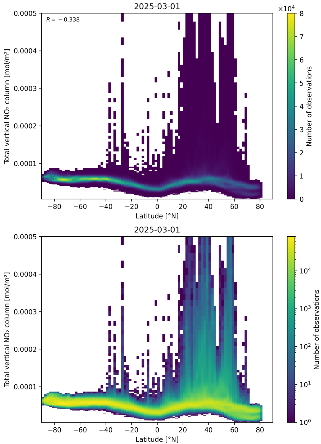
Figure 90: Scatter density plot of “Latitude” against “Total vertical NO 2 column” for 2025-03-01 to 2025-03-02.
