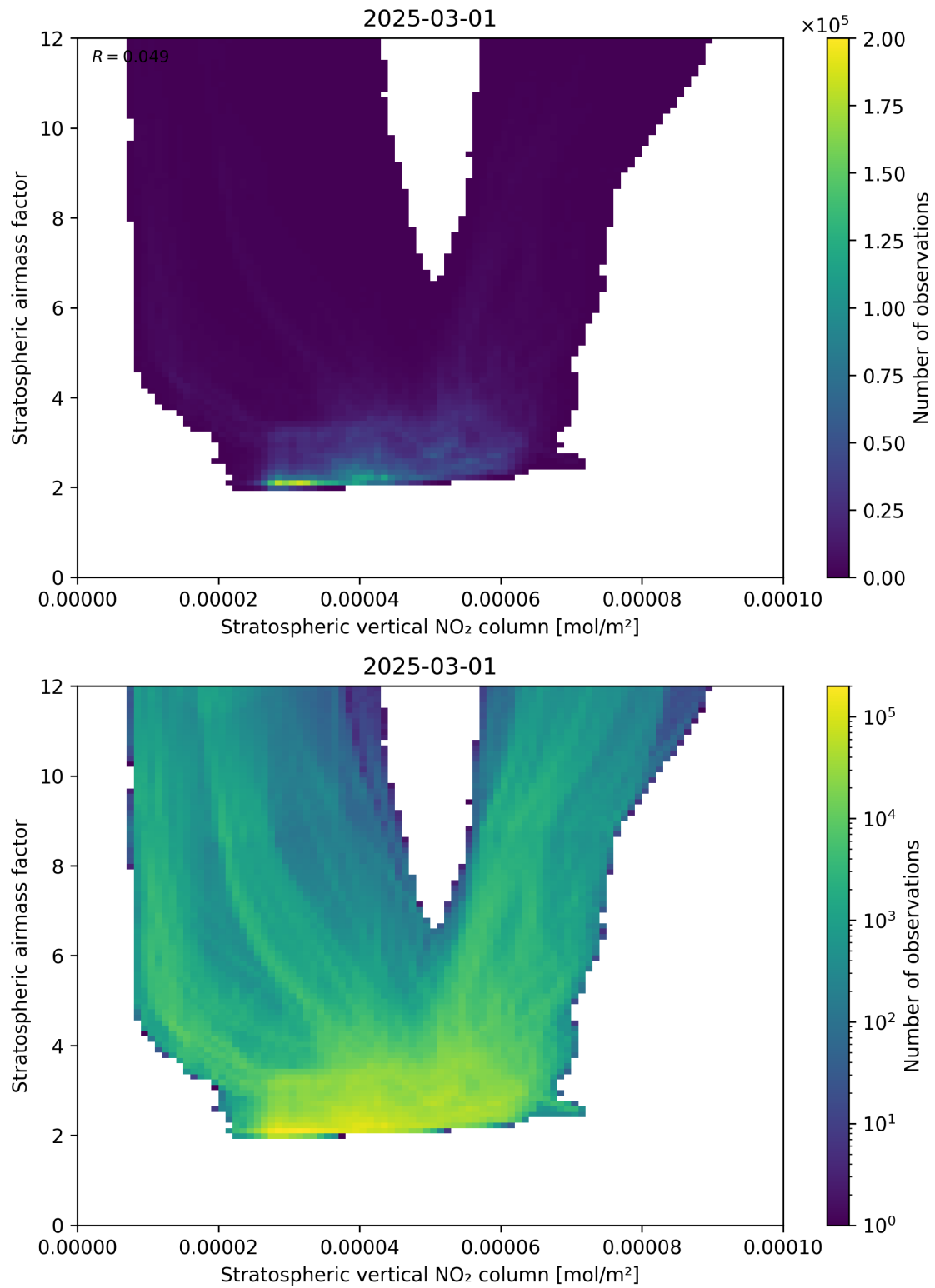
Figure 96: Scatter density plot of “Stratospheric vertical NO 2 column” against “Stratospheric airmass factor” for 2025-03-01 to 2025-03-02.
