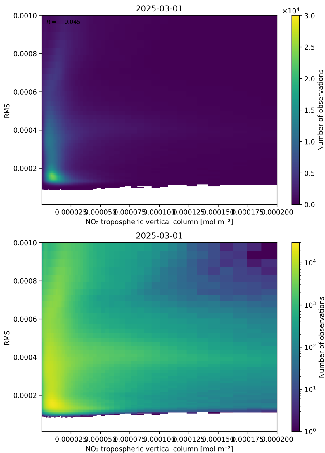
Figure 142: Scatter density plot of “NO 2 tropospheric vertical column” against “RMS” for 2025-03-01 to 2025-03-02.
