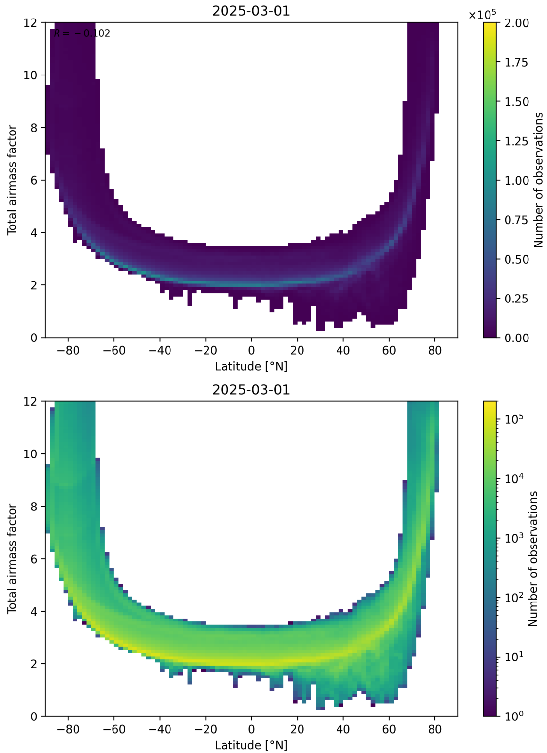
Figure 84: Scatter density plot of “Latitude” against “Total airmass factor” for 2025-03-01 to 2025-03-02.
