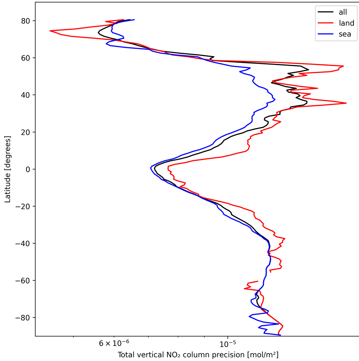
Figure 22: Zonal average of “Total vertical NO 2 column precision” for 2025-03-01 to 2025-03-02.
