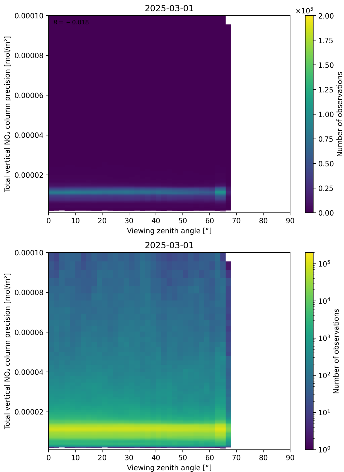
Figure 168: Scatter density plot of “Viewing zenith angle” against “Total vertical NO 2 column precision” for 2025-03-01 to 2025-03-02.
