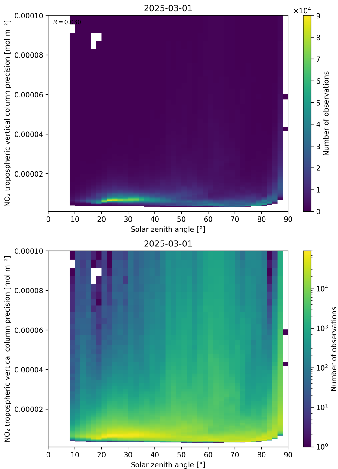
Figure 156: Scatter density plot of “Solar zenith angle” against “NO 2 tropospheric vertical column precision” for 2025-03-01 to 2025-03-02.
