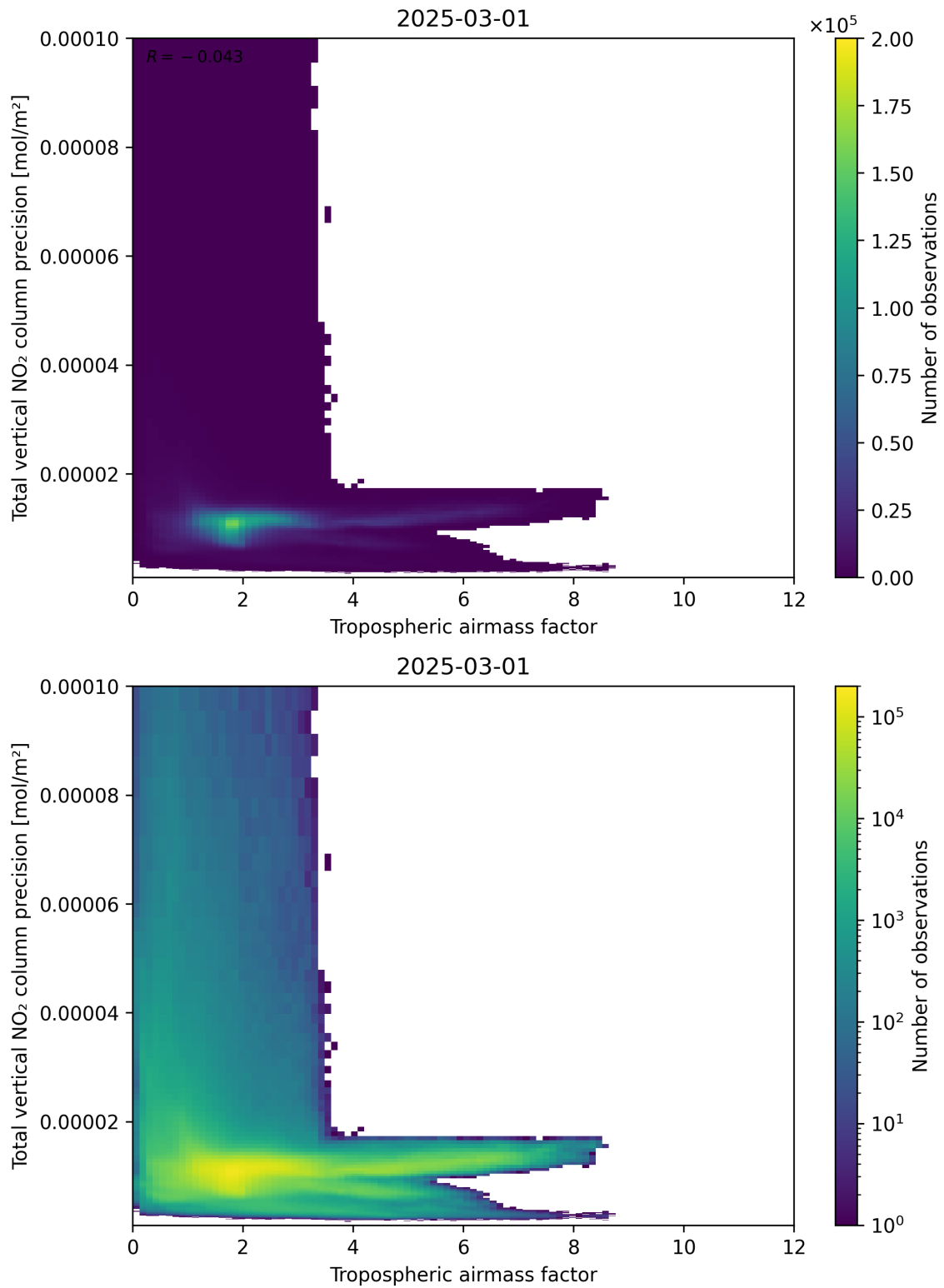
Figure 78: Scatter density plot of “Tropospheric airmass factor” against “Total vertical NO 2 column precision” for 2025-03-01 to 2025-03-02.
