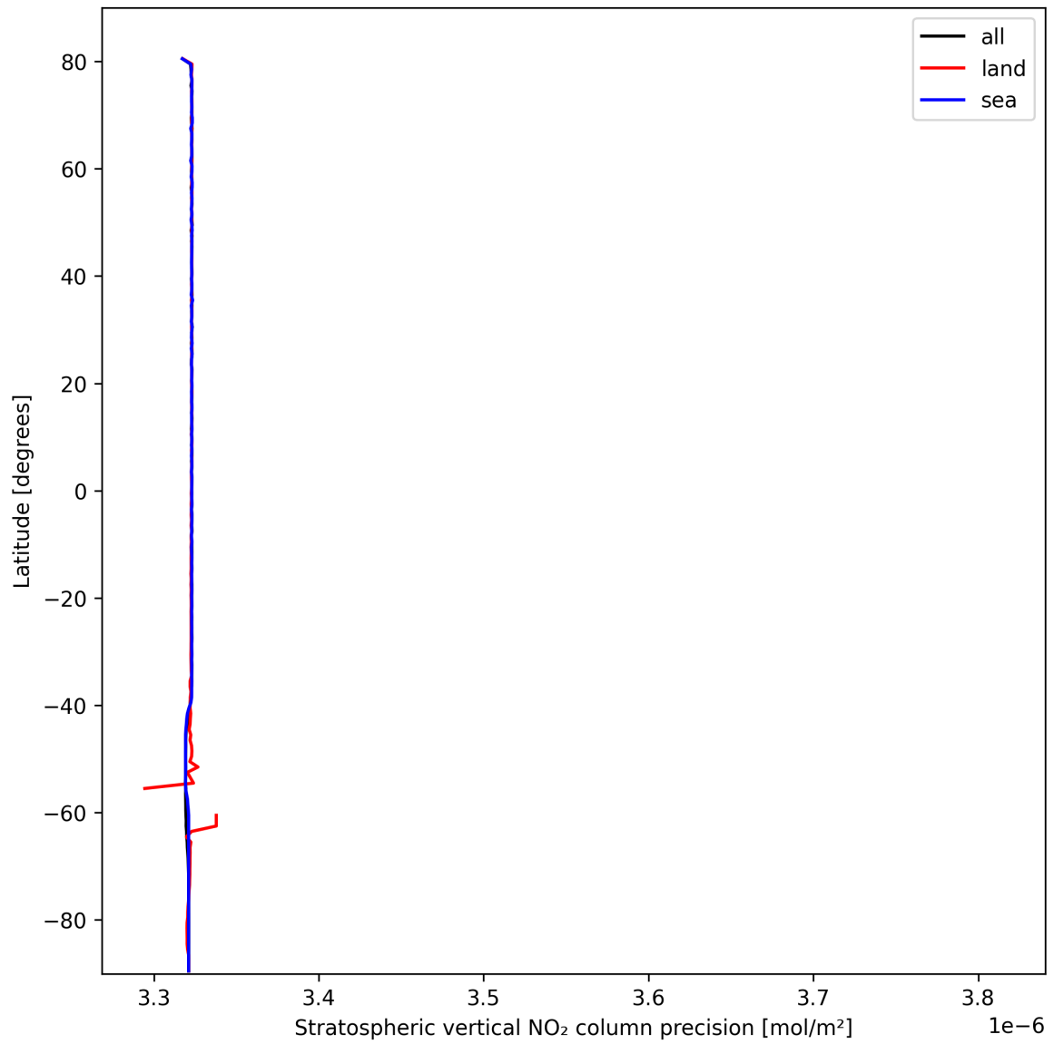
Figure 20: Zonal average of “Stratospheric vertical NO 2 column precision” for 2025-03-01 to 2025-03-02.
