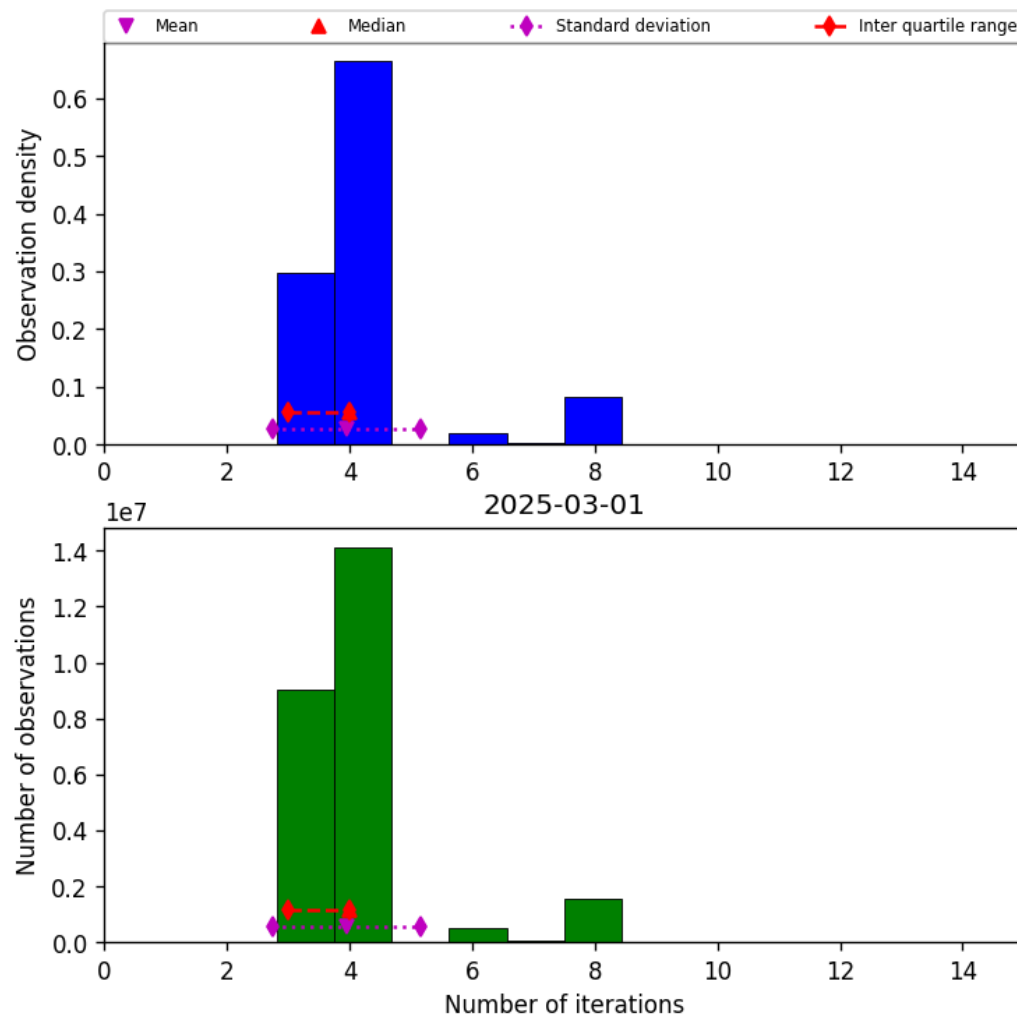
Figure 34: Histogram of “Number of iterations” for 2025-03-01 to 2025-03-02
