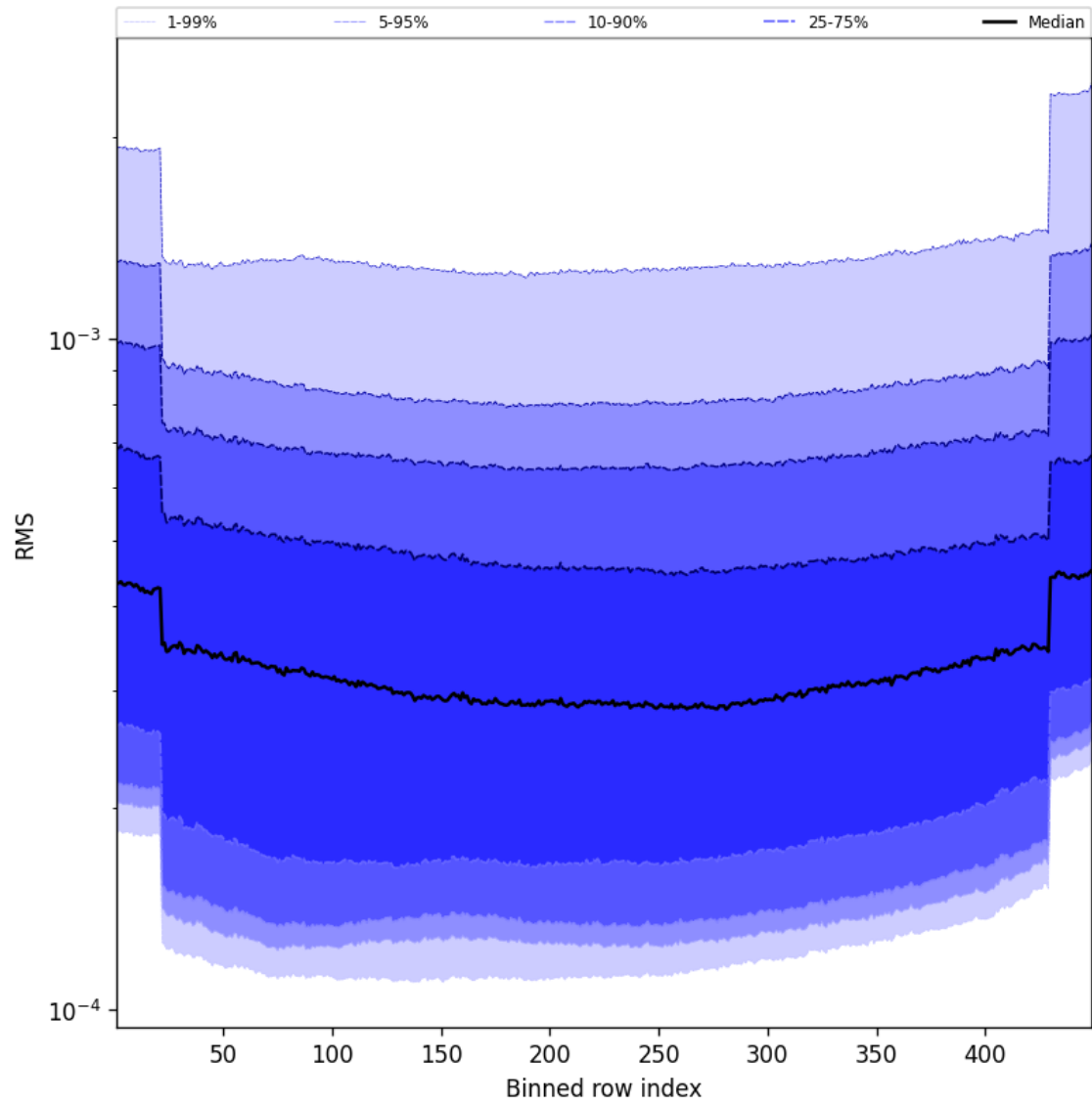
Figure 60: Along track statistics of “RMS” for 2025-03-01 to 2025-03-02
