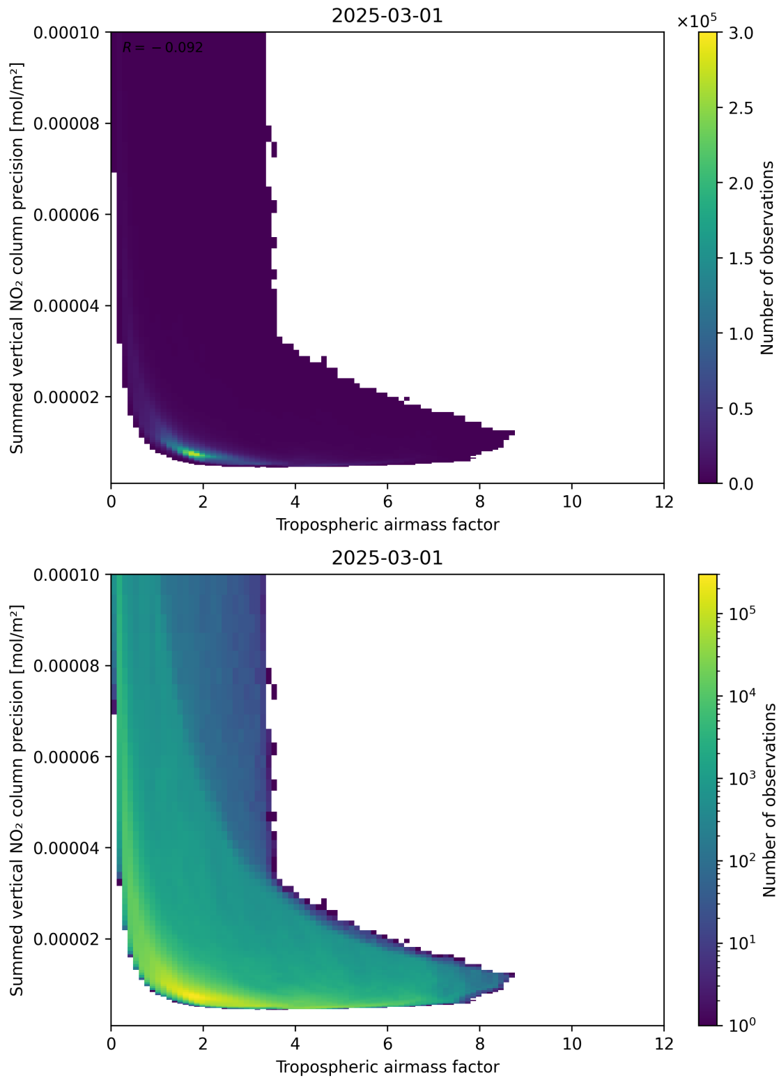
Figure 76: Scatter density plot of “Tropospheric air mass factor” against “Summed vertical NO 2 column precision” for 2025-03-01 to 2025-03-02.
