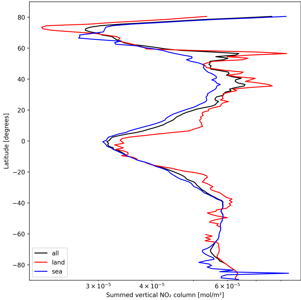
Figure 23: Zonal average of “Summed vertical NO 2 column” for 2025-03-01 to 2025-03-02.
