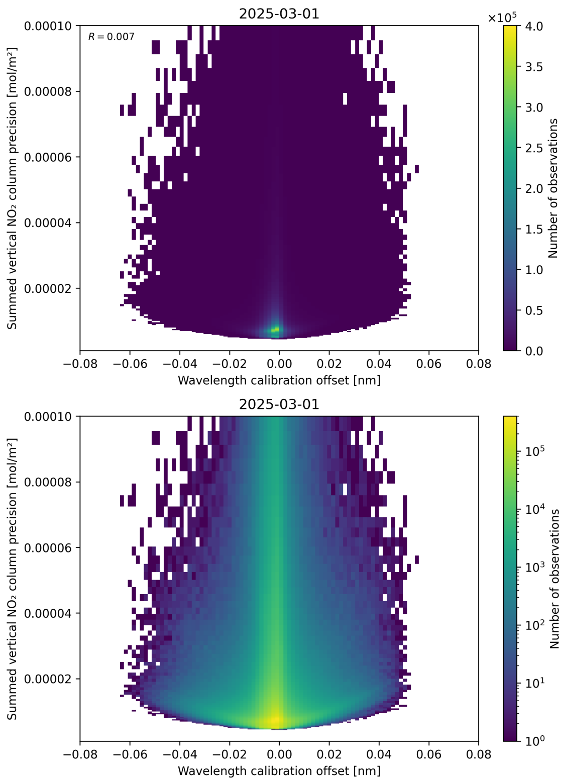
Figure 178: Scatter density plot of “Wavelength calibration offset” against “Summed vertical NO 2 column precision” for 2025-03-01 to 2025-03-02.
