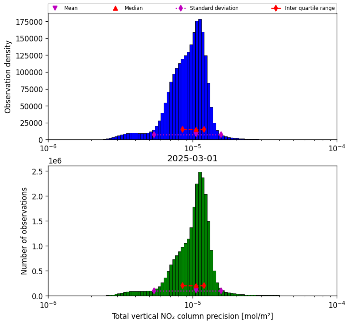
Figure 39: Histogram of “Total vertical NO 2 column precision” for 2025-03-01 to 2025-03-02
