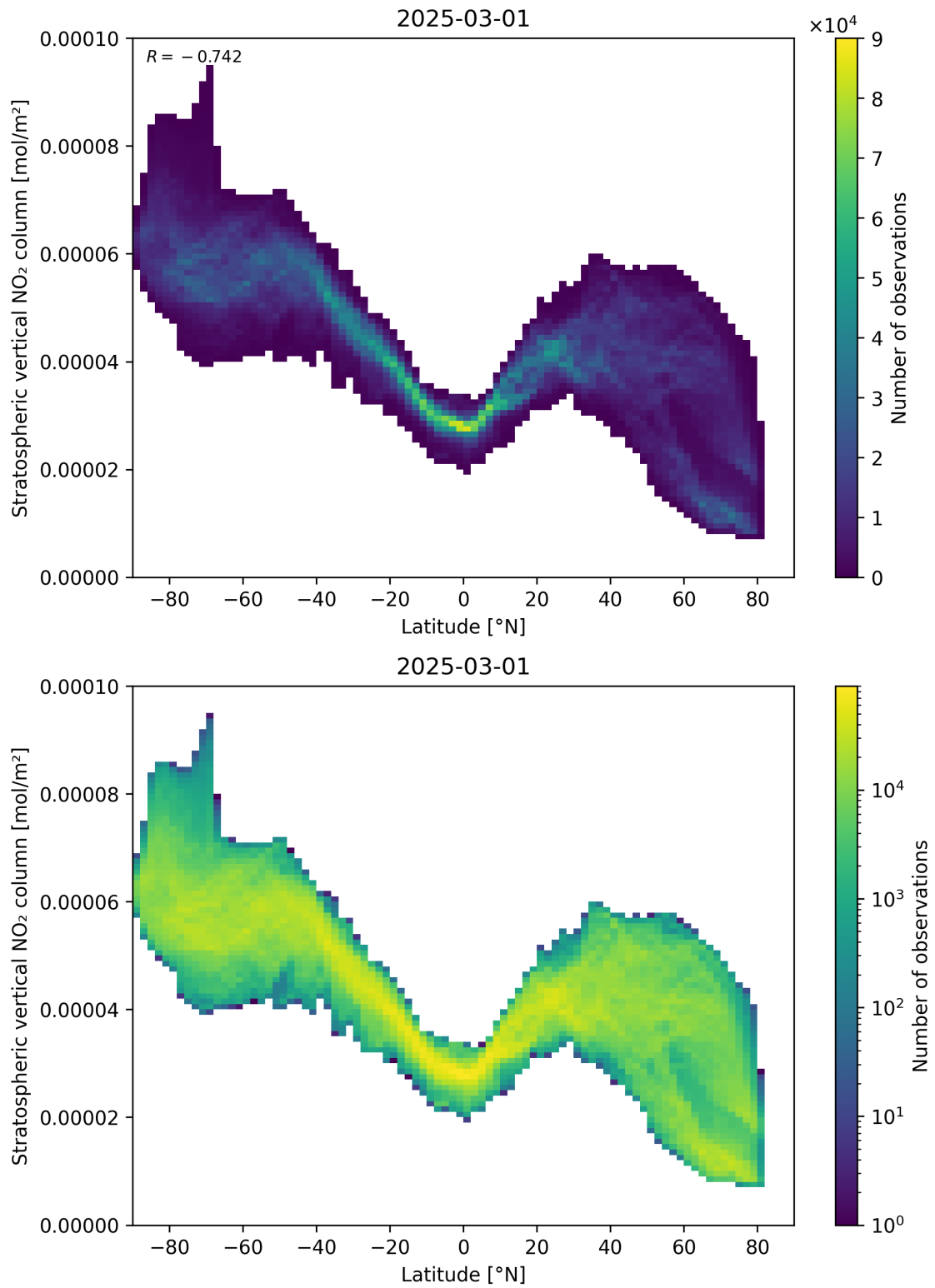
Figure 87: Scatter density plot of “Latitude” against “Stratospheric vertical NO 2 column” for 2025-03-01 to 2025-03-02.
