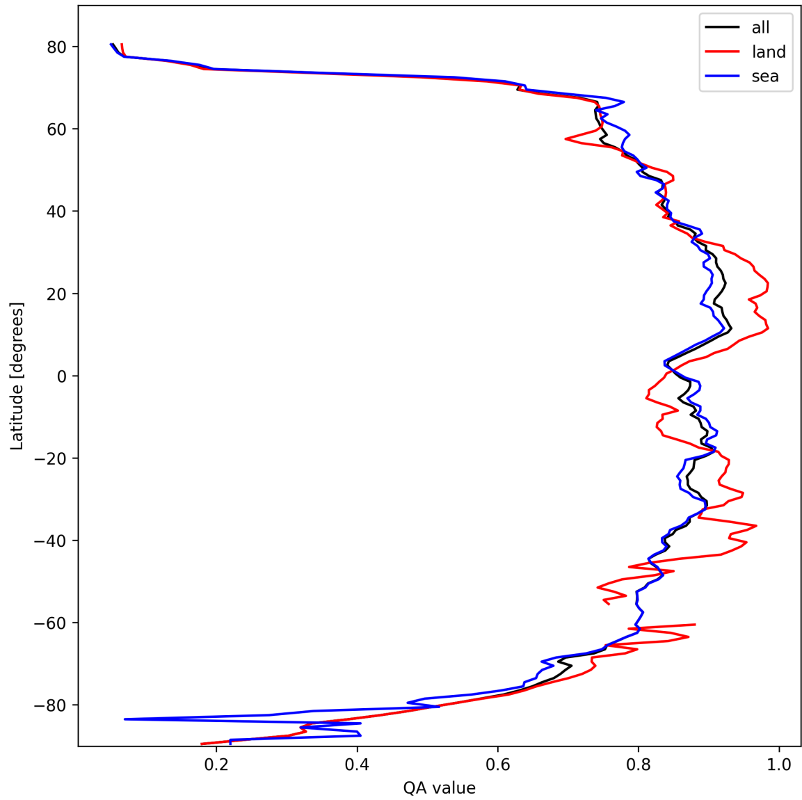
Figure 11: Zonal average of “QA value” for 2025-03-01 to 2025-03-02.
