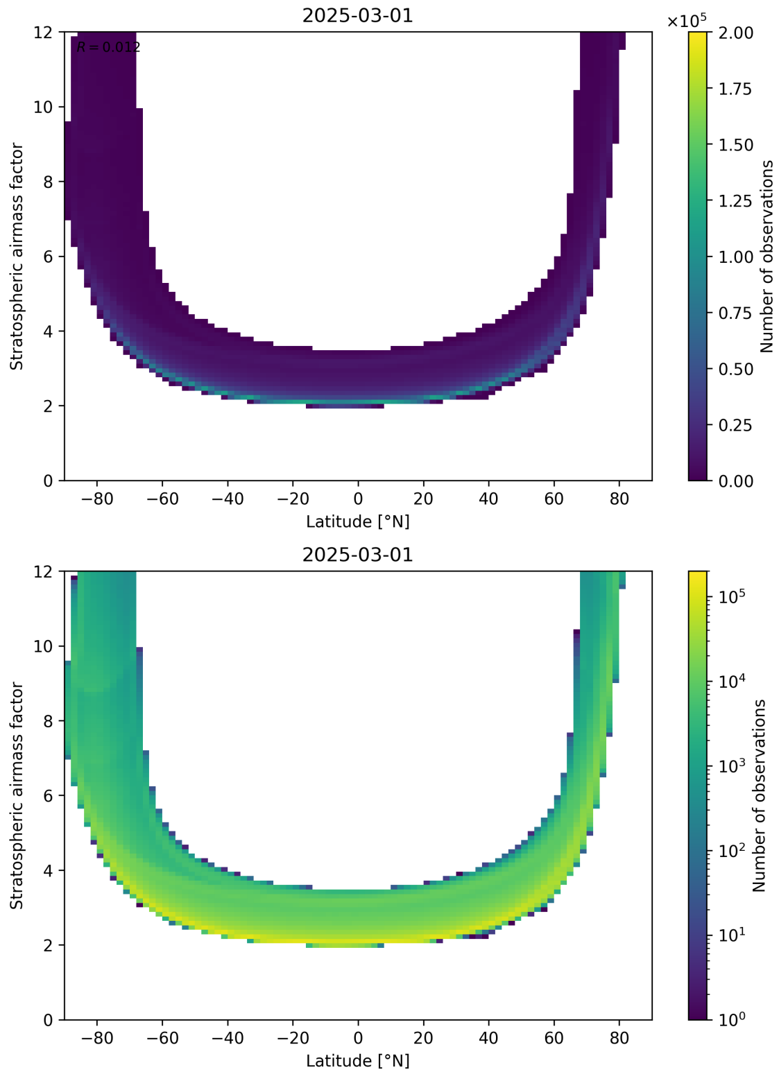
Figure 83: Scatter density plot of “Latitude” against “Stratospheric airmass factor” for 2025-03-01 to 2025-03-02.
