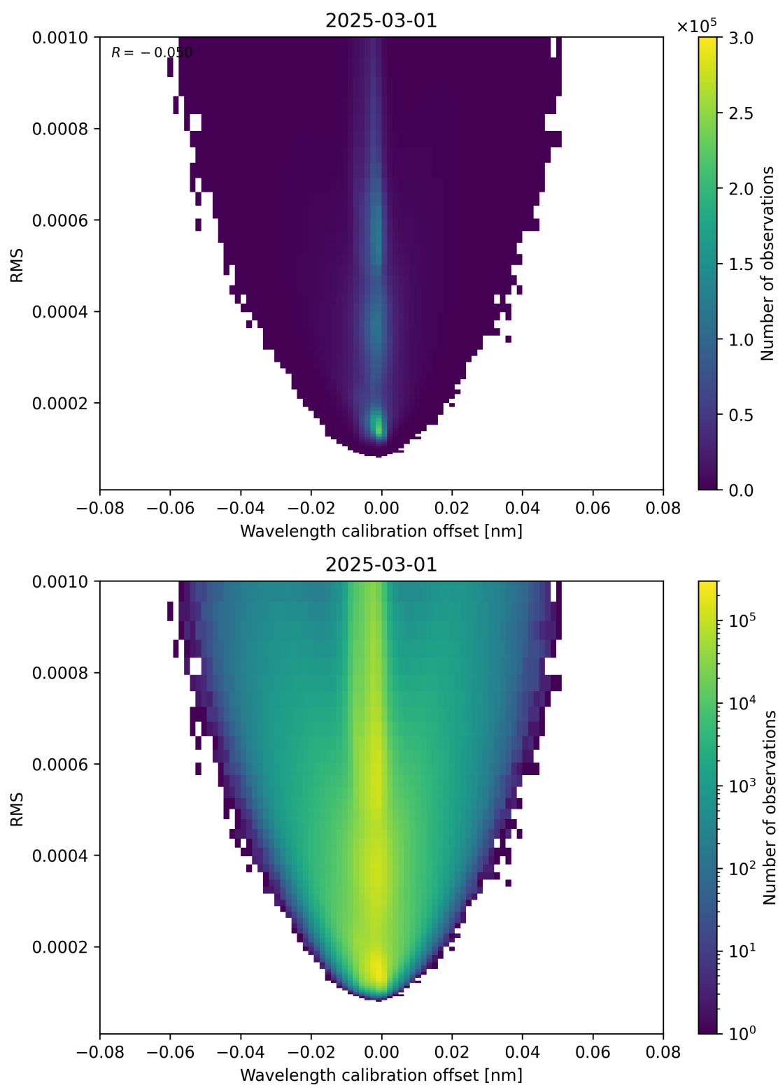
Figure 181: Scatter density plot of “Wavelength calibration offset” against “RMS” for 2025-03-01 to 2025-03-02.
