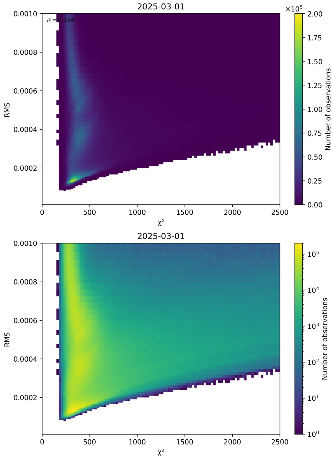
Figure 82: Scatter density plot of “ \chi^2 ” against “RMS” for 2025-03-01 to 2025-03-02.
