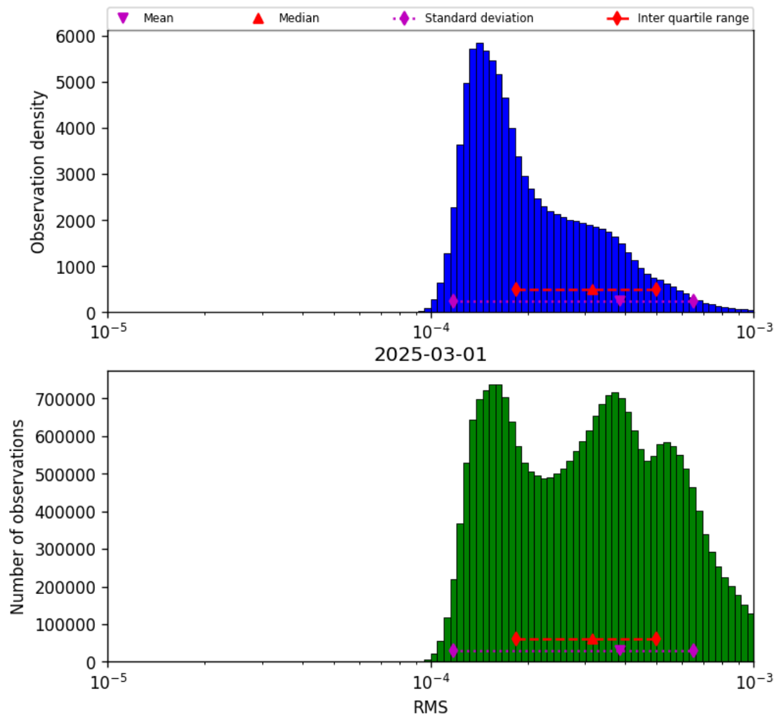
Figure 43: Histogram of “RMS” for 2025-03-01 to 2025-03-02
