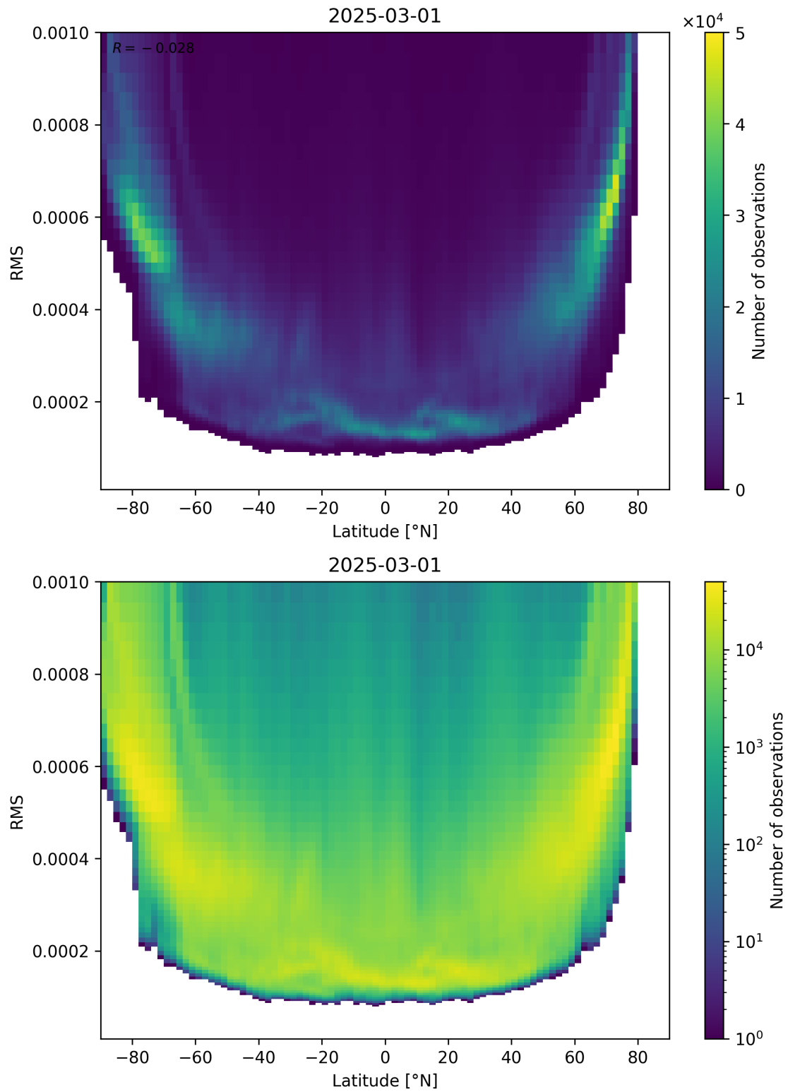
Figure 94: Scatter density plot of “Latitude” against “RMS” for 2025-03-01 to 2025-03-02.
