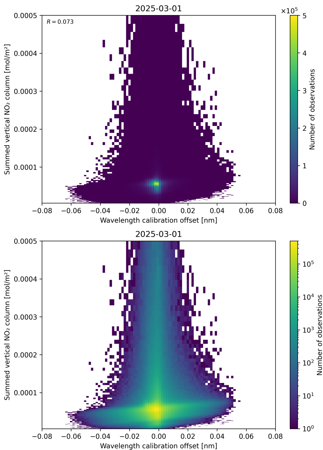
Figure 177: Scatter density plot of “Wavelength calibration offset” against “Summed vertical NO 2 column” for 2025-03-01 to 2025-03-02.
