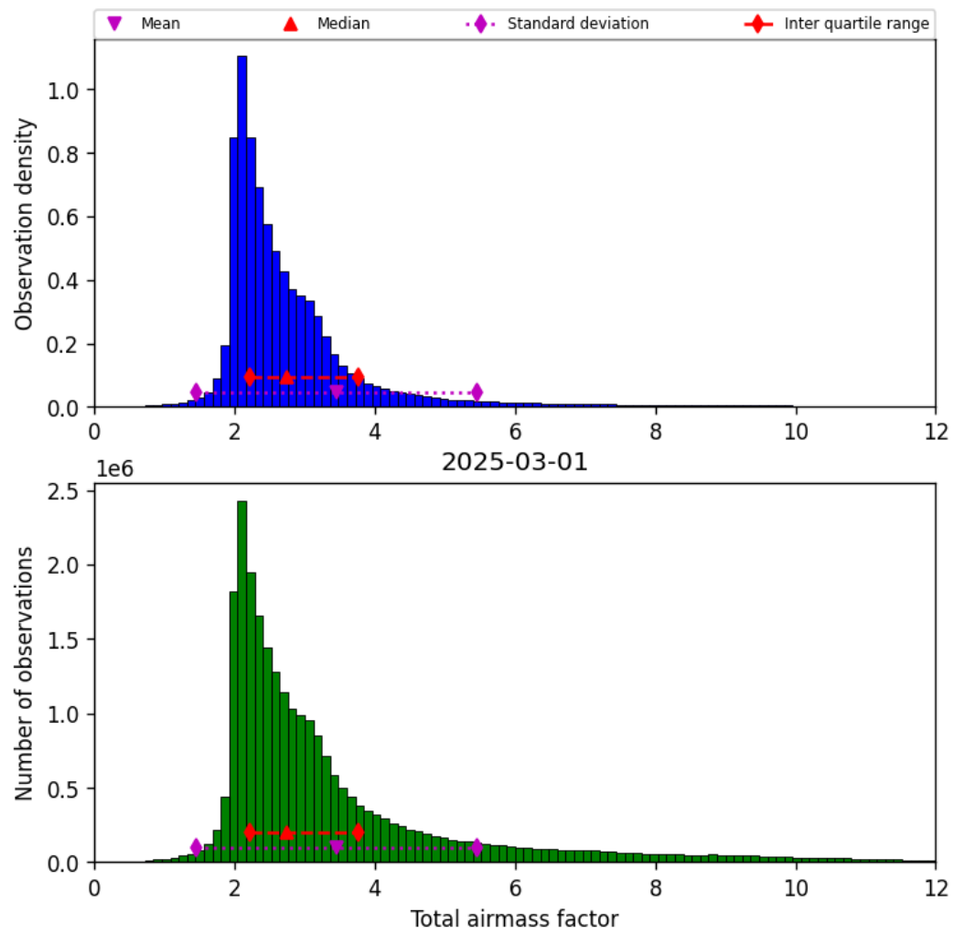
Figure 32: Histogram of “Total airmass factor” for 2025-03-01 to 2025-03-02
