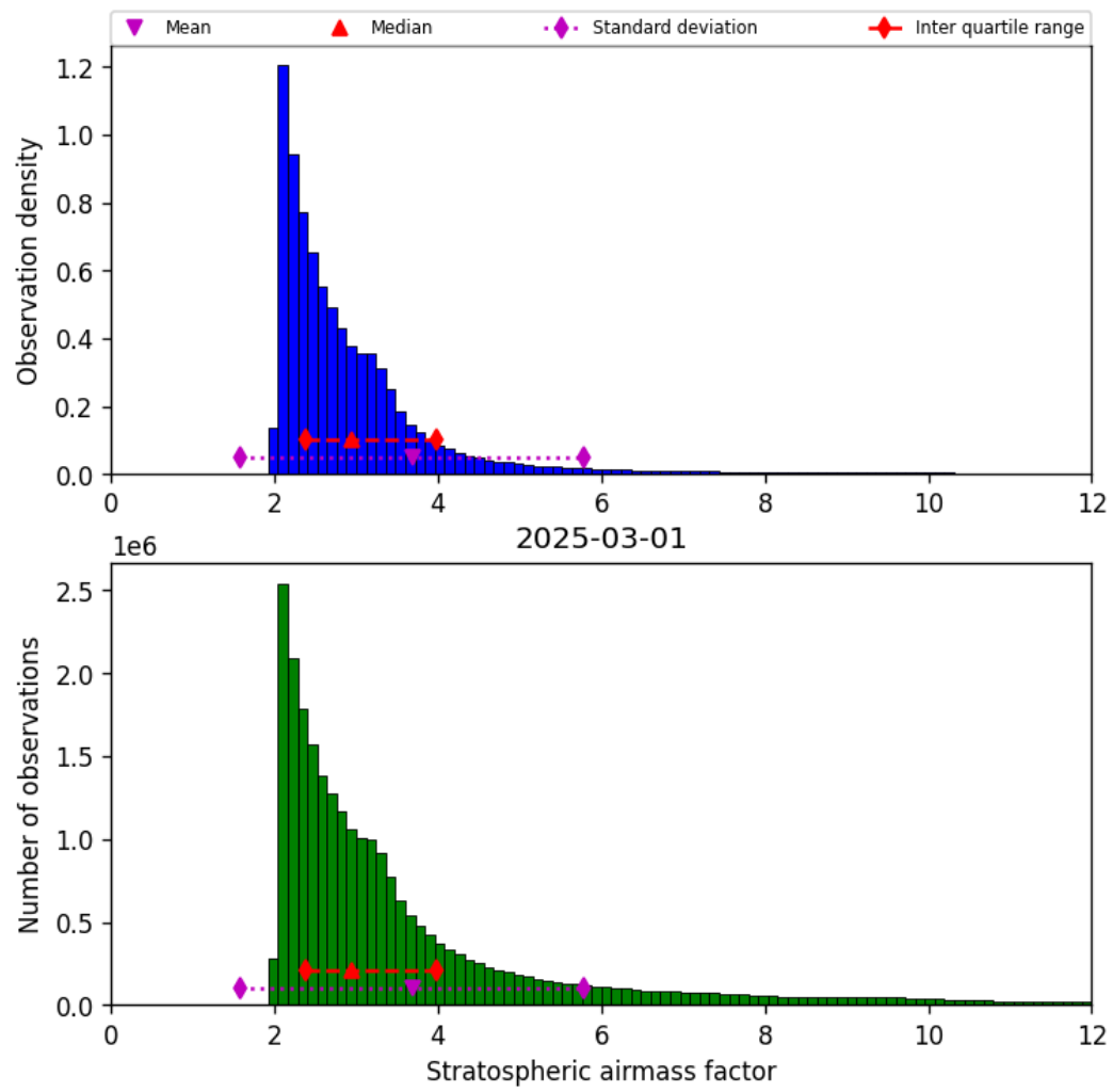
Figure 44: Histogram of “Stratospheric airmass factor” for 2025-03-01 to 2025-03-02
