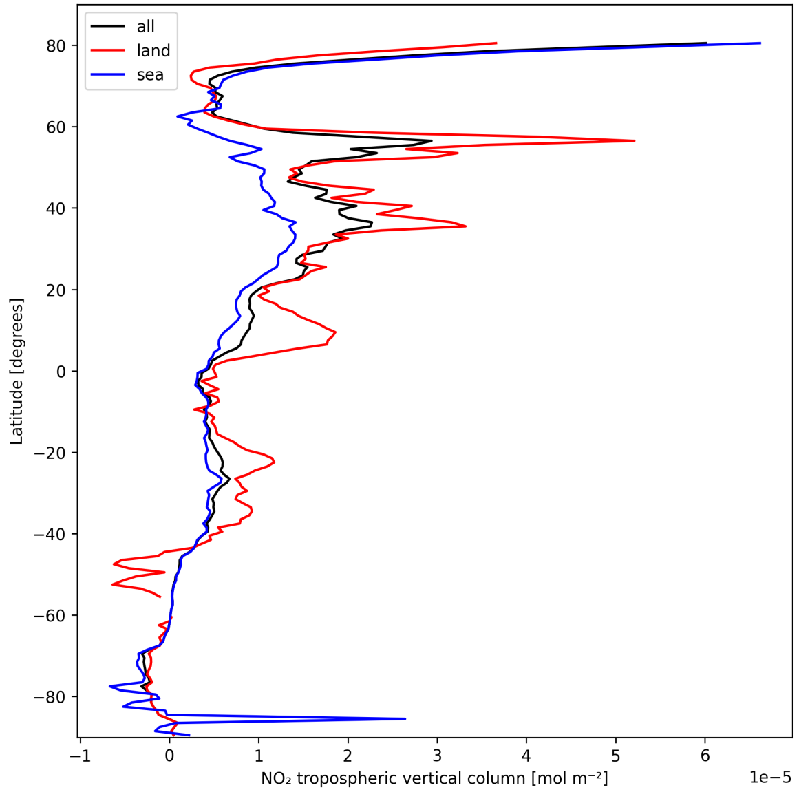
Figure 12: Zonal average of “NO 2 tropospheric vertical column” for 2025-03-01 to 2025-03-02.
