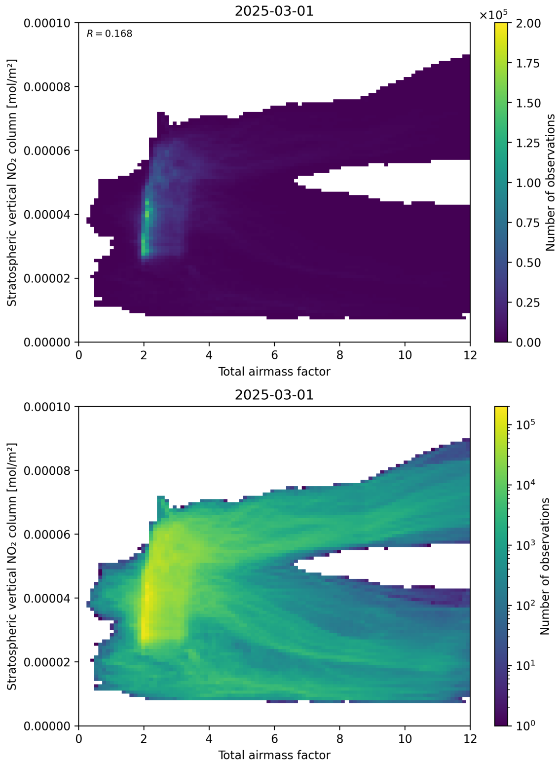
Figure 64: Scatter density plot of “Total airmass factor” against “Stratospheric vertical \text{NO}_2 column” for 2025-03-01 to 2025-03-02.
