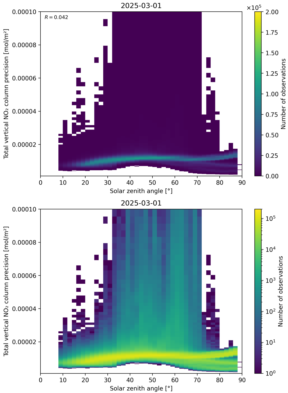
Figure 154: Scatter density plot of “Solar zenith angle” against “Total vertical NO 2 column precision” for 2025-03-01 to 2025-03-02.
