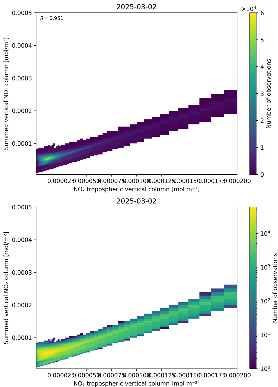
Figure 126: Scatter density plot of “NO 2 tropospheric vertical column” against “Summed vertical NO 2 column” for 2025-03-01 to 2025-03-03.
