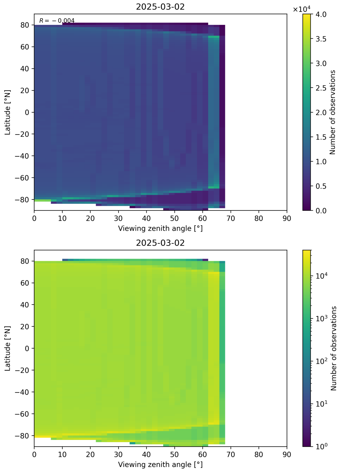
Figure 163: Scatter density plot of “Viewing zenith angle” against “Latitude” for 2025-03-01 to 2025-03-03.
