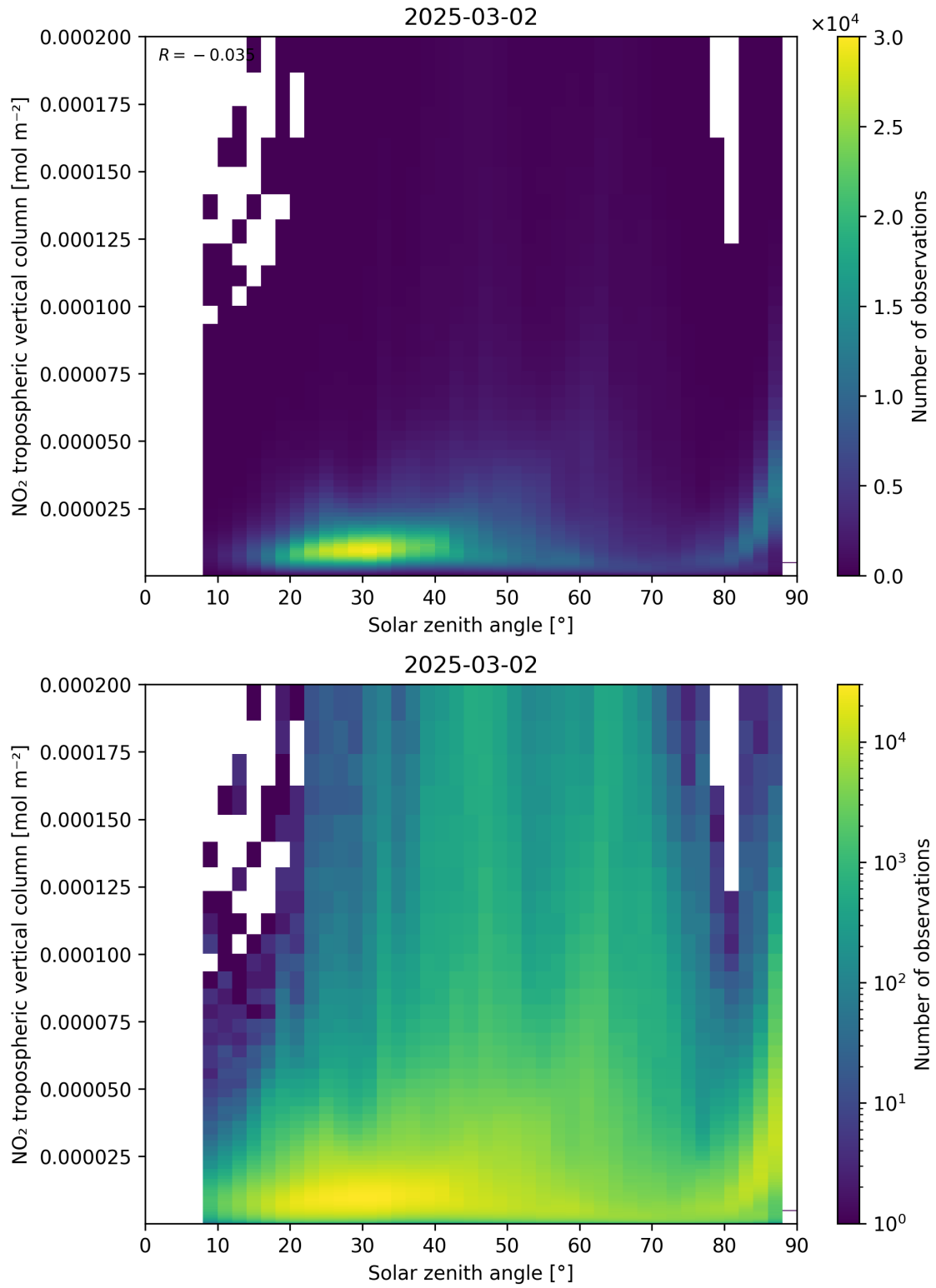
Figure 155: Scatter density plot of “Solar zenith angle” against “NO 2 tropospheric vertical column” for 2025-03-01 to 2025-03-03.
