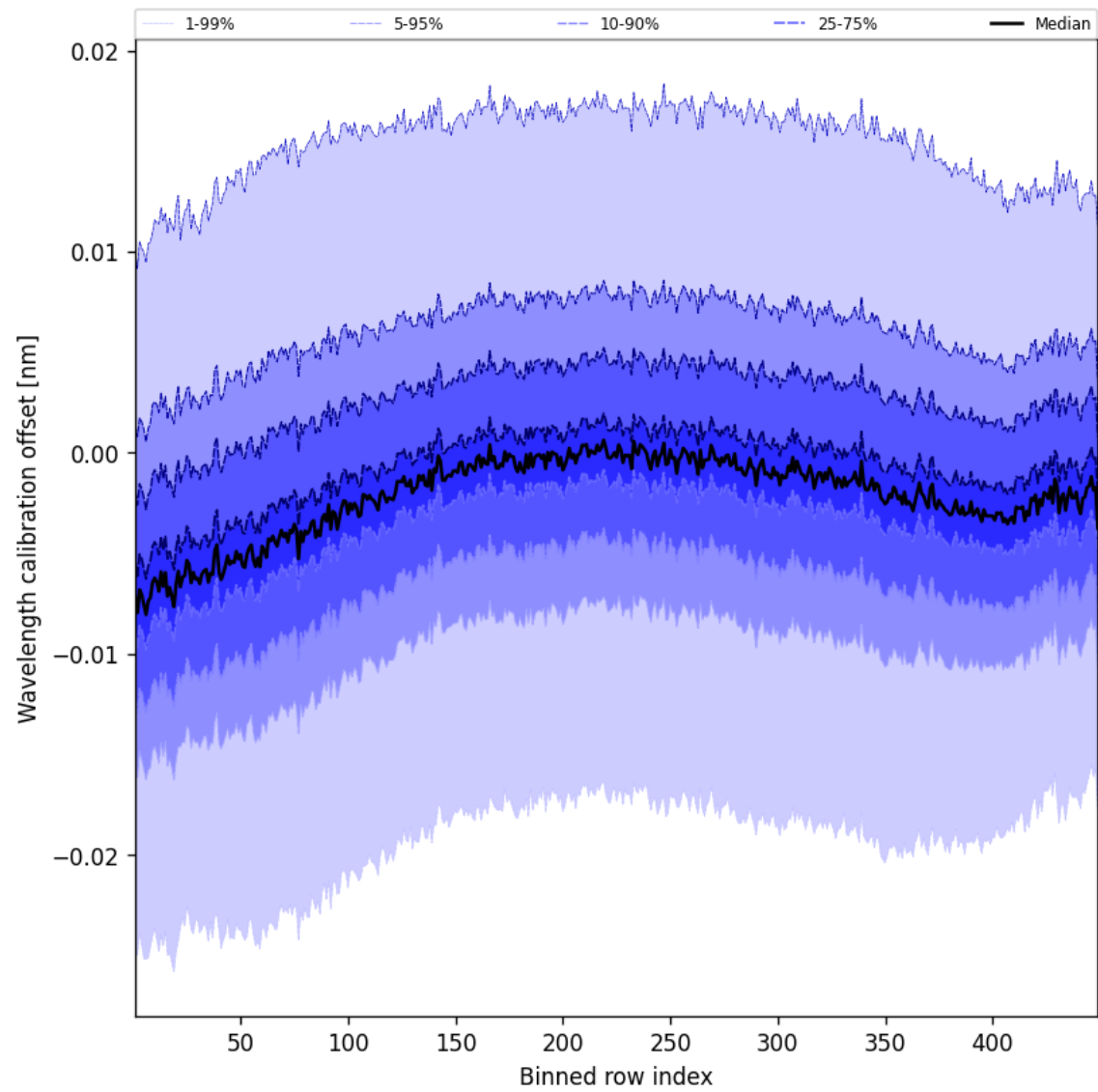
Figure 52: Along track statistics of “Wavelength calibration offset” for 2025-03-01 to 2025-03-03
