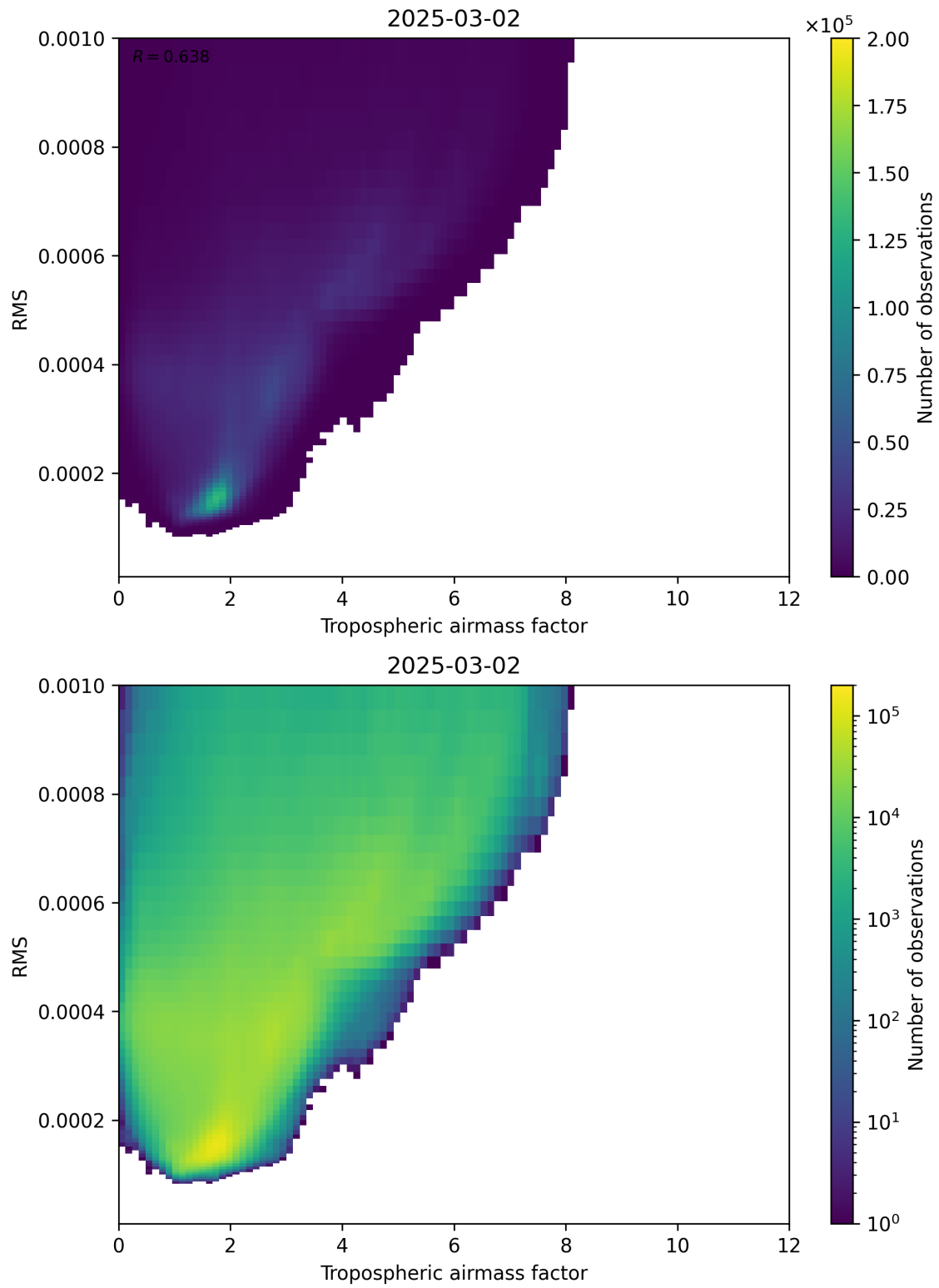
Figure 79: Scatter density plot of “Tropospheric airmass factor” against “RMS” for 2025-03-01 to 2025-03-03.
