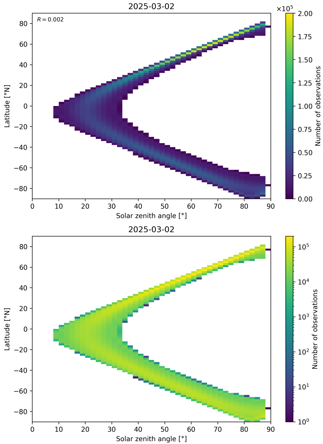
Figure 149: Scatter density plot of “Solar zenith angle” against “Latitude” for 2025-03-01 to 2025-03-03.
