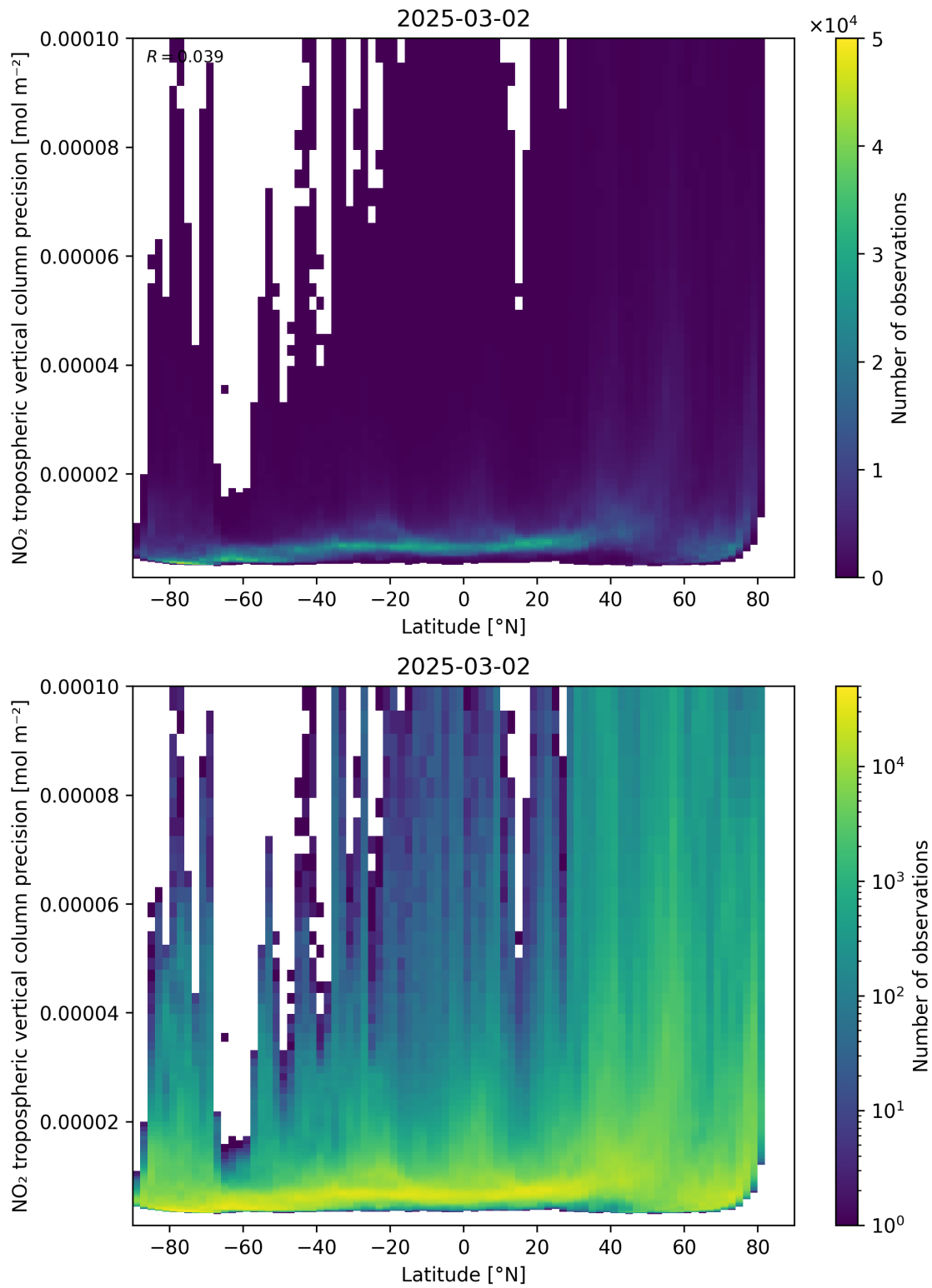
Figure 93: Scatter density plot of “Latitude” against “NO 2 tropospheric vertical column precision” for 2025-03-01 to 2025-03-03.
