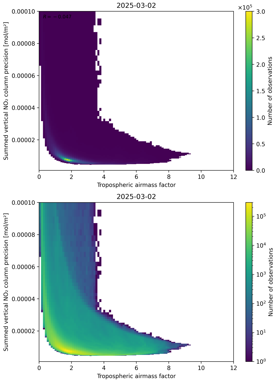
Figure 76: Scatter density plot of “Tropospheric airmass factor” against “Summed vertical NO 2 column precision” for 2025-03-01 to 2025-03-03.
