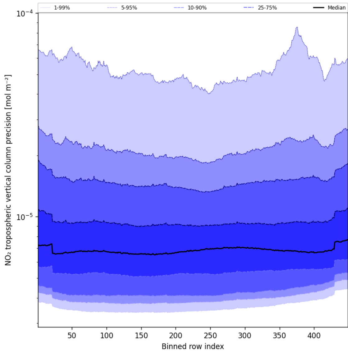
Figure 47: Along track statistics of “NO 2 tropospheric vertical column precision” for 2025-03-01 to 2025-03-03
