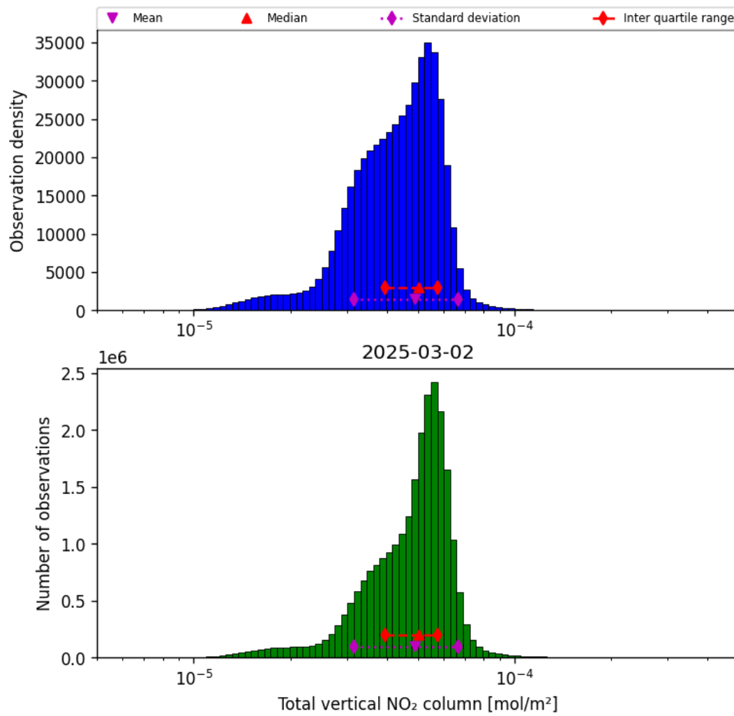
Figure 38: Histogram of “Total vertical NO 2 column” for 2025-03-01 to 2025-03-03
