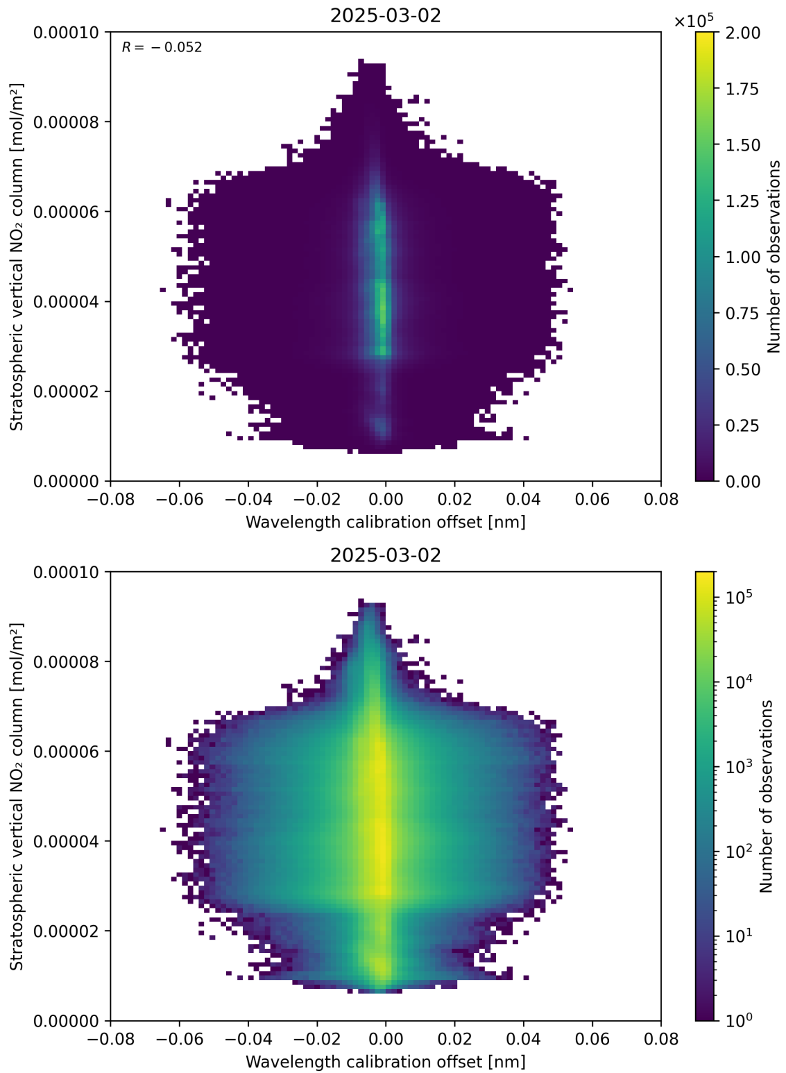
Figure 176: Scatter density plot of “Wavelength calibration offset” against “Stratospheric vertical NO 2 column” for 2025-03-01 to 2025-03-03.
