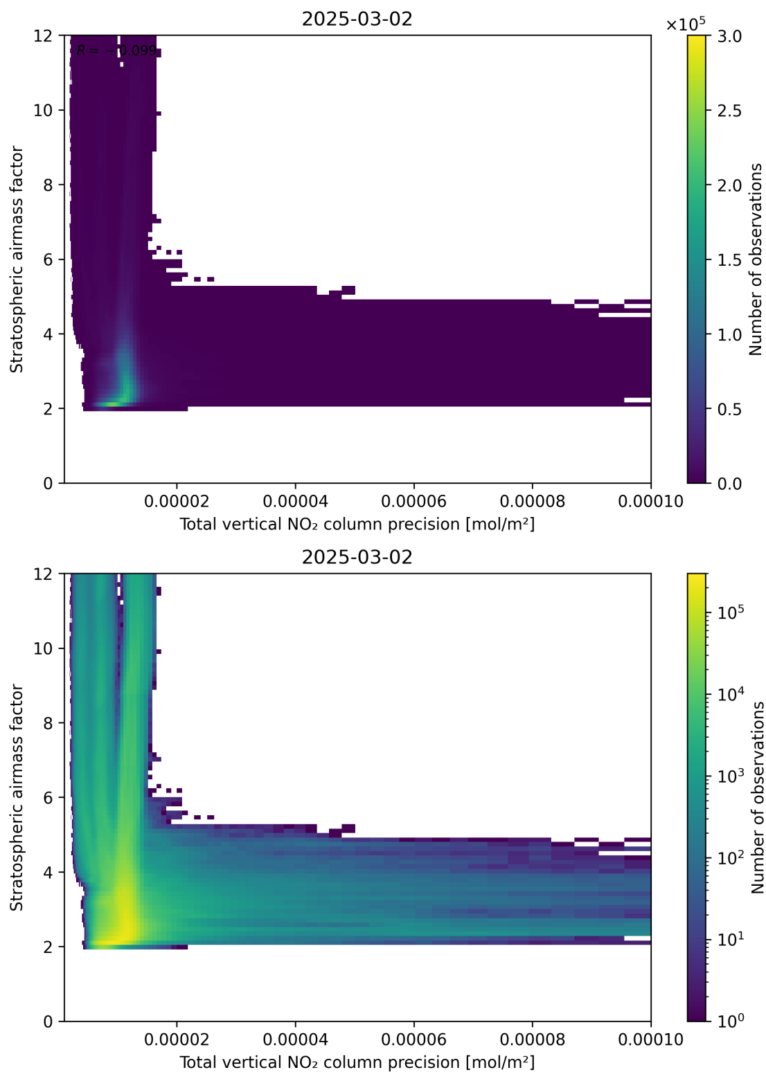
Figure 115: Scatter density plot of “Total vertical NO 2 column precision” against “Stratospheric airmass factor” for 2025-03-01 to 2025-03-03.
