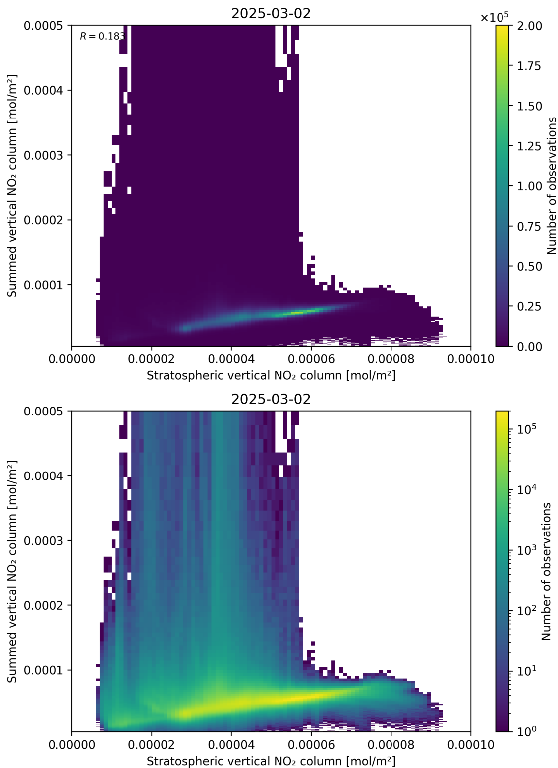
Figure 98: Scatter density plot of “Stratospheric vertical NO 2 column” against “Summed vertical NO 2 column” for 2025-03-01 to 2025-03-03.
