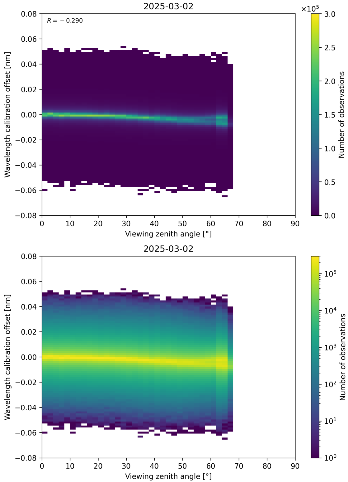
Figure 173: Scatter density plot of “Viewing zenith angle” against “Wavelength calibration offset” for 2025-03-01 to 2025-03-03.
