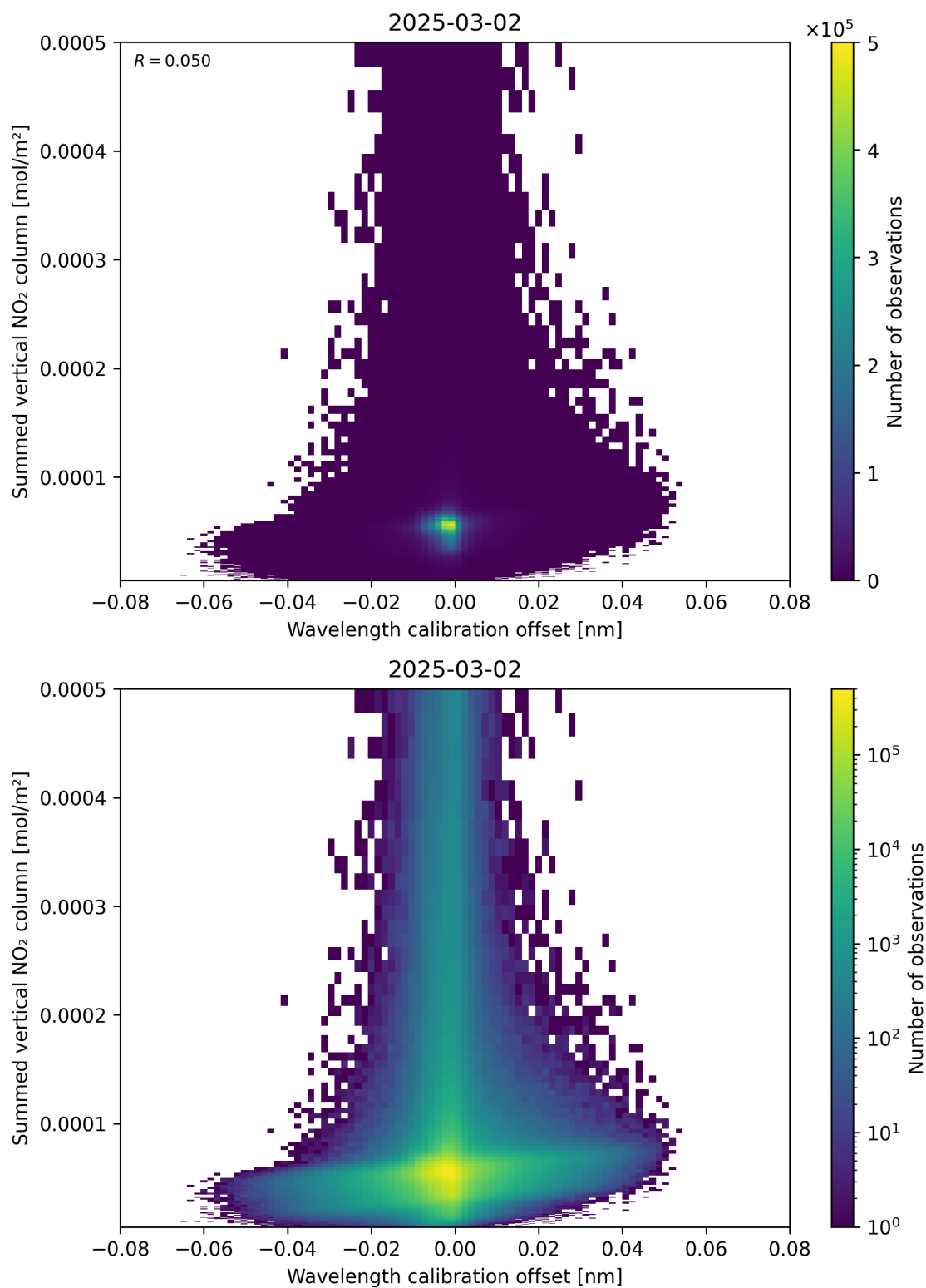
Figure 177: Scatter density plot of “Wavelength calibration offset” against “Summed vertical NO 2 column” for 2025-03-01 to 2025-03-03.
