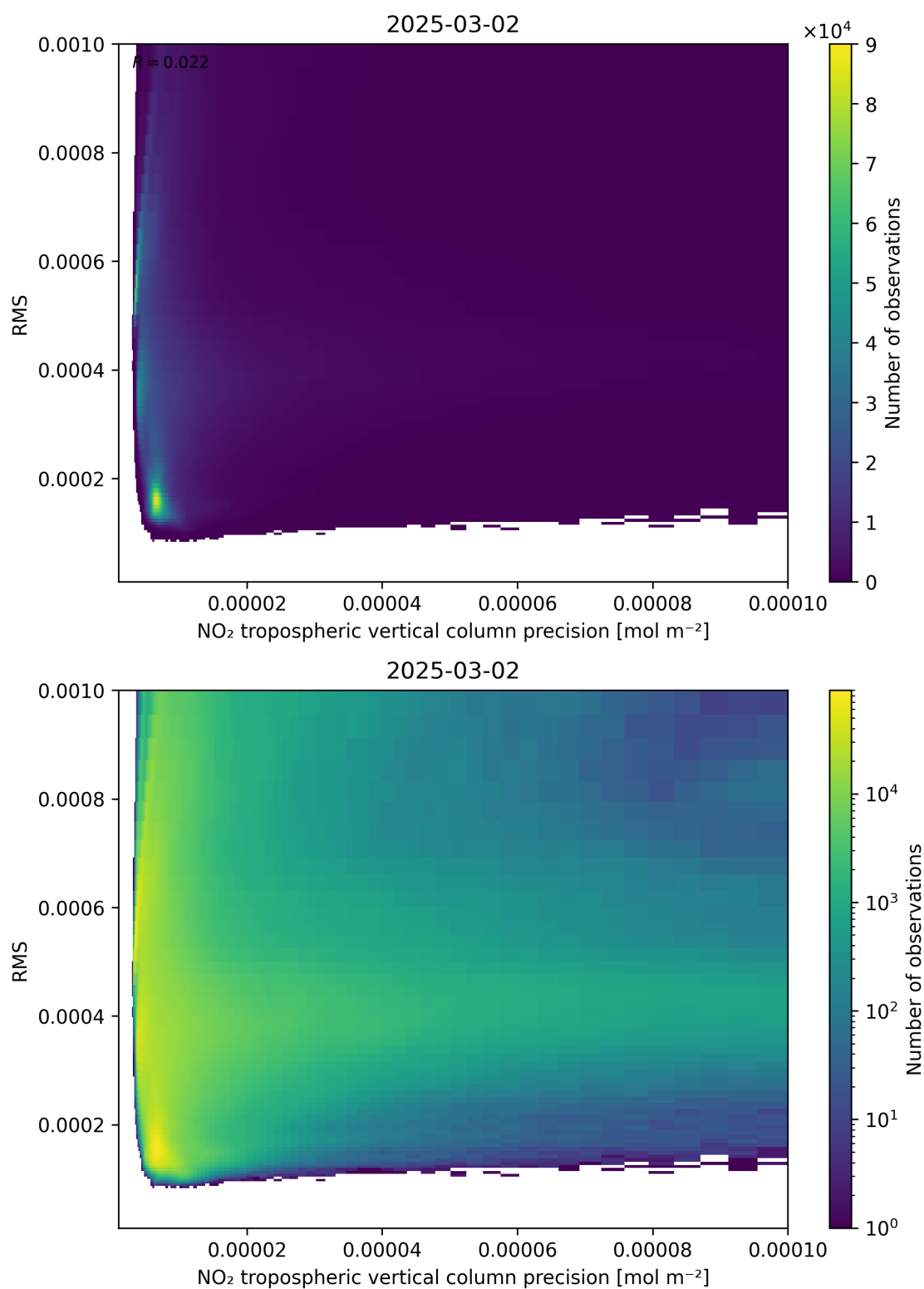
Figure 140: Scatter density plot of “NO 2 tropospheric vertical column precision” against “RMS” for 2025-03-01 to 2025-03-03.
