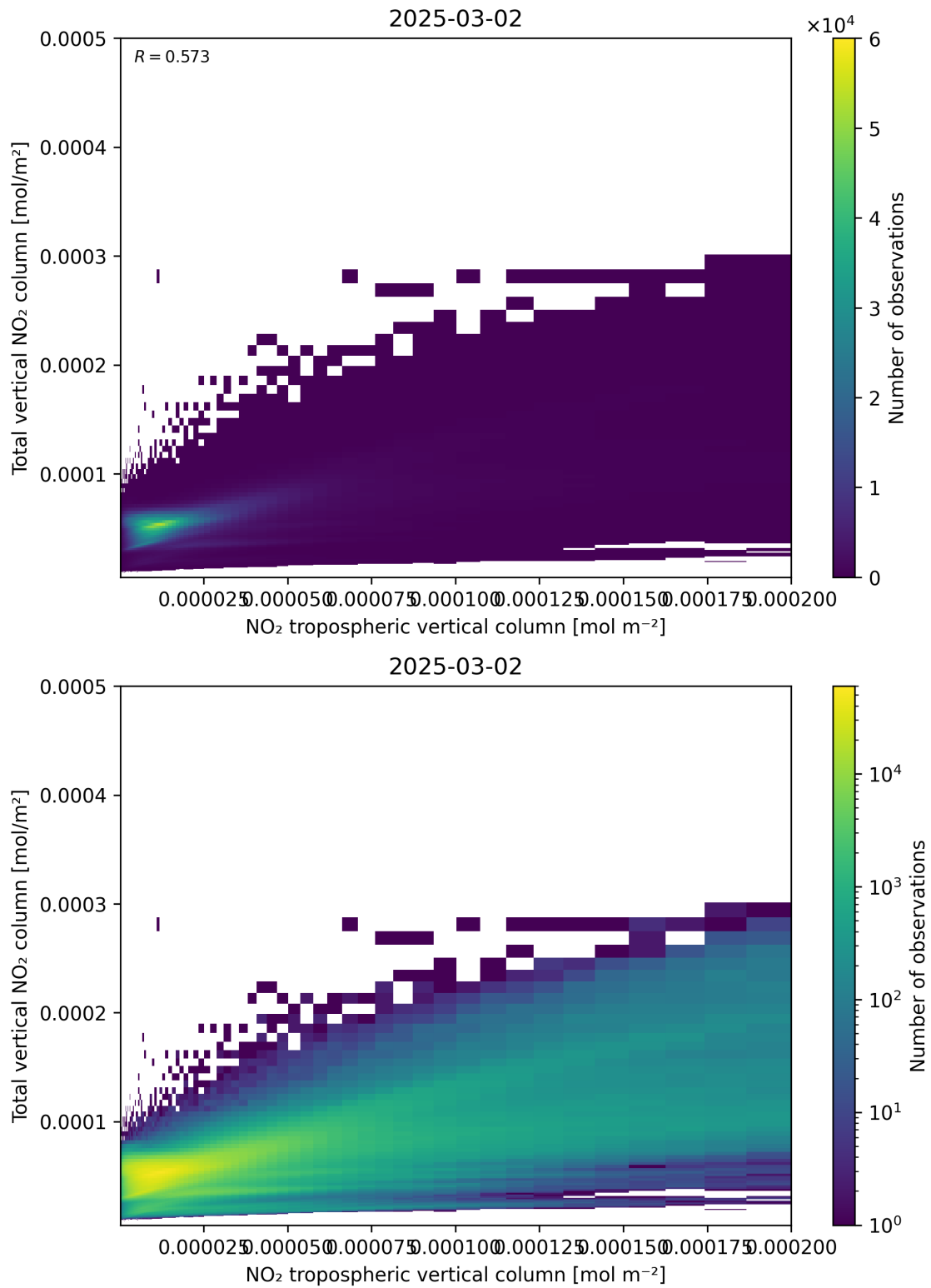
Figure 128: Scatter density plot of “NO 2 tropospheric vertical column” against “Total vertical NO 2 column” for 2025-03-01 to 2025-03-03.
