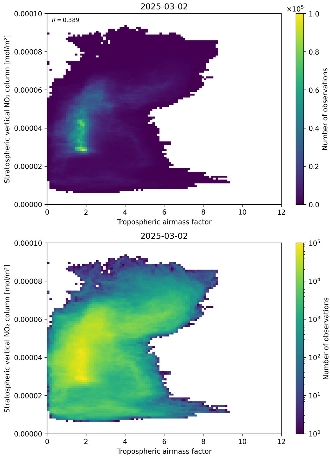
Figure 74: Scatter density plot of “Tropospheric airmass factor” against “Stratospheric vertical NO 2 column” for 2025-03-01 to 2025-03-03.
