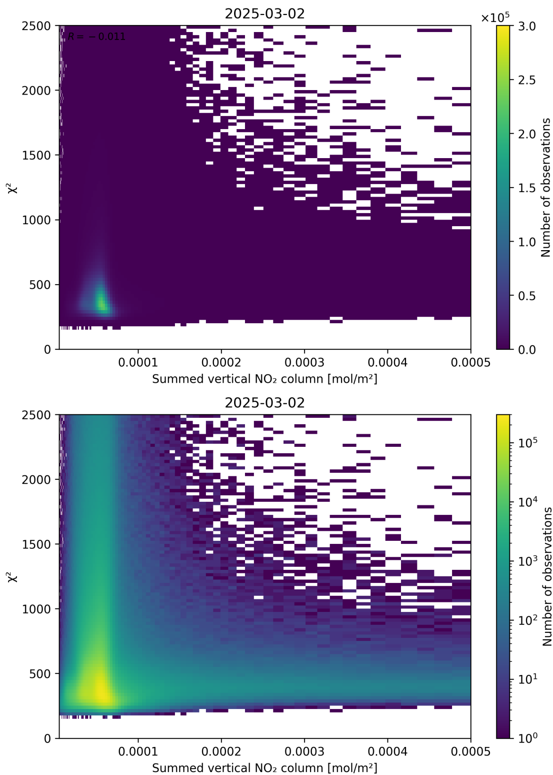
Figure 104: Scatter density plot of “Summed vertical NO 2 column” against “ \chi^2 ” for 2025-03-01 to 2025-03-03.
