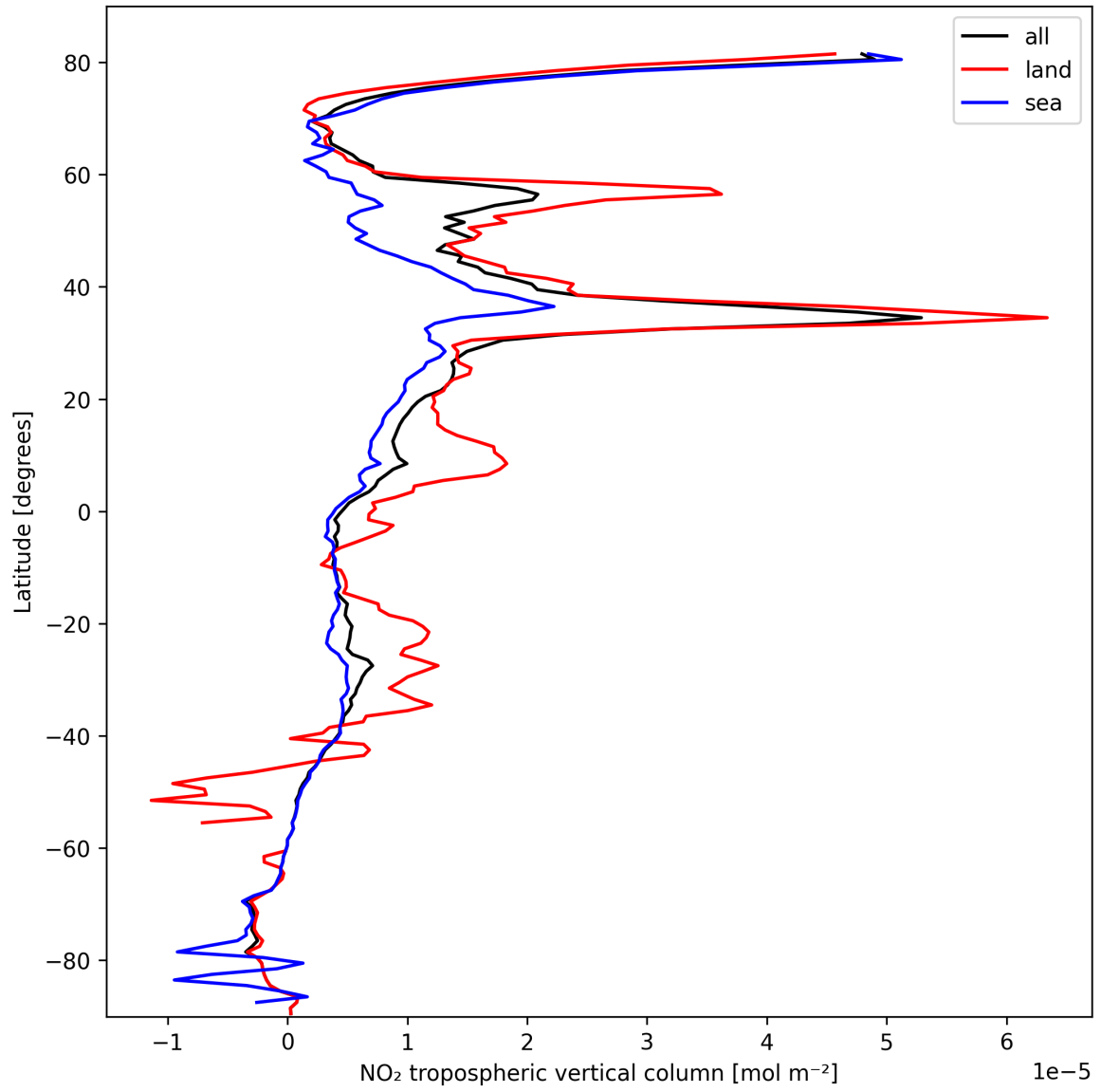
Figure 12: Zonal average of “NO 2 tropospheric vertical column” for 2025-03-01 to 2025-03-03.
