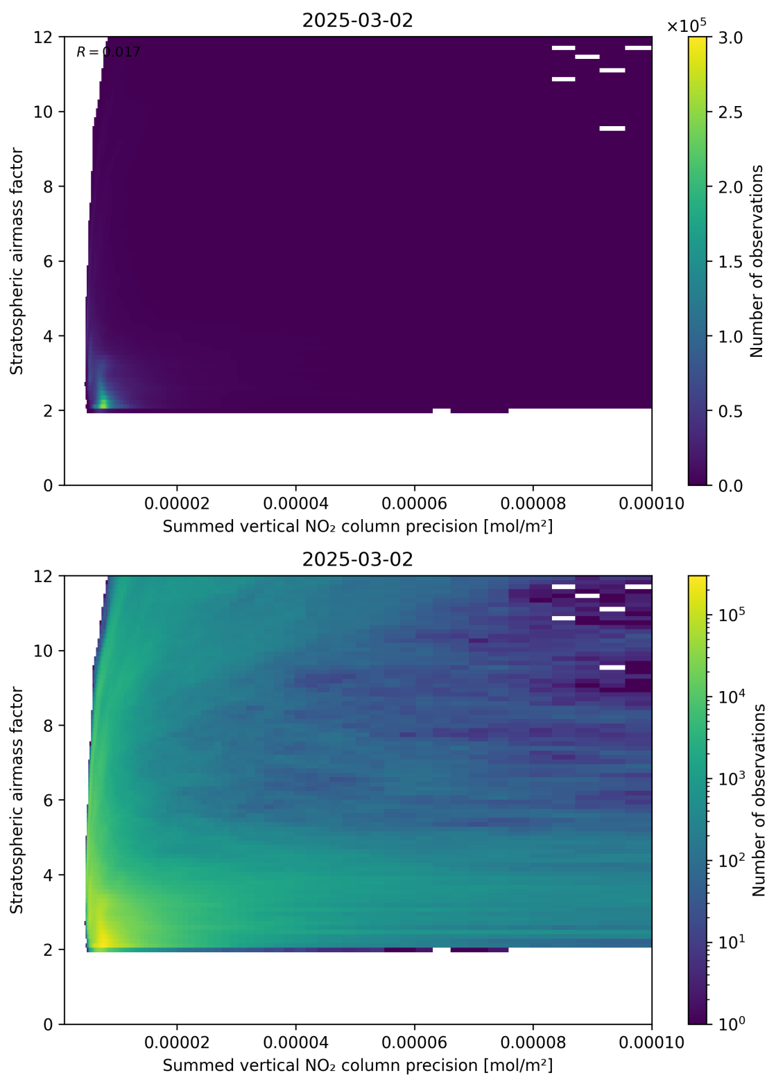
Figure 106: Scatter density plot of “Summed vertical NO 2 column precision” against “Stratospheric airmass factor” for 2025-03-01 to 2025-03-03.
