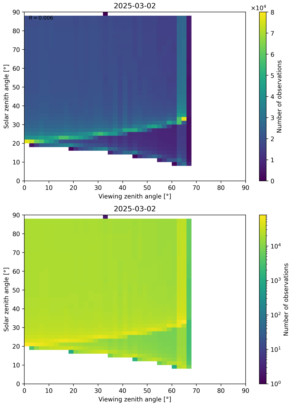
Figure 172: Scatter density plot of “Viewing zenith angle” against “Solar zenith angle” for 2025-03-01 to 2025-03-03.
