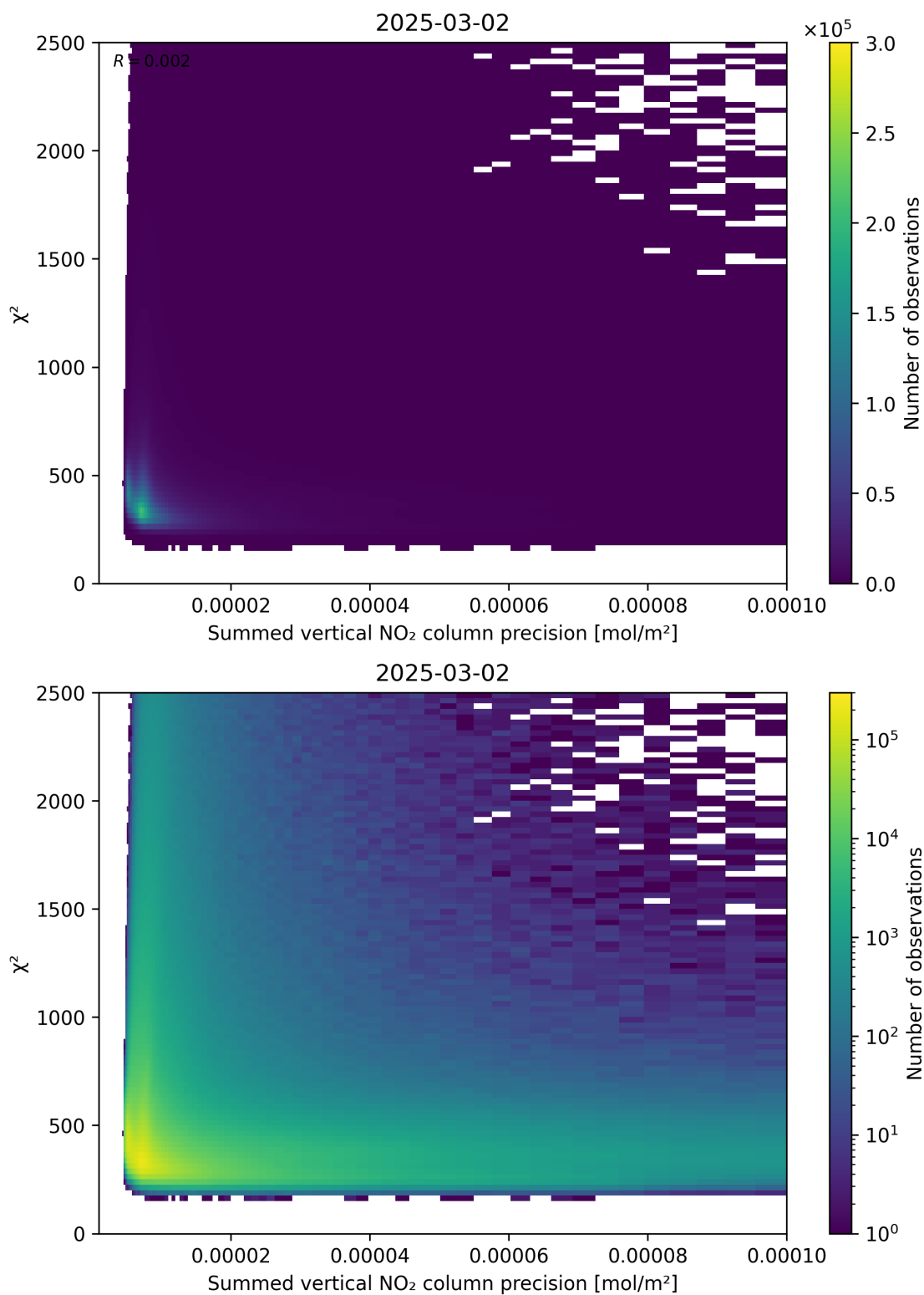
Figure 107: Scatter density plot of “Summed vertical NO 2 column precision” against “ \chi^2 ” for 2025-03-01 to 2025-03-03.
