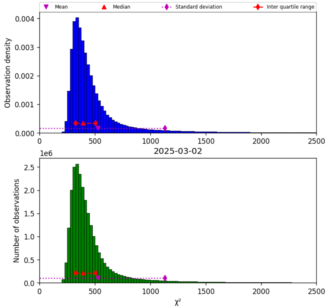
Figure 42: Histogram of “ \chi^2 ” for 2025-03-01 to 2025-03-03
