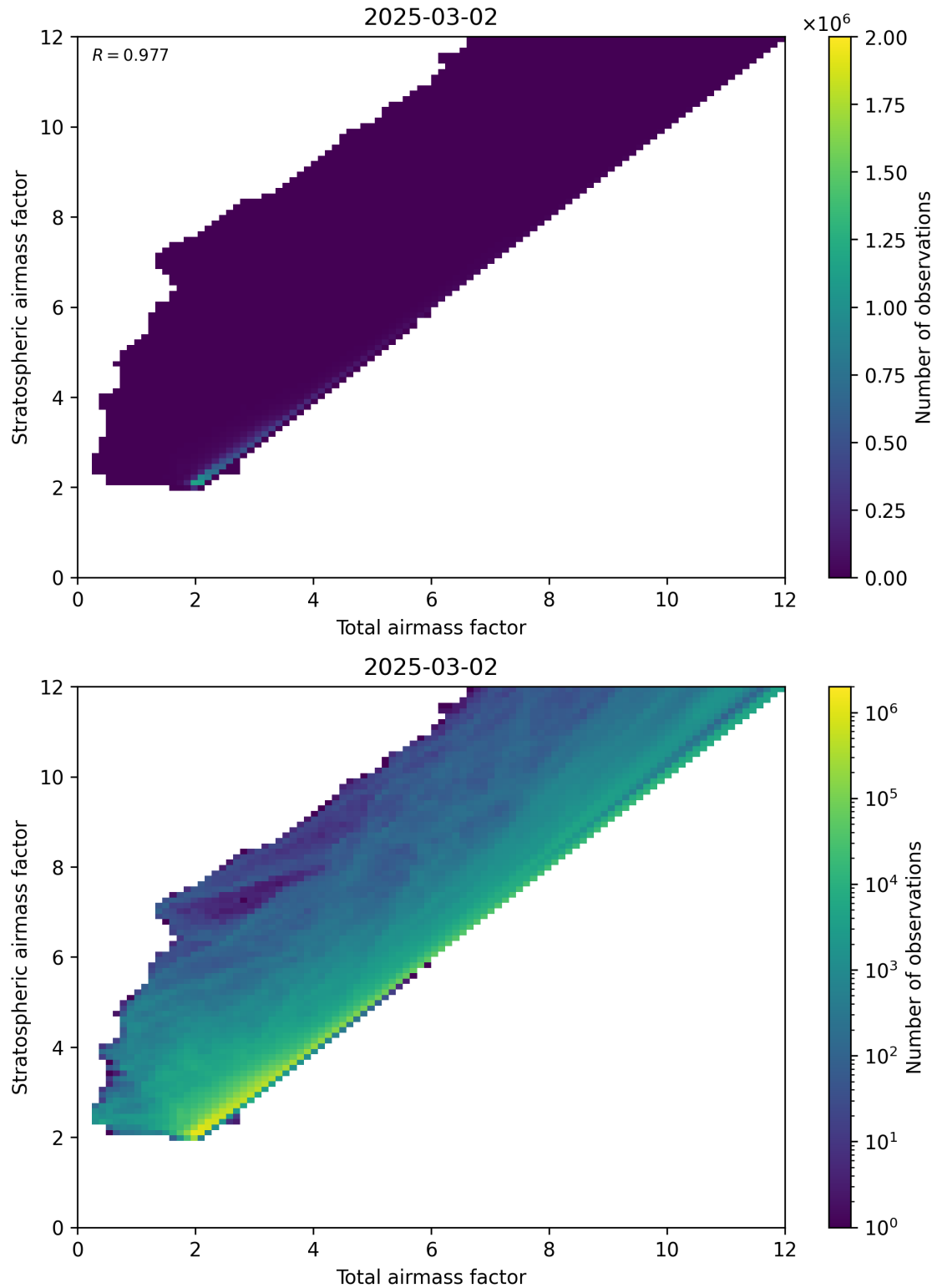
Figure 62: Scatter density plot of “Total airmass factor” against “Stratospheric airmass factor” for 2025-03-01 to 2025-03-03.
