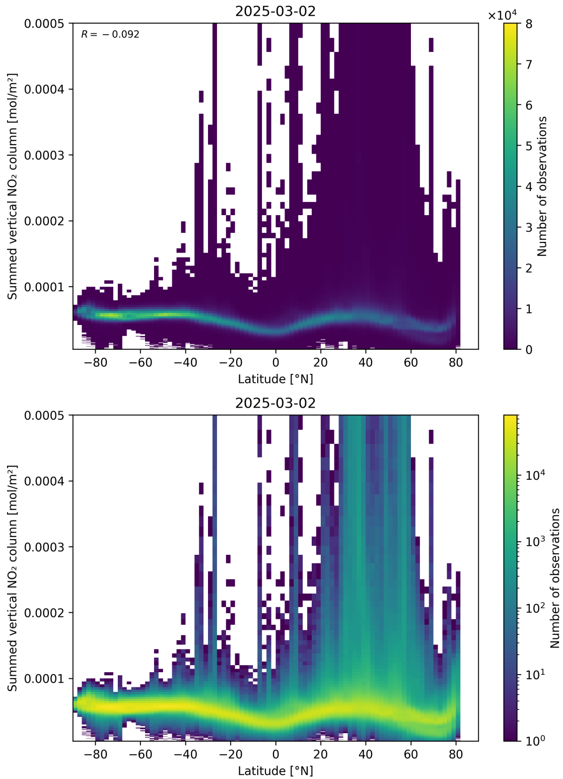
Figure 88: Scatter density plot of “Latitude” against “Summed vertical NO 2 column” for 2025-03-01 to 2025-03-03.
