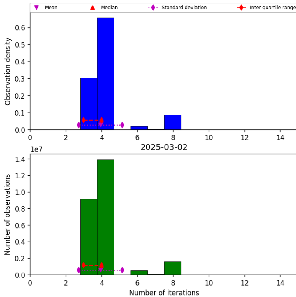
Figure 34: Histogram of “Number of iterations” for 2025-03-01 to 2025-03-03
