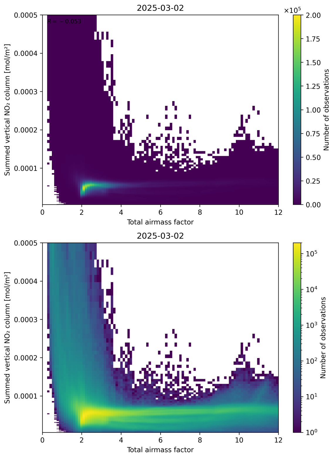
Figure 65: Scatter density plot of “Total airmass factor” against “Summed vertical NO 2 column” for 2025-03-01 to 2025-03-03.
