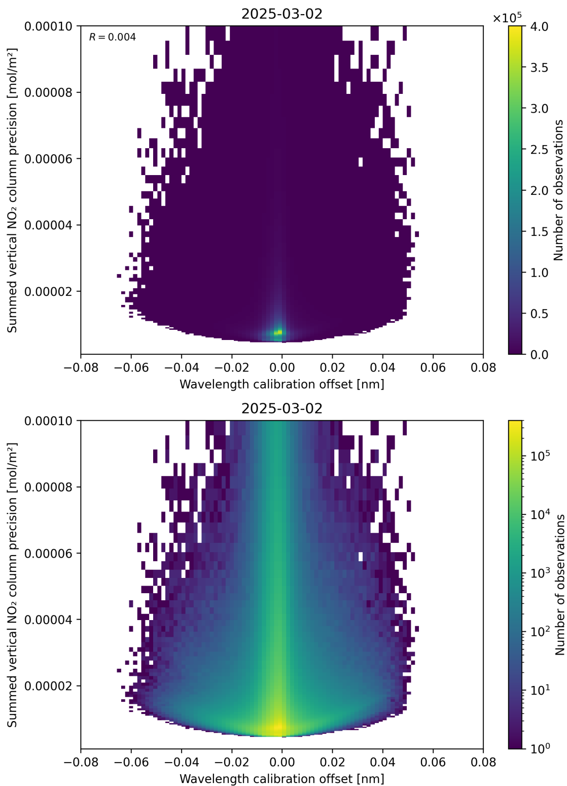
Figure 178: Scatter density plot of “Wavelength calibration offset” against “Summed vertical NO 2 column precision” for 2025-03-01 to 2025-03-03.
