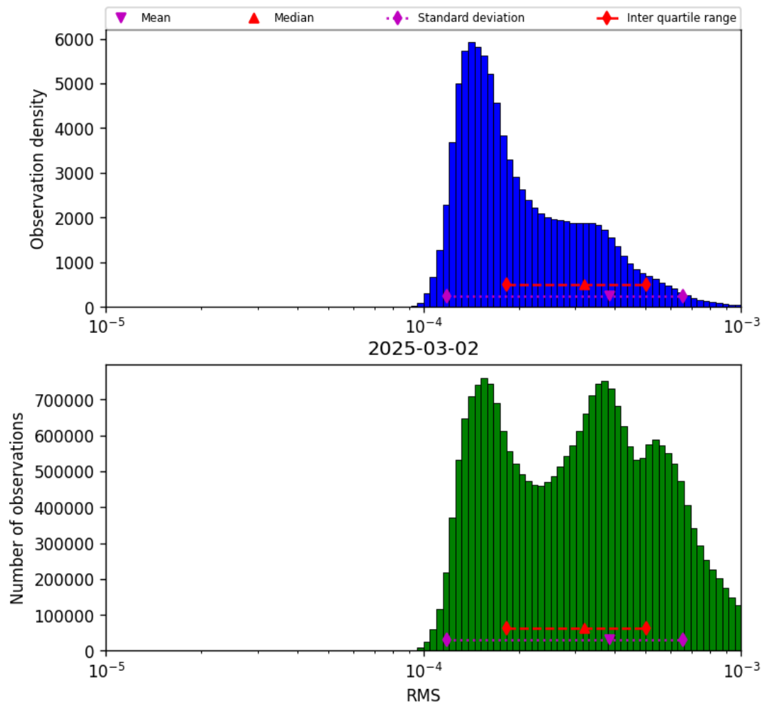
Figure 43: Histogram of “RMS” for 2025-03-01 to 2025-03-03
