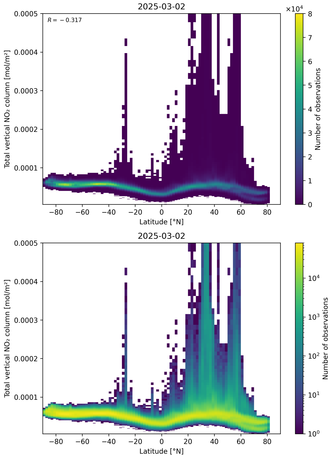
Figure 90: Scatter density plot of “Latitude” against “Total vertical NO 2 column” for 2025-03-01 to 2025-03-03.
