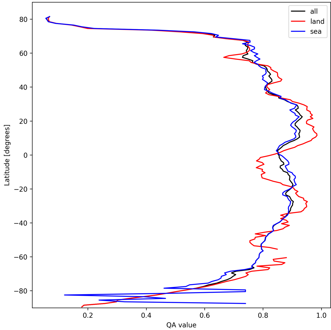
Figure 11: Zonal average of “QA value” for 2025-03-01 to 2025-03-03.
