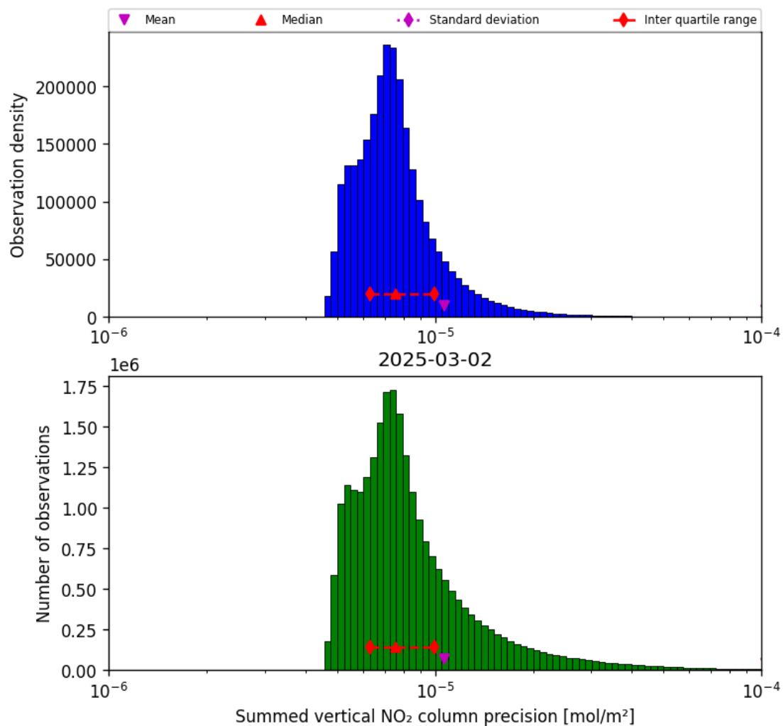
Figure 41: Histogram of "Summed vertical NO 2 column precision" for 2025-03-01 to 2025-03-03
