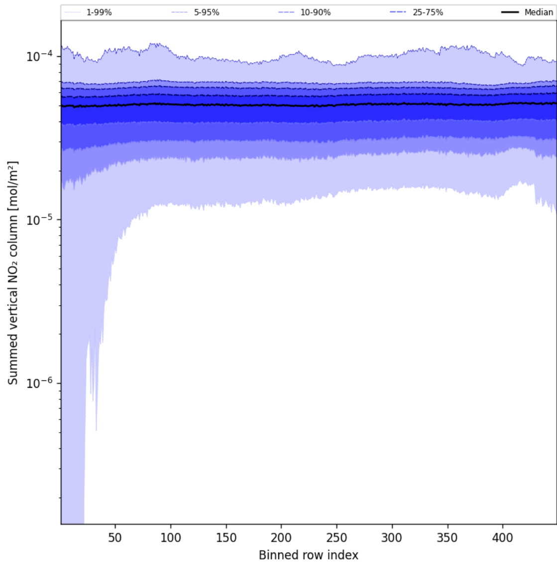
Figure 57: Along track statistics of “Summed vertical NO 2 column” for 2025-03-01 to 2025-03-03
