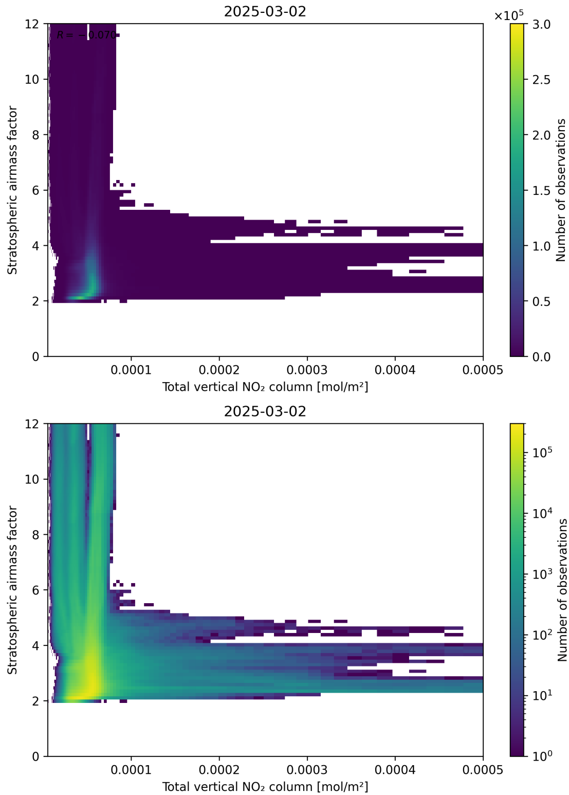
Figure 110: Scatter density plot of “Total vertical NO 2 column” against “Stratospheric airmass factor” for 2025-03-01 to 2025-03-03.
