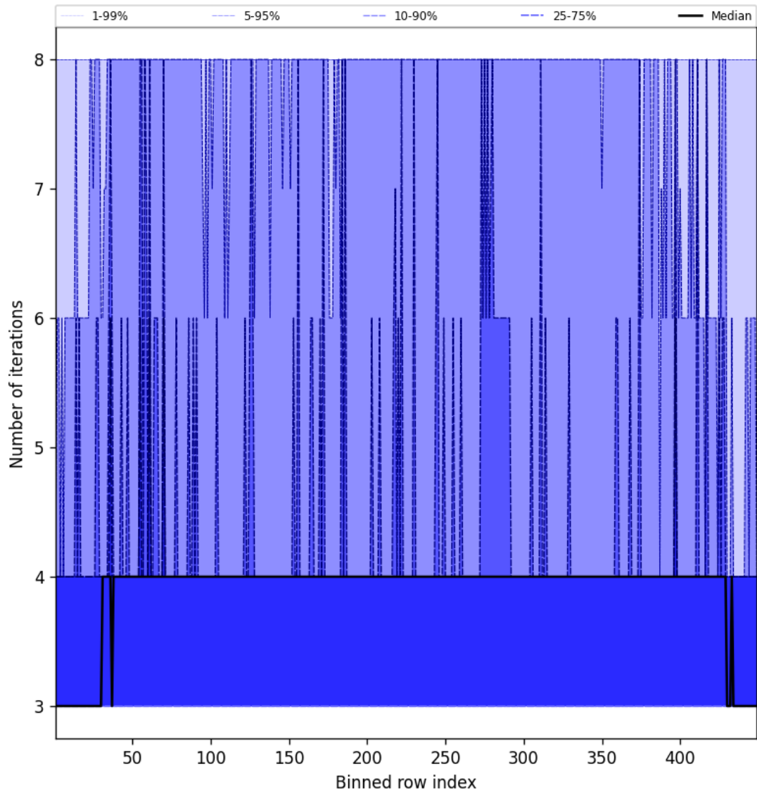
Figure 51: Along track statistics of “Number of iterations” for 2025-03-01 to 2025-03-03
