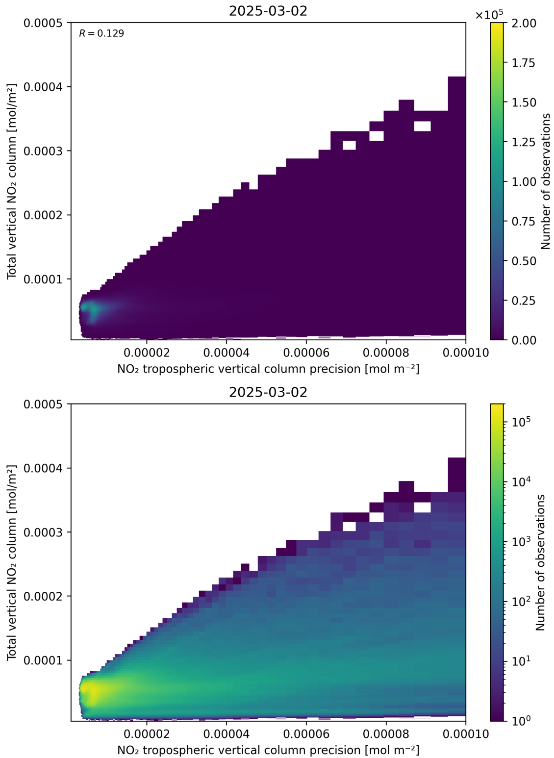
Figure 138: Scatter density plot of “NO 2 tropospheric vertical column precision” against “Total vertical NO 2 column” for 2025-03-01 to 2025-03-03.
