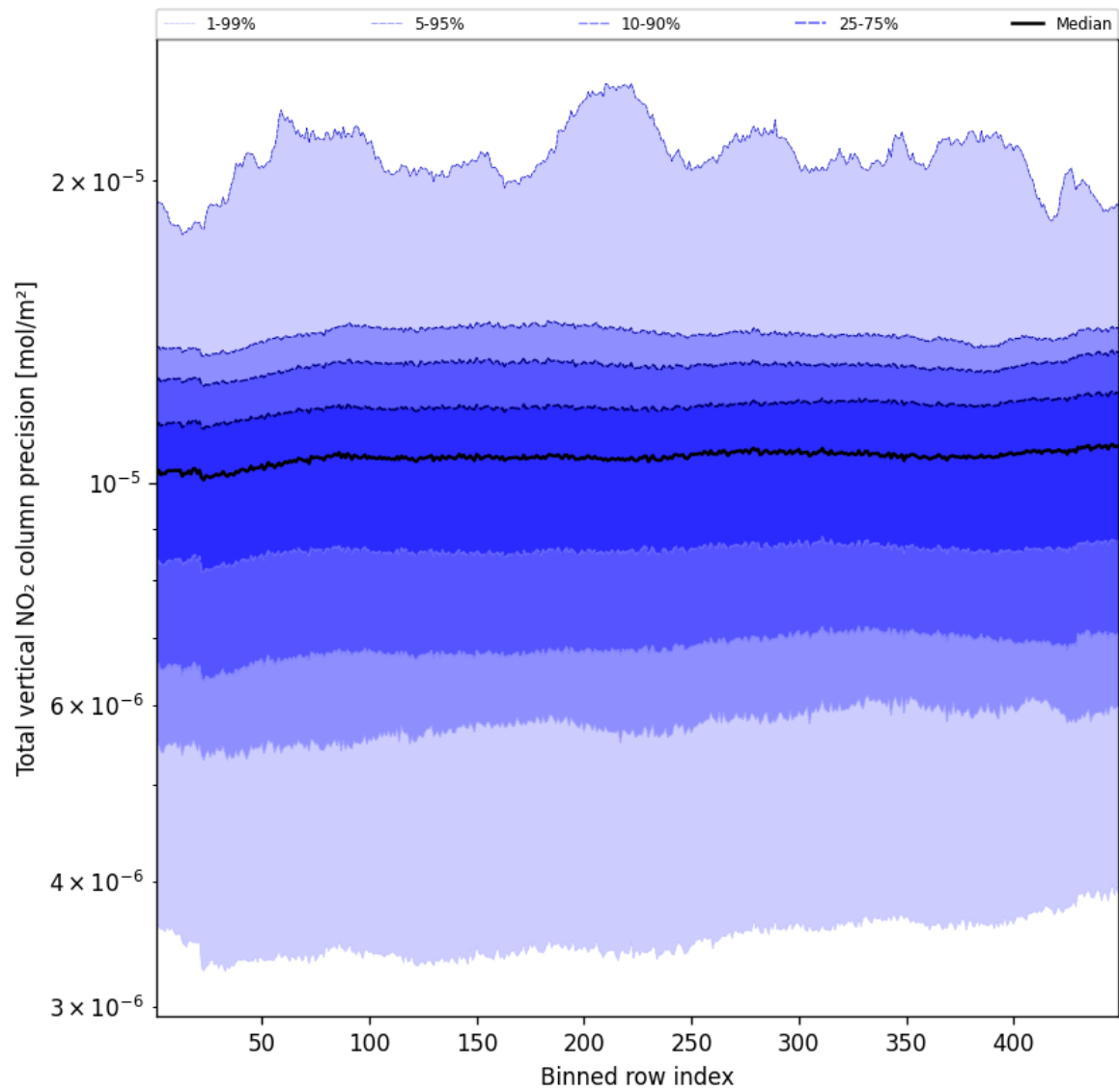
Figure 56: Along track statistics of “Total vertical NO 2 column precision” for 2025-03-01 to 2025-03-03
