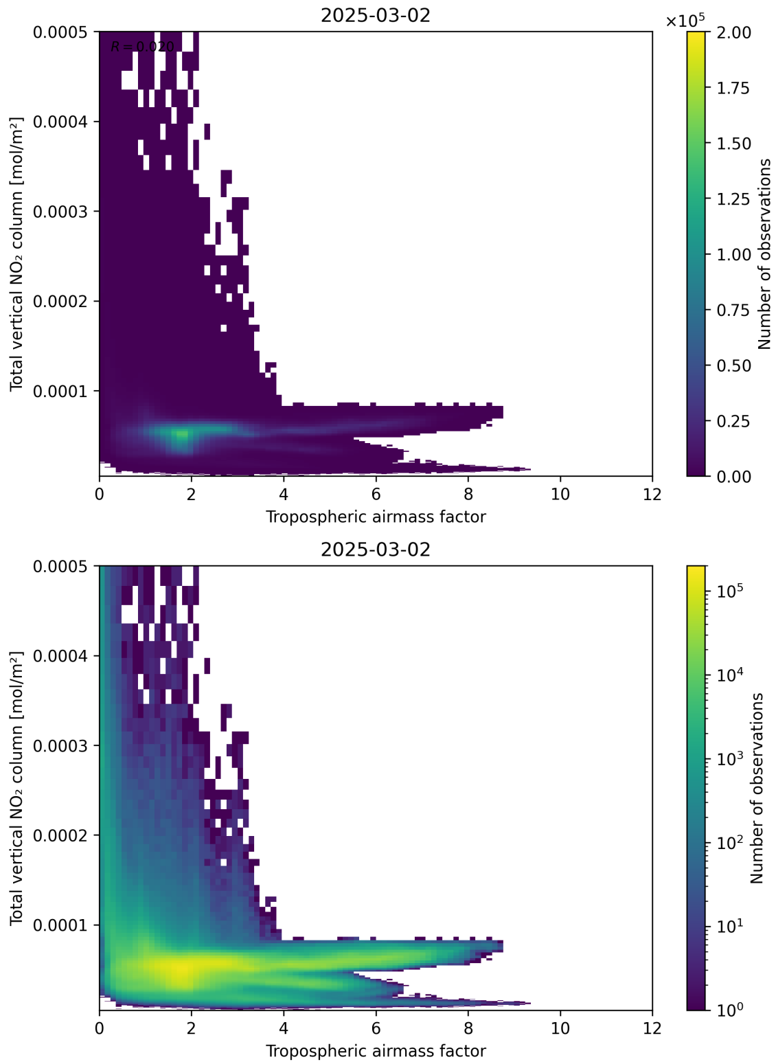
Figure 77: Scatter density plot of “Tropospheric airmass factor” against “Total vertical NO 2 column” for 2025-03-01 to 2025-03-03.
