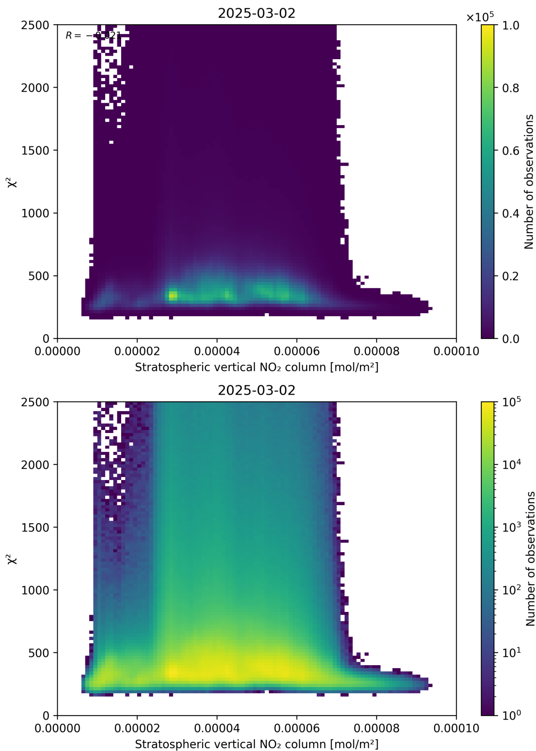
Figure 97: Scatter density plot of “Stratospheric vertical NO 2 column” against “ \chi^2 ” for 2025-03-01 to 2025-03-03.
