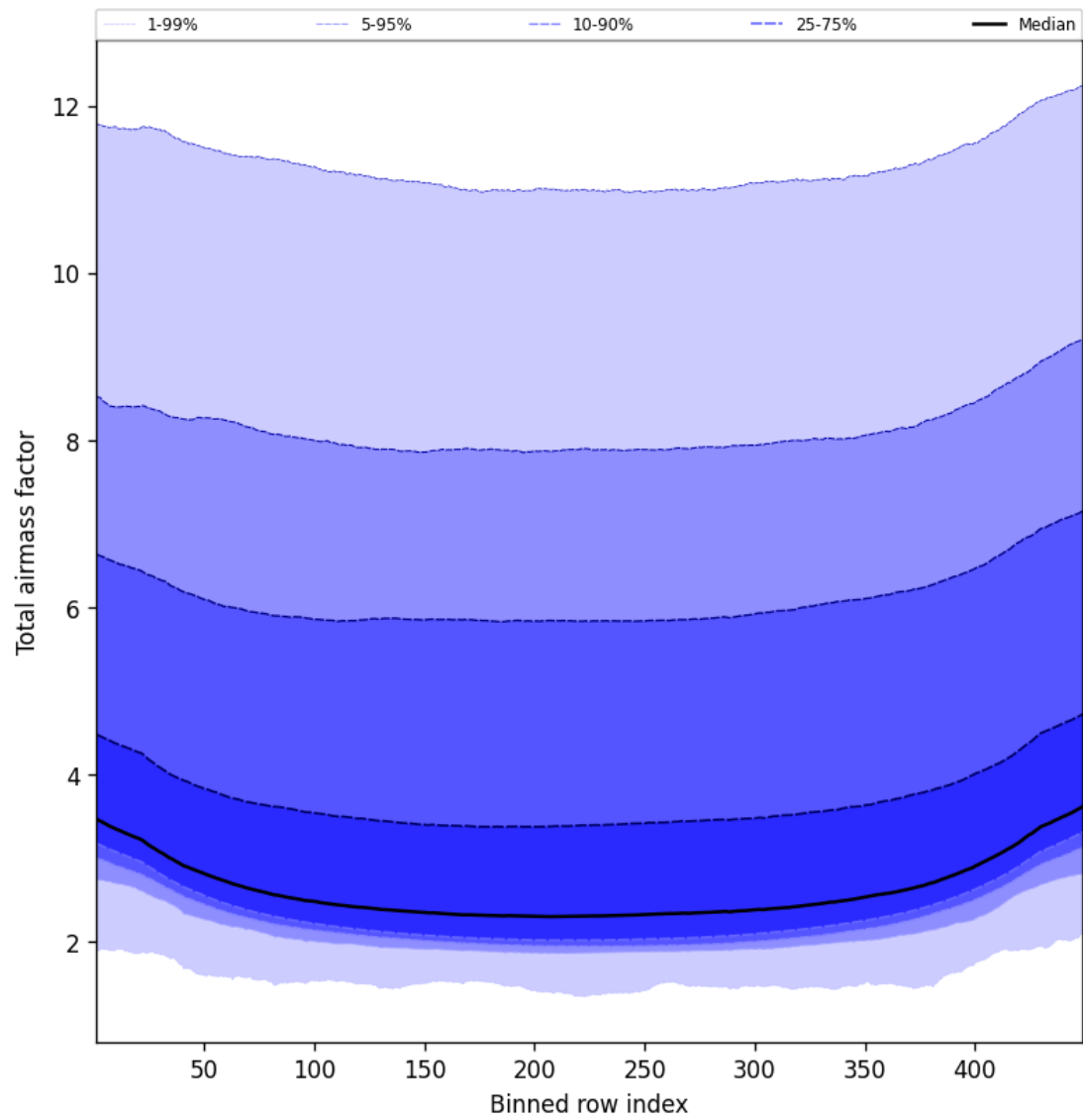
Figure 49: Along track statistics of “Total airmass factor” for 2025-03-01 to 2025-03-03
