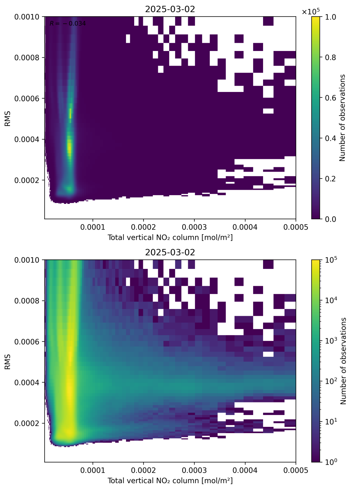
Figure 120: Scatter density plot of “Total vertical NO 2 column” against “RMS” for 2025-03-01 to 2025-03-03.
