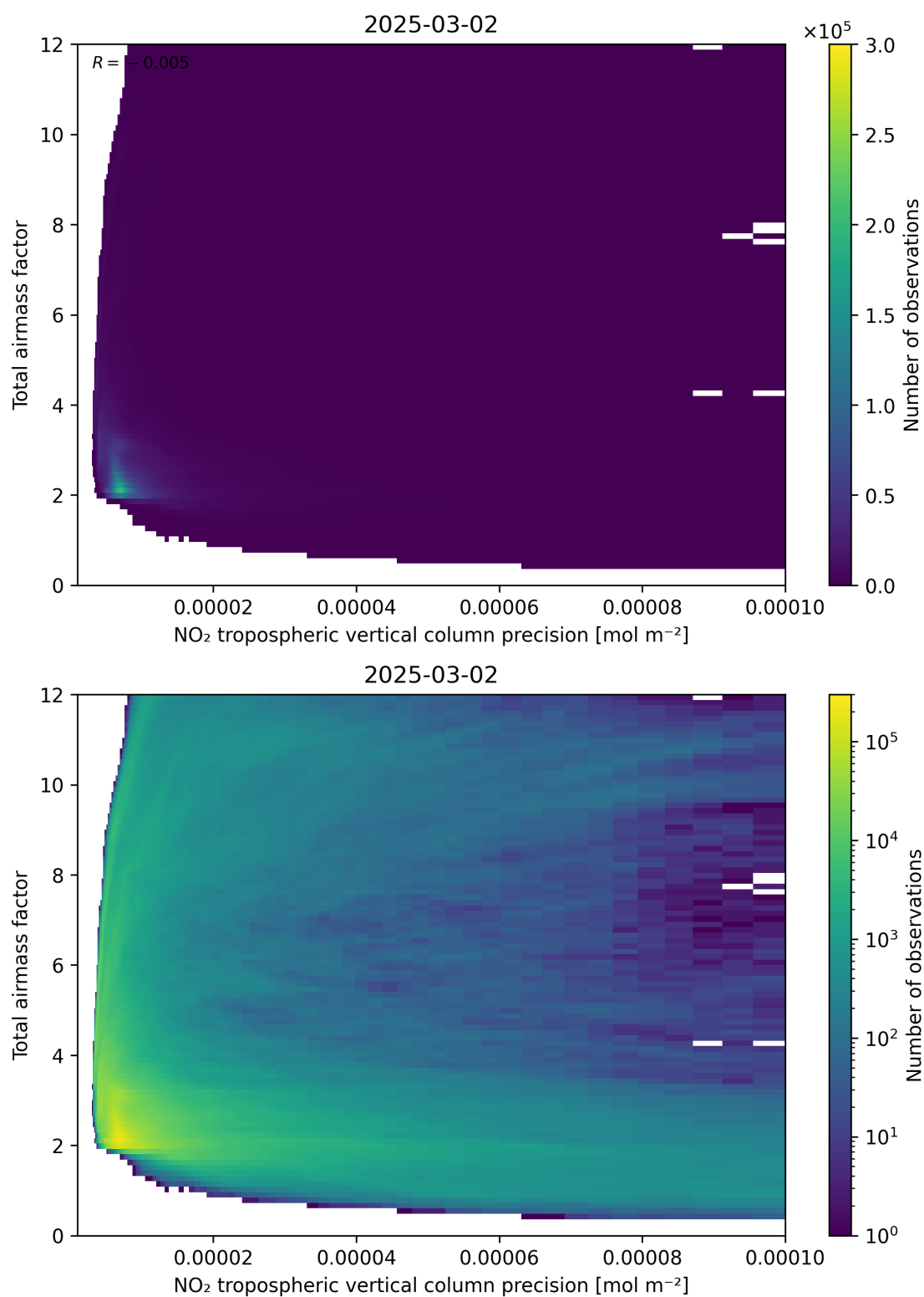
Figure 132: Scatter density plot of “NO 2 tropospheric vertical column precision” against “Total air mass factor” for 2025-03-01 to 2025-03-03.
