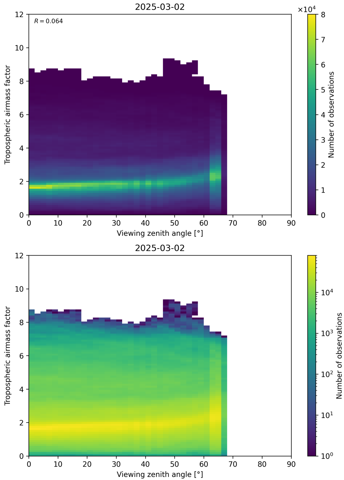
Figure 161: Scatter density plot of “Viewing zenith angle” against “Tropospheric airmass factor” for 2025-03-01 to 2025-03-03.
