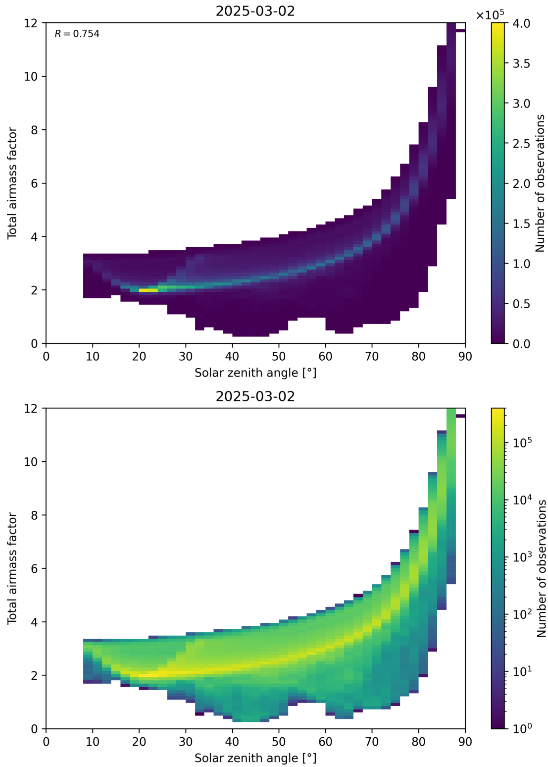
Figure 146: Scatter density plot of “Solar zenith angle” against “Total air mass factor” for 2025-03-01 to 2025-03-03.
