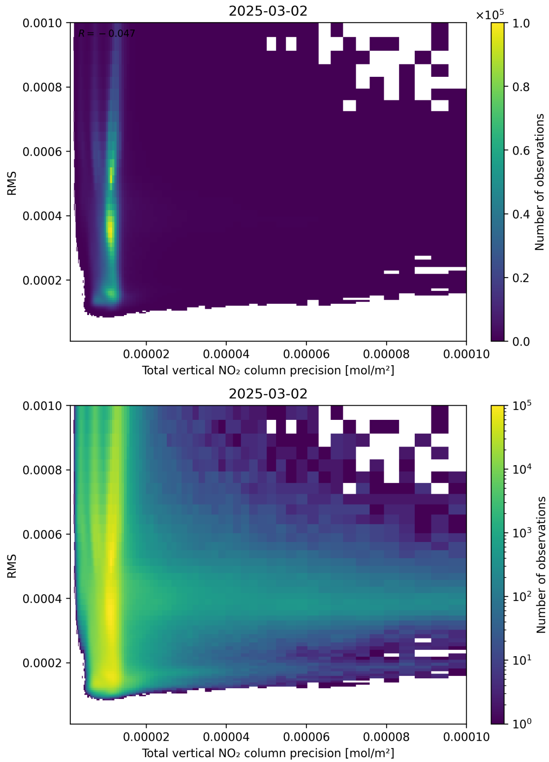
Figure 119: Scatter density plot of “Total vertical NO 2 column precision” against “RMS” for 2025-03-01 to 2025-03-03.
