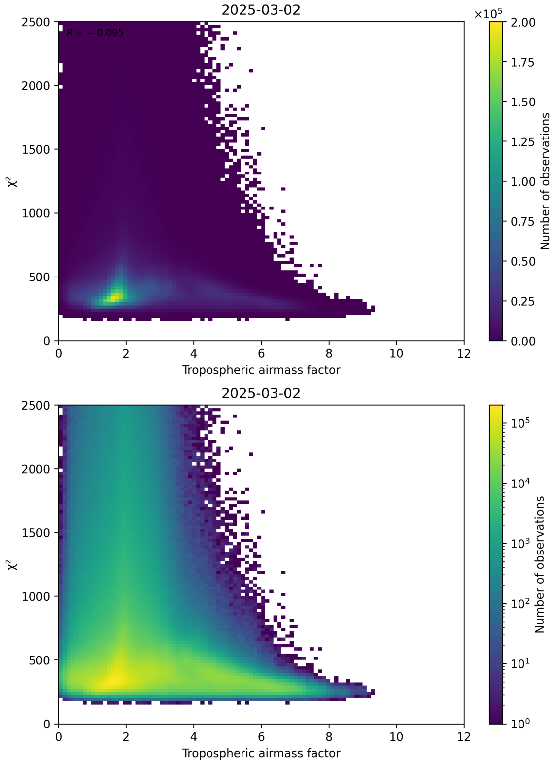
Figure 73: Scatter density plot of “Tropospheric airmass factor” against “ \chi^2 ” for 2025-03-01 to 2025-03-03.
