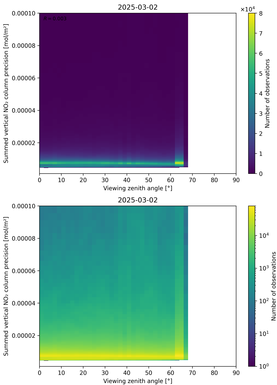
Figure 166: Scatter density plot of “Viewing zenith angle” against “Summed vertical NO 2 column precision” for 2025-03-01 to 2025-03-03.
