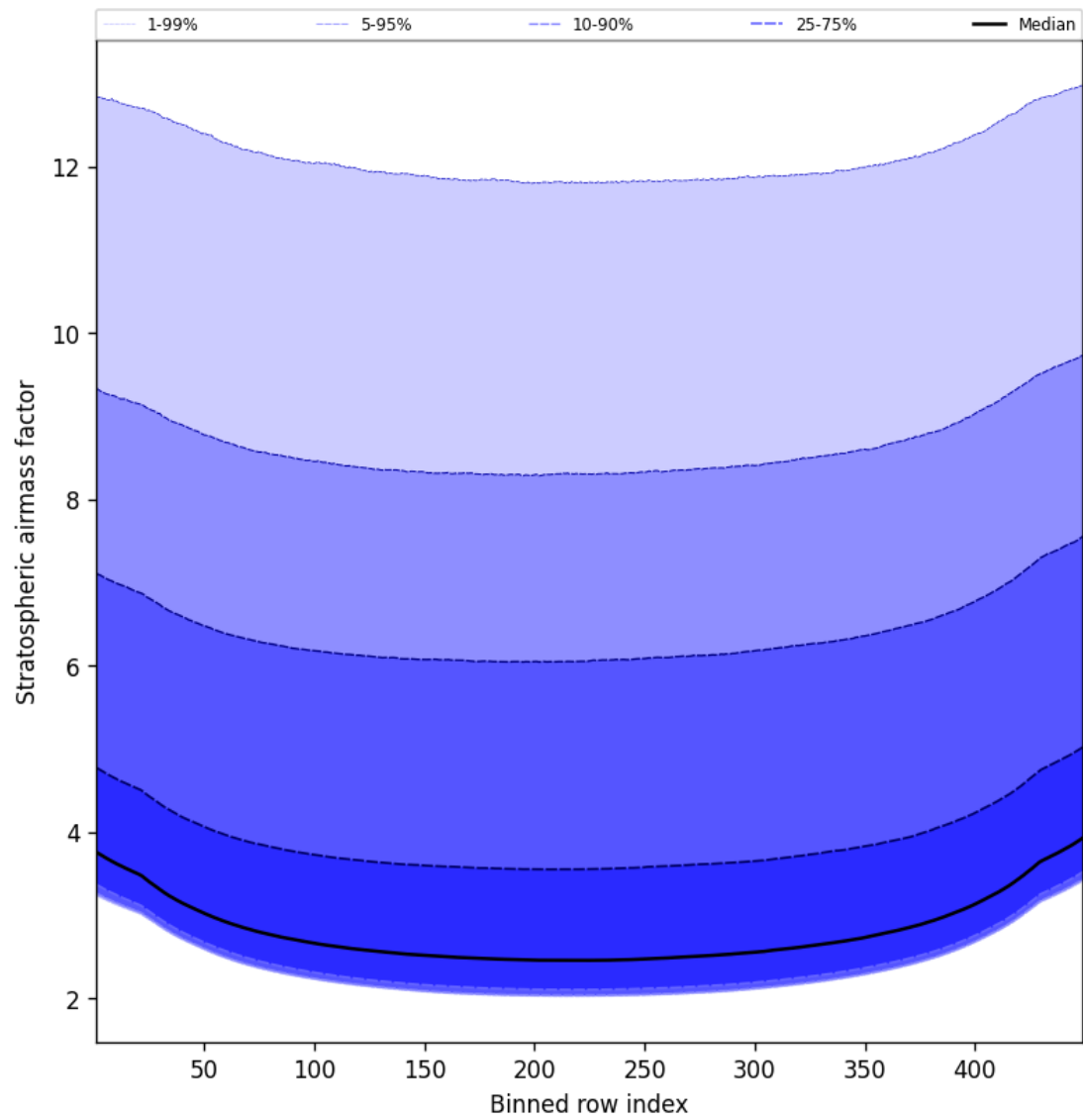
Figure 61: Along track statistics of “Stratospheric air mass factor” for 2025-03-01 to 2025-03-03
