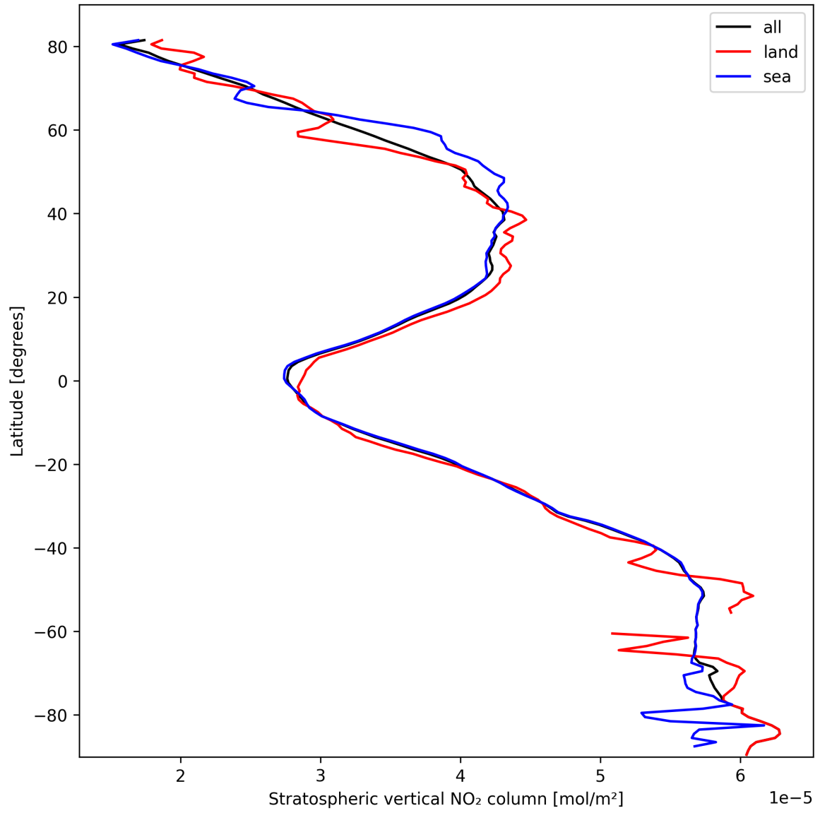
Figure 19: Zonal average of “Stratospheric vertical NO 2 column” for 2025-03-01 to 2025-03-03.
