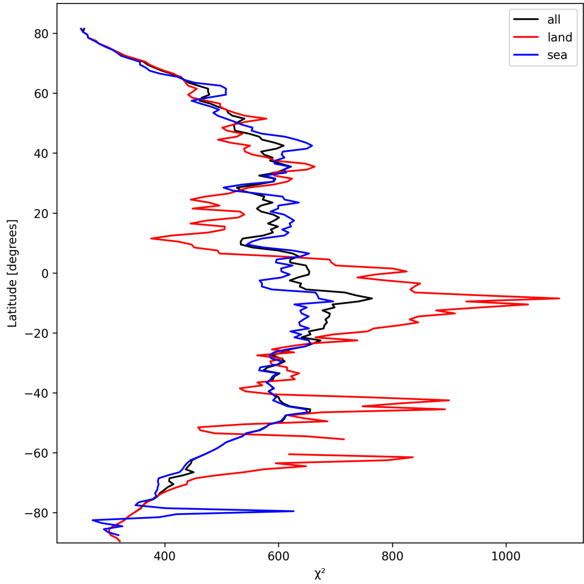
Figure 25: Zonal average of “ \chi^2 ” for 2025-03-01 to 2025-03-03.
