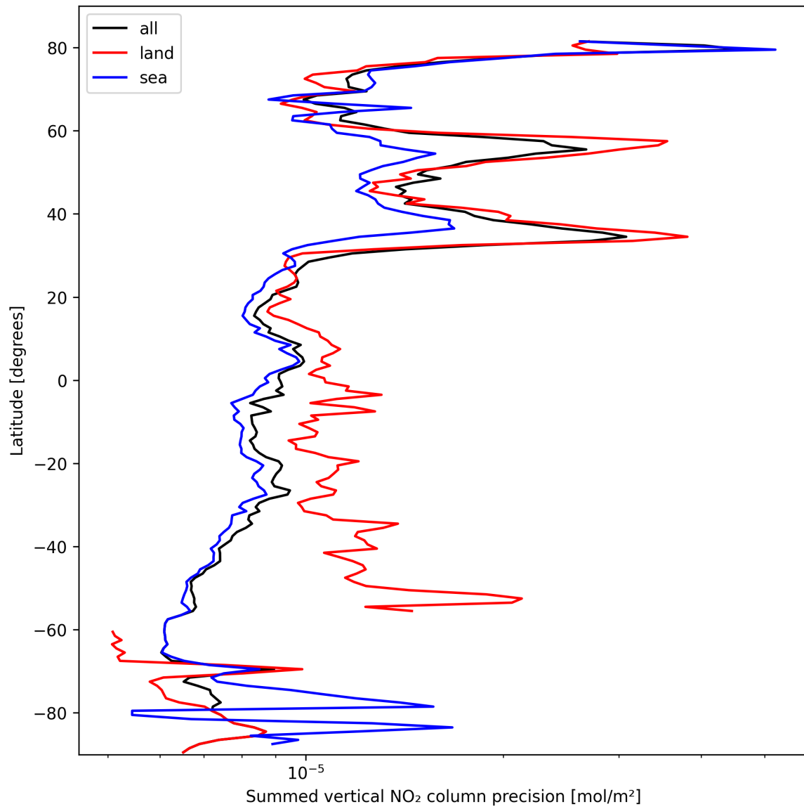
Figure 24: Zonal average of “Summed vertical NO 2 column precision” for 2025-03-01 to 2025-03-03.
