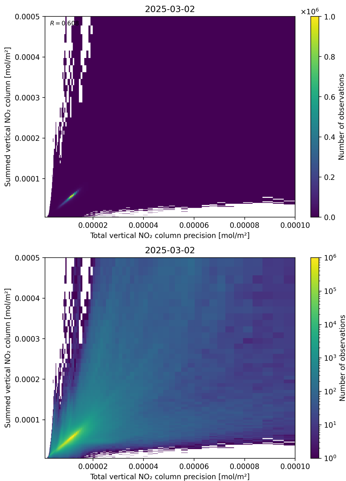
Figure 117: Scatter density plot of “Total vertical NO 2 column precision” against “Summed vertical NO 2 column” for 2025-03-01 to 2025-03-03.
