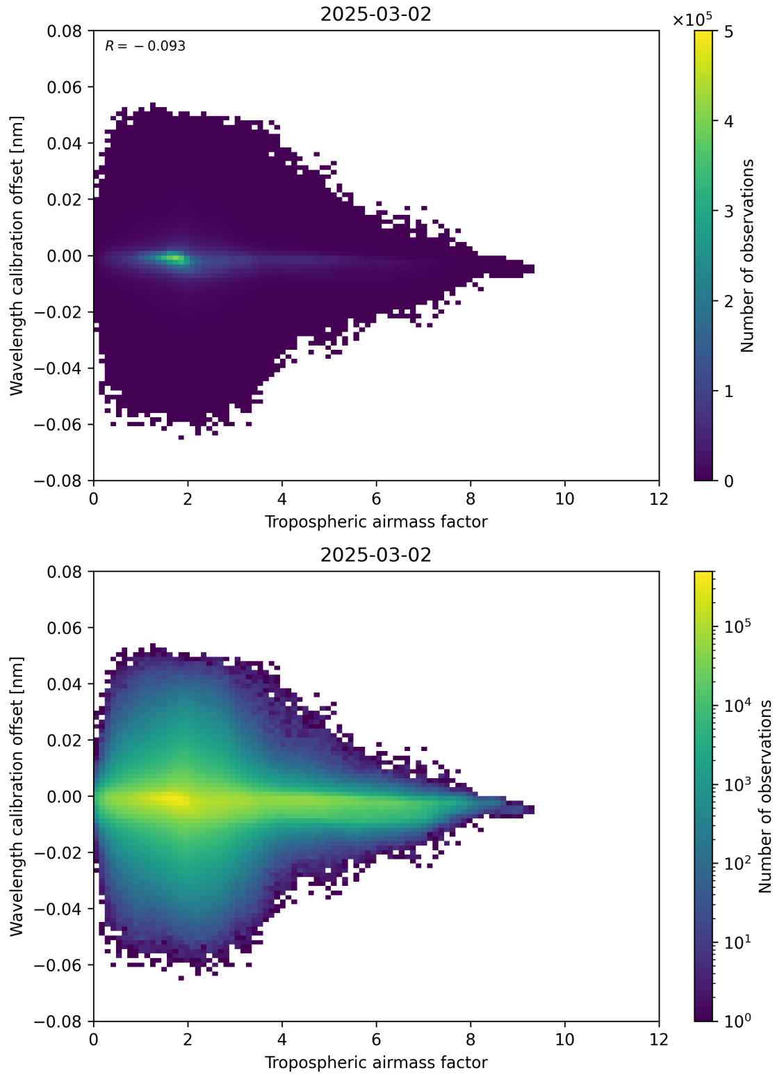
Figure 80: Scatter density plot of “Tropospheric airmass factor” against “Wavelength calibration offset” for 2025-03-01 to 2025-03-03.
