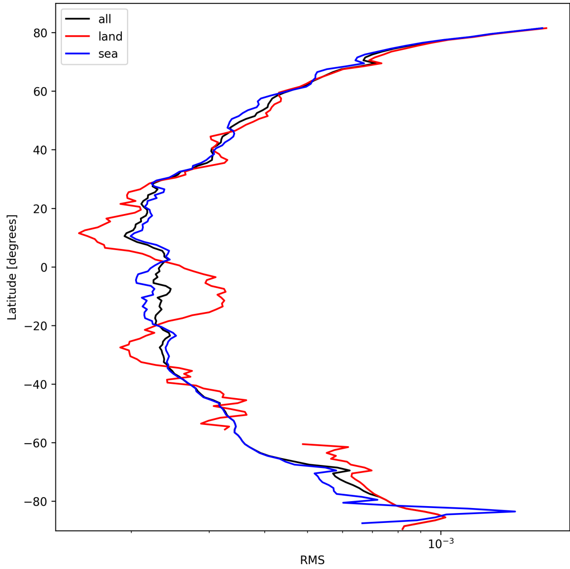
Figure 26: Zonal average of “RMS” for 2025-03-01 to 2025-03-03.
