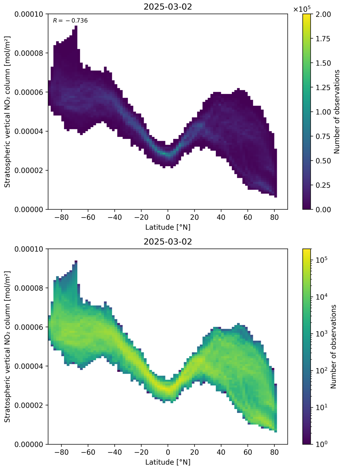
Figure 87: Scatter density plot of “Latitude” against “Stratospheric vertical NO 2 column” for 2025-03-01 to 2025-03-03.
