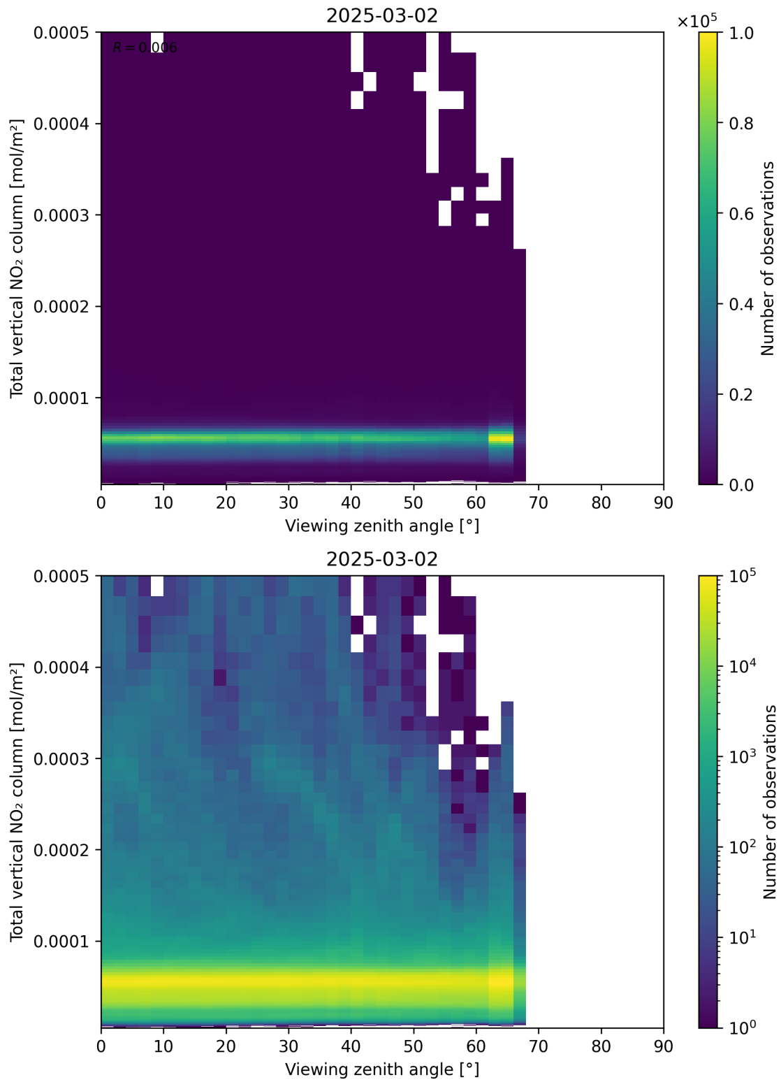
Figure 167: Scatter density plot of “Viewing zenith angle” against “Total vertical NO 2 column” for 2025-03-01 to 2025-03-03.
