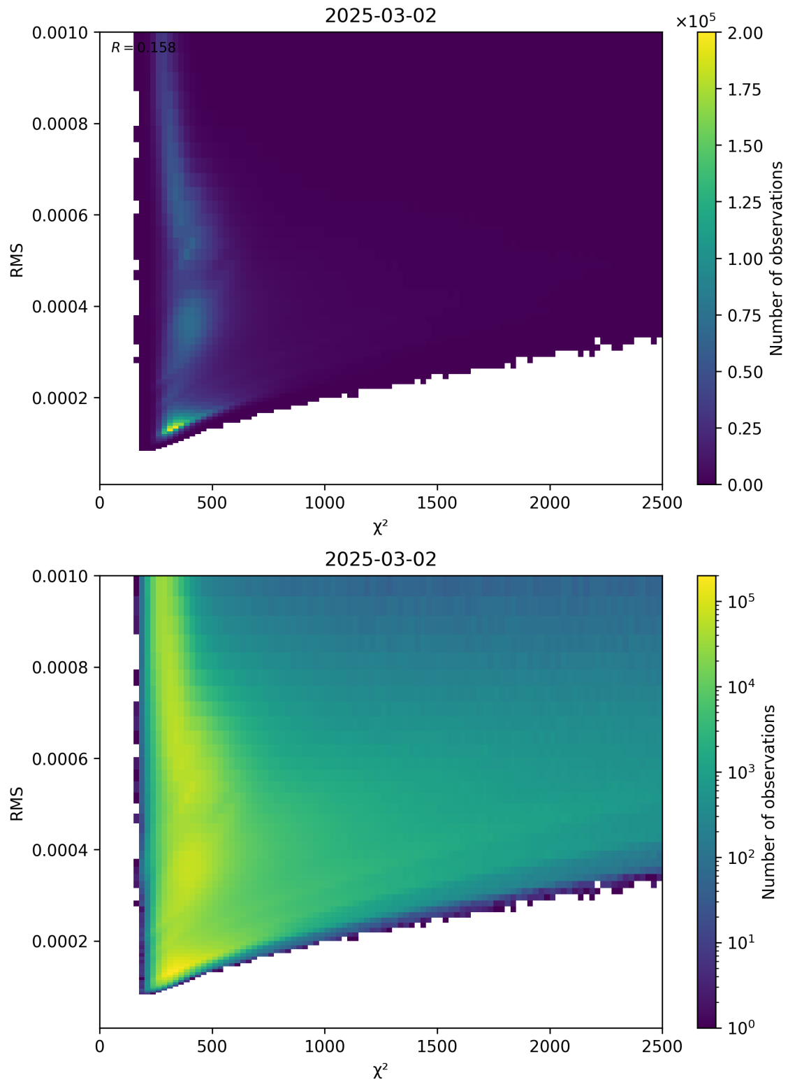
Figure 82: Scatter density plot of “ \chi^2 ” against “RMS” for 2025-03-01 to 2025-03-03.
