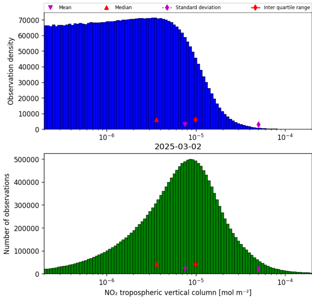
Figure 29: Histogram of “NO 2 tropospheric vertical column” for 2025-03-01 to 2025-03-03
