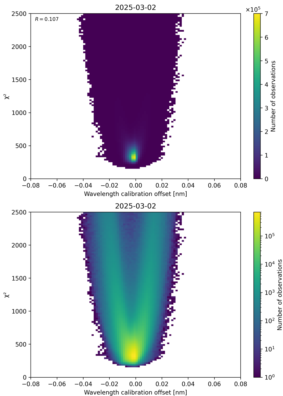
Figure 175: Scatter density plot of “Wavelength calibration offset” against “ \chi^2 ” for 2025-03-01 to 2025-03-03.
