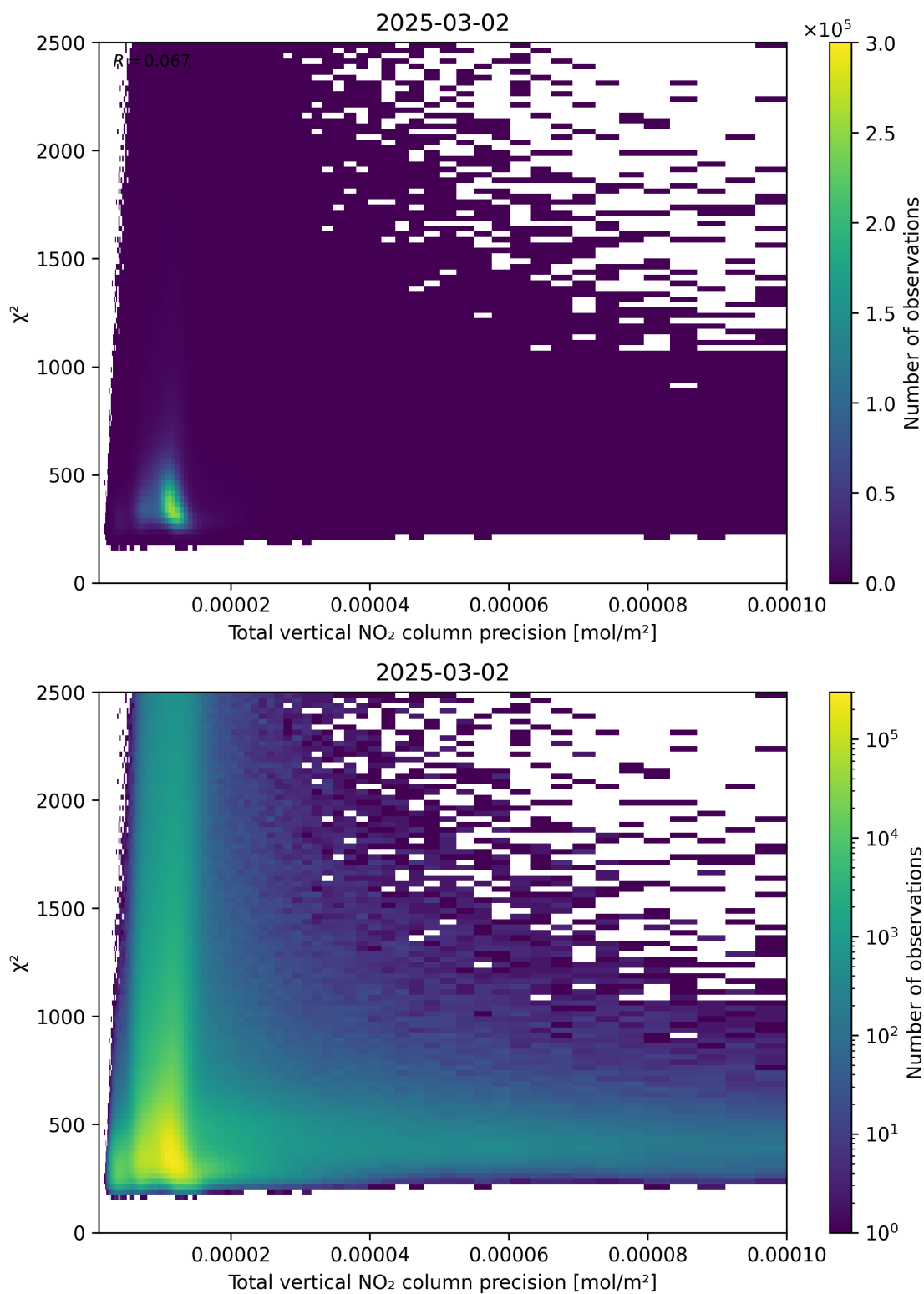
Figure 116: Scatter density plot of “Total vertical NO 2 column precision” against “ \chi^2 ” for 2025-03-01 to 2025-03-03.
