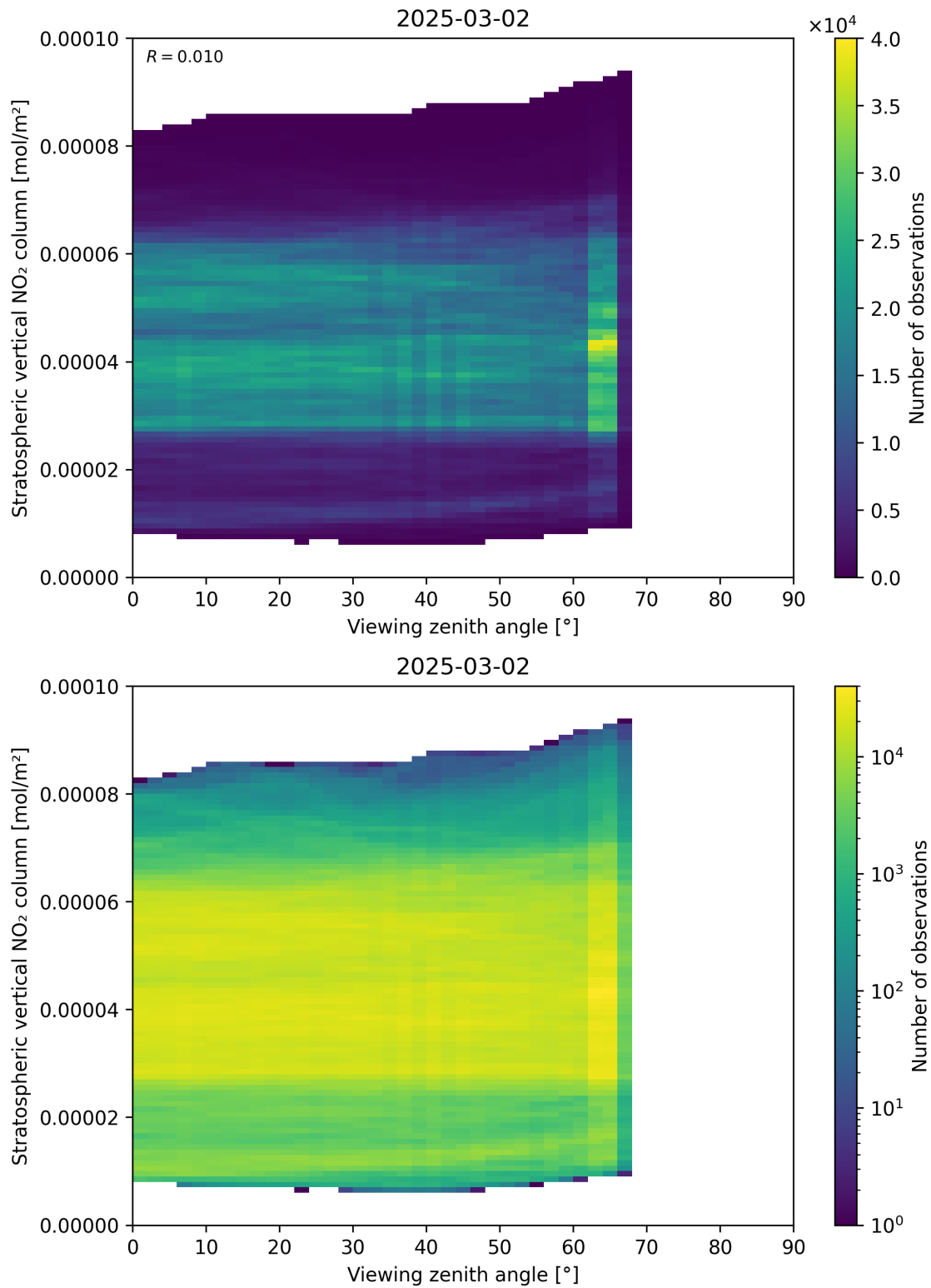
Figure 164: Scatter density plot of “Viewing zenith angle” against “Stratospheric vertical NO 2 column” for 2025-03-01 to 2025-03-03.
