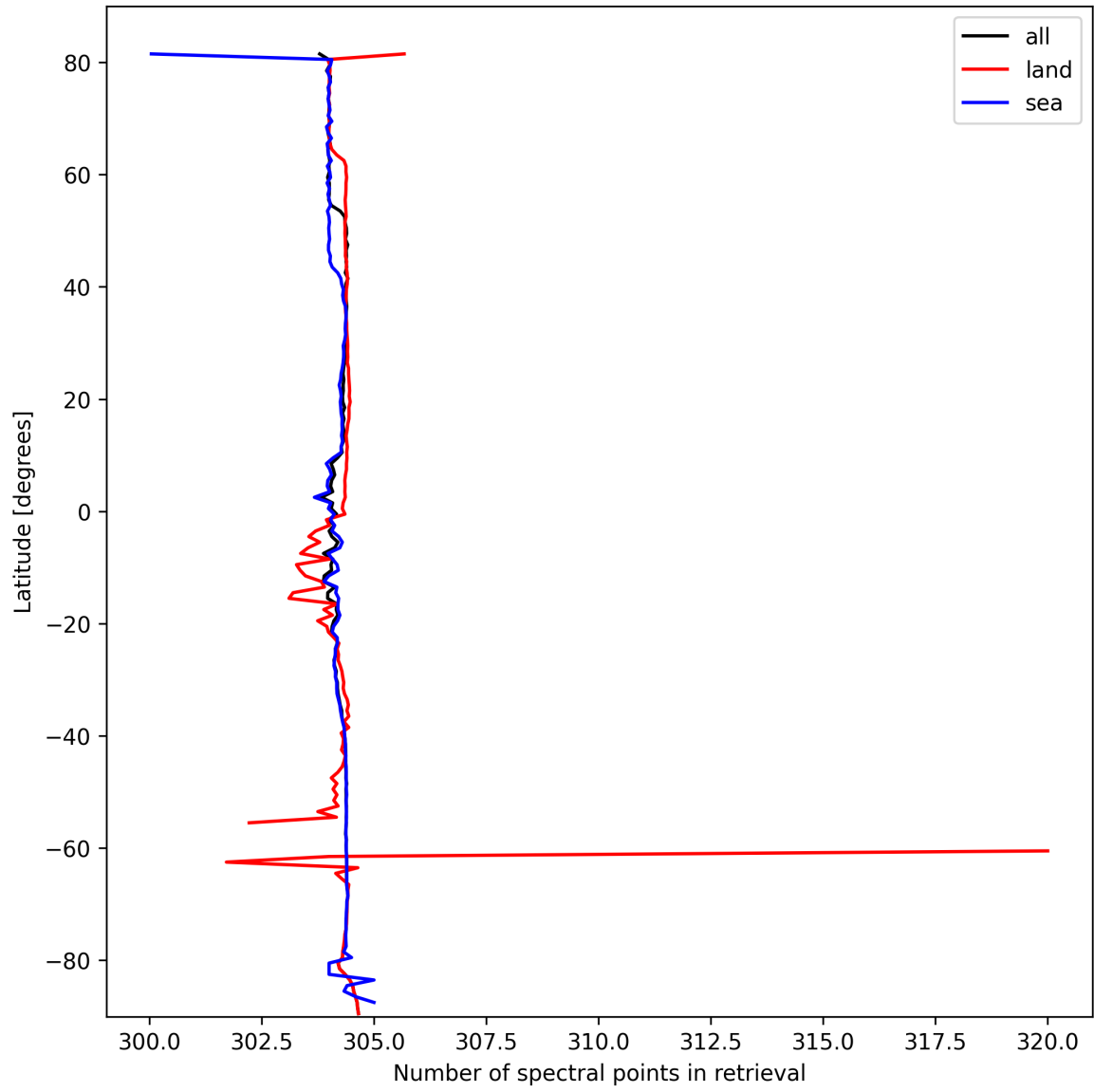
Figure 16: Zonal average of “Number of spectral points in retrieval” for 2025-03-01 to 2025-03-03.
