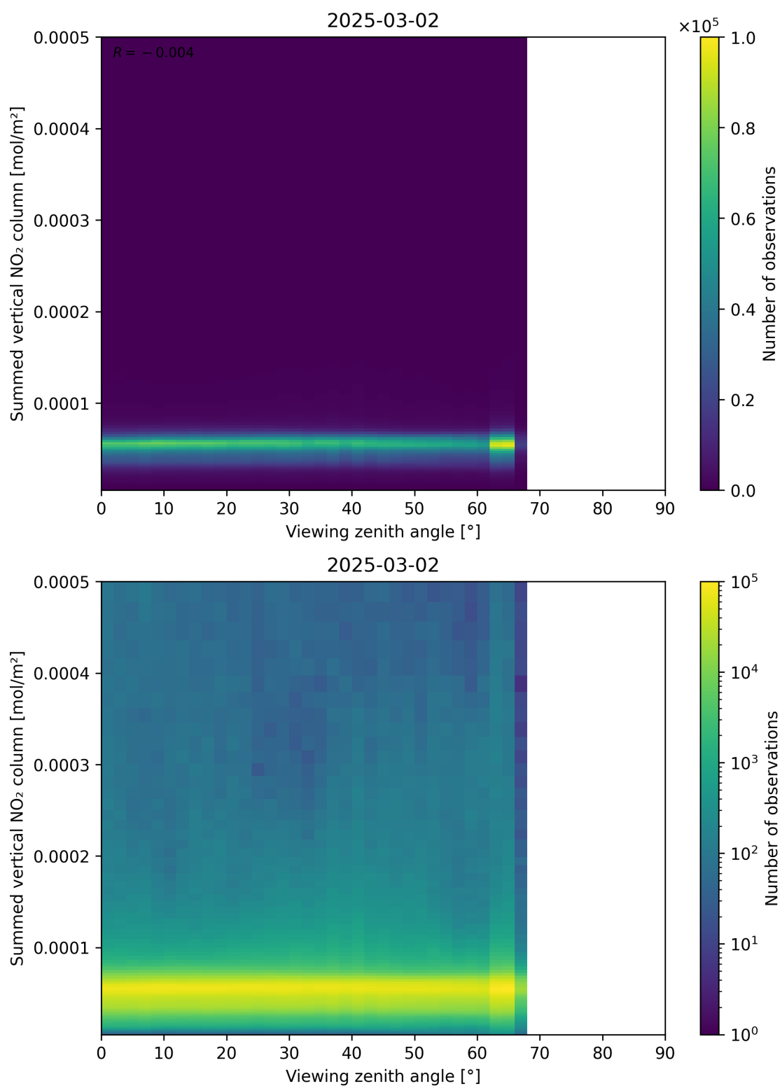
Figure 165: Scatter density plot of “Viewing zenith angle” against “Summed vertical NO 2 column” for 2025-03-01 to 2025-03-03.
