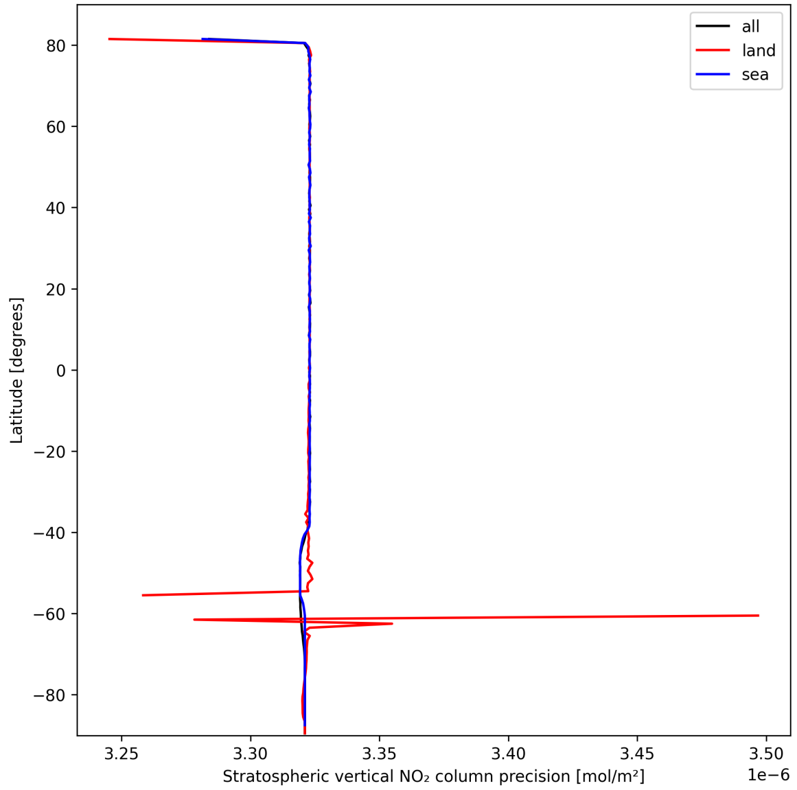
Figure 20: Zonal average of “Stratospheric vertical NO 2 column precision” for 2025-03-01 to 2025-03-03.
