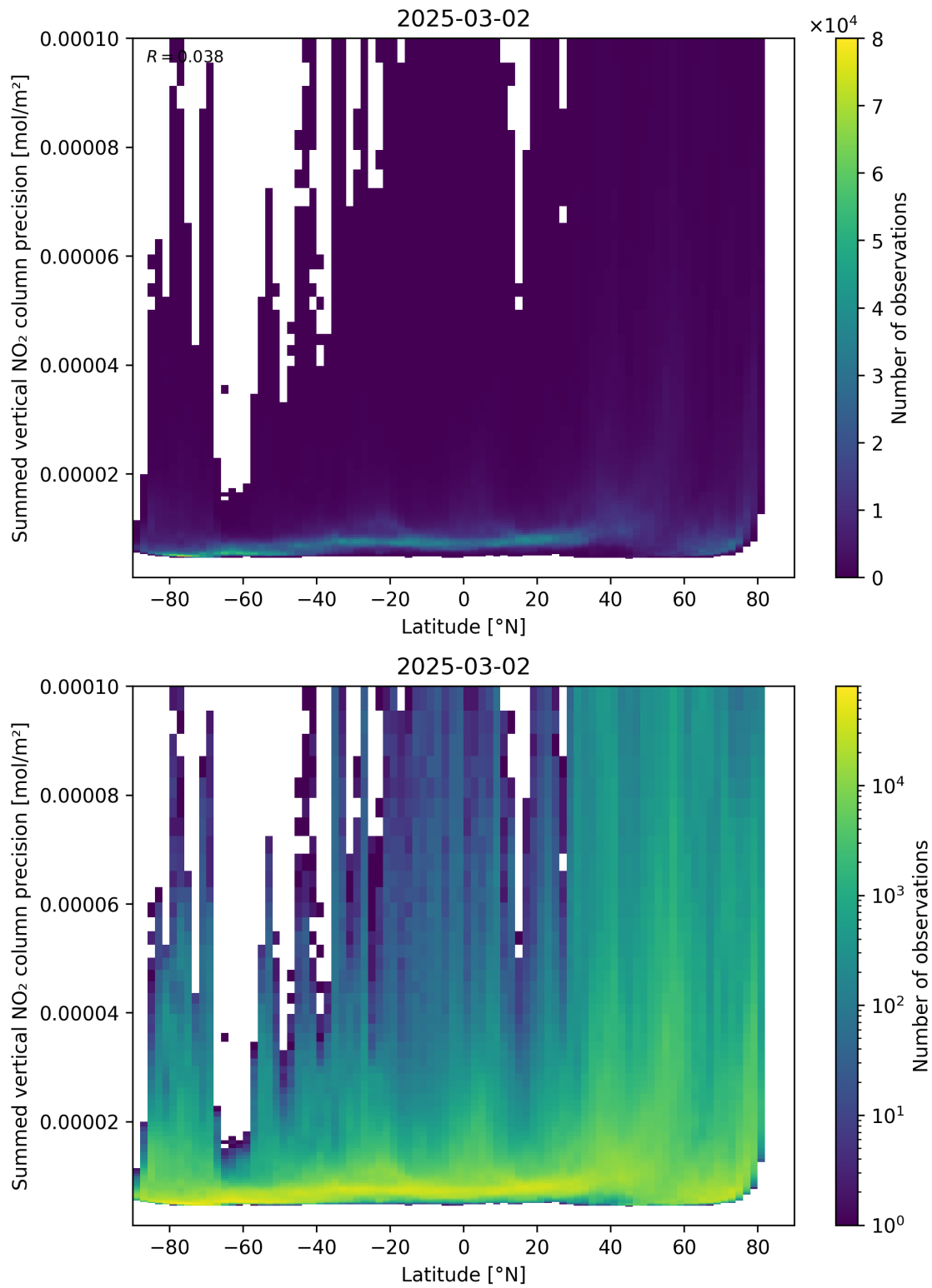
Figure 89: Scatter density plot of “Latitude” against “Summed vertical NO 2 column precision” for 2025-03-01 to 2025-03-03.
