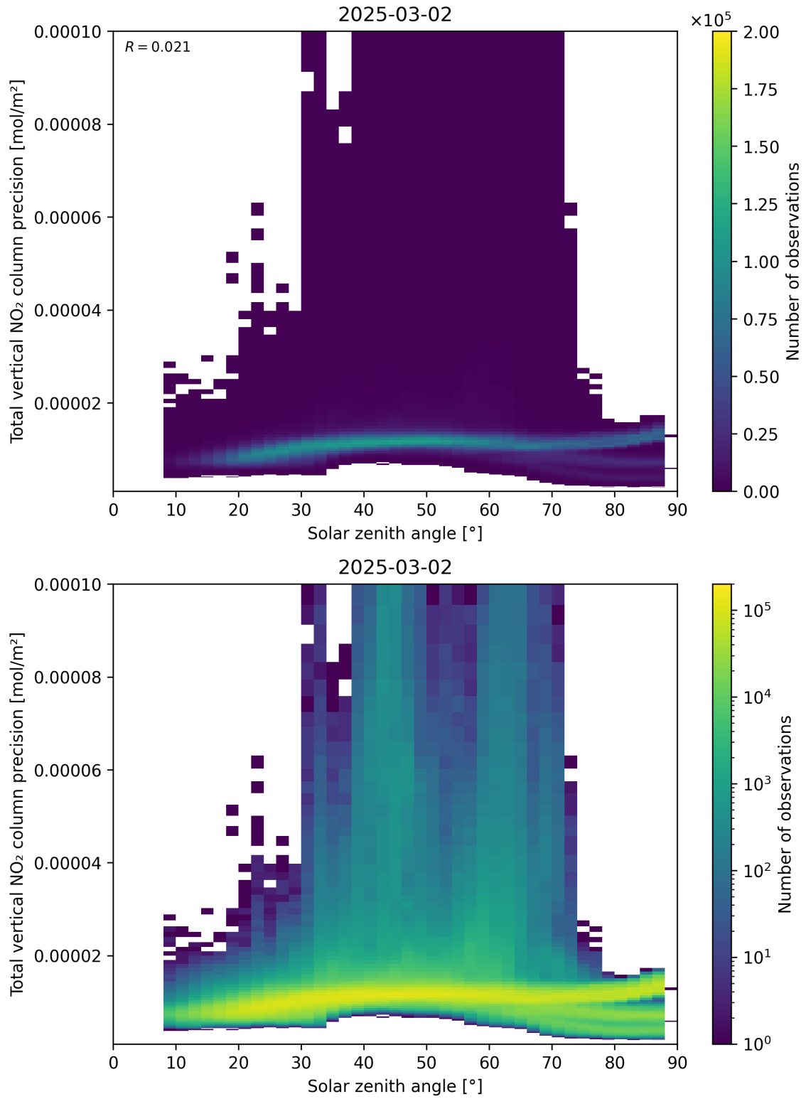
Figure 154: Scatter density plot of “Solar zenith angle” against “Total vertical NO 2 column precision” for 2025-03-01 to 2025-03-03.
