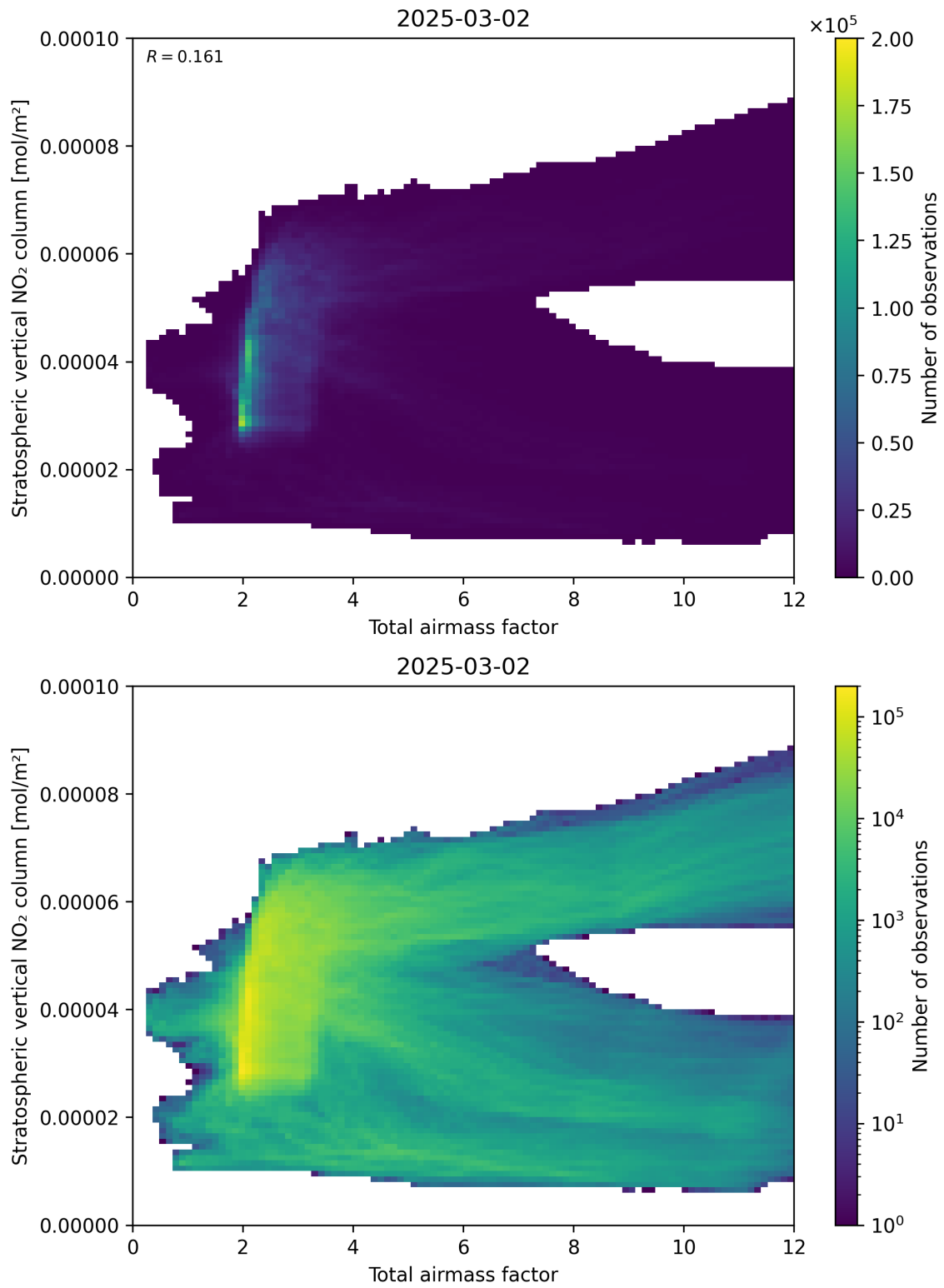
Figure 64: Scatter density plot of “Total airmass factor” against “Stratospheric vertical NO 2 column” for 2025-03-01 to 2025-03-03.
