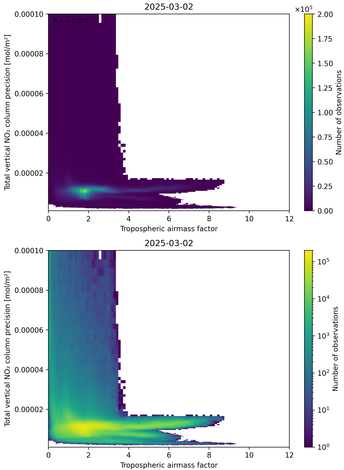
Figure 78: Scatter density plot of “Tropospheric airmass factor” against “Total vertical NO 2 column precision” for 2025-03-01 to 2025-03-03.
