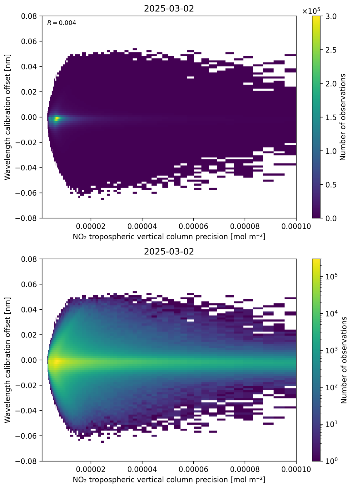
Figure 141: Scatter density plot of “NO 2 tropospheric vertical column precision” against “Wavelength calibration offset” for 2025-03-01 to 2025-03-03.
