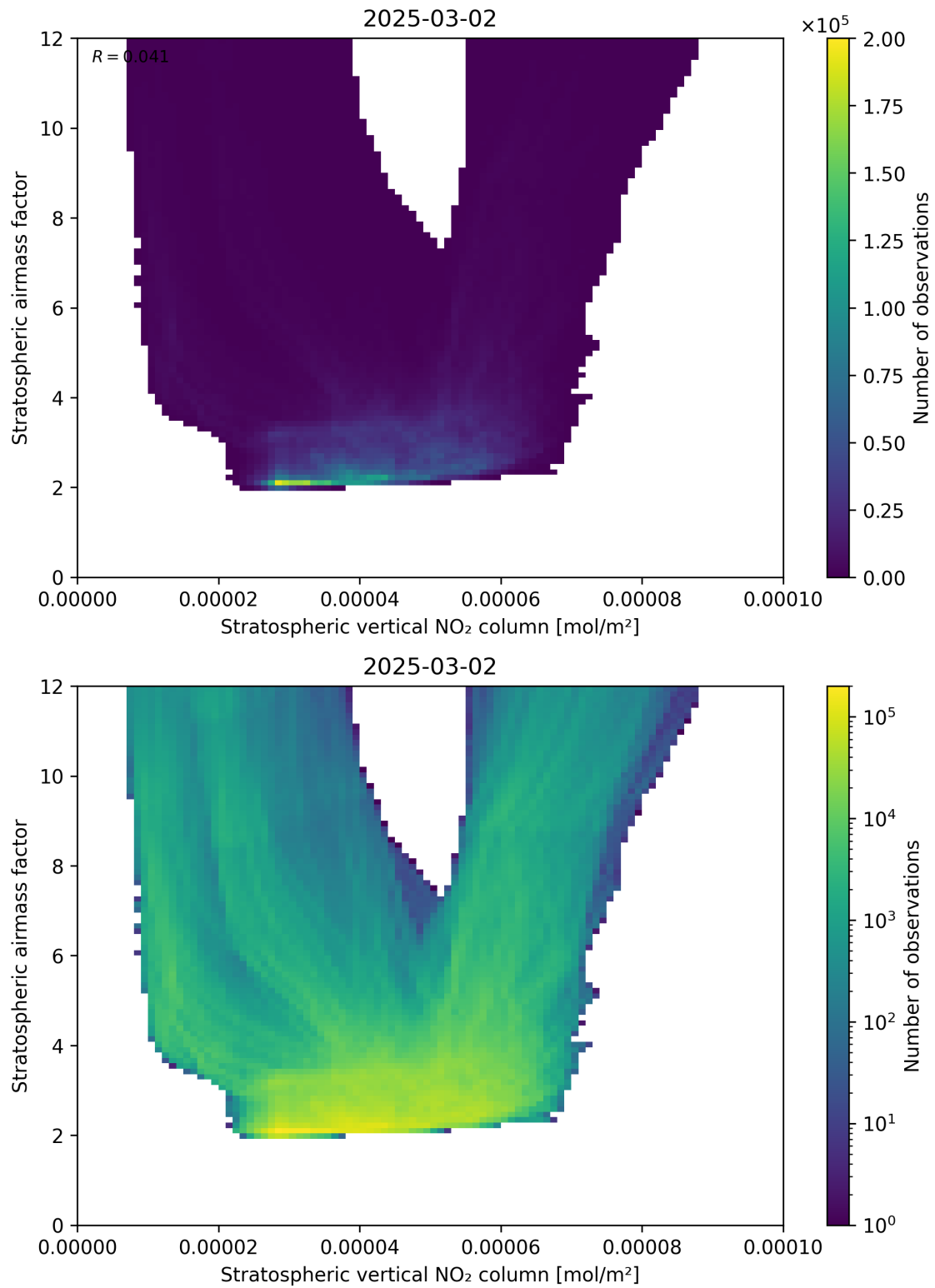
Figure 96: Scatter density plot of “Stratospheric vertical NO 2 column” against “Stratospheric airmass factor” for 2025-03-01 to 2025-03-03.
