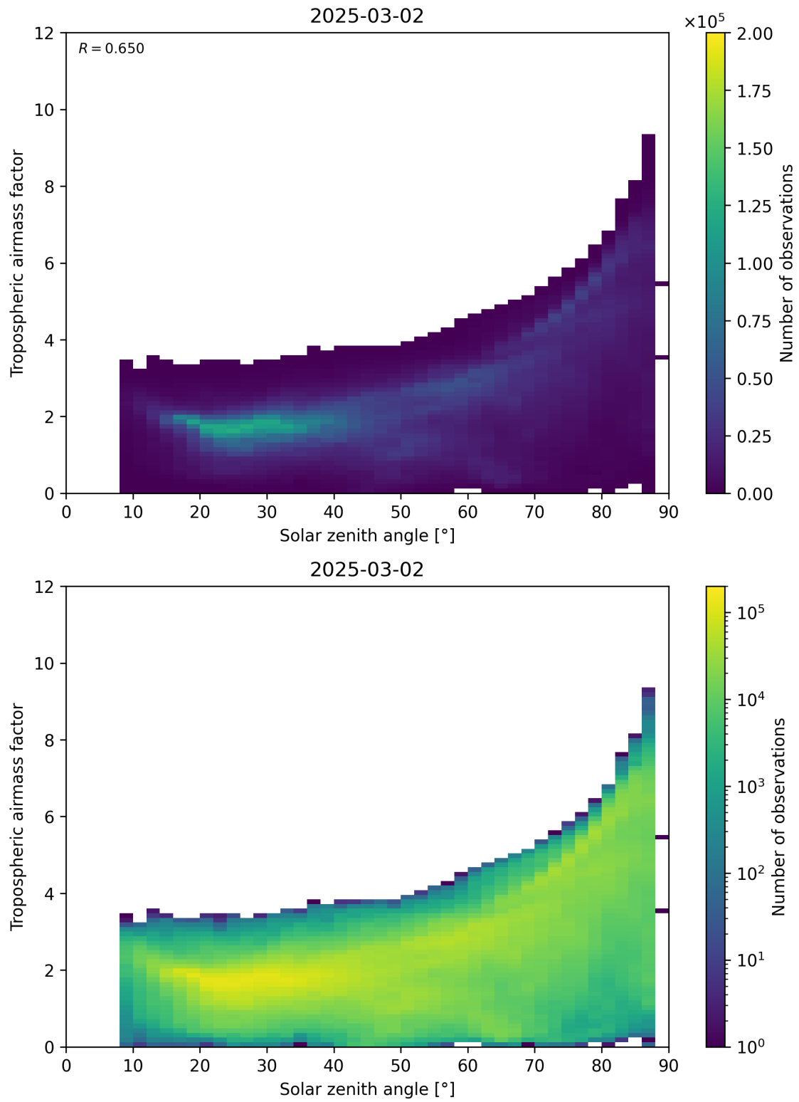
Figure 147: Scatter density plot of “Solar zenith angle” against “Tropospheric airmass factor” for 2025-03-01 to 2025-03-03.
