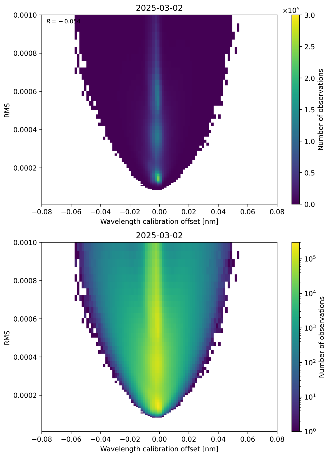
Figure 181: Scatter density plot of “Wavelength calibration offset” against “RMS” for 2025-03-01 to 2025-03-03.
