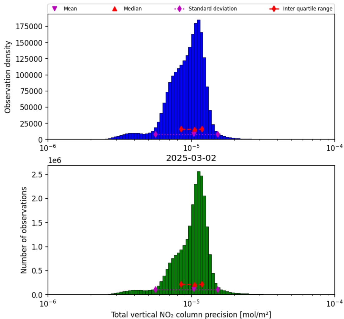
Figure 39: Histogram of “Total vertical NO 2 column precision” for 2025-03-01 to 2025-03-03
