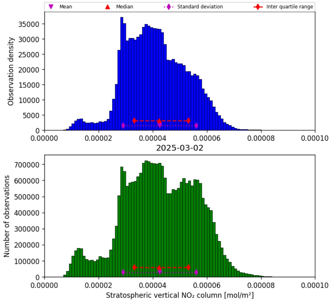
Figure 36: Histogram of “Stratospheric vertical NO 2 column” for 2025-03-01 to 2025-03-03
