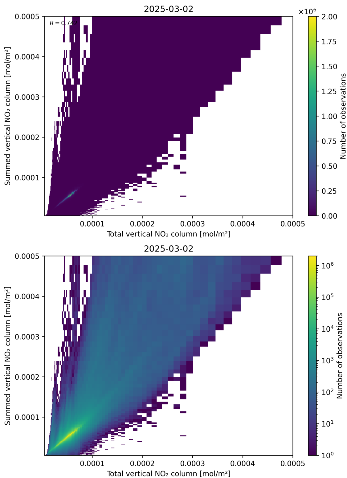
Figure 112: Scatter density plot of “Total vertical NO 2 column” against “Summed vertical NO 2 column” for 2025-03-01 to 2025-03-03.
