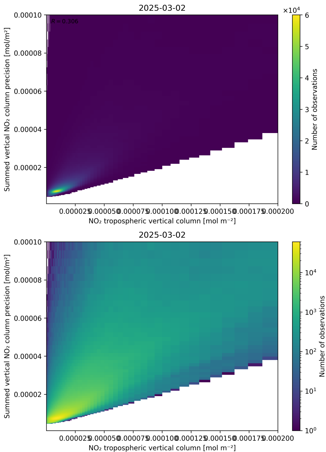
Figure 127: Scatter density plot of “NO 2 tropospheric vertical column” against “Summed vertical NO 2 column precision” for 2025-03-01 to 2025-03-03.
