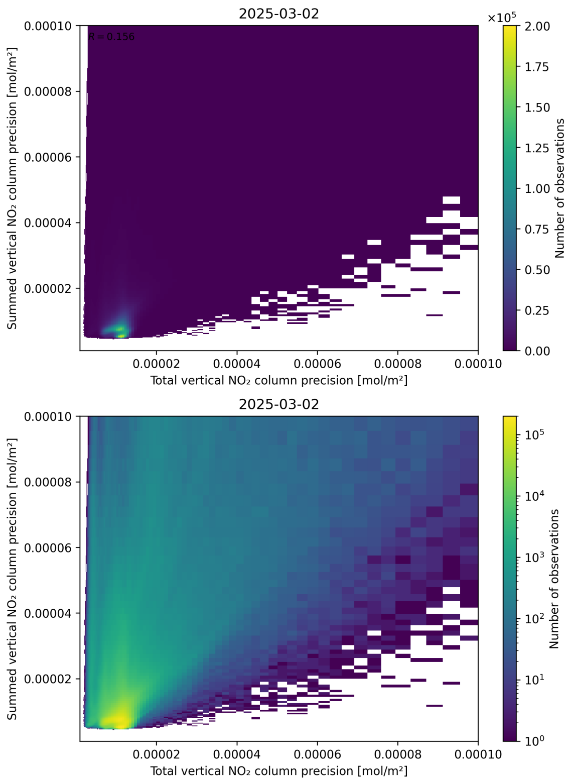
Figure 118: Scatter density plot of “Total vertical NO 2 column precision” against “Summed vertical NO 2 column precision” for 2025-03-01 to 2025-03-03.
