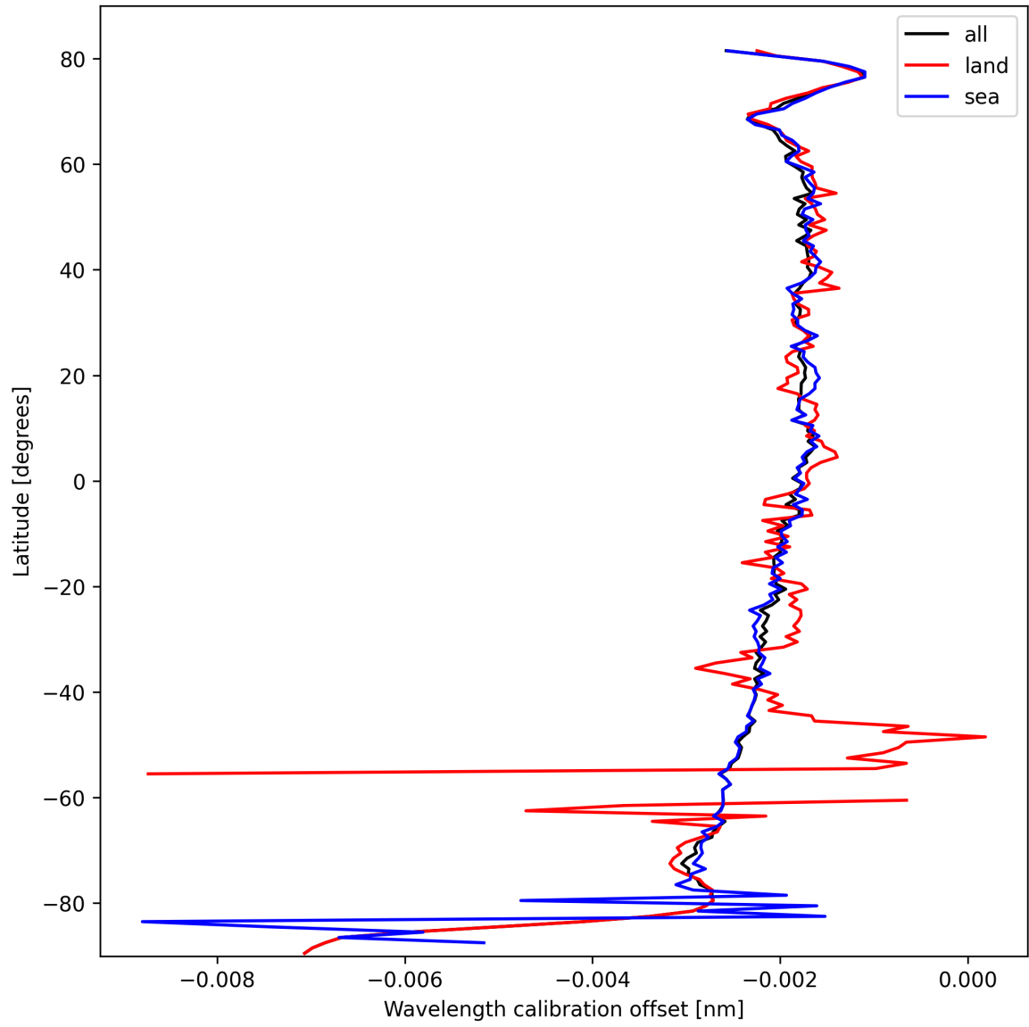
Figure 18: Zonal average of “Wavelength calibration offset” for 2025-03-01 to 2025-03-03.
