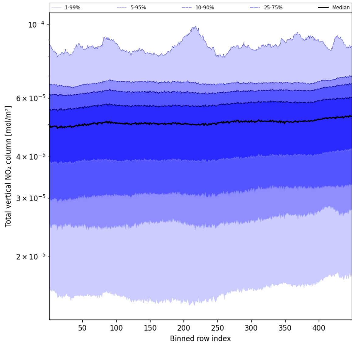
Figure 55: Along track statistics of “Total vertical NO 2 column” for 2025-03-01 to 2025-03-03
