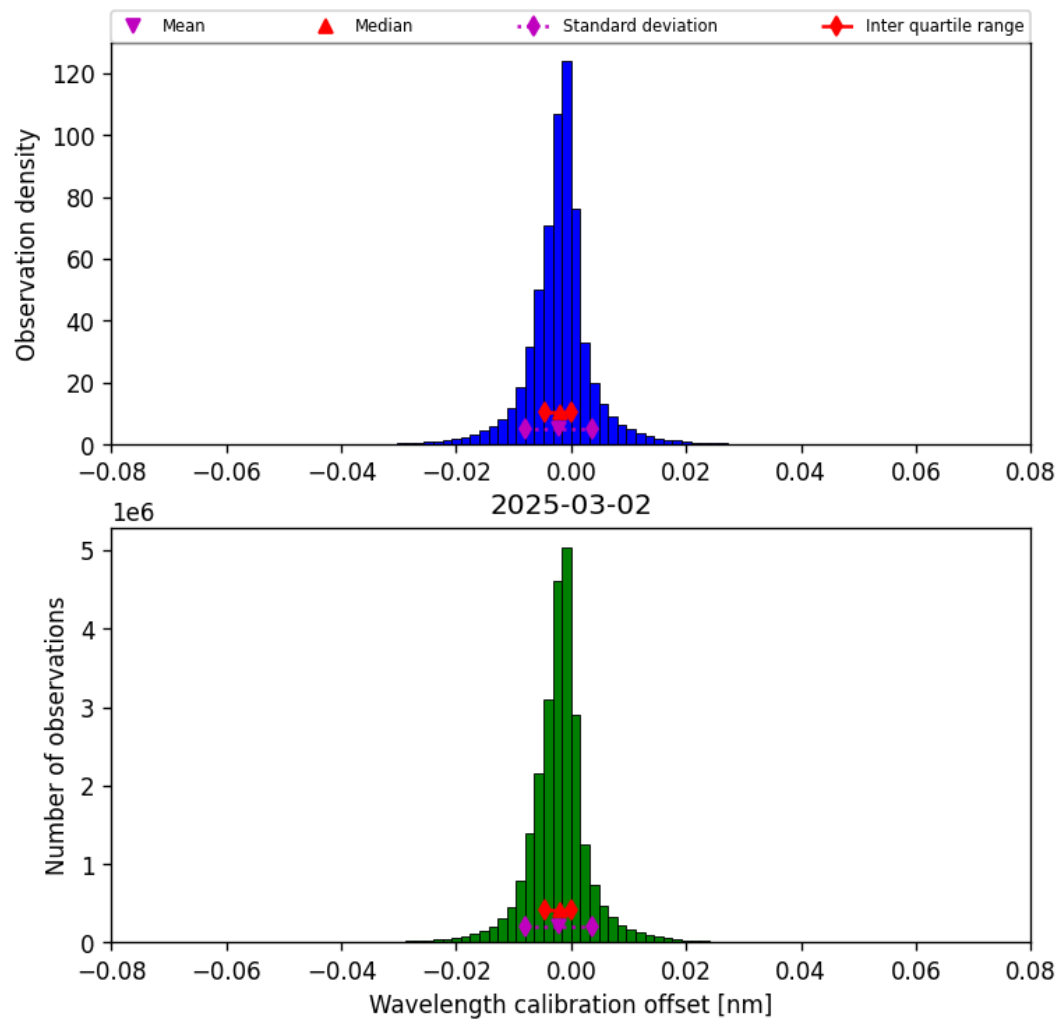
Figure 35: Histogram of “Wavelength calibration offset” for 2025-03-01 to 2025-03-03
