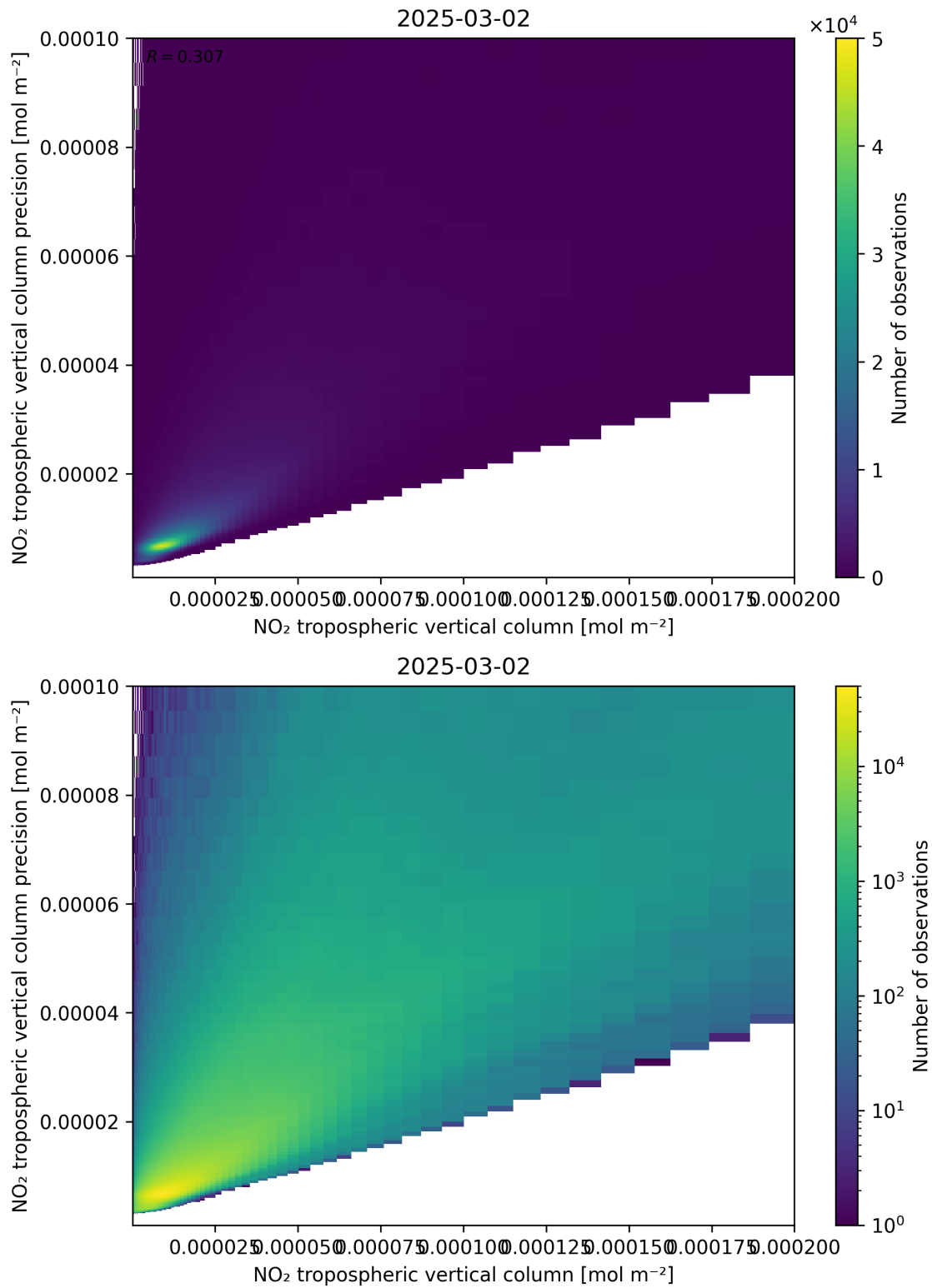
Figure 130: Scatter density plot of “NO 2 tropospheric vertical column” against “NO 2 tropospheric vertical column precision” for 2025-03-01 to 2025-03-03.
