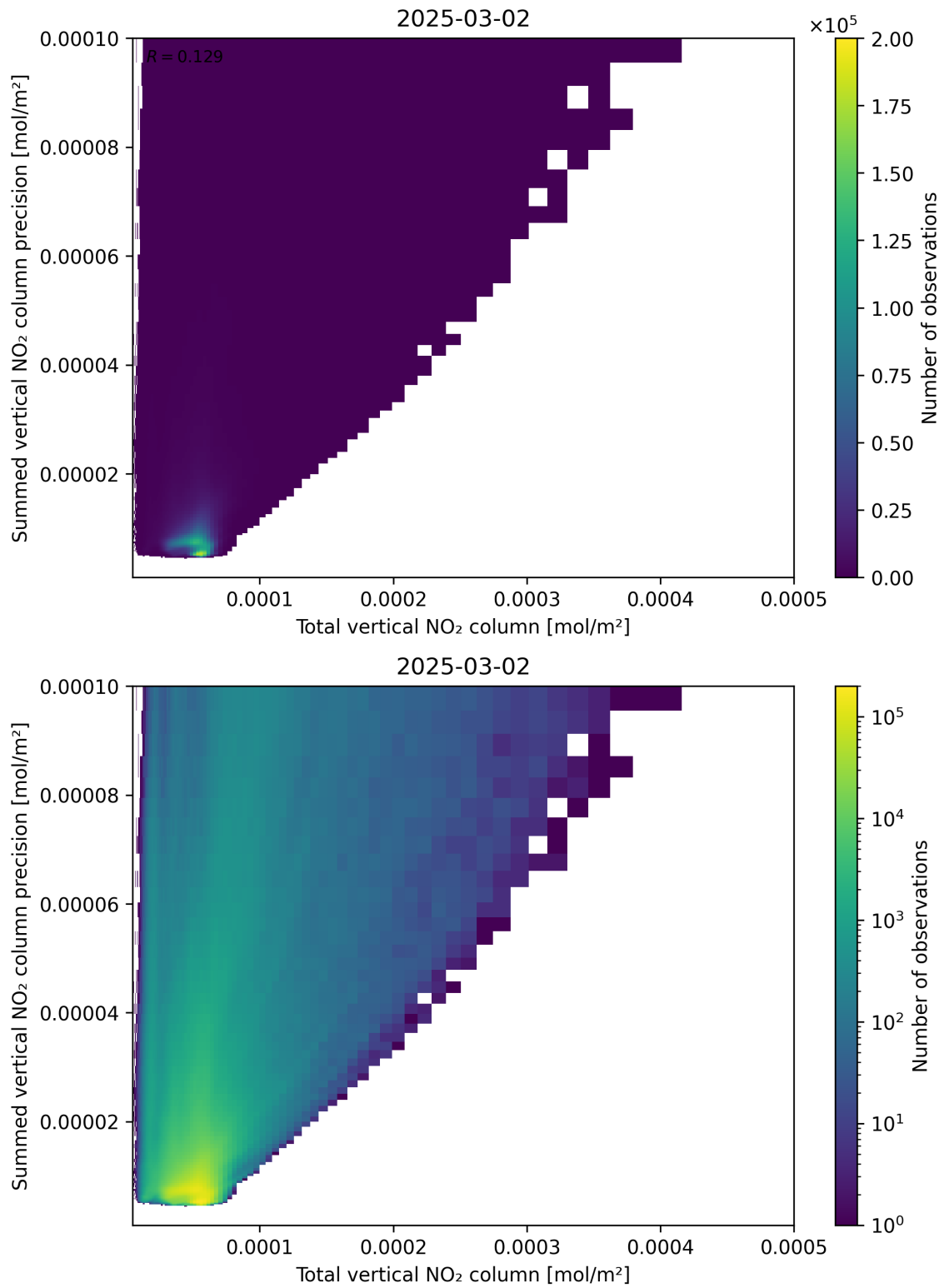
Figure 113: Scatter density plot of “Total vertical NO 2 column” against “Summed vertical NO 2 column precision” for 2025-03-01 to 2025-03-03.
