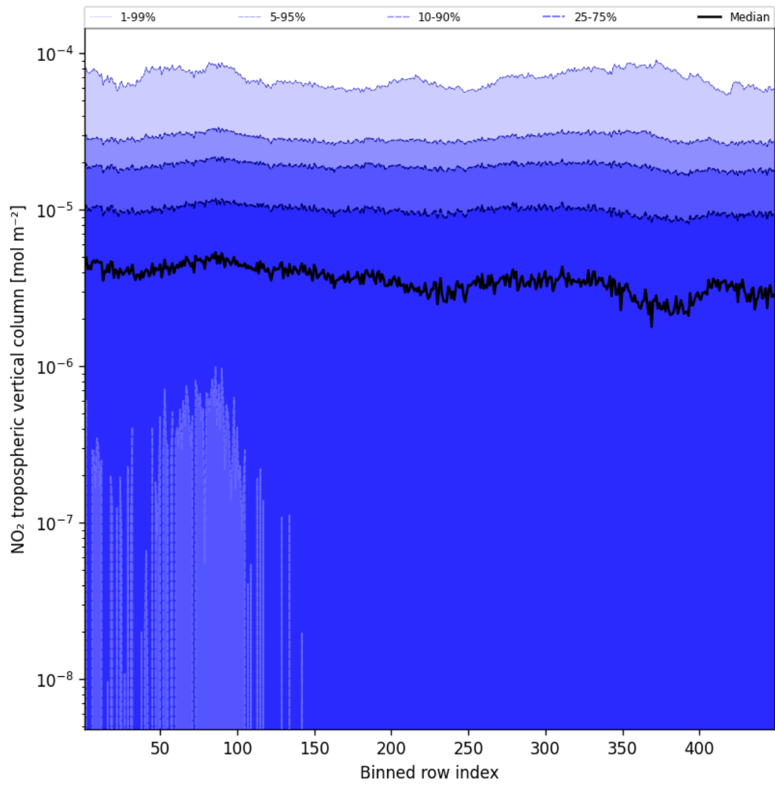
Figure 46: Along track statistics of “NO 2 tropospheric vertical column” for 2025-03-01 to 2025-03-03
