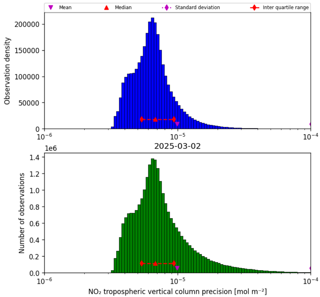
Figure 30: Histogram of “NO 2 tropospheric vertical column precision” for 2025-03-01 to 2025-03-03
