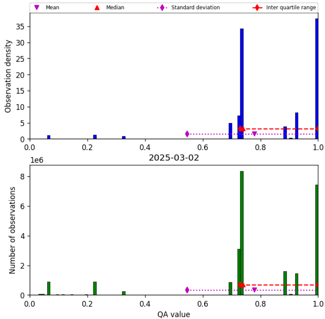
Figure 28: Histogram of “QA value” for 2025-03-01 to 2025-03-03
