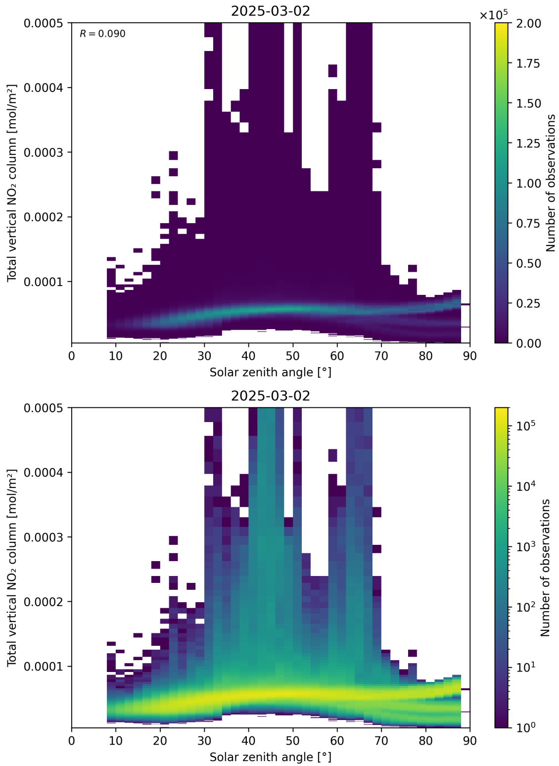
Figure 153: Scatter density plot of “Solar zenith angle” against “Total vertical NO 2 column” for 2025-03-01 to 2025-03-03.
