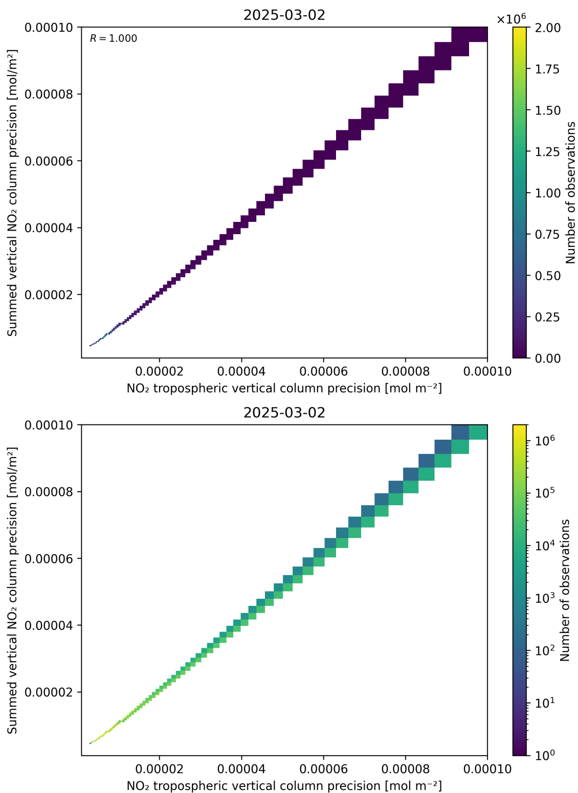
Figure 137: Scatter density plot of “NO 2 tropospheric vertical column precision” against “Summed vertical NO 2 column precision” for 2025-03-01 to 2025-03-03.
