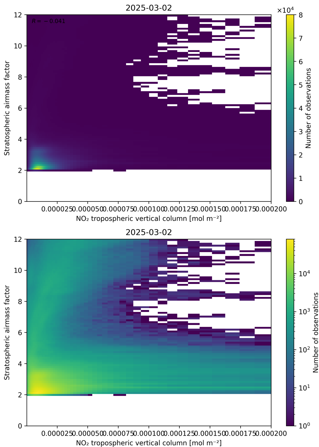
Figure 121: Scatter density plot of “NO 2 tropospheric vertical column” against “Stratospheric airmass factor” for 2025-03-01 to 2025-03-03.
