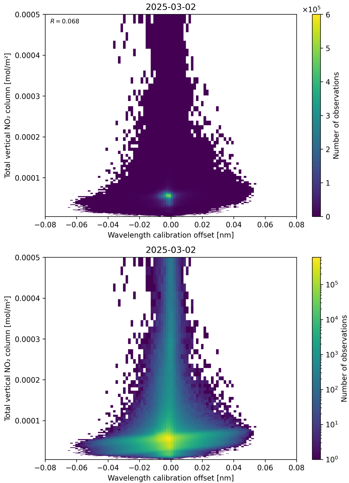
Figure 179: Scatter density plot of “Wavelength calibration offset” against “Total vertical NO 2 column” for 2025-03-01 to 2025-03-03.
