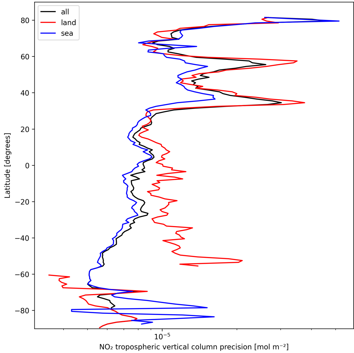
Figure 13: Zonal average of “NO 2 tropospheric vertical column precision” for 2025-03-01 to 2025-03-03.
