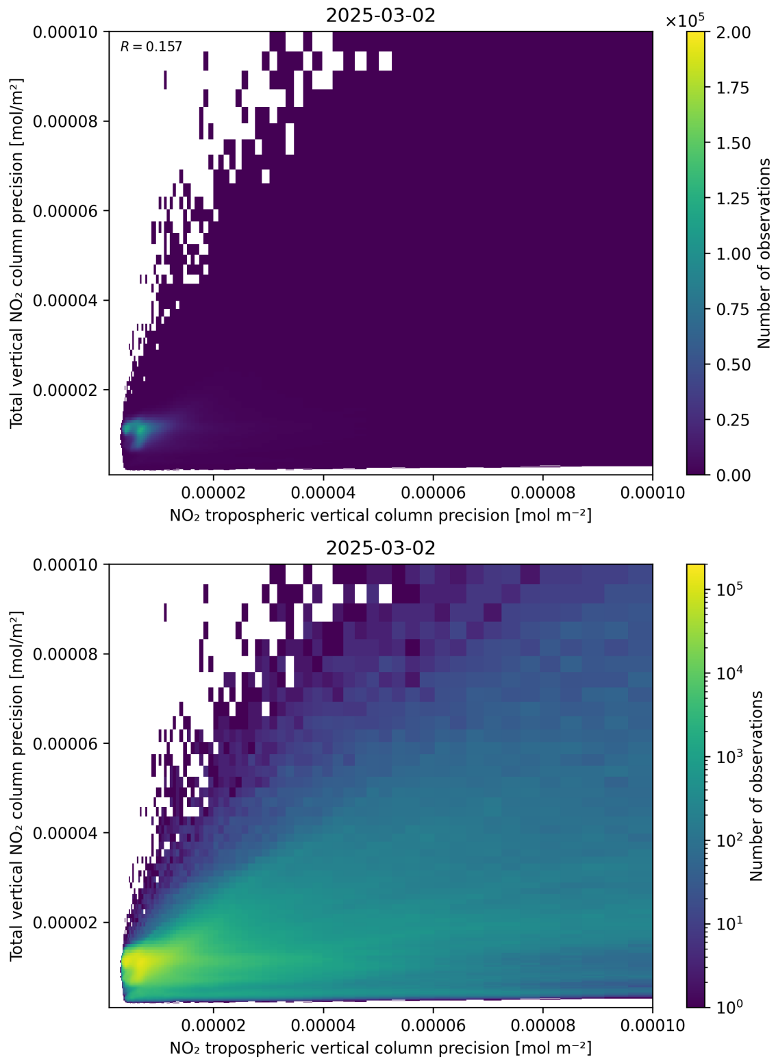
Figure 139: Scatter density plot of “NO 2 tropospheric vertical column precision” against “Total vertical NO 2 column precision” for 2025-03-01 to 2025-03-03.
