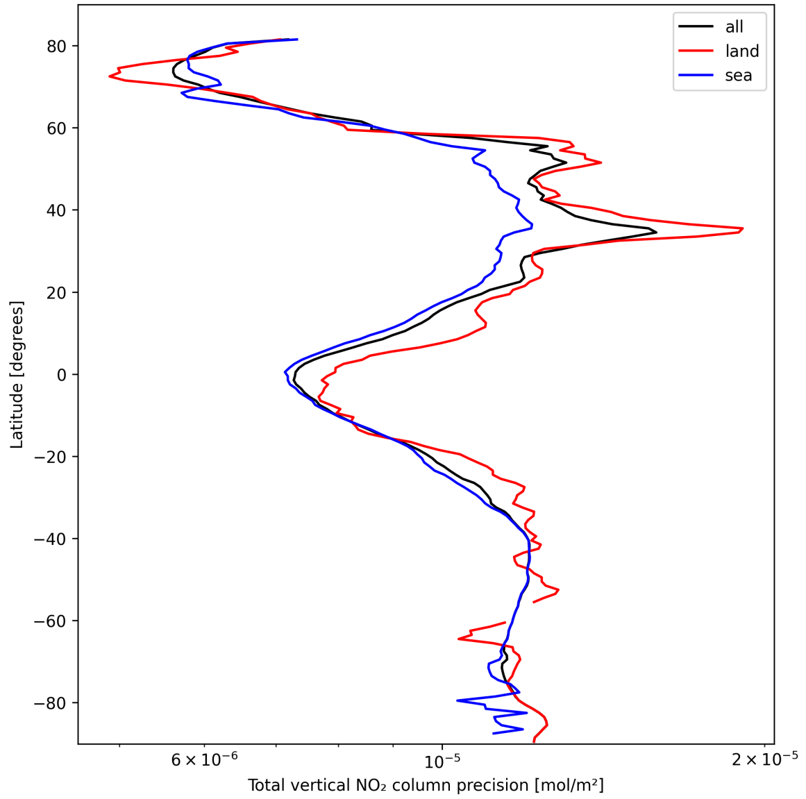
Figure 22: Zonal average of “Total vertical NO 2 column precision” for 2025-03-01 to 2025-03-03.
