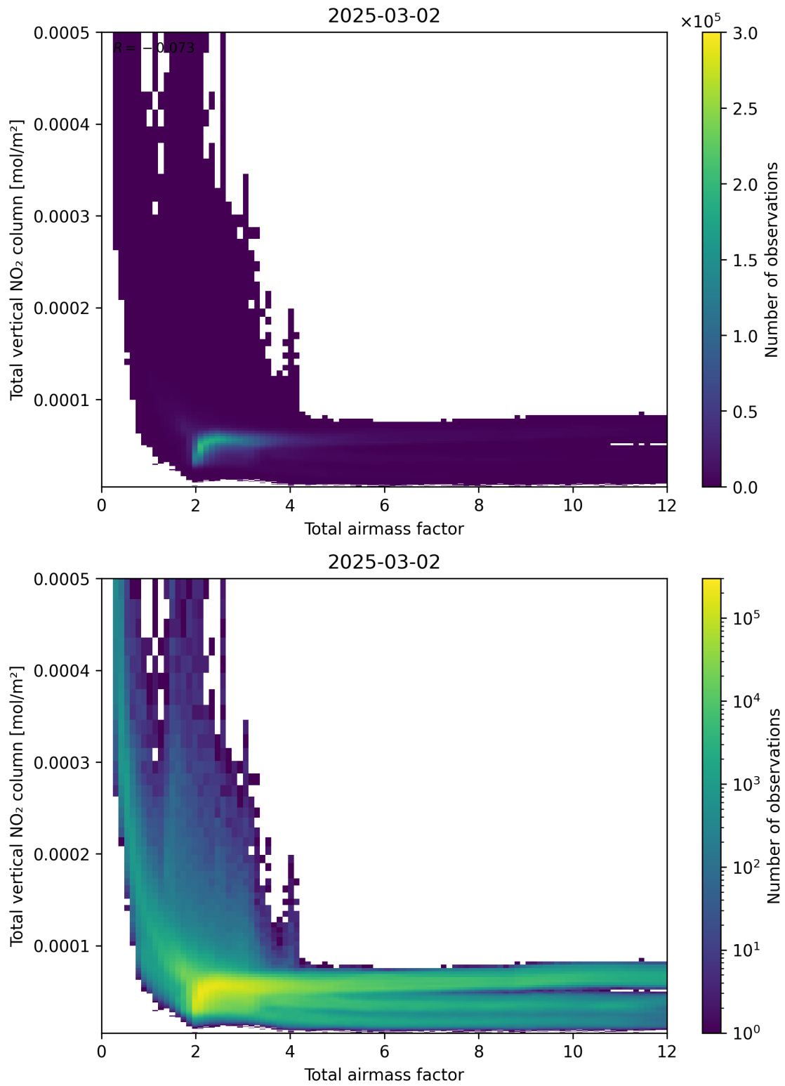
Figure 67: Scatter density plot of “Total air mass factor” against “Total vertical NO 2 column” for 2025-03-01 to 2025-03-03.
