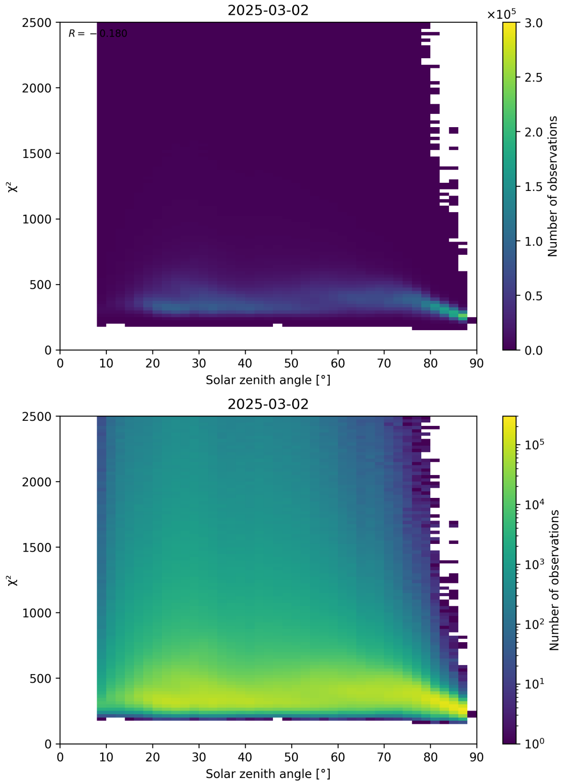
Figure 148: Scatter density plot of “Solar zenith angle” against “ \chi^2 ” for 2025-03-01 to 2025-03-03.
