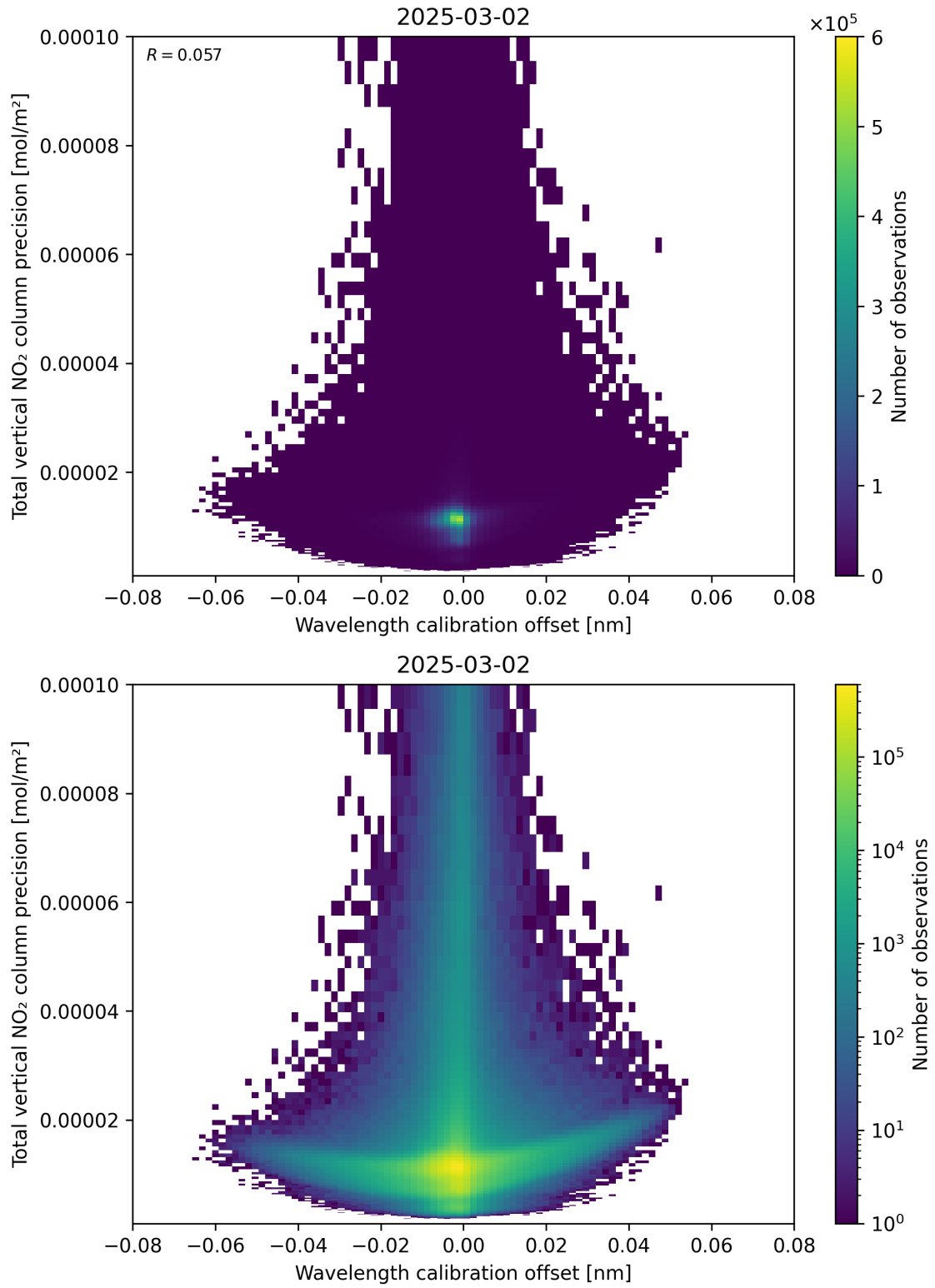
Figure 180: Scatter density plot of “Wavelength calibration offset” against “Total vertical NO 2 column precision” for 2025-03-01 to 2025-03-03.
