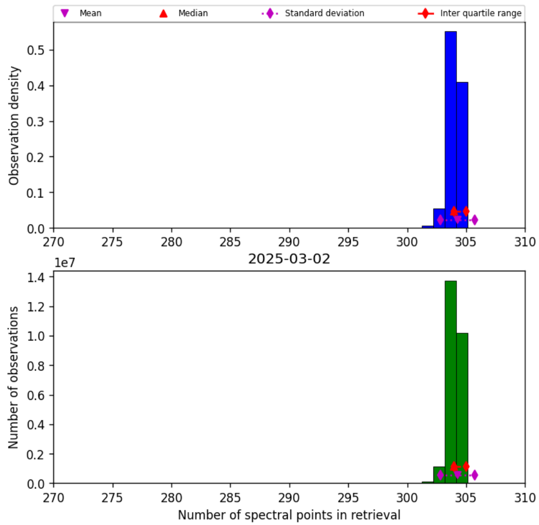
Figure 33: Histogram of “Number of spectral points in retrieval” for 2025-03-01 to 2025-03-03
