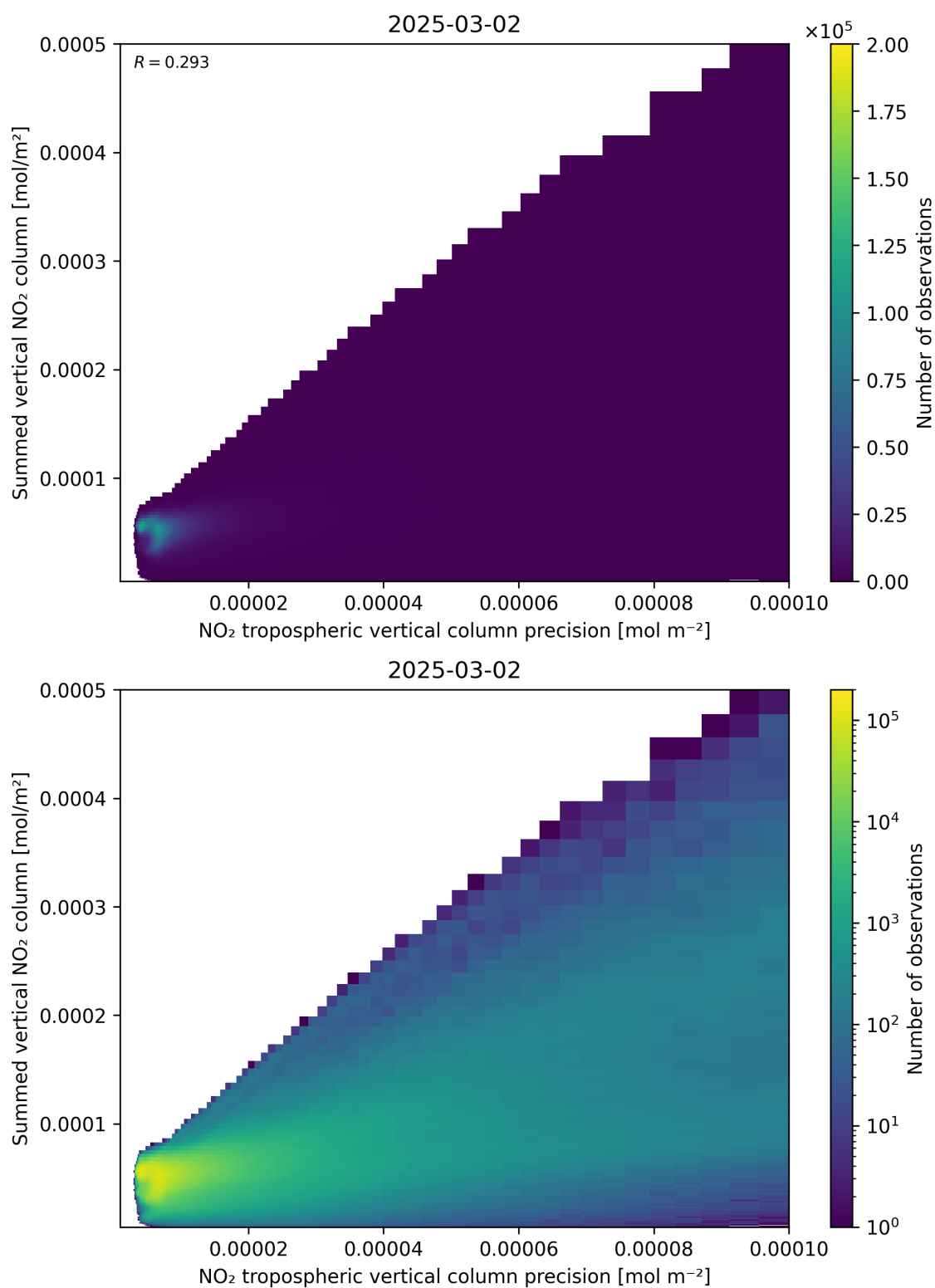
Figure 136: Scatter density plot of “NO 2 tropospheric vertical column precision” against “Summed vertical NO 2 column” for 2025-03-01 to 2025-03-03.
