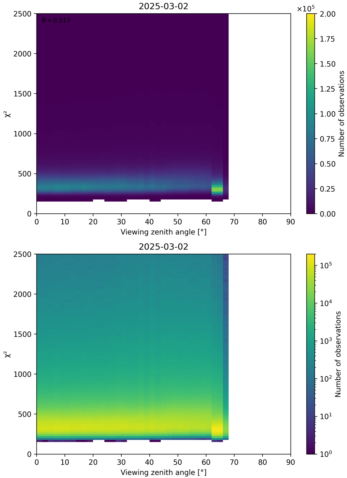
Figure 162: Scatter density plot of “Viewing zenith angle” against “ \chi^2 ” for 2025-03-01 to 2025-03-03.
