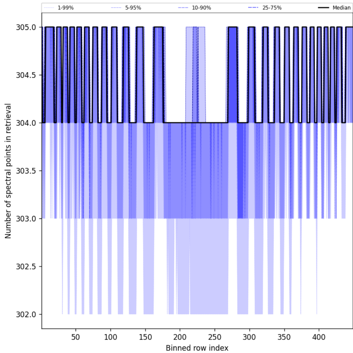
Figure 50: Along track statistics of “Number of spectral points in retrieval” for 2025-03-01 to 2025-03-03
