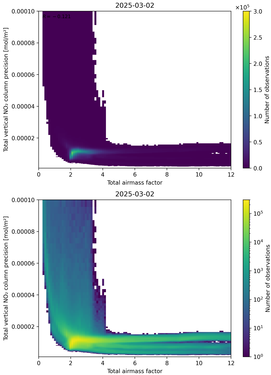
Figure 68: Scatter density plot of “Total airmass factor” against “Total vertical NO 2 column precision” for 2025-03-01 to 2025-03-03.
