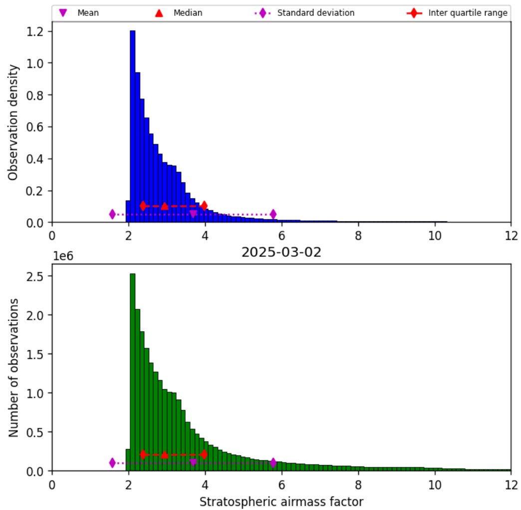
Figure 44: Histogram of “Stratospheric airmass factor” for 2025-03-01 to 2025-03-03
