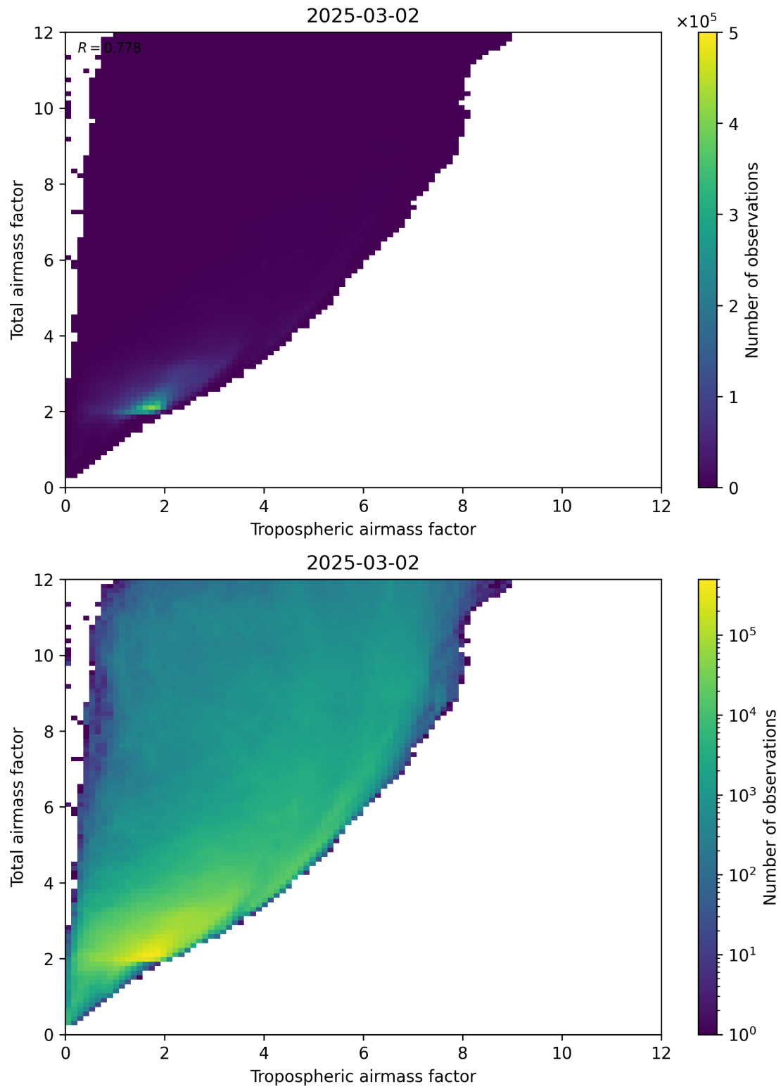
Figure 72: Scatter density plot of “Tropospheric airmass factor” against “Total airmass factor” for 2025-03-01 to 2025-03-03.
