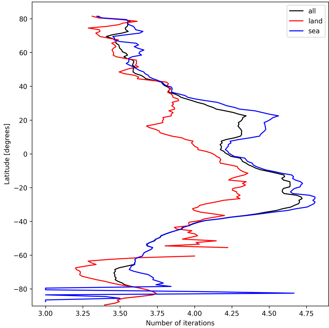
Figure 17: Zonal average of “Number of iterations” for 2025-03-01 to 2025-03-03.
