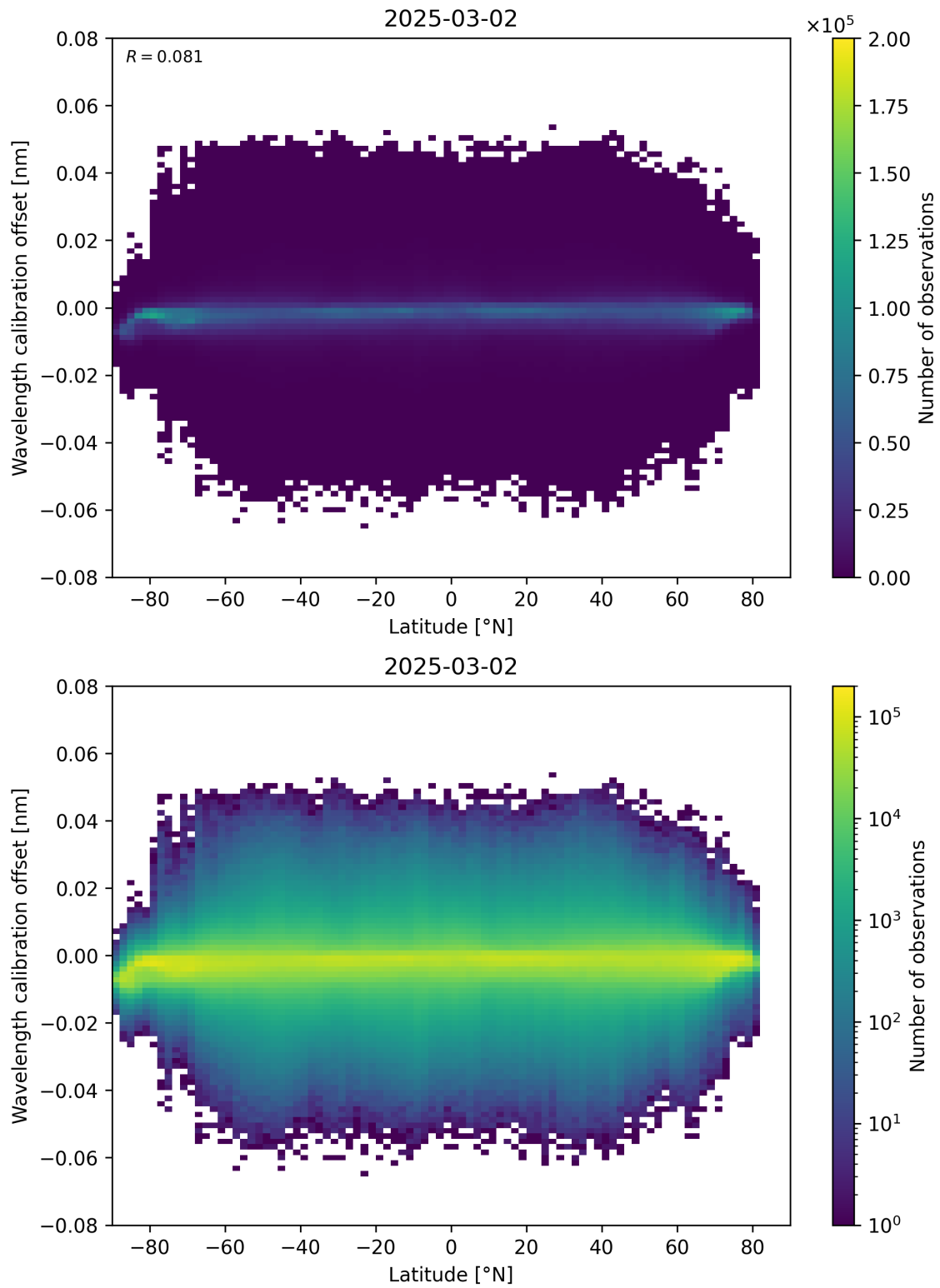
Figure 95: Scatter density plot of “Latitude” against “Wavelength calibration offset” for 2025-03-01 to 2025-03-03.
