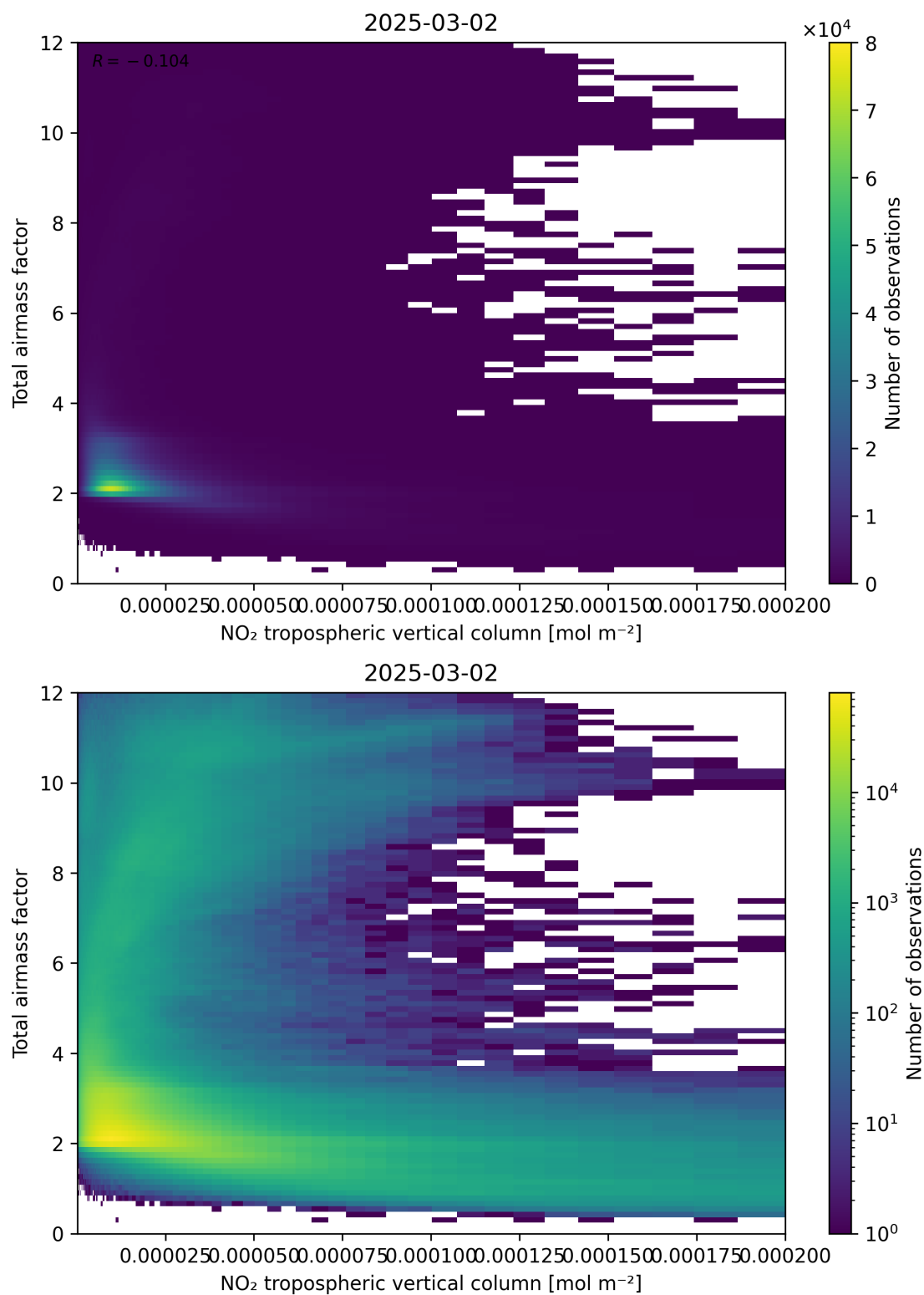
Figure 122: Scatter density plot of “NO 2 tropospheric vertical column” against “Total air mass factor” for 2025-03-01 to 2025-03-03.
