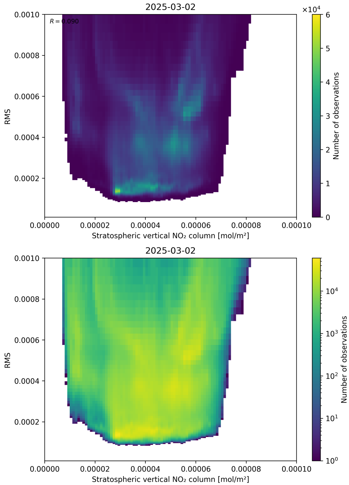
Figure 102: Scatter density plot of “Stratospheric vertical NO 2 column” against “RMS” for 2025-03-01 to 2025-03-03.
