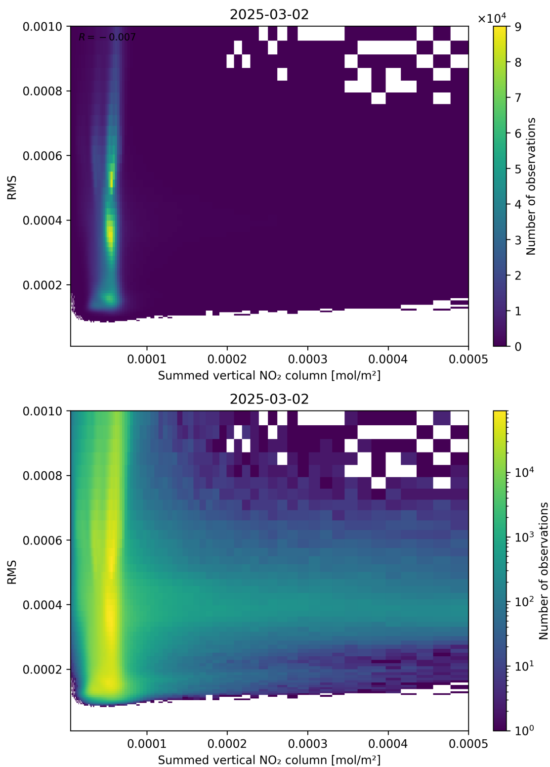
Figure 109: Scatter density plot of “Summed vertical NO 2 column” against “RMS” for 2025-03-01 to 2025-03-03.
