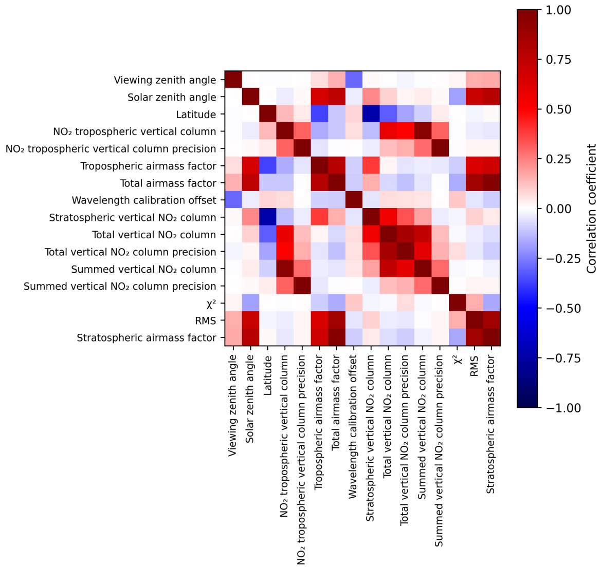
Figure 2: Map of correlation matrix for 2025-03-01 to 2025-03-03.
