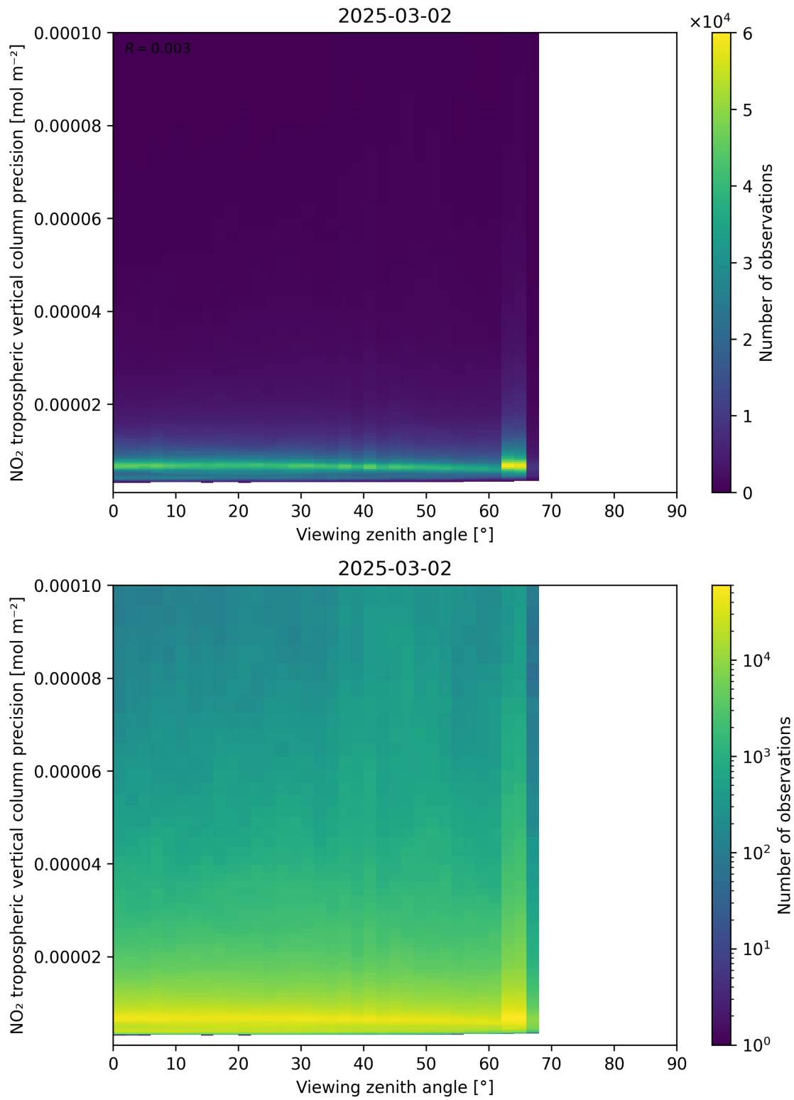
Figure 170: Scatter density plot of “Viewing zenith angle” against “NO 2 tropospheric vertical column precision” for 2025-03-01 to 2025-03-03.
