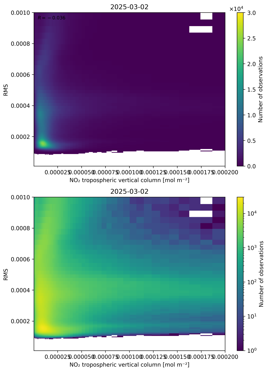
Figure 142: Scatter density plot of “NO 2 tropospheric vertical column” against “RMS” for 2025-03-01 to 2025-03-03.
