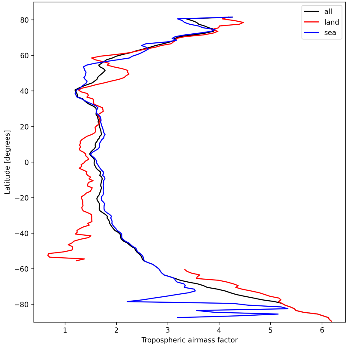
Figure 14: Zonal average of “Tropospheric air mass factor” for 2025-03-01 to 2025-03-03.
