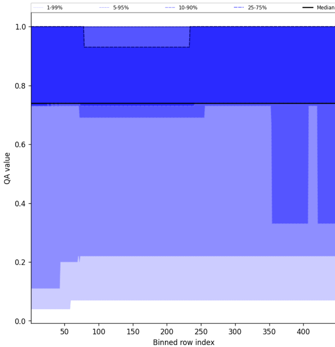
Figure 45: Along track statistics of “QA value” for 2025-03-01 to 2025-03-03
