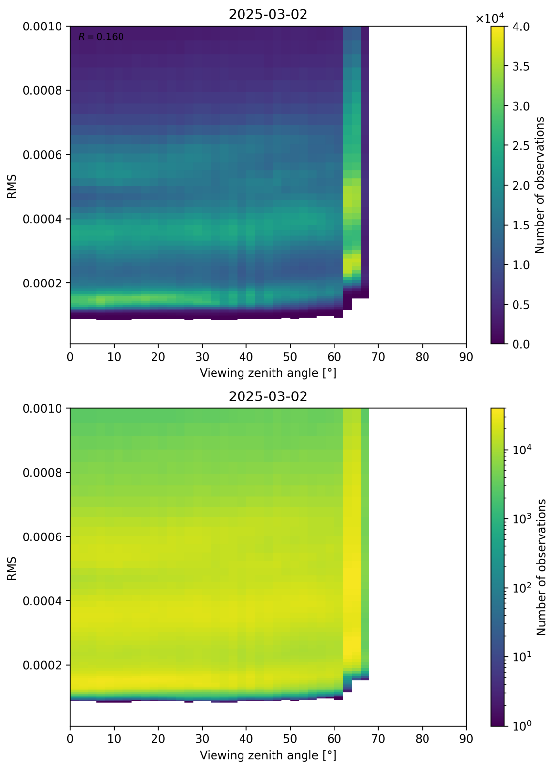
Figure 171: Scatter density plot of “Viewing zenith angle” against “RMS” for 2025-03-01 to 2025-03-03.
