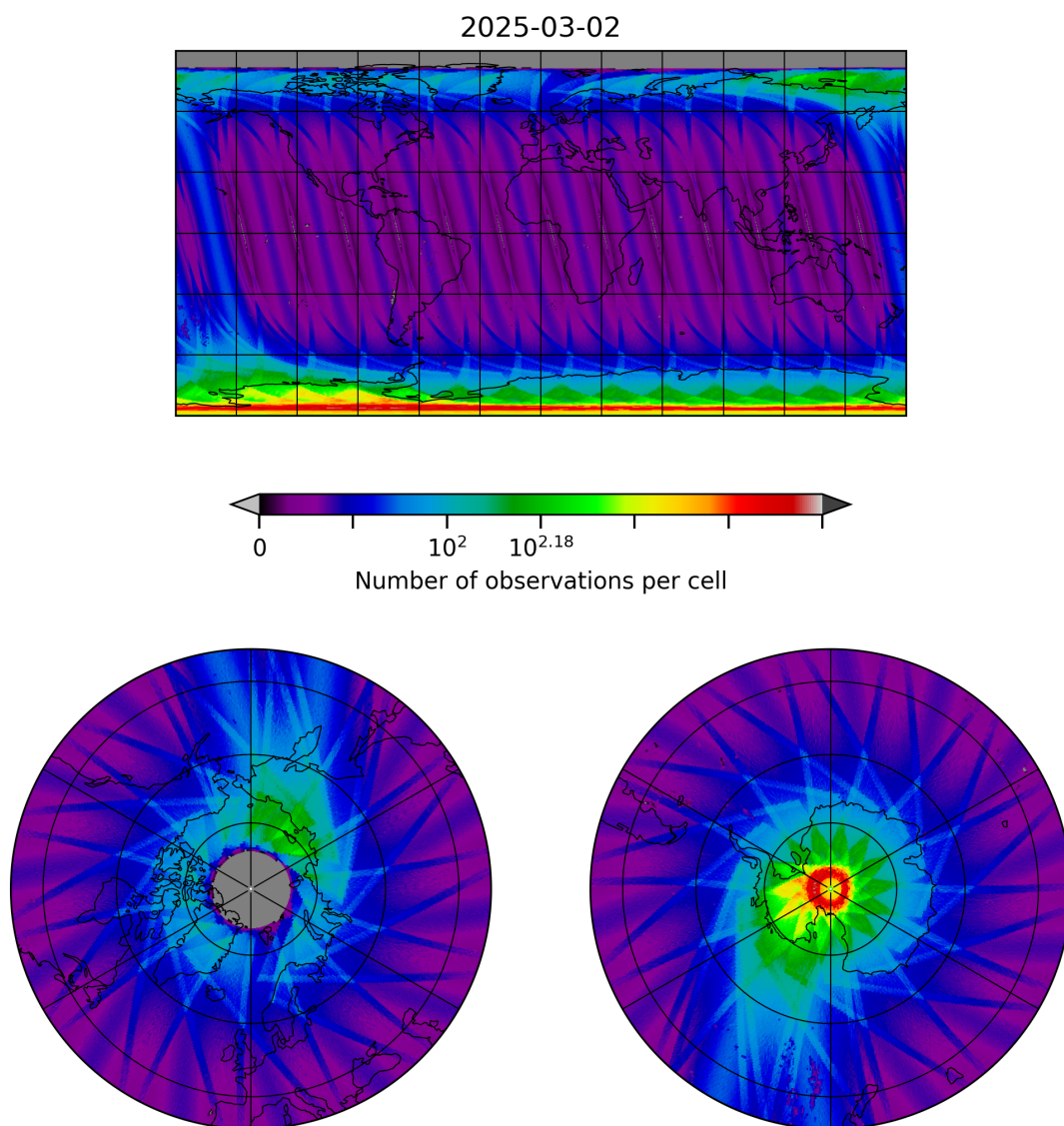
Figure 10: Map of the number of observations for 2025-03-01 to 2025-03-03
