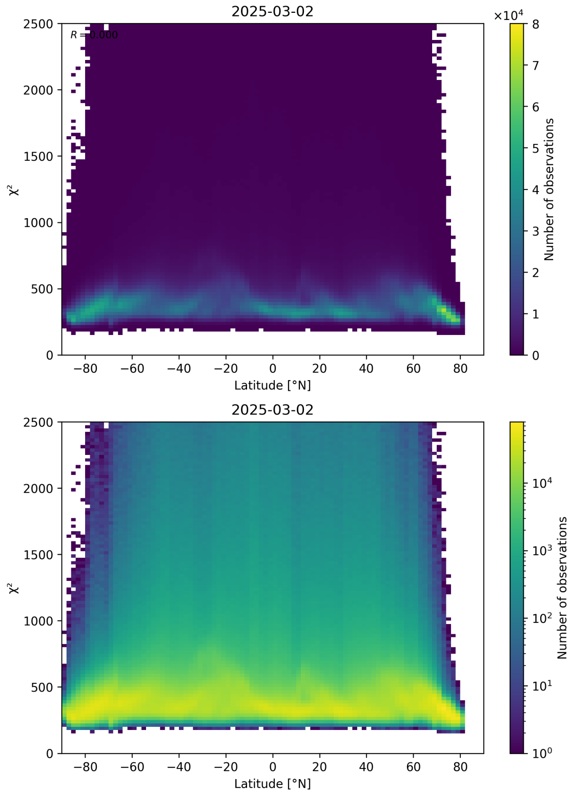
Figure 86: Scatter density plot of “Latitude” against “ \chi^2 ” for 2025-03-01 to 2025-03-03.
