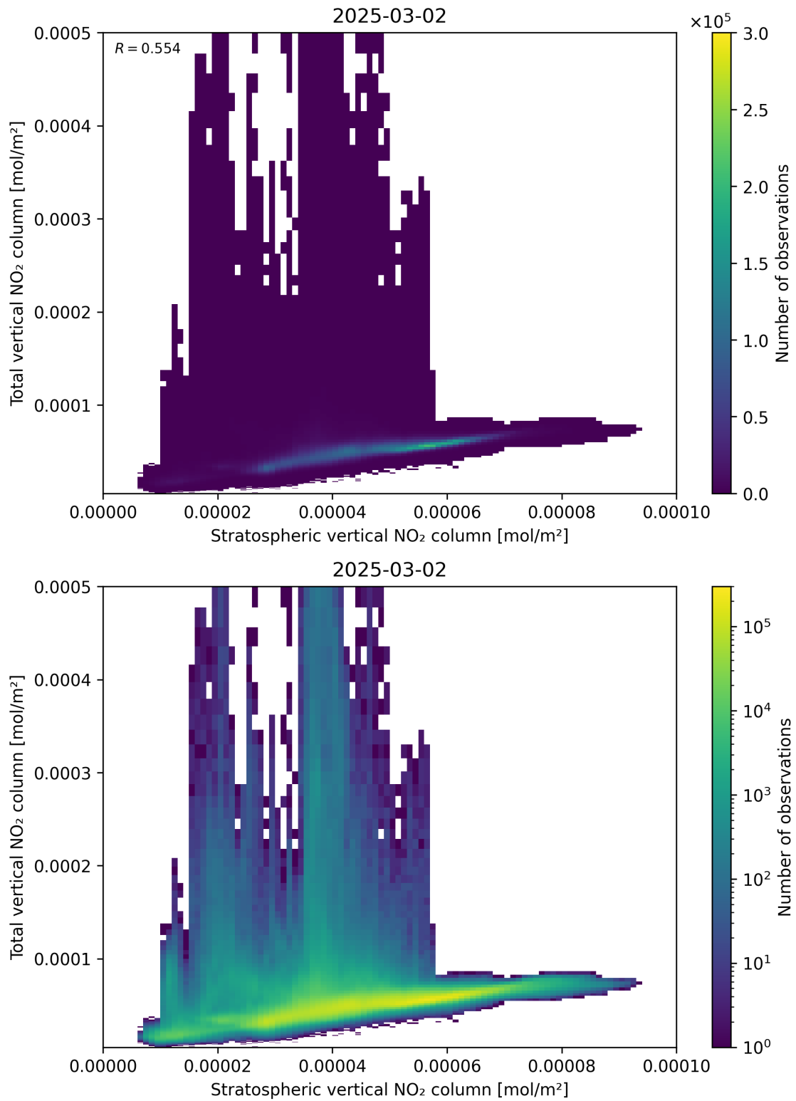
Figure 100: Scatter density plot of “Stratospheric vertical NO 2 column” against “Total vertical NO 2 column” for 2025-03-01 to 2025-03-03.
