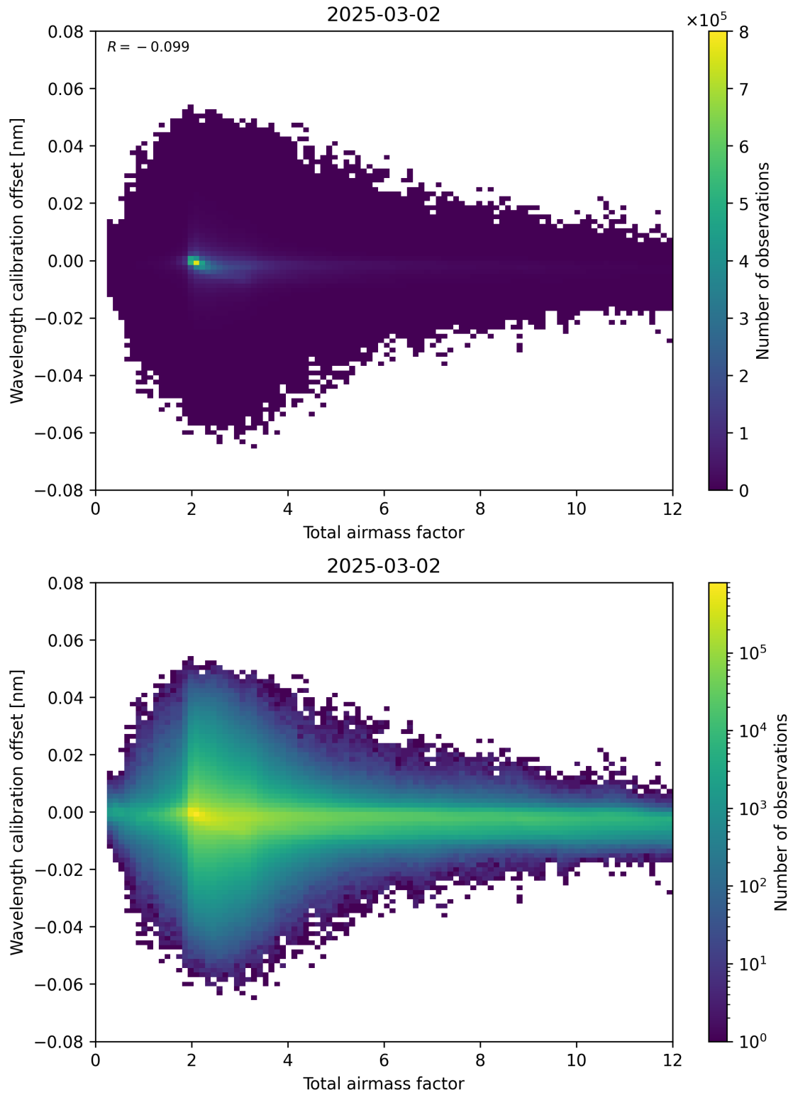
Figure 70: Scatter density plot of “Total airmass factor” against “Wavelength calibration offset” for 2025-03-01 to 2025-03-03.
