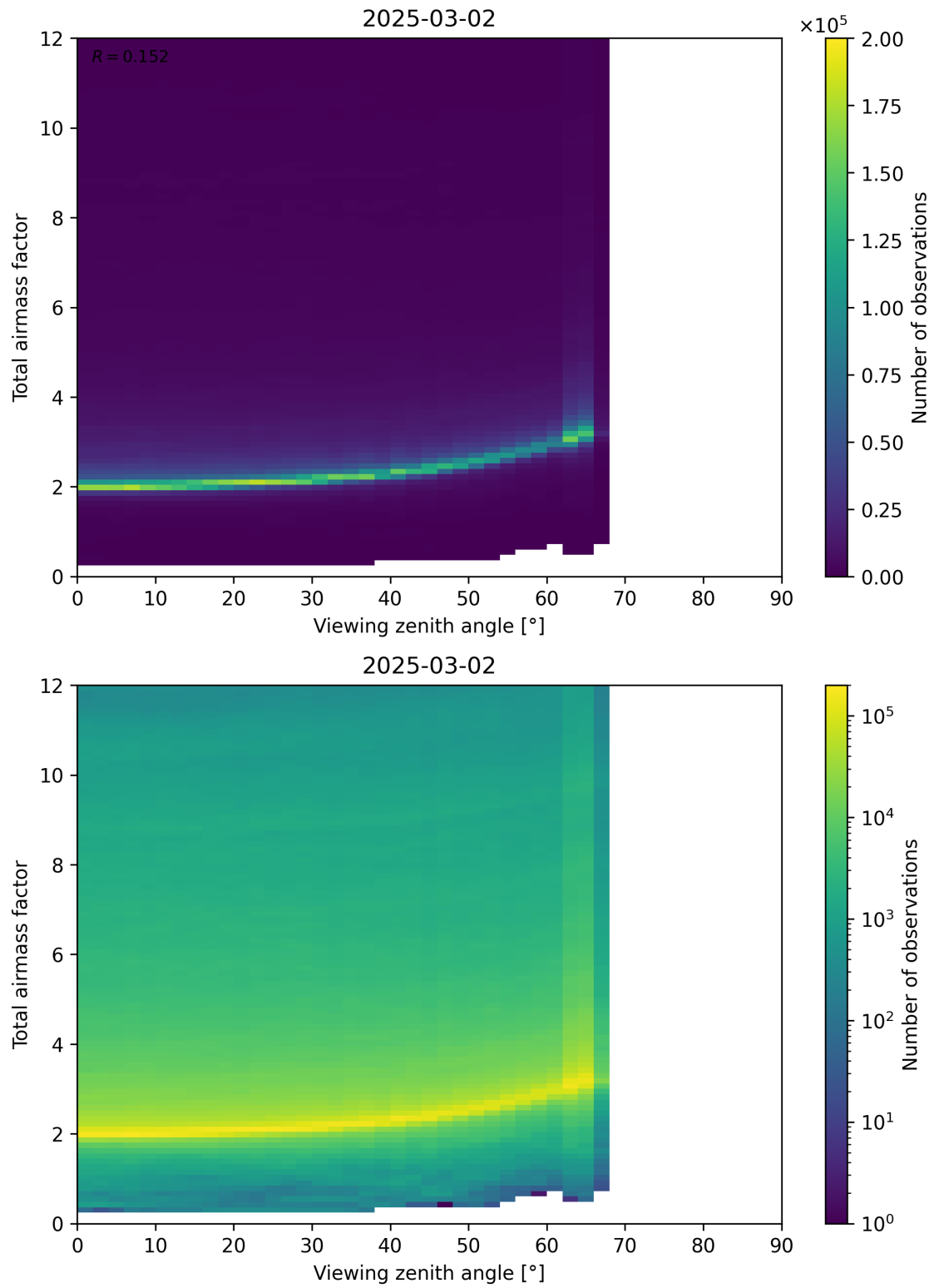
Figure 160: Scatter density plot of “Viewing zenith angle” against “Total airmass factor” for 2025-03-01 to 2025-03-03.
