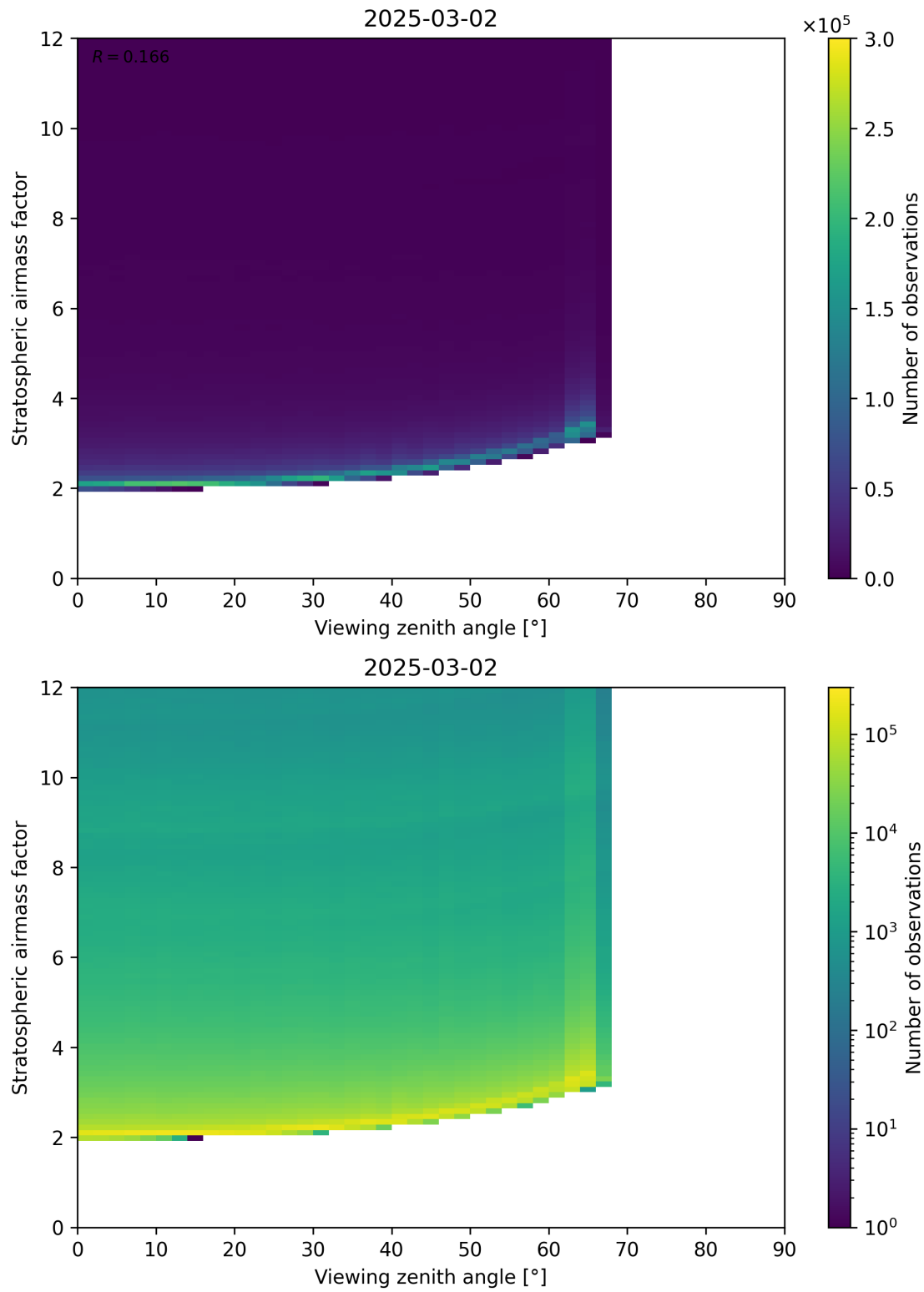
Figure 159: Scatter density plot of “Viewing zenith angle” against “Stratospheric airmass factor” for 2025-03-01 to 2025-03-03.
