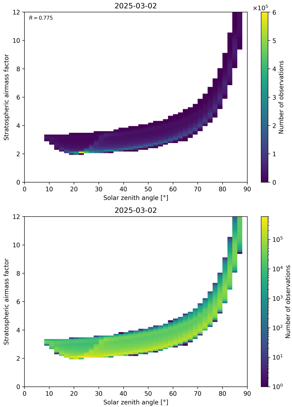
Figure 145: Scatter density plot of “Solar zenith angle” against “Stratospheric airmass factor” for 2025-03-01 to 2025-03-03.
