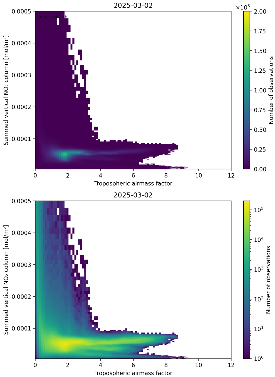
Figure 75: Scatter density plot of “Tropospheric air mass factor” against “Summed vertical NO 2 column” for 2025-03-01 to 2025-03-03.
