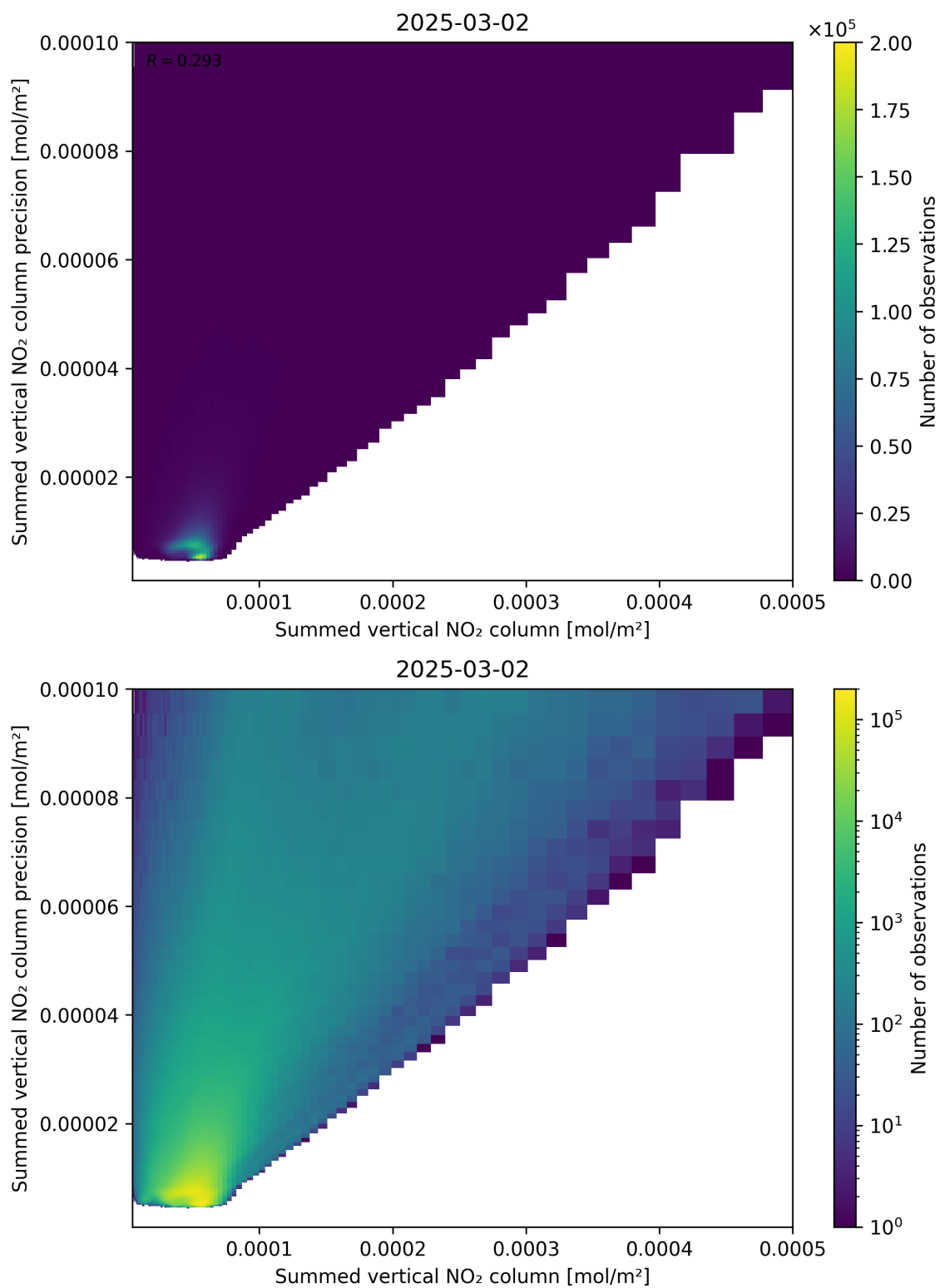
Figure 105: Scatter density plot of “Summed vertical NO 2 column” against “Summed vertical NO 2 column precision” for 2025-03-01 to 2025-03-03.
