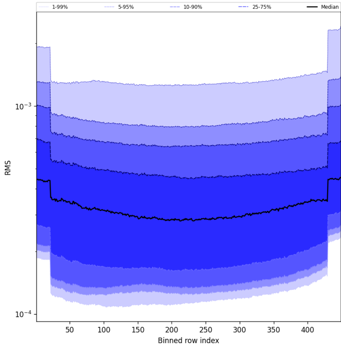
Figure 60: Along track statistics of “RMS” for 2025-03-01 to 2025-03-03
