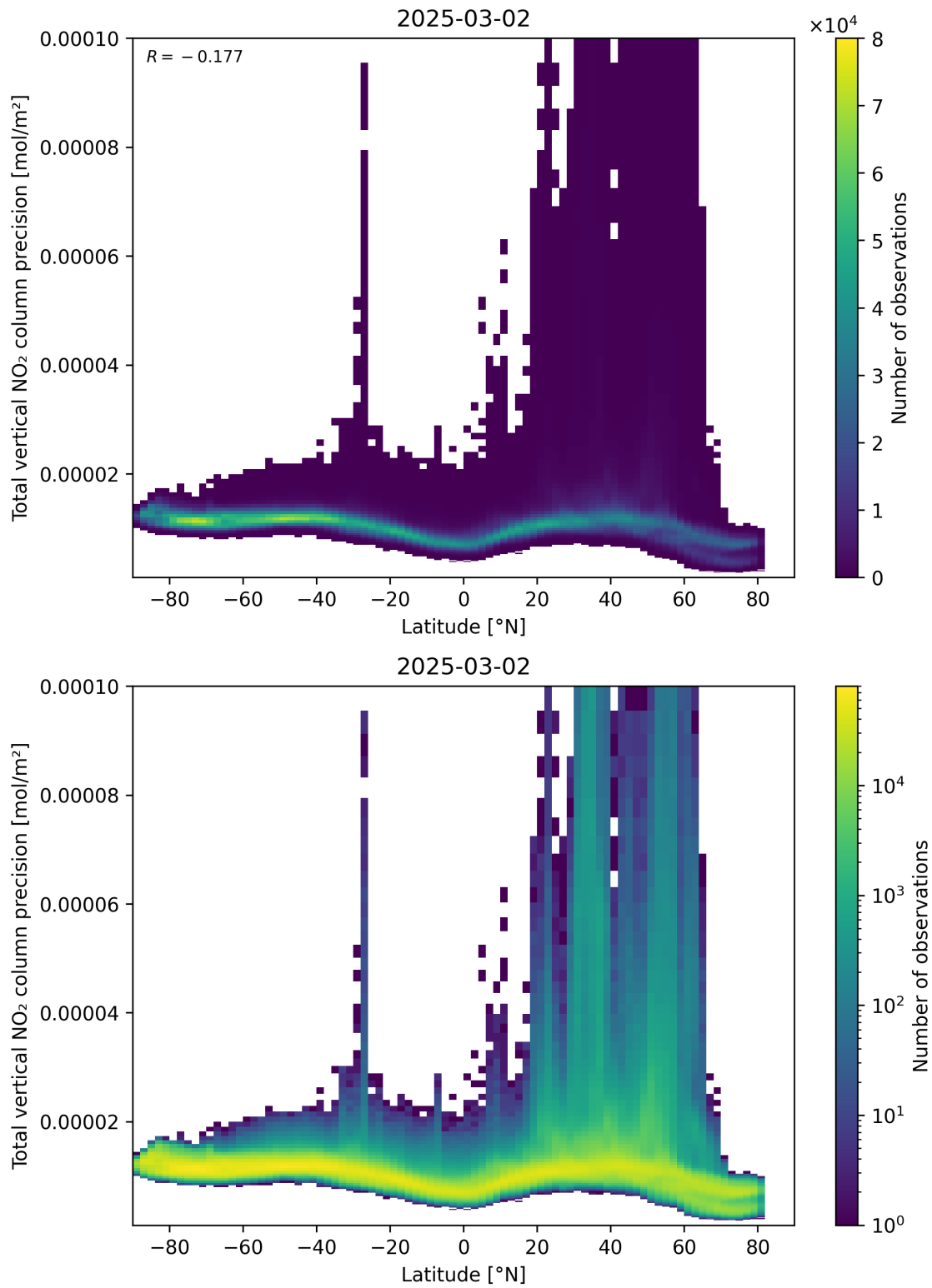
Figure 91: Scatter density plot of “Latitude” against “Total vertical NO 2 column precision” for 2025-03-01 to 2025-03-03.
