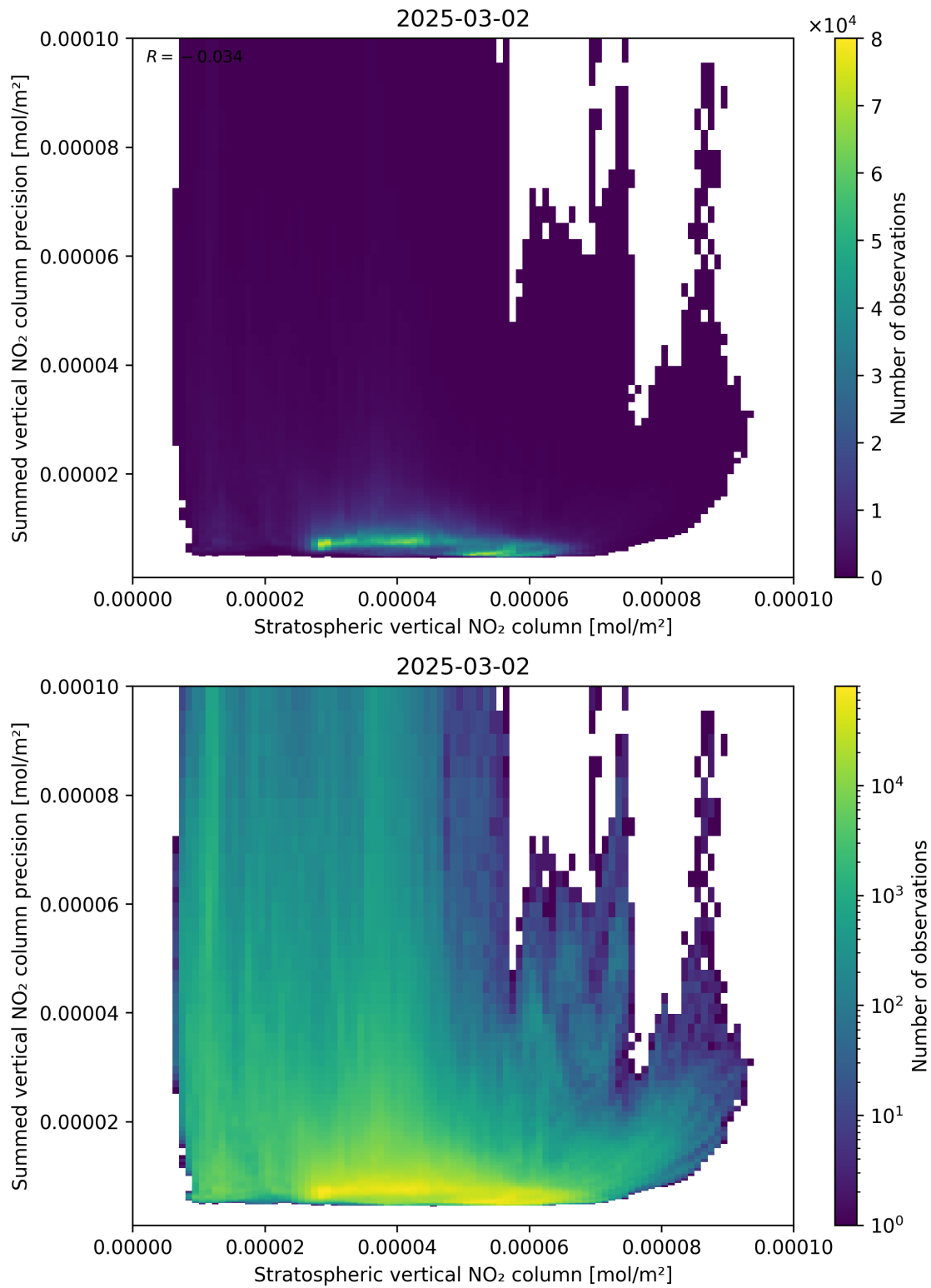
Figure 99: Scatter density plot of “Stratospheric vertical NO 2 column” against “Summed vertical NO 2 column precision” for 2025-03-01 to 2025-03-03.
