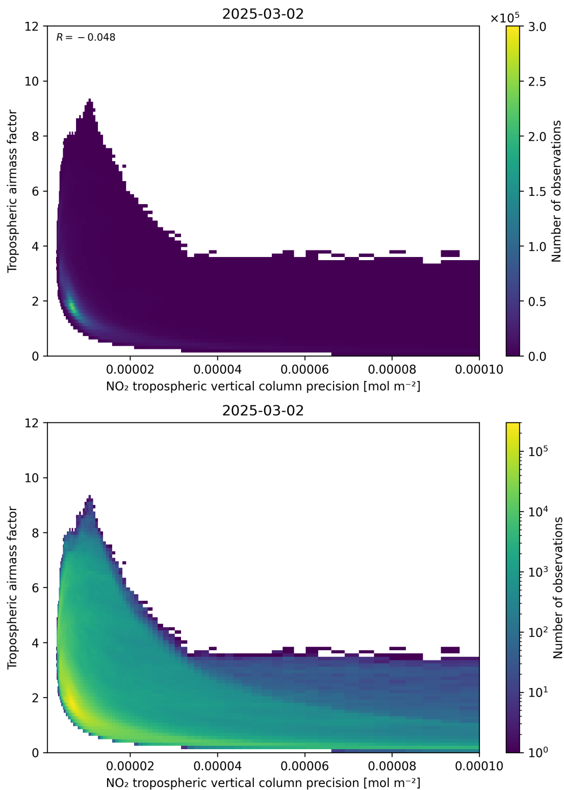
Figure 133: Scatter density plot of “NO 2 tropospheric vertical column precision” against “Tropospheric airmass factor” for 2025-03-01 to 2025-03-03.
