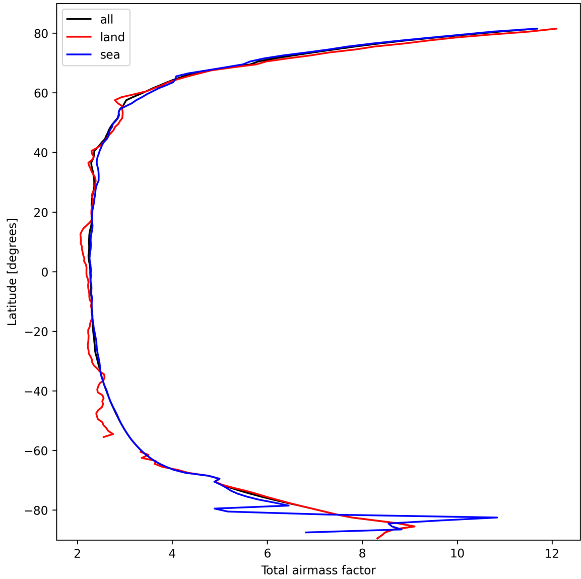
Figure 15: Zonal average of “Total airmass factor” for 2025-03-01 to 2025-03-03.
