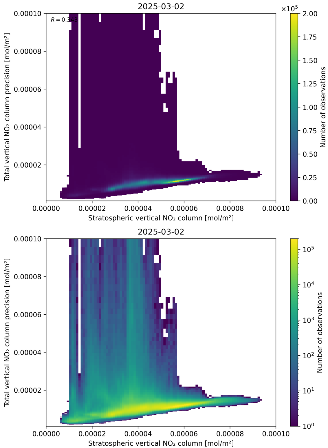
Figure 101: Scatter density plot of “Stratospheric vertical NO 2 column” against “Total vertical NO 2 column precision” for 2025-03-01 to 2025-03-03.
