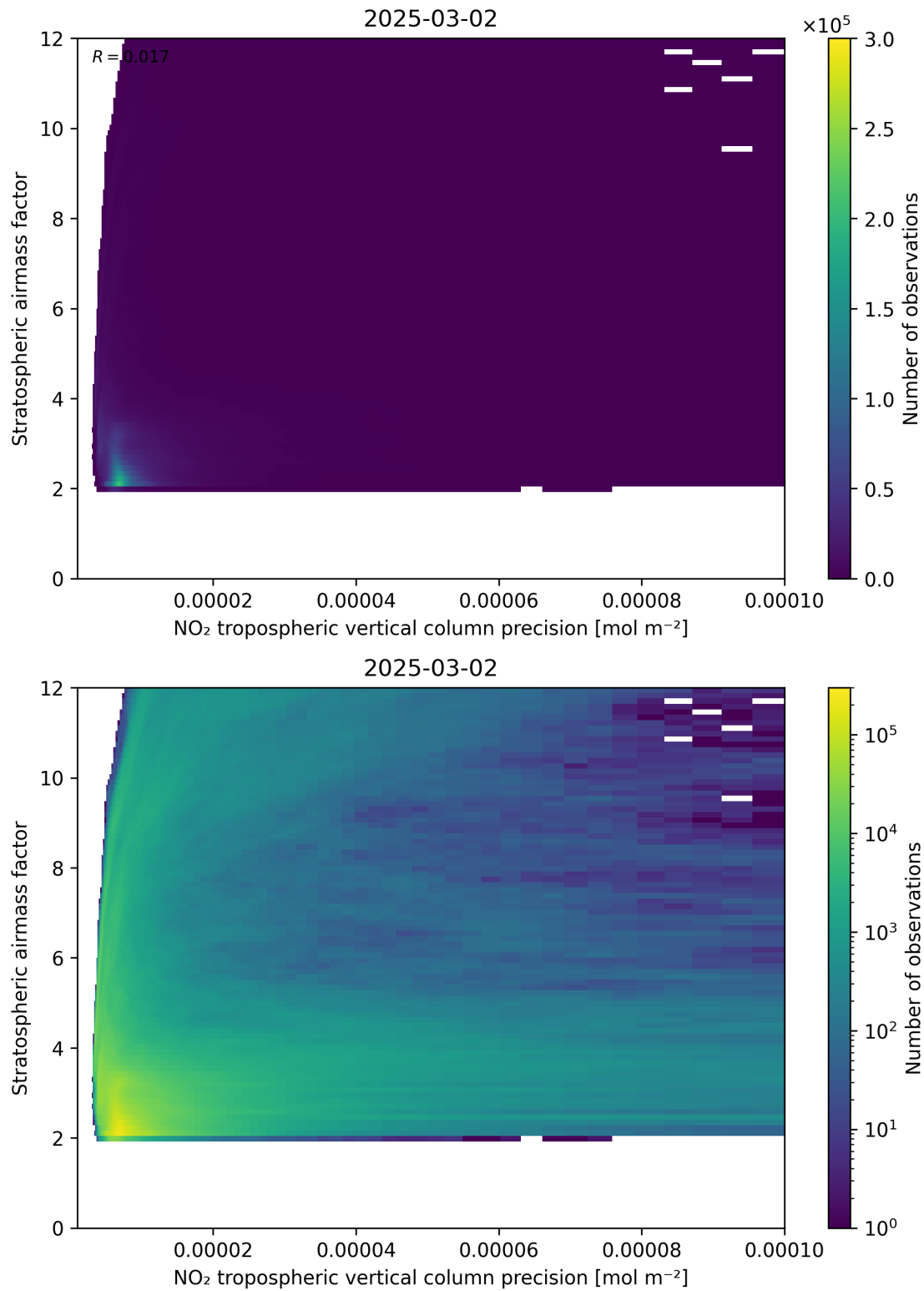
Figure 131: Scatter density plot of “NO 2 tropospheric vertical column precision” against “Stratospheric airmass factor” for 2025-03-01 to 2025-03-03.
