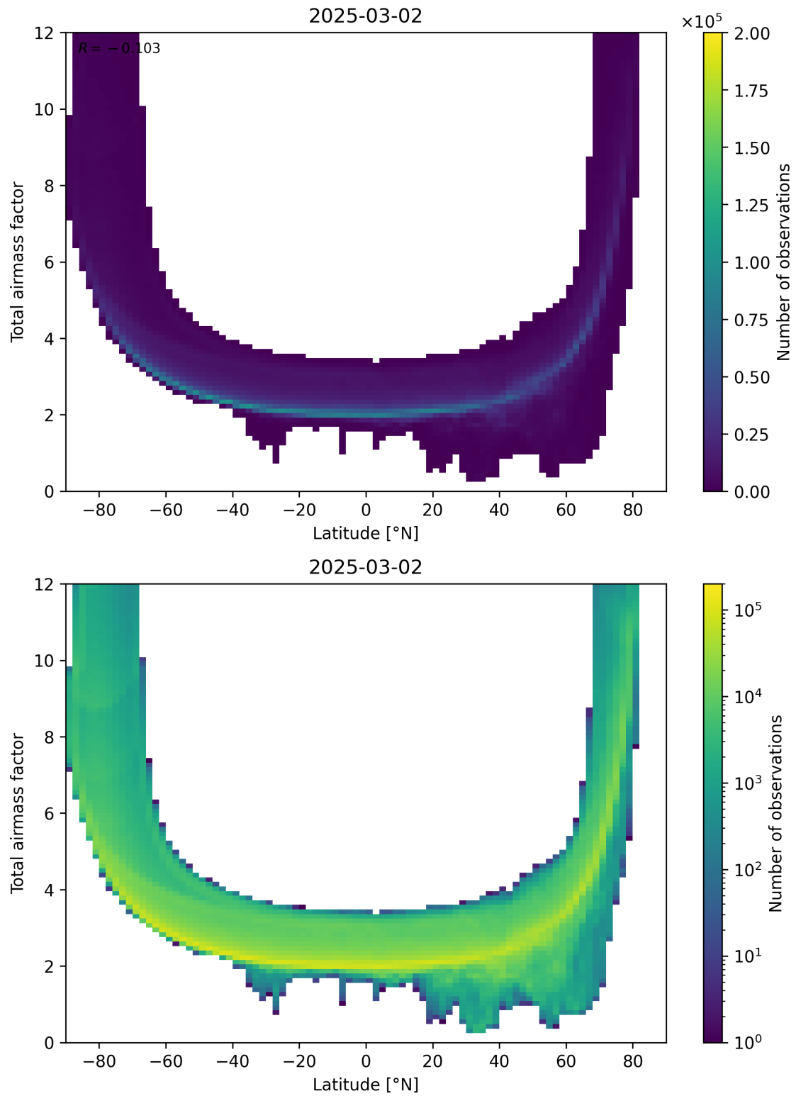
Figure 84: Scatter density plot of “Latitude” against “Total airmass factor” for 2025-03-01 to 2025-03-03.
