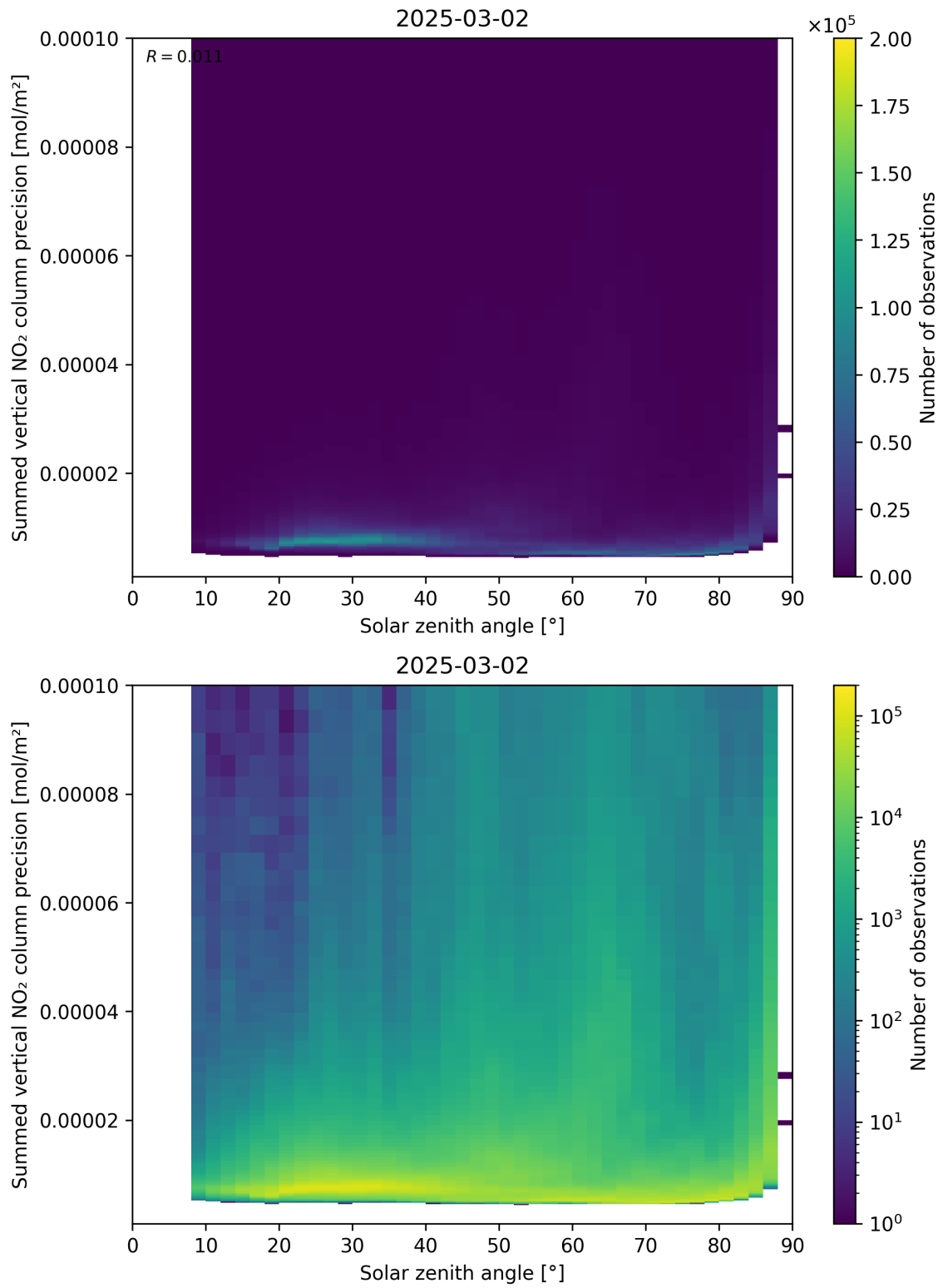
Figure 152: Scatter density plot of “Solar zenith angle” against “Summed vertical NO 2 column precision” for 2025-03-01 to 2025-03-03.
