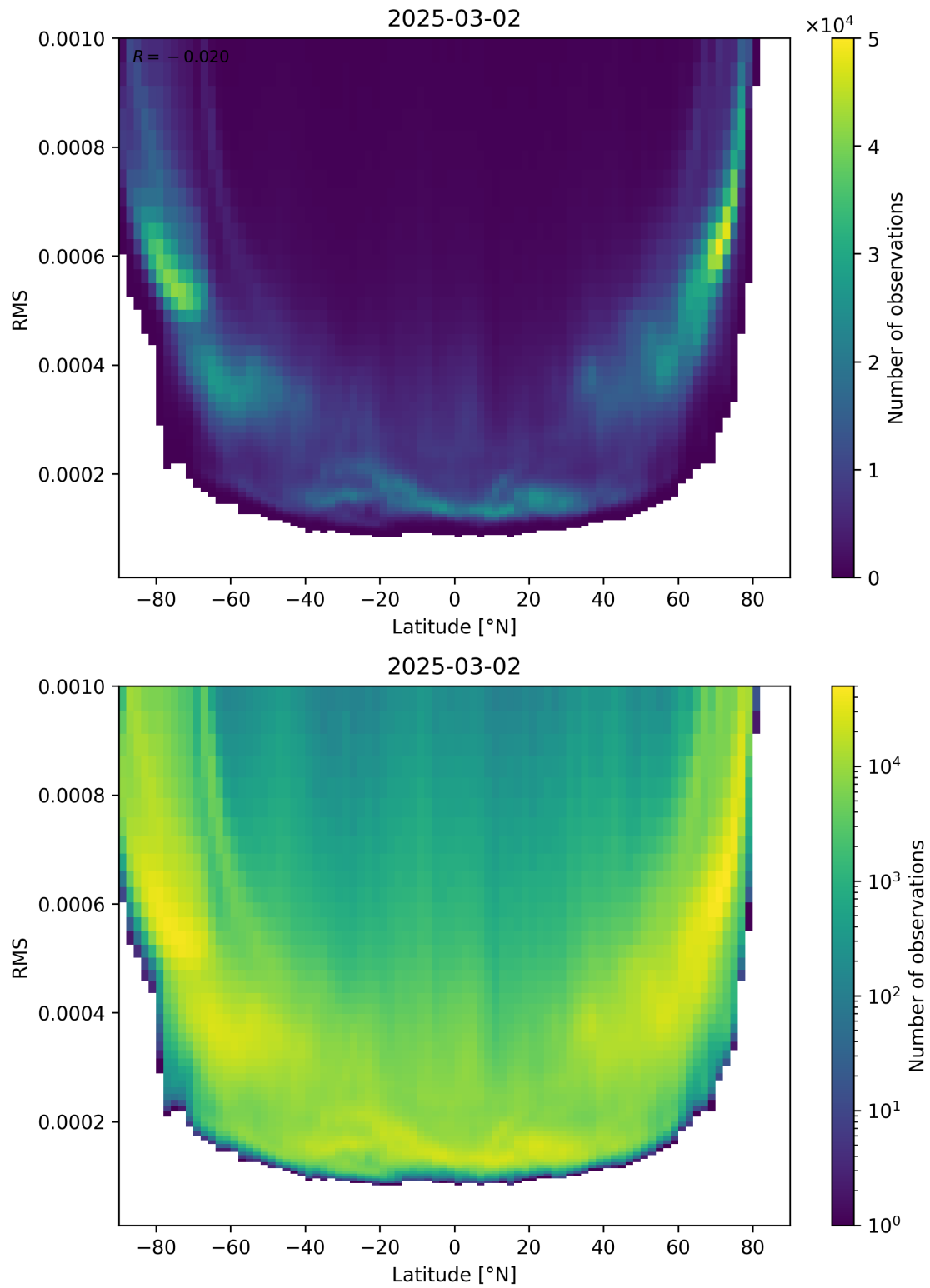
Figure 94: Scatter density plot of “Latitude” against “RMS” for 2025-03-01 to 2025-03-03.
