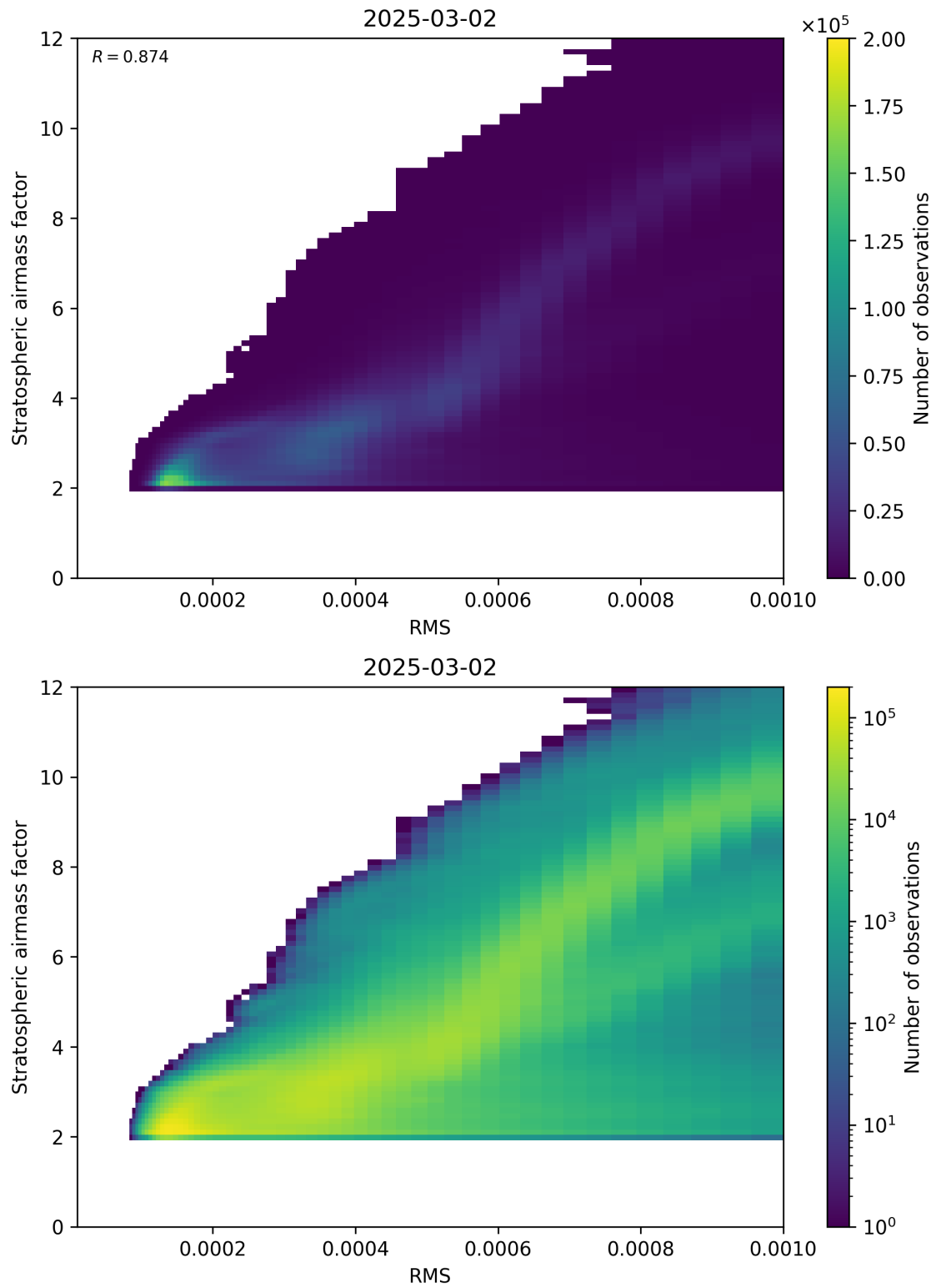
Figure 144: Scatter density plot of “RMS” against “Stratospheric airmass factor” for 2025-03-01 to 2025-03-03.
