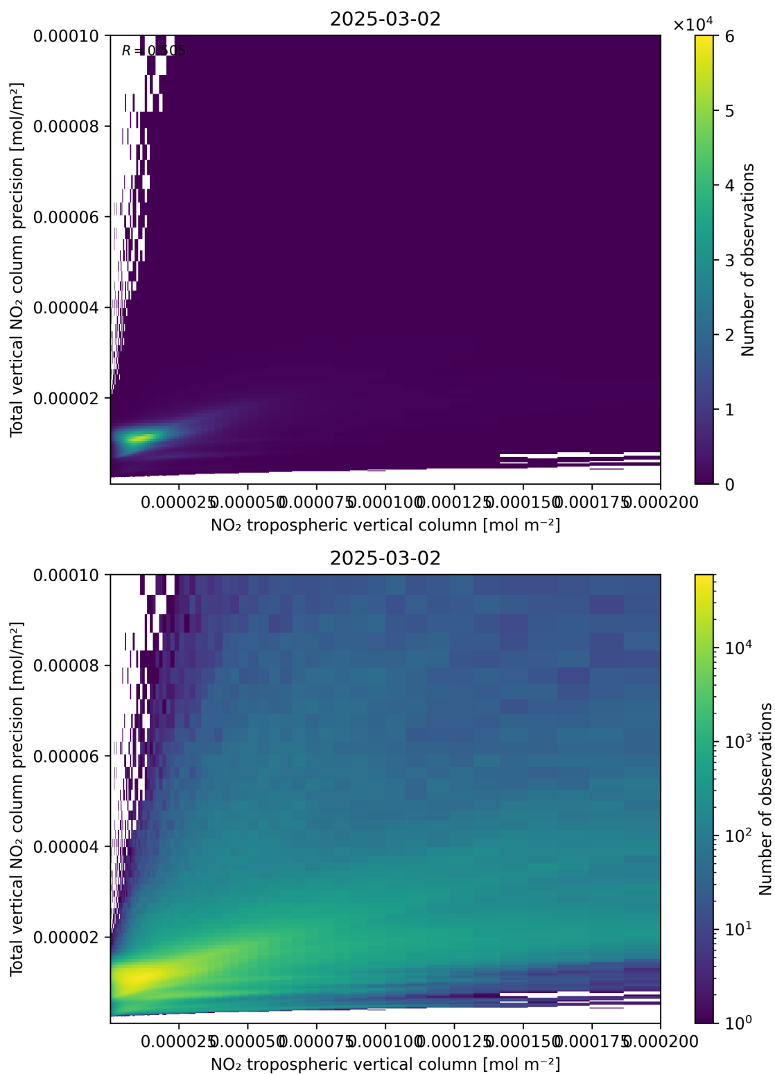
Figure 129: Scatter density plot of “NO 2 tropospheric vertical column” against “Total vertical NO 2 column precision” for 2025-03-01 to 2025-03-03.
