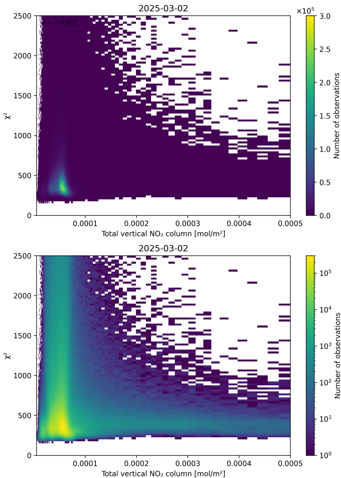
Figure 111: Scatter density plot of “Total vertical NO 2 column” against “ \chi^2 ” for 2025-03-01 to 2025-03-03.
