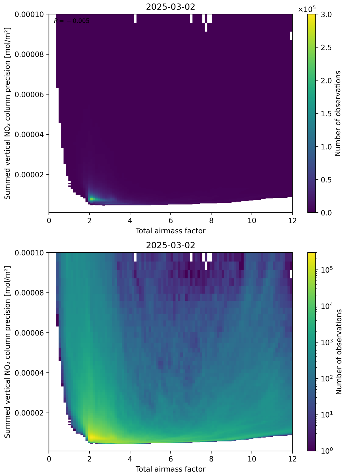
Figure 66: Scatter density plot of “Total airmass factor” against “Summed vertical NO 2 column precision” for 2025-03-01 to 2025-03-03.
