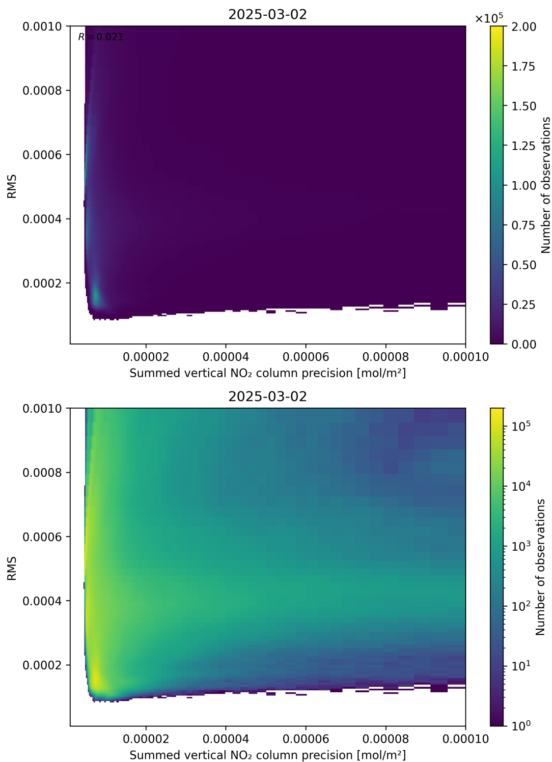
Figure 108: Scatter density plot of “Summed vertical NO 2 column precision” against “RMS” for 2025-03-01 to 2025-03-03.
