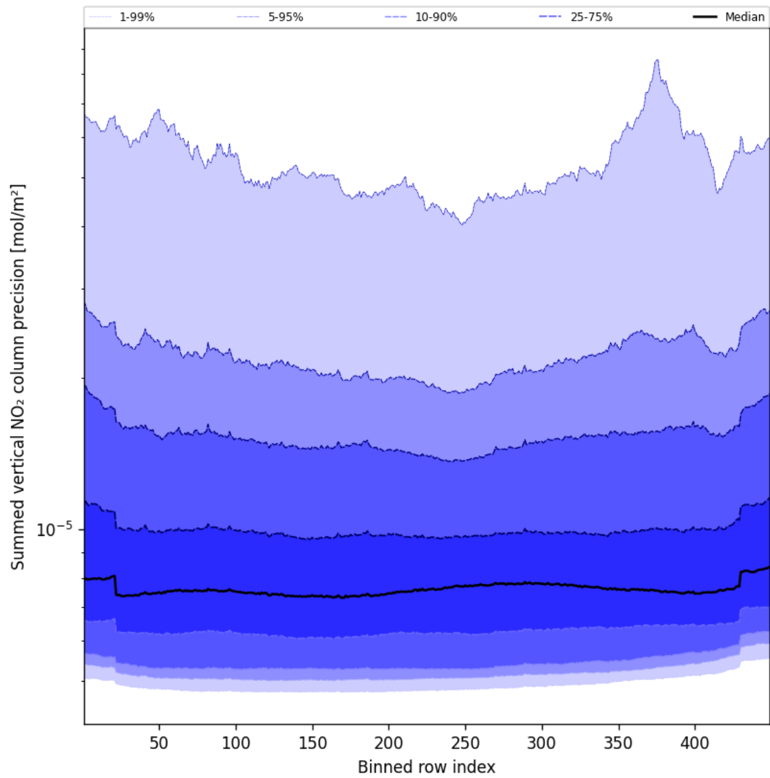
Figure 58: Along track statistics of “Summed vertical NO 2 column precision” for 2025-03-01 to 2025-03-03
