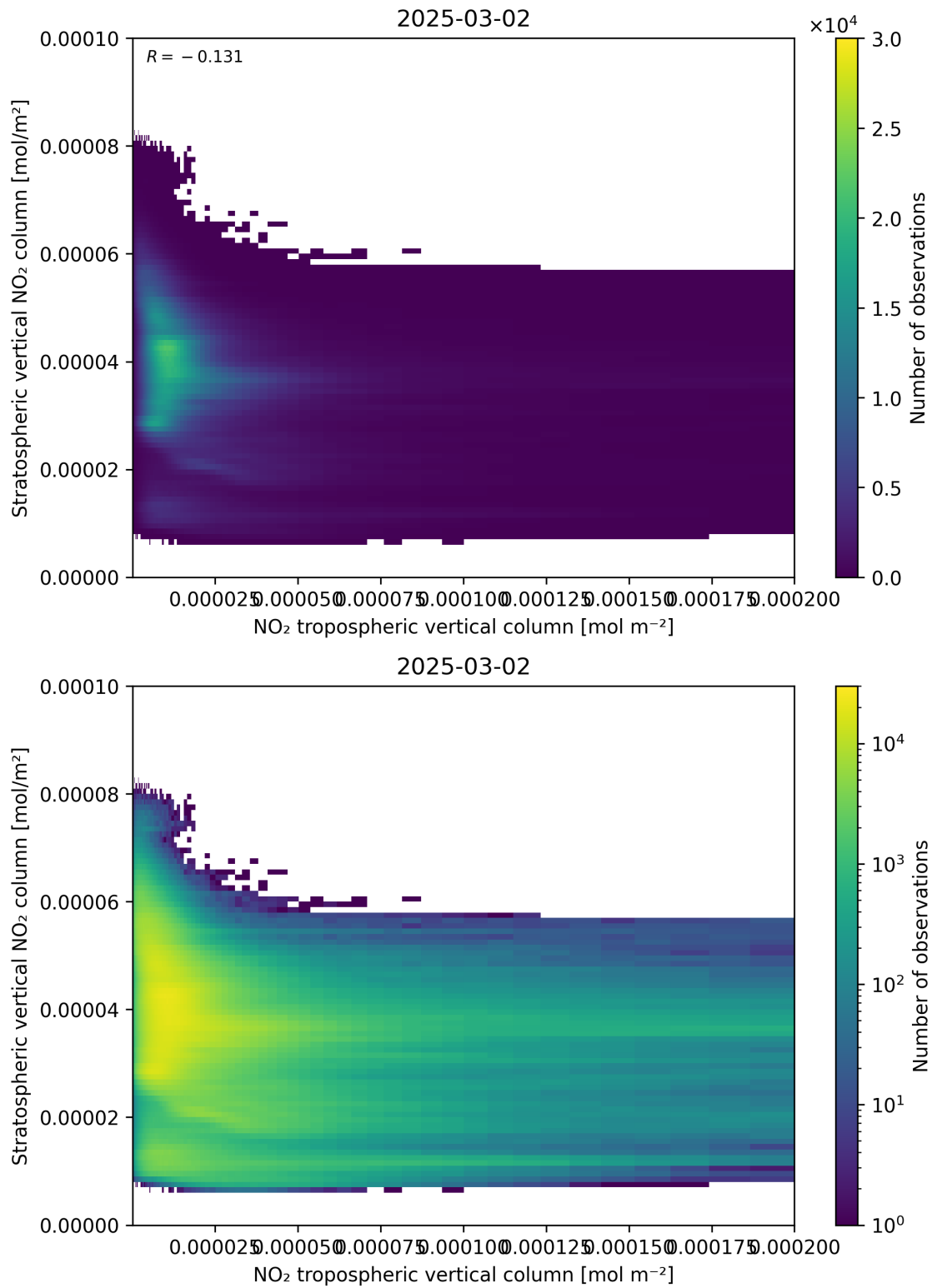
Figure 125: Scatter density plot of “NO 2 tropospheric vertical column” against “Stratospheric vertical NO 2 column” for 2025-03-01 to 2025-03-03.
