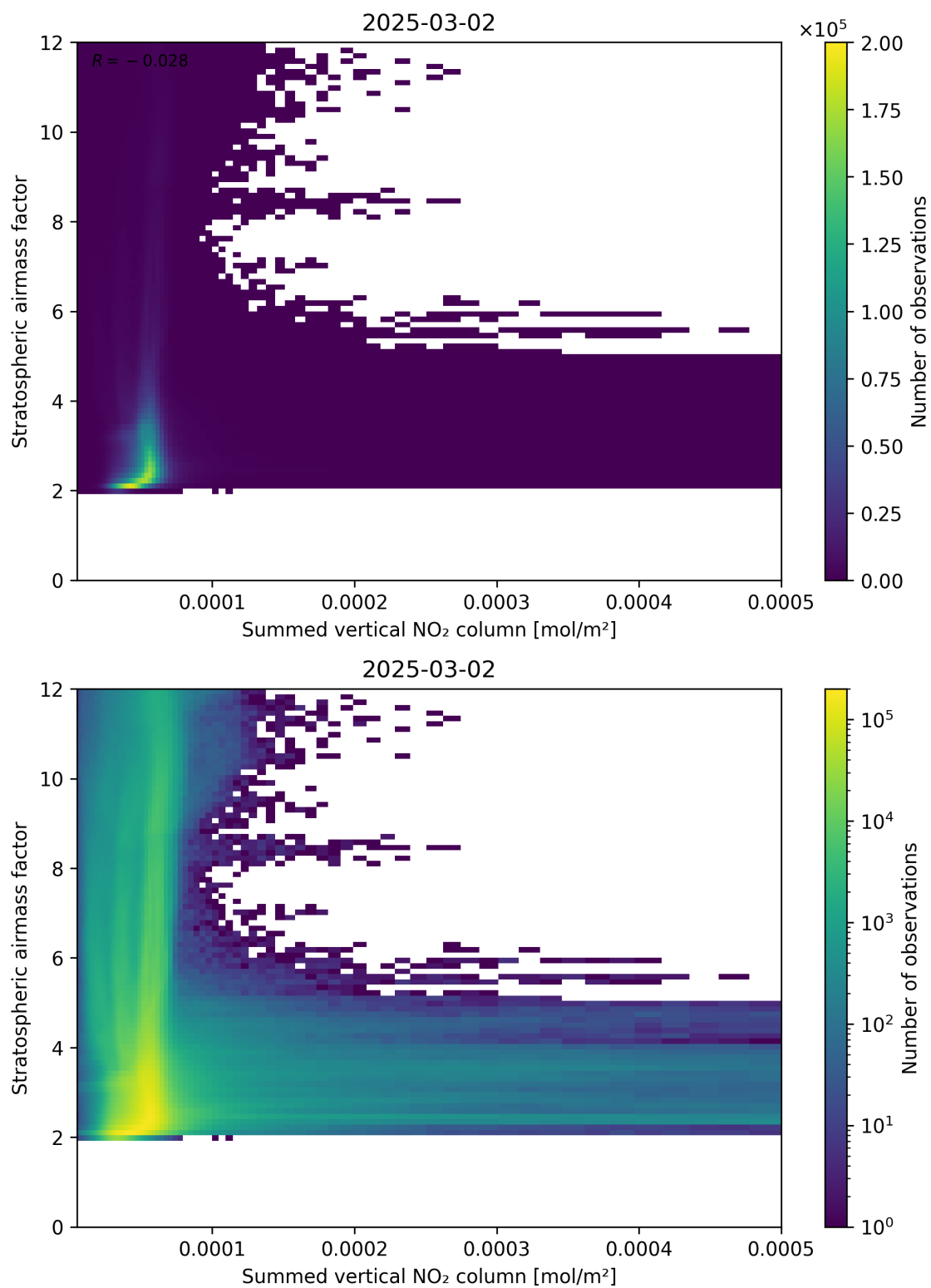
Figure 103: Scatter density plot of “Summed vertical NO 2 column” against “Stratospheric air mass factor” for 2025-03-01 to 2025-03-03.
