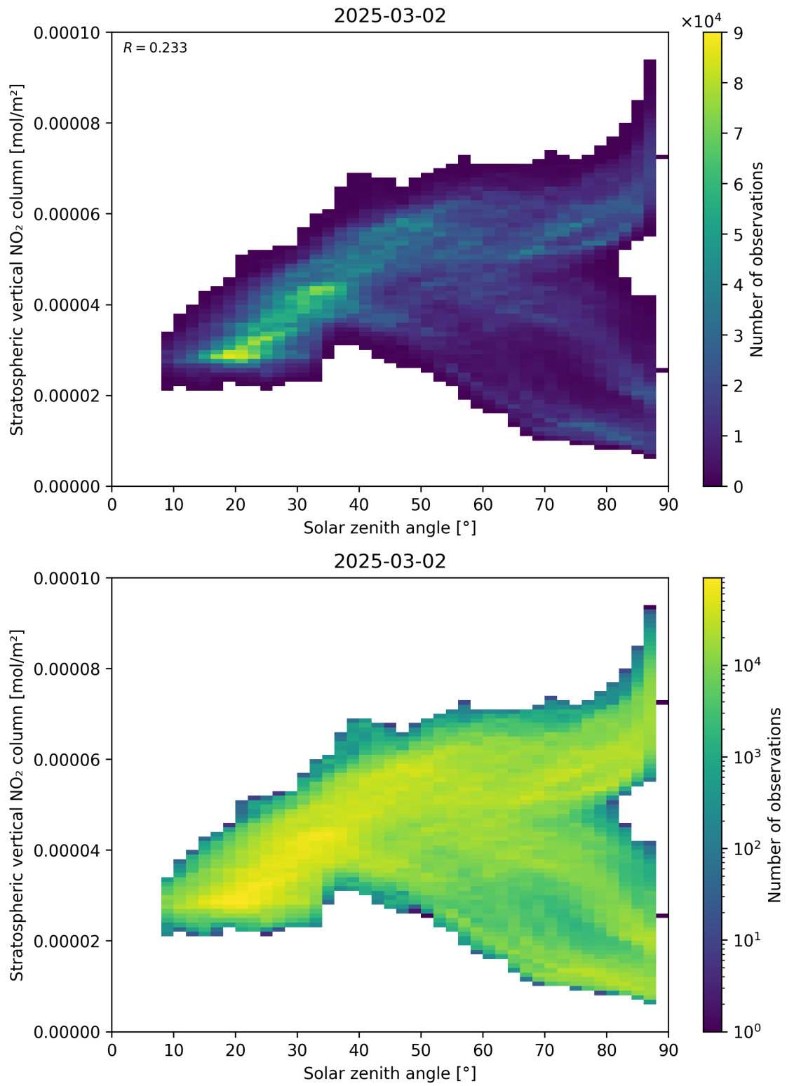
Figure 150: Scatter density plot of “Solar zenith angle” against “Stratospheric vertical NO 2 column” for 2025-03-01 to 2025-03-03.
