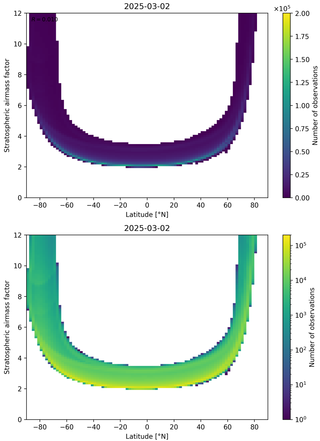
Figure 83: Scatter density plot of “Latitude” against “Stratospheric airmass factor” for 2025-03-01 to 2025-03-03.
