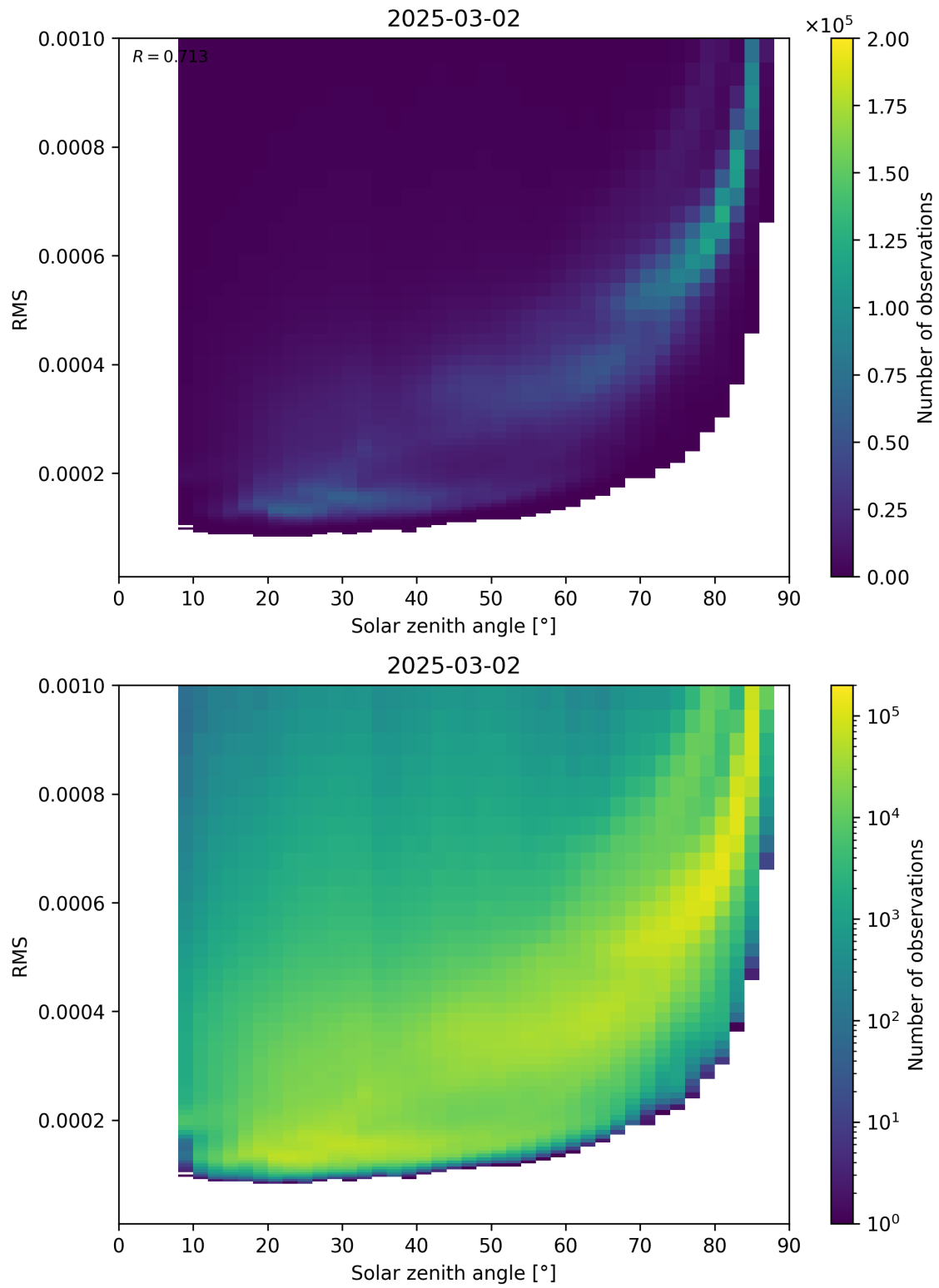
Figure 157: Scatter density plot of “Solar zenith angle” against “RMS” for 2025-03-01 to 2025-03-03.
