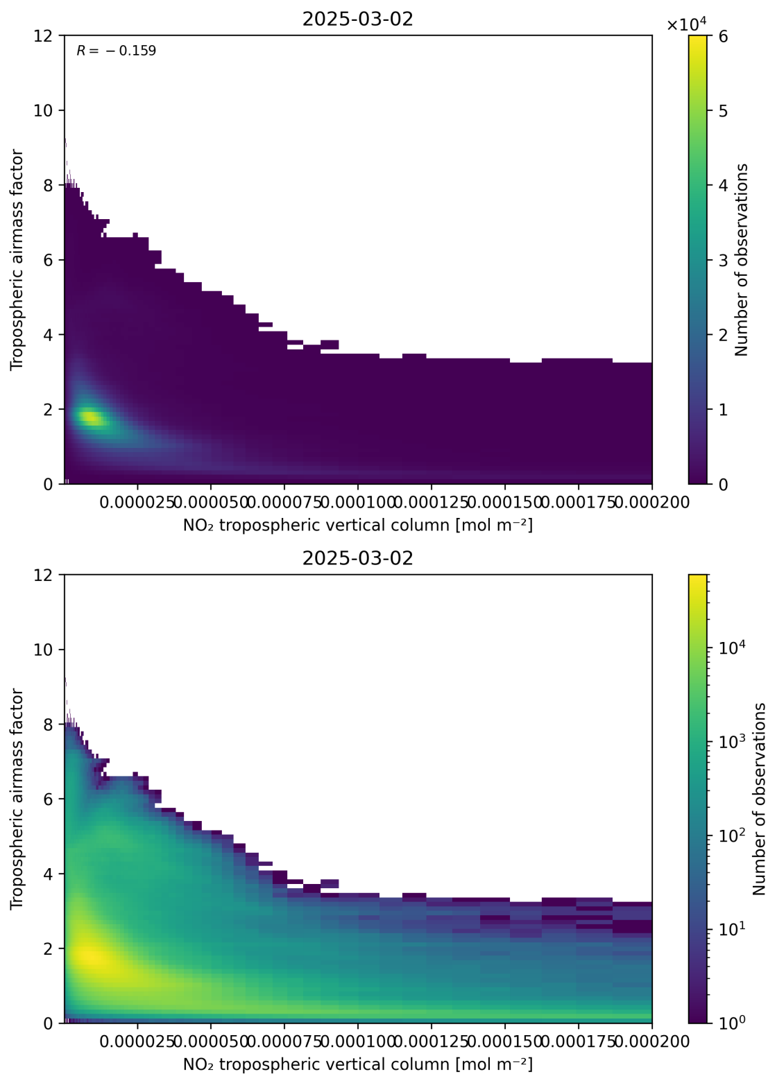
Figure 123: Scatter density plot of “NO 2 tropospheric vertical column” against “Tropospheric air mass factor” for 2025-03-01 to 2025-03-03.
