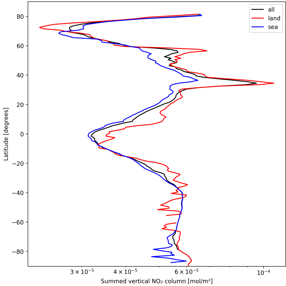
Figure 23: Zonal average of “Summed vertical NO 2 column” for 2025-03-01 to 2025-03-03.
