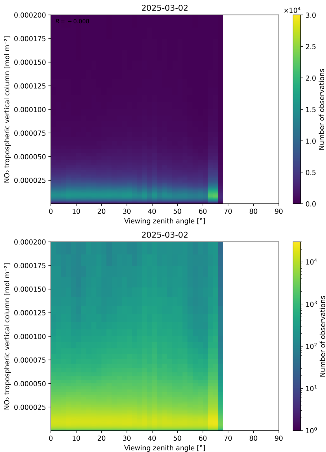
Figure 169: Scatter density plot of “Viewing zenith angle” against “NO 2 tropospheric vertical column” for 2025-03-01 to 2025-03-03.
