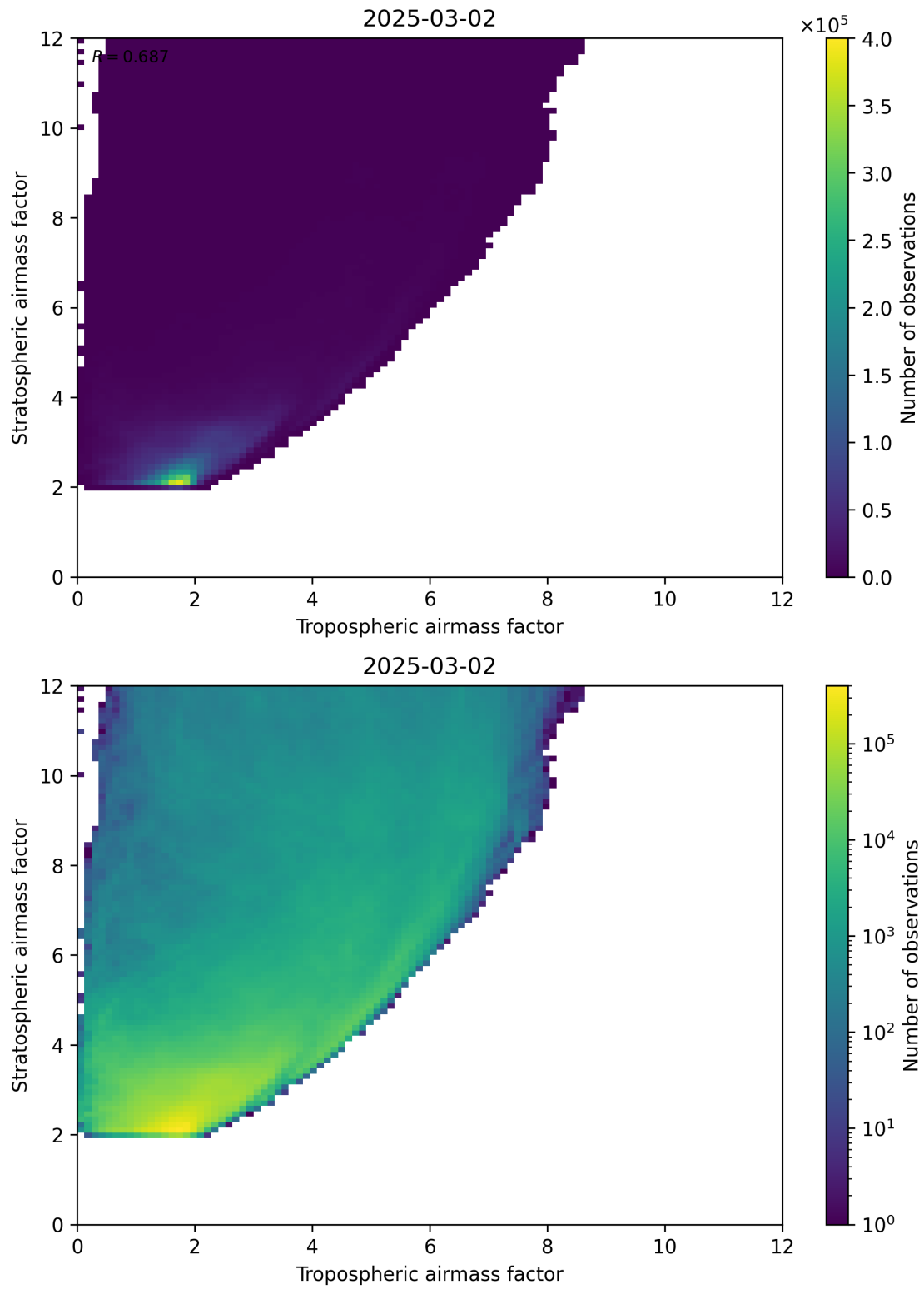
Figure 71: Scatter density plot of “Tropospheric airmass factor” against “Stratospheric airmass factor” for 2025-03-01 to 2025-03-03.
