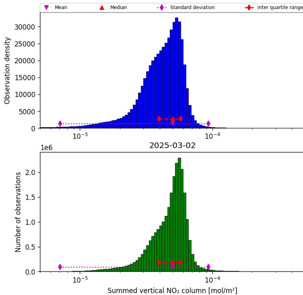
Figure 40: Histogram of “Summed vertical NO 2 column” for 2025-03-01 to 2025-03-03
