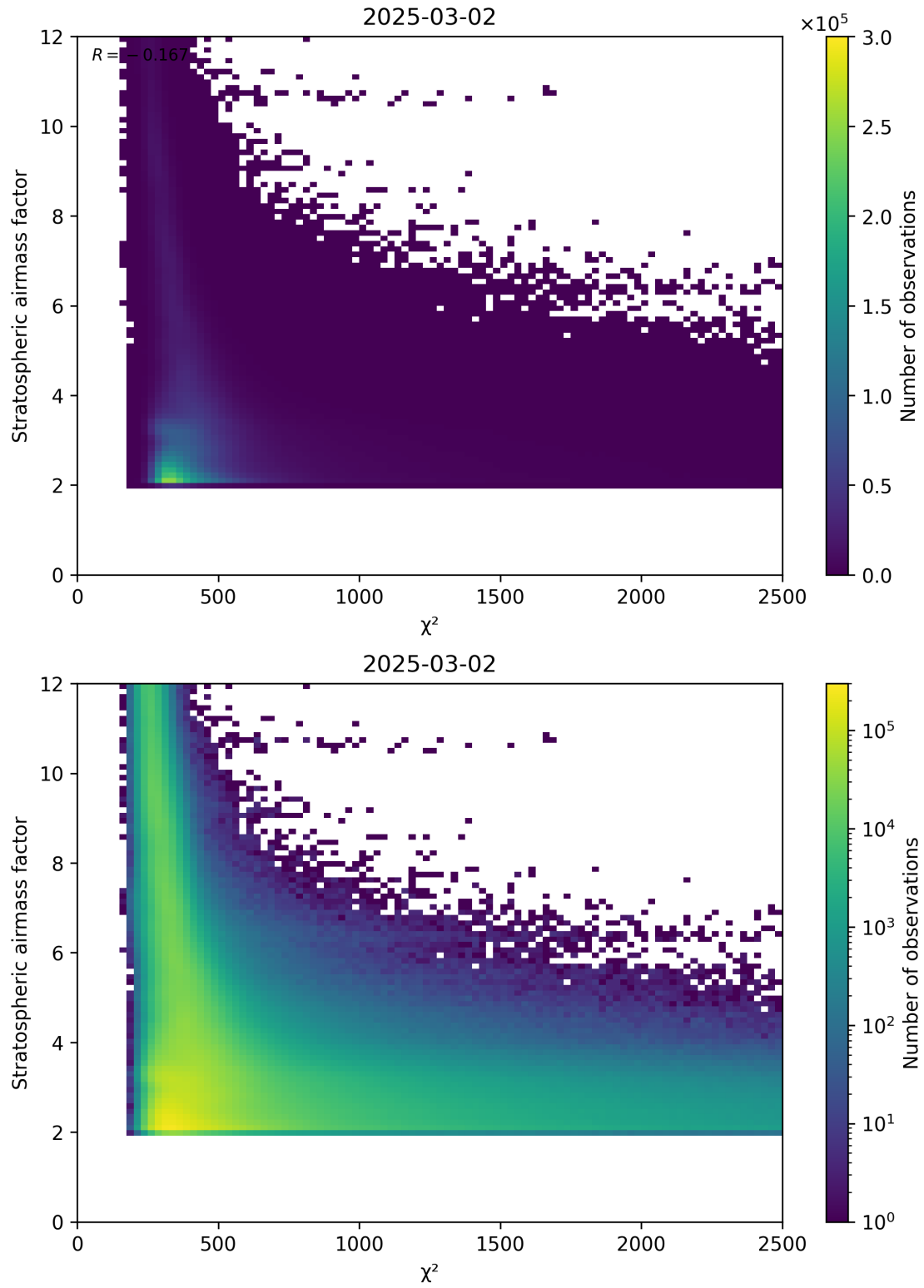
Figure 81: Scatter density plot of “ \chi^2 ” against “Stratospheric airmass factor” for 2025-03-01 to 2025-03-03.
