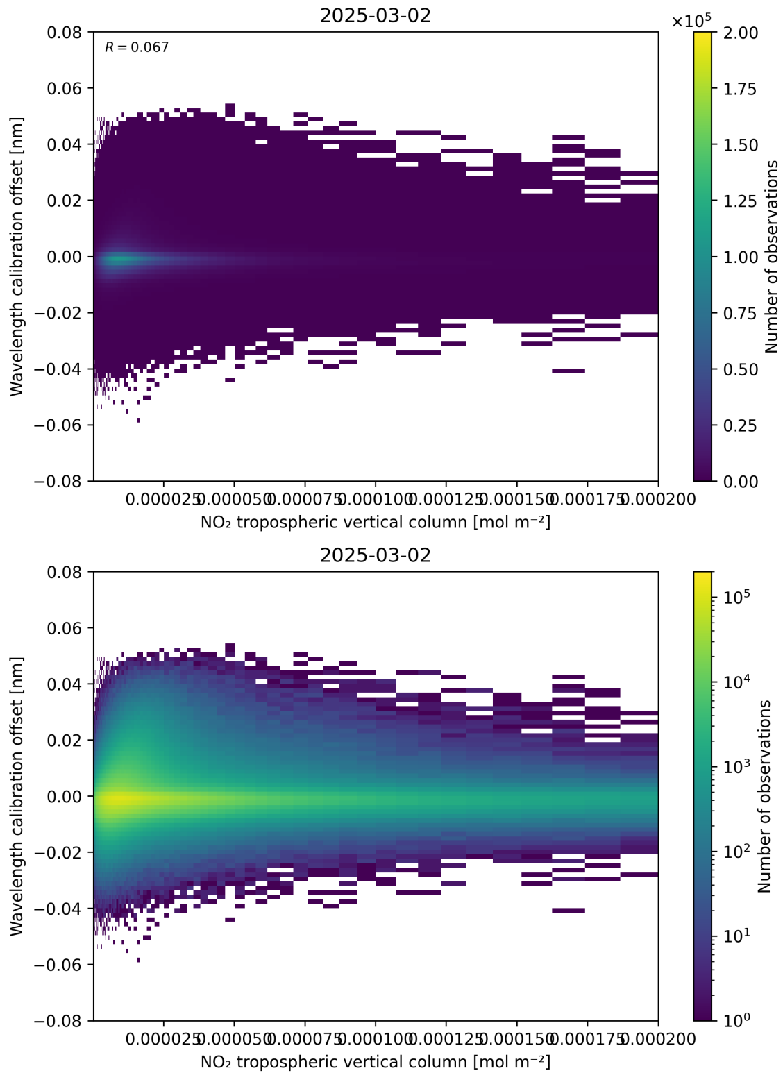
Figure 143: Scatter density plot of “NO 2 tropospheric vertical column” against “Wavelength calibration offset” for 2025-03-01 to 2025-03-03.
