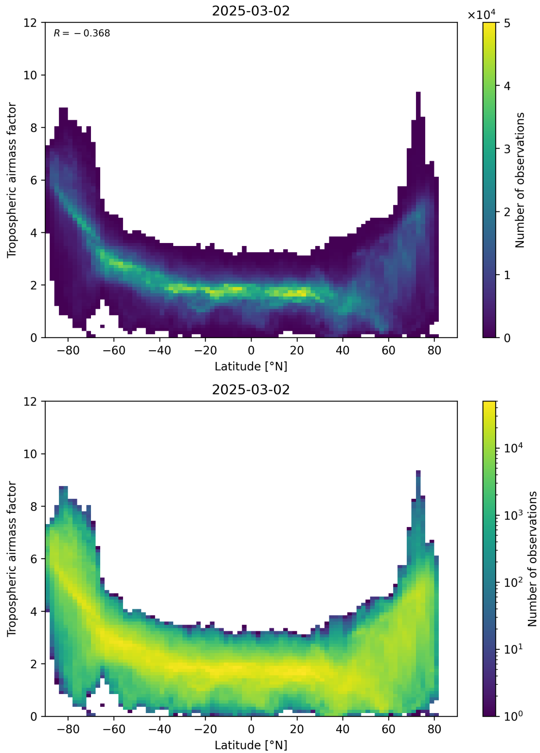
Figure 85: Scatter density plot of “Latitude” against “Tropospheric airmass factor” for 2025-03-01 to 2025-03-03.
