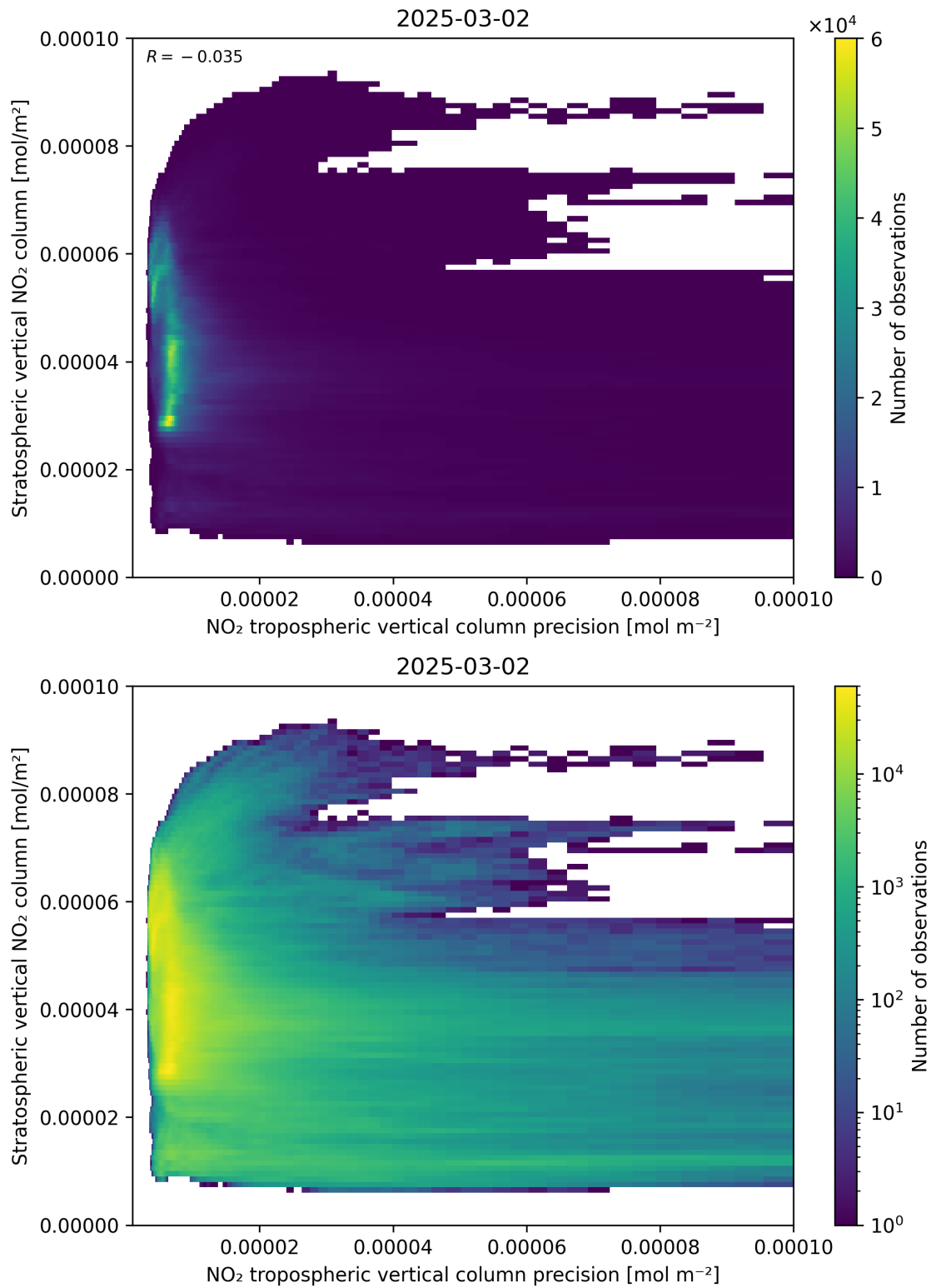
Figure 135: Scatter density plot of “NO 2 tropospheric vertical column precision” against “Stratospheric vertical NO 2 column” for 2025-03-01 to 2025-03-03.
