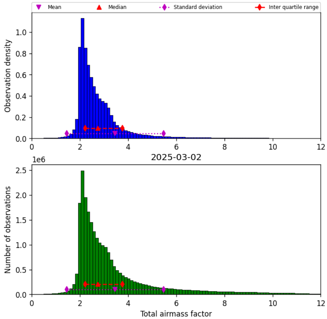
Figure 32: Histogram of “Total airmass factor” for 2025-03-01 to 2025-03-03
