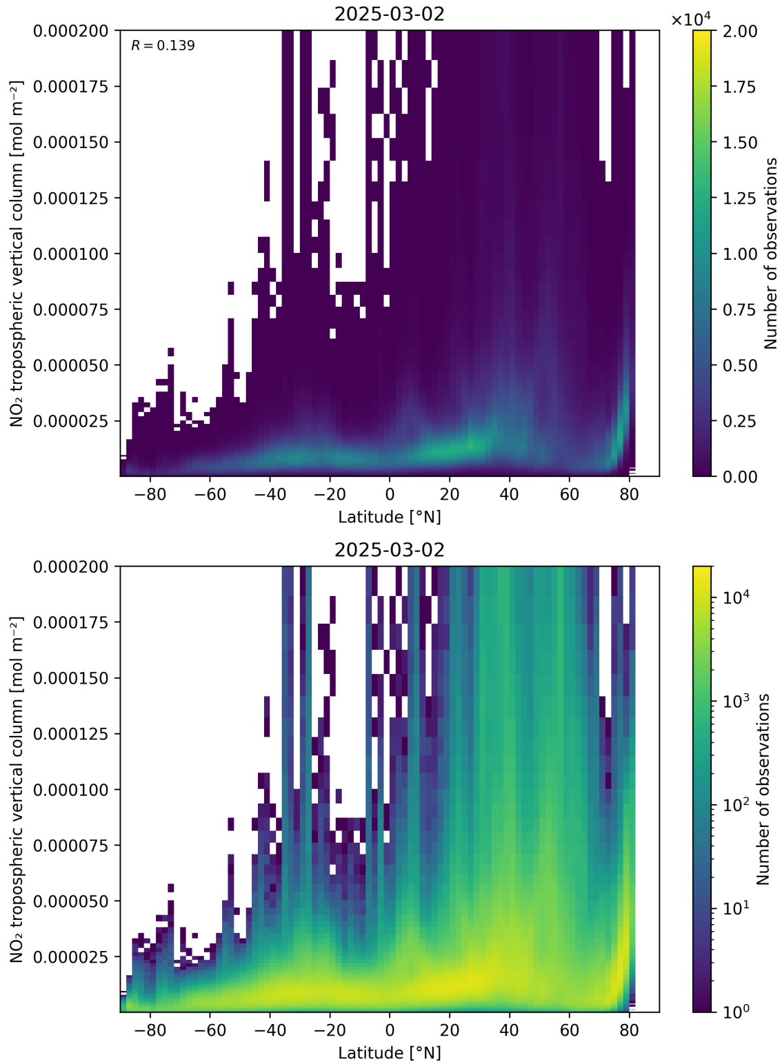
Figure 92: Scatter density plot of “Latitude” against “NO 2 tropospheric vertical column” for 2025-03-01 to 2025-03-03.
