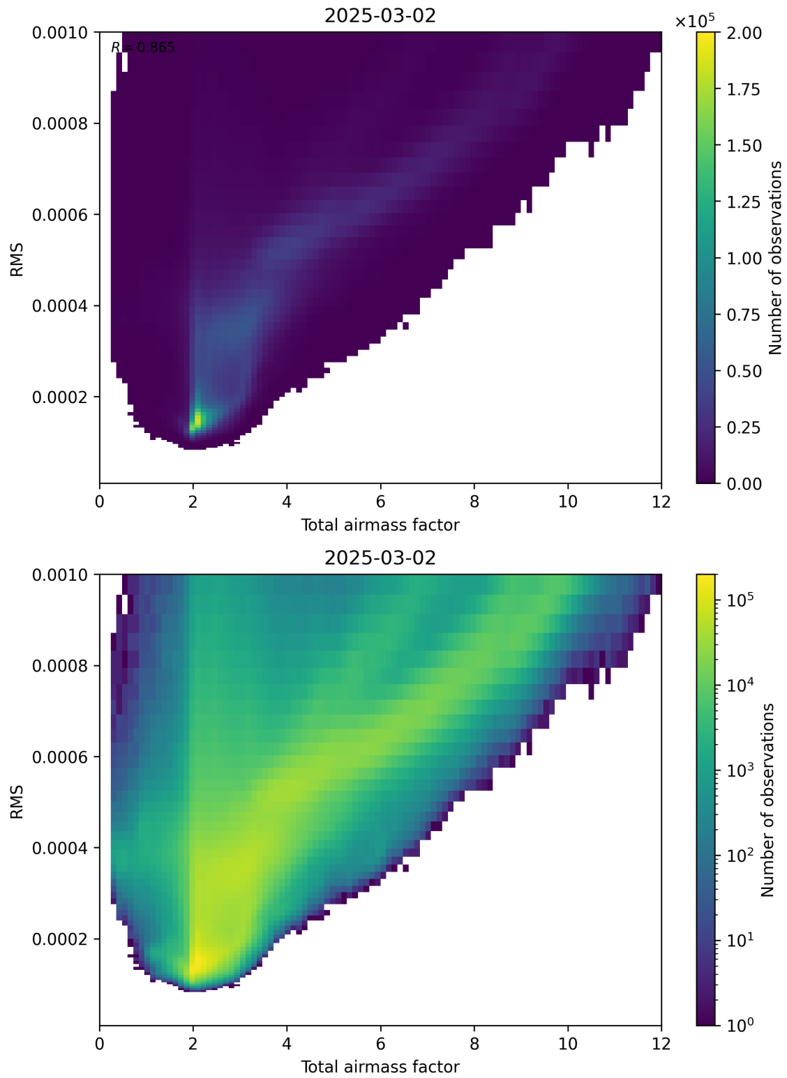
Figure 69: Scatter density plot of “Total airmass factor” against “RMS” for 2025-03-01 to 2025-03-03.
