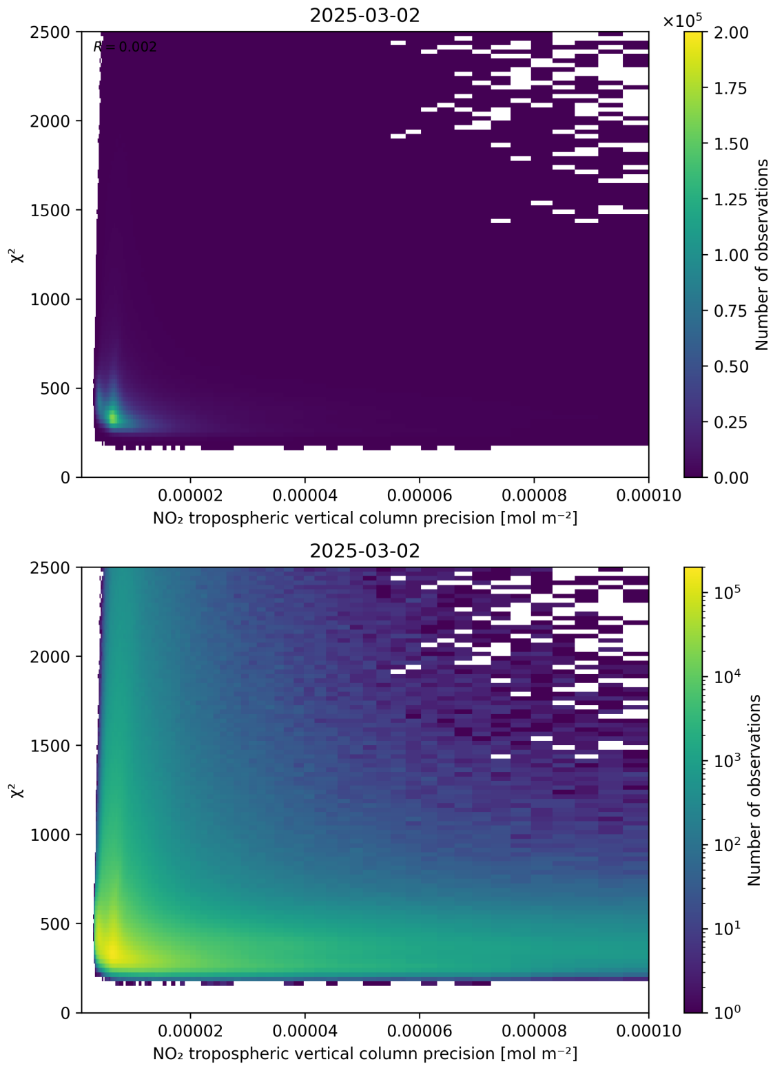
Figure 134: Scatter density plot of "NO 2 tropospheric vertical column precision" against " \chi^2 " for 2025-03-01 to 2025-03-03.
