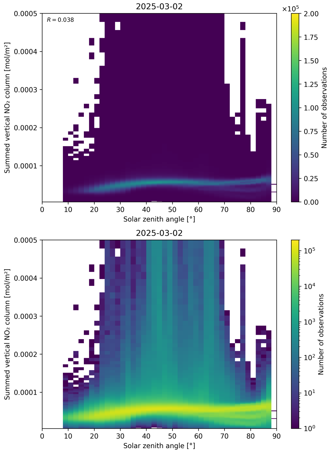
Figure 151: Scatter density plot of “Solar zenith angle” against “Summed vertical NO 2 column” for 2025-03-01 to 2025-03-03.
