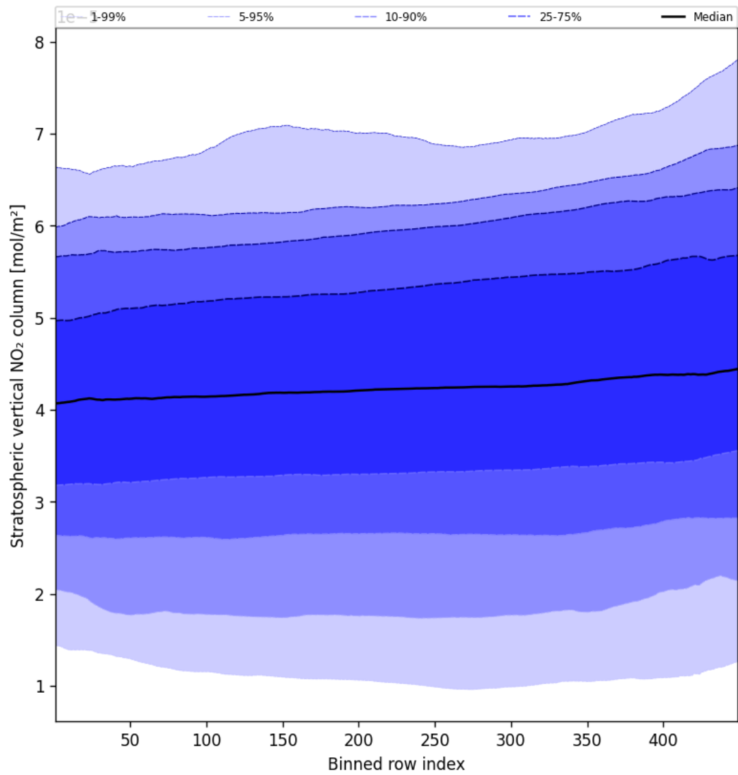
Figure 53: Along track statistics of “Stratospheric vertical NO 2 column” for 2025-03-01 to 2025-03-03
