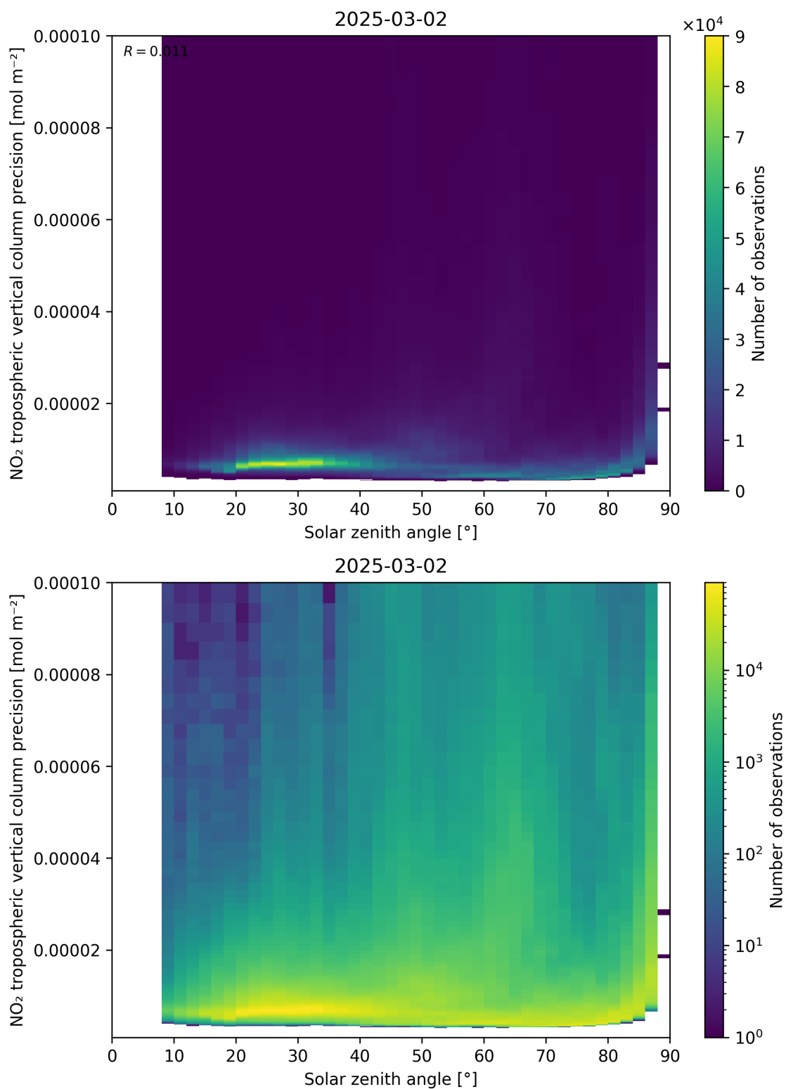
Figure 156: Scatter density plot of “Solar zenith angle” against “NO 2 tropospheric vertical column precision” for 2025-03-01 to 2025-03-03.
