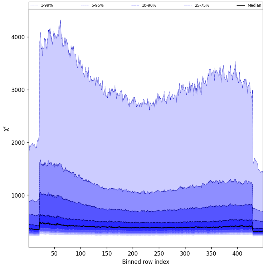
Figure 59: Along track statistics of “ \chi^2 ” for 2025-03-01 to 2025-03-03
