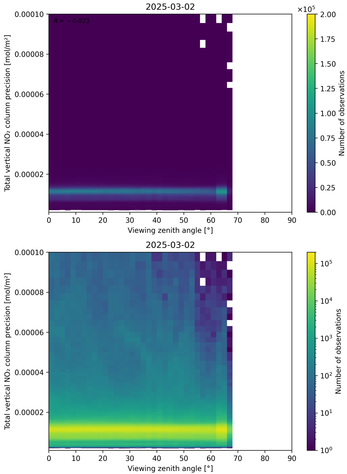
Figure 168: Scatter density plot of “Viewing zenith angle” against “Total vertical NO 2 column precision” for 2025-03-01 to 2025-03-03.
