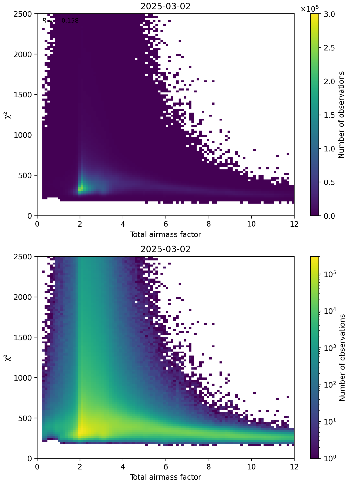
Figure 63: Scatter density plot of “Total airmass factor” against “ \chi^2 ” for 2025-03-01 to 2025-03-03.
