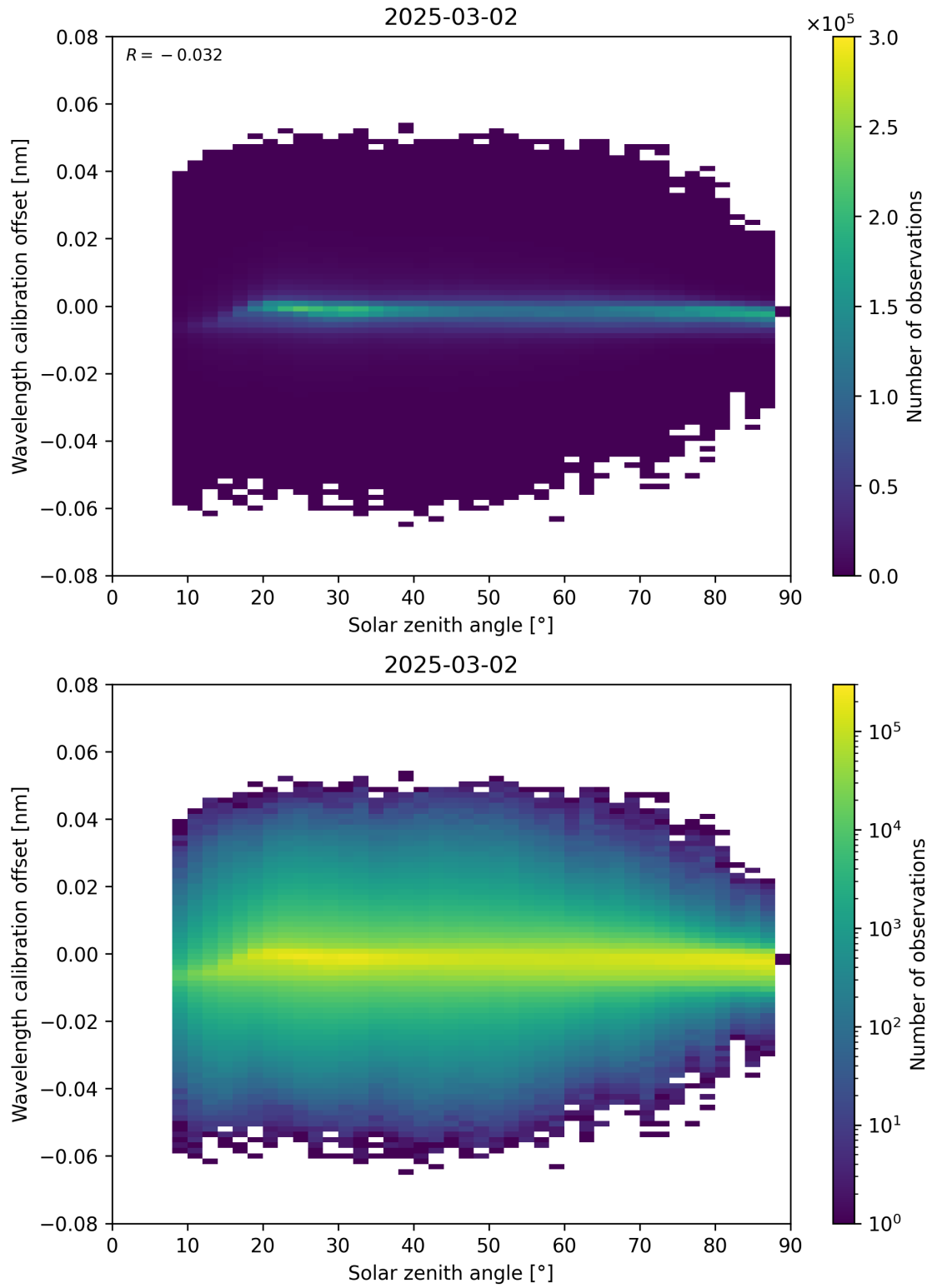
Figure 158: Scatter density plot of “Solar zenith angle” against “Wavelength calibration offset” for 2025-03-01 to 2025-03-03.
