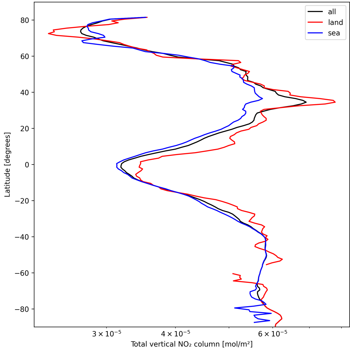
Figure 21: Zonal average of “Total vertical NO 2 column” for 2025-03-01 to 2025-03-03.
