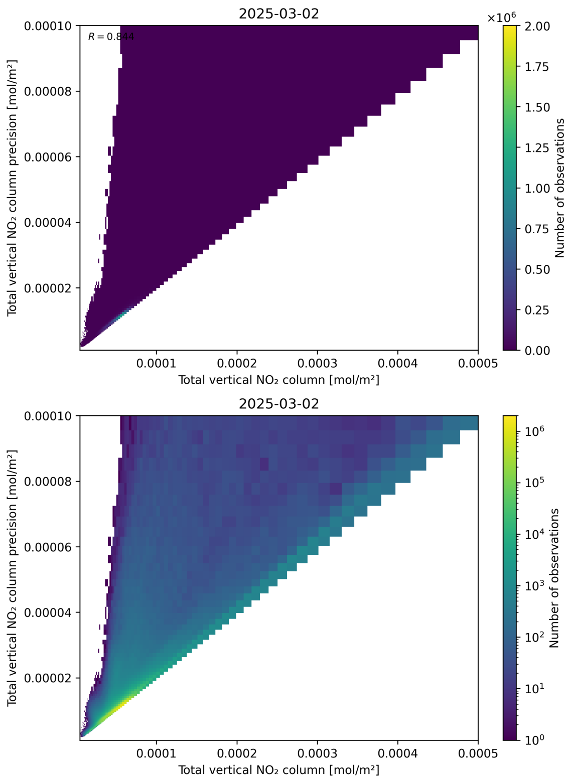
Figure 114: Scatter density plot of “Total vertical NO 2 column” against “Total vertical NO 2 column precision” for 2025-03-01 to 2025-03-03.
