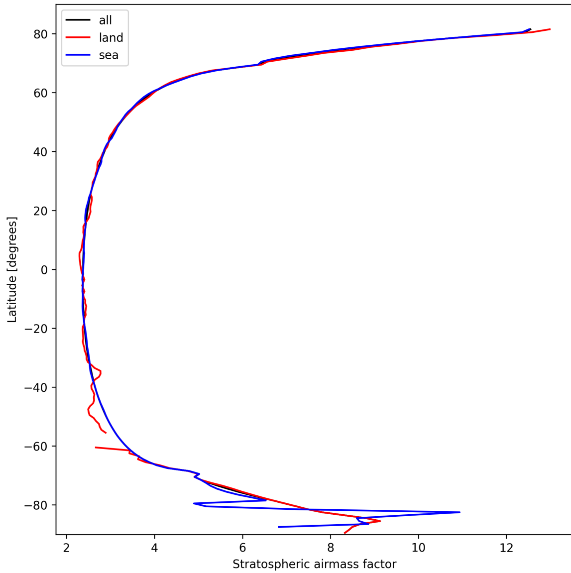
Figure 27: Zonal average of “Stratospheric air mass factor” for 2025-03-01 to 2025-03-03.
