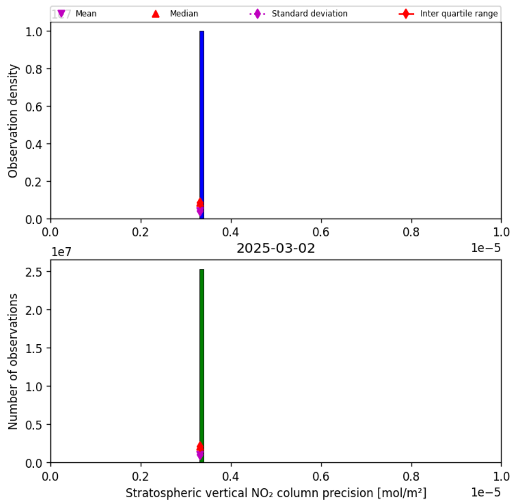
Figure 37: Histogram of “Stratospheric vertical NO 2 column precision” for 2025-03-01 to 2025-03-03
