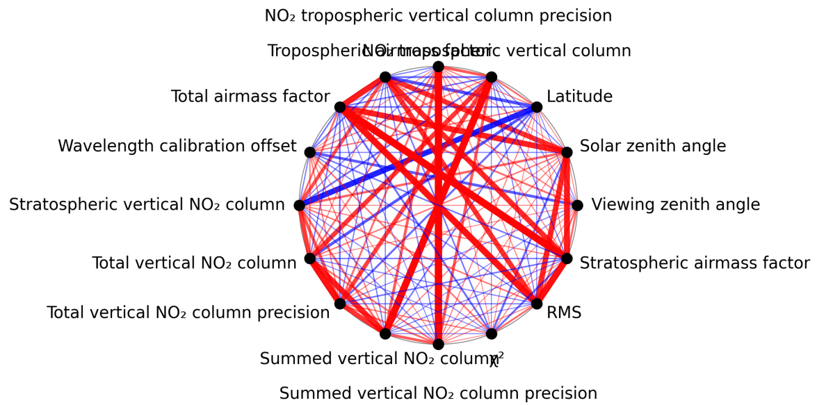
Figure 1: Map of correlation graph for 2025-03-01 to 2025-03-03.
