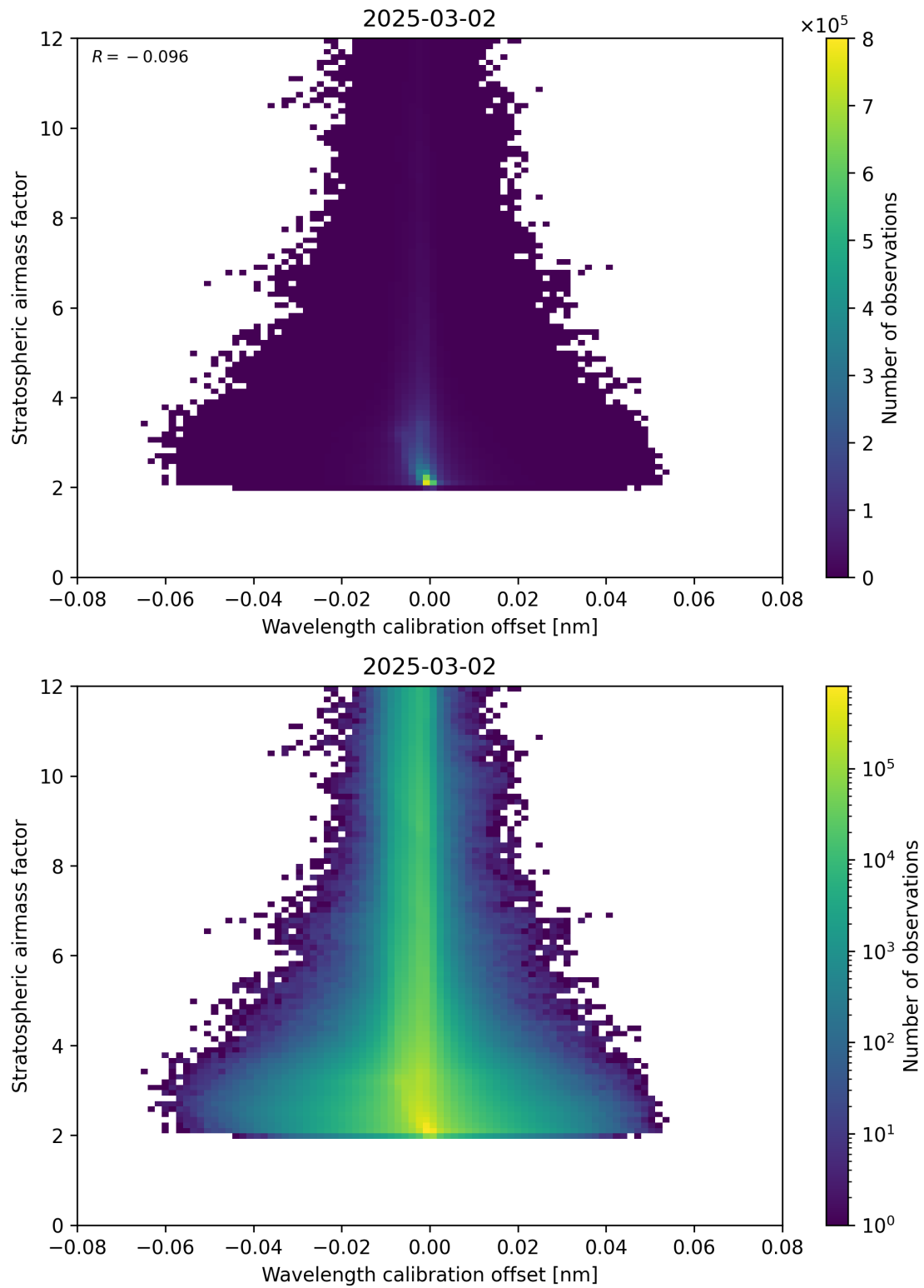
Figure 174: Scatter density plot of “Wavelength calibration offset” against “Stratospheric airmass factor” for 2025-03-01 to 2025-03-03.
