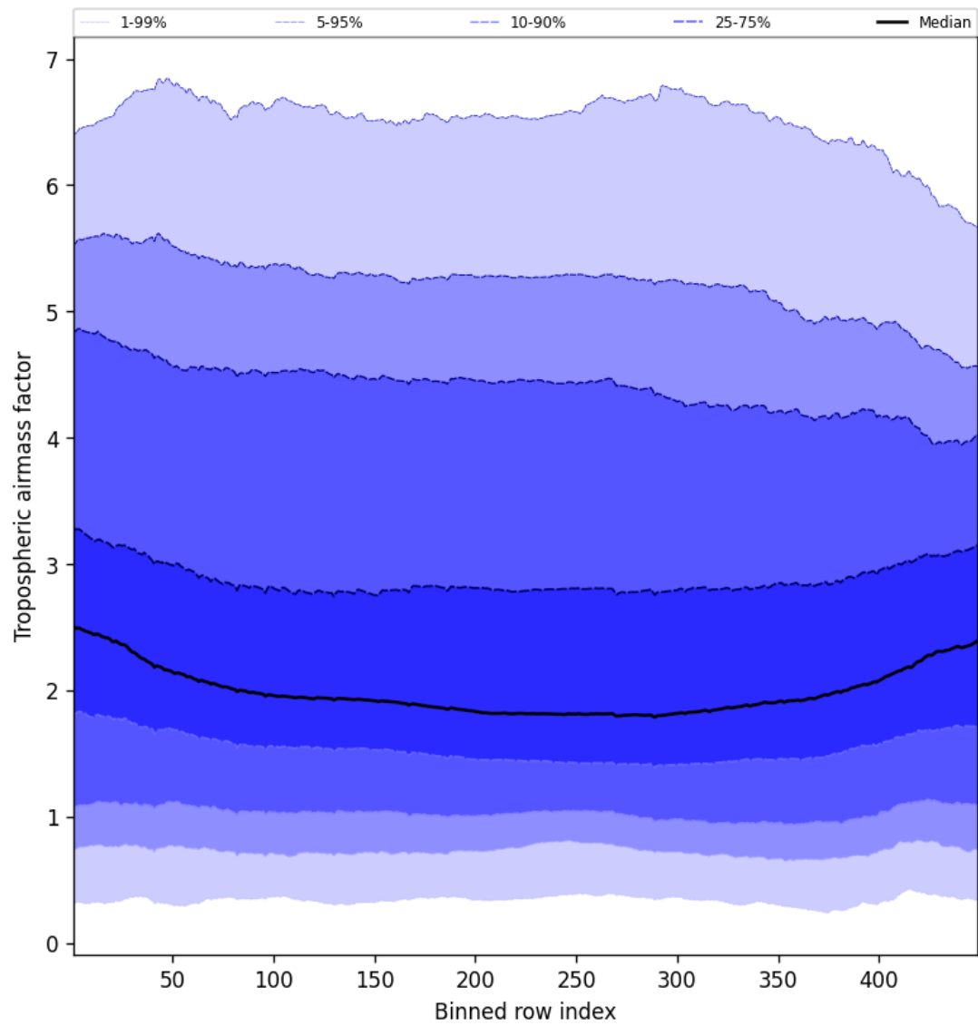
Figure 48: Along track statistics of “Tropospheric airmass factor” for 2025-03-01 to 2025-03-03
