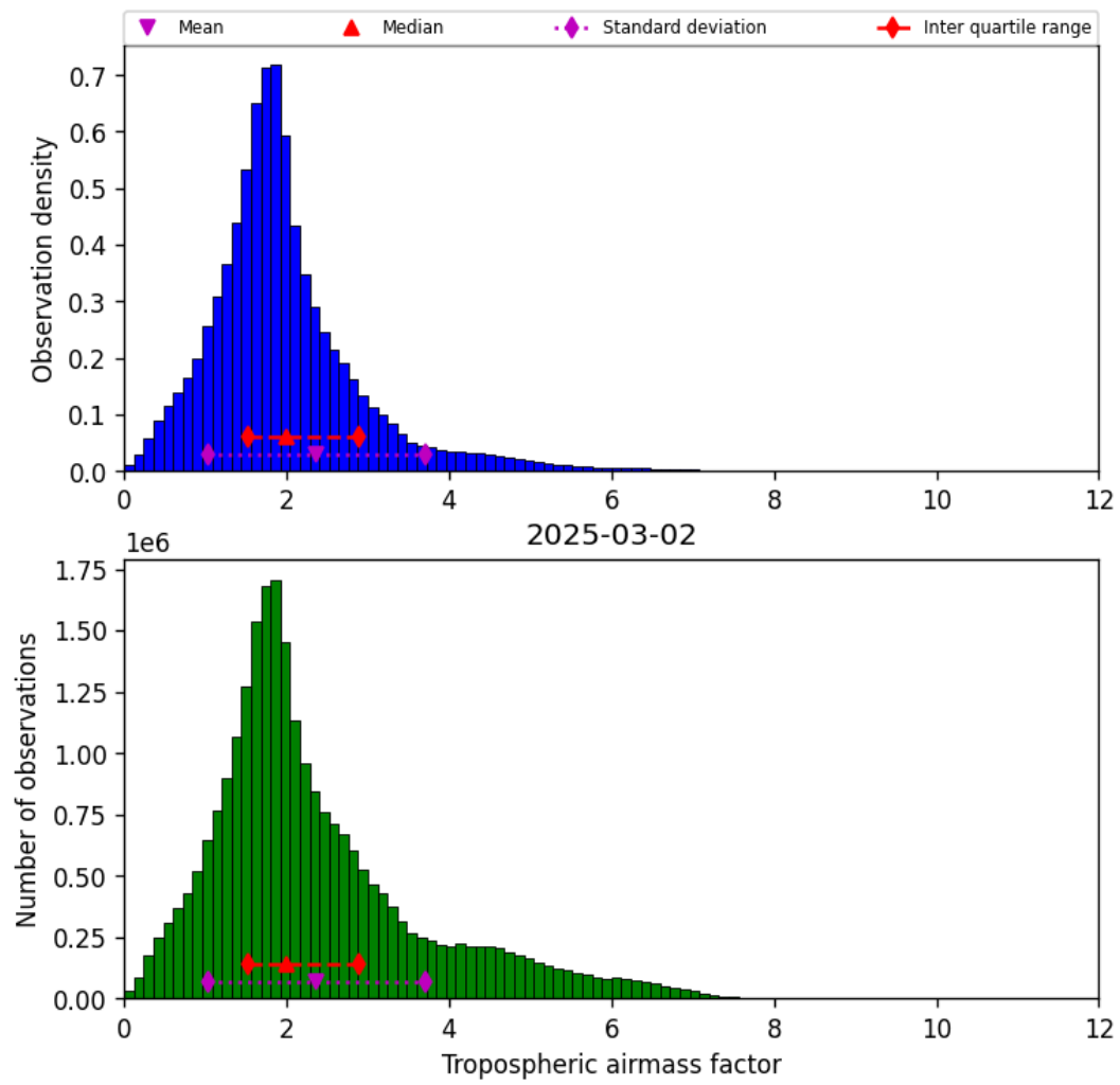
Figure 31: Histogram of “Tropospheric airmass factor” for 2025-03-01 to 2025-03-03
