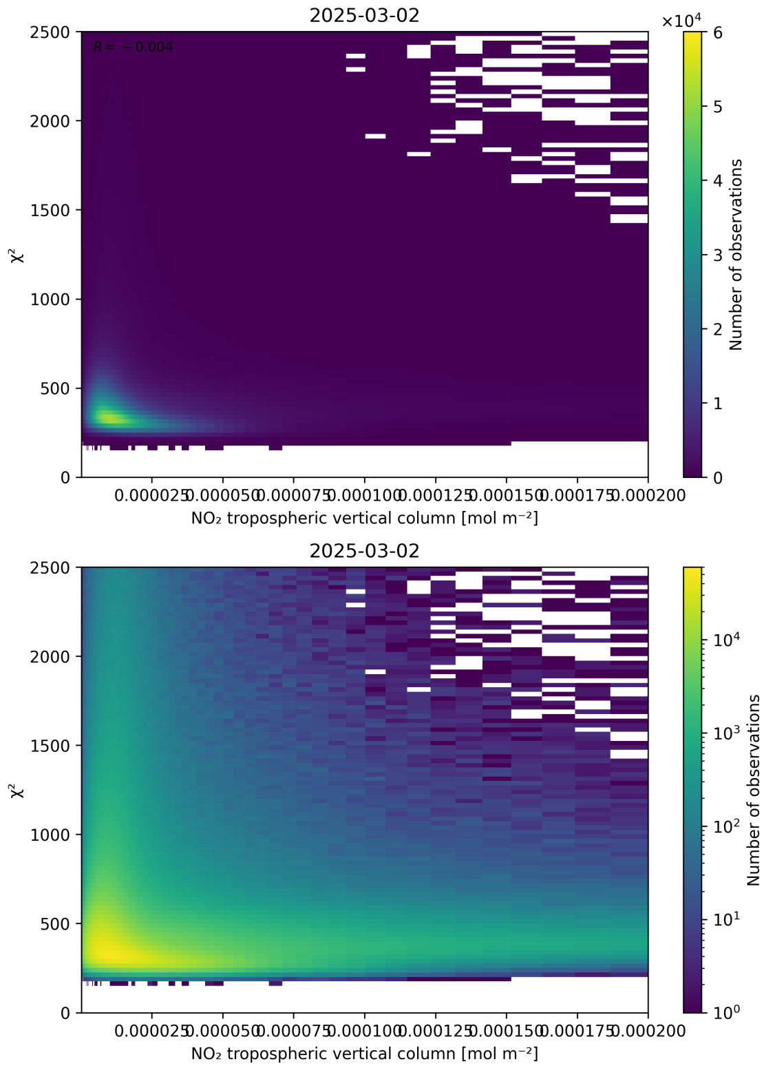
Figure 124: Scatter density plot of “NO 2 tropospheric vertical column” against “ \chi^2 ” for 2025-03-01 to 2025-03-03.
