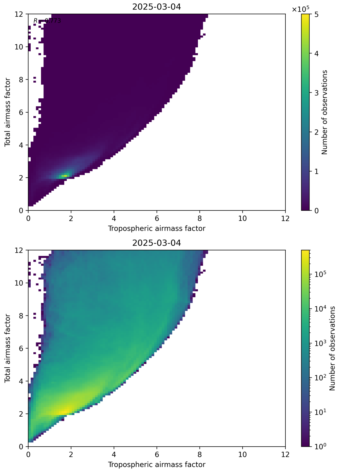
Figure 72: Scatter density plot of “Tropospheric airmass factor” against “Total airmass factor” for 2025-03-03 to 2025-03-05.
