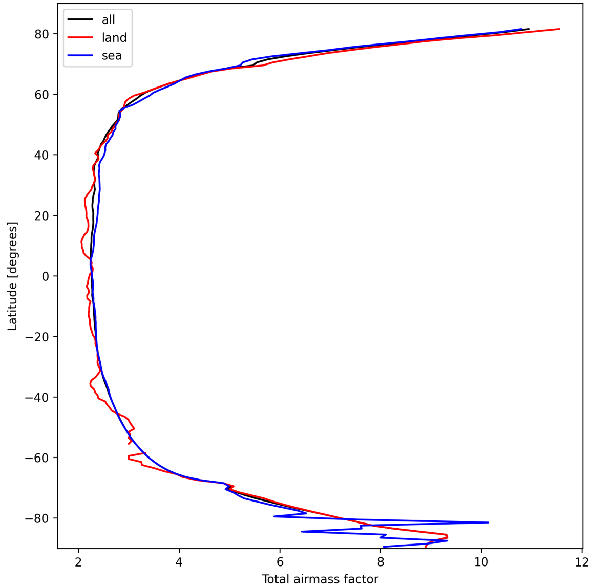
Figure 15: Zonal average of “Total airmass factor” for 2025-03-03 to 2025-03-05.
