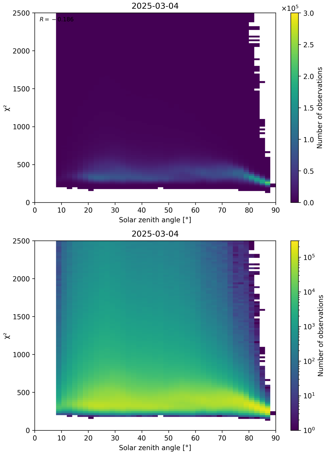
Figure 148: Scatter density plot of “Solar zenith angle” against “ \chi^2 ” for 2025-03-03 to 2025-03-05.
