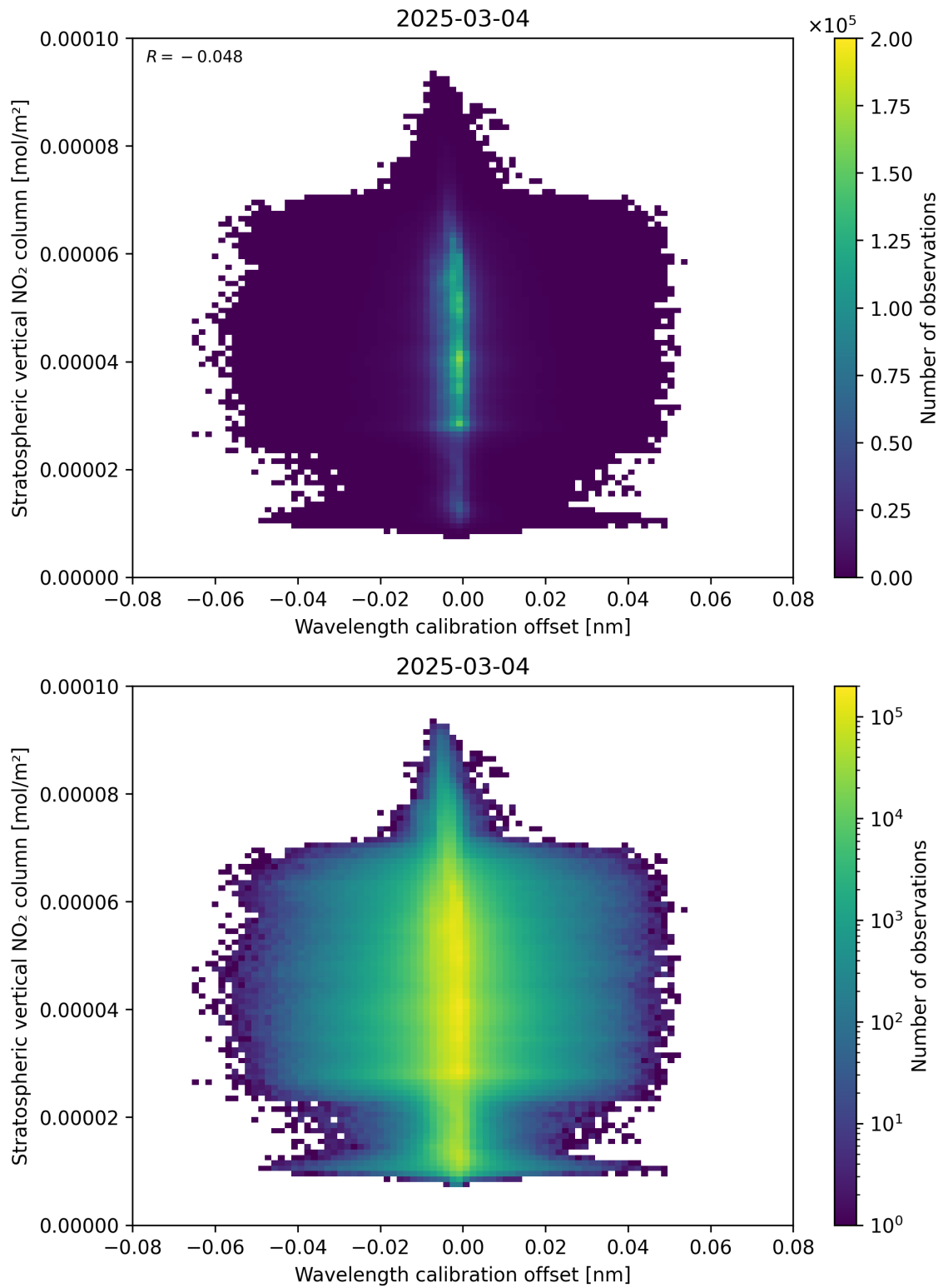
Figure 176: Scatter density plot of “Wavelength calibration offset” against “Stratospheric vertical NO 2 column” for 2025-03-03 to 2025-03-05.
