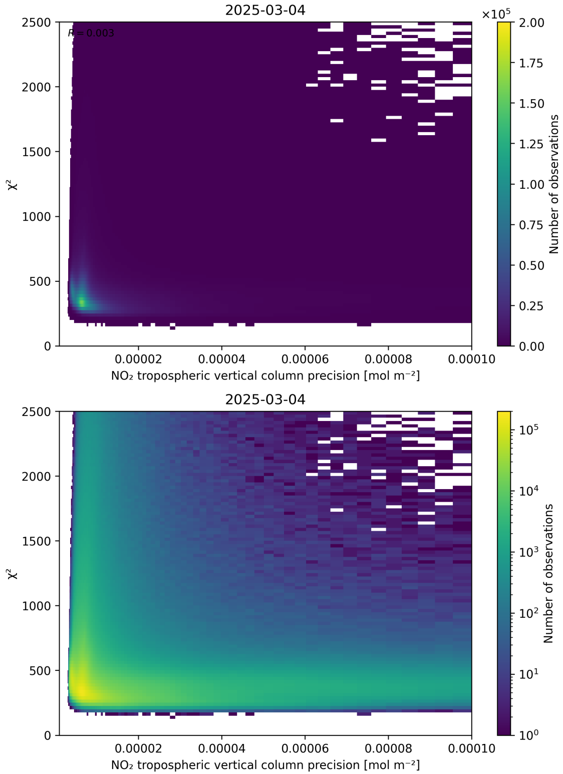
Figure 134: Scatter density plot of “NO 2 tropospheric vertical column precision” against “ \chi^2 ” for 2025-03-03 to 2025-03-05.
