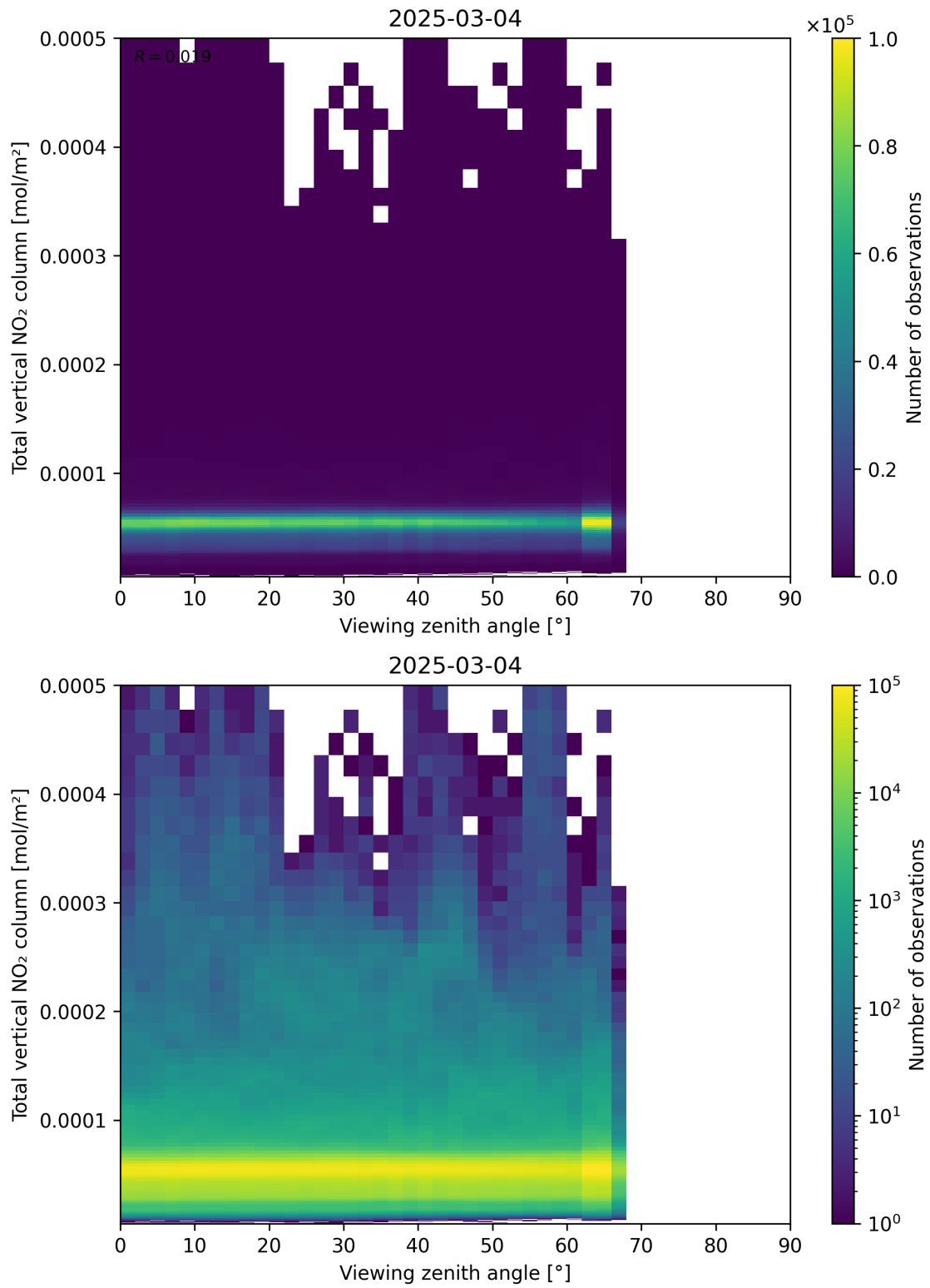
Figure 167: Scatter density plot of “Viewing zenith angle” against “Total vertical NO 2 column” for 2025-03-03 to 2025-03-05.
