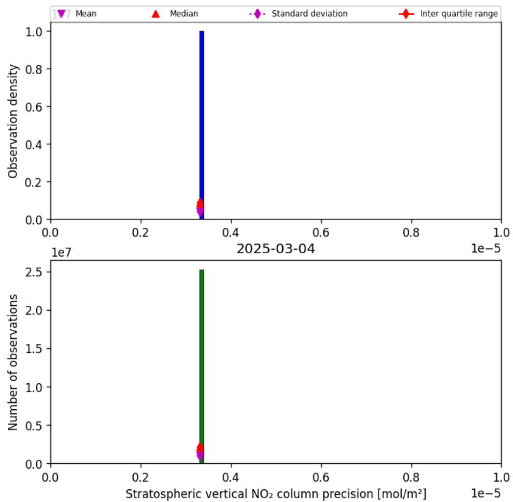
Figure 37: Histogram of “Stratospheric vertical NO 2 column precision” for 2025-03-03 to 2025-03-05
