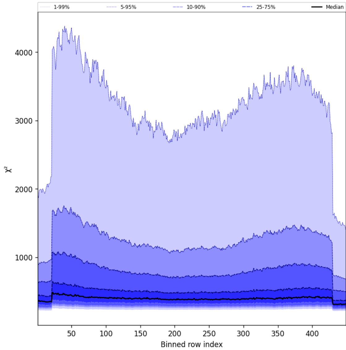
Figure 59: Along track statistics of “ \chi^2 ” for 2025-03-03 to 2025-03-05
