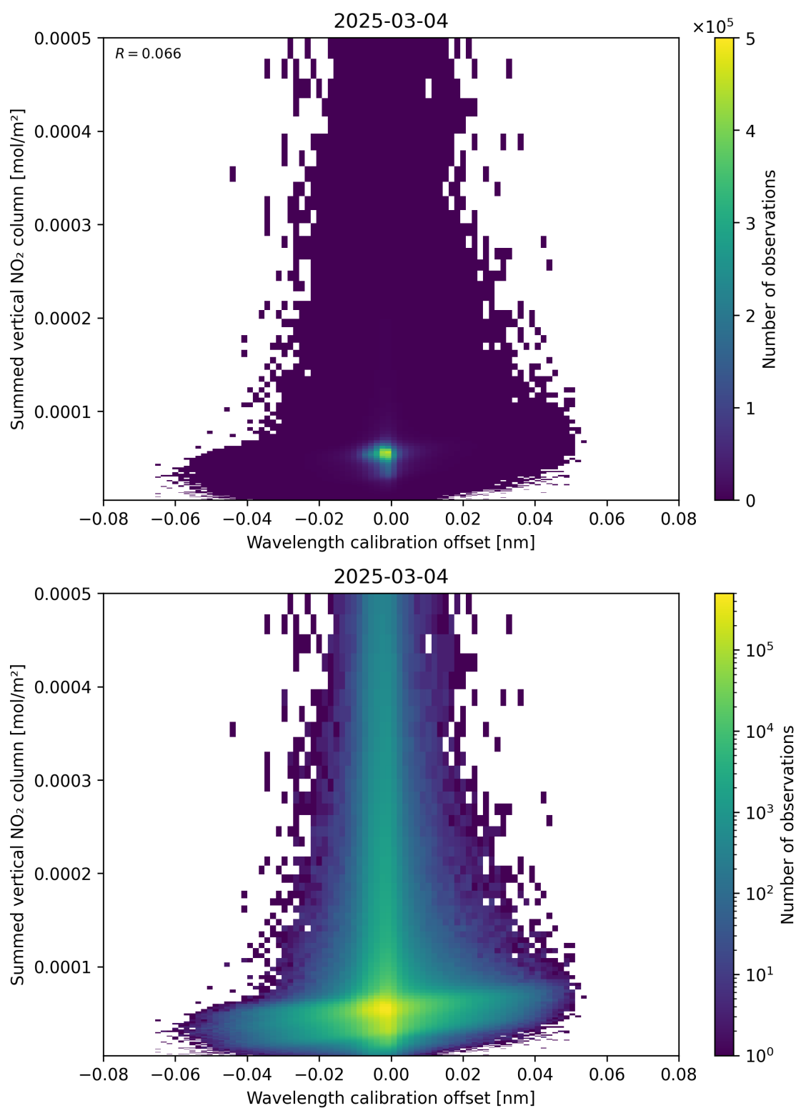
Figure 177: Scatter density plot of “Wavelength calibration offset” against “Summed vertical NO 2 column” for 2025-03-03 to 2025-03-05.
