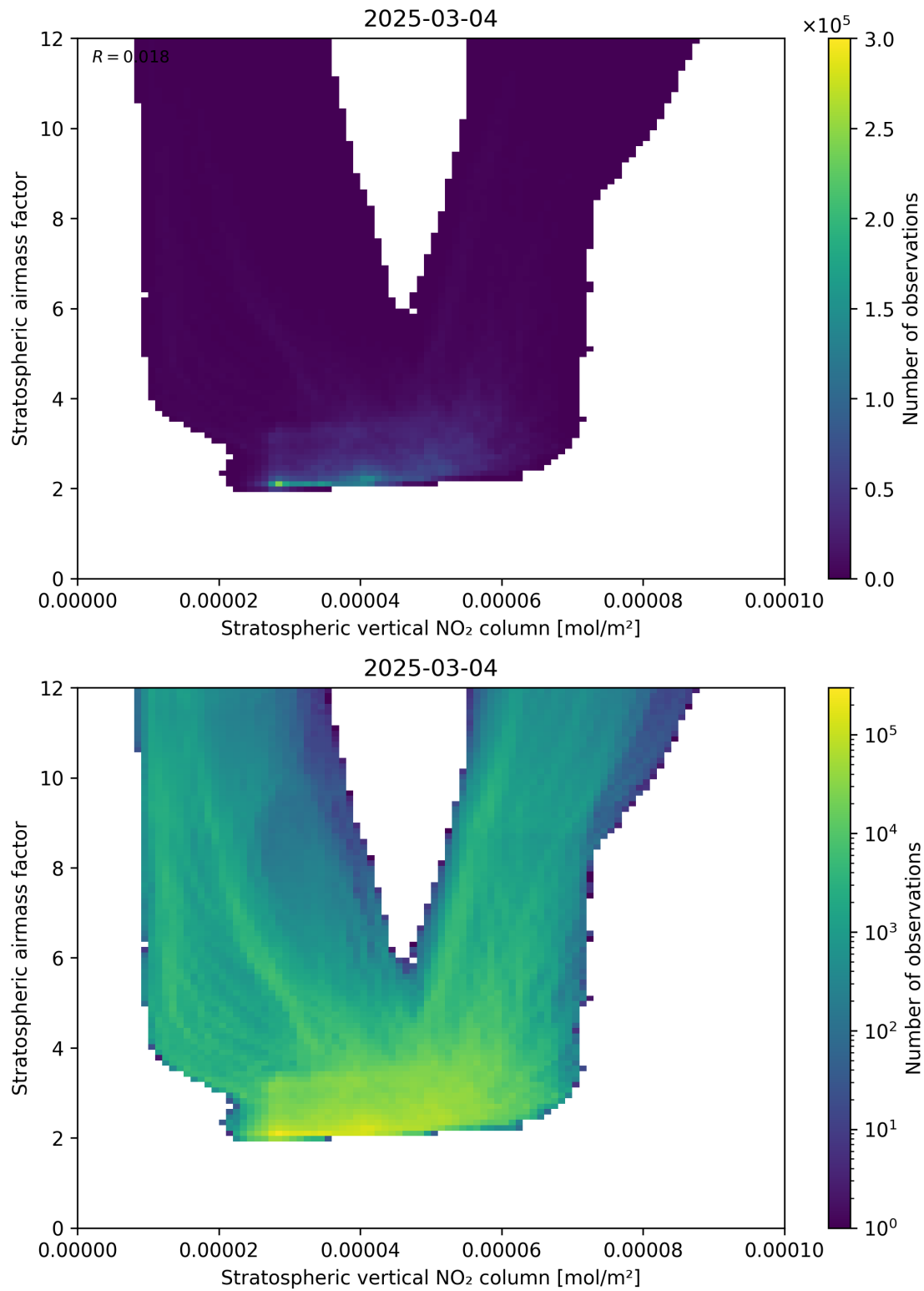
Figure 96: Scatter density plot of “Stratospheric vertical NO 2 column” against “Stratospheric airmass factor” for 2025-03-03 to 2025-03-05.
