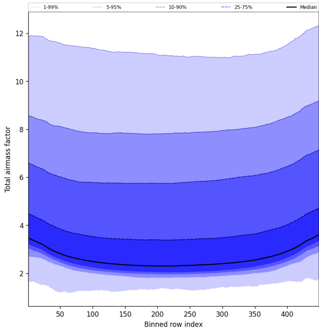
Figure 49: Along track statistics of “Total airmass factor” for 2025-03-03 to 2025-03-05
