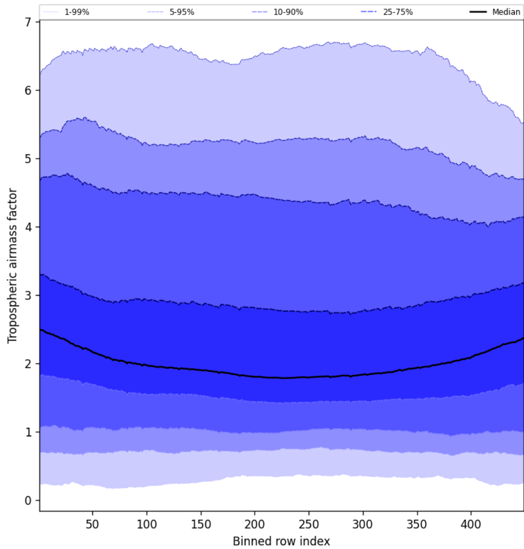
Figure 48: Along track statistics of “Tropospheric air mass factor” for 2025-03-03 to 2025-03-05
