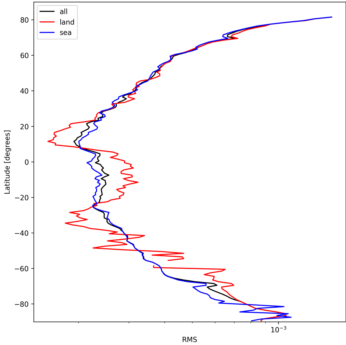
Figure 26: Zonal average of “RMS” for 2025-03-03 to 2025-03-05.
