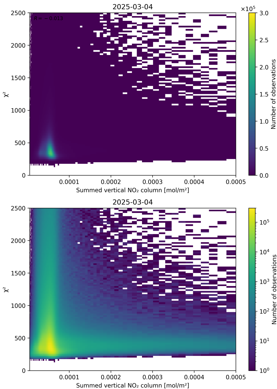
Figure 104: Scatter density plot of “Summed vertical NO 2 column” against “ \chi^2 ” for 2025-03-03 to 2025-03-05.
