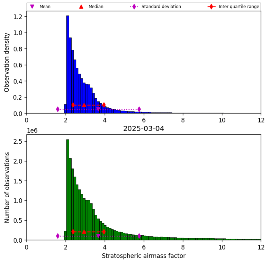
Figure 44: Histogram of “Stratospheric airmass factor” for 2025-03-03 to 2025-03-05
