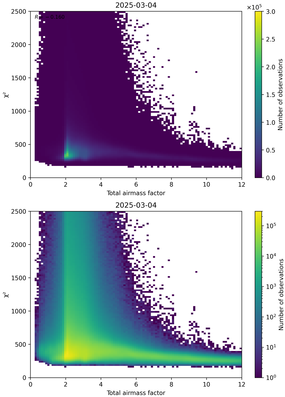
Figure 63: Scatter density plot of “Total airmass factor” against “ \chi^2 ” for 2025-03-03 to 2025-03-05.
