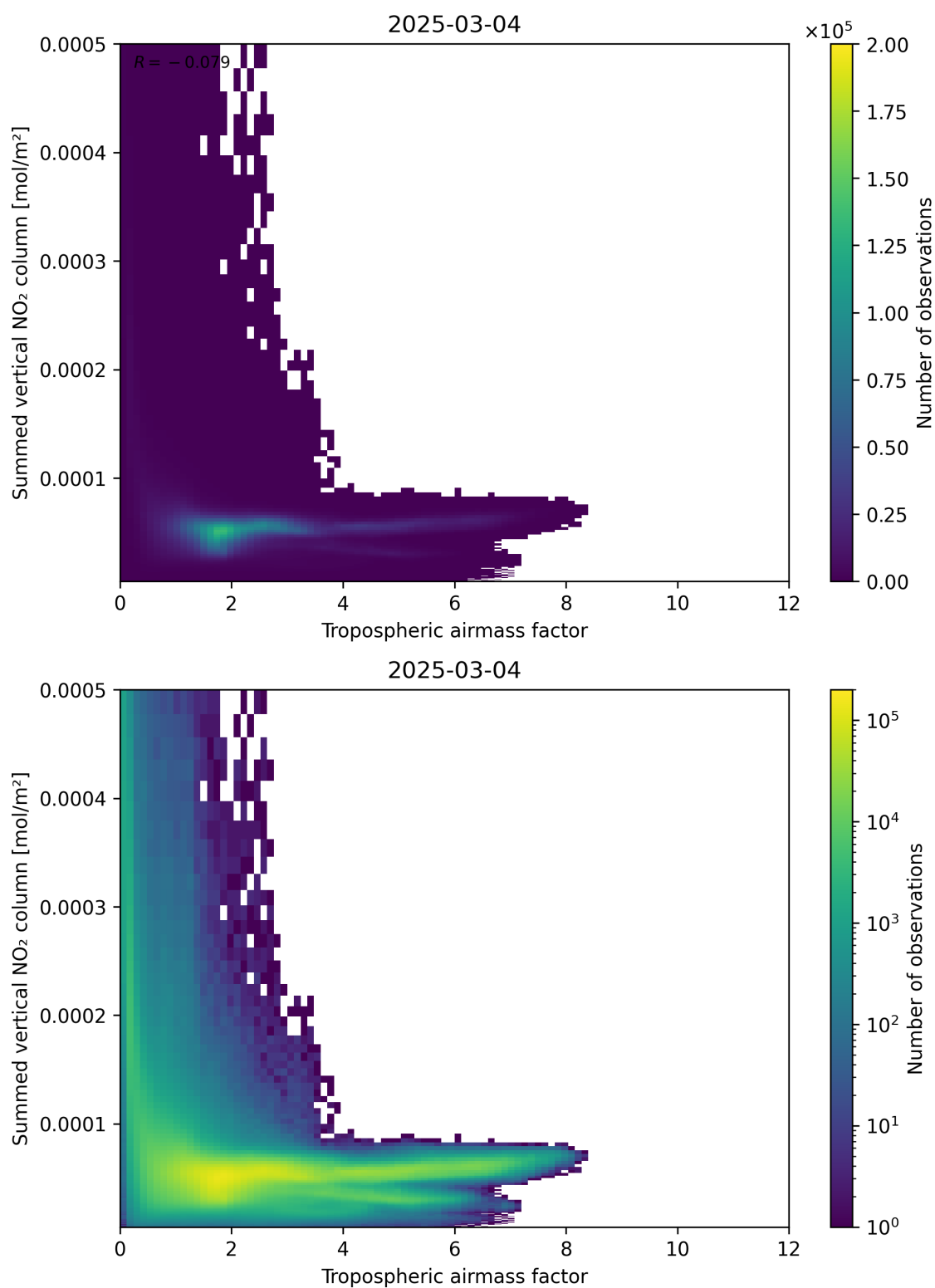
Figure 75: Scatter density plot of “Tropospheric air mass factor” against “Summed vertical NO 2 column” for 2025-03-03 to 2025-03-05.
