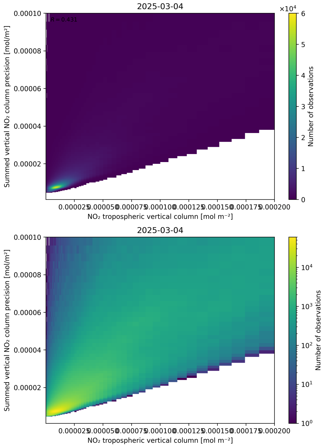
Figure 127: Scatter density plot of “NO 2 tropospheric vertical column” against “Summed vertical NO 2 column precision” for 2025-03-03 to 2025-03-05.
