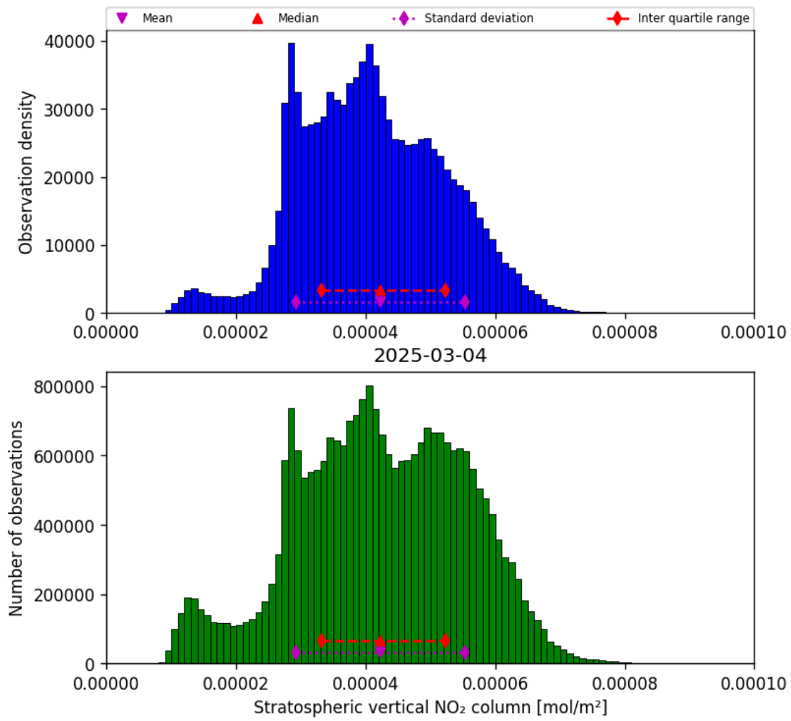
Figure 36: Histogram of “Stratospheric vertical NO 2 column” for 2025-03-03 to 2025-03-05
