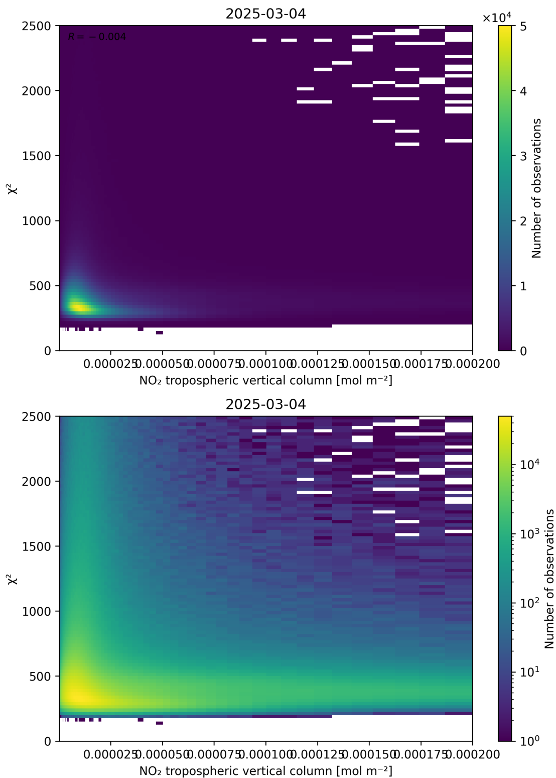
Figure 124: Scatter density plot of “NO 2 tropospheric vertical column” against “ \chi^2 ” for 2025-03-03 to 2025-03-05.
