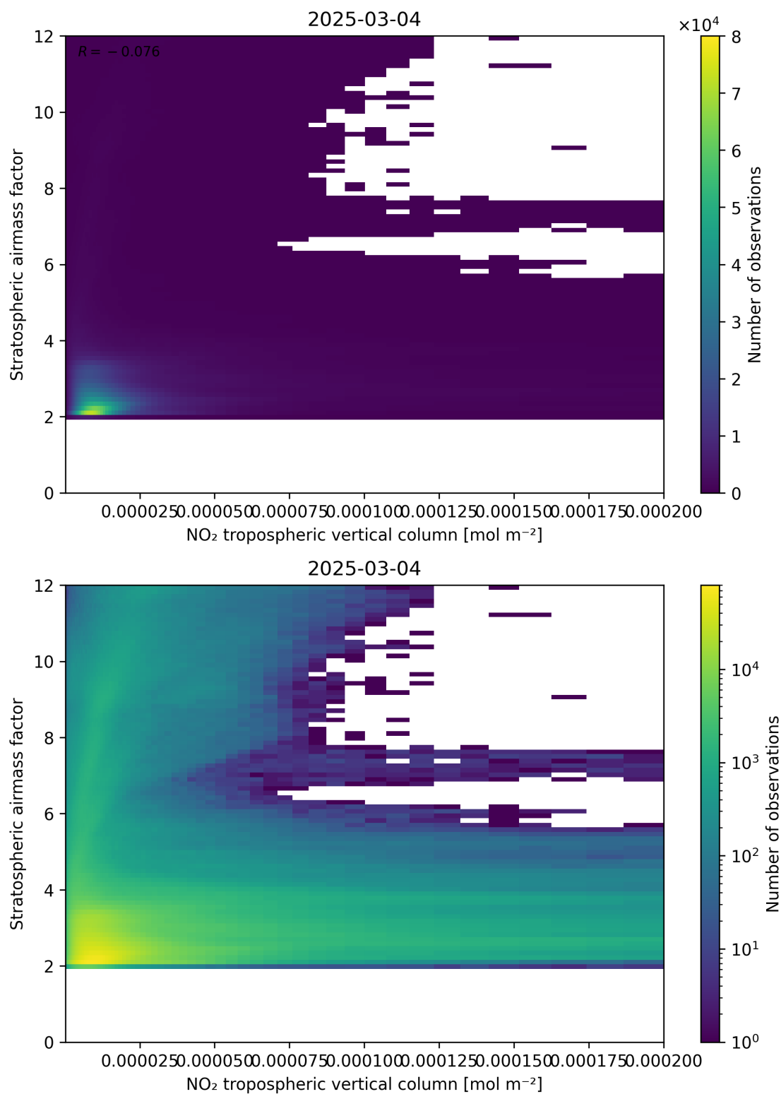
Figure 121: Scatter density plot of “NO 2 tropospheric vertical column” against “Stratospheric air mass factor” for 2025-03-03 to 2025-03-05.
