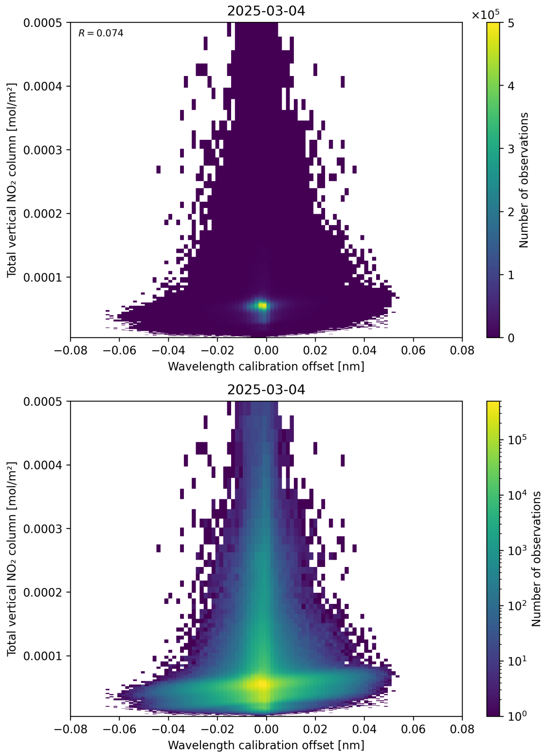
Figure 179: Scatter density plot of “Wavelength calibration offset” against “Total vertical NO 2 column” for 2025-03-03 to 2025-03-05.
