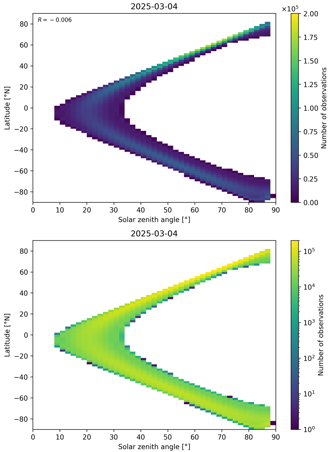
Figure 149: Scatter density plot of “Solar zenith angle” against “Latitude” for 2025-03-03 to 2025-03-05.
