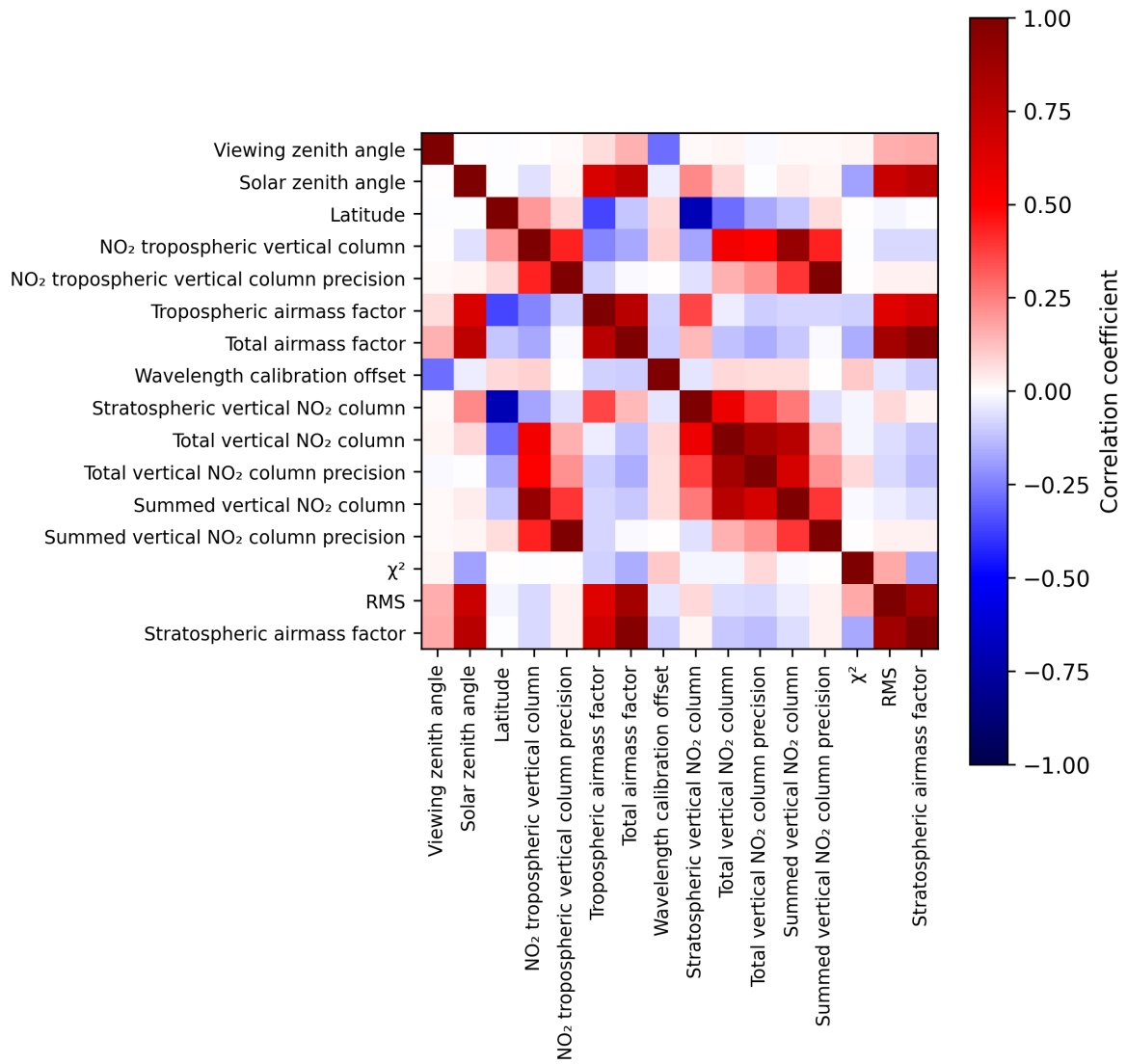
Figure 2: Map of correlation matrix for 2025-03-03 to 2025-03-05.
