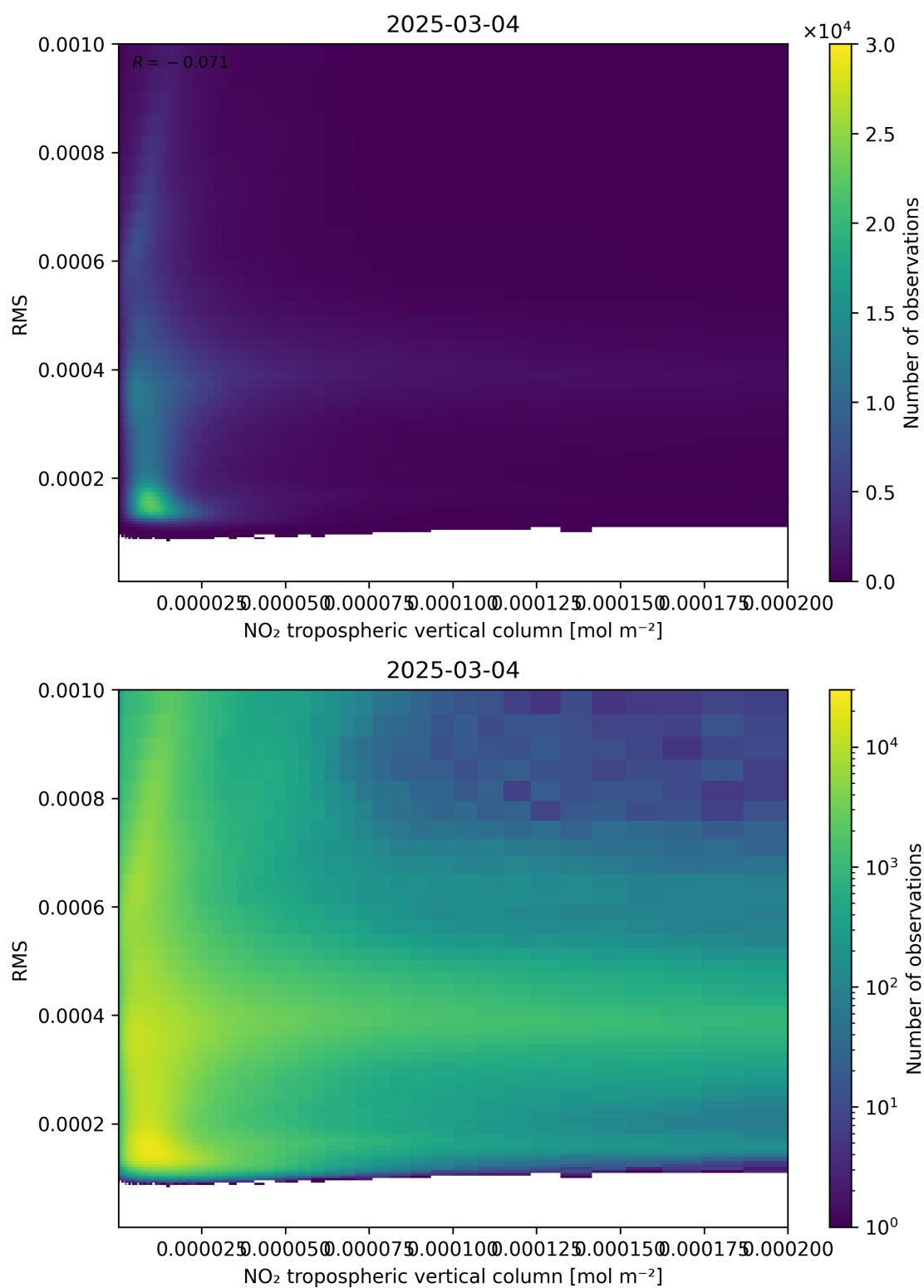
Figure 142: Scatter density plot of “NO 2 tropospheric vertical column” against “RMS” for 2025-03-03 to 2025-03-05.
