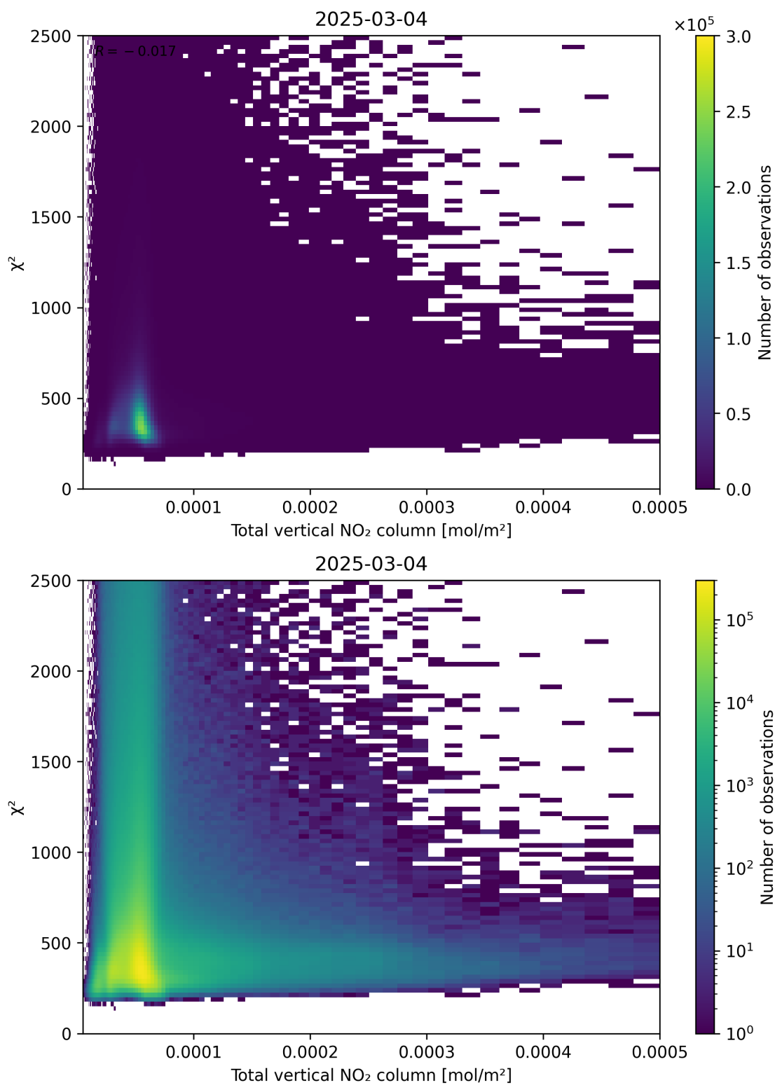
Figure 111: Scatter density plot of “Total vertical NO 2 column” against “ \chi^2 ” for 2025-03-03 to 2025-03-05.
