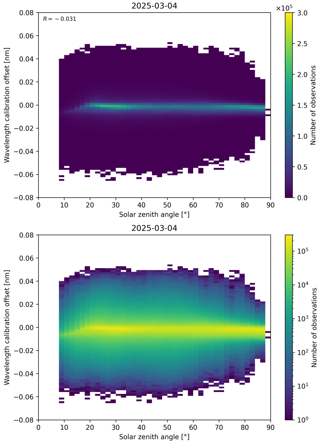
Figure 158: Scatter density plot of “Solar zenith angle” against “Wavelength calibration offset” for 2025-03-03 to 2025-03-05.
