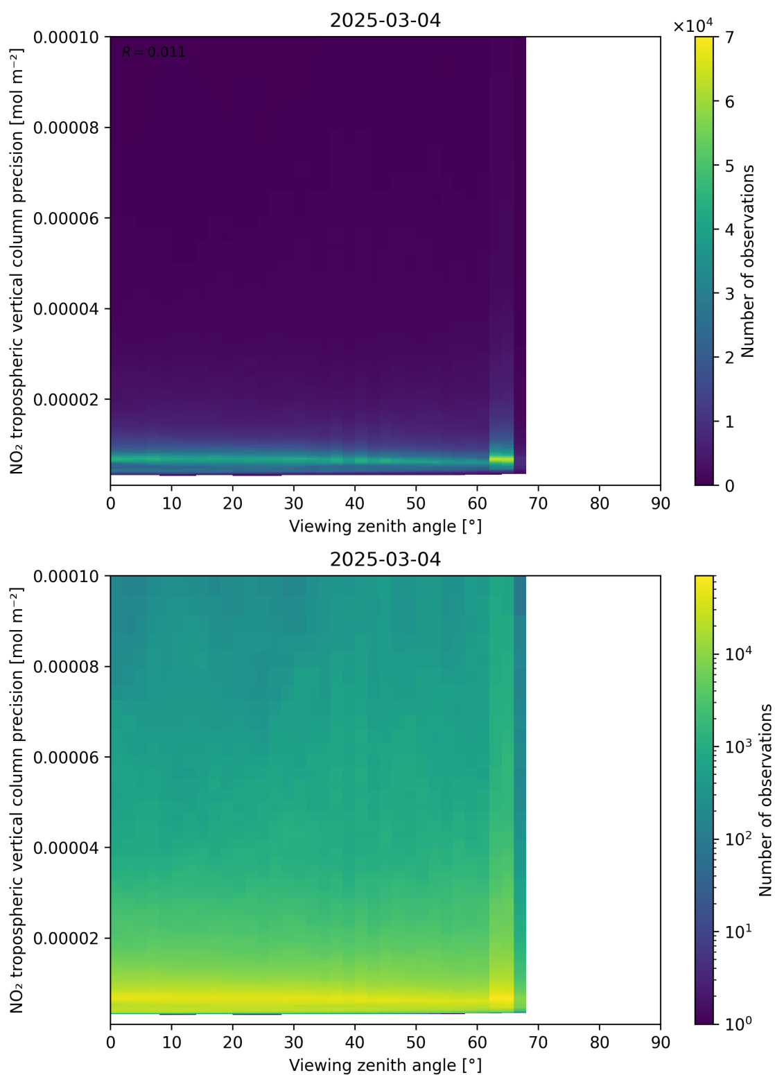
Figure 170: Scatter density plot of “Viewing zenith angle” against “NO 2 tropospheric vertical column precision” for 2025-03-03 to 2025-03-05.
