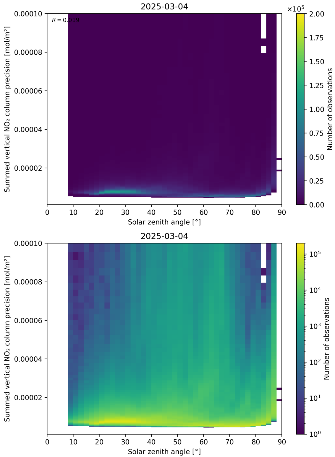
Figure 152: Scatter density plot of “Solar zenith angle” against “Summed vertical NO 2 column precision” for 2025-03-03 to 2025-03-05.
