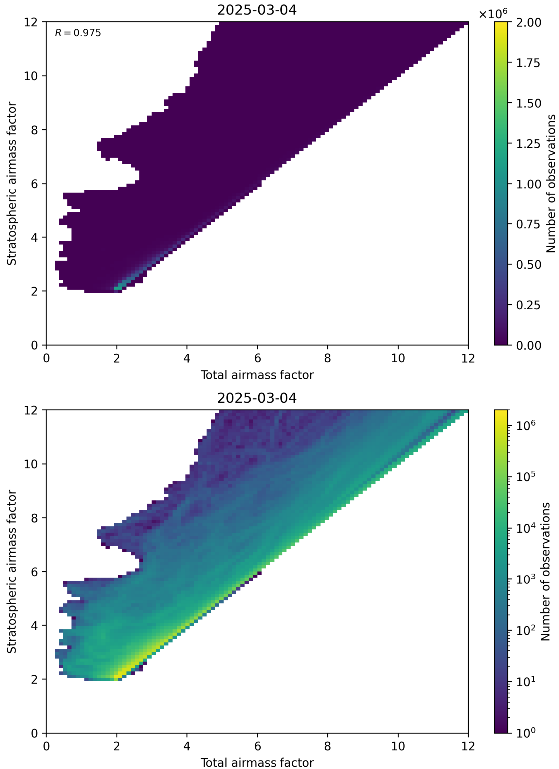
Figure 62: Scatter density plot of “Total airmass factor” against “Stratospheric airmass factor” for 2025-03-03 to 2025-03-05.
