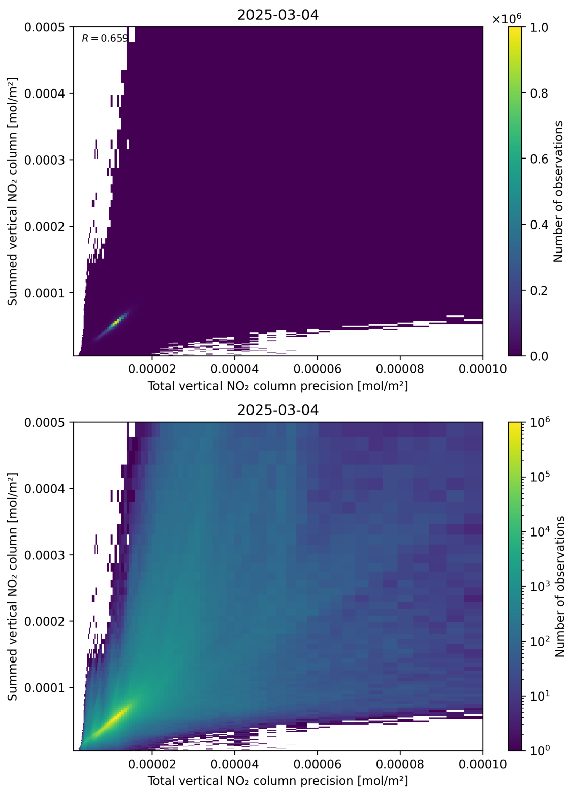
Figure 117: Scatter density plot of “Total vertical NO 2 column precision” against “Summed vertical NO 2 column” for 2025-03-03 to 2025-03-05.
