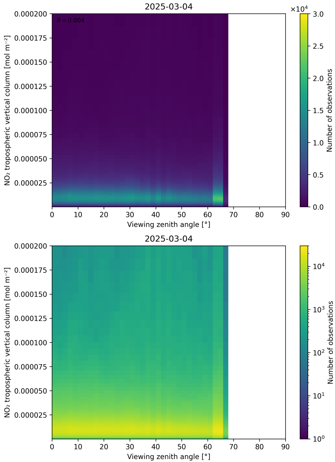
Figure 169: Scatter density plot of “Viewing zenith angle” against “NO 2 tropospheric vertical column” for 2025-03-03 to 2025-03-05.
