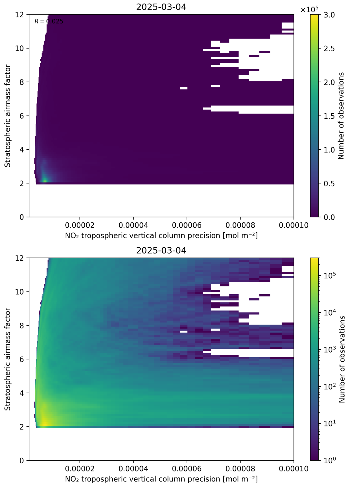
Figure 131: Scatter density plot of “NO 2 tropospheric vertical column precision” against “Stratospheric airmass factor” for 2025-03-03 to 2025-03-05.
