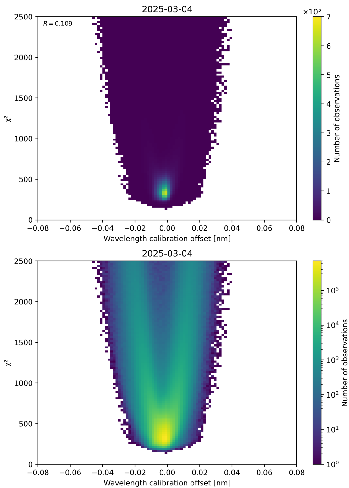
Figure 175: Scatter density plot of “Wavelength calibration offset” against “ \chi^2 ” for 2025-03-03 to 2025-03-05.
