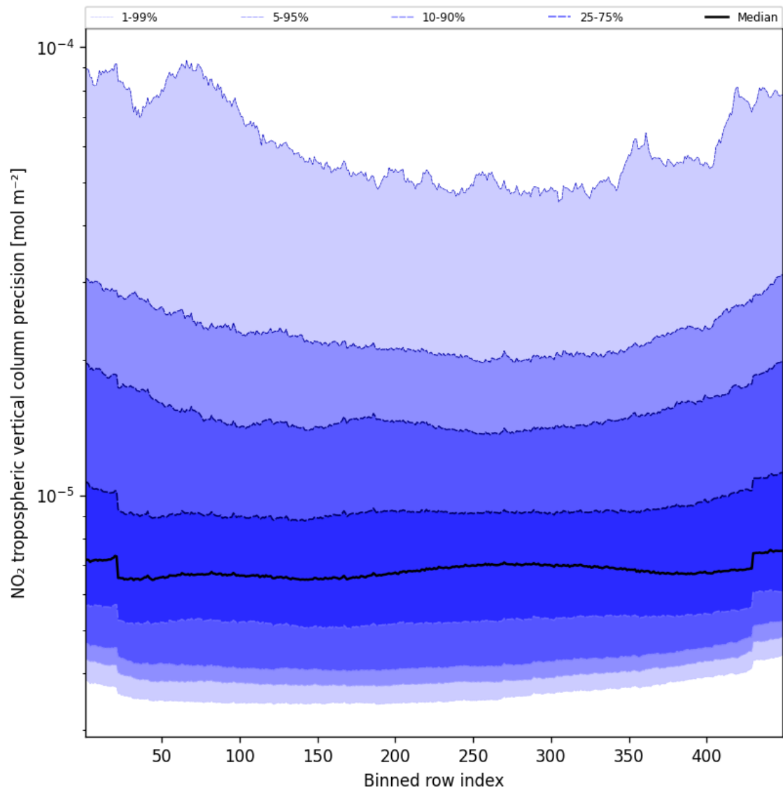
Figure 47: Along track statistics of “NO 2 tropospheric vertical column precision” for 2025-03-03 to 2025-03-05
