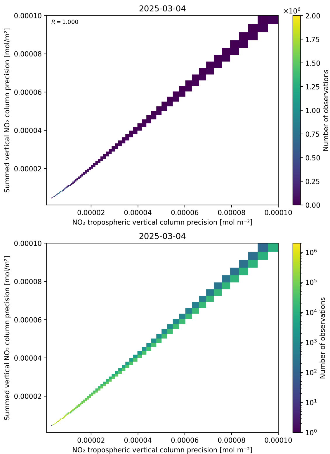
Figure 137: Scatter density plot of “NO 2 tropospheric vertical column precision” against “Summed vertical NO 2 column precision” for 2025-03-03 to 2025-03-05.
