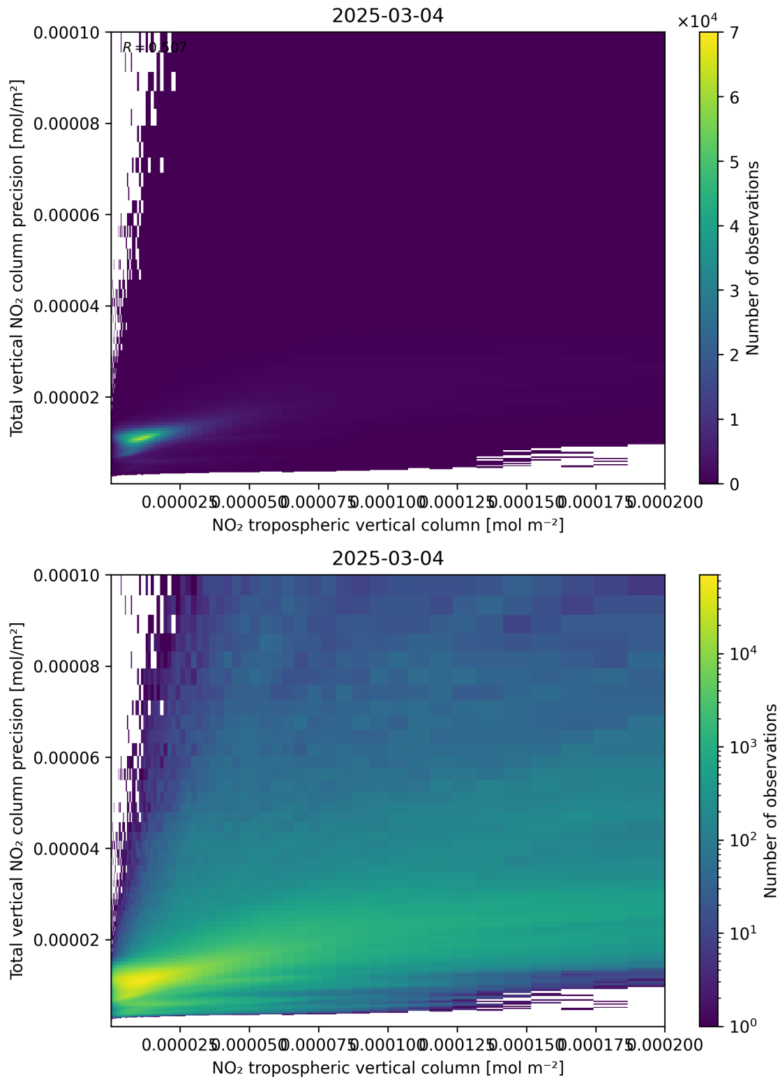
Figure 129: Scatter density plot of “NO 2 tropospheric vertical column” against “Total vertical NO 2 column precision” for 2025-03-03 to 2025-03-05.
