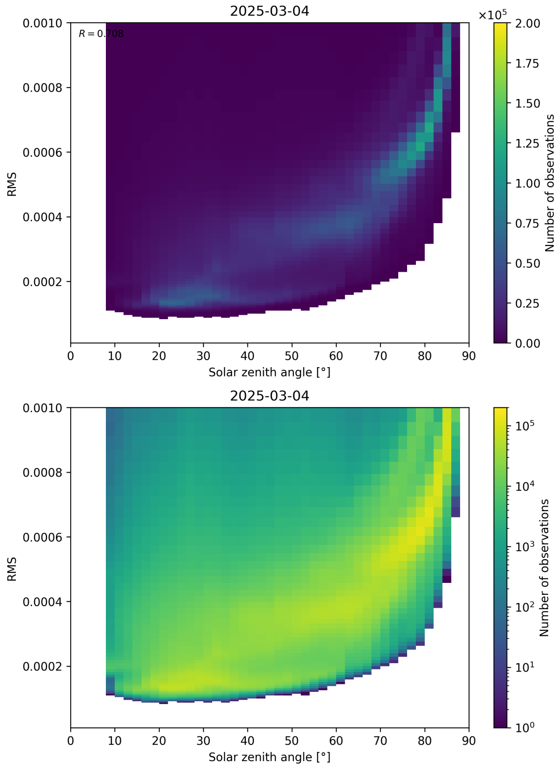
Figure 157: Scatter density plot of “Solar zenith angle” against “RMS” for 2025-03-03 to 2025-03-05.
