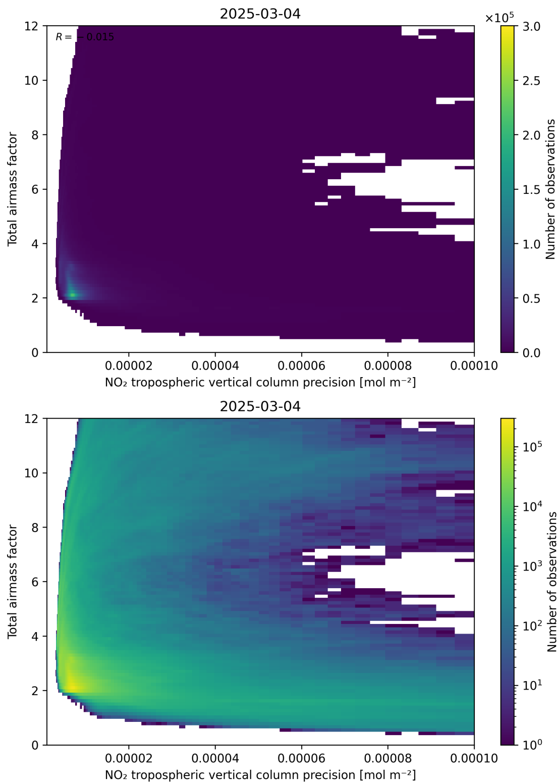
Figure 132: Scatter density plot of “NO 2 tropospheric vertical column precision” against “Total air mass factor” for 2025-03-03 to 2025-03-05.
