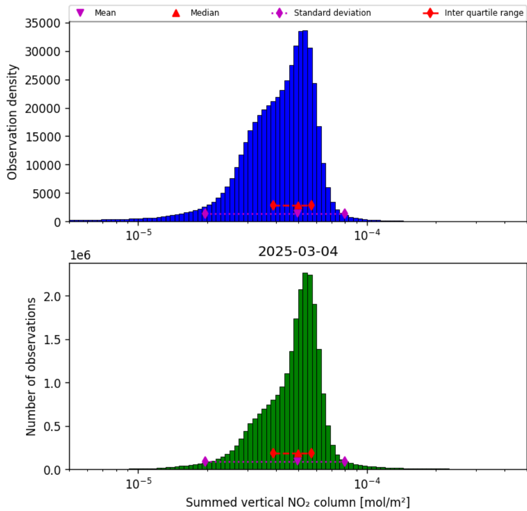
Figure 40: Histogram of “Summed vertical NO 2 column” for 2025-03-03 to 2025-03-05
