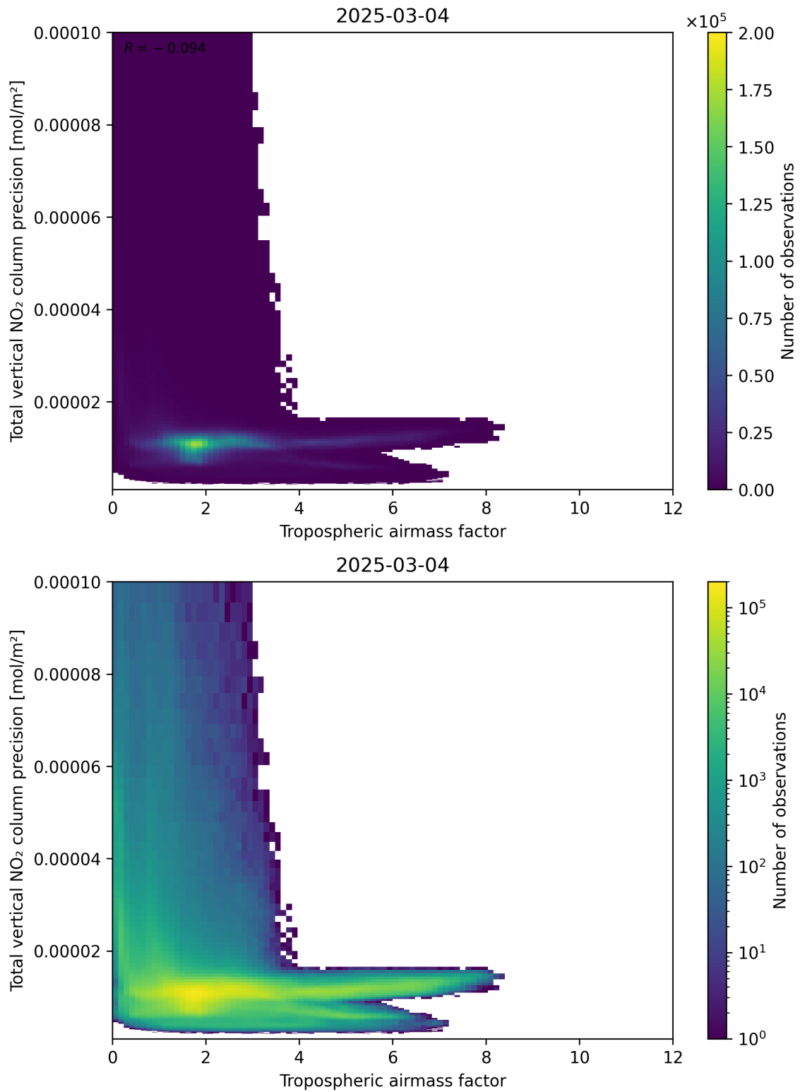
Figure 78: Scatter density plot of “Tropospheric air mass factor” against “Total vertical NO 2 column precision” for 2025-03-03 to 2025-03-05.
