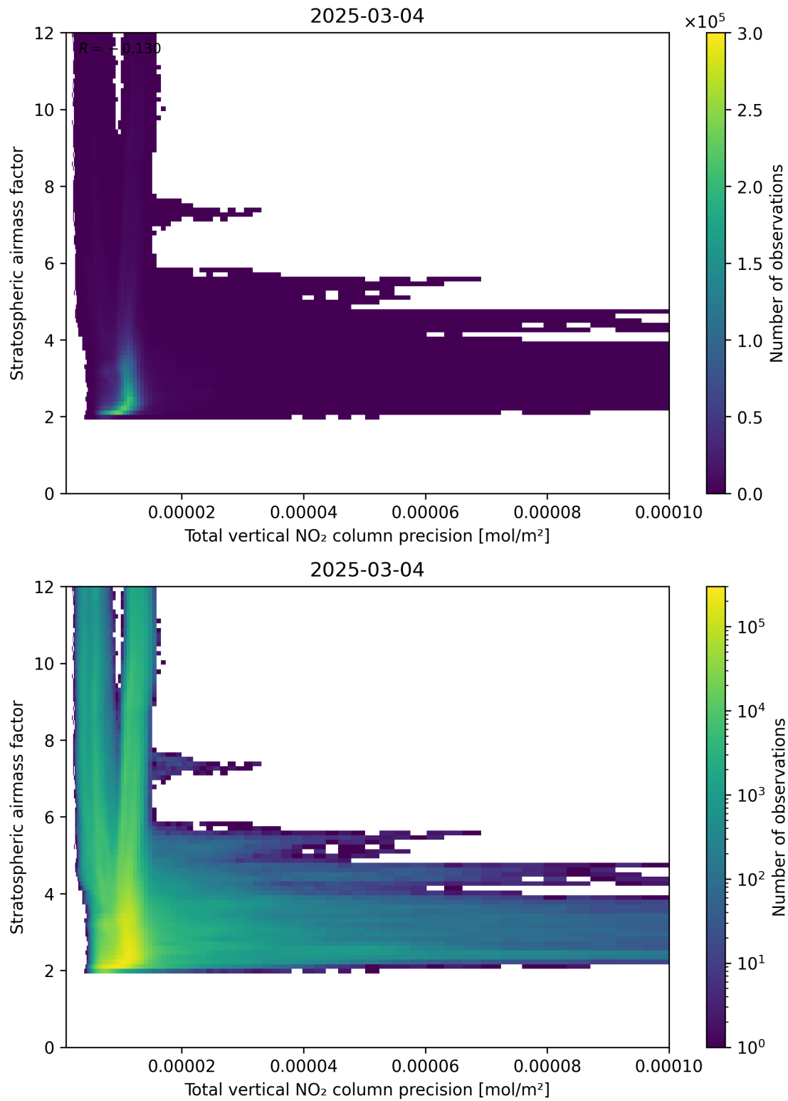
Figure 115: Scatter density plot of “Total vertical NO 2 column precision” against “Stratospheric air mass factor” for 2025-03-03 to 2025-03-05.
