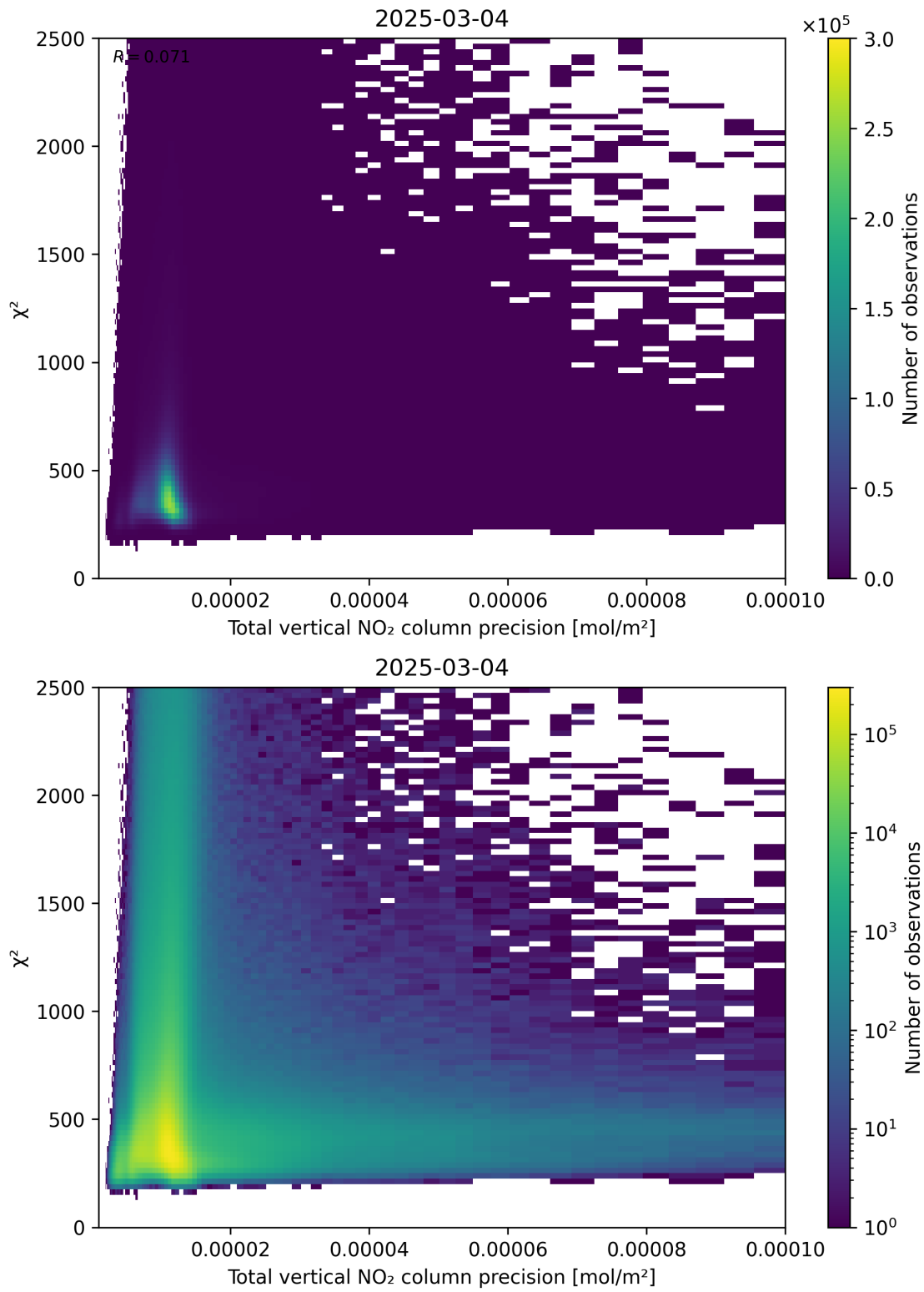
Figure 116: Scatter density plot of “Total vertical NO 2 column precision” against “ \chi^2 ” for 2025-03-03 to 2025-03-05.
