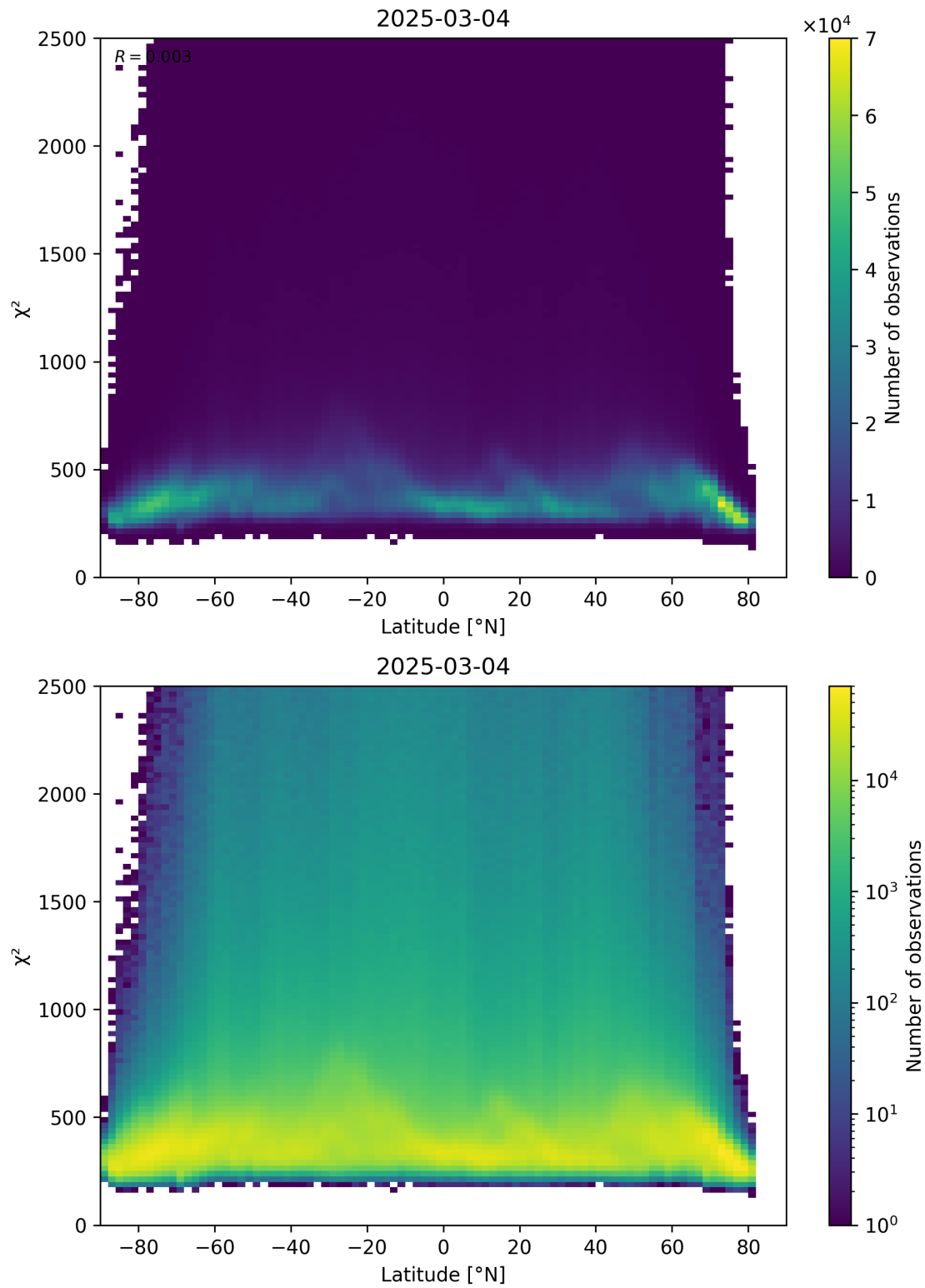
Figure 86: Scatter density plot of “Latitude” against “ \chi^2 ” for 2025-03-03 to 2025-03-05.
