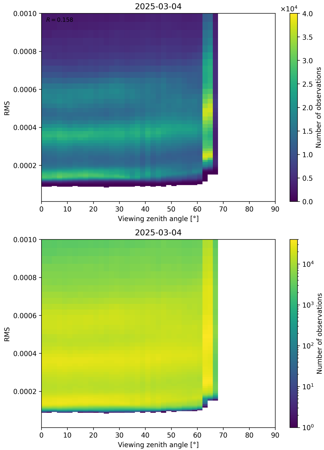
Figure 171: Scatter density plot of “Viewing zenith angle” against “RMS” for 2025-03-03 to 2025-03-05.
