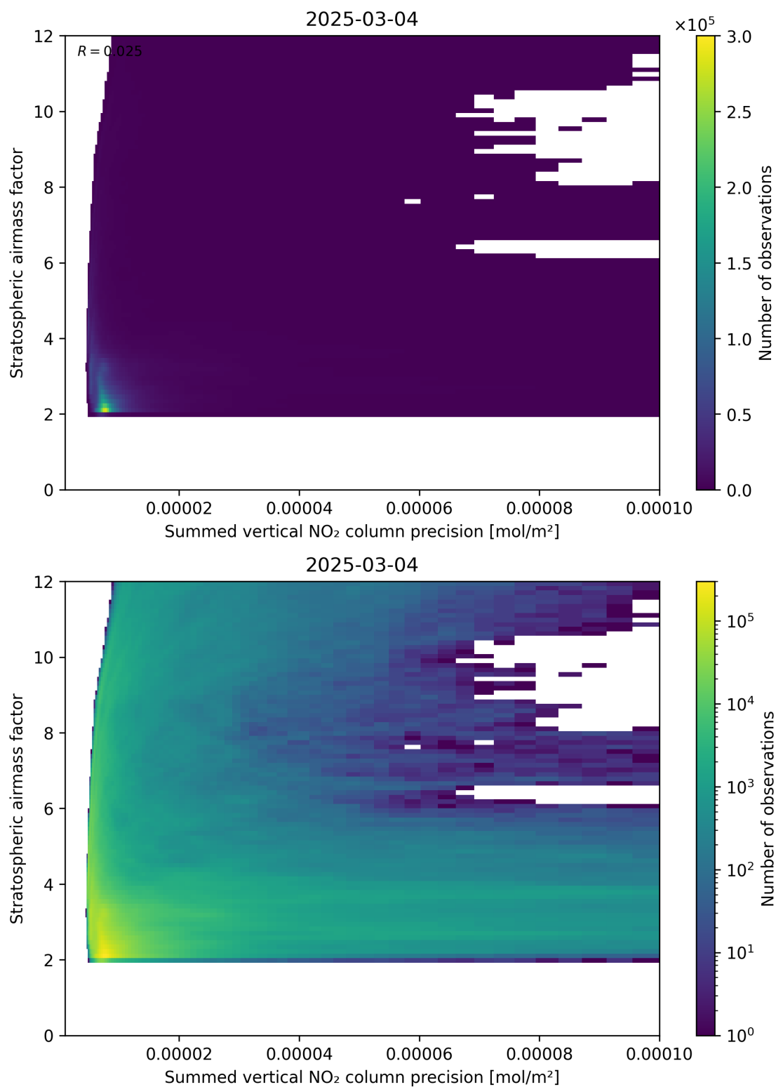
Figure 106: Scatter density plot of “Summed vertical NO 2 column precision” against “Stratospheric airmass factor” for 2025-03-03 to 2025-03-05.
