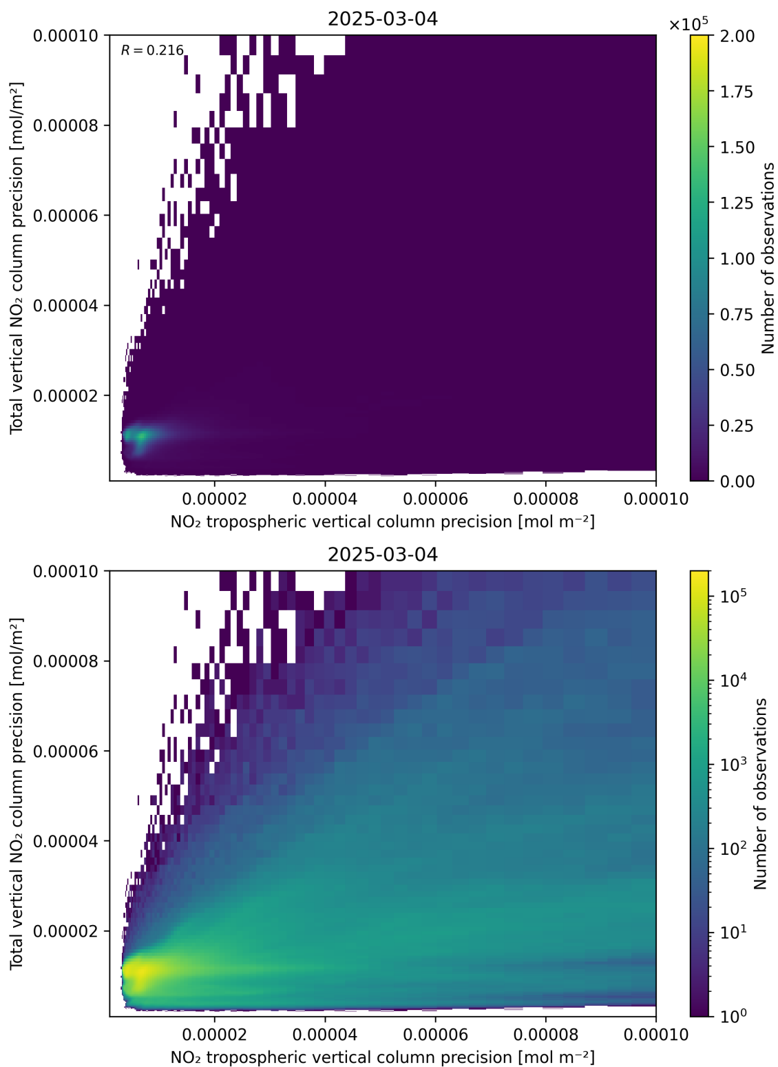
Figure 139: Scatter density plot of “NO 2 tropospheric vertical column precision” against “Total vertical NO 2 column precision” for 2025-03-03 to 2025-03-05.
