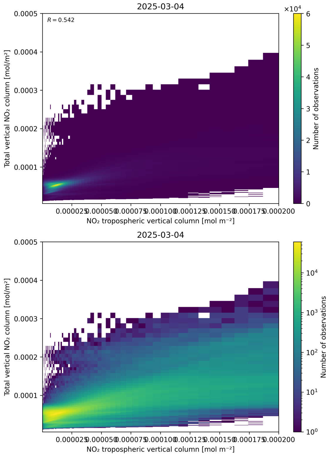
Figure 128: Scatter density plot of “NO 2 tropospheric vertical column” against “Total vertical NO 2 column” for 2025-03-03 to 2025-03-05.
