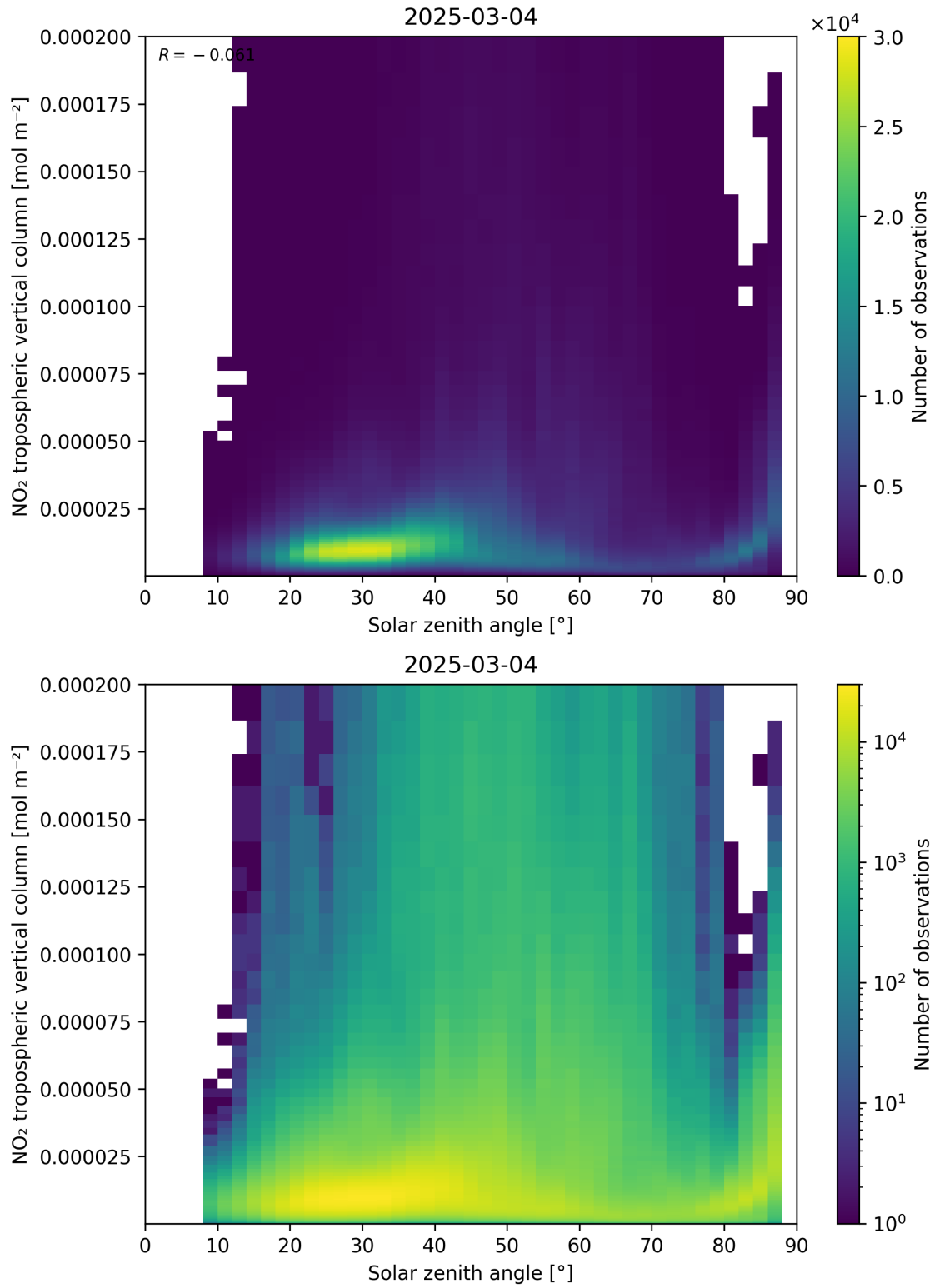
Figure 155: Scatter density plot of “Solar zenith angle” against “NO 2 tropospheric vertical column” for 2025-03-03 to 2025-03-05.
