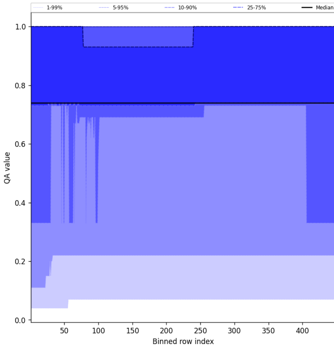
Figure 45: Along track statistics of “QA value” for 2025-03-03 to 2025-03-05
