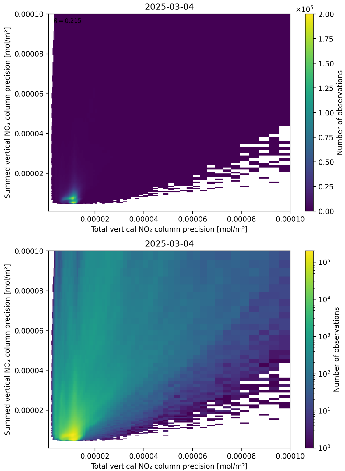
Figure 118: Scatter density plot of “Total vertical NO 2 column precision” against “Summed vertical NO 2 column precision” for 2025-03-03 to 2025-03-05.
