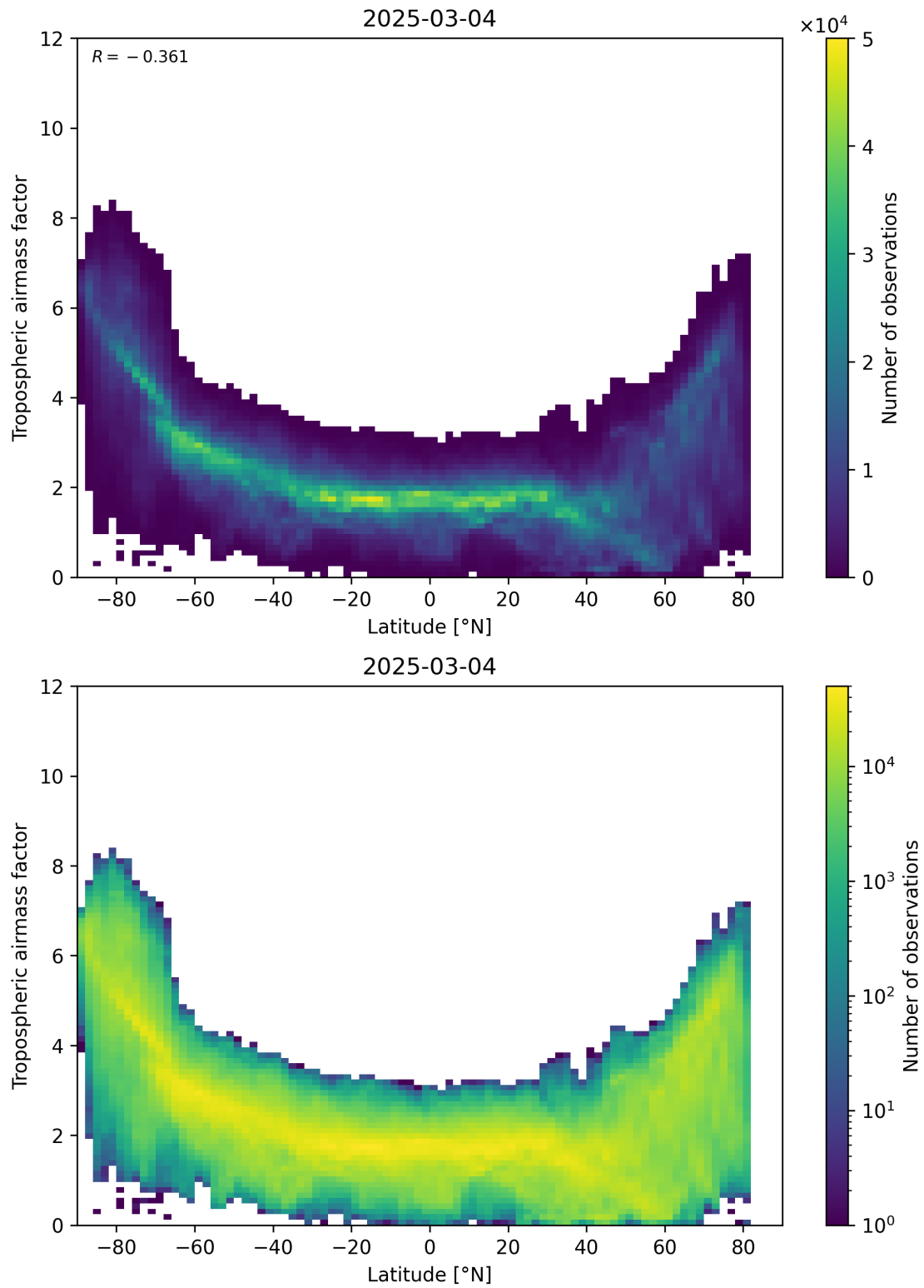
Figure 85: Scatter density plot of “Latitude” against “Tropospheric airmass factor” for 2025-03-03 to 2025-03-05.
