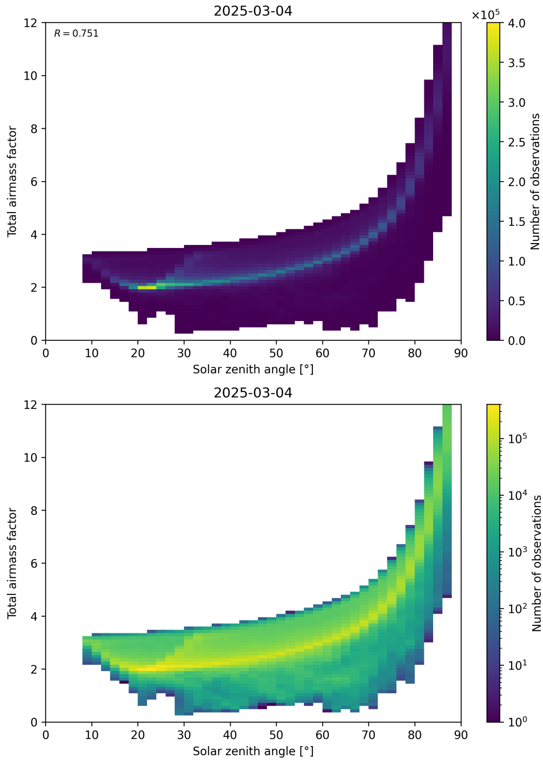
Figure 146: Scatter density plot of “Solar zenith angle” against “Total air mass factor” for 2025-03-03 to 2025-03-05.
