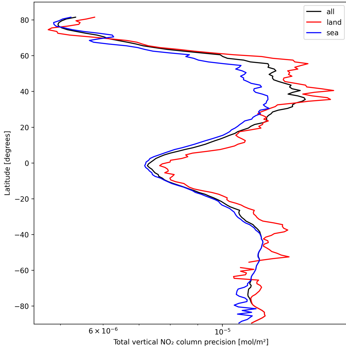
Figure 22: Zonal average of "Total vertical NO 2 column precision" for 2025-03-03 to 2025-03-05.
