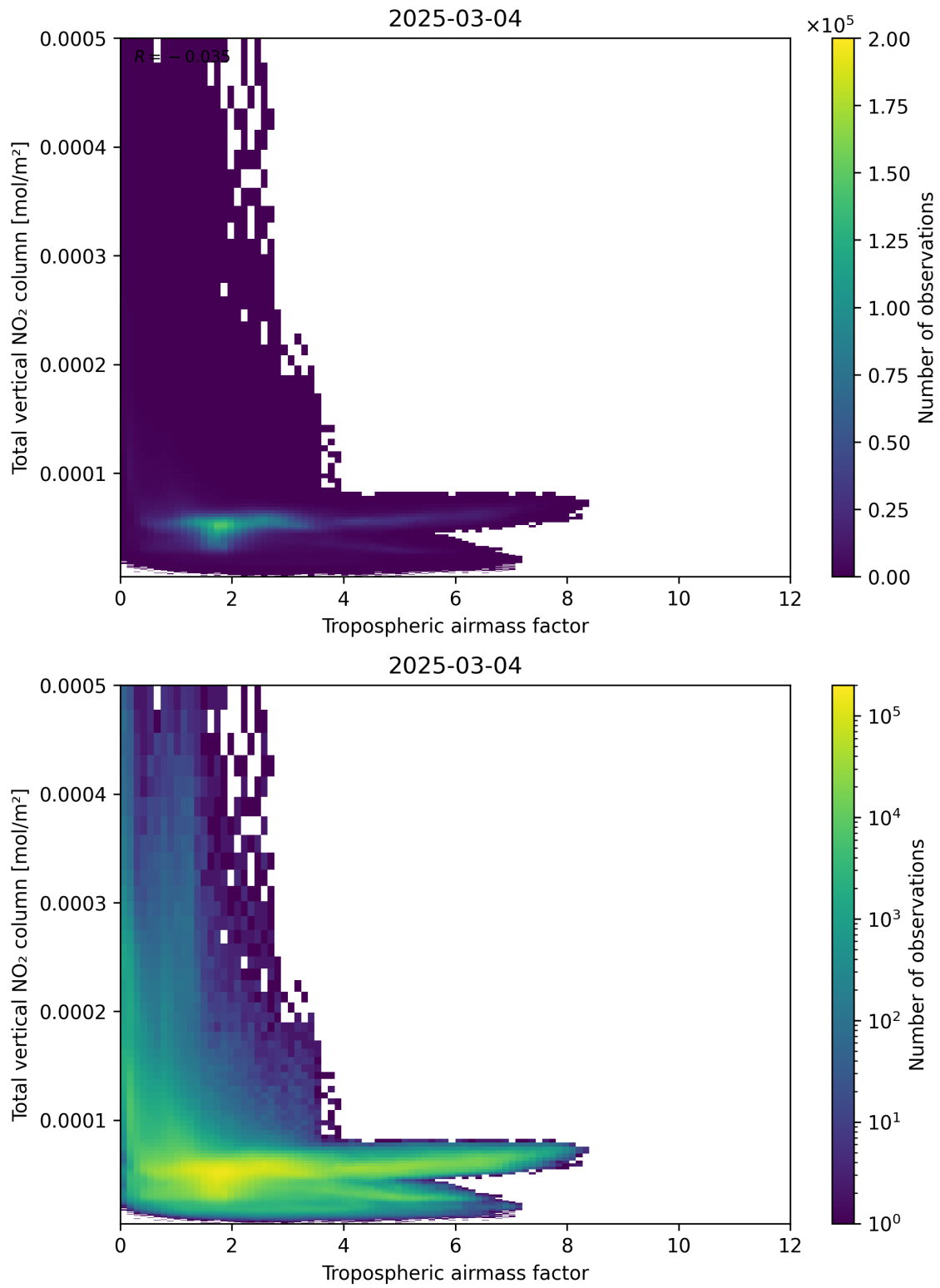
Figure 77: Scatter density plot of “Tropospheric airmass factor” against “Total vertical NO 2 column” for 2025-03-03 to 2025-03-05.
