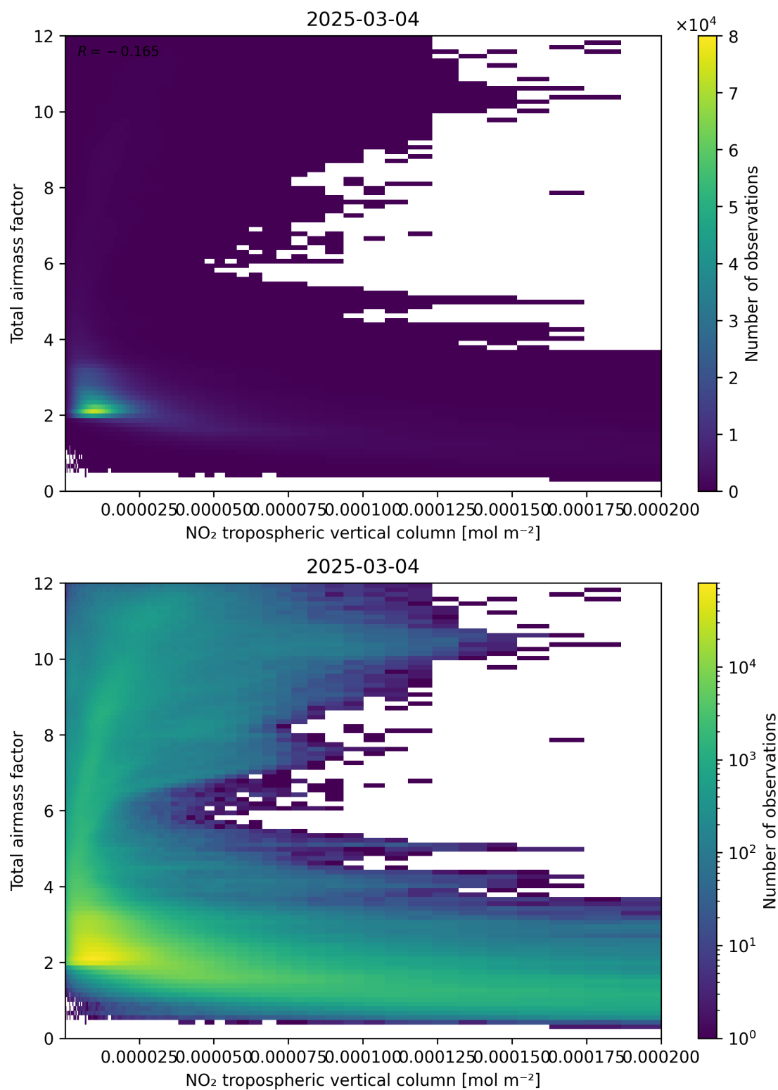
Figure 122: Scatter density plot of “NO 2 tropospheric vertical column” against “Total air mass factor” for 2025-03-03 to 2025-03-05.
