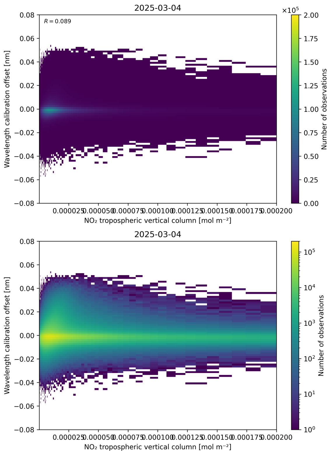
Figure 143: Scatter density plot of “NO 2 tropospheric vertical column” against “Wavelength calibration offset” for 2025-03-03 to 2025-03-05.
