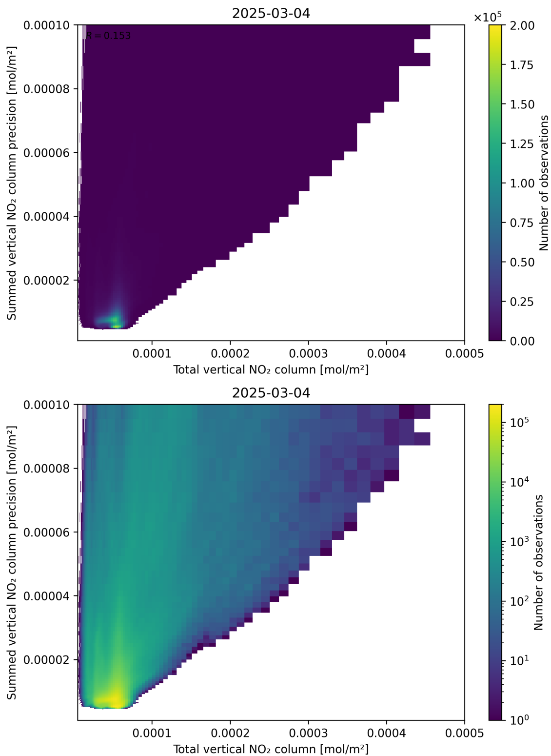
Figure 113: Scatter density plot of “Total vertical NO 2 column” against “Summed vertical NO 2 column precision” for 2025-03-03 to 2025-03-05.
