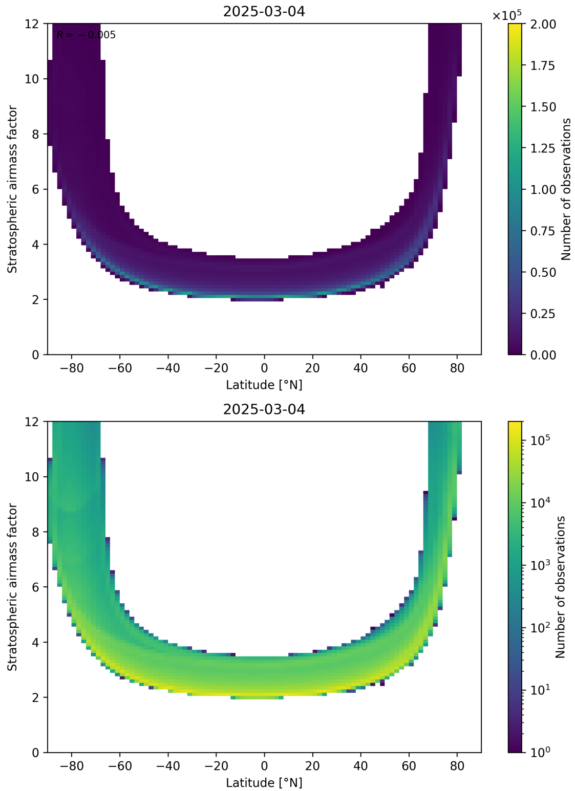
Figure 83: Scatter density plot of “Latitude” against “Stratospheric airmass factor” for 2025-03-03 to 2025-03-05.
