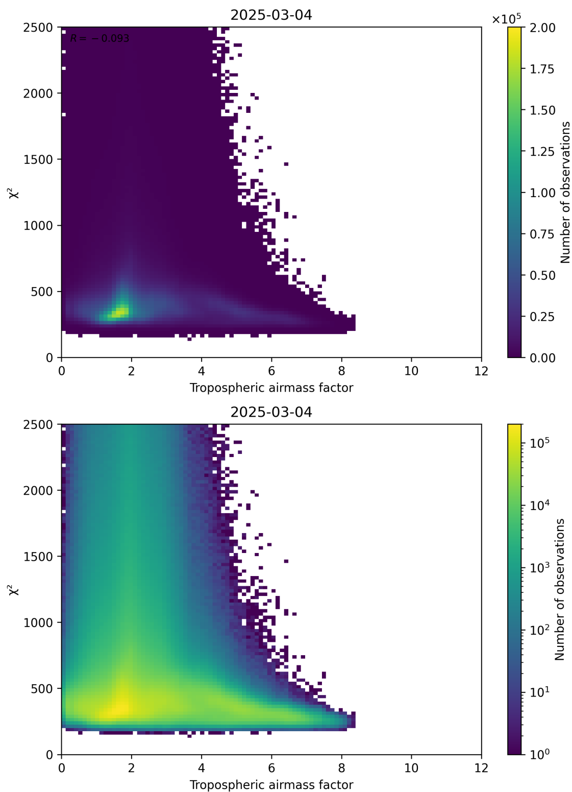
Figure 73: Scatter density plot of “Tropospheric airmass factor” against “ \chi^2 ” for 2025-03-03 to 2025-03-05.
