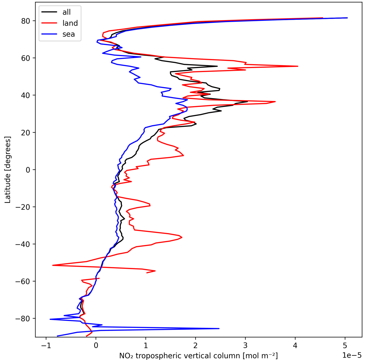
Figure 12: Zonal average of “NO 2 tropospheric vertical column” for 2025-03-03 to 2025-03-05.
