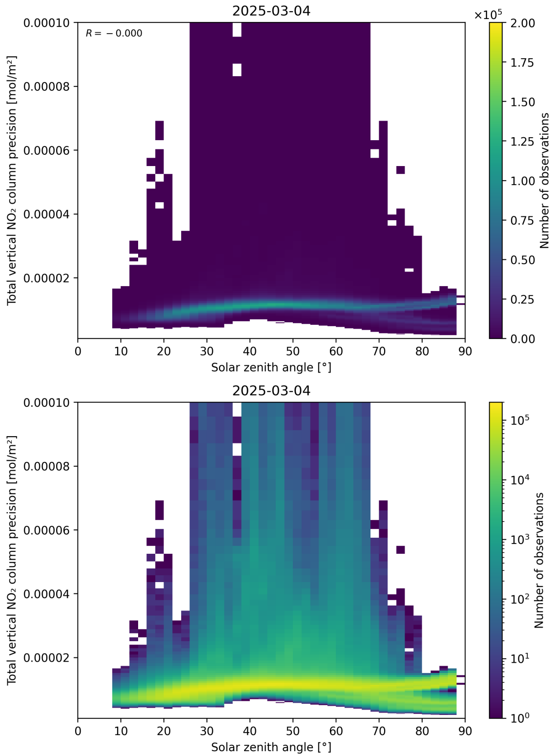
Figure 154: Scatter density plot of “Solar zenith angle” against “Total vertical NO 2 column precision” for 2025-03-03 to 2025-03-05.
