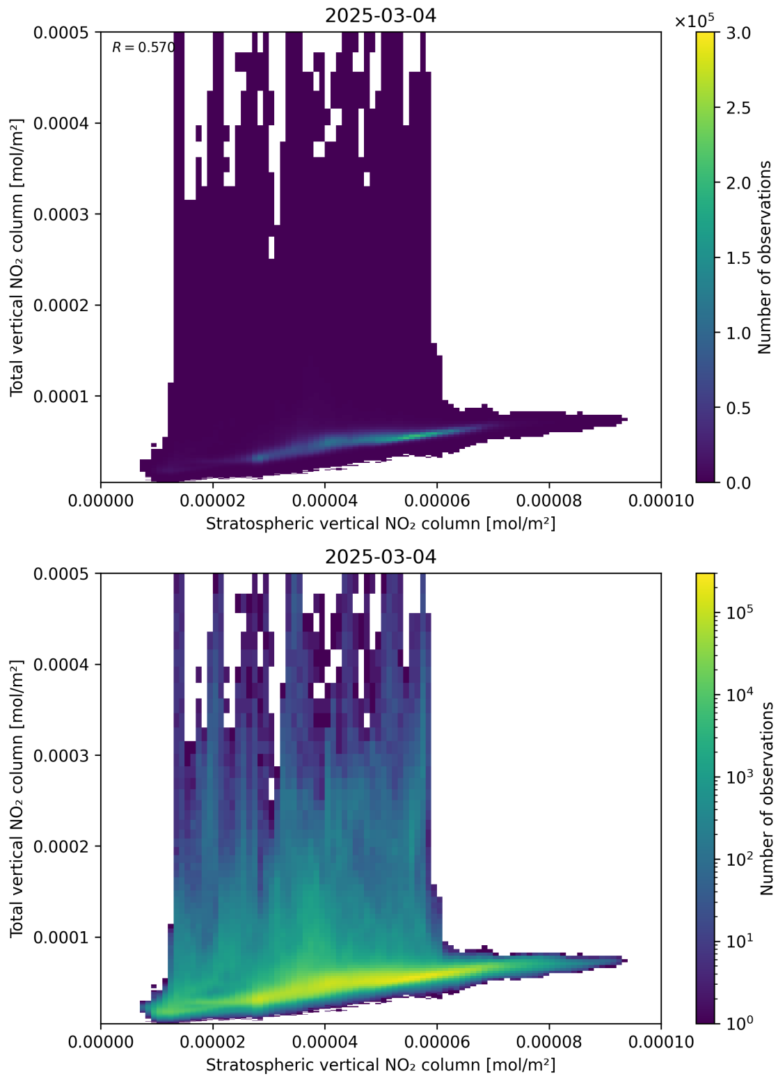
Figure 100: Scatter density plot of “Stratospheric vertical NO 2 column” against “Total vertical NO 2 column” for 2025-03-03 to 2025-03-05.
