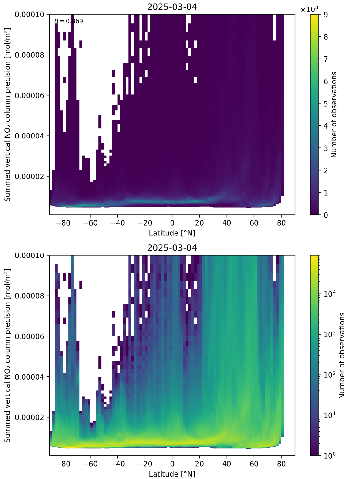
Figure 89: Scatter density plot of “Latitude” against “Summed vertical NO 2 column precision” for 2025-03-03 to 2025-03-05.
