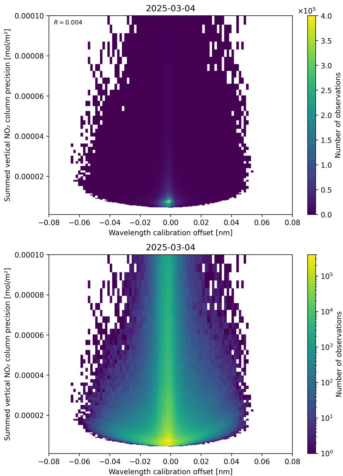
Figure 178: Scatter density plot of “Wavelength calibration offset” against “Summed vertical NO 2 column precision” for 2025-03-03 to 2025-03-05.
