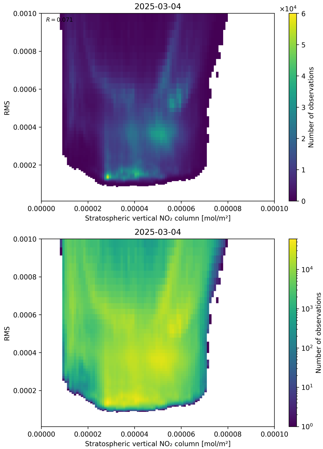
Figure 102: Scatter density plot of “Stratospheric vertical NO 2 column” against “RMS” for 2025-03-03 to 2025-03-05.
