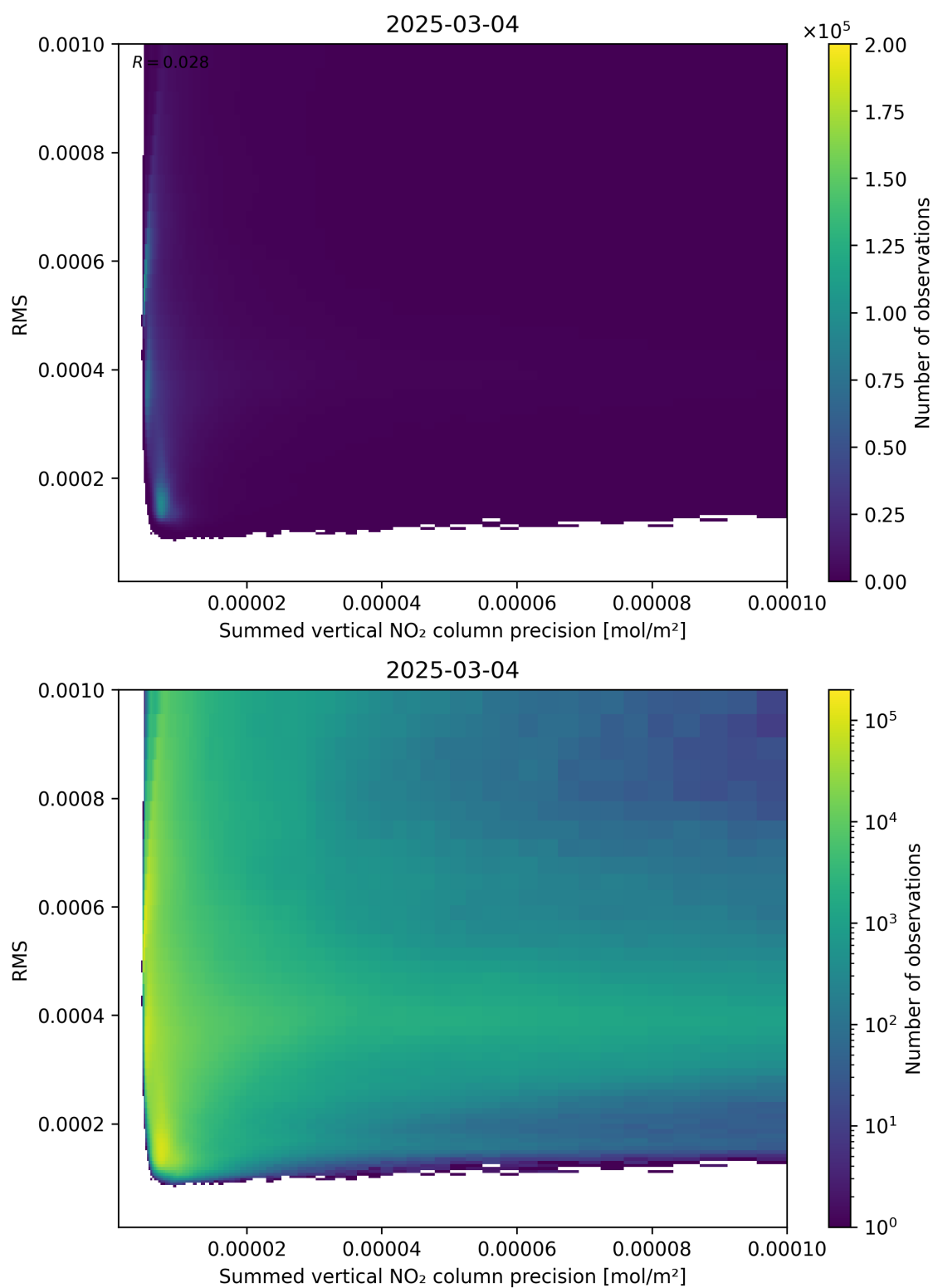
Figure 108: Scatter density plot of “Summed vertical NO 2 column precision” against “RMS” for 2025-03-03 to 2025-03-05.
