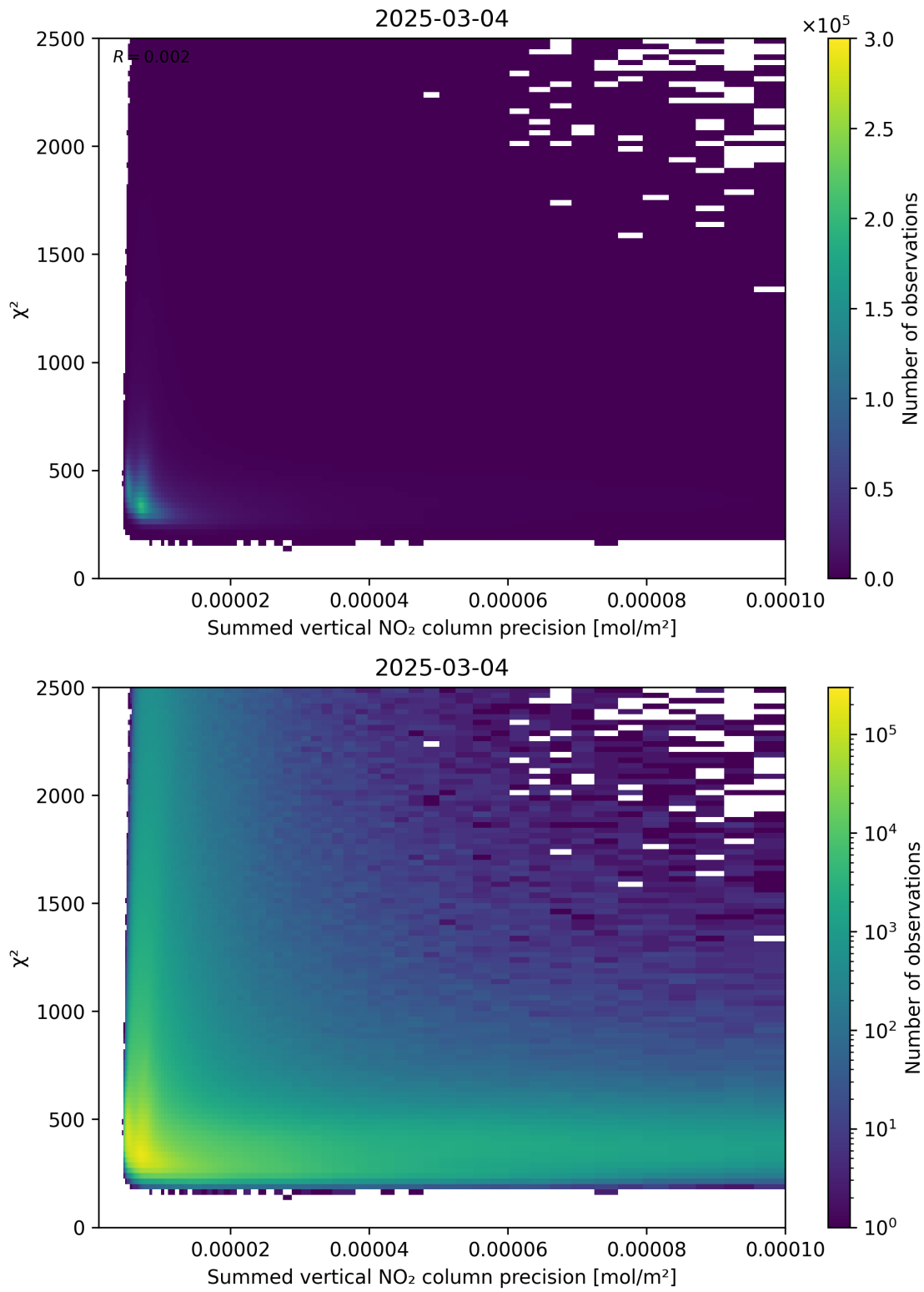
Figure 107: Scatter density plot of “Summed vertical NO 2 column precision” against “ \chi^2 ” for 2025-03-03 to 2025-03-05.
