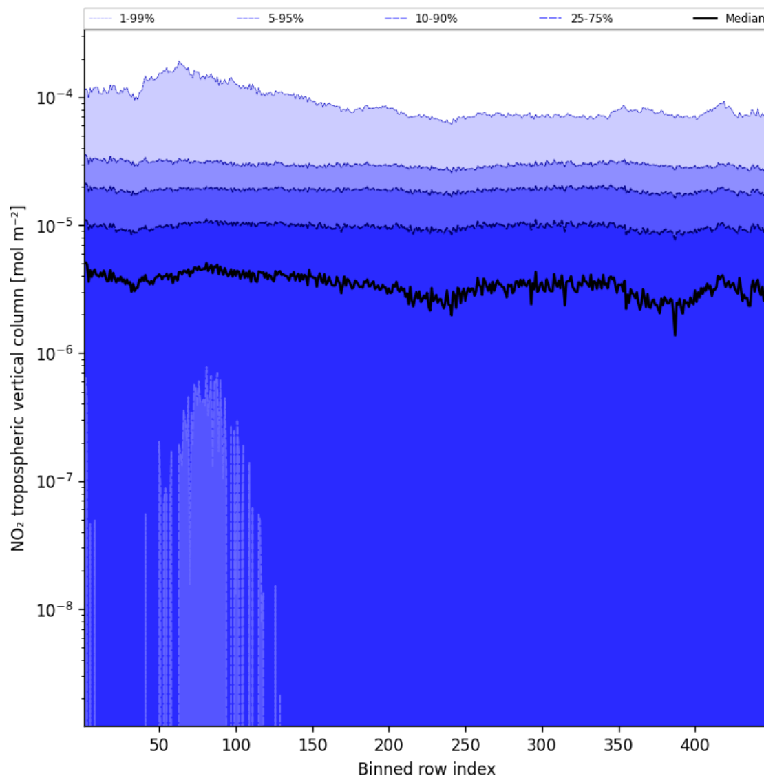
Figure 46: Along track statistics of “NO 2 tropospheric vertical column” for 2025-03-03 to 2025-03-05
