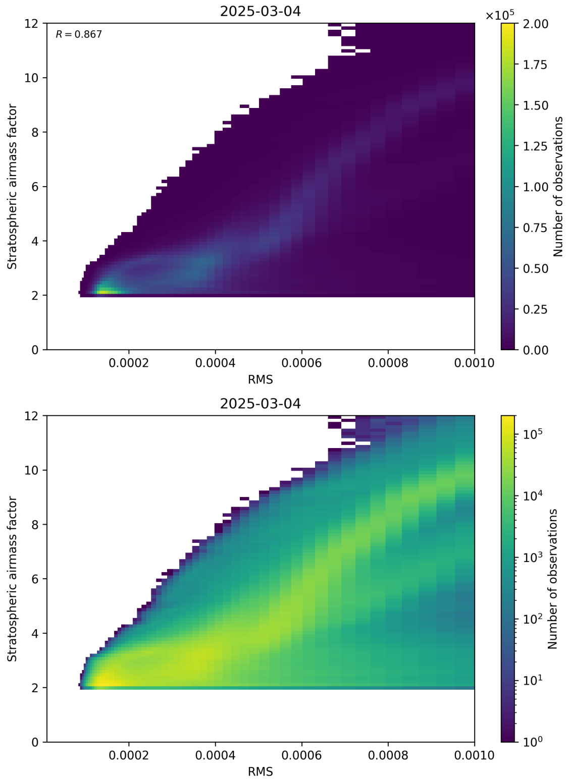
Figure 144: Scatter density plot of “RMS” against “Stratospheric airmass factor” for 2025-03-03 to 2025-03-05.
