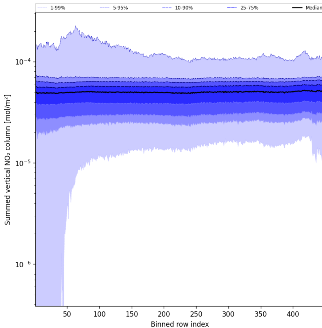
Figure 57: Along track statistics of “Summed vertical NO 2 column” for 2025-03-03 to 2025-03-05
