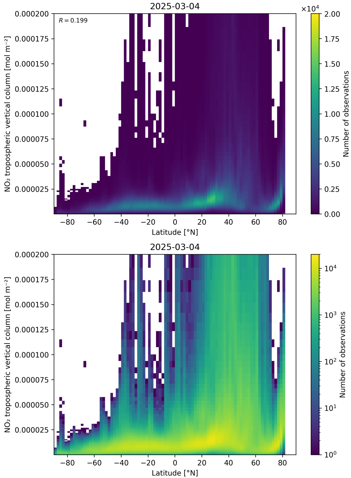
Figure 92: Scatter density plot of “Latitude” against “NO 2 tropospheric vertical column” for 2025-03-03 to 2025-03-05.
