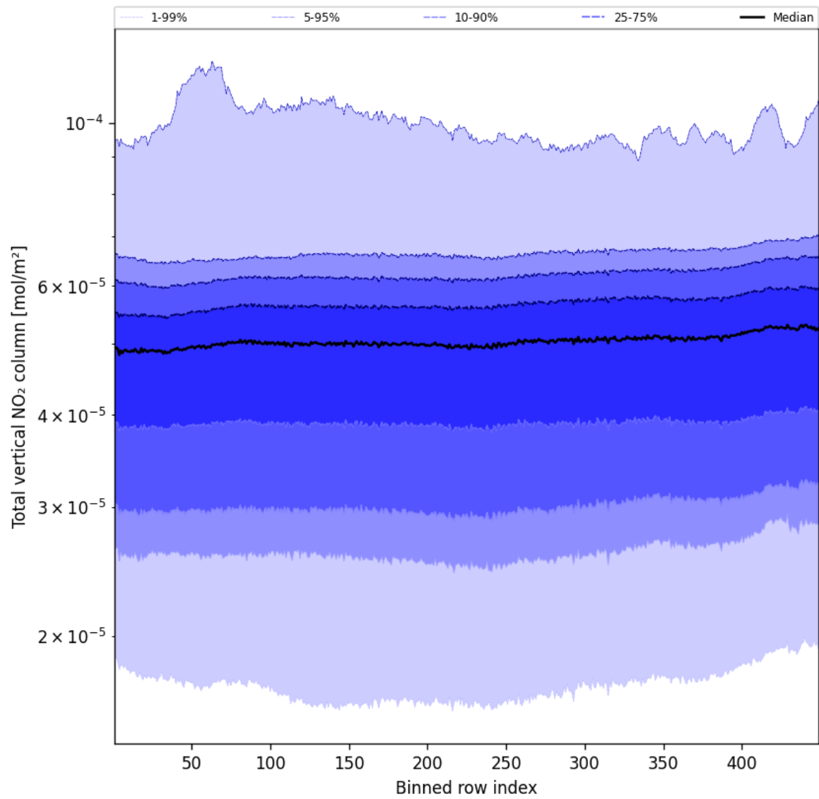
Figure 55: Along track statistics of “Total vertical NO 2 column” for 2025-03-03 to 2025-03-05
