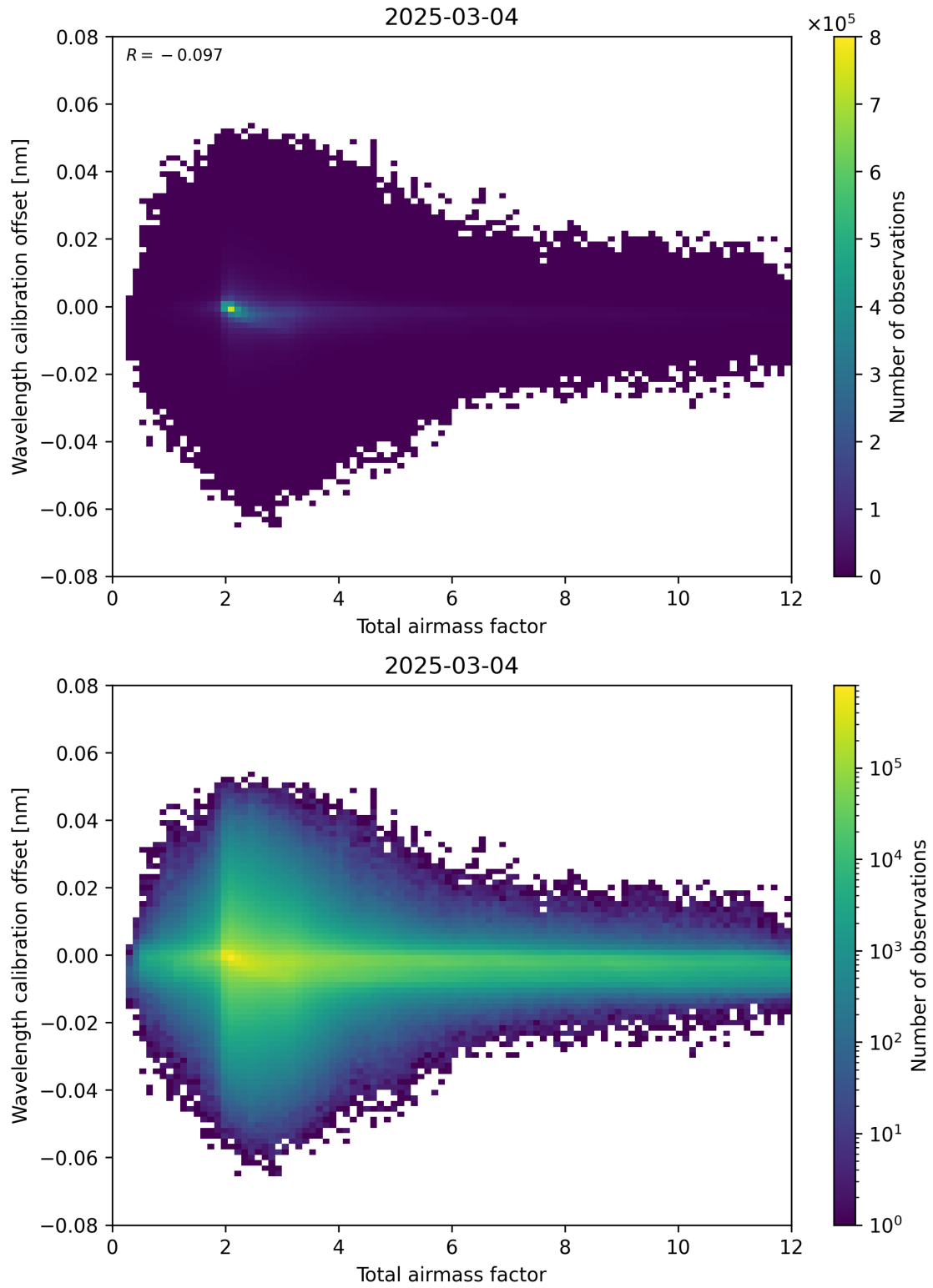
Figure 70: Scatter density plot of “Total airmass factor” against “Wavelength calibration offset” for 2025-03-03 to 2025-03-05.
