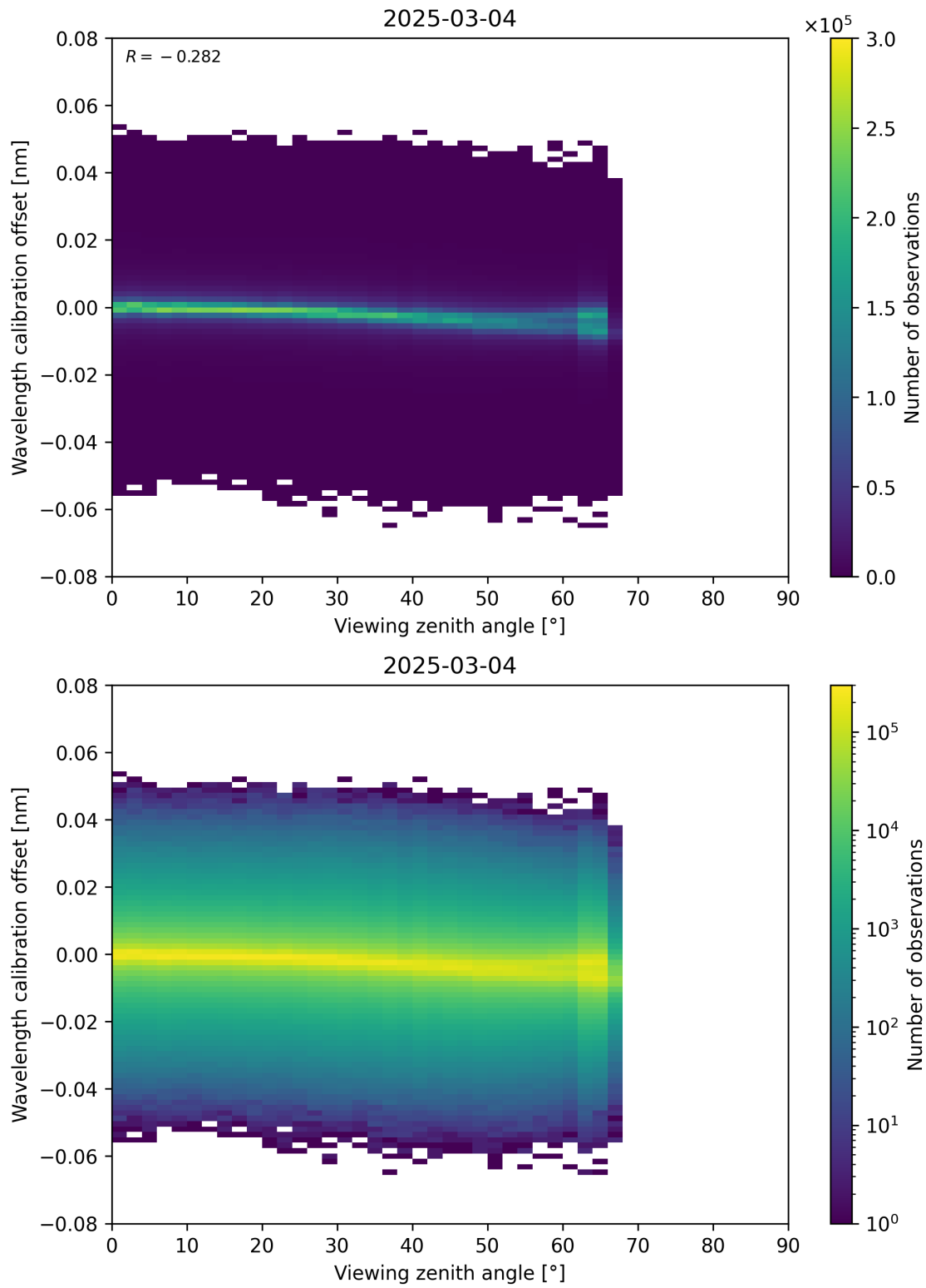
Figure 173: Scatter density plot of “Viewing zenith angle” against “Wavelength calibration offset” for 2025-03-03 to 2025-03-05.
