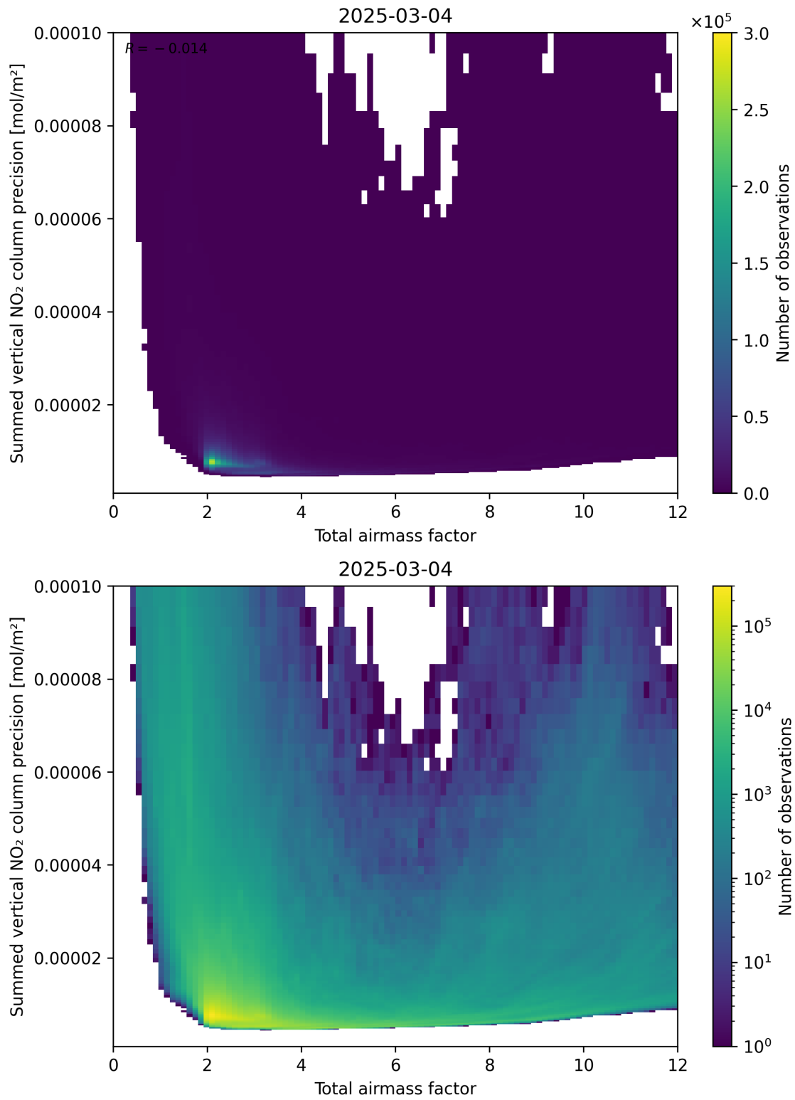
Figure 66: Scatter density plot of “Total airmass factor” against “Summed vertical NO 2 column precision” for 2025-03-03 to 2025-03-05.
