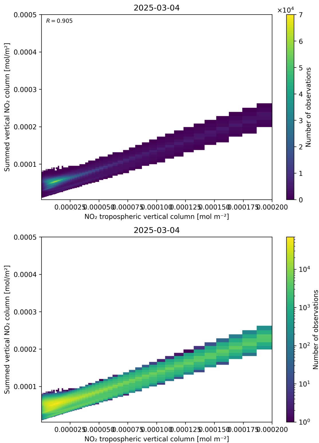
Figure 126: Scatter density plot of “NO 2 tropospheric vertical column” against “Summed vertical NO 2 column” for 2025-03-03 to 2025-03-05.
