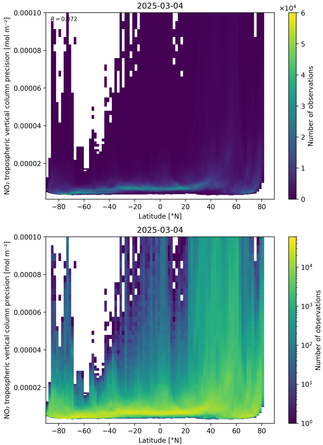
Figure 93: Scatter density plot of “Latitude” against “NO 2 tropospheric vertical column precision” for 2025-03-03 to 2025-03-05.
