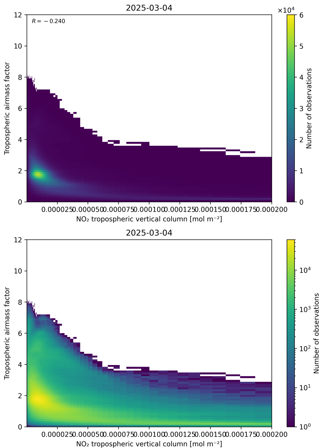
Figure 123: Scatter density plot of “NO 2 tropospheric vertical column” against “Tropospheric air mass factor” for 2025-03-03 to 2025-03-05.
