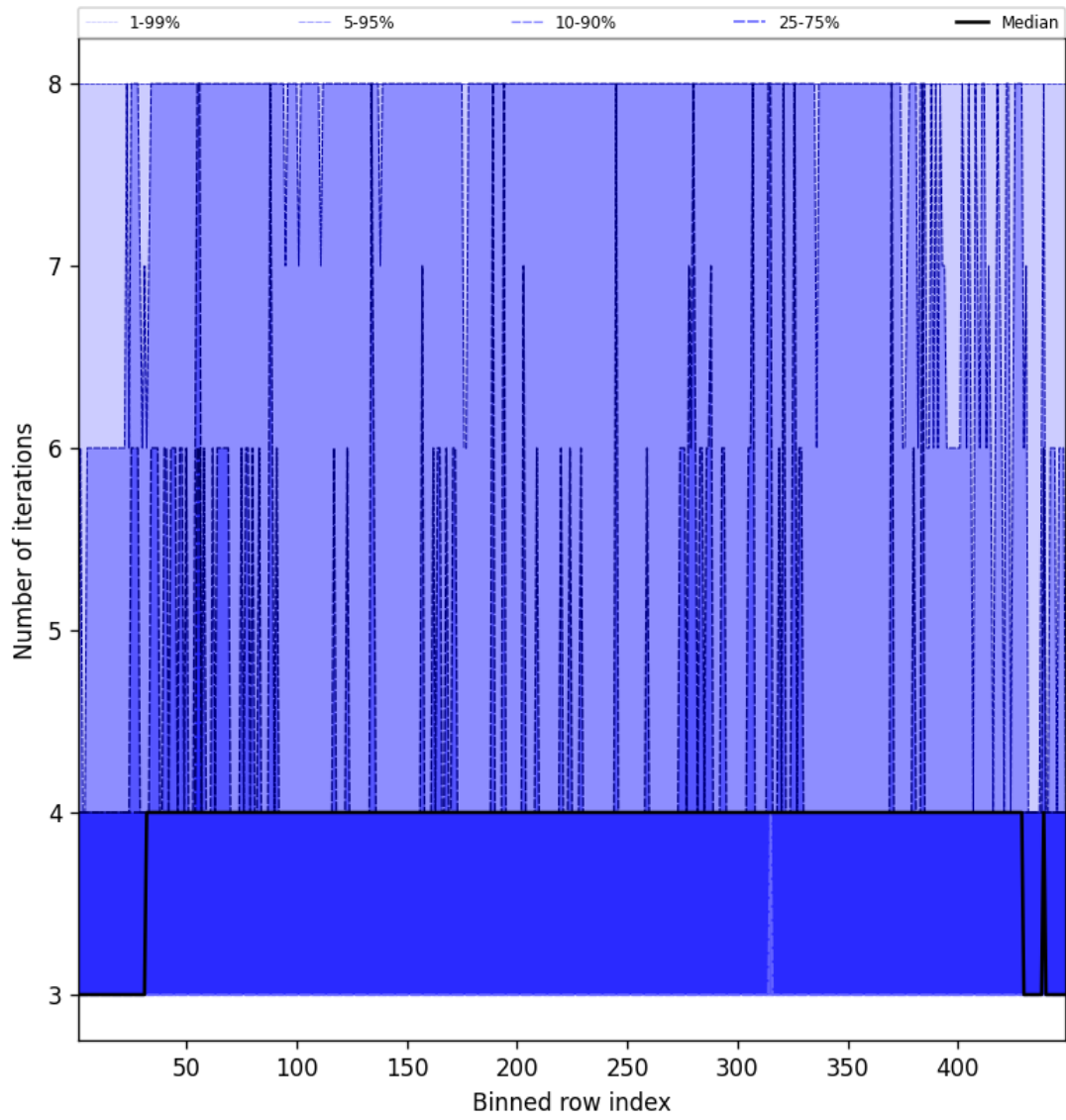
Figure 51: Along track statistics of “Number of iterations” for 2025-03-03 to 2025-03-05
