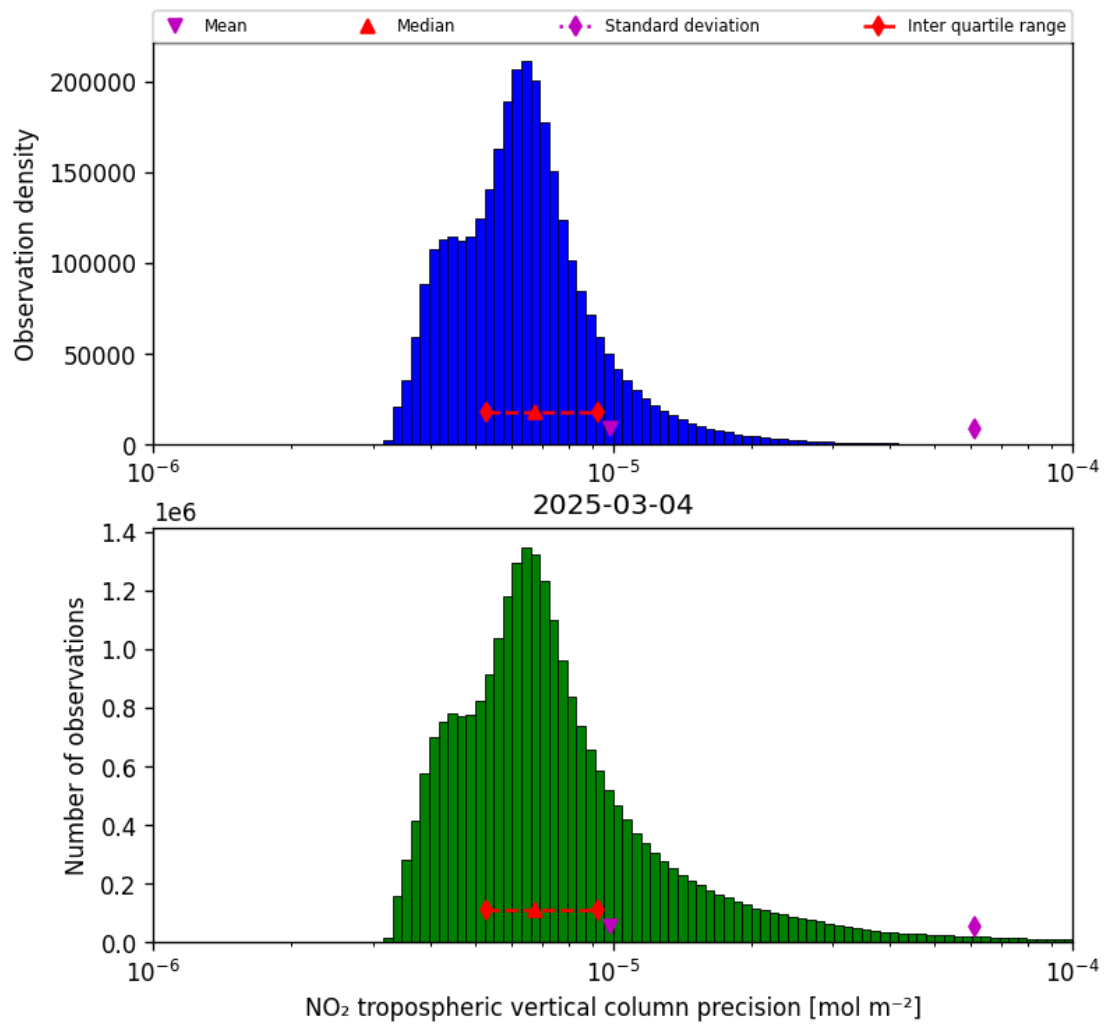
Figure 30: Histogram of “NO 2 tropospheric vertical column precision” for 2025-03-03 to 2025-03-05
