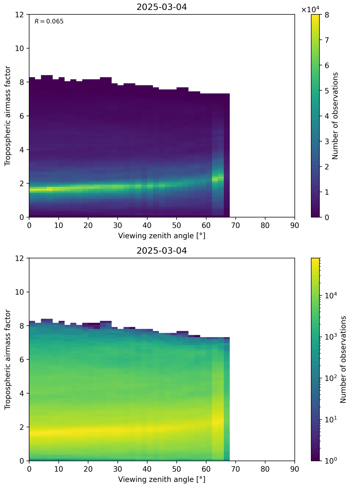
Figure 161: Scatter density plot of “Viewing zenith angle” against “Tropospheric airmass factor” for 2025-03-03 to 2025-03-05.
