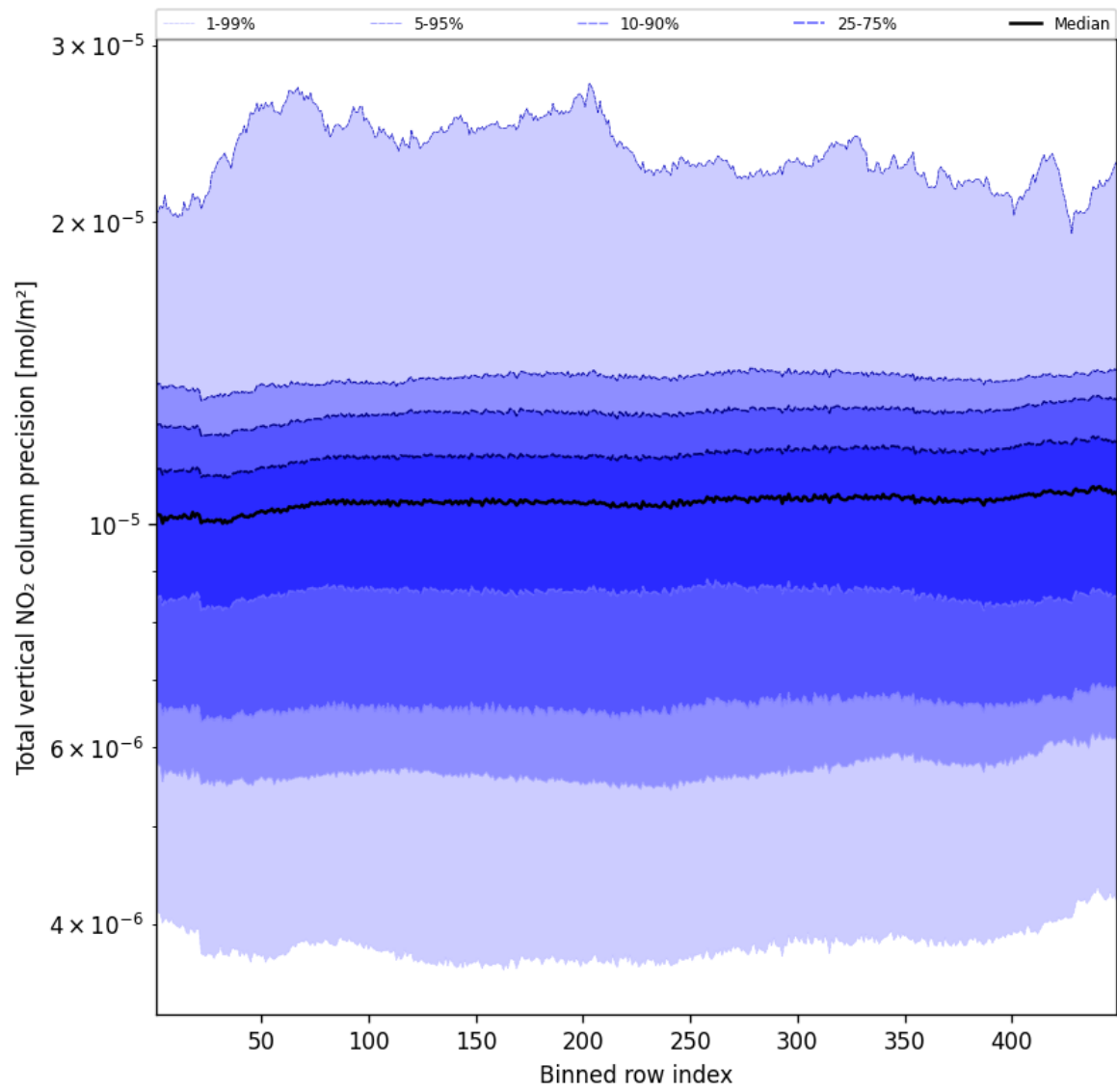
Figure 56: Along track statistics of “Total vertical NO 2 column precision” for 2025-03-03 to 2025-03-05
