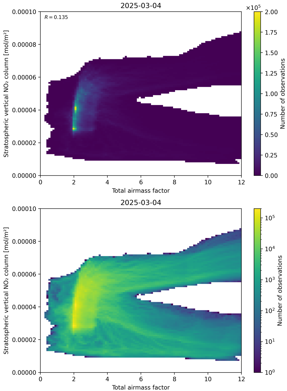
Figure 64: Scatter density plot of “Total airmass factor” against “Stratospheric vertical \text{NO}_2 column” for 2025-03-03 to 2025-03-05.
