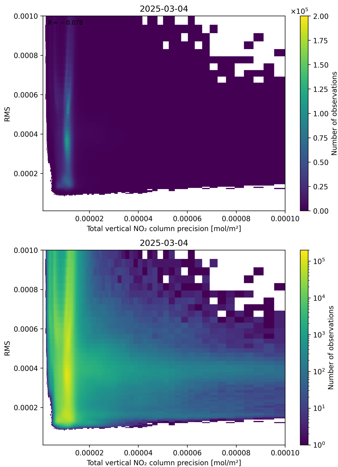
Figure 119: Scatter density plot of “Total vertical NO 2 column precision” against “RMS” for 2025-03-03 to 2025-03-05.
