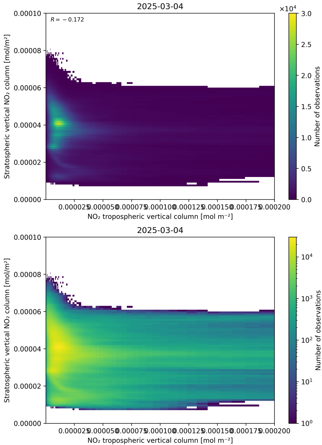
Figure 125: Scatter density plot of “NO 2 tropospheric vertical column” against “Stratospheric vertical NO 2 column” for 2025-03-03 to 2025-03-05.
