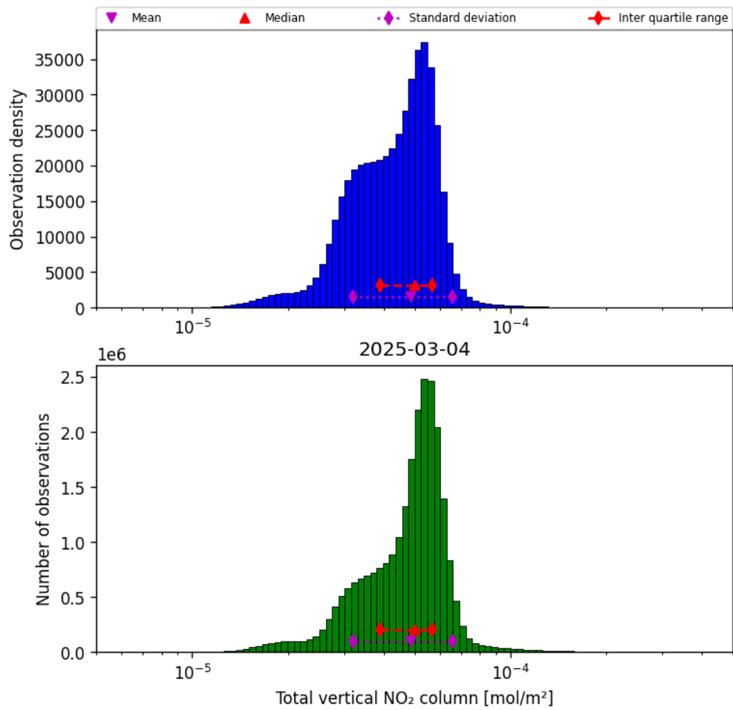
Figure 38: Histogram of “Total vertical NO 2 column” for 2025-03-03 to 2025-03-05
