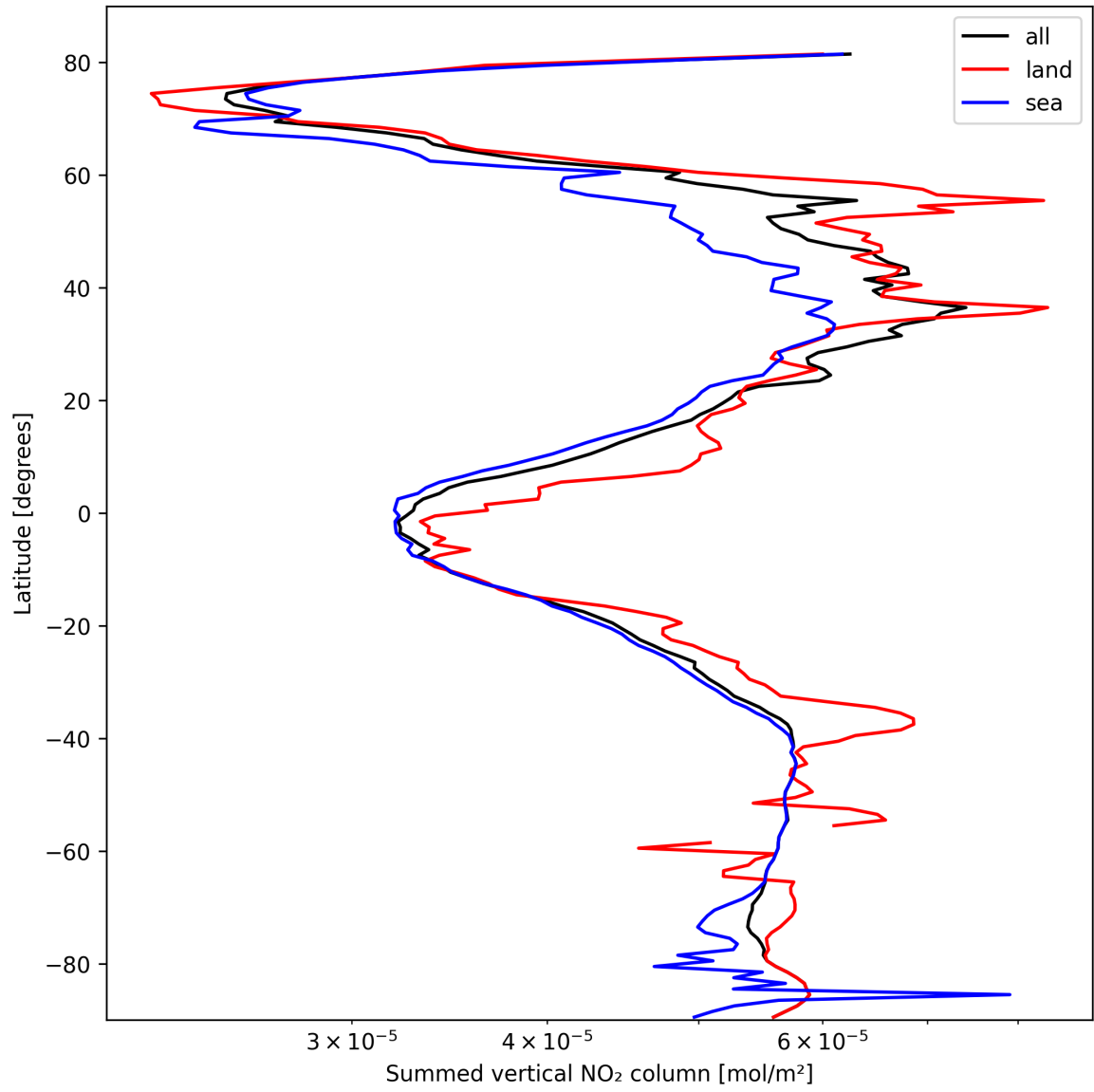
Figure 23: Zonal average of “Summed vertical NO 2 column” for 2025-03-03 to 2025-03-05.
