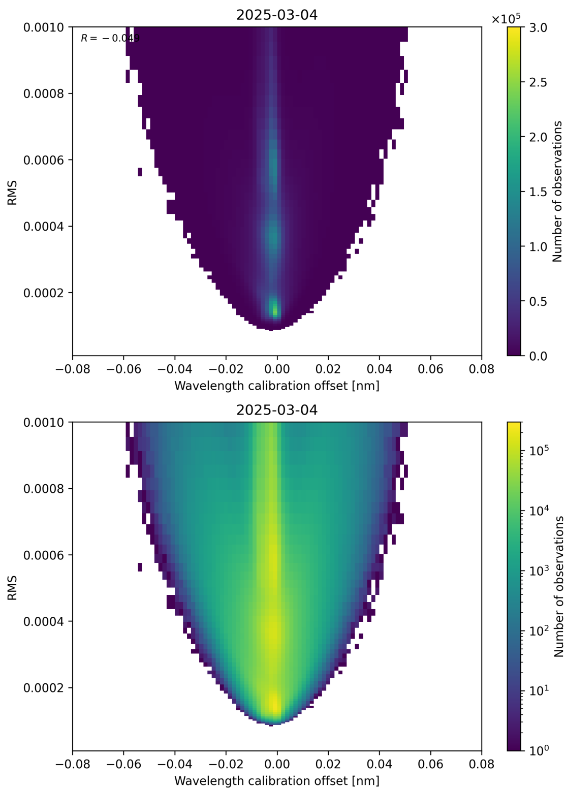
Figure 181: Scatter density plot of “Wavelength calibration offset” against “RMS” for 2025-03-03 to 2025-03-05.
