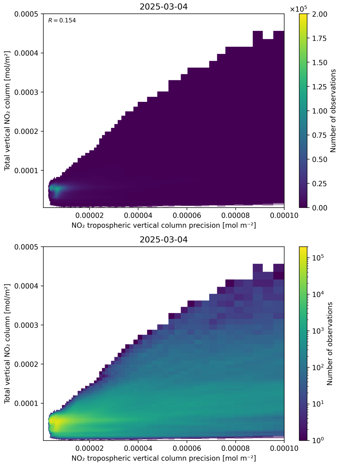
Figure 138: Scatter density plot of “NO 2 tropospheric vertical column precision” against “Total vertical NO 2 column” for 2025-03-03 to 2025-03-05.
