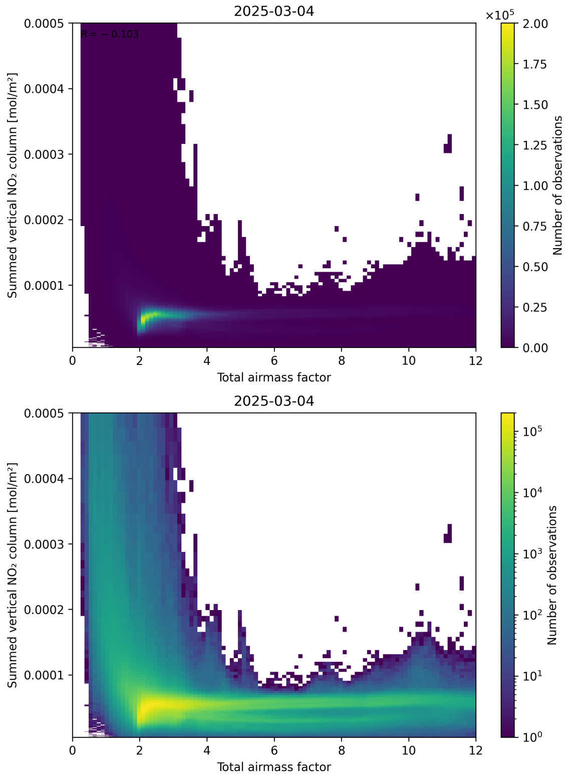
Figure 65: Scatter density plot of “Total airmass factor” against “Summed vertical NO 2 column” for 2025-03-03 to 2025-03-05.
