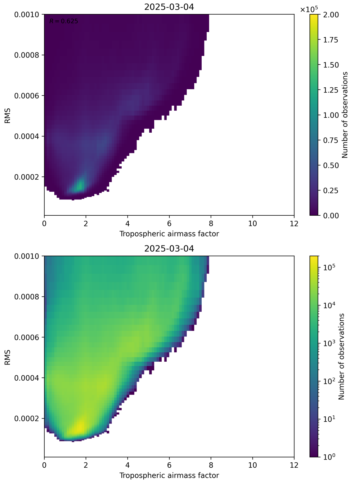
Figure 79: Scatter density plot of “Tropospheric airmass factor” against “RMS” for 2025-03-03 to 2025-03-05.
