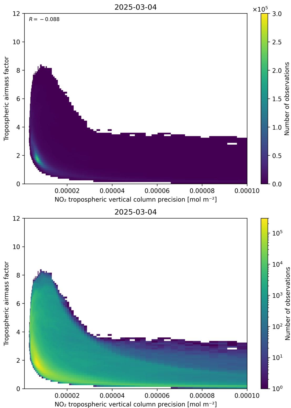
Figure 133: Scatter density plot of “NO 2 tropospheric vertical column precision” against “Tropospheric airmass factor” for 2025-03-03 to 2025-03-05.
