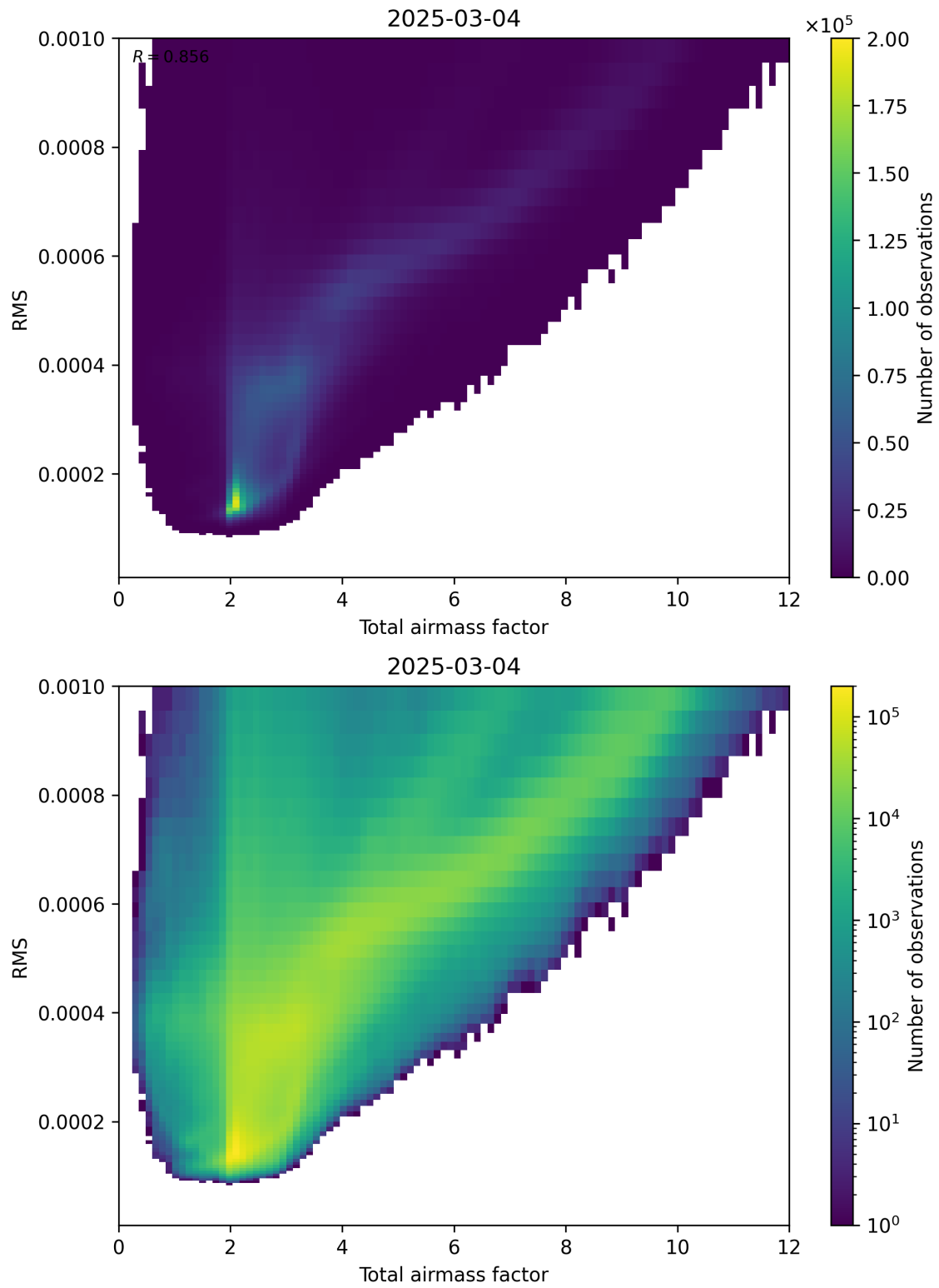
Figure 69: Scatter density plot of “Total airmass factor” against “RMS” for 2025-03-03 to 2025-03-05.
