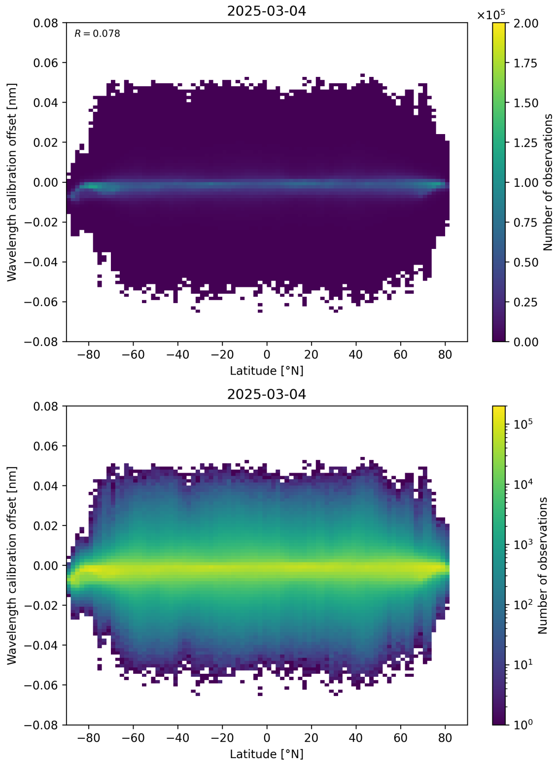
Figure 95: Scatter density plot of “Latitude” against “Wavelength calibration offset” for 2025-03-03 to 2025-03-05.
