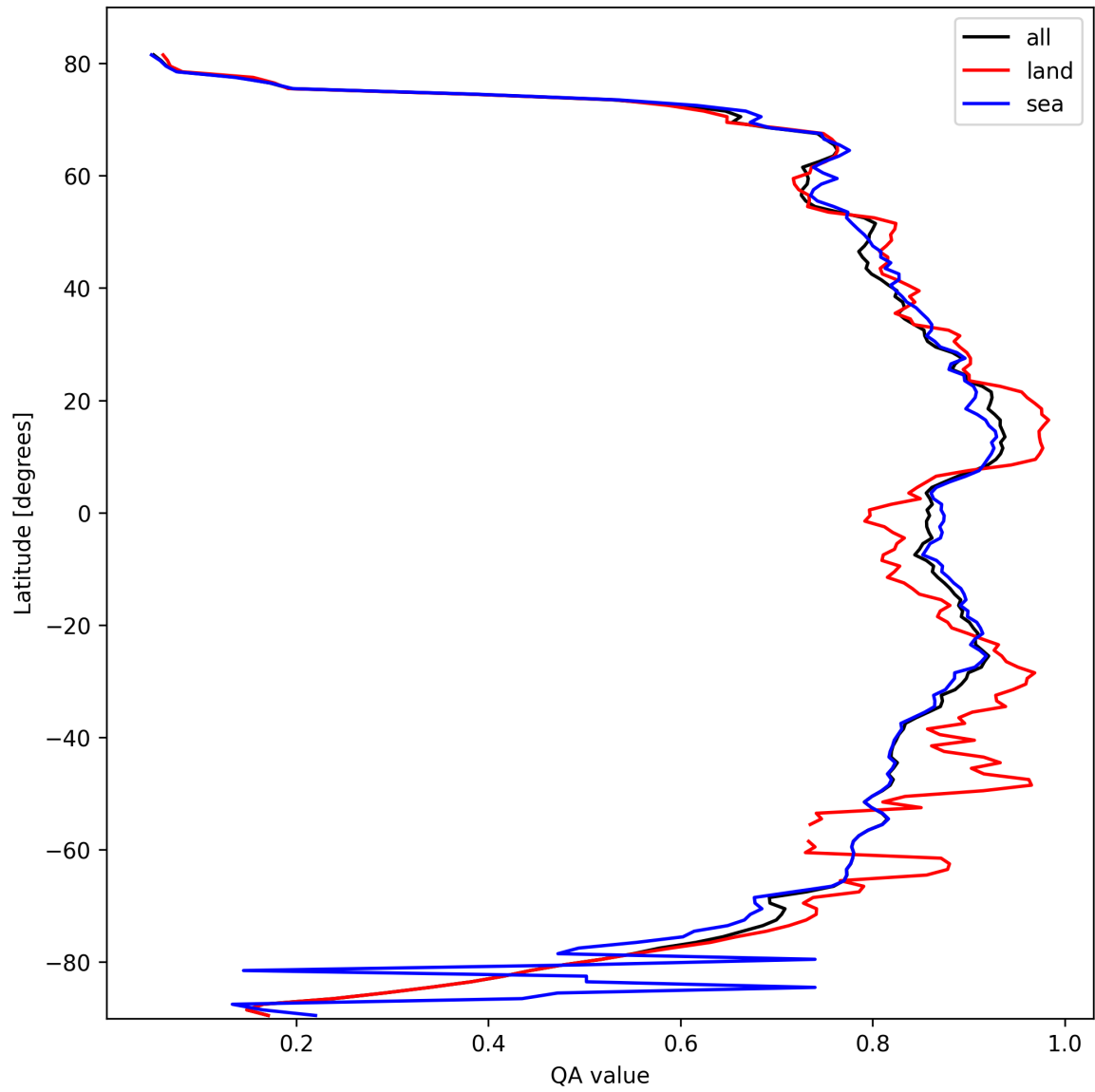
Figure 11: Zonal average of “QA value” for 2025-03-03 to 2025-03-05.
