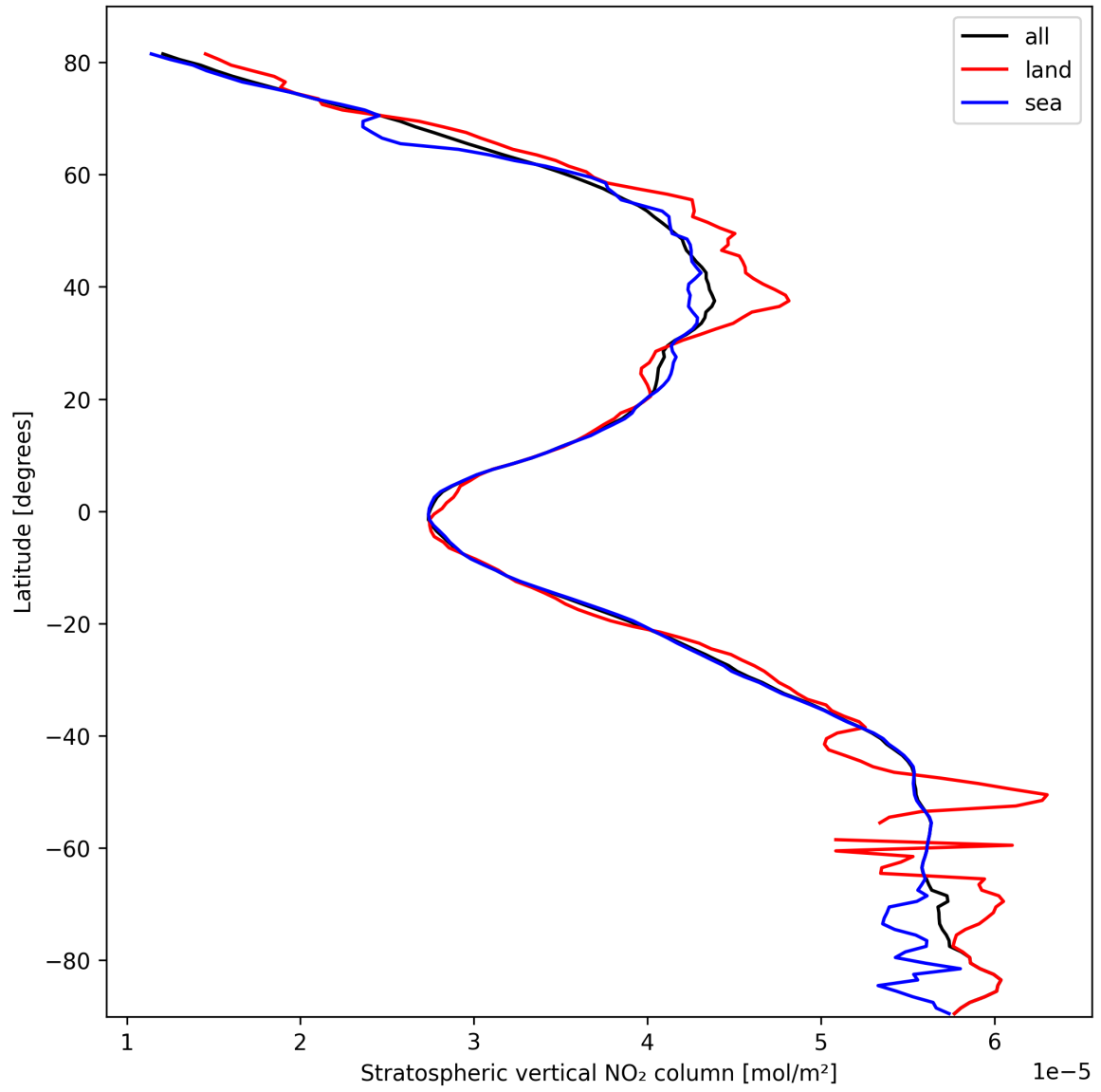
Figure 19: Zonal average of “Stratospheric vertical NO 2 column” for 2025-03-03 to 2025-03-05.
