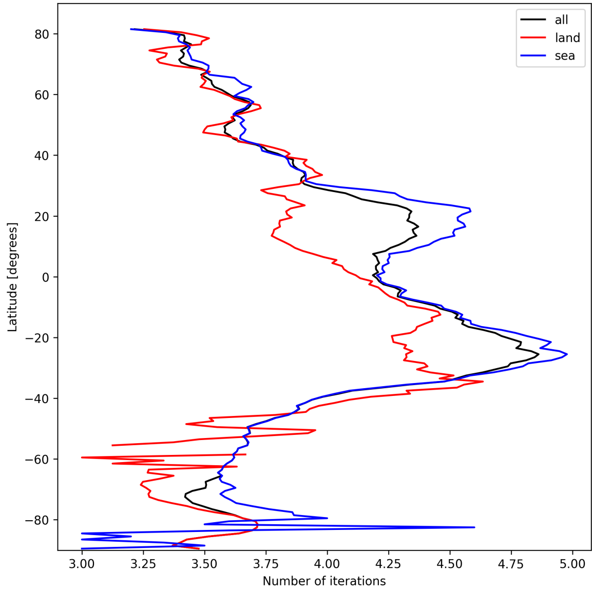
Figure 17: Zonal average of “Number of iterations” for 2025-03-03 to 2025-03-05.
