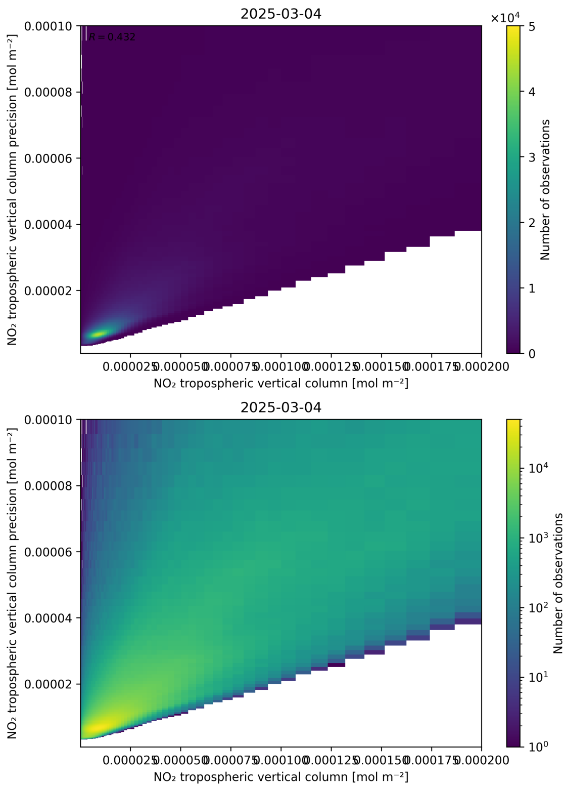
Figure 130: Scatter density plot of “NO 2 tropospheric vertical column” against “NO 2 tropospheric vertical column precision” for 2025-03-03 to 2025-03-05.
