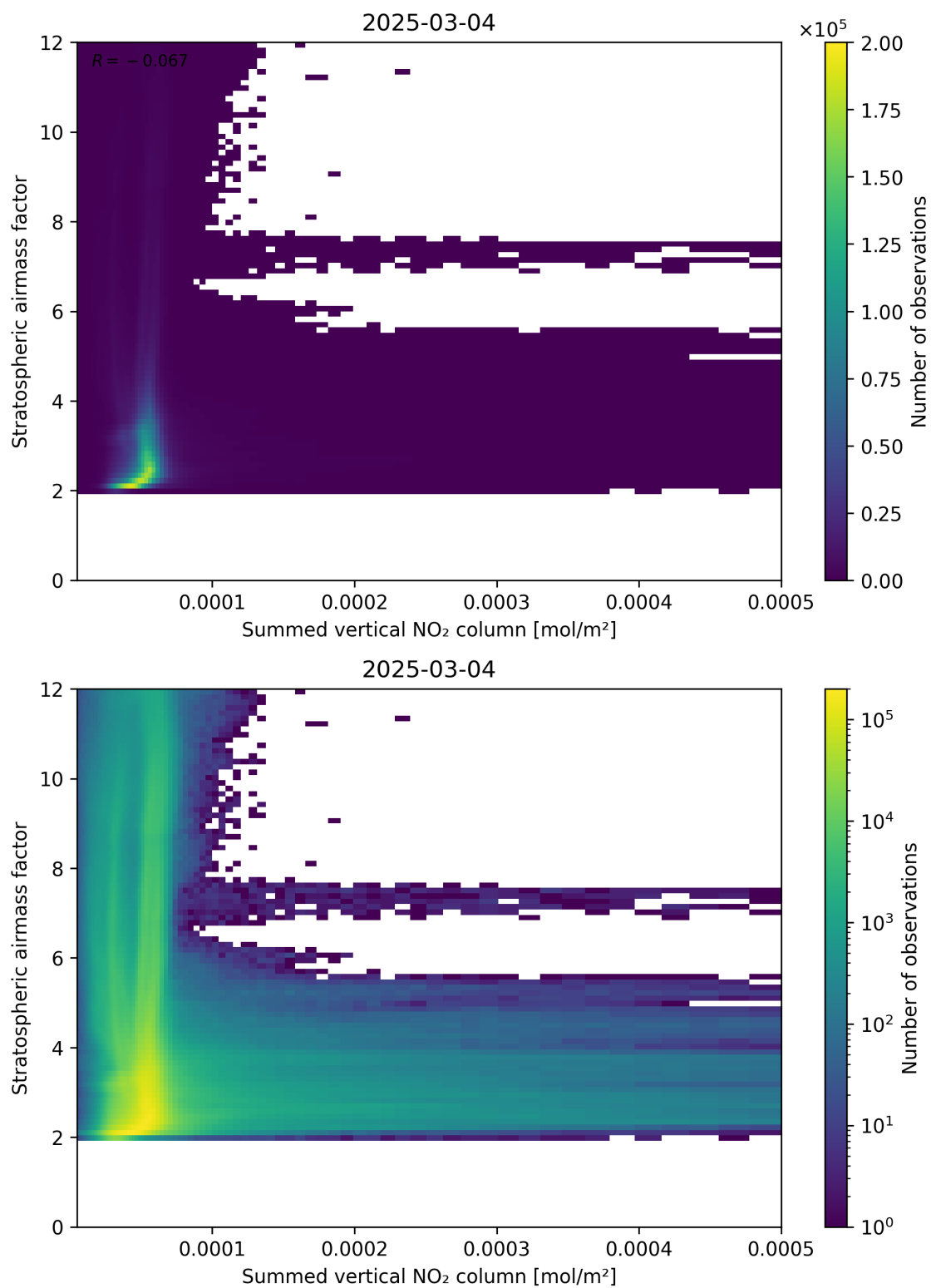
Figure 103: Scatter density plot of “Summed vertical NO 2 column” against “Stratospheric air mass factor” for 2025-03-03 to 2025-03-05.
