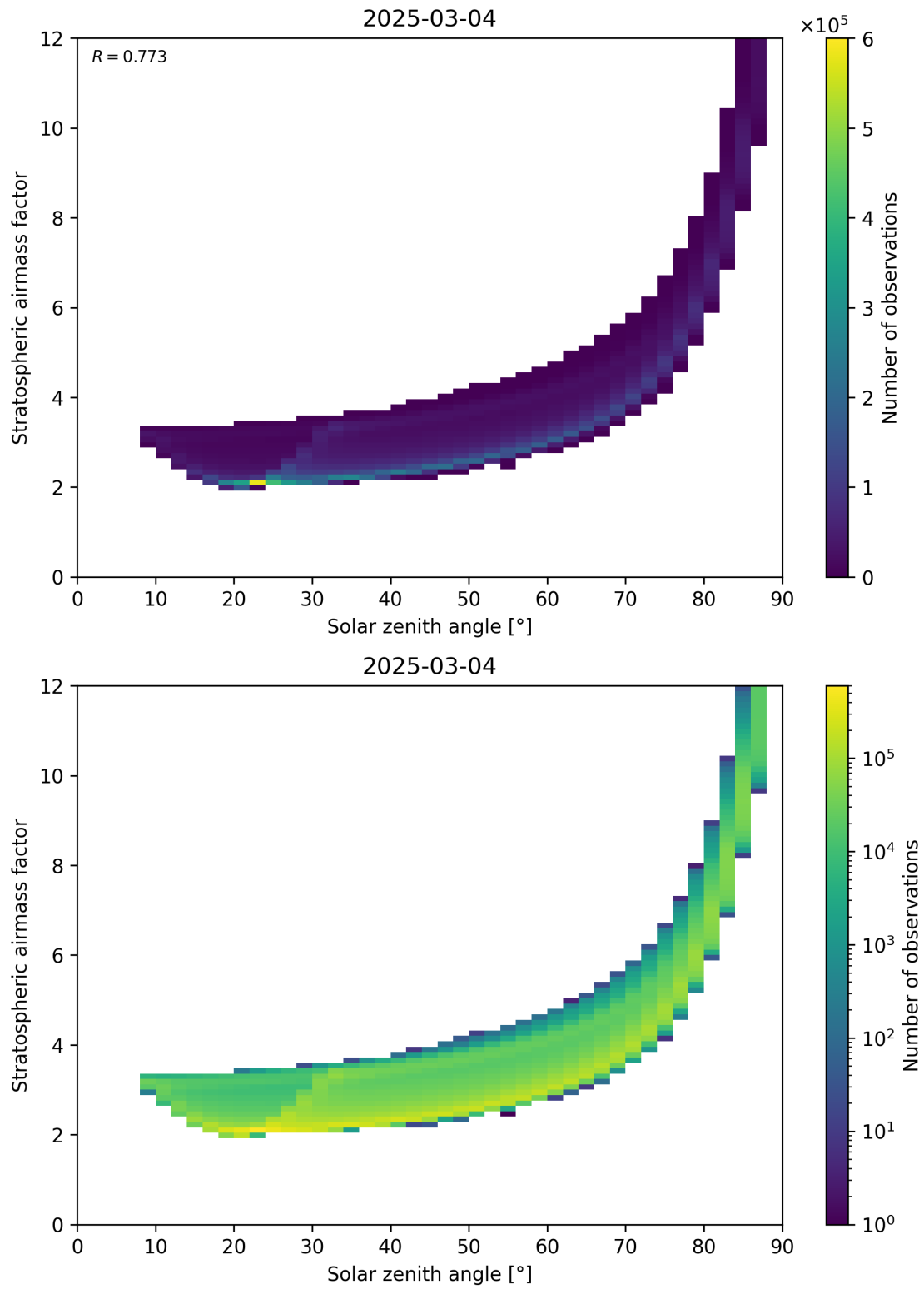
Figure 145: Scatter density plot of “Solar zenith angle” against “Stratospheric airmass factor” for 2025-03-03 to 2025-03-05.
