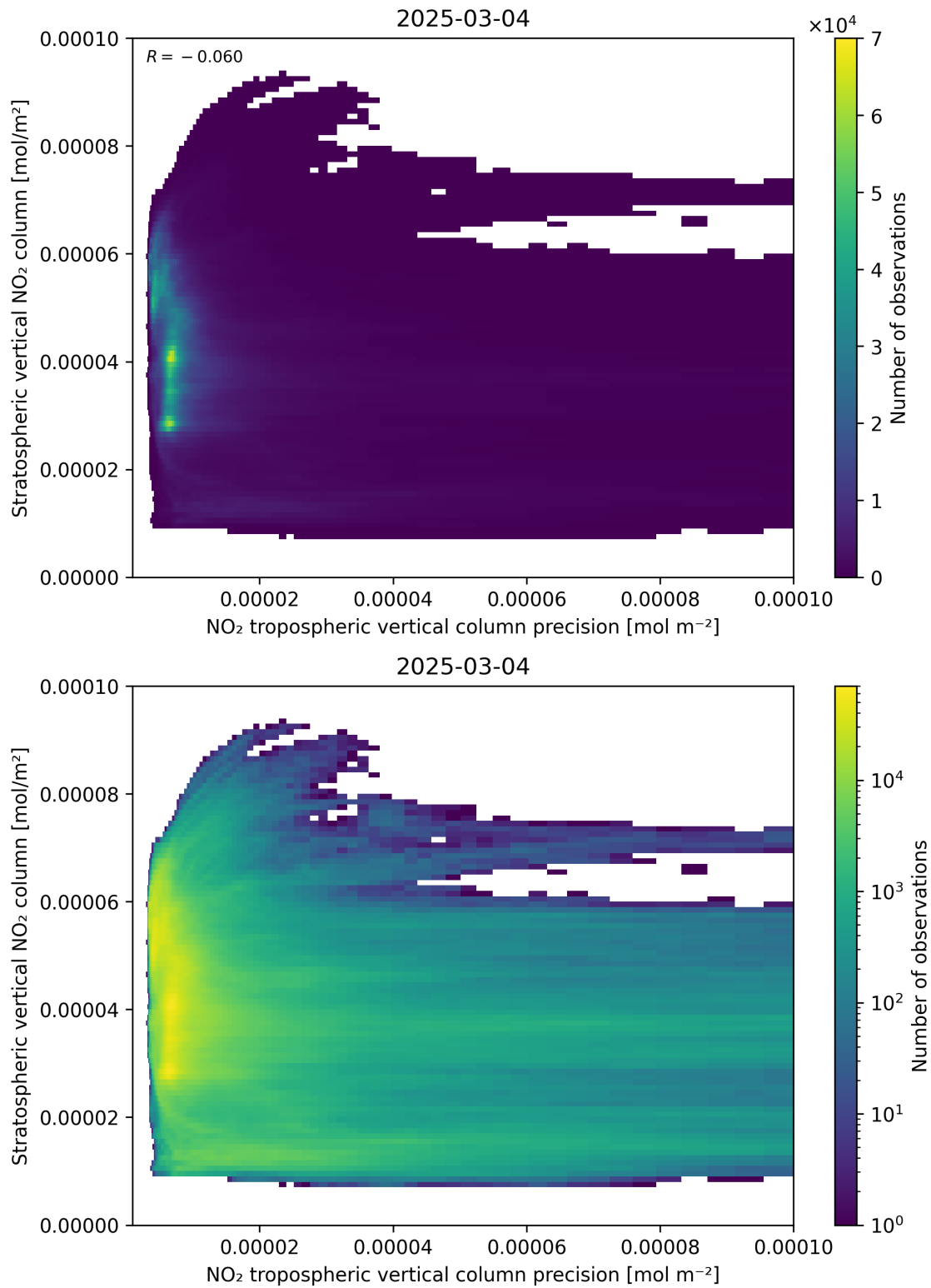
Figure 135: Scatter density plot of “NO 2 tropospheric vertical column precision” against “Stratospheric vertical NO 2 column” for 2025-03-03 to 2025-03-05.
