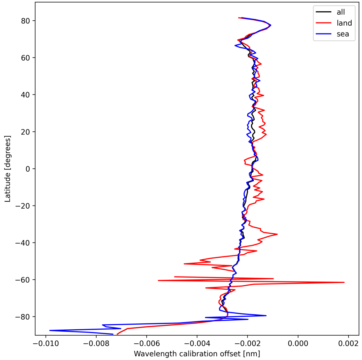
Figure 18: Zonal average of “Wavelength calibration offset” for 2025-03-03 to 2025-03-05.
