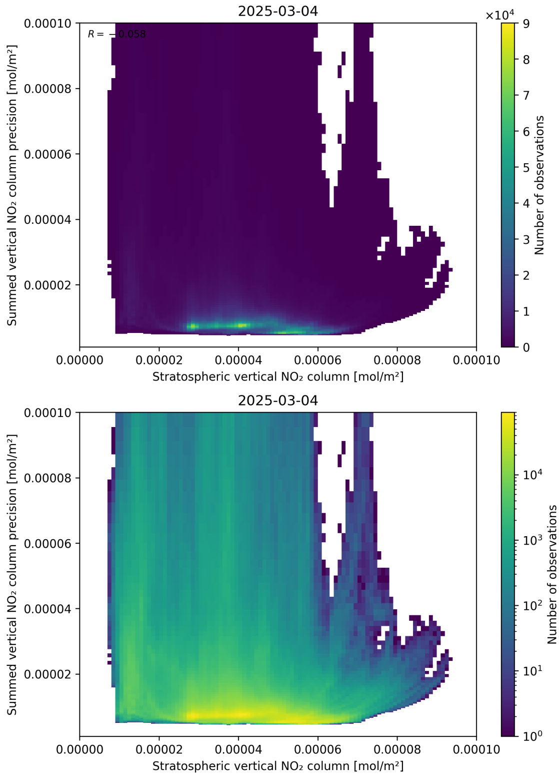
Figure 99: Scatter density plot of “Stratospheric vertical NO 2 column” against “Summed vertical NO 2 column precision” for 2025-03-03 to 2025-03-05.
