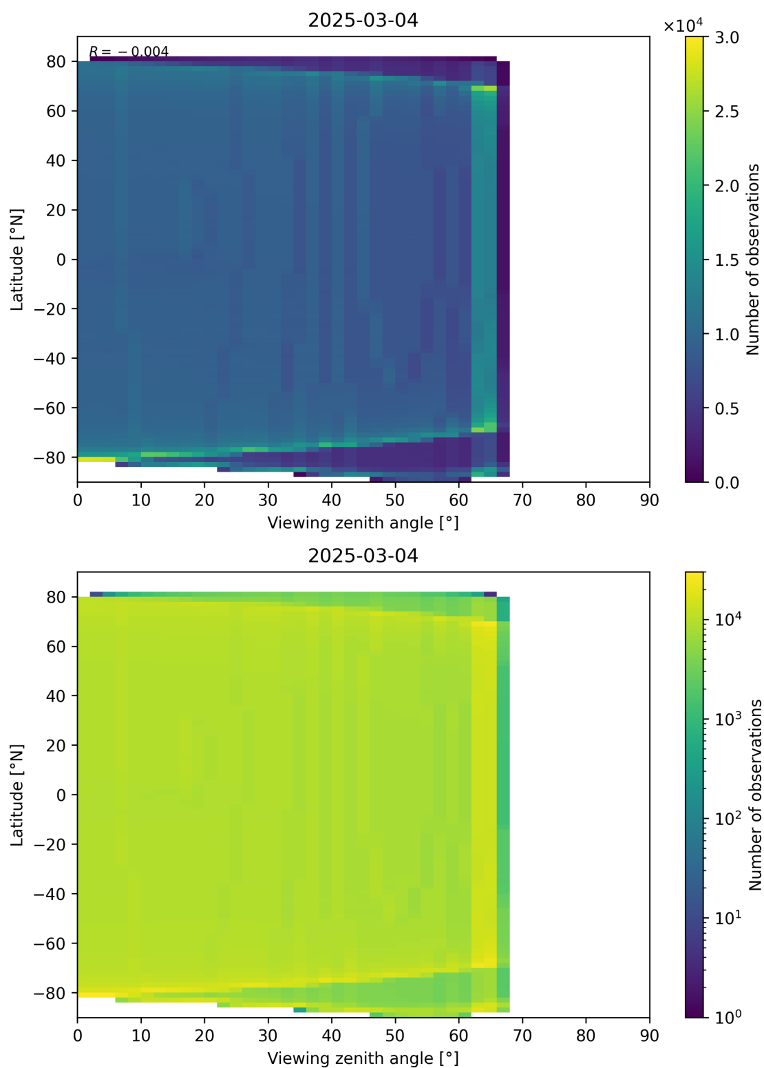
Figure 163: Scatter density plot of “Viewing zenith angle” against “Latitude” for 2025-03-03 to 2025-03-05.
