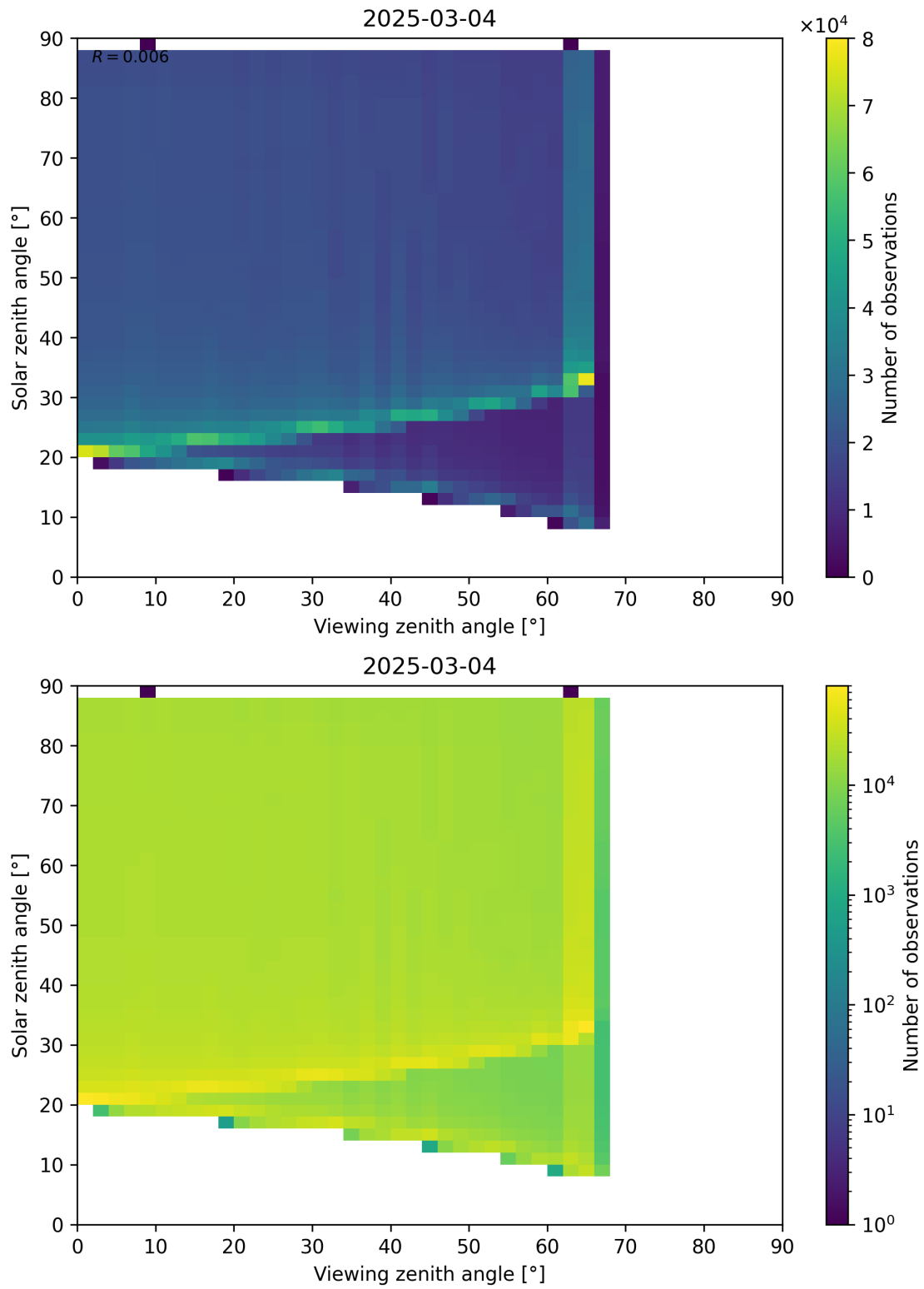
Figure 172: Scatter density plot of “Viewing zenith angle” against “Solar zenith angle” for 2025-03-03 to 2025-03-05.
