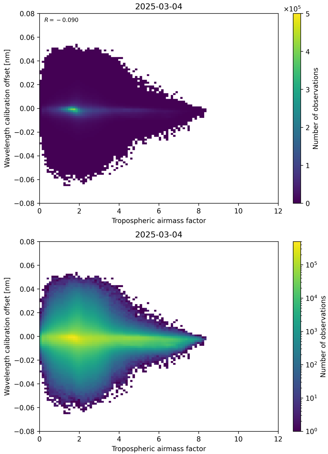
Figure 80: Scatter density plot of “Tropospheric airmass factor” against “Wavelength calibration offset” for 2025-03-03 to 2025-03-05.
