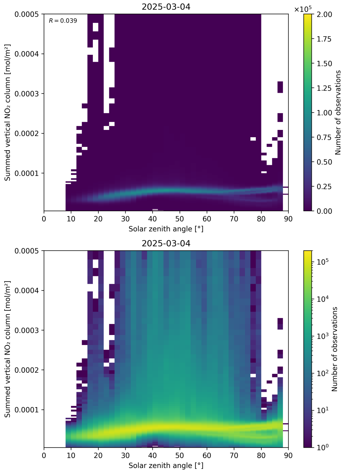
Figure 151: Scatter density plot of “Solar zenith angle” against “Summed vertical NO 2 column” for 2025-03-03 to 2025-03-05.
