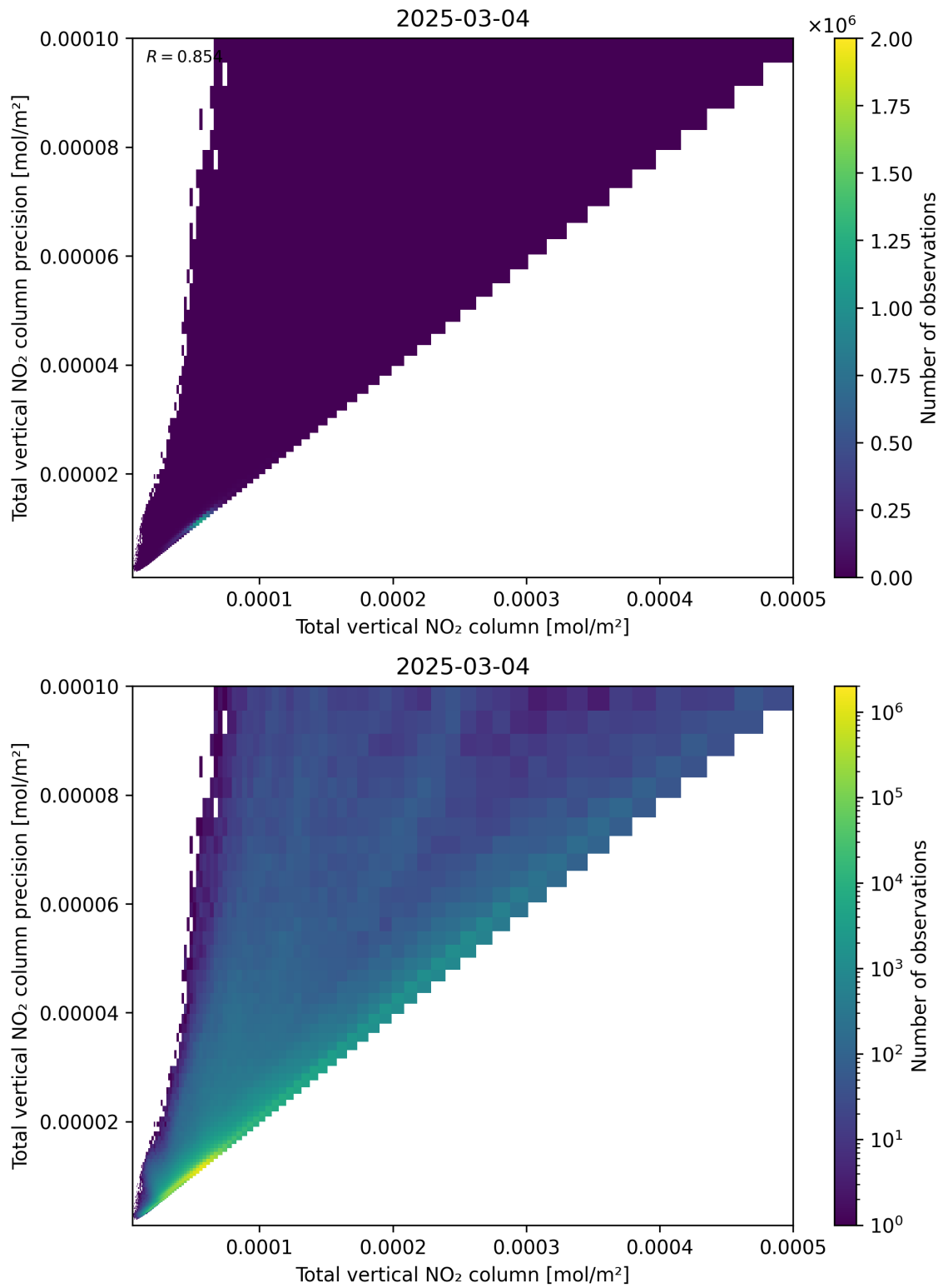
Figure 114: Scatter density plot of “Total vertical NO 2 column” against “Total vertical NO 2 column precision” for 2025-03-03 to 2025-03-05.
