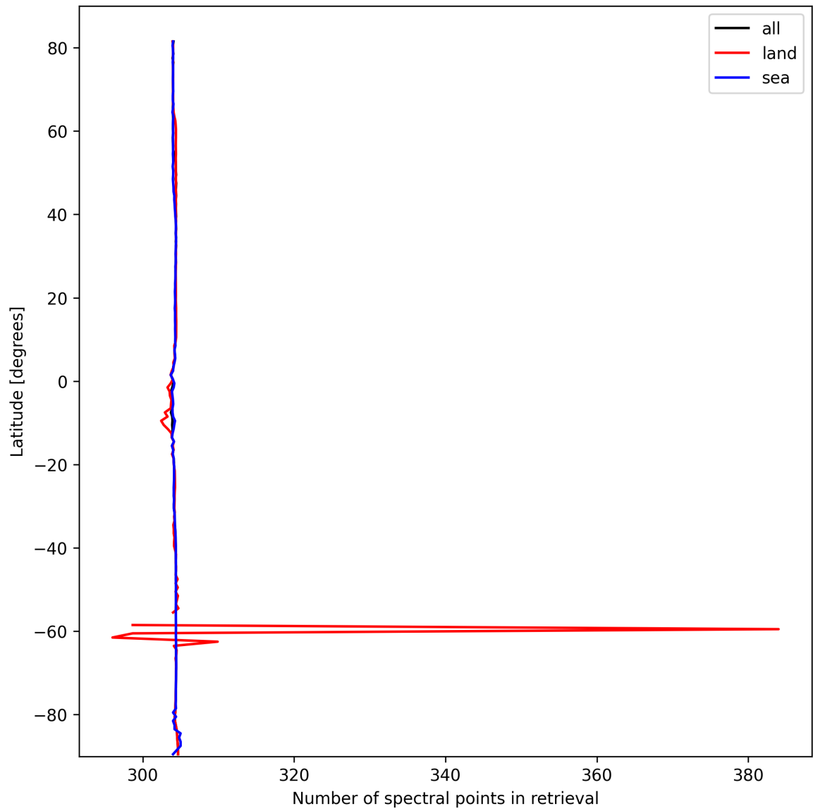
Figure 16: Zonal average of “Number of spectral points in retrieval” for 2025-03-03 to 2025-03-05.
