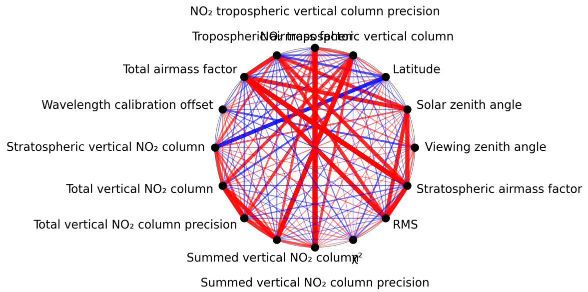
Figure 1: Map of correlation graph for 2025-03-03 to 2025-03-05.
