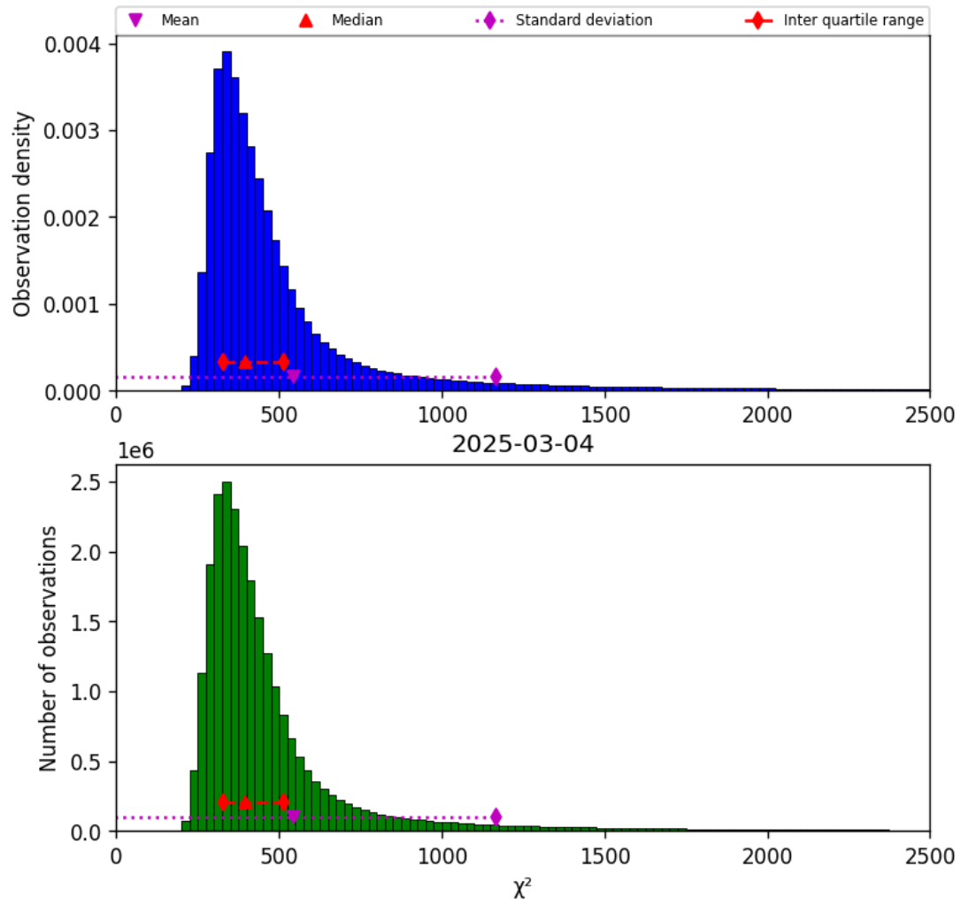
Figure 42: Histogram of " \chi^2 " for 2025-03-03 to 2025-03-05
