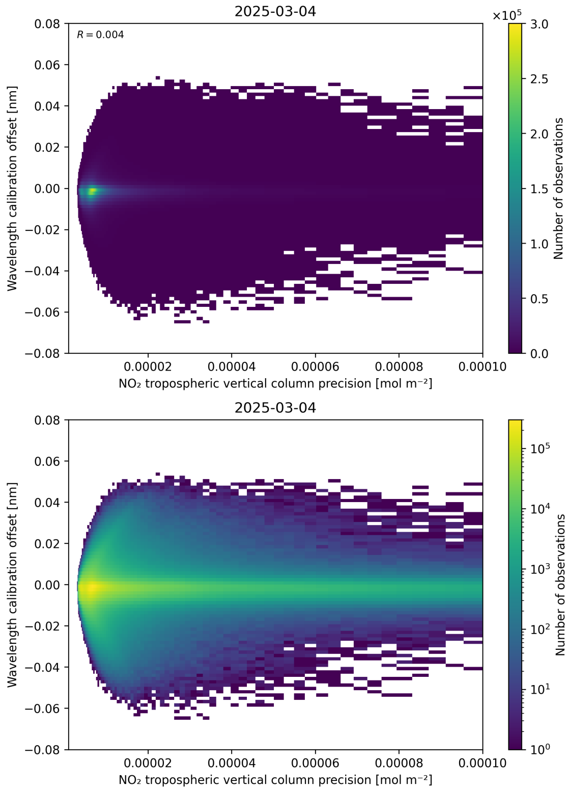
Figure 141: Scatter density plot of “NO 2 tropospheric vertical column precision” against “Wavelength calibration offset” for 2025-03-03 to 2025-03-05.
