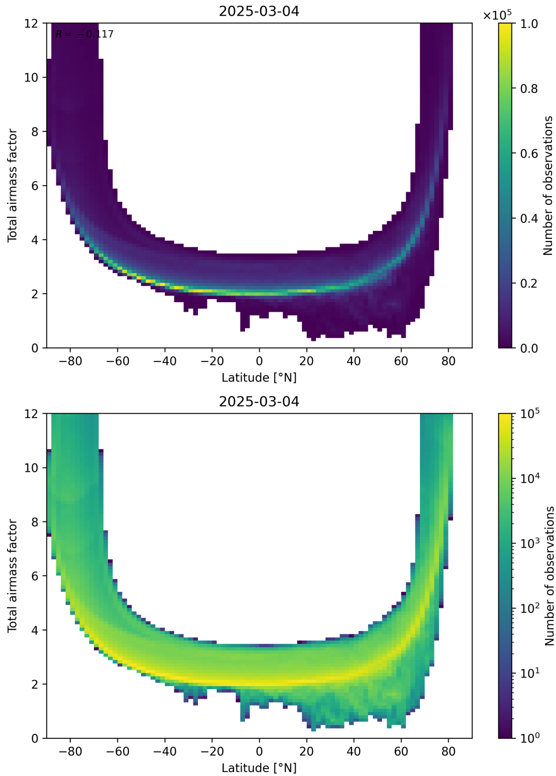
Figure 84: Scatter density plot of “Latitude” against “Total airmass factor” for 2025-03-03 to 2025-03-05.
