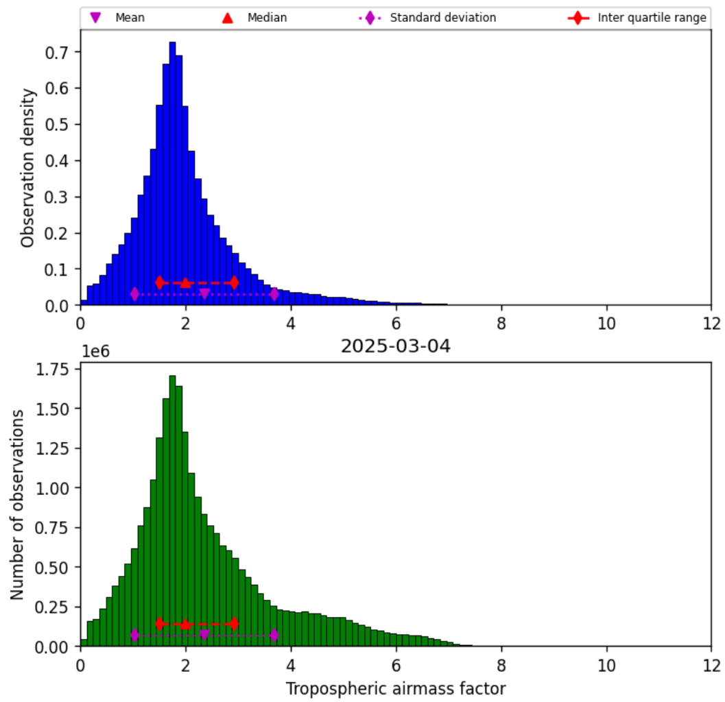
Figure 31: Histogram of “Tropospheric airmass factor” for 2025-03-03 to 2025-03-05
