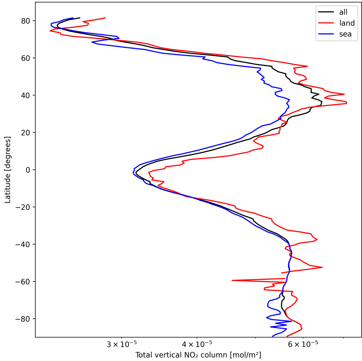
Figure 21: Zonal average of “Total vertical NO 2 column” for 2025-03-03 to 2025-03-05.
