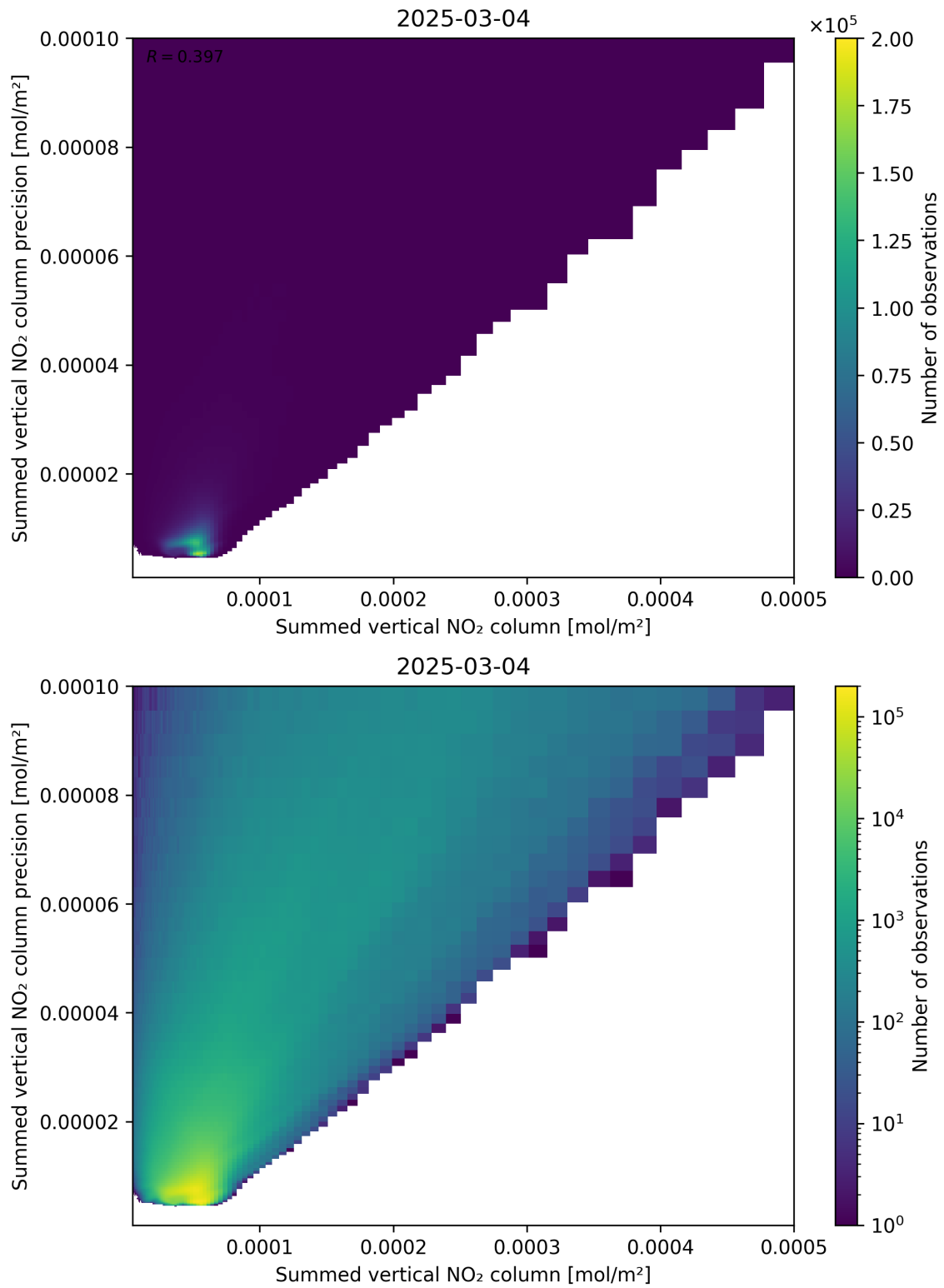
Figure 105: Scatter density plot of “Summed vertical NO 2 column” against “Summed vertical NO 2 column precision” for 2025-03-03 to 2025-03-05.
