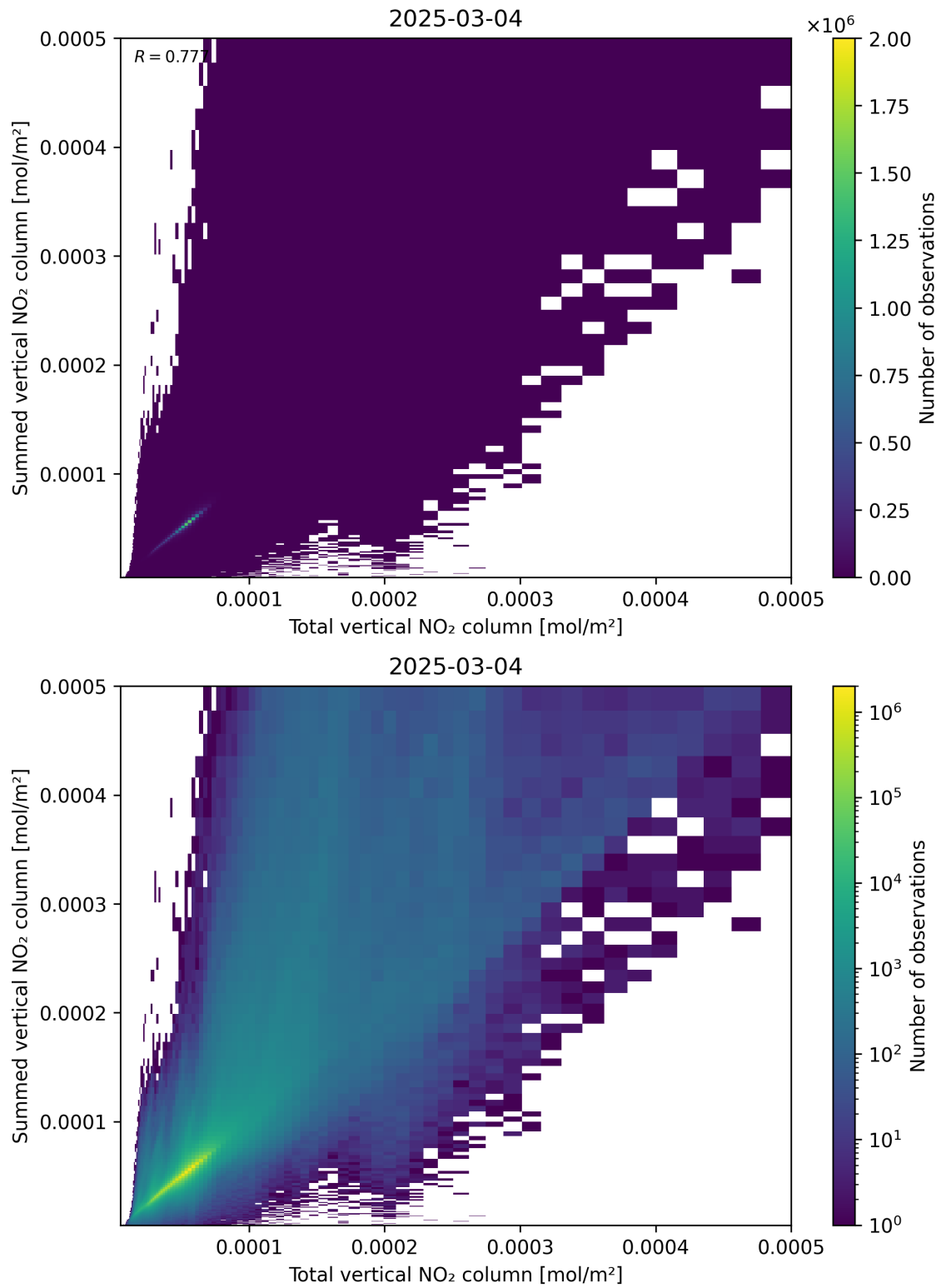
Figure 112: Scatter density plot of “Total vertical NO 2 column” against “Summed vertical NO 2 column” for 2025-03-03 to 2025-03-05.
