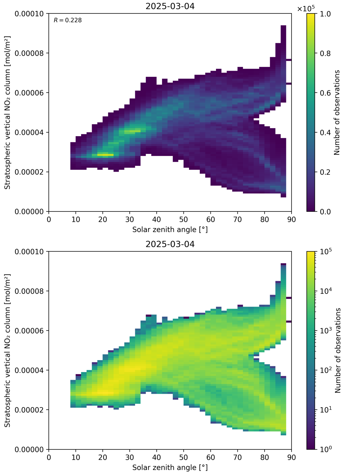
Figure 150: Scatter density plot of “Solar zenith angle” against “Stratospheric vertical NO 2 column” for 2025-03-03 to 2025-03-05.
