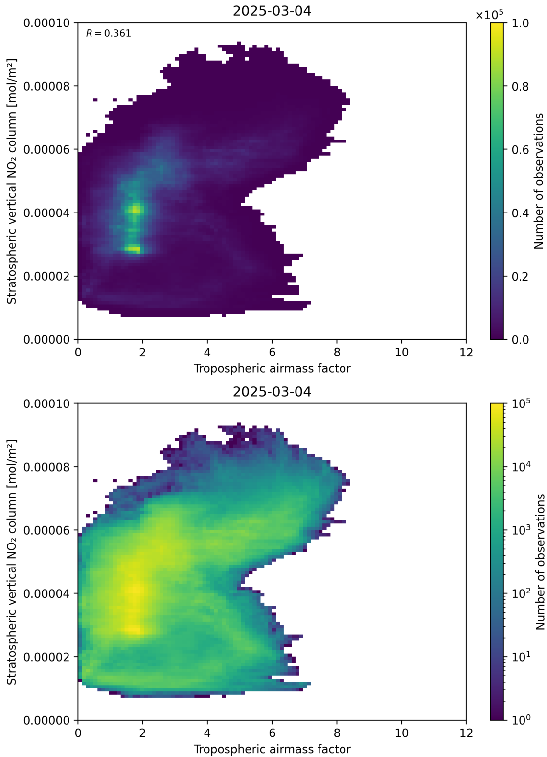
Figure 74: Scatter density plot of “Tropospheric airmass factor” against “Stratospheric vertical \text{NO}_2 column” for 2025-03-03 to 2025-03-05.
