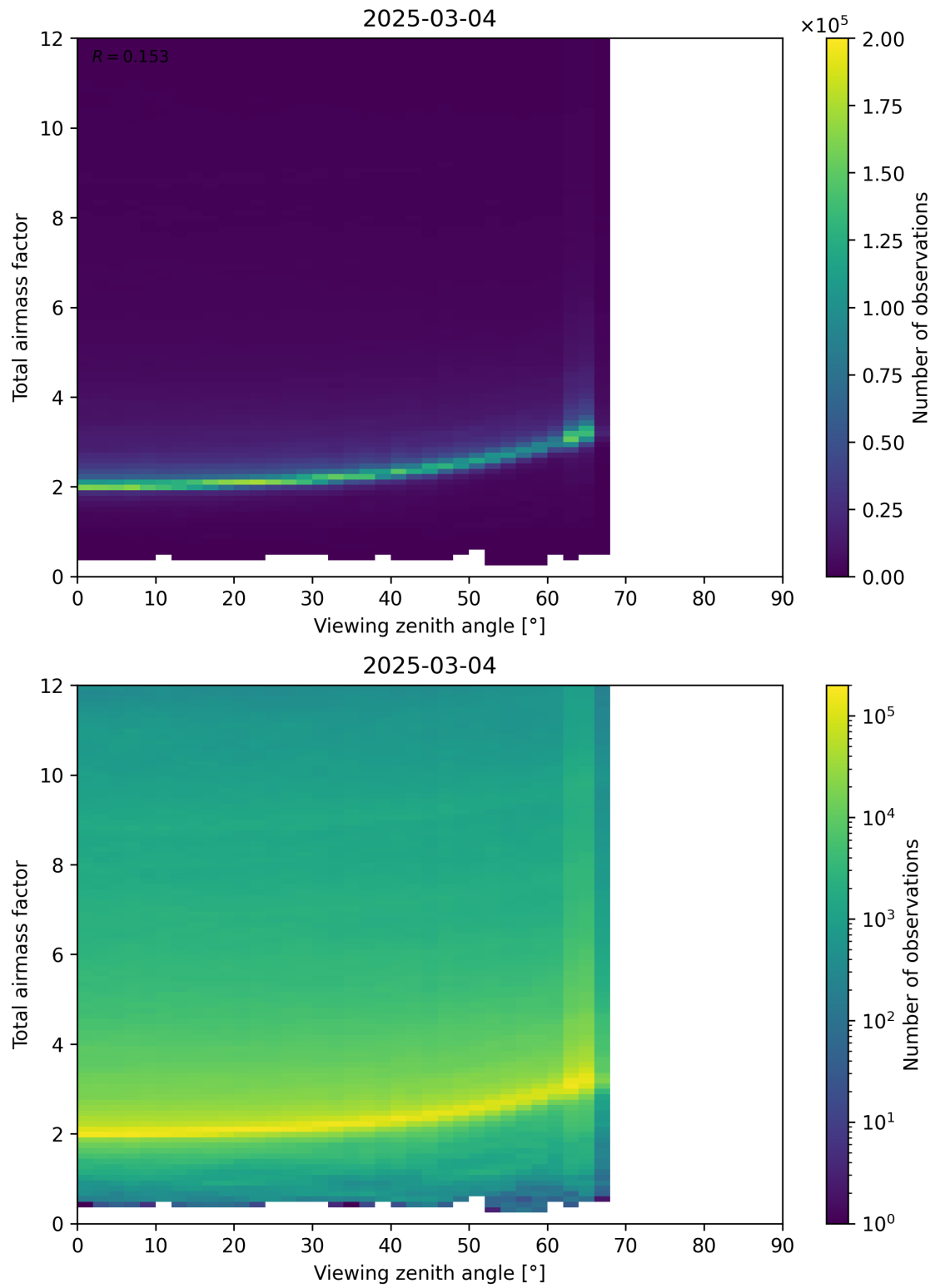
Figure 160: Scatter density plot of “Viewing zenith angle” against “Total airmass factor” for 2025-03-03 to 2025-03-05.
