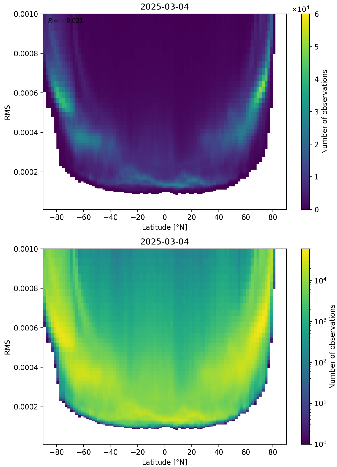
Figure 94: Scatter density plot of “Latitude” against “RMS” for 2025-03-03 to 2025-03-05.
