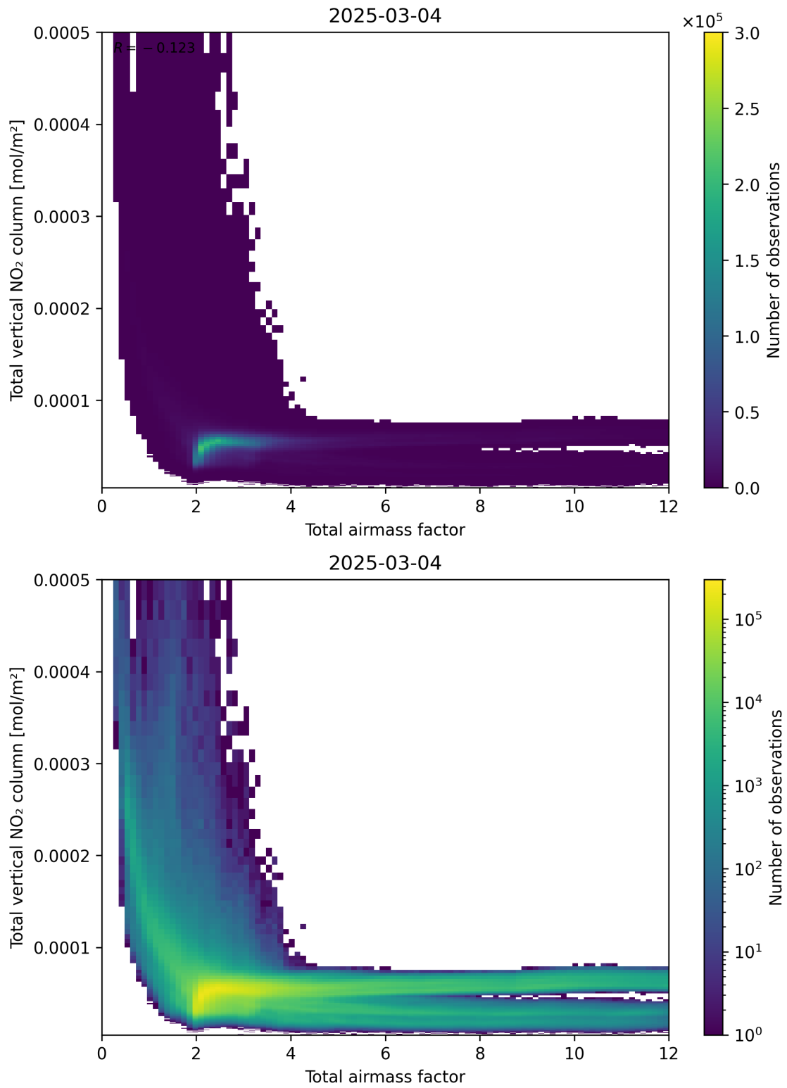
Figure 67: Scatter density plot of “Total airmass factor” against “Total vertical \text{NO}_2 column” for 2025-03-03 to 2025-03-05.
