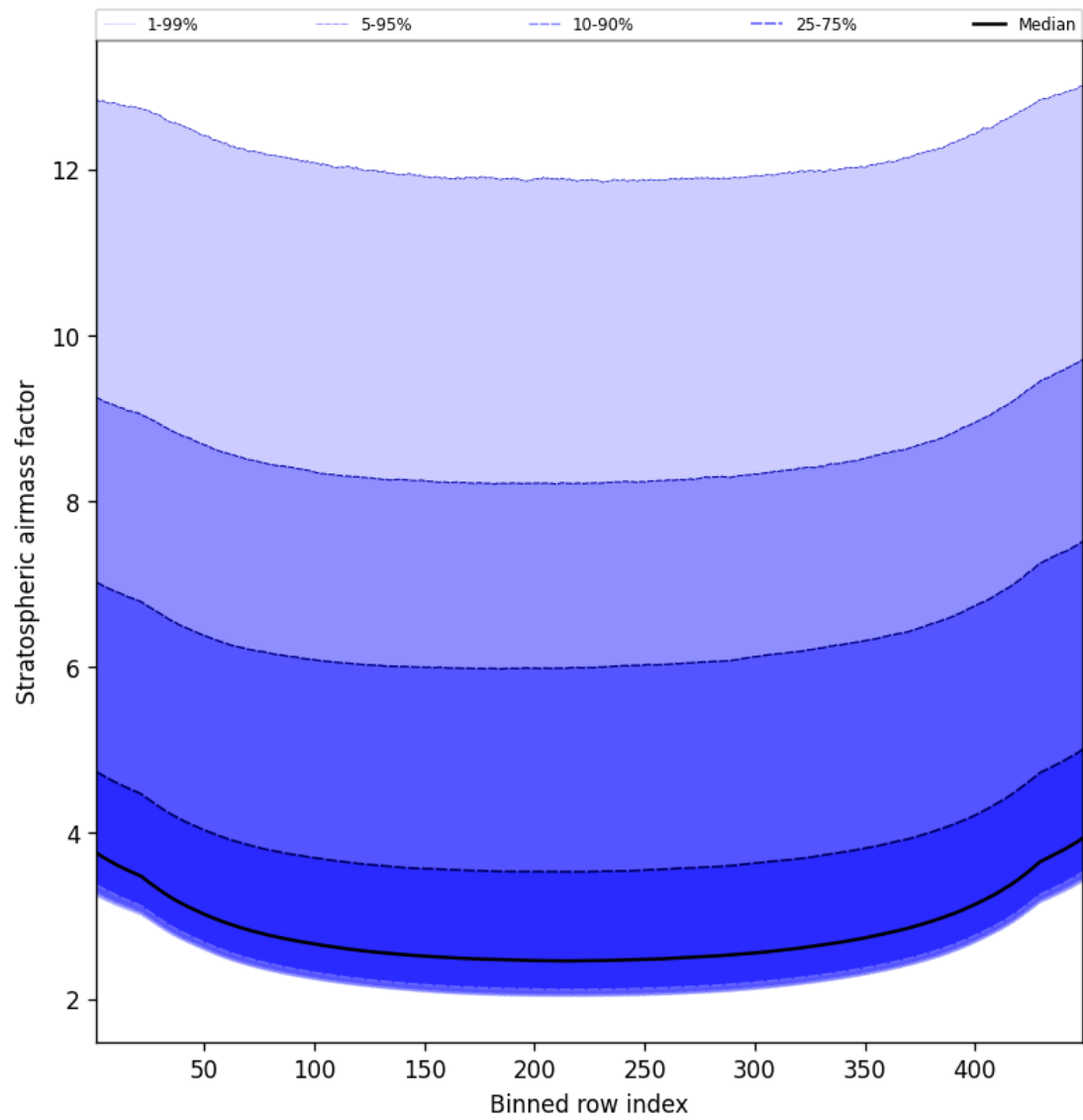
Figure 61: Along track statistics of “Stratospheric air mass factor” for 2025-03-03 to 2025-03-05
