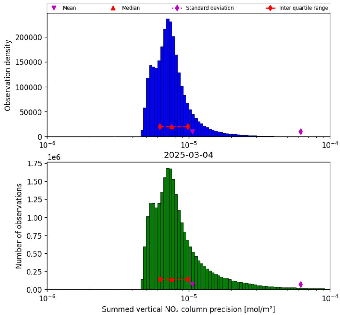
Figure 41: Histogram of “Summed vertical NO 2 column precision” for 2025-03-03 to 2025-03-05
