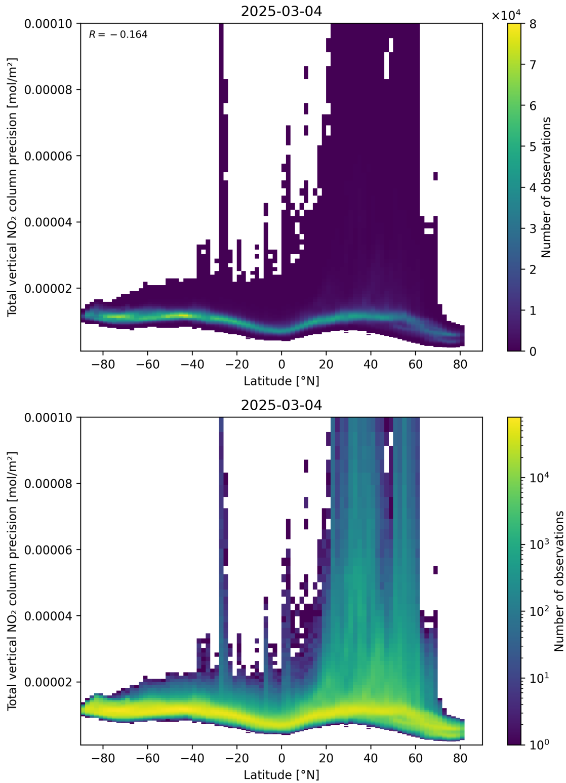
Figure 91: Scatter density plot of “Latitude” against “Total vertical NO 2 column precision” for 2025-03-03 to 2025-03-05.
