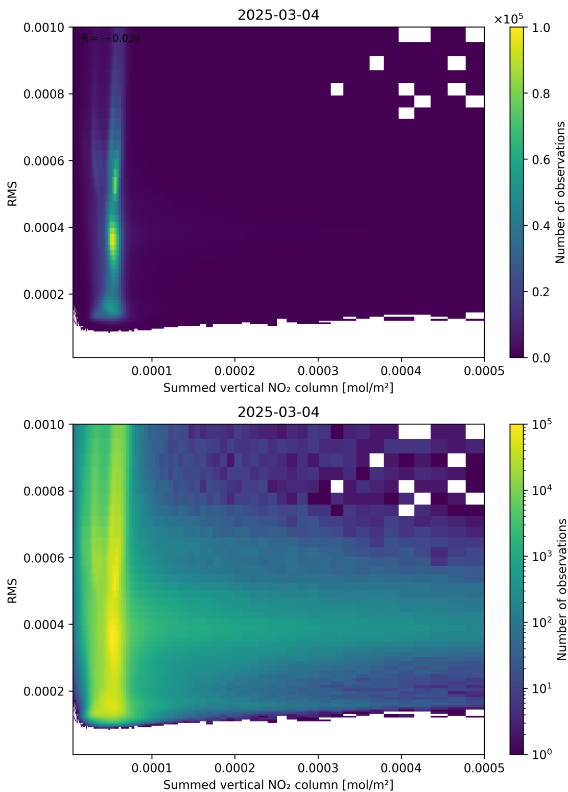
Figure 109: Scatter density plot of “Summed vertical NO 2 column” against “RMS” for 2025-03-03 to 2025-03-05.
