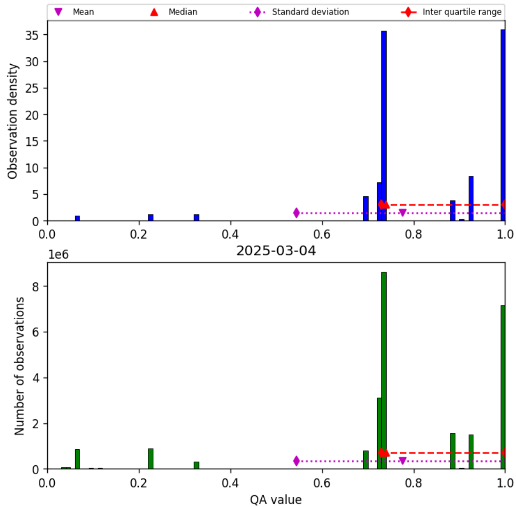
Figure 28: Histogram of “QA value” for 2025-03-03 to 2025-03-05
