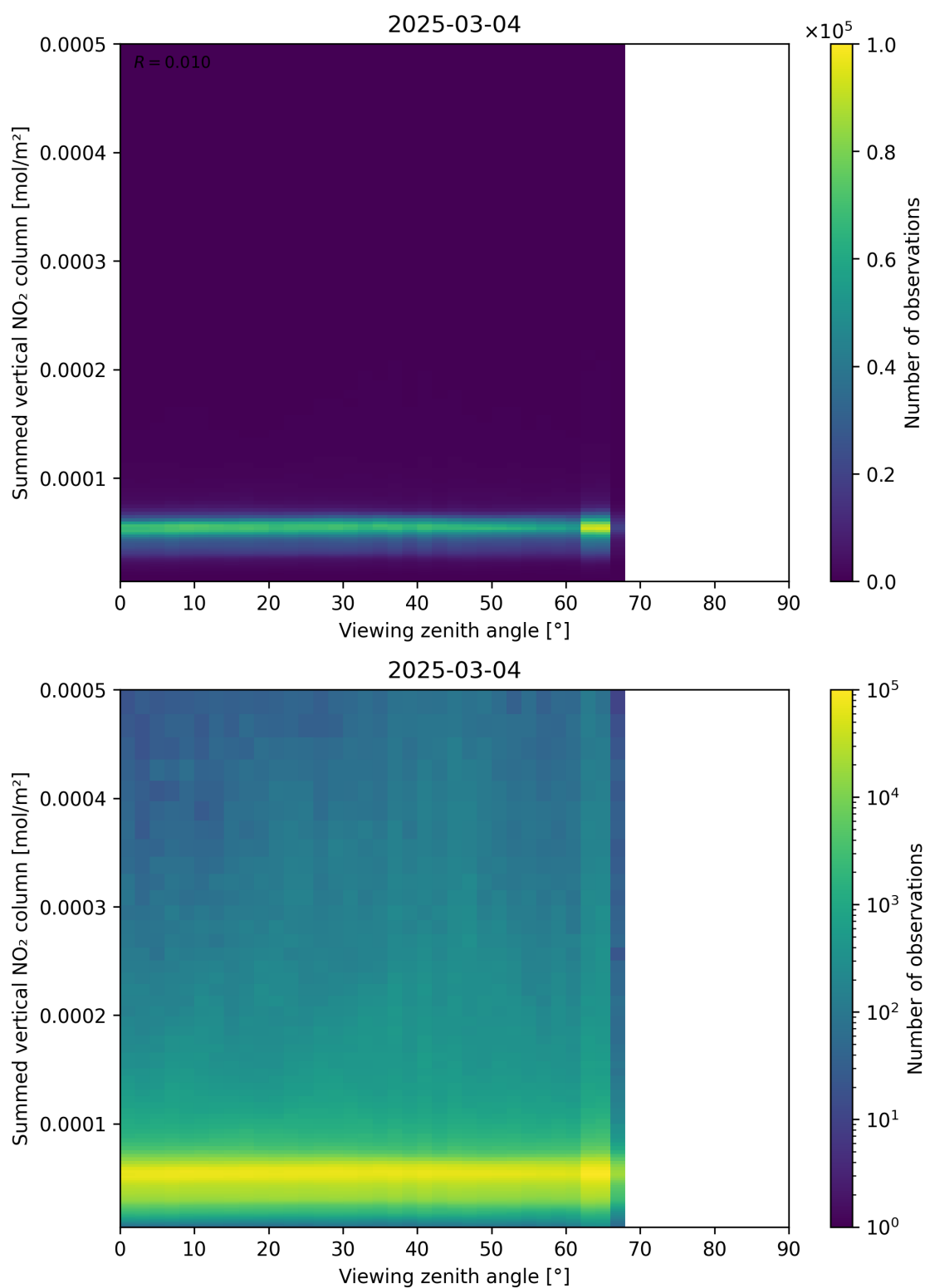
Figure 165: Scatter density plot of “Viewing zenith angle” against “Summed vertical NO 2 column” for 2025-03-03 to 2025-03-05.
