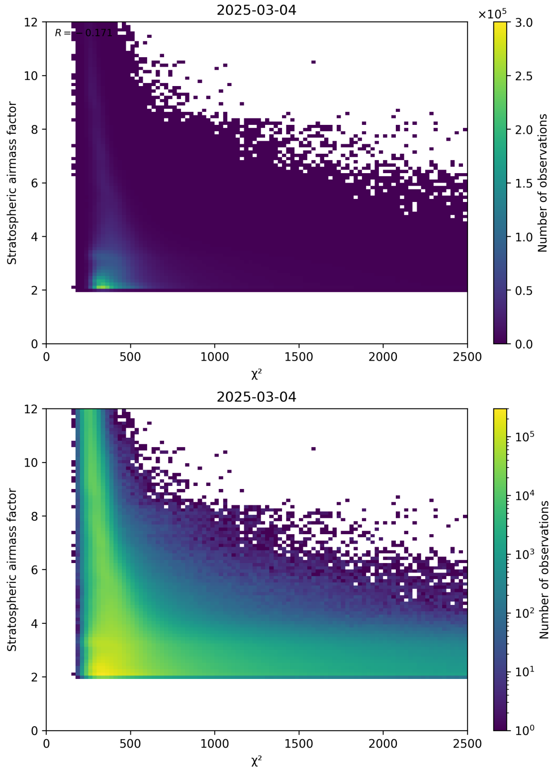
Figure 81: Scatter density plot of “ \chi^2 ” against “Stratospheric airmass factor” for 2025-03-03 to 2025-03-05.
