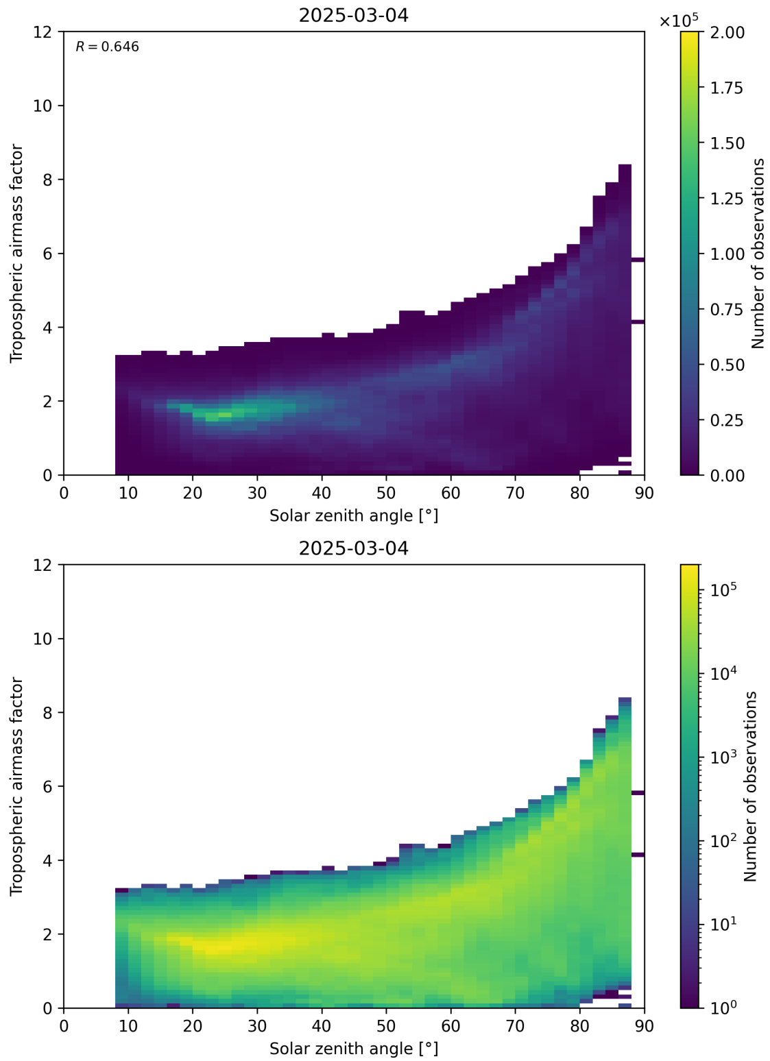
Figure 147: Scatter density plot of “Solar zenith angle” against “Tropospheric airmass factor” for 2025-03-03 to 2025-03-05.
