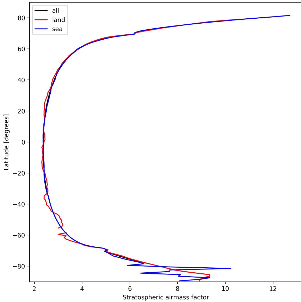
Figure 27: Zonal average of “Stratospheric air mass factor” for 2025-03-03 to 2025-03-05.
