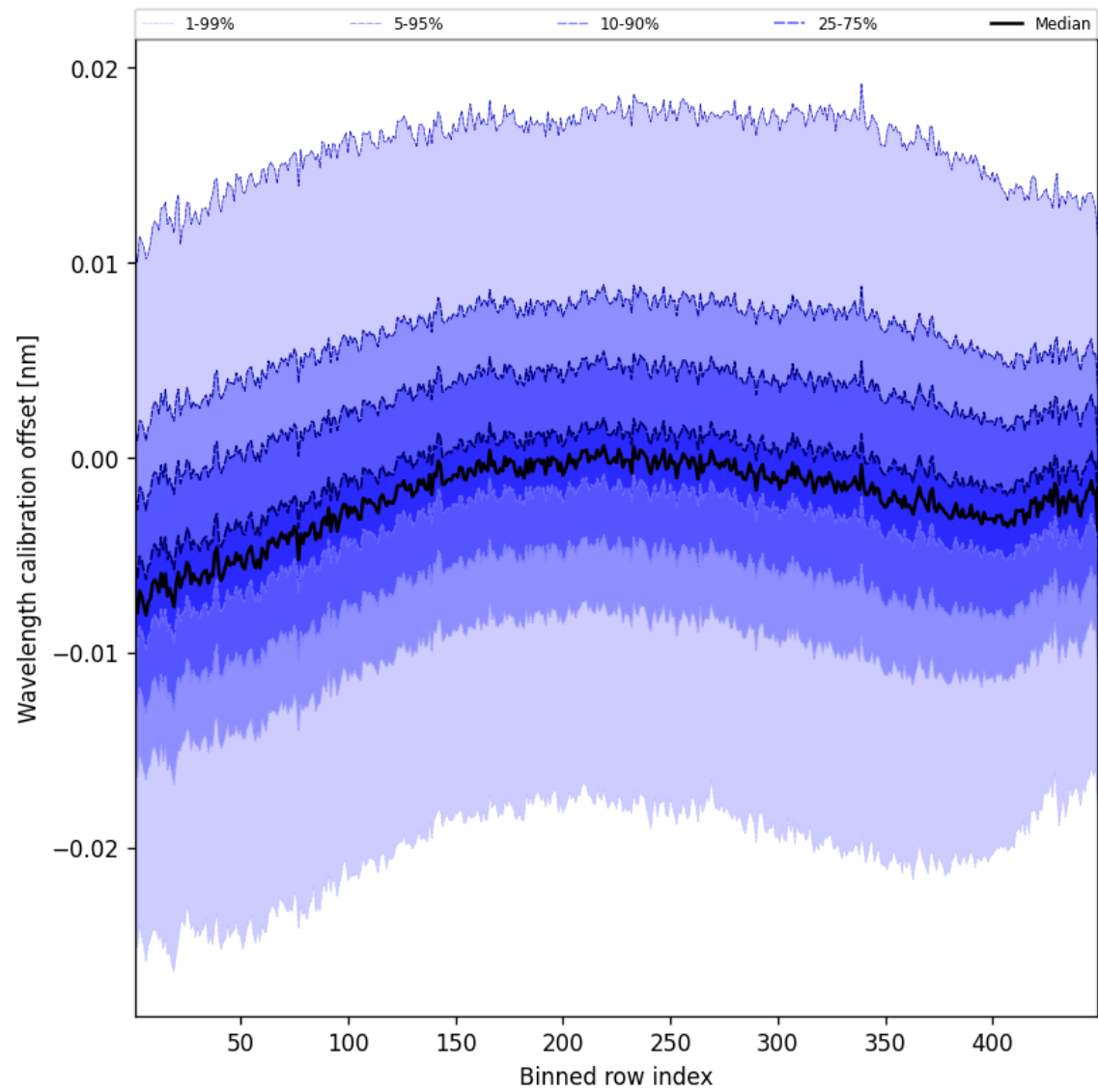
Figure 52: Along track statistics of “Wavelength calibration offset” for 2025-03-03 to 2025-03-05
