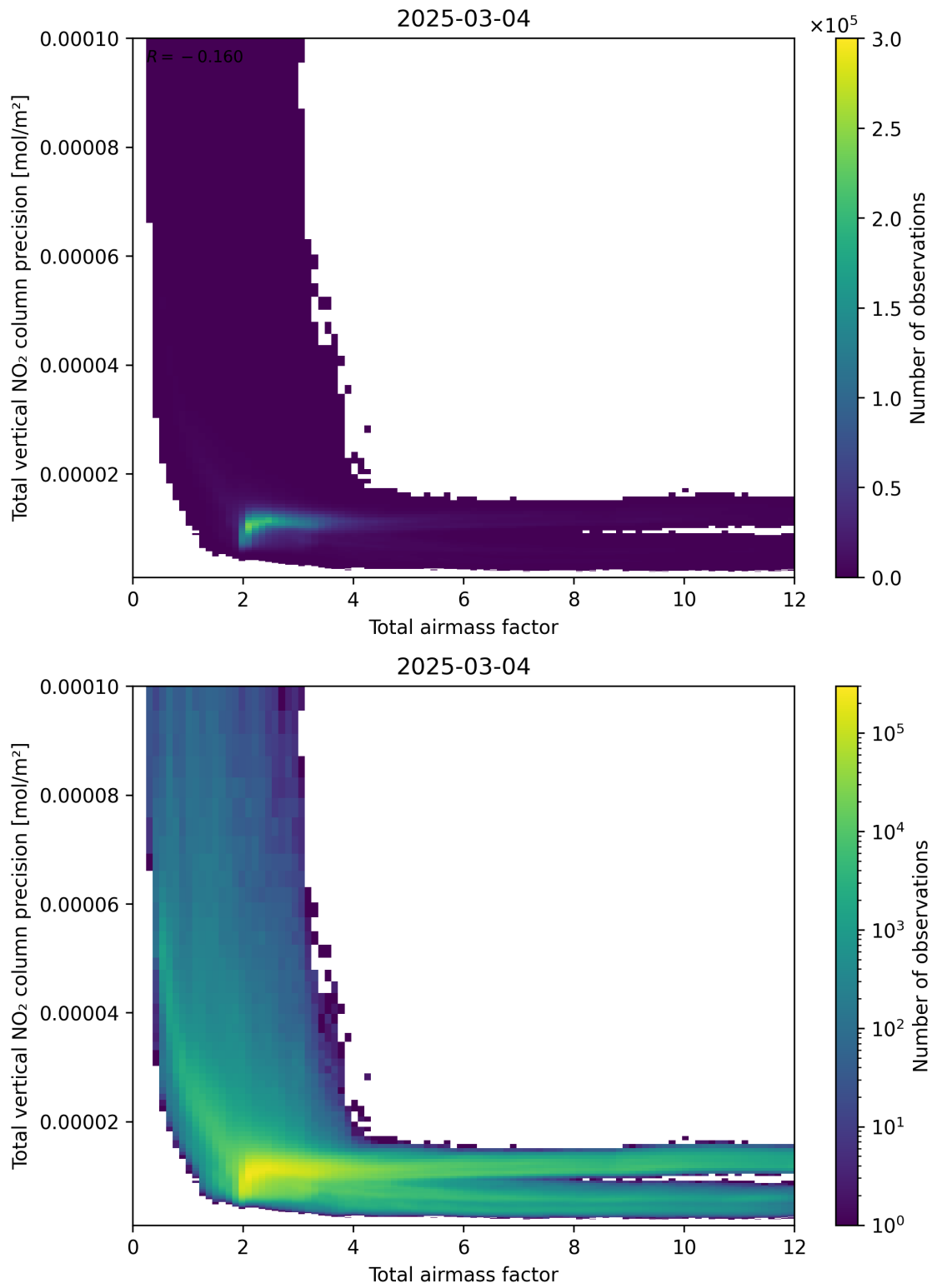
Figure 68: Scatter density plot of “Total airmass factor” against “Total vertical NO 2 column precision” for 2025-03-03 to 2025-03-05.
