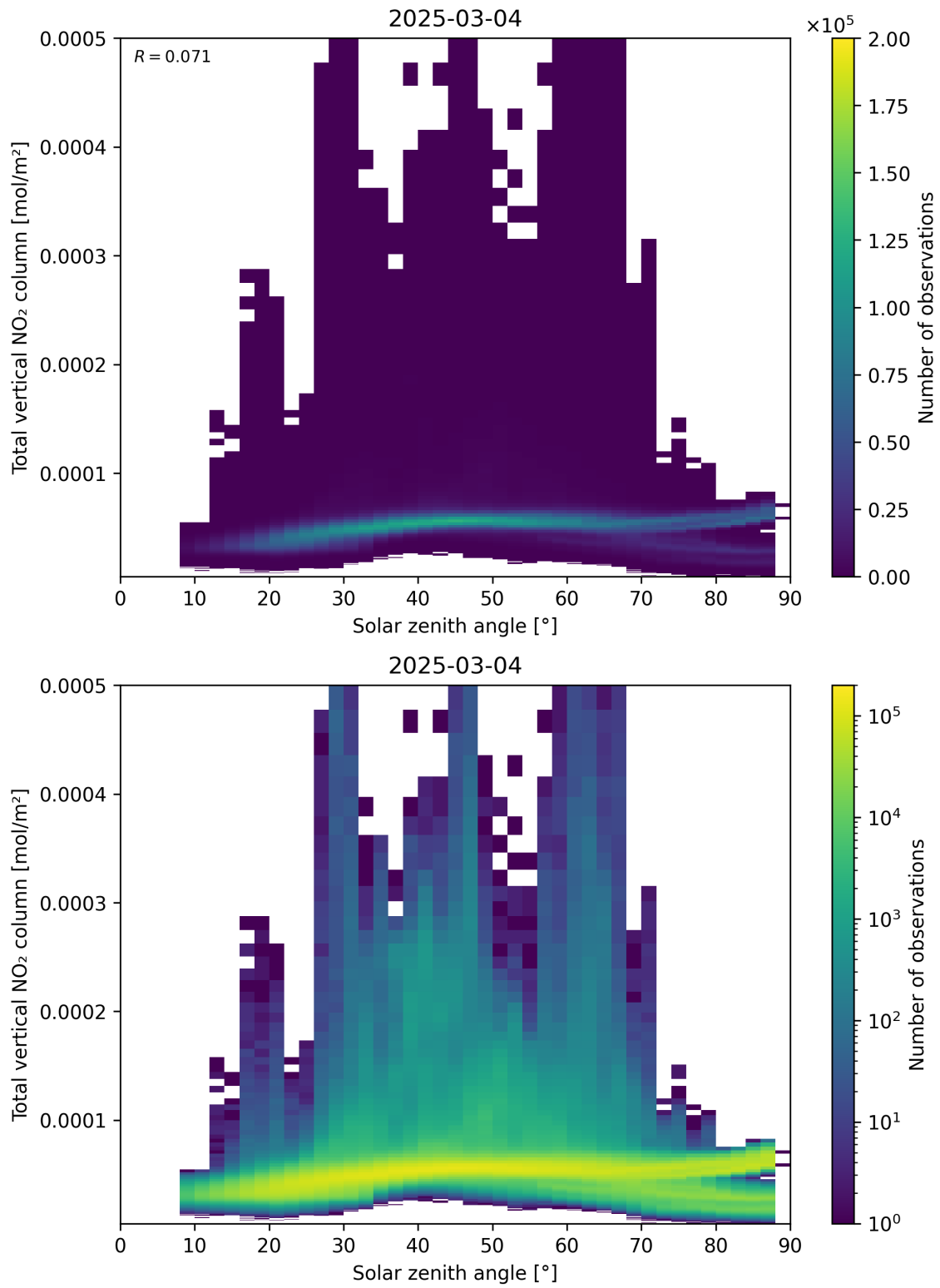
Figure 153: Scatter density plot of “Solar zenith angle” against “Total vertical NO 2 column” for 2025-03-03 to 2025-03-05.
