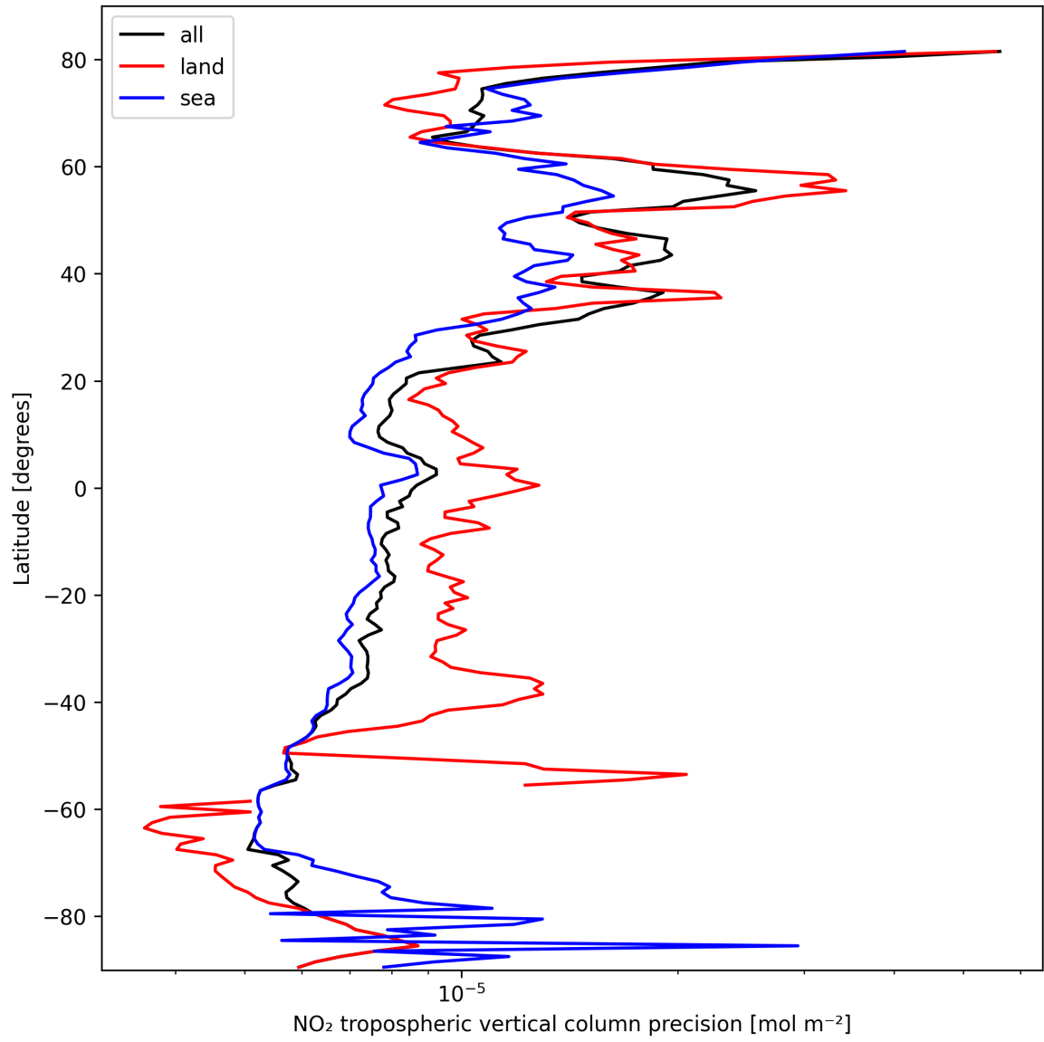
Figure 13: Zonal average of “NO 2 tropospheric vertical column precision” for 2025-03-03 to 2025-03-05.
