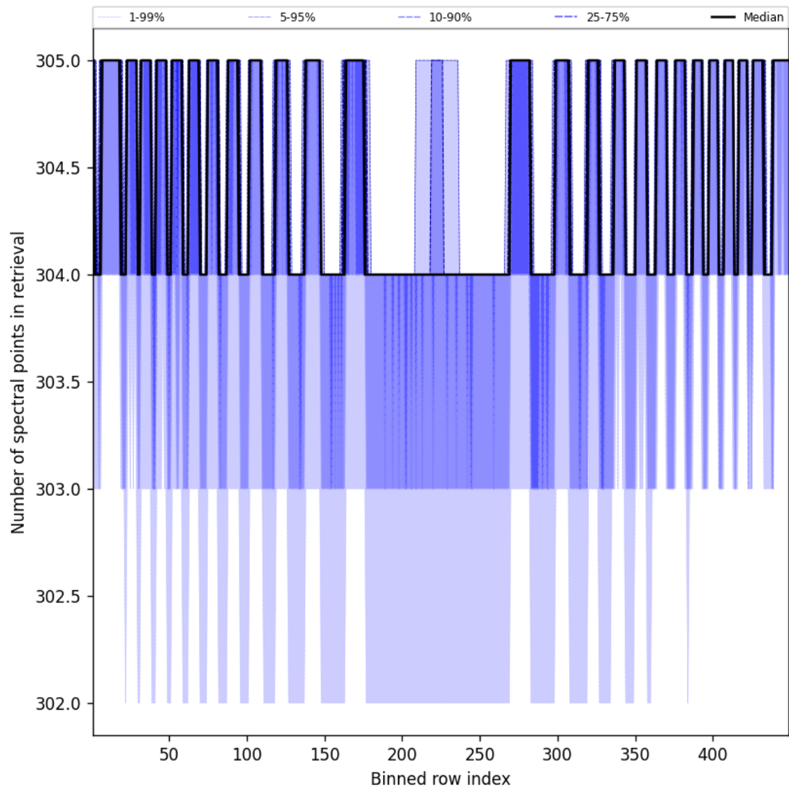
Figure 50: Along track statistics of “Number of spectral points in retrieval” for 2025-03-03 to 2025-03-05
