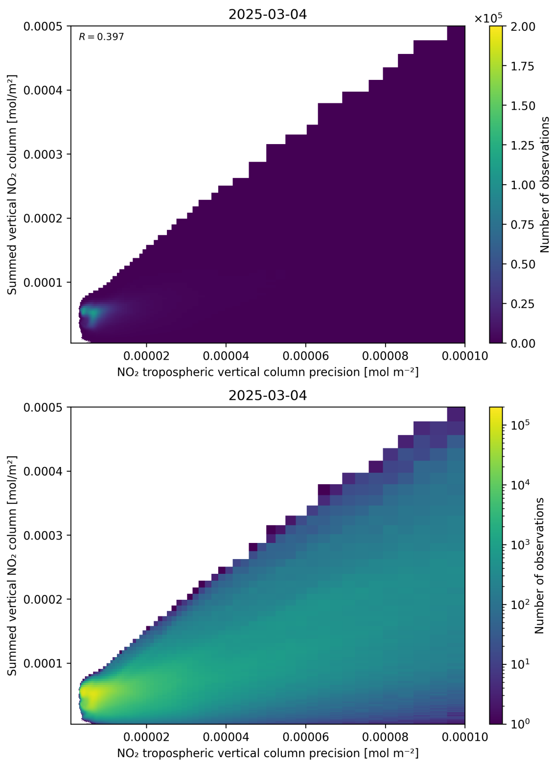
Figure 136: Scatter density plot of “NO 2 tropospheric vertical column precision” against “Summed vertical NO 2 column” for 2025-03-03 to 2025-03-05.
