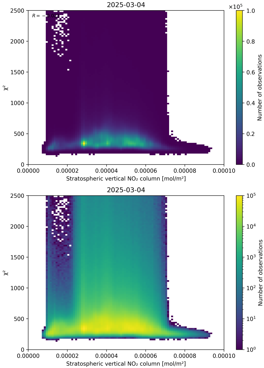
Figure 97: Scatter density plot of “Stratospheric vertical NO 2 column” against “ \chi^2 ” for 2025-03-03 to 2025-03-05.
