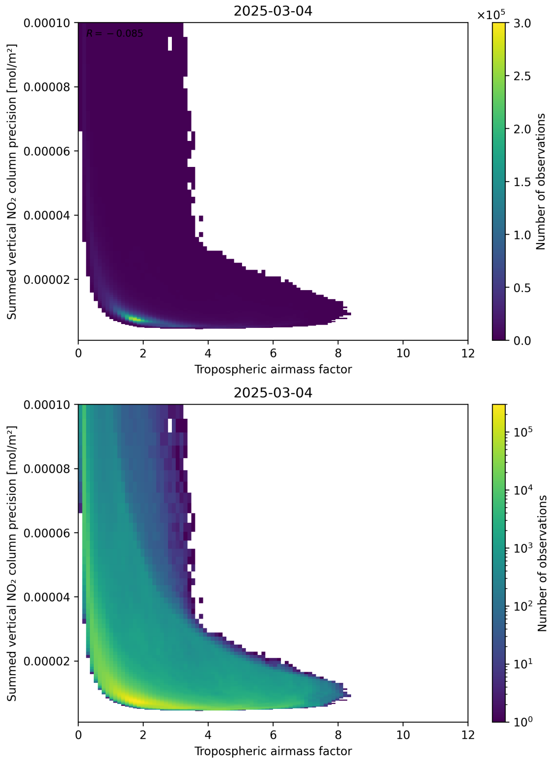
Figure 76: Scatter density plot of “Tropospheric air mass factor” against “Summed vertical NO 2 column precision” for 2025-03-03 to 2025-03-05.
