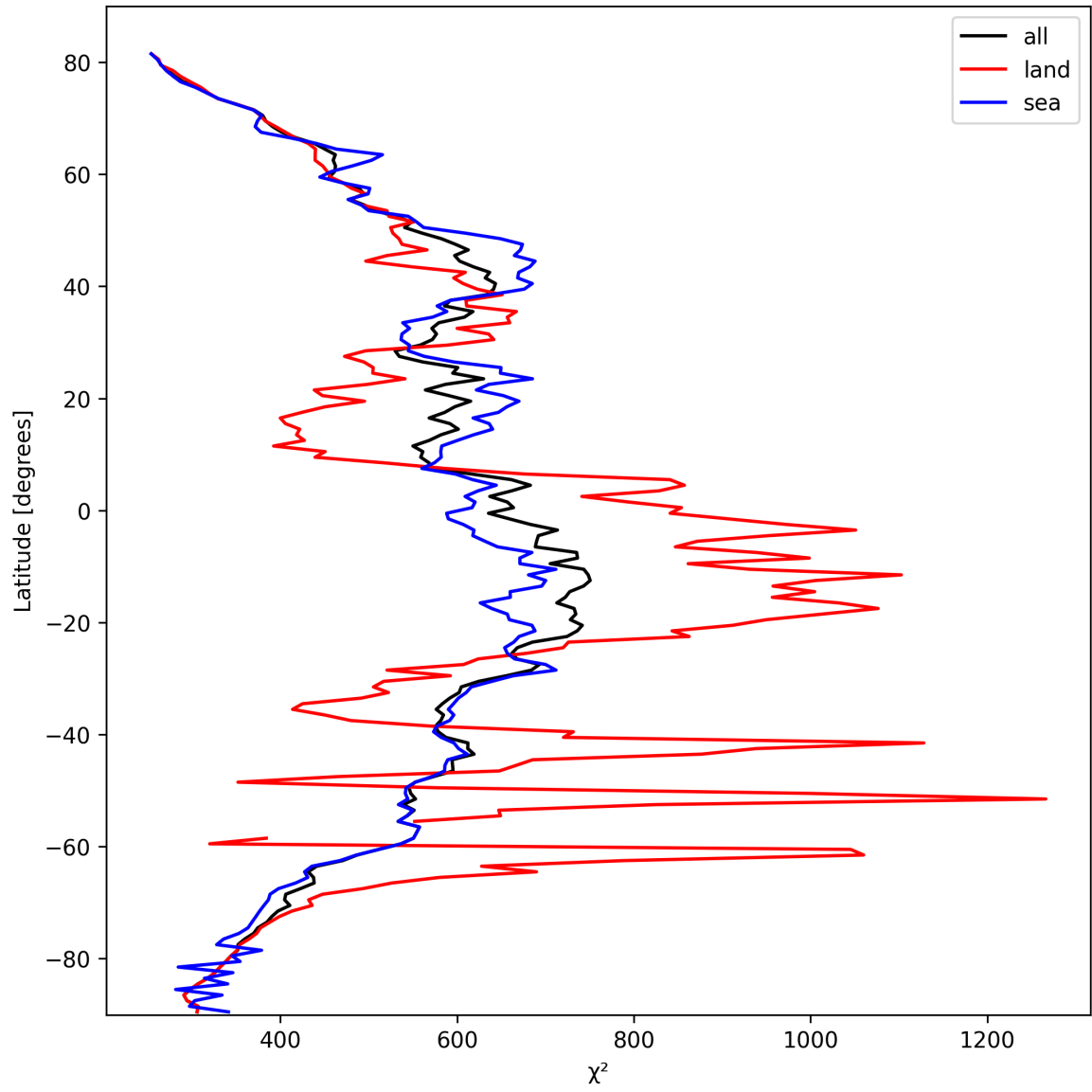
Figure 25: Zonal average of “ \chi^2 ” for 2025-03-03 to 2025-03-05.
