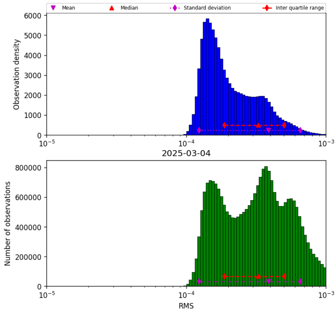
Figure 43: Histogram of “RMS” for 2025-03-03 to 2025-03-05
