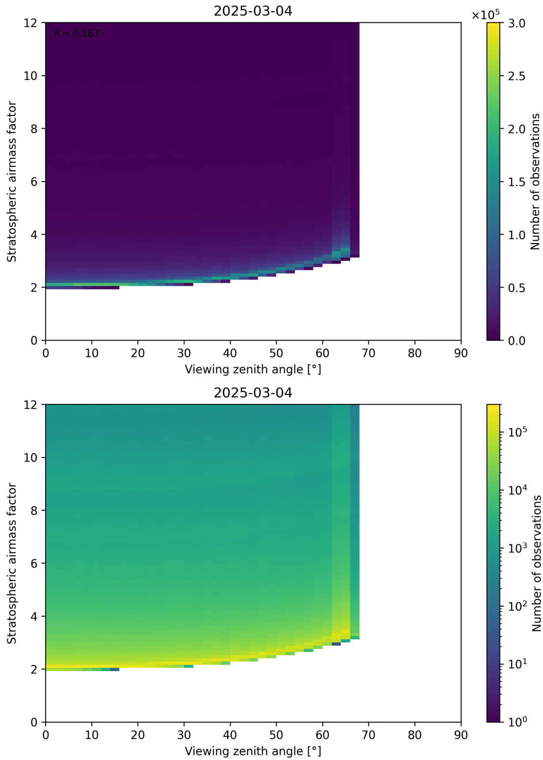
Figure 159: Scatter density plot of “Viewing zenith angle” against “Stratospheric airmass factor” for 2025-03-03 to 2025-03-05.
