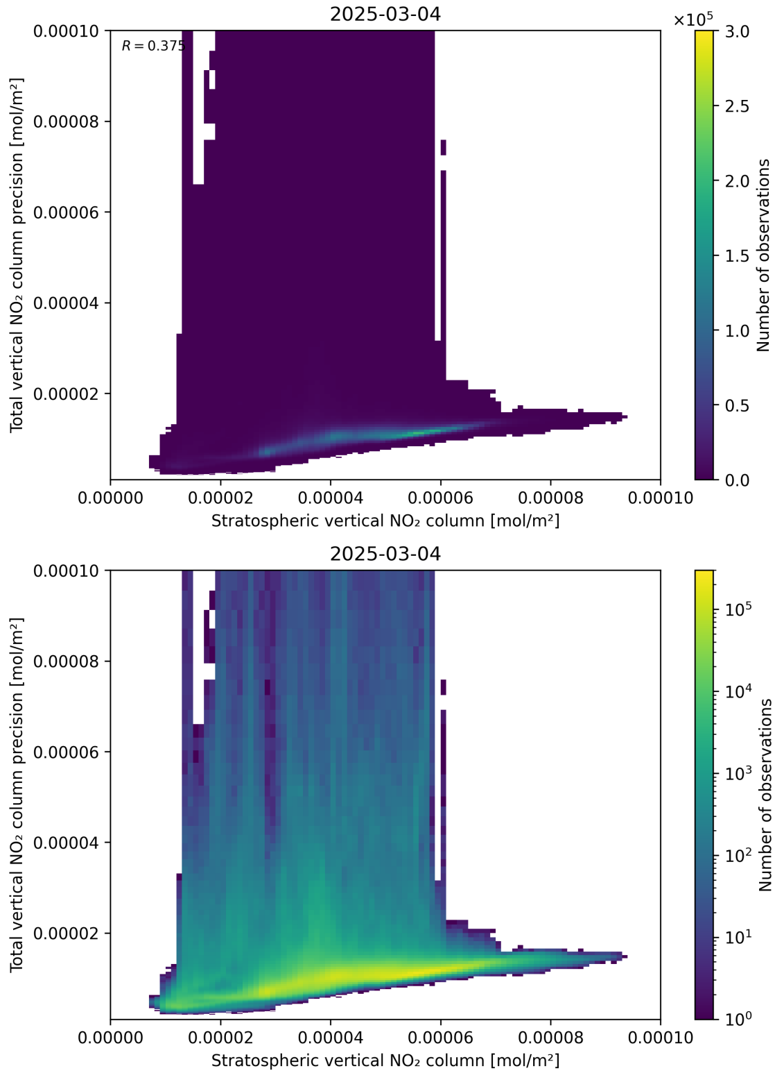
Figure 101: Scatter density plot of “Stratospheric vertical NO 2 column” against “Total vertical NO 2 column precision” for 2025-03-03 to 2025-03-05.
