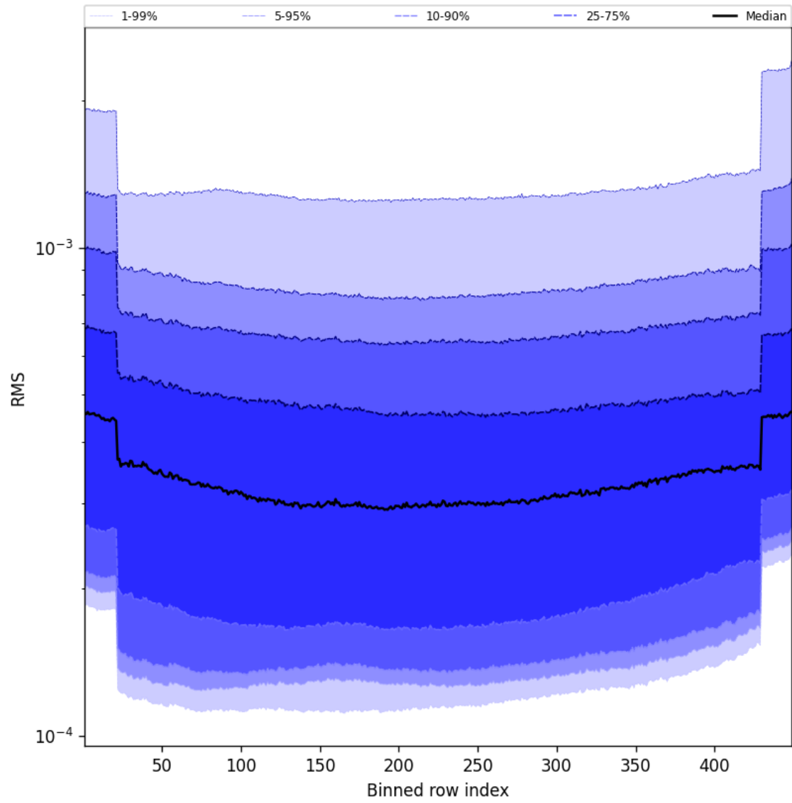
Figure 60: Along track statistics of “RMS” for 2025-03-03 to 2025-03-05
