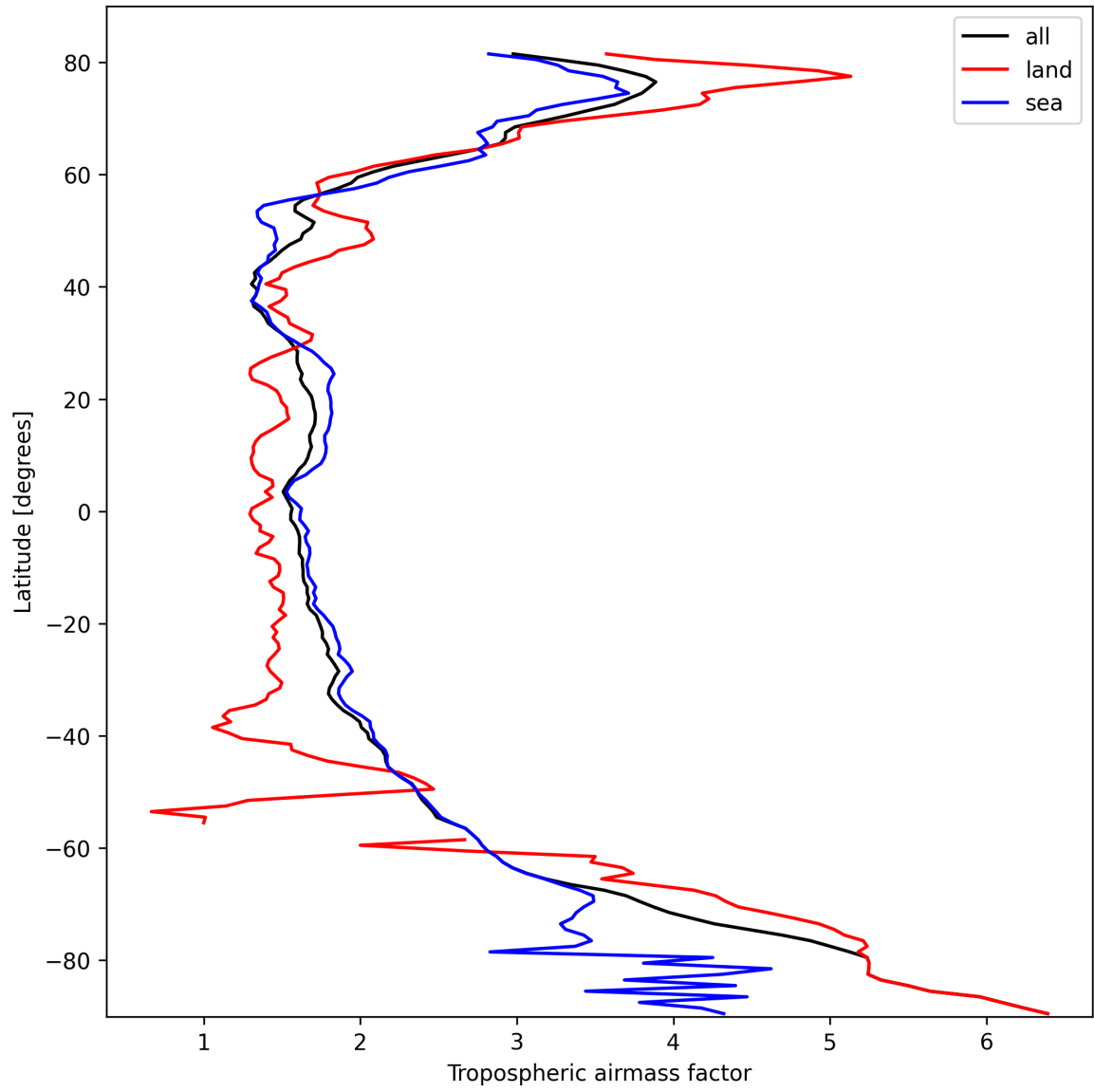
Figure 14: Zonal average of “Tropospheric airmass factor” for 2025-03-03 to 2025-03-05.
