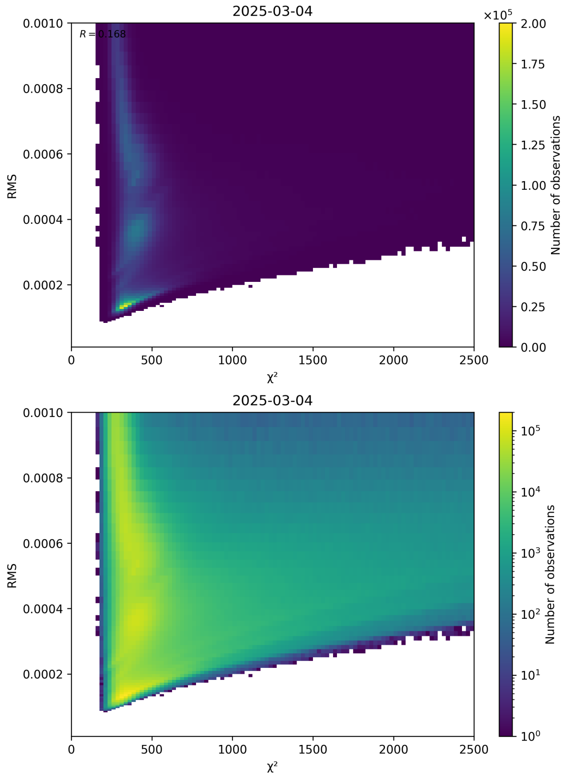
Figure 82: Scatter density plot of “ \chi^2 ” against “RMS” for 2025-03-03 to 2025-03-05.
