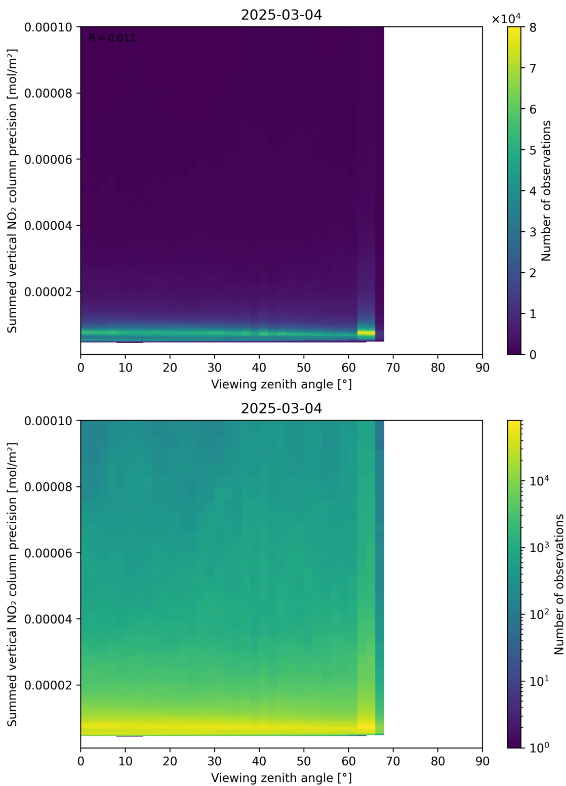
Figure 166: Scatter density plot of “Viewing zenith angle” against “Summed vertical NO 2 column precision” for 2025-03-03 to 2025-03-05.
