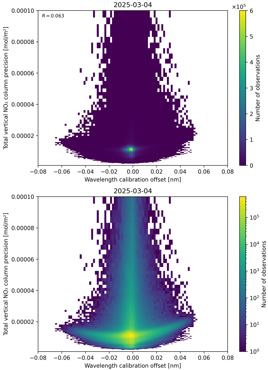
Figure 180: Scatter density plot of “Wavelength calibration offset” against “Total vertical NO 2 column precision” for 2025-03-03 to 2025-03-05.
