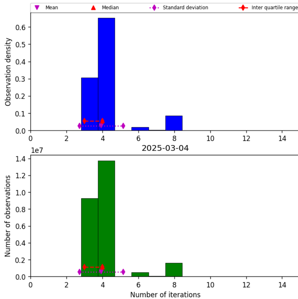
Figure 34: Histogram of “Number of iterations” for 2025-03-03 to 2025-03-05
