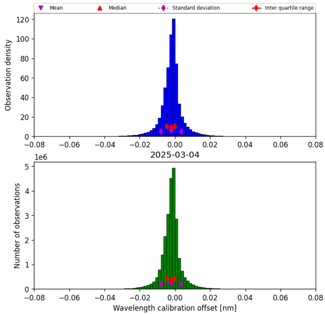
Figure 35: Histogram of “Wavelength calibration offset” for 2025-03-03 to 2025-03-05
