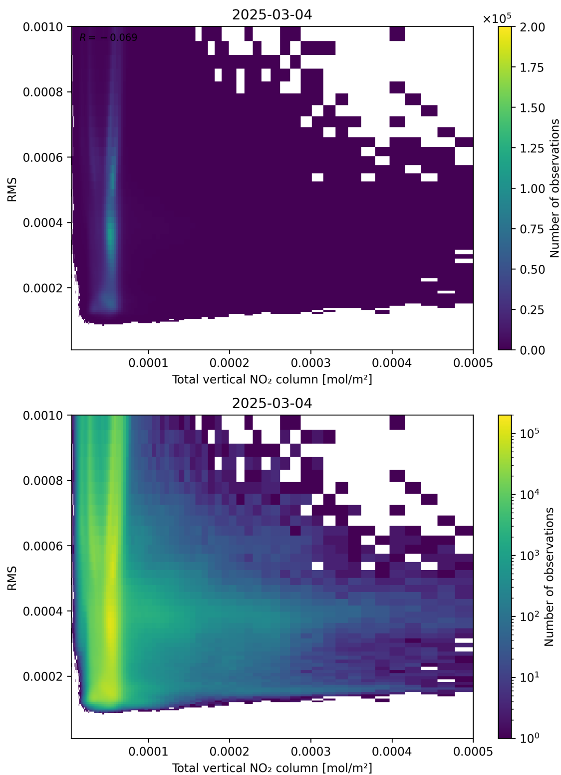
Figure 120: Scatter density plot of “Total vertical NO 2 column” against “RMS” for 2025-03-03 to 2025-03-05.
