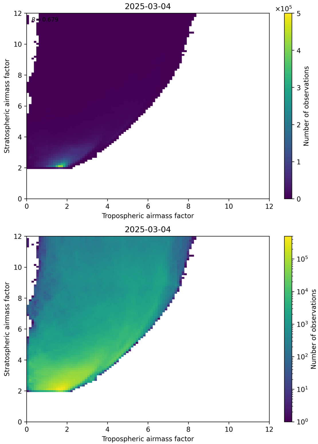
Figure 71: Scatter density plot of “Tropospheric airmass factor” against “Stratospheric airmass factor” for 2025-03-03 to 2025-03-05.
