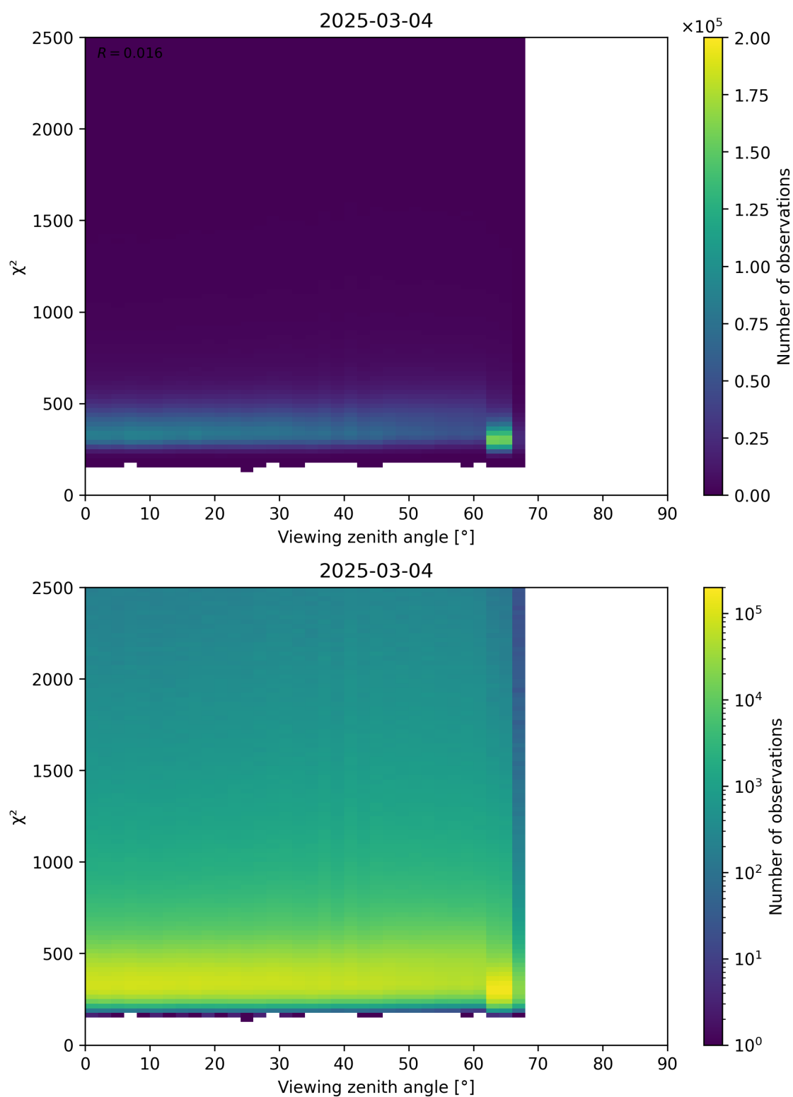
Figure 162: Scatter density plot of “Viewing zenith angle” against “ \chi^2 ” for 2025-03-03 to 2025-03-05.
