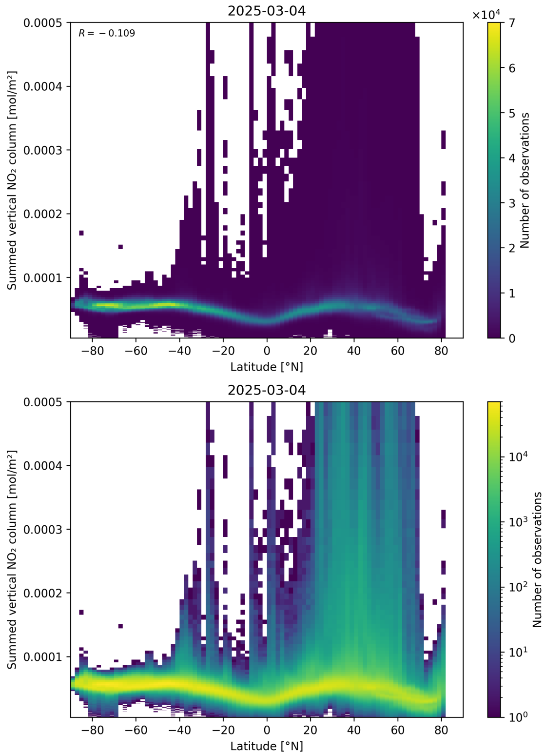
Figure 88: Scatter density plot of “Latitude” against “Summed vertical NO 2 column” for 2025-03-03 to 2025-03-05.
