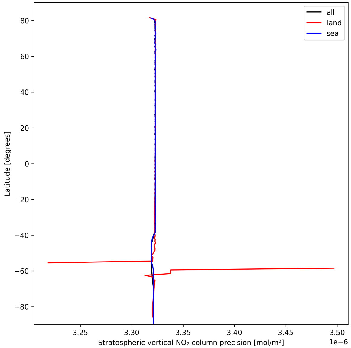
Figure 20: Zonal average of “Stratospheric vertical NO 2 column precision” for 2025-03-03 to 2025-03-05.
