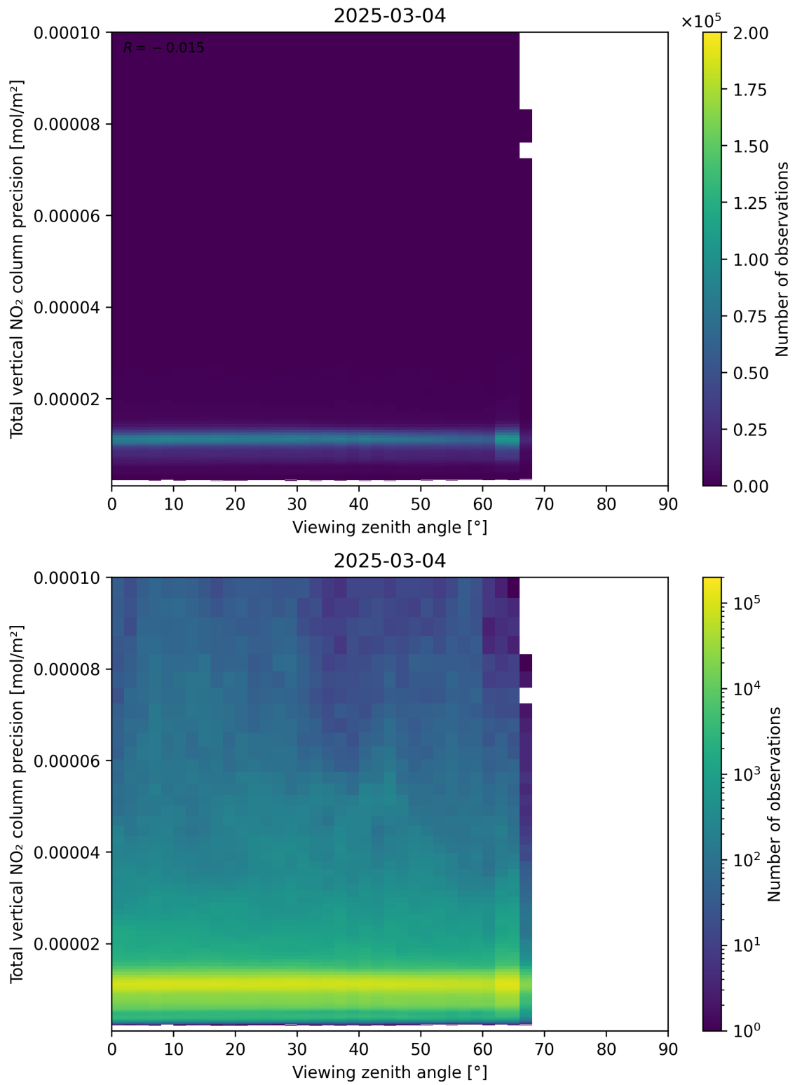
Figure 168: Scatter density plot of “Viewing zenith angle” against “Total vertical NO 2 column precision” for 2025-03-03 to 2025-03-05.
