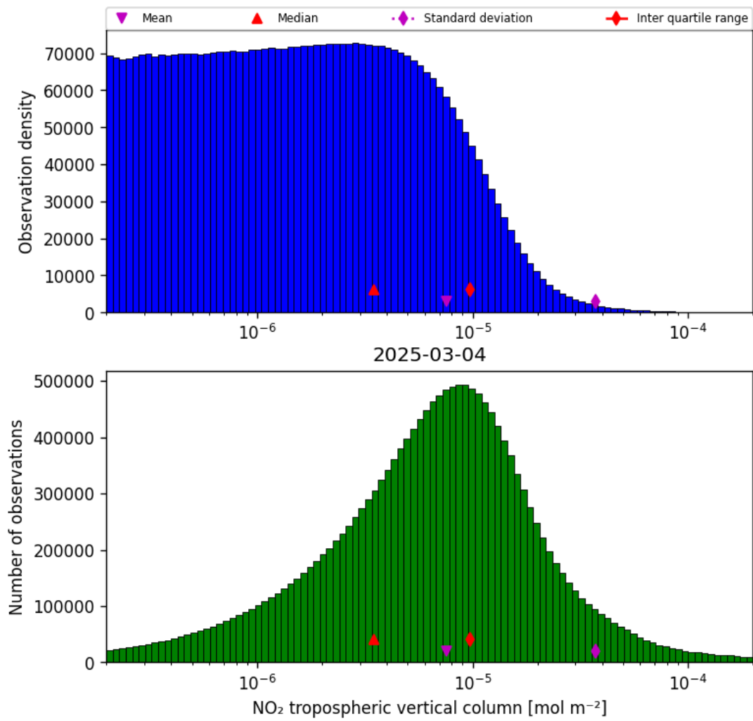
Figure 29: Histogram of “NO 2 tropospheric vertical column” for 2025-03-03 to 2025-03-05
