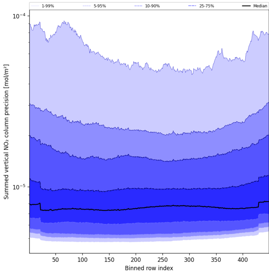
Figure 58: Along track statistics of “Summed vertical NO 2 column precision” for 2025-03-03 to 2025-03-05
