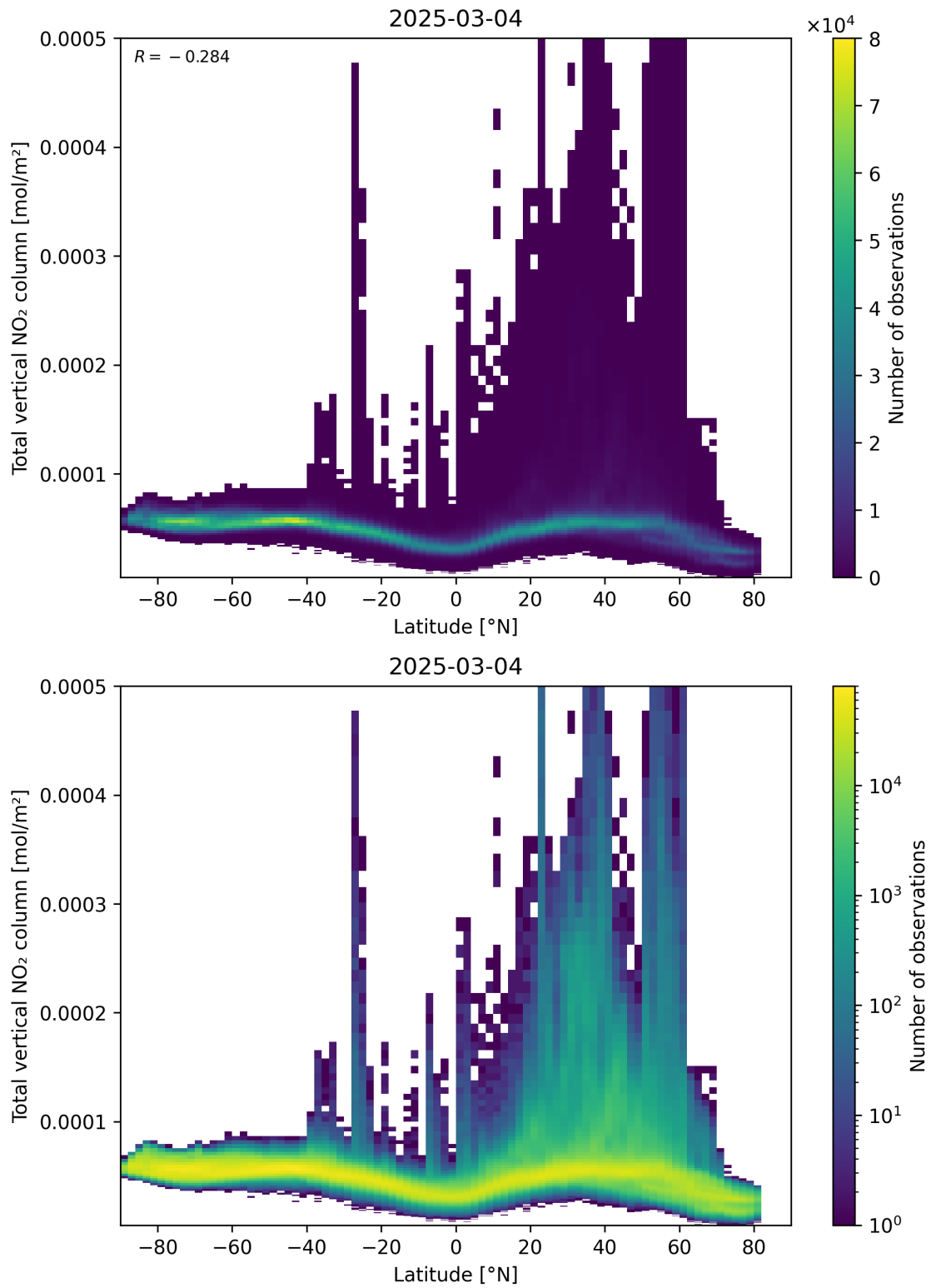
Figure 90: Scatter density plot of “Latitude” against “Total vertical NO 2 column” for 2025-03-03 to 2025-03-05.
