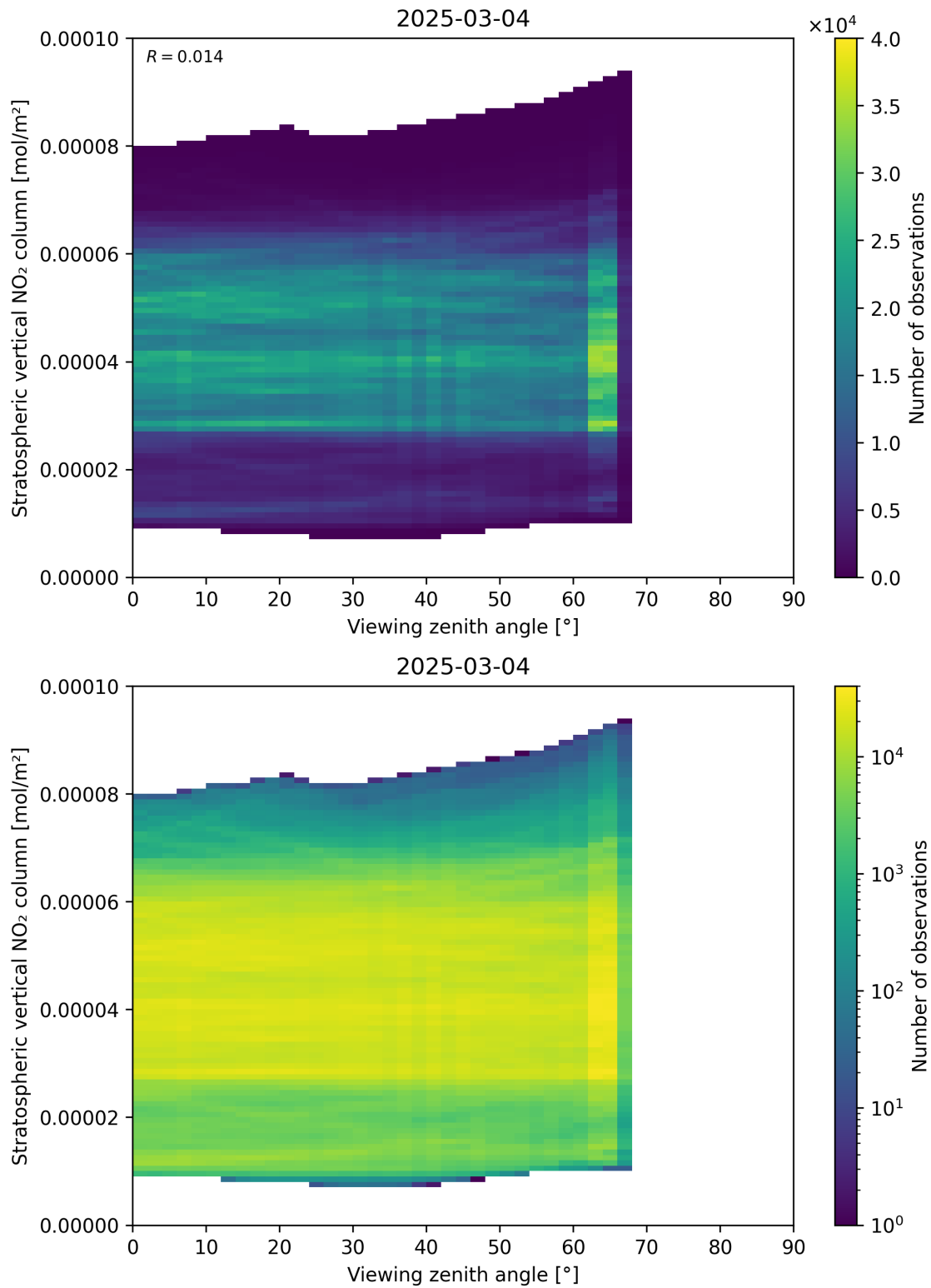
Figure 164: Scatter density plot of “Viewing zenith angle” against “Stratospheric vertical NO 2 column” for 2025-03-03 to 2025-03-05.
