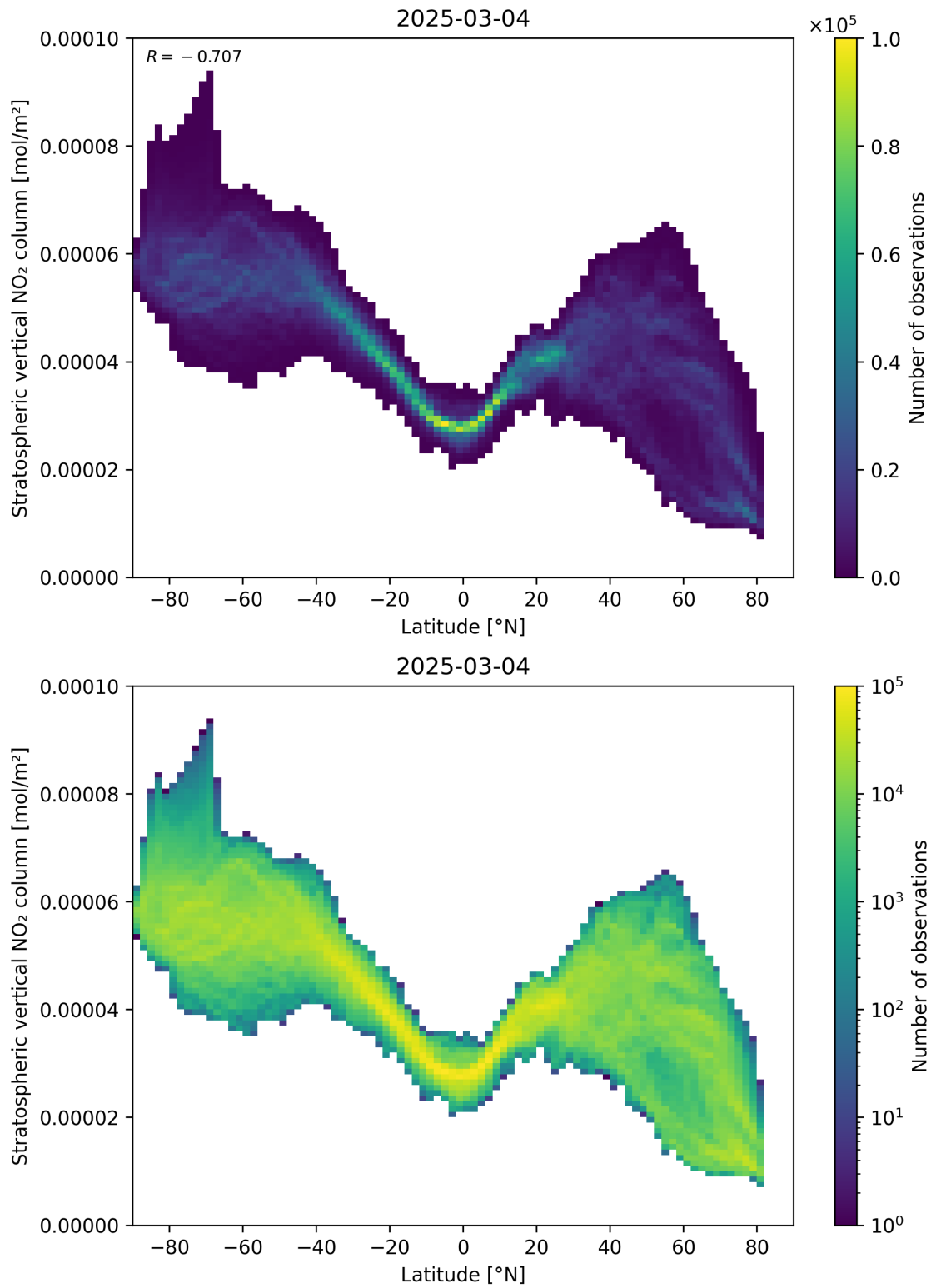
Figure 87: Scatter density plot of “Latitude” against “Stratospheric vertical NO 2 column” for 2025-03-03 to 2025-03-05.
