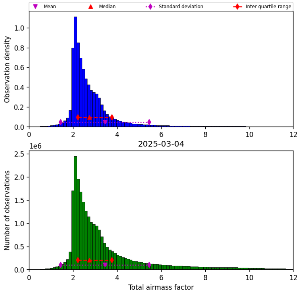
Figure 32: Histogram of “Total airmass factor” for 2025-03-03 to 2025-03-05
