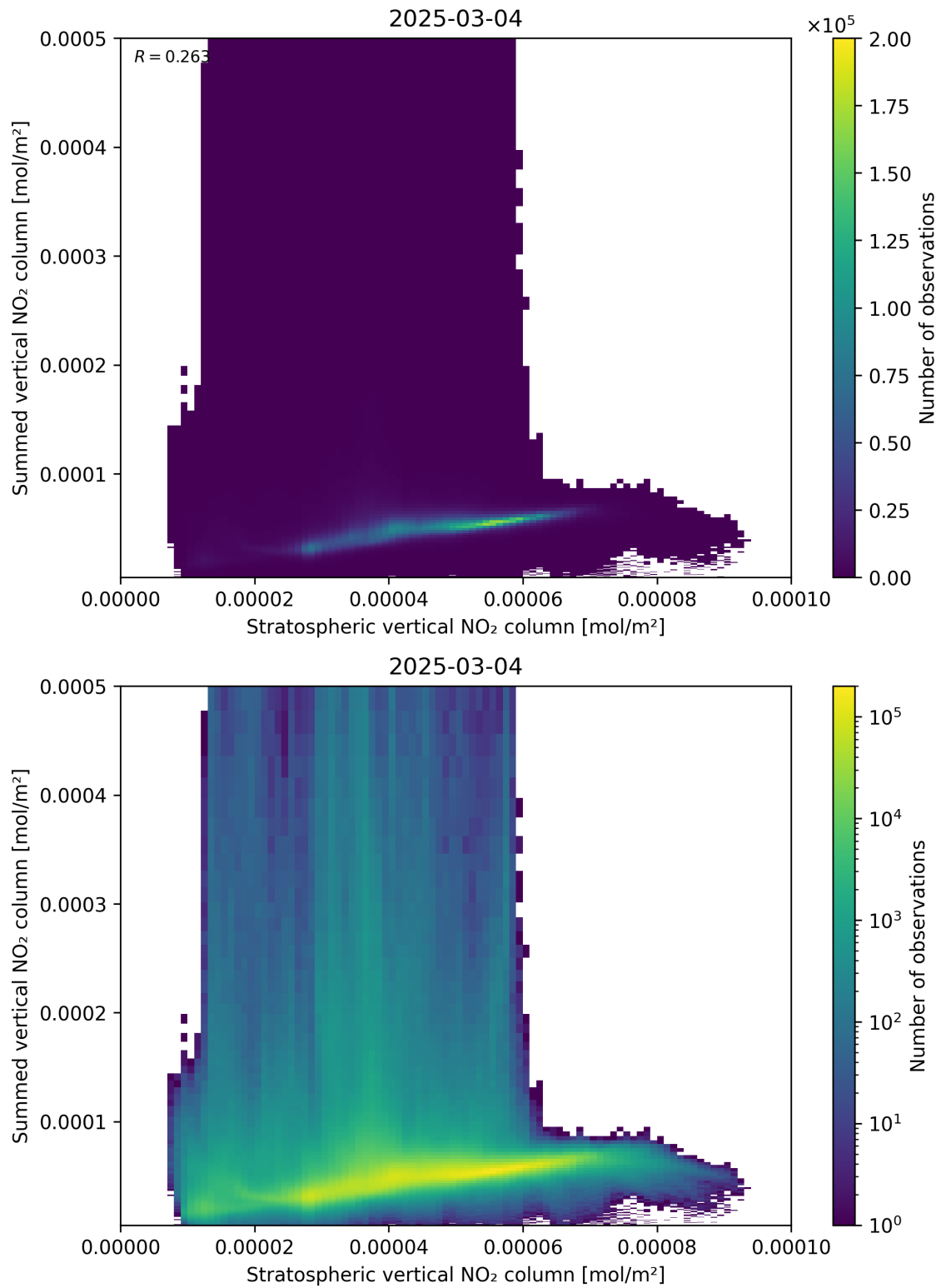
Figure 98: Scatter density plot of “Stratospheric vertical NO 2 column” against “Summed vertical NO 2 column” for 2025-03-03 to 2025-03-05.
