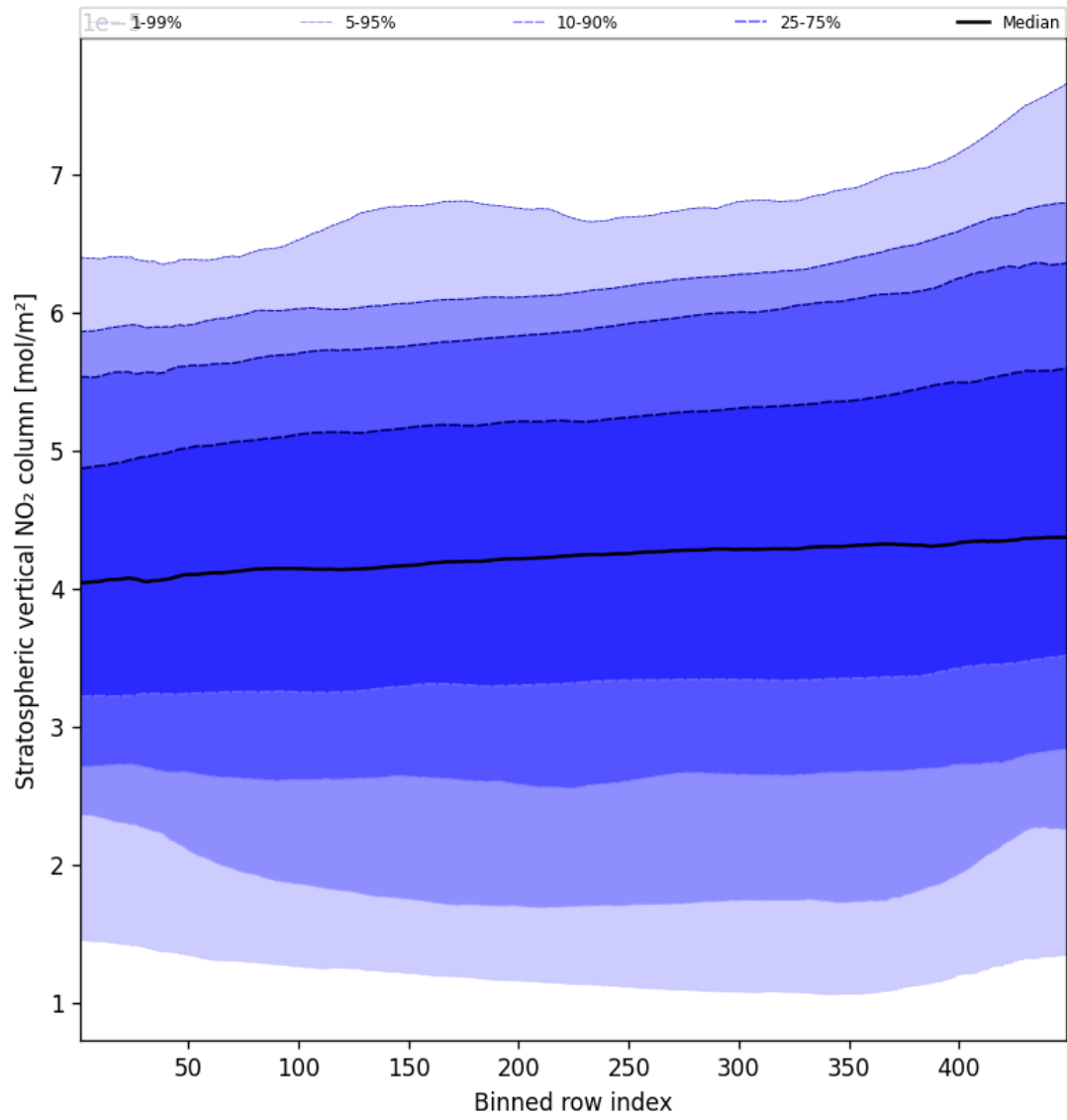
Figure 53: Along track statistics of “Stratospheric vertical NO 2 column” for 2025-03-03 to 2025-03-05
