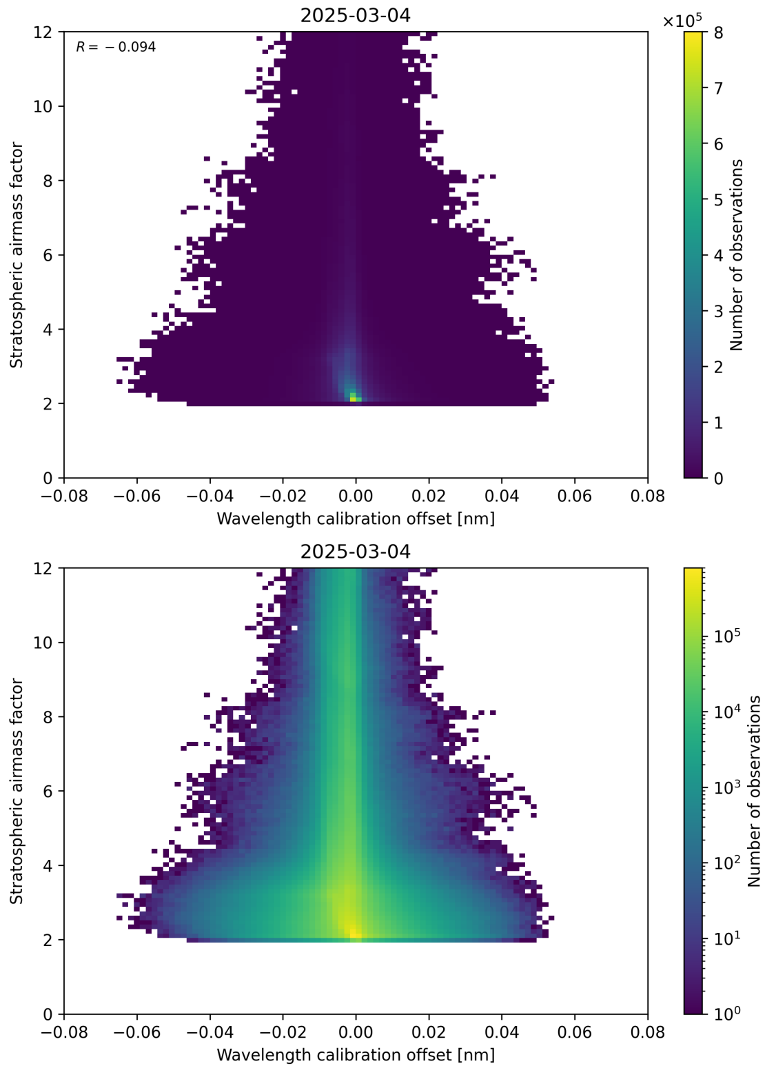
Figure 174: Scatter density plot of “Wavelength calibration offset” against “Stratospheric airmass factor” for 2025-03-03 to 2025-03-05.
