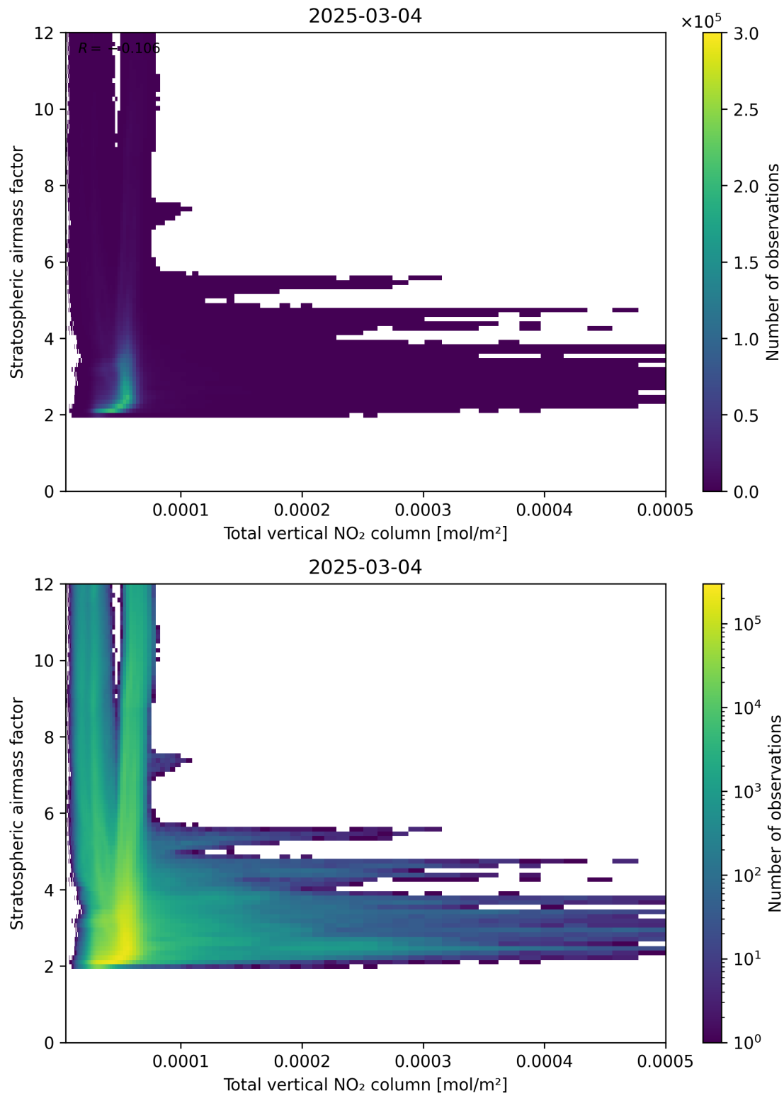
Figure 110: Scatter density plot of “Total vertical NO 2 column” against “Stratospheric airmass factor” for 2025-03-03 to 2025-03-05.
