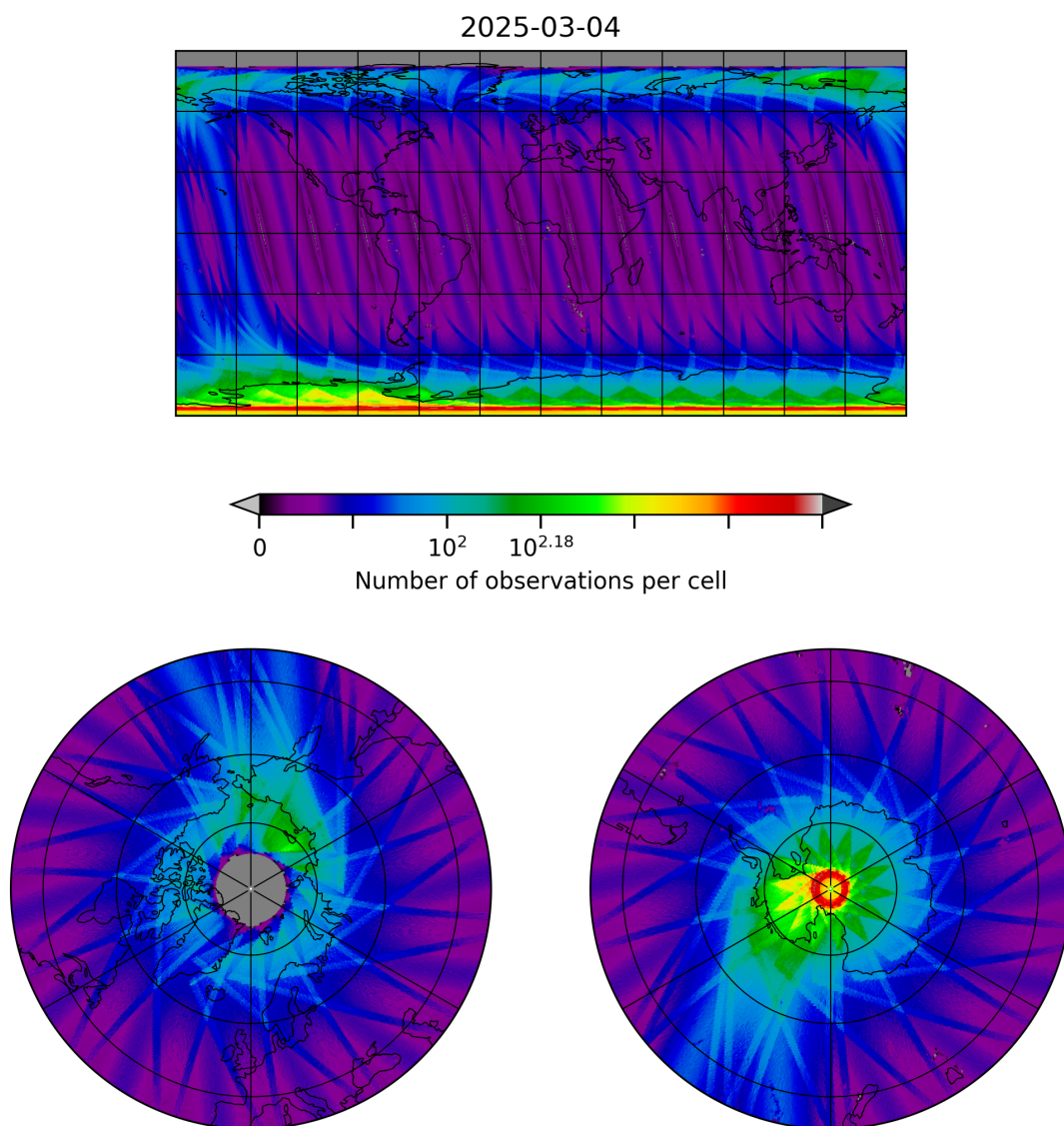
Figure 10: Map of the number of observations for 2025-03-03 to 2025-03-05
