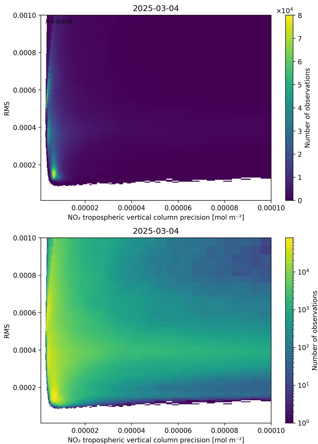
Figure 140: Scatter density plot of “NO 2 tropospheric vertical column precision” against “RMS” for 2025-03-03 to 2025-03-05.
