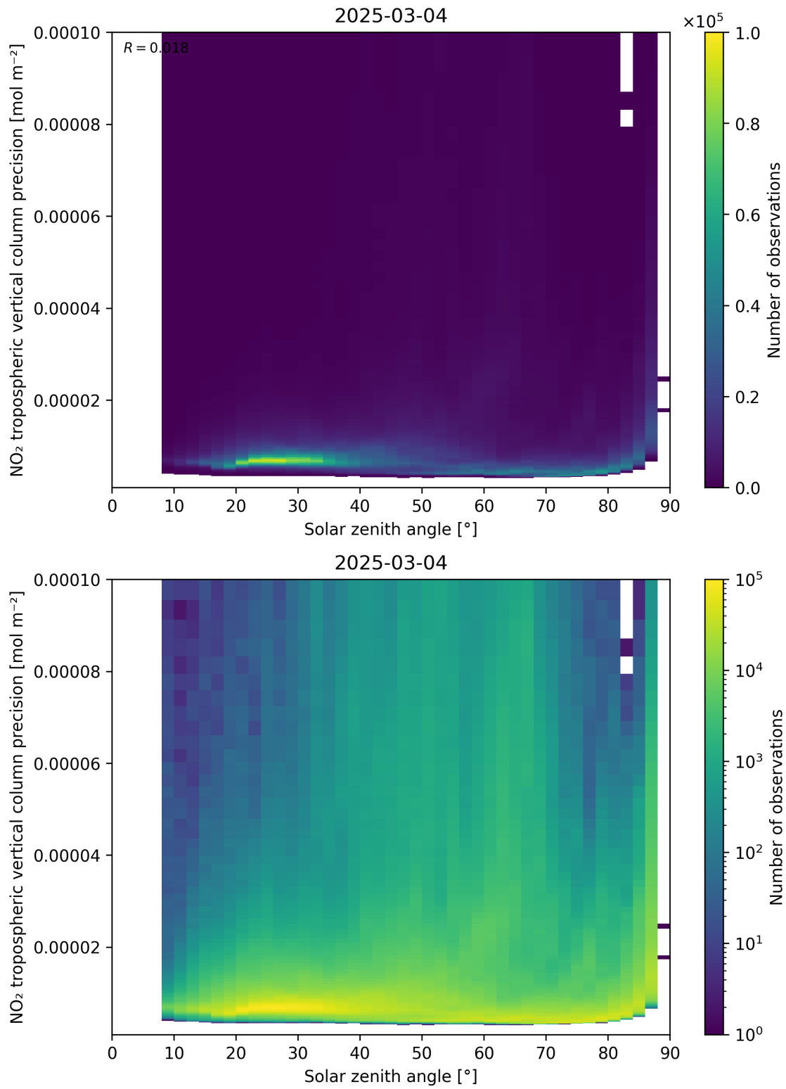
Figure 156: Scatter density plot of “Solar zenith angle” against “NO 2 tropospheric vertical column precision” for 2025-03-03 to 2025-03-05.
