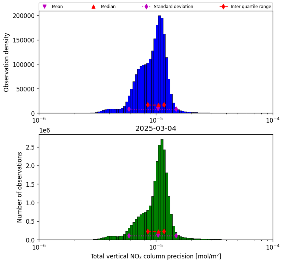
Figure 39: Histogram of “Total vertical NO 2 column precision” for 2025-03-03 to 2025-03-05
