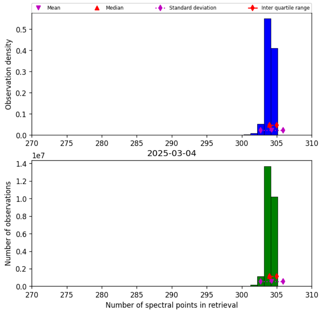
Figure 33: Histogram of “Number of spectral points in retrieval” for 2025-03-03 to 2025-03-05
