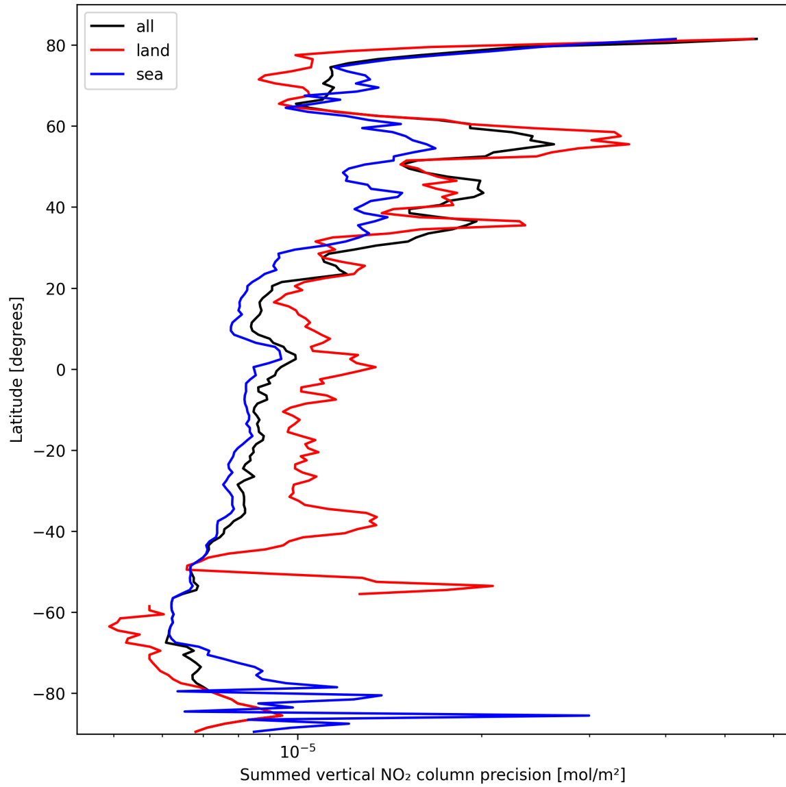
Figure 24: Zonal average of “Summed vertical NO 2 column precision” for 2025-03-03 to 2025-03-05.
