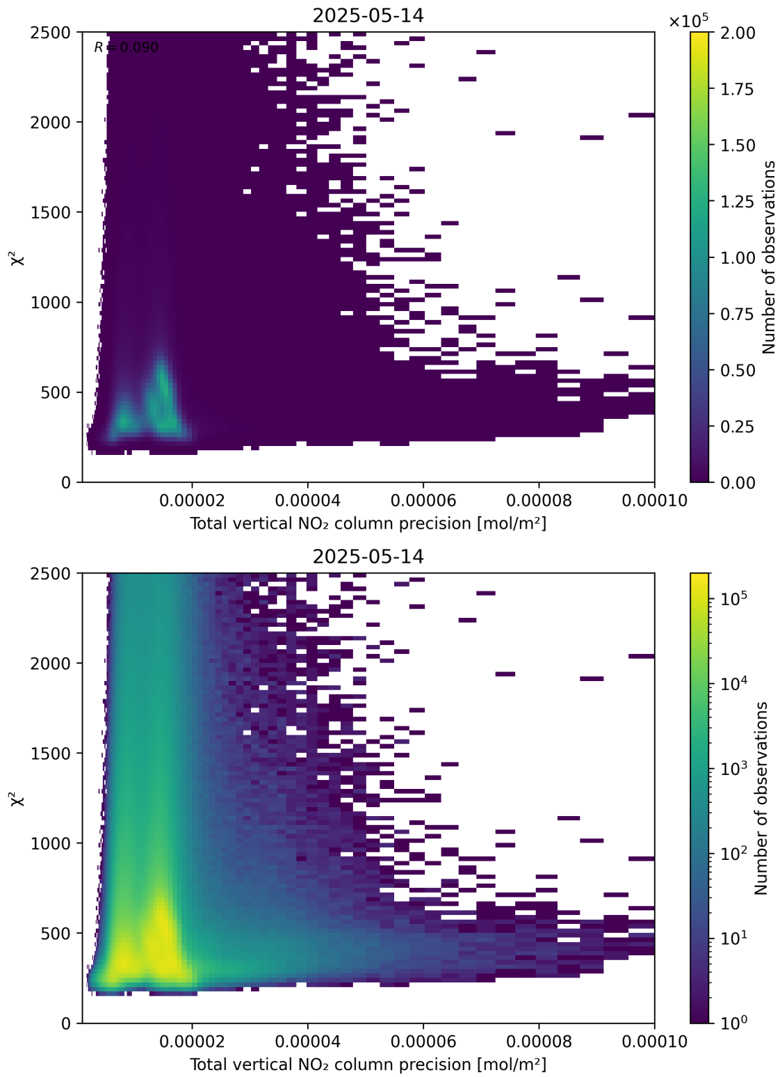
Figure 116: Scatter density plot of “Total vertical NO 2 column precision” against “ \chi^2 ” for 2025-05-13 to 2025-05-15.
