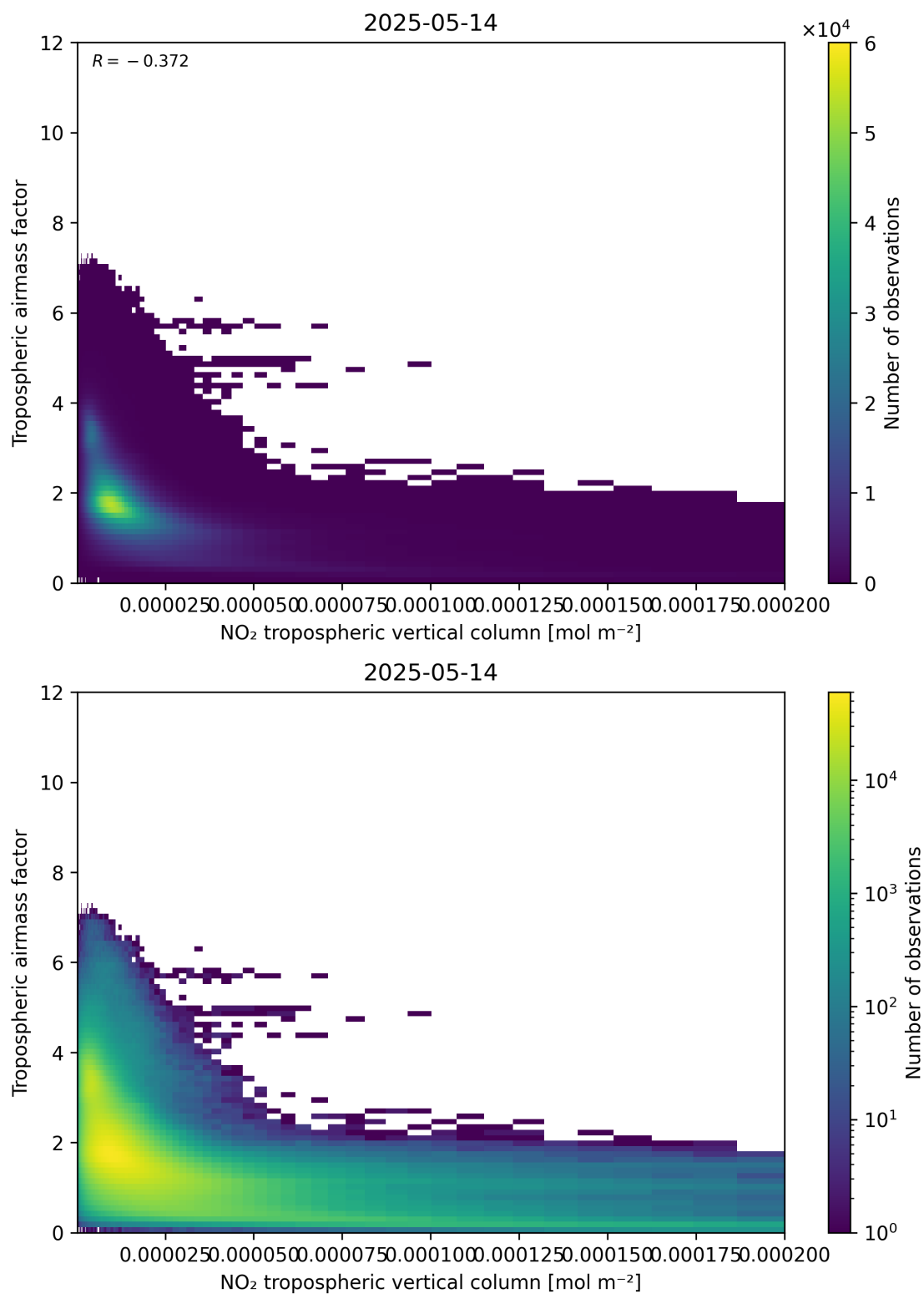
Figure 123: Scatter density plot of “NO 2 tropospheric vertical column” against “Tropospheric air mass factor” for 2025-05-13 to 2025-05-15.
