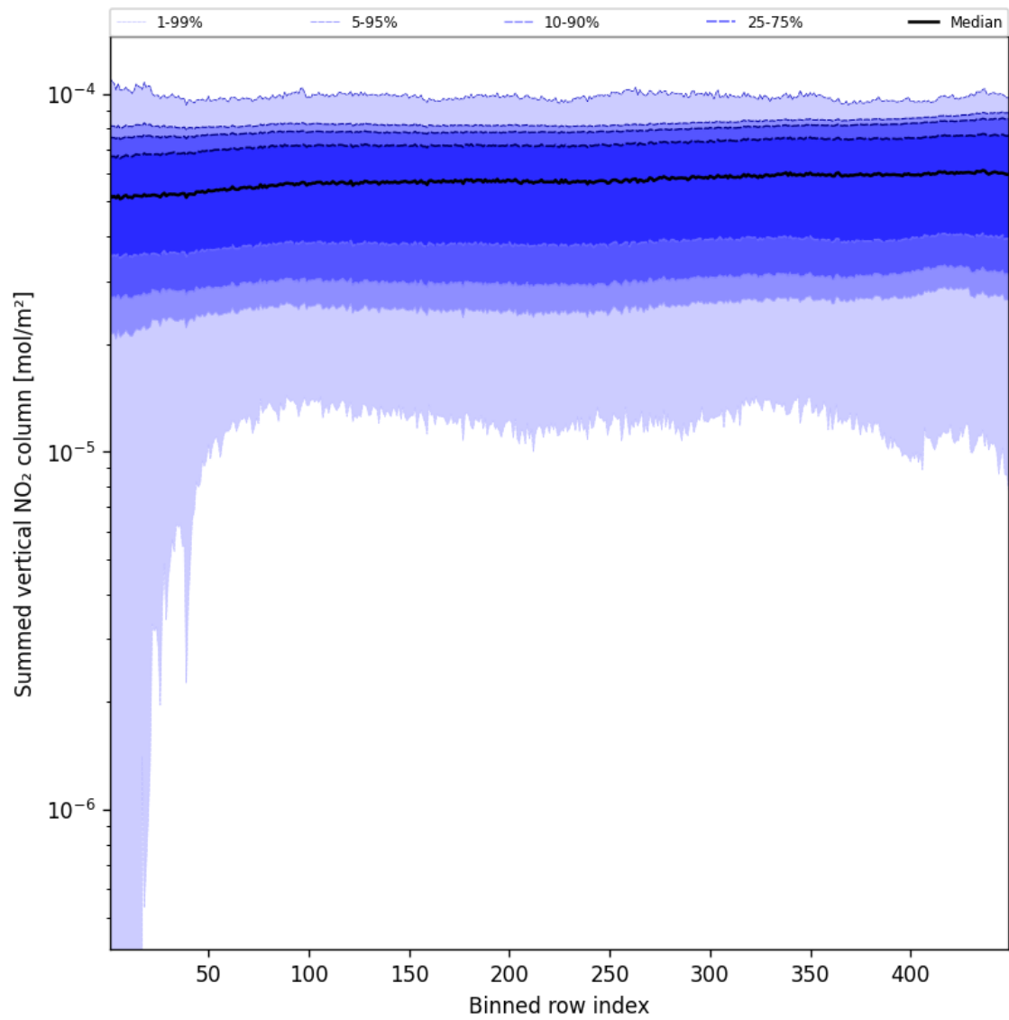
Figure 57: Along track statistics of “Summed vertical NO 2 column” for 2025-05-13 to 2025-05-15
