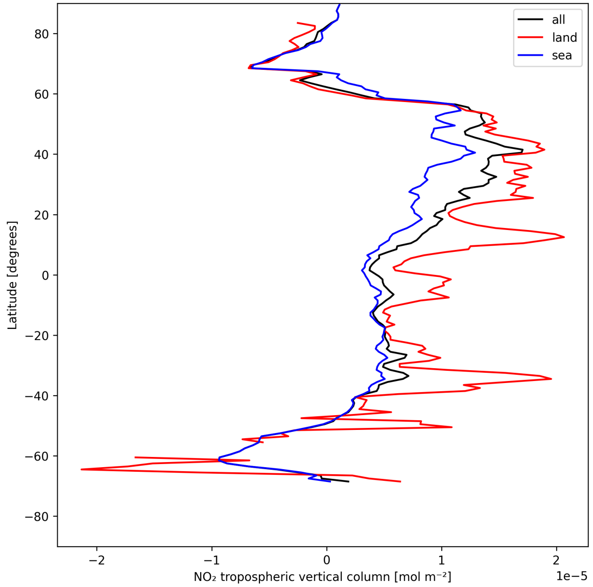
Figure 12: Zonal average of “NO 2 tropospheric vertical column” for 2025-05-13 to 2025-05-15.
