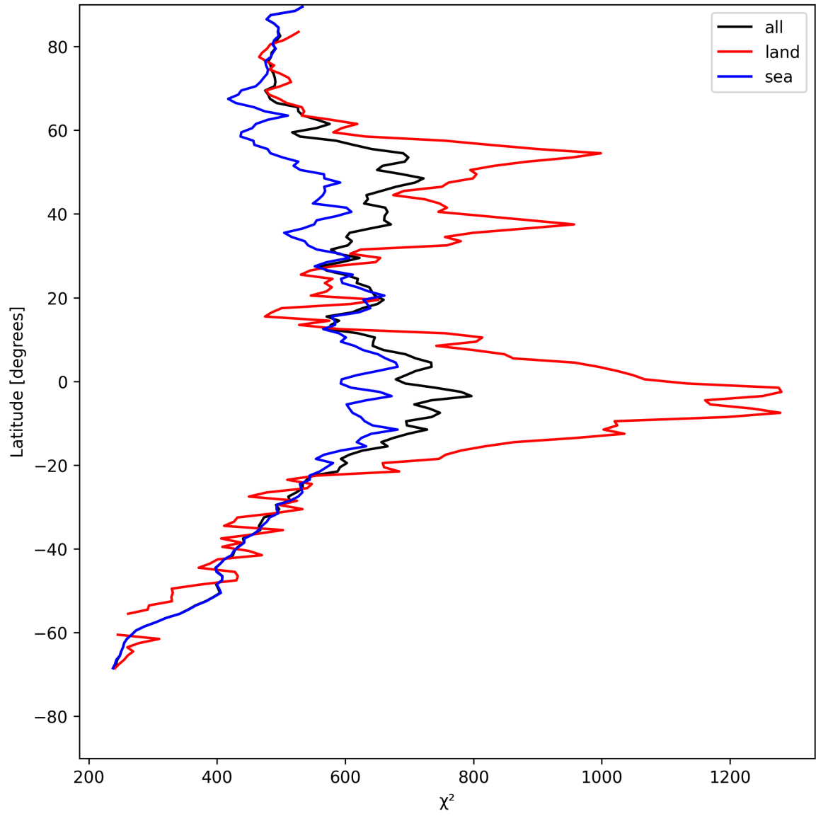
Figure 25: Zonal average of “ \chi^2 ” for 2025-05-13 to 2025-05-15.
