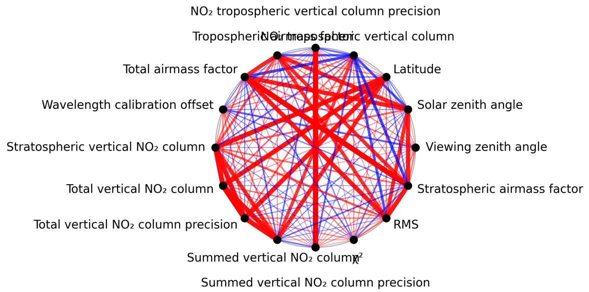
Figure 1: Map of correlation graph for 2025-05-13 to 2025-05-15.
