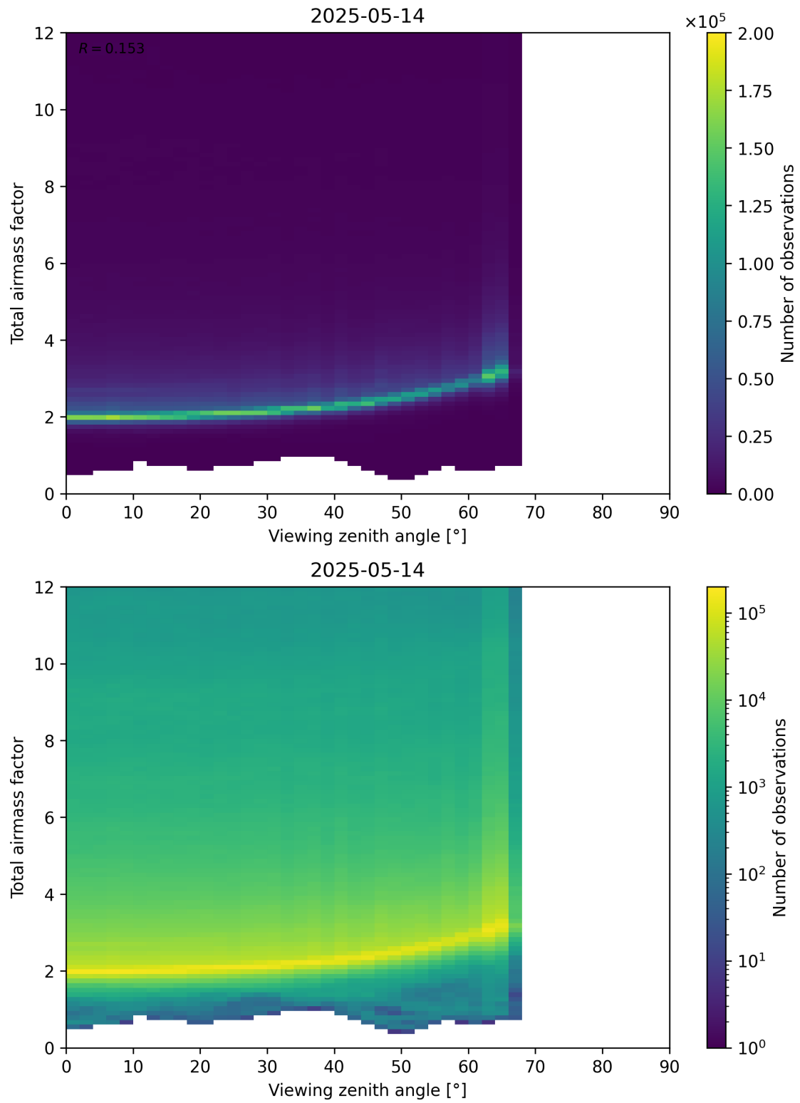
Figure 160: Scatter density plot of “Viewing zenith angle” against “Total airmass factor” for 2025-05-13 to 2025-05-15.
