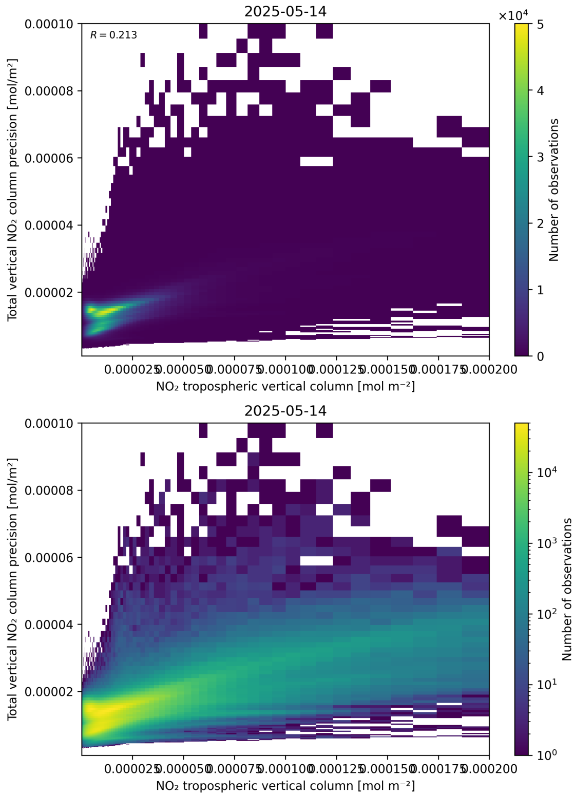
Figure 129: Scatter density plot of “NO 2 tropospheric vertical column” against “Total vertical NO 2 column precision” for 2025-05-13 to 2025-05-15.
