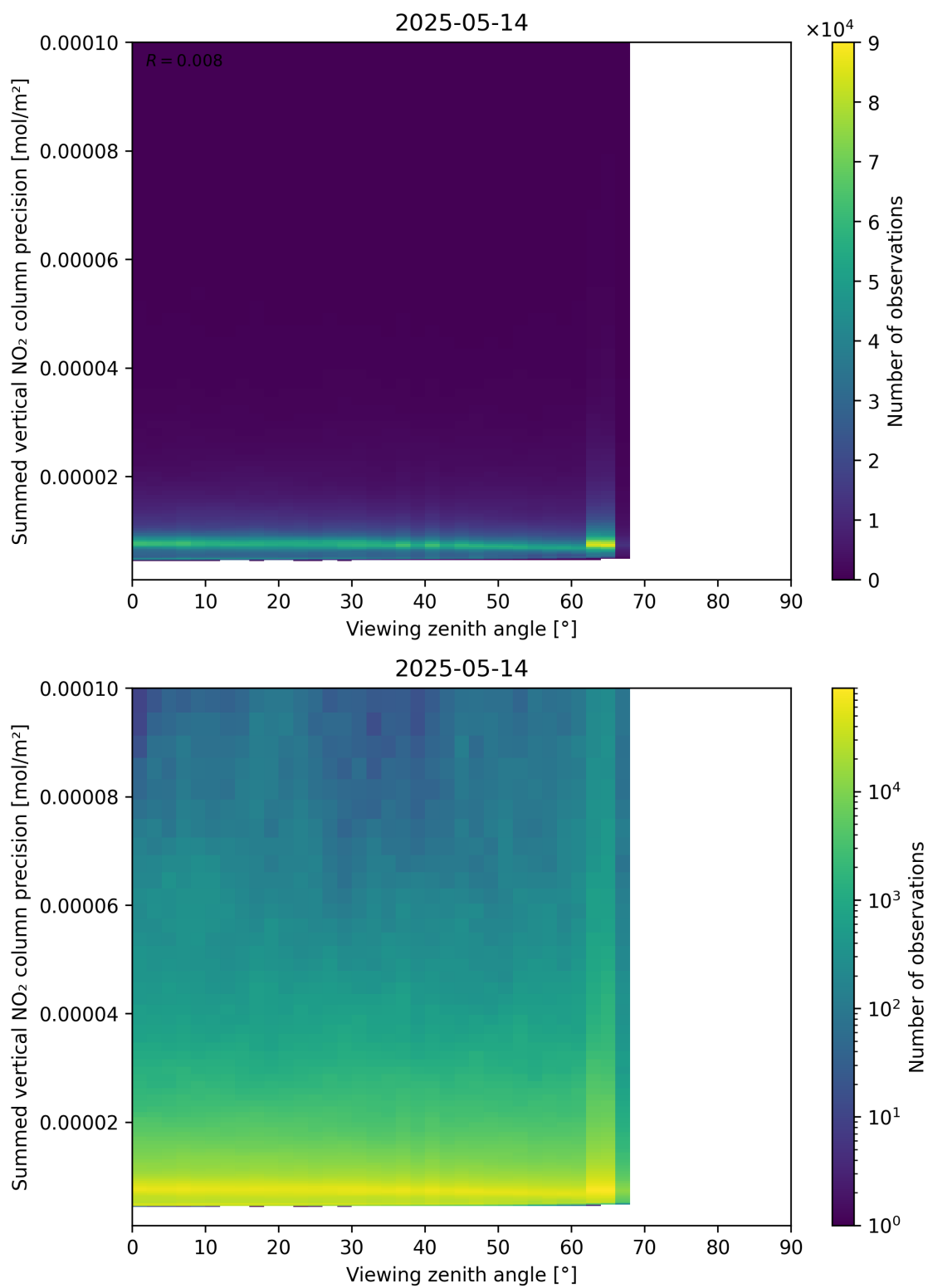
Figure 166: Scatter density plot of “Viewing zenith angle” against “Summed vertical NO 2 column precision” for 2025-05-13 to 2025-05-15.
