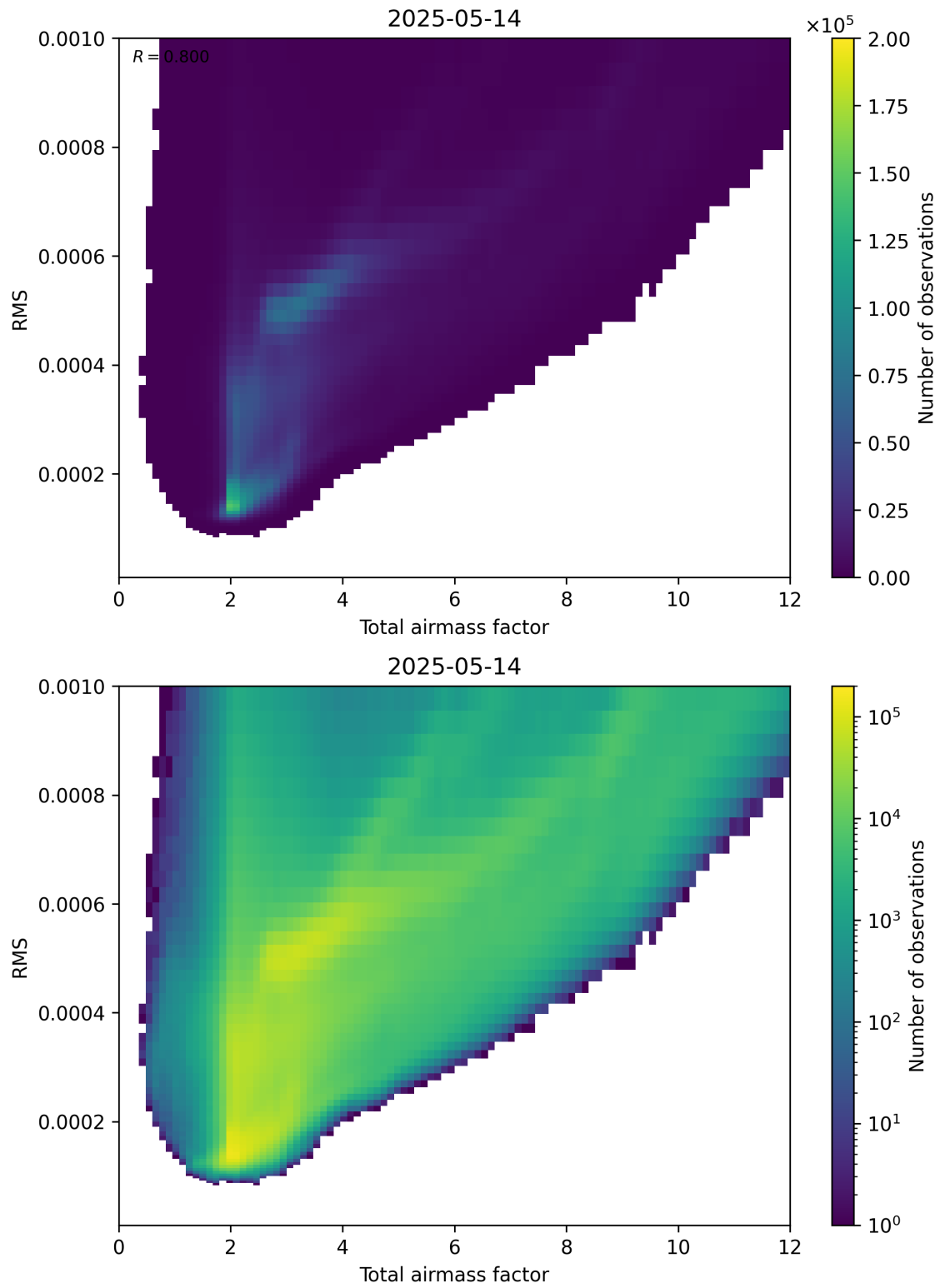
Figure 69: Scatter density plot of “Total airmass factor” against “RMS” for 2025-05-13 to 2025-05-15.
