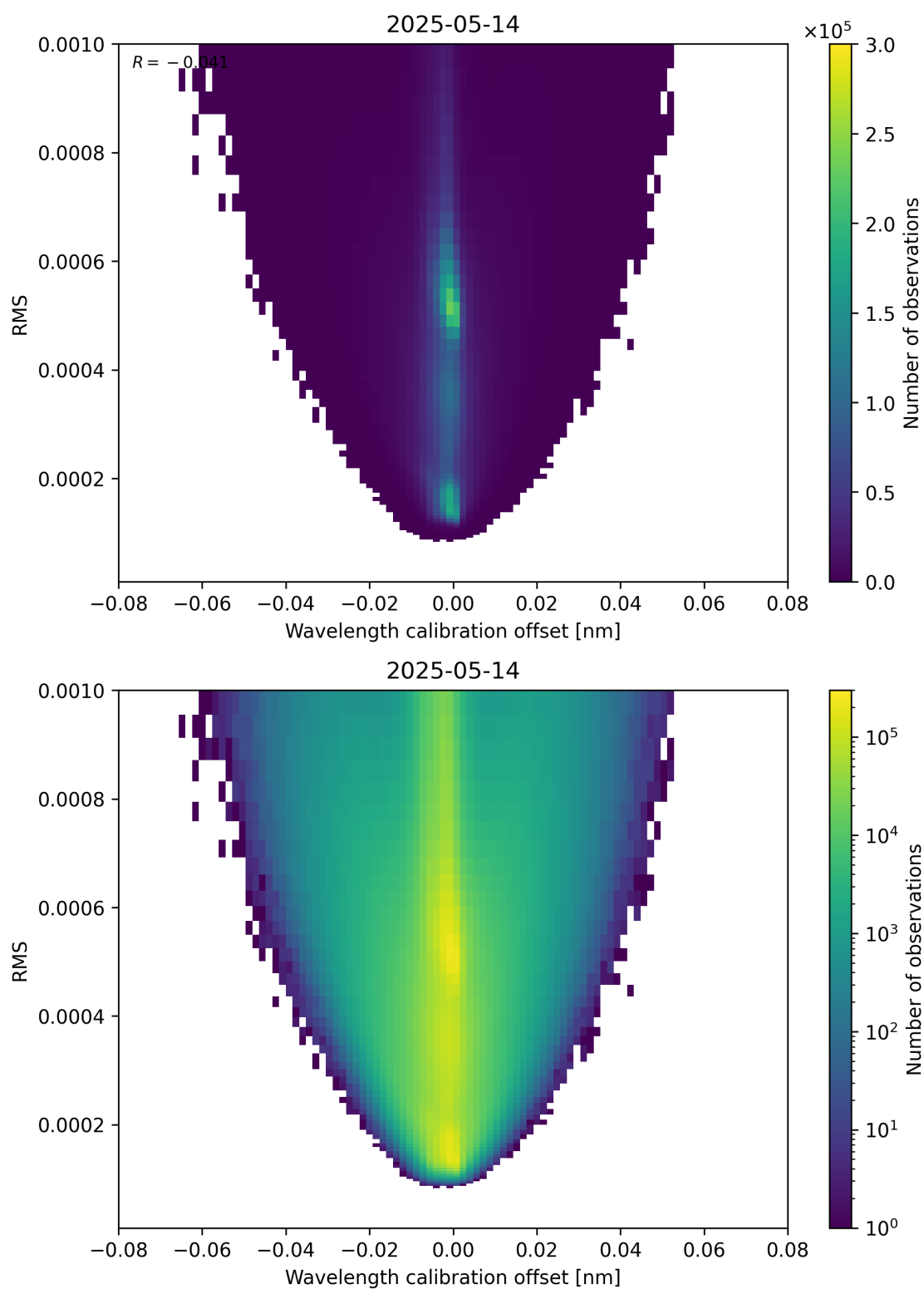
Figure 181: Scatter density plot of “Wavelength calibration offset” against “RMS” for 2025-05-13 to 2025-05-15.
