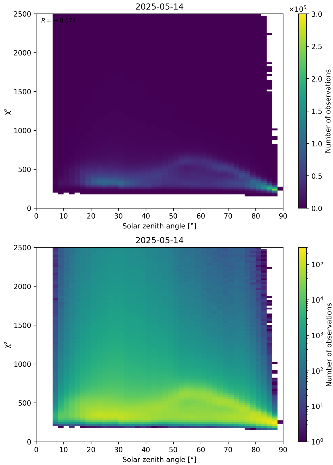
Figure 148: Scatter density plot of “Solar zenith angle” against “ \chi^2 ” for 2025-05-13 to 2025-05-15.
