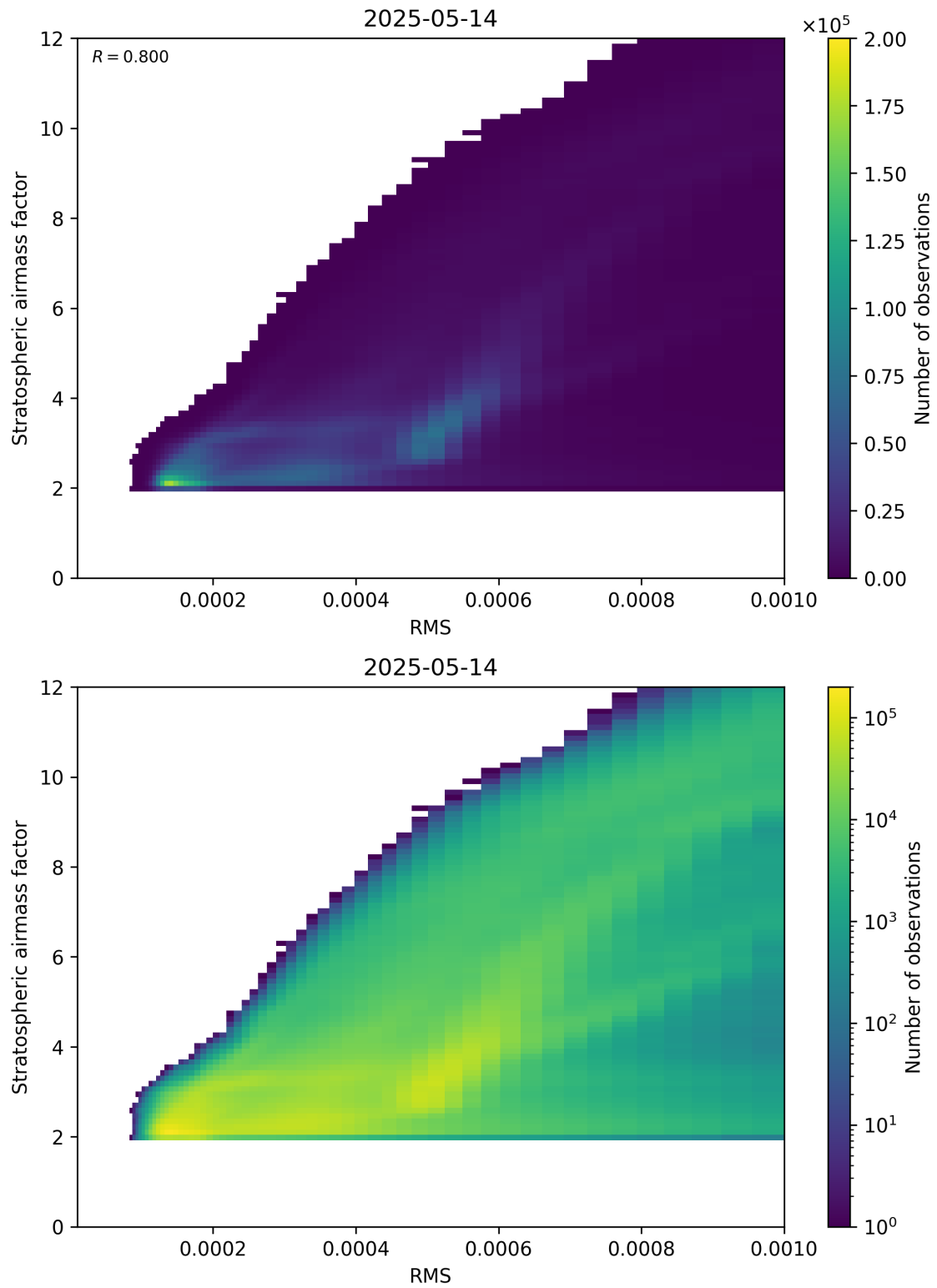
Figure 144: Scatter density plot of “RMS” against “Stratospheric airmass factor” for 2025-05-13 to 2025-05-15.
