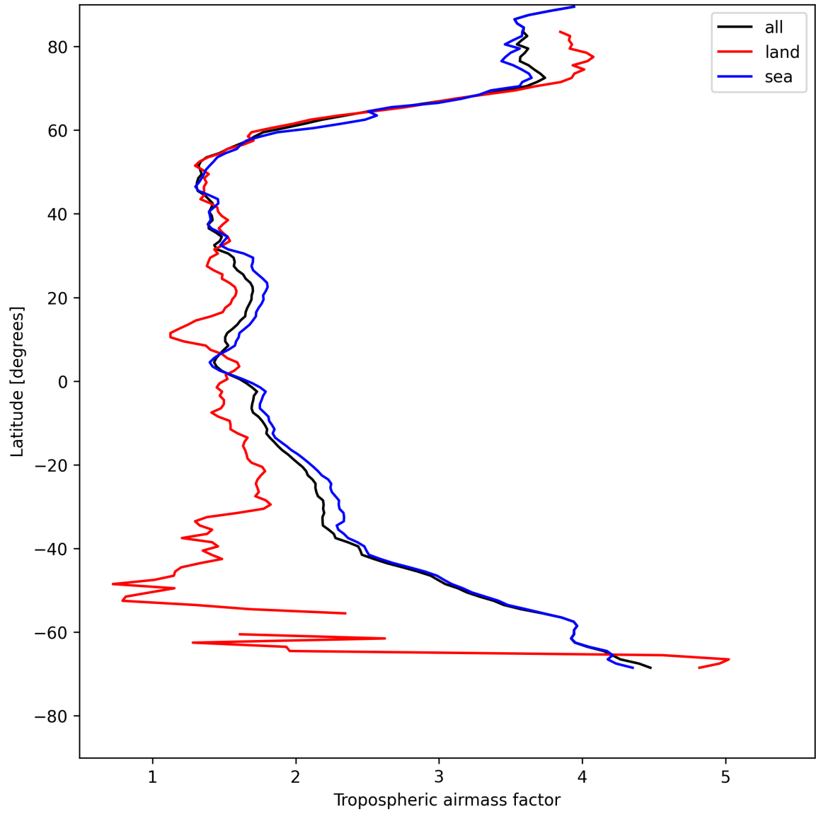
Figure 14: Zonal average of “Tropospheric airmass factor” for 2025-05-13 to 2025-05-15.
