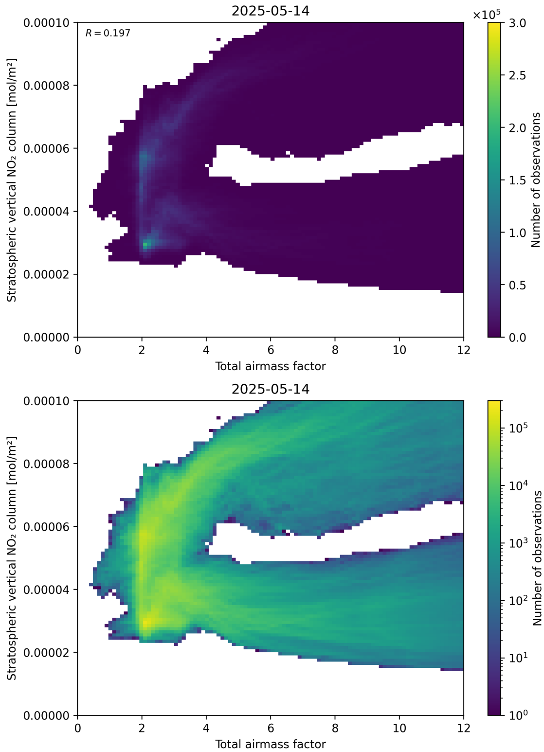
Figure 64: Scatter density plot of “Total airmass factor” against “Stratospheric vertical \text{NO}_2 column” for 2025-05-13 to 2025-05-15.
