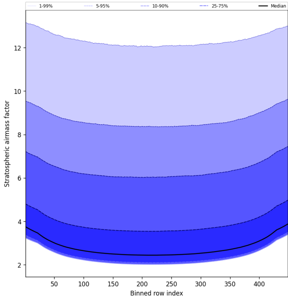
Figure 61: Along track statistics of “Stratospheric airmass factor” for 2025-05-13 to 2025-05-15
