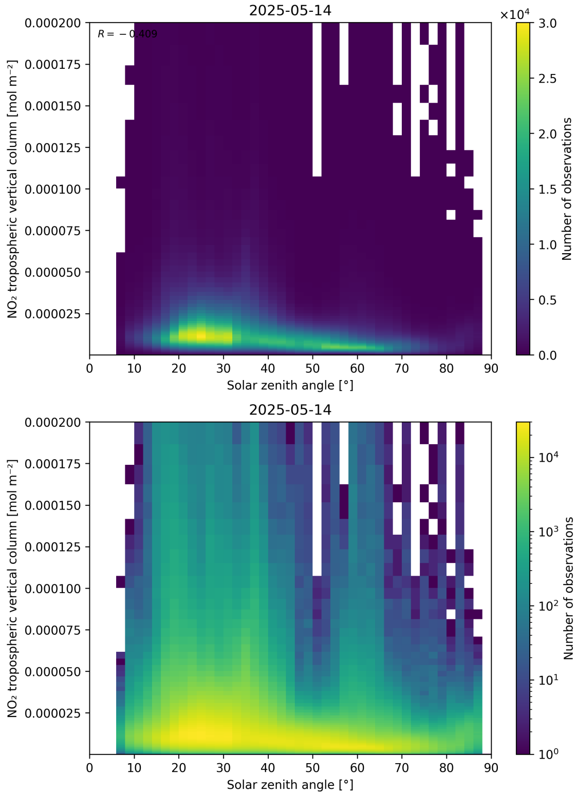
Figure 155: Scatter density plot of “Solar zenith angle” against “NO 2 tropospheric vertical column” for 2025-05-13 to 2025-05-15.
