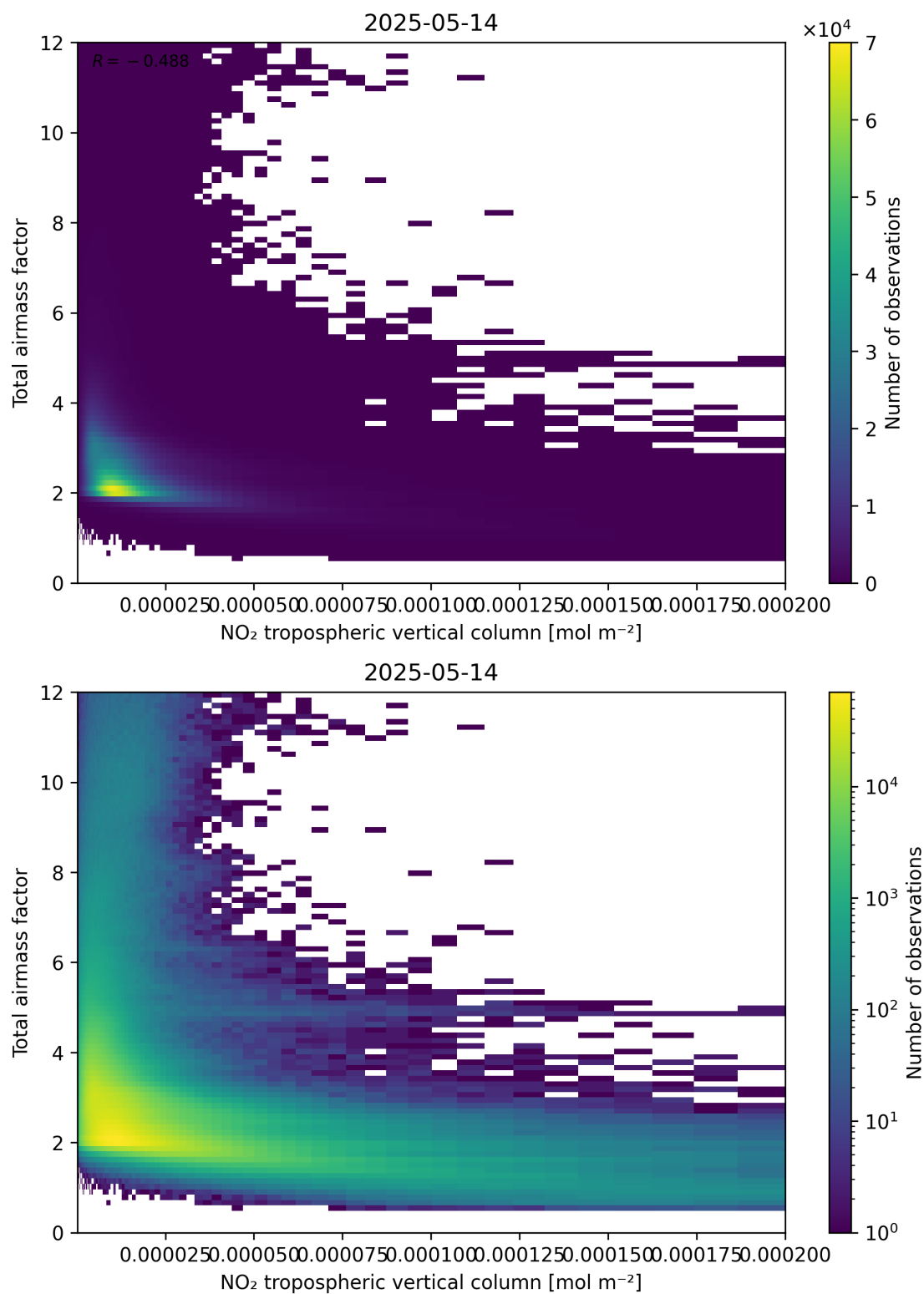
Figure 122: Scatter density plot of “NO 2 tropospheric vertical column” against “Total air mass factor” for 2025-05-13 to 2025-05-15.
