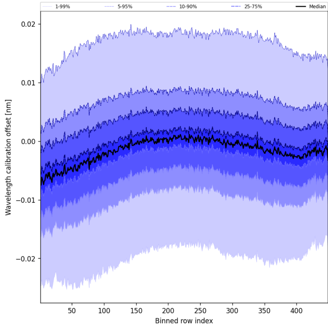
Figure 52: Along track statistics of “Wavelength calibration offset” for 2025-05-13 to 2025-05-15
