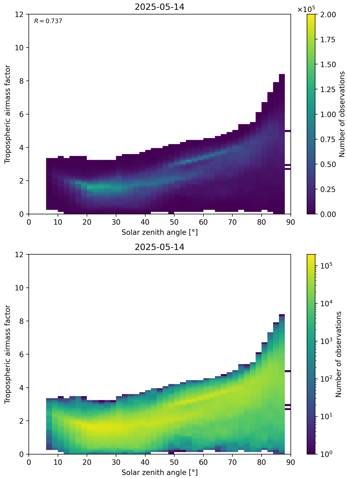
Figure 147: Scatter density plot of “Solar zenith angle” against “Tropospheric airmass factor” for 2025-05-13 to 2025-05-15.
