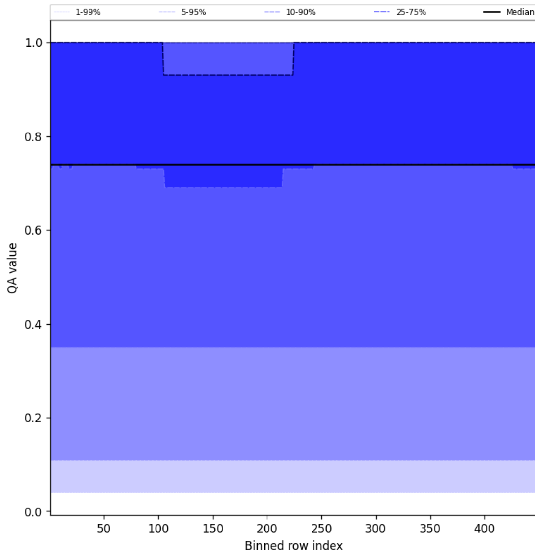
Figure 45: Along track statistics of “QA value” for 2025-05-13 to 2025-05-15
