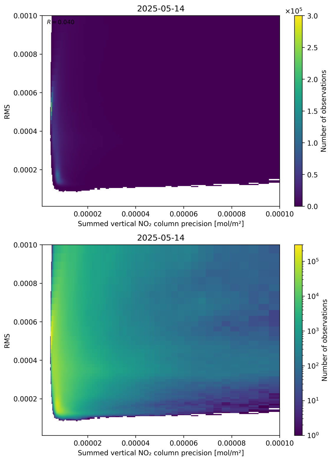
Figure 108: Scatter density plot of “Summed vertical NO 2 column precision” against “RMS” for 2025-05-13 to 2025-05-15.
