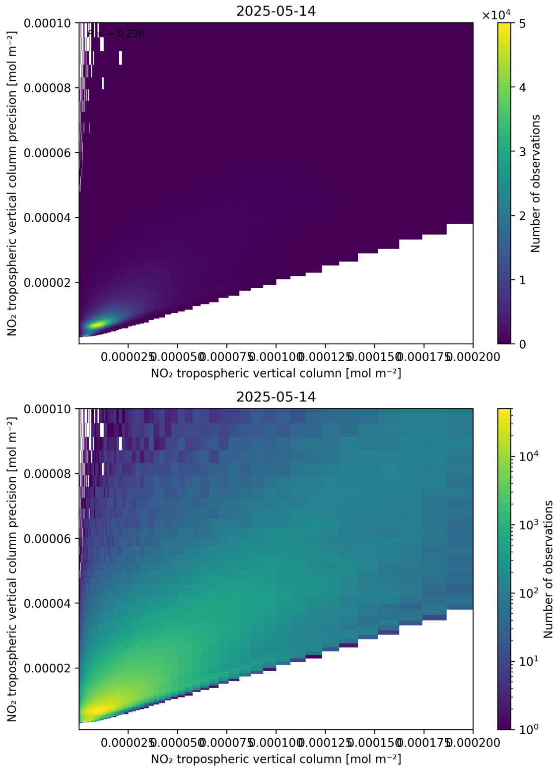
Figure 130: Scatter density plot of “NO 2 tropospheric vertical column” against “NO 2 tropospheric vertical column precision” for 2025-05-13 to 2025-05-15.
