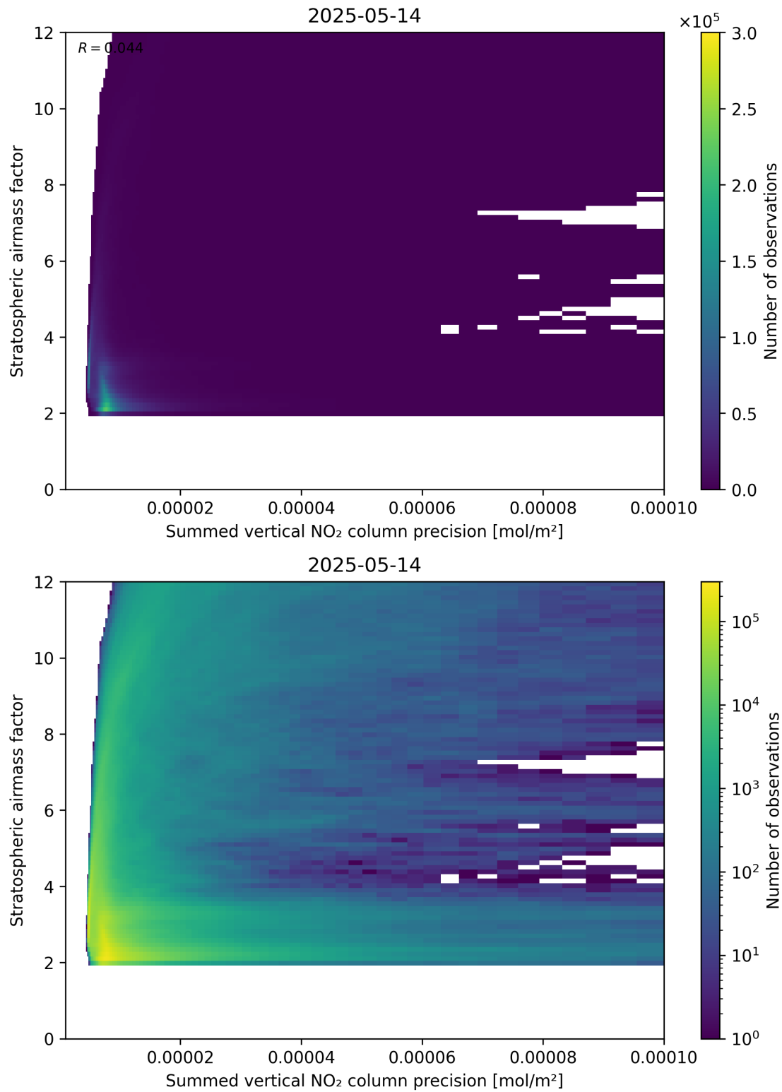
Figure 106: Scatter density plot of “Summed vertical NO 2 column precision” against “Stratospheric airmass factor” for 2025-05-13 to 2025-05-15.
