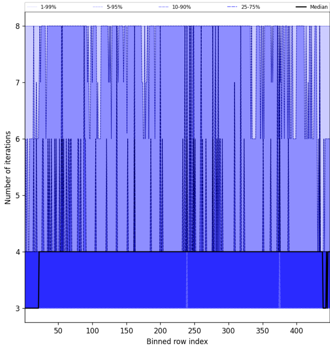
Figure 51: Along track statistics of “Number of iterations” for 2025-05-13 to 2025-05-15
