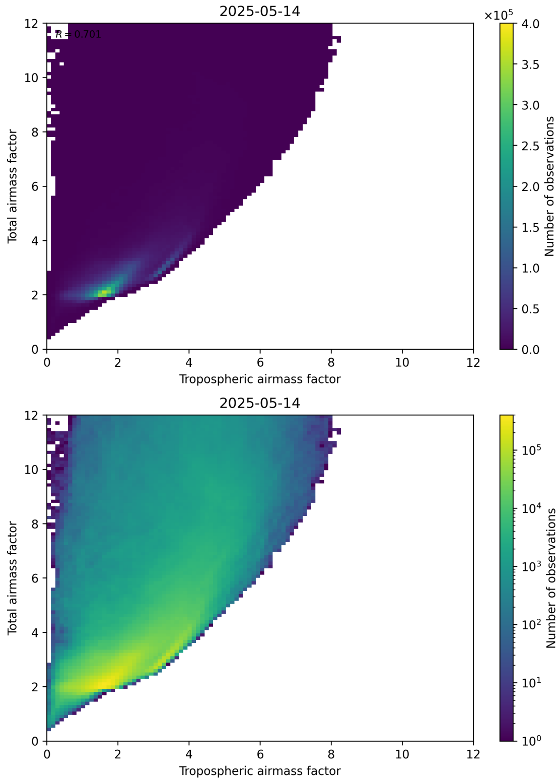
Figure 72: Scatter density plot of “Tropospheric airmass factor” against “Total airmass factor” for 2025-05-13 to 2025-05-15.
