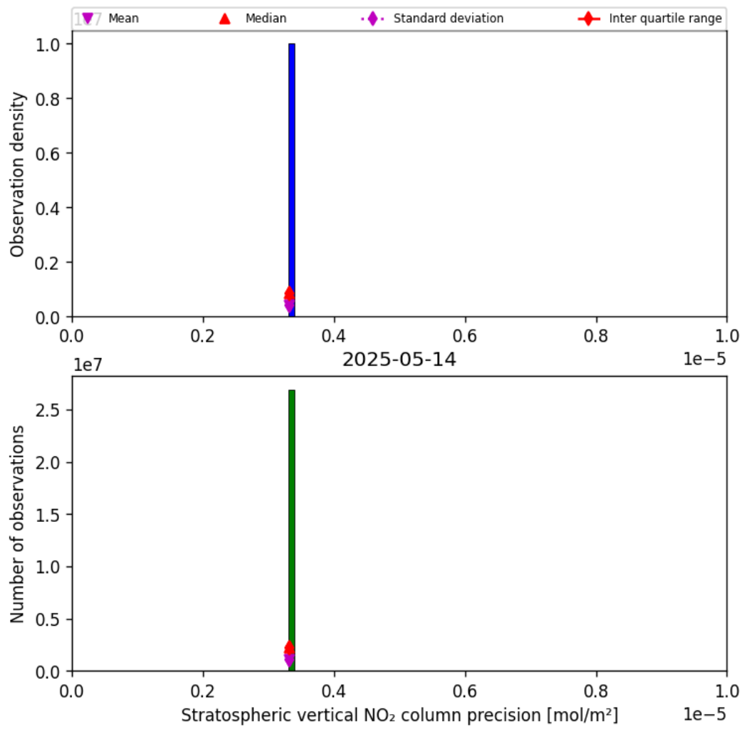
Figure 37: Histogram of “Stratospheric vertical NO 2 column precision” for 2025-05-13 to 2025-05-15
