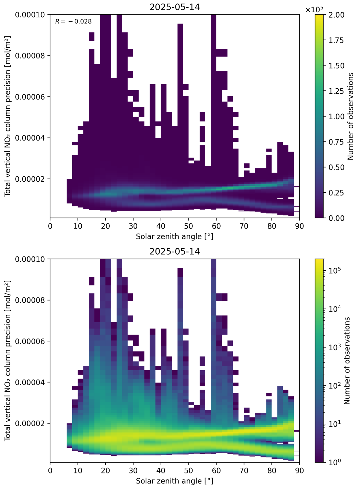
Figure 154: Scatter density plot of “Solar zenith angle” against “Total vertical NO 2 column precision” for 2025-05-13 to 2025-05-15.
