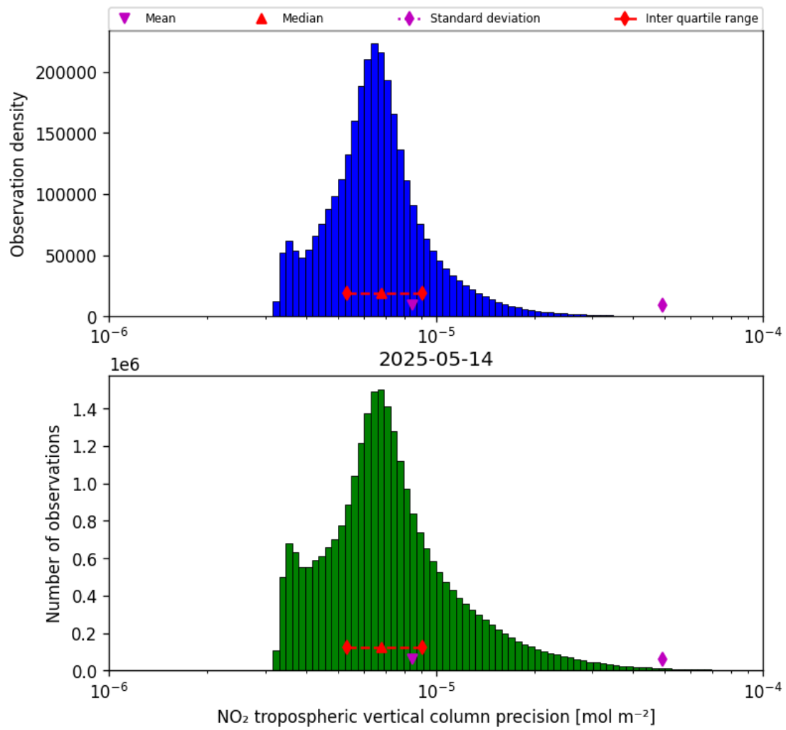
Figure 30: Histogram of “NO 2 tropospheric vertical column precision” for 2025-05-13 to 2025-05-15
