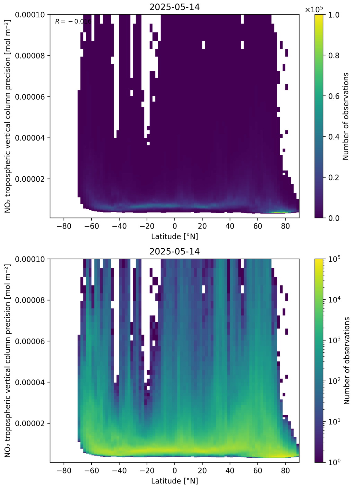
Figure 93: Scatter density plot of “Latitude” against “NO 2 tropospheric vertical column precision” for 2025-05-13 to 2025-05-15.
