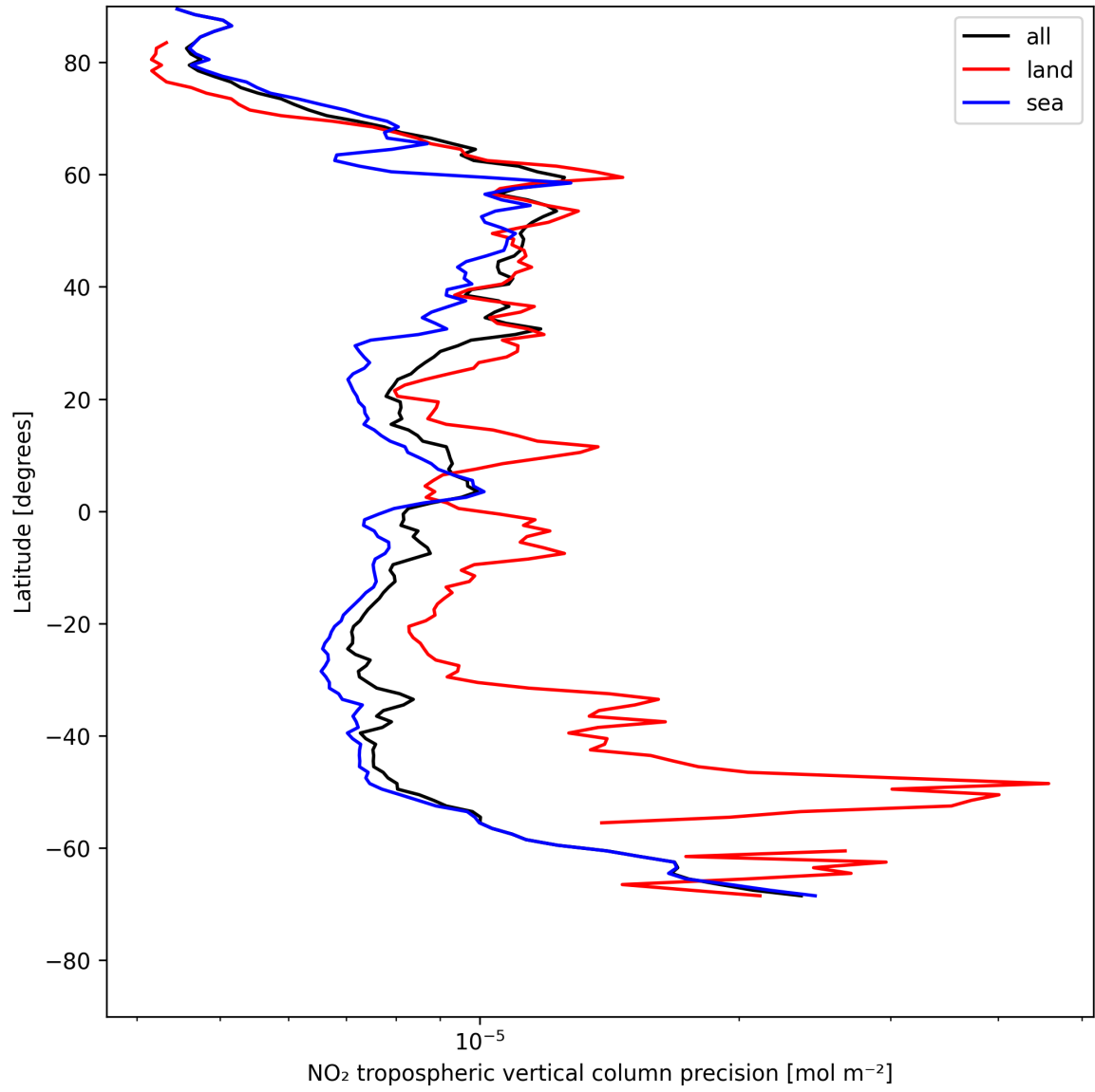
Figure 13: Zonal average of “NO 2 tropospheric vertical column precision” for 2025-05-13 to 2025-05-15.
