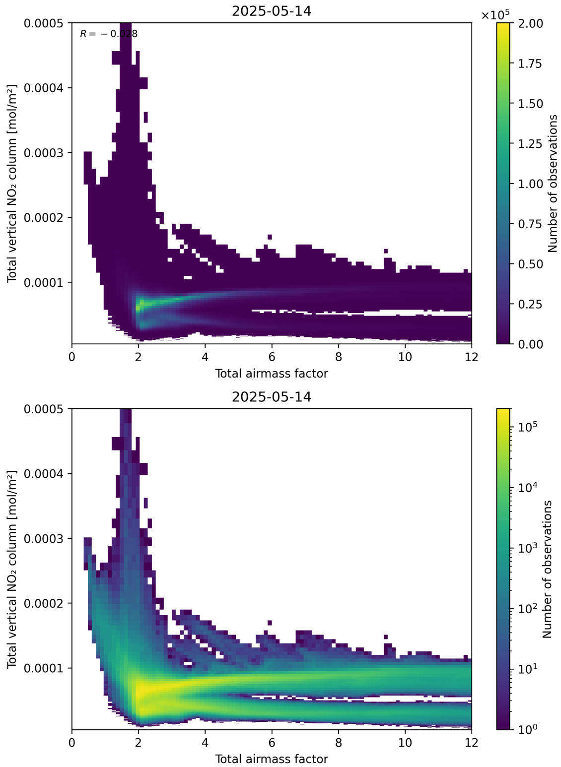
Figure 67: Scatter density plot of “Total airmass factor” against “Total vertical NO 2 column” for 2025-05-13 to 2025-05-15.
