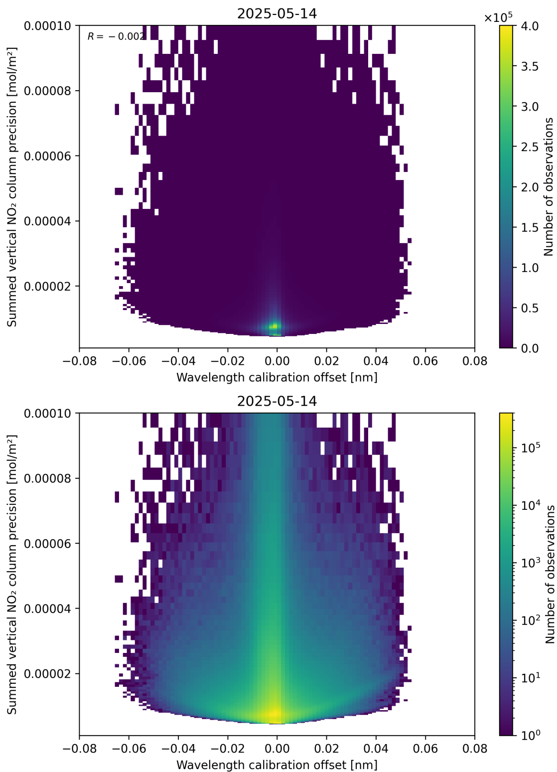
Figure 178: Scatter density plot of “Wavelength calibration offset” against “Summed vertical NO 2 column precision” for 2025-05-13 to 2025-05-15.
