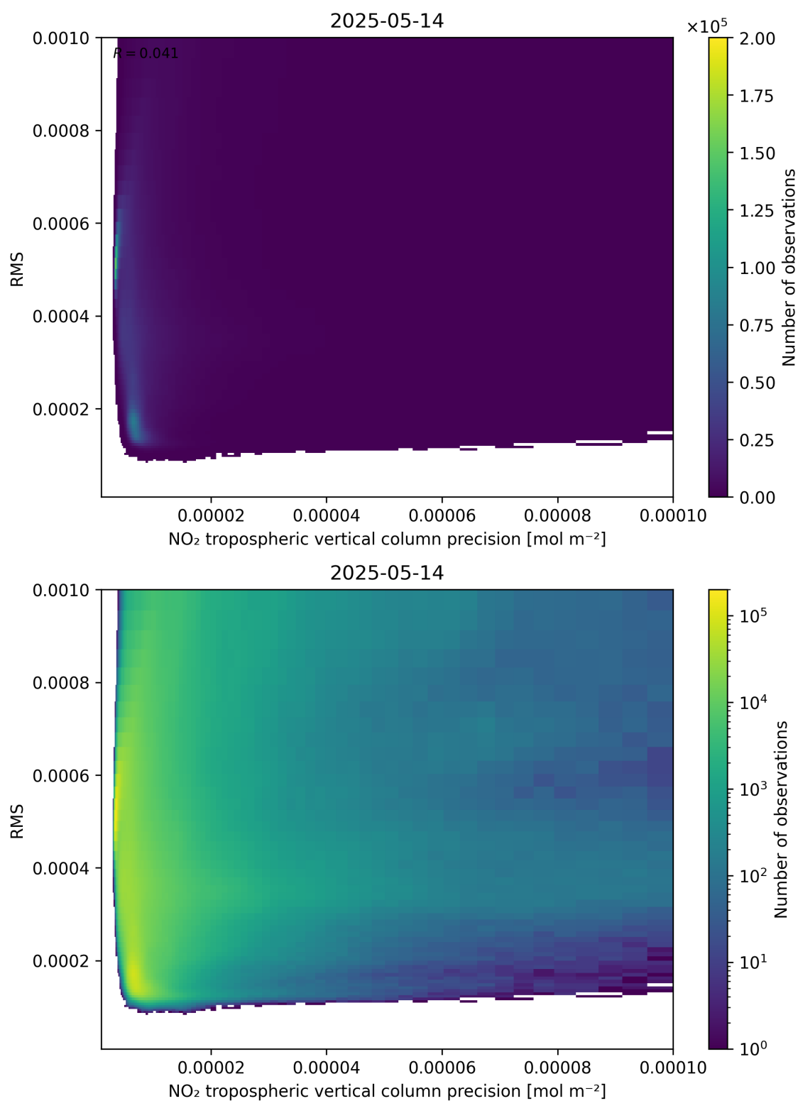
Figure 140: Scatter density plot of “NO 2 tropospheric vertical column precision” against “RMS” for 2025-05-13 to 2025-05-15.
