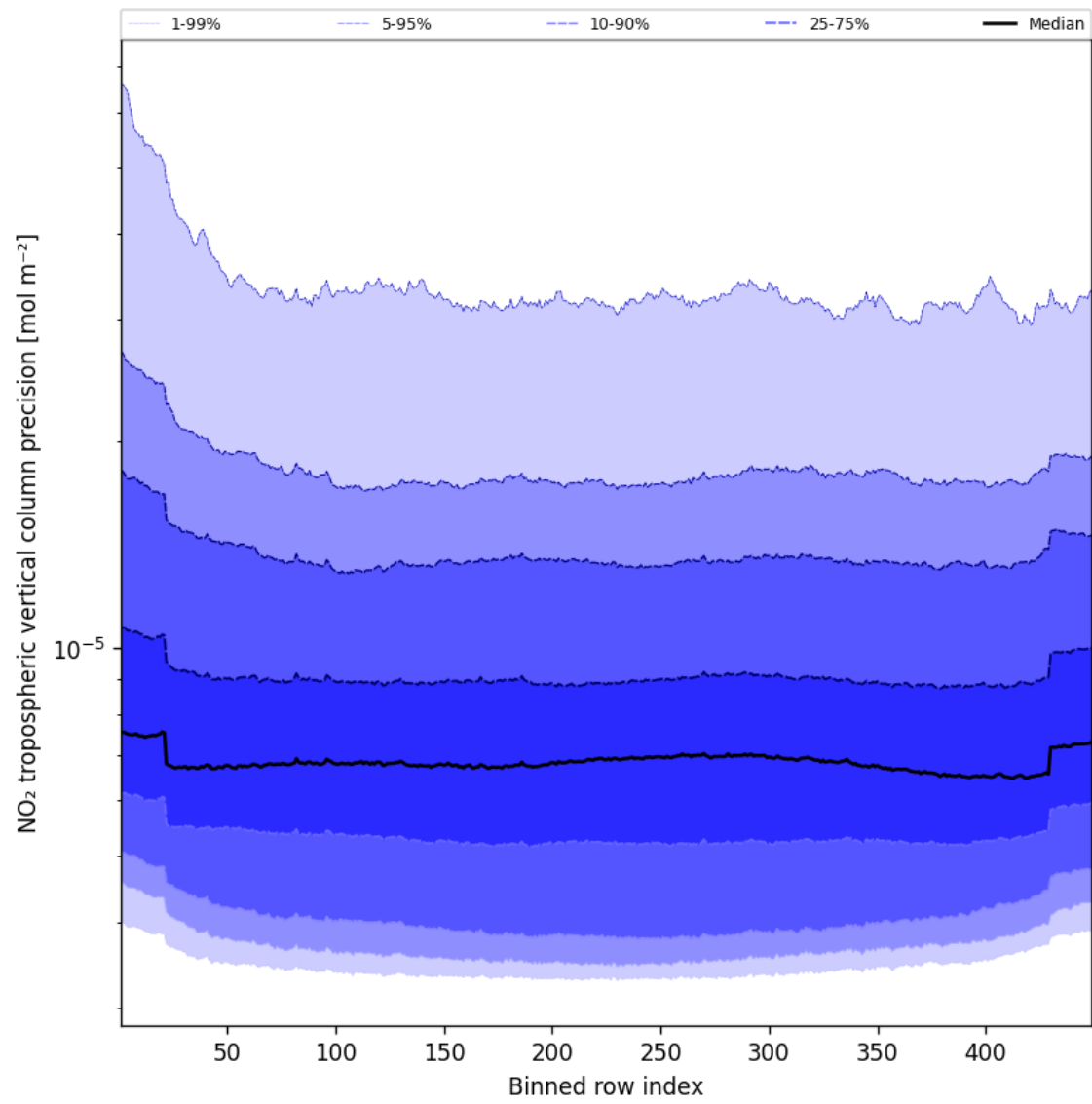
Figure 47: Along track statistics of “NO 2 tropospheric vertical column precision” for 2025-05-13 to 2025-05-15
