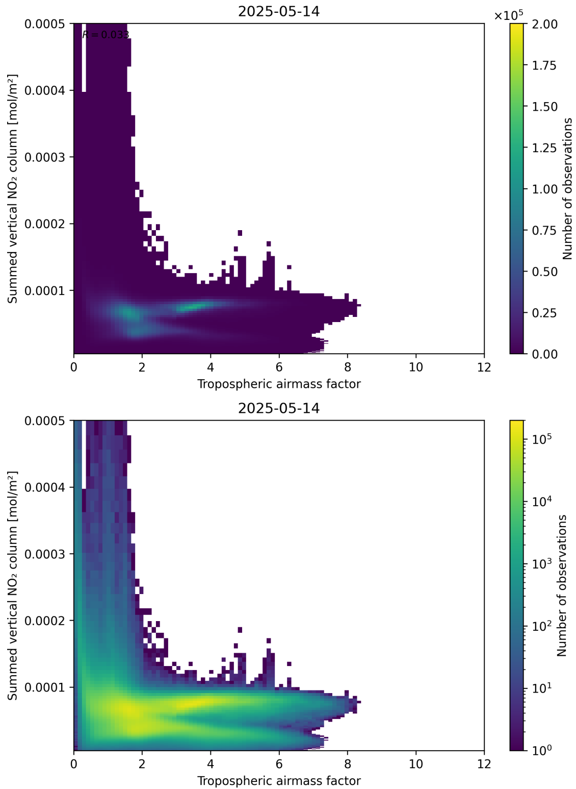
Figure 75: Scatter density plot of “Tropospheric air mass factor” against “Summed vertical NO 2 column” for 2025-05-13 to 2025-05-15.
