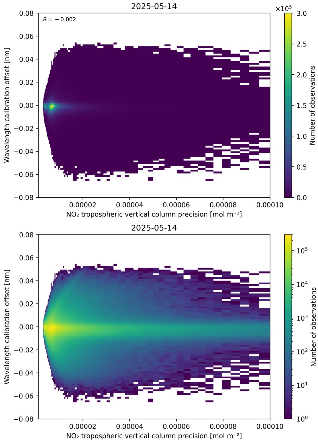
Figure 141: Scatter density plot of “NO 2 tropospheric vertical column precision” against “Wavelength calibration offset” for 2025-05-13 to 2025-05-15.
