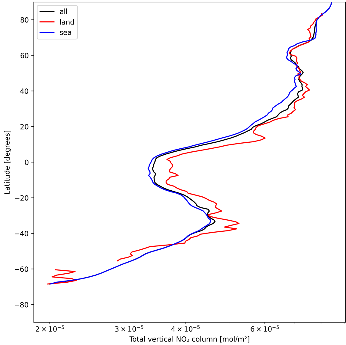
Figure 21: Zonal average of “Total vertical NO 2 column” for 2025-05-13 to 2025-05-15.
