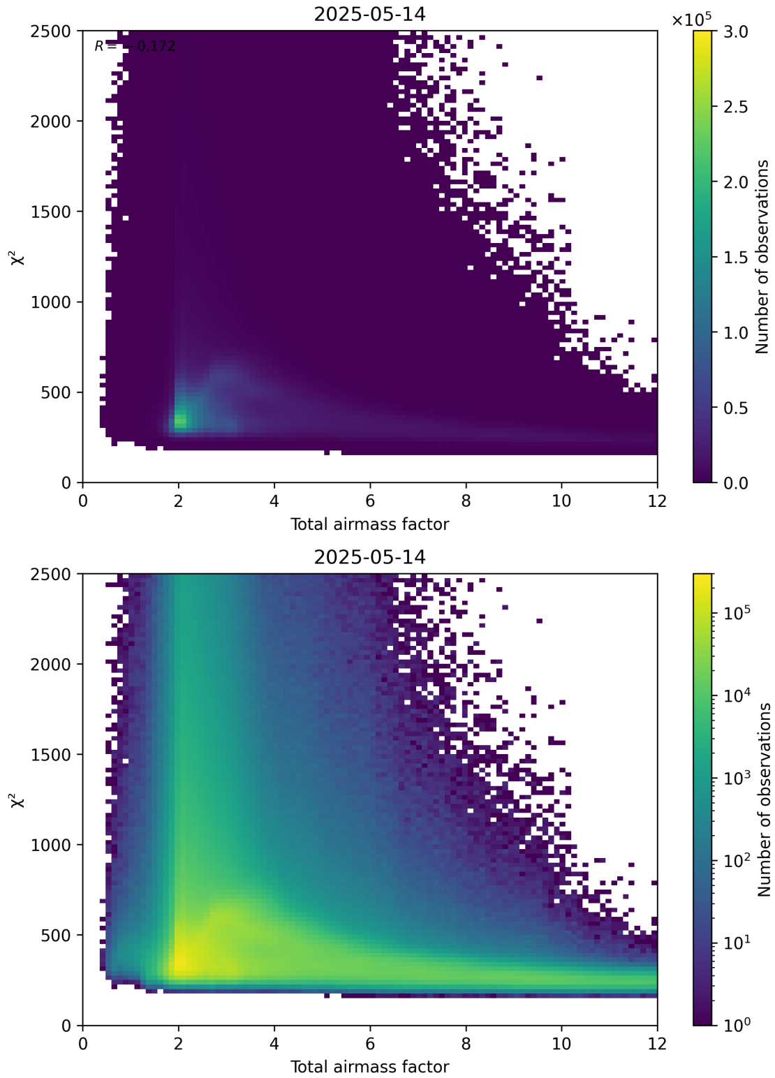
Figure 63: Scatter density plot of “Total airmass factor” against “ \chi^2 ” for 2025-05-13 to 2025-05-15.
