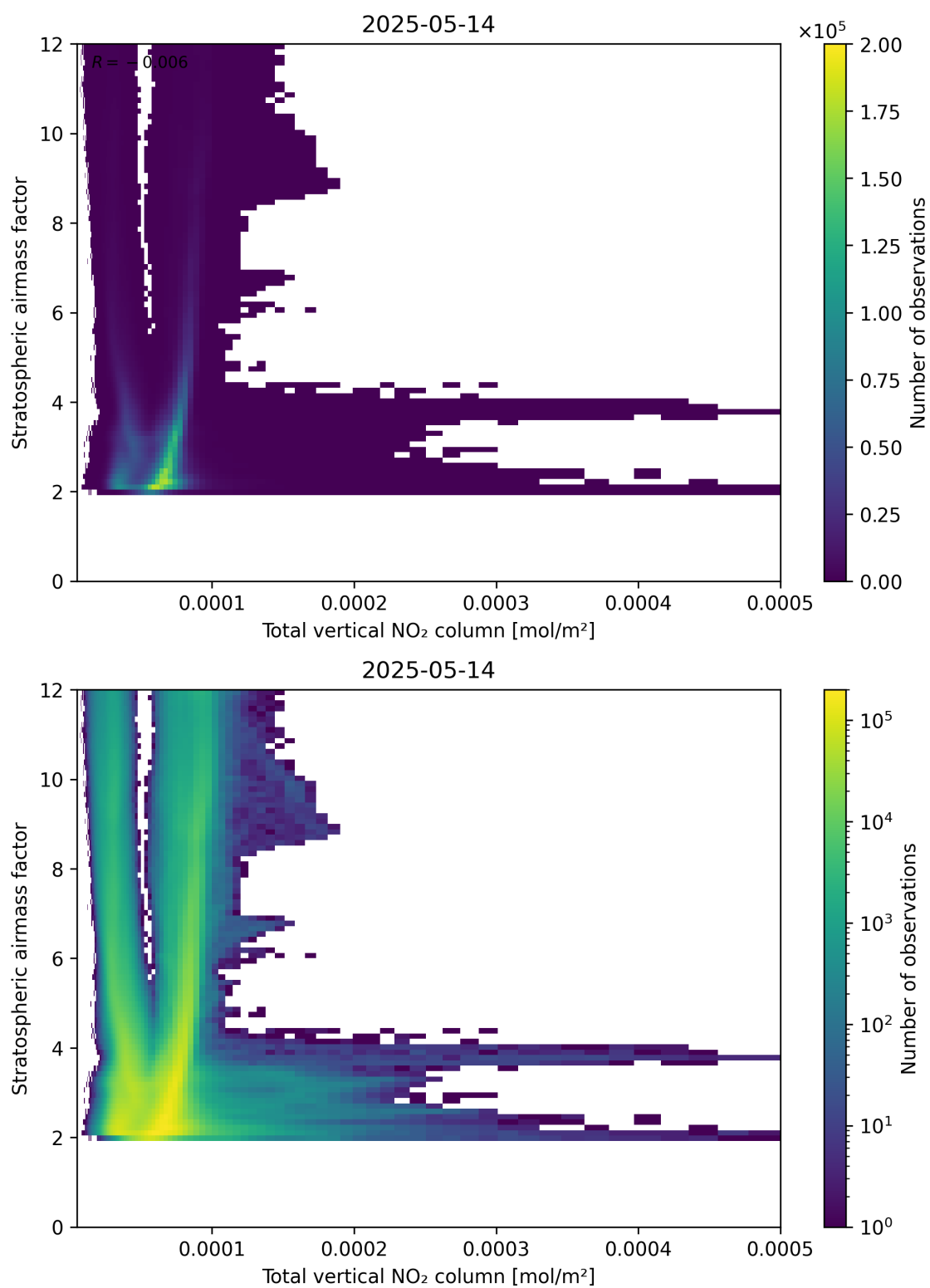
Figure 110: Scatter density plot of “Total vertical NO 2 column” against “Stratospheric airmass factor” for 2025-05-13 to 2025-05-15.
