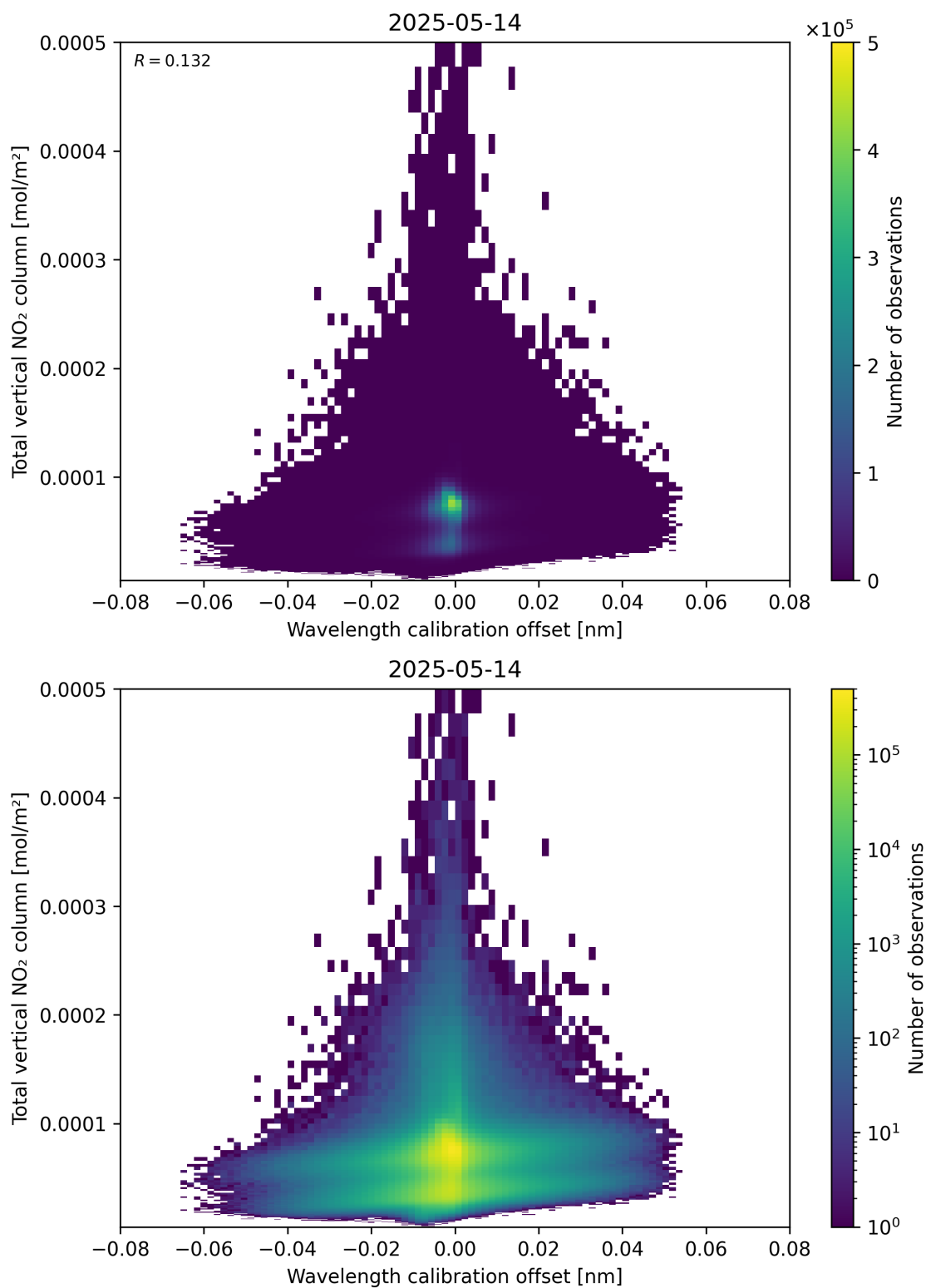
Figure 179: Scatter density plot of “Wavelength calibration offset” against “Total vertical NO 2 column” for 2025-05-13 to 2025-05-15.
