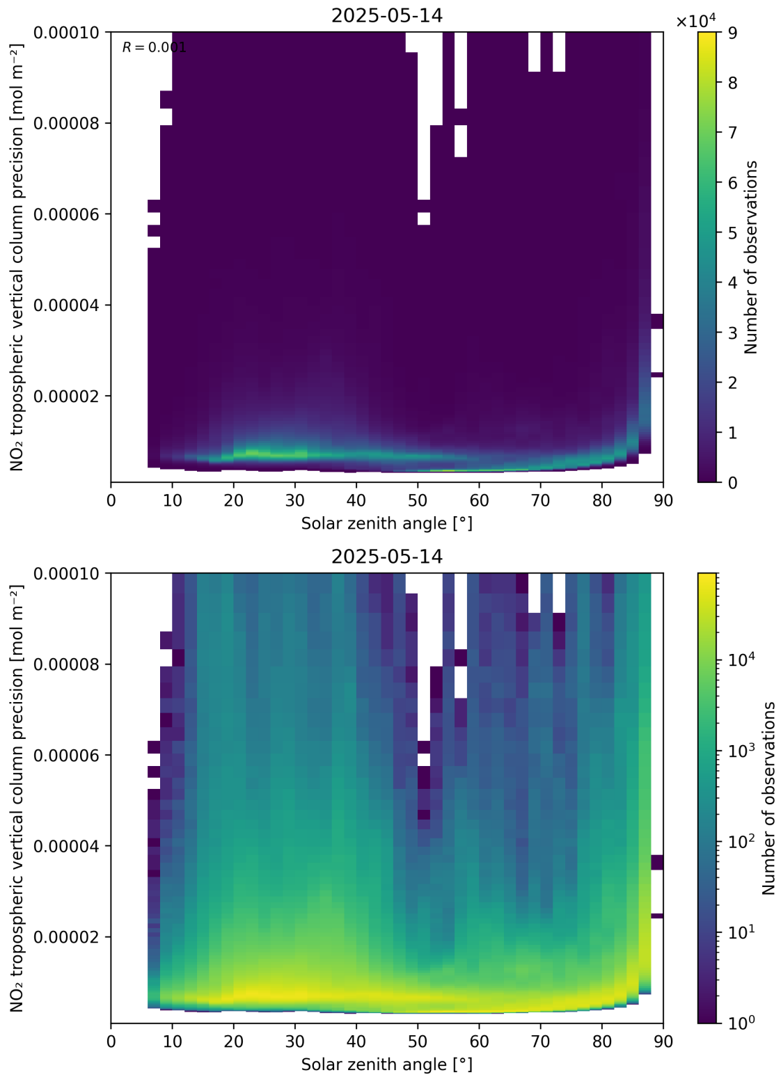
Figure 156: Scatter density plot of “Solar zenith angle” against “NO 2 tropospheric vertical column precision” for 2025-05-13 to 2025-05-15.
