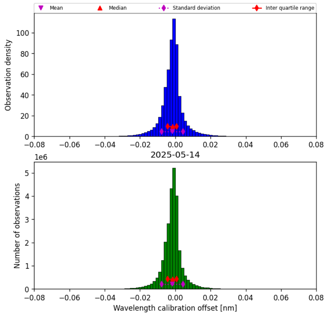
Figure 35: Histogram of “Wavelength calibration offset” for 2025-05-13 to 2025-05-15
