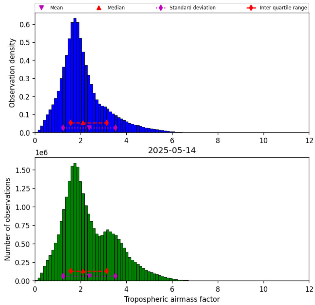
Figure 31: Histogram of “Tropospheric airmass factor” for 2025-05-13 to 2025-05-15
