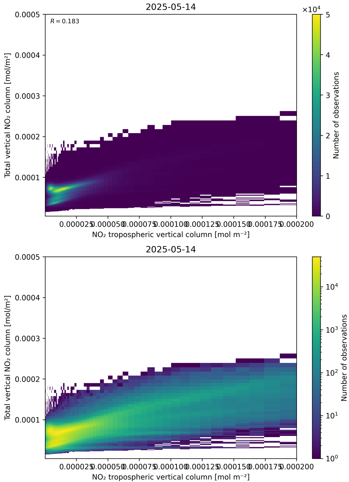
Figure 128: Scatter density plot of “NO 2 tropospheric vertical column” against “Total vertical NO 2 column” for 2025-05-13 to 2025-05-15.
