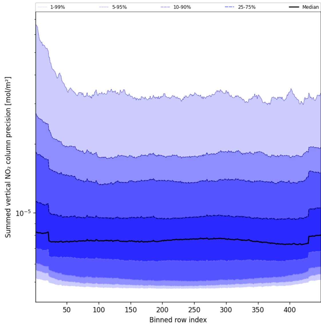
Figure 58: Along track statistics of “Summed vertical NO 2 column precision” for 2025-05-13 to 2025-05-15
