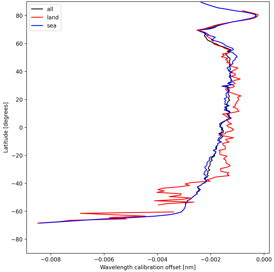
Figure 18: Zonal average of “Wavelength calibration offset” for 2025-05-13 to 2025-05-15.
