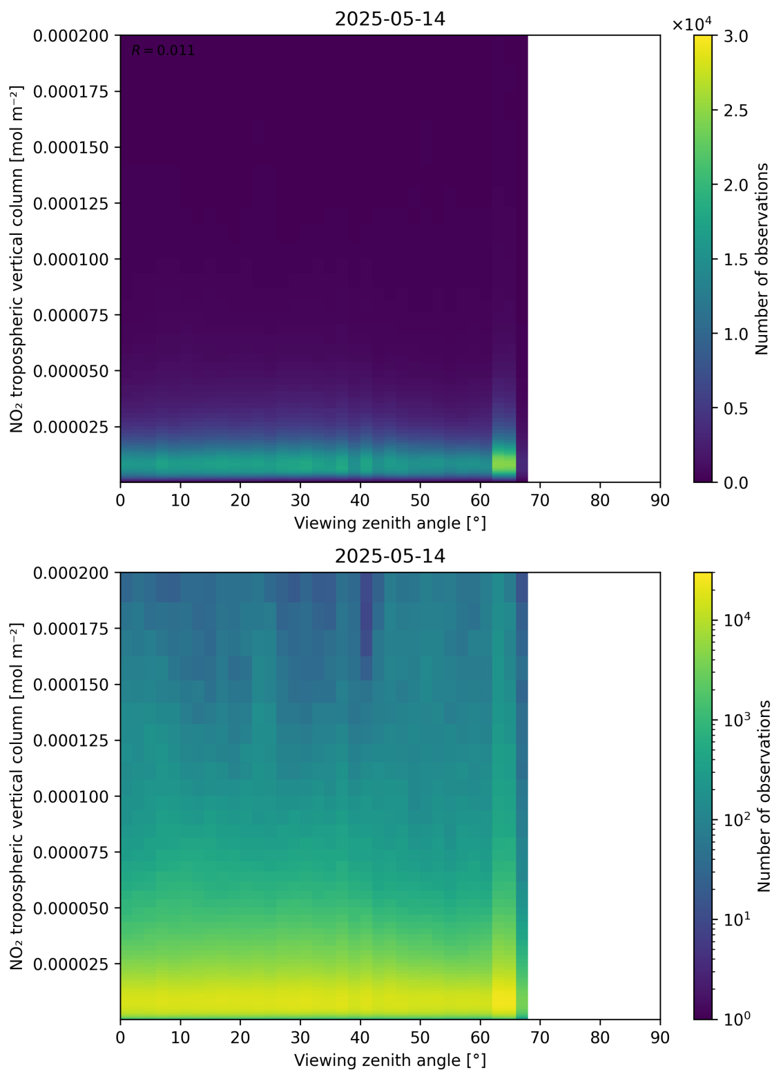
Figure 169: Scatter density plot of “Viewing zenith angle” against “NO 2 tropospheric vertical column” for 2025-05-13 to 2025-05-15.
