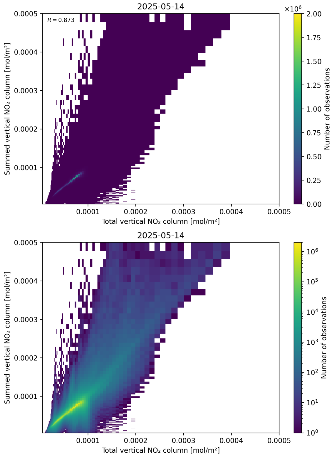
Figure 112: Scatter density plot of “Total vertical NO 2 column” against “Summed vertical NO 2 column” for 2025-05-13 to 2025-05-15.
