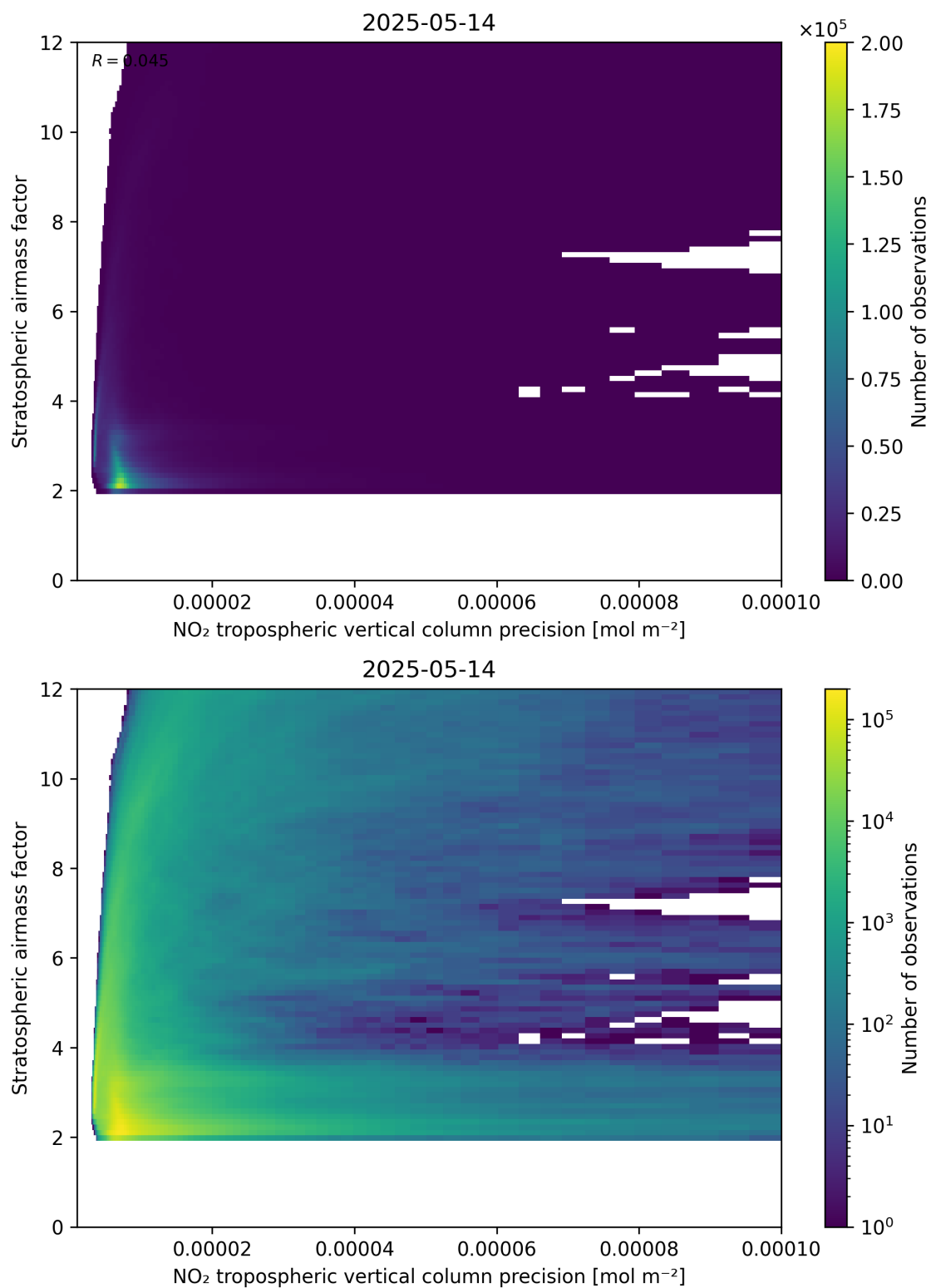
Figure 131: Scatter density plot of “NO 2 tropospheric vertical column precision” against “Stratospheric airmass factor” for 2025-05-13 to 2025-05-15.
