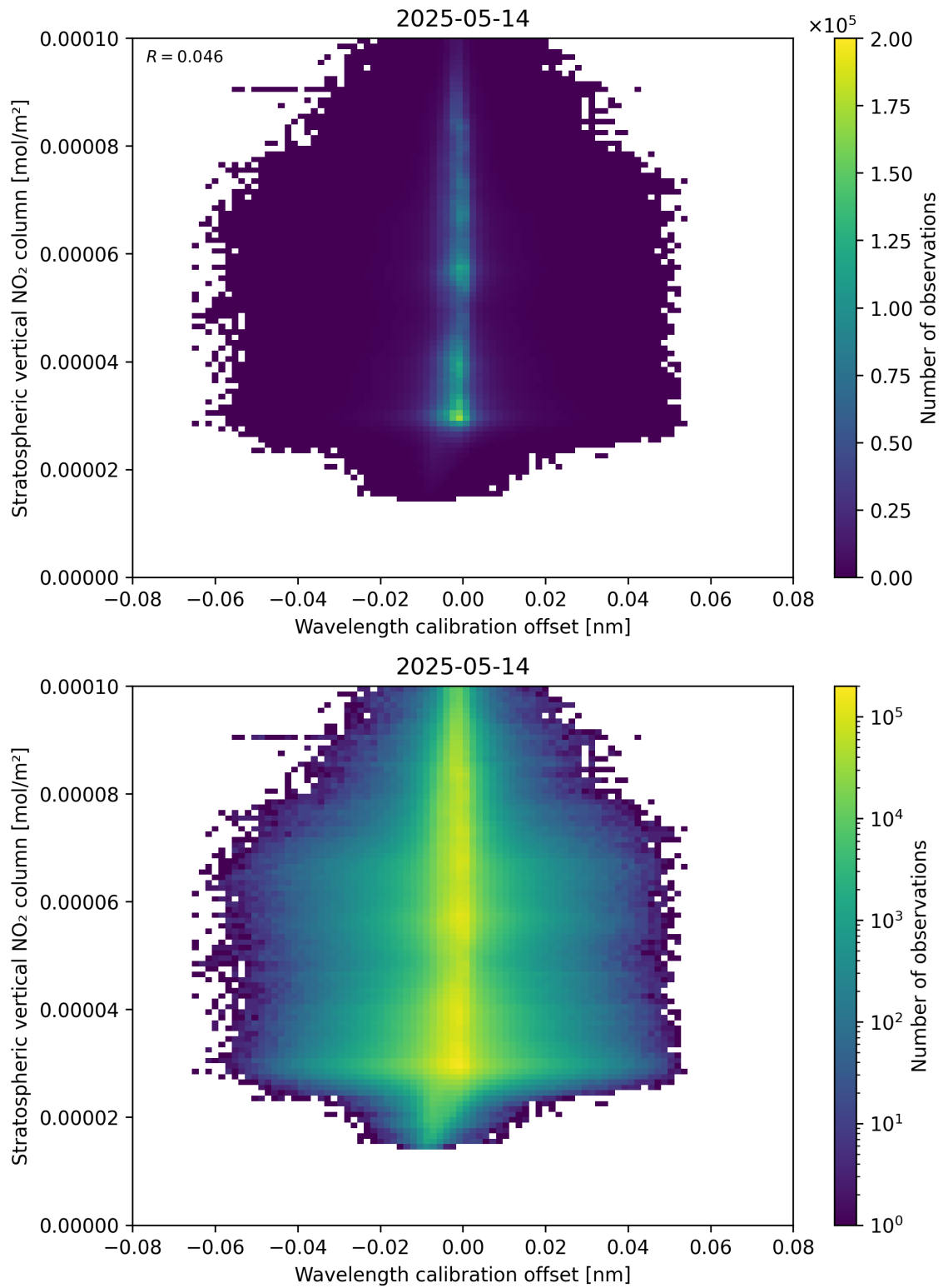
Figure 176: Scatter density plot of “Wavelength calibration offset” against “Stratospheric vertical NO 2 column” for 2025-05-13 to 2025-05-15.
