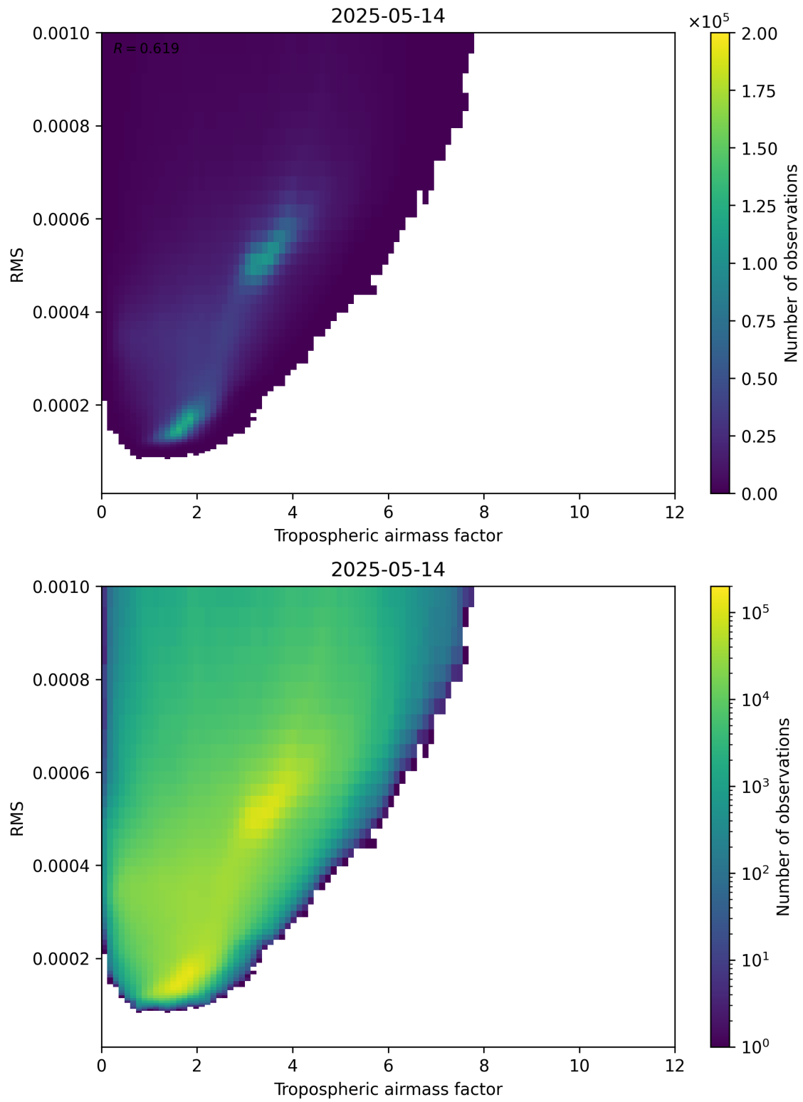
Figure 79: Scatter density plot of “Tropospheric airmass factor” against “RMS” for 2025-05-13 to 2025-05-15.
