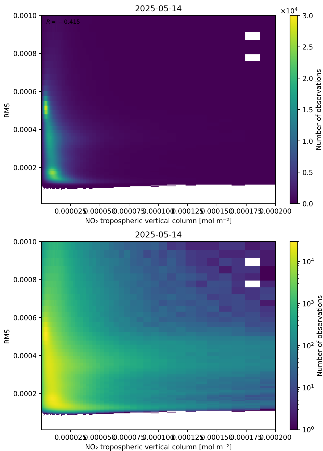
Figure 142: Scatter density plot of “NO 2 tropospheric vertical column” against “RMS” for 2025-05-13 to 2025-05-15.
