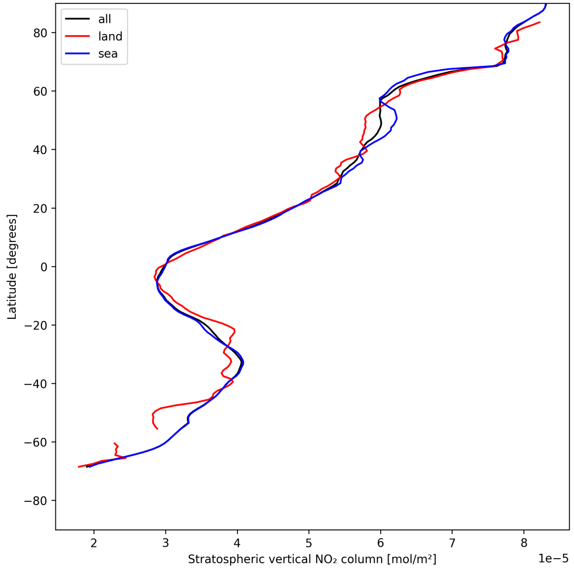
Figure 19: Zonal average of “Stratospheric vertical NO 2 column” for 2025-05-13 to 2025-05-15.
