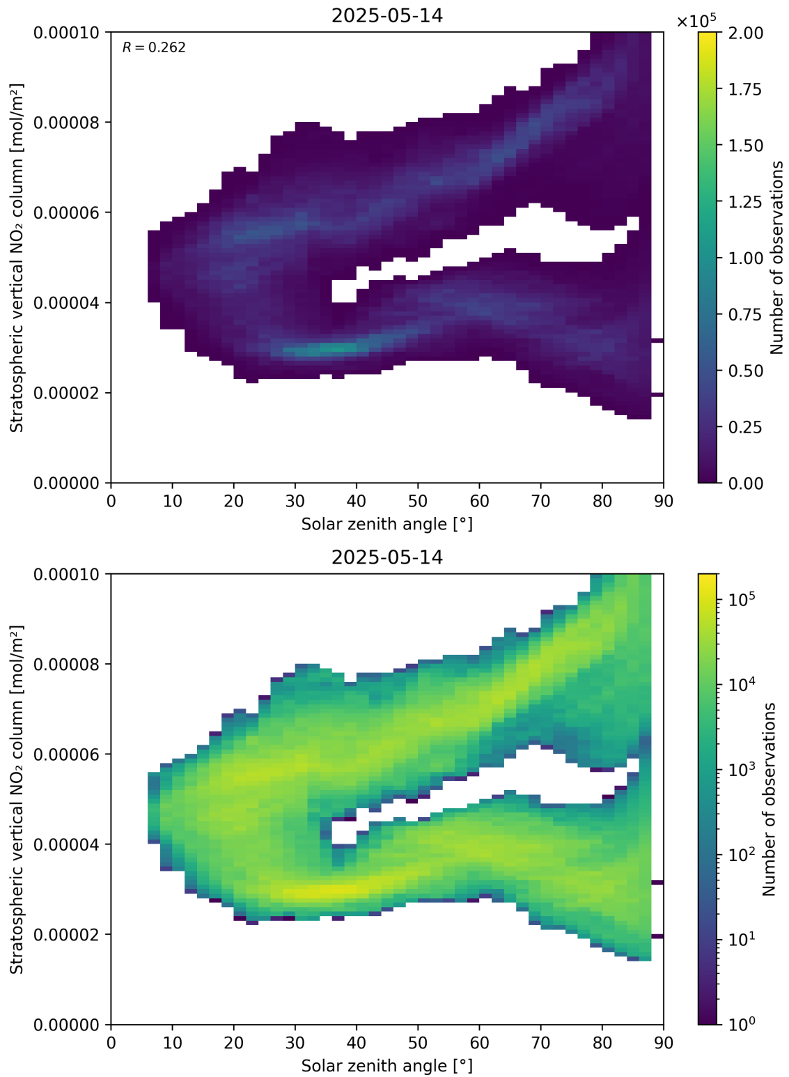
Figure 150: Scatter density plot of “Solar zenith angle” against “Stratospheric vertical NO 2 column” for 2025-05-13 to 2025-05-15.
