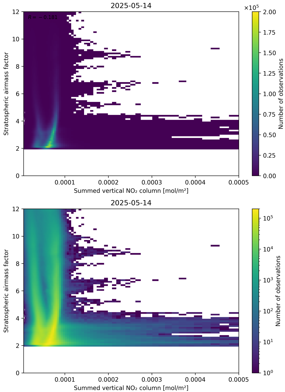
Figure 103: Scatter density plot of “Summed vertical NO 2 column” against “Stratospheric air mass factor” for 2025-05-13 to 2025-05-15.
