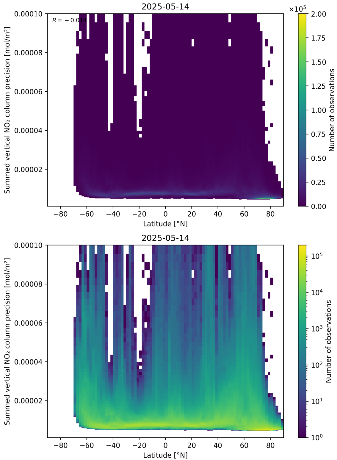
Figure 89: Scatter density plot of “Latitude” against “Summed vertical NO 2 column precision” for 2025-05-13 to 2025-05-15.
