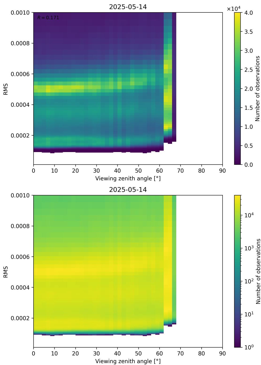
Figure 171: Scatter density plot of “Viewing zenith angle” against “RMS” for 2025-05-13 to 2025-05-15.
