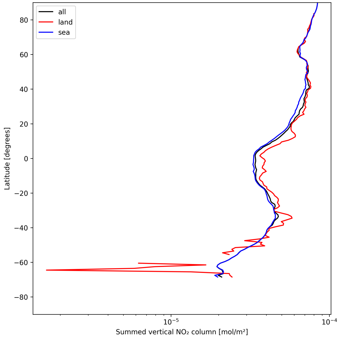
Figure 23: Zonal average of “Summed vertical NO 2 column” for 2025-05-13 to 2025-05-15.
