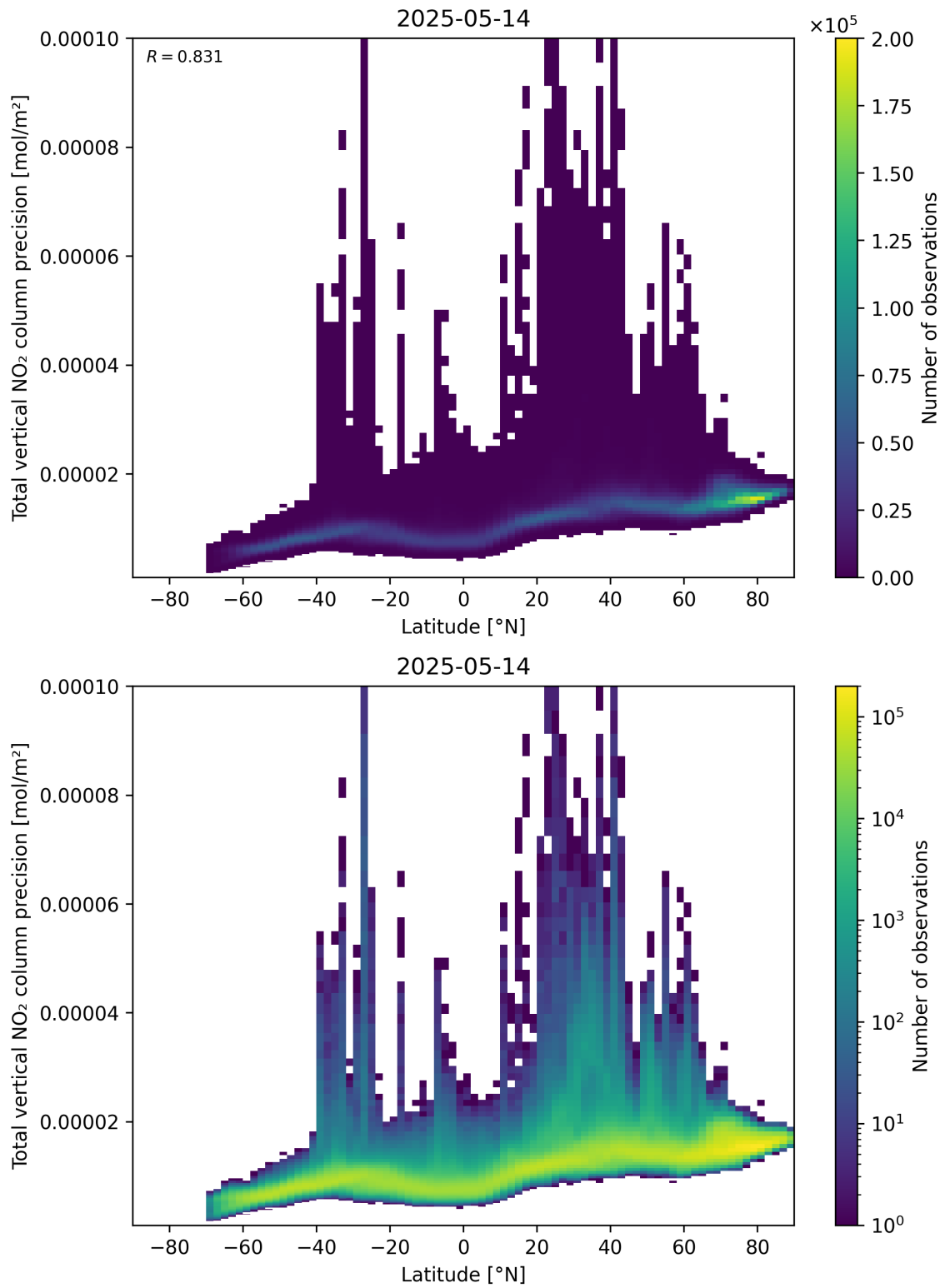
Figure 91: Scatter density plot of “Latitude” against “Total vertical NO 2 column precision” for 2025-05-13 to 2025-05-15.
