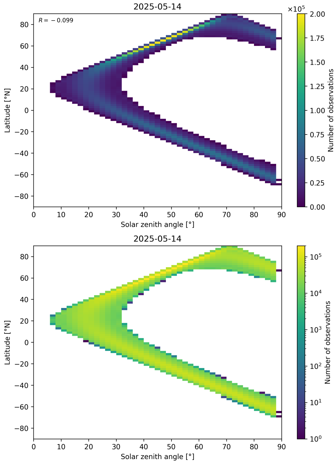
Figure 149: Scatter density plot of “Solar zenith angle” against “Latitude” for 2025-05-13 to 2025-05-15.
