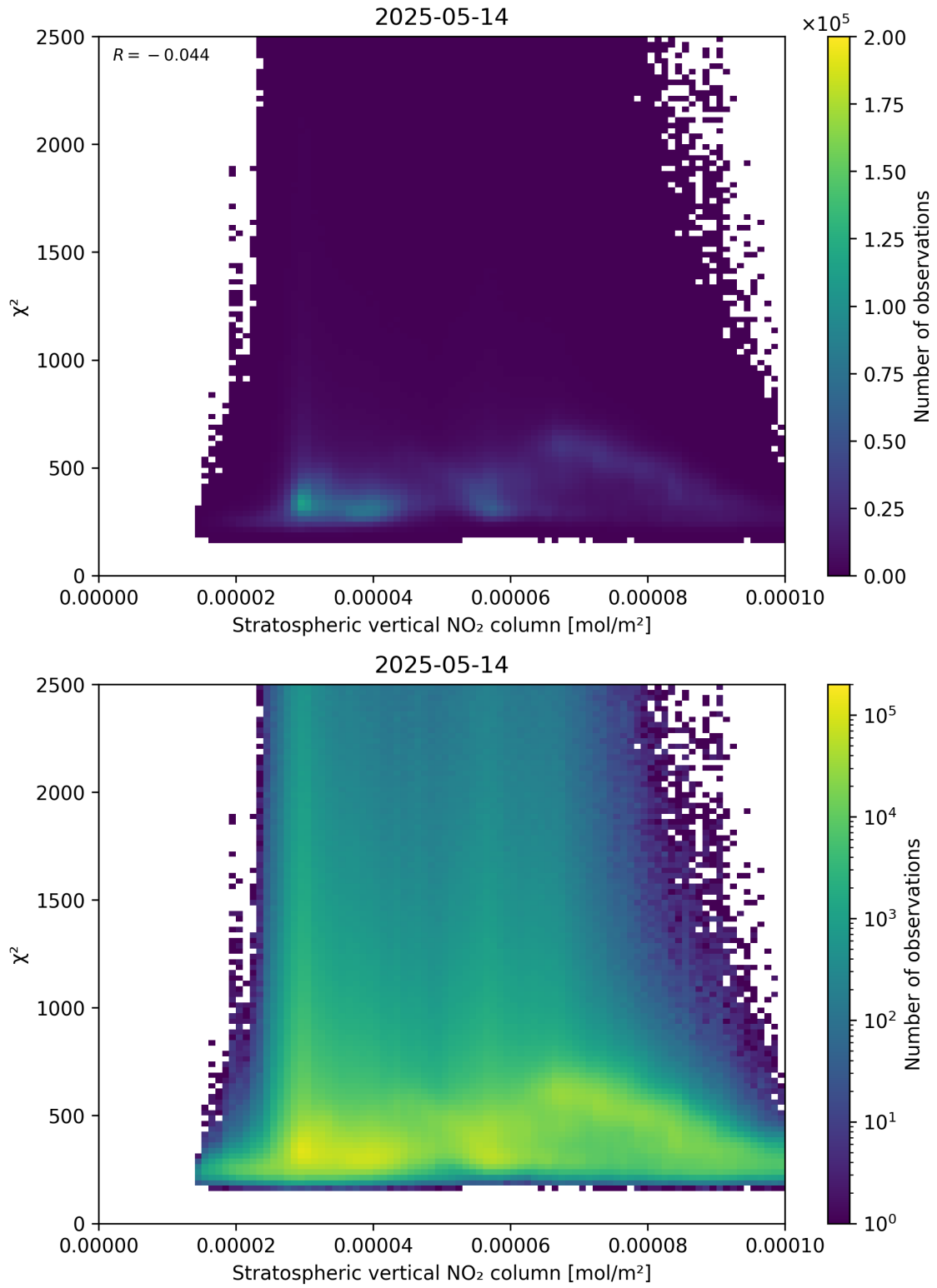
Figure 97: Scatter density plot of “Stratospheric vertical NO 2 column” against “ \chi^2 ” for 2025-05-13 to 2025-05-15.
