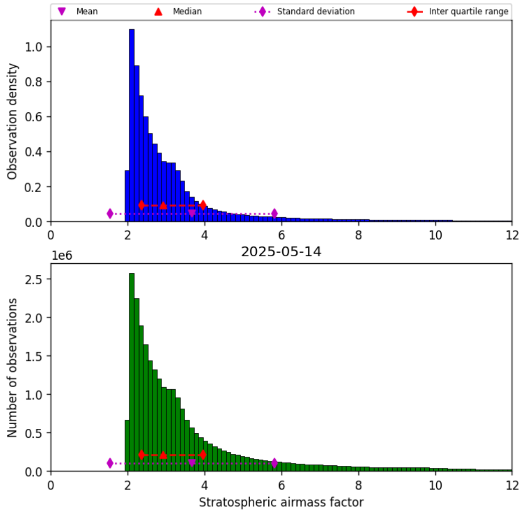
Figure 44: Histogram of “Stratospheric airmass factor” for 2025-05-13 to 2025-05-15
