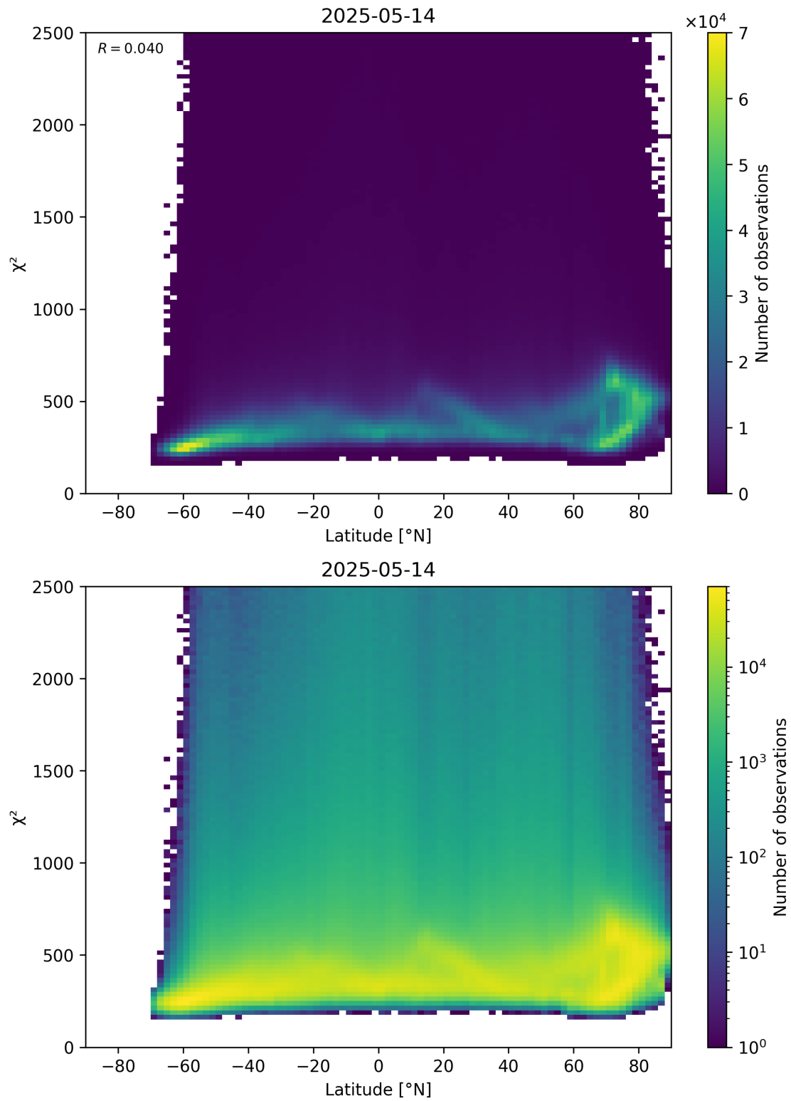
Figure 86: Scatter density plot of “Latitude” against “ \chi^2 ” for 2025-05-13 to 2025-05-15.
