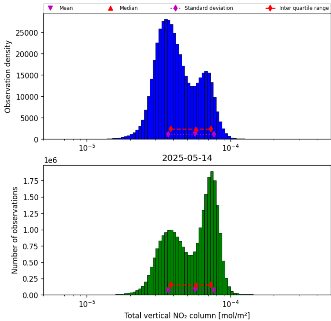
Figure 38: Histogram of “Total vertical NO 2 column” for 2025-05-13 to 2025-05-15
