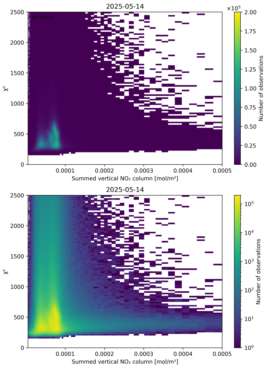
Figure 104: Scatter density plot of “Summed vertical NO 2 column” against “ \chi^2 ” for 2025-05-13 to 2025-05-15.
