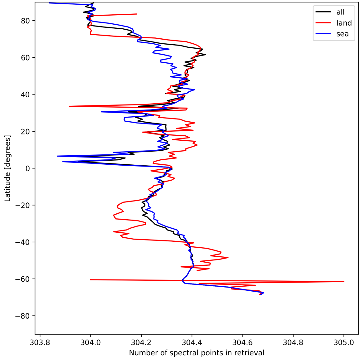
Figure 16: Zonal average of “Number of spectral points in retrieval” for 2025-05-13 to 2025-05-15.
