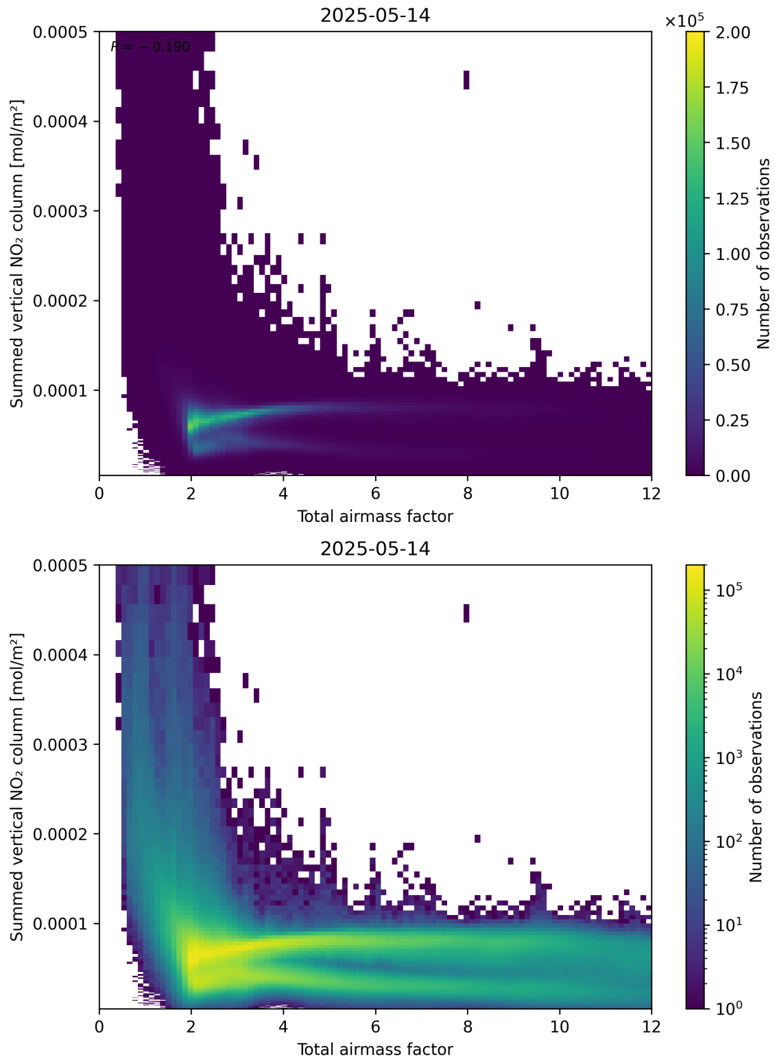
Figure 65: Scatter density plot of “Total airmass factor” against “Summed vertical NO 2 column” for 2025-05-13 to 2025-05-15.
