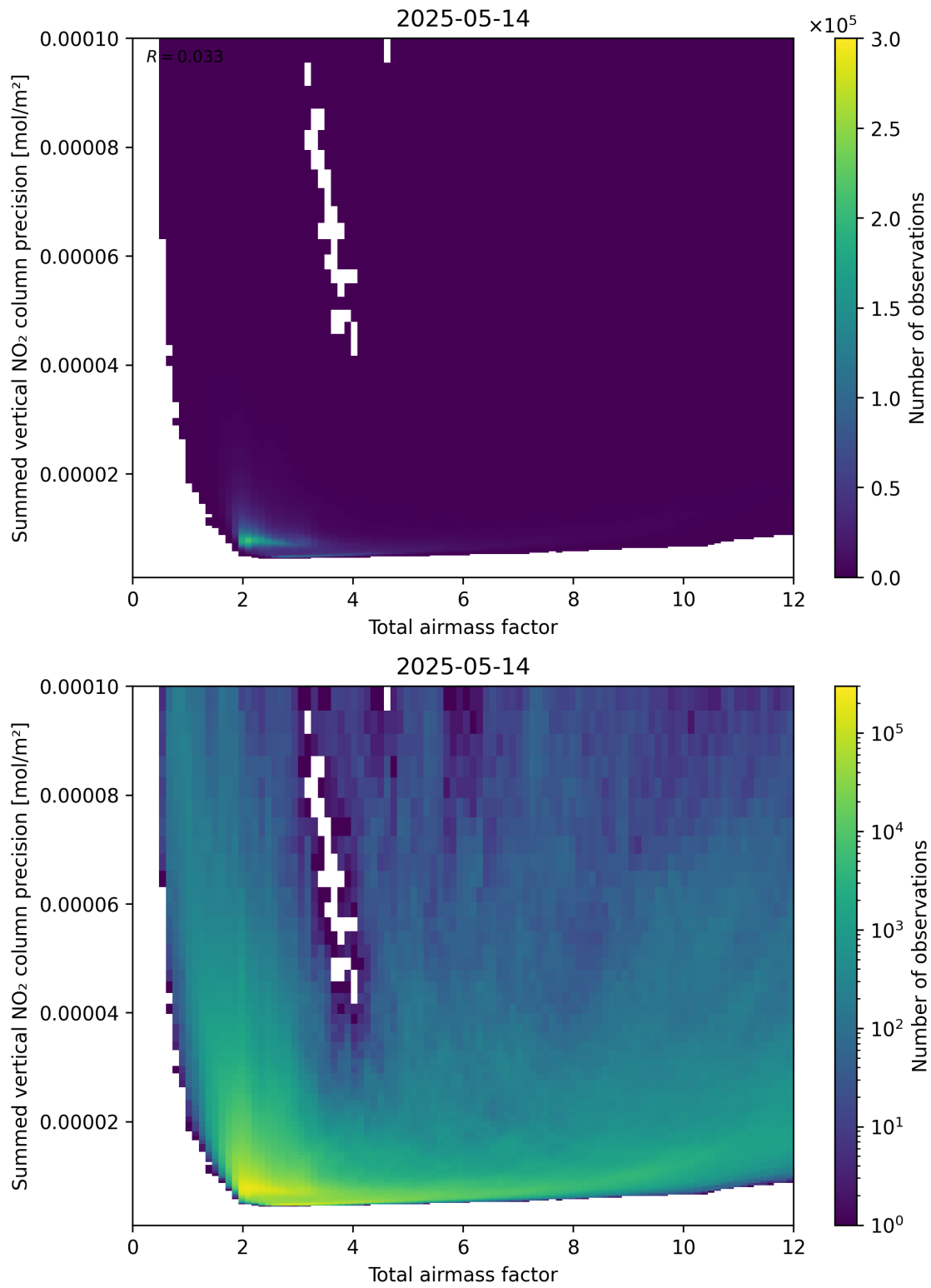
Figure 66: Scatter density plot of “Total airmass factor” against “Summed vertical NO 2 column precision” for 2025-05-13 to 2025-05-15.
