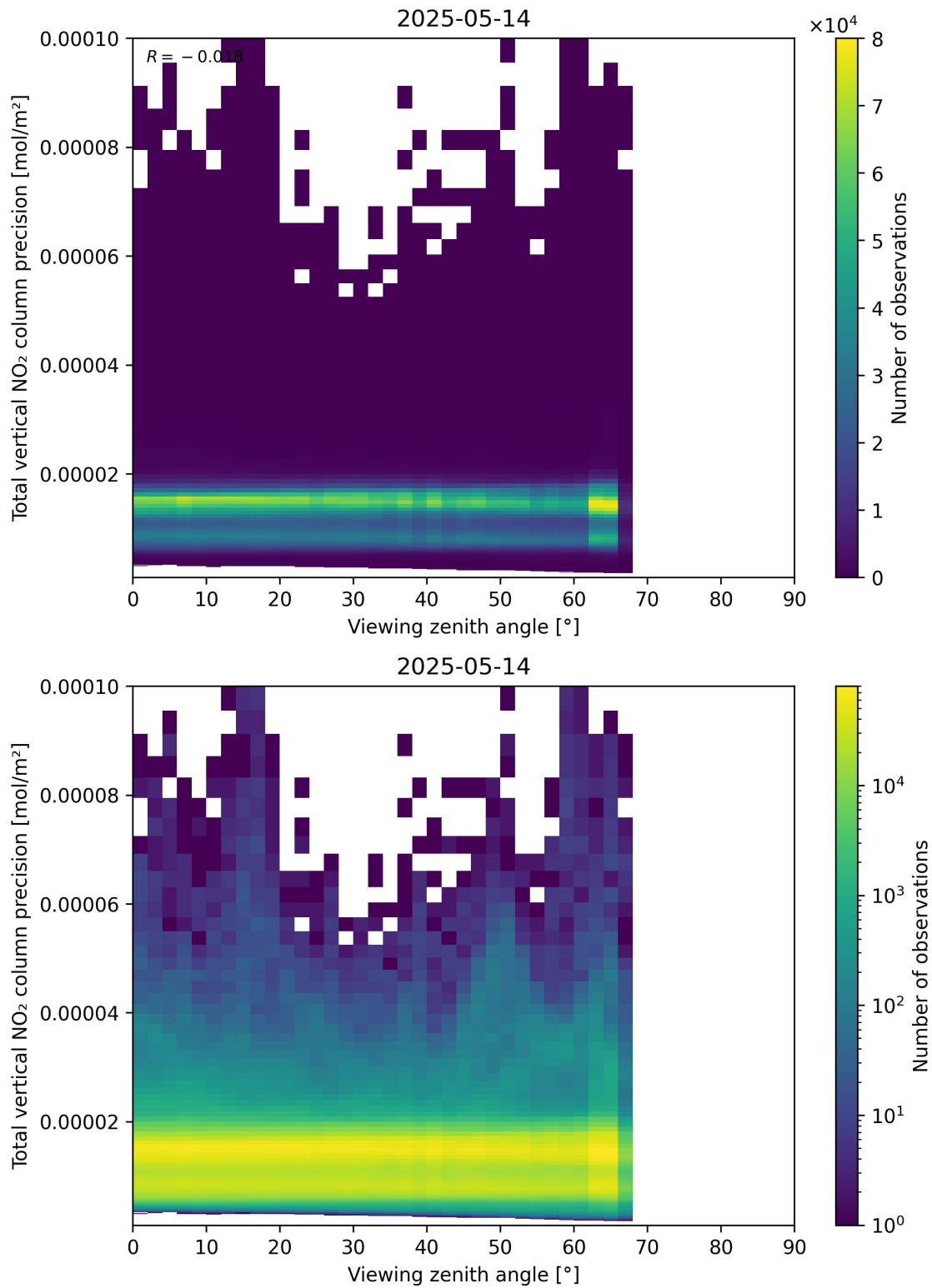
Figure 168: Scatter density plot of “Viewing zenith angle” against “Total vertical NO 2 column precision” for 2025-05-13 to 2025-05-15.
