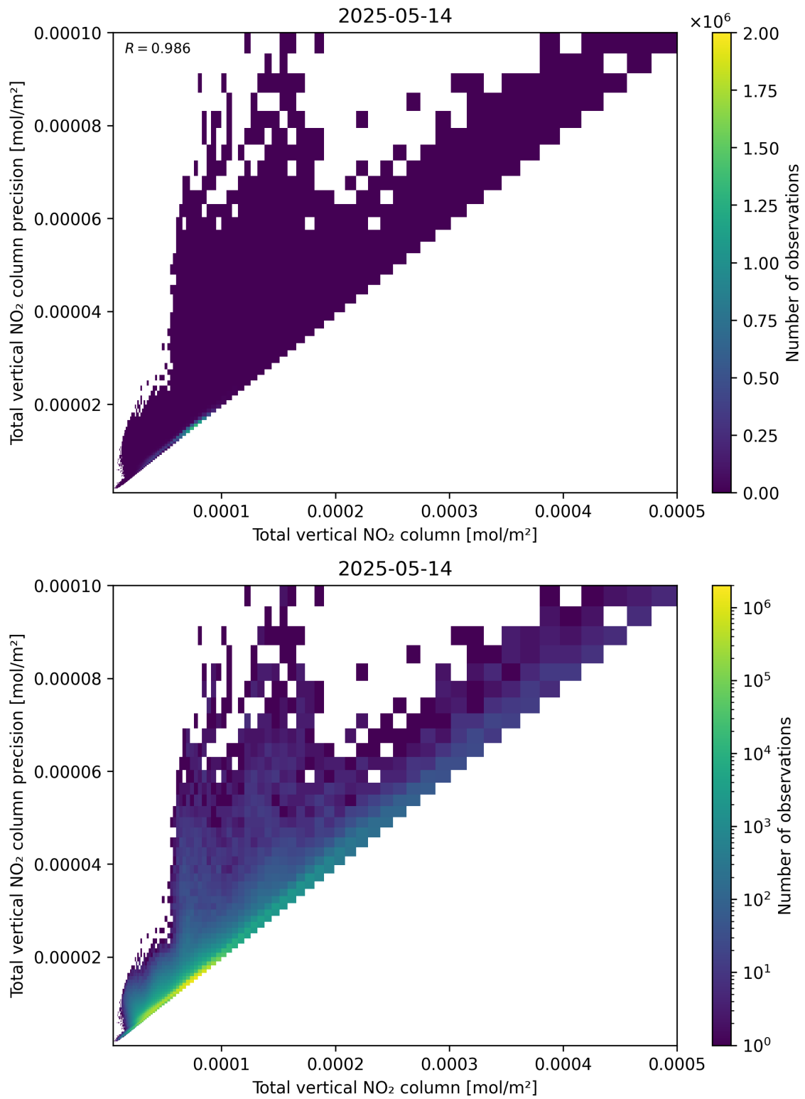
Figure 114: Scatter density plot of “Total vertical NO 2 column” against “Total vertical NO 2 column precision” for 2025-05-13 to 2025-05-15.
