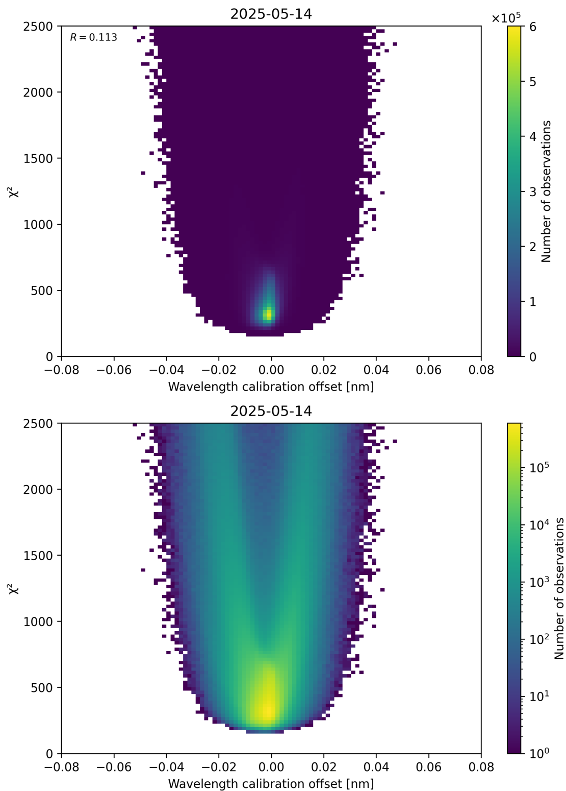
Figure 175: Scatter density plot of “Wavelength calibration offset” against “ \chi^2 ” for 2025-05-13 to 2025-05-15.
