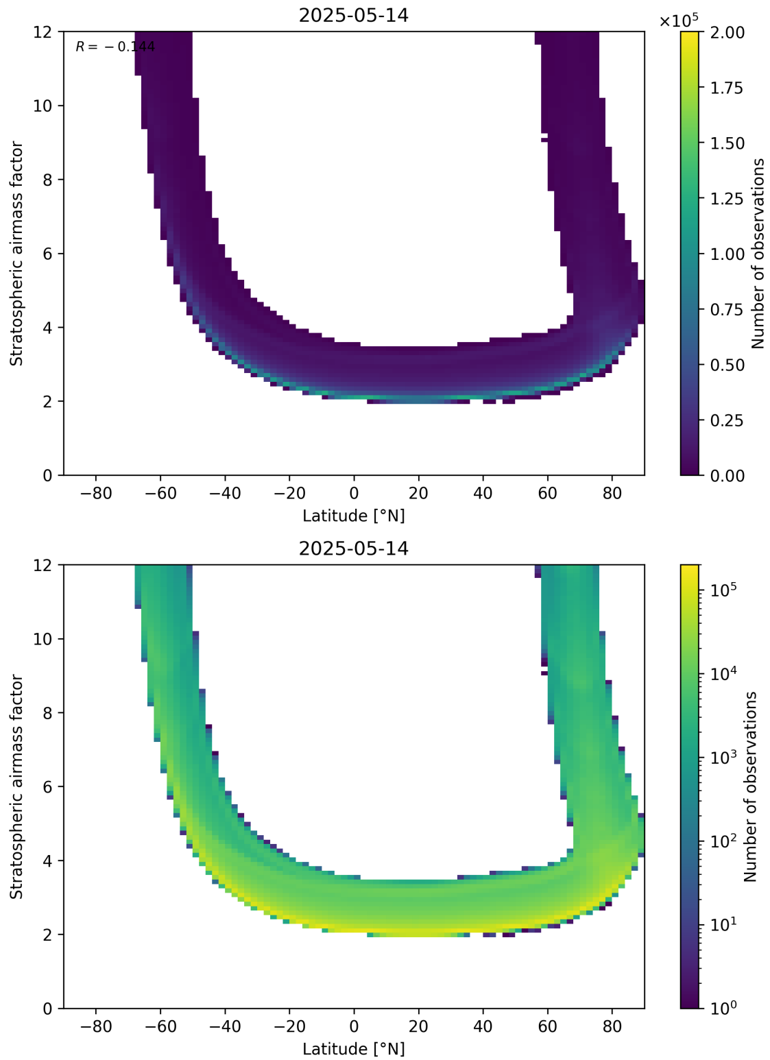
Figure 83: Scatter density plot of “Latitude” against “Stratospheric air mass factor” for 2025-05-13 to 2025-05-15.
