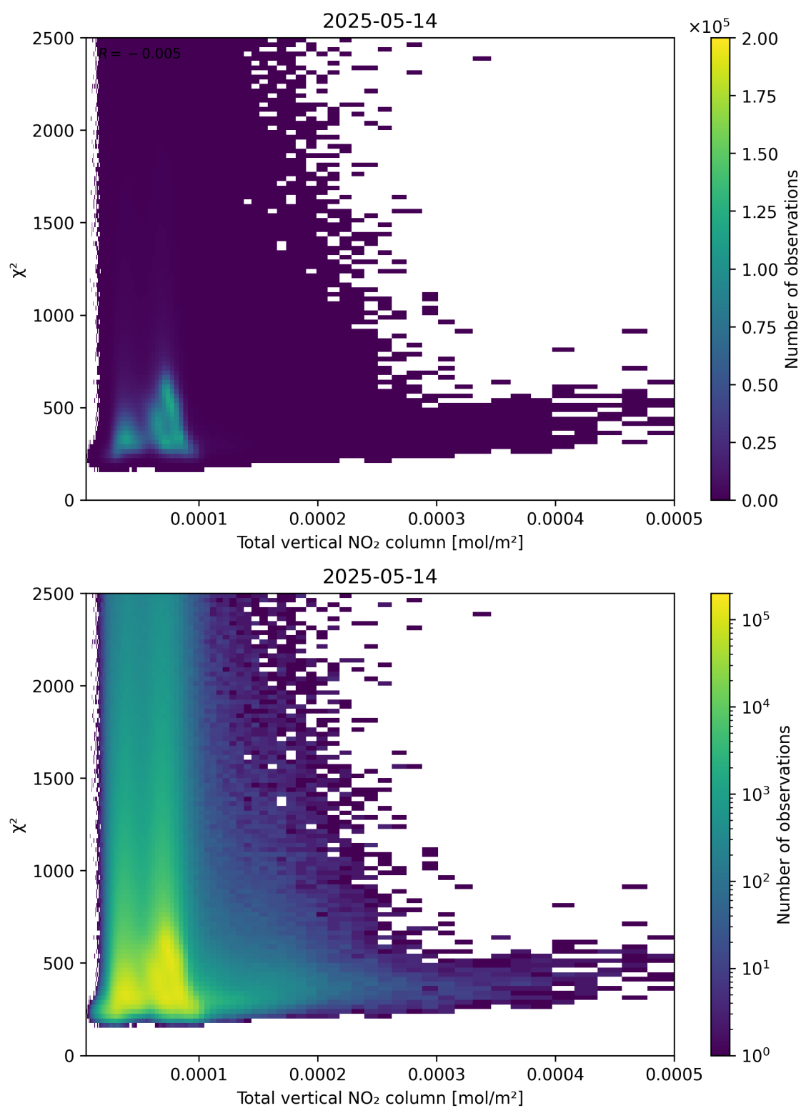
Figure 111: Scatter density plot of “Total vertical NO 2 column” against “ \chi^2 ” for 2025-05-13 to 2025-05-15.
