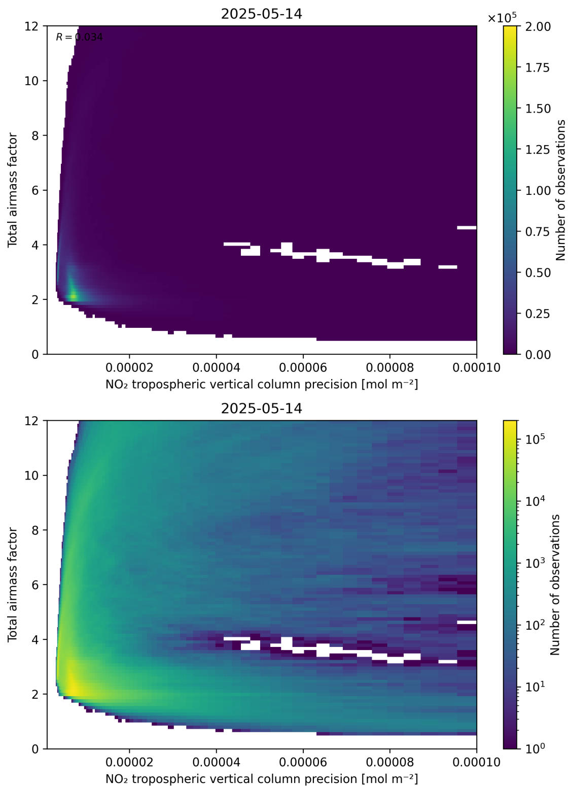
Figure 132: Scatter density plot of “NO 2 tropospheric vertical column precision” against “Total airmass factor” for 2025-05-13 to 2025-05-15.
