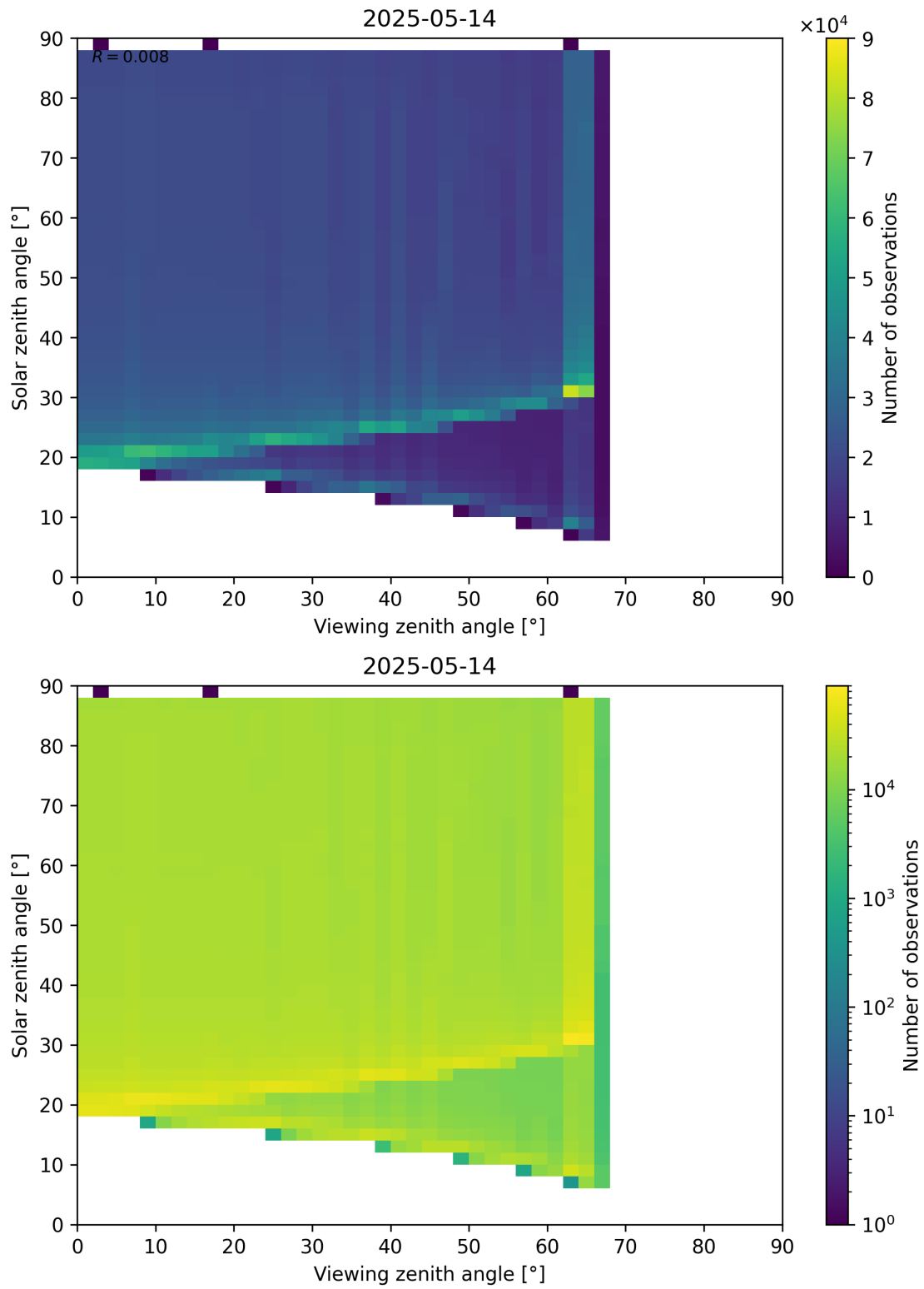
Figure 172: Scatter density plot of “Viewing zenith angle” against “Solar zenith angle” for 2025-05-13 to 2025-05-15.
