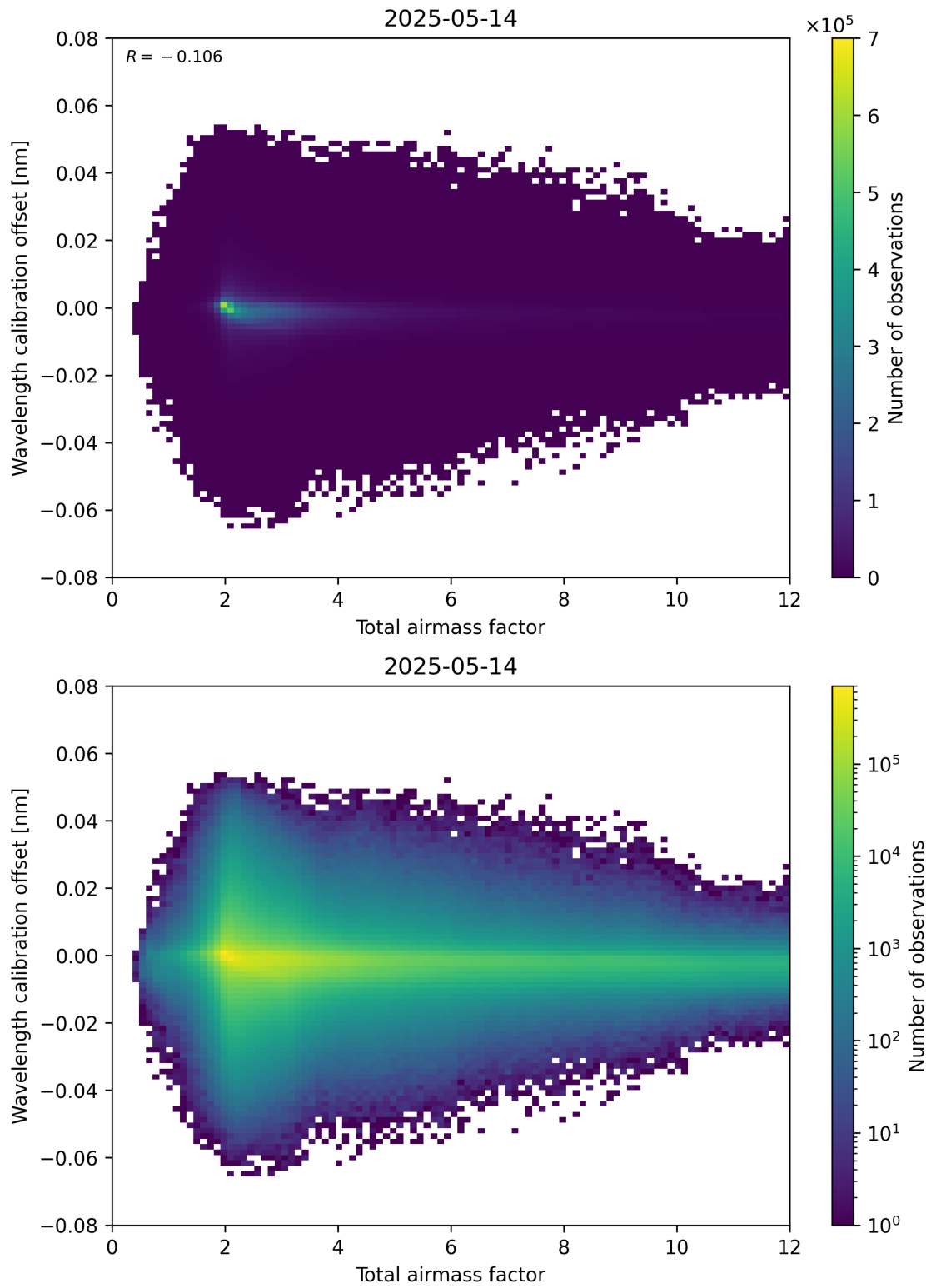
Figure 70: Scatter density plot of “Total airmass factor” against “Wavelength calibration offset” for 2025-05-13 to 2025-05-15.
