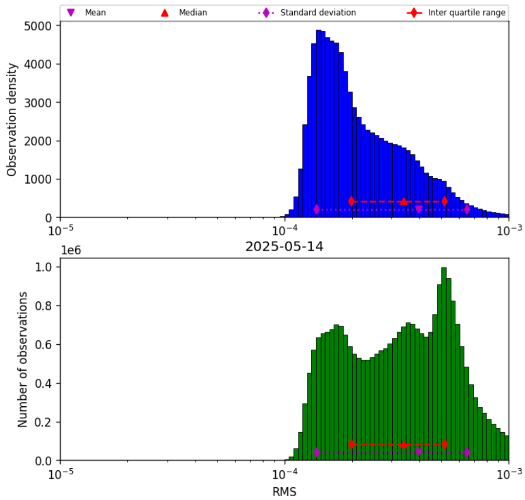
Figure 43: Histogram of “RMS” for 2025-05-13 to 2025-05-15
