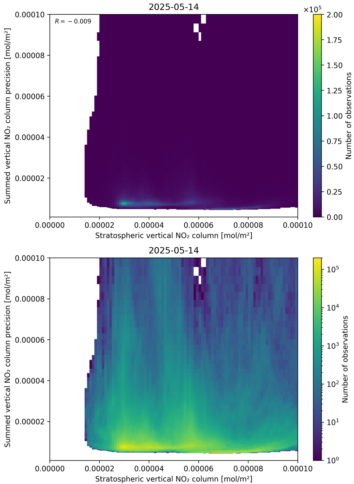
Figure 99: Scatter density plot of “Stratospheric vertical NO 2 column” against “Summed vertical NO 2 column precision” for 2025-05-13 to 2025-05-15.
