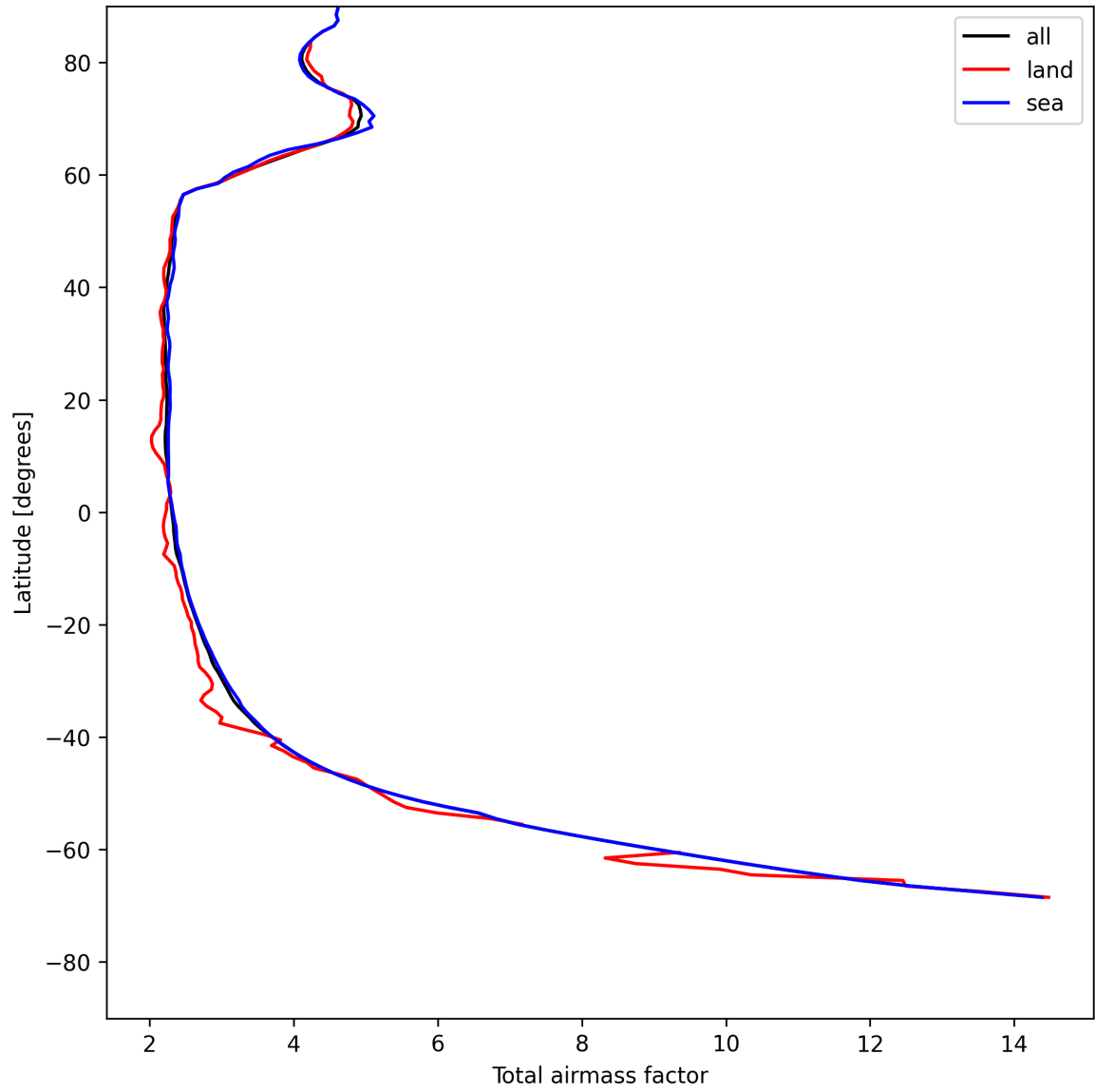
Figure 15: Zonal average of “Total airmass factor” for 2025-05-13 to 2025-05-15.
