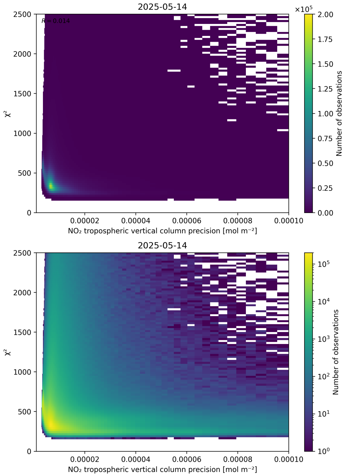
Figure 134: Scatter density plot of “NO 2 tropospheric vertical column precision” against “ \chi^2 ” for 2025-05-13 to 2025-05-15.
