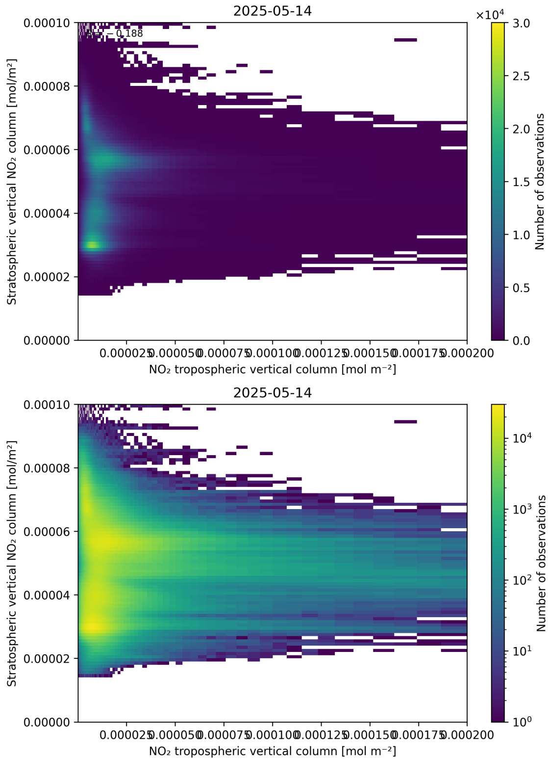
Figure 125: Scatter density plot of “NO 2 tropospheric vertical column” against “Stratospheric vertical NO 2 column” for 2025-05-13 to 2025-05-15.
