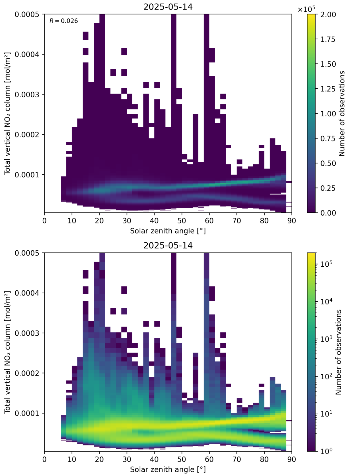
Figure 153: Scatter density plot of “Solar zenith angle” against “Total vertical NO 2 column” for 2025-05-13 to 2025-05-15.
