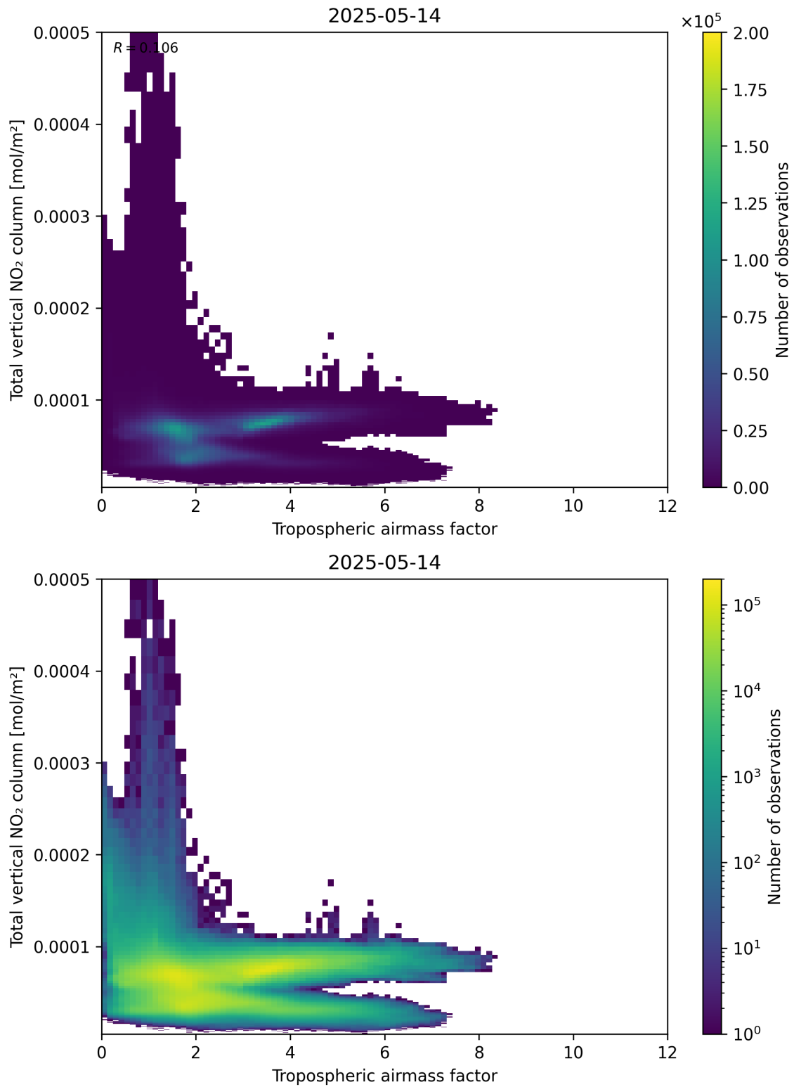
Figure 77: Scatter density plot of “Tropospheric airmass factor” against “Total vertical NO 2 column” for 2025-05-13 to 2025-05-15.
