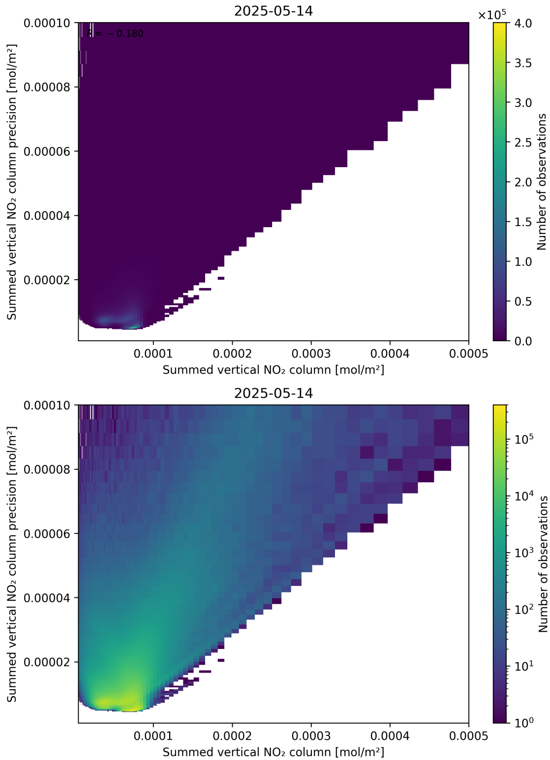
Figure 105: Scatter density plot of “Summed vertical NO 2 column” against “Summed vertical NO 2 column precision” for 2025-05-13 to 2025-05-15.
