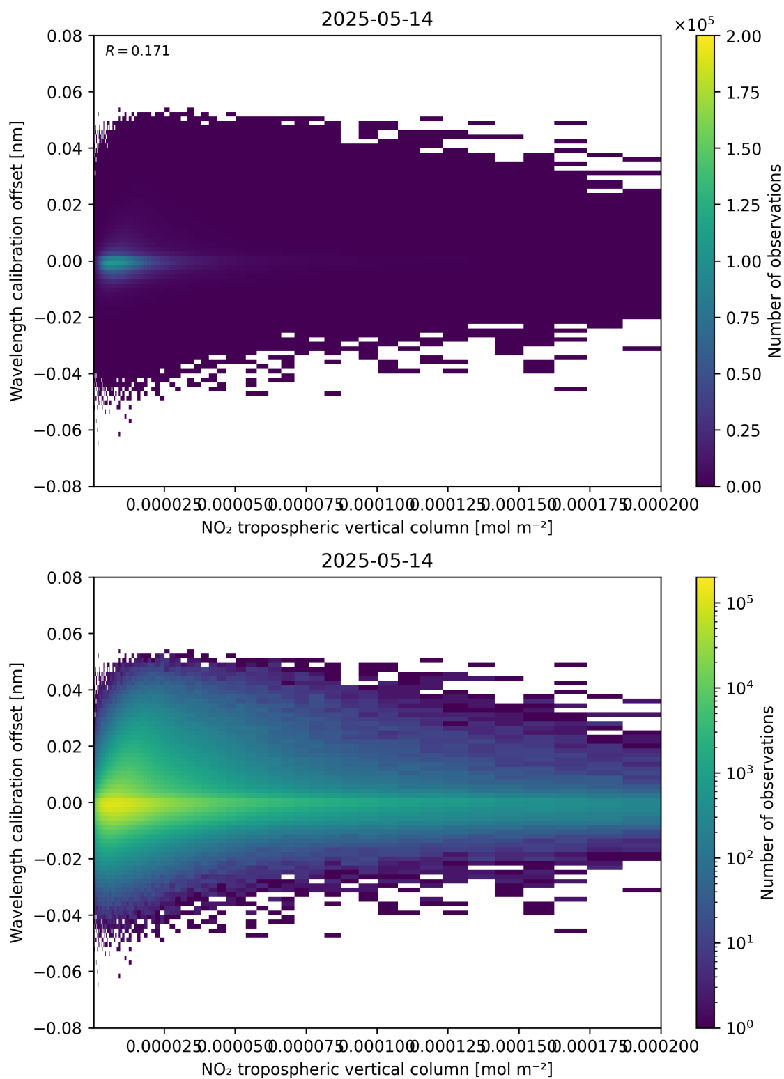
Figure 143: Scatter density plot of “NO 2 tropospheric vertical column” against “Wavelength calibration offset” for 2025-05-13 to 2025-05-15.
