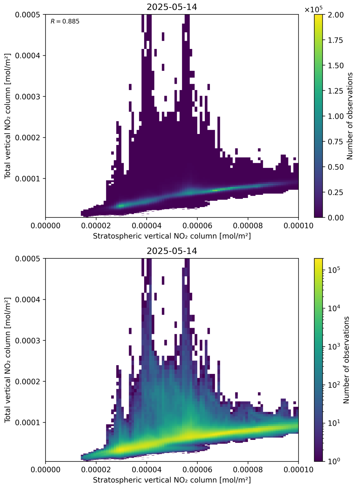
Figure 100: Scatter density plot of “Stratospheric vertical NO 2 column” against “Total vertical NO 2 column” for 2025-05-13 to 2025-05-15.
