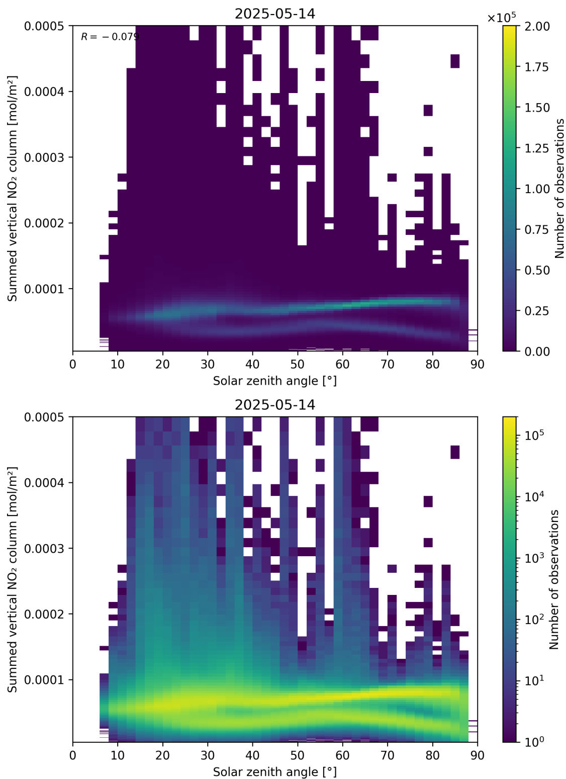
Figure 151: Scatter density plot of “Solar zenith angle” against “Summed vertical NO 2 column” for 2025-05-13 to 2025-05-15.
