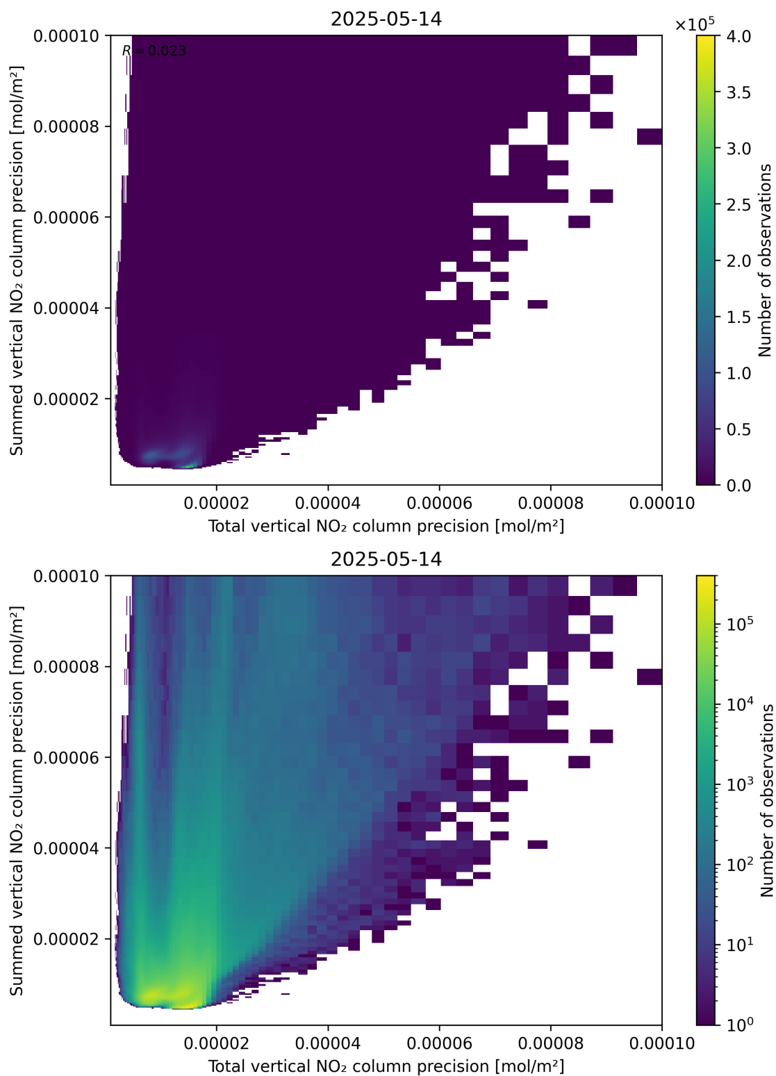
Figure 118: Scatter density plot of “Total vertical NO 2 column precision” against “Summed vertical NO 2 column precision” for 2025-05-13 to 2025-05-15.
