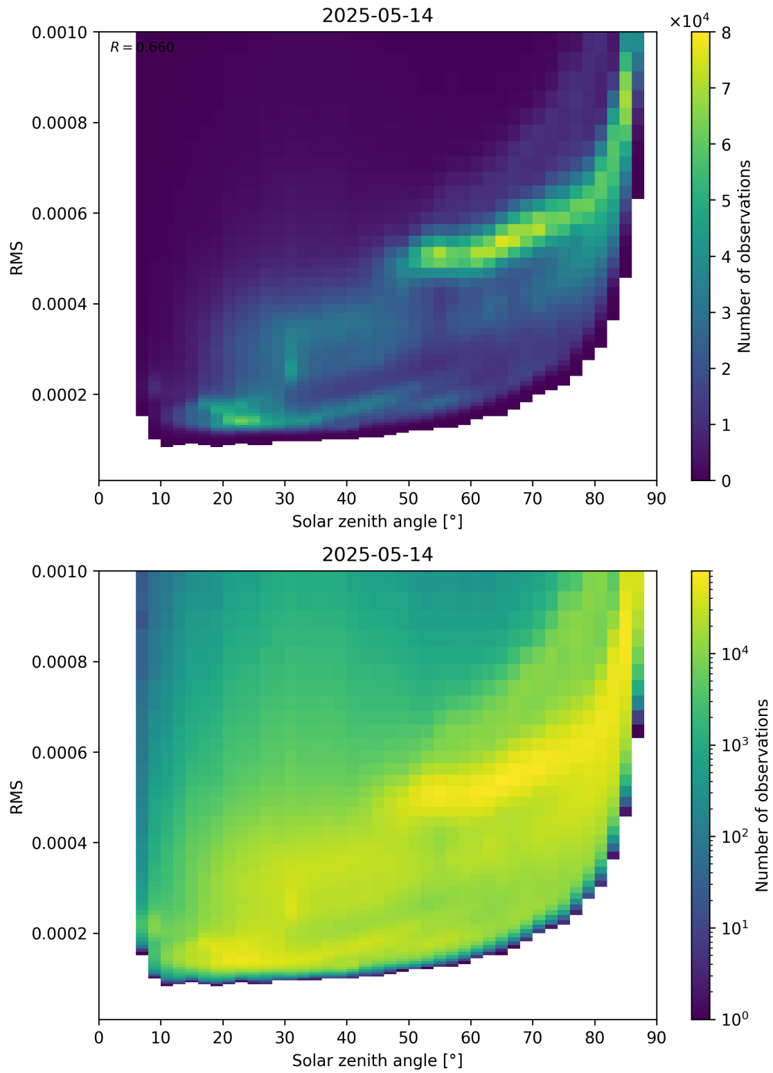
Figure 157: Scatter density plot of “Solar zenith angle” against “RMS” for 2025-05-13 to 2025-05-15.
