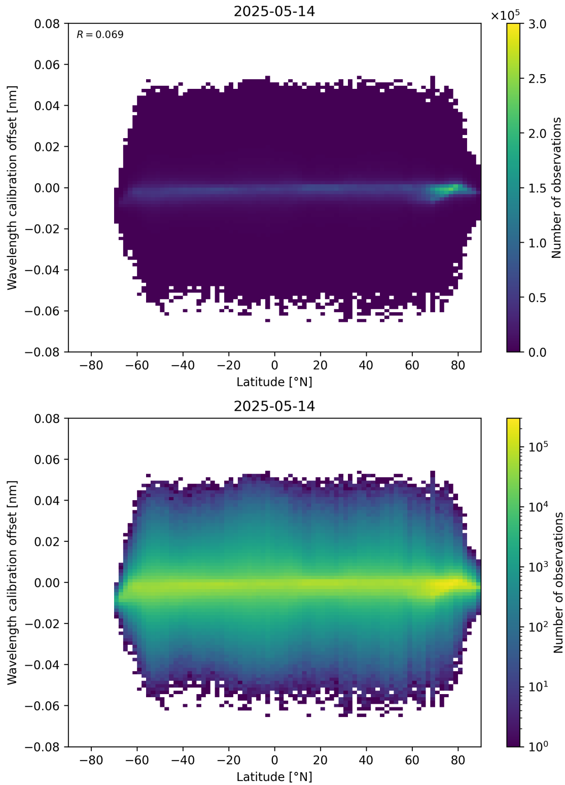
Figure 95: Scatter density plot of “Latitude” against “Wavelength calibration offset” for 2025-05-13 to 2025-05-15.
