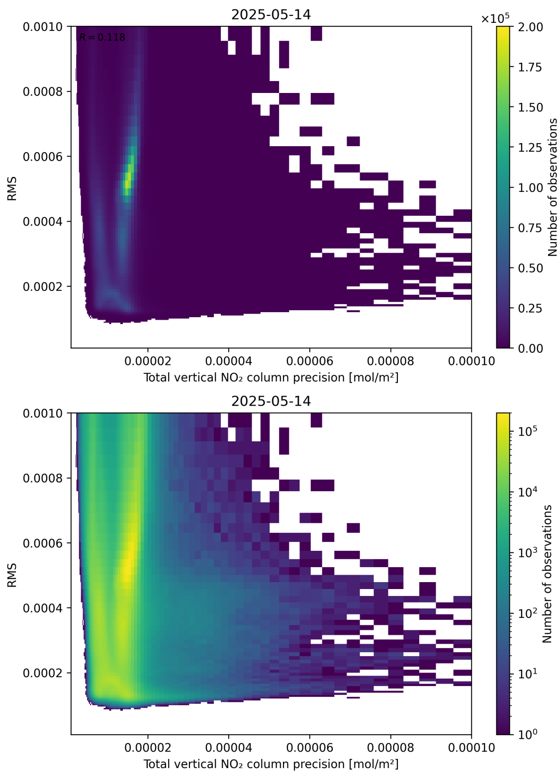
Figure 119: Scatter density plot of “Total vertical NO 2 column precision” against “RMS” for 2025-05-13 to 2025-05-15.
