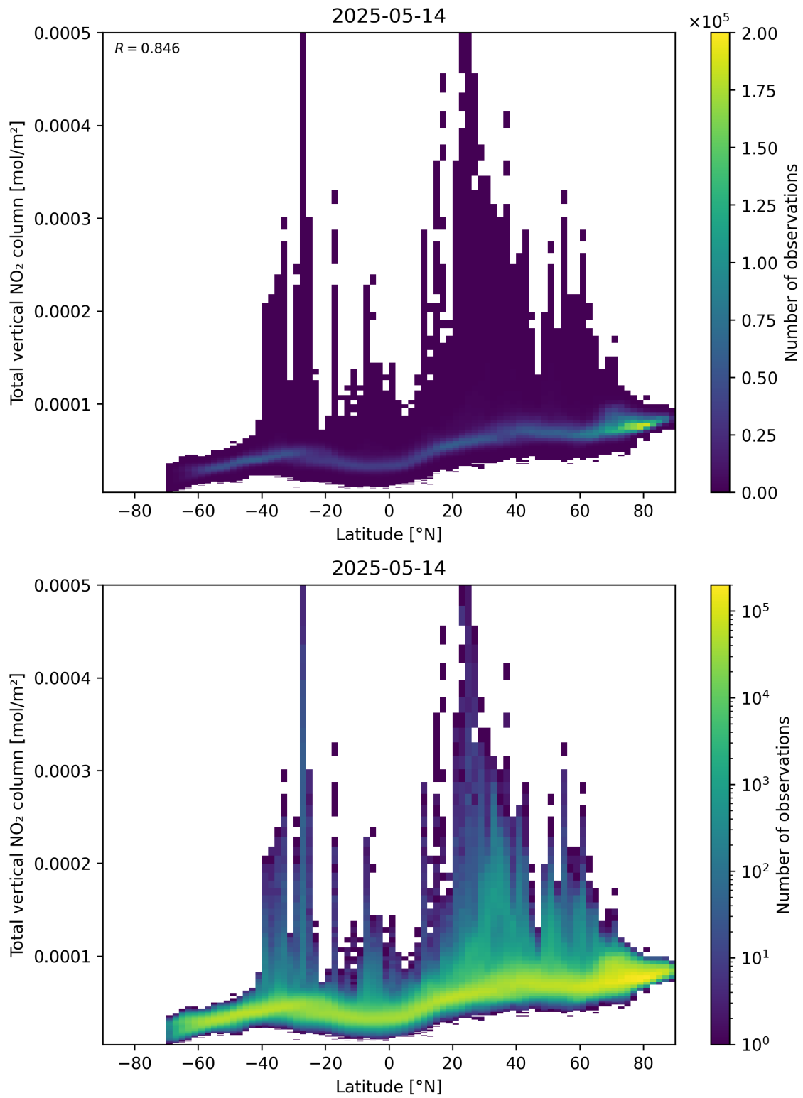
Figure 90: Scatter density plot of “Latitude” against “Total vertical NO 2 column” for 2025-05-13 to 2025-05-15.
