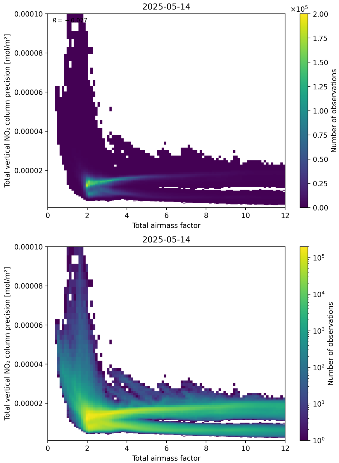
Figure 68: Scatter density plot of “Total airmass factor” against “Total vertical NO 2 column precision” for 2025-05-13 to 2025-05-15.
