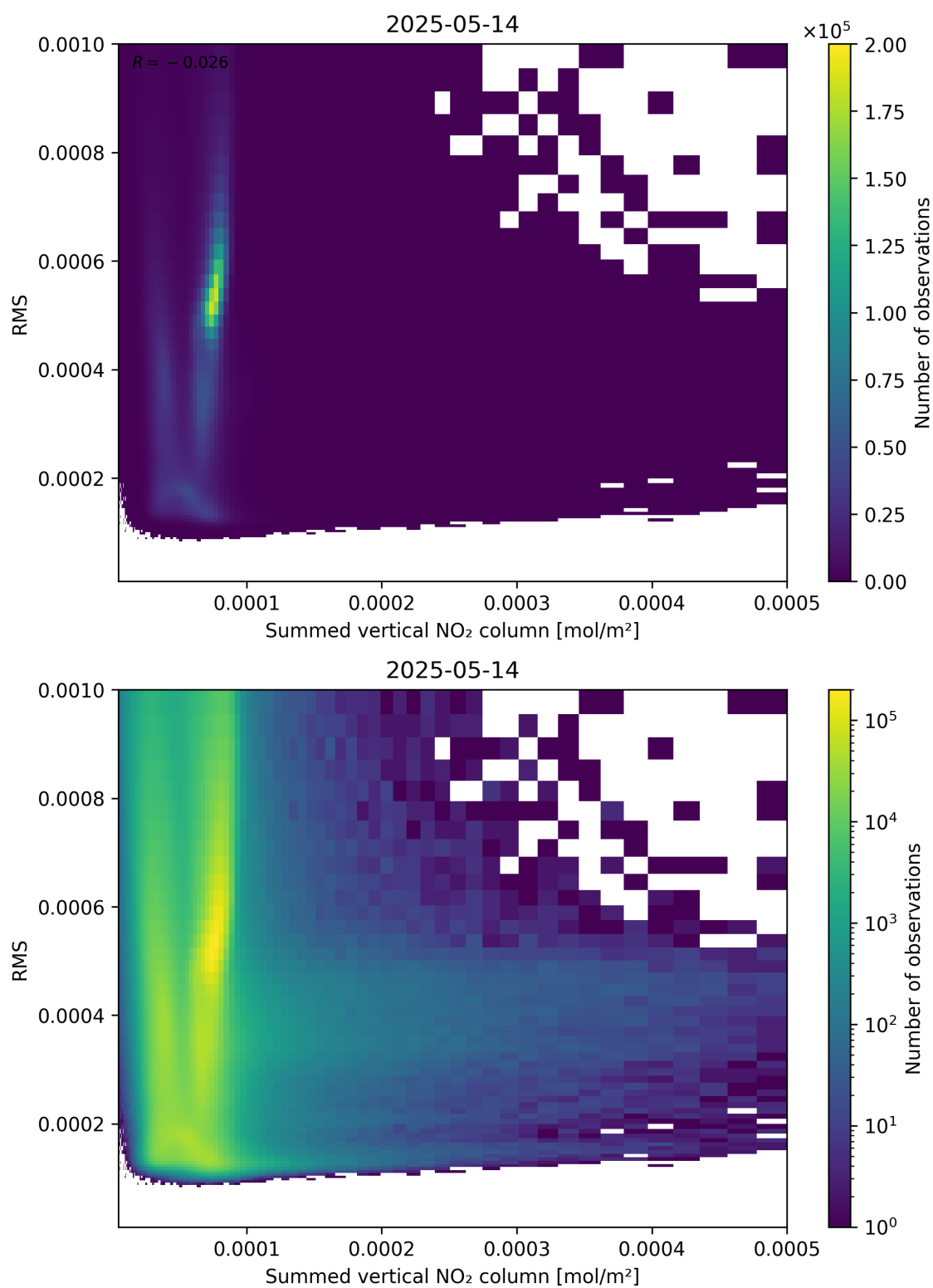
Figure 109: Scatter density plot of “Summed vertical NO 2 column” against “RMS” for 2025-05-13 to 2025-05-15.
