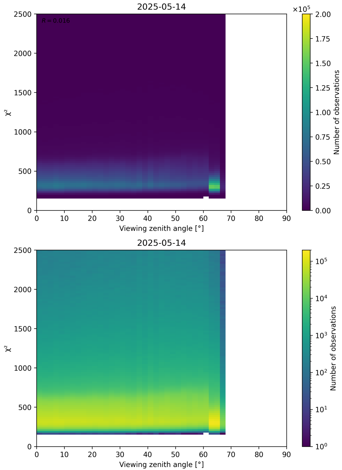
Figure 162: Scatter density plot of “Viewing zenith angle” against “ \chi^2 ” for 2025-05-13 to 2025-05-15.
