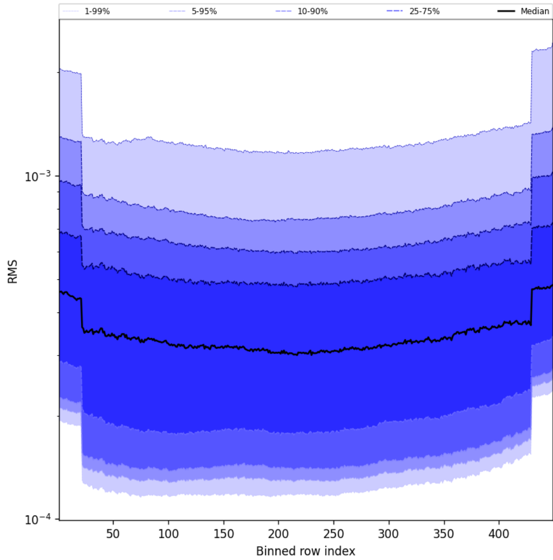
Figure 60: Along track statistics of “RMS” for 2025-05-13 to 2025-05-15
