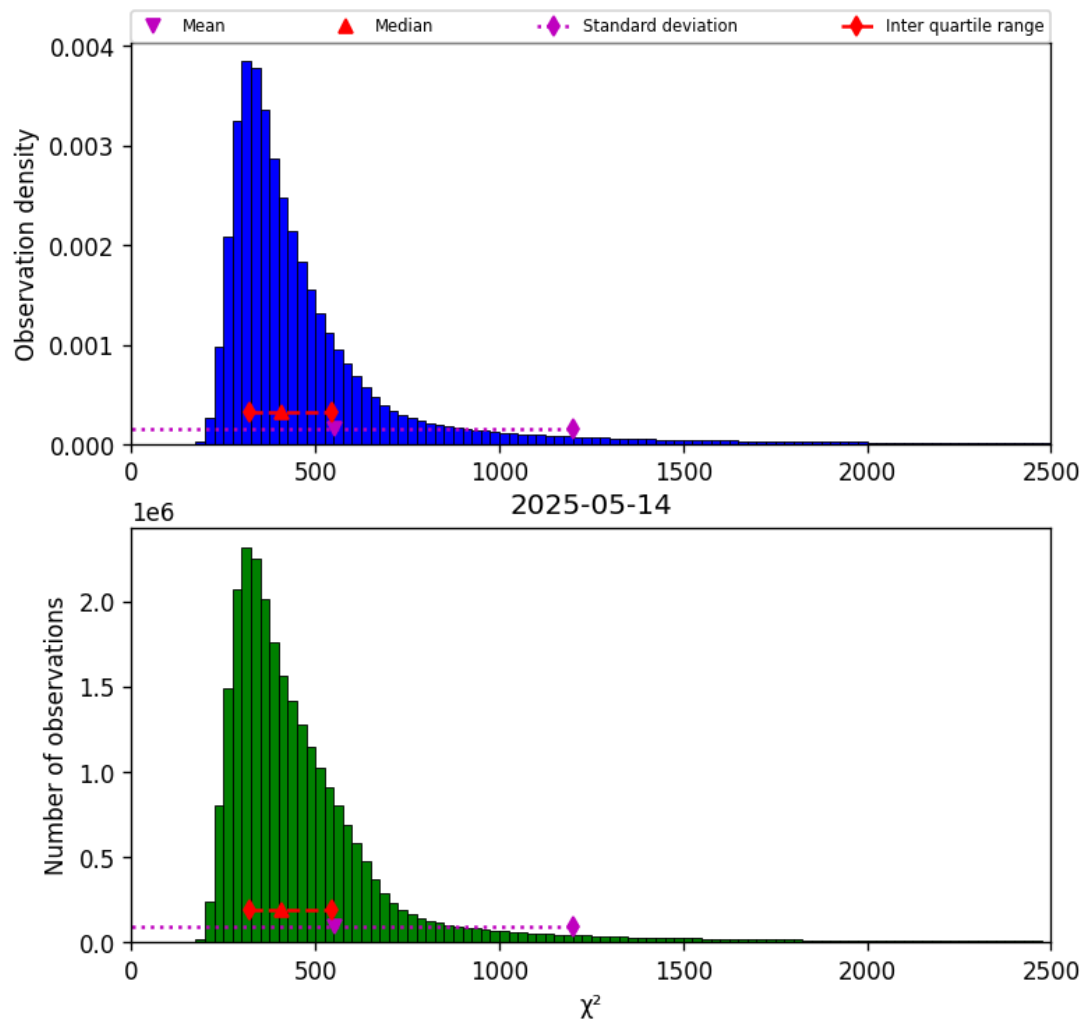
Figure 42: Histogram of “ \chi^2 ” for 2025-05-13 to 2025-05-15
