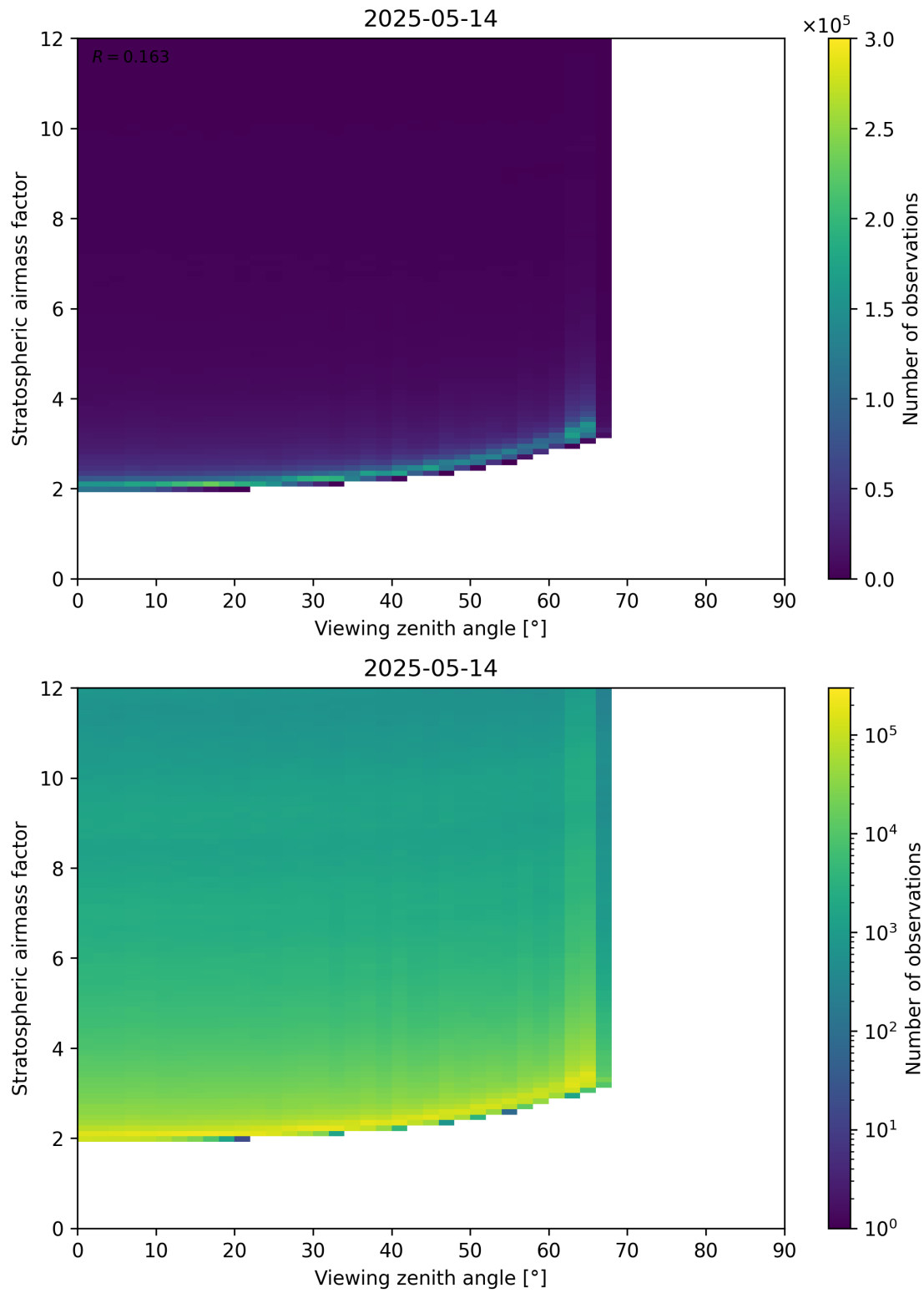
Figure 159: Scatter density plot of “Viewing zenith angle” against “Stratospheric airmass factor” for 2025-05-13 to 2025-05-15.
