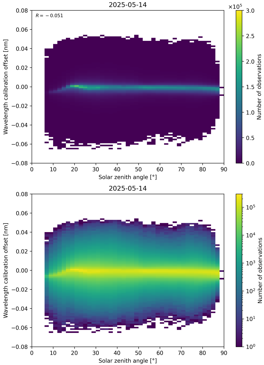
Figure 158: Scatter density plot of “Solar zenith angle” against “Wavelength calibration offset” for 2025-05-13 to 2025-05-15.
