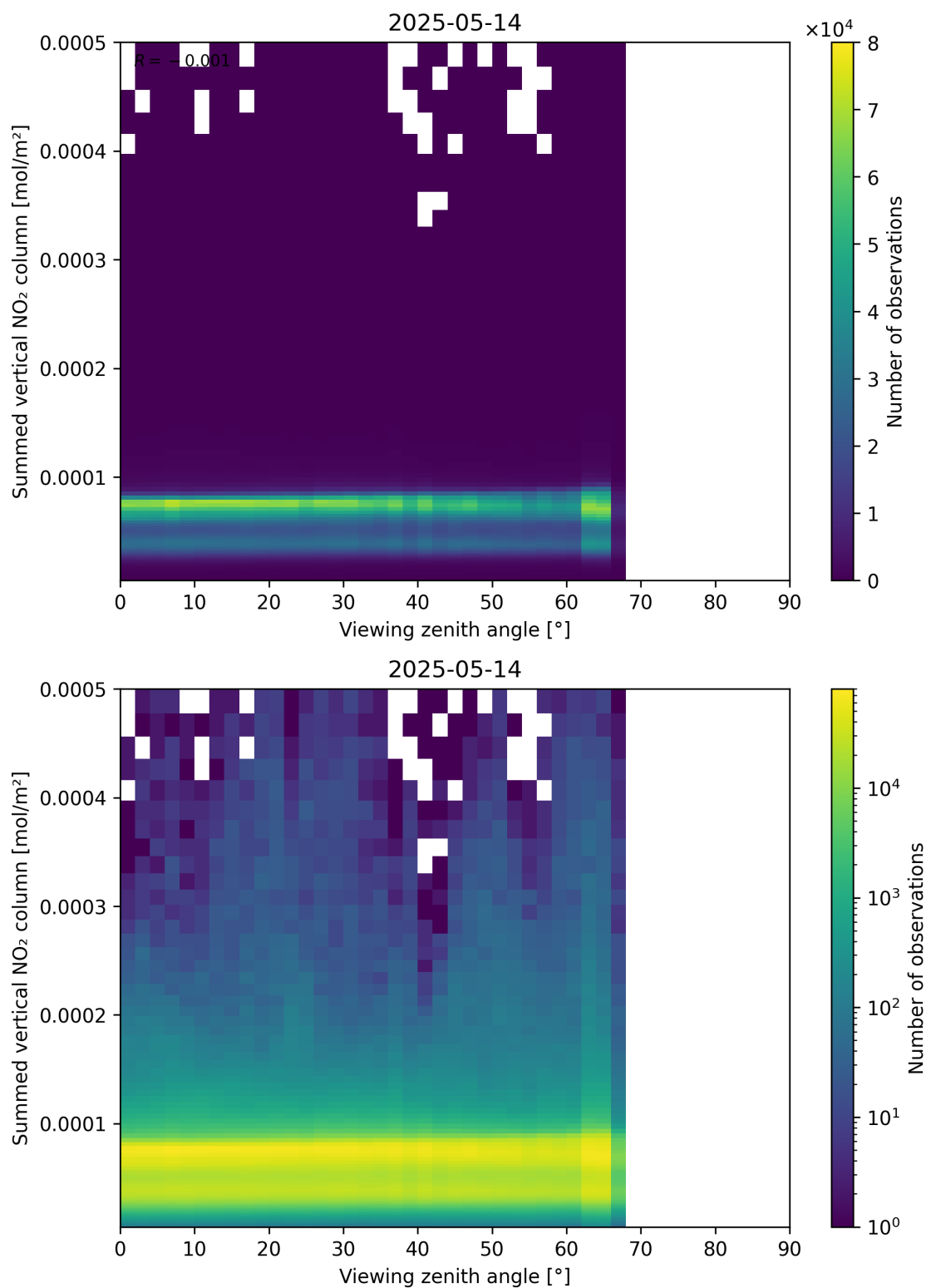
Figure 165: Scatter density plot of “Viewing zenith angle” against “Summed vertical NO 2 column” for 2025-05-13 to 2025-05-15.
