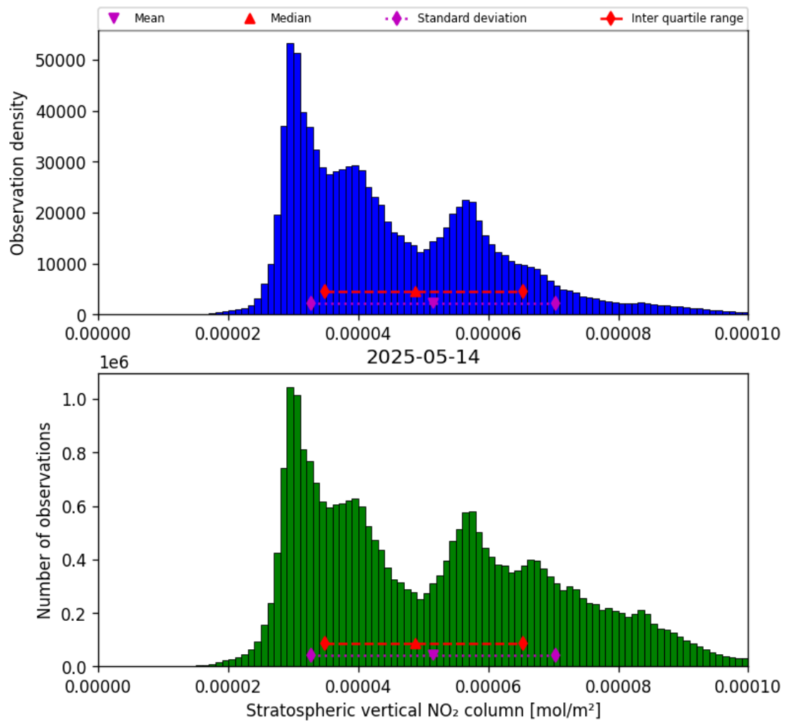
Figure 36: Histogram of “Stratospheric vertical NO 2 column” for 2025-05-13 to 2025-05-15
