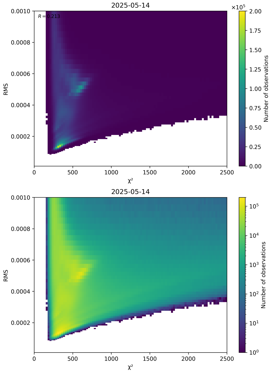
Figure 82: Scatter density plot of “ \chi^2 ” against “RMS” for 2025-05-13 to 2025-05-15.
