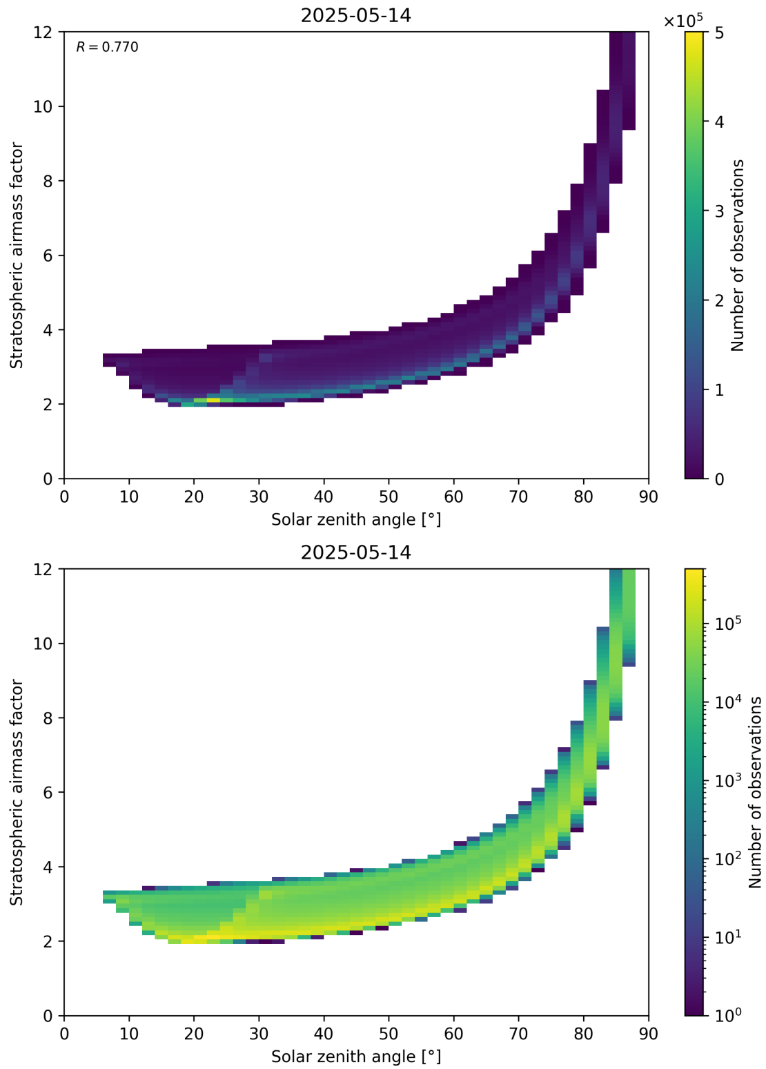
Figure 145: Scatter density plot of “Solar zenith angle” against “Stratospheric airmass factor” for 2025-05-13 to 2025-05-15.
