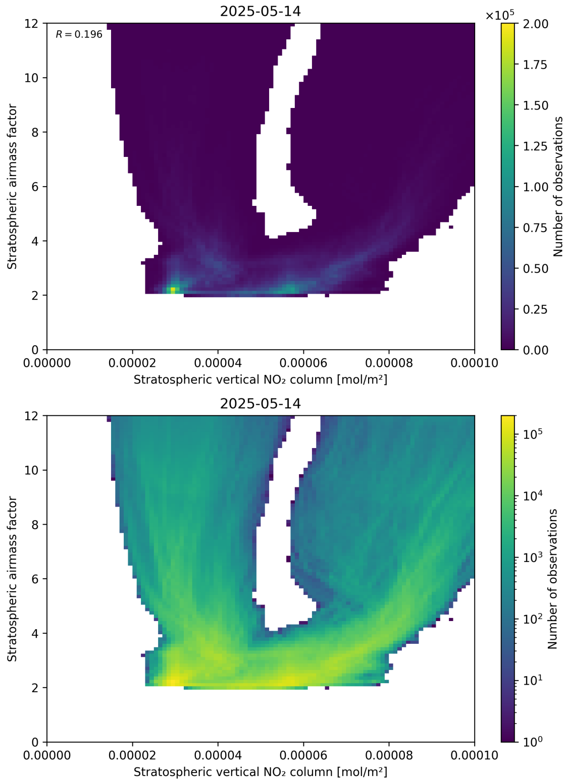
Figure 96: Scatter density plot of “Stratospheric vertical NO 2 column” against “Stratospheric airmass factor” for 2025-05-13 to 2025-05-15.
