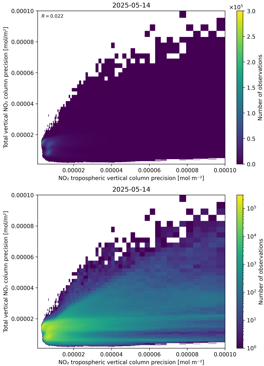
Figure 139: Scatter density plot of “NO 2 tropospheric vertical column precision” against “Total vertical NO 2 column precision” for 2025-05-13 to 2025-05-15.
