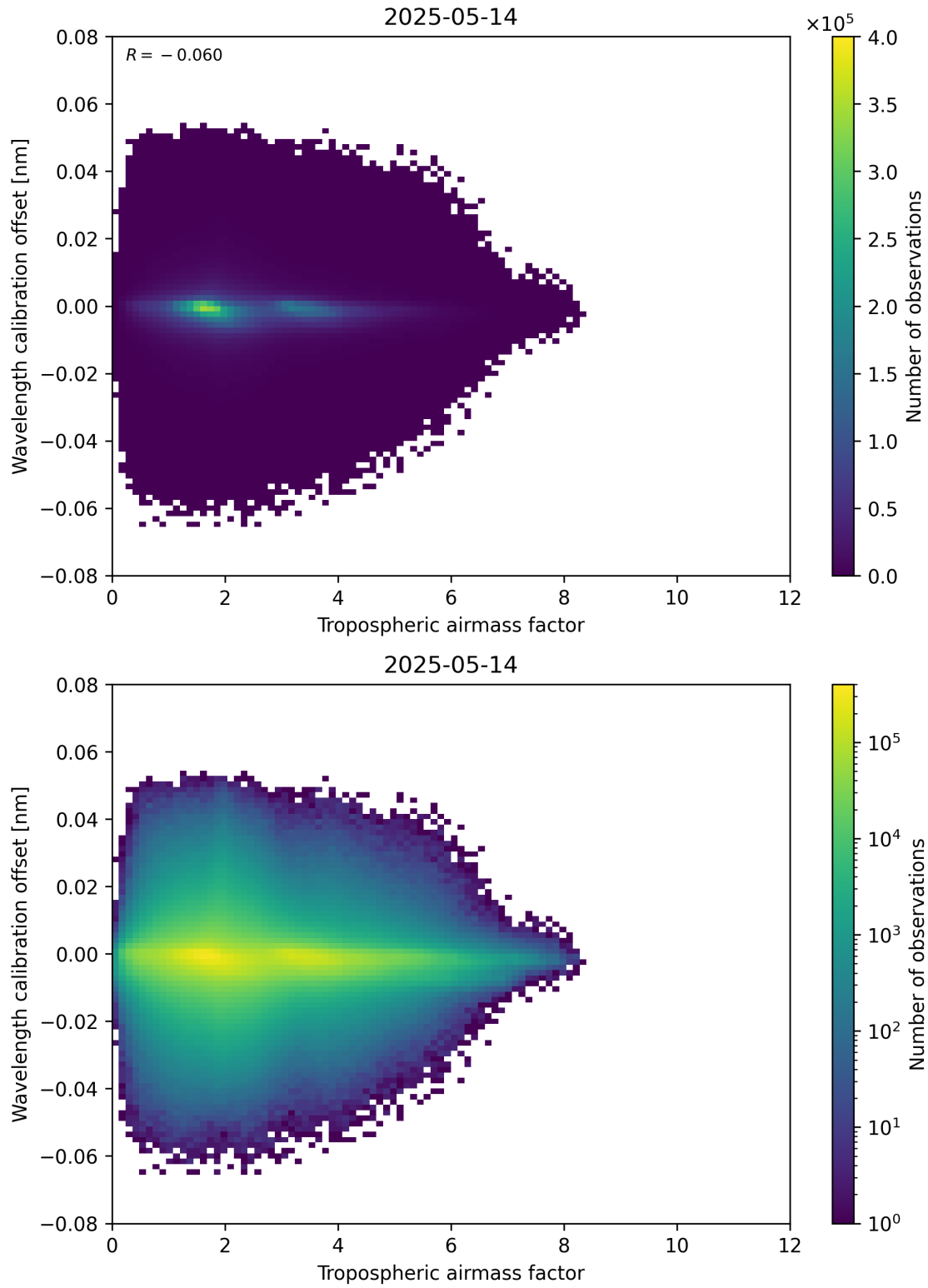
Figure 80: Scatter density plot of “Tropospheric airmass factor” against “Wavelength calibration offset” for 2025-05-13 to 2025-05-15.
