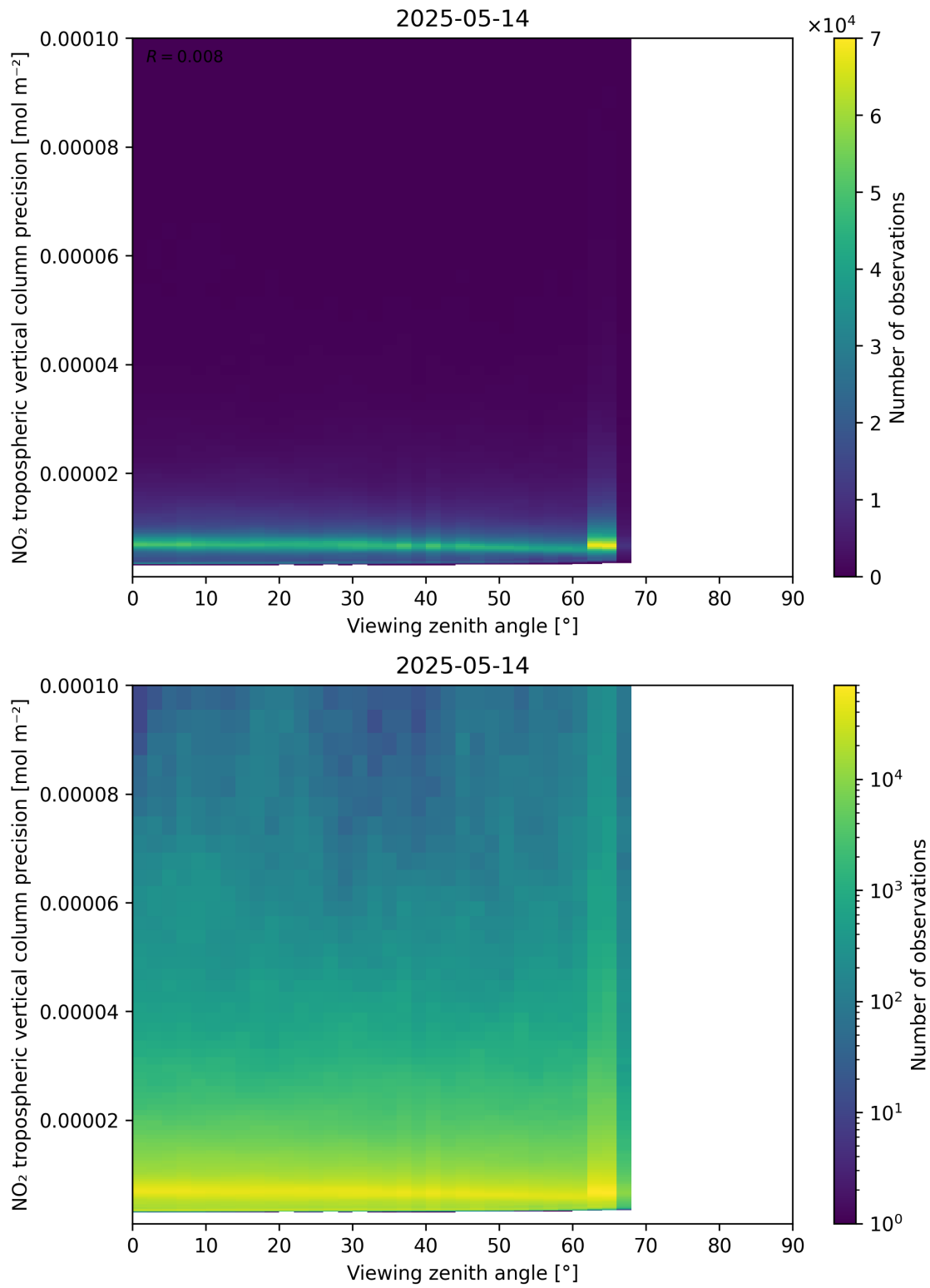
Figure 170: Scatter density plot of “Viewing zenith angle” against “NO 2 tropospheric vertical column precision” for 2025-05-13 to 2025-05-15.
