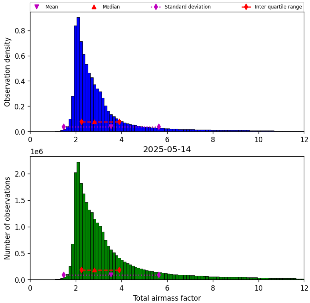
Figure 32: Histogram of “Total airmass factor” for 2025-05-13 to 2025-05-15
