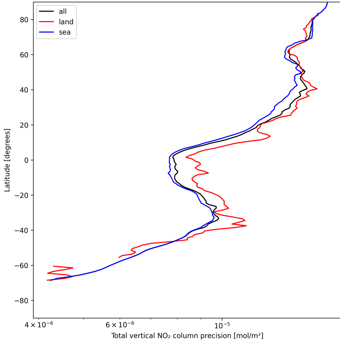
Figure 22: Zonal average of “Total vertical NO 2 column precision” for 2025-05-13 to 2025-05-15.
