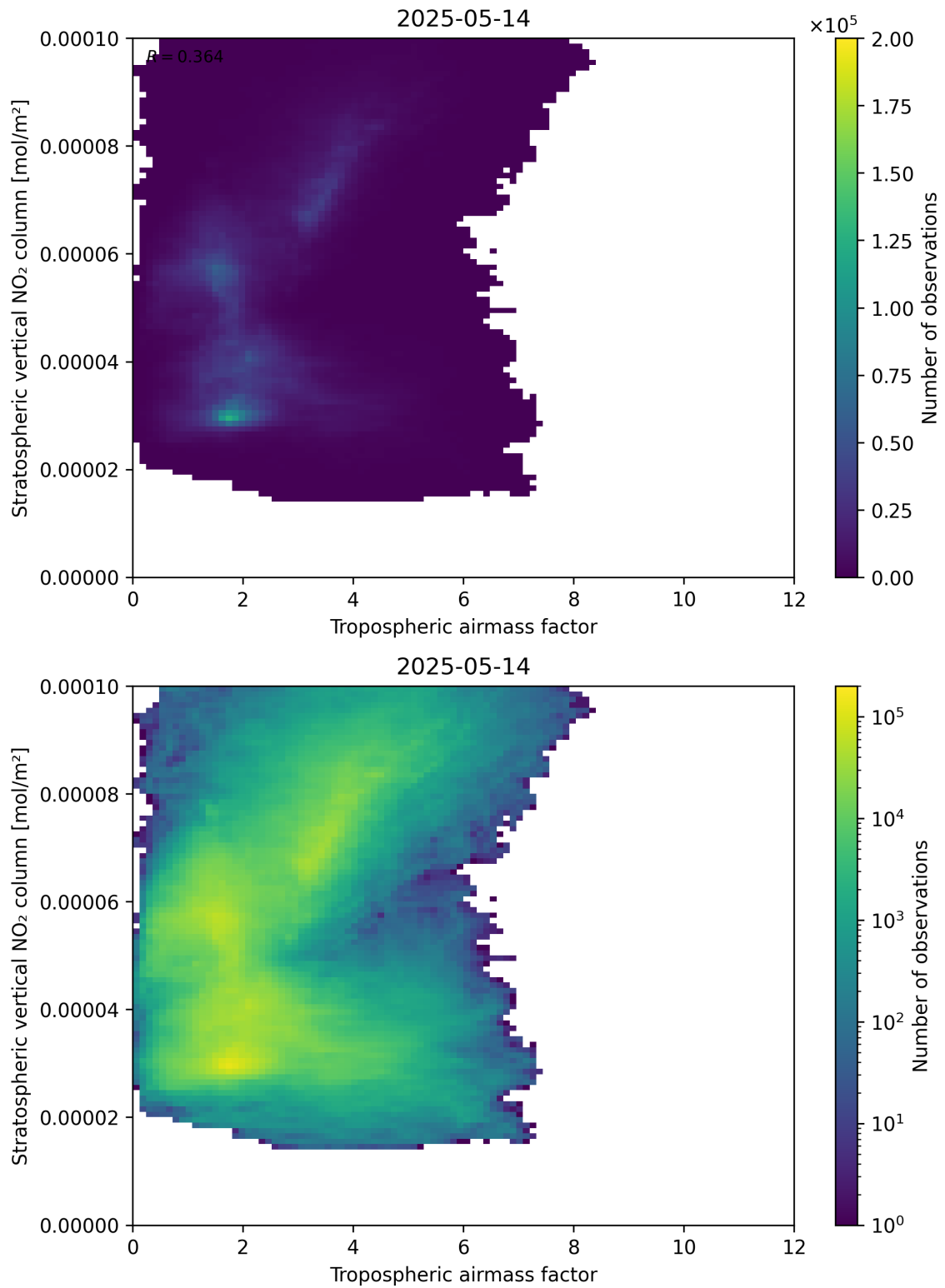
Figure 74: Scatter density plot of “Tropospheric air mass factor” against “Stratospheric vertical NO 2 column” for 2025-05-13 to 2025-05-15.
