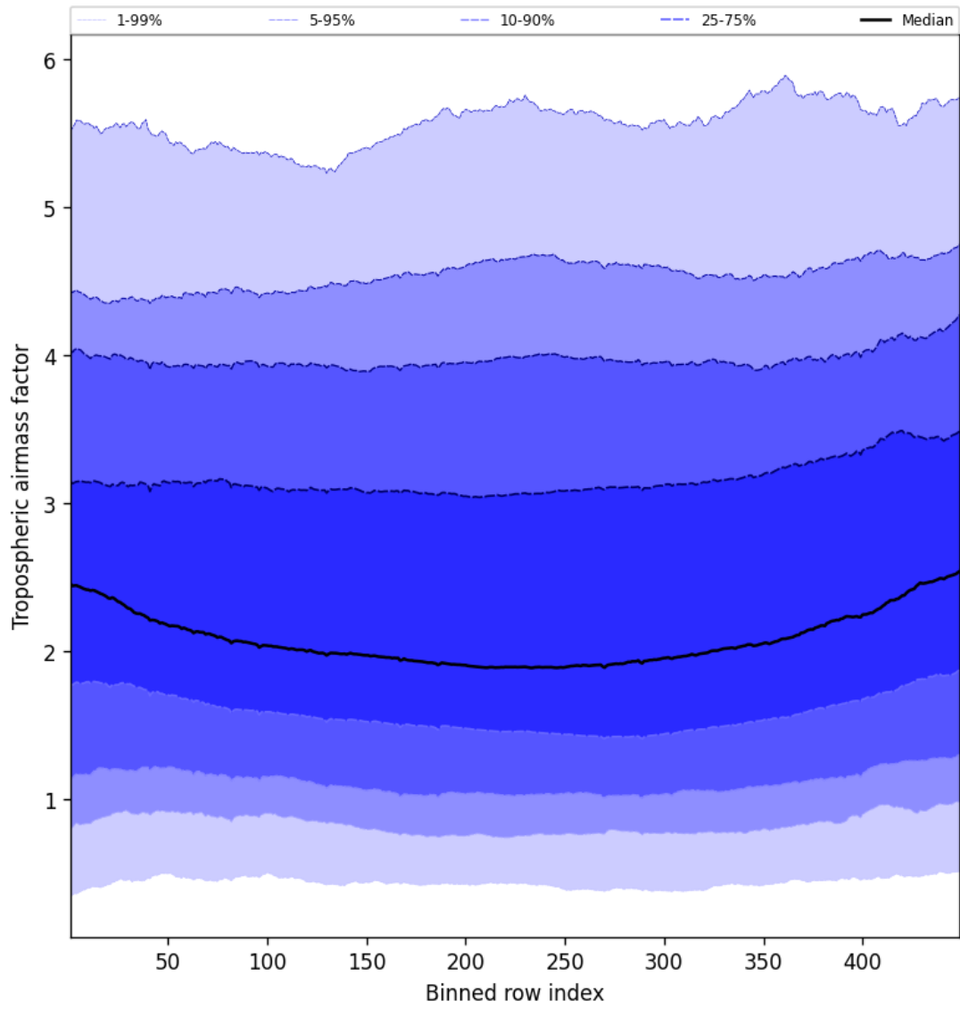
Figure 48: Along track statistics of “Tropospheric airmass factor” for 2025-05-13 to 2025-05-15
