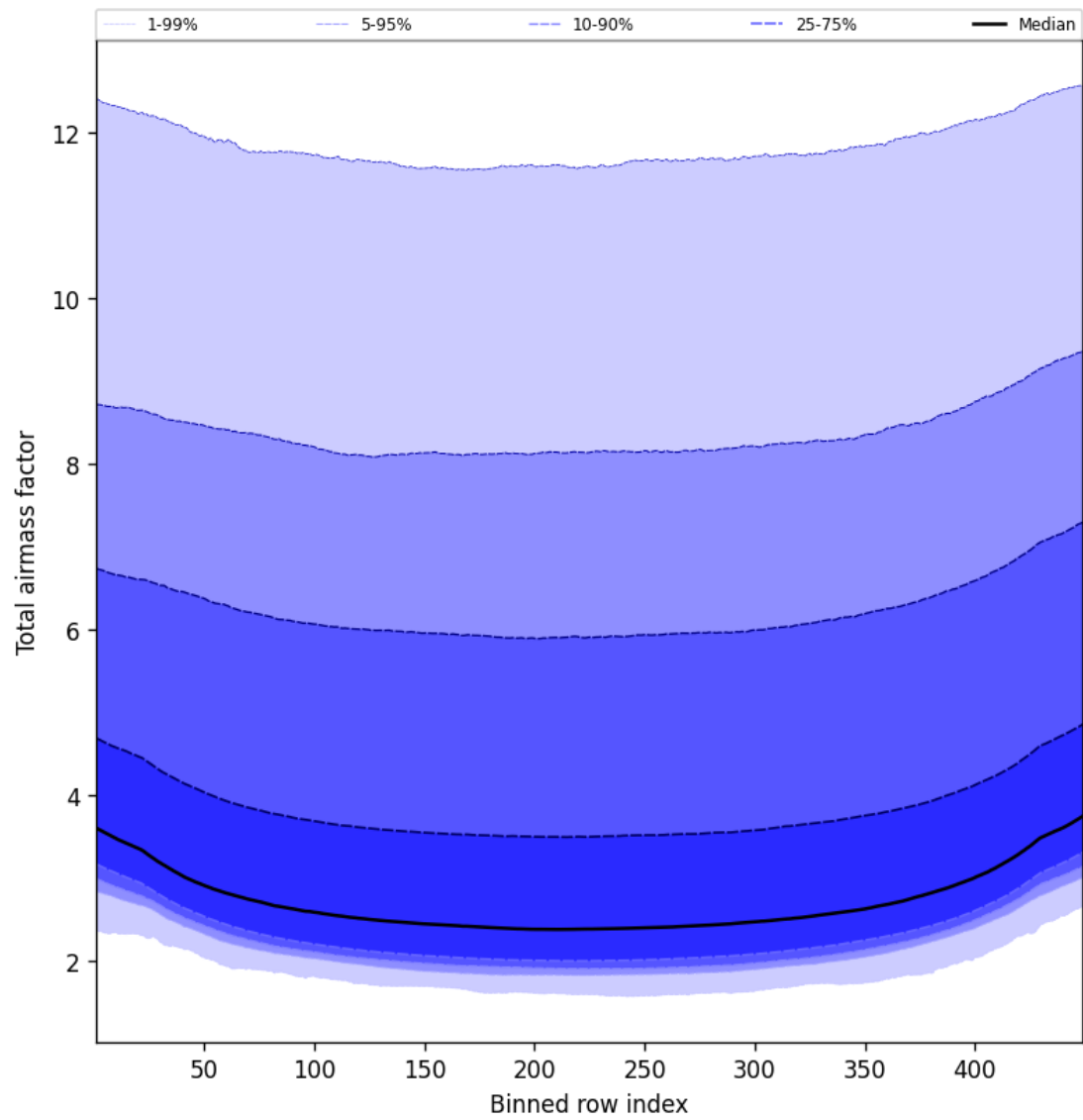
Figure 49: Along track statistics of “Total airmass factor” for 2025-05-13 to 2025-05-15
