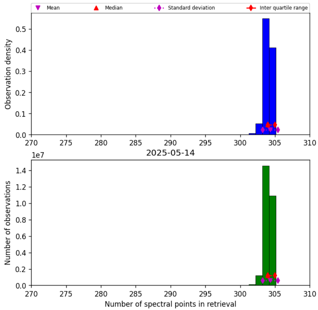
Figure 33: Histogram of “Number of spectral points in retrieval” for 2025-05-13 to 2025-05-15
