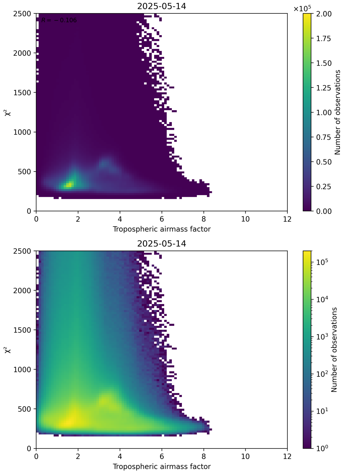
Figure 73: Scatter density plot of “Tropospheric airmass factor” against “ \chi^2 ” for 2025-05-13 to 2025-05-15.
