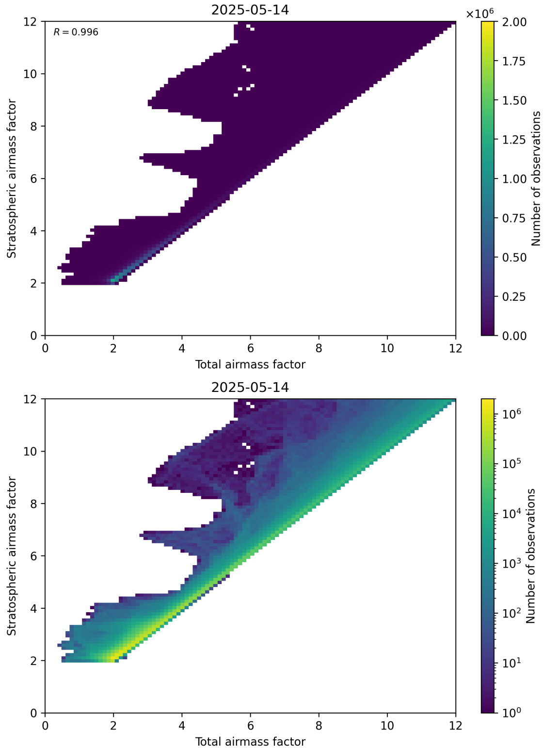
Figure 62: Scatter density plot of “Total airmass factor” against “Stratospheric airmass factor” for 2025-05-13 to 2025-05-15.
