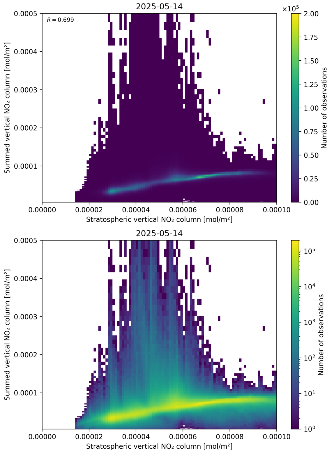
Figure 98: Scatter density plot of “Stratospheric vertical NO 2 column” against “Summed vertical NO 2 column” for 2025-05-13 to 2025-05-15.
