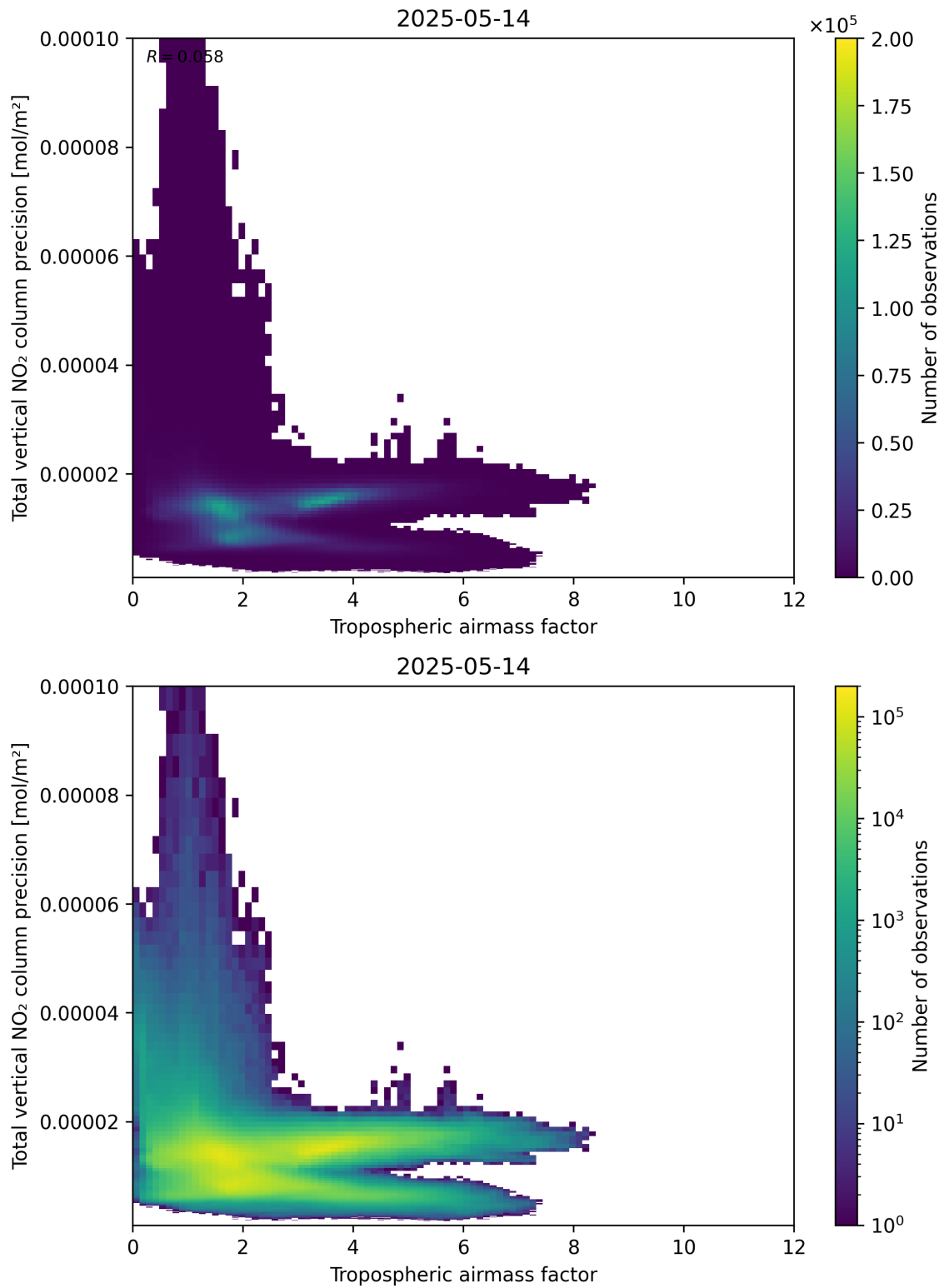
Figure 78: Scatter density plot of “Tropospheric airmass factor” against “Total vertical NO 2 column precision” for 2025-05-13 to 2025-05-15.
