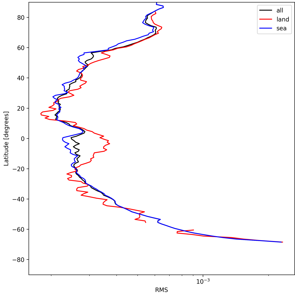
Figure 26: Zonal average of “RMS” for 2025-05-13 to 2025-05-15.
