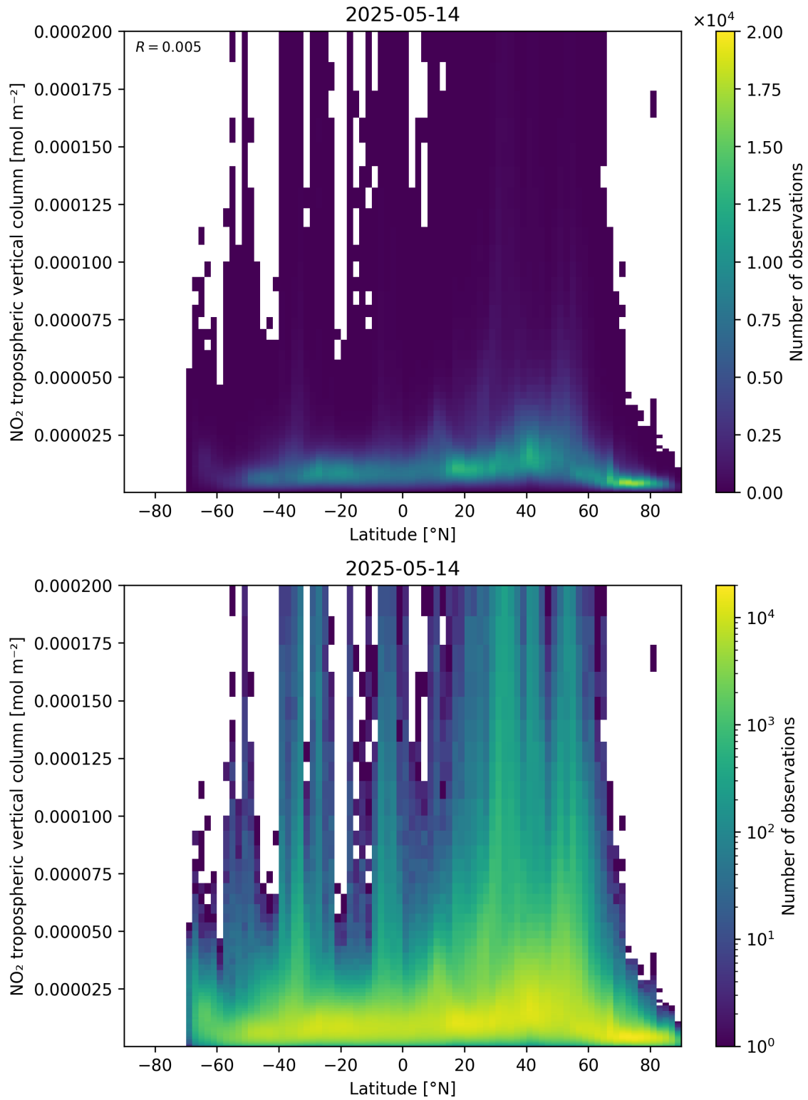
Figure 92: Scatter density plot of “Latitude” against “NO 2 tropospheric vertical column” for 2025-05-13 to 2025-05-15.
