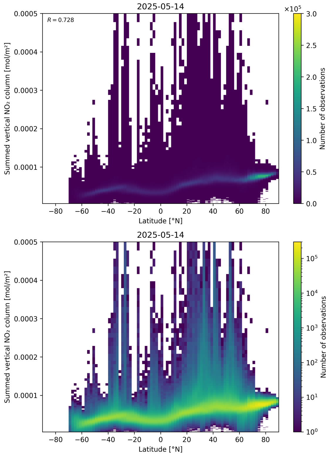
Figure 88: Scatter density plot of “Latitude” against “Summed vertical NO 2 column” for 2025-05-13 to 2025-05-15.
