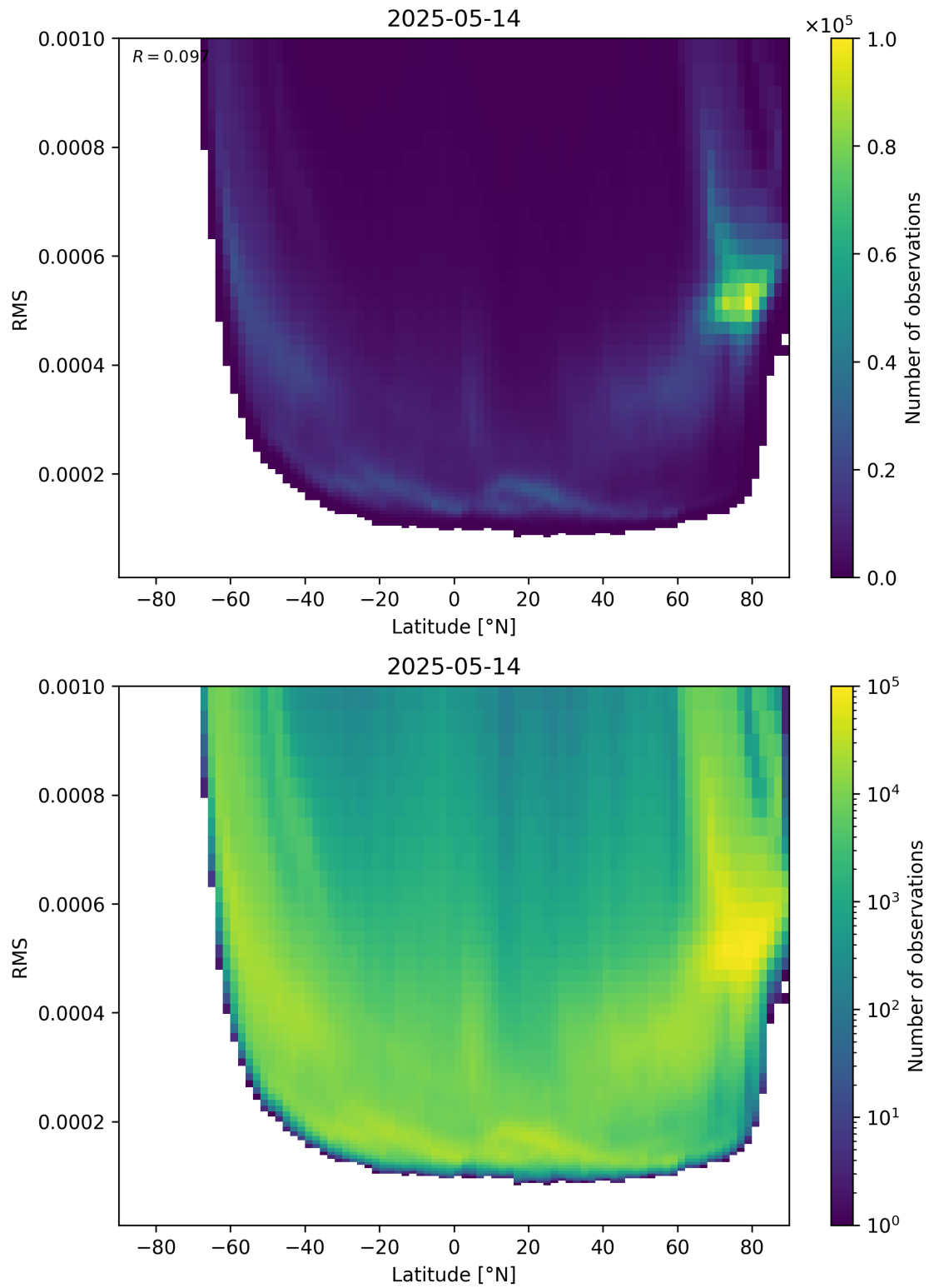
Figure 94: Scatter density plot of “Latitude” against “RMS” for 2025-05-13 to 2025-05-15.
