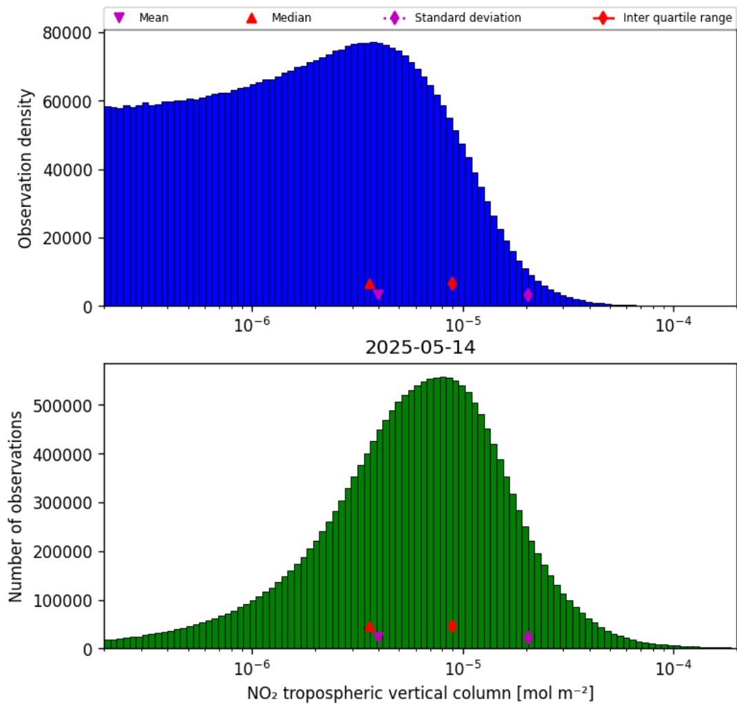
Figure 29: Histogram of “NO 2 tropospheric vertical column” for 2025-05-13 to 2025-05-15
