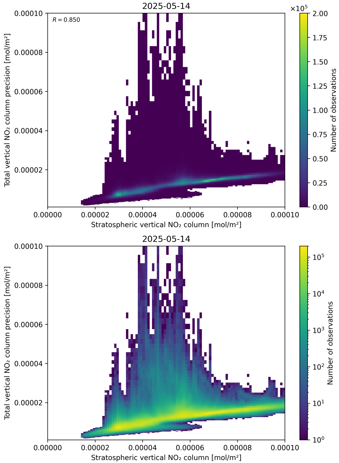
Figure 101: Scatter density plot of “Stratospheric vertical NO 2 column” against “Total vertical NO 2 column precision” for 2025-05-13 to 2025-05-15.
