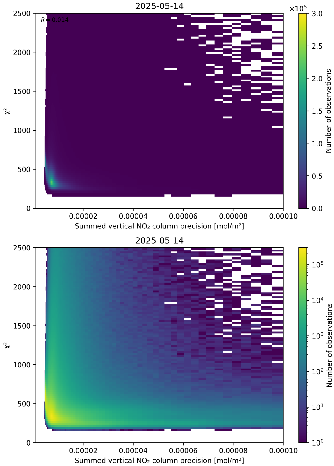
Figure 107: Scatter density plot of “Summed vertical NO 2 column precision” against “ \chi^2 ” for 2025-05-13 to 2025-05-15.
