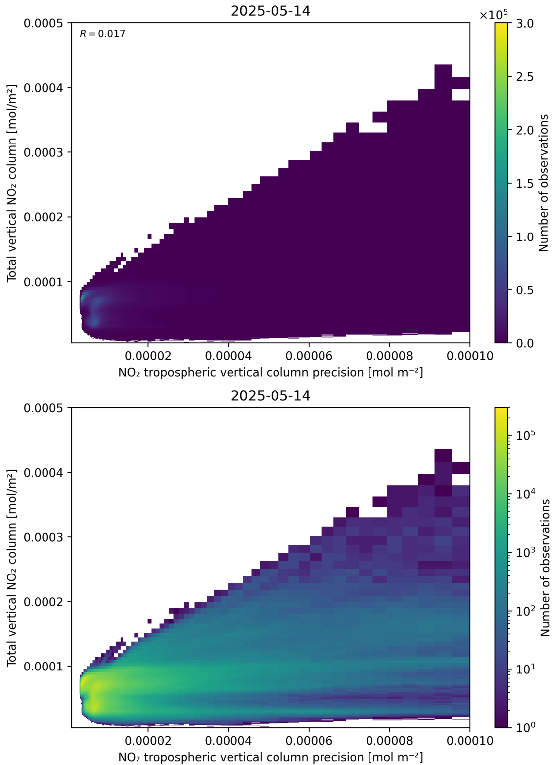
Figure 138: Scatter density plot of “NO 2 tropospheric vertical column precision” against “Total vertical NO 2 column” for 2025-05-13 to 2025-05-15.
