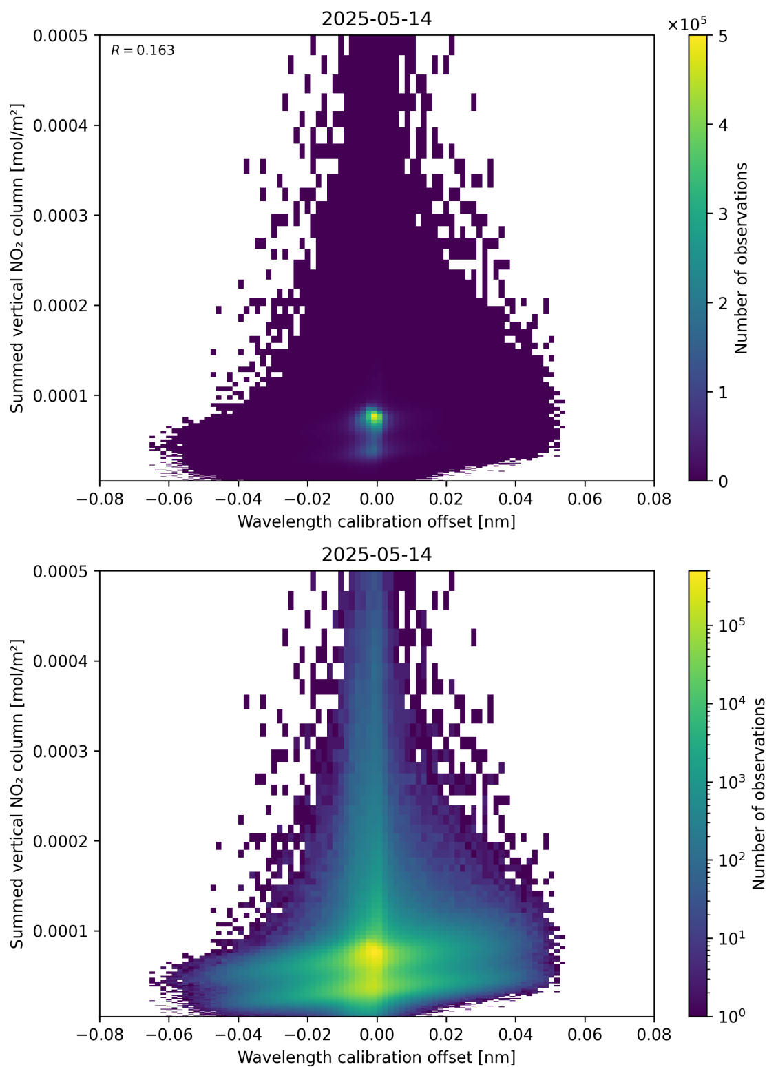
Figure 177: Scatter density plot of “Wavelength calibration offset” against “Summed vertical NO 2 column” for 2025-05-13 to 2025-05-15.
