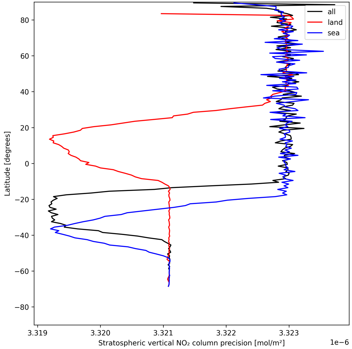
Figure 20: Zonal average of “Stratospheric vertical NO 2 column precision” for 2025-05-13 to 2025-05-15.
