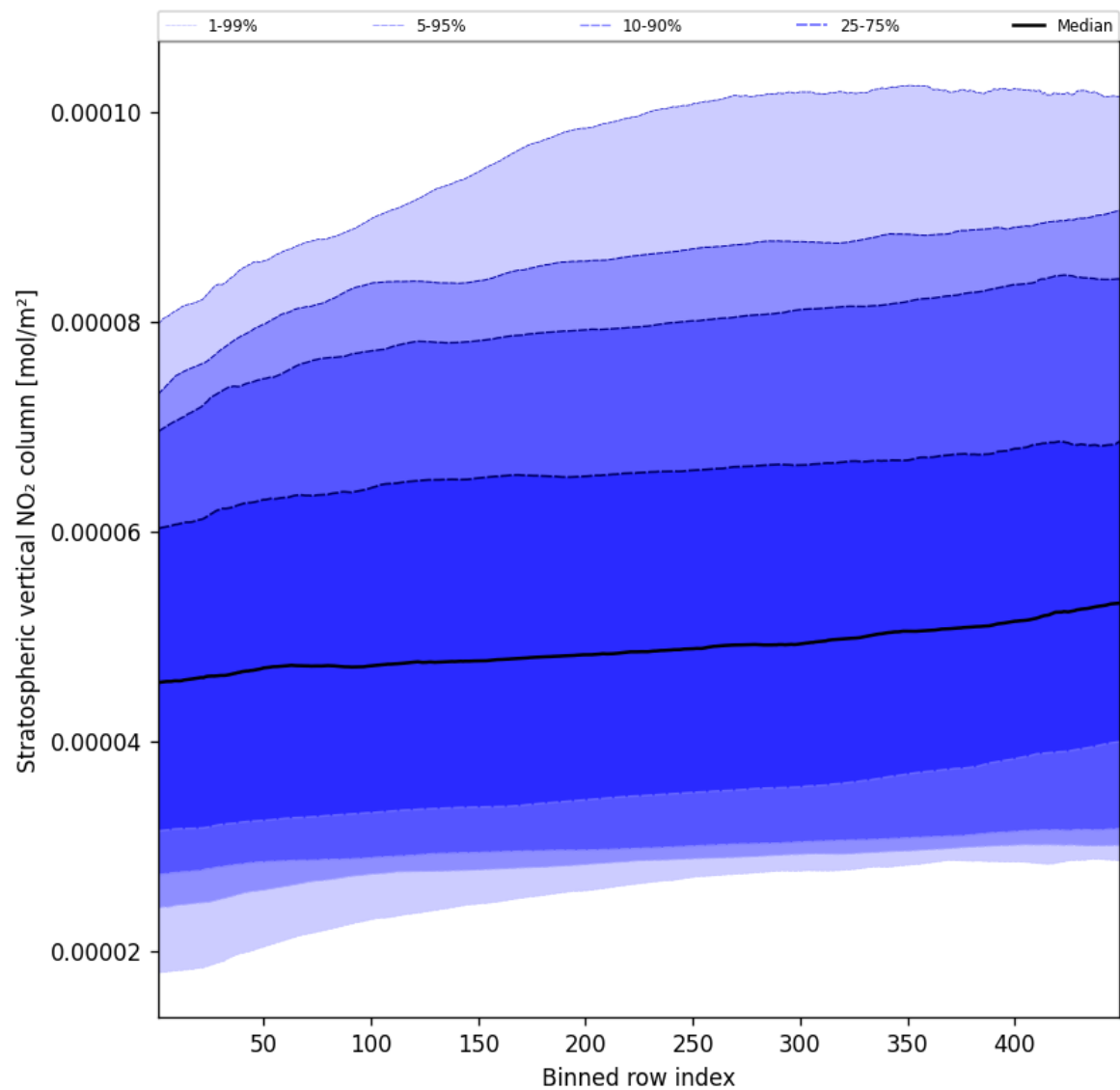
Figure 53: Along track statistics of “Stratospheric vertical NO 2 column” for 2025-05-13 to 2025-05-15
