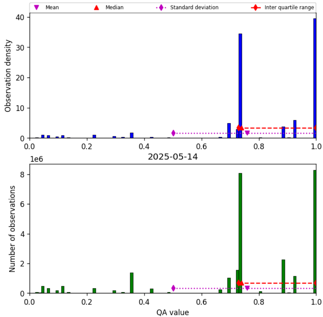
Figure 28: Histogram of “QA value” for 2025-05-13 to 2025-05-15
