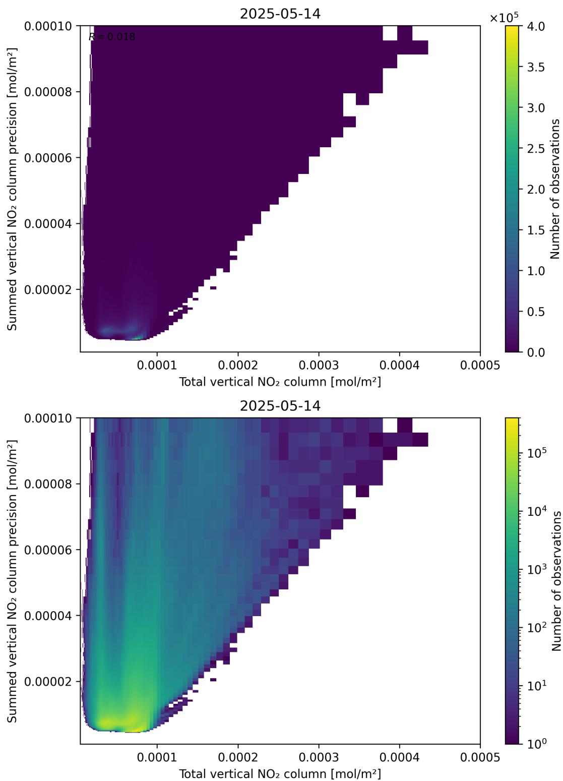
Figure 113: Scatter density plot of “Total vertical NO 2 column” against “Summed vertical NO 2 column precision” for 2025-05-13 to 2025-05-15.
