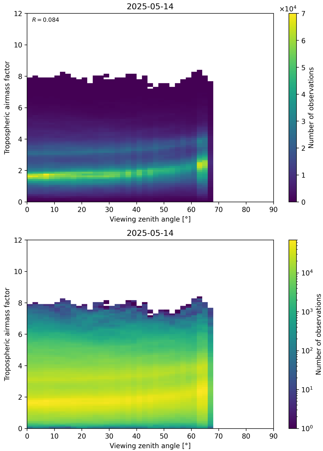
Figure 161: Scatter density plot of “Viewing zenith angle” against “Tropospheric airmass factor” for 2025-05-13 to 2025-05-15.
