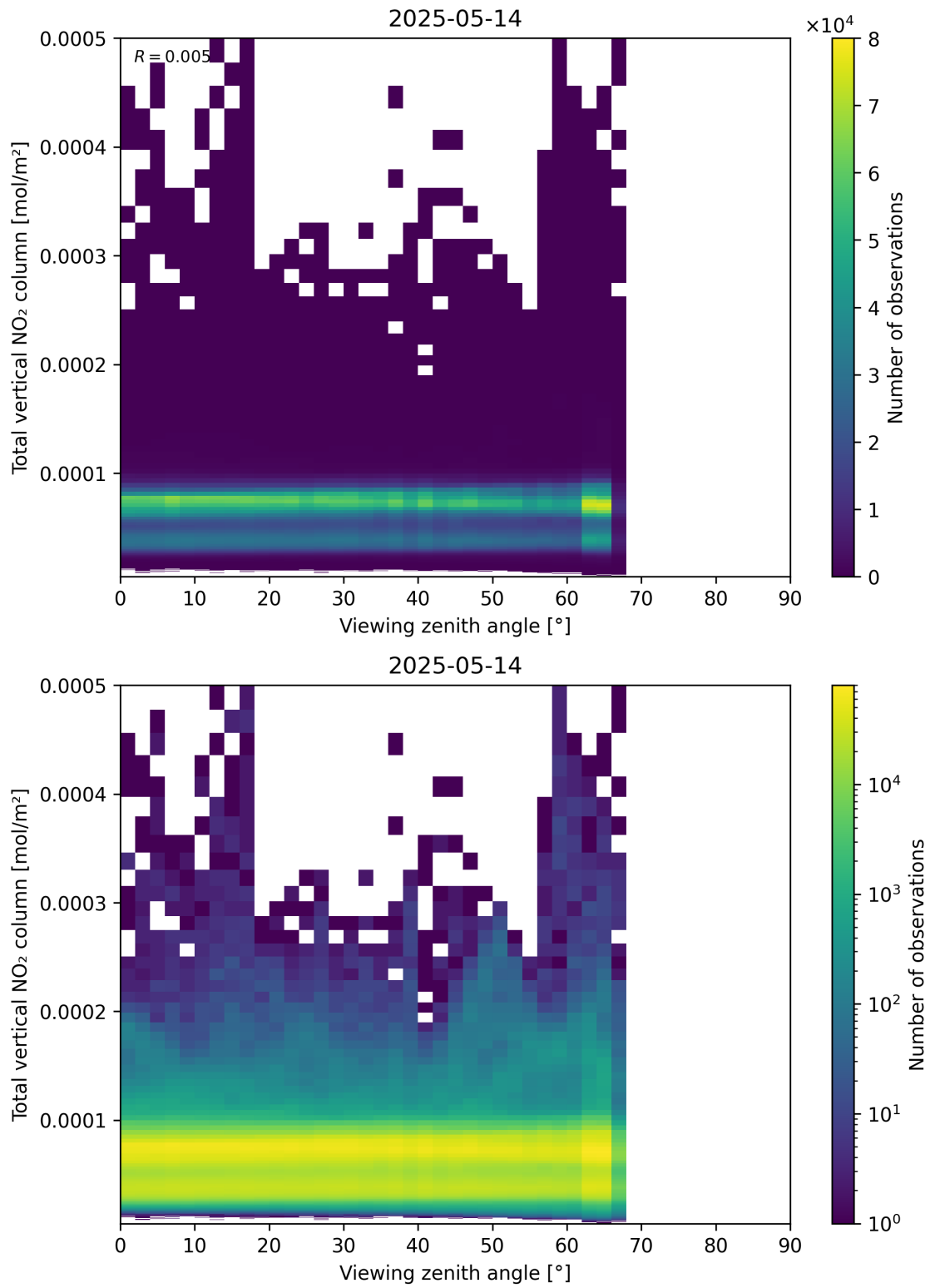
Figure 167: Scatter density plot of “Viewing zenith angle” against “Total vertical NO 2 column” for 2025-05-13 to 2025-05-15.
