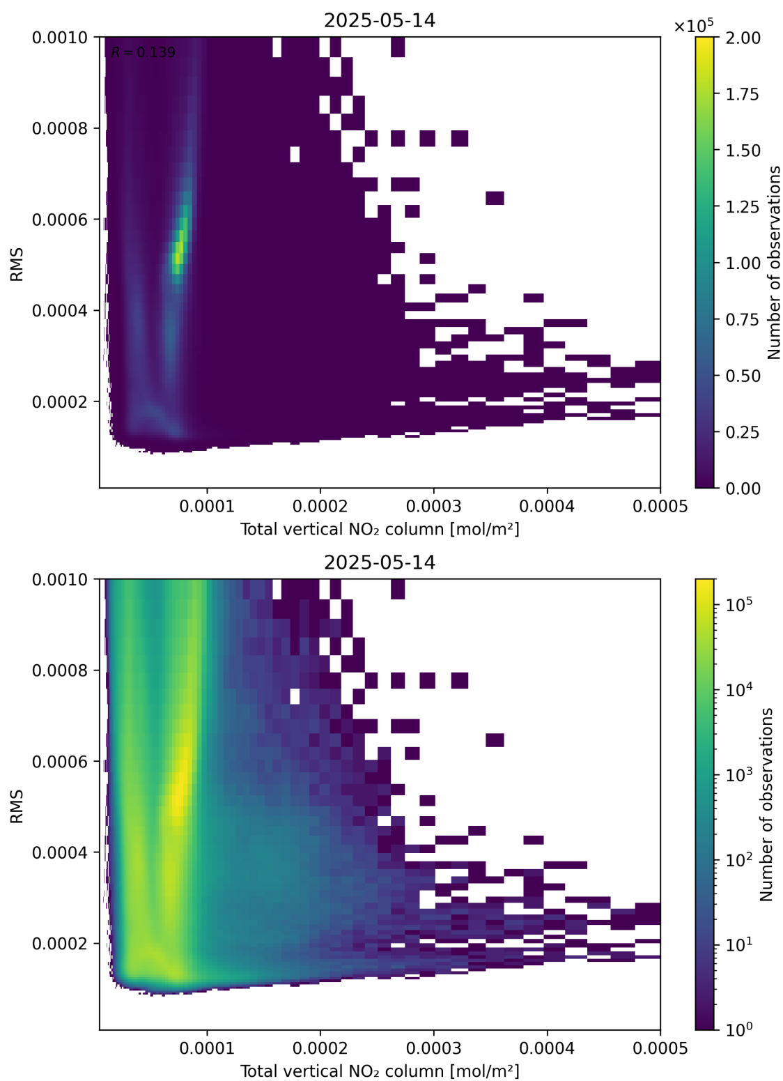
Figure 120: Scatter density plot of “Total vertical NO 2 column” against “RMS” for 2025-05-13 to 2025-05-15.
