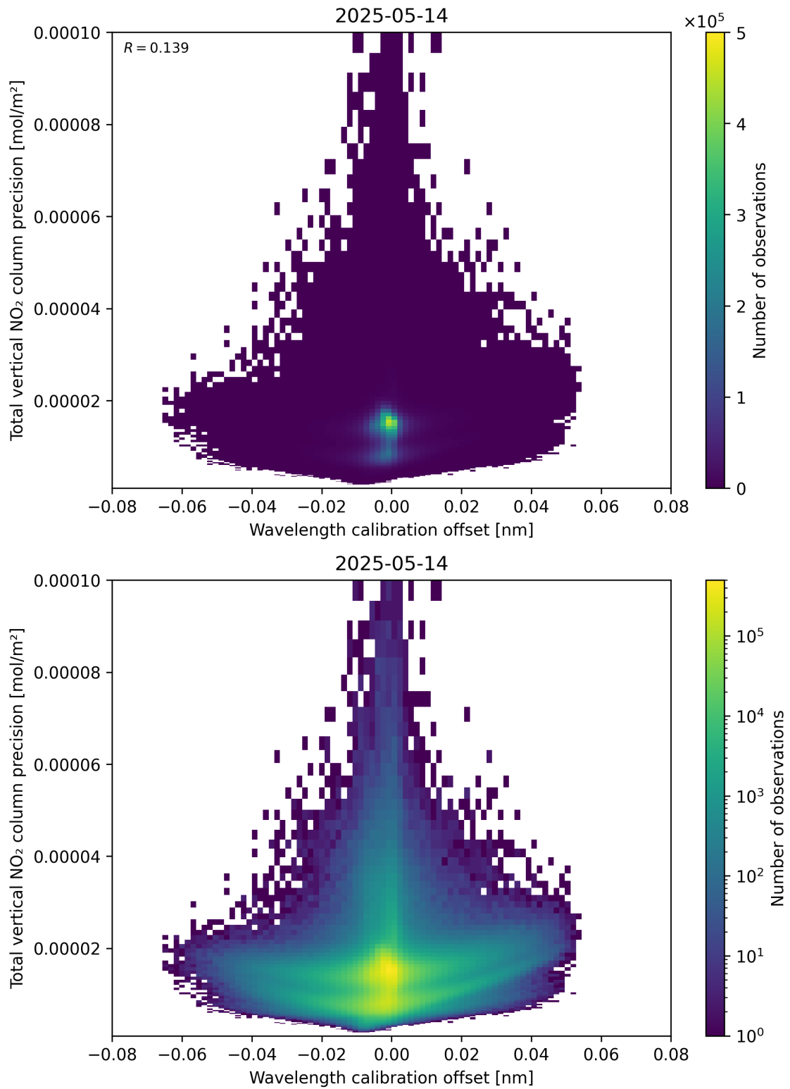
Figure 180: Scatter density plot of “Wavelength calibration offset” against “Total vertical NO 2 column precision” for 2025-05-13 to 2025-05-15.
