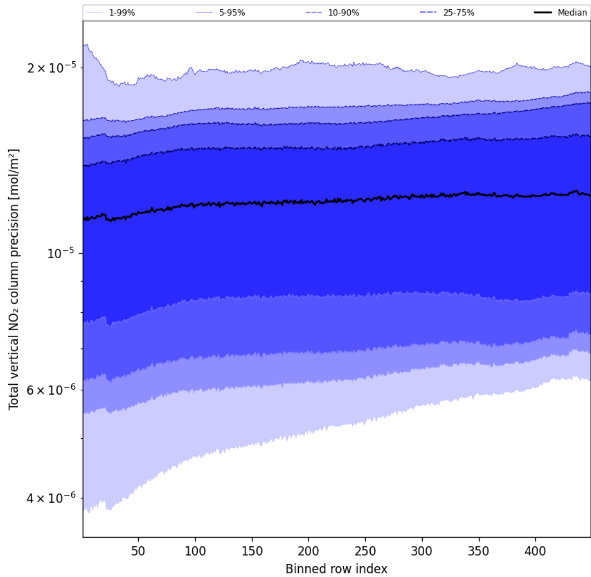
Figure 56: Along track statistics of “Total vertical NO 2 column precision” for 2025-05-13 to 2025-05-15
