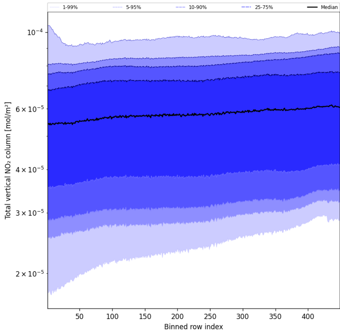
Figure 55: Along track statistics of “Total vertical NO 2 column” for 2025-05-13 to 2025-05-15
