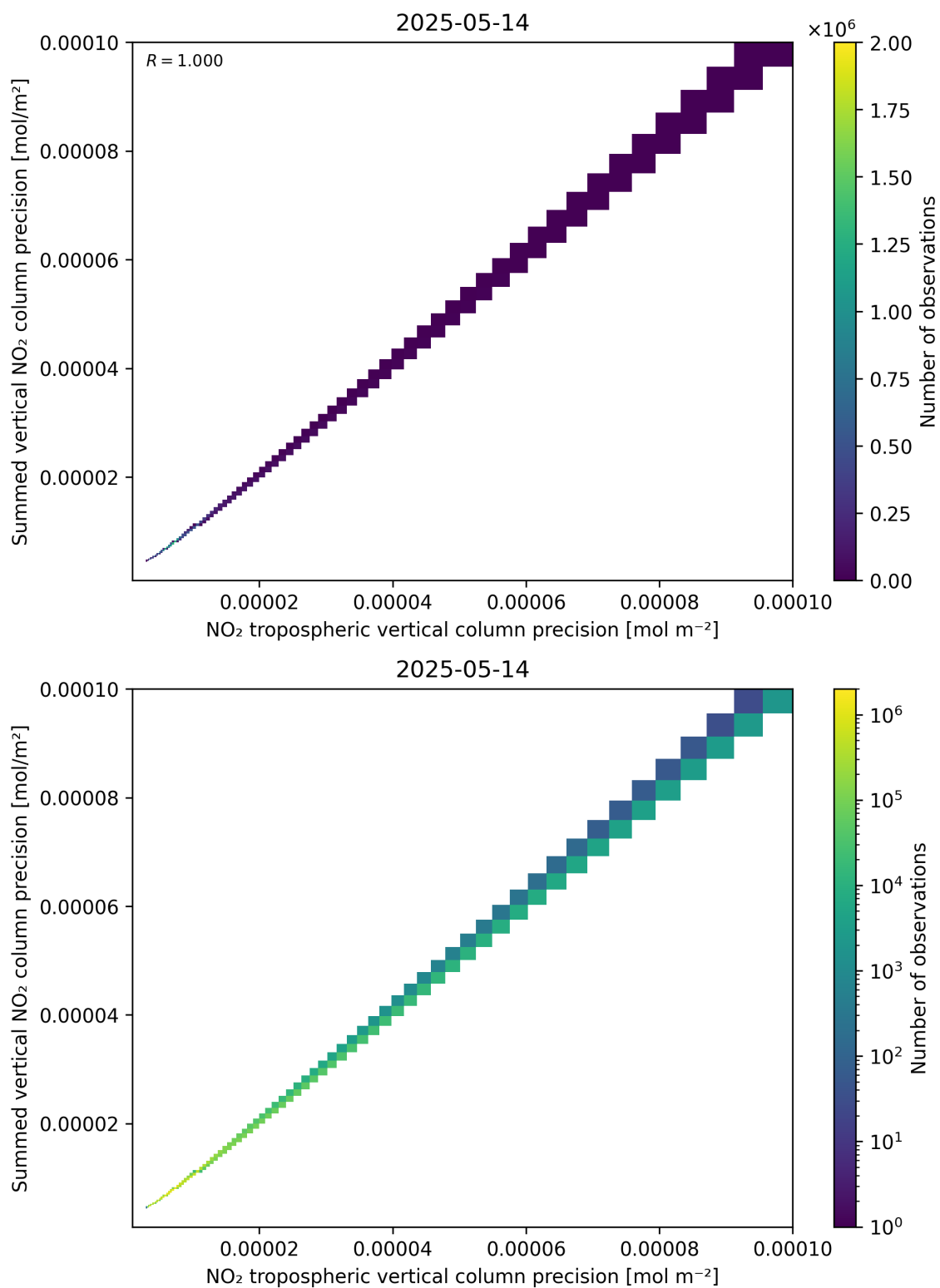
Figure 137: Scatter density plot of “NO 2 tropospheric vertical column precision” against “Summed vertical NO 2 column precision” for 2025-05-13 to 2025-05-15.
