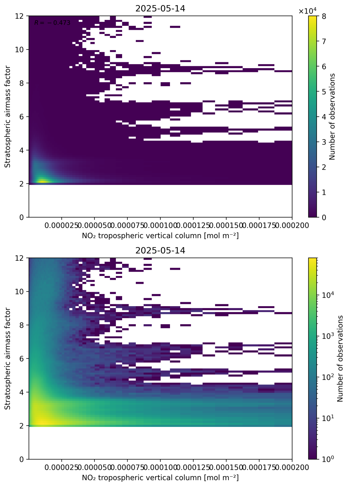
Figure 121: Scatter density plot of “NO 2 tropospheric vertical column” against “Stratospheric air mass factor” for 2025-05-13 to 2025-05-15.
