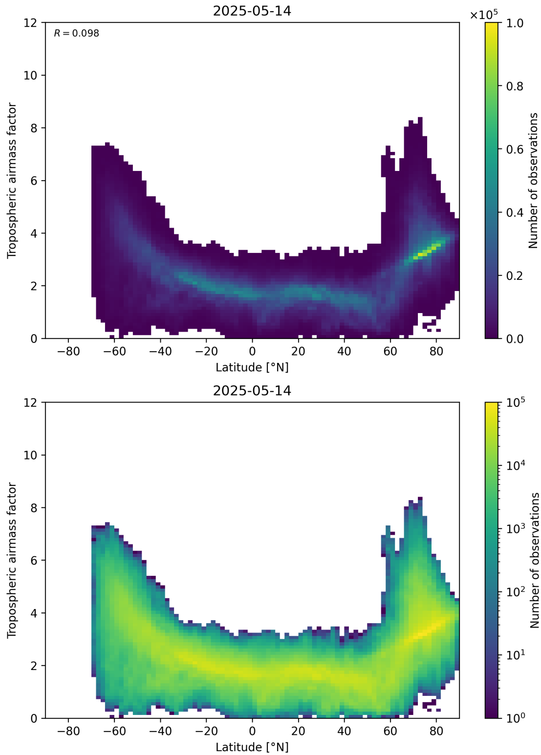
Figure 85: Scatter density plot of “Latitude” against “Tropospheric air mass factor” for 2025-05-13 to 2025-05-15.
