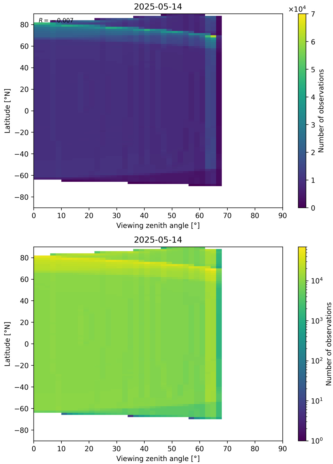
Figure 163: Scatter density plot of “Viewing zenith angle” against “Latitude” for 2025-05-13 to 2025-05-15.
