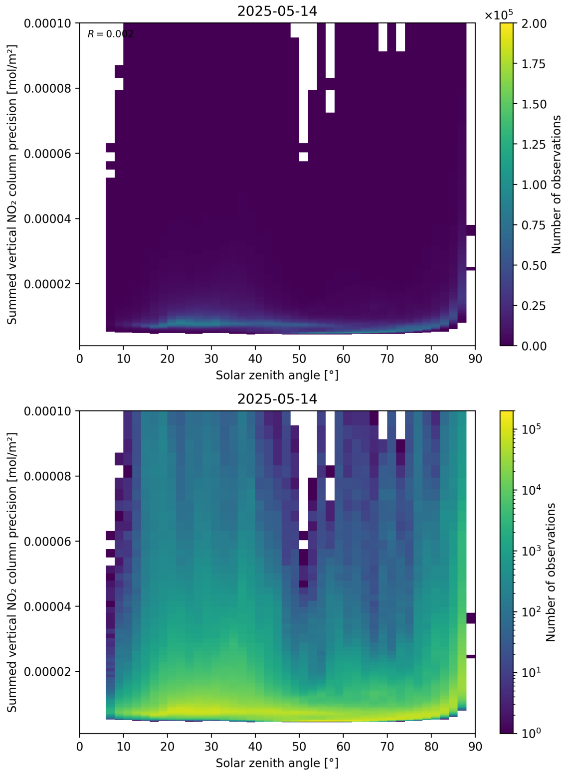
Figure 152: Scatter density plot of “Solar zenith angle” against “Summed vertical NO 2 column precision” for 2025-05-13 to 2025-05-15.
