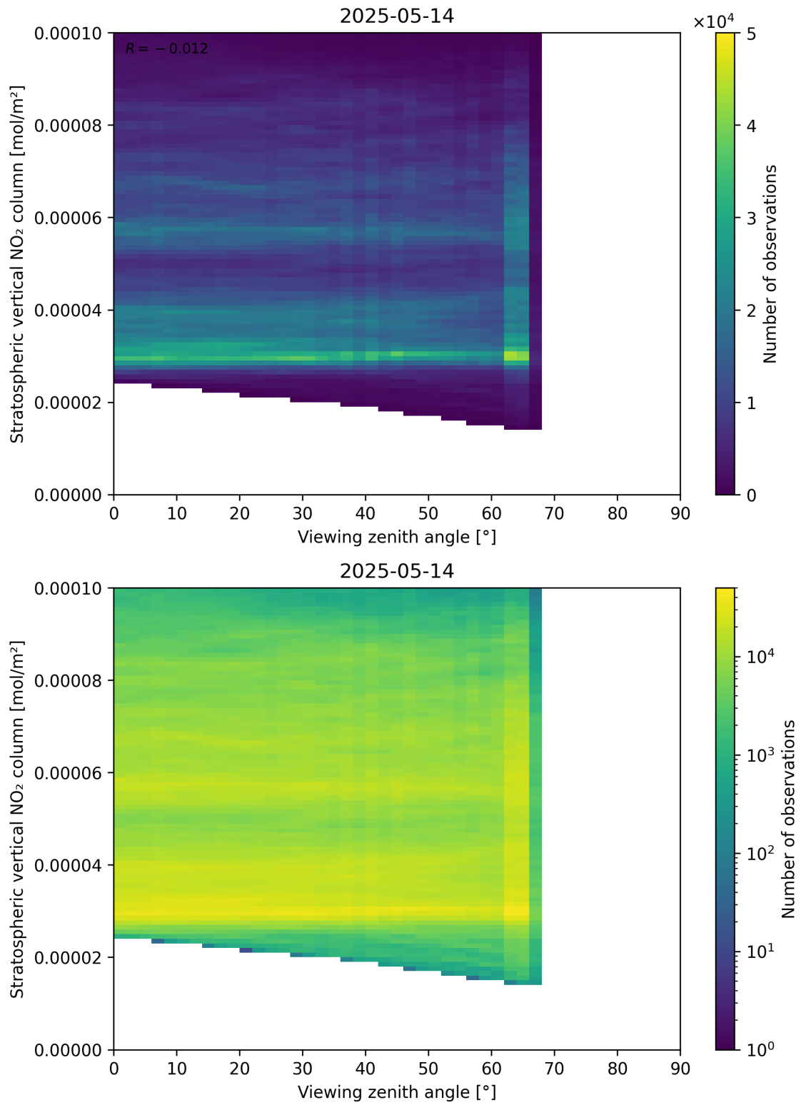
Figure 164: Scatter density plot of “Viewing zenith angle” against “Stratospheric vertical NO 2 column” for 2025-05-13 to 2025-05-15.
