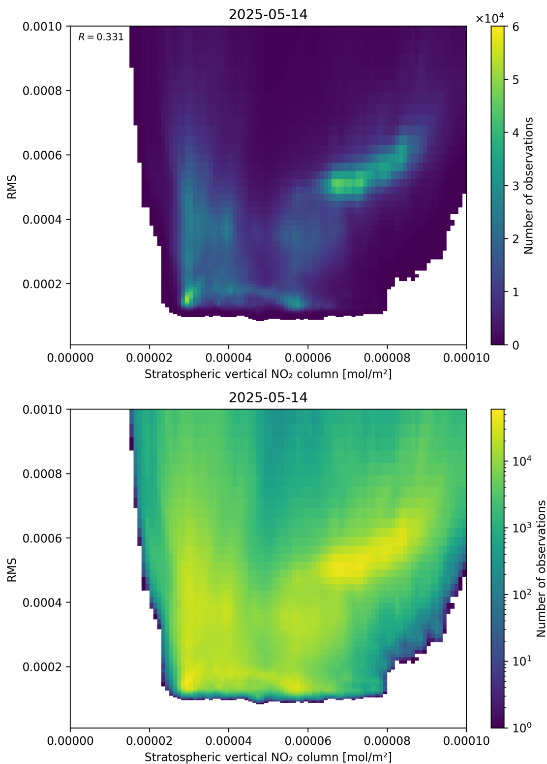
Figure 102: Scatter density plot of “Stratospheric vertical NO 2 column” against “RMS” for 2025-05-13 to 2025-05-15.
