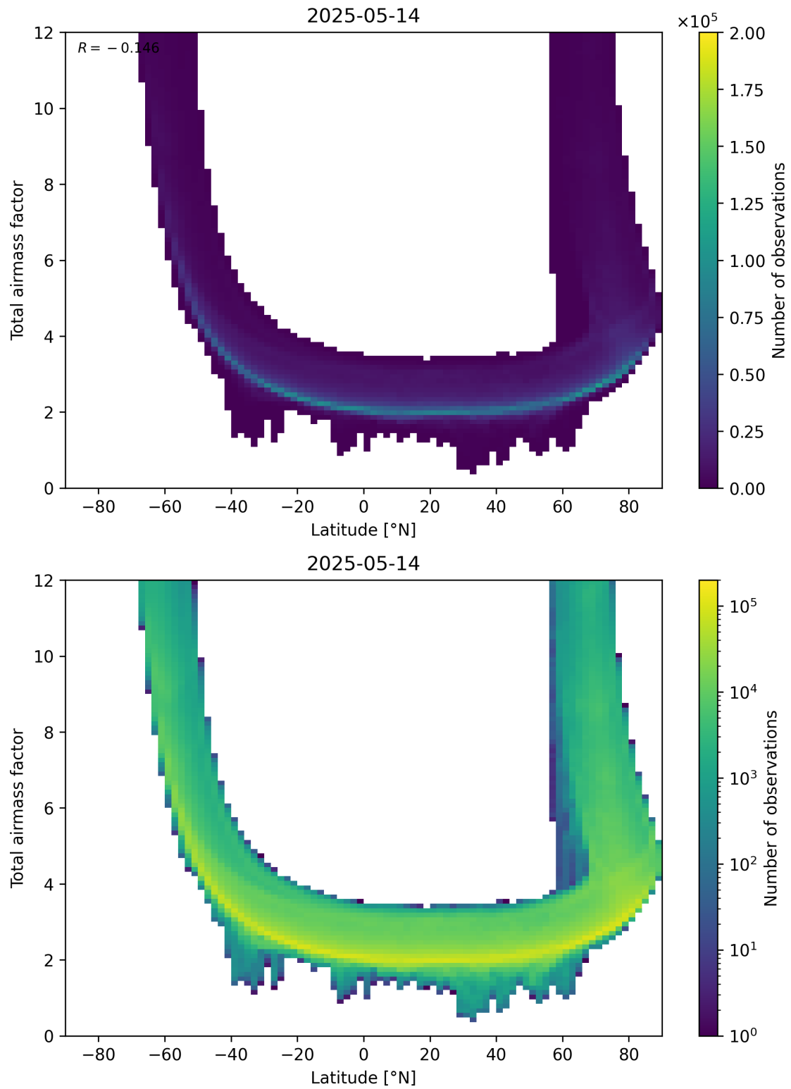
Figure 84: Scatter density plot of “Latitude” against “Total airmass factor” for 2025-05-13 to 2025-05-15.
