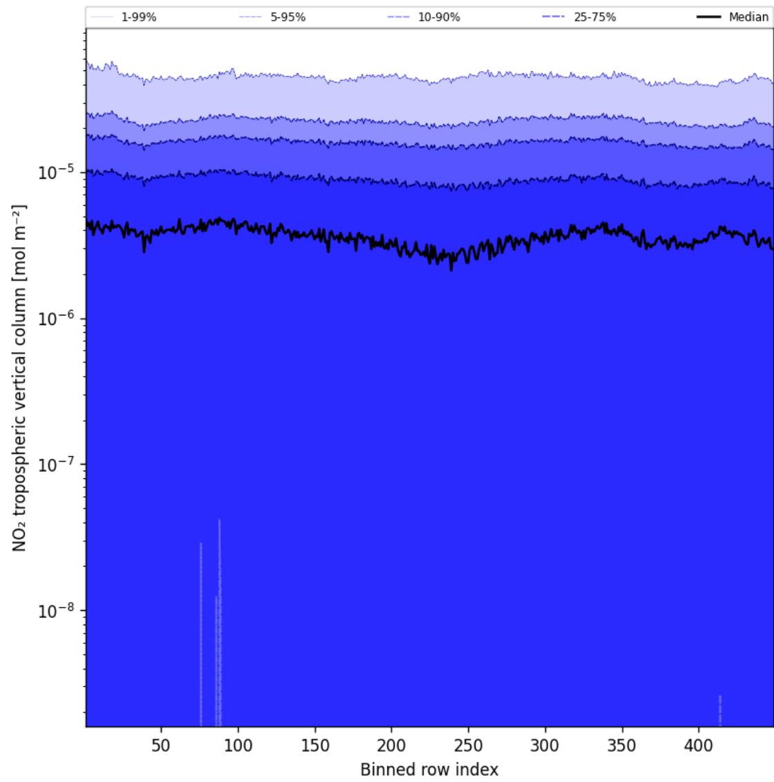
Figure 46: Along track statistics of “NO 2 tropospheric vertical column” for 2025-05-13 to 2025-05-15
