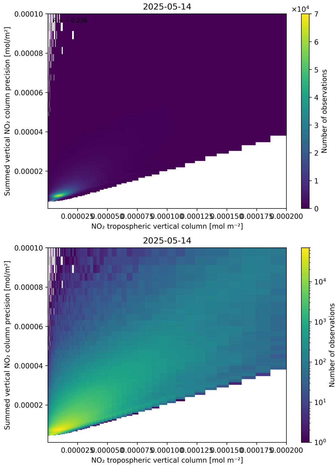
Figure 127: Scatter density plot of “NO 2 tropospheric vertical column” against “Summed vertical NO 2 column precision” for 2025-05-13 to 2025-05-15.
