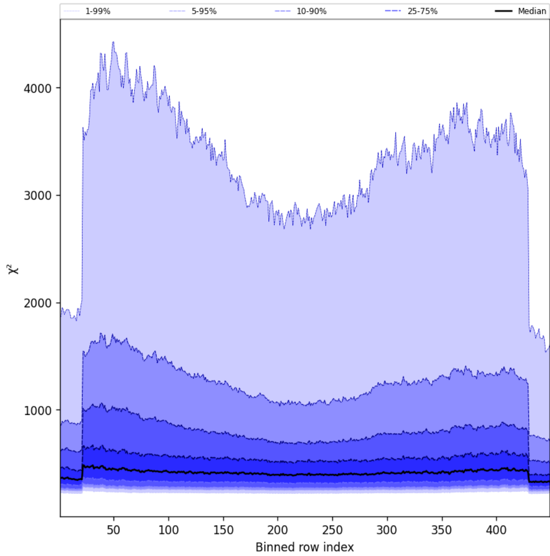
Figure 59: Along track statistics of “ \chi^2 ” for 2025-05-13 to 2025-05-15
