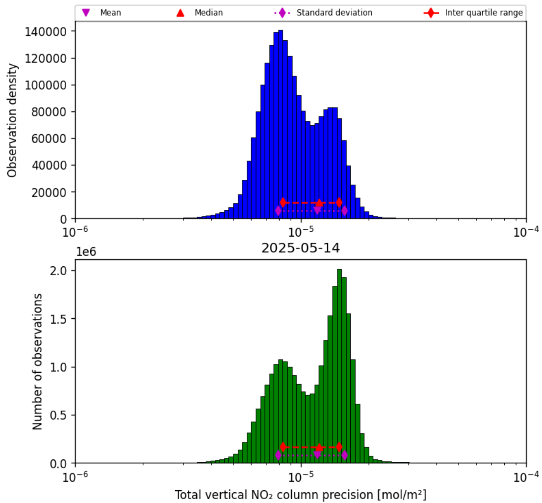
Figure 39: Histogram of “Total vertical NO 2 column precision” for 2025-05-13 to 2025-05-15
