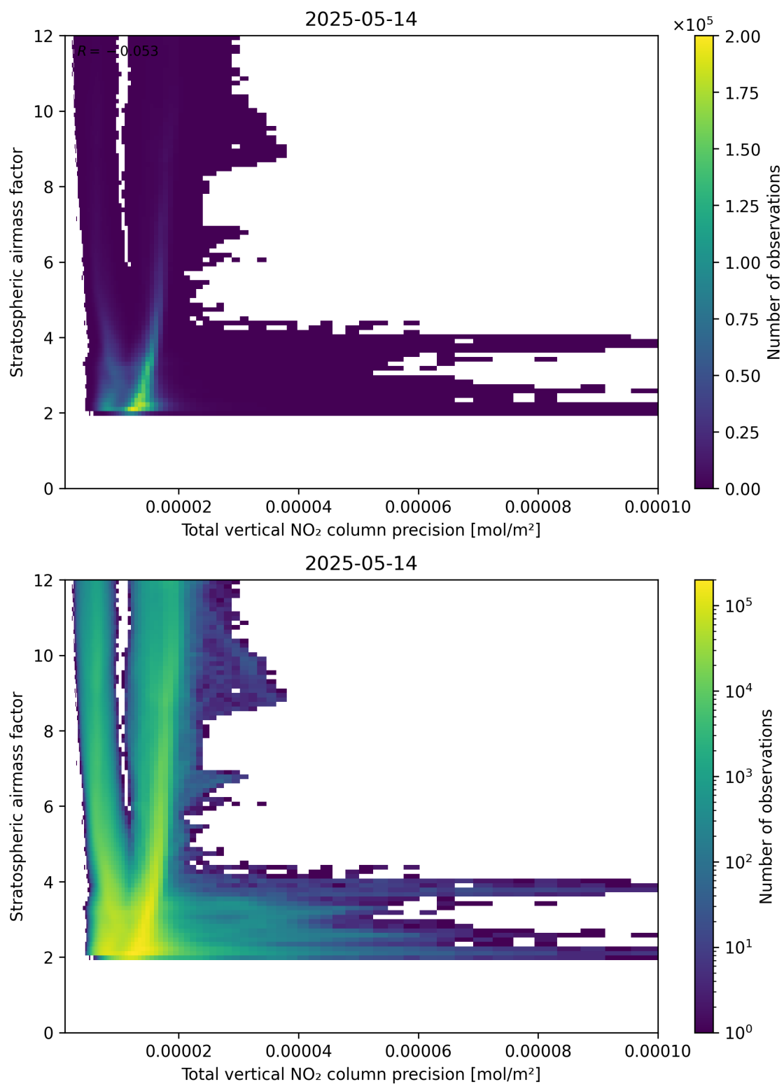
Figure 115: Scatter density plot of “Total vertical NO 2 column precision” against “Stratospheric air mass factor” for 2025-05-13 to 2025-05-15.
