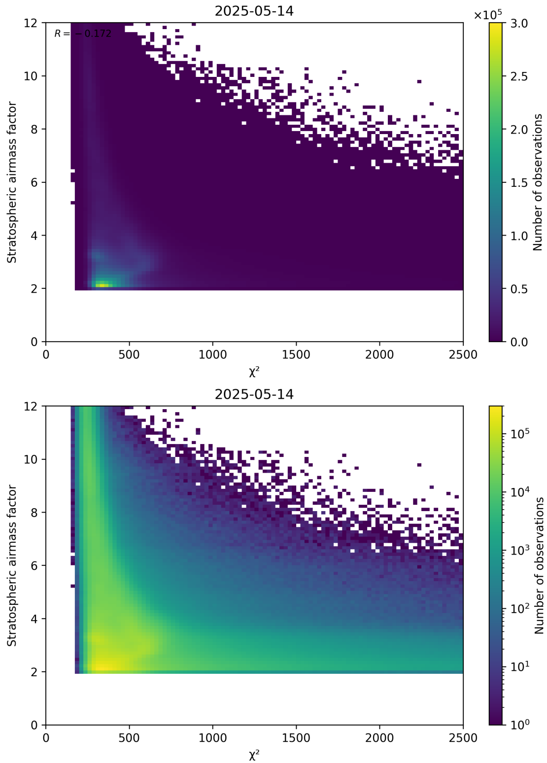
Figure 81: Scatter density plot of “ \chi^2 ” against “Stratospheric airmass factor” for 2025-05-13 to 2025-05-15.
