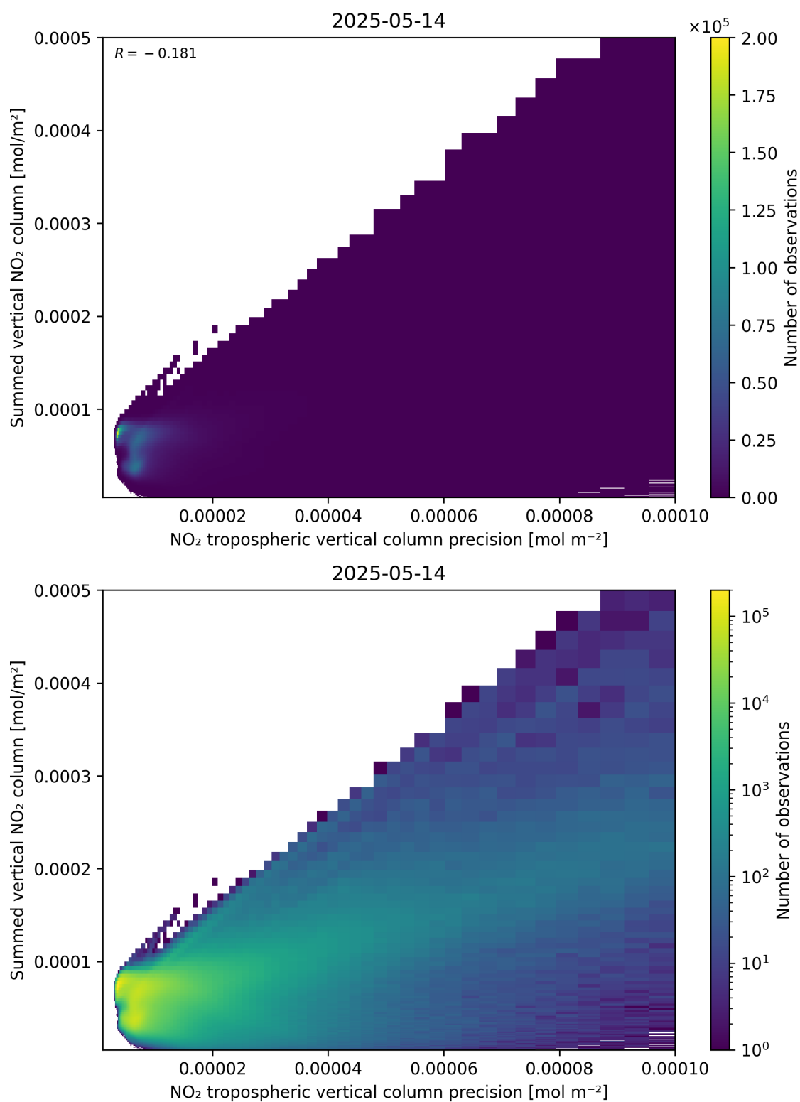
Figure 136: Scatter density plot of “NO 2 tropospheric vertical column precision” against “Summed vertical NO 2 column” for 2025-05-13 to 2025-05-15.
