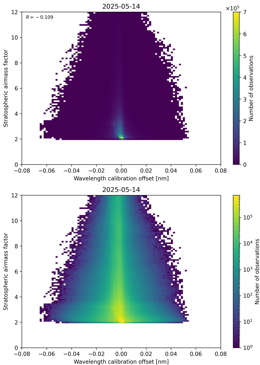
Figure 174: Scatter density plot of “Wavelength calibration offset” against “Stratospheric airmass factor” for 2025-05-13 to 2025-05-15.
