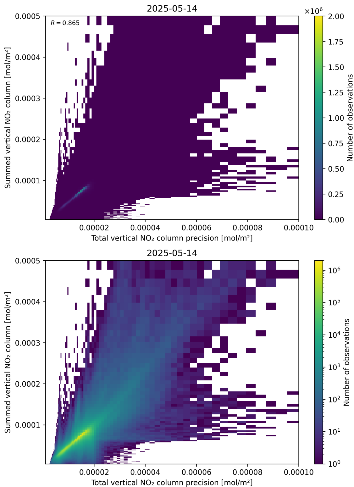
Figure 117: Scatter density plot of “Total vertical NO 2 column precision” against “Summed vertical NO 2 column” for 2025-05-13 to 2025-05-15.
