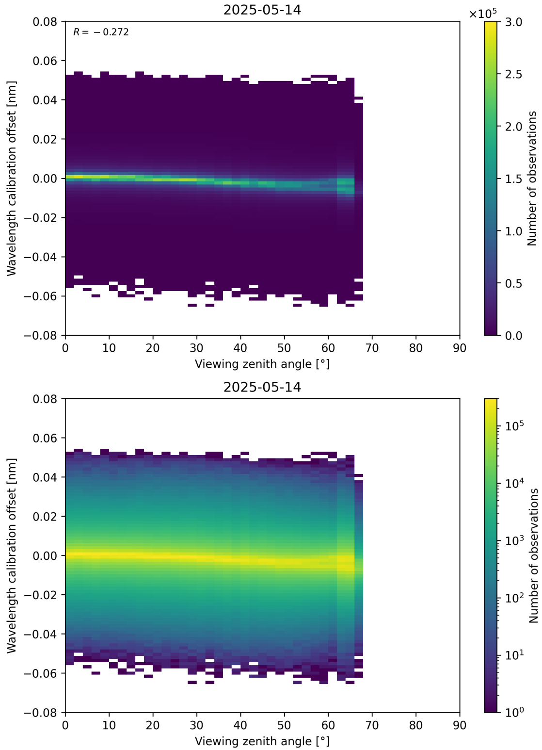
Figure 173: Scatter density plot of “Viewing zenith angle” against “Wavelength calibration offset” for 2025-05-13 to 2025-05-15.
