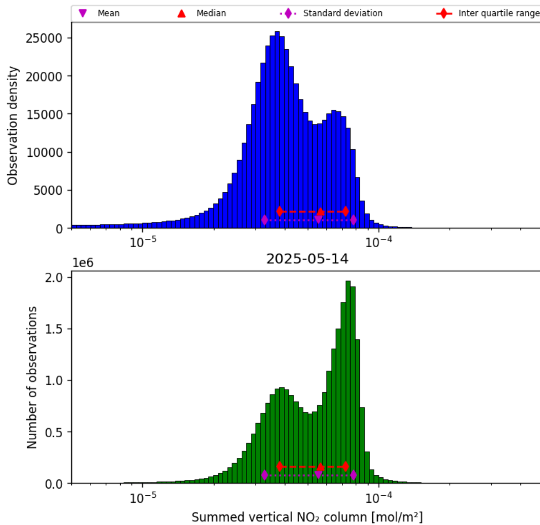
Figure 40: Histogram of “Summed vertical NO 2 column” for 2025-05-13 to 2025-05-15
