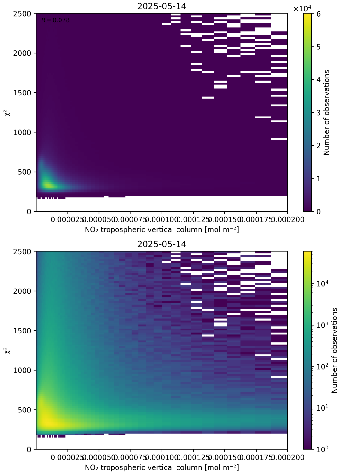
Figure 124: Scatter density plot of “NO 2 tropospheric vertical column” against “ \chi^2 ” for 2025-05-13 to 2025-05-15.
