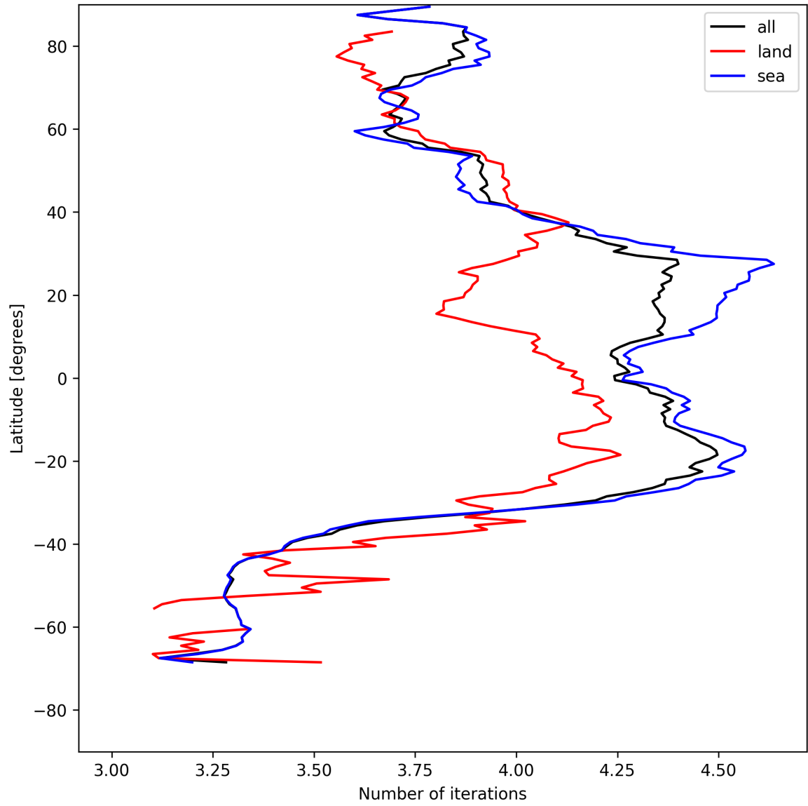
Figure 17: Zonal average of “Number of iterations” for 2025-05-13 to 2025-05-15.
