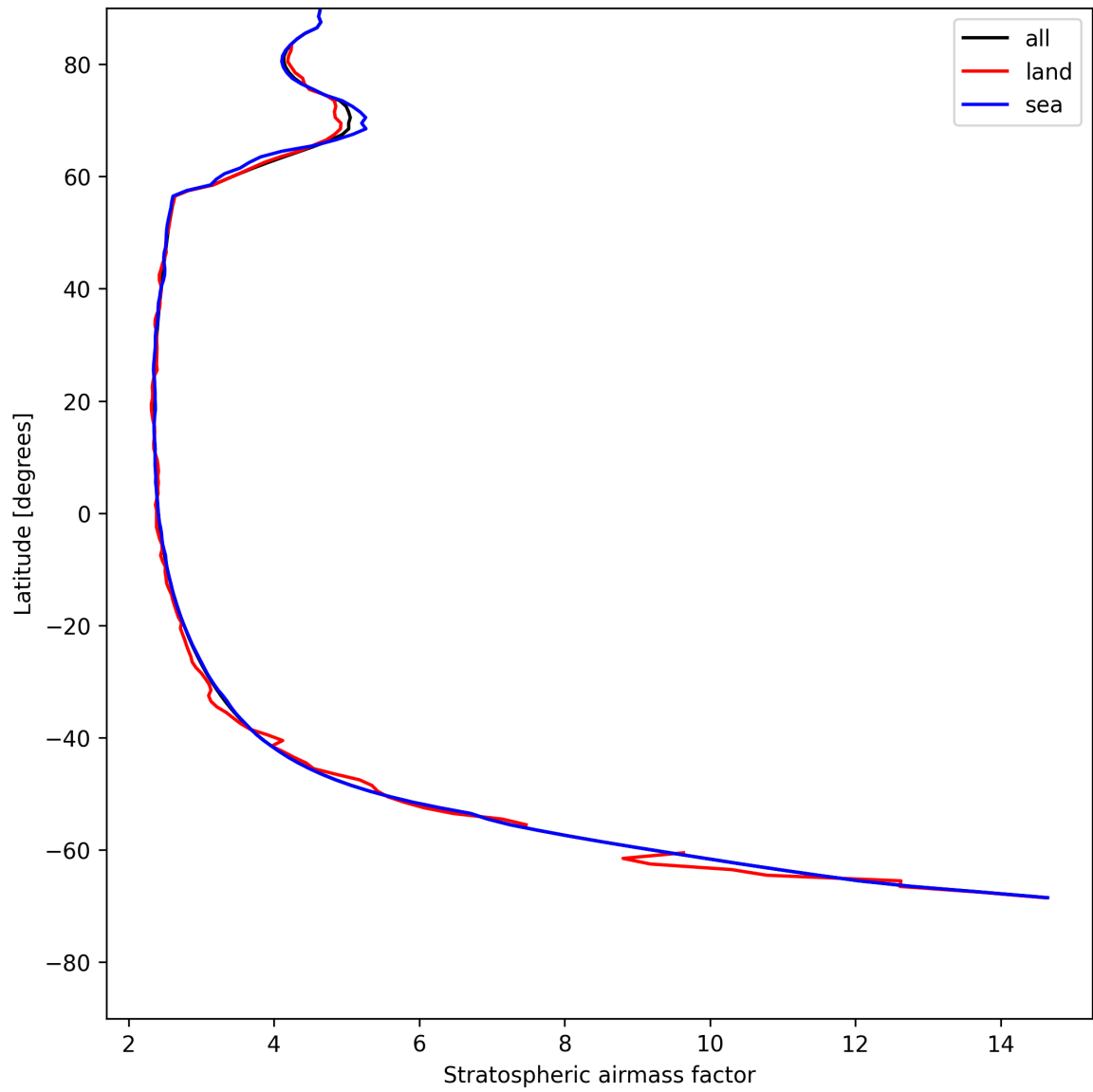
Figure 27: Zonal average of “Stratospheric air mass factor” for 2025-05-13 to 2025-05-15.
