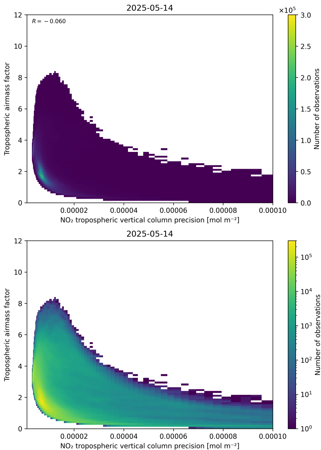
Figure 133: Scatter density plot of “NO 2 tropospheric vertical column precision” against “Tropospheric air mass factor” for 2025-05-13 to 2025-05-15.
