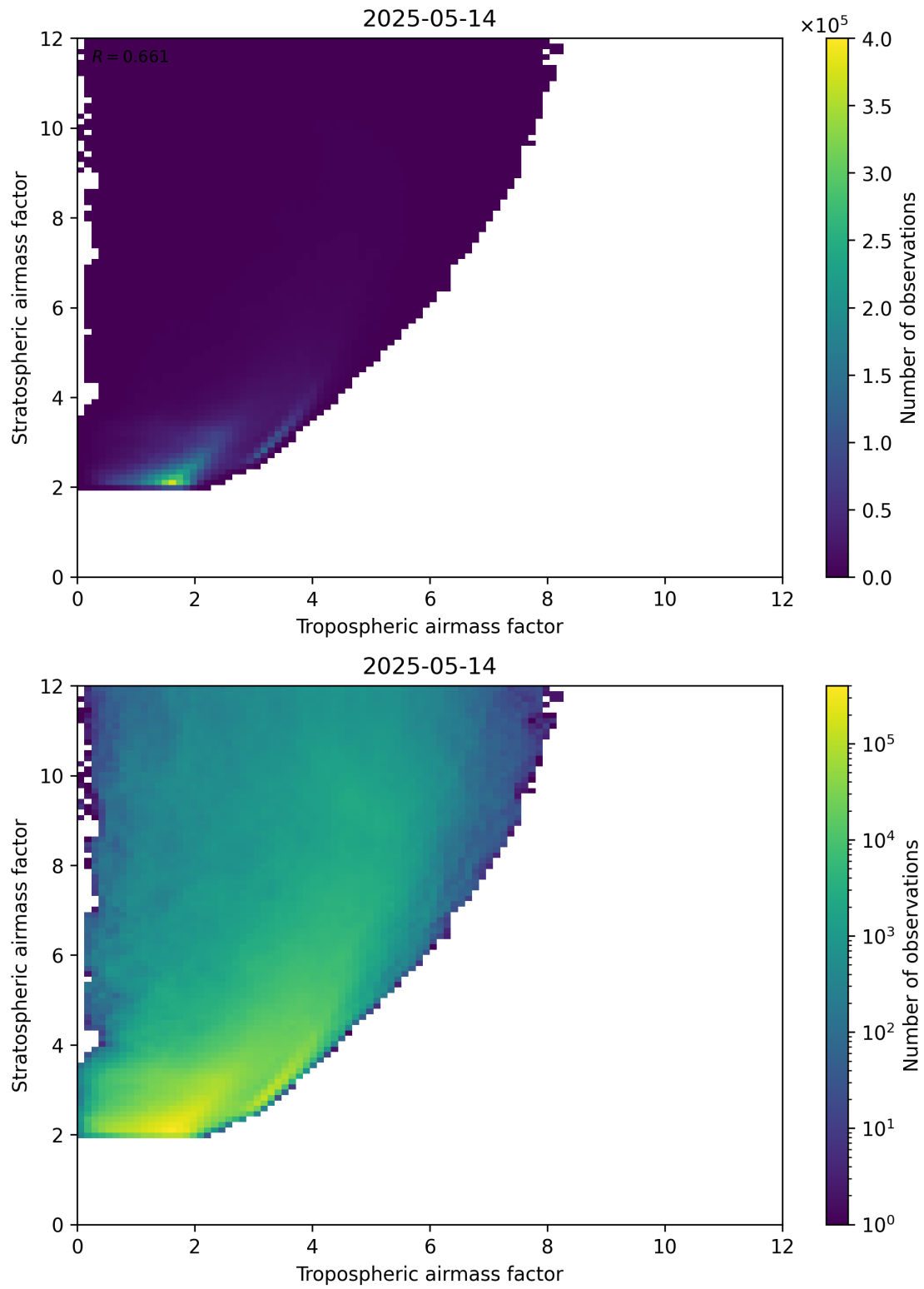
Figure 71: Scatter density plot of “Tropospheric airmass factor” against “Stratospheric airmass factor” for 2025-05-13 to 2025-05-15.
