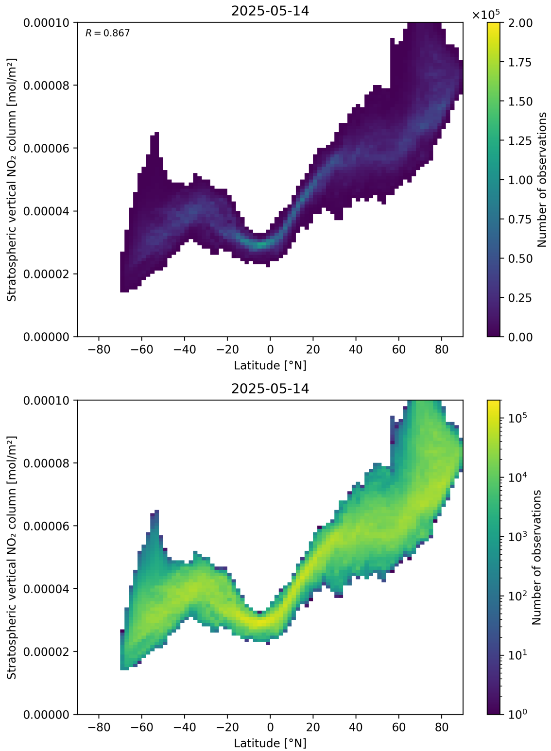
Figure 87: Scatter density plot of “Latitude” against “Stratospheric vertical NO 2 column” for 2025-05-13 to 2025-05-15.
