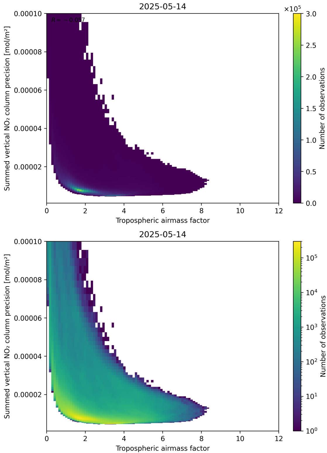
Figure 76: Scatter density plot of “Tropospheric airmass factor” against “Summed vertical NO 2 column precision” for 2025-05-13 to 2025-05-15.
