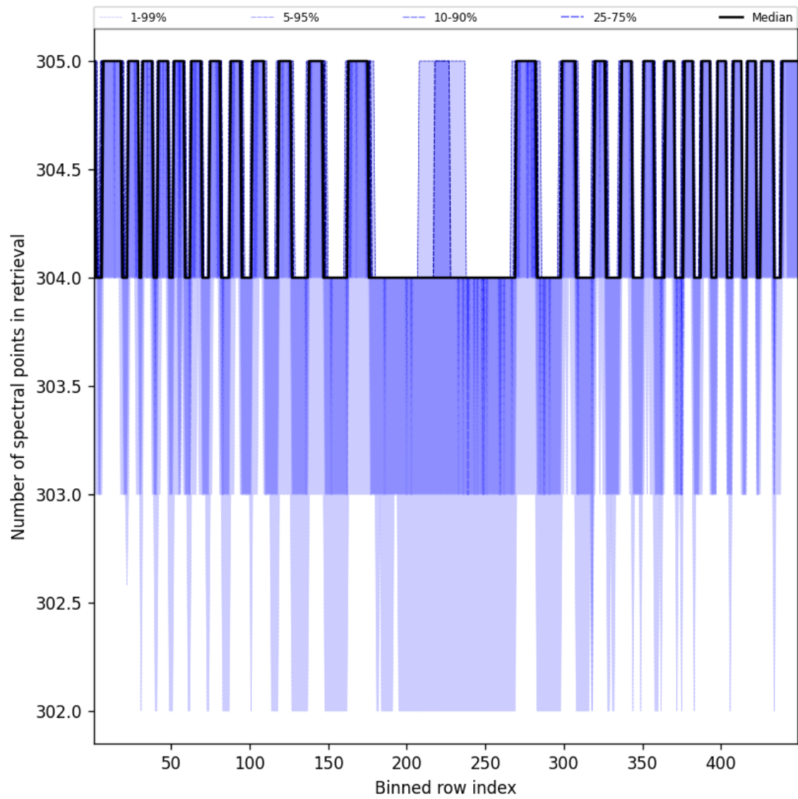
Figure 50: Along track statistics of “Number of spectral points in retrieval” for 2025-05-13 to 2025-05-15
