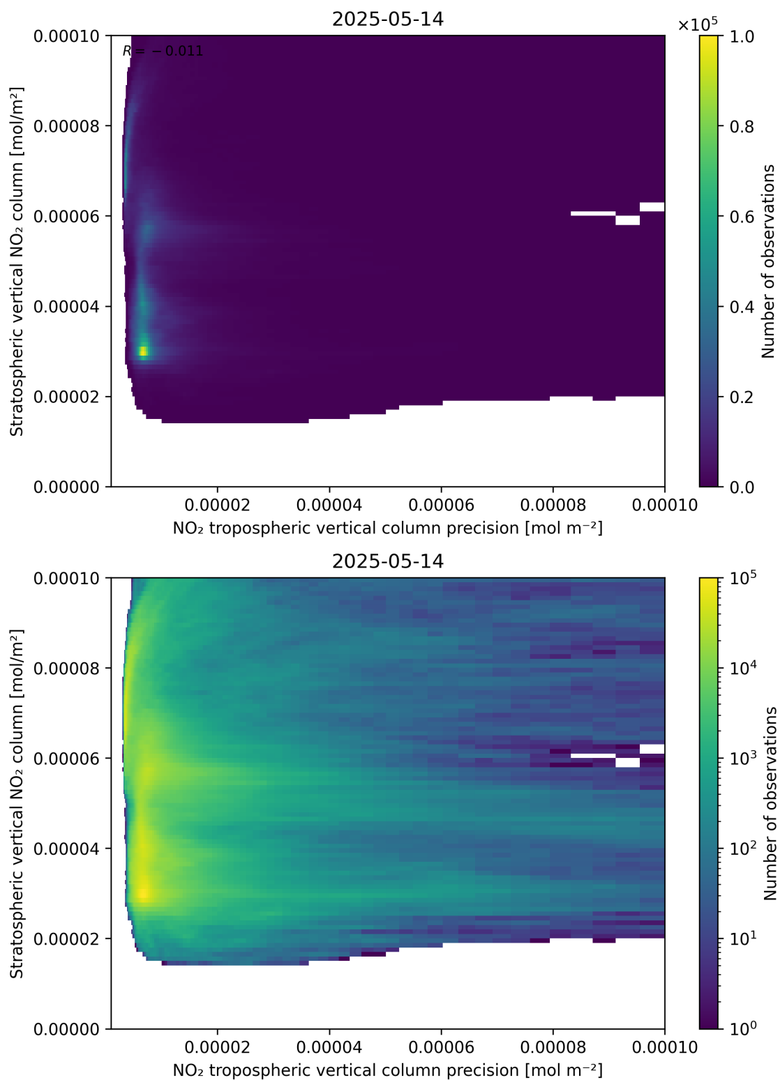
Figure 135: Scatter density plot of “NO 2 tropospheric vertical column precision” against “Stratospheric vertical NO 2 column” for 2025-05-13 to 2025-05-15.
