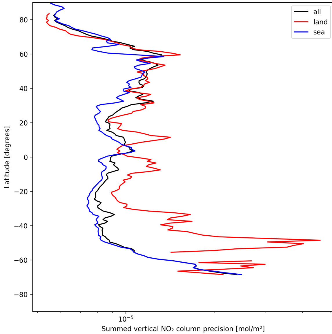
Figure 24: Zonal average of “Summed vertical NO 2 column precision” for 2025-05-13 to 2025-05-15.
