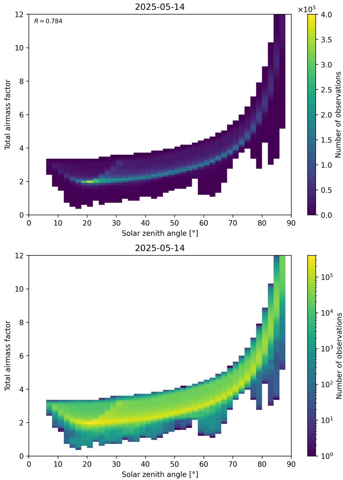
Figure 146: Scatter density plot of “Solar zenith angle” against “Total air mass factor” for 2025-05-13 to 2025-05-15.
