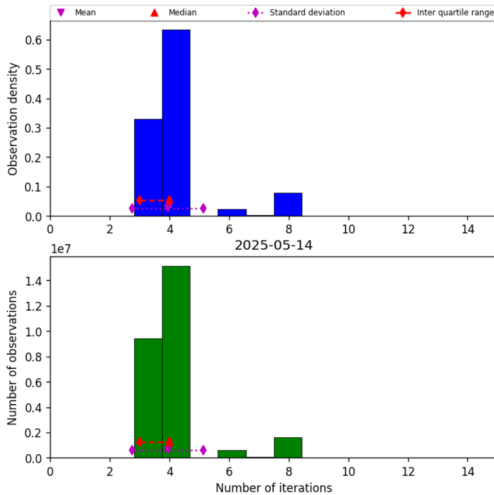
Figure 34: Histogram of “Number of iterations” for 2025-05-13 to 2025-05-15
