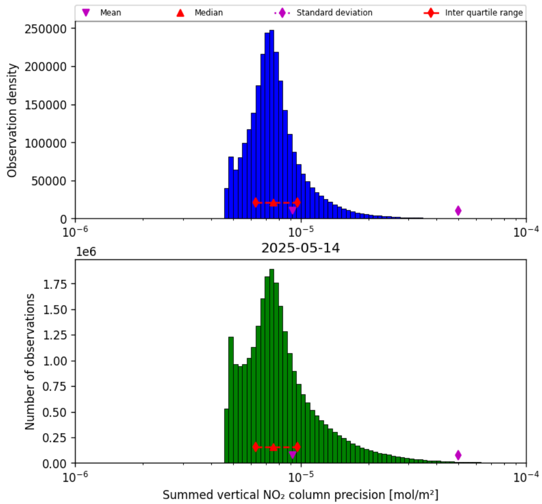
Figure 41: Histogram of "Summed vertical NO 2 column precision" for 2025-05-13 to 2025-05-15
