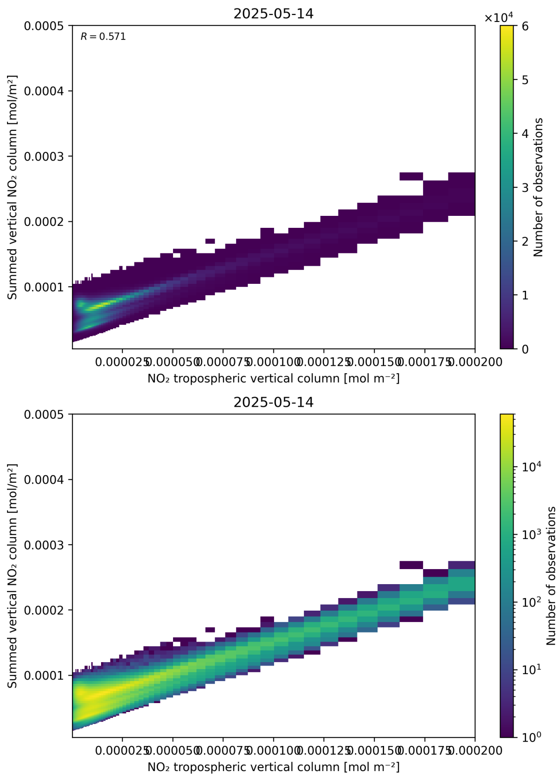
Figure 126: Scatter density plot of “NO 2 tropospheric vertical column” against “Summed vertical NO 2 column” for 2025-05-13 to 2025-05-15.
