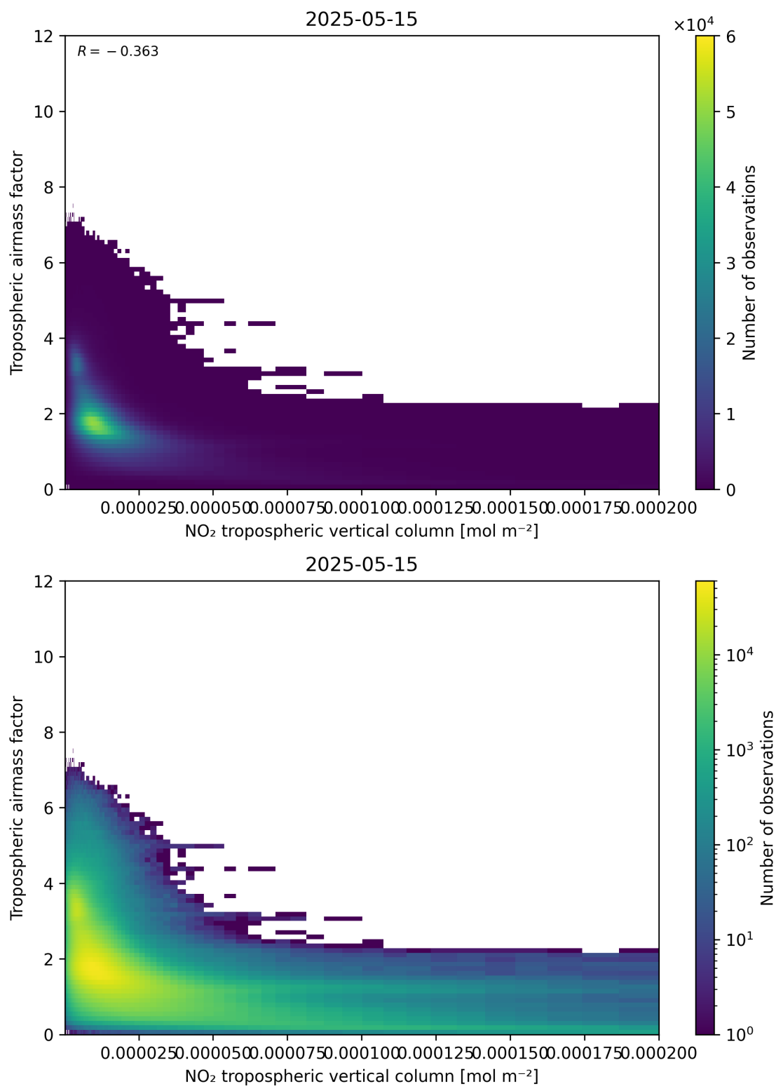
Figure 123: Scatter density plot of “NO 2 tropospheric vertical column” against “Tropospheric air mass factor” for 2025-05-15 to 2025-05-16.
