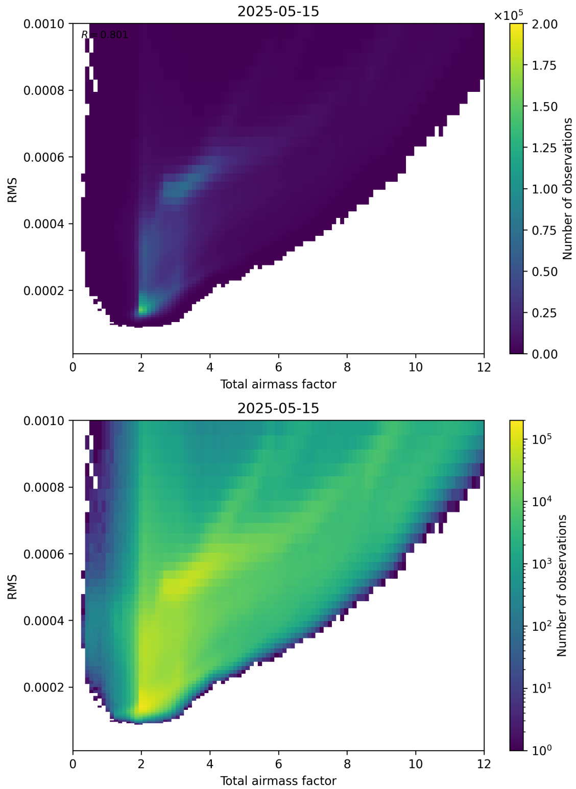
Figure 69: Scatter density plot of “Total airmass factor” against “RMS” for 2025-05-15 to 2025-05-16.
