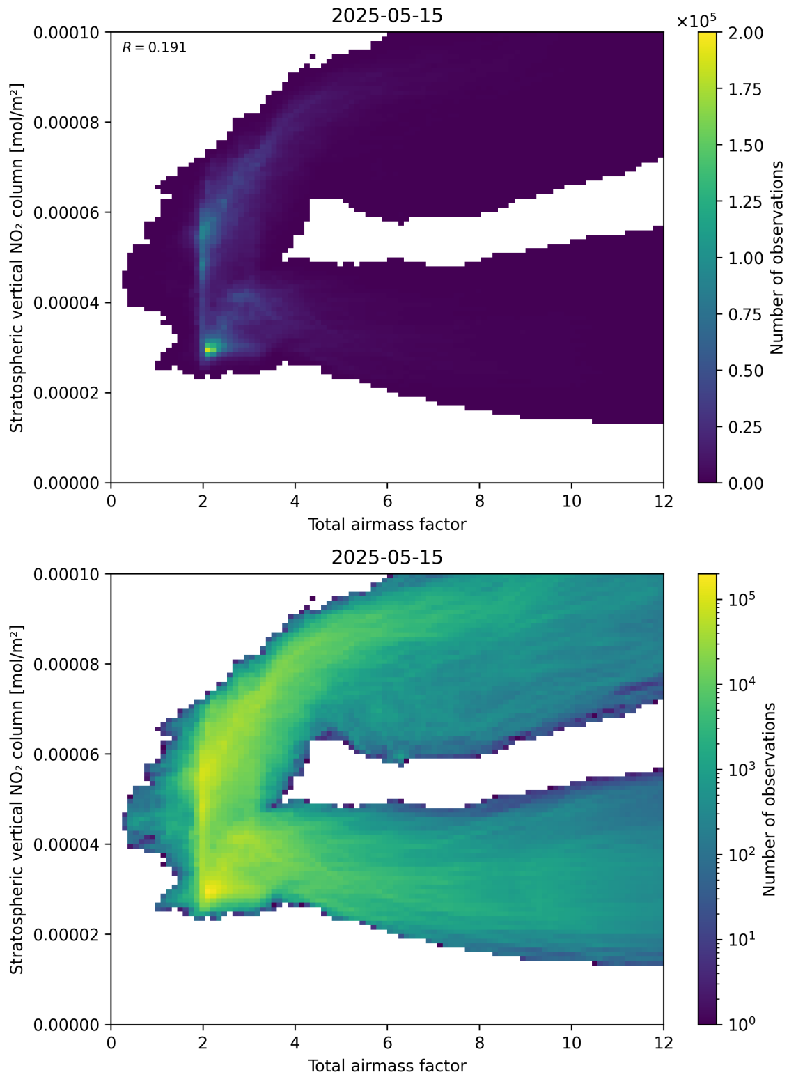
Figure 64: Scatter density plot of “Total airmass factor” against “Stratospheric vertical \text{NO}_2 column” for 2025-05-15 to 2025-05-16.
