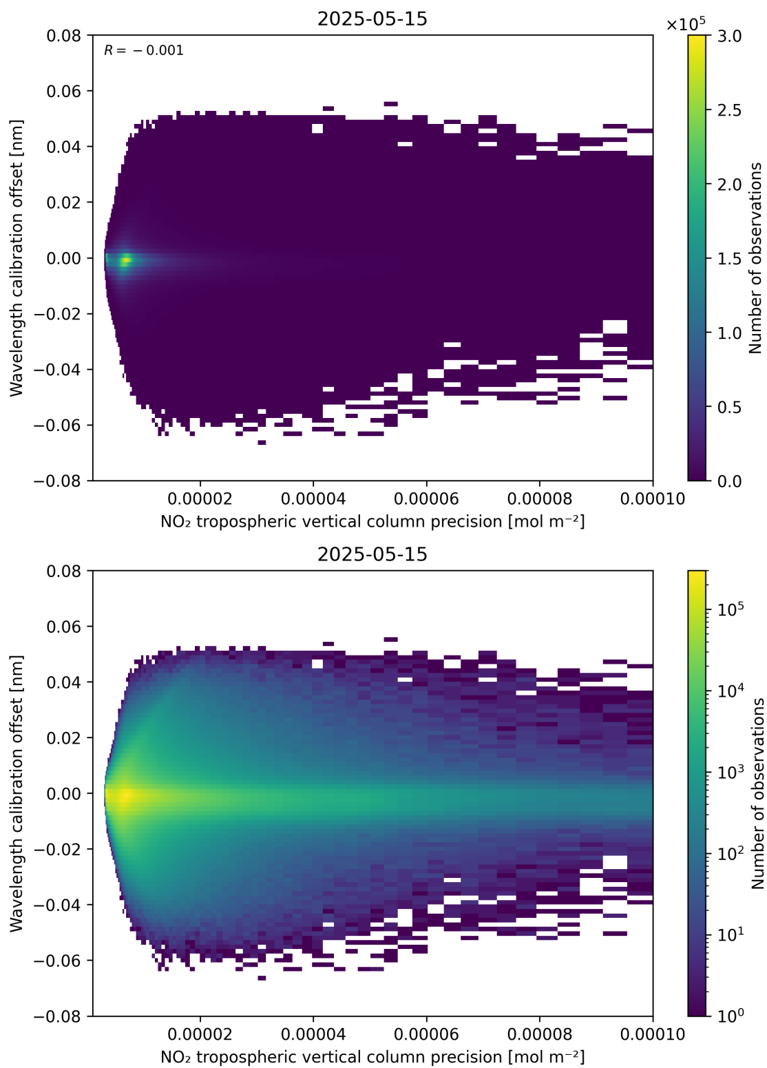
Figure 141: Scatter density plot of “NO 2 tropospheric vertical column precision” against “Wavelength calibration offset” for 2025-05-15 to 2025-05-16.
