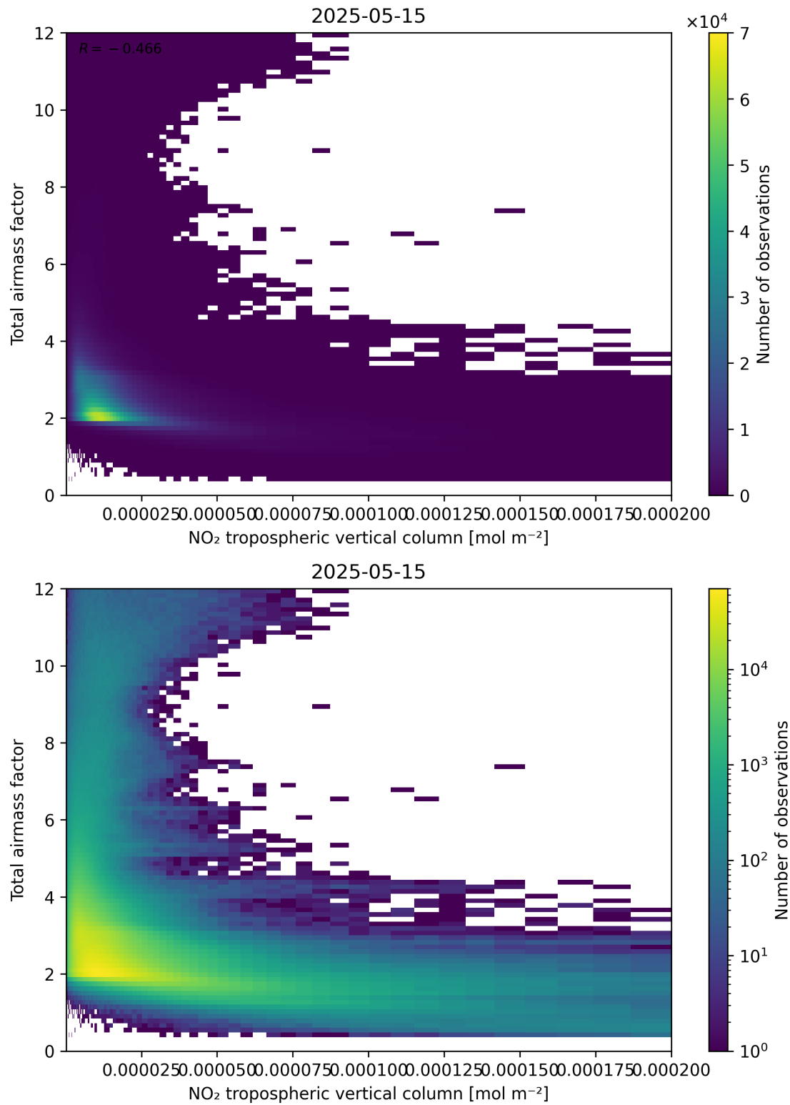
Figure 122: Scatter density plot of “NO 2 tropospheric vertical column” against “Total air mass factor” for 2025-05-15 to 2025-05-16.
