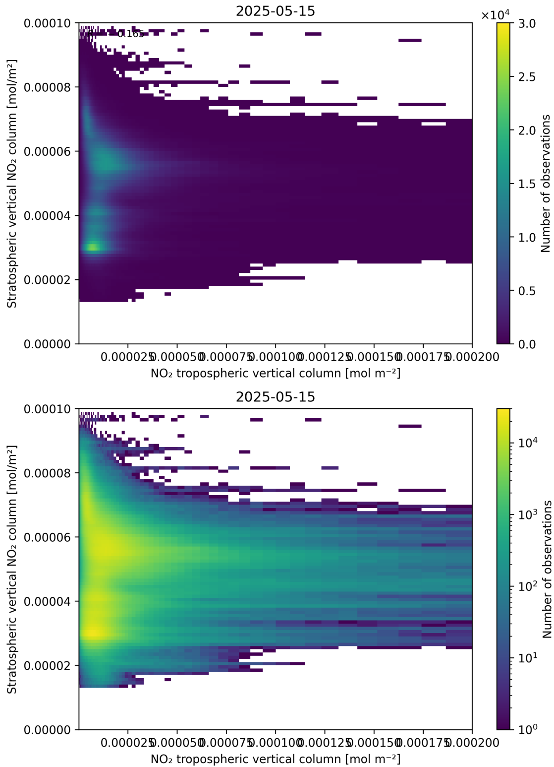
Figure 125: Scatter density plot of “NO 2 tropospheric vertical column” against “Stratospheric vertical NO 2 column” for 2025-05-15 to 2025-05-16.
