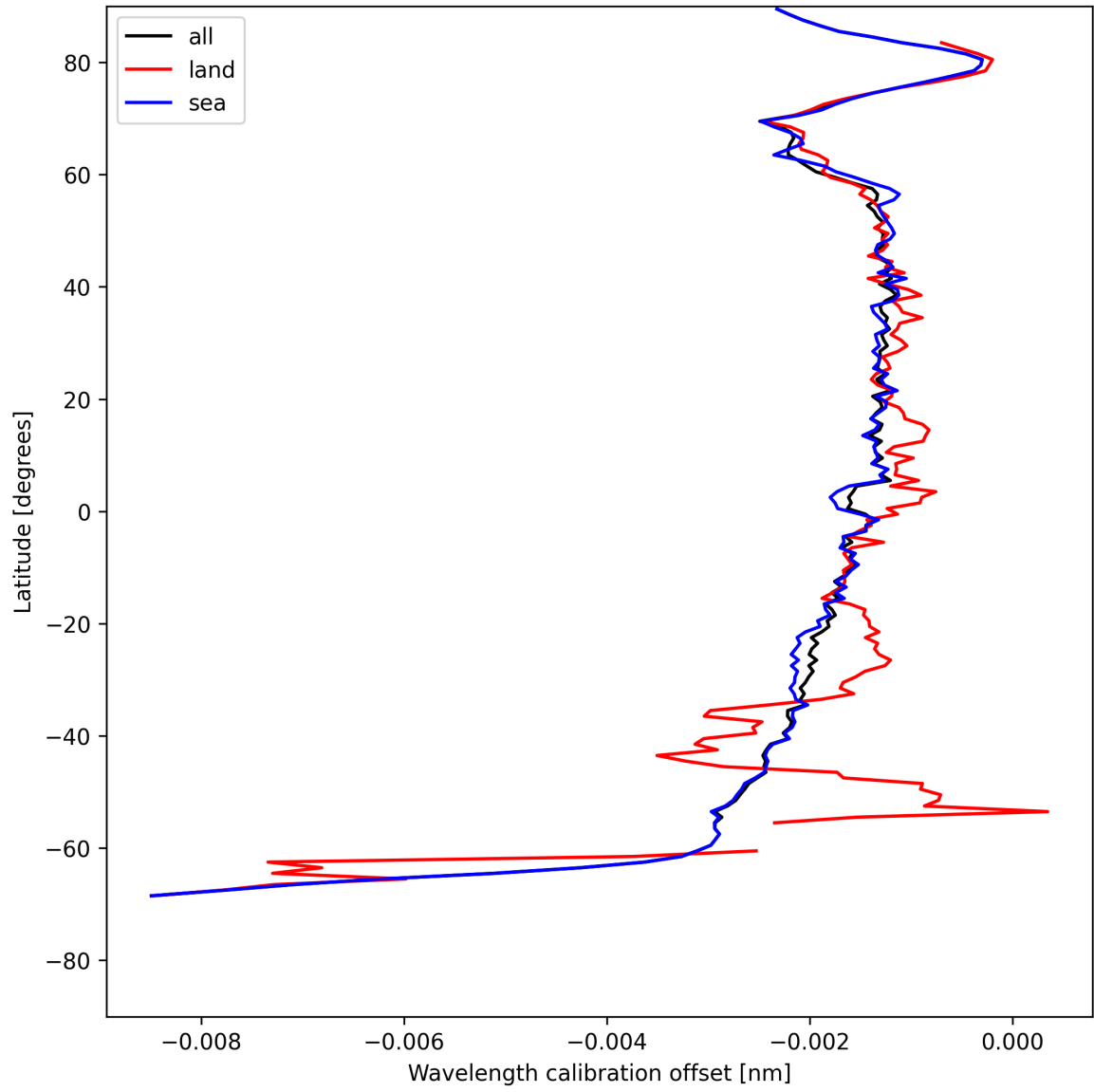
Figure 18: Zonal average of “Wavelength calibration offset” for 2025-05-15 to 2025-05-16.
