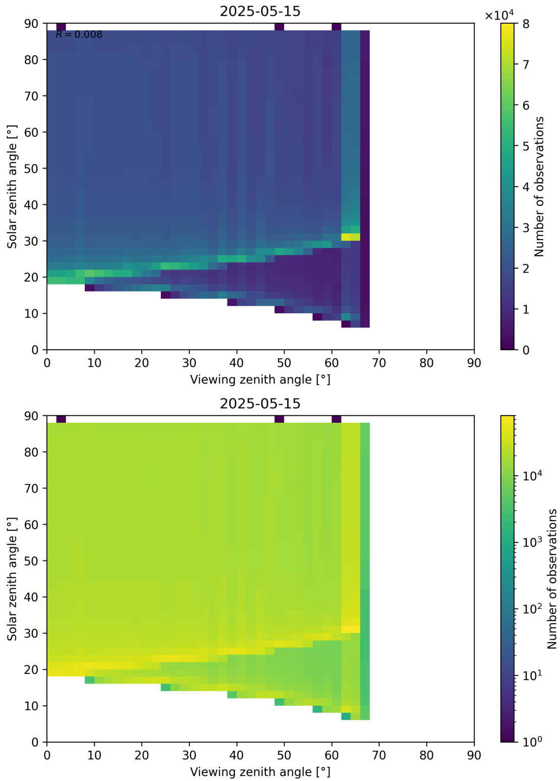
Figure 172: Scatter density plot of “Viewing zenith angle” against “Solar zenith angle” for 2025-05-15 to 2025-05-16.
