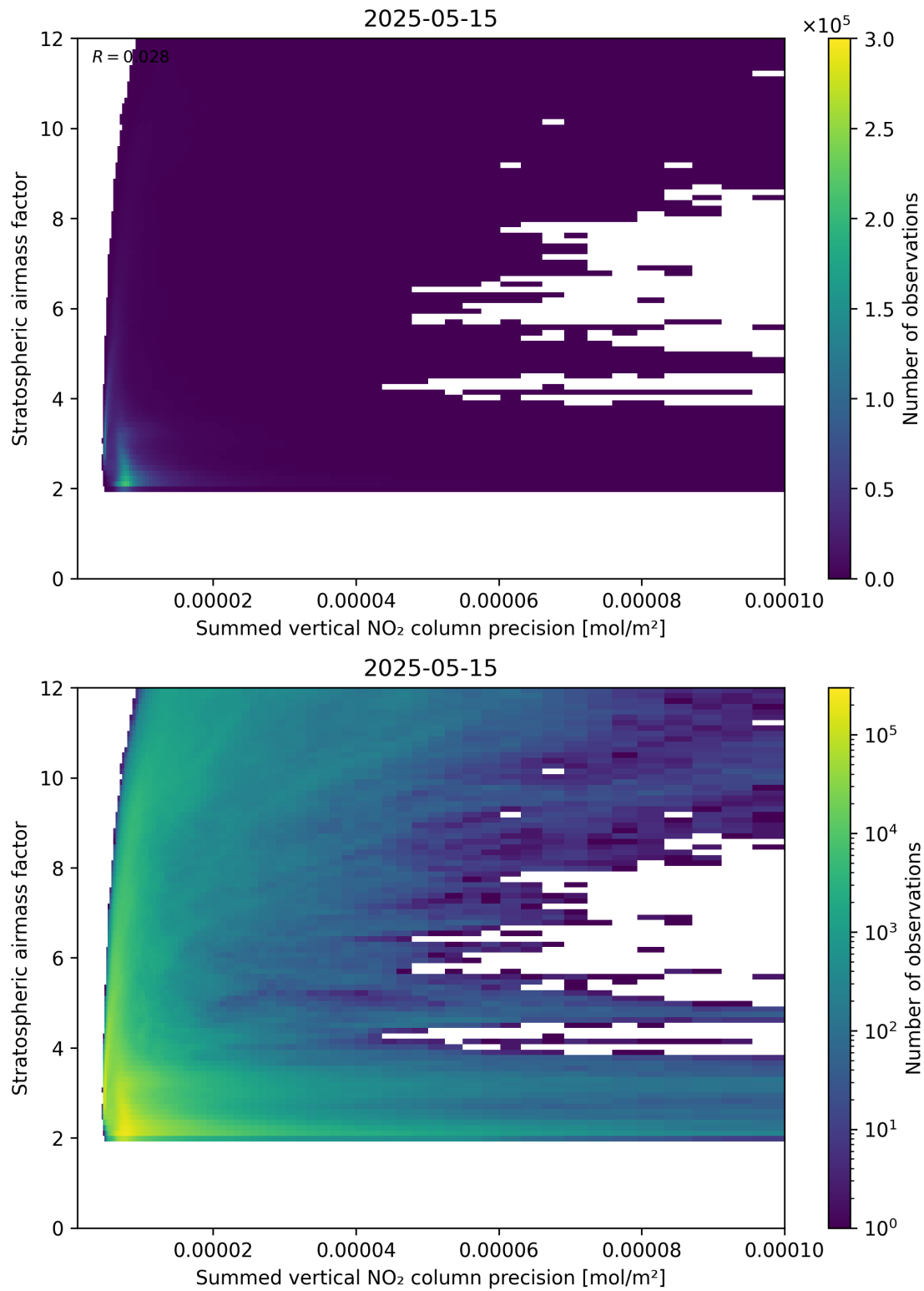
Figure 106: Scatter density plot of “Summed vertical NO 2 column precision” against “Stratospheric airmass factor” for 2025-05-15 to 2025-05-16.
