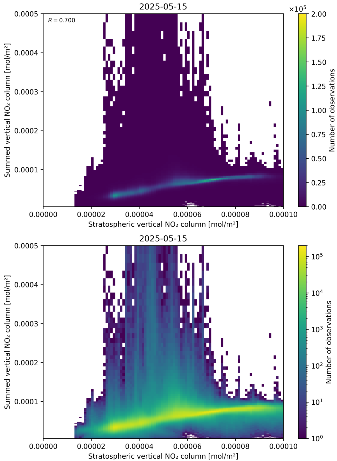
Figure 98: Scatter density plot of “Stratospheric vertical NO 2 column” against “Summed vertical NO 2 column” for 2025-05-15 to 2025-05-16.
