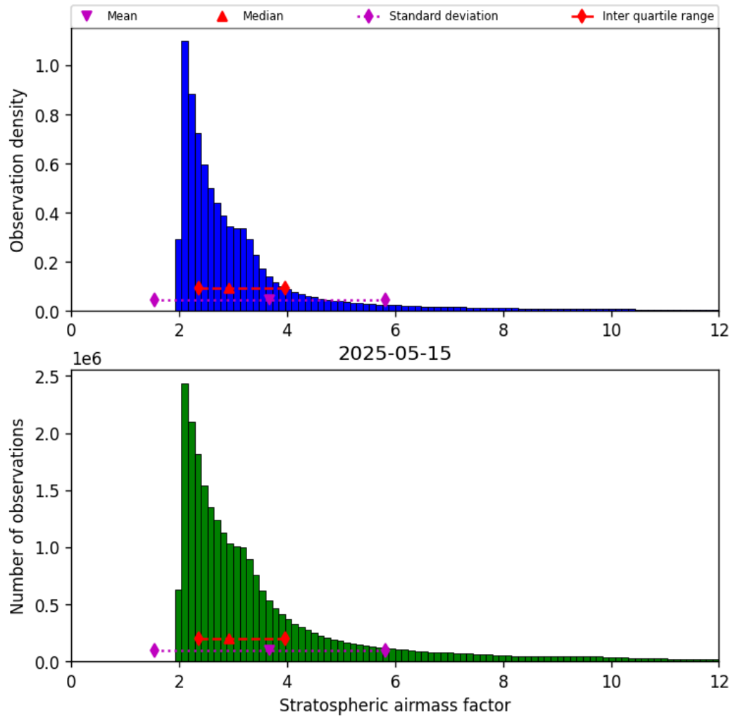
Figure 44: Histogram of “Stratospheric airmass factor” for 2025-05-15 to 2025-05-16
