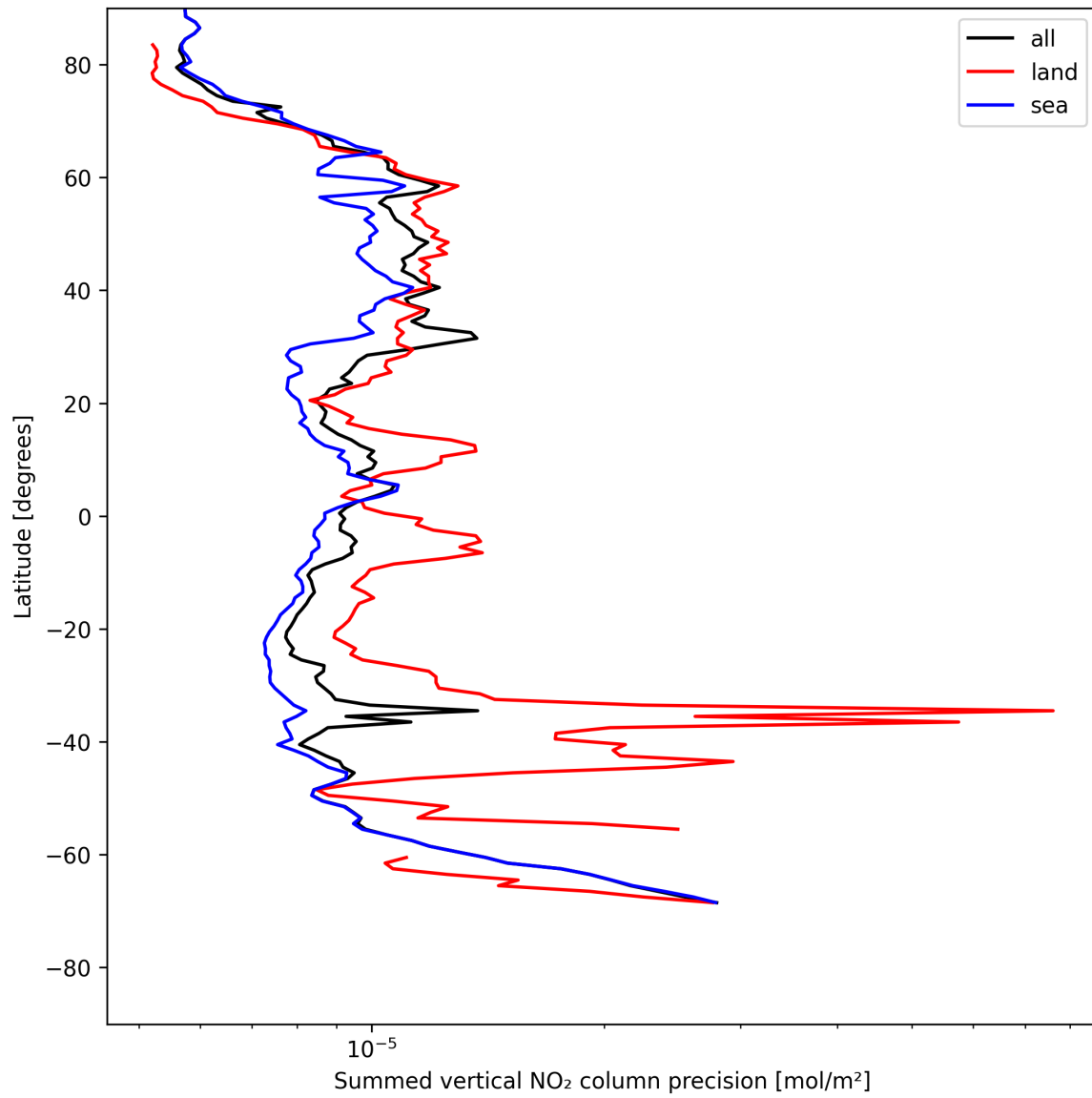
Figure 24: Zonal average of “Summed vertical NO 2 column precision” for 2025-05-15 to 2025-05-16.
