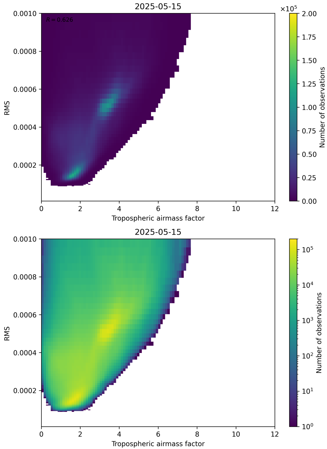
Figure 79: Scatter density plot of “Tropospheric airmass factor” against “RMS” for 2025-05-15 to 2025-05-16.
