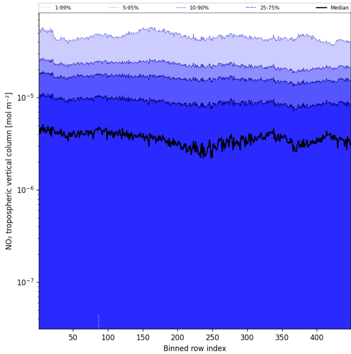
Figure 46: Along track statistics of “NO 2 tropospheric vertical column” for 2025-05-15 to 2025-05-16
