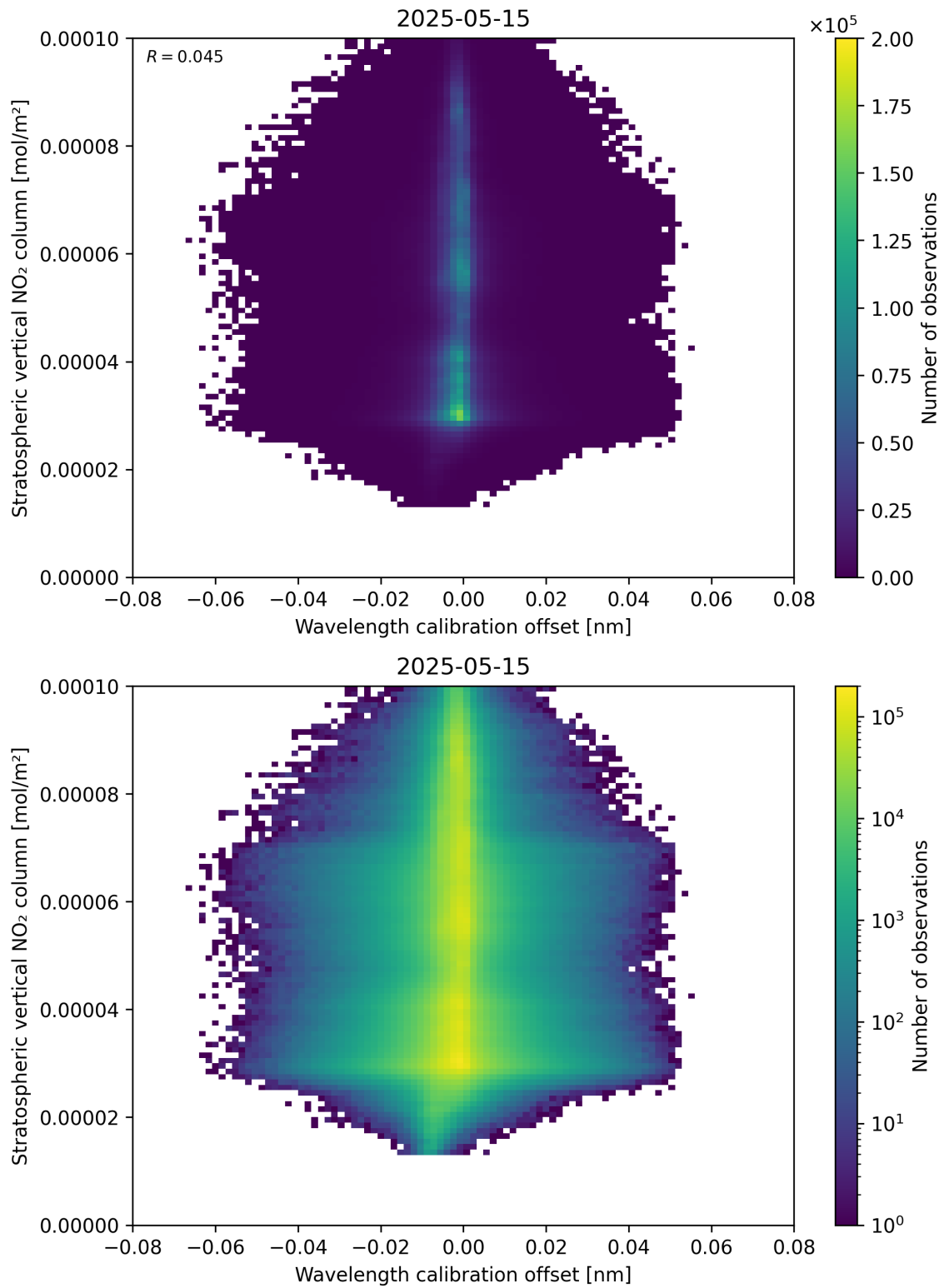
Figure 176: Scatter density plot of “Wavelength calibration offset” against “Stratospheric vertical NO 2 column” for 2025-05-15 to 2025-05-16.
