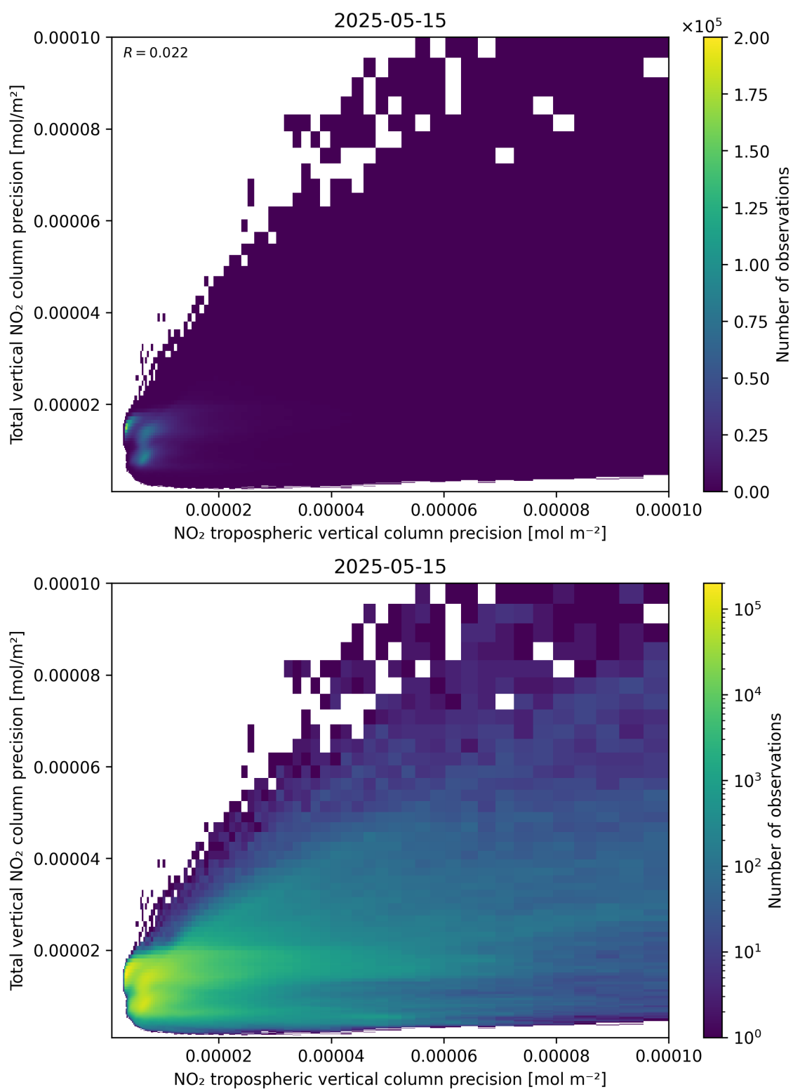
Figure 139: Scatter density plot of “NO 2 tropospheric vertical column precision” against “Total vertical NO 2 column precision” for 2025-05-15 to 2025-05-16.
