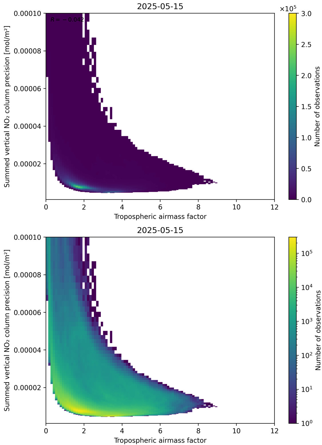
Figure 76: Scatter density plot of “Tropospheric air mass factor” against “Summed vertical NO 2 column precision” for 2025-05-15 to 2025-05-16.
