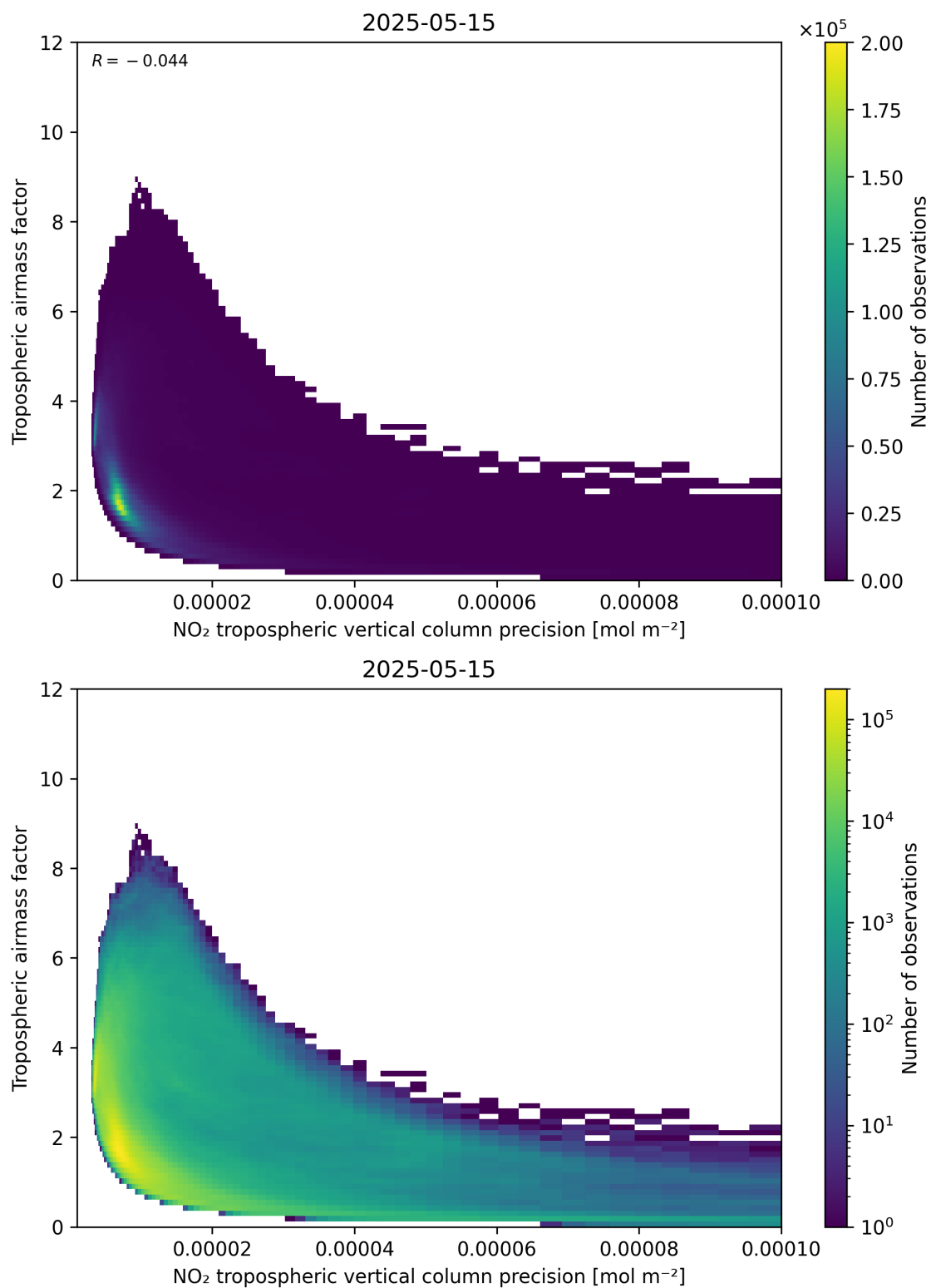
Figure 133: Scatter density plot of “NO 2 tropospheric vertical column precision” against “Tropospheric air mass factor” for 2025-05-15 to 2025-05-16.
