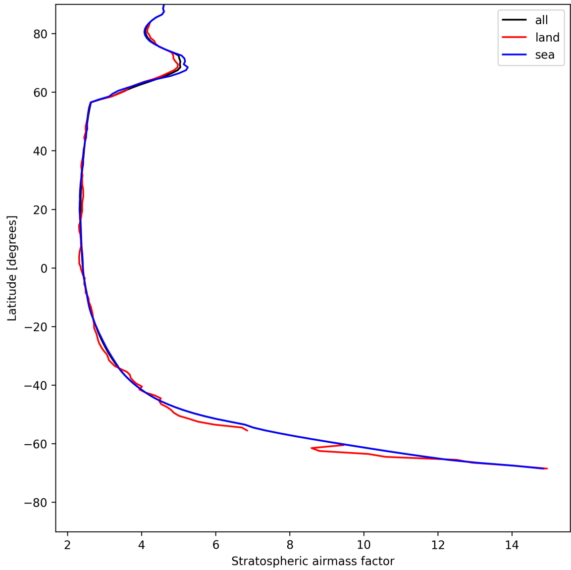
Figure 27: Zonal average of “Stratospheric air mass factor” for 2025-05-15 to 2025-05-16.
