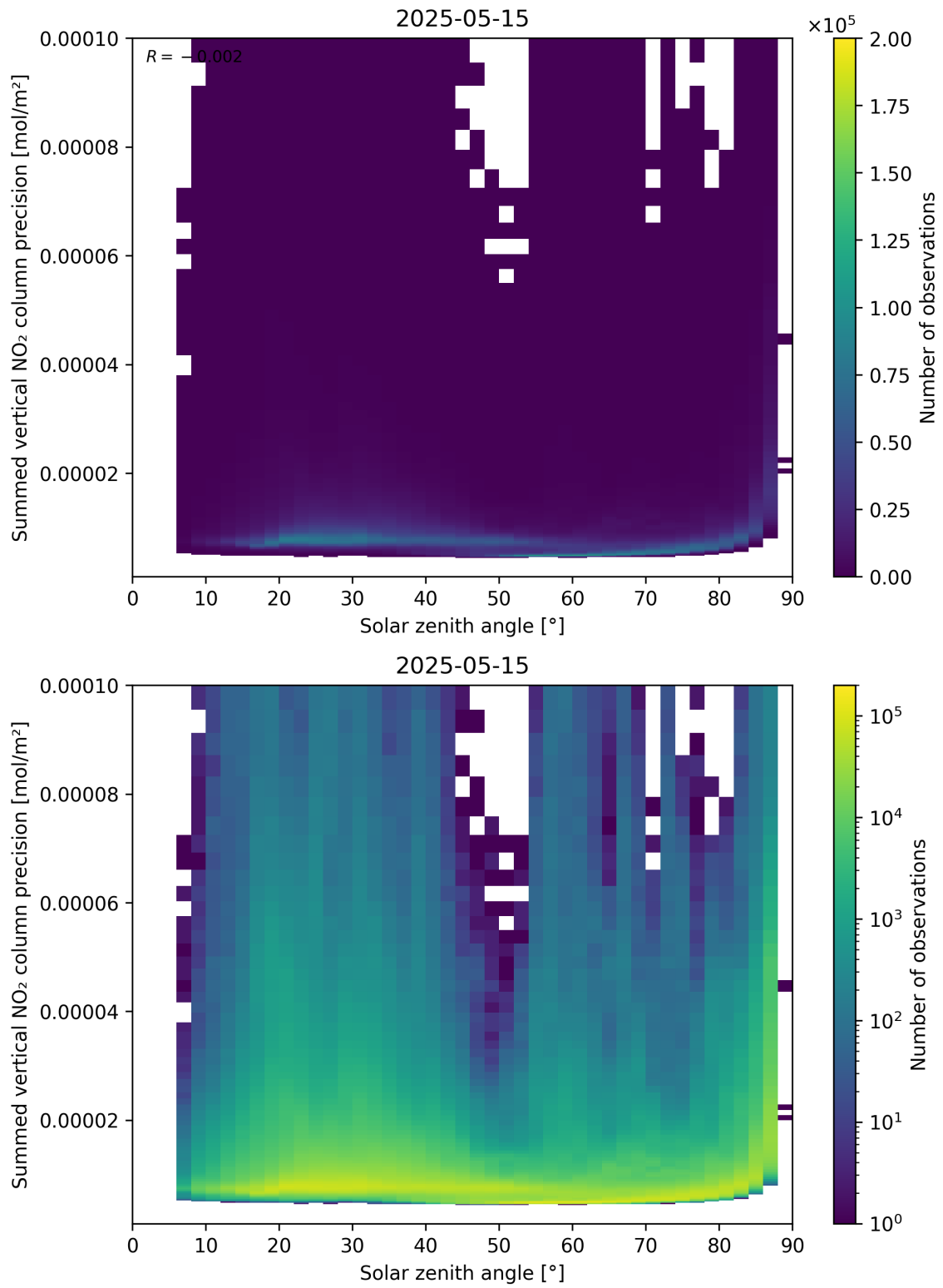
Figure 152: Scatter density plot of “Solar zenith angle” against “Summed vertical NO 2 column precision” for 2025-05-15 to 2025-05-16.
