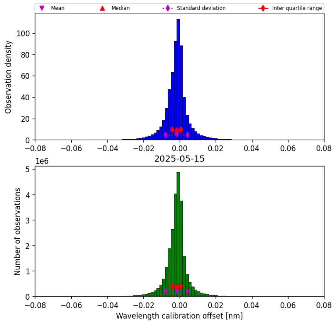
Figure 35: Histogram of “Wavelength calibration offset” for 2025-05-15 to 2025-05-16
