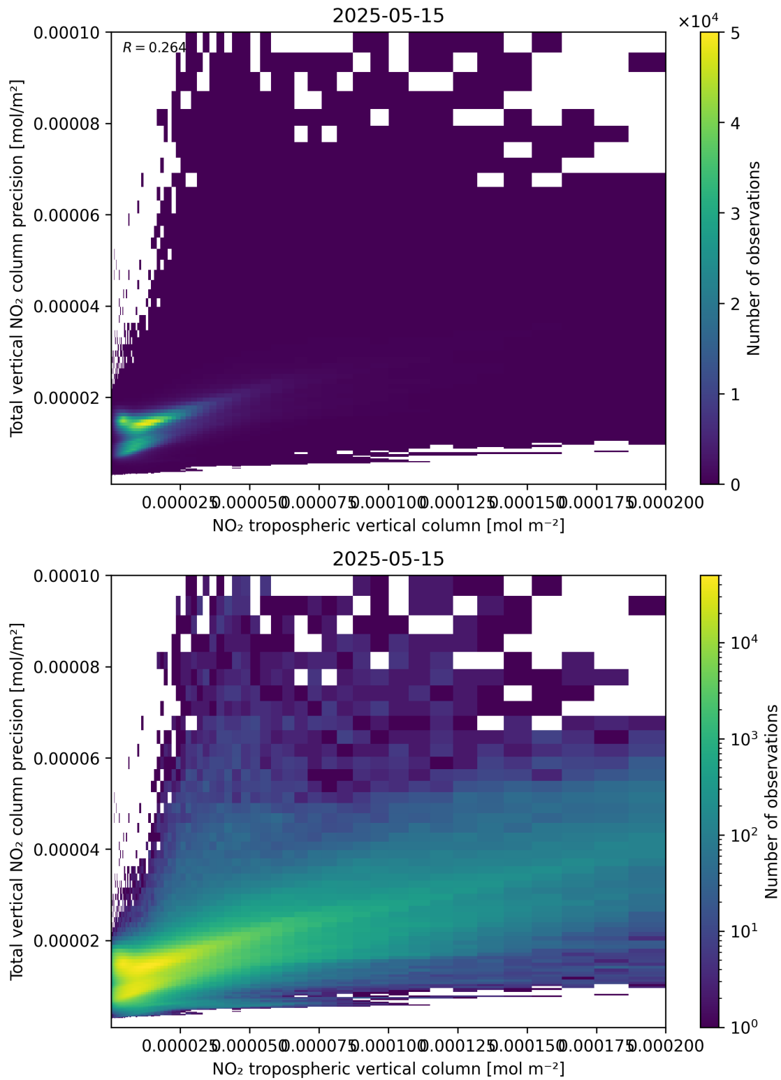
Figure 129: Scatter density plot of “NO 2 tropospheric vertical column” against “Total vertical NO 2 column precision” for 2025-05-15 to 2025-05-16.
