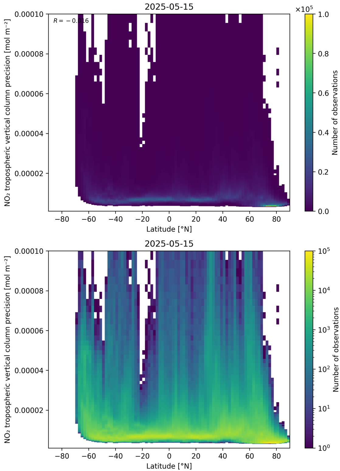
Figure 93: Scatter density plot of “Latitude” against “NO 2 tropospheric vertical column precision” for 2025-05-15 to 2025-05-16.
