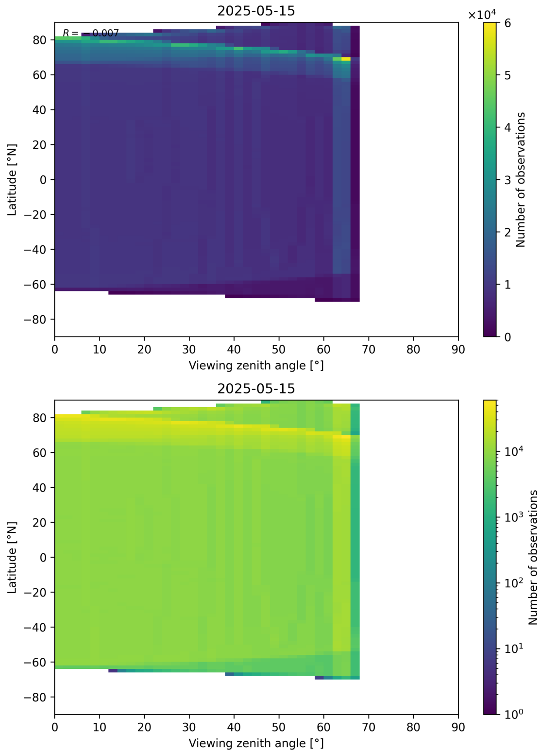
Figure 163: Scatter density plot of “Viewing zenith angle” against “Latitude” for 2025-05-15 to 2025-05-16.
