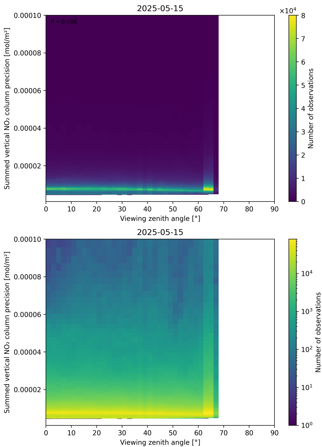
Figure 166: Scatter density plot of “Viewing zenith angle” against “Summed vertical NO 2 column precision” for 2025-05-15 to 2025-05-16.
