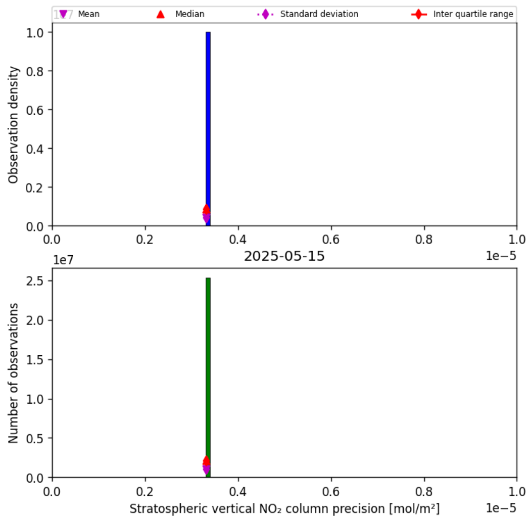
Figure 37: Histogram of “Stratospheric vertical NO 2 column precision” for 2025-05-15 to 2025-05-16
