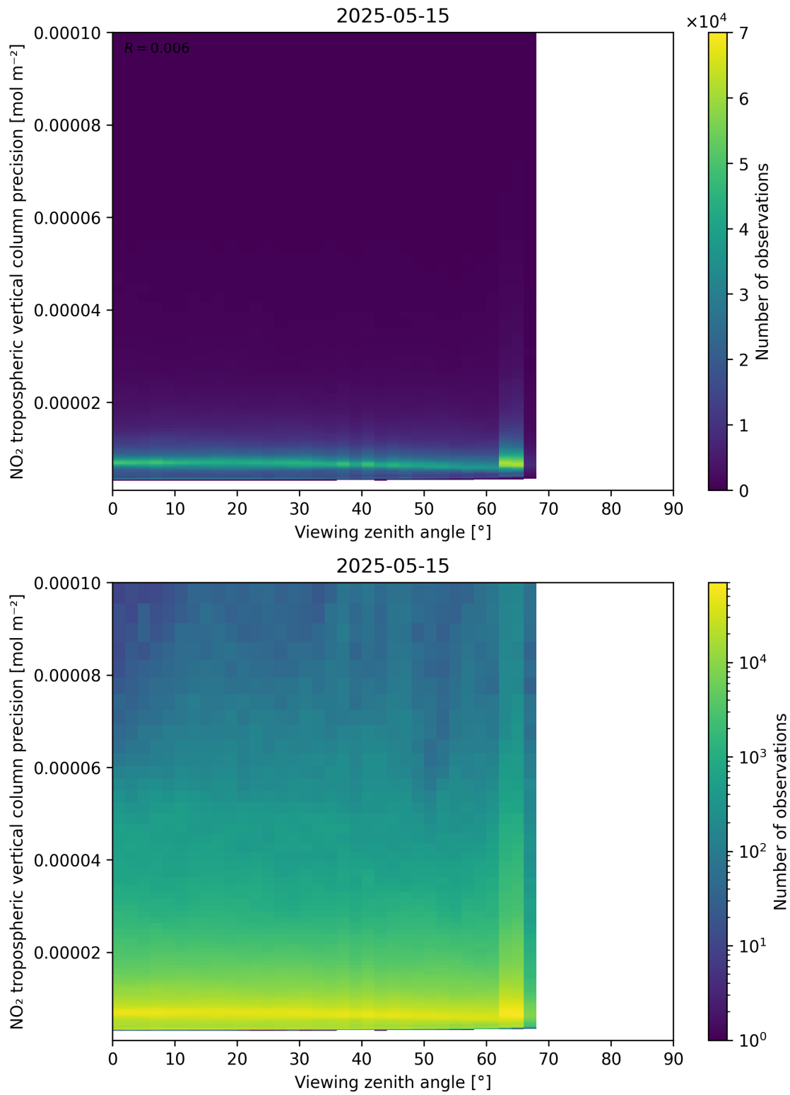
Figure 170: Scatter density plot of “Viewing zenith angle” against “NO 2 tropospheric vertical column precision” for 2025-05-15 to 2025-05-16.
