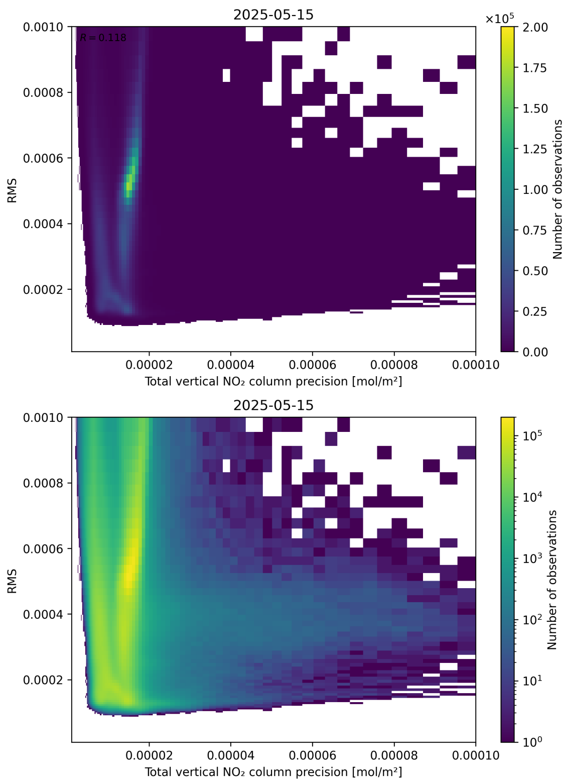
Figure 119: Scatter density plot of “Total vertical NO 2 column precision” against “RMS” for 2025-05-15 to 2025-05-16.
