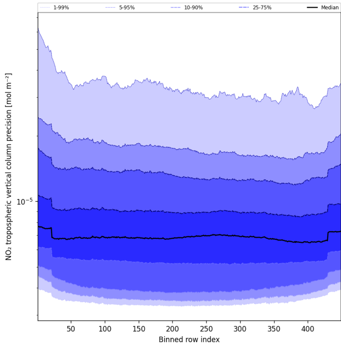
Figure 47: Along track statistics of “NO 2 tropospheric vertical column precision” for 2025-05-15 to 2025-05-16
