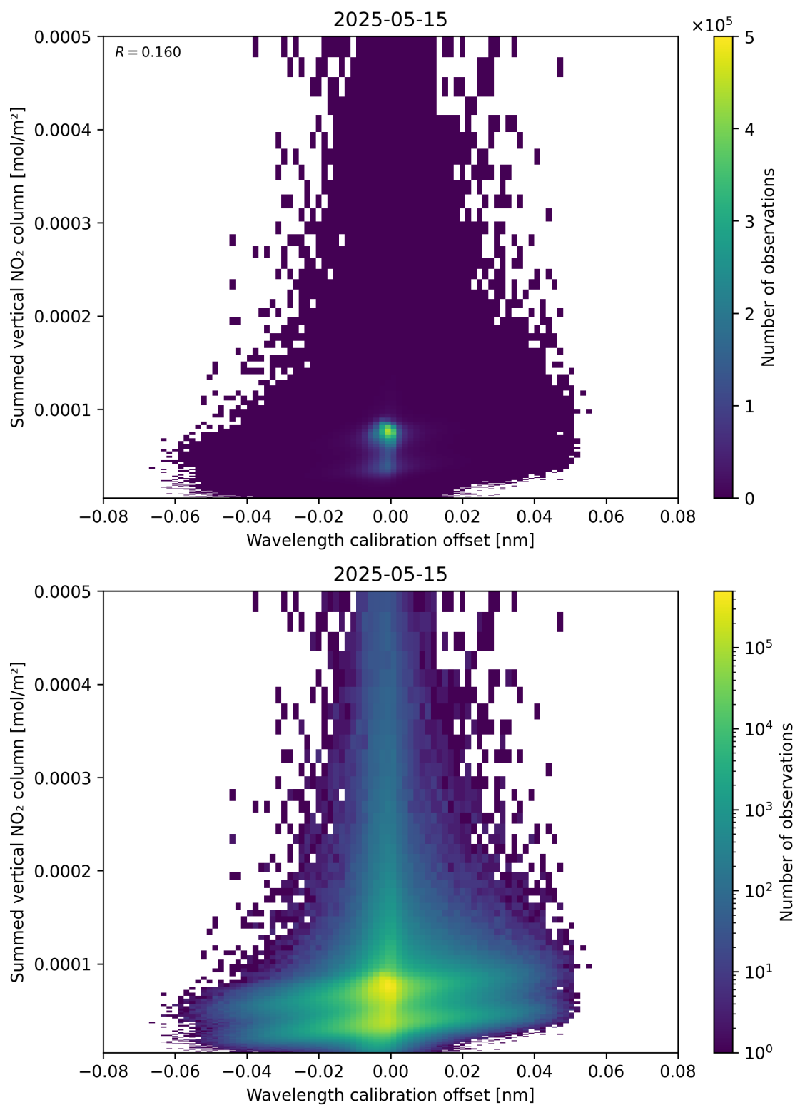
Figure 177: Scatter density plot of “Wavelength calibration offset” against “Summed vertical NO 2 column” for 2025-05-15 to 2025-05-16.
