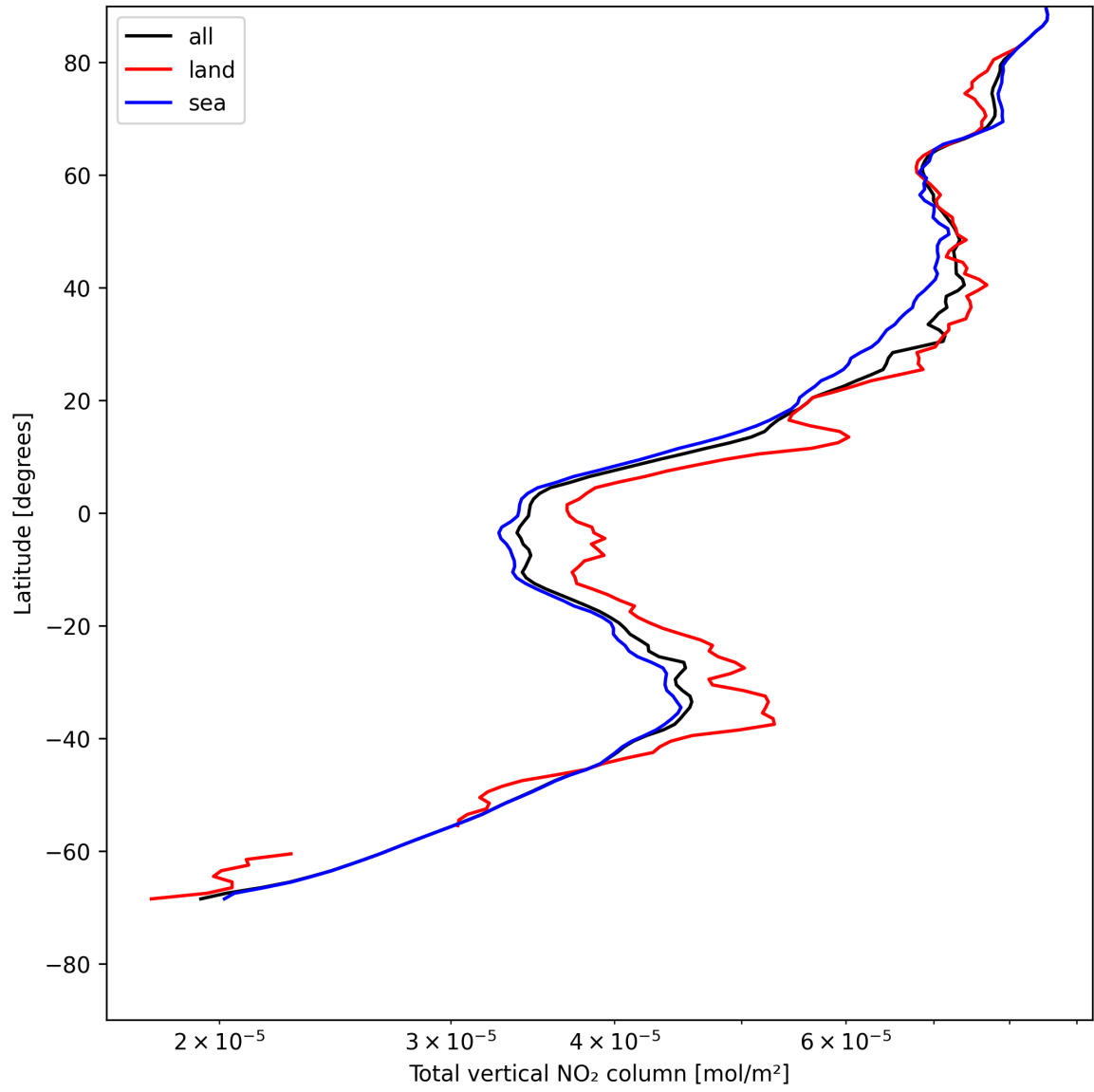
Figure 21: Zonal average of “Total vertical NO 2 column” for 2025-05-15 to 2025-05-16.
