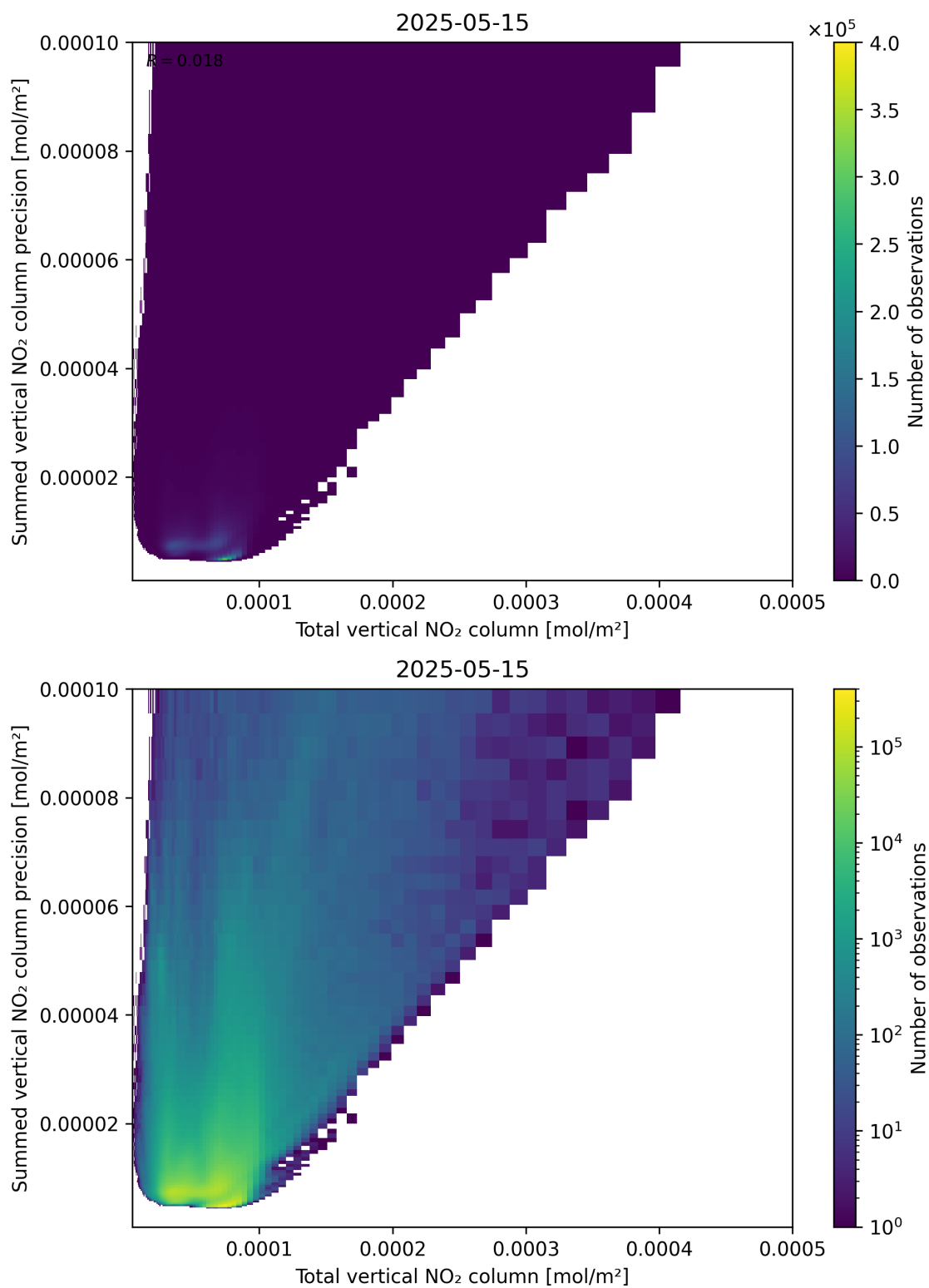
Figure 113: Scatter density plot of “Total vertical NO 2 column” against “Summed vertical NO 2 column precision” for 2025-05-15 to 2025-05-16.
