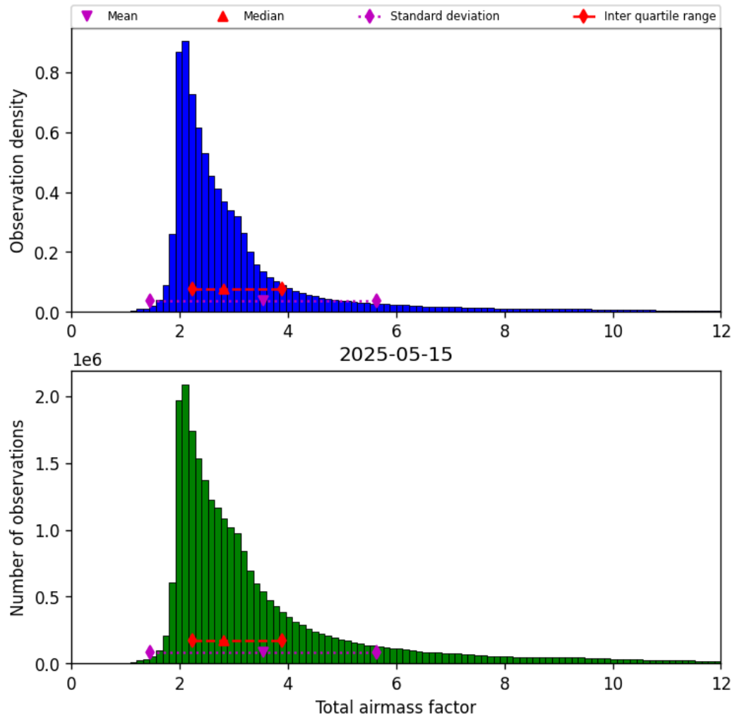
Figure 32: Histogram of “Total airmass factor” for 2025-05-15 to 2025-05-16
