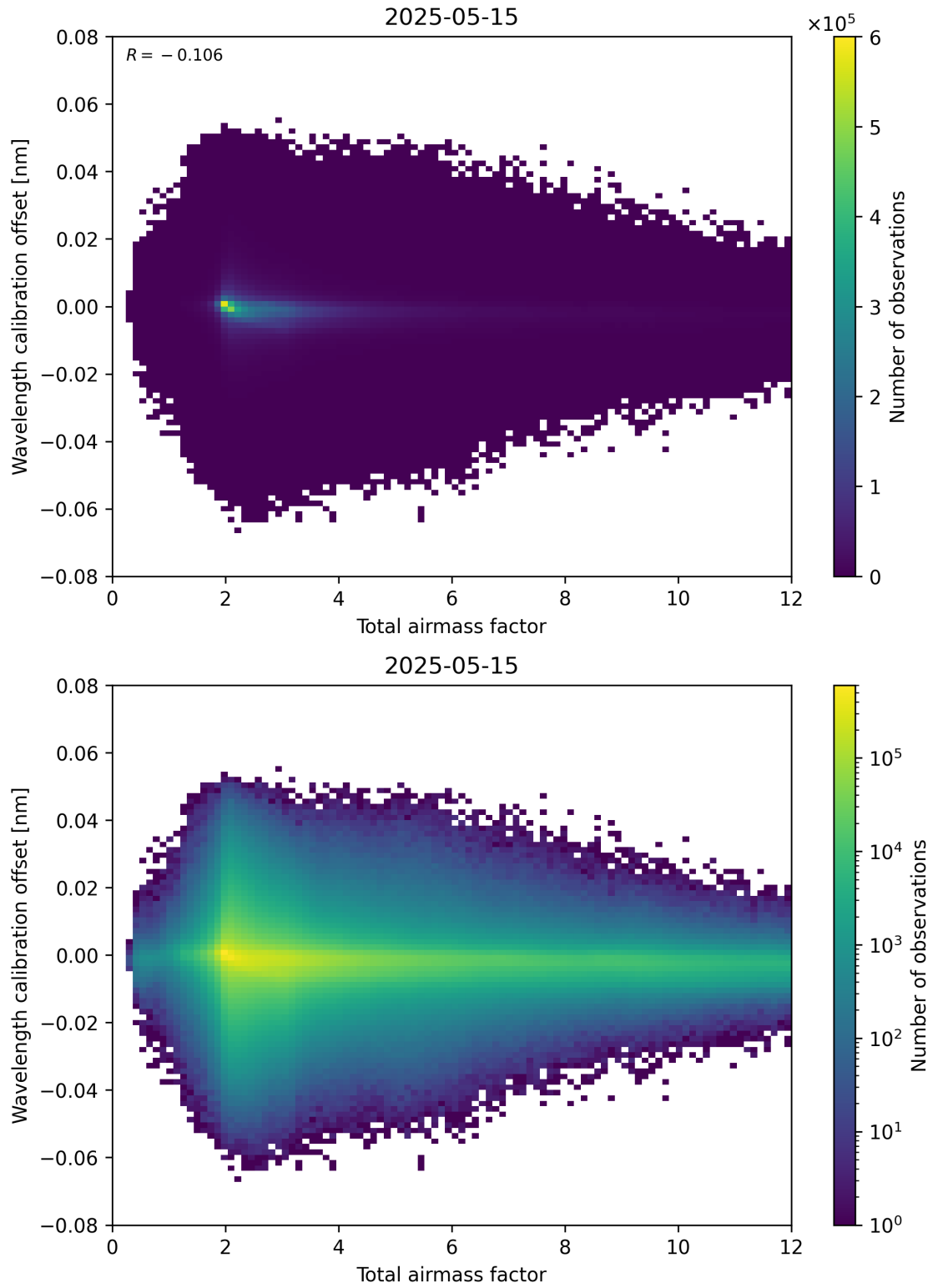
Figure 70: Scatter density plot of “Total airmass factor” against “Wavelength calibration offset” for 2025-05-15 to 2025-05-16.
