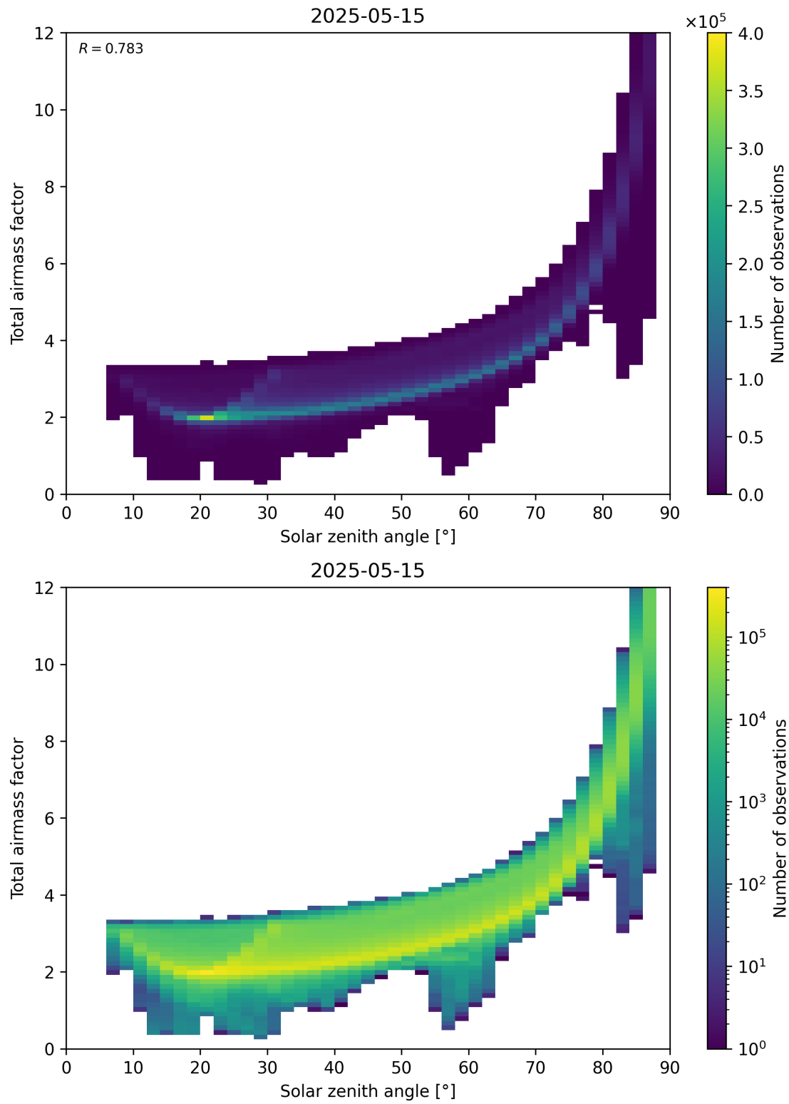
Figure 146: Scatter density plot of “Solar zenith angle” against “Total air mass factor” for 2025-05-15 to 2025-05-16.
