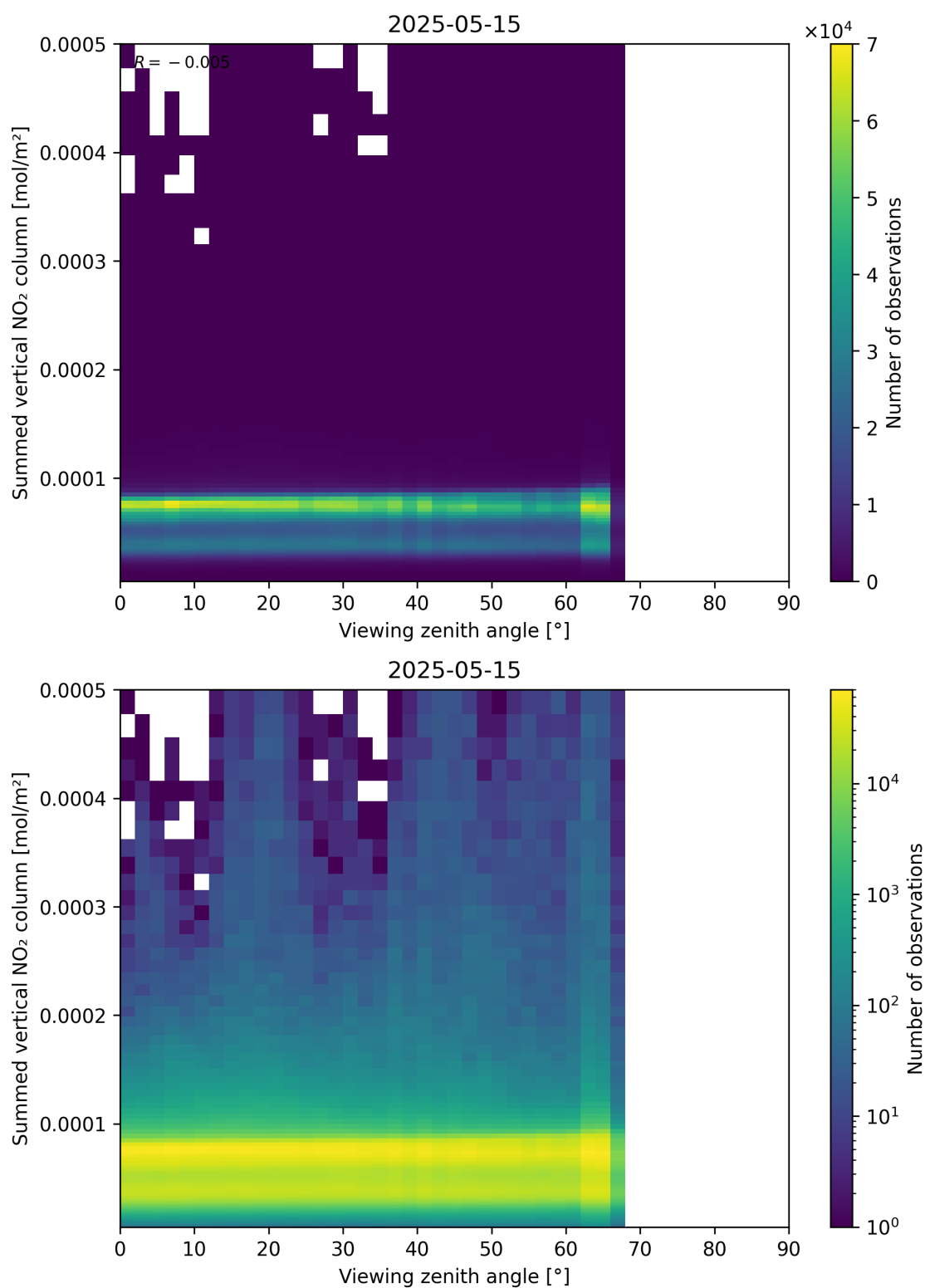
Figure 165: Scatter density plot of “Viewing zenith angle” against “Summed vertical NO 2 column” for 2025-05-15 to 2025-05-16.
