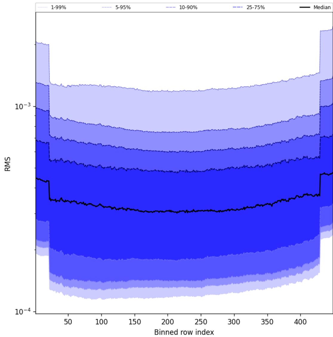
Figure 60: Along track statistics of “RMS” for 2025-05-15 to 2025-05-16
