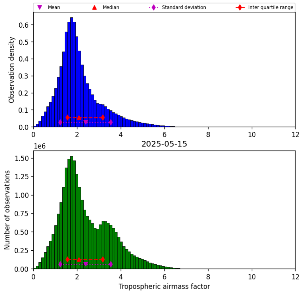
Figure 31: Histogram of “Tropospheric airmass factor” for 2025-05-15 to 2025-05-16
