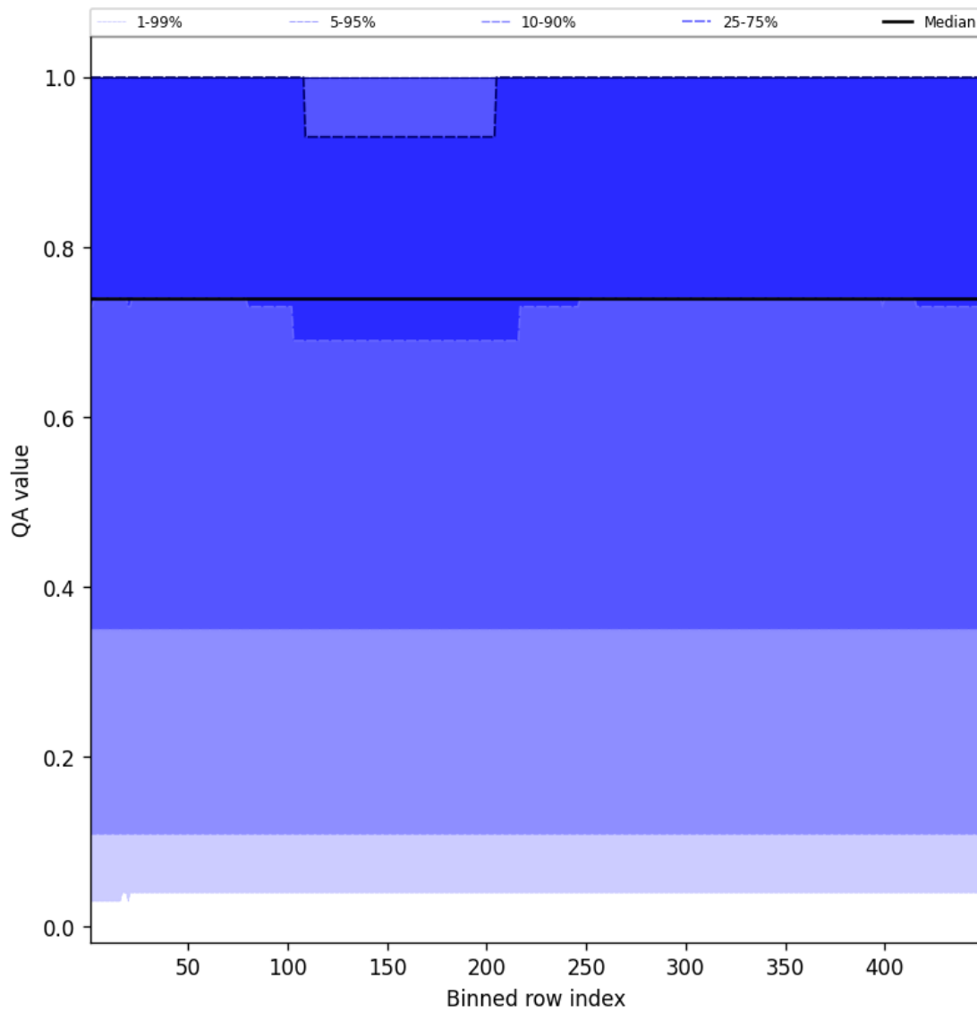
Figure 45: Along track statistics of “QA value” for 2025-05-15 to 2025-05-16
