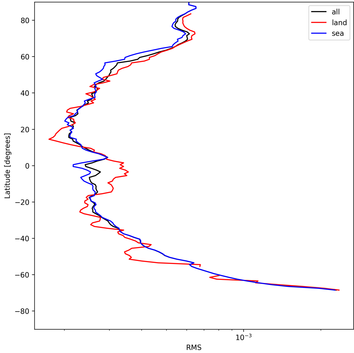
Figure 26: Zonal average of “RMS” for 2025-05-15 to 2025-05-16.
