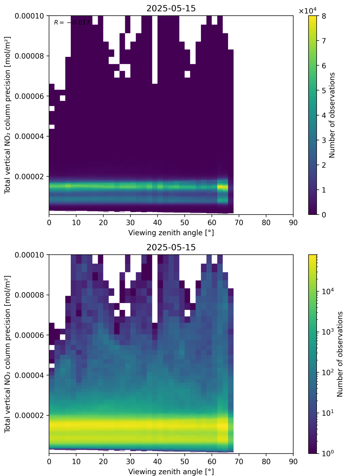
Figure 168: Scatter density plot of “Viewing zenith angle” against “Total vertical NO 2 column precision” for 2025-05-15 to 2025-05-16.
