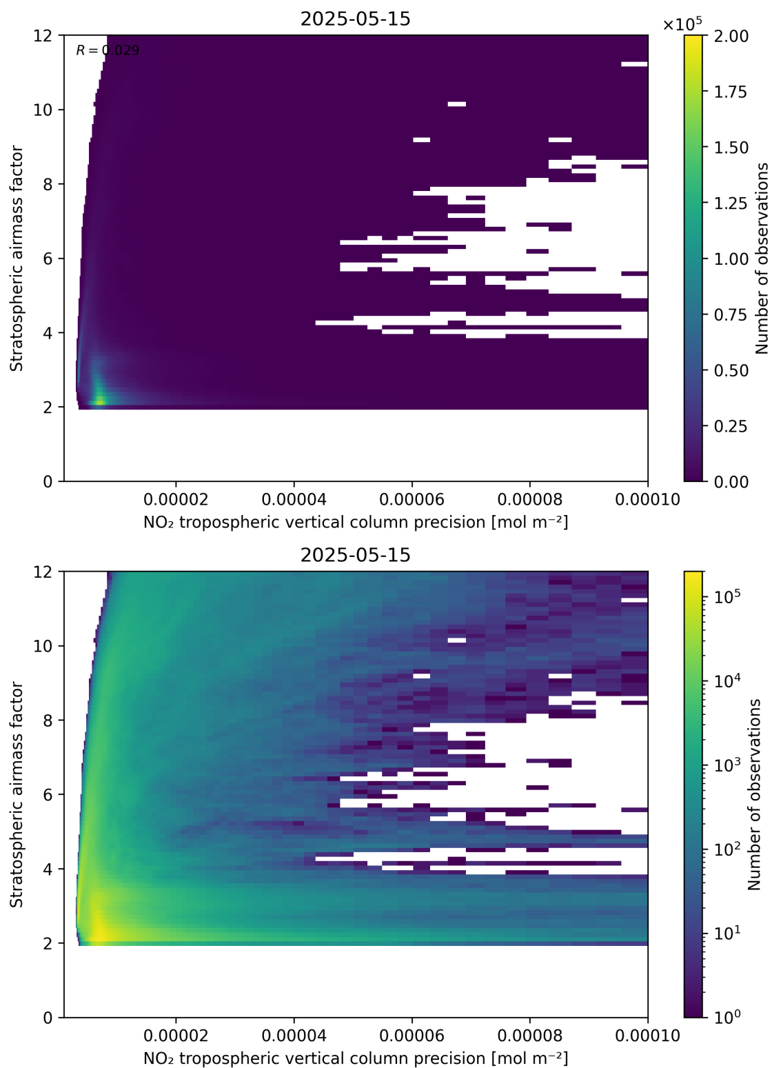
Figure 131: Scatter density plot of “NO 2 tropospheric vertical column precision” against “Stratospheric airmass factor” for 2025-05-15 to 2025-05-16.
