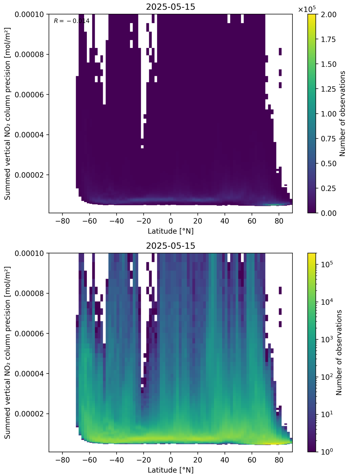
Figure 89: Scatter density plot of “Latitude” against “Summed vertical NO 2 column precision” for 2025-05-15 to 2025-05-16.
