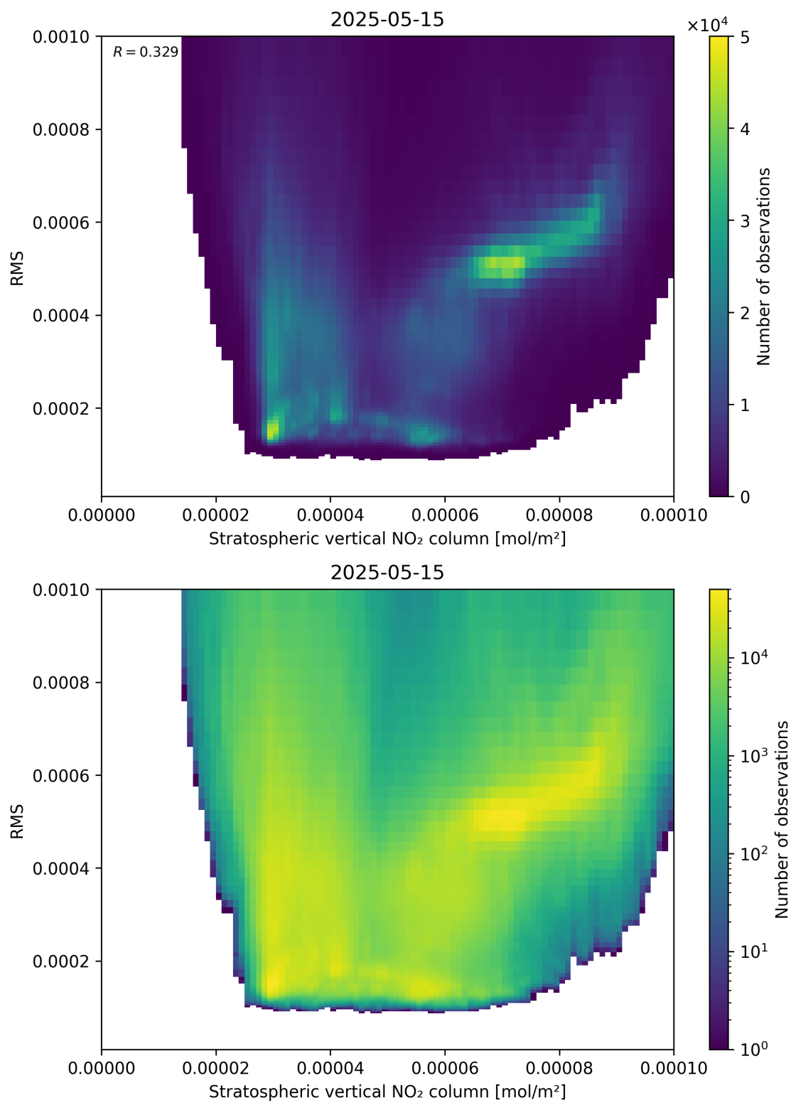
Figure 102: Scatter density plot of “Stratospheric vertical NO 2 column” against “RMS” for 2025-05-15 to 2025-05-16.
