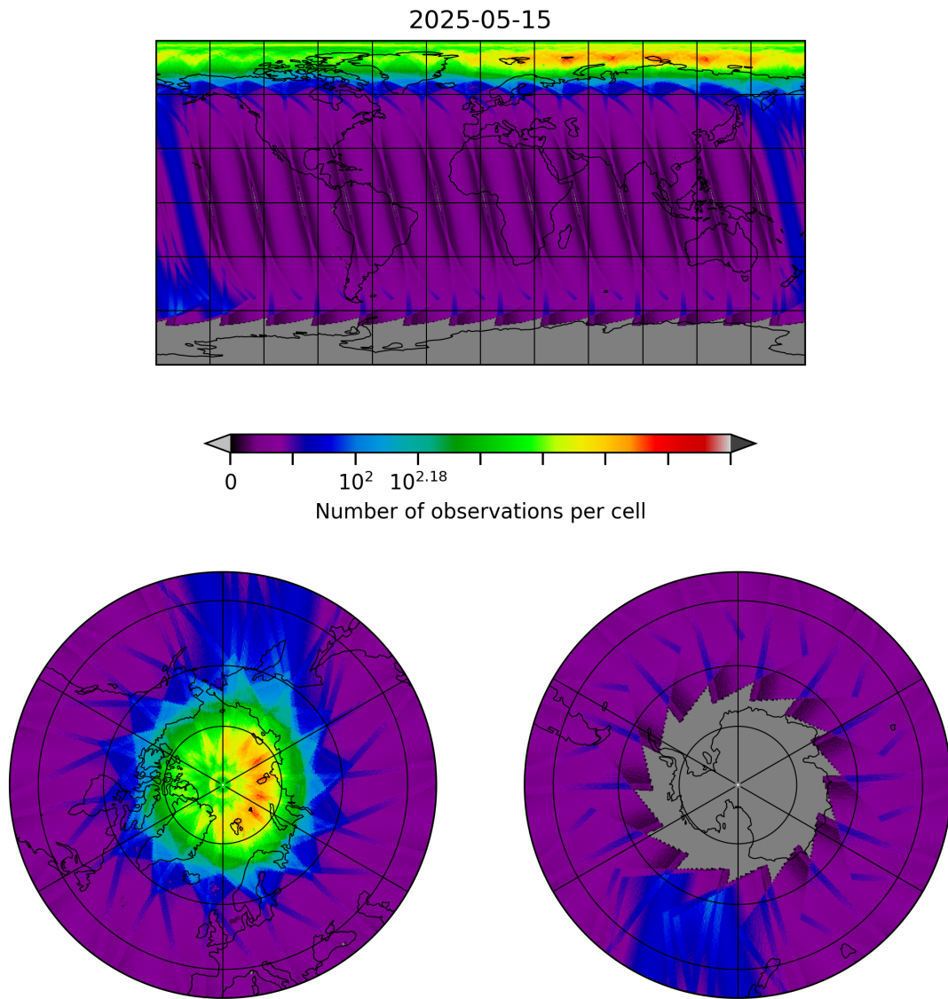
Figure 10: Map of the number of observations for 2025-05-15 to 2025-05-16
