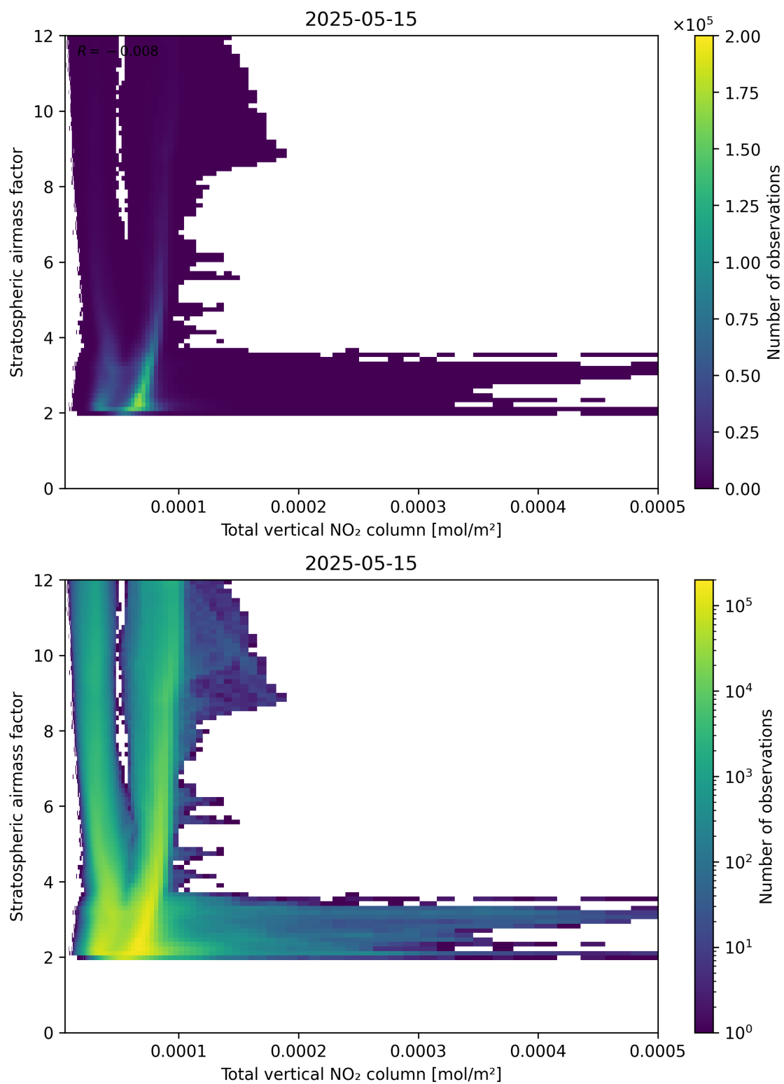
Figure 110: Scatter density plot of “Total vertical NO 2 column” against “Stratospheric airmass factor” for 2025-05-15 to 2025-05-16.
