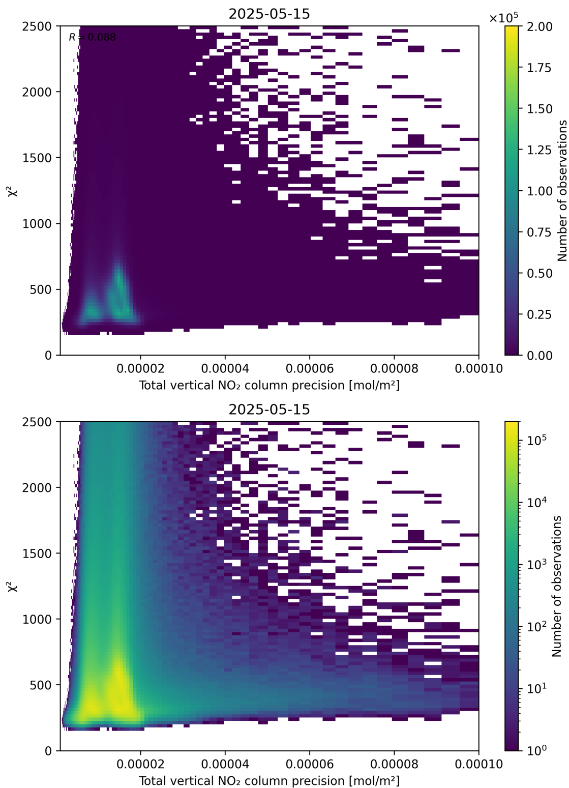
Figure 116: Scatter density plot of “Total vertical NO 2 column precision” against “ \chi^2 ” for 2025-05-15 to 2025-05-16.
