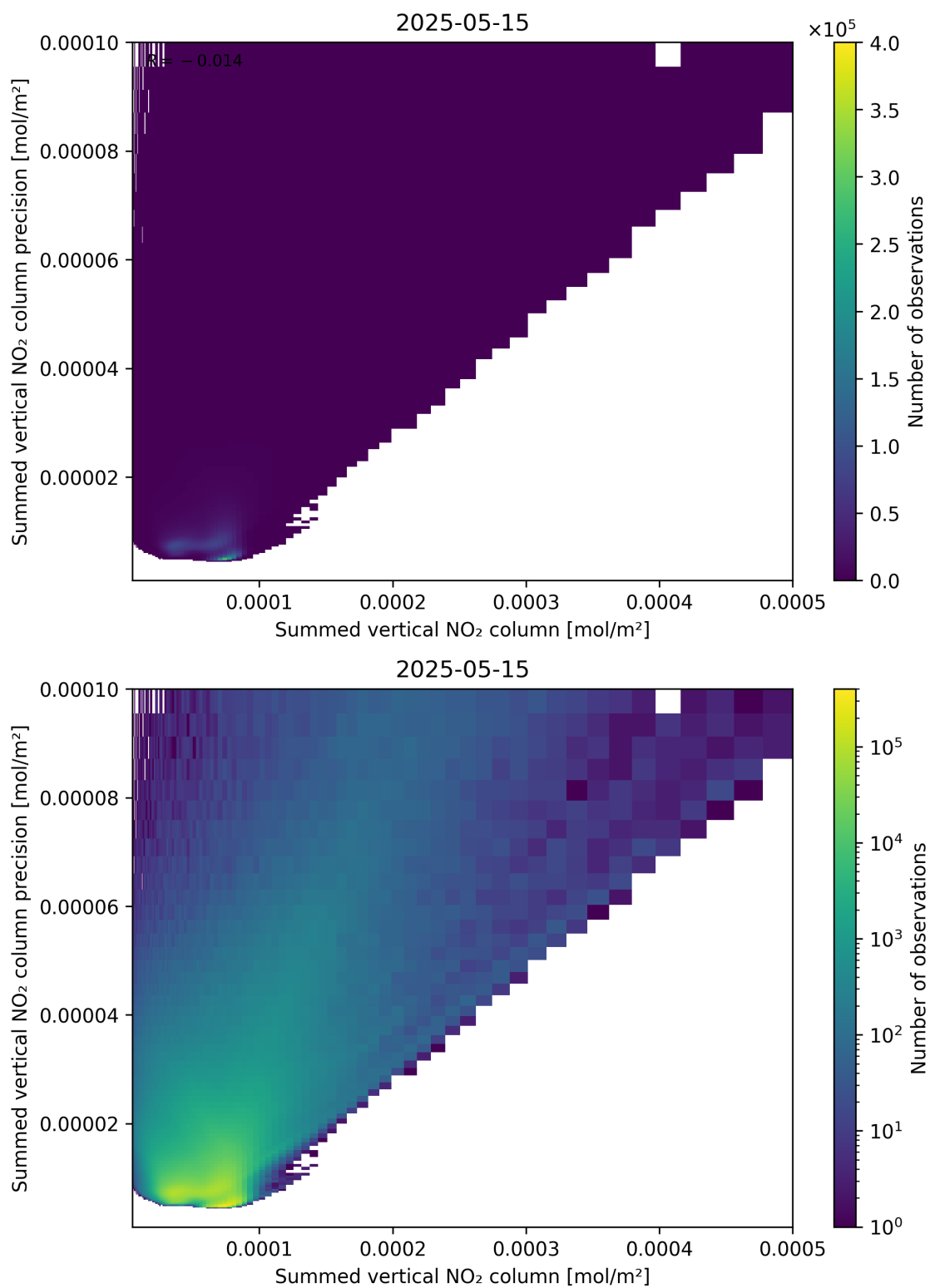
Figure 105: Scatter density plot of “Summed vertical NO 2 column” against “Summed vertical NO 2 column precision” for 2025-05-15 to 2025-05-16.
