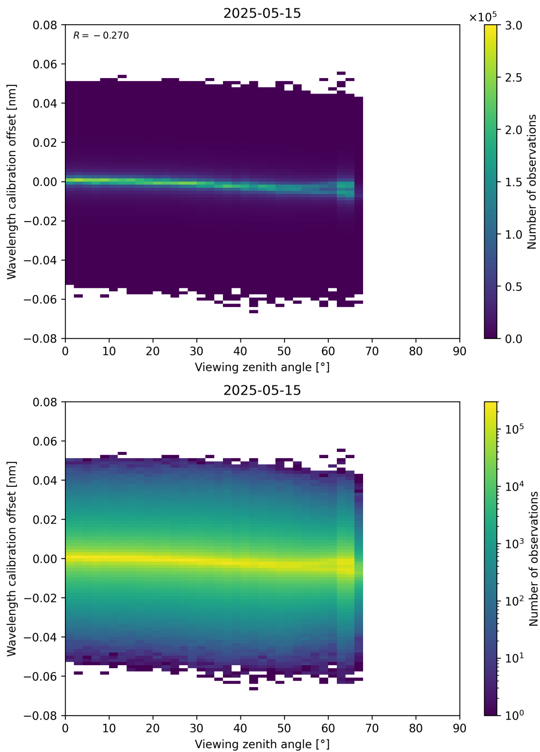
Figure 173: Scatter density plot of “Viewing zenith angle” against “Wavelength calibration offset” for 2025-05-15 to 2025-05-16.
