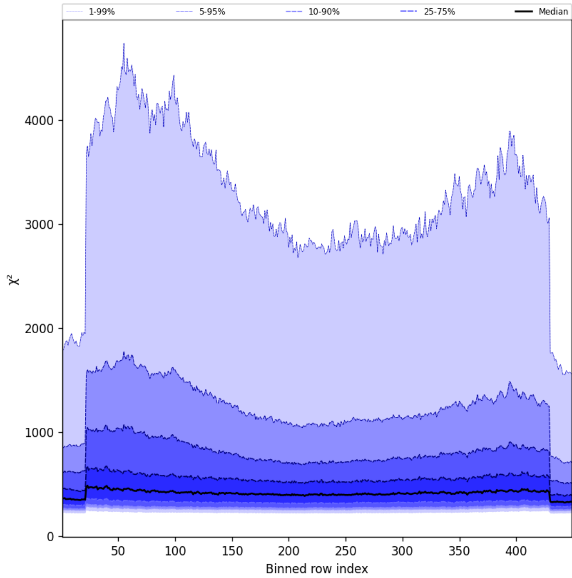
Figure 59: Along track statistics of “ \chi^2 ” for 2025-05-15 to 2025-05-16
