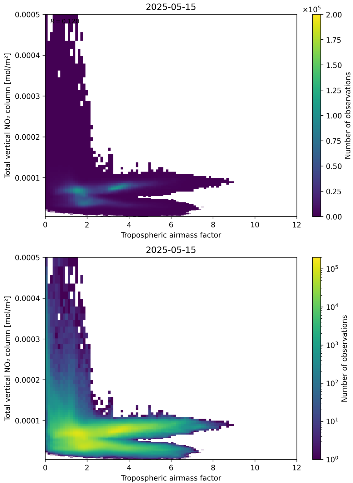
Figure 77: Scatter density plot of “Tropospheric airmass factor” against “Total vertical NO 2 column” for 2025-05-15 to 2025-05-16.
