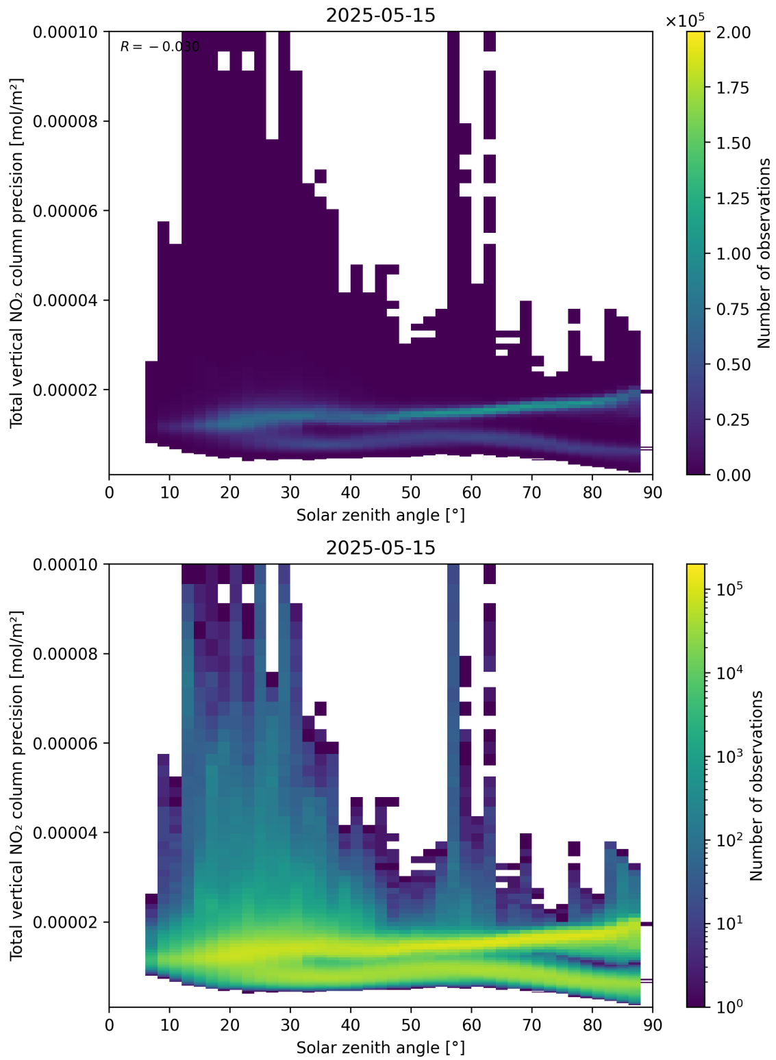
Figure 154: Scatter density plot of “Solar zenith angle” against “Total vertical NO 2 column precision” for 2025-05-15 to 2025-05-16.
