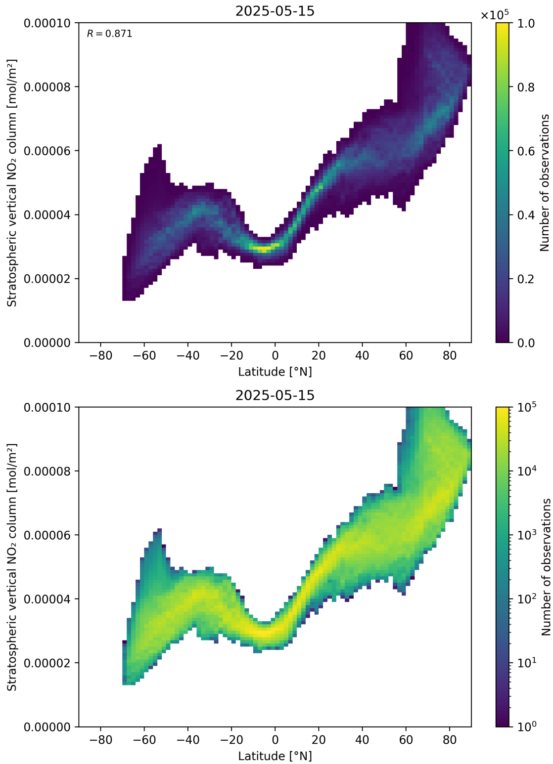
Figure 87: Scatter density plot of “Latitude” against “Stratospheric vertical \text{NO}_2 column” for 2025-05-15 to 2025-05-16.
