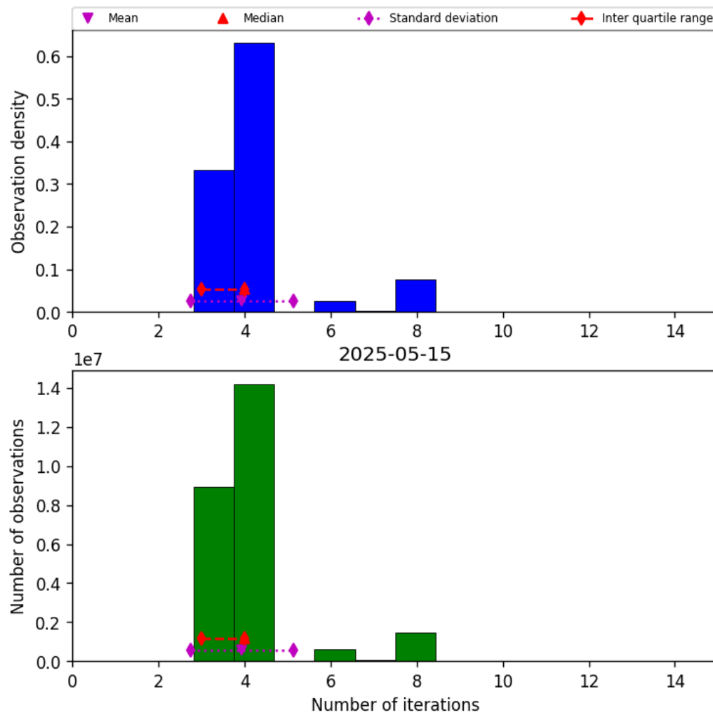
Figure 34: Histogram of “Number of iterations” for 2025-05-15 to 2025-05-16
