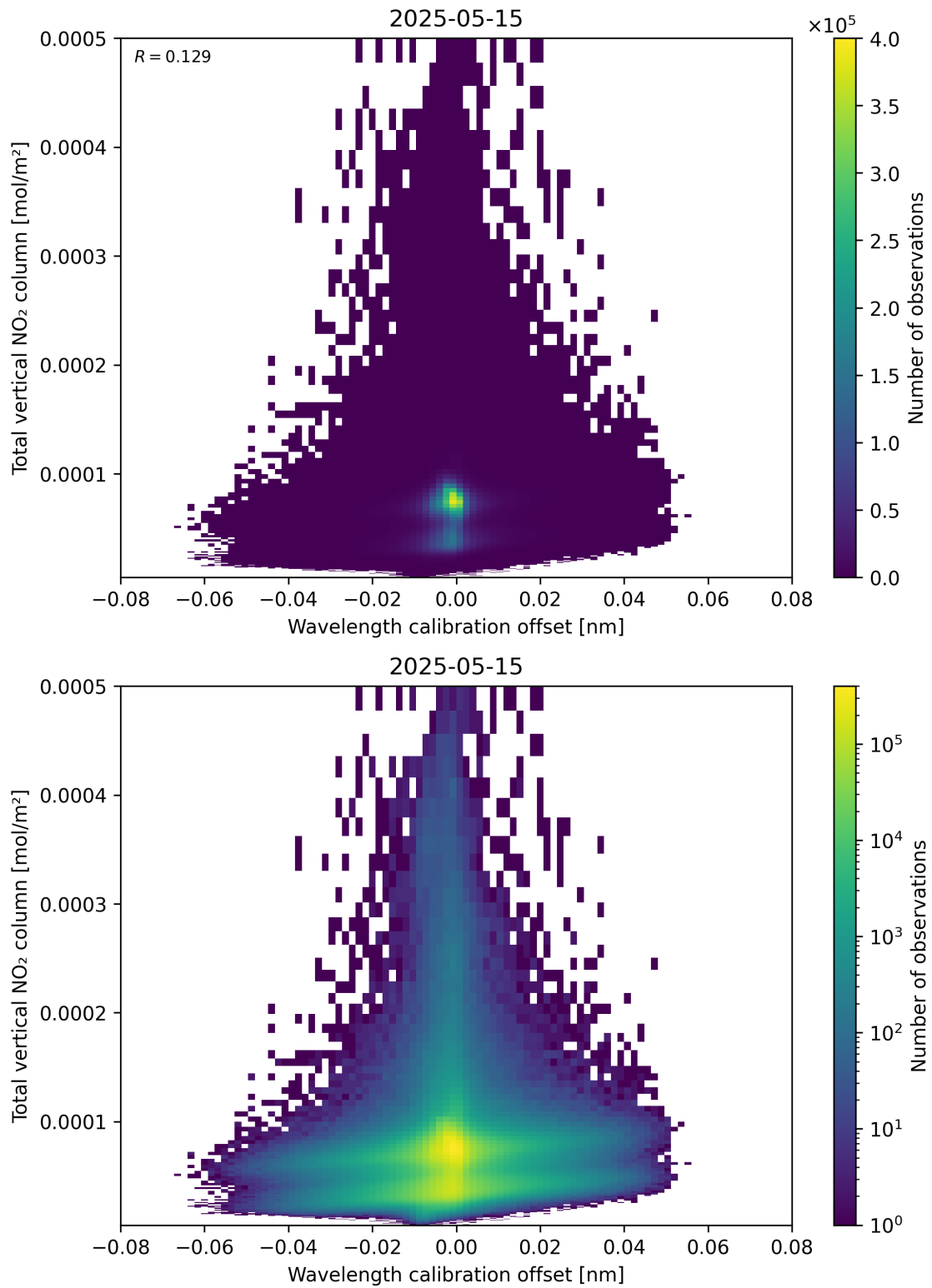
Figure 179: Scatter density plot of “Wavelength calibration offset” against “Total vertical NO 2 column” for 2025-05-15 to 2025-05-16.
