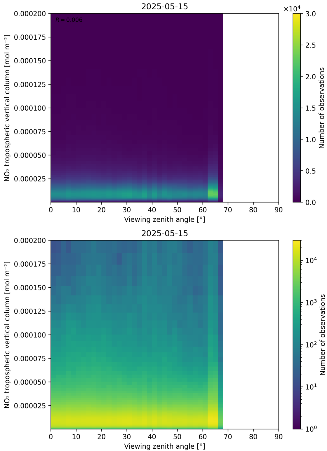
Figure 169: Scatter density plot of “Viewing zenith angle” against “NO 2 tropospheric vertical column” for 2025-05-15 to 2025-05-16.
