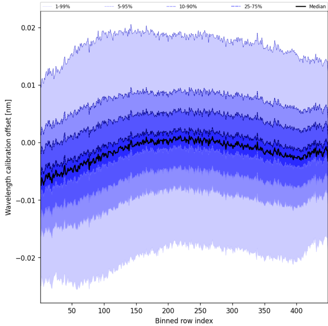
Figure 52: Along track statistics of “Wavelength calibration offset” for 2025-05-15 to 2025-05-16
