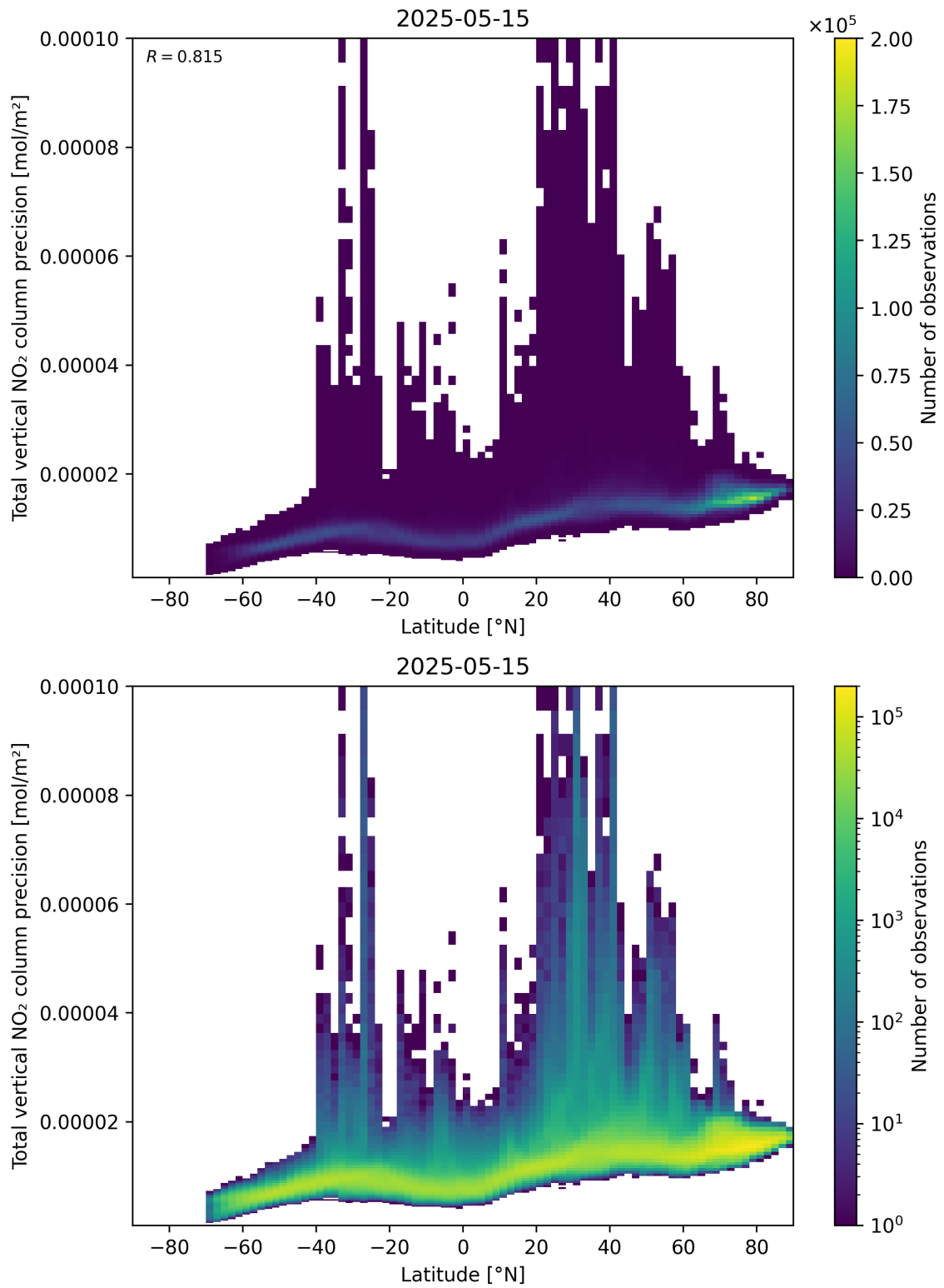
Figure 91: Scatter density plot of “Latitude” against “Total vertical NO 2 column precision” for 2025-05-15 to 2025-05-16.
