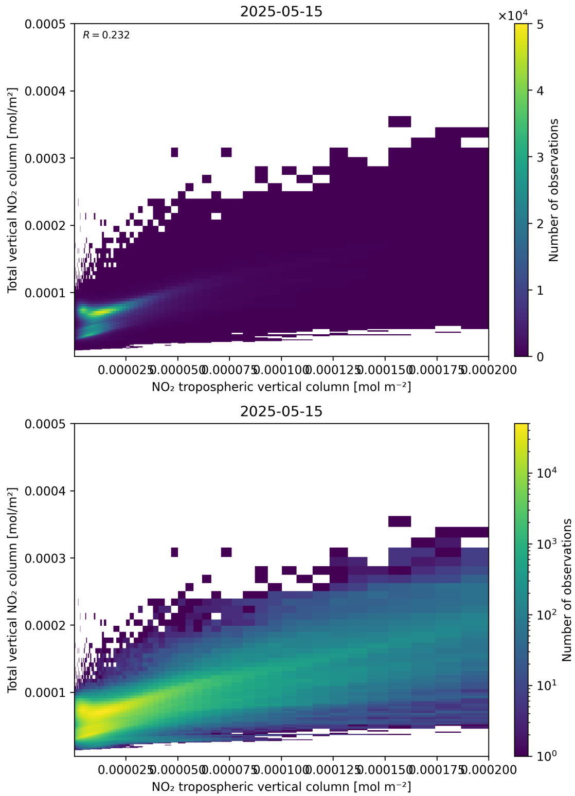
Figure 128: Scatter density plot of “NO 2 tropospheric vertical column” against “Total vertical NO 2 column” for 2025-05-15 to 2025-05-16.
