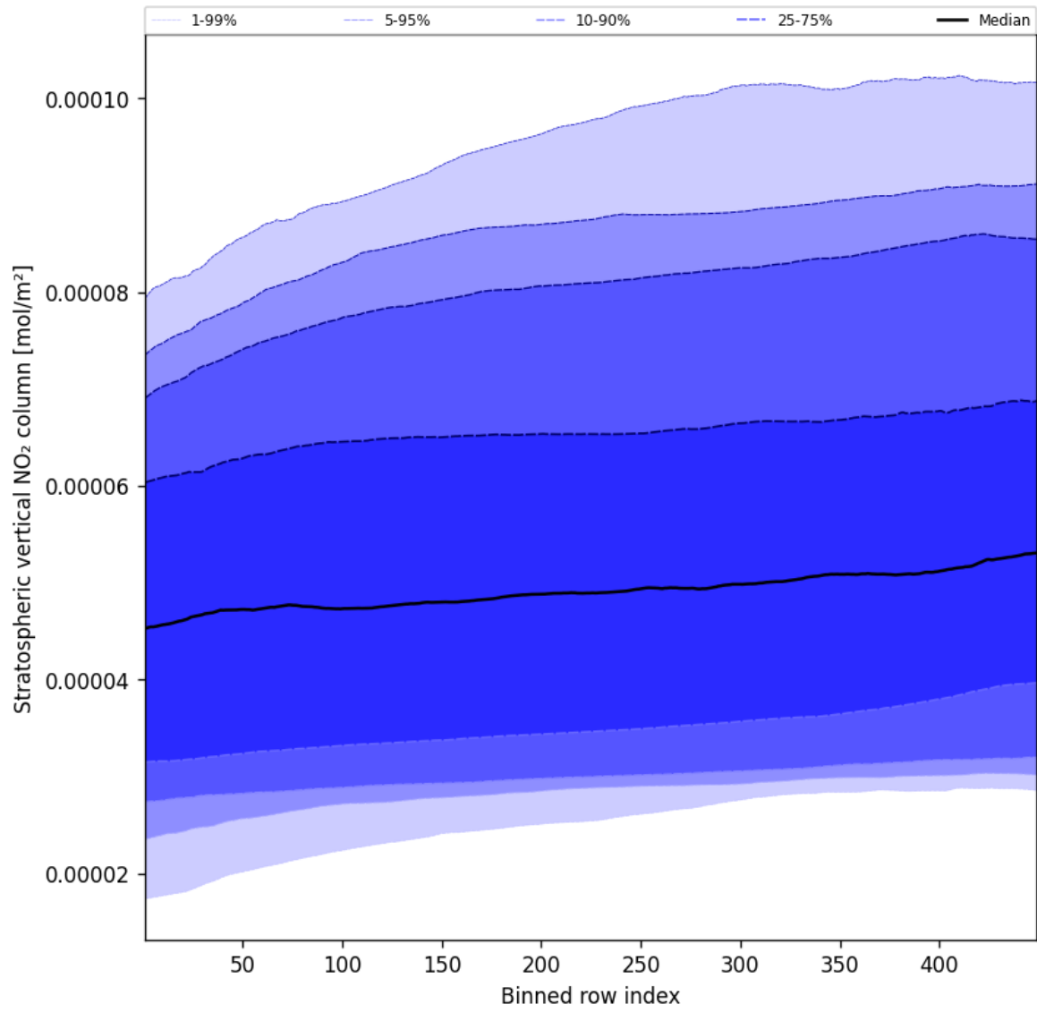
Figure 53: Along track statistics of “Stratospheric vertical NO 2 column” for 2025-05-15 to 2025-05-16
