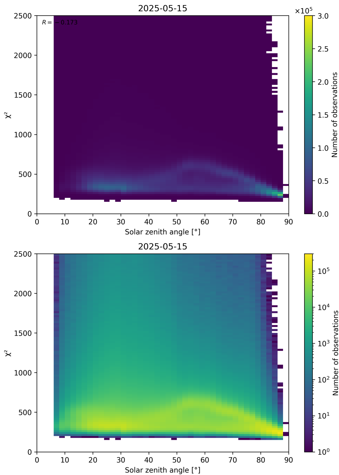
Figure 148: Scatter density plot of “Solar zenith angle” against “ \chi^2 ” for 2025-05-15 to 2025-05-16.
