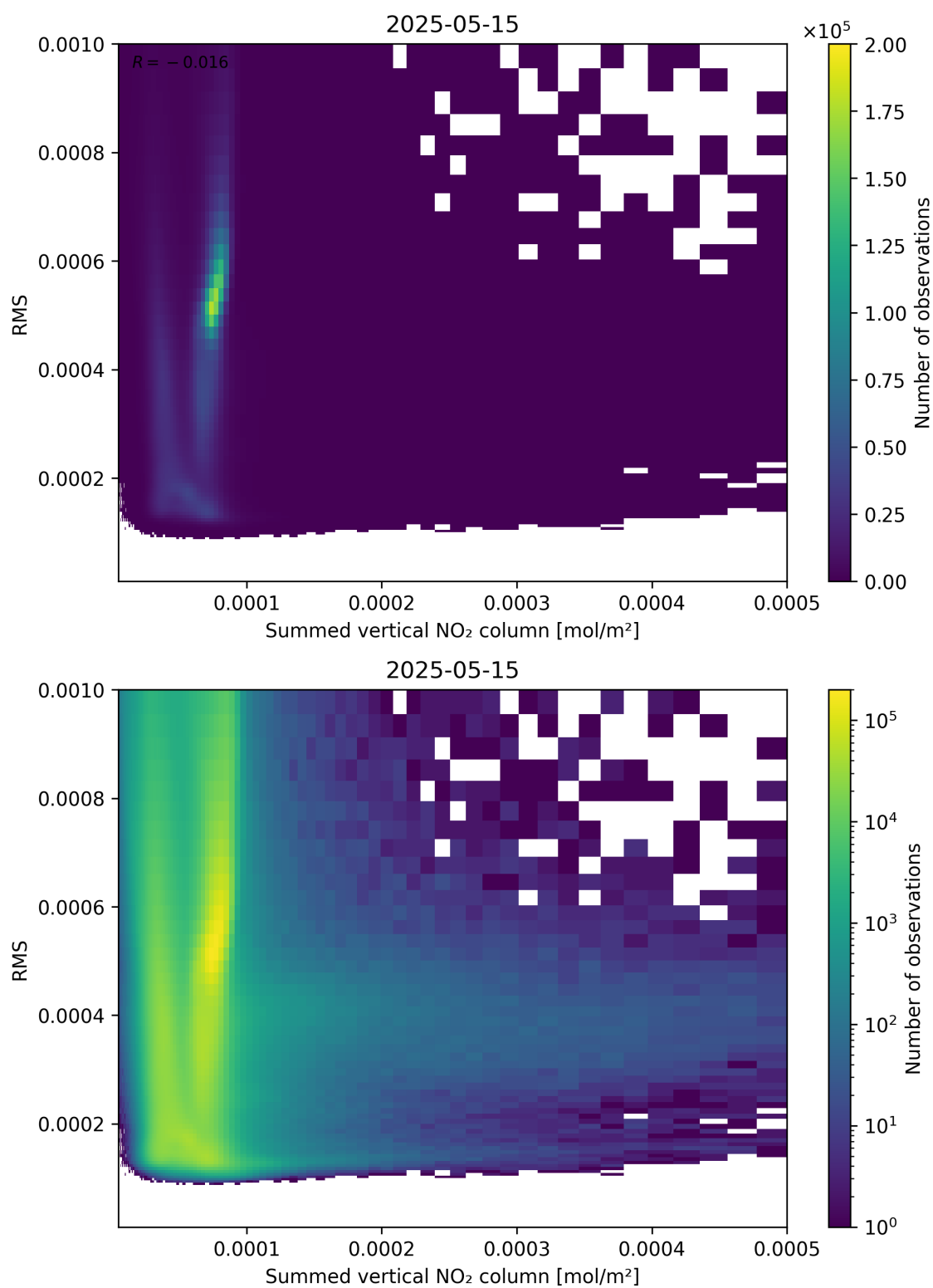
Figure 109: Scatter density plot of “Summed vertical NO 2 column” against “RMS” for 2025-05-15 to 2025-05-16.
