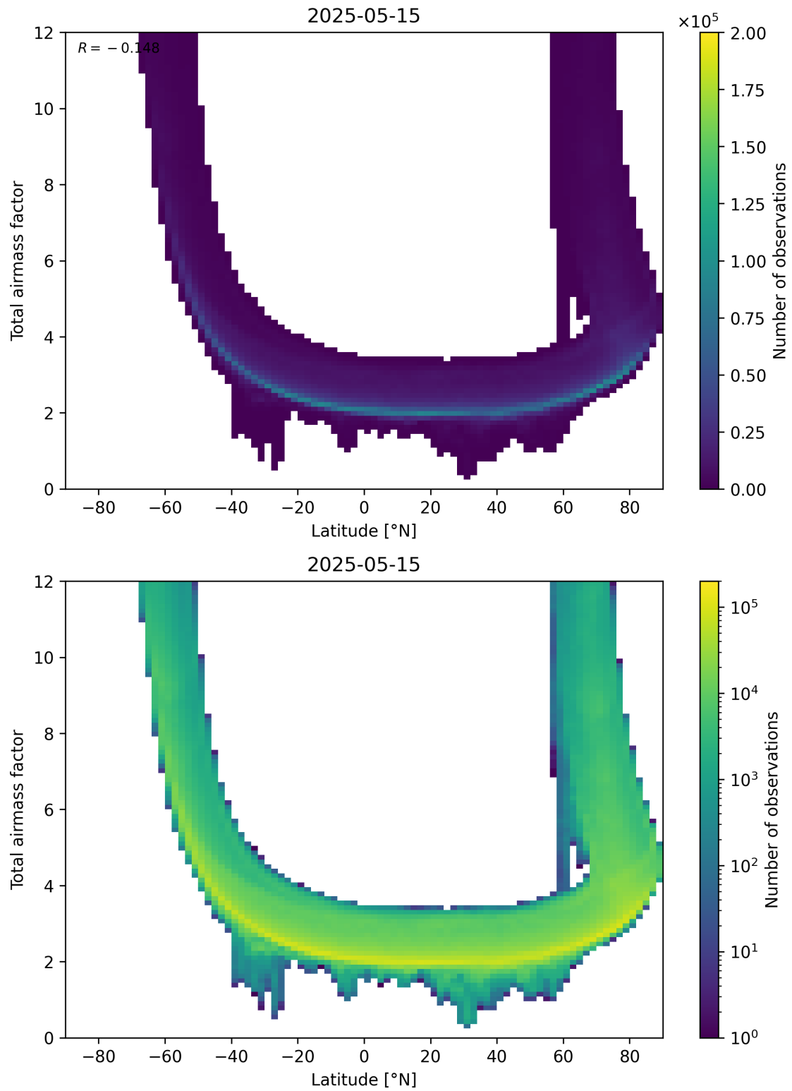
Figure 84: Scatter density plot of “Latitude” against “Total airmass factor” for 2025-05-15 to 2025-05-16.
