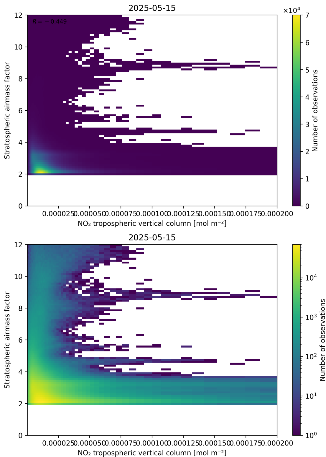
Figure 121: Scatter density plot of “NO 2 tropospheric vertical column” against “Stratospheric air mass factor” for 2025-05-15 to 2025-05-16.
