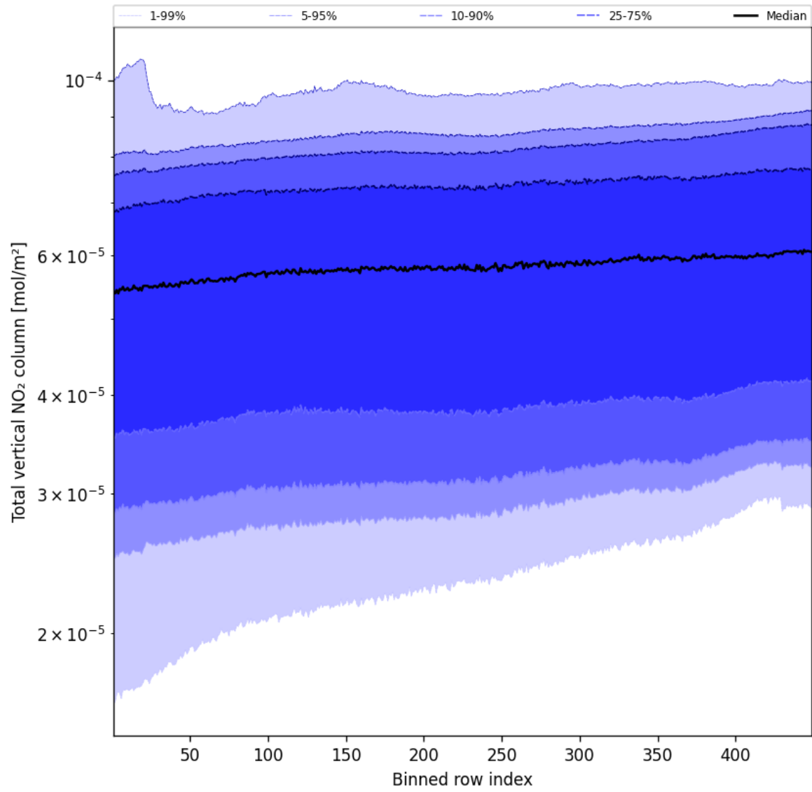
Figure 55: Along track statistics of “Total vertical NO 2 column” for 2025-05-15 to 2025-05-16
