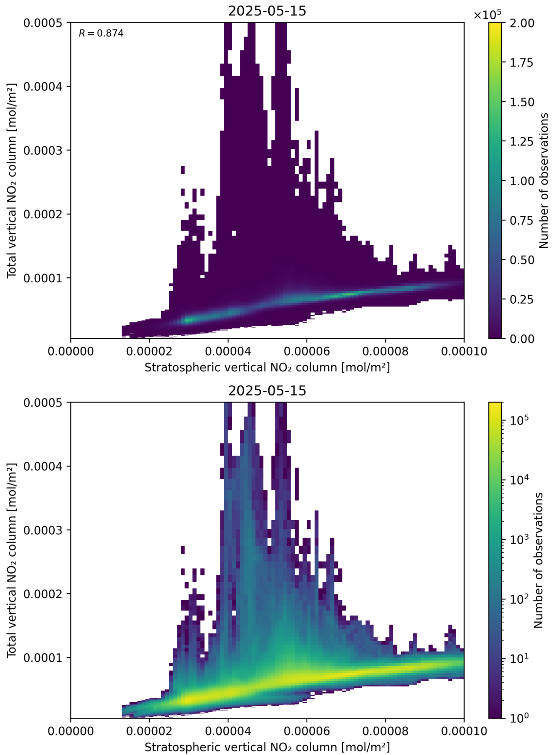
Figure 100: Scatter density plot of “Stratospheric vertical NO 2 column” against “Total vertical NO 2 column” for 2025-05-15 to 2025-05-16.
