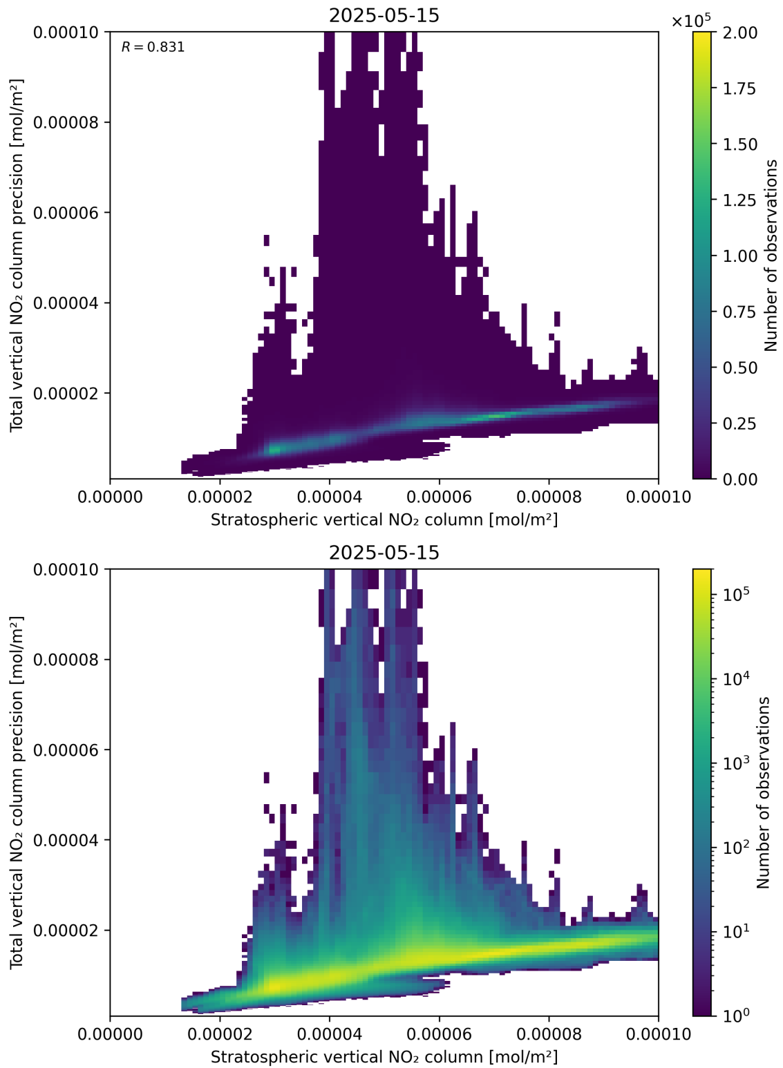
Figure 101: Scatter density plot of “Stratospheric vertical NO 2 column” against “Total vertical NO 2 column precision” for 2025-05-15 to 2025-05-16.
