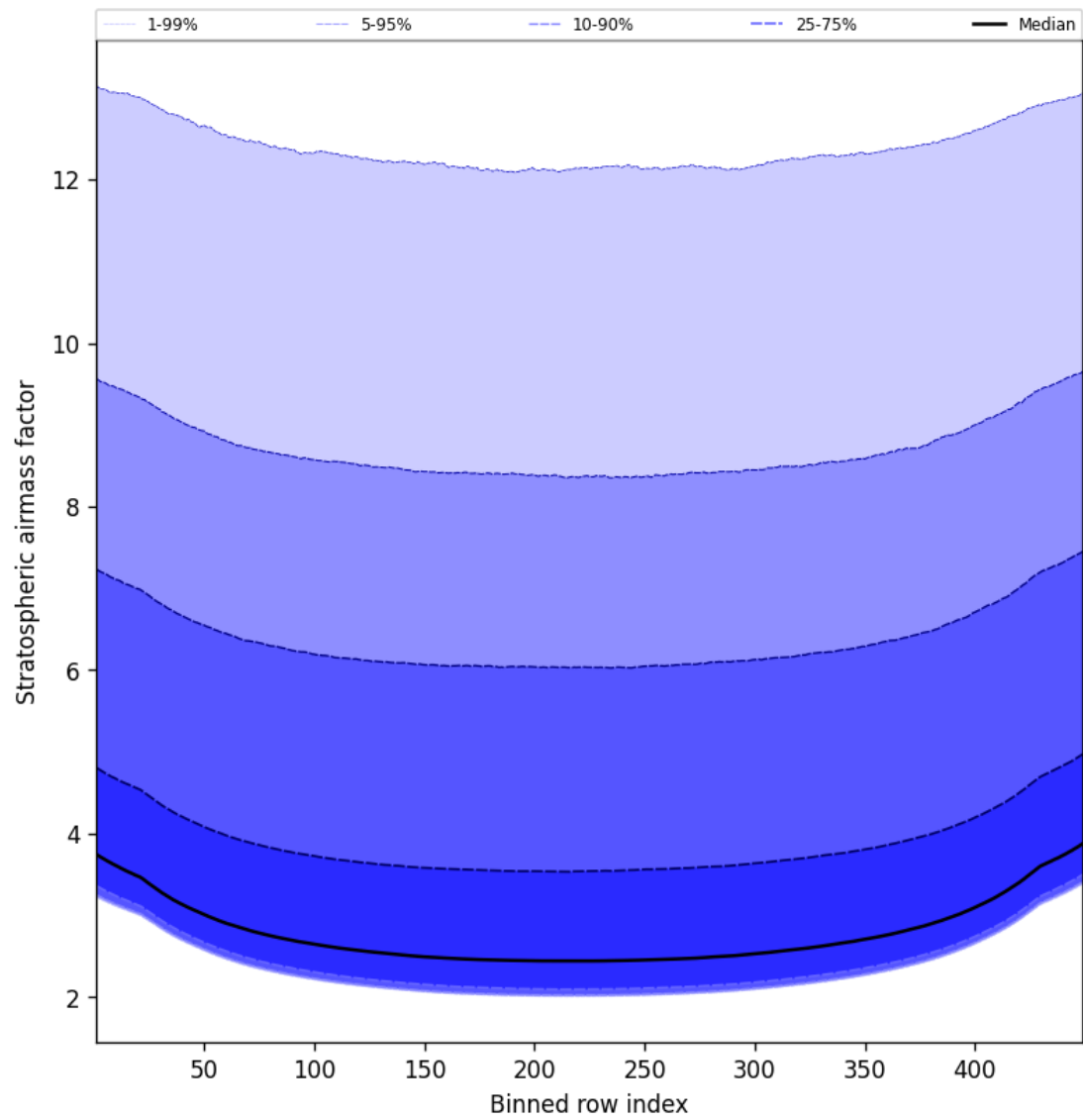
Figure 61: Along track statistics of “Stratospheric air mass factor” for 2025-05-15 to 2025-05-16
