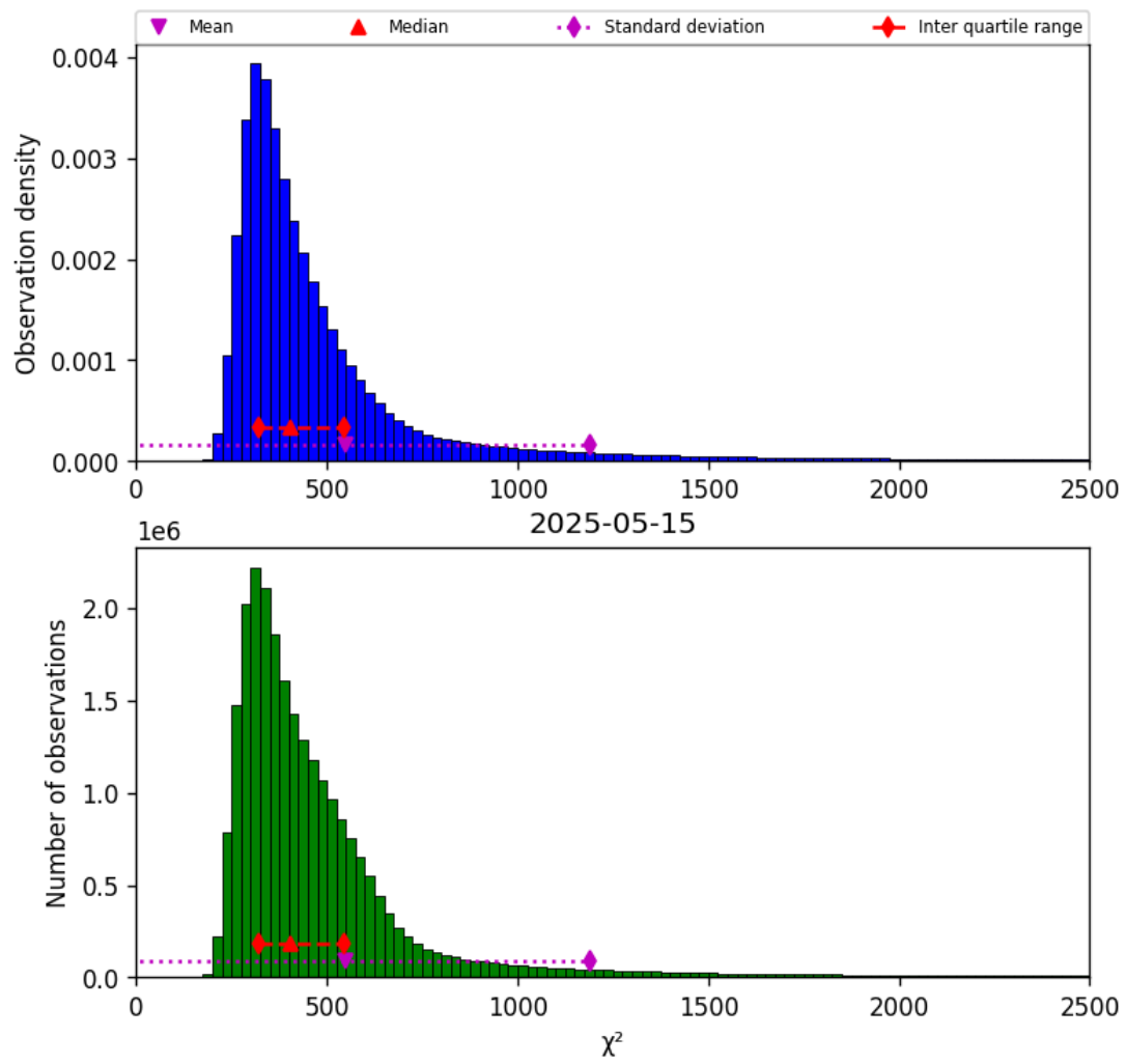
Figure 42: Histogram of “ \chi^2 ” for 2025-05-15 to 2025-05-16
