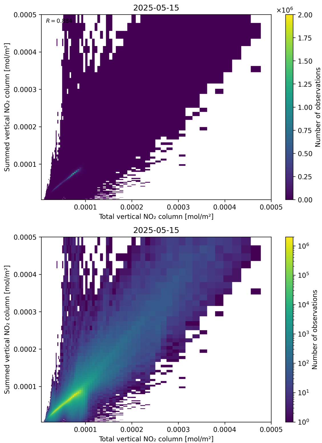
Figure 112: Scatter density plot of “Total vertical NO 2 column” against “Summed vertical NO 2 column” for 2025-05-15 to 2025-05-16.
