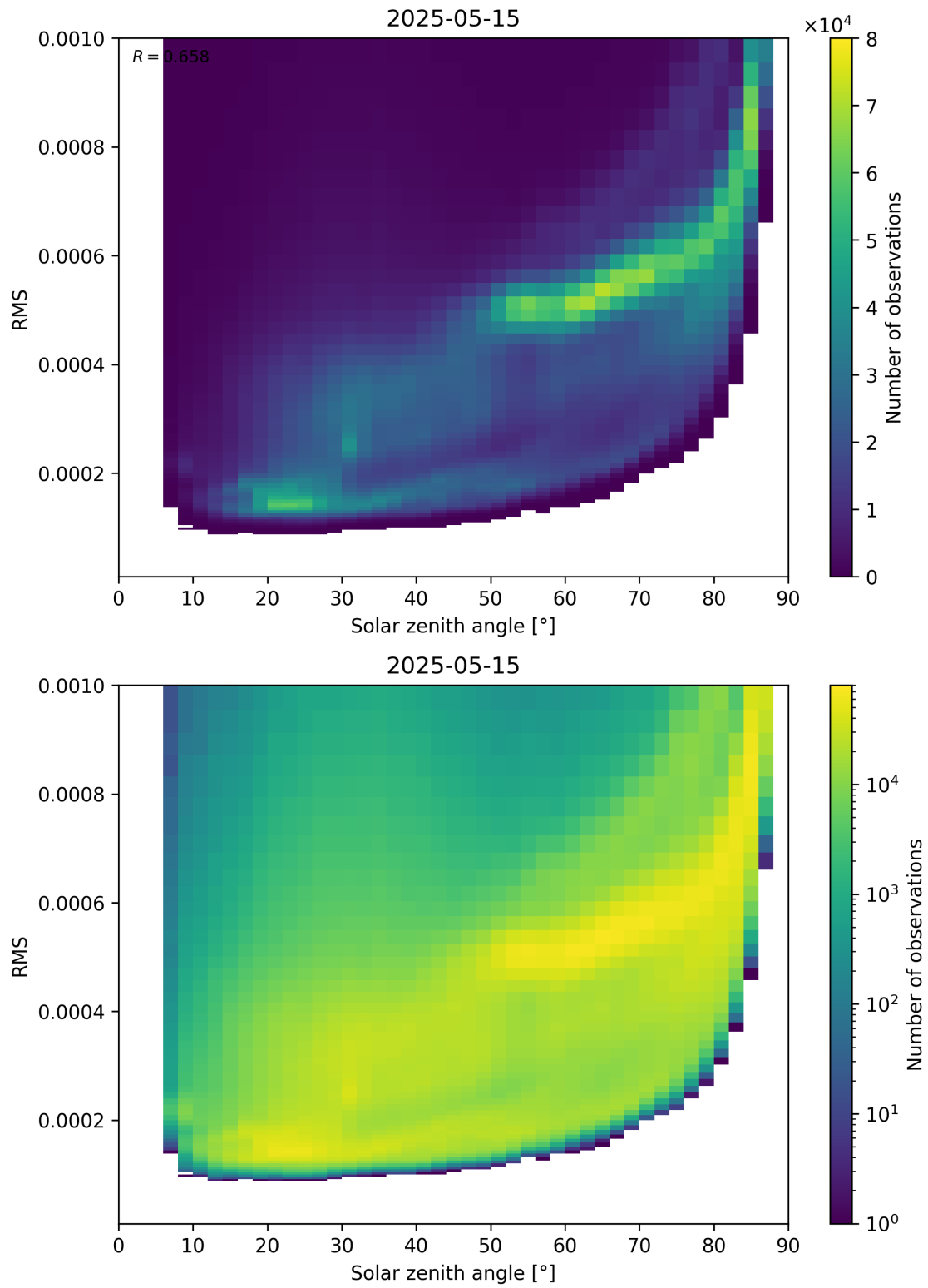
Figure 157: Scatter density plot of “Solar zenith angle” against “RMS” for 2025-05-15 to 2025-05-16.
