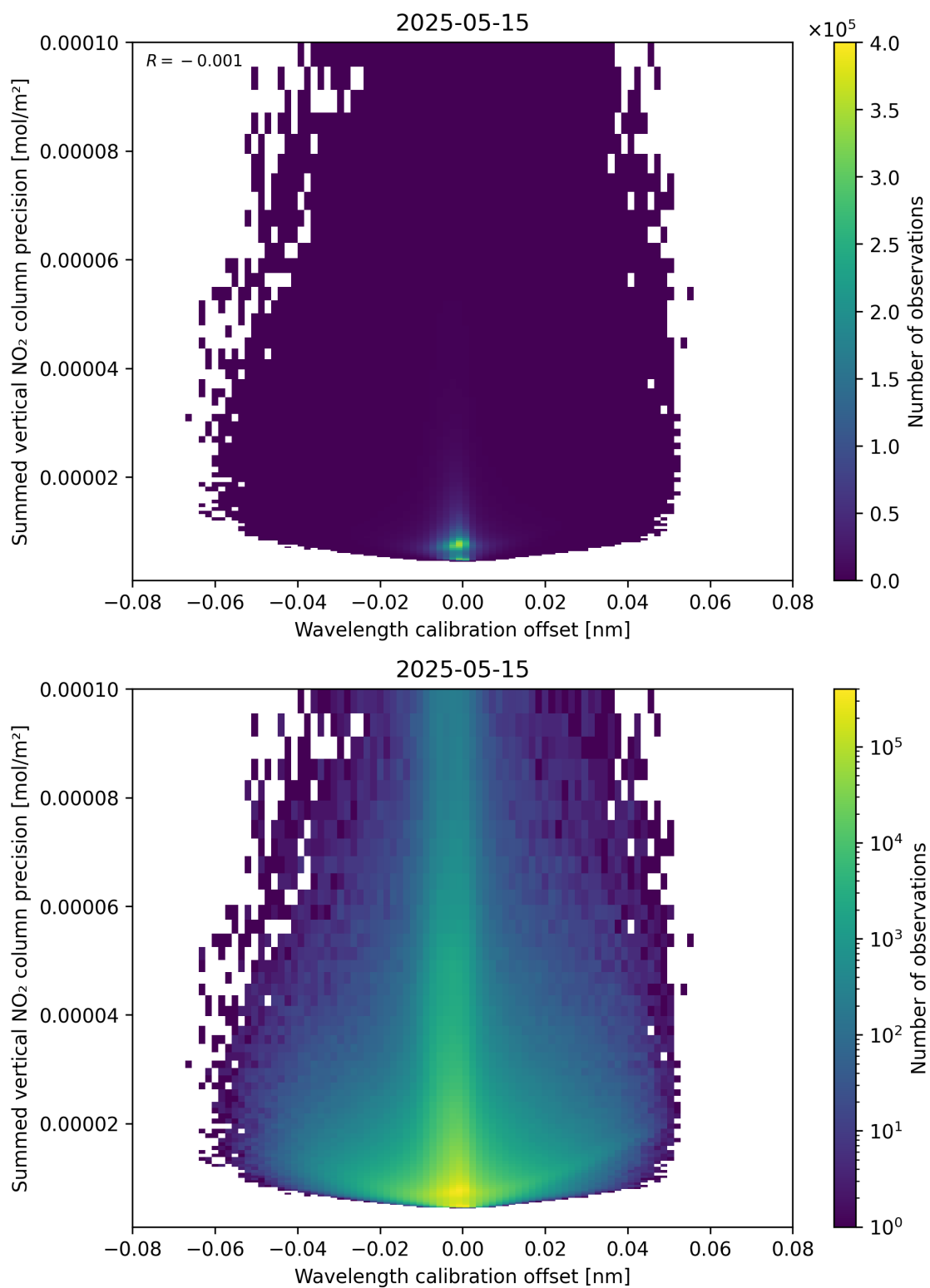
Figure 178: Scatter density plot of “Wavelength calibration offset” against “Summed vertical NO 2 column precision” for 2025-05-15 to 2025-05-16.
