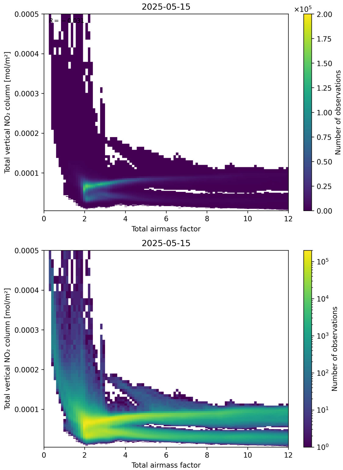
Figure 67: Scatter density plot of “Total airmass factor” against “Total vertical NO 2 column” for 2025-05-15 to 2025-05-16.
