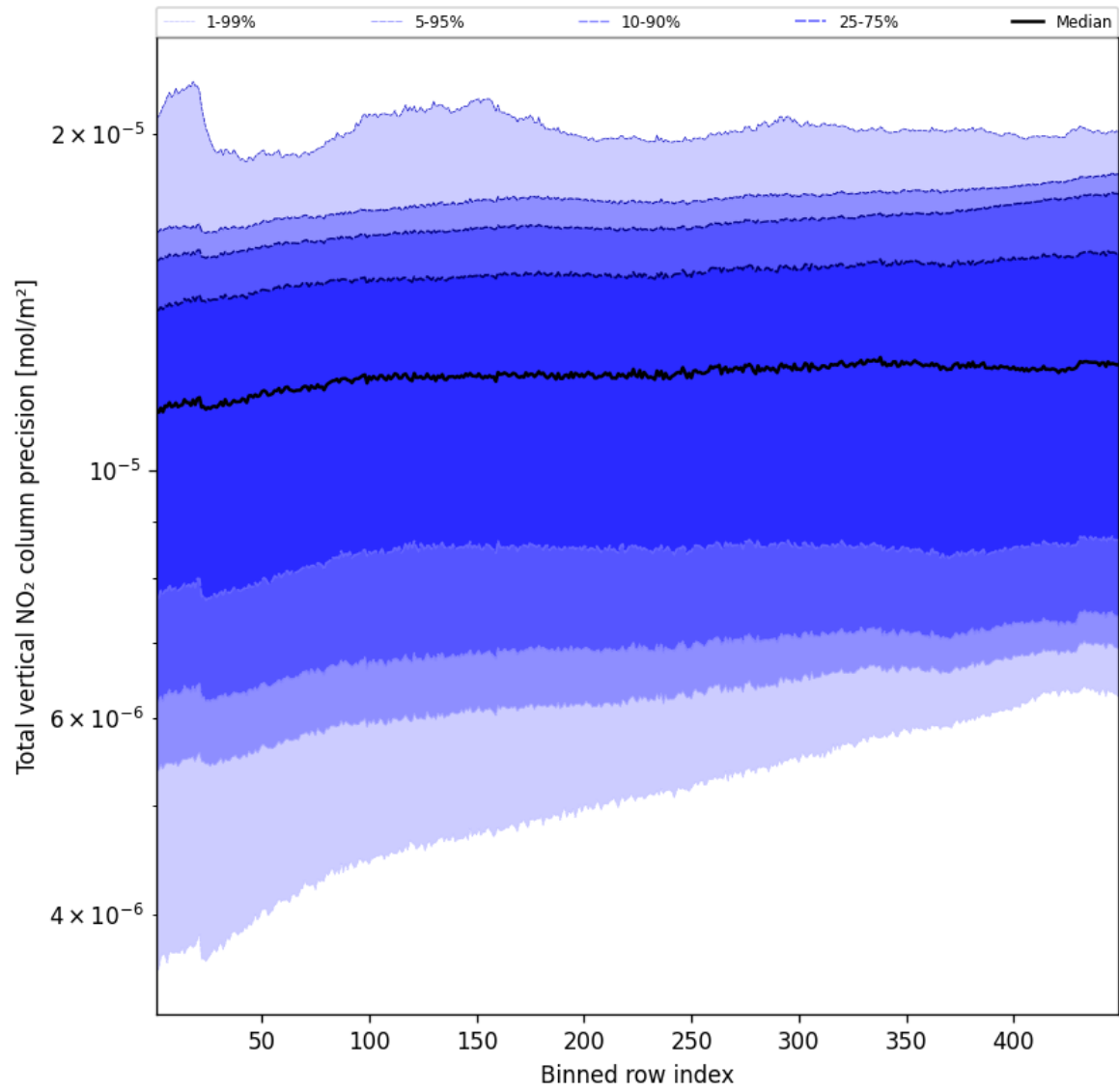
Figure 56: Along track statistics of “Total vertical NO 2 column precision” for 2025-05-15 to 2025-05-16
