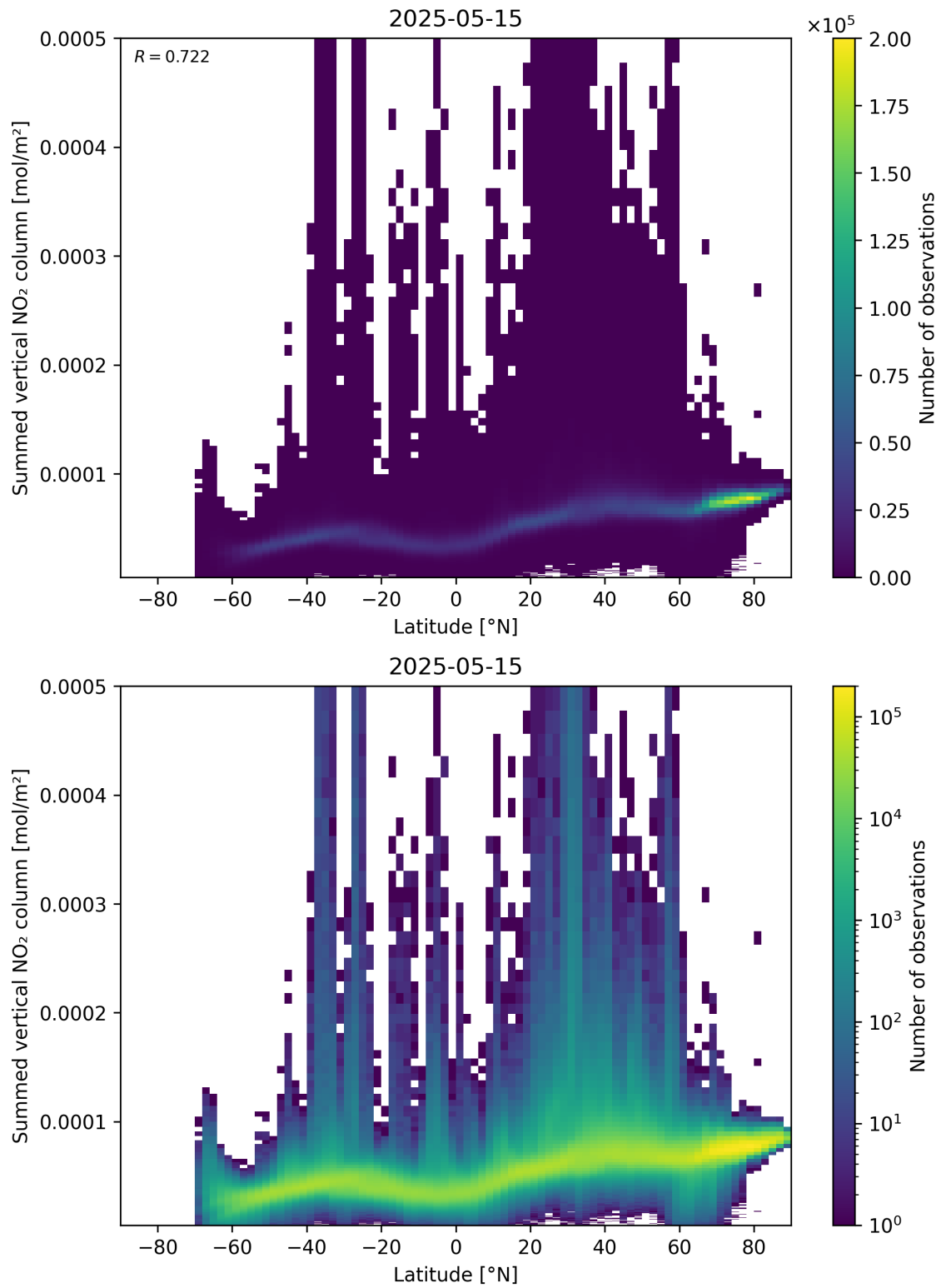
Figure 88: Scatter density plot of “Latitude” against “Summed vertical NO 2 column” for 2025-05-15 to 2025-05-16.
