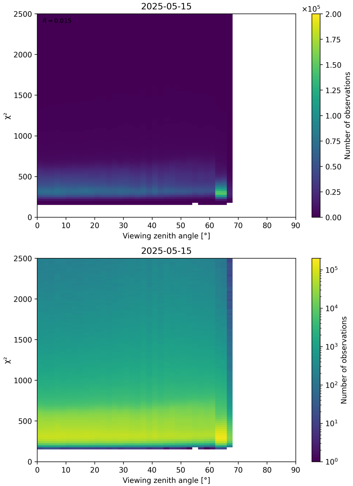
Figure 162: Scatter density plot of “Viewing zenith angle” against “ \chi^2 ” for 2025-05-15 to 2025-05-16.
