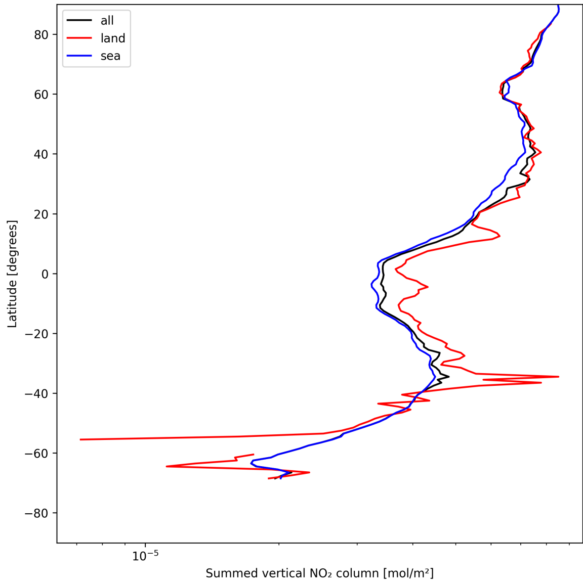
Figure 23: Zonal average of “Summed vertical NO 2 column” for 2025-05-15 to 2025-05-16.
