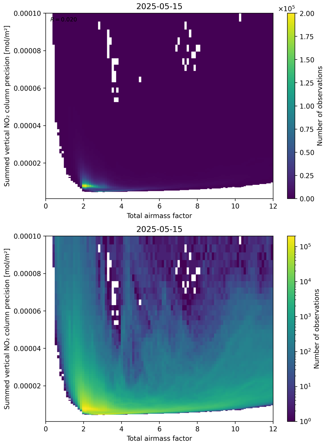
Figure 66: Scatter density plot of “Total airmass factor” against “Summed vertical NO 2 column precision” for 2025-05-15 to 2025-05-16.
