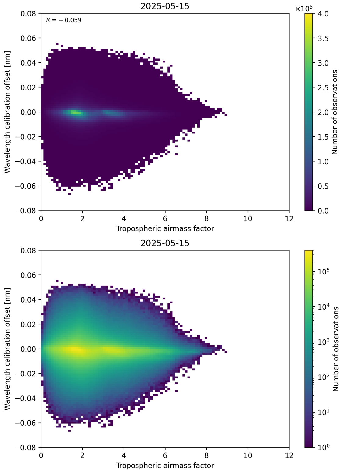
Figure 80: Scatter density plot of “Tropospheric airmass factor” against “Wavelength calibration offset” for 2025-05-15 to 2025-05-16.
