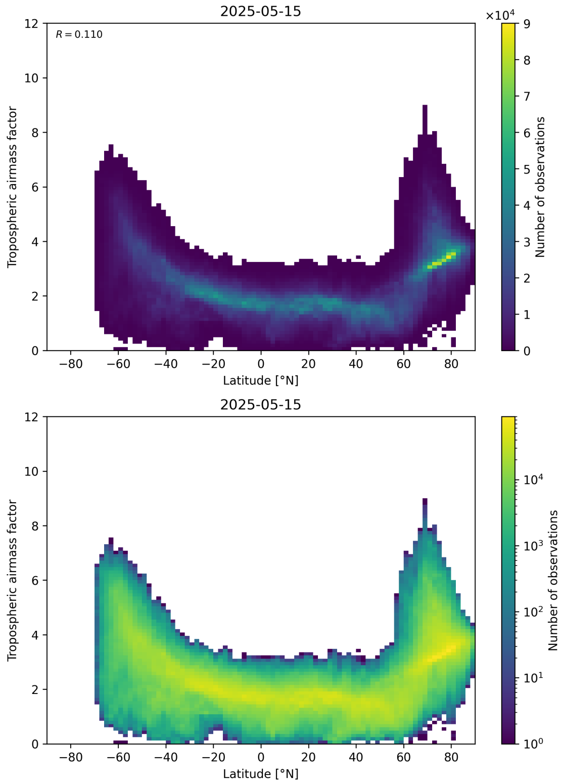
Figure 85: Scatter density plot of “Latitude” against “Tropospheric airmass factor” for 2025-05-15 to 2025-05-16.
