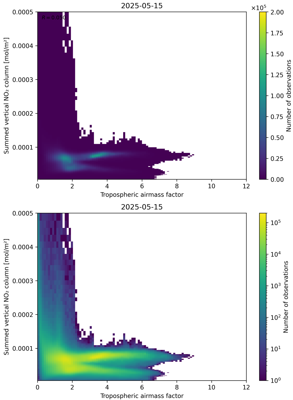
Figure 75: Scatter density plot of “Tropospheric airmass factor” against “Summed vertical NO 2 column” for 2025-05-15 to 2025-05-16.
