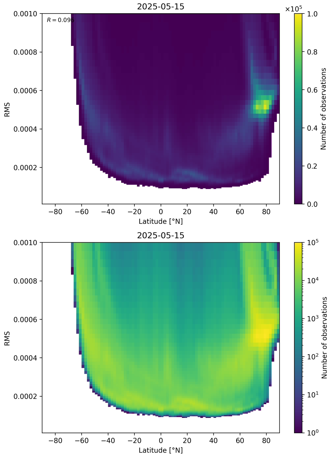
Figure 94: Scatter density plot of “Latitude” against “RMS” for 2025-05-15 to 2025-05-16.
