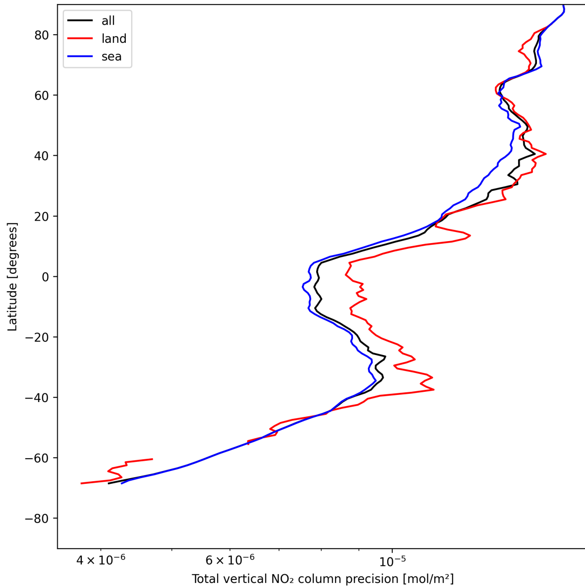
Figure 22: Zonal average of “Total vertical NO 2 column precision” for 2025-05-15 to 2025-05-16.
