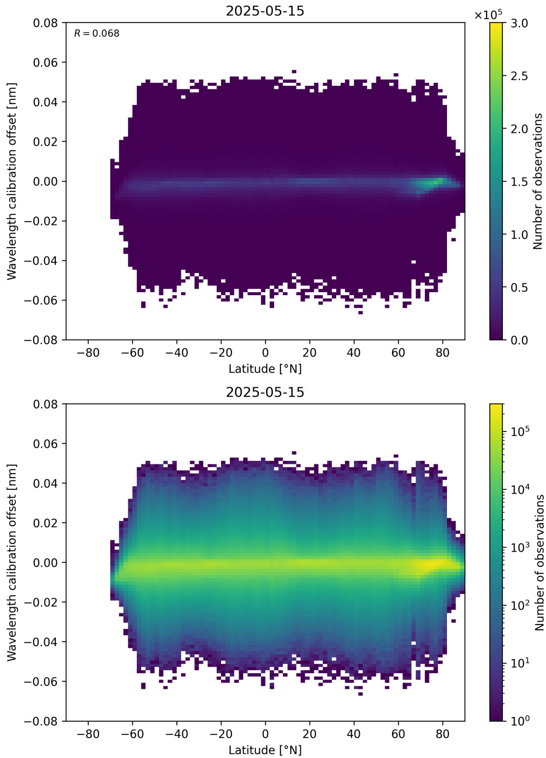
Figure 95: Scatter density plot of “Latitude” against “Wavelength calibration offset” for 2025-05-15 to 2025-05-16.
