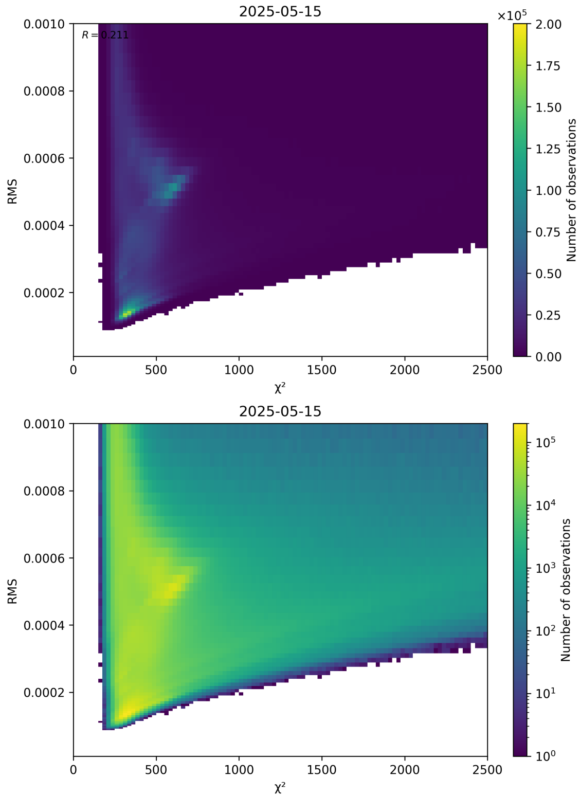
Figure 82: Scatter density plot of “ \chi^2 ” against “RMS” for 2025-05-15 to 2025-05-16.
