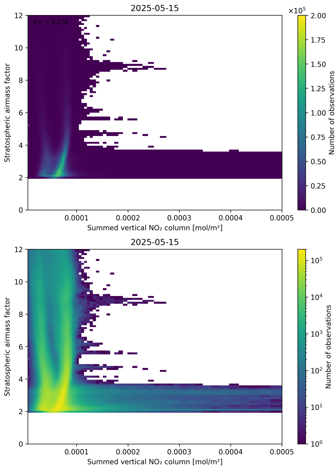
Figure 103: Scatter density plot of “Summed vertical NO 2 column” against “Stratospheric air mass factor” for 2025-05-15 to 2025-05-16.
