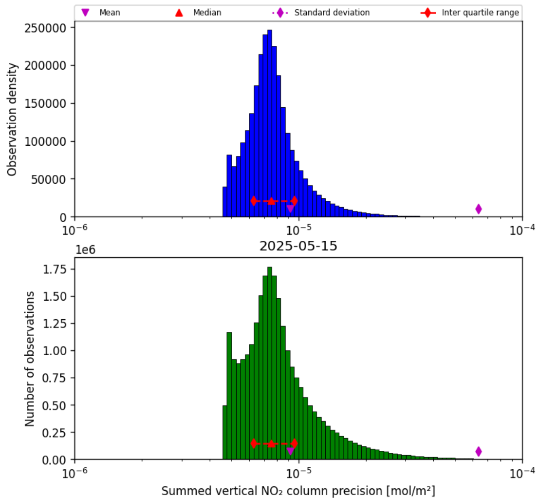
Figure 41: Histogram of “Summed vertical NO 2 column precision” for 2025-05-15 to 2025-05-16
