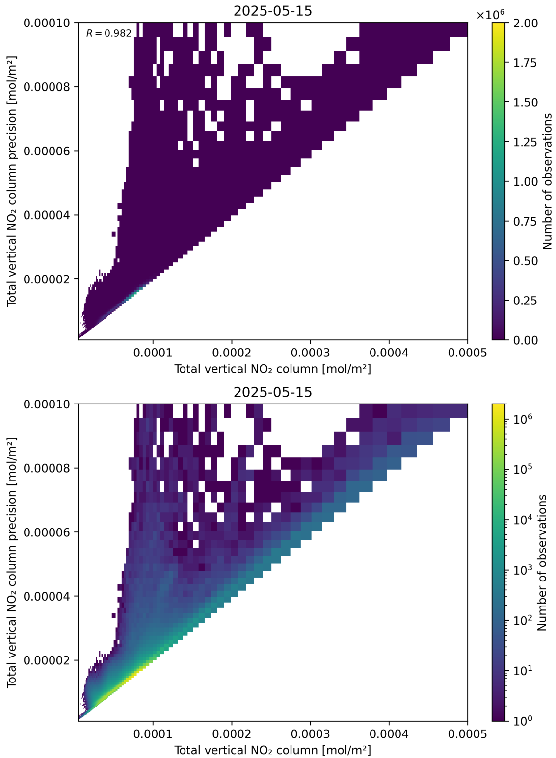
Figure 114: Scatter density plot of “Total vertical NO 2 column” against “Total vertical NO 2 column precision” for 2025-05-15 to 2025-05-16.
