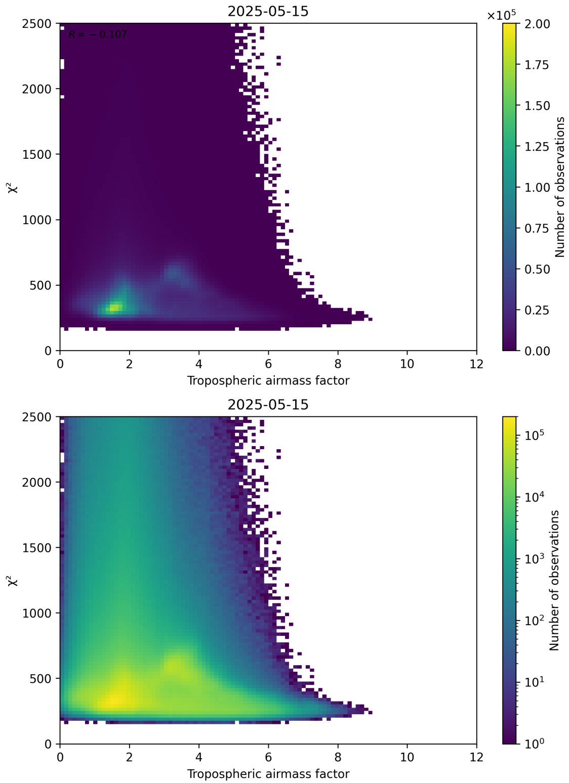
Figure 73: Scatter density plot of “Tropospheric airmass factor” against “ \chi^2 ” for 2025-05-15 to 2025-05-16.
