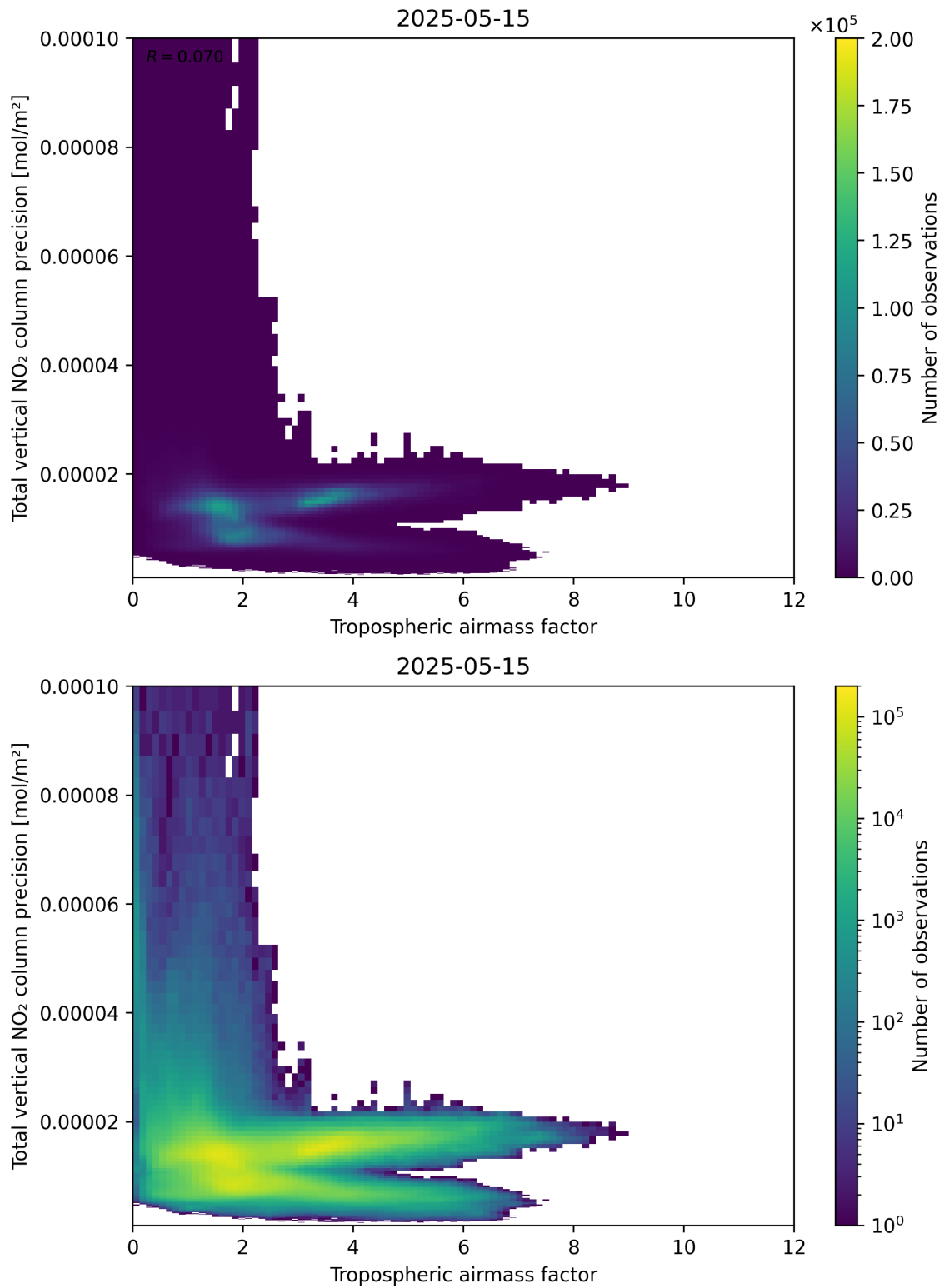
Figure 78: Scatter density plot of “Tropospheric air mass factor” against “Total vertical NO 2 column precision” for 2025-05-15 to 2025-05-16.
