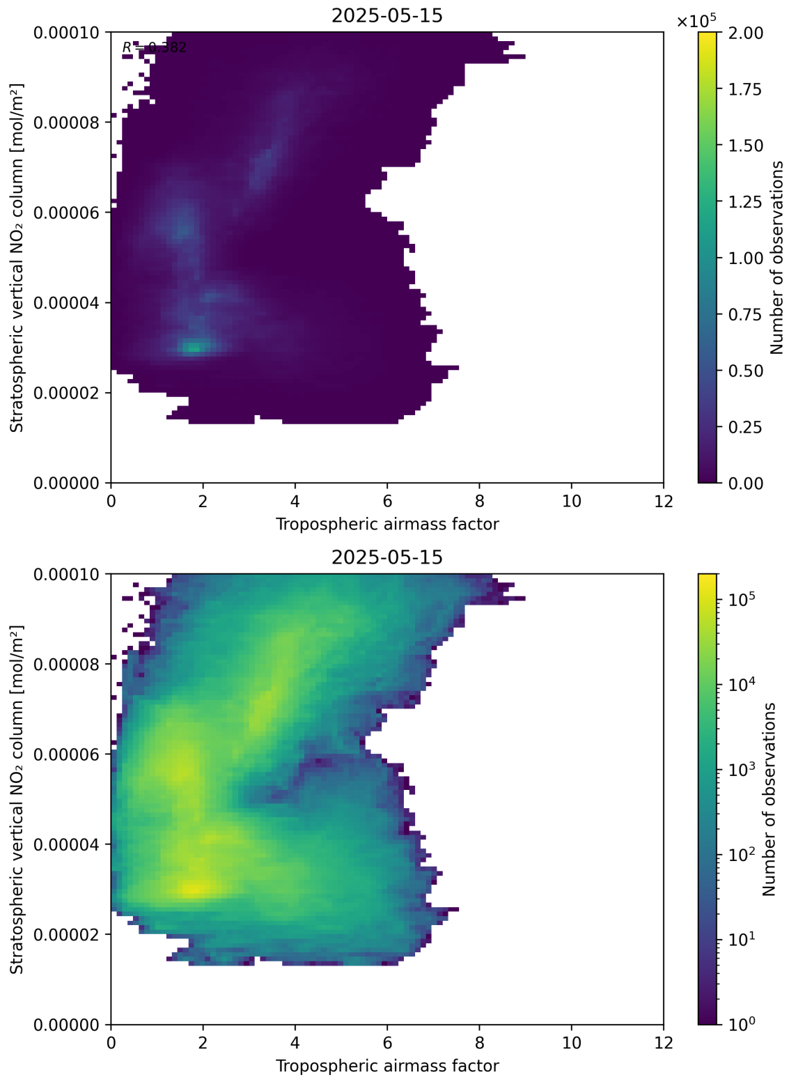
Figure 74: Scatter density plot of “Tropospheric airmass factor” against “Stratospheric vertical NO 2 column” for 2025-05-15 to 2025-05-16.
