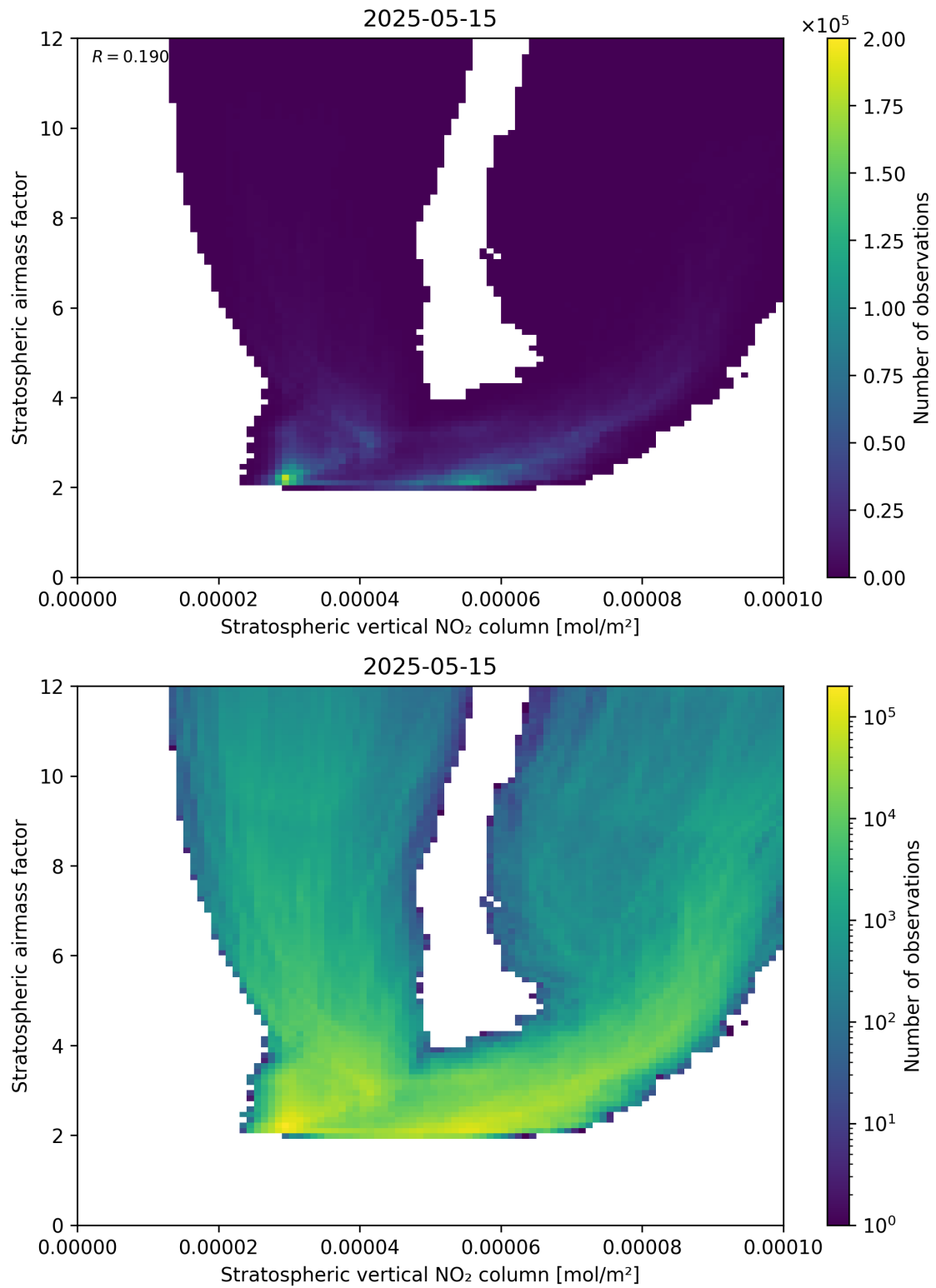
Figure 96: Scatter density plot of “Stratospheric vertical NO 2 column” against “Stratospheric airmass factor” for 2025-05-15 to 2025-05-16.
