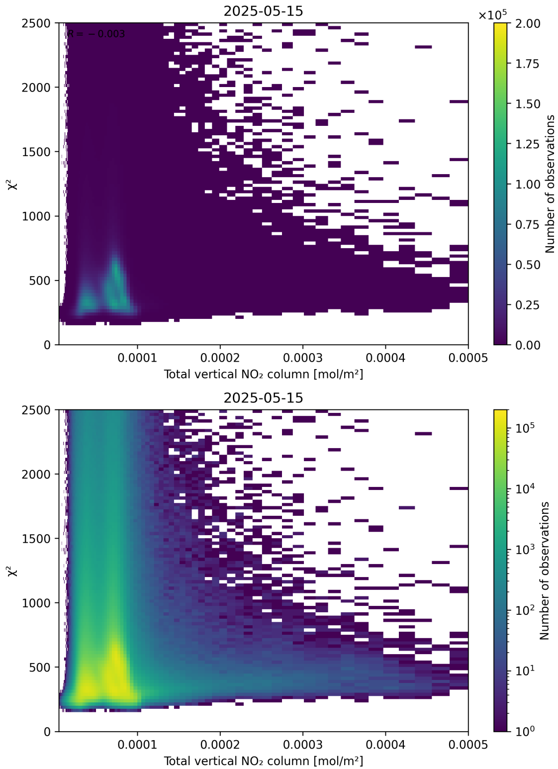
Figure 111: Scatter density plot of “Total vertical NO 2 column” against “ \chi^2 ” for 2025-05-15 to 2025-05-16.
