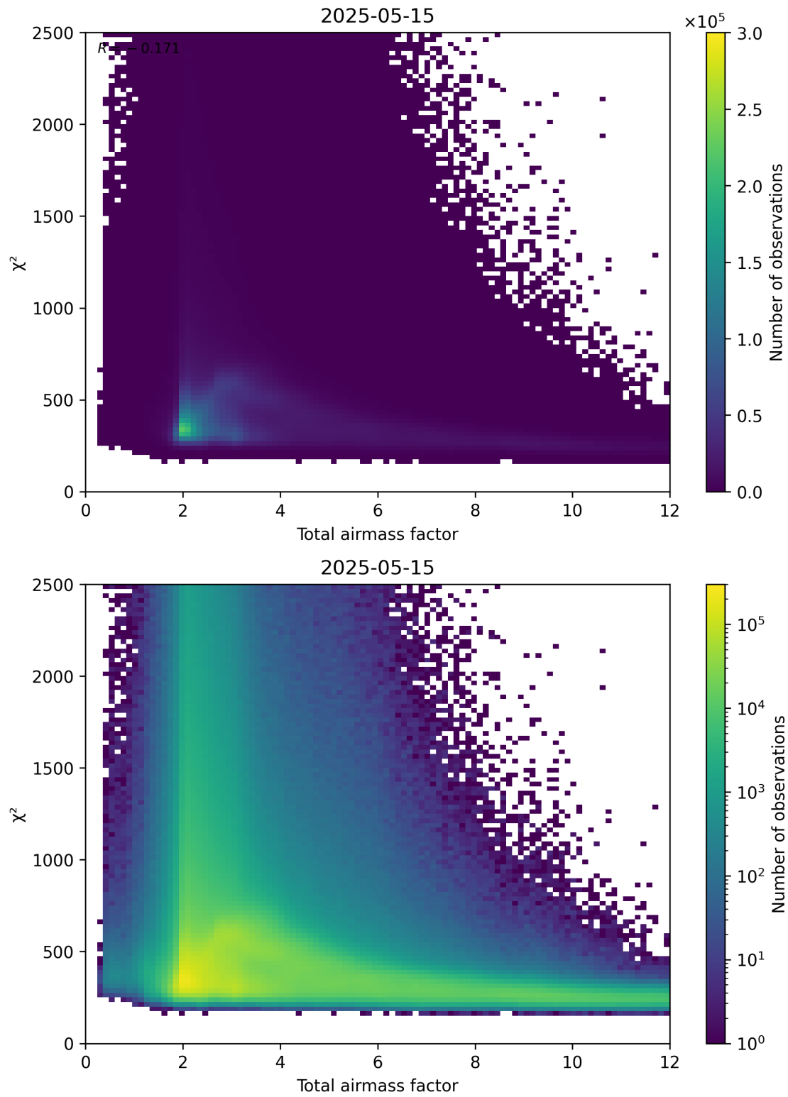
Figure 63: Scatter density plot of “Total airmass factor” against “ \chi^2 ” for 2025-05-15 to 2025-05-16.
