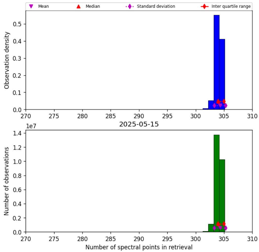
Figure 33: Histogram of “Number of spectral points in retrieval” for 2025-05-15 to 2025-05-16
