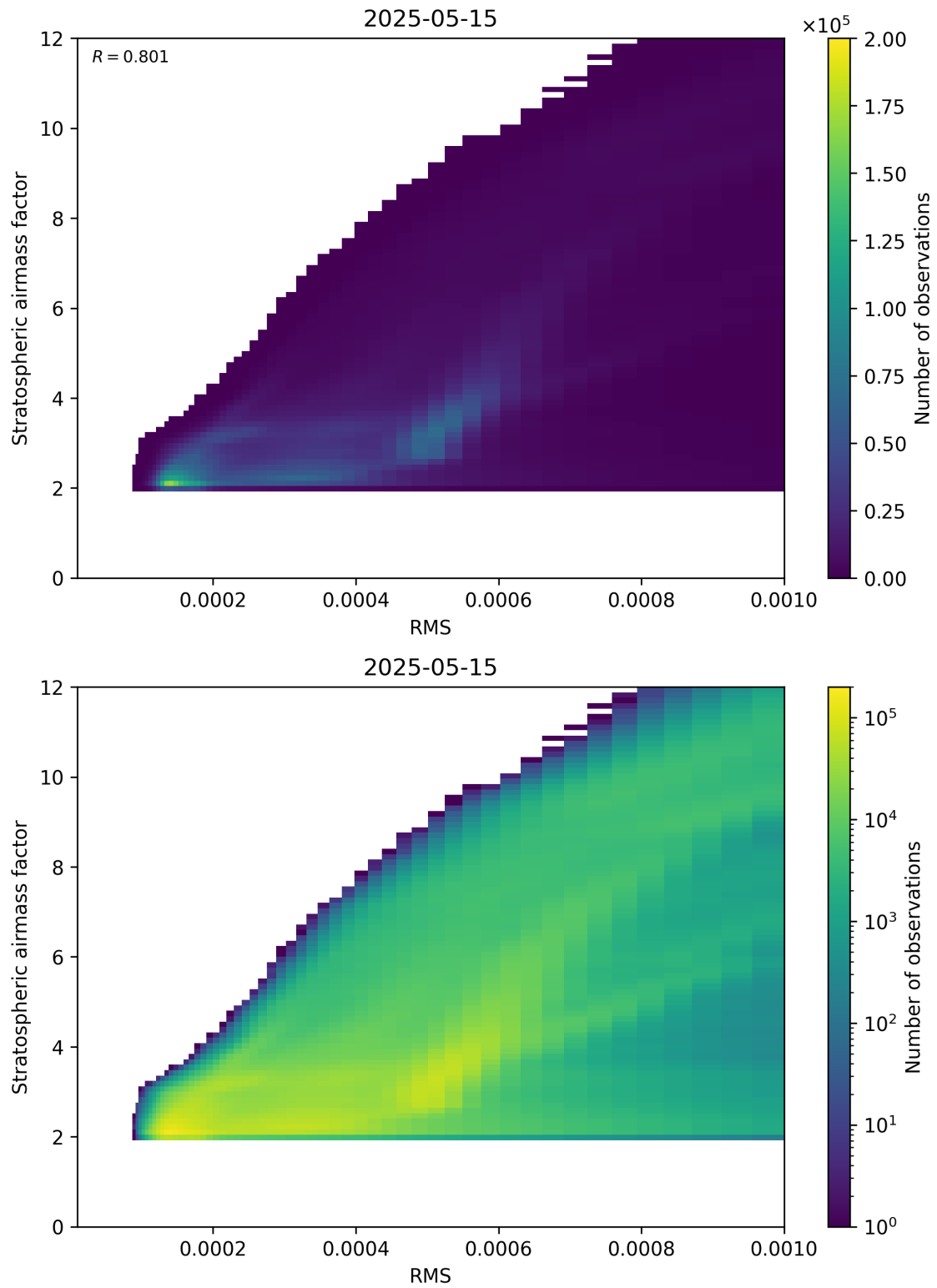
Figure 144: Scatter density plot of “RMS” against “Stratospheric airmass factor” for 2025-05-15 to 2025-05-16.
