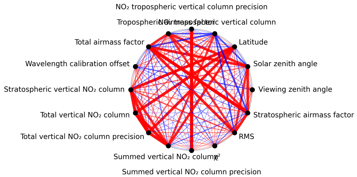
Figure 1: Map of correlation graph for 2025-05-15 to 2025-05-16.
