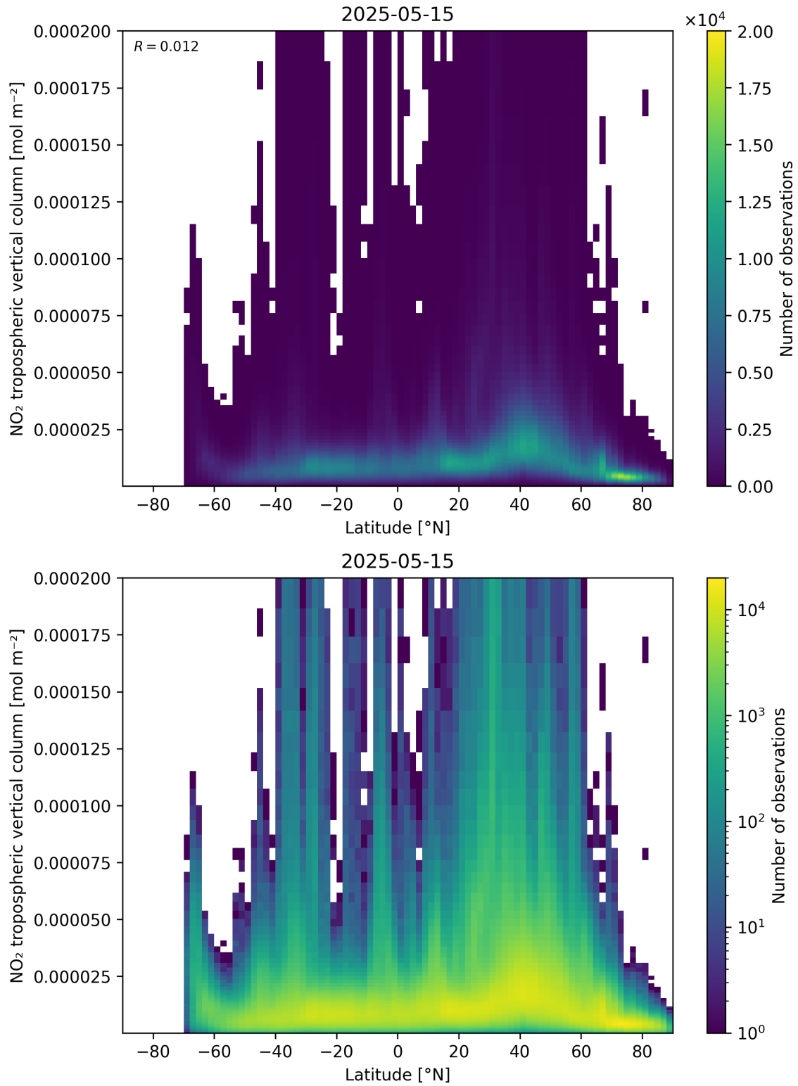
Figure 92: Scatter density plot of “Latitude” against “NO 2 tropospheric vertical column” for 2025-05-15 to 2025-05-16.
