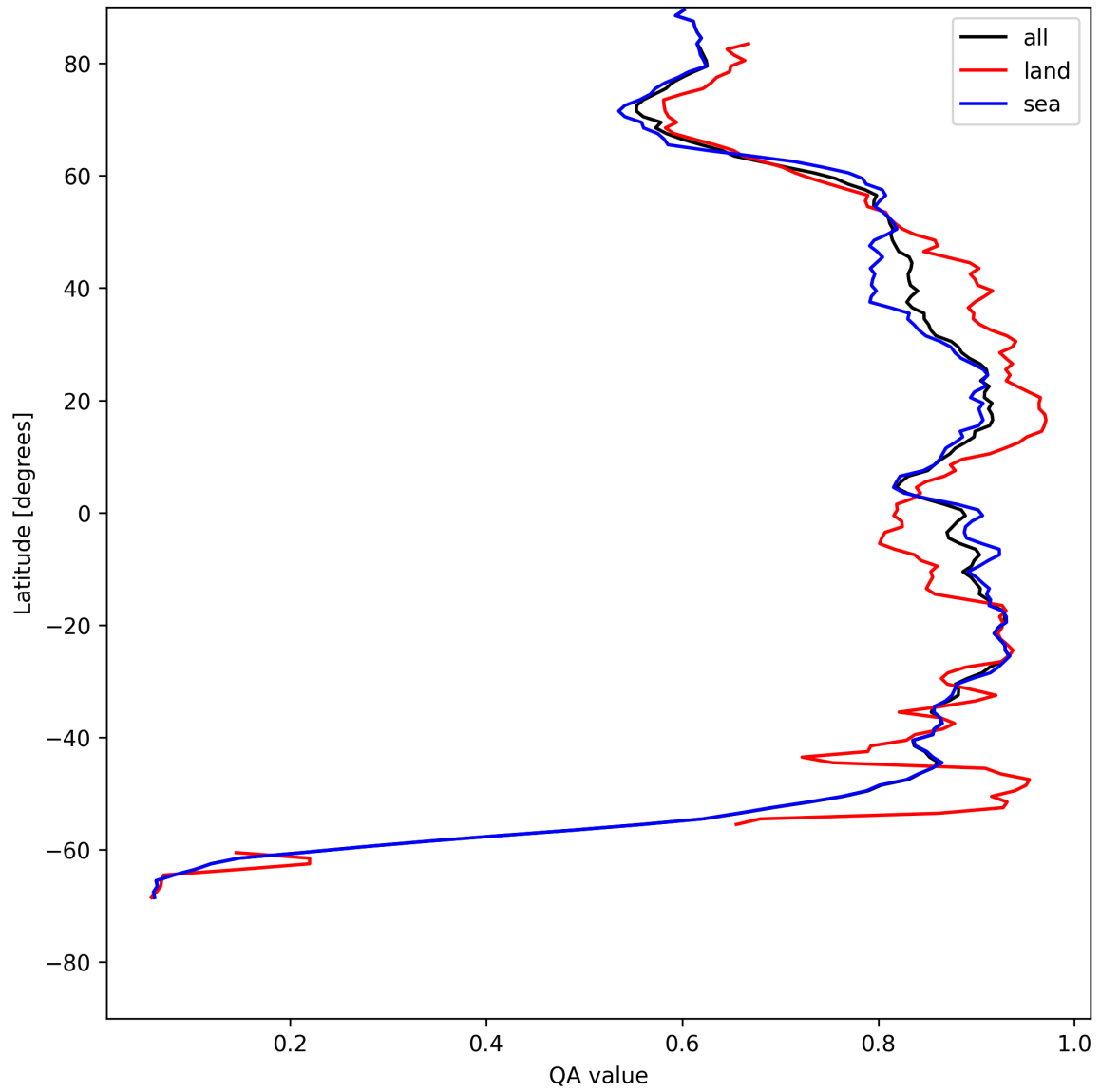
Figure 11: Zonal average of “QA value” for 2025-05-15 to 2025-05-16.
