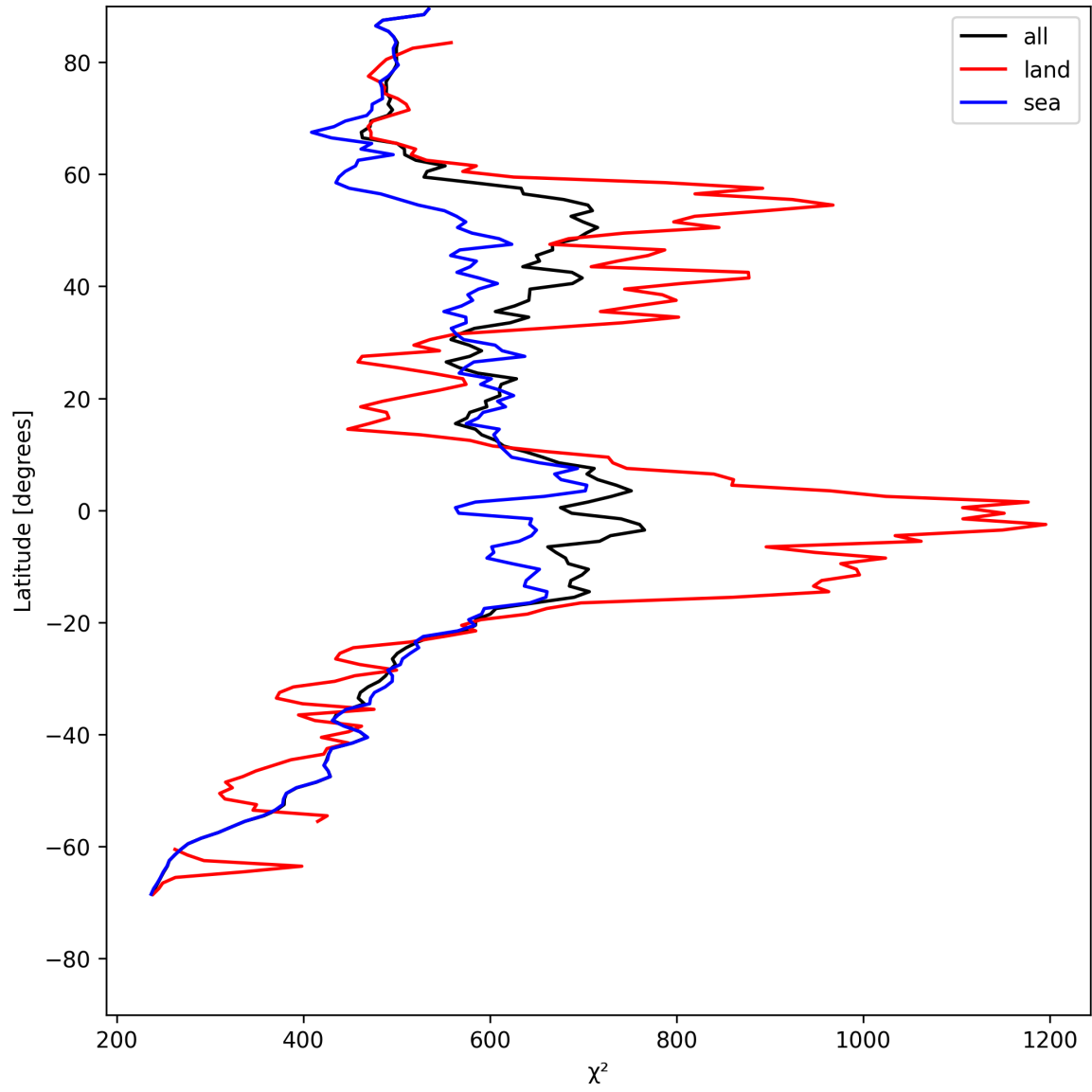
Figure 25: Zonal average of “ \chi^2 ” for 2025-05-15 to 2025-05-16.
