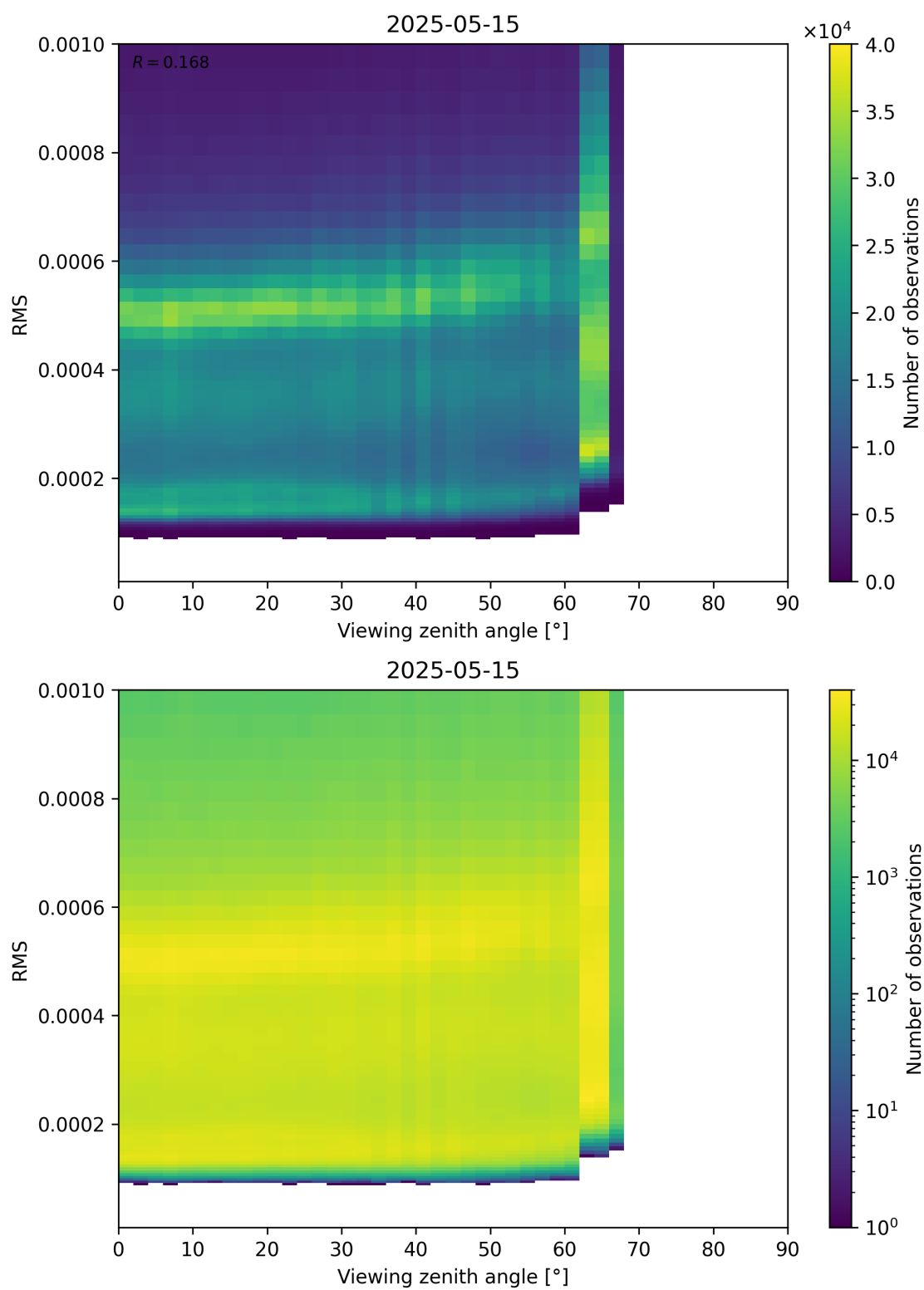
Figure 171: Scatter density plot of “Viewing zenith angle” against “RMS” for 2025-05-15 to 2025-05-16.
