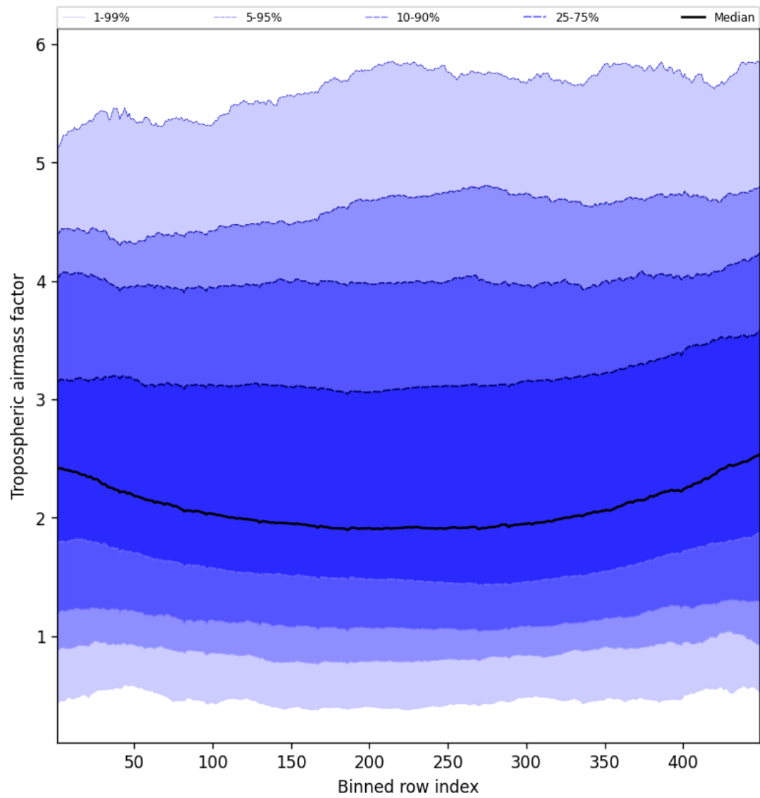
Figure 48: Along track statistics of “Tropospheric airmass factor” for 2025-05-15 to 2025-05-16
