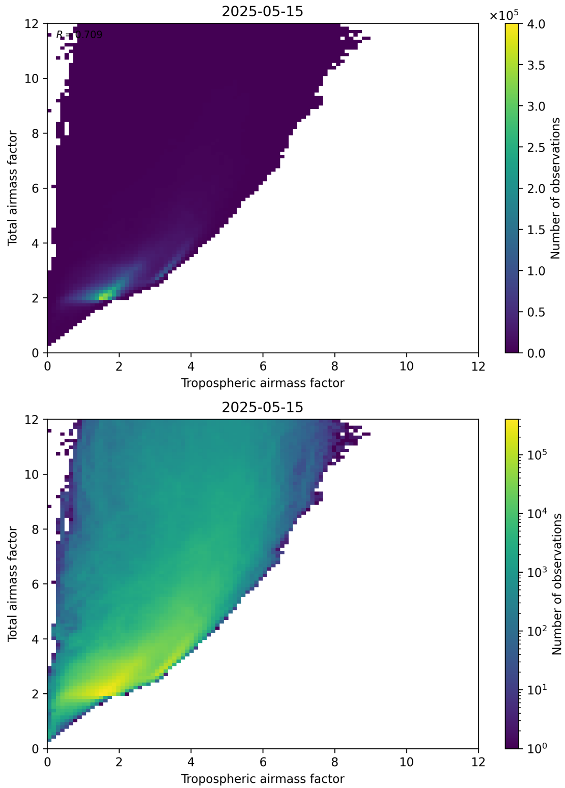
Figure 72: Scatter density plot of “Tropospheric airmass factor” against “Total airmass factor” for 2025-05-15 to 2025-05-16.
