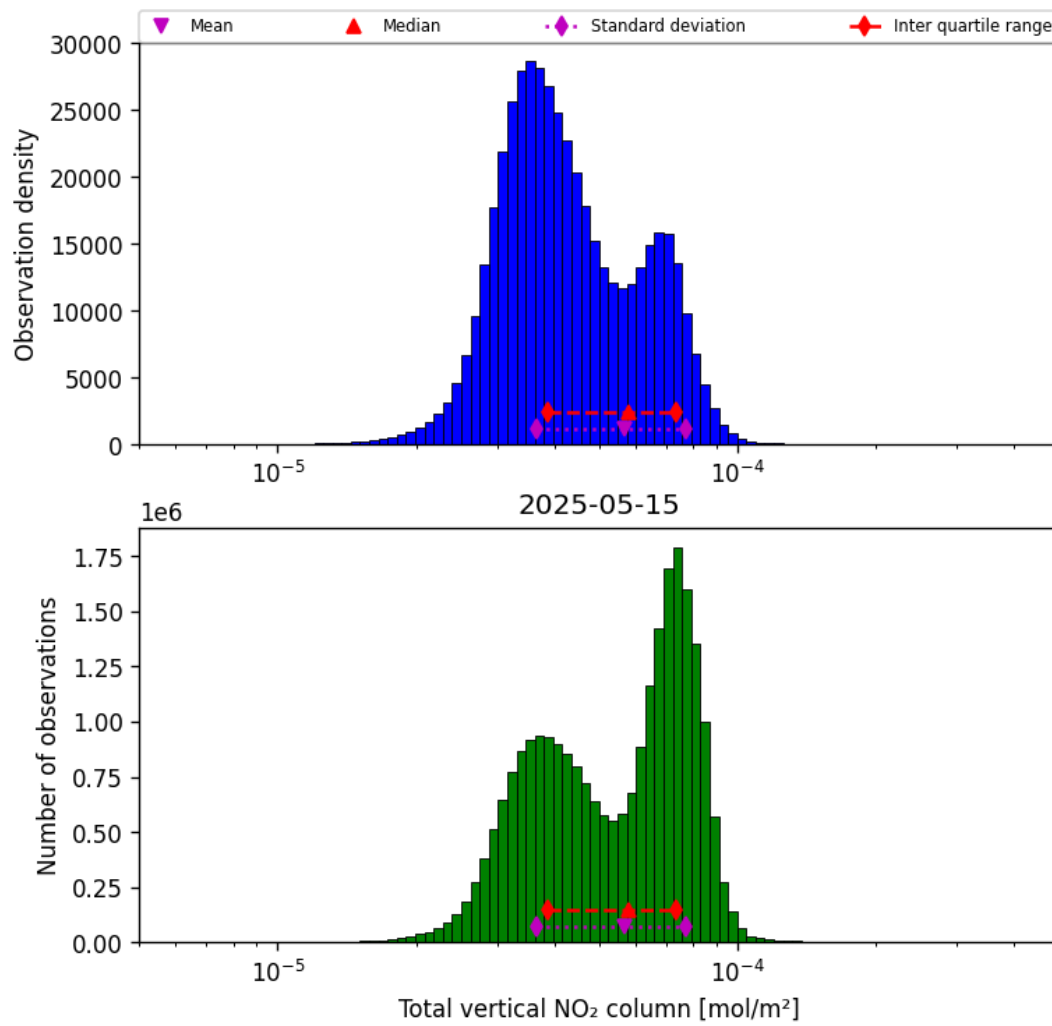
Figure 38: Histogram of “Total vertical NO 2 column” for 2025-05-15 to 2025-05-16
