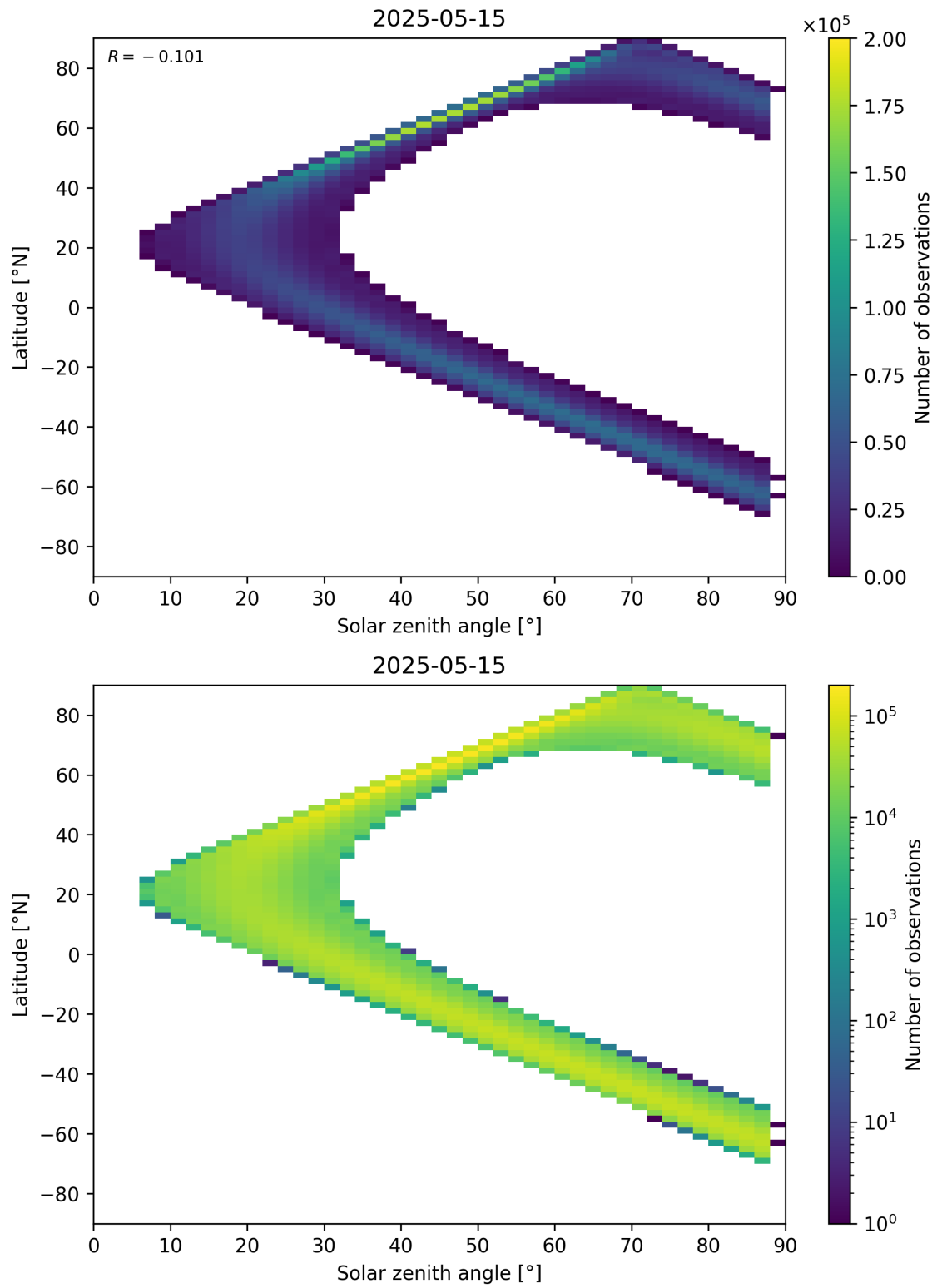
Figure 149: Scatter density plot of “Solar zenith angle” against “Latitude” for 2025-05-15 to 2025-05-16.
