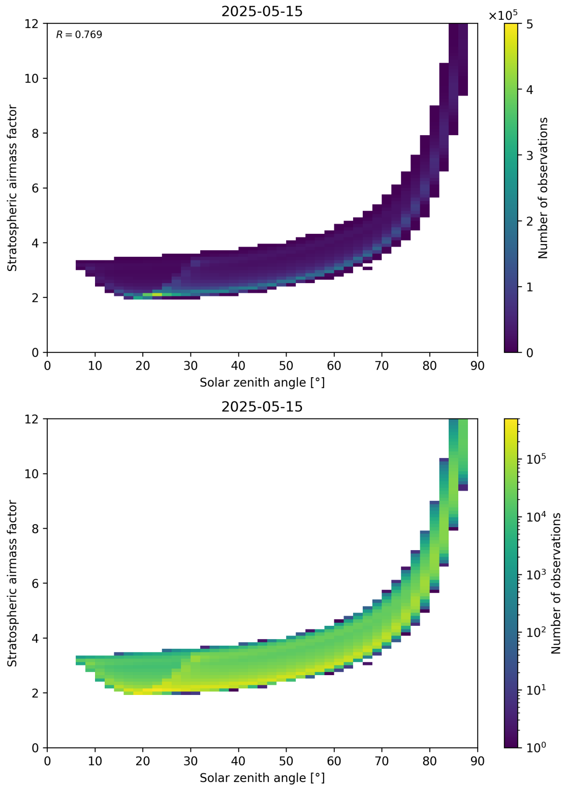
Figure 145: Scatter density plot of “Solar zenith angle” against “Stratospheric airmass factor” for 2025-05-15 to 2025-05-16.
