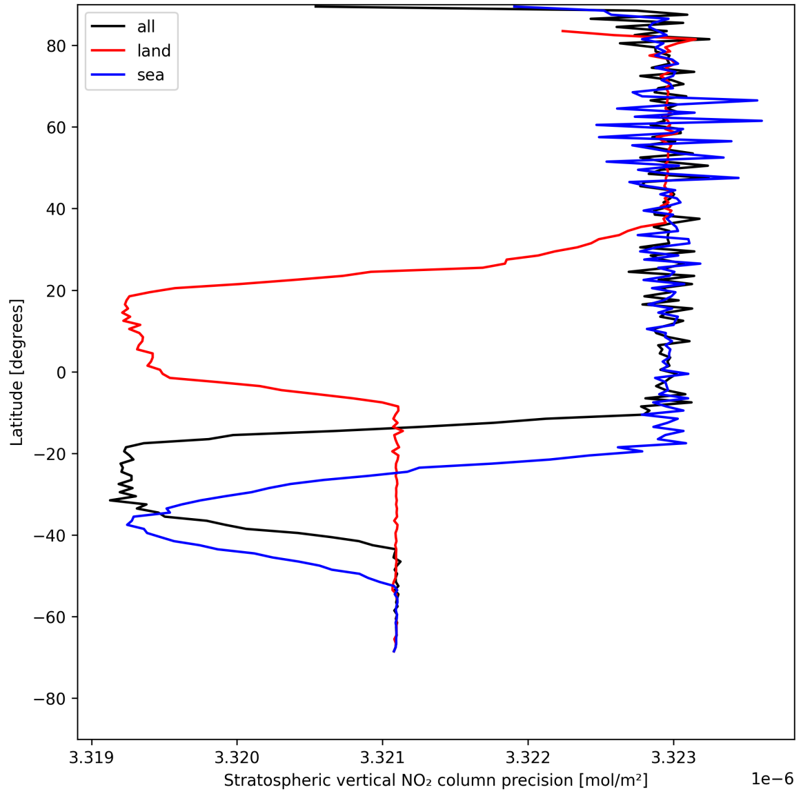
Figure 20: Zonal average of “Stratospheric vertical NO 2 column precision” for 2025-05-15 to 2025-05-16.
