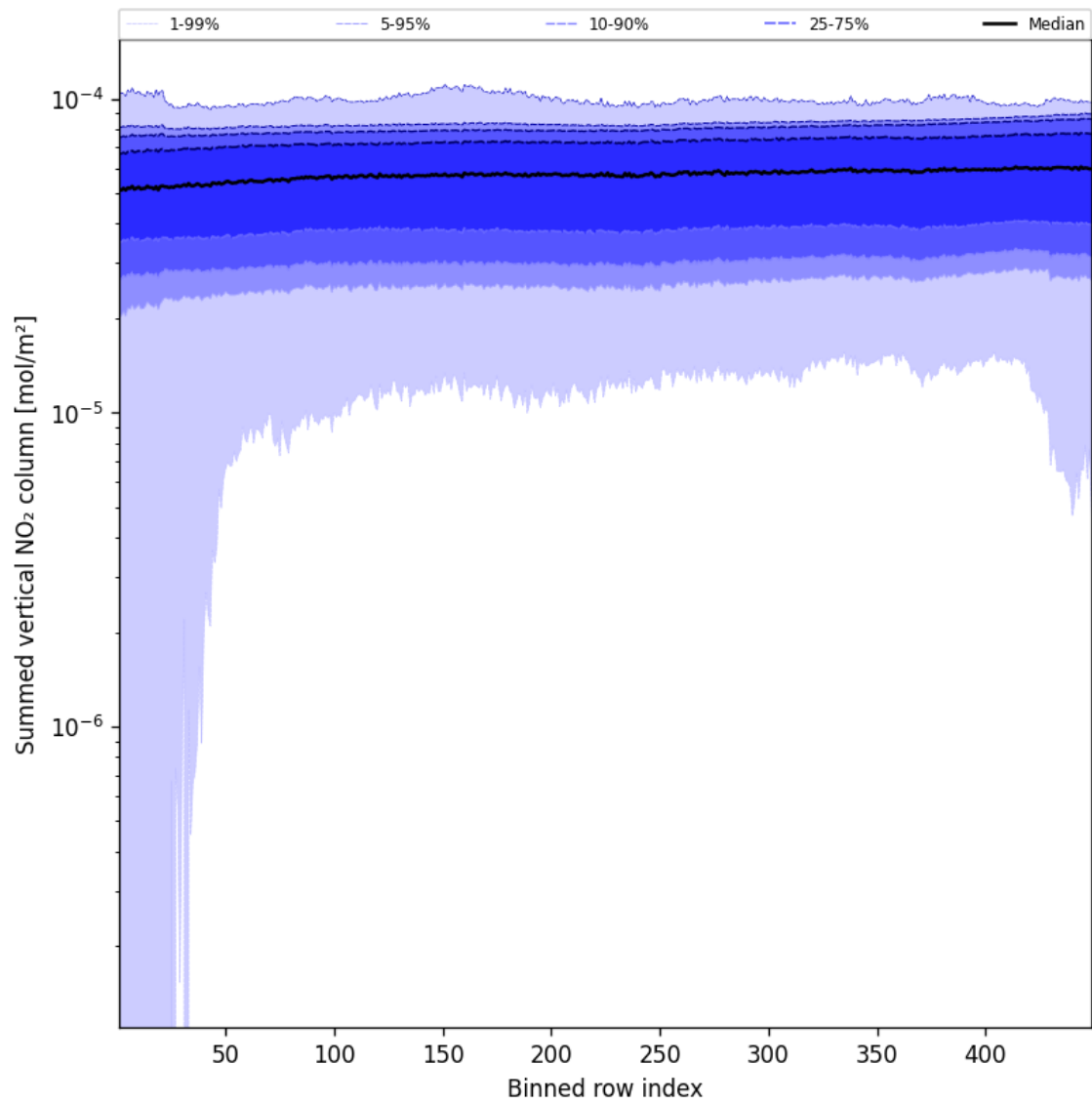
Figure 57: Along track statistics of “Summed vertical NO 2 column” for 2025-05-15 to 2025-05-16
