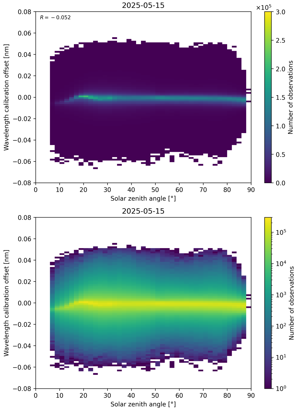
Figure 158: Scatter density plot of “Solar zenith angle” against “Wavelength calibration offset” for 2025-05-15 to 2025-05-16.
