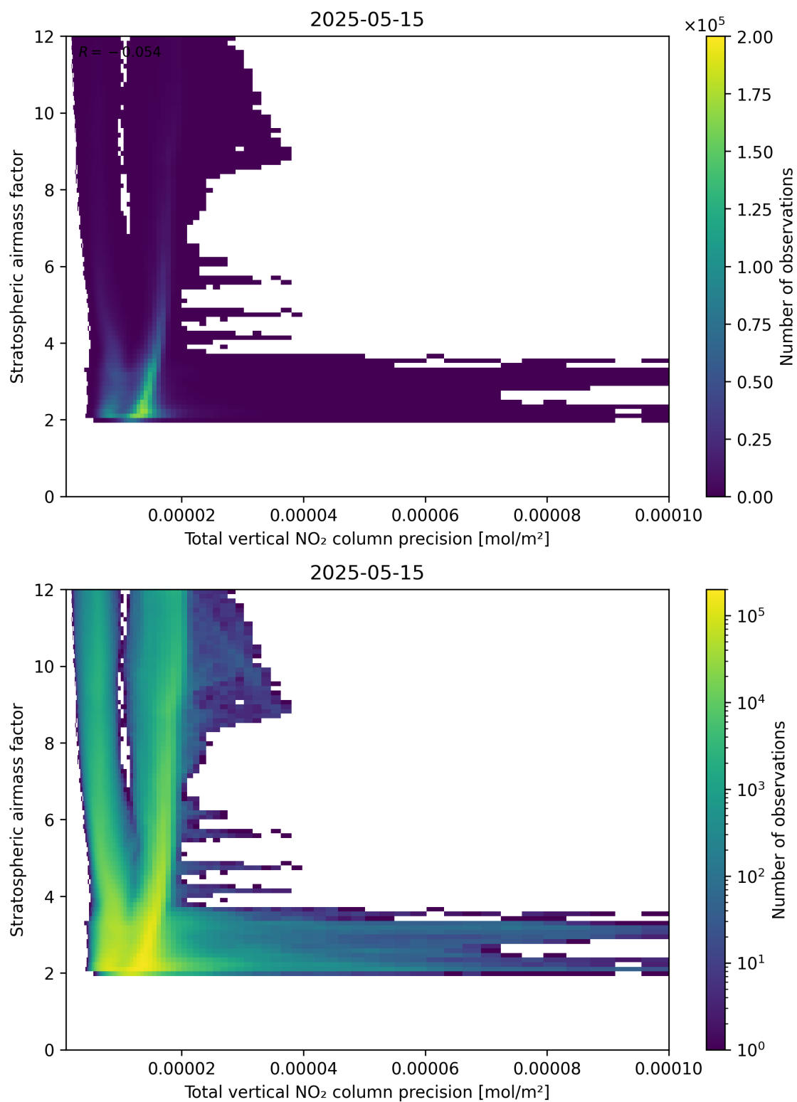
Figure 115: Scatter density plot of “Total vertical NO 2 column precision” against “Stratospheric air mass factor” for 2025-05-15 to 2025-05-16.
