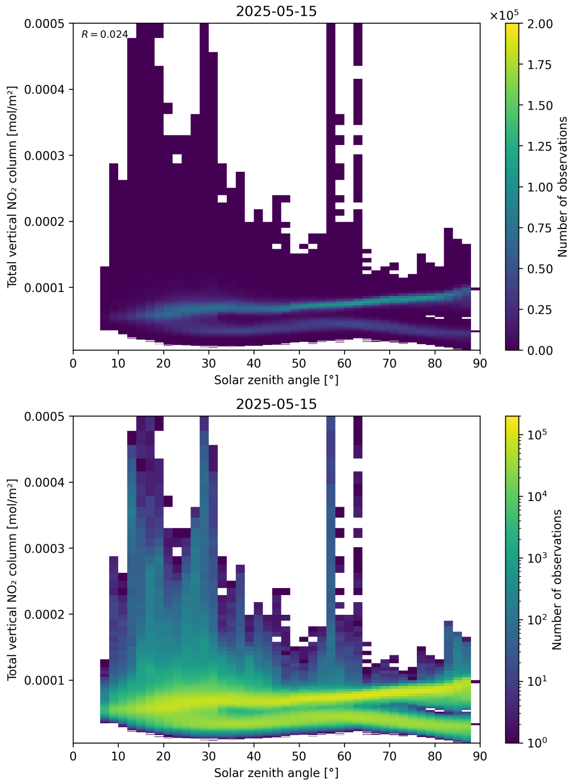
Figure 153: Scatter density plot of “Solar zenith angle” against “Total vertical NO 2 column” for 2025-05-15 to 2025-05-16.
