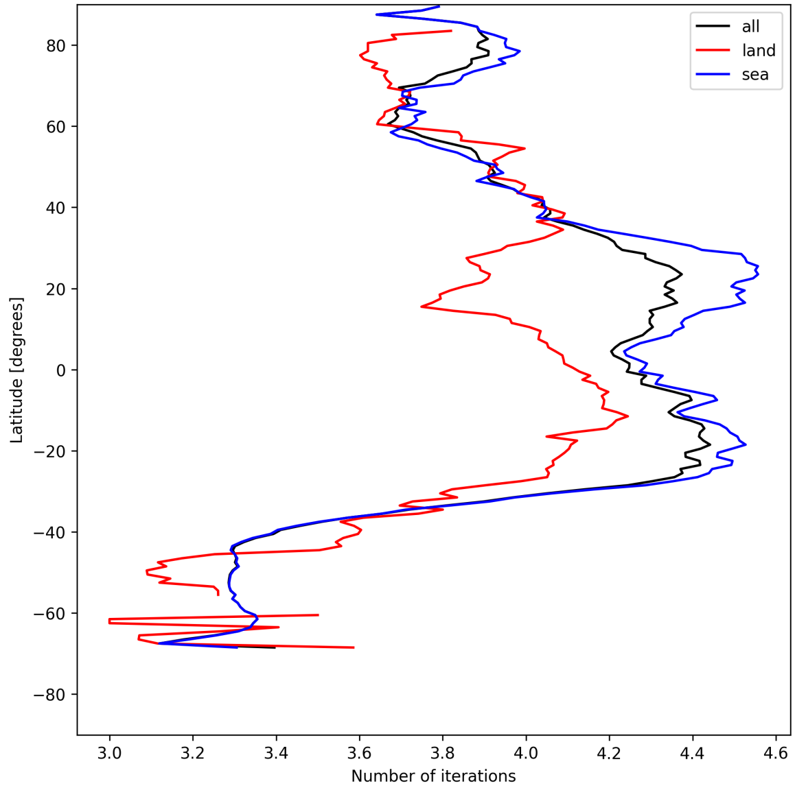
Figure 17: Zonal average of “Number of iterations” for 2025-05-15 to 2025-05-16.
