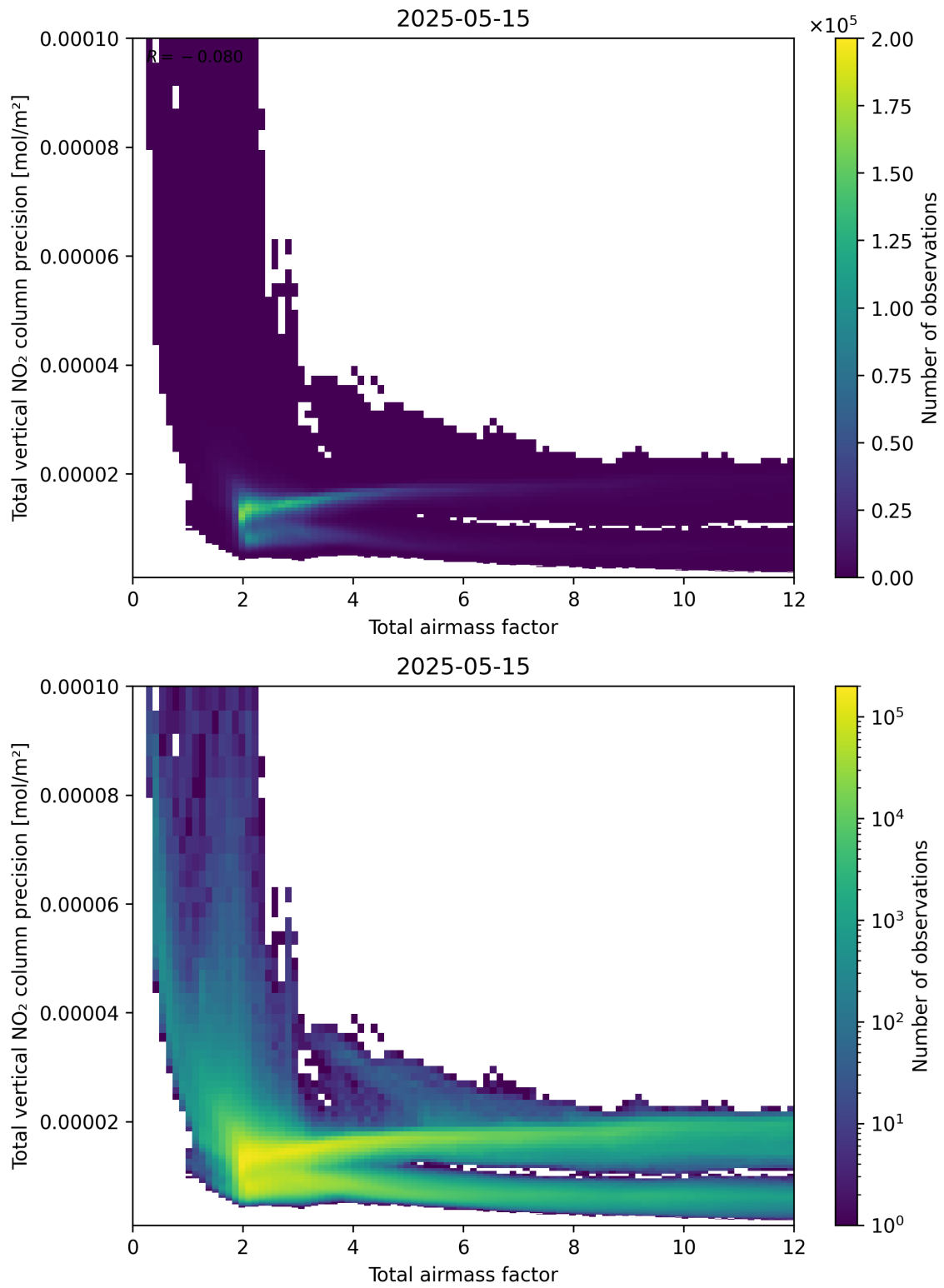
Figure 68: Scatter density plot of “Total airmass factor” against “Total vertical NO 2 column precision” for 2025-05-15 to 2025-05-16.
