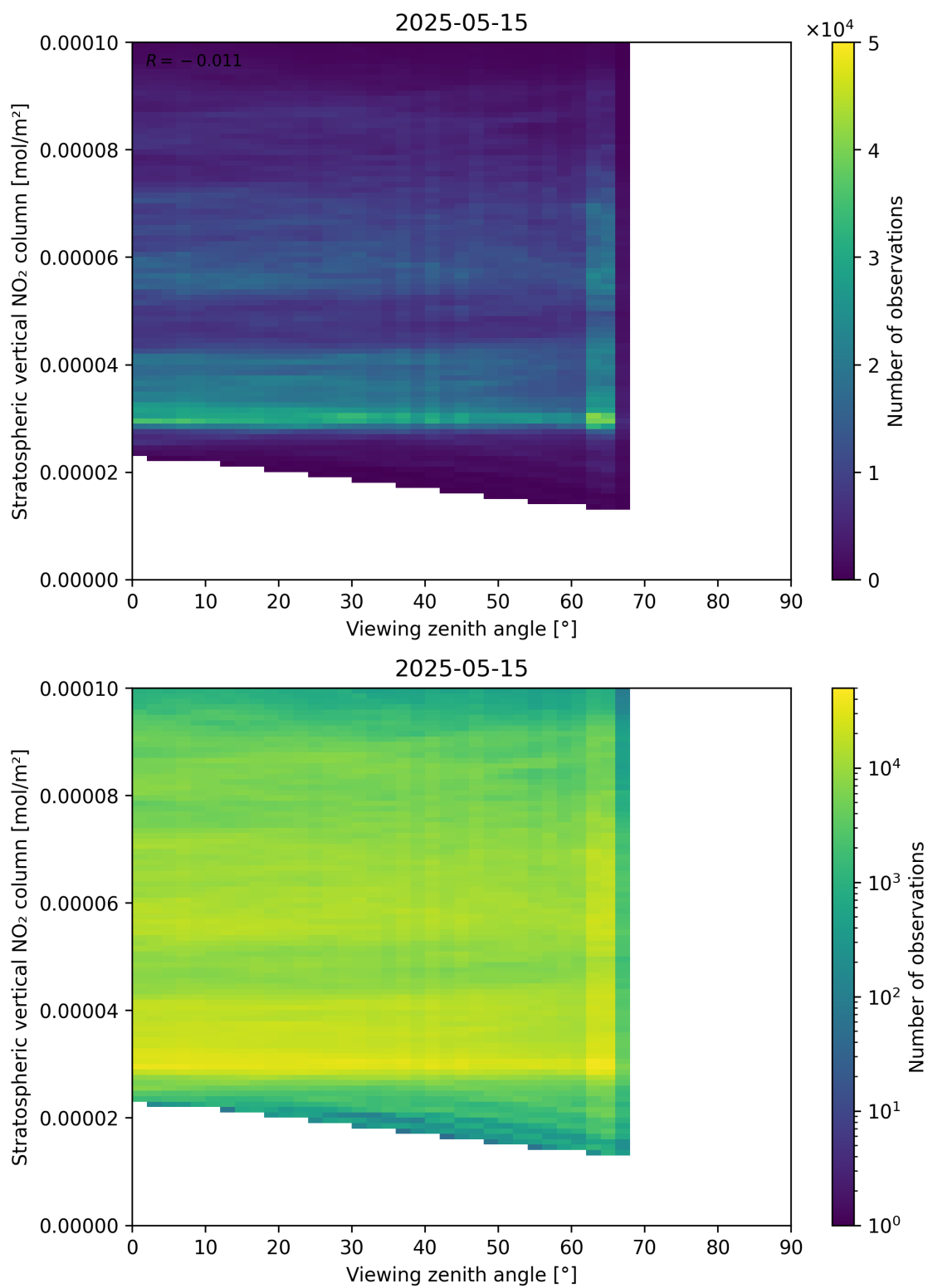
Figure 164: Scatter density plot of “Viewing zenith angle” against “Stratospheric vertical NO 2 column” for 2025-05-15 to 2025-05-16.
