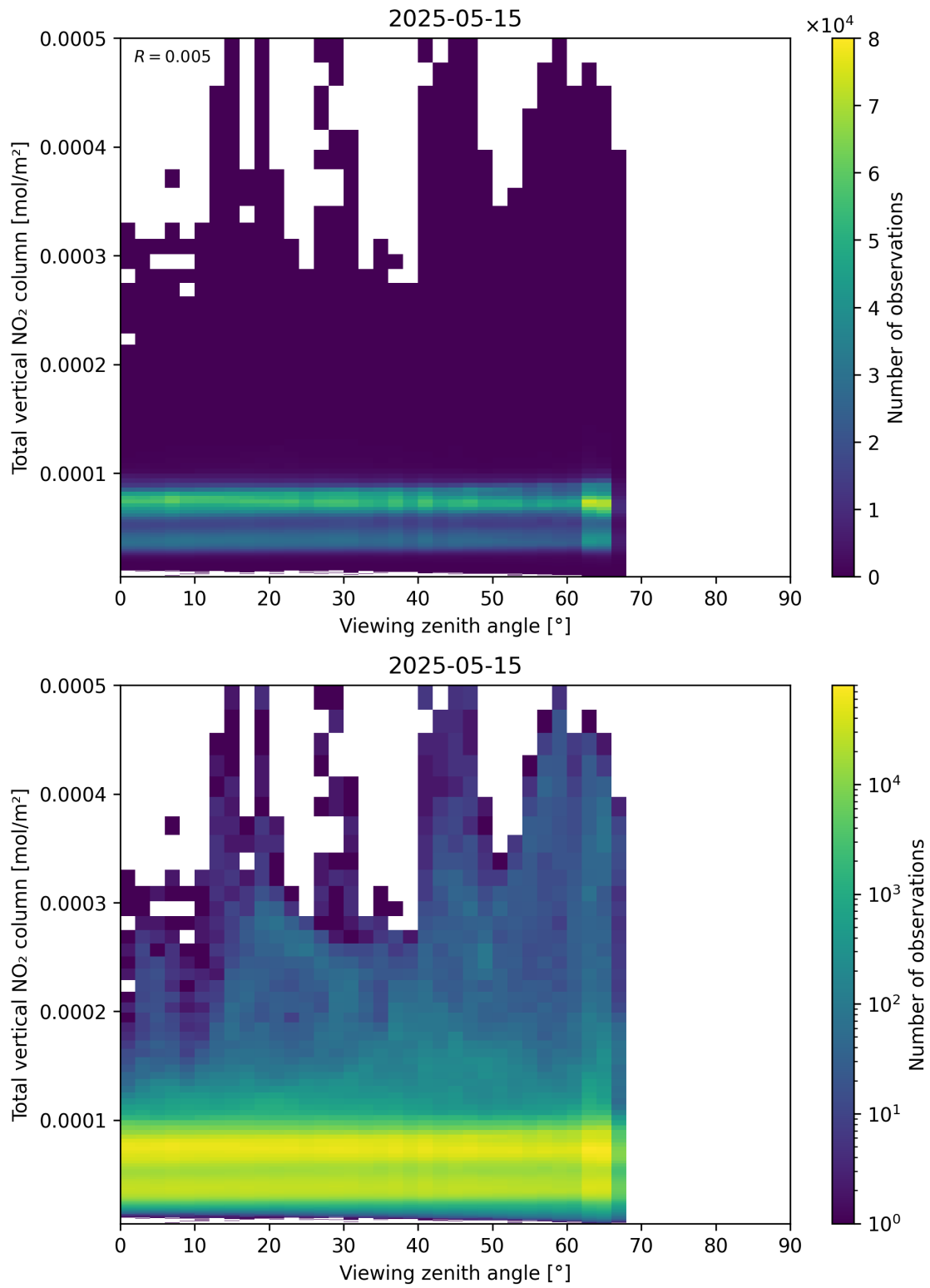
Figure 167: Scatter density plot of “Viewing zenith angle” against “Total vertical NO 2 column” for 2025-05-15 to 2025-05-16.
