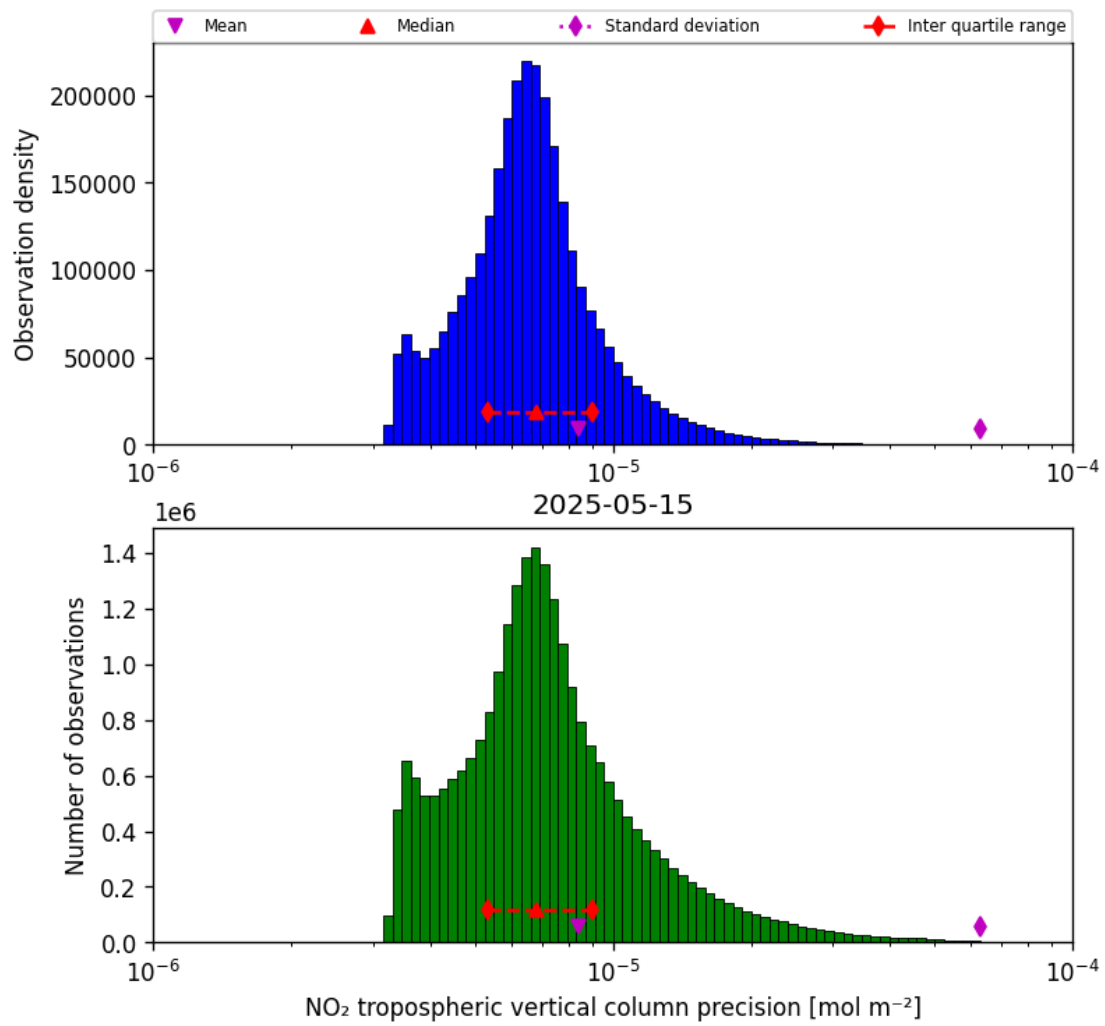
Figure 30: Histogram of “NO 2 tropospheric vertical column precision” for 2025-05-15 to 2025-05-16
