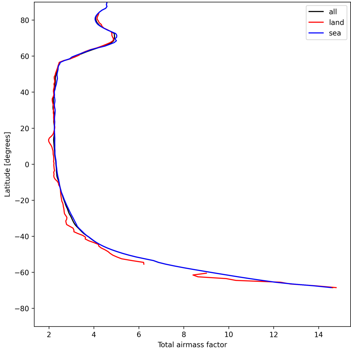
Figure 15: Zonal average of “Total airmass factor” for 2025-05-15 to 2025-05-16.
