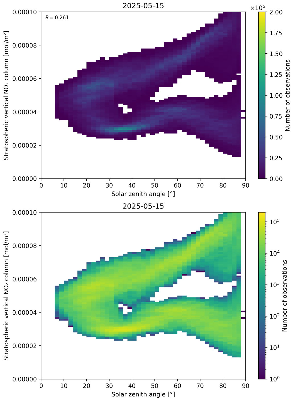
Figure 150: Scatter density plot of “Solar zenith angle” against “Stratospheric vertical NO 2 column” for 2025-05-15 to 2025-05-16.
