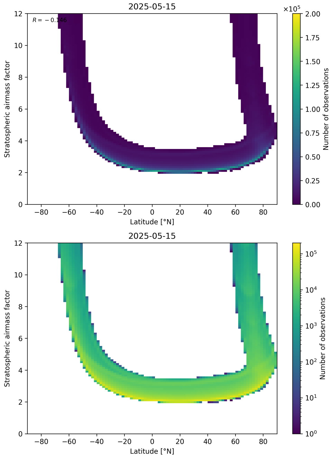
Figure 83: Scatter density plot of “Latitude” against “Stratospheric air mass factor” for 2025-05-15 to 2025-05-16.
