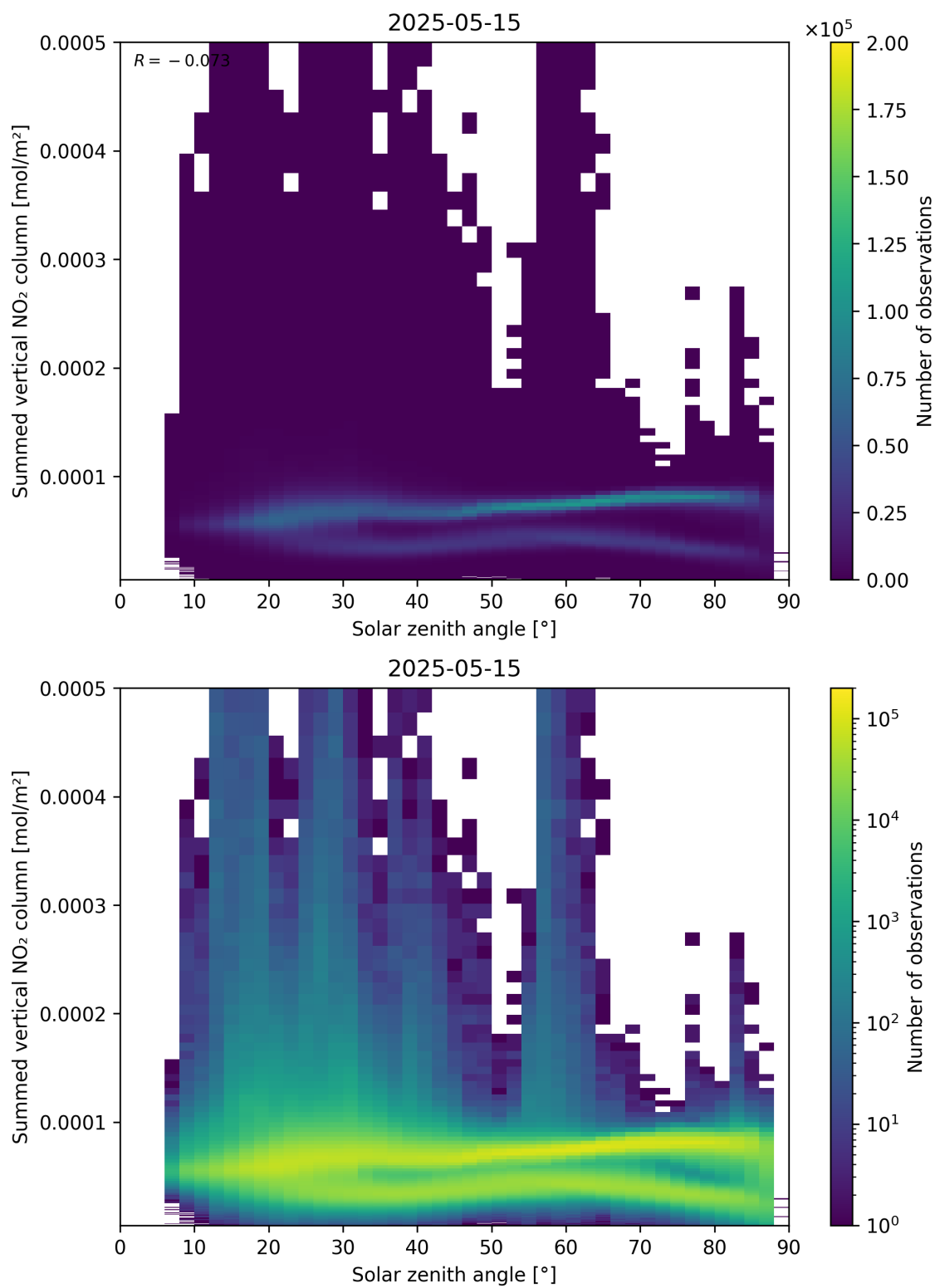
Figure 151: Scatter density plot of “Solar zenith angle” against “Summed vertical NO 2 column” for 2025-05-15 to 2025-05-16.
