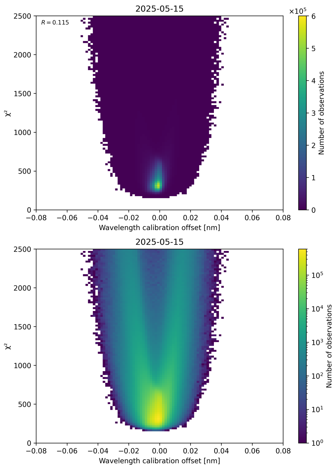
Figure 175: Scatter density plot of “Wavelength calibration offset” against “ \chi^2 ” for 2025-05-15 to 2025-05-16.
