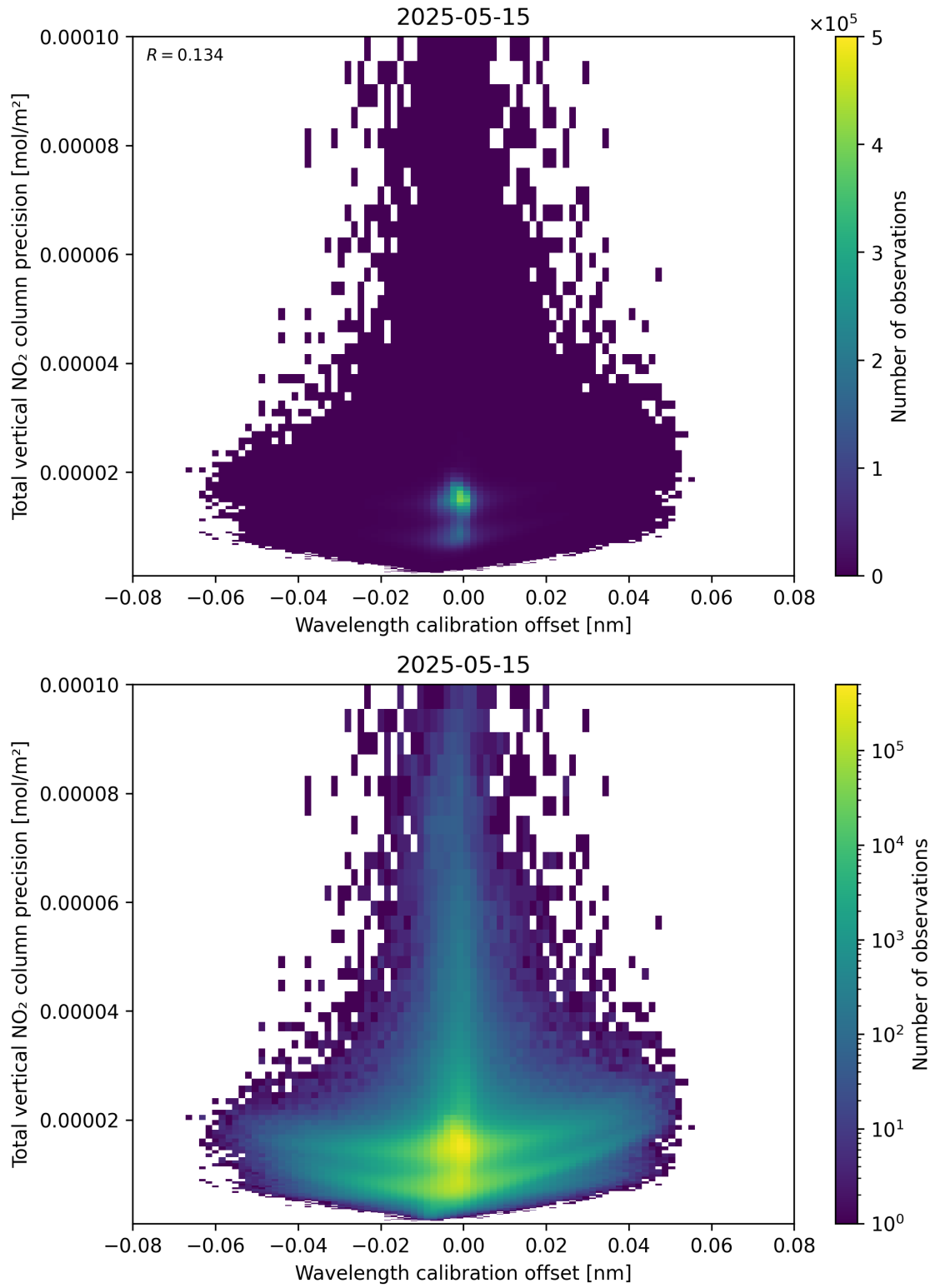
Figure 180: Scatter density plot of “Wavelength calibration offset” against “Total vertical NO 2 column precision” for 2025-05-15 to 2025-05-16.
