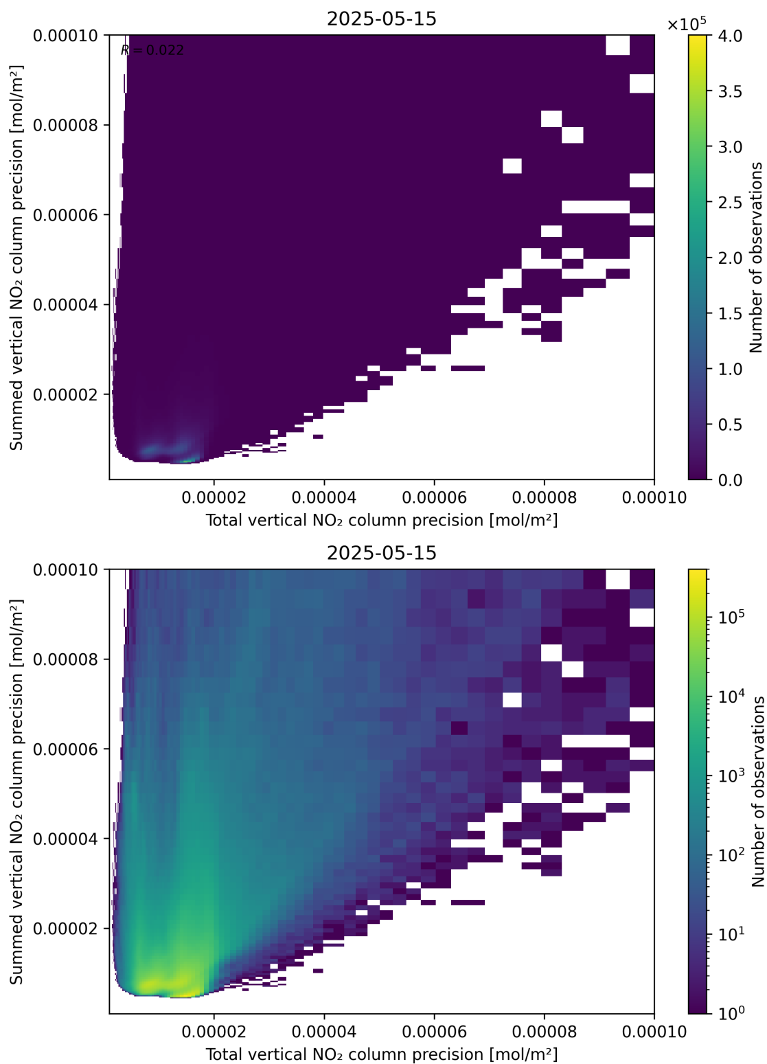
Figure 118: Scatter density plot of “Total vertical NO 2 column precision” against “Summed vertical NO 2 column precision” for 2025-05-15 to 2025-05-16.
