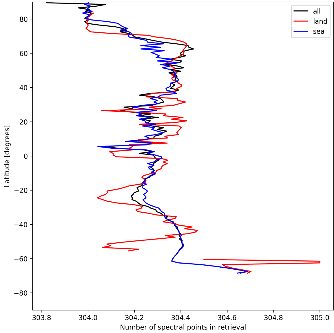
Figure 16: Zonal average of “Number of spectral points in retrieval” for 2025-05-15 to 2025-05-16.
