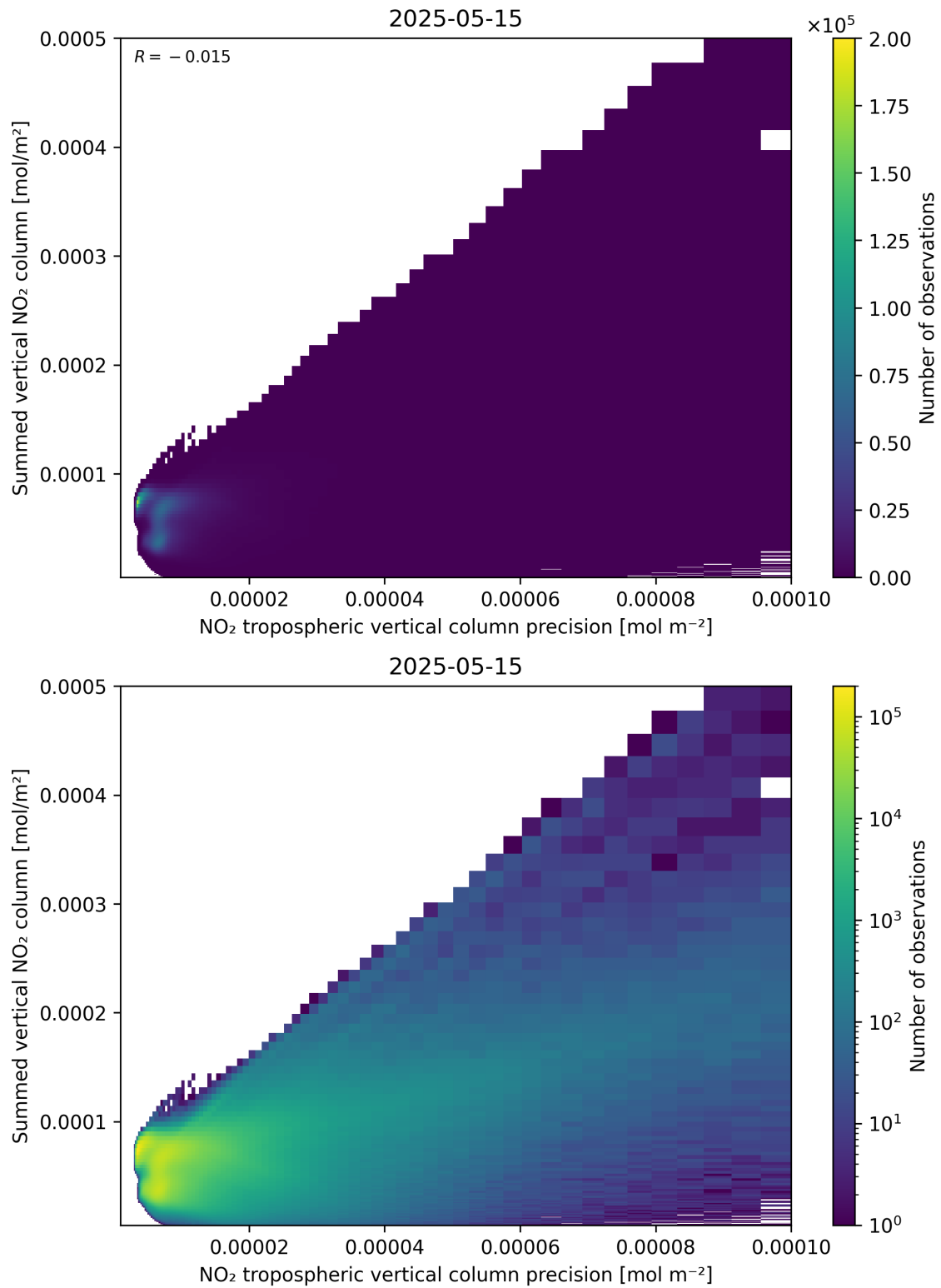
Figure 136: Scatter density plot of “NO 2 tropospheric vertical column precision” against “Summed vertical NO 2 column” for 2025-05-15 to 2025-05-16.
