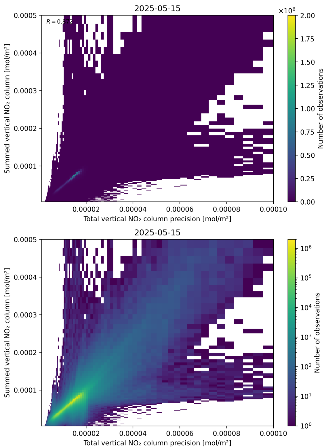
Figure 117: Scatter density plot of “Total vertical NO 2 column precision” against “Summed vertical NO 2 column” for 2025-05-15 to 2025-05-16.
