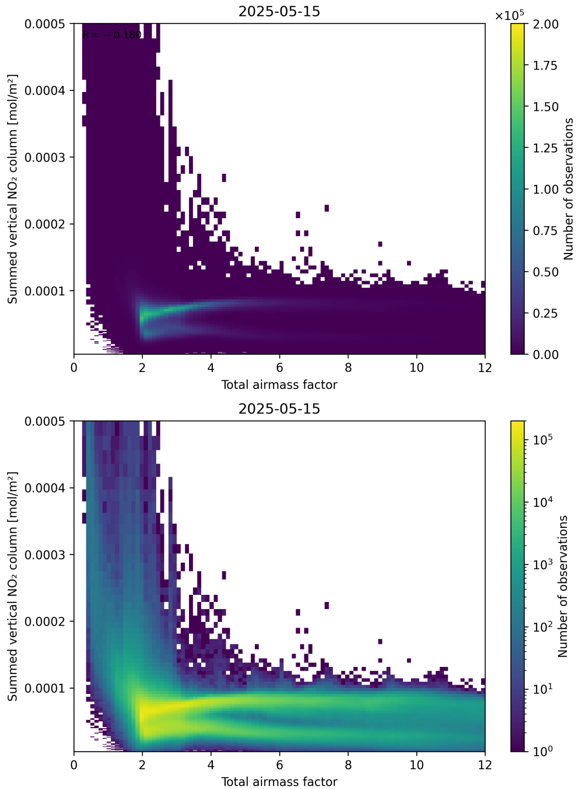
Figure 65: Scatter density plot of “Total airmass factor” against “Summed vertical NO 2 column” for 2025-05-15 to 2025-05-16.
