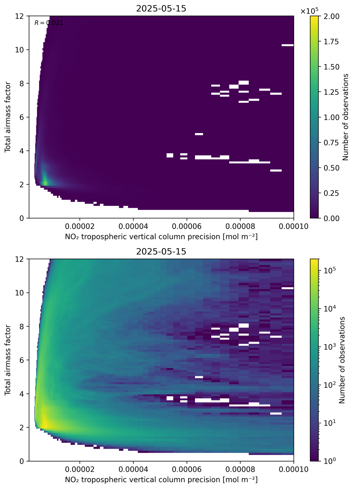
Figure 132: Scatter density plot of “NO 2 tropospheric vertical column precision” against “Total air mass factor” for 2025-05-15 to 2025-05-16.
