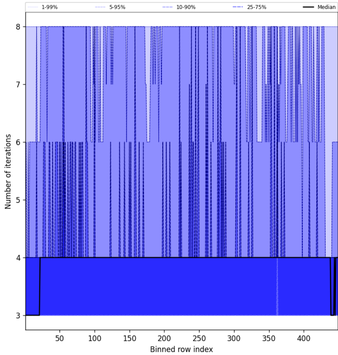
Figure 51: Along track statistics of “Number of iterations” for 2025-05-15 to 2025-05-16
