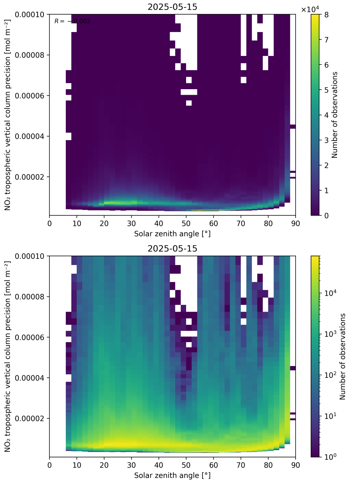
Figure 156: Scatter density plot of “Solar zenith angle” against “NO 2 tropospheric vertical column precision” for 2025-05-15 to 2025-05-16.
