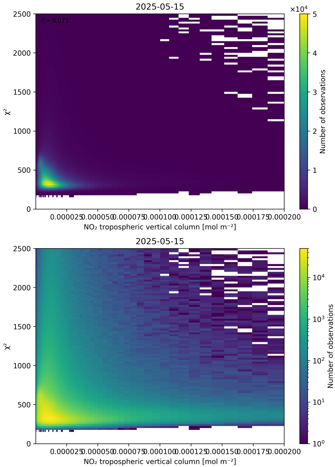
Figure 124: Scatter density plot of “NO 2 tropospheric vertical column” against “ \chi^2 ” for 2025-05-15 to 2025-05-16.
