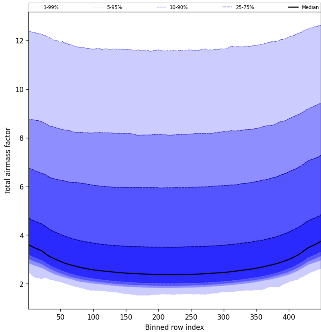
Figure 49: Along track statistics of “Total airmass factor” for 2025-05-15 to 2025-05-16
