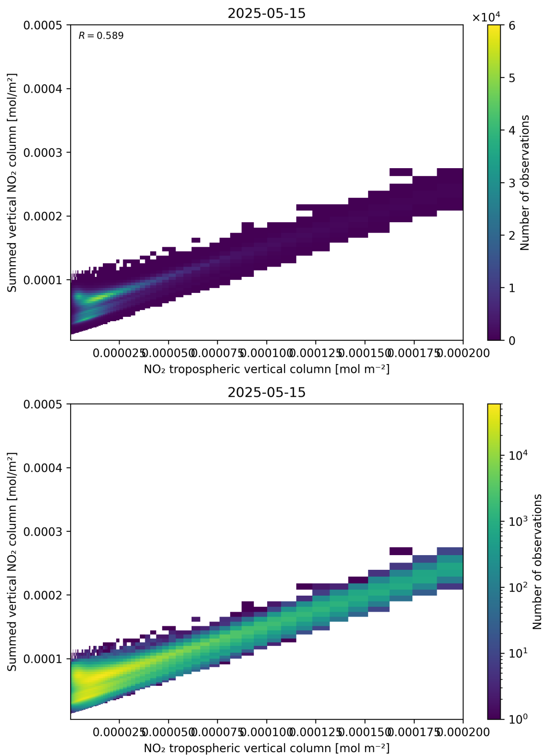
Figure 126: Scatter density plot of “NO 2 tropospheric vertical column” against “Summed vertical NO 2 column” for 2025-05-15 to 2025-05-16.
