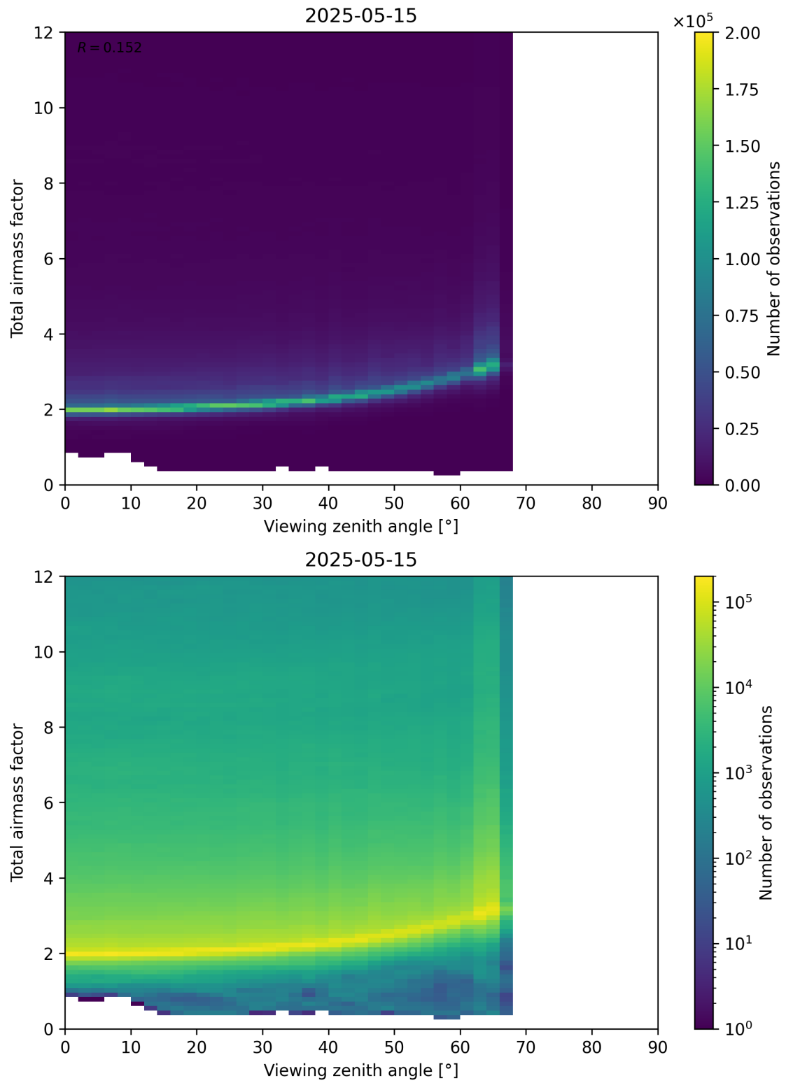
Figure 160: Scatter density plot of “Viewing zenith angle” against “Total airmass factor” for 2025-05-15 to 2025-05-16.
