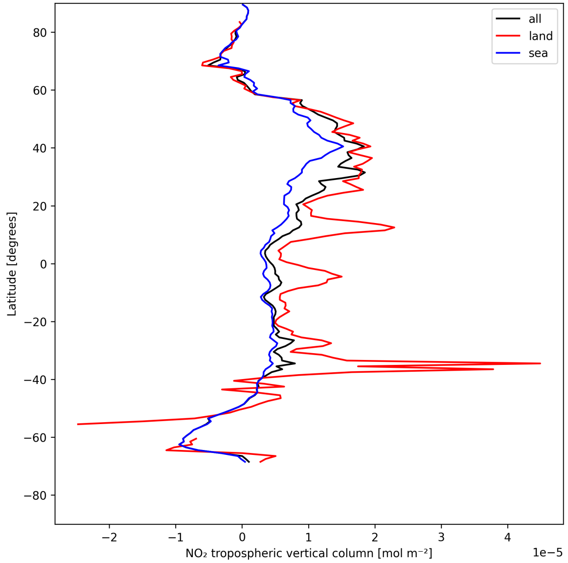
Figure 12: Zonal average of “NO 2 tropospheric vertical column” for 2025-05-15 to 2025-05-16.
