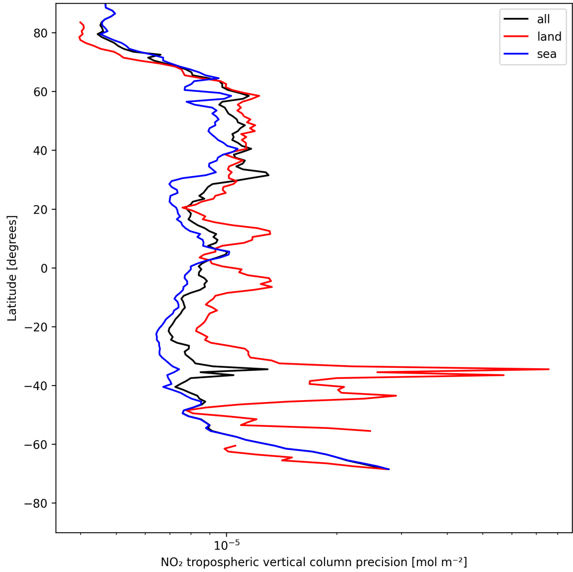
Figure 13: Zonal average of “NO 2 tropospheric vertical column precision” for 2025-05-15 to 2025-05-16.
