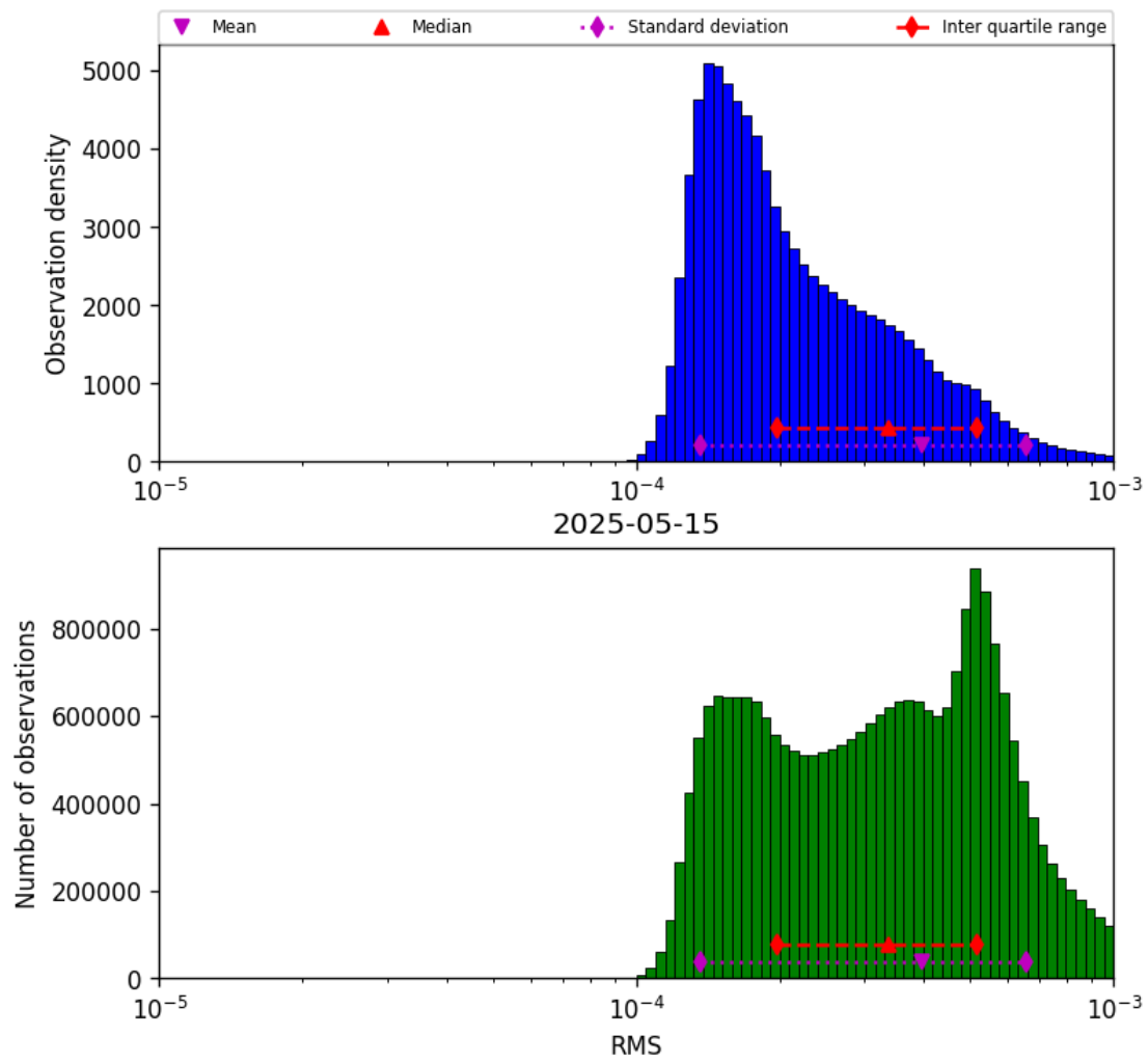
Figure 43: Histogram of “RMS” for 2025-05-15 to 2025-05-16
