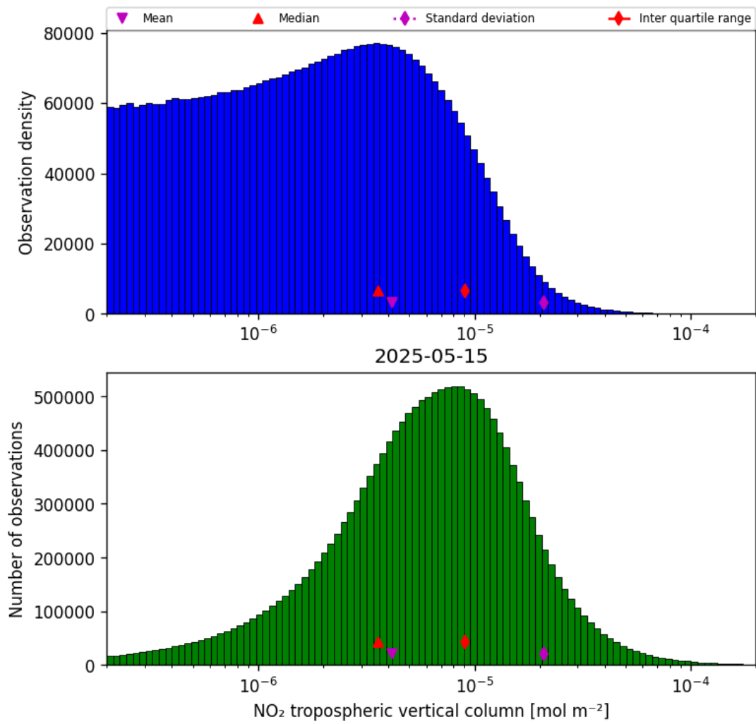
Figure 29: Histogram of “NO 2 tropospheric vertical column” for 2025-05-15 to 2025-05-16
