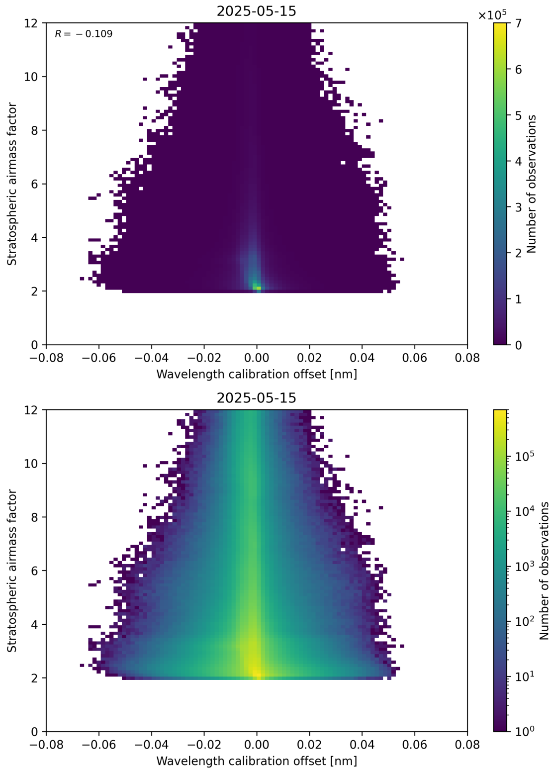
Figure 174: Scatter density plot of “Wavelength calibration offset” against “Stratospheric airmass factor” for 2025-05-15 to 2025-05-16.
