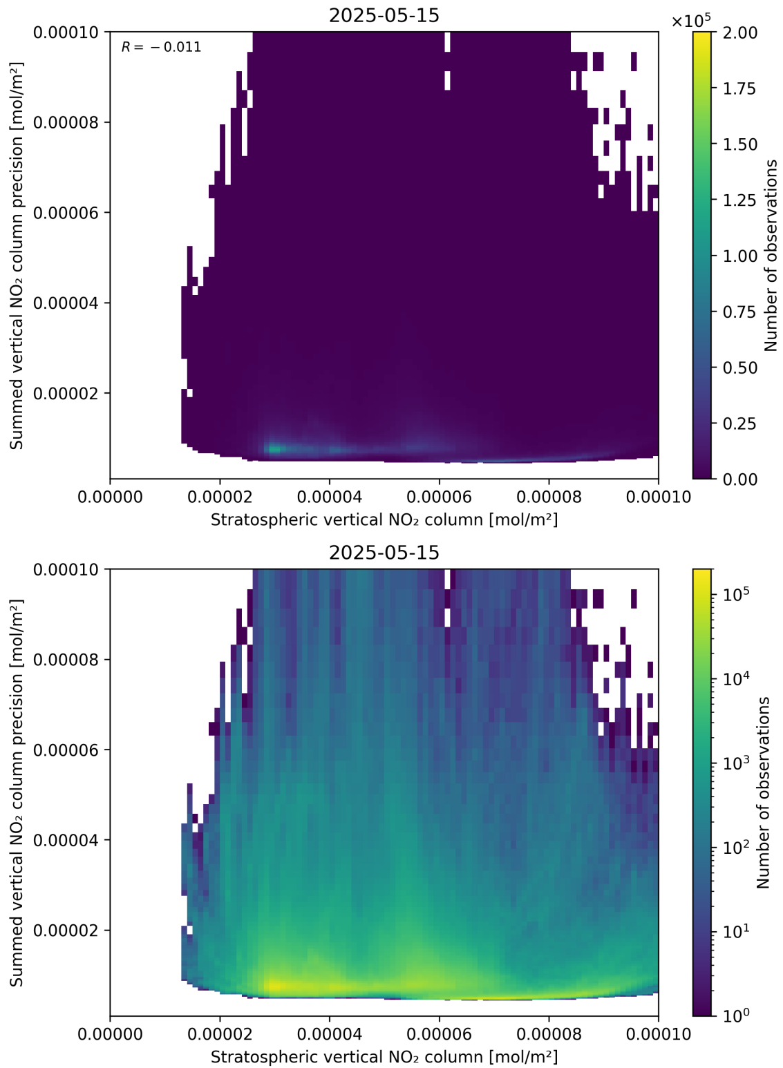
Figure 99: Scatter density plot of “Stratospheric vertical NO 2 column” against “Summed vertical NO 2 column precision” for 2025-05-15 to 2025-05-16.
