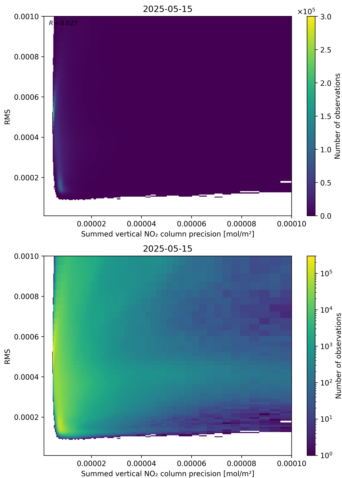
Figure 108: Scatter density plot of “Summed vertical NO 2 column precision” against “RMS” for 2025-05-15 to 2025-05-16.
