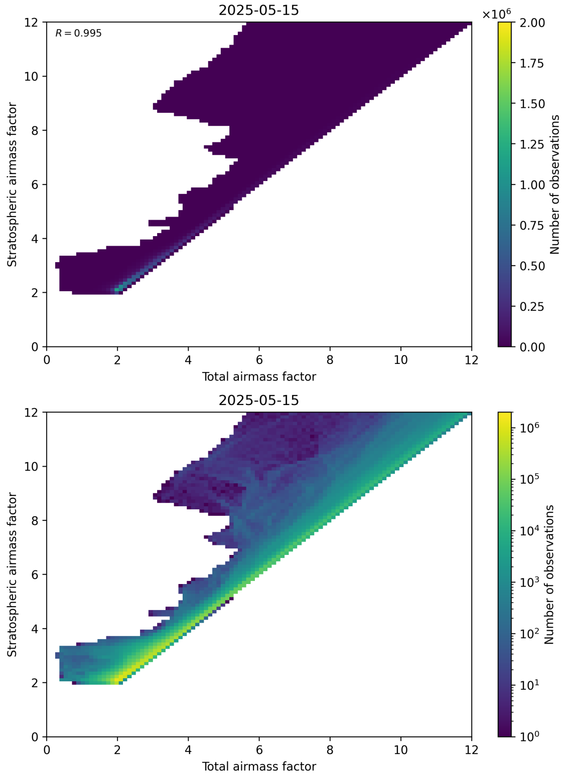
Figure 62: Scatter density plot of “Total airmass factor” against “Stratospheric airmass factor” for 2025-05-15 to 2025-05-16.
