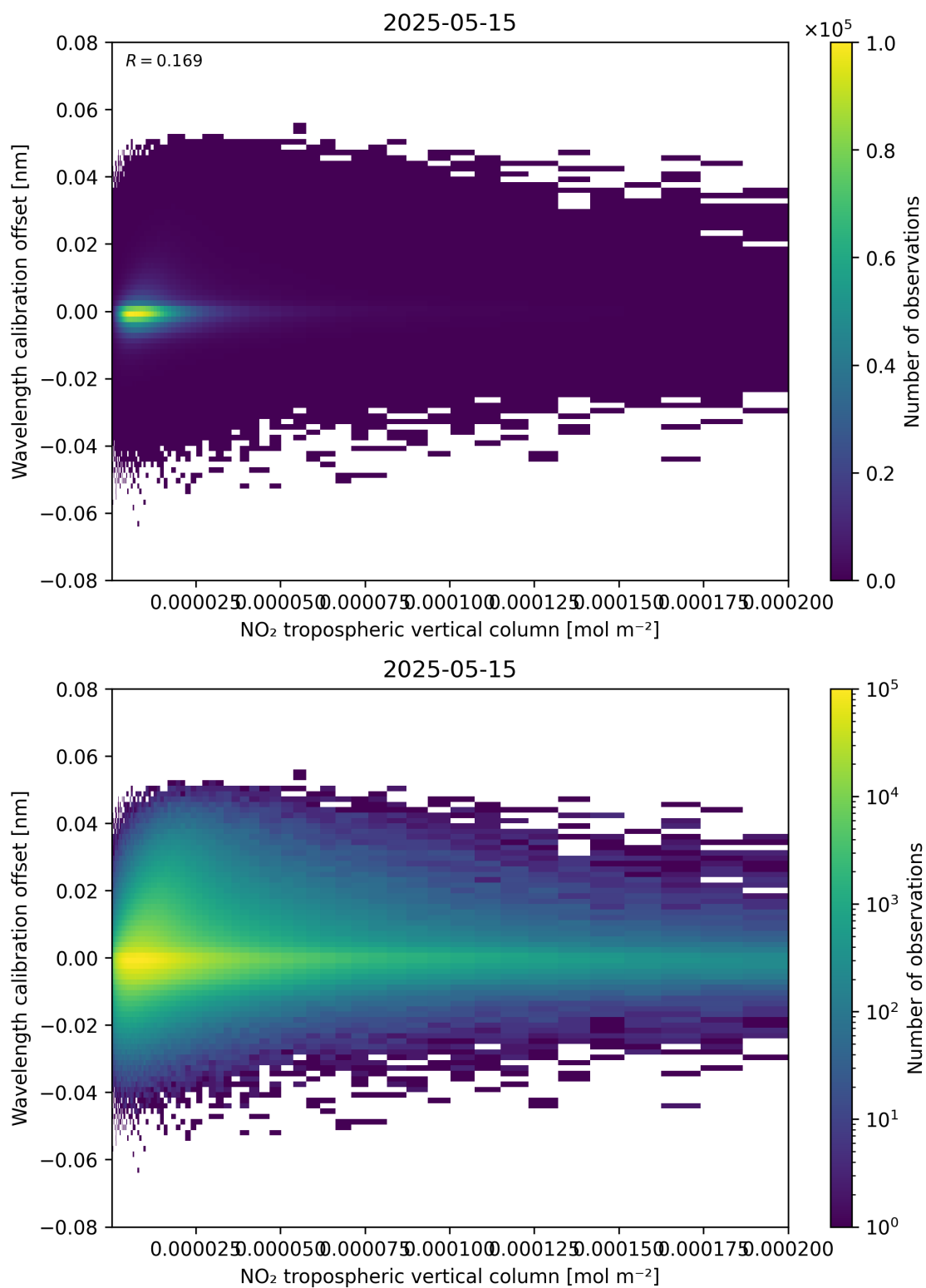
Figure 143: Scatter density plot of “NO 2 tropospheric vertical column” against “Wavelength calibration offset” for 2025-05-15 to 2025-05-16.
