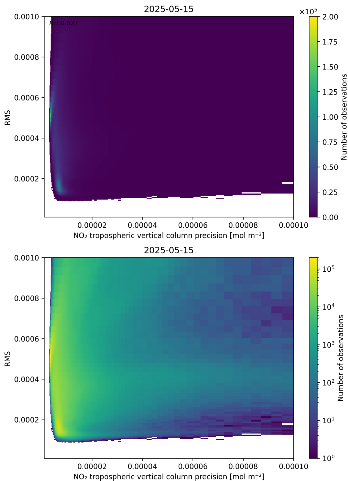
Figure 140: Scatter density plot of “NO 2 tropospheric vertical column precision” against “RMS” for 2025-05-15 to 2025-05-16.
