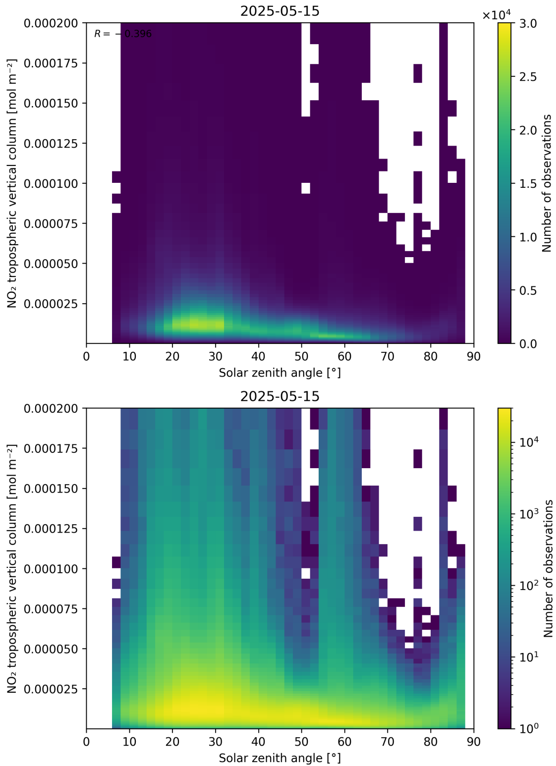
Figure 155: Scatter density plot of “Solar zenith angle” against “NO 2 tropospheric vertical column” for 2025-05-15 to 2025-05-16.
