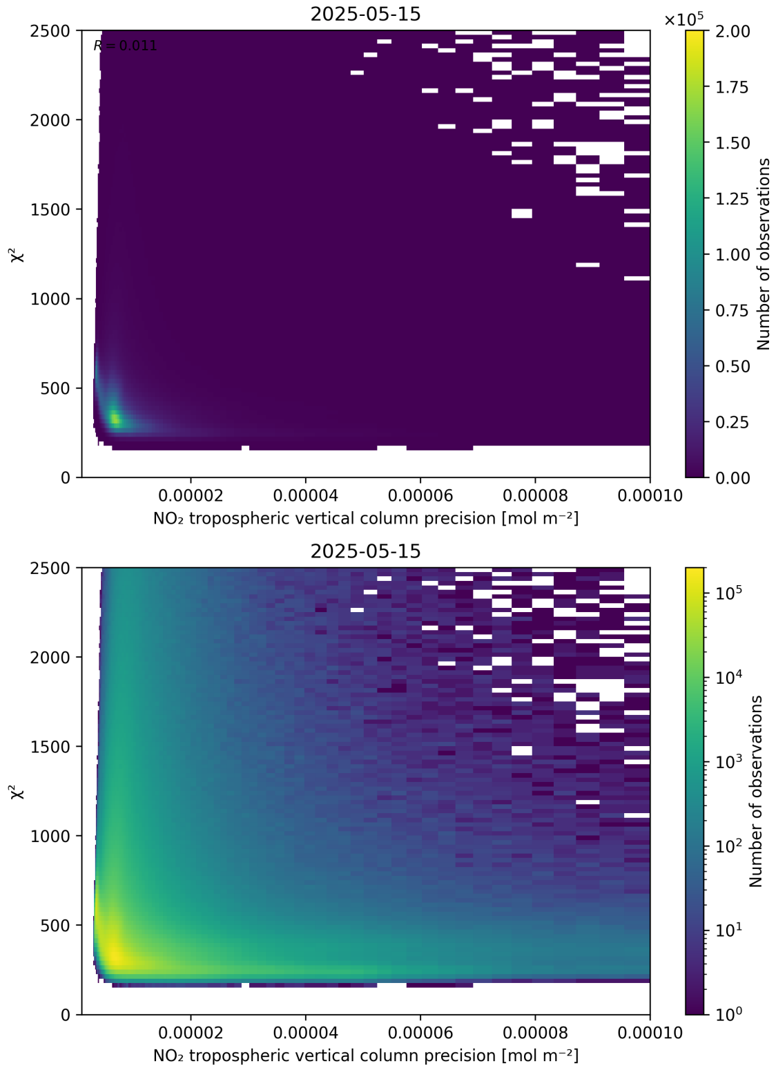
Figure 134: Scatter density plot of “NO 2 tropospheric vertical column precision” against “ \chi^2 ” for 2025-05-15 to 2025-05-16.
