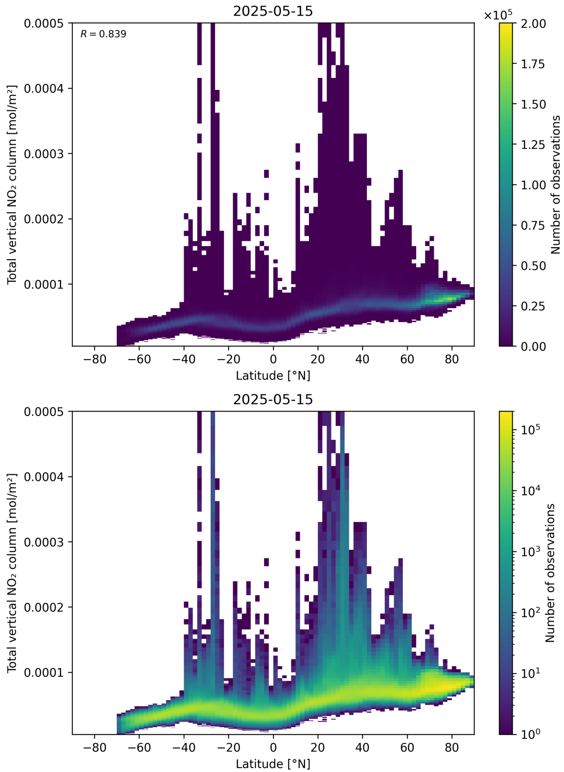
Figure 90: Scatter density plot of “Latitude” against “Total vertical NO 2 column” for 2025-05-15 to 2025-05-16.
