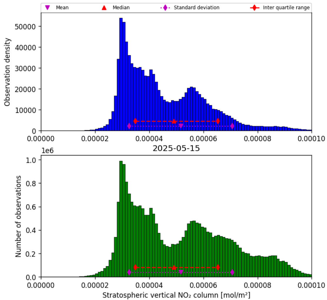
Figure 36: Histogram of “Stratospheric vertical NO 2 column” for 2025-05-15 to 2025-05-16
