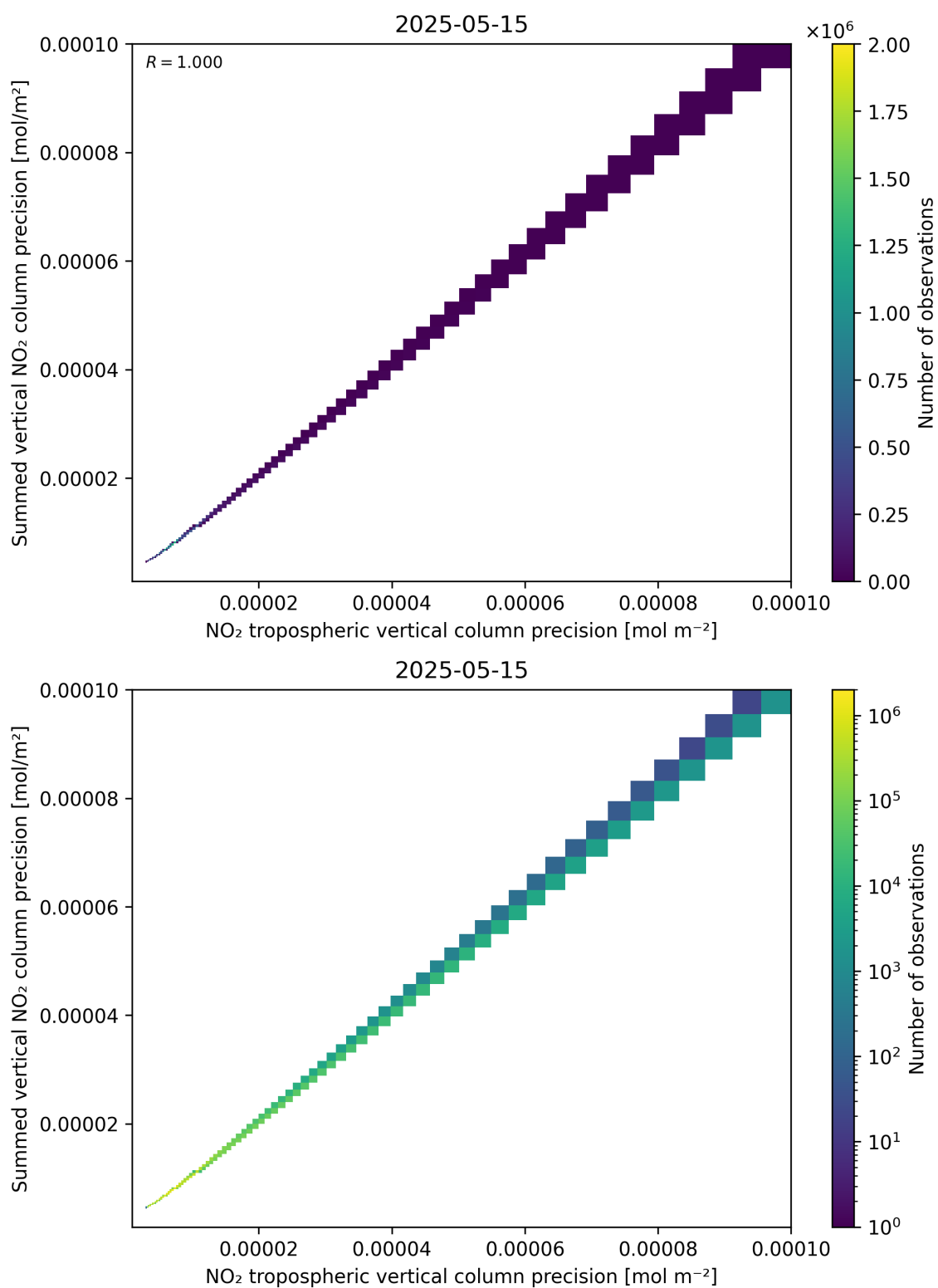
Figure 137: Scatter density plot of “NO 2 tropospheric vertical column precision” against “Summed vertical NO 2 column precision” for 2025-05-15 to 2025-05-16.
