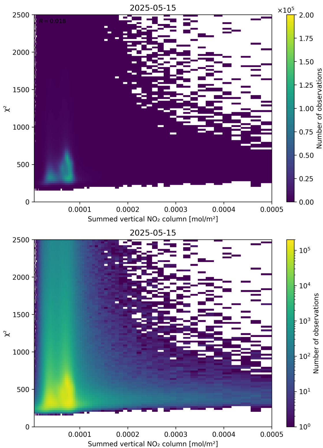
Figure 104: Scatter density plot of “Summed vertical NO 2 column” against “ \chi^2 ” for 2025-05-15 to 2025-05-16.
