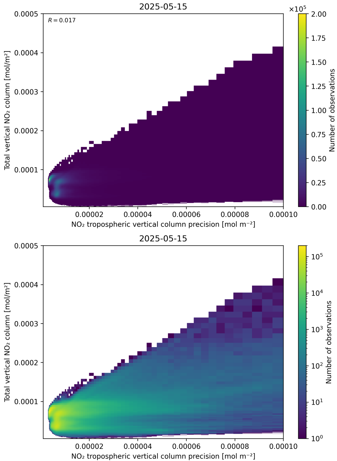
Figure 138: Scatter density plot of “NO 2 tropospheric vertical column precision” against “Total vertical NO 2 column” for 2025-05-15 to 2025-05-16.
