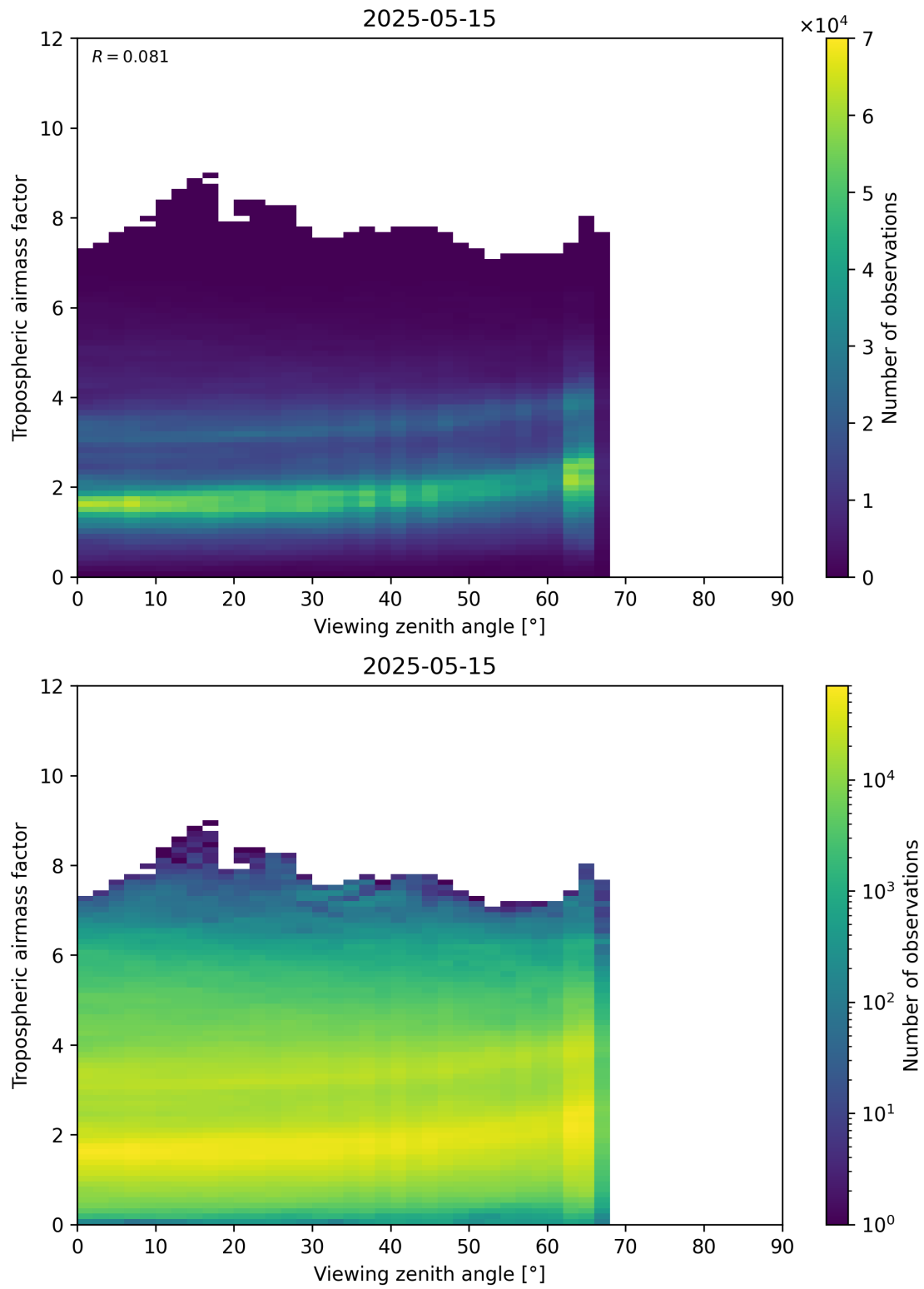
Figure 161: Scatter density plot of “Viewing zenith angle” against “Tropospheric airmass factor” for 2025-05-15 to 2025-05-16.
