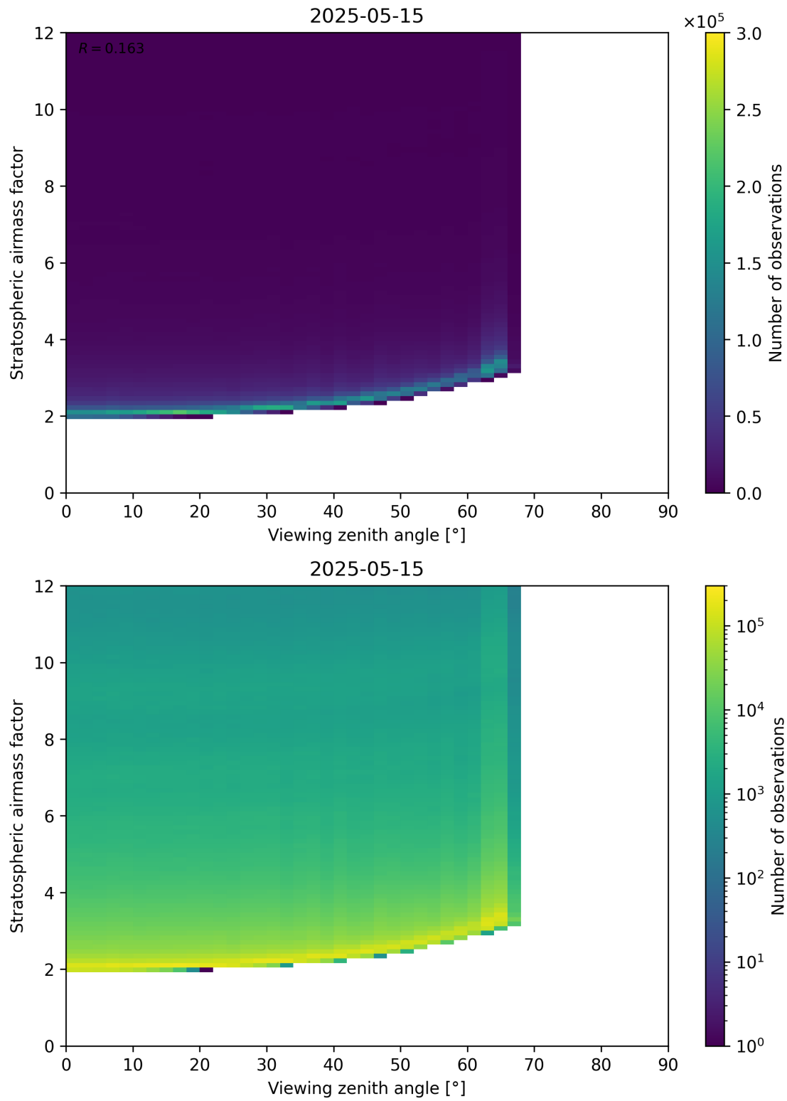
Figure 159: Scatter density plot of “Viewing zenith angle” against “Stratospheric airmass factor” for 2025-05-15 to 2025-05-16.
