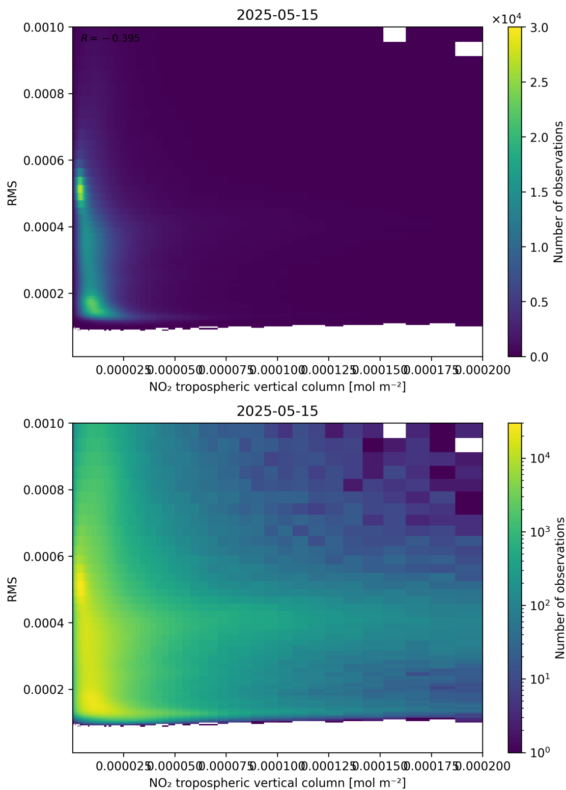
Figure 142: Scatter density plot of “NO 2 tropospheric vertical column” against “RMS” for 2025-05-15 to 2025-05-16.
