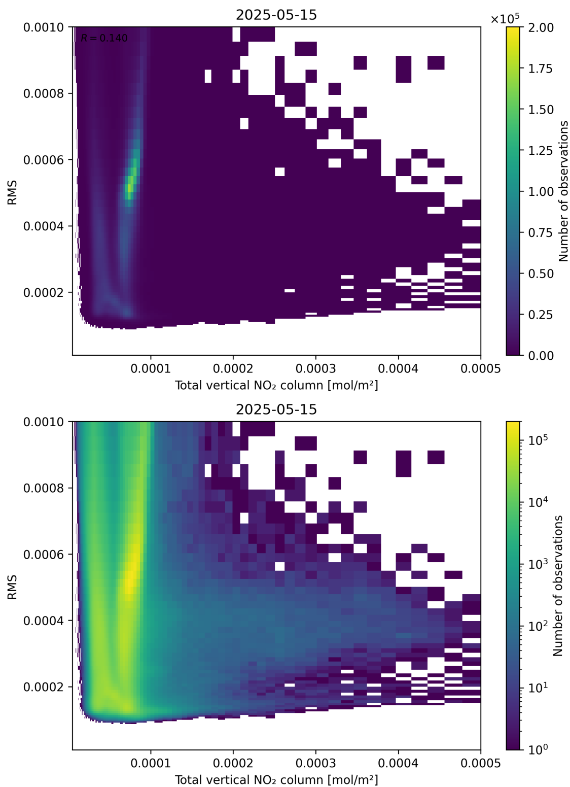
Figure 120: Scatter density plot of “Total vertical NO 2 column” against “RMS” for 2025-05-15 to 2025-05-16.
