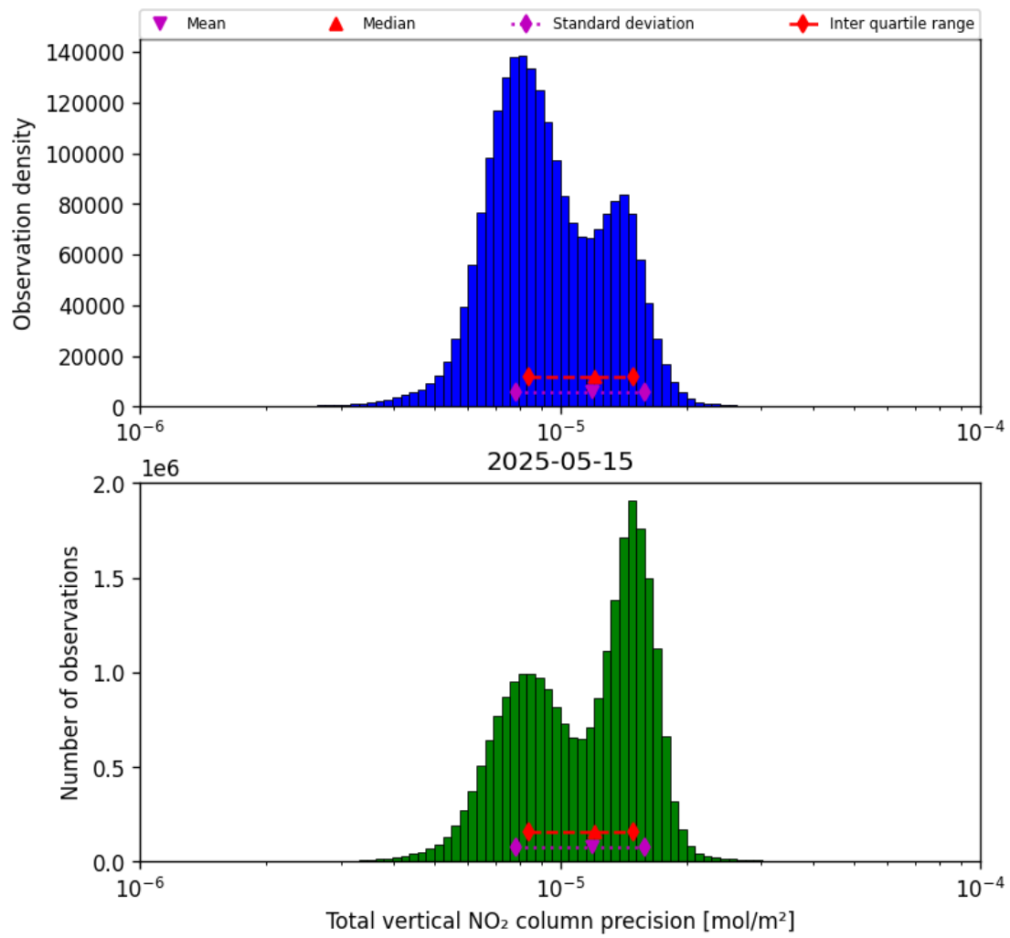
Figure 39: Histogram of “Total vertical NO 2 column precision” for 2025-05-15 to 2025-05-16
