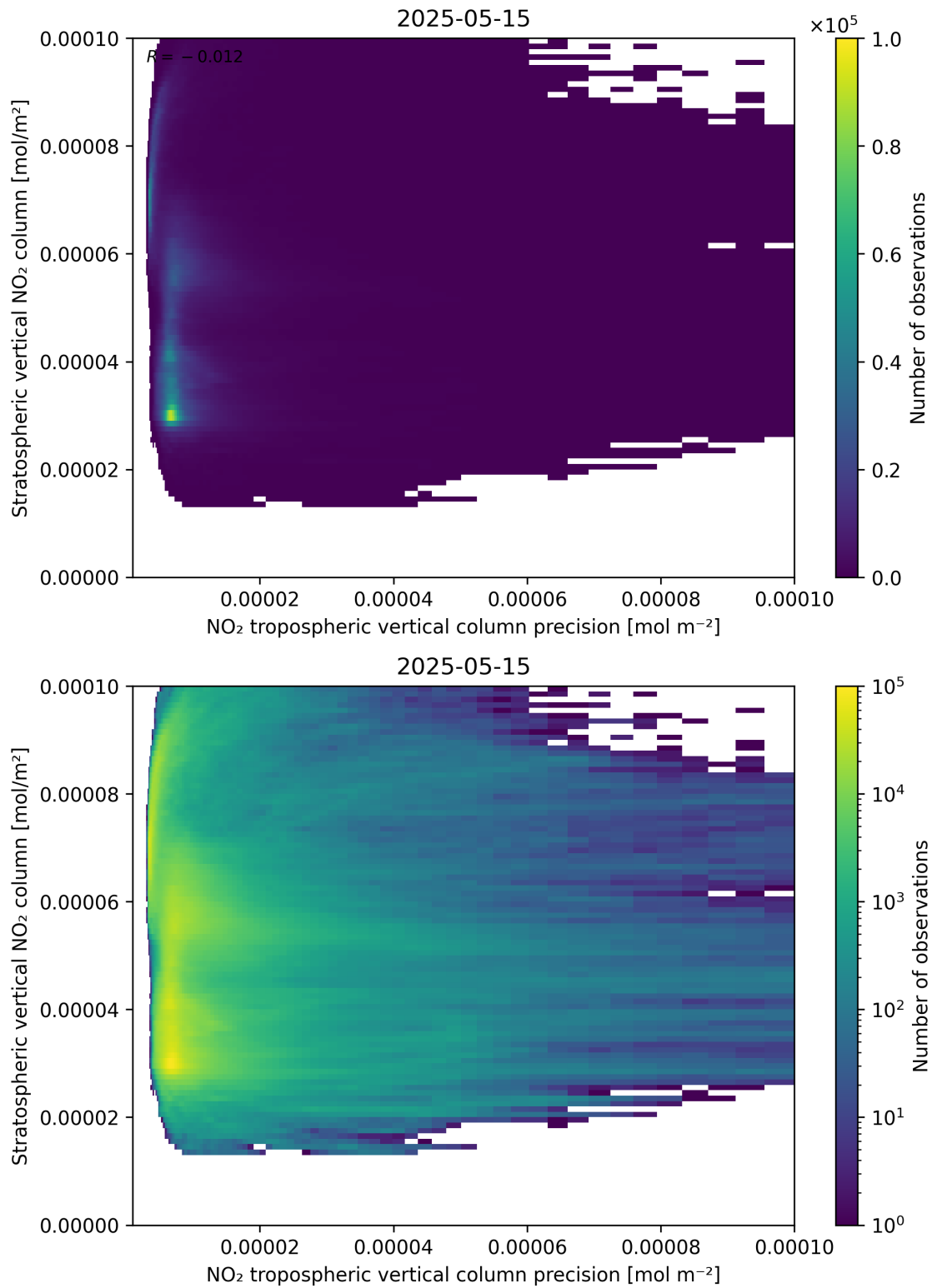
Figure 135: Scatter density plot of “ \text{NO}_2 tropospheric vertical column precision” against “Stratospheric vertical \text{NO}_2 column” for 2025-05-15 to 2025-05-16.
