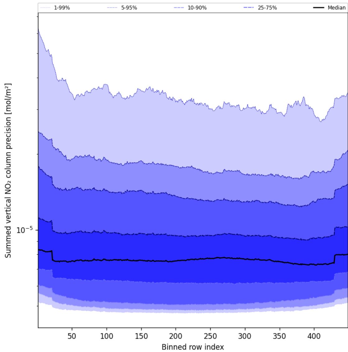
Figure 58: Along track statistics of “Summed vertical NO 2 column precision” for 2025-05-15 to 2025-05-16
