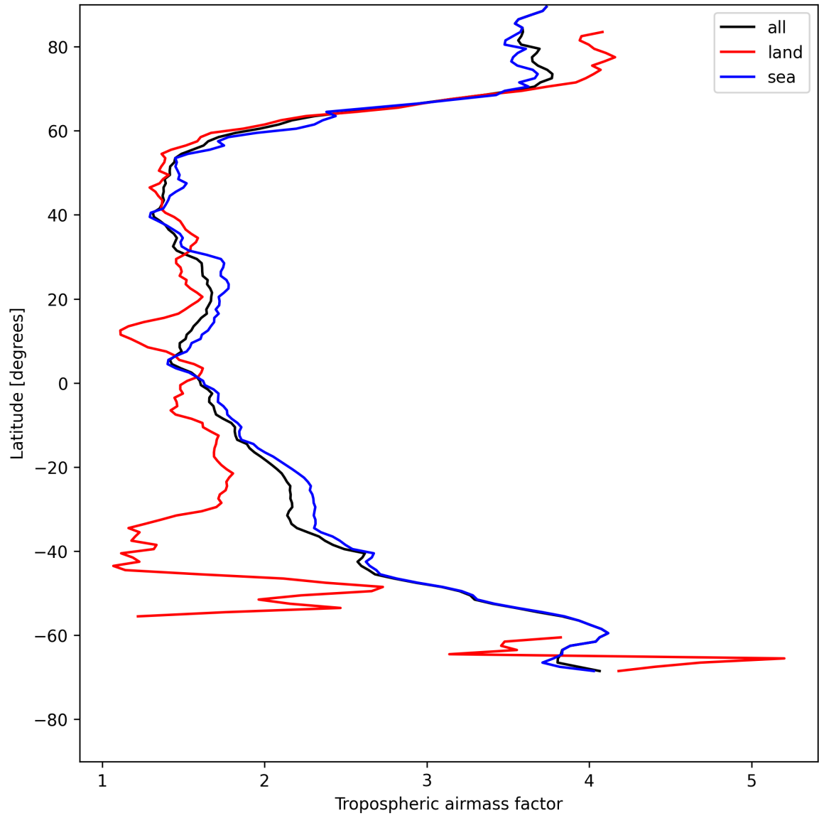
Figure 14: Zonal average of “Tropospheric airmass factor” for 2025-05-15 to 2025-05-16.
