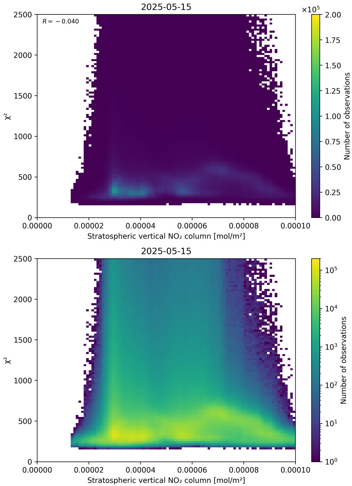
Figure 97: Scatter density plot of “Stratospheric vertical NO 2 column” against “ \chi^2 ” for 2025-05-15 to 2025-05-16.
