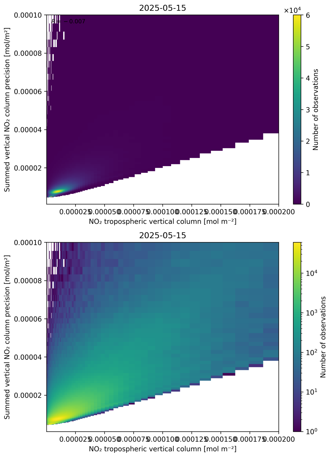
Figure 127: Scatter density plot of “NO 2 tropospheric vertical column” against “Summed vertical NO 2 column precision” for 2025-05-15 to 2025-05-16.
