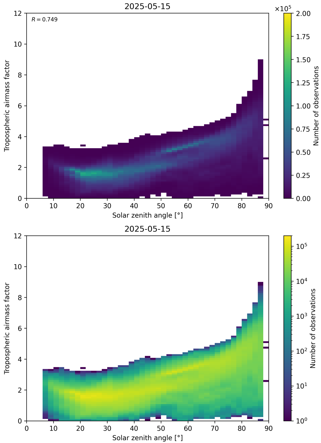
Figure 147: Scatter density plot of “Solar zenith angle” against “Tropospheric airmass factor” for 2025-05-15 to 2025-05-16.
