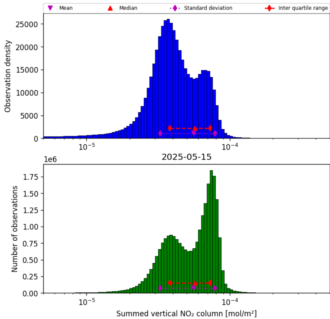
Figure 40: Histogram of “Summed vertical NO 2 column” for 2025-05-15 to 2025-05-16
