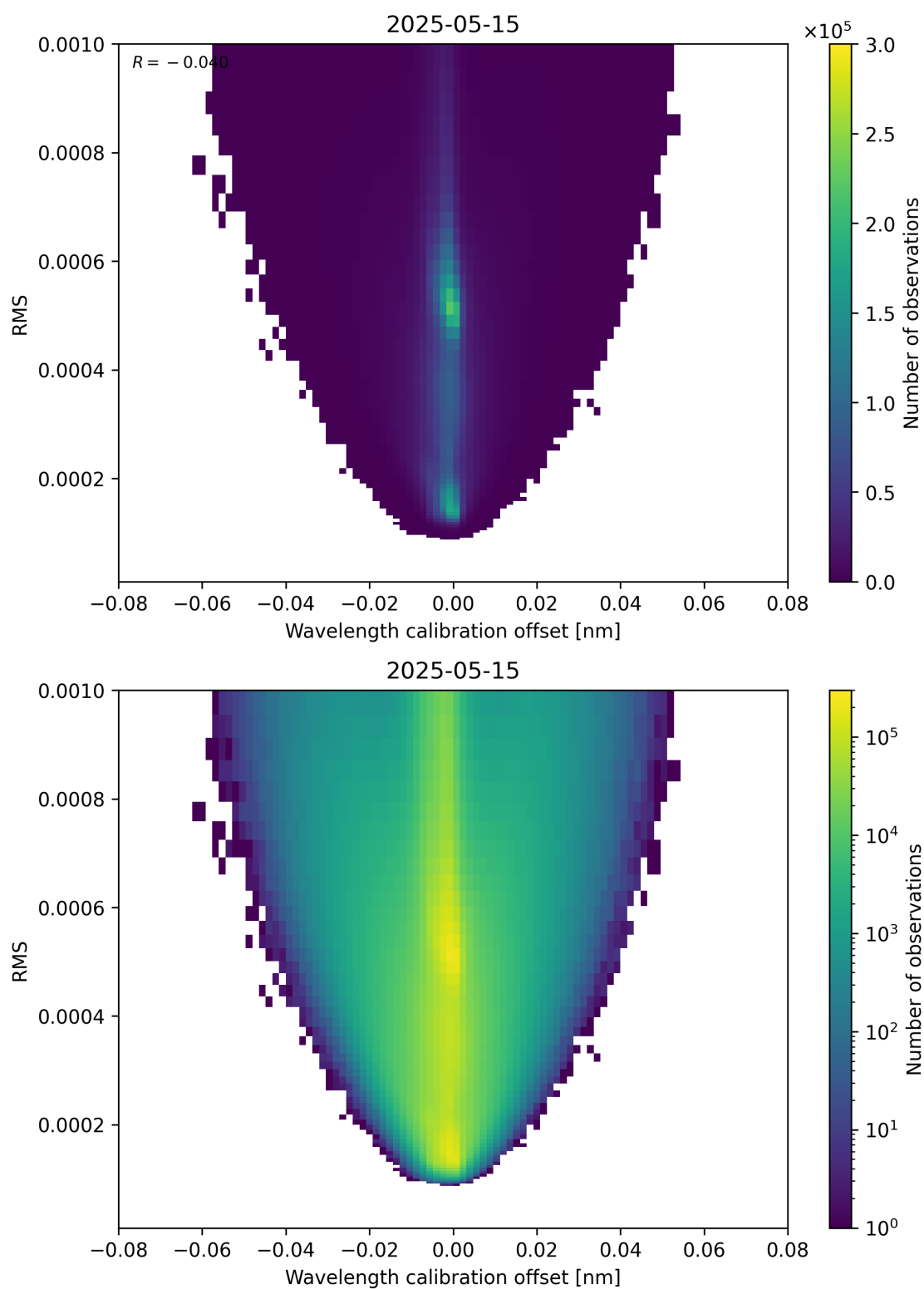
Figure 181: Scatter density plot of “Wavelength calibration offset” against “RMS” for 2025-05-15 to 2025-05-16.
