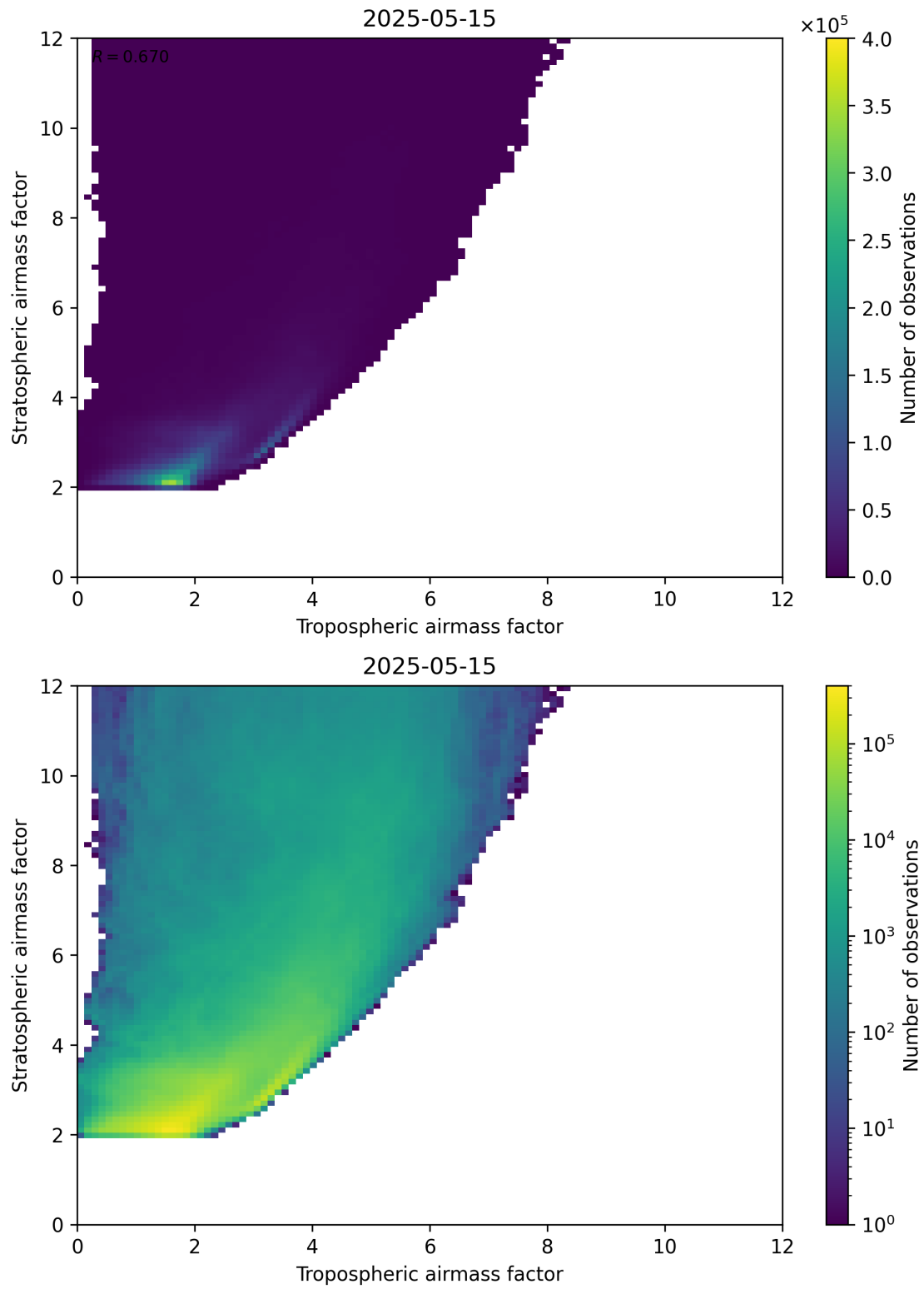
Figure 71: Scatter density plot of “Tropospheric airmass factor” against “Stratospheric airmass factor” for 2025-05-15 to 2025-05-16.
