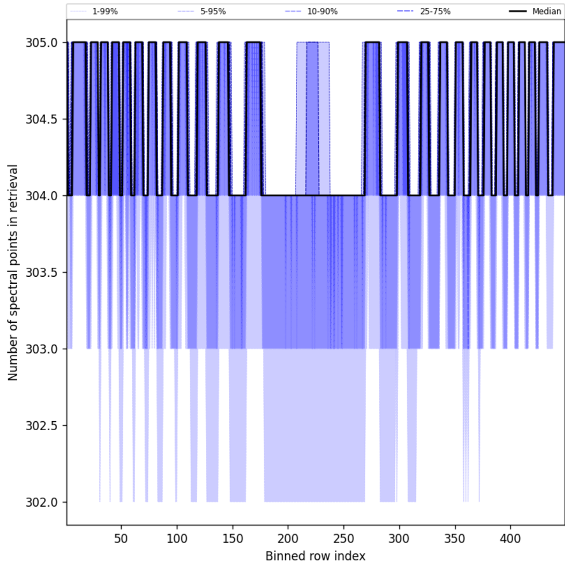
Figure 50: Along track statistics of “Number of spectral points in retrieval” for 2025-05-15 to 2025-05-16
