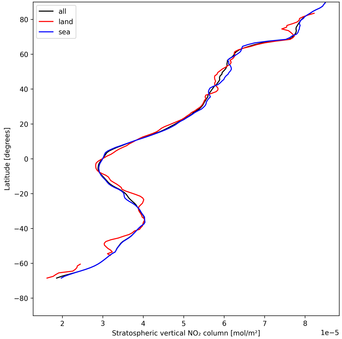
Figure 19: Zonal average of “Stratospheric vertical NO 2 column” for 2025-05-15 to 2025-05-16.
