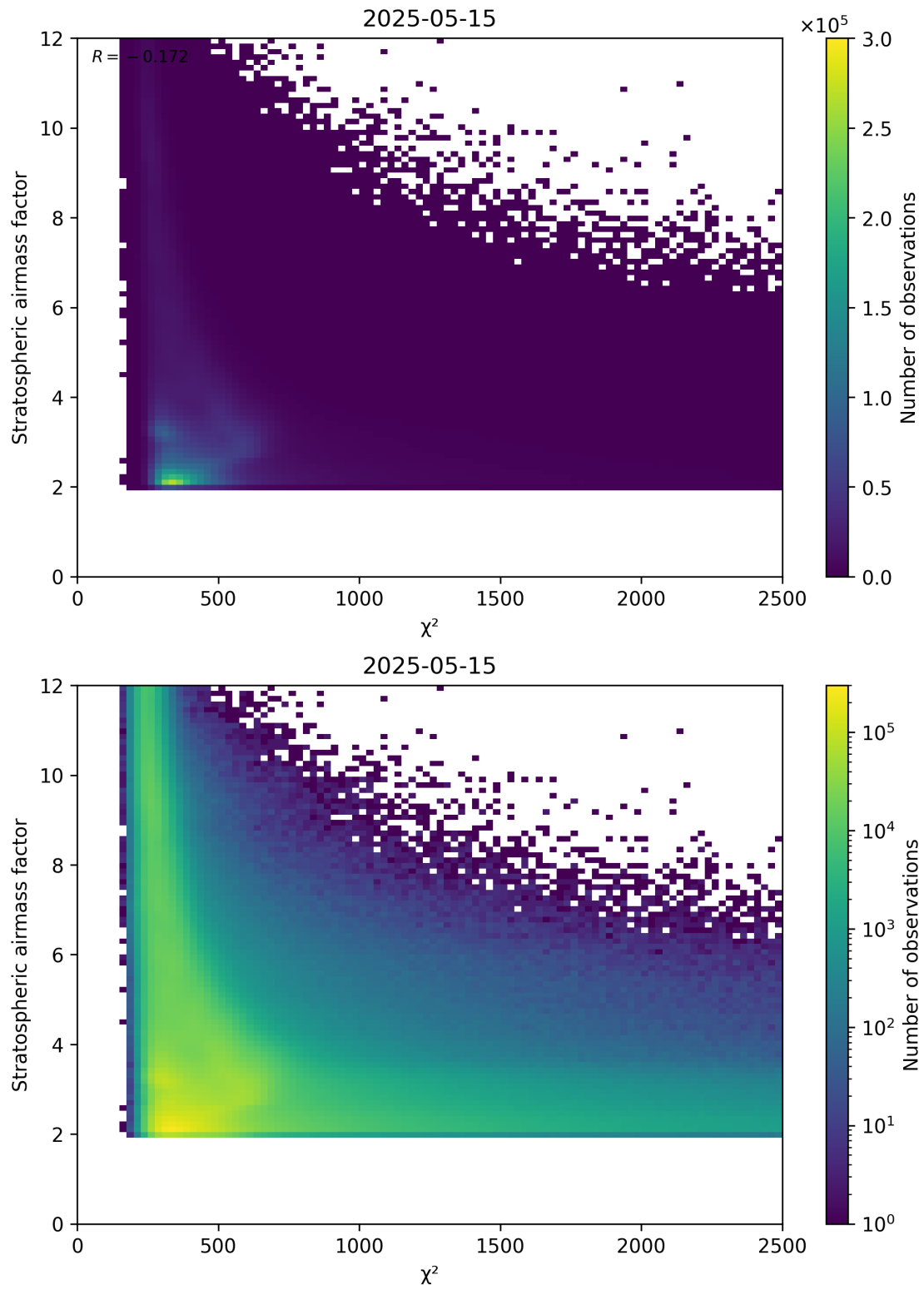
Figure 81: Scatter density plot of “ \chi^2 ” against “Stratospheric airmass factor” for 2025-05-15 to 2025-05-16.
