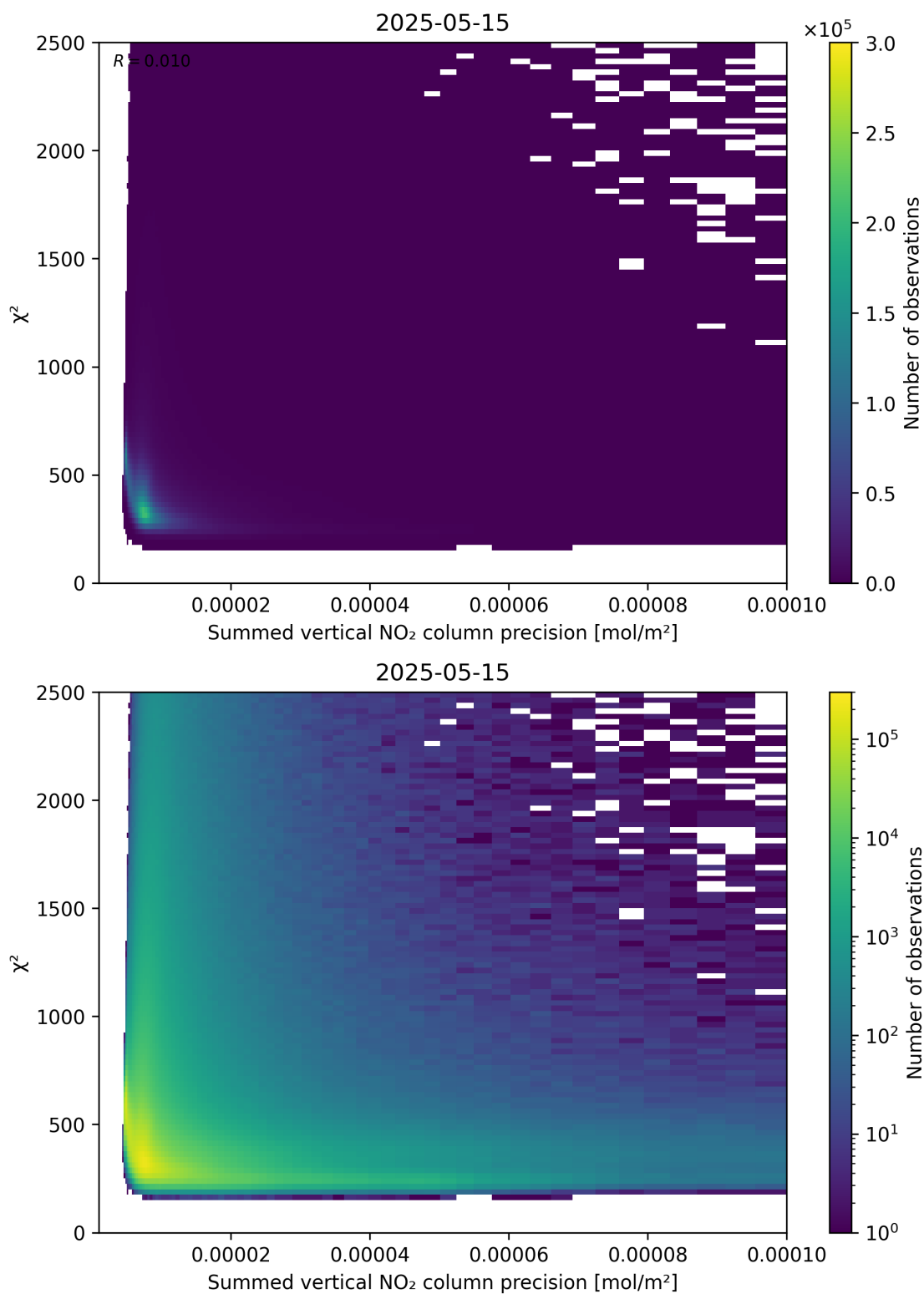
Figure 107: Scatter density plot of “Summed vertical NO 2 column precision” against “ \chi^2 ” for 2025-05-15 to 2025-05-16.
