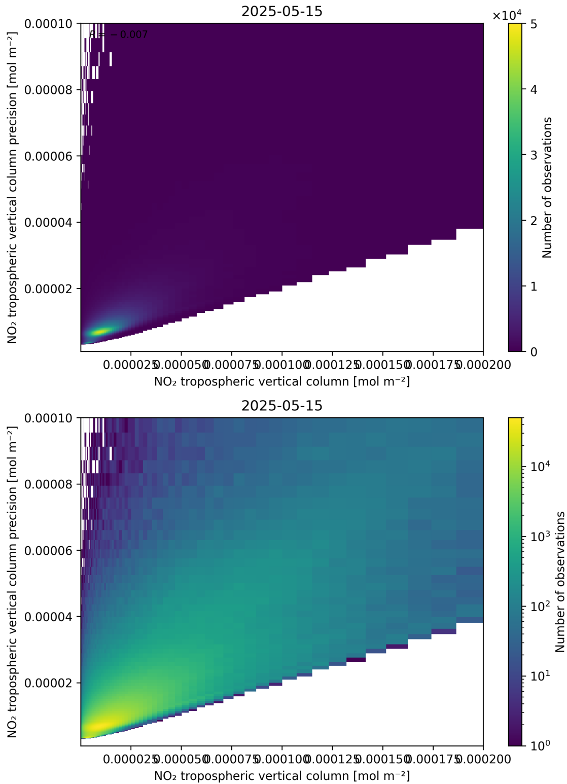
Figure 130: Scatter density plot of “NO 2 tropospheric vertical column” against “NO 2 tropospheric vertical column precision” for 2025-05-15 to 2025-05-16.
