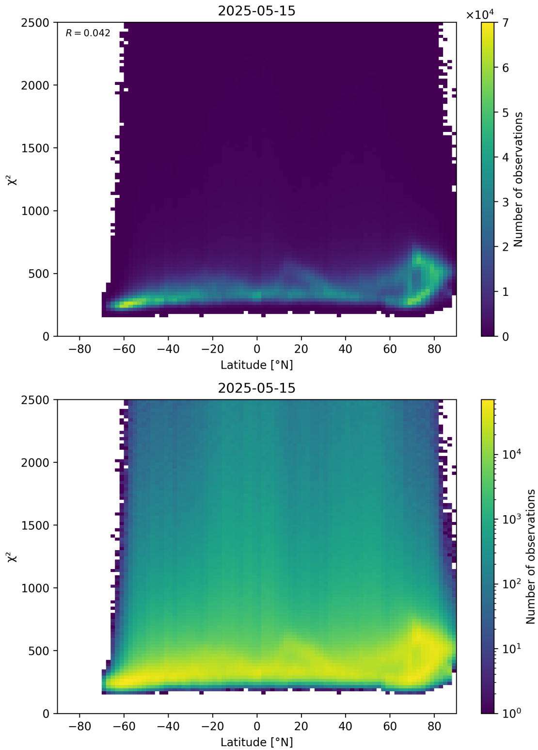
Figure 86: Scatter density plot of “Latitude” against “ \chi^2 ” for 2025-05-15 to 2025-05-16.
