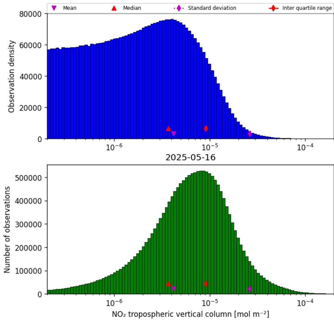
Figure 29: Histogram of “NO 2 tropospheric vertical column” for 2025-05-15 to 2025-05-17
