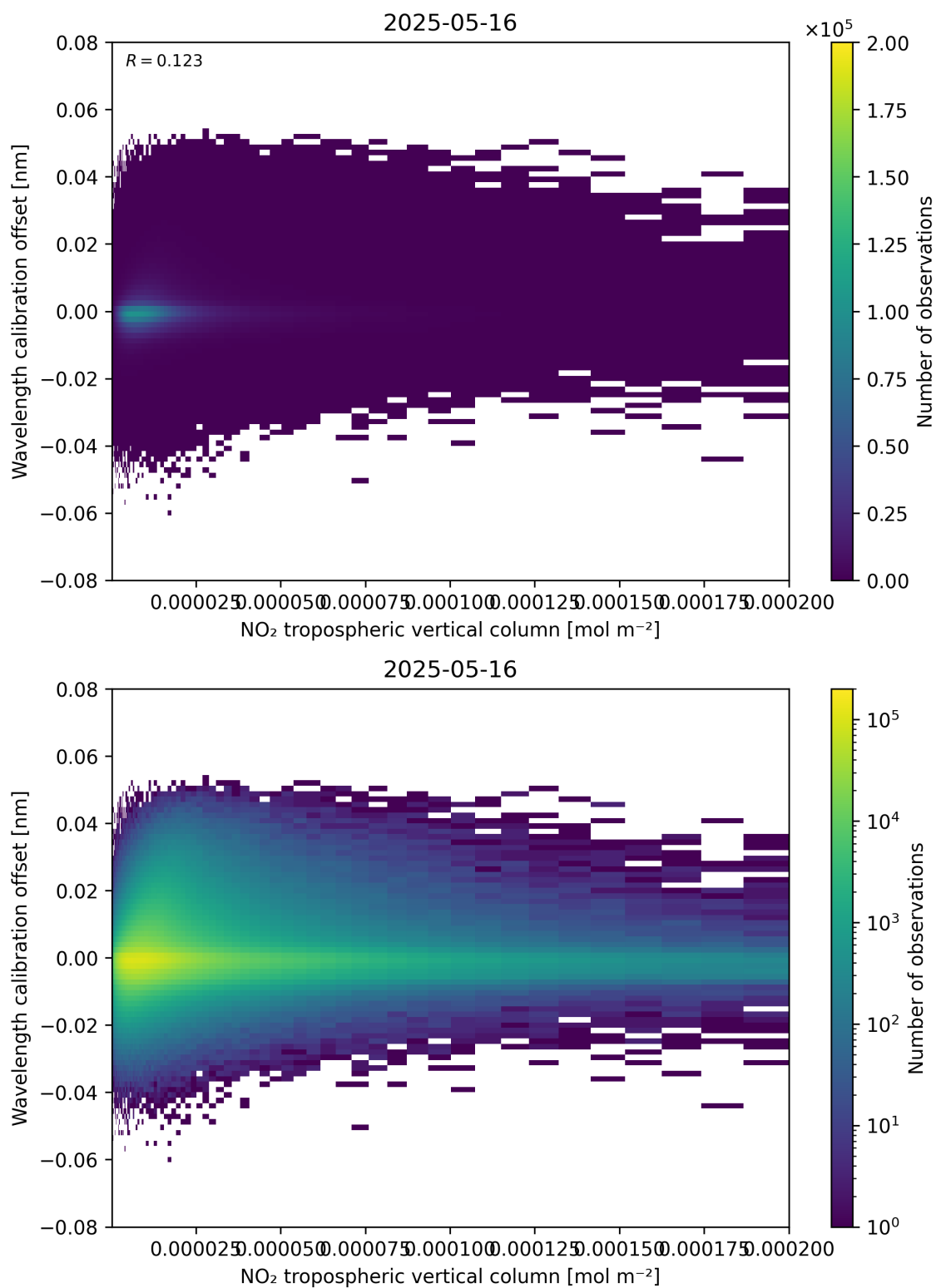
Figure 143: Scatter density plot of “NO 2 tropospheric vertical column” against “Wavelength calibration offset” for 2025-05-15 to 2025-05-17.
