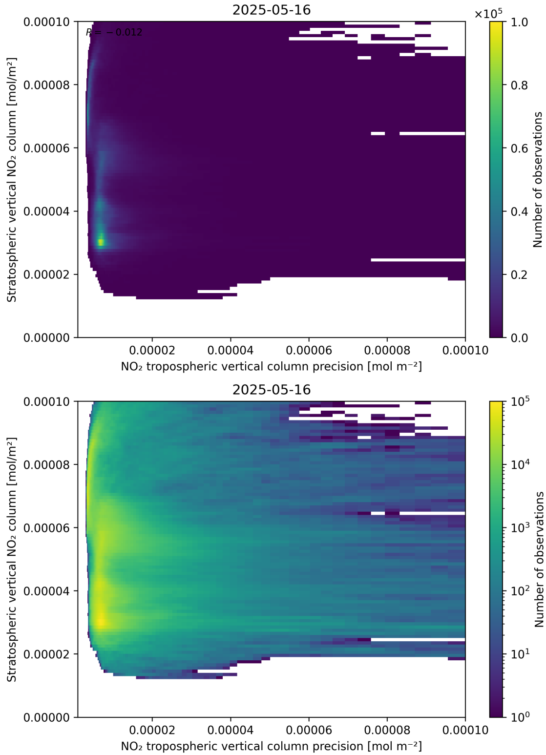
Figure 135: Scatter density plot of “NO 2 tropospheric vertical column precision” against “Stratospheric vertical NO 2 column” for 2025-05-15 to 2025-05-17.
