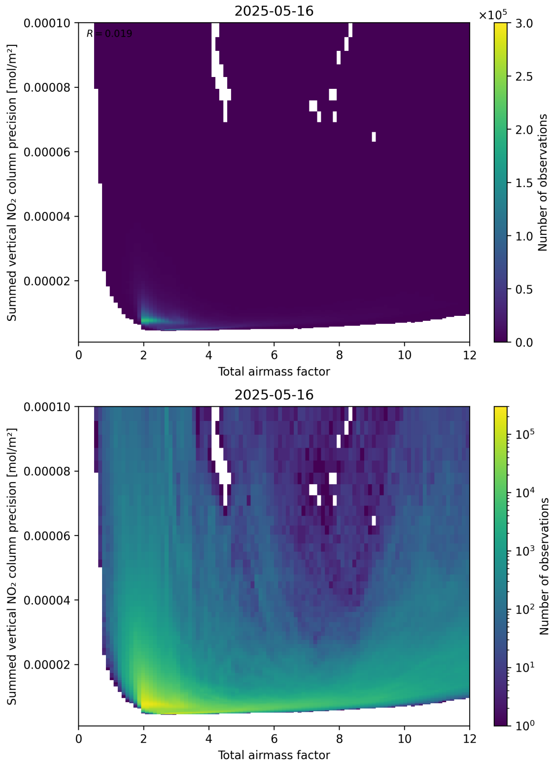
Figure 66: Scatter density plot of “Total airmass factor” against “Summed vertical NO 2 column precision” for 2025-05-15 to 2025-05-17.
