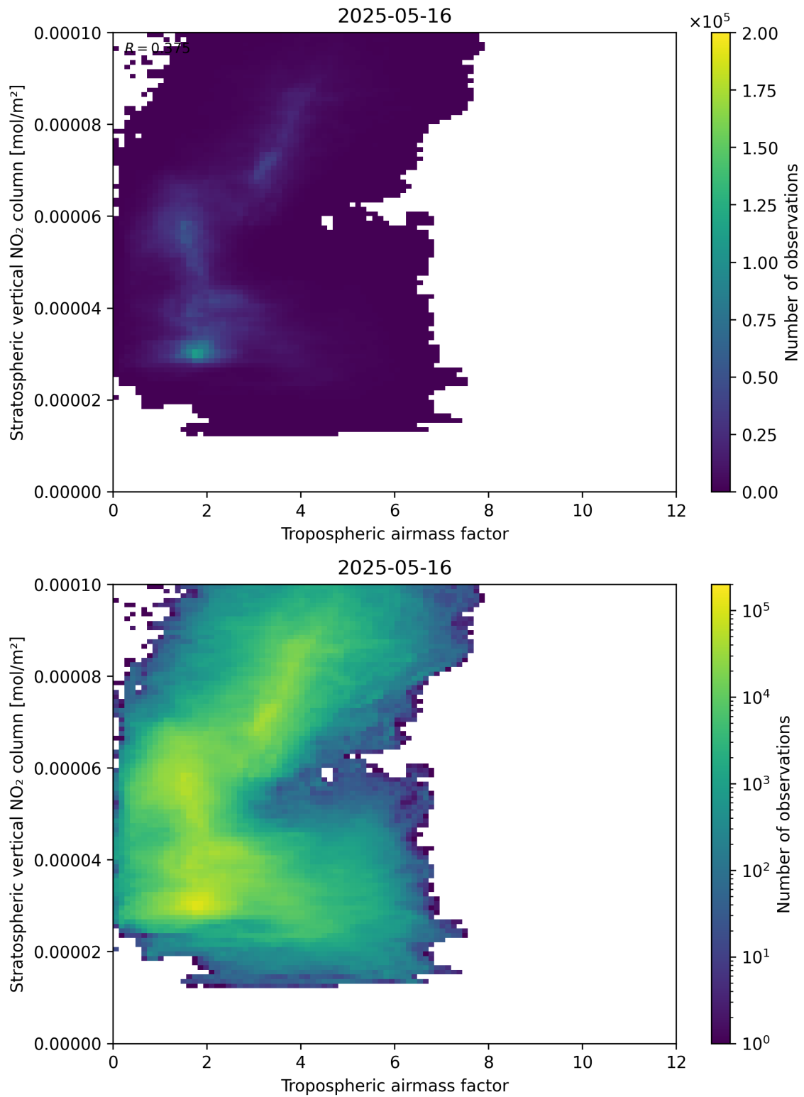
Figure 74: Scatter density plot of “Tropospheric air mass factor” against “Stratospheric vertical NO 2 column” for 2025-05-15 to 2025-05-17.
