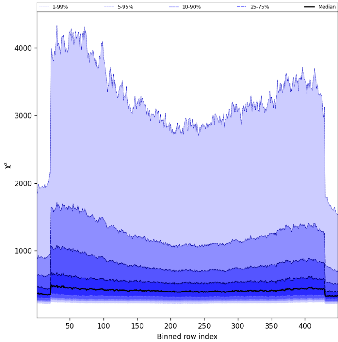
Figure 59: Along track statistics of “ \chi^2 ” for 2025-05-15 to 2025-05-17
