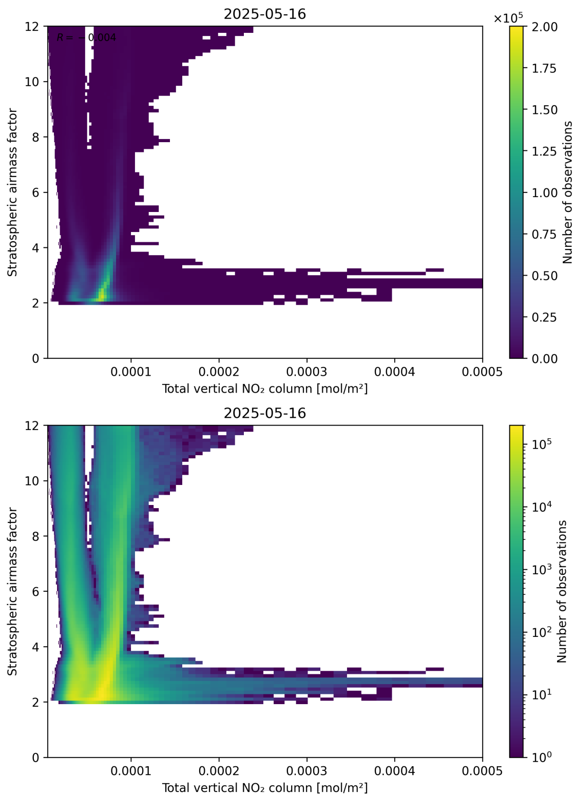
Figure 110: Scatter density plot of “Total vertical NO 2 column” against “Stratospheric airmass factor” for 2025-05-15 to 2025-05-17.
