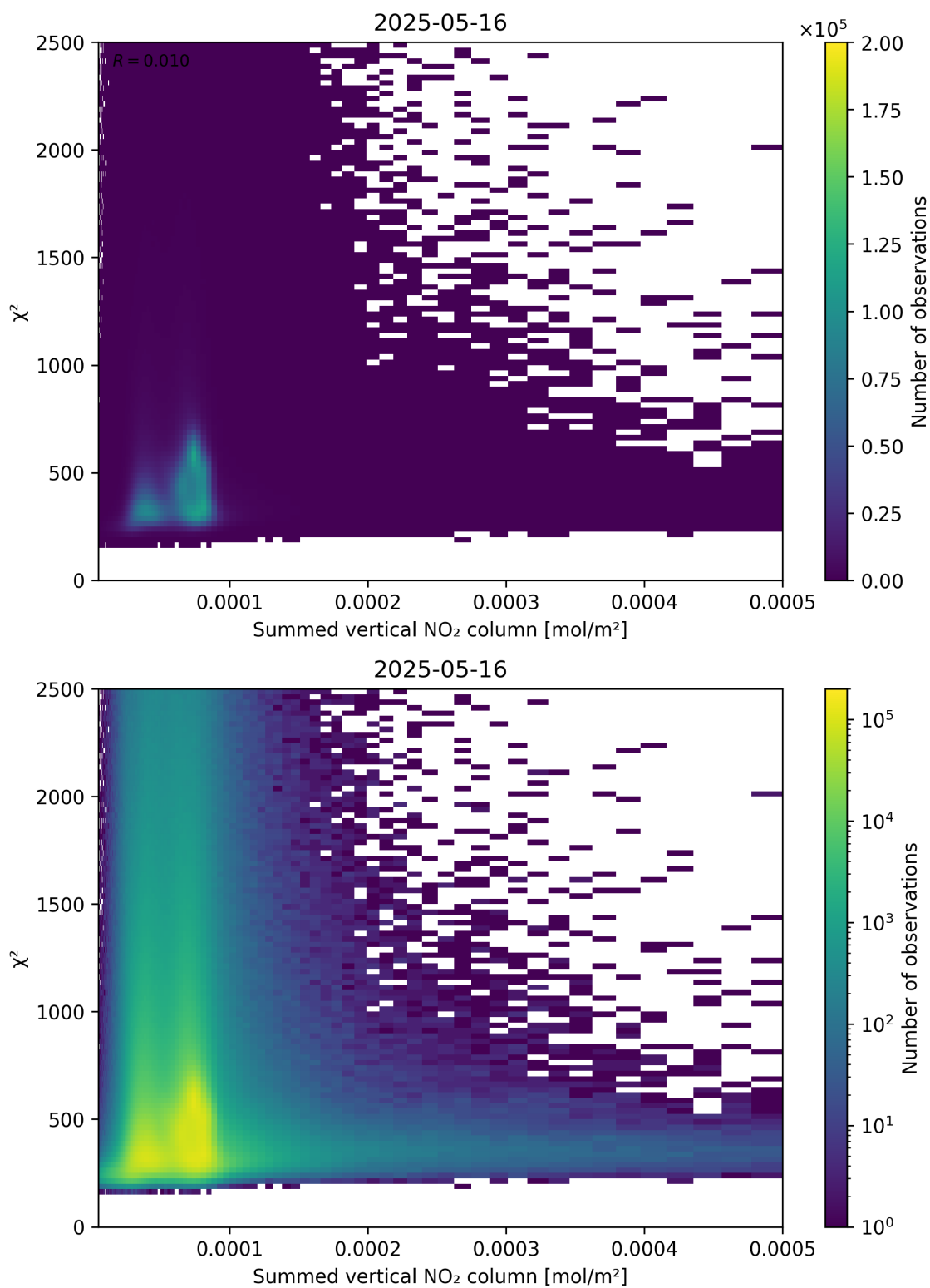
Figure 104: Scatter density plot of “Summed vertical NO 2 column” against “ \chi^2 ” for 2025-05-15 to 2025-05-17.
