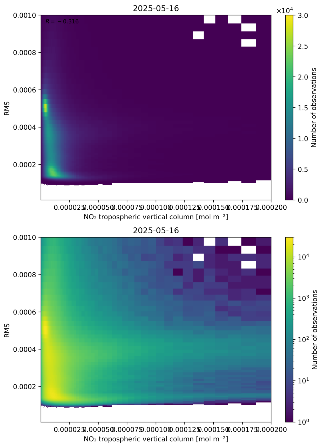
Figure 142: Scatter density plot of “NO 2 tropospheric vertical column” against “RMS” for 2025-05-15 to 2025-05-17.
