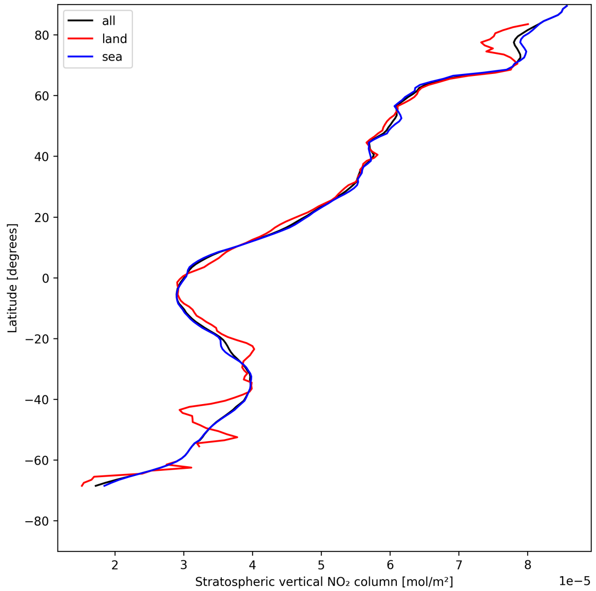
Figure 19: Zonal average of “Stratospheric vertical NO 2 column” for 2025-05-15 to 2025-05-17.
