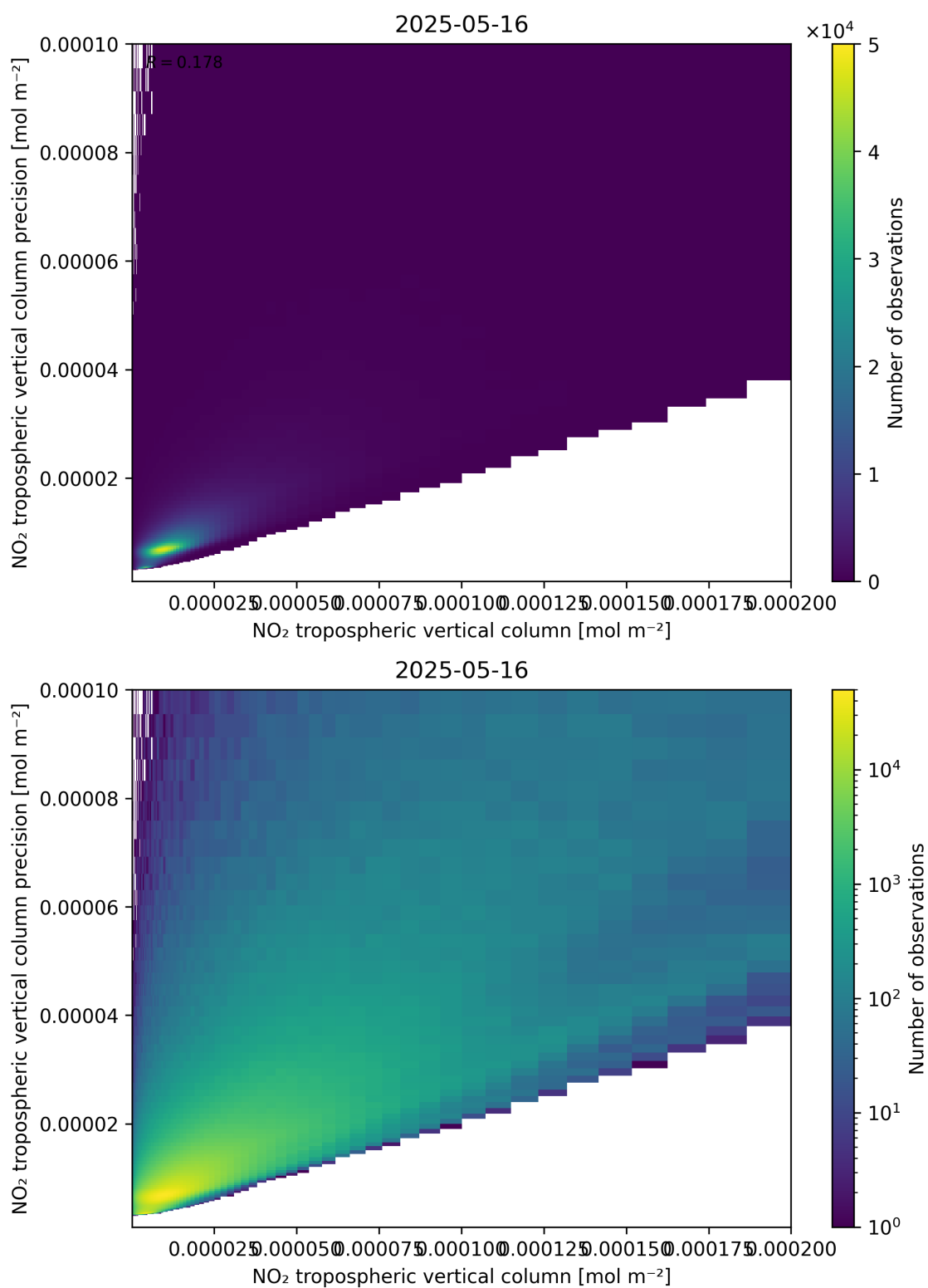
Figure 130: Scatter density plot of “NO 2 tropospheric vertical column” against “NO 2 tropospheric vertical column precision” for 2025-05-15 to 2025-05-17.
