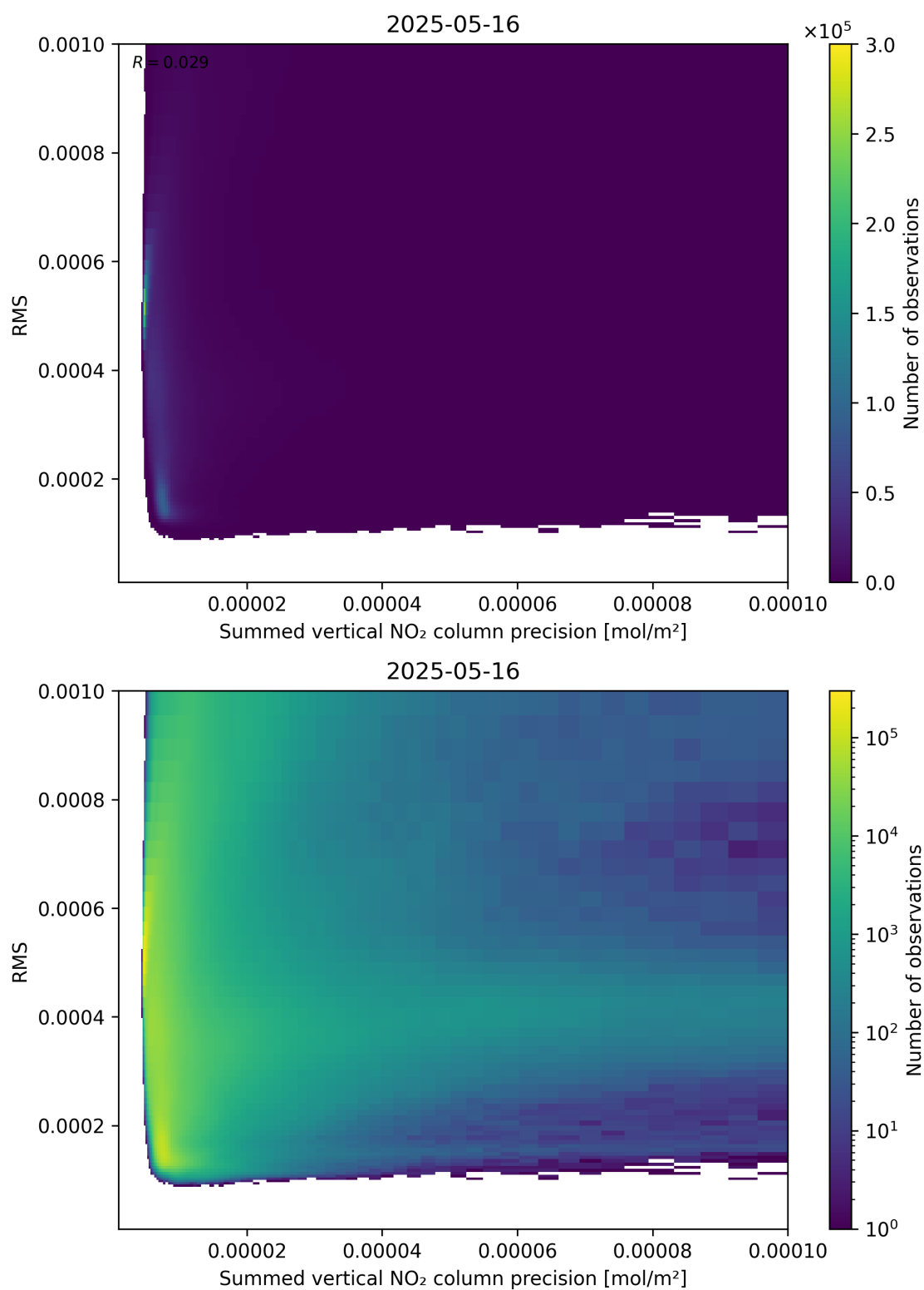
Figure 108: Scatter density plot of “Summed vertical NO 2 column precision” against “RMS” for 2025-05-15 to 2025-05-17.
