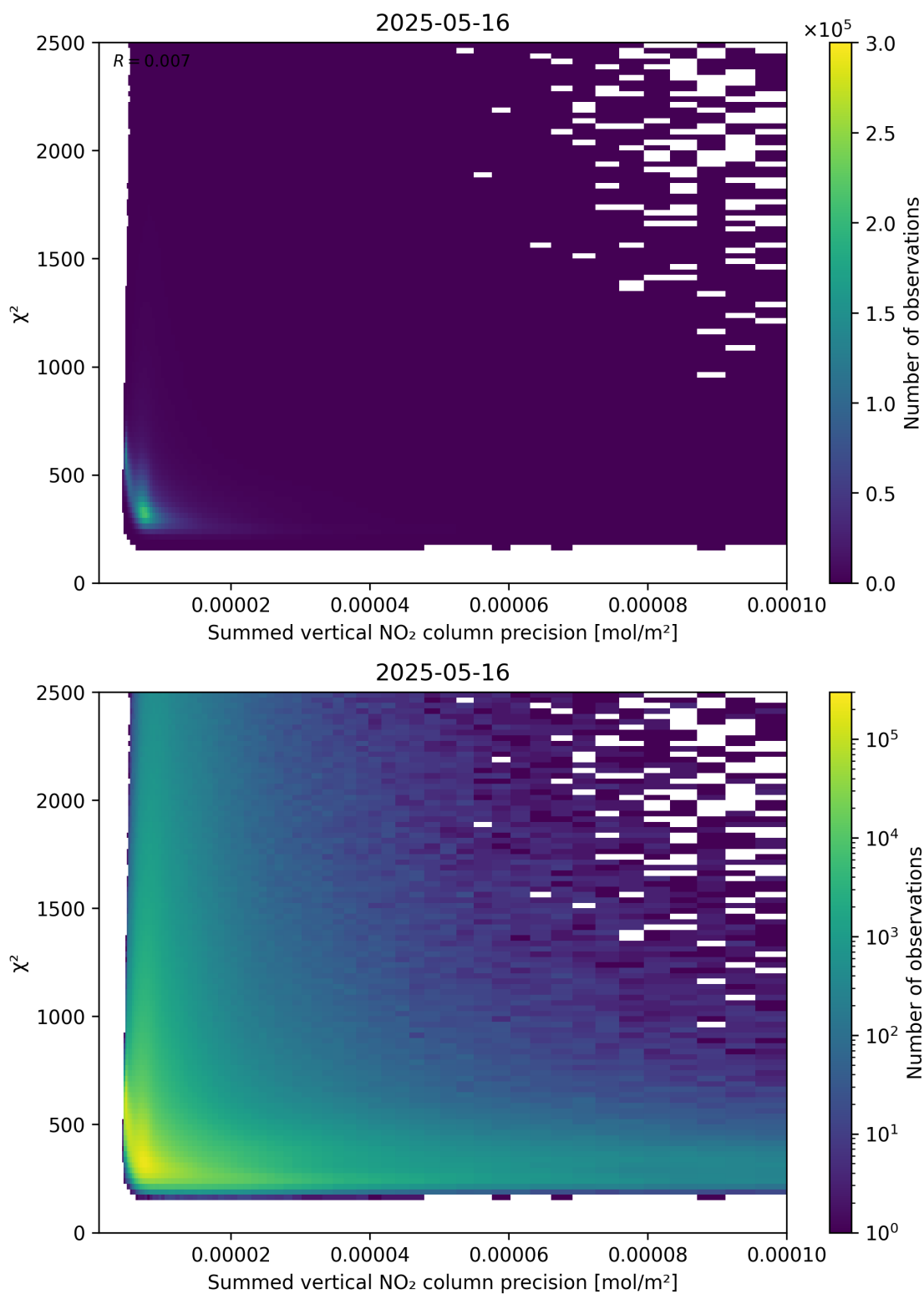
Figure 107: Scatter density plot of “Summed vertical NO 2 column precision” against “ \chi^2 ” for 2025-05-15 to 2025-05-17.
