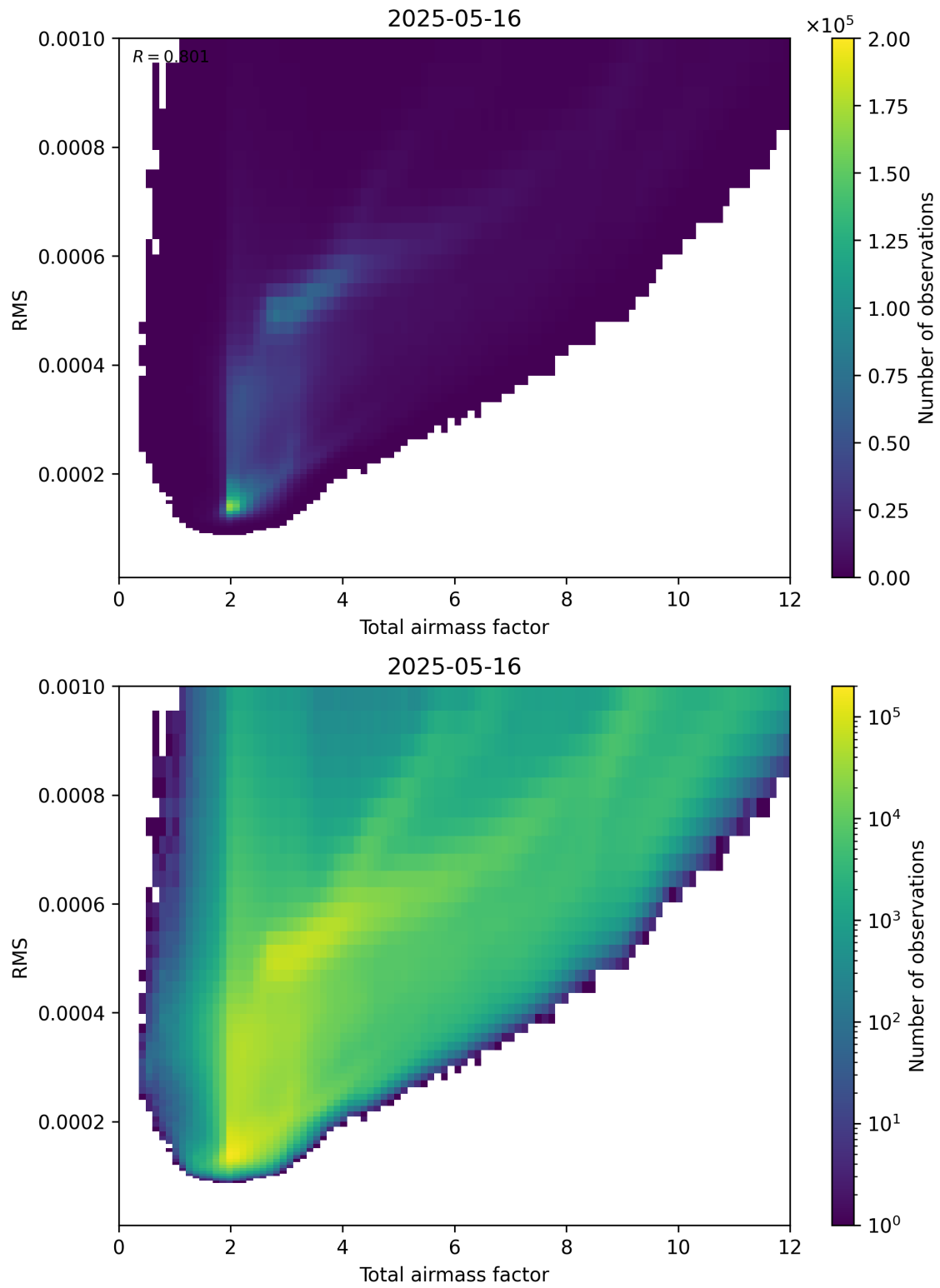
Figure 69: Scatter density plot of “Total airmass factor” against “RMS” for 2025-05-15 to 2025-05-17.
