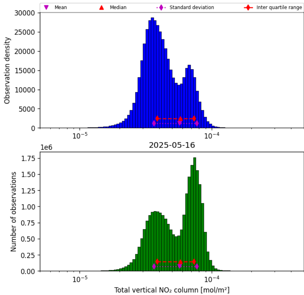
Figure 38: Histogram of “Total vertical NO 2 column” for 2025-05-15 to 2025-05-17
