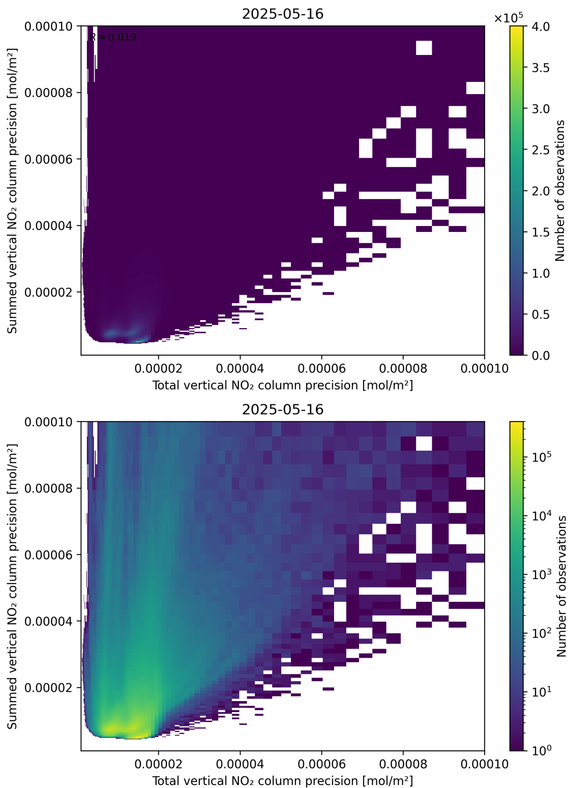
Figure 118: Scatter density plot of “Total vertical NO 2 column precision” against “Summed vertical NO 2 column precision” for 2025-05-15 to 2025-05-17.
