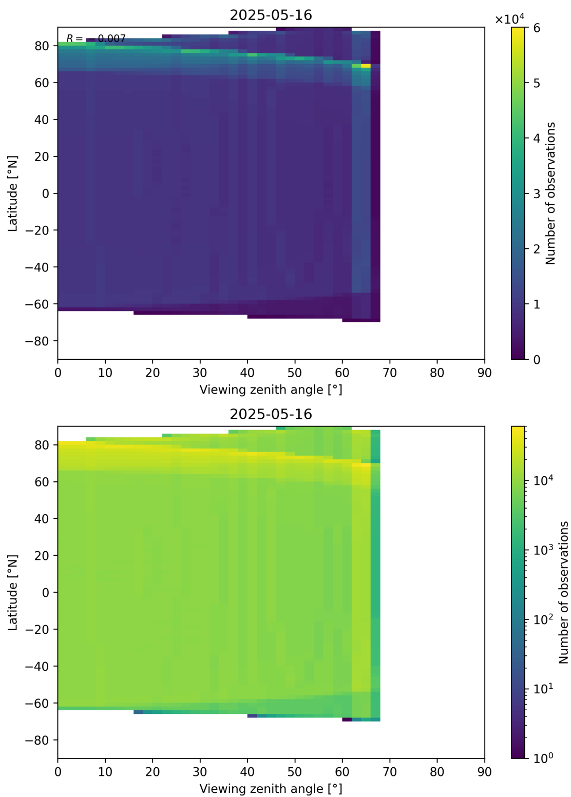
Figure 163: Scatter density plot of “Viewing zenith angle” against “Latitude” for 2025-05-15 to 2025-05-17.
