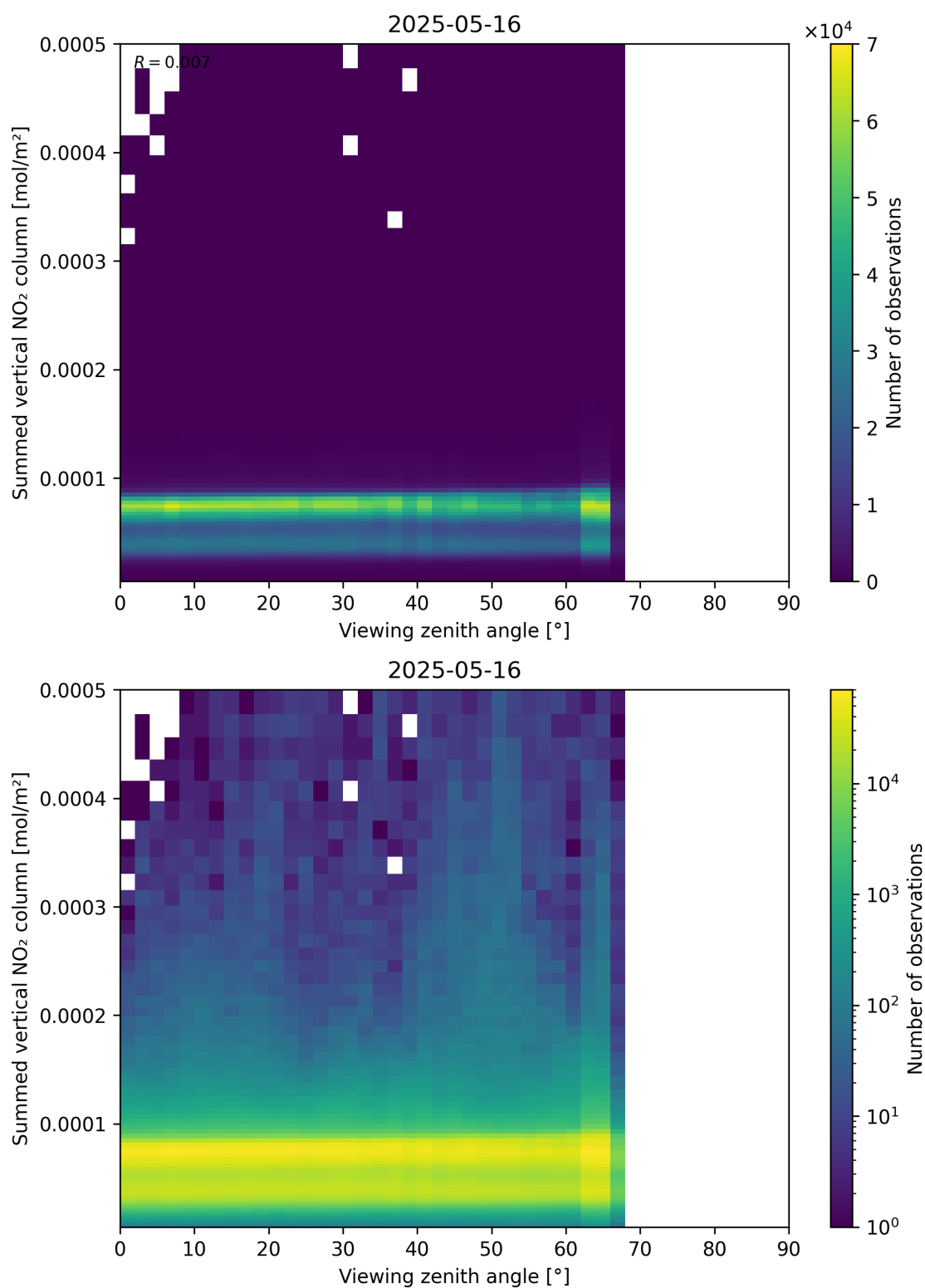
Figure 165: Scatter density plot of “Viewing zenith angle” against “Summed vertical NO 2 column” for 2025-05-15 to 2025-05-17.
