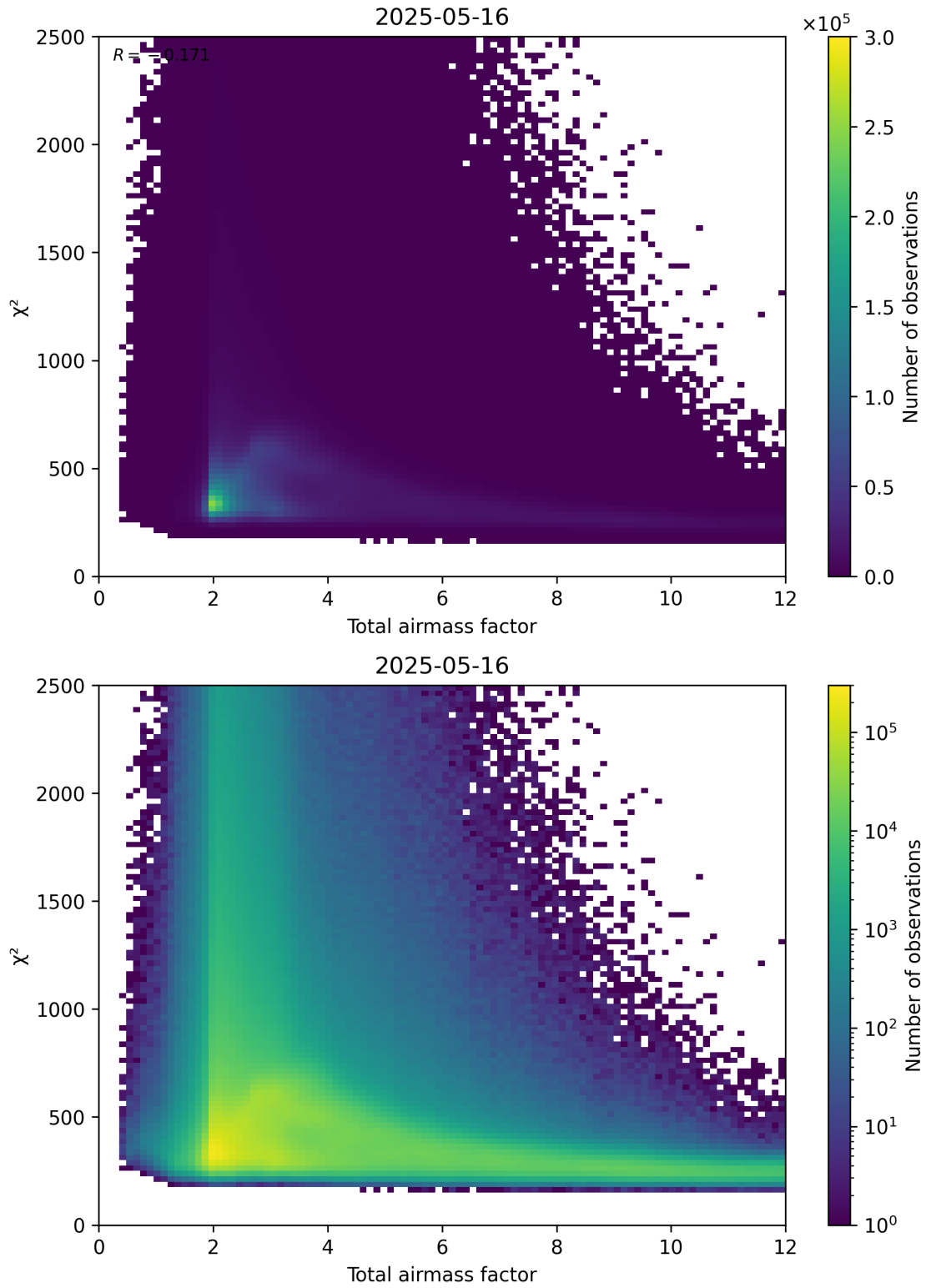
Figure 63: Scatter density plot of “Total airmass factor” against “ \chi^2 ” for 2025-05-15 to 2025-05-17.
