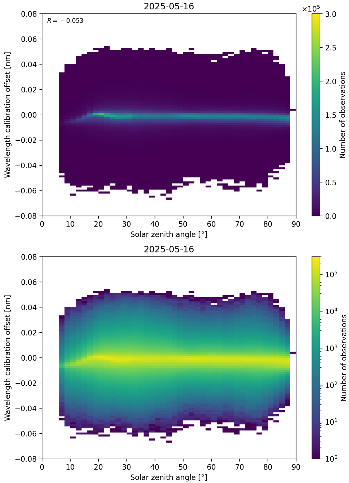
Figure 158: Scatter density plot of “Solar zenith angle” against “Wavelength calibration offset” for 2025-05-15 to 2025-05-17.
