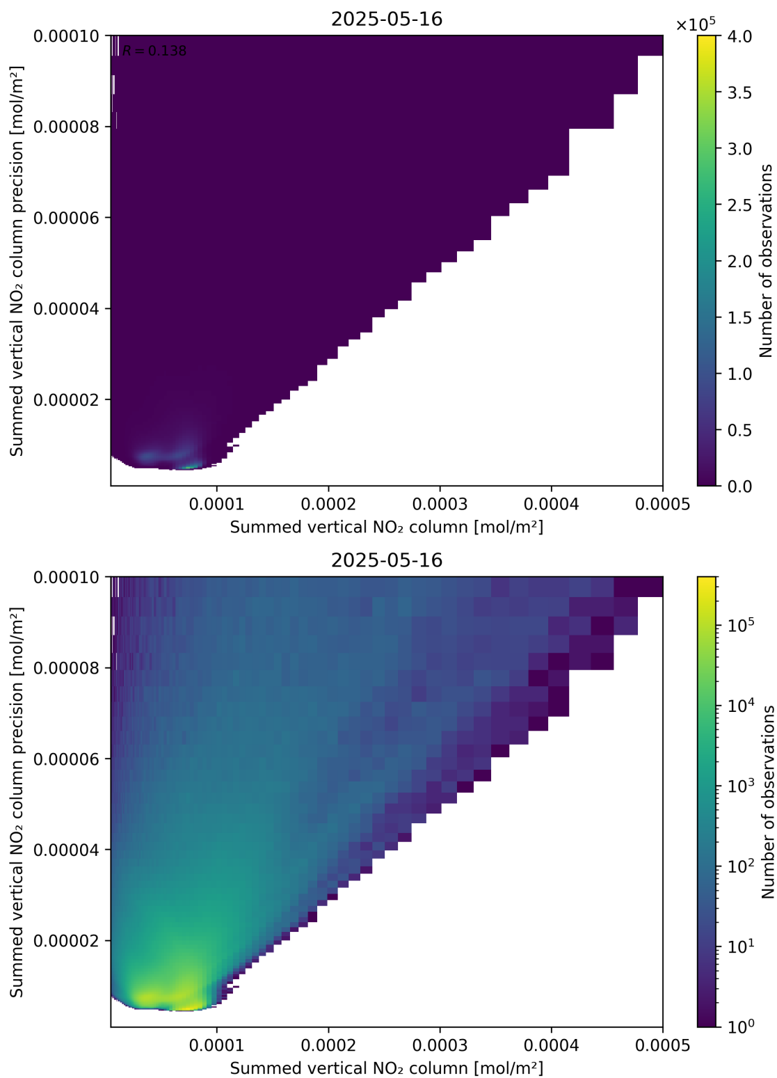
Figure 105: Scatter density plot of “Summed vertical NO 2 column” against “Summed vertical NO 2 column precision” for 2025-05-15 to 2025-05-17.
