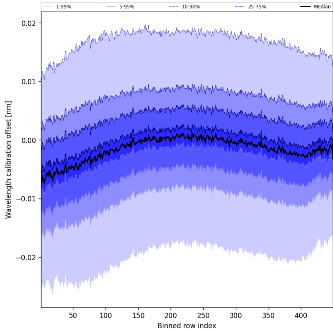
Figure 52: Along track statistics of “Wavelength calibration offset” for 2025-05-15 to 2025-05-17
