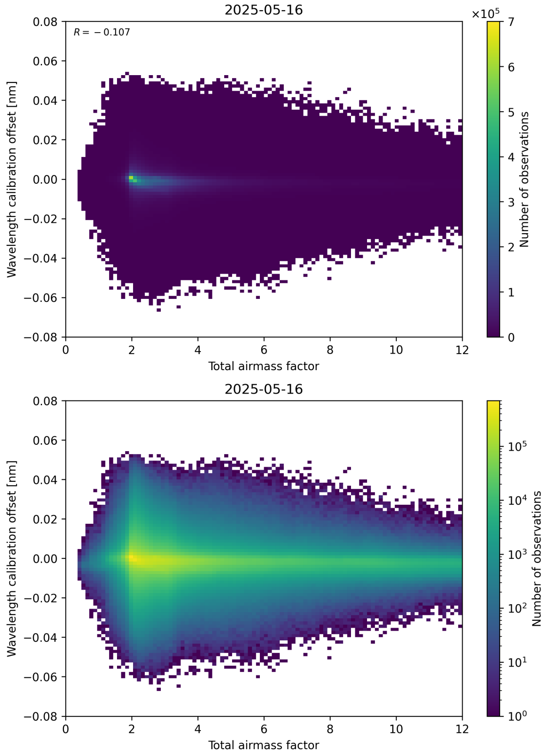
Figure 70: Scatter density plot of “Total airmass factor” against “Wavelength calibration offset” for 2025-05-15 to 2025-05-17.
