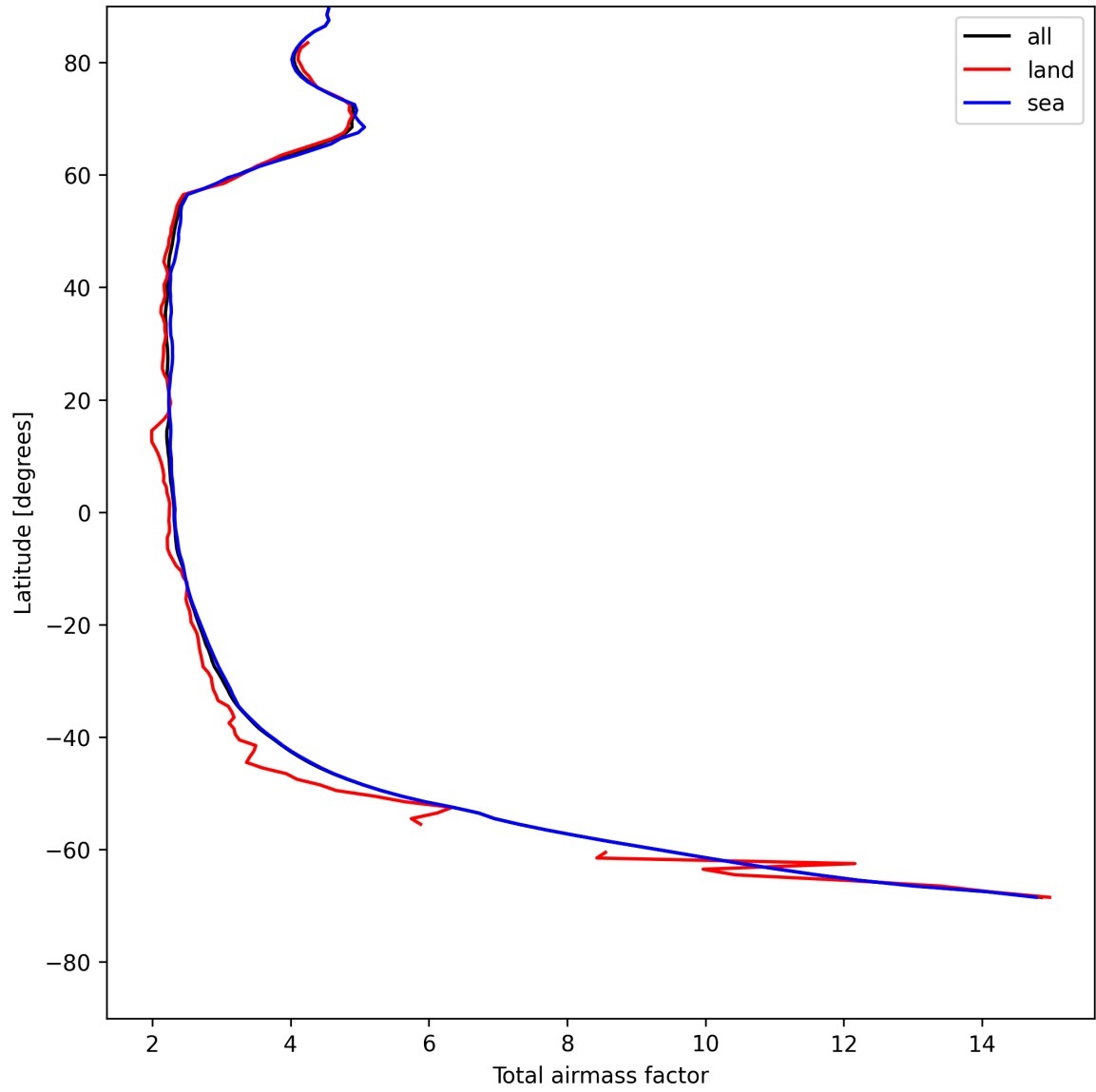
Figure 15: Zonal average of “Total airmass factor” for 2025-05-15 to 2025-05-17.
