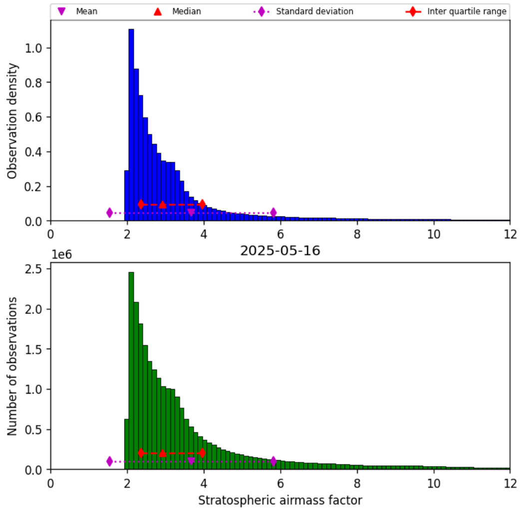
Figure 44: Histogram of “Stratospheric airmass factor” for 2025-05-15 to 2025-05-17
