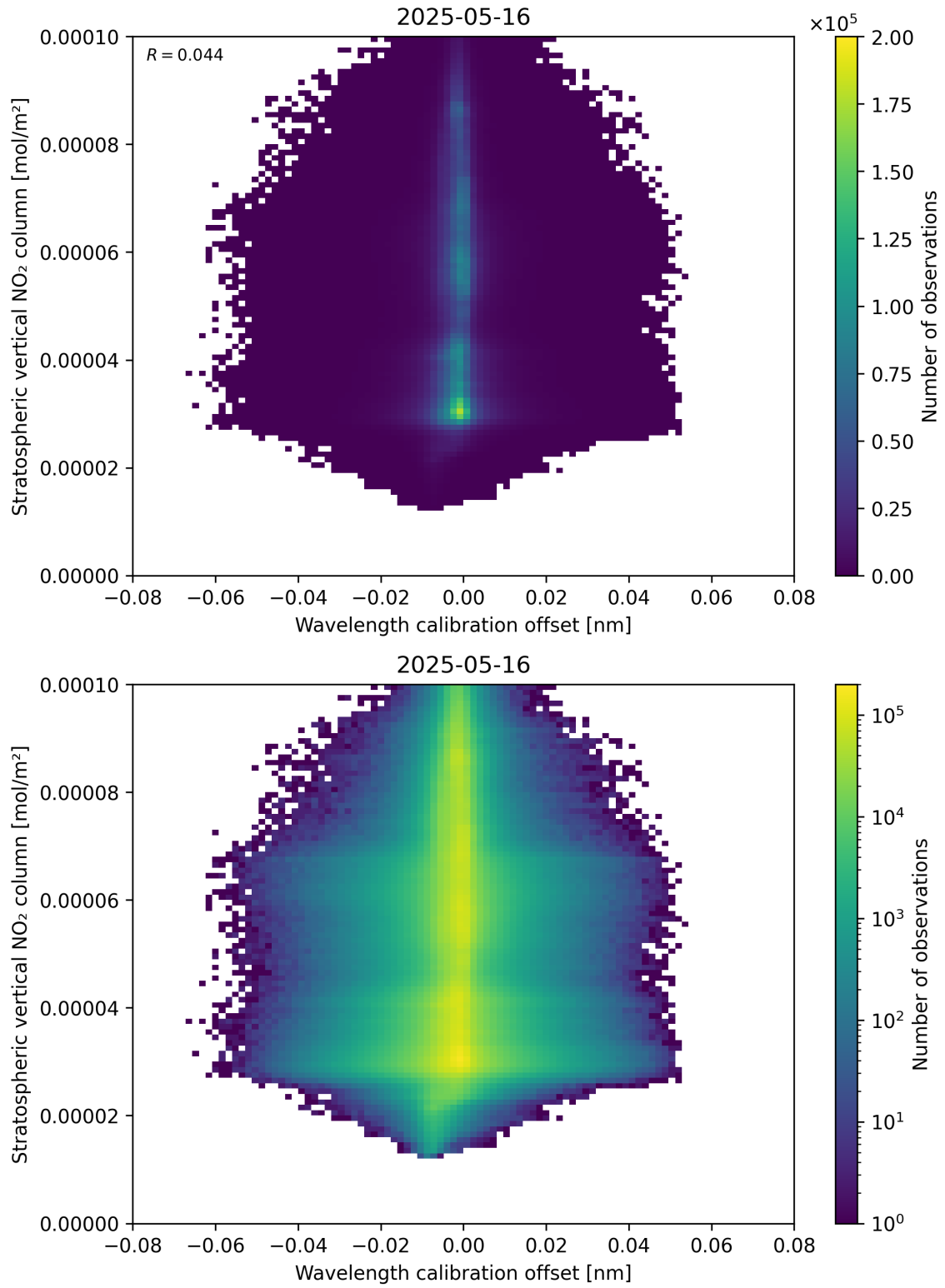
Figure 176: Scatter density plot of “Wavelength calibration offset” against “Stratospheric vertical NO 2 column” for 2025-05-15 to 2025-05-17.
