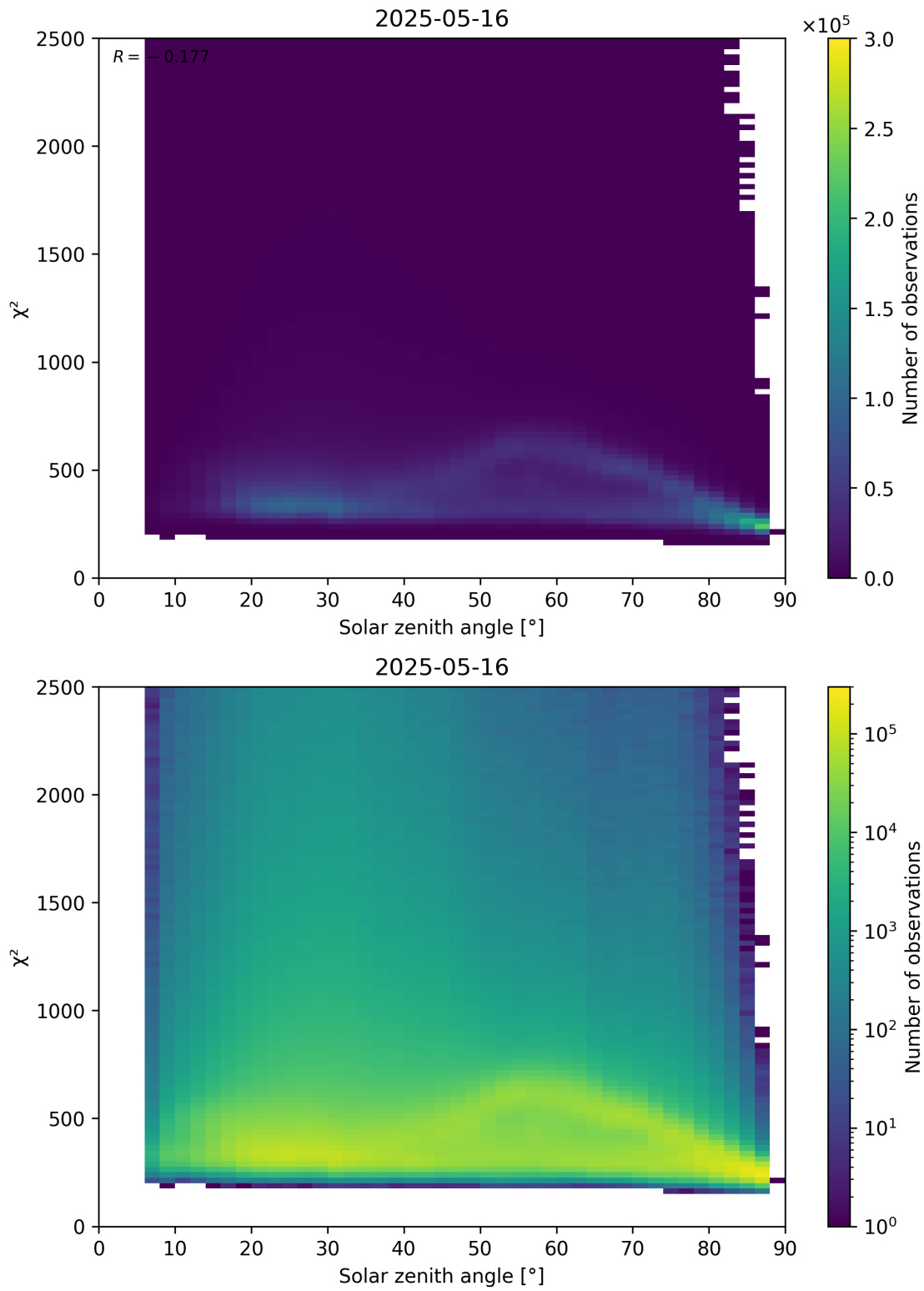
Figure 148: Scatter density plot of “Solar zenith angle” against “ \chi^2 ” for 2025-05-15 to 2025-05-17.
