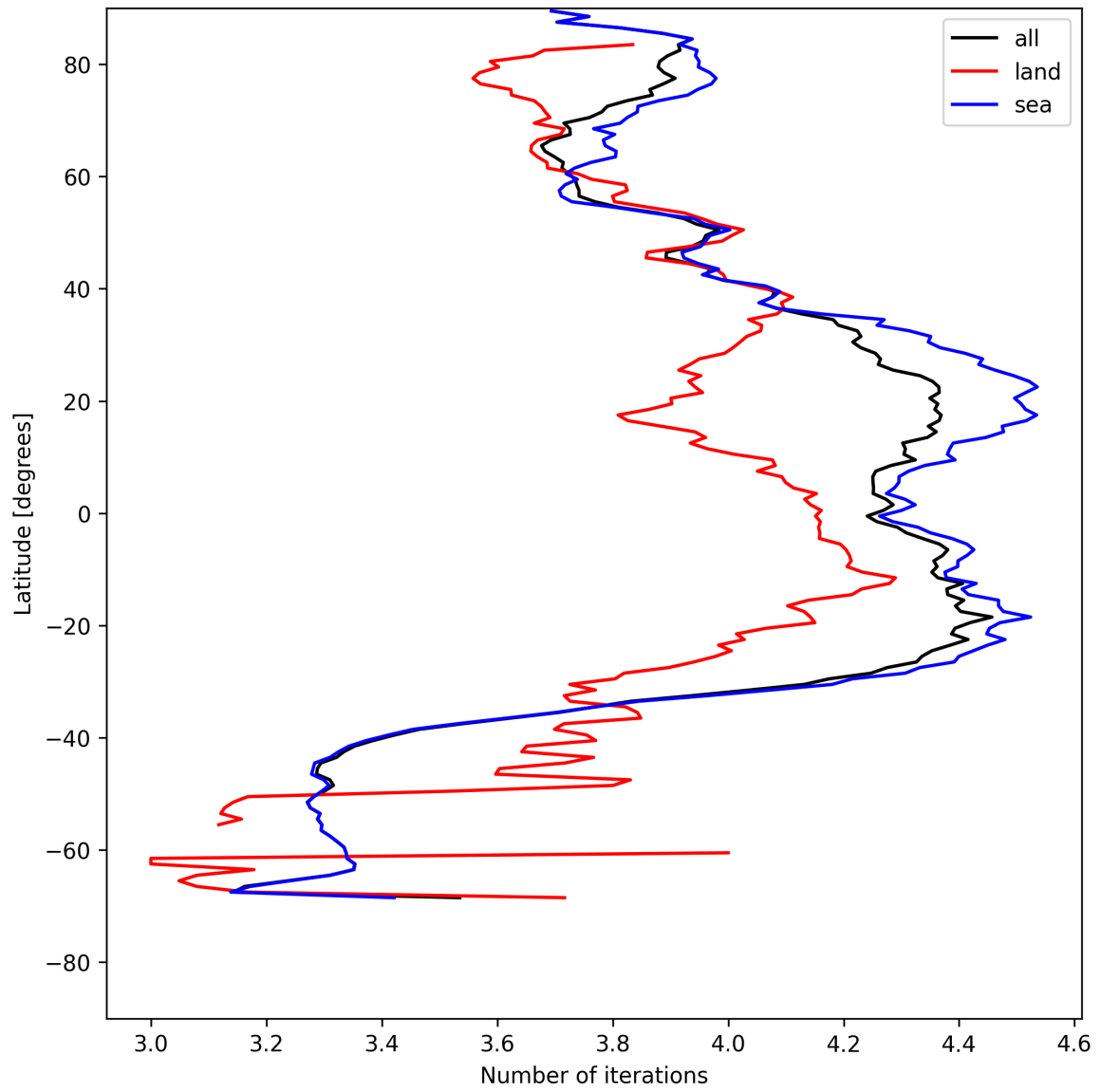
Figure 17: Zonal average of “Number of iterations” for 2025-05-15 to 2025-05-17.
