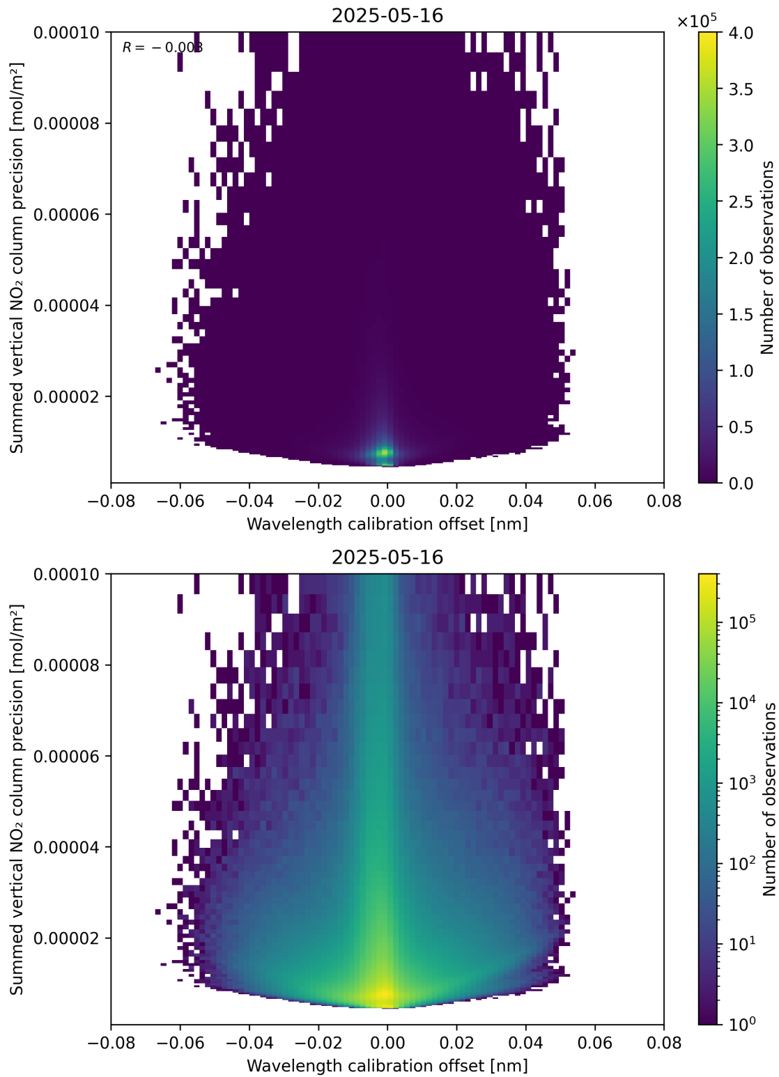
Figure 178: Scatter density plot of “Wavelength calibration offset” against “Summed vertical NO 2 column precision” for 2025-05-15 to 2025-05-17.
