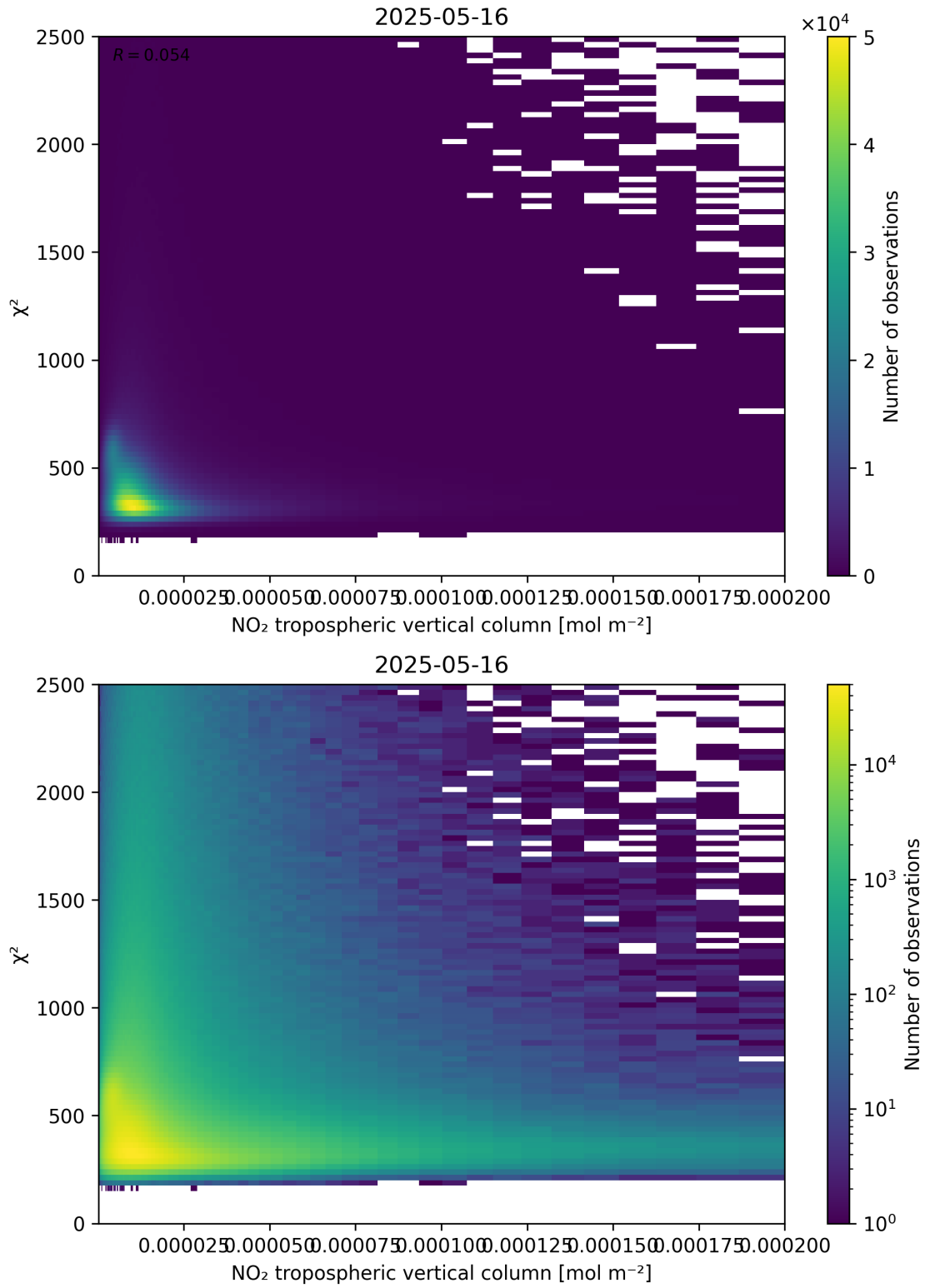
Figure 124: Scatter density plot of “NO 2 tropospheric vertical column” against “ \chi^2 ” for 2025-05-15 to 2025-05-17.
