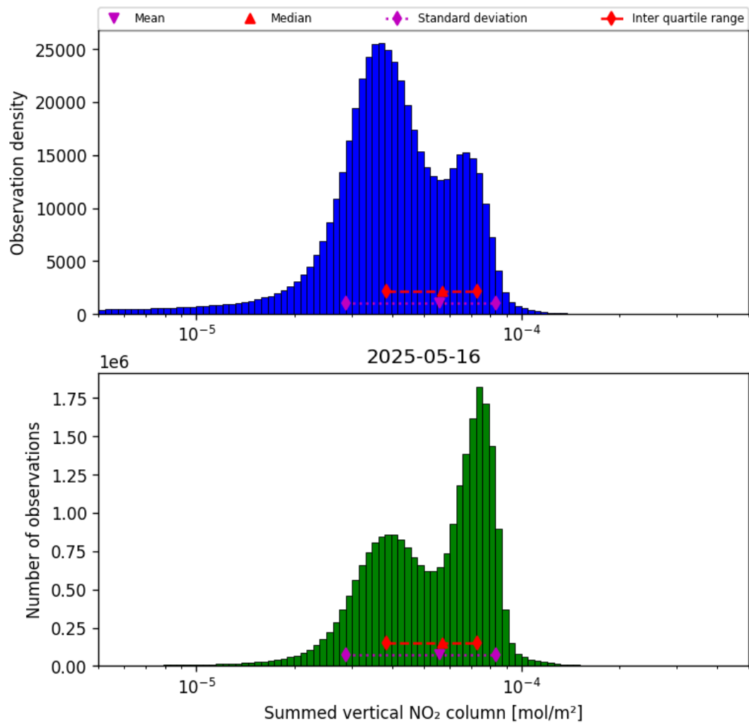
Figure 40: Histogram of “Summed vertical NO 2 column” for 2025-05-15 to 2025-05-17
