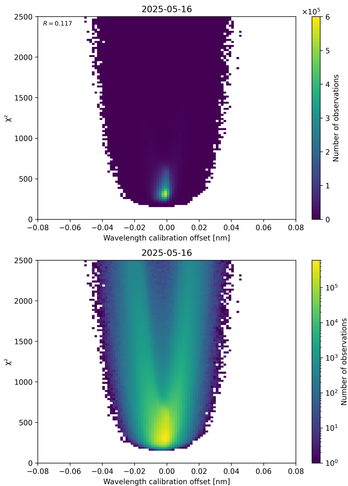
Figure 175: Scatter density plot of “Wavelength calibration offset” against “ \chi^2 ” for 2025-05-15 to 2025-05-17.
