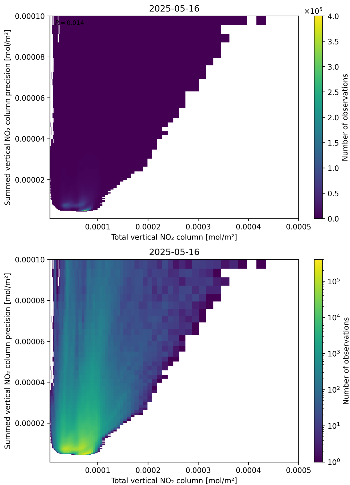
Figure 113: Scatter density plot of “Total vertical NO 2 column” against “Summed vertical NO 2 column precision” for 2025-05-15 to 2025-05-17.
