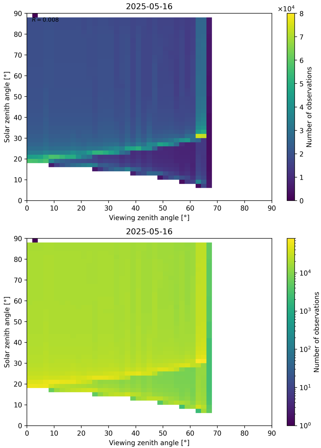
Figure 172: Scatter density plot of “Viewing zenith angle” against “Solar zenith angle” for 2025-05-15 to 2025-05-17.
