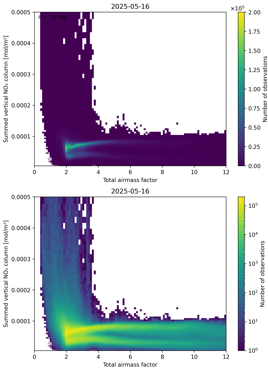
Figure 65: Scatter density plot of “Total airmass factor” against “Summed vertical NO 2 column” for 2025-05-15 to 2025-05-17.
