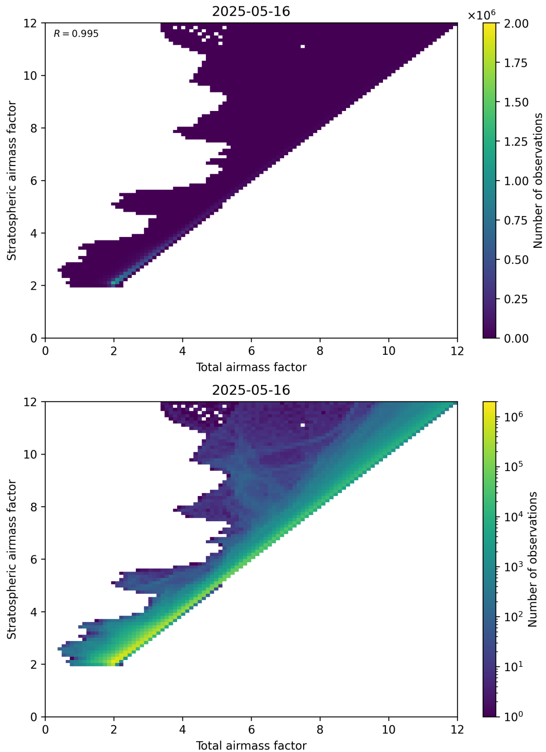
Figure 62: Scatter density plot of “Total airmass factor” against “Stratospheric airmass factor” for 2025-05-15 to 2025-05-17.
