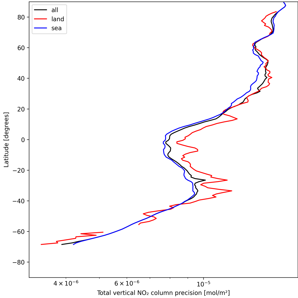
Figure 22: Zonal average of “Total vertical NO 2 column precision” for 2025-05-15 to 2025-05-17.
