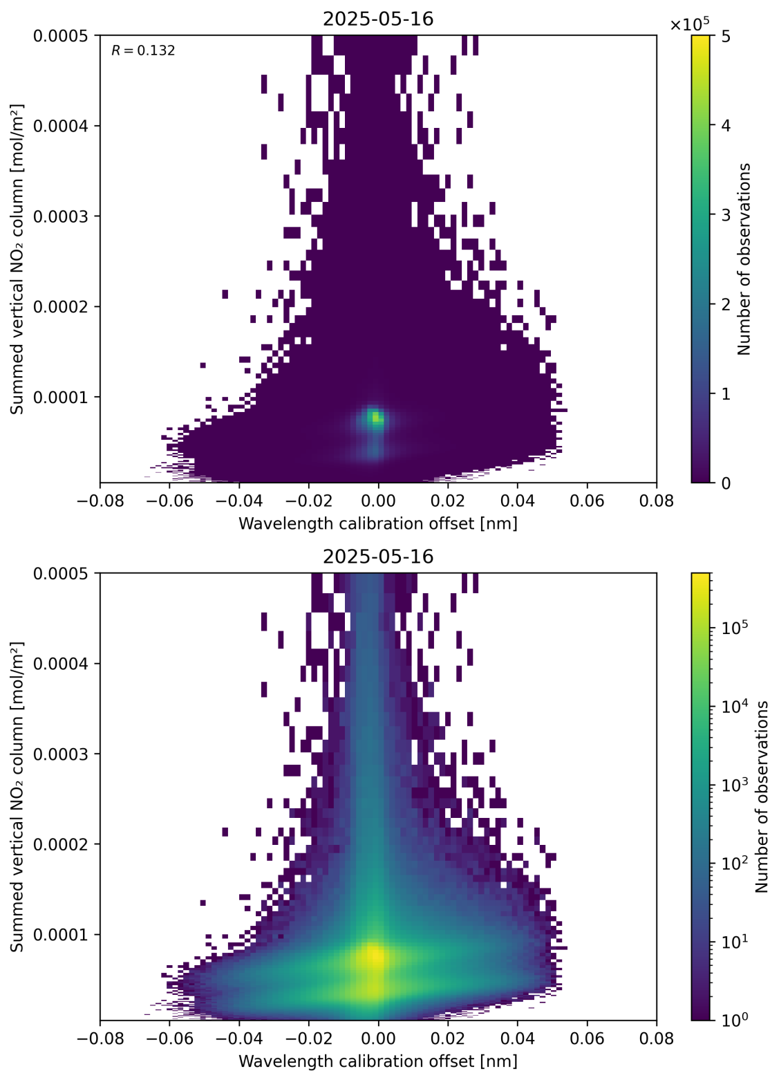
Figure 177: Scatter density plot of “Wavelength calibration offset” against “Summed vertical NO 2 column” for 2025-05-15 to 2025-05-17.
