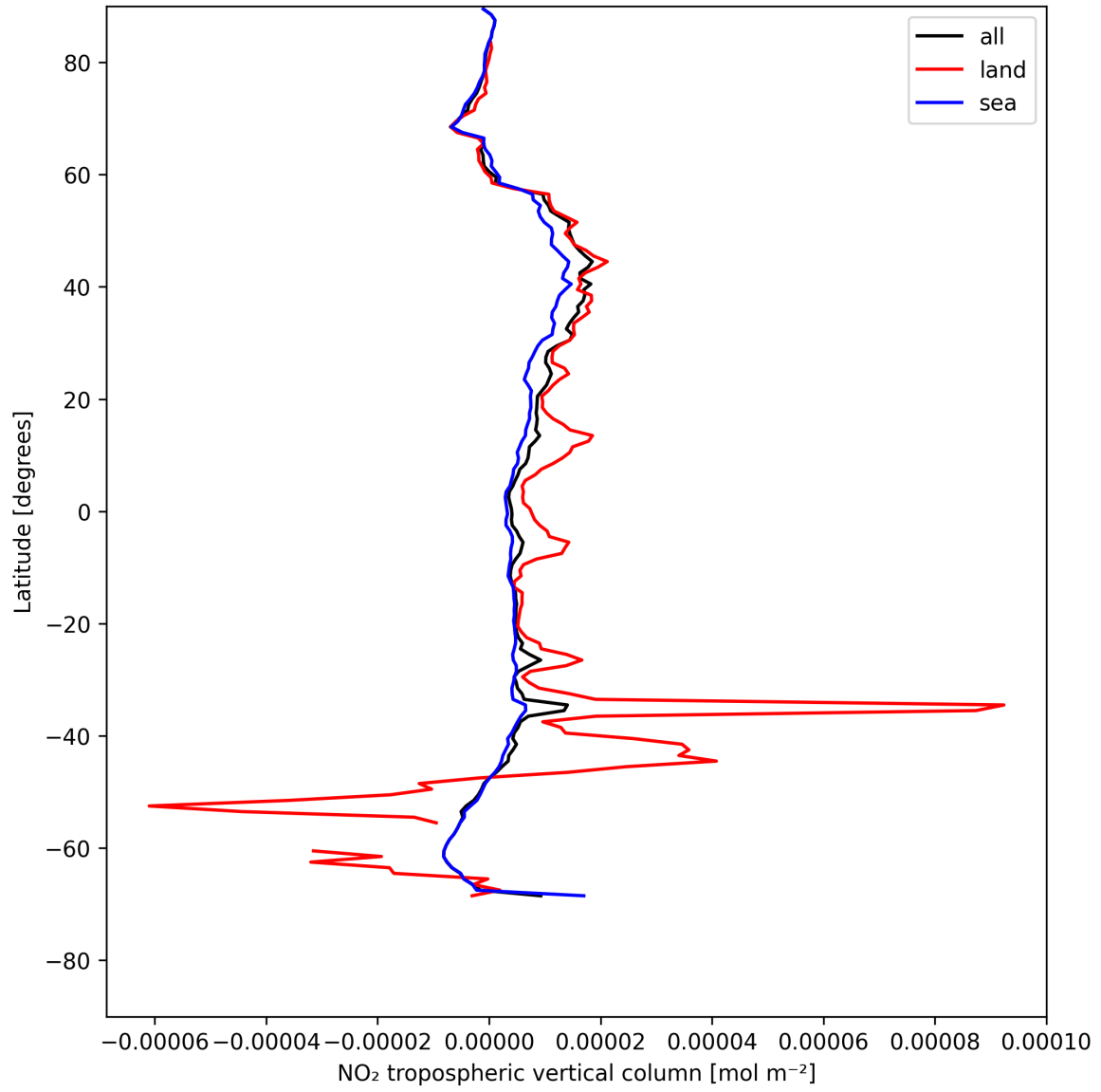
Figure 12: Zonal average of “NO 2 tropospheric vertical column” for 2025-05-15 to 2025-05-17.
