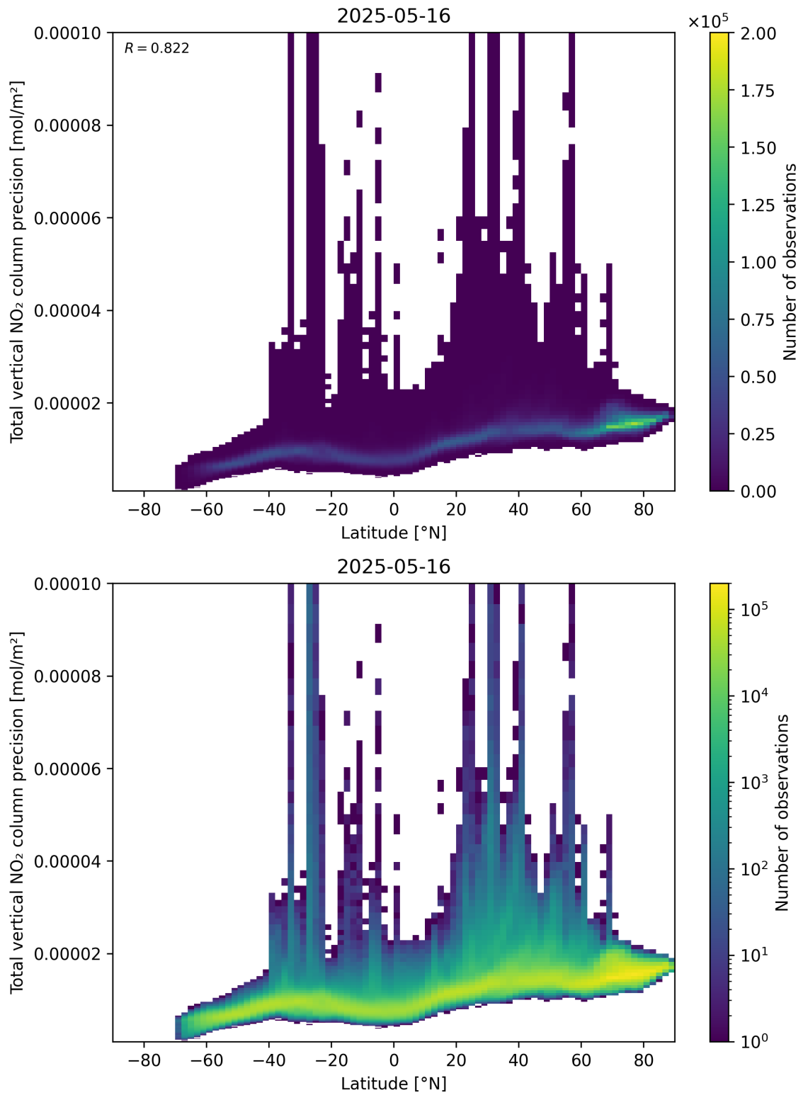
Figure 91: Scatter density plot of “Latitude” against “Total vertical NO 2 column precision” for 2025-05-15 to 2025-05-17.
