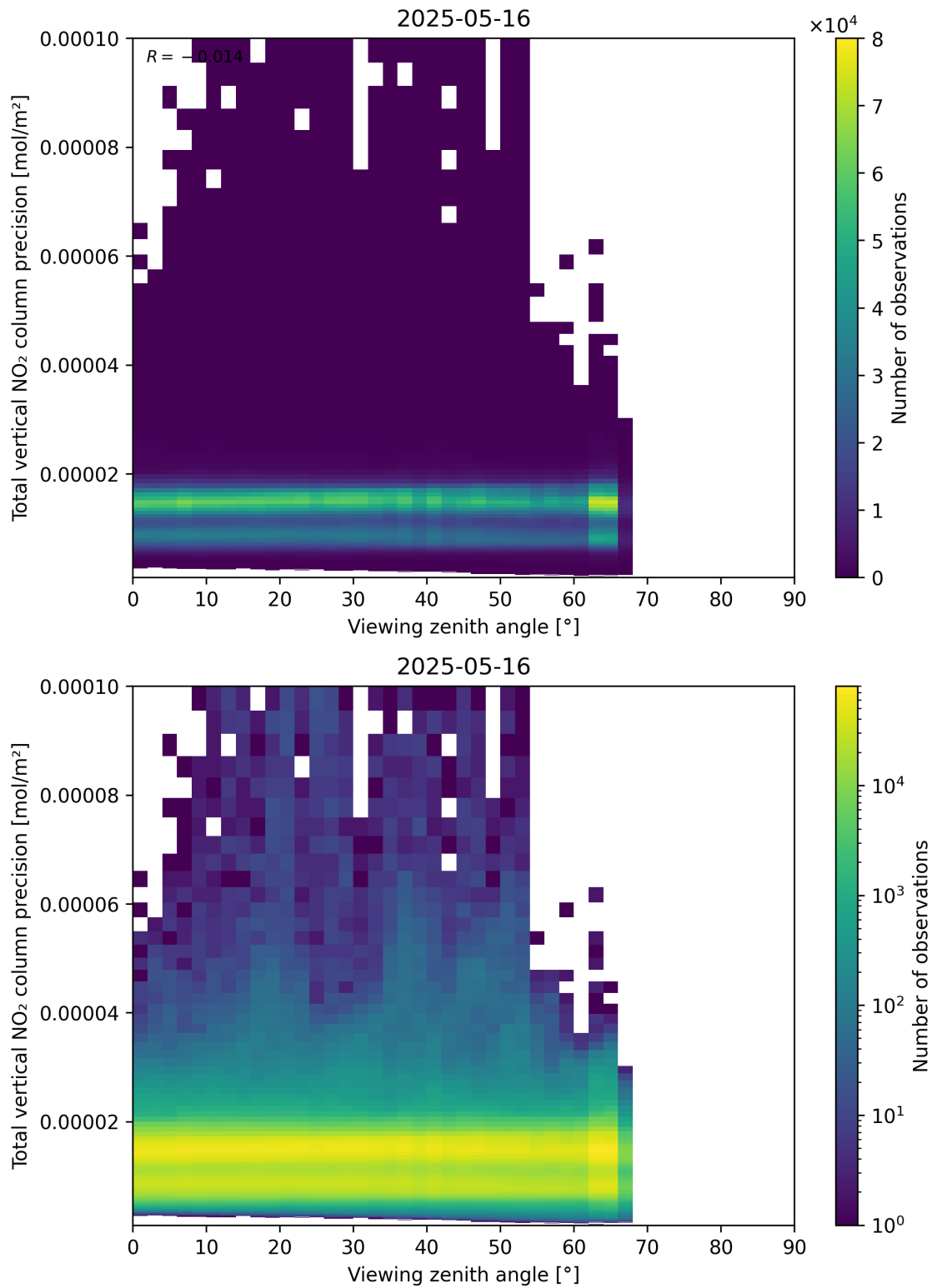
Figure 168: Scatter density plot of “Viewing zenith angle” against “Total vertical NO 2 column precision” for 2025-05-15 to 2025-05-17.
