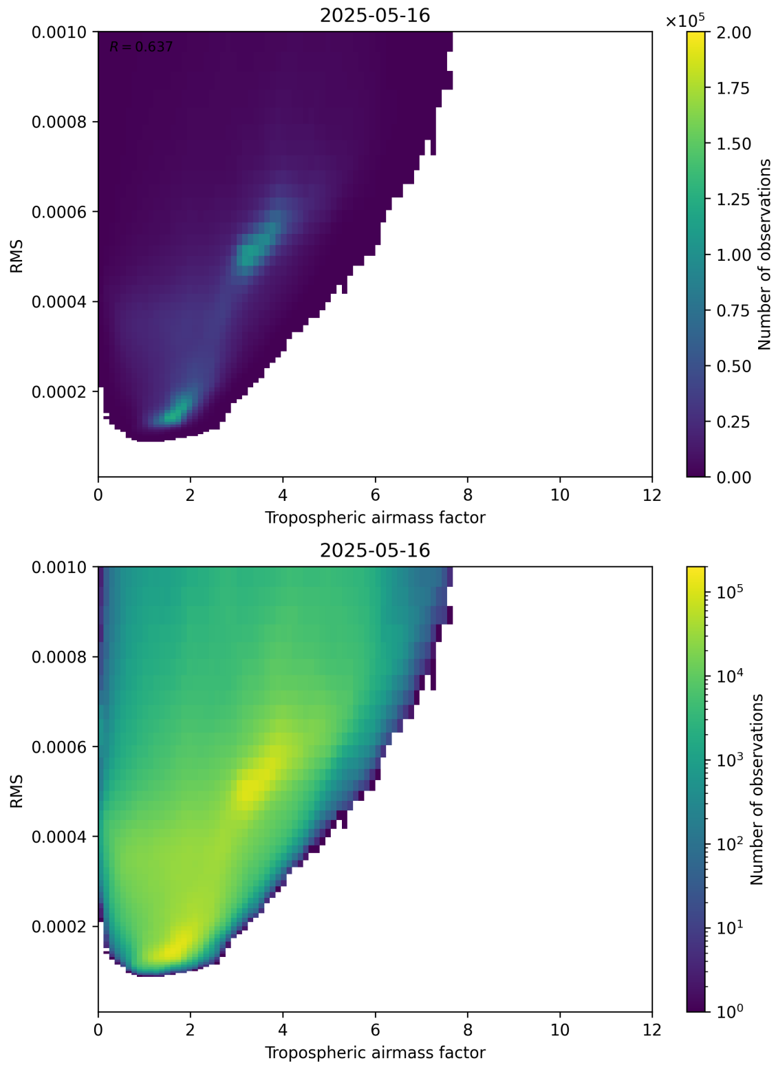
Figure 79: Scatter density plot of “Tropospheric airmass factor” against “RMS” for 2025-05-15 to 2025-05-17.
