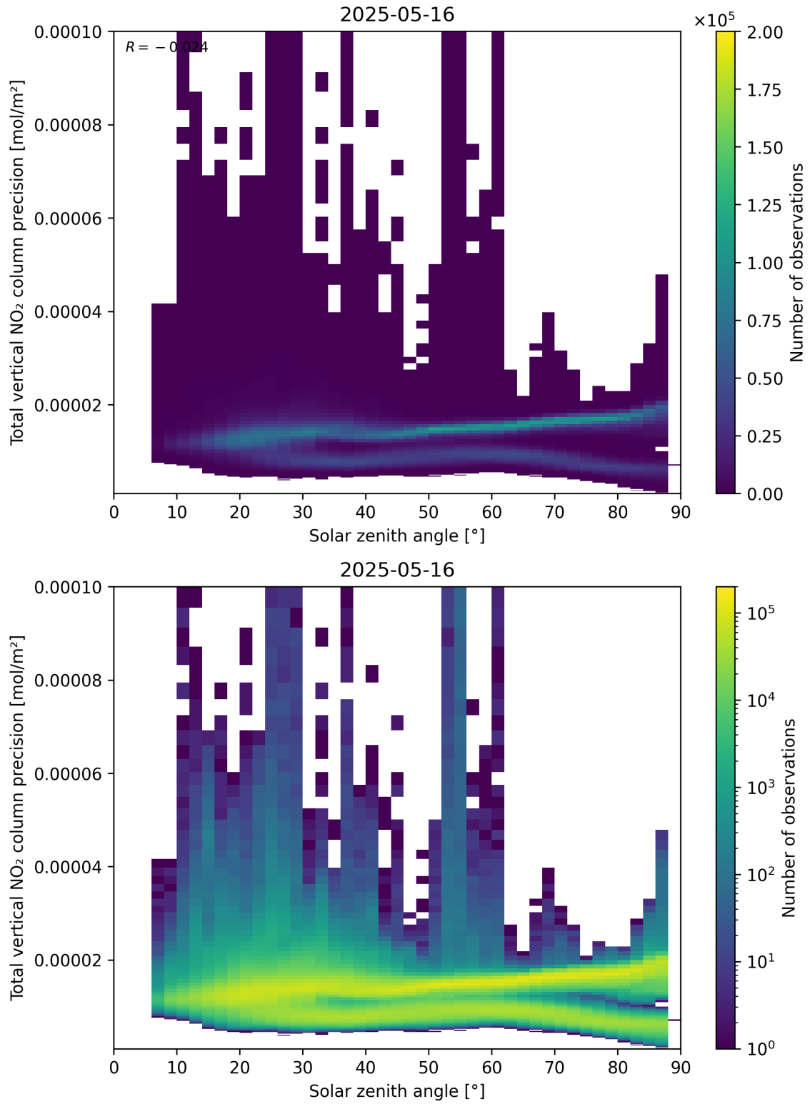
Figure 154: Scatter density plot of “Solar zenith angle” against “Total vertical NO 2 column precision” for 2025-05-15 to 2025-05-17.
