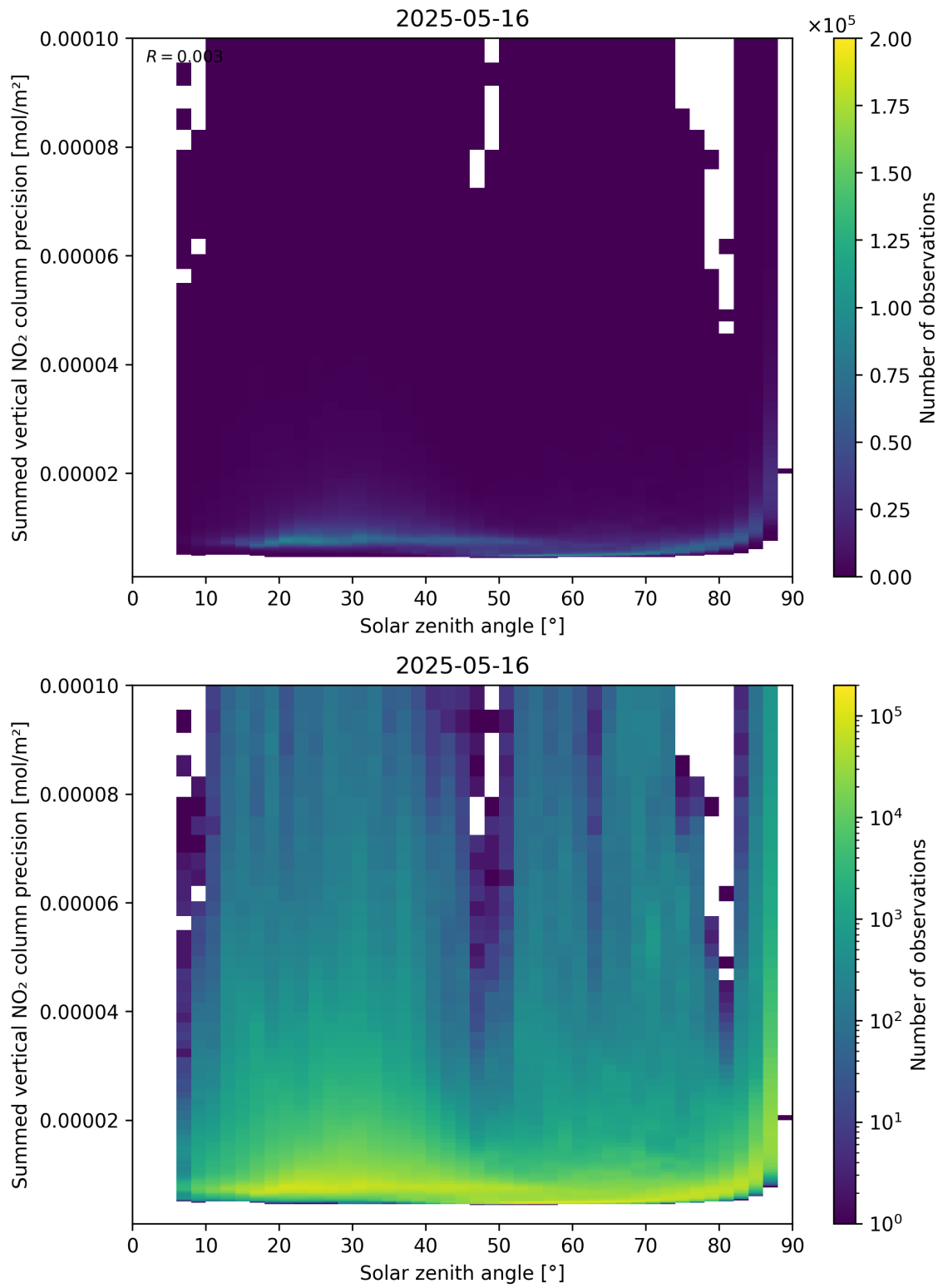
Figure 152: Scatter density plot of “Solar zenith angle” against “Summed vertical NO 2 column precision” for 2025-05-15 to 2025-05-17.
