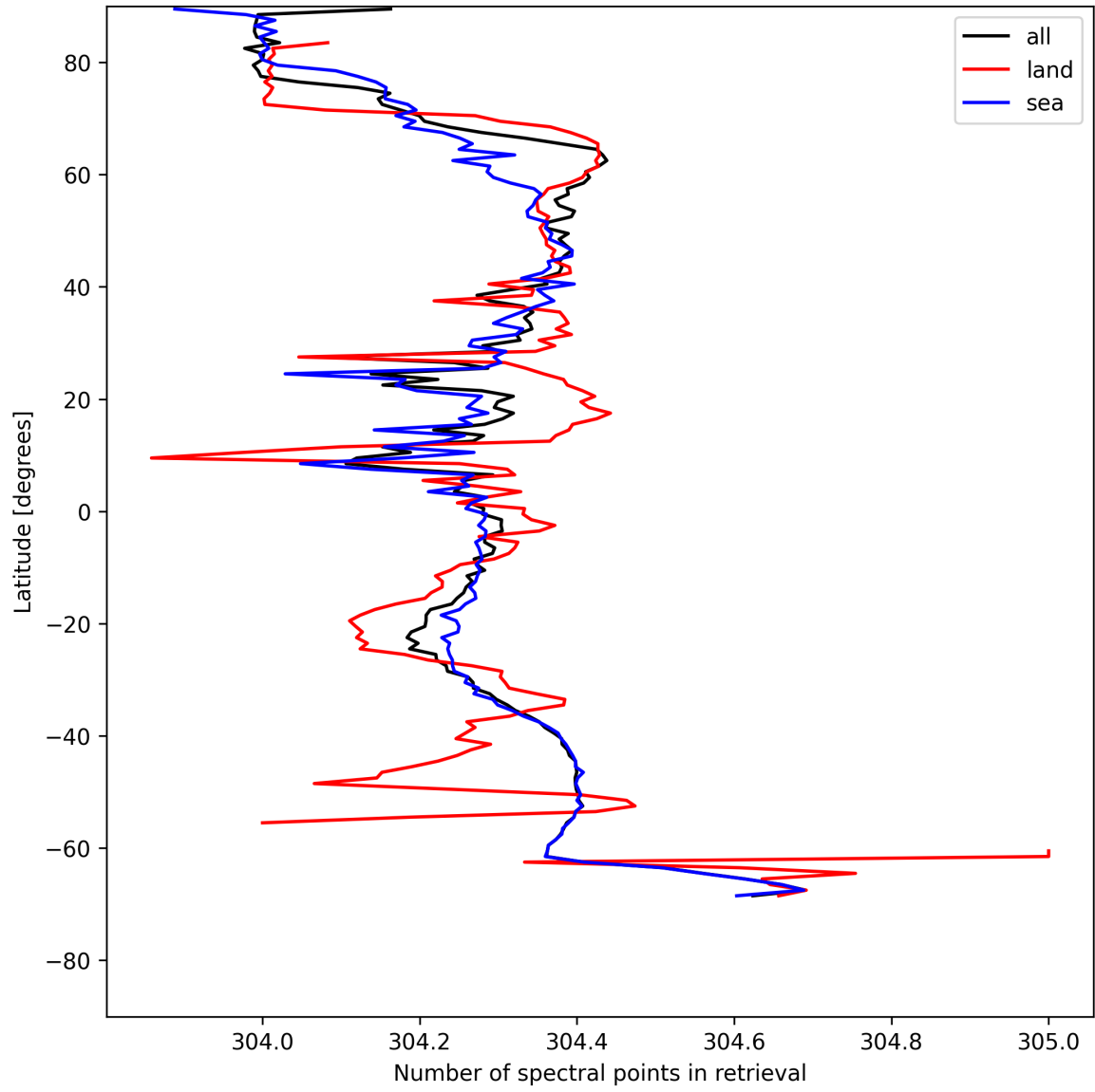
Figure 16: Zonal average of “Number of spectral points in retrieval” for 2025-05-15 to 2025-05-17.
