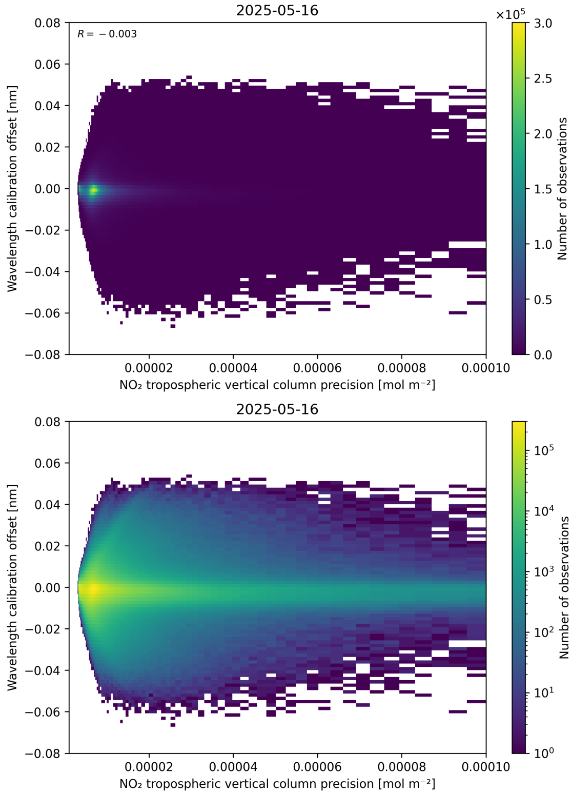
Figure 141: Scatter density plot of “NO 2 tropospheric vertical column precision” against “Wavelength calibration offset” for 2025-05-15 to 2025-05-17.
