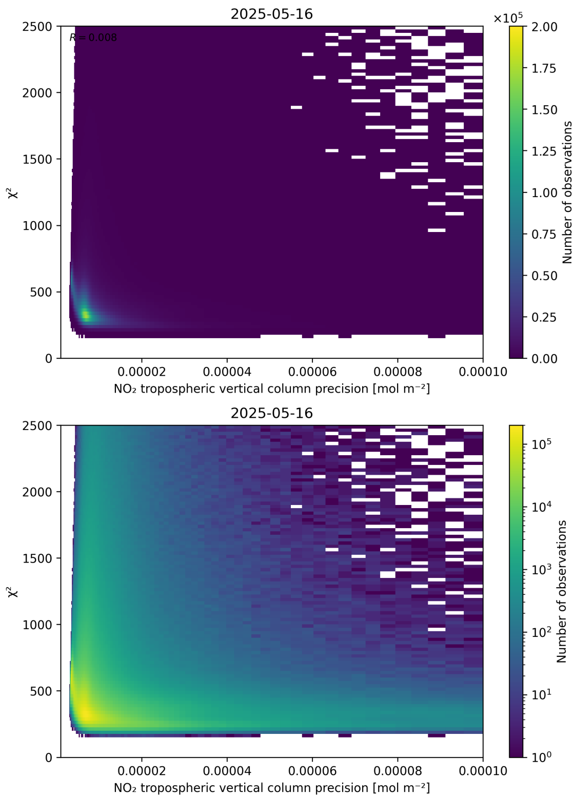
Figure 134: Scatter density plot of “NO 2 tropospheric vertical column precision” against “ \chi^2 ” for 2025-05-15 to 2025-05-17.
