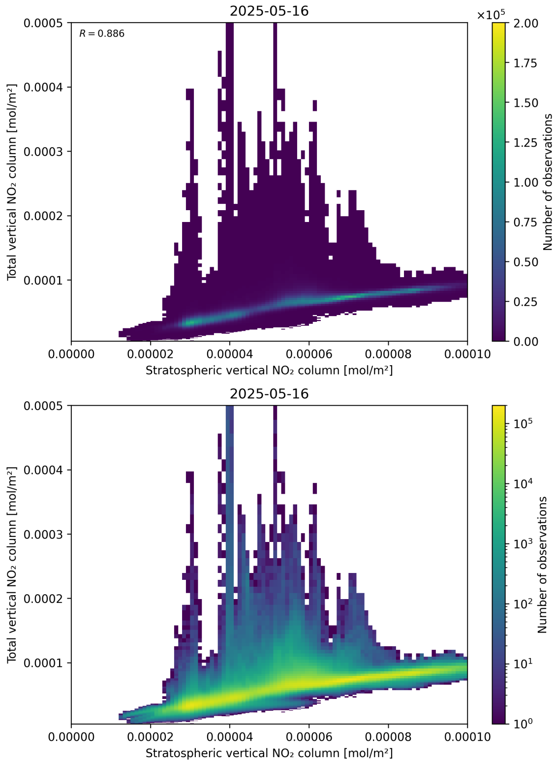
Figure 100: Scatter density plot of “Stratospheric vertical NO 2 column” against “Total vertical NO 2 column” for 2025-05-15 to 2025-05-17.
