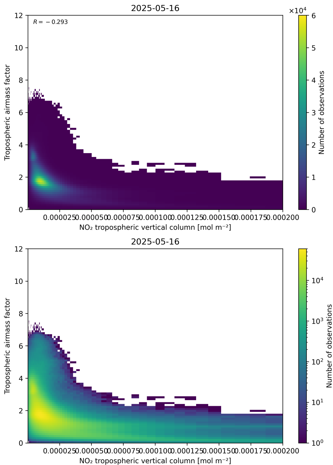
Figure 123: Scatter density plot of “NO 2 tropospheric vertical column” against “Tropospheric air mass factor” for 2025-05-15 to 2025-05-17.
