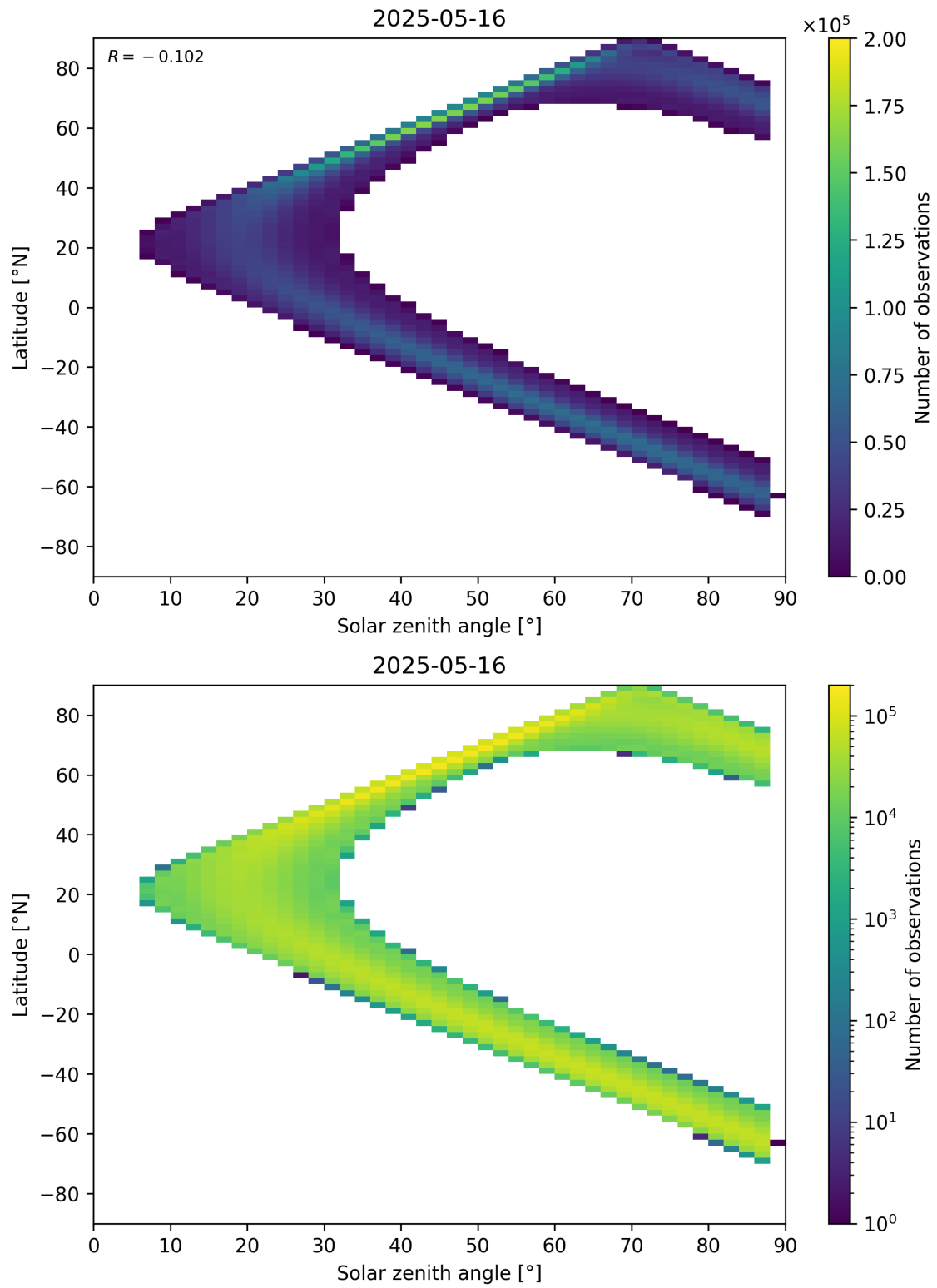
Figure 149: Scatter density plot of “Solar zenith angle” against “Latitude” for 2025-05-15 to 2025-05-17.
