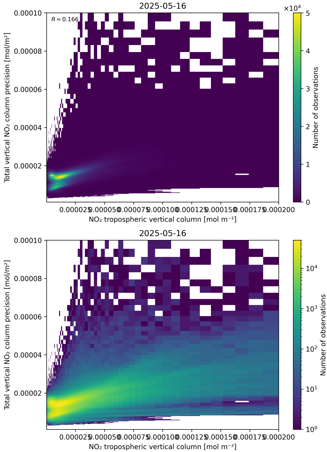
Figure 129: Scatter density plot of “NO 2 tropospheric vertical column” against “Total vertical NO 2 column precision” for 2025-05-15 to 2025-05-17.
