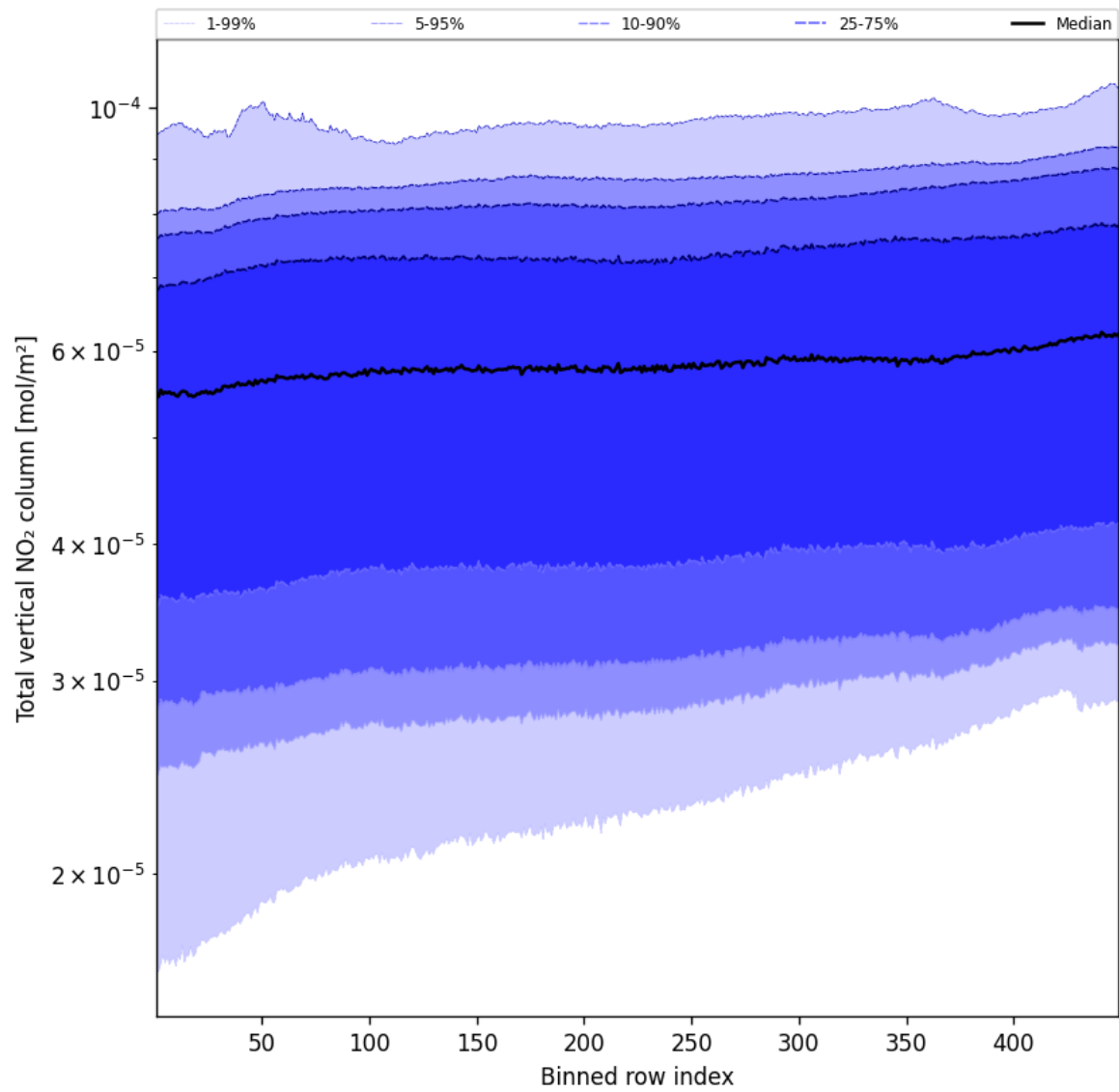
Figure 55: Along track statistics of “Total vertical NO 2 column” for 2025-05-15 to 2025-05-17
