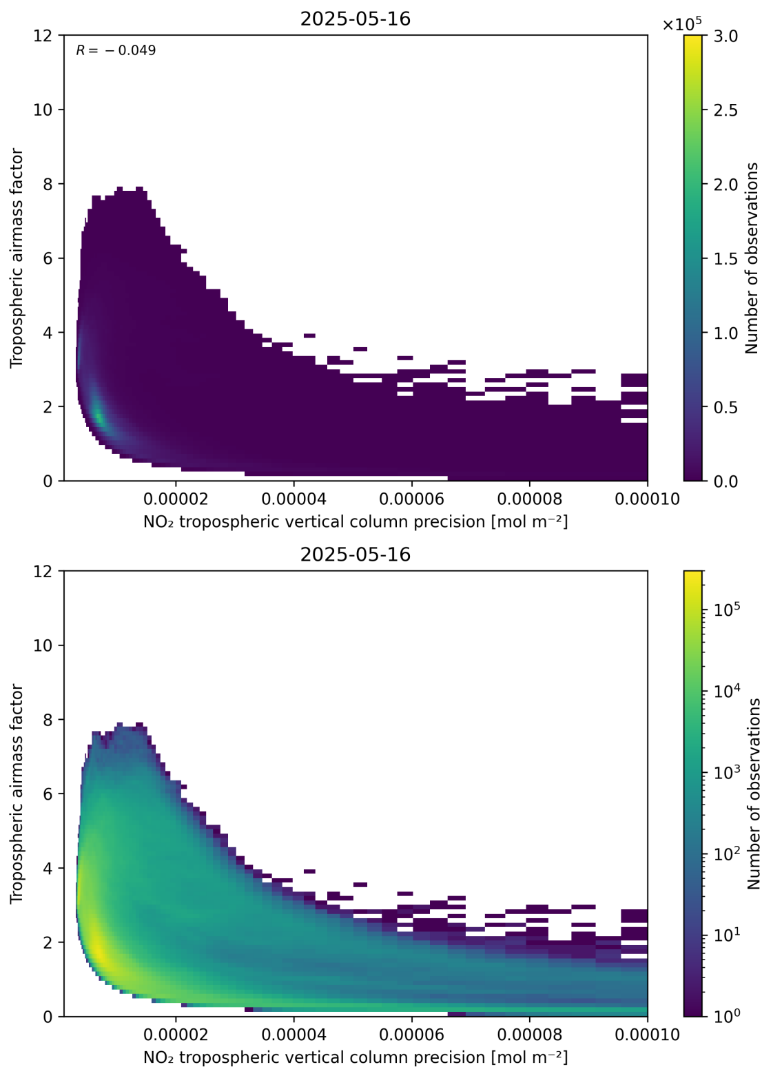
Figure 133: Scatter density plot of “NO 2 tropospheric vertical column precision” against “Tropospheric airmass factor” for 2025-05-15 to 2025-05-17.
