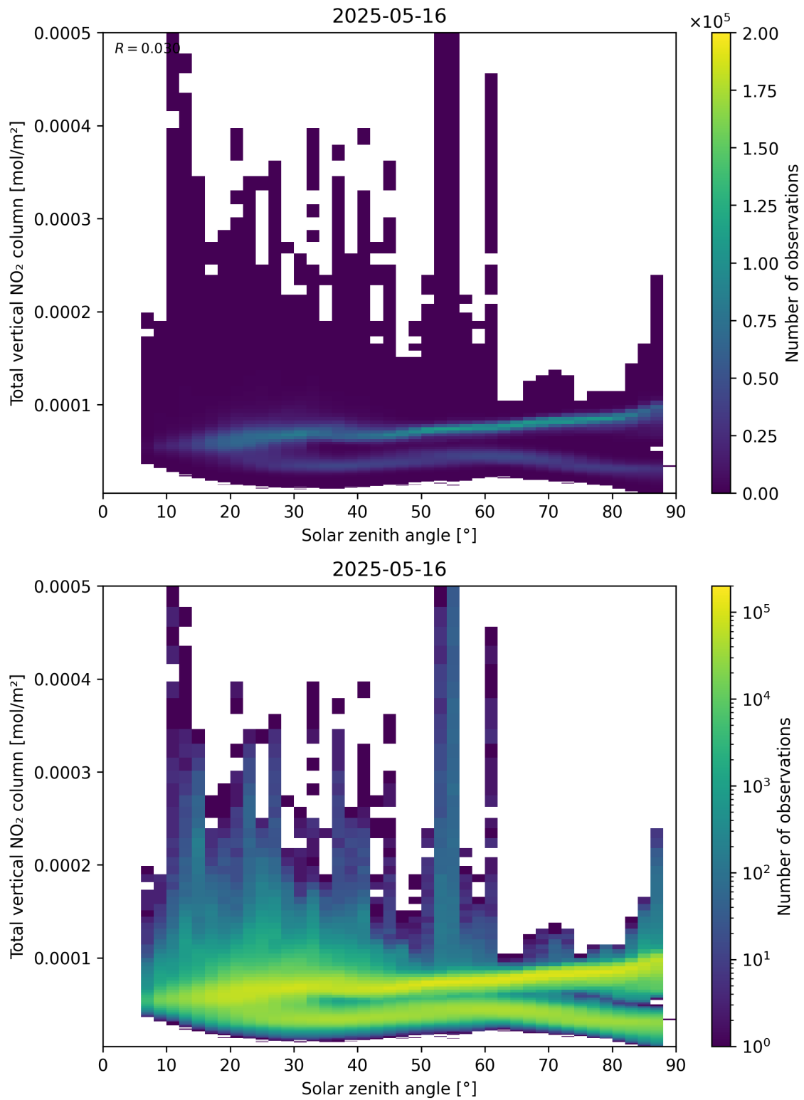
Figure 153: Scatter density plot of “Solar zenith angle” against “Total vertical NO 2 column” for 2025-05-15 to 2025-05-17.
