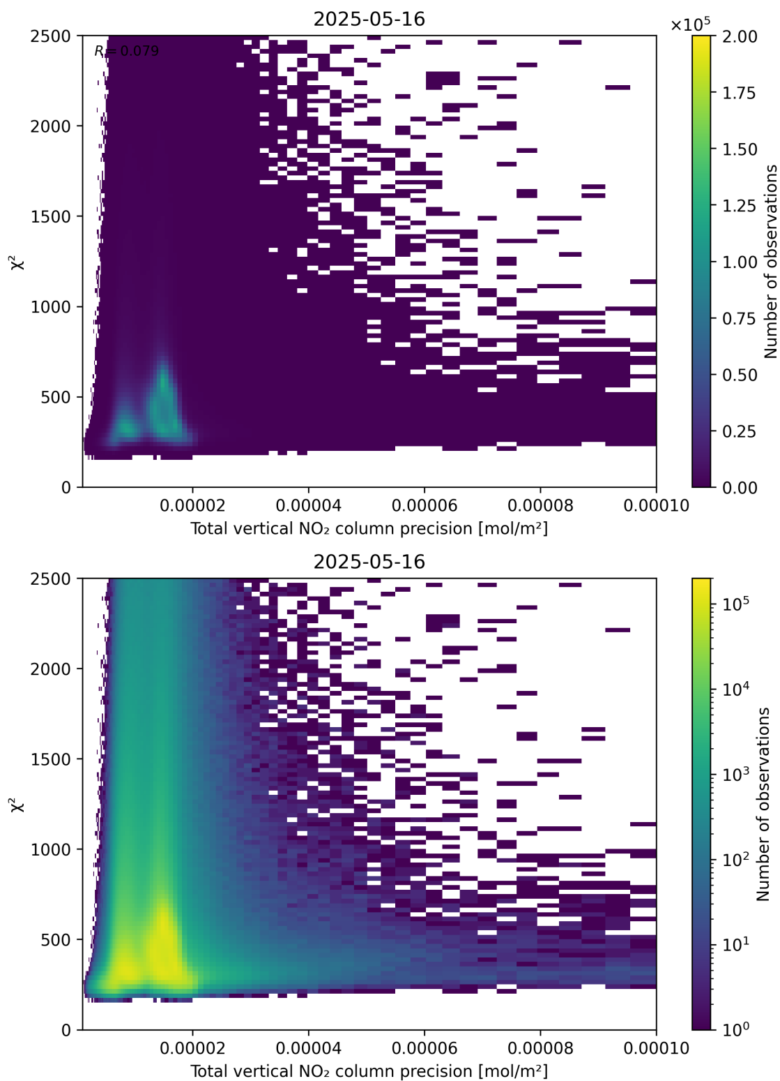
Figure 116: Scatter density plot of “Total vertical NO 2 column precision” against “ \chi^2 ” for 2025-05-15 to 2025-05-17.
