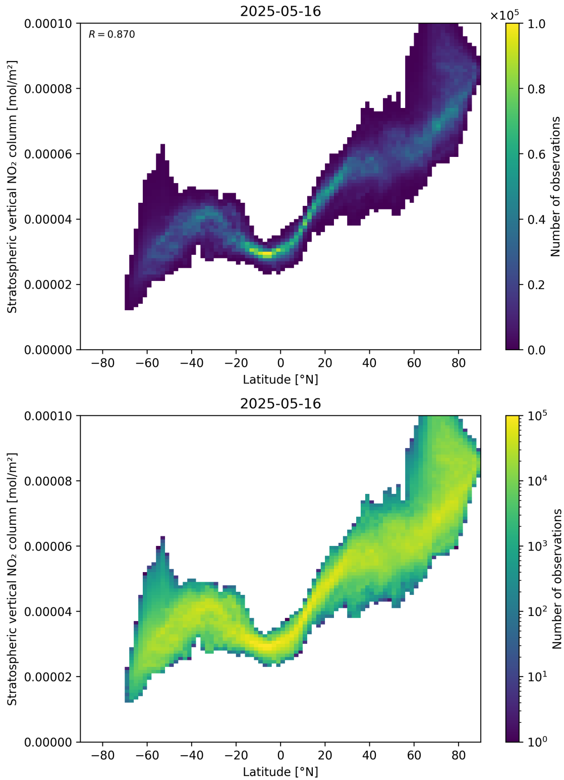
Figure 87: Scatter density plot of “Latitude” against “Stratospheric vertical NO 2 column” for 2025-05-15 to 2025-05-17.
