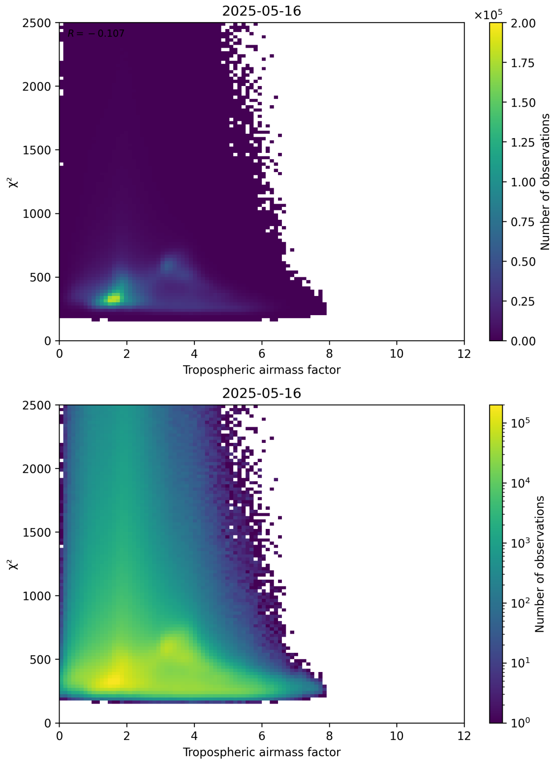
Figure 73: Scatter density plot of “Tropospheric airmass factor” against “ \chi^2 ” for 2025-05-15 to 2025-05-17.
