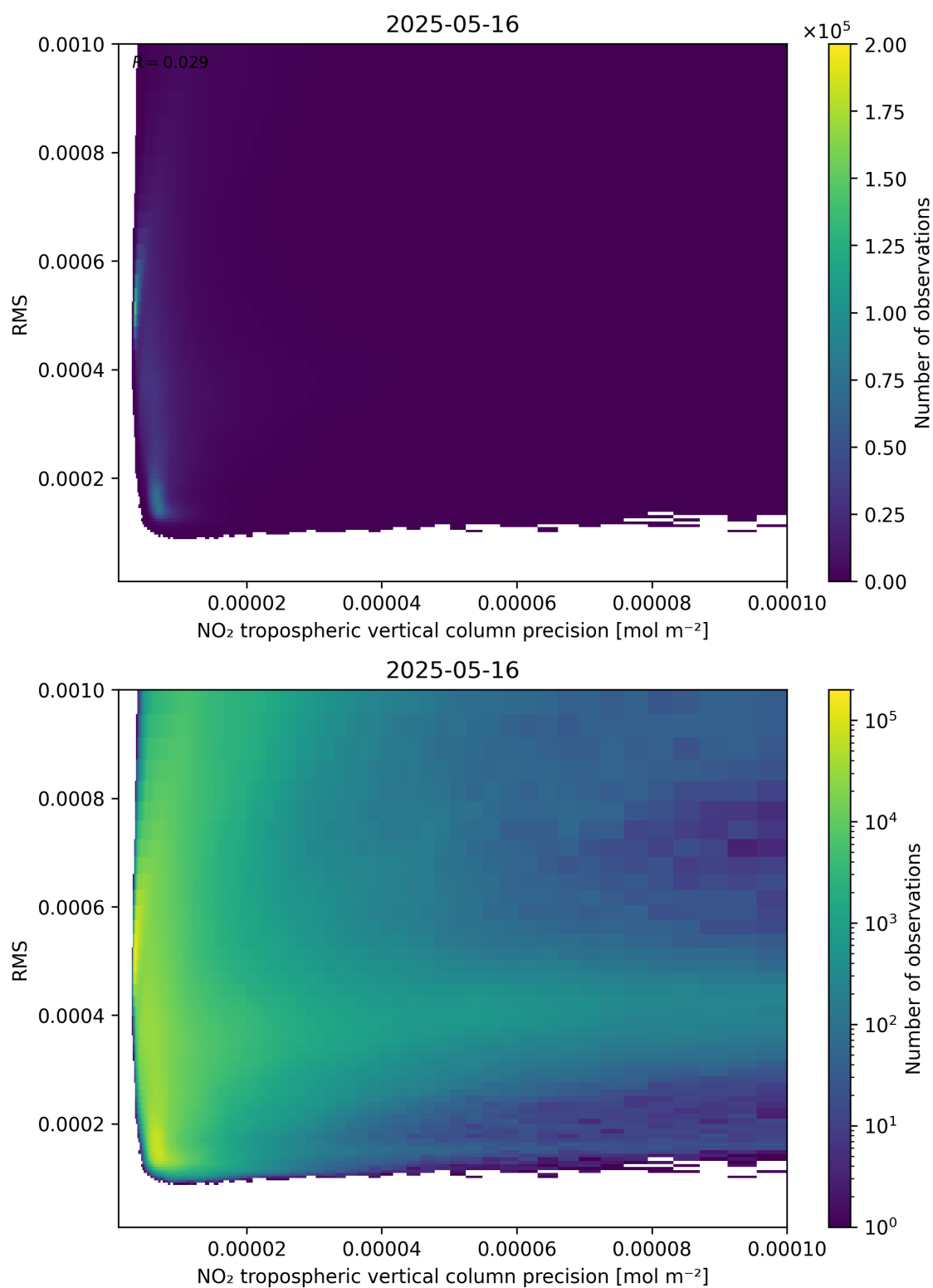
Figure 140: Scatter density plot of “NO 2 tropospheric vertical column precision” against “RMS” for 2025-05-15 to 2025-05-17.
