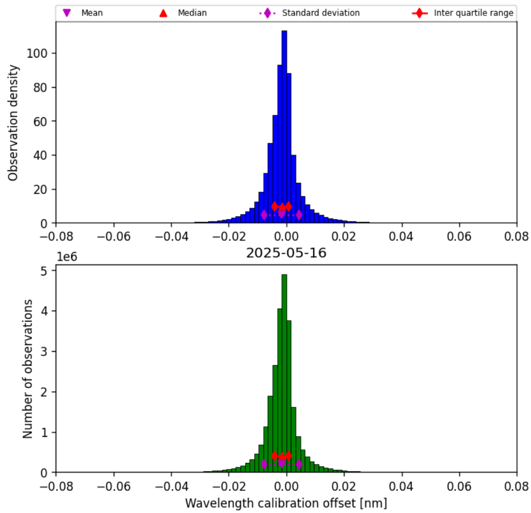
Figure 35: Histogram of “Wavelength calibration offset” for 2025-05-15 to 2025-05-17
