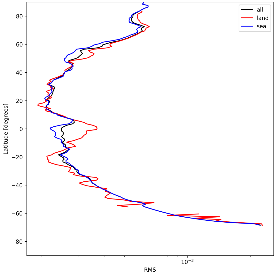
Figure 26: Zonal average of “RMS” for 2025-05-15 to 2025-05-17.
