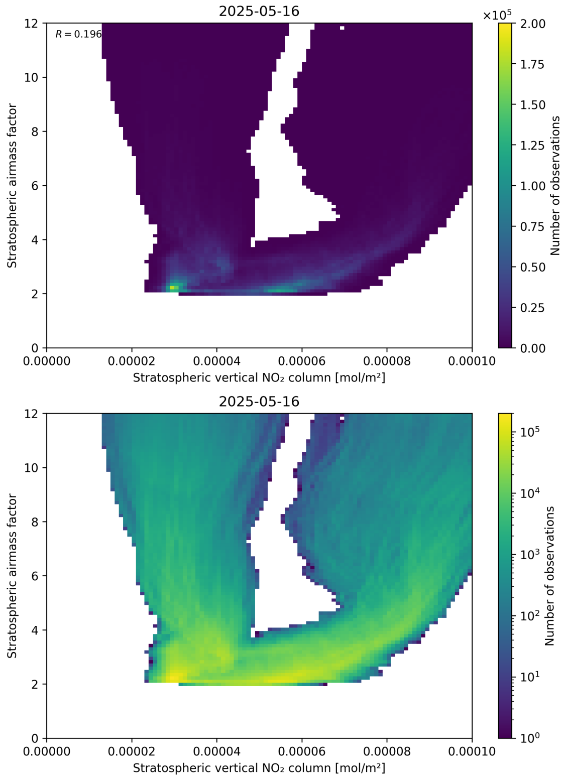
Figure 96: Scatter density plot of “Stratospheric vertical NO 2 column” against “Stratospheric airmass factor” for 2025-05-15 to 2025-05-17.
