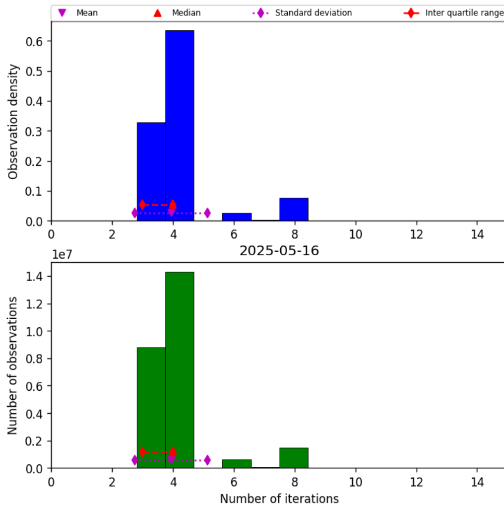
Figure 34: Histogram of “Number of iterations” for 2025-05-15 to 2025-05-17
