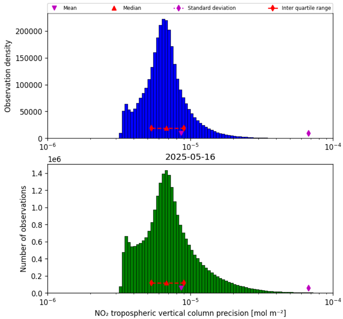
Figure 30: Histogram of “NO 2 tropospheric vertical column precision” for 2025-05-15 to 2025-05-17
