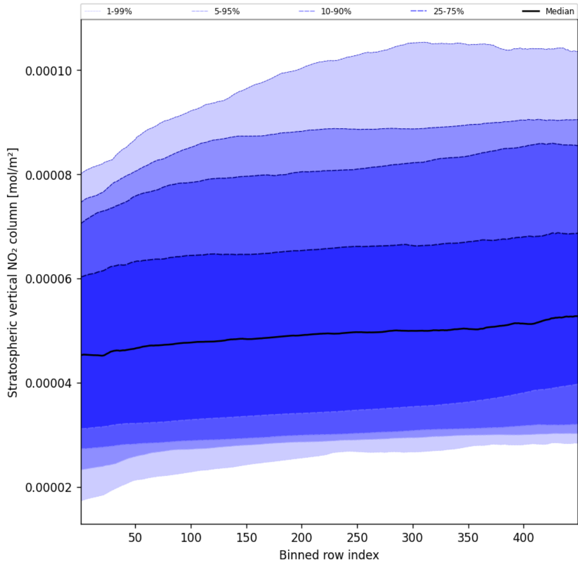
Figure 53: Along track statistics of “Stratospheric vertical NO 2 column” for 2025-05-15 to 2025-05-17
