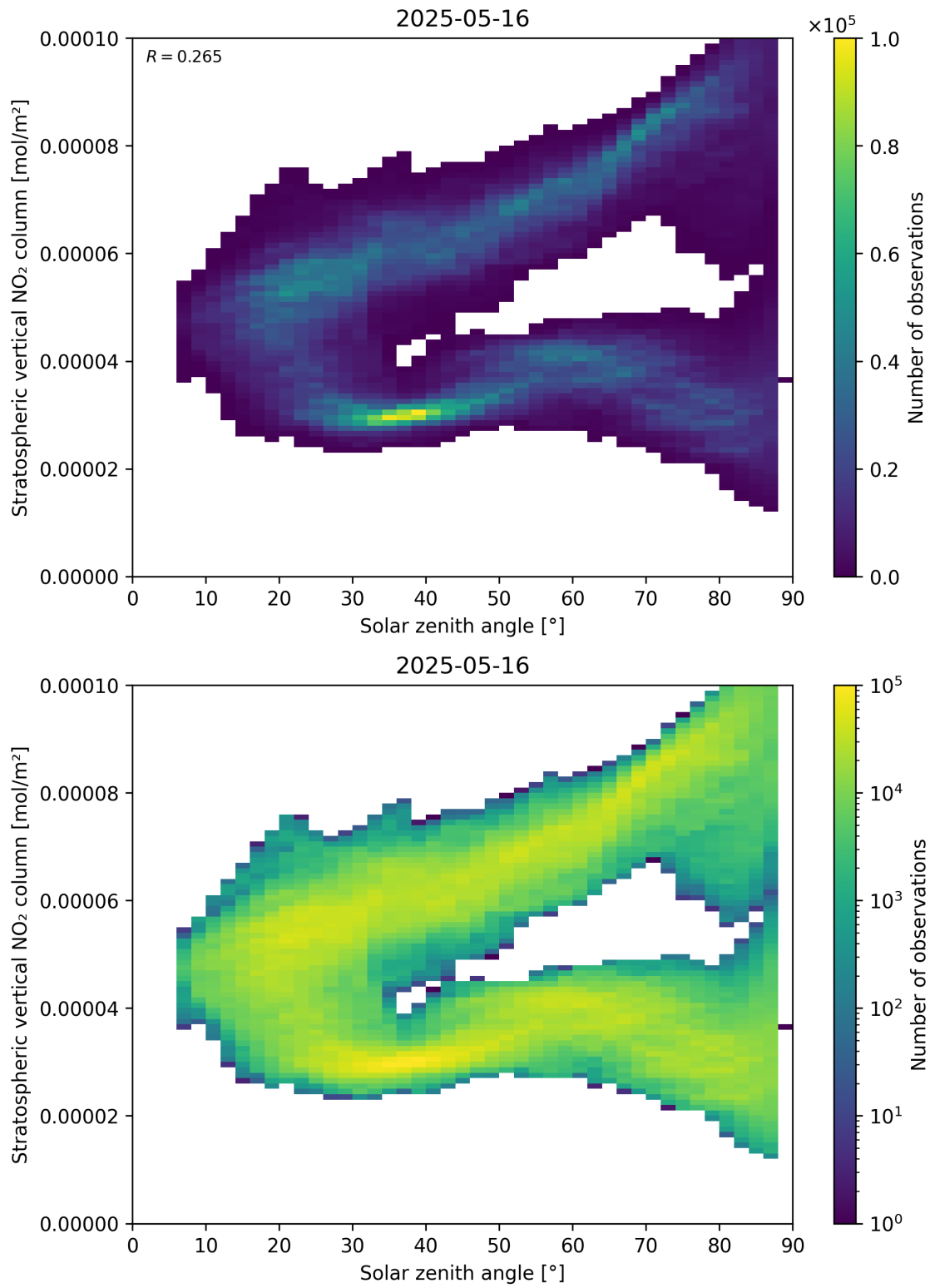
Figure 150: Scatter density plot of “Solar zenith angle” against “Stratospheric vertical \text{NO}_2 column” for 2025-05-15 to 2025-05-17.
