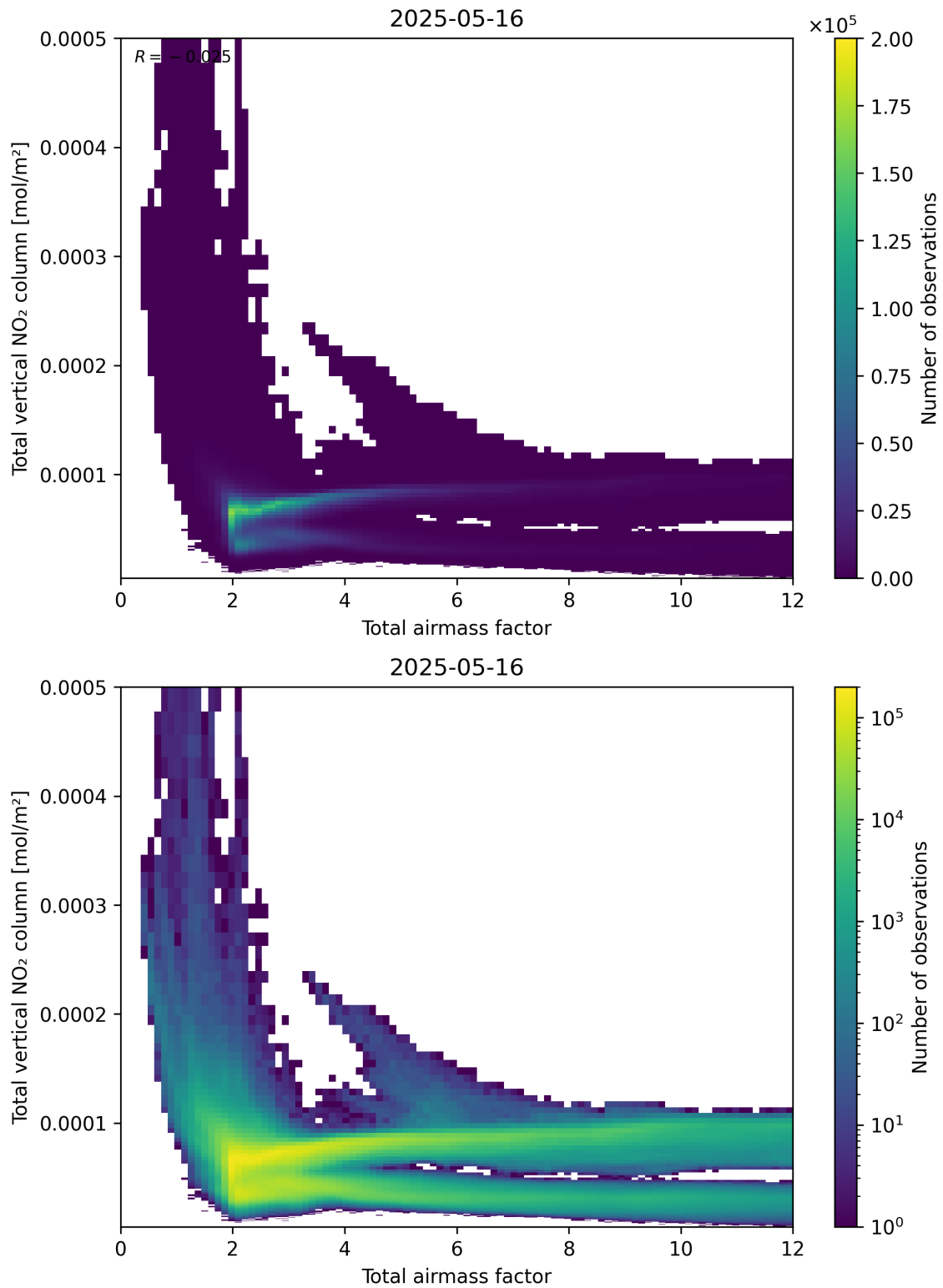
Figure 67: Scatter density plot of “Total airmass factor” against “Total vertical NO 2 column” for 2025-05-15 to 2025-05-17.
