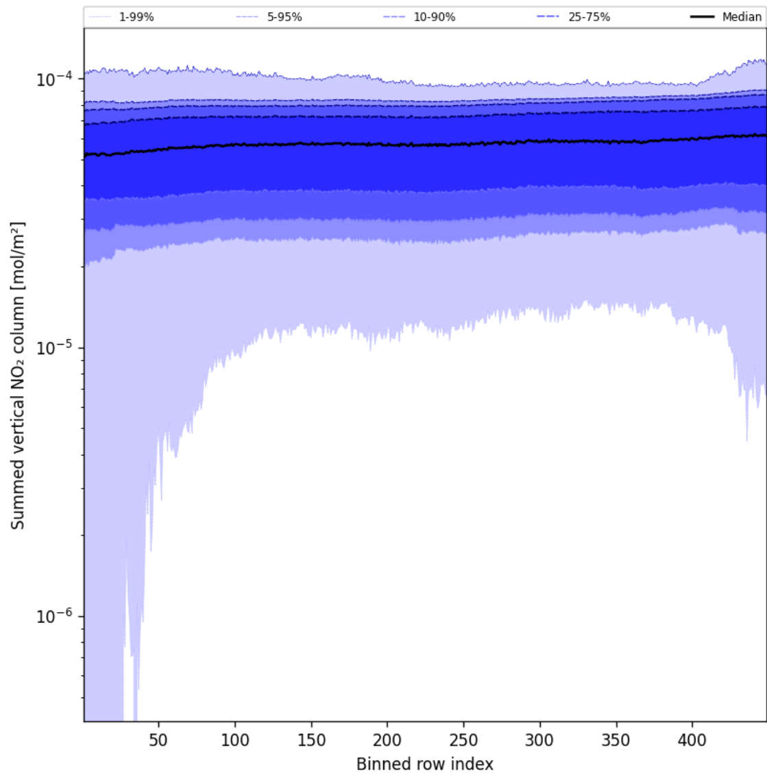
Figure 57: Along track statistics of “Summed vertical NO 2 column” for 2025-05-15 to 2025-05-17
