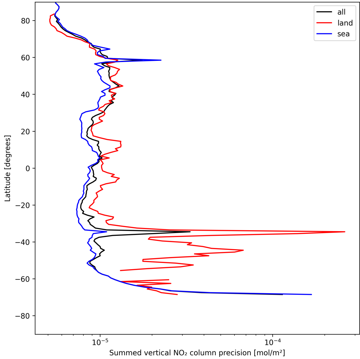
Figure 24: Zonal average of “Summed vertical NO 2 column precision” for 2025-05-15 to 2025-05-17.
