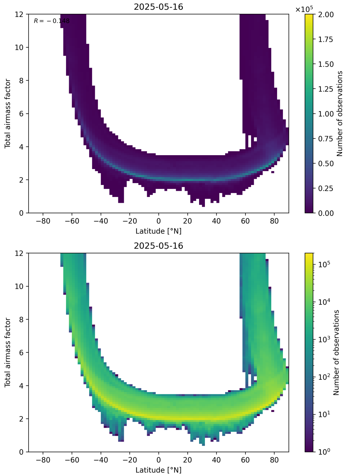
Figure 84: Scatter density plot of “Latitude” against “Total airmass factor” for 2025-05-15 to 2025-05-17.
