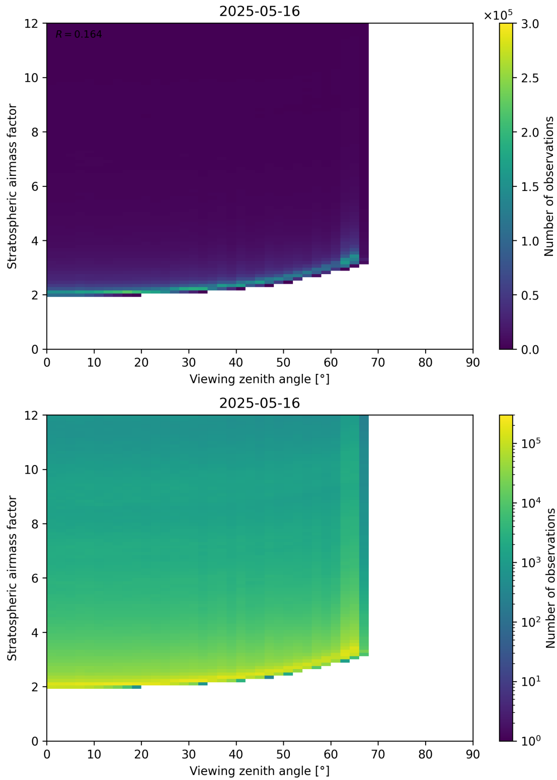
Figure 159: Scatter density plot of “Viewing zenith angle” against “Stratospheric airmass factor” for 2025-05-15 to 2025-05-17.
