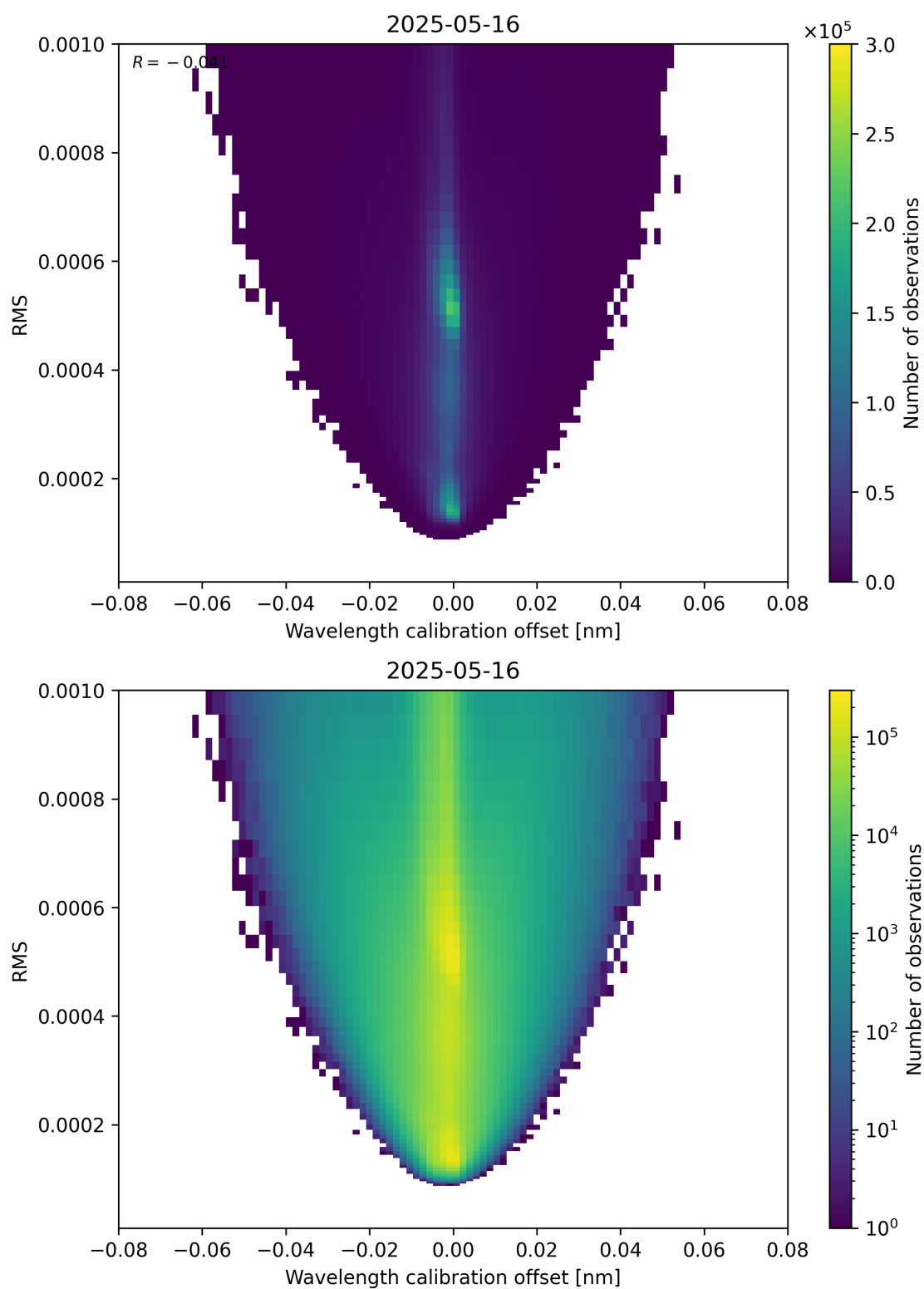
Figure 181: Scatter density plot of “Wavelength calibration offset” against “RMS” for 2025-05-15 to 2025-05-17.
