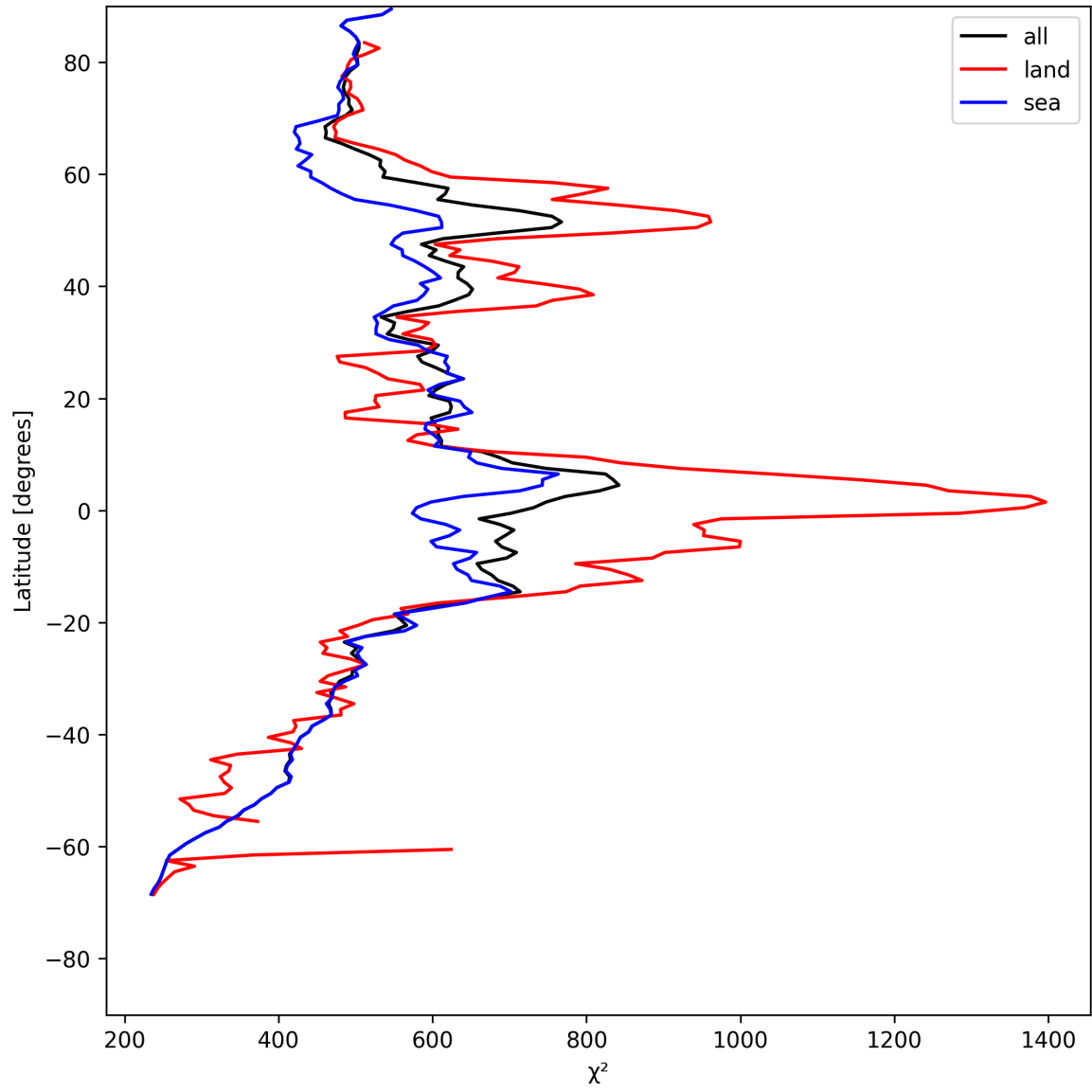
Figure 25: Zonal average of “ \chi^2 ” for 2025-05-15 to 2025-05-17.
