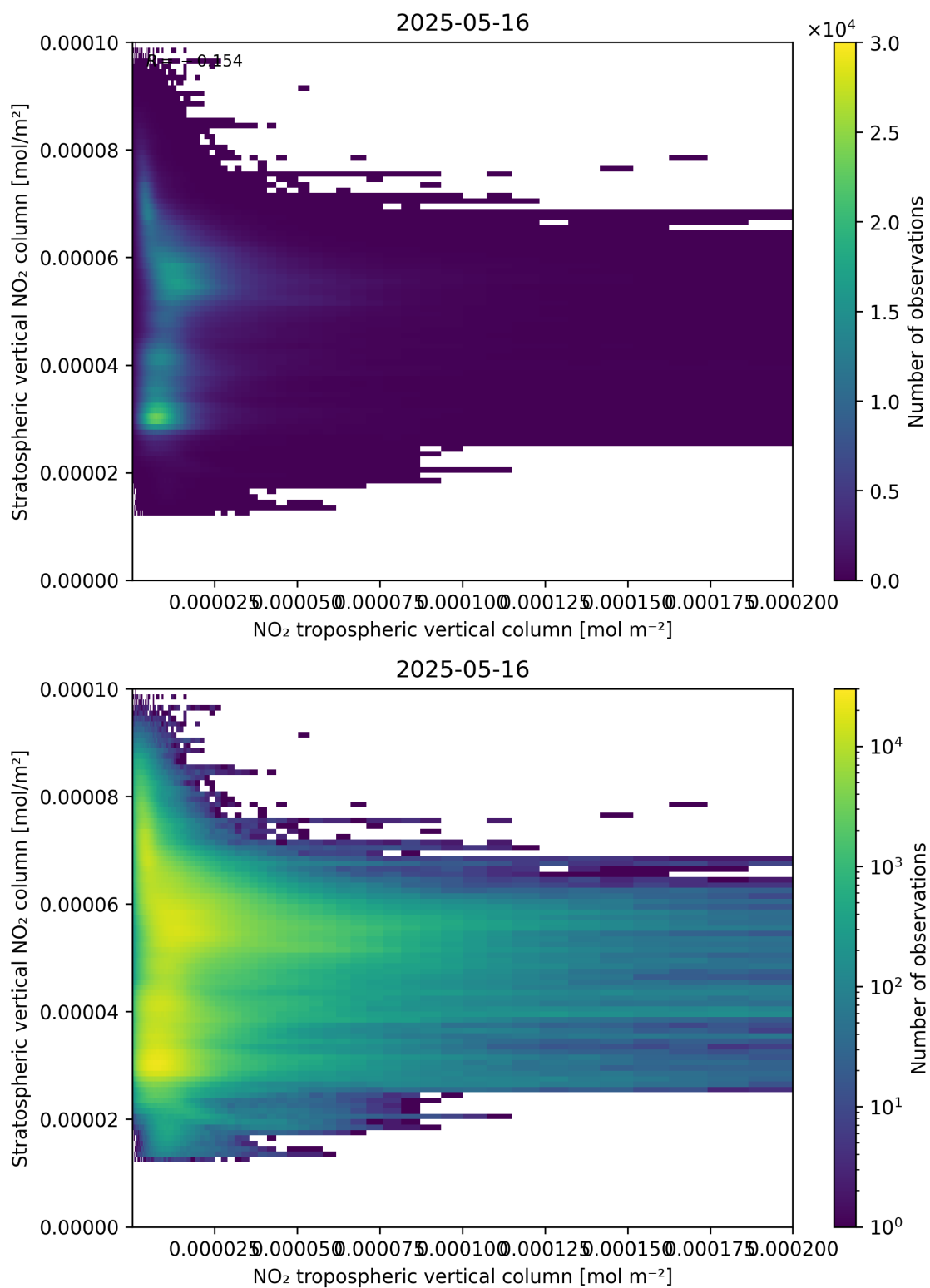
Figure 125: Scatter density plot of “NO 2 tropospheric vertical column” against “Stratospheric vertical NO 2 column” for 2025-05-15 to 2025-05-17.
