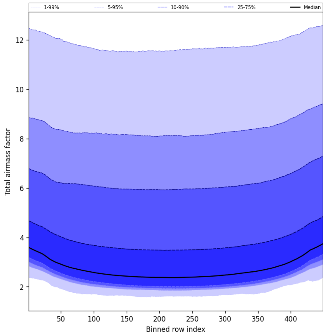
Figure 49: Along track statistics of “Total airmass factor” for 2025-05-15 to 2025-05-17
