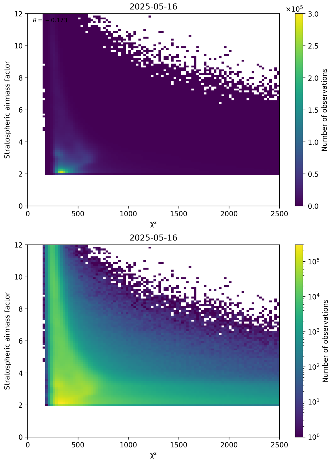
Figure 81: Scatter density plot of “ \chi^2 ” against “Stratospheric airmass factor” for 2025-05-15 to 2025-05-17.
