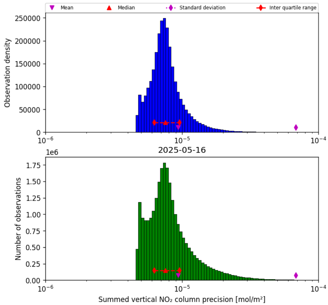
Figure 41: Histogram of “Summed vertical NO 2 column precision” for 2025-05-15 to 2025-05-17
