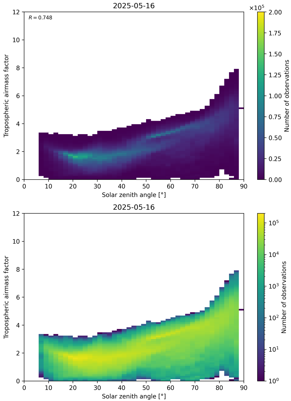
Figure 147: Scatter density plot of “Solar zenith angle” against “Tropospheric airmass factor” for 2025-05-15 to 2025-05-17.
