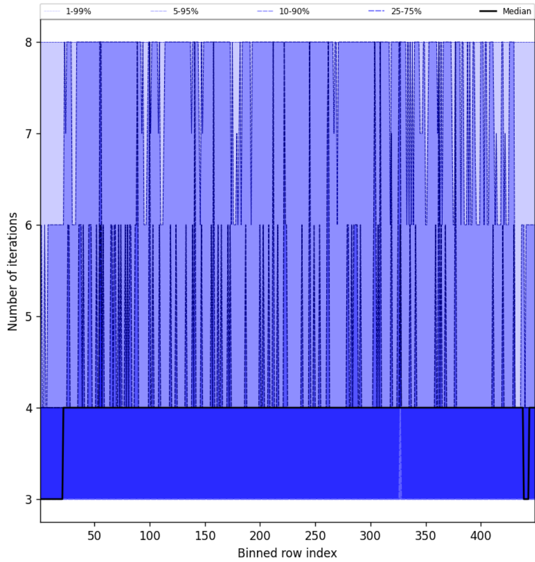
Figure 51: Along track statistics of “Number of iterations” for 2025-05-15 to 2025-05-17
