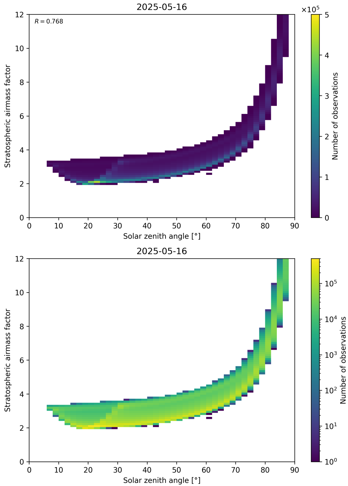
Figure 145: Scatter density plot of “Solar zenith angle” against “Stratospheric airmass factor” for 2025-05-15 to 2025-05-17.
