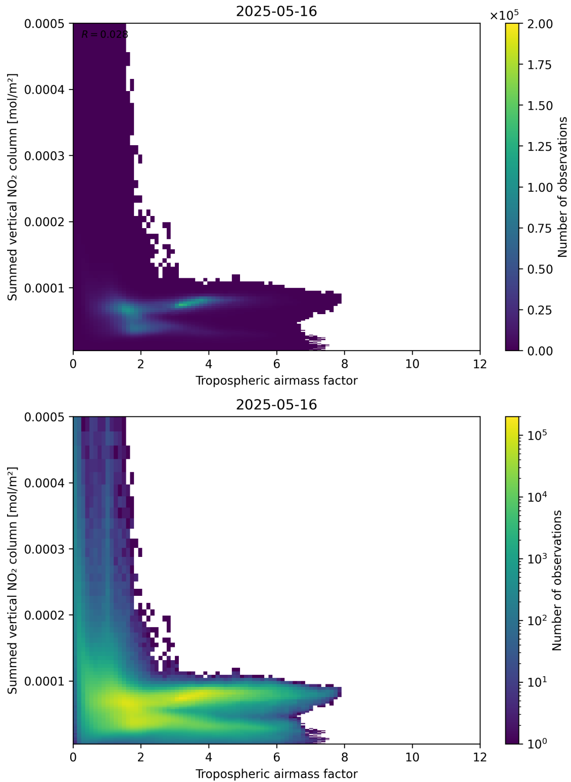
Figure 75: Scatter density plot of “Tropospheric air mass factor” against “Summed vertical NO 2 column” for 2025-05-15 to 2025-05-17.
