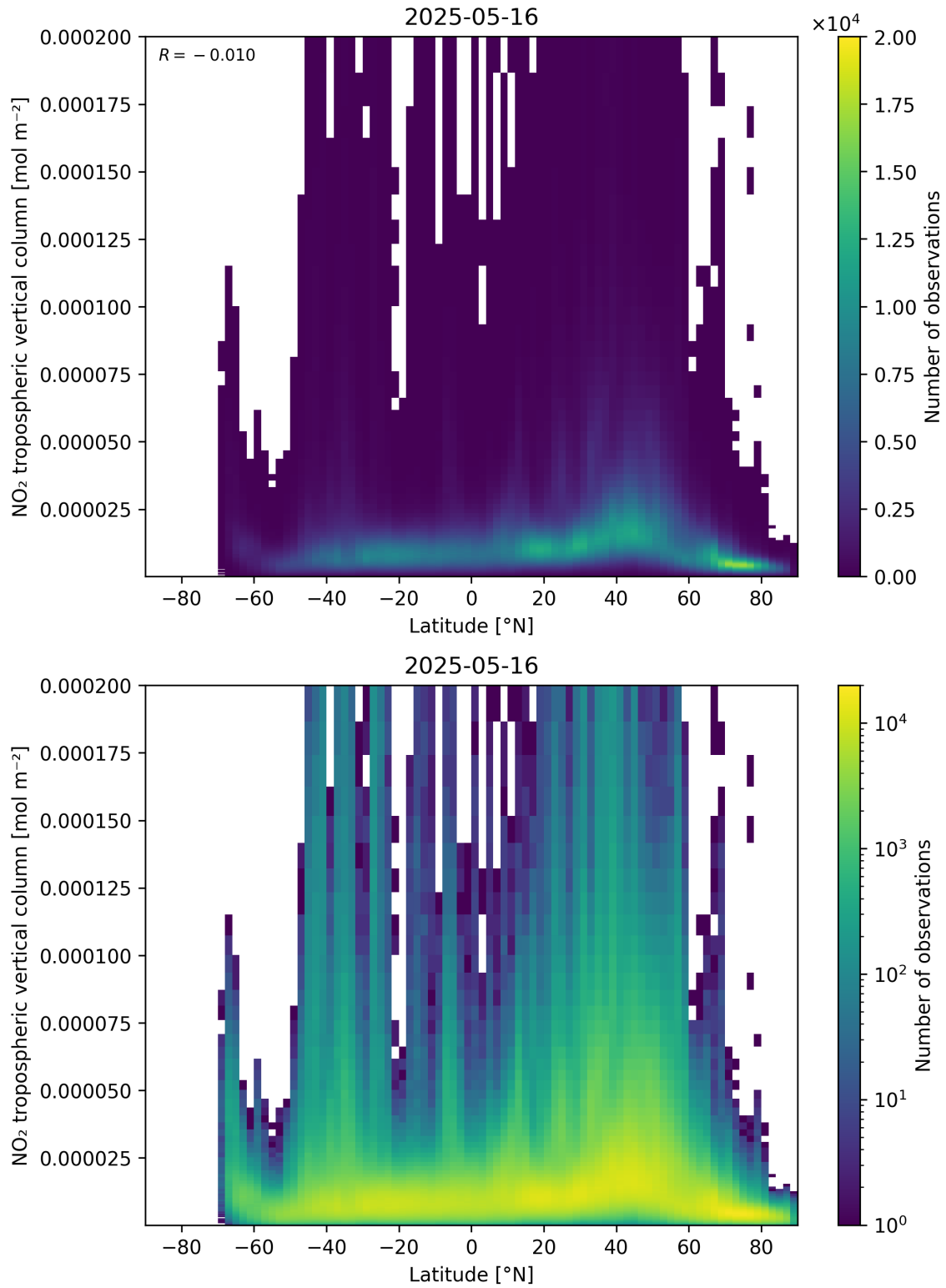
Figure 92: Scatter density plot of “Latitude” against “NO 2 tropospheric vertical column” for 2025-05-15 to 2025-05-17.
