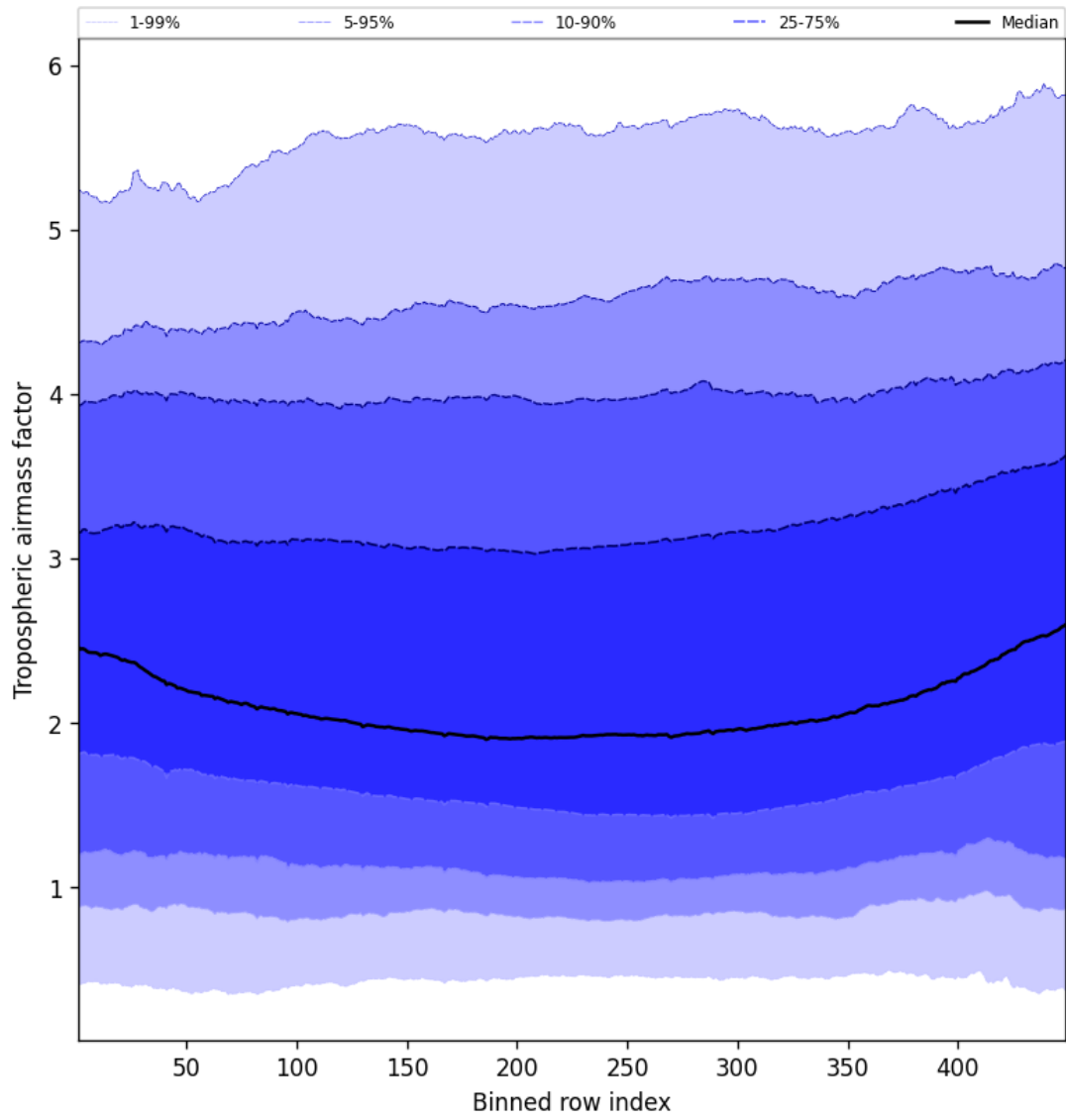
Figure 48: Along track statistics of “Tropospheric airmass factor” for 2025-05-15 to 2025-05-17
