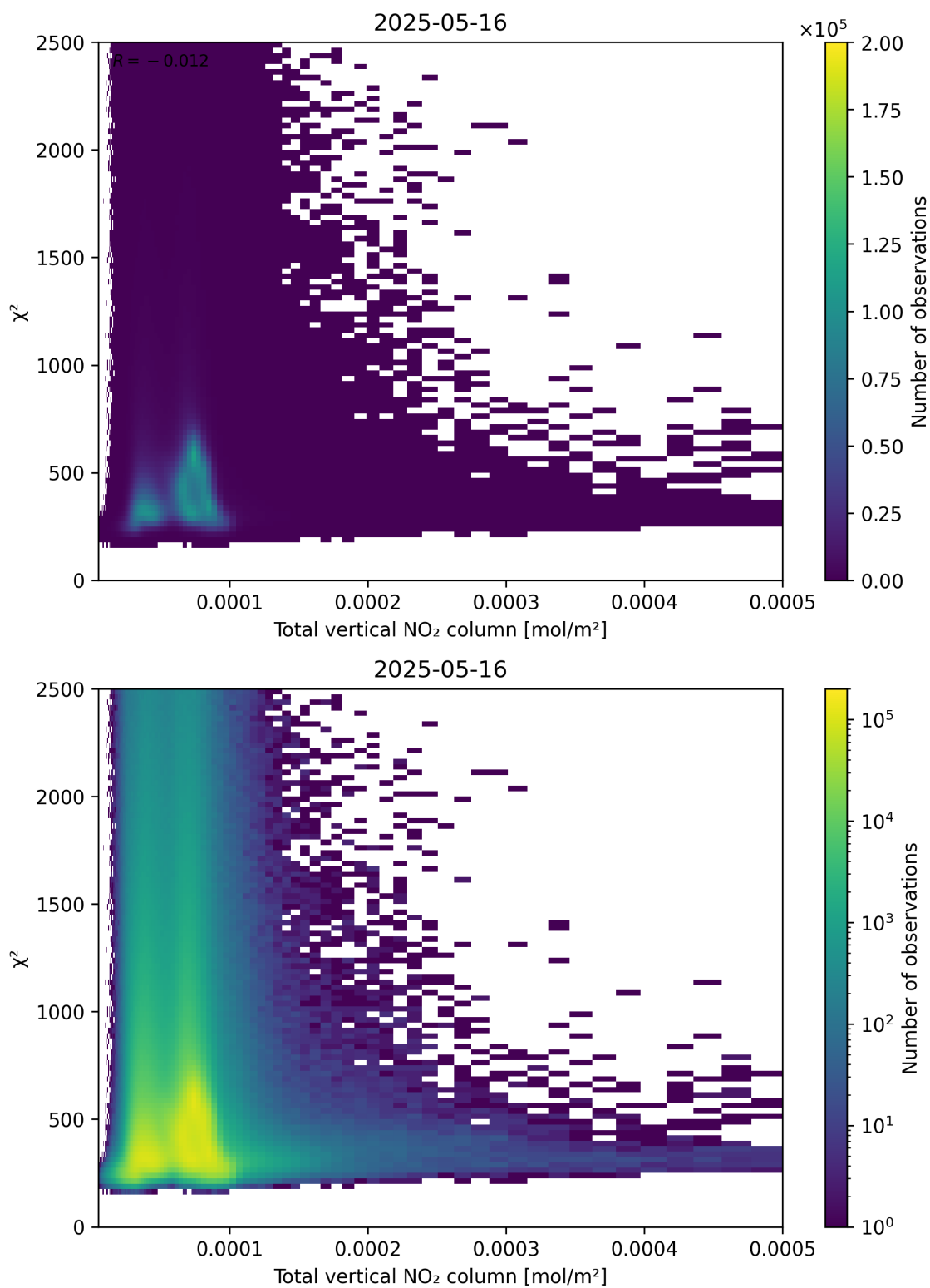
Figure 111: Scatter density plot of “Total vertical NO 2 column” against “ \chi^2 ” for 2025-05-15 to 2025-05-17.
