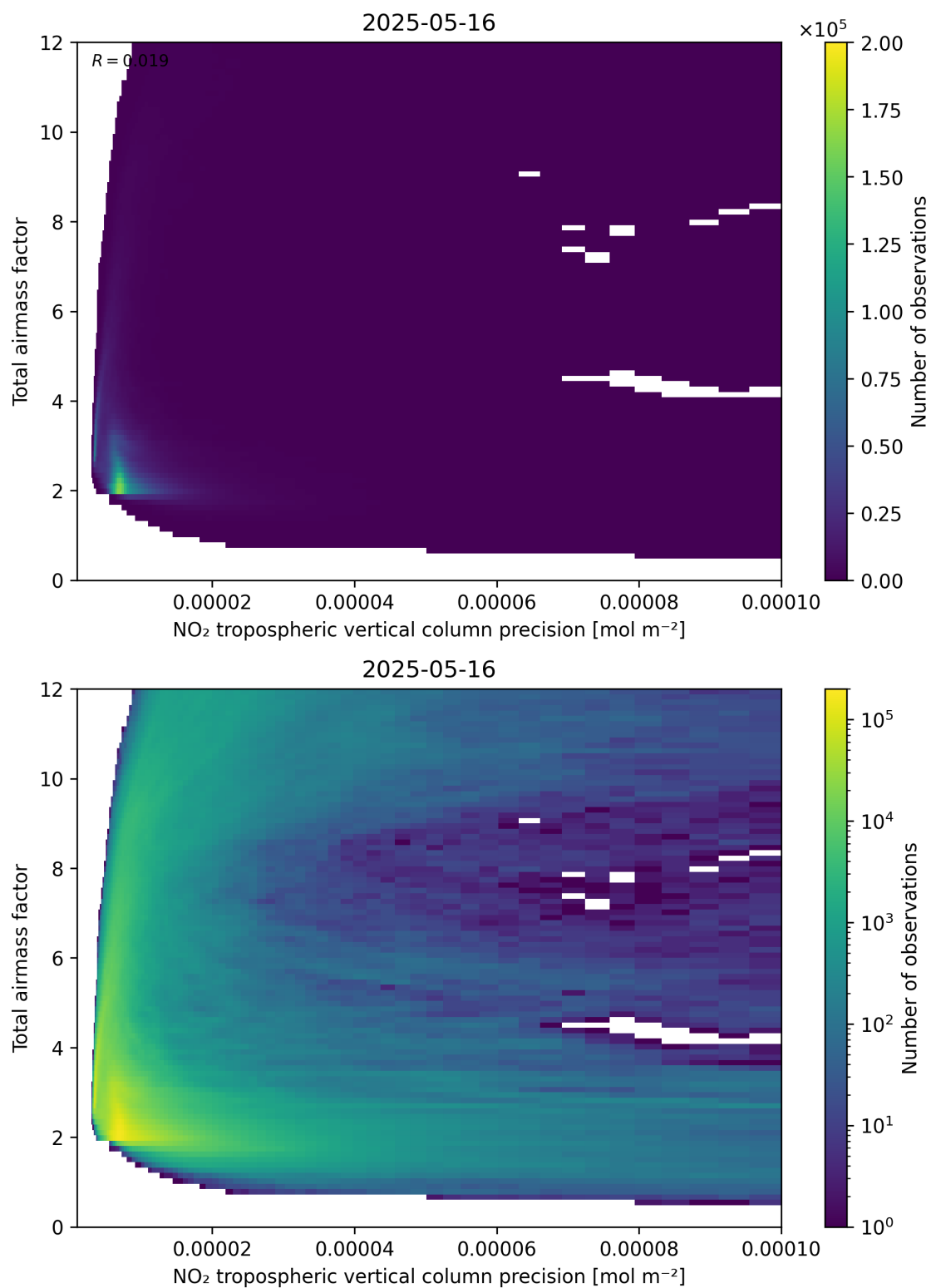
Figure 132: Scatter density plot of “NO 2 tropospheric vertical column precision” against “Total air mass factor” for 2025-05-15 to 2025-05-17.
