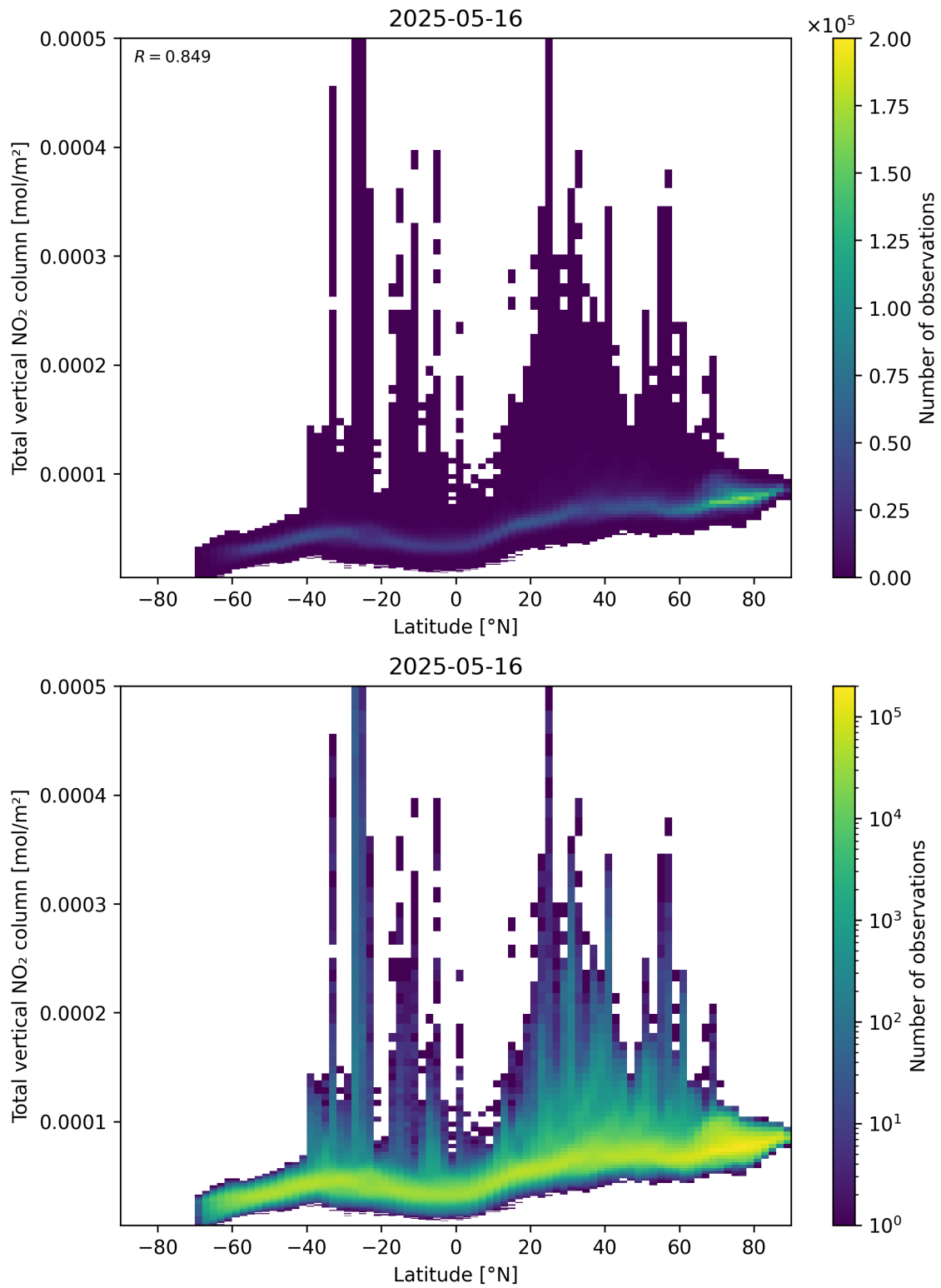
Figure 90: Scatter density plot of “Latitude” against “Total vertical NO 2 column” for 2025-05-15 to 2025-05-17.
