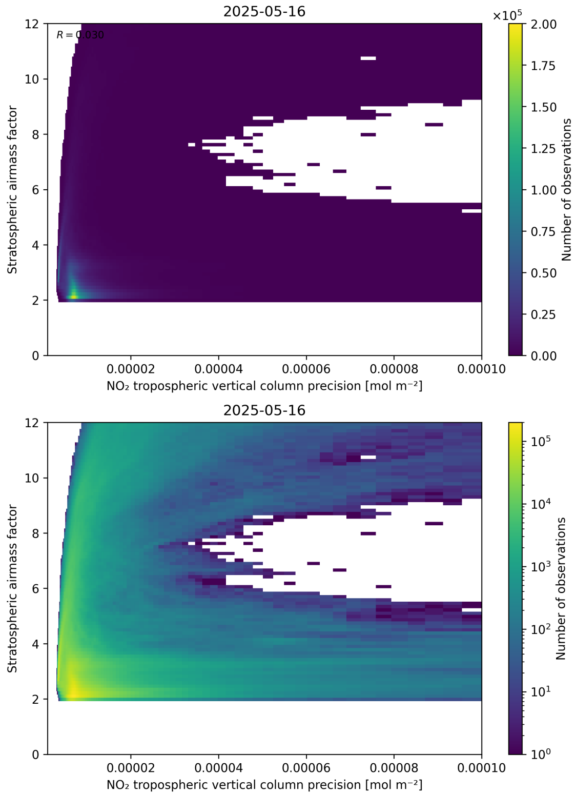
Figure 131: Scatter density plot of “NO 2 tropospheric vertical column precision” against “Stratospheric airmass factor” for 2025-05-15 to 2025-05-17.
