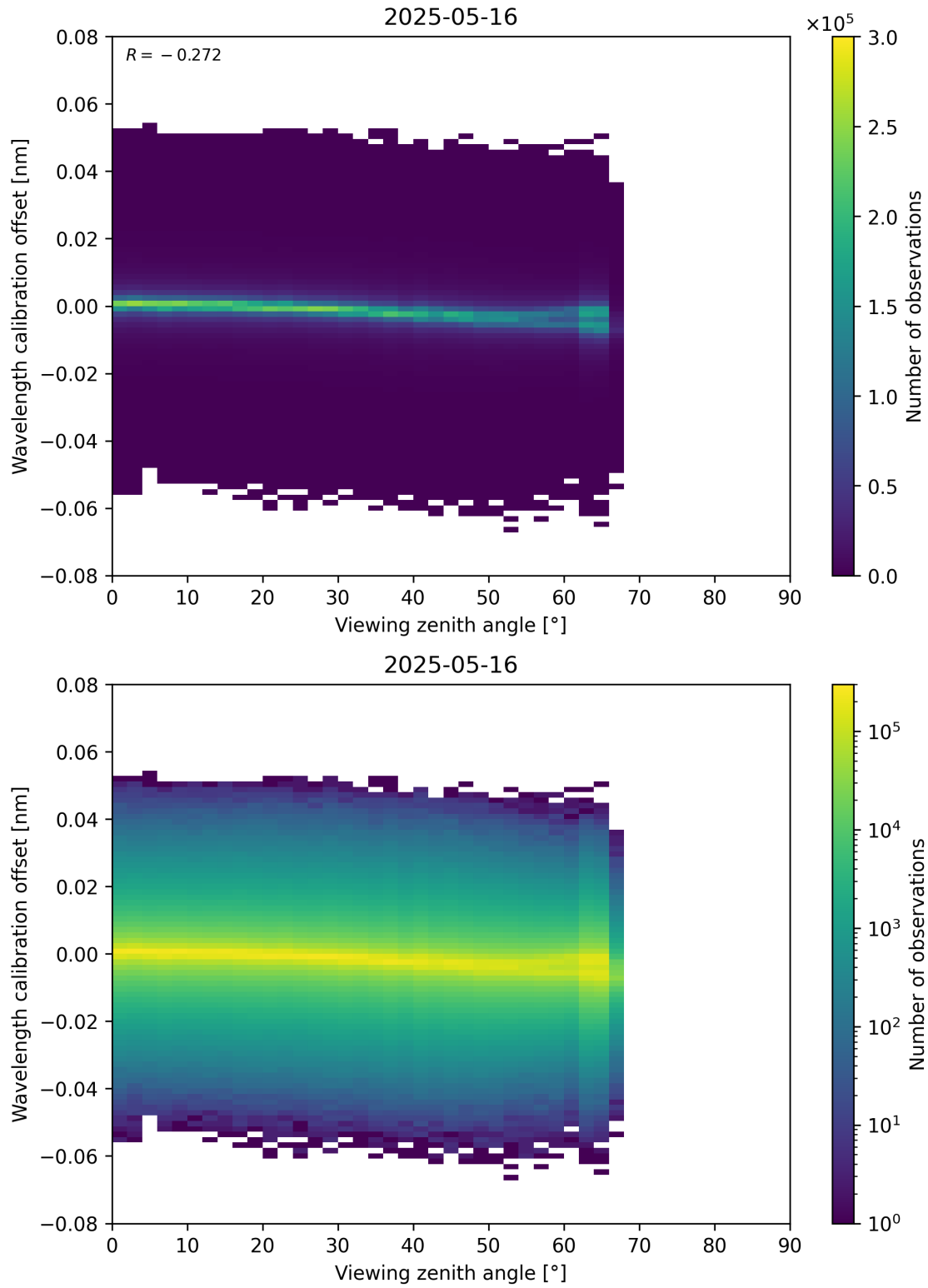
Figure 173: Scatter density plot of “Viewing zenith angle” against “Wavelength calibration offset” for 2025-05-15 to 2025-05-17.
