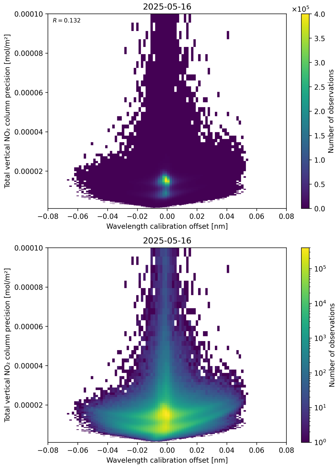
Figure 180: Scatter density plot of “Wavelength calibration offset” against “Total vertical NO 2 column precision” for 2025-05-15 to 2025-05-17.
