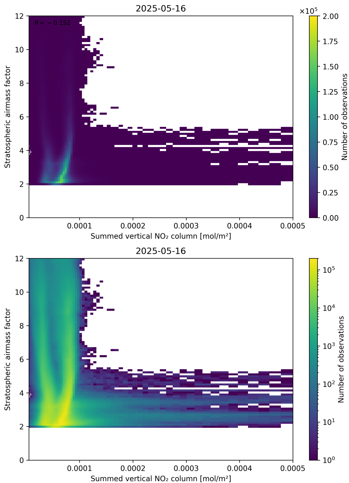
Figure 103: Scatter density plot of “Summed vertical NO 2 column” against “Stratospheric airmass factor” for 2025-05-15 to 2025-05-17.
