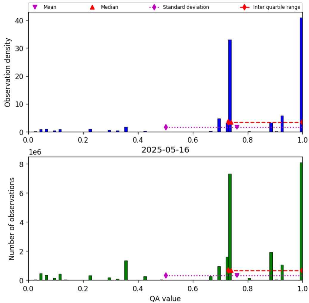
Figure 28: Histogram of “QA value” for 2025-05-15 to 2025-05-17
