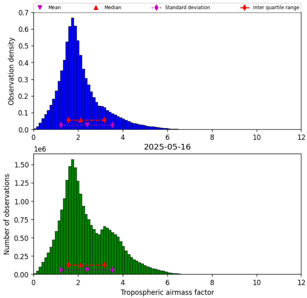
Figure 31: Histogram of “Tropospheric airmass factor” for 2025-05-15 to 2025-05-17
