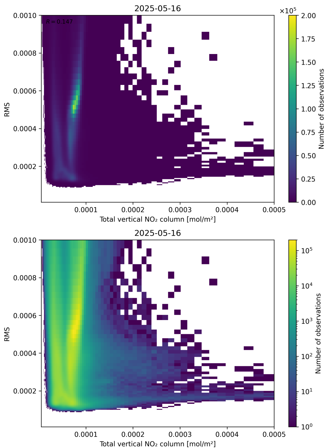
Figure 120: Scatter density plot of “Total vertical NO 2 column” against “RMS” for 2025-05-15 to 2025-05-17.
