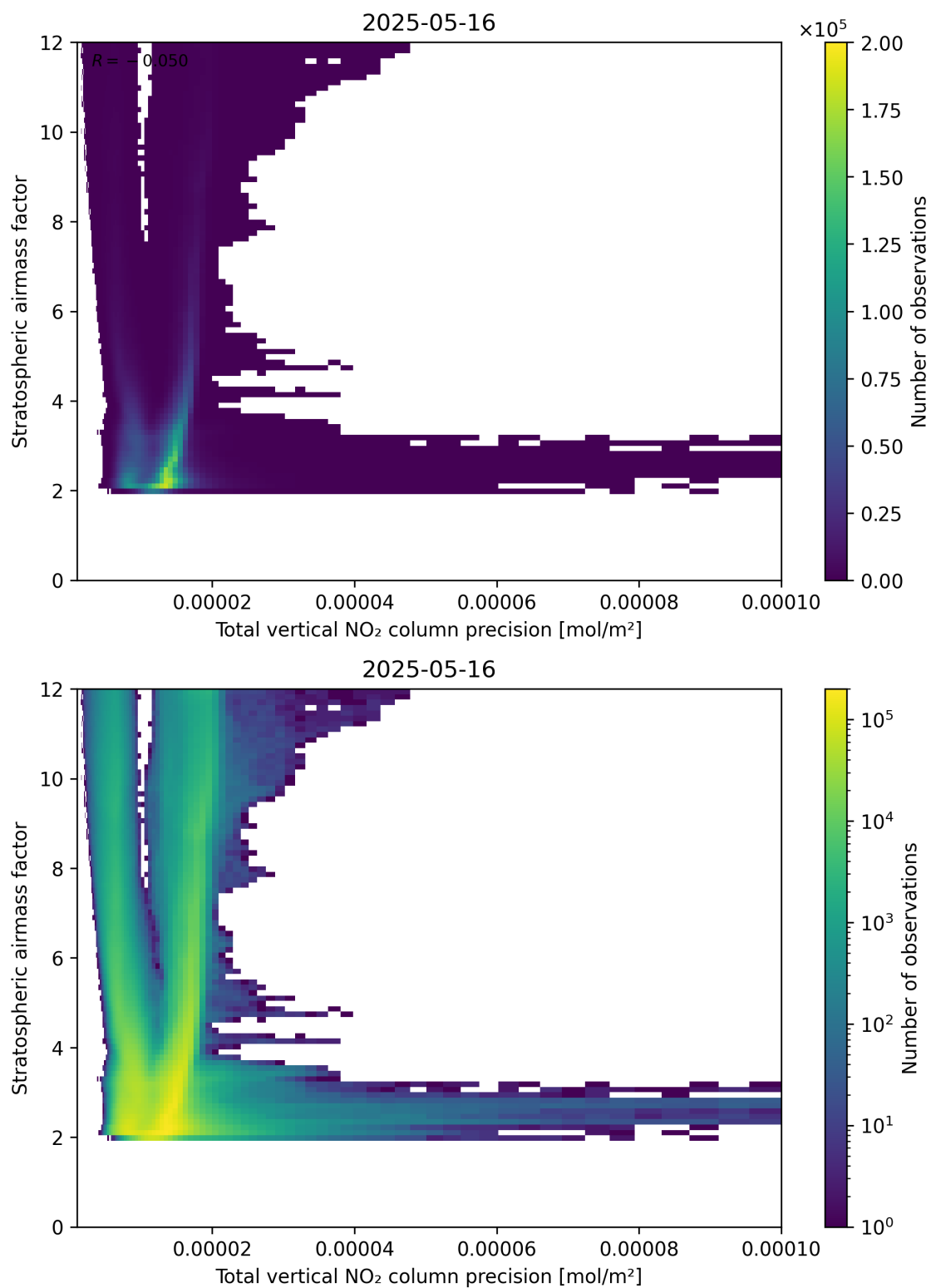
Figure 115: Scatter density plot of “Total vertical NO 2 column precision” against “Stratospheric airmass factor” for 2025-05-15 to 2025-05-17.
