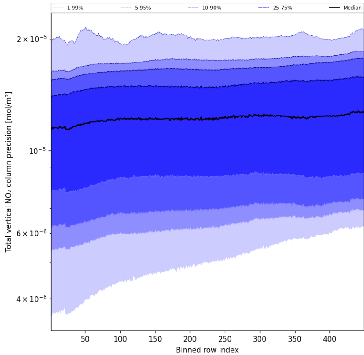
Figure 56: Along track statistics of "Total vertical NO 2 column precision" for 2025-05-15 to 2025-05-17
