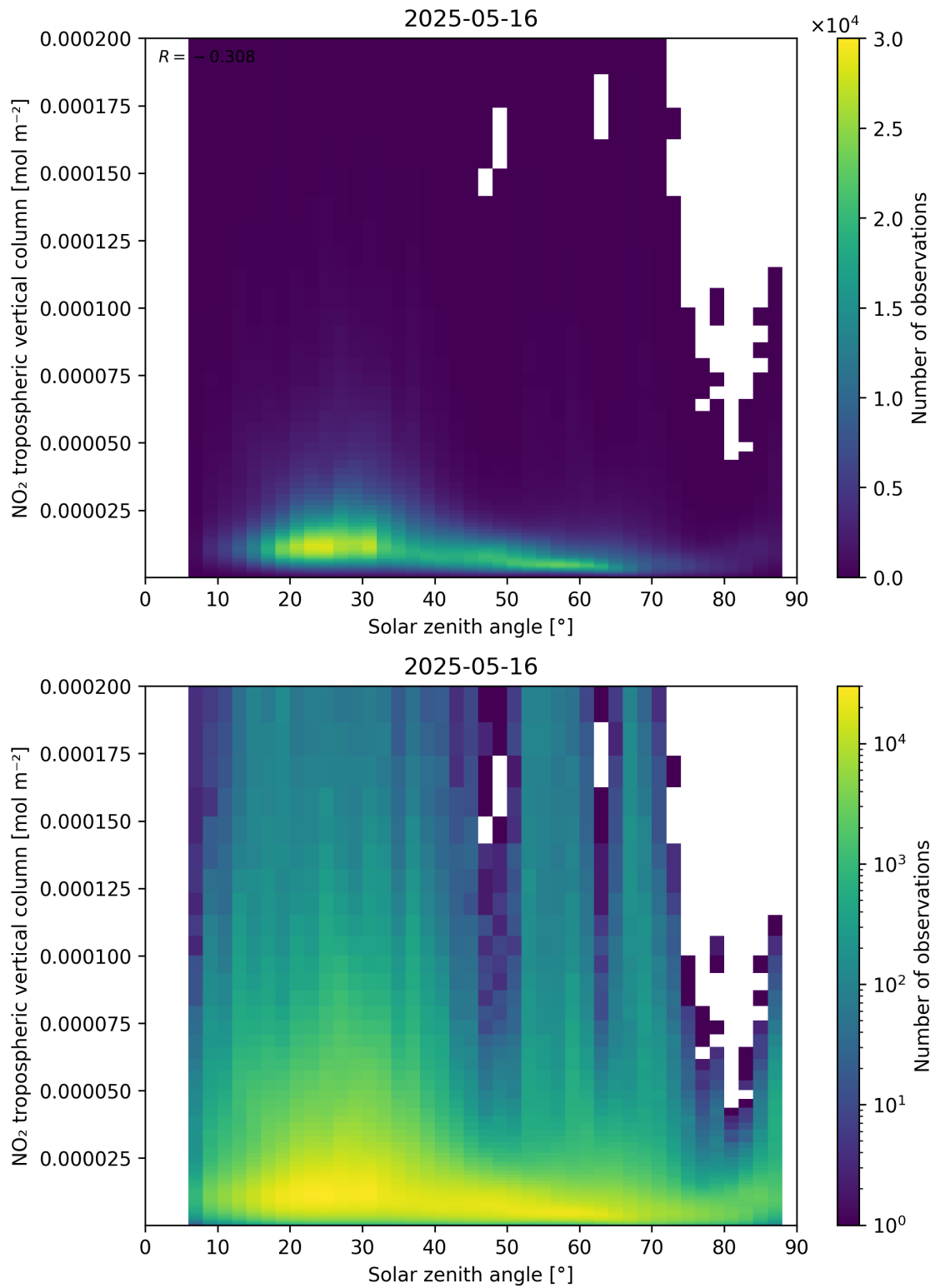
Figure 155: Scatter density plot of “Solar zenith angle” against “NO 2 tropospheric vertical column” for 2025-05-15 to 2025-05-17.
