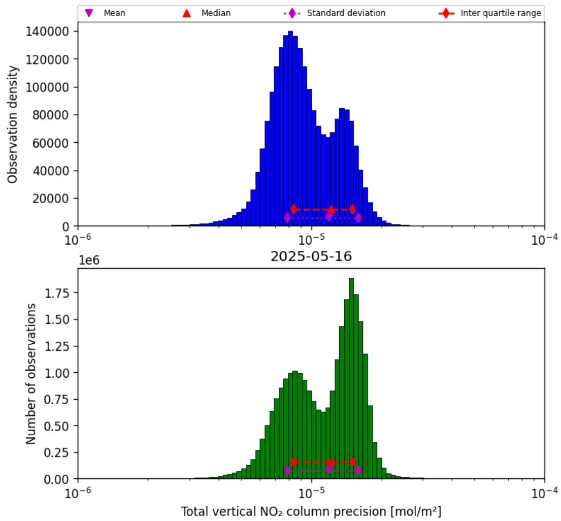
Figure 39: Histogram of “Total vertical NO 2 column precision” for 2025-05-15 to 2025-05-17
