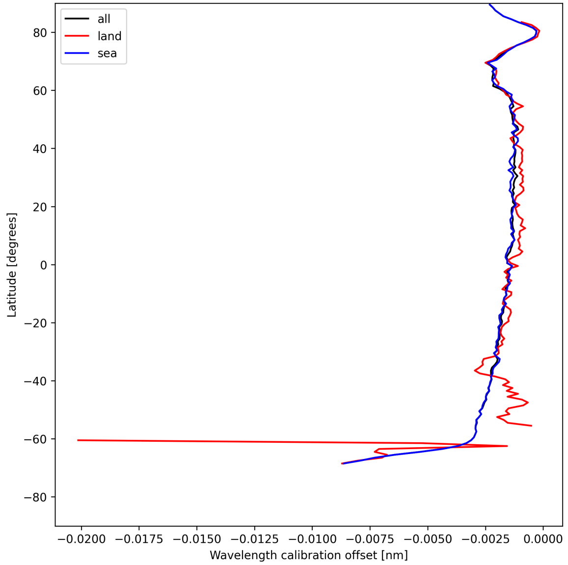
Figure 18: Zonal average of “Wavelength calibration offset” for 2025-05-15 to 2025-05-17.
