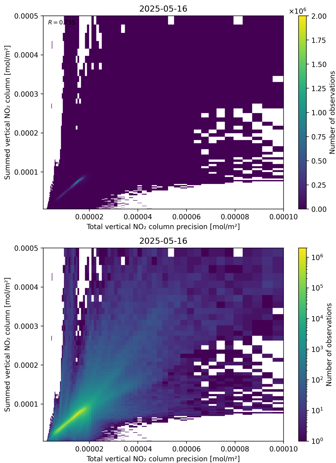
Figure 117: Scatter density plot of “Total vertical NO 2 column precision” against “Summed vertical NO 2 column” for 2025-05-15 to 2025-05-17.
