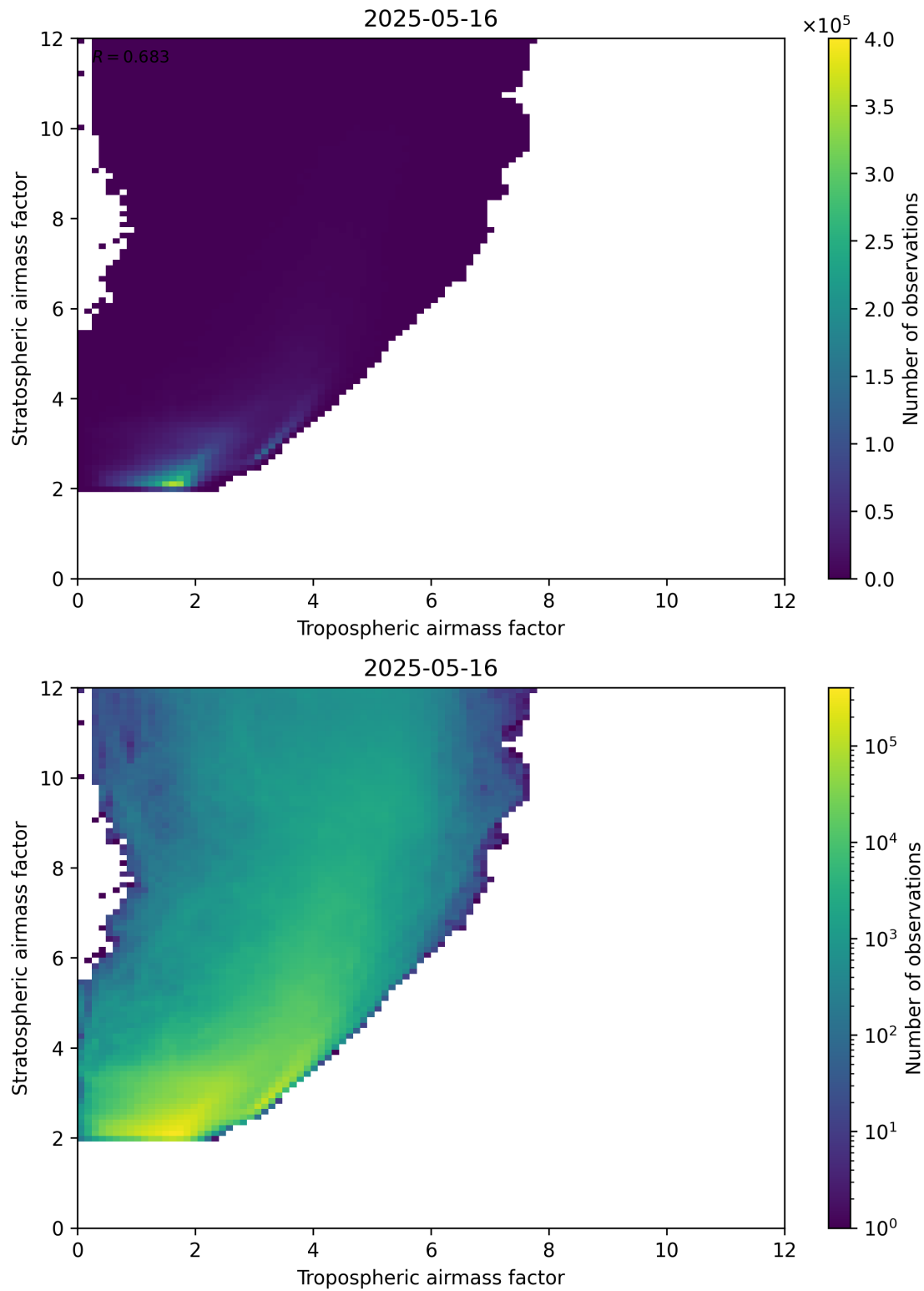
Figure 71: Scatter density plot of “Tropospheric airmass factor” against “Stratospheric airmass factor” for 2025-05-15 to 2025-05-17.
