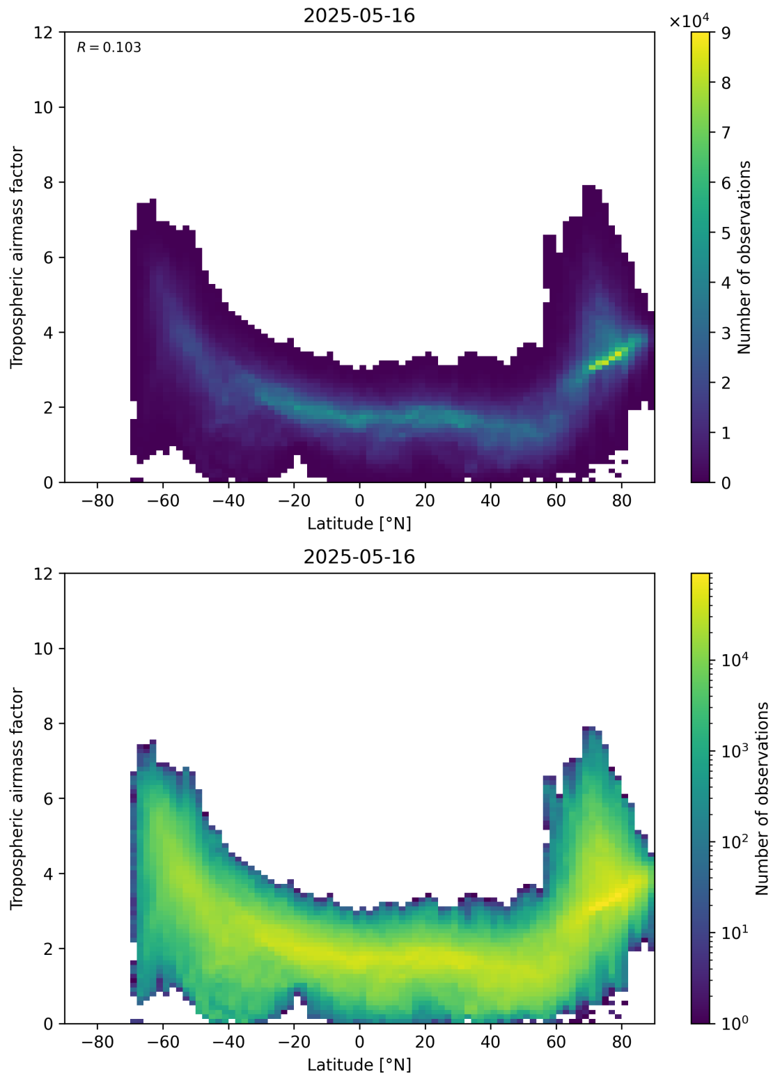
Figure 85: Scatter density plot of “Latitude” against “Tropospheric airmass factor” for 2025-05-15 to 2025-05-17.
