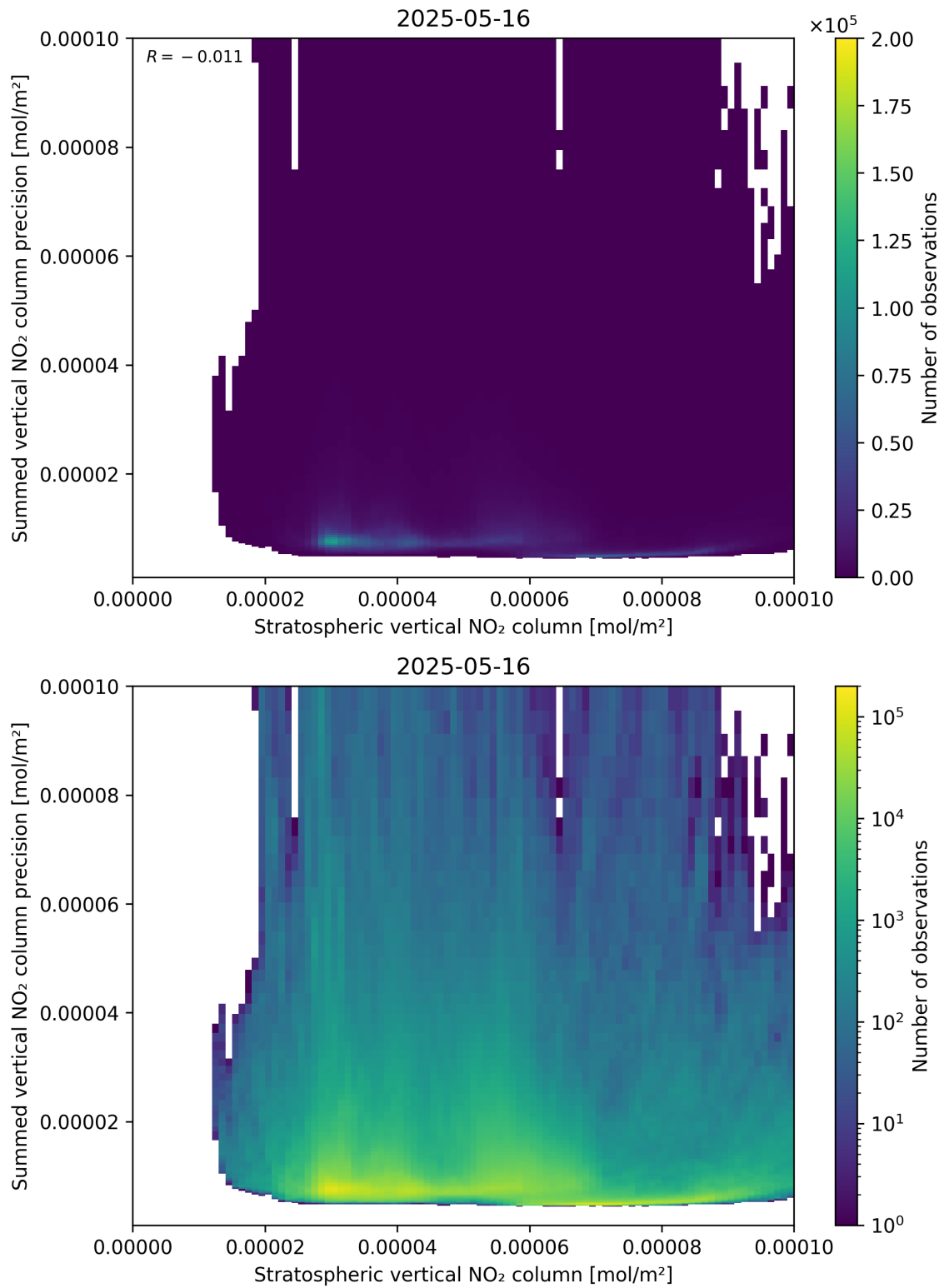
Figure 99: Scatter density plot of “Stratospheric vertical NO 2 column” against “Summed vertical NO 2 column precision” for 2025-05-15 to 2025-05-17.
