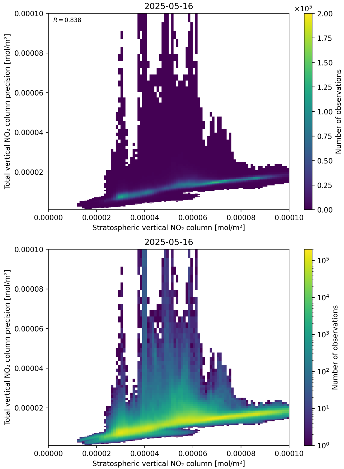
Figure 101: Scatter density plot of “Stratospheric vertical NO 2 column” against “Total vertical NO 2 column precision” for 2025-05-15 to 2025-05-17.
