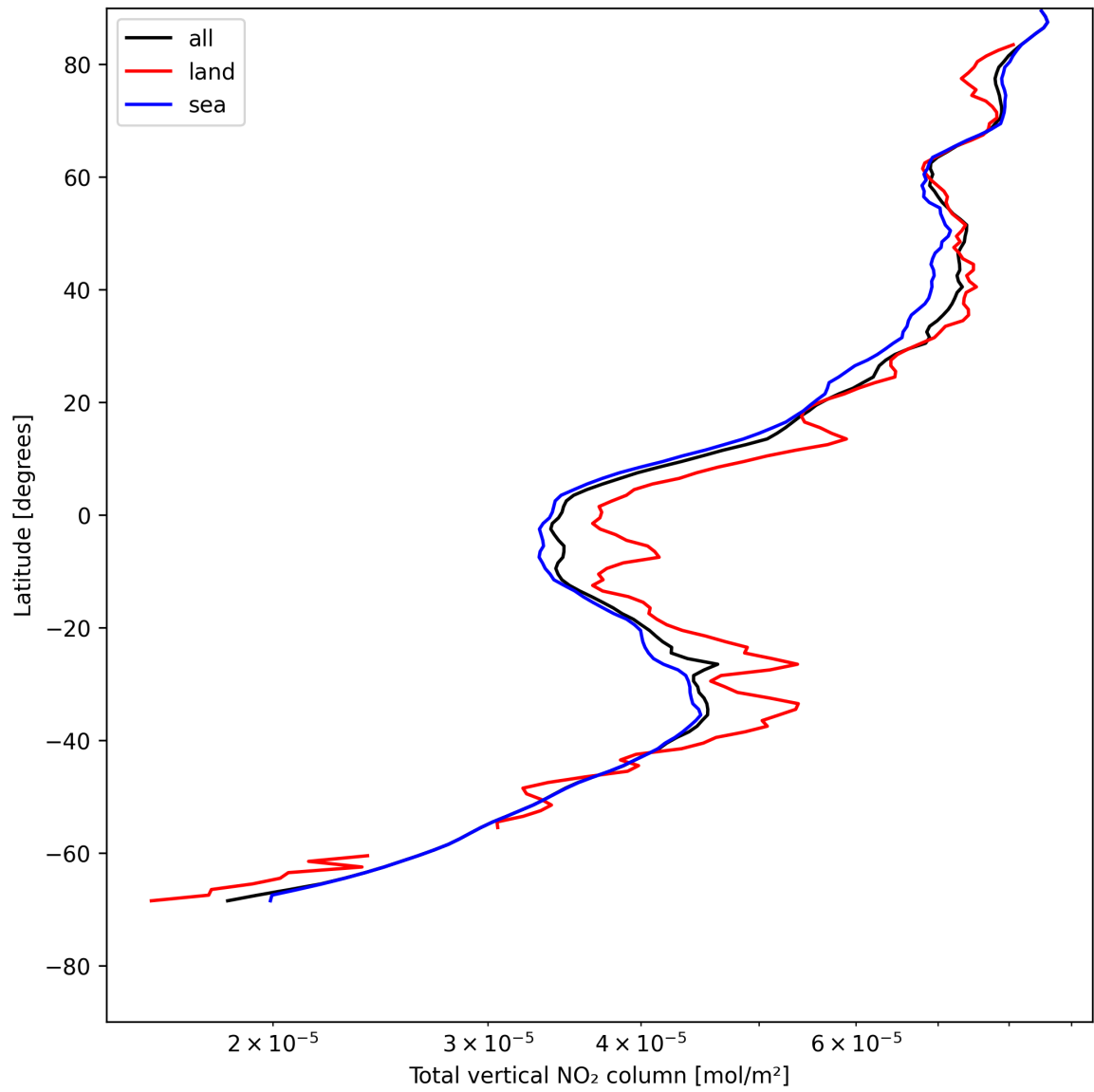
Figure 21: Zonal average of “Total vertical NO 2 column” for 2025-05-15 to 2025-05-17.
