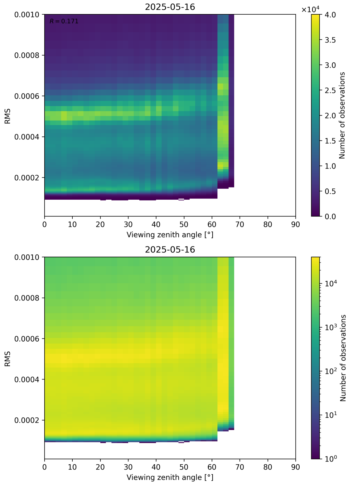
Figure 171: Scatter density plot of “Viewing zenith angle” against “RMS” for 2025-05-15 to 2025-05-17.
