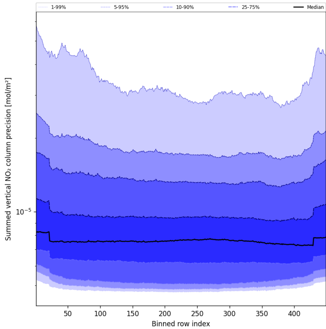
Figure 58: Along track statistics of “Summed vertical NO 2 column precision” for 2025-05-15 to 2025-05-17
