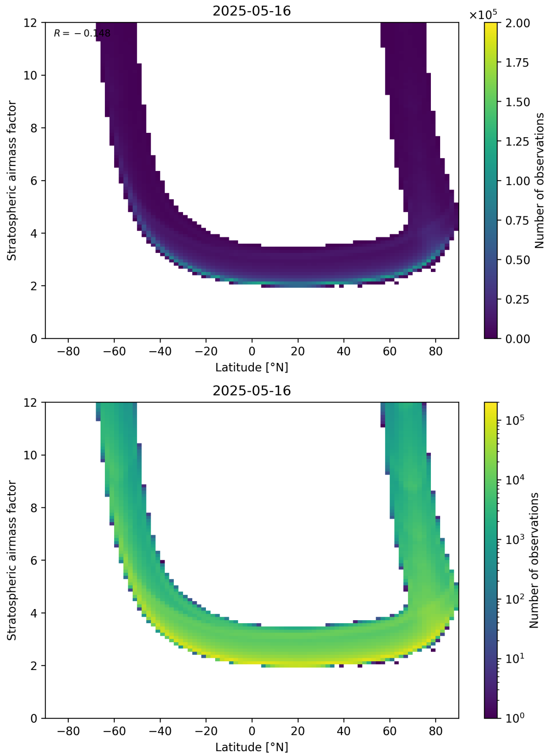
Figure 83: Scatter density plot of “Latitude” against “Stratospheric air mass factor” for 2025-05-15 to 2025-05-17.
