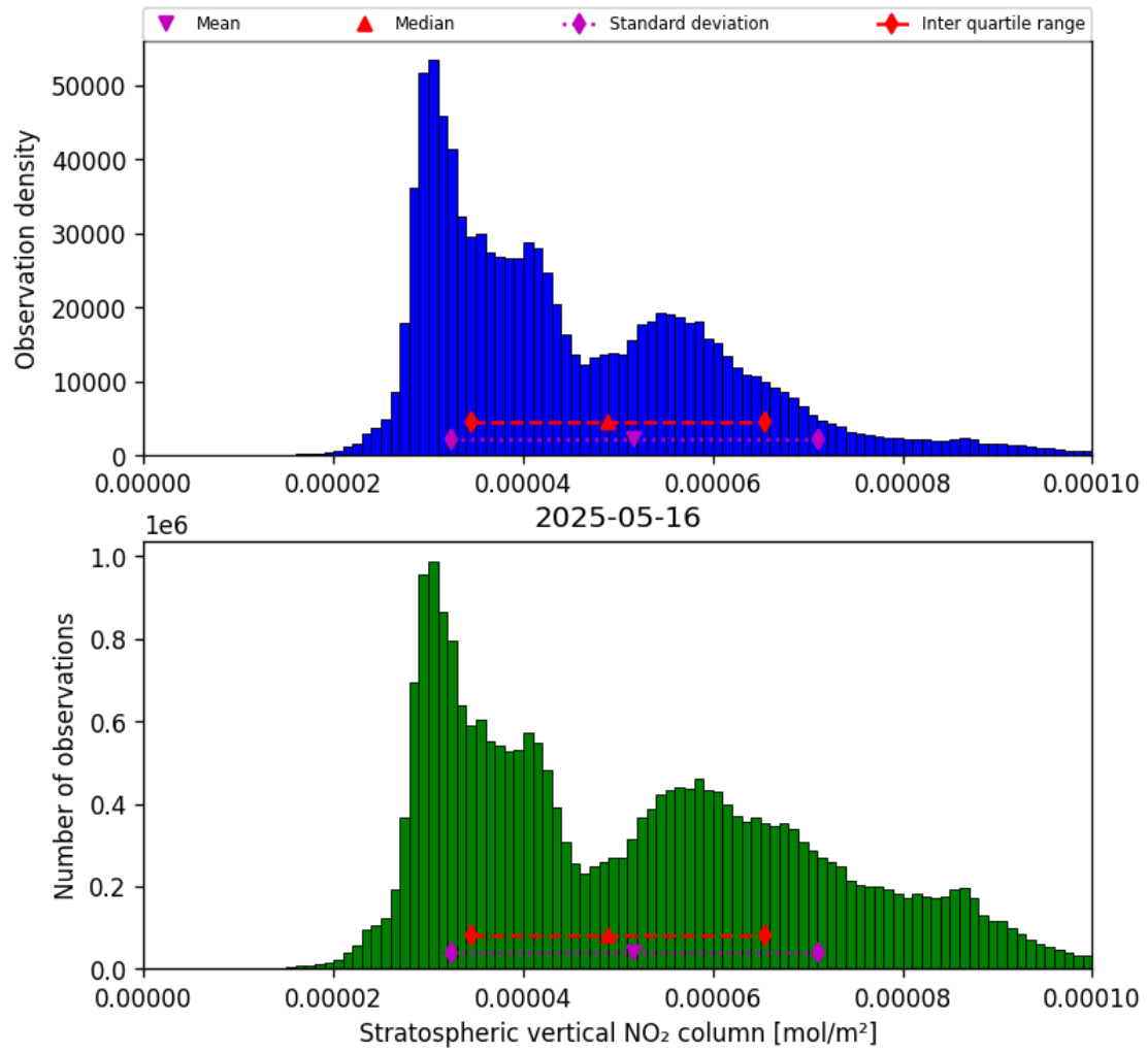
Figure 36: Histogram of “Stratospheric vertical NO 2 column” for 2025-05-15 to 2025-05-17
