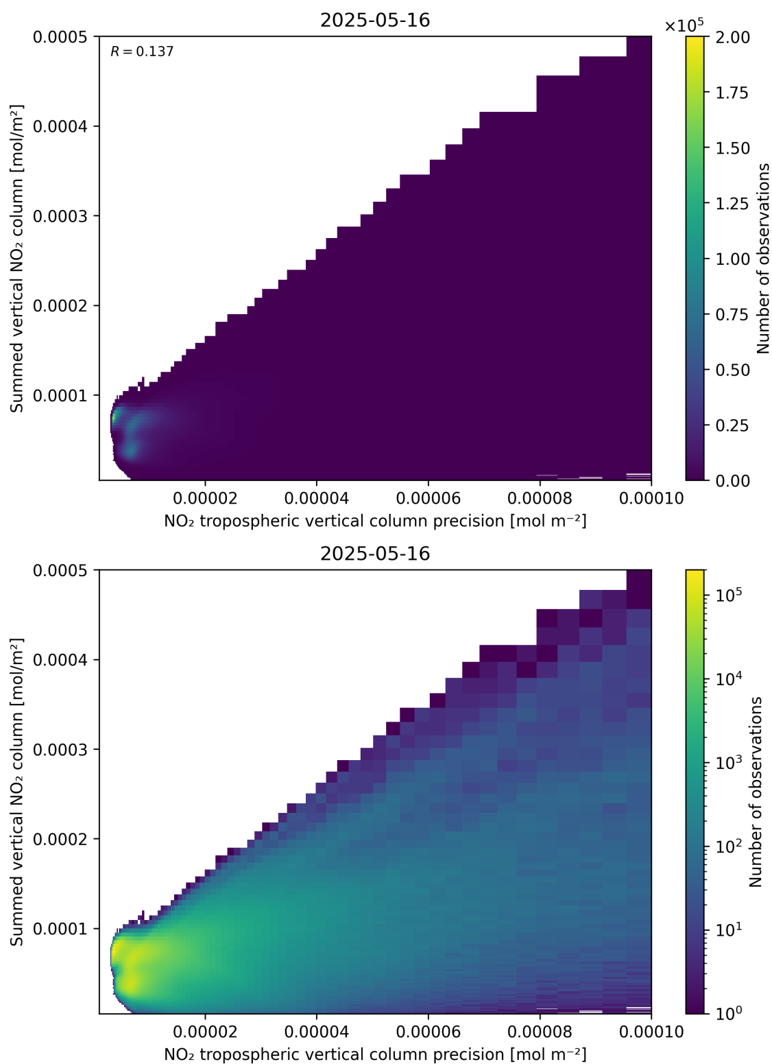
Figure 136: Scatter density plot of “NO 2 tropospheric vertical column precision” against “Summed vertical NO 2 column” for 2025-05-15 to 2025-05-17.
