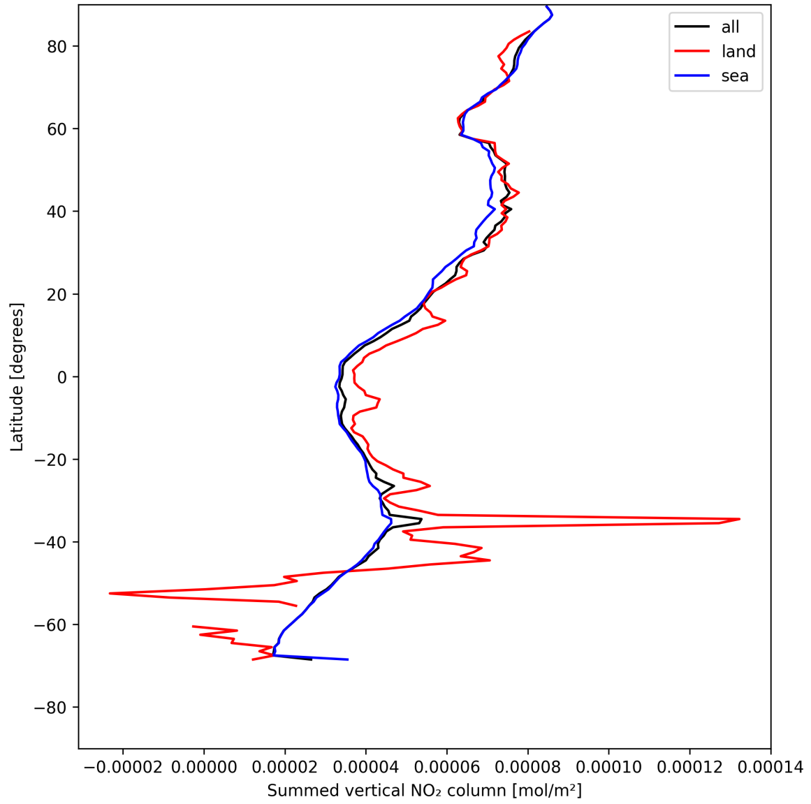
Figure 23: Zonal average of “Summed vertical NO 2 column” for 2025-05-15 to 2025-05-17.
