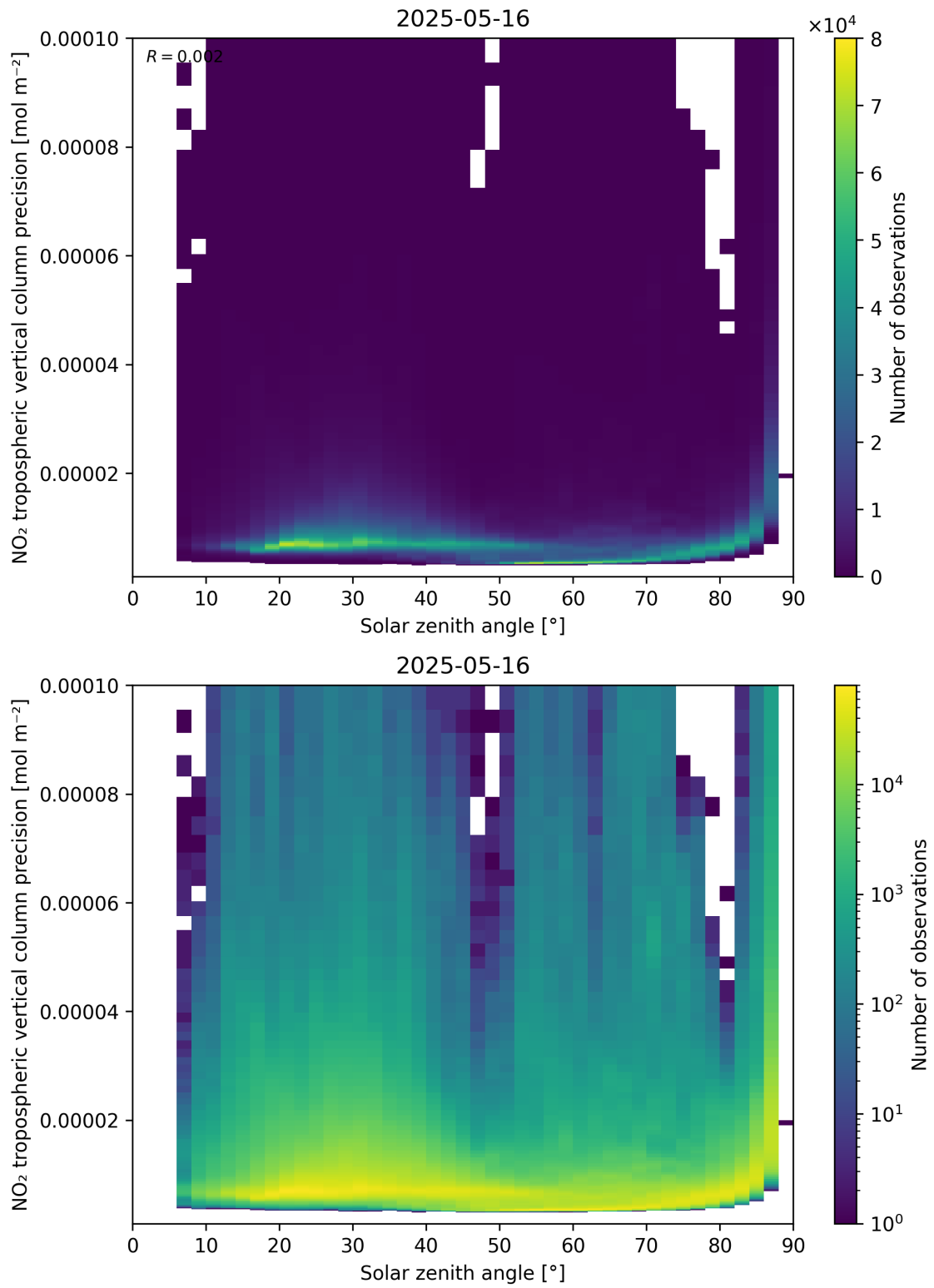
Figure 156: Scatter density plot of “Solar zenith angle” against “NO 2 tropospheric vertical column precision” for 2025-05-15 to 2025-05-17.
