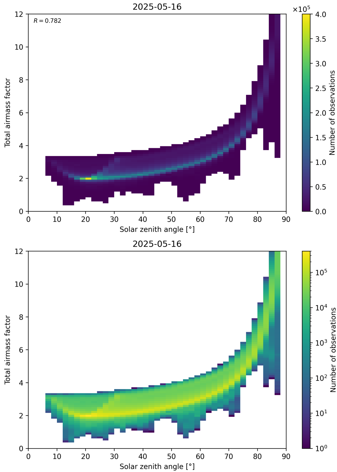
Figure 146: Scatter density plot of “Solar zenith angle” against “Total air mass factor” for 2025-05-15 to 2025-05-17.
