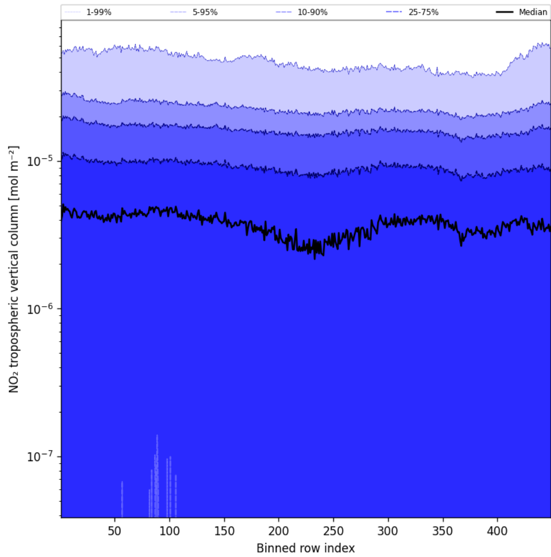
Figure 46: Along track statistics of “NO 2 tropospheric vertical column” for 2025-05-15 to 2025-05-17
