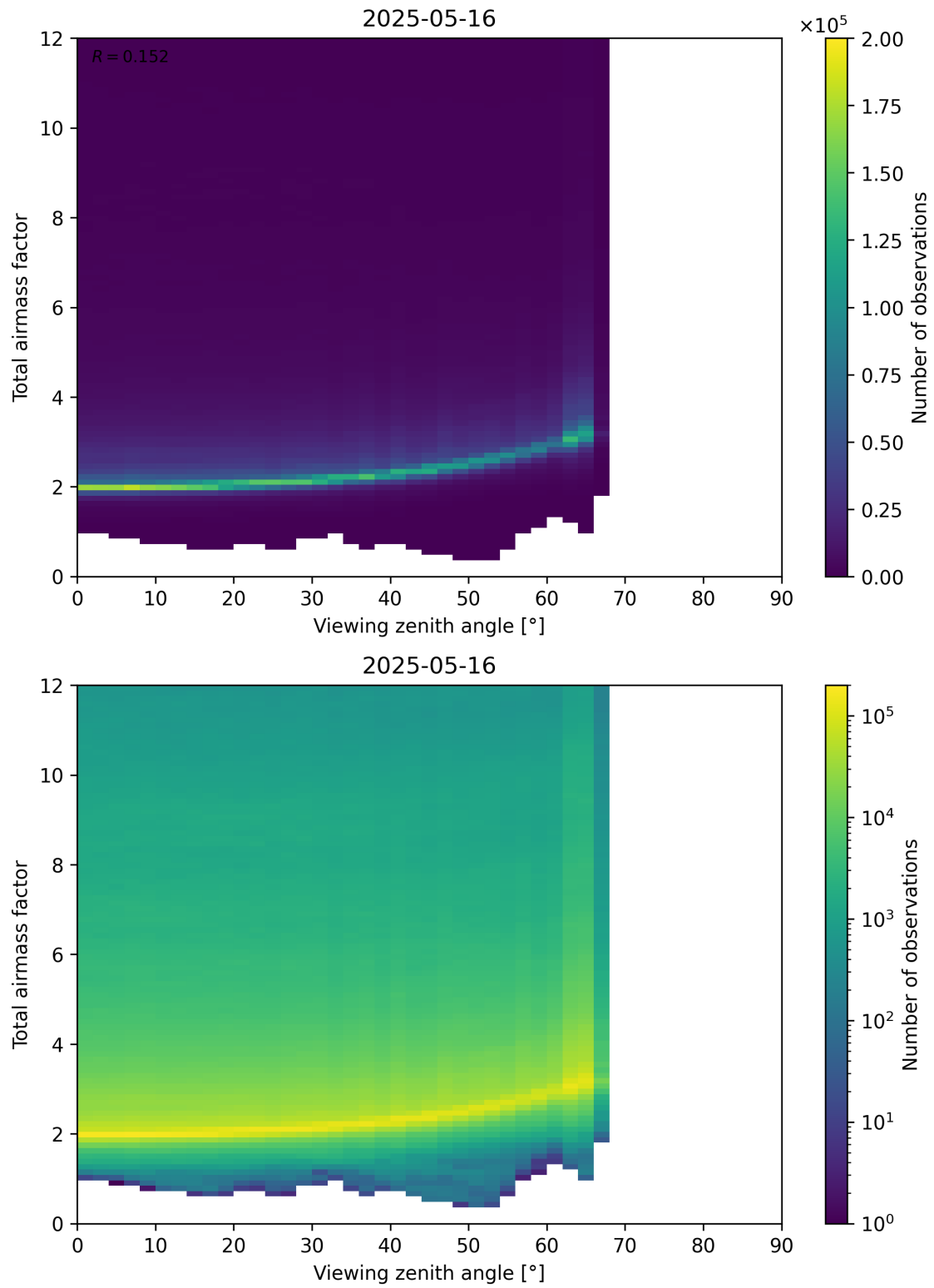
Figure 160: Scatter density plot of “Viewing zenith angle” against “Total airmass factor” for 2025-05-15 to 2025-05-17.
