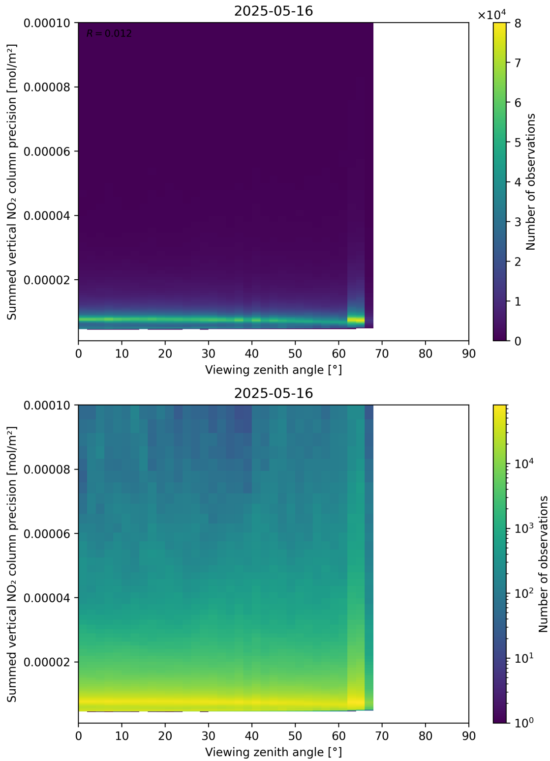
Figure 166: Scatter density plot of “Viewing zenith angle” against “Summed vertical NO 2 column precision” for 2025-05-15 to 2025-05-17.
