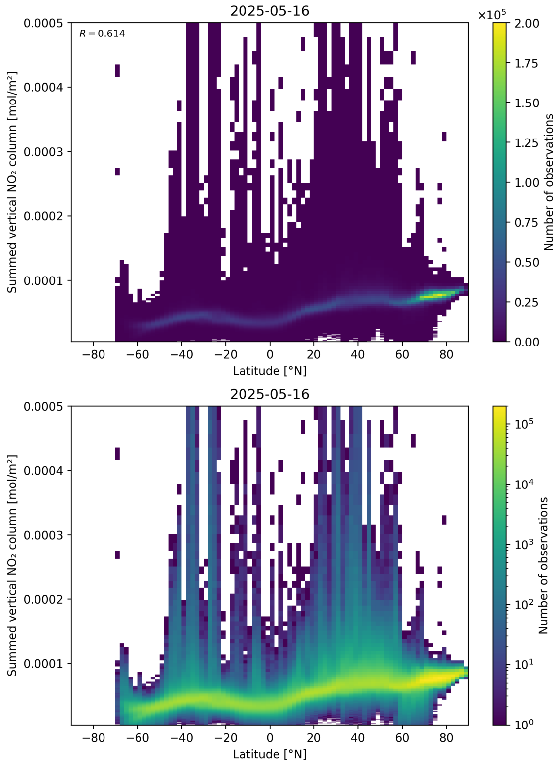
Figure 88: Scatter density plot of “Latitude” against “Summed vertical NO 2 column” for 2025-05-15 to 2025-05-17.
