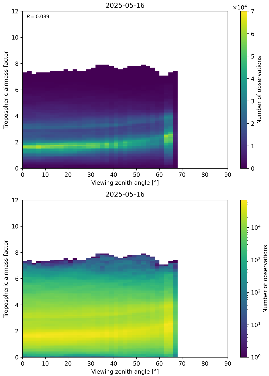
Figure 161: Scatter density plot of “Viewing zenith angle” against “Tropospheric airmass factor” for 2025-05-15 to 2025-05-17.
