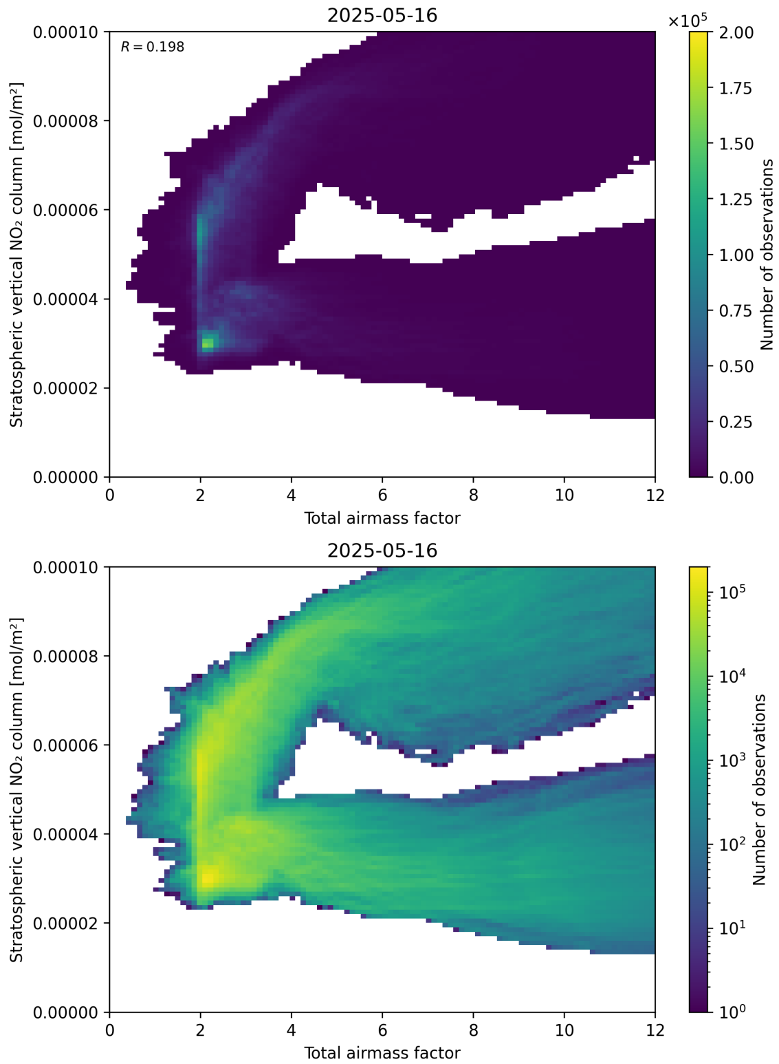
Figure 64: Scatter density plot of “Total airmass factor” against “Stratospheric vertical \text{NO}_2 column” for 2025-05-15 to 2025-05-17.
