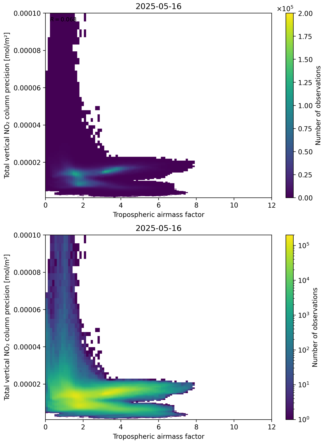
Figure 78: Scatter density plot of “Tropospheric air mass factor” against “Total vertical NO 2 column precision” for 2025-05-15 to 2025-05-17.
