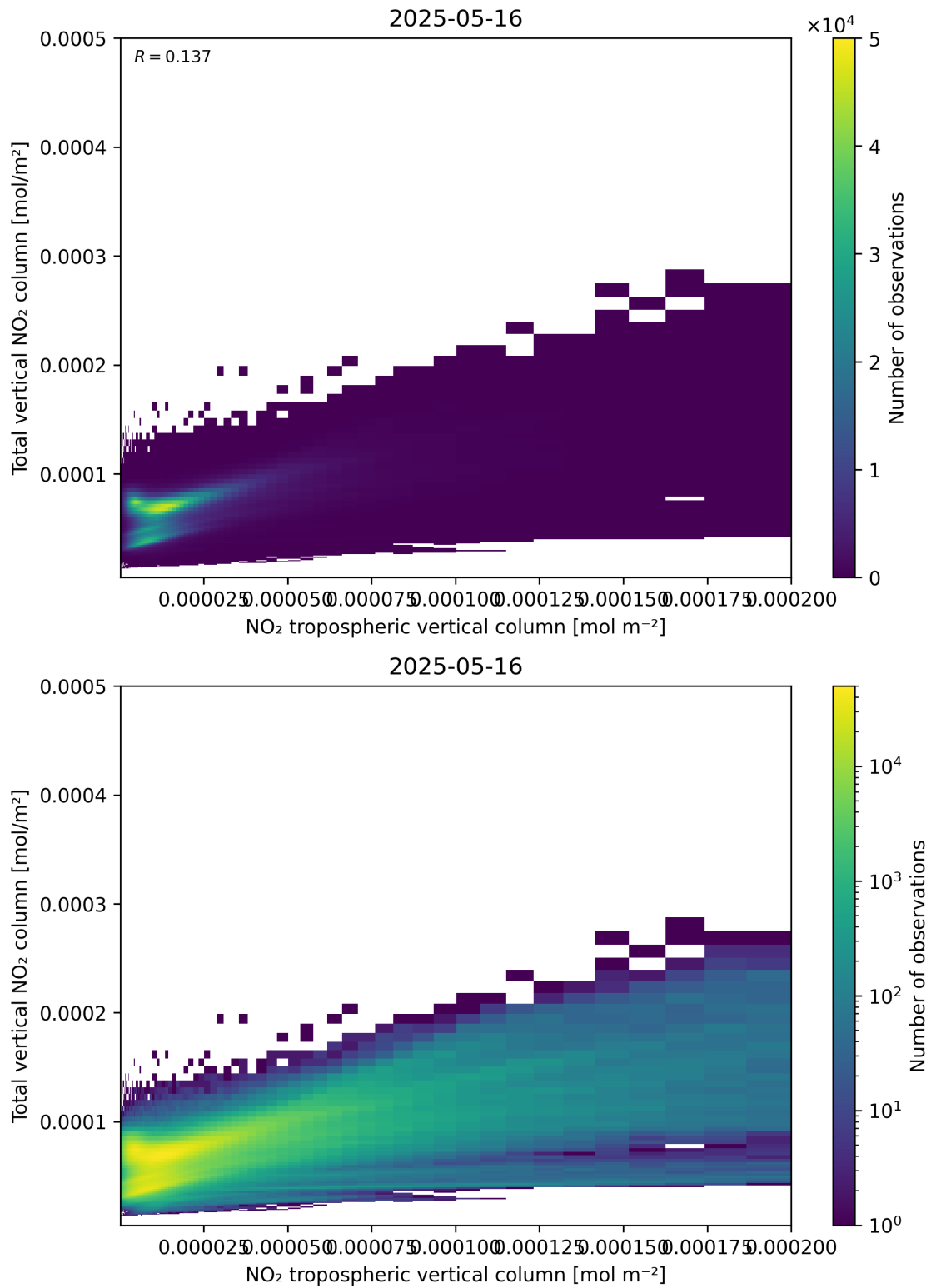
Figure 128: Scatter density plot of “NO 2 tropospheric vertical column” against “Total vertical NO 2 column” for 2025-05-15 to 2025-05-17.
