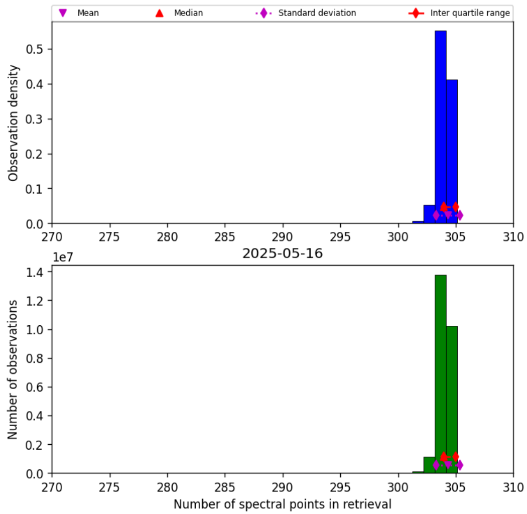
Figure 33: Histogram of “Number of spectral points in retrieval” for 2025-05-15 to 2025-05-17
