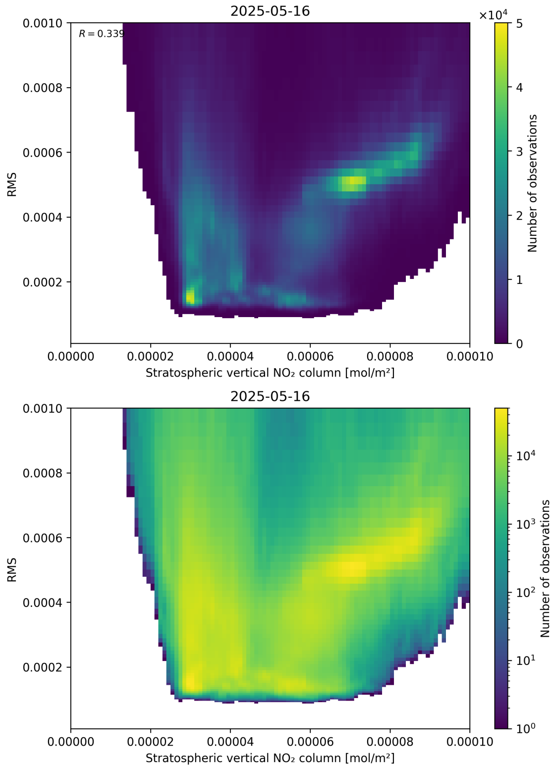
Figure 102: Scatter density plot of “Stratospheric vertical NO 2 column” against “RMS” for 2025-05-15 to 2025-05-17.
