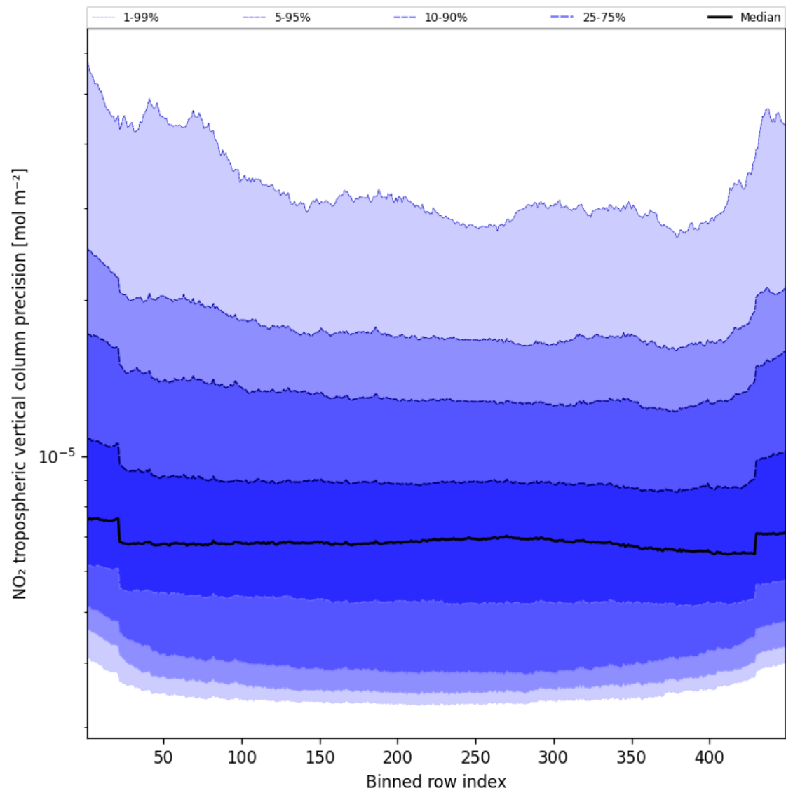
Figure 47: Along track statistics of “NO 2 tropospheric vertical column precision” for 2025-05-15 to 2025-05-17
