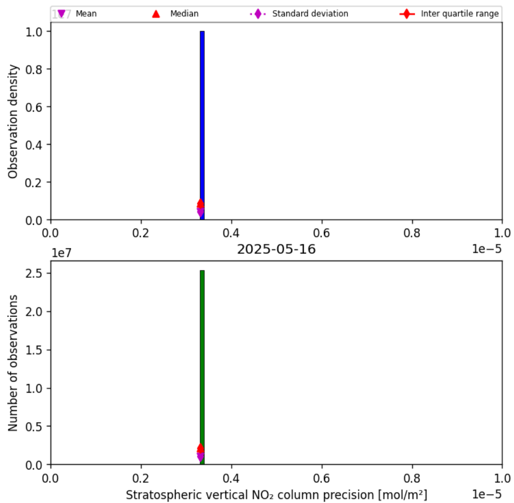
Figure 37: Histogram of “Stratospheric vertical NO 2 column precision” for 2025-05-15 to 2025-05-17
