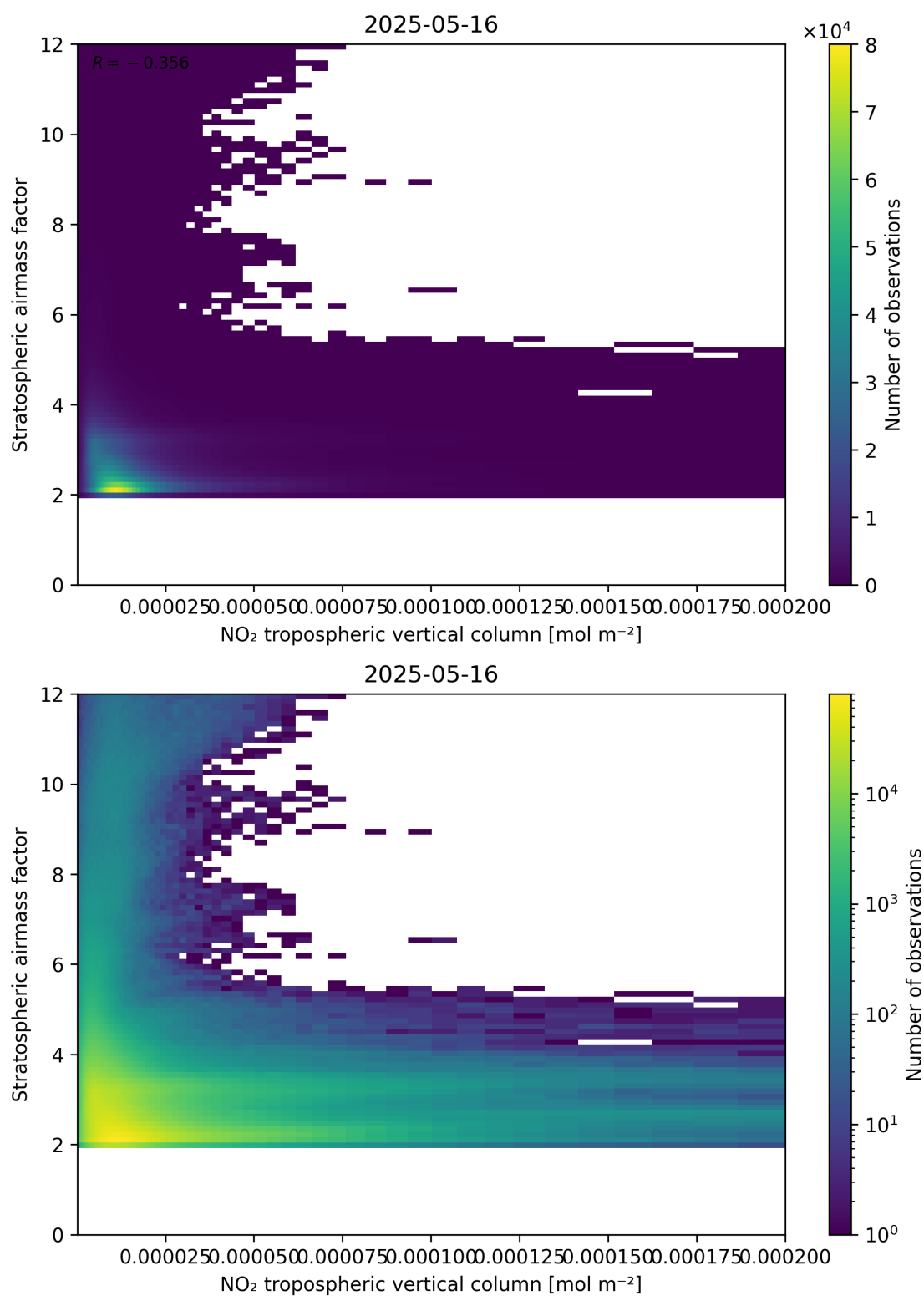
Figure 121: Scatter density plot of “NO 2 tropospheric vertical column” against “Stratospheric air mass factor” for 2025-05-15 to 2025-05-17.
