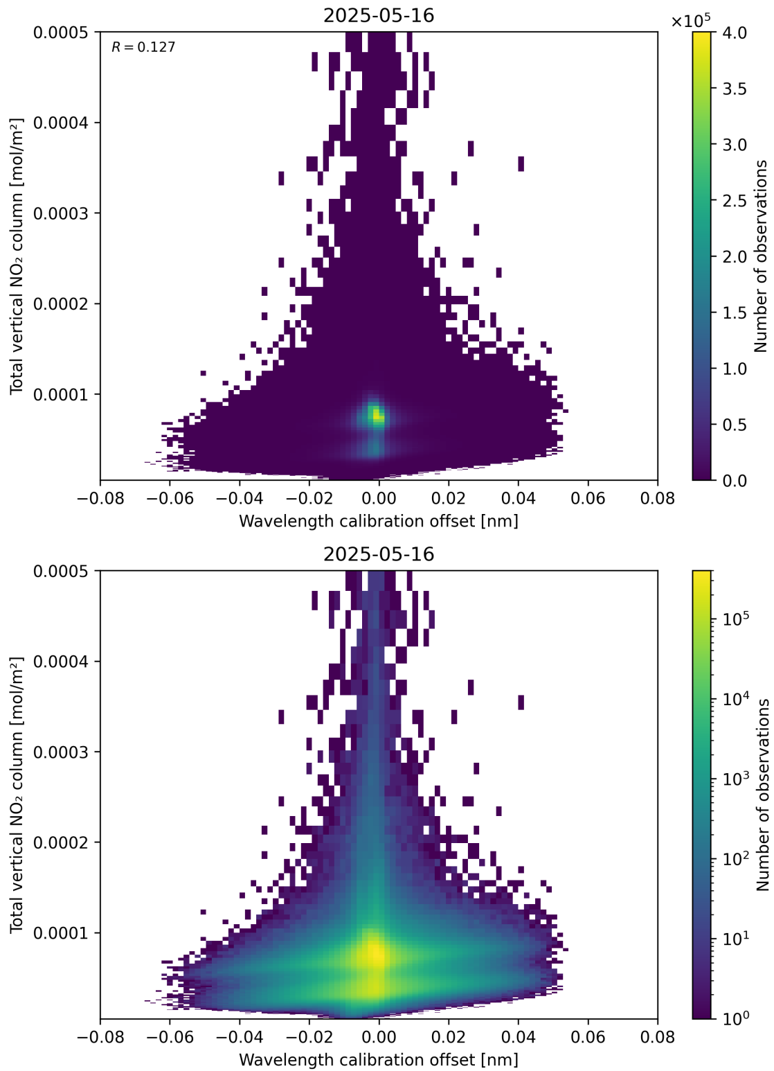
Figure 179: Scatter density plot of “Wavelength calibration offset” against “Total vertical NO 2 column” for 2025-05-15 to 2025-05-17.
