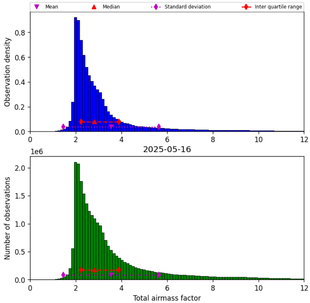
Figure 32: Histogram of “Total airmass factor” for 2025-05-15 to 2025-05-17
