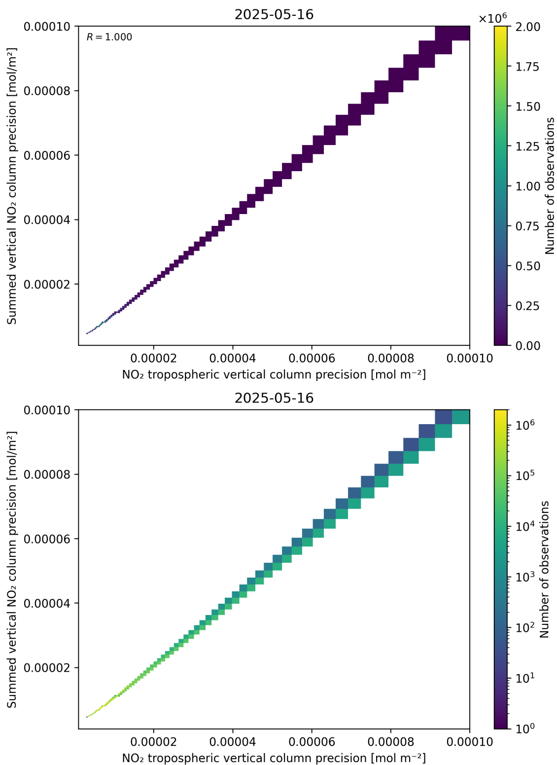
Figure 137: Scatter density plot of “NO 2 tropospheric vertical column precision” against “Summed vertical NO 2 column precision” for 2025-05-15 to 2025-05-17.
