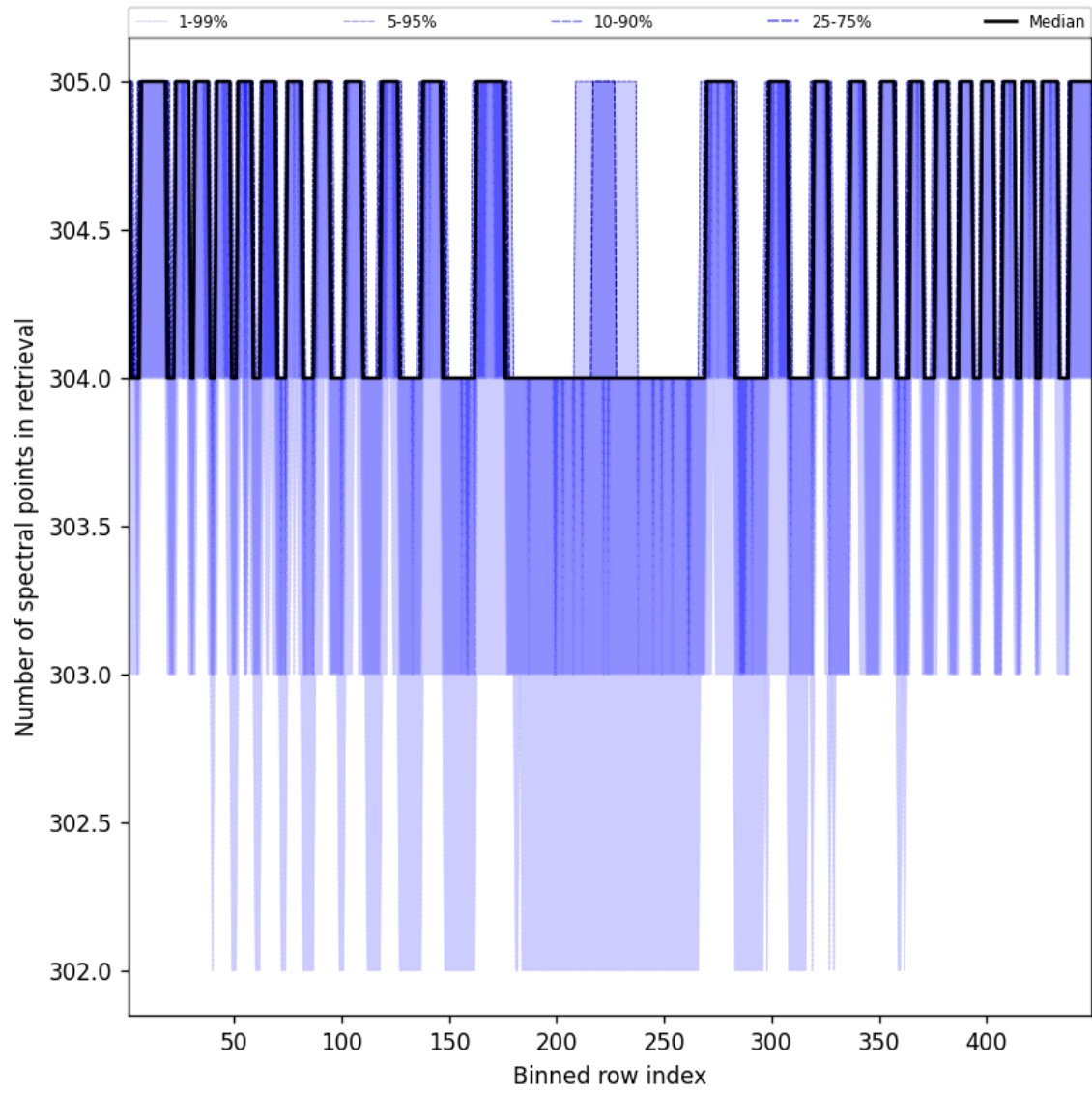
Figure 50: Along track statistics of “Number of spectral points in retrieval” for 2025-05-15 to 2025-05-17
