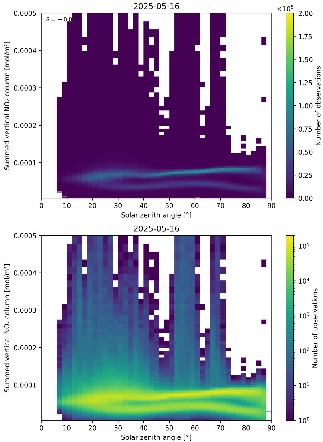
Figure 151: Scatter density plot of “Solar zenith angle” against “Summed vertical NO 2 column” for 2025-05-15 to 2025-05-17.
