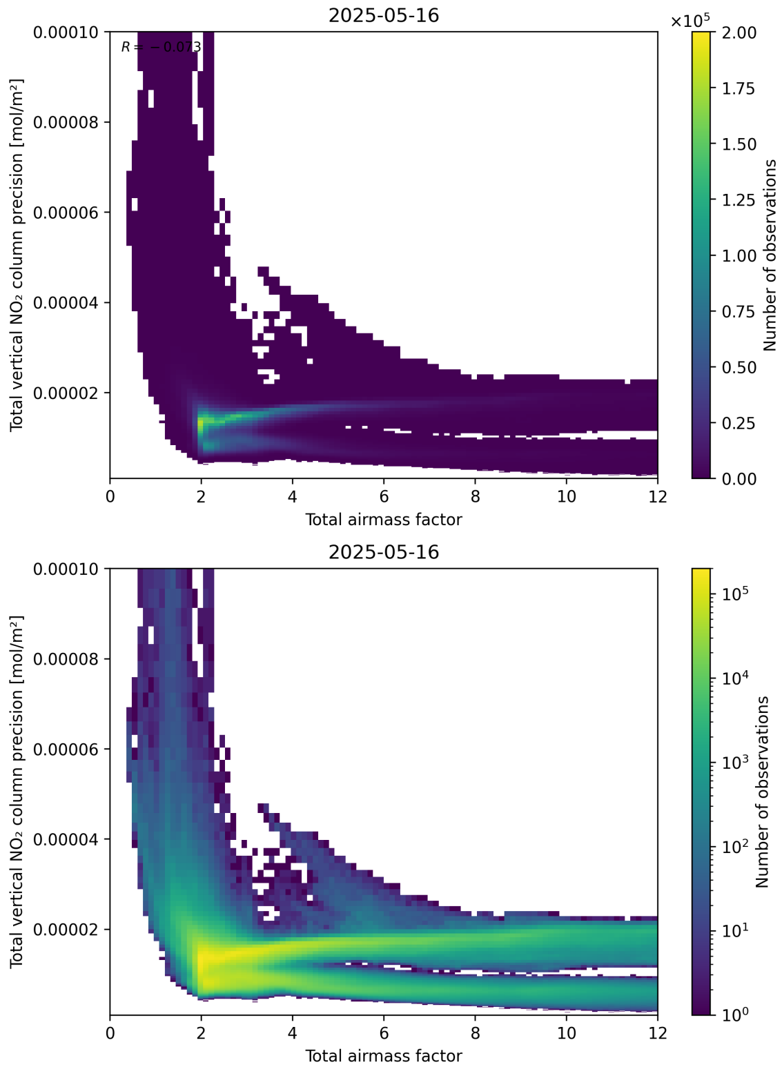
Figure 68: Scatter density plot of “Total airmass factor” against “Total vertical NO 2 column precision” for 2025-05-15 to 2025-05-17.
