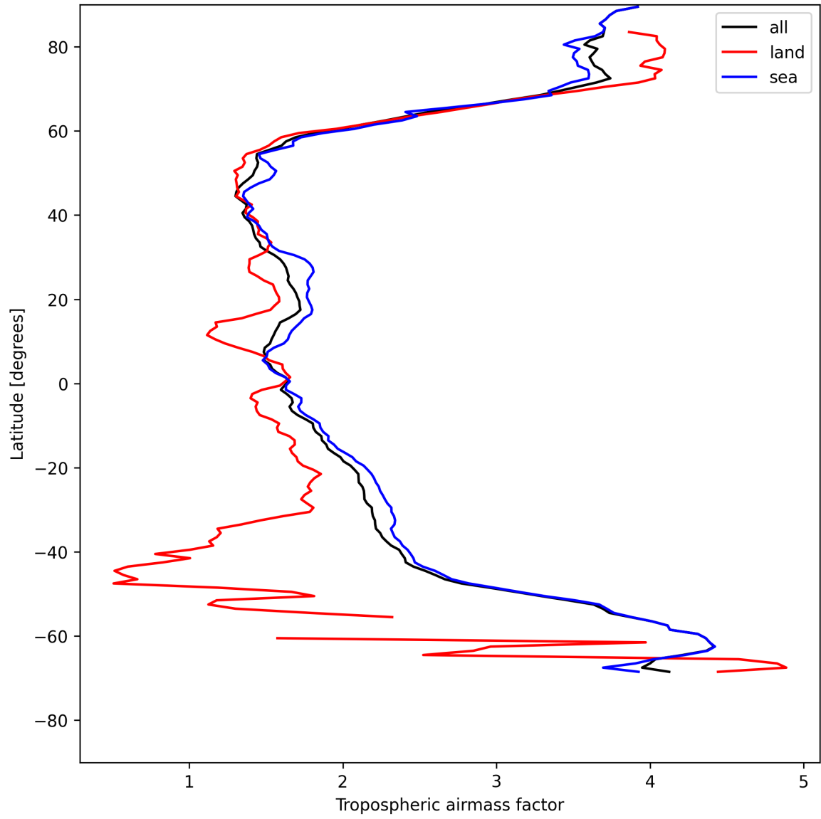
Figure 14: Zonal average of “Tropospheric airmass factor” for 2025-05-15 to 2025-05-17.
