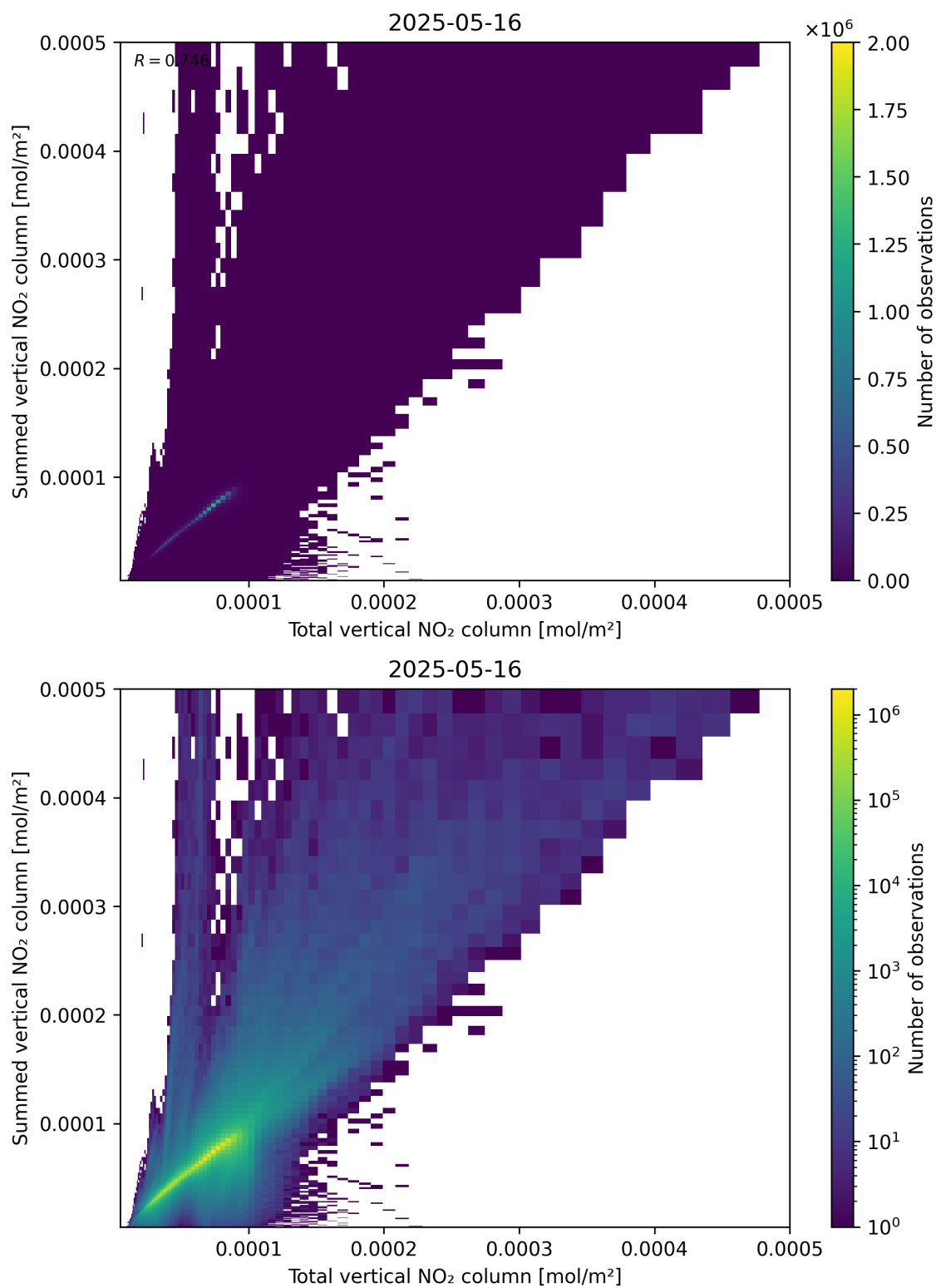
Figure 112: Scatter density plot of “Total vertical NO 2 column” against “Summed vertical NO 2 column” for 2025-05-15 to 2025-05-17.
