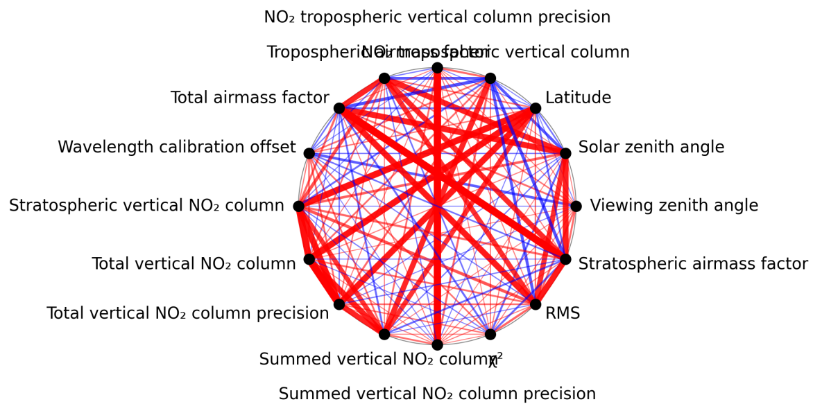
Figure 1: Map of correlation graph for 2025-05-15 to 2025-05-17.
