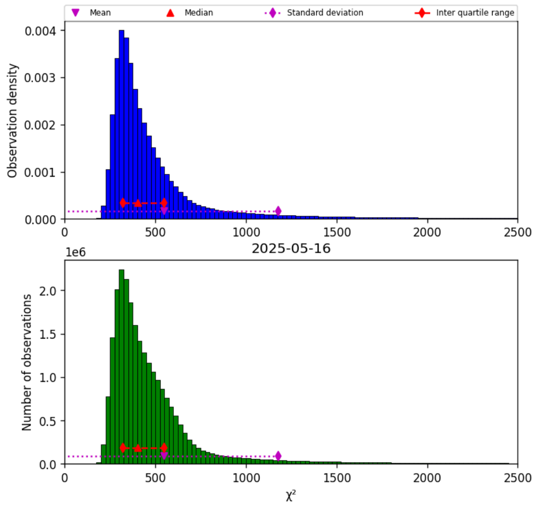
Figure 42: Histogram of “ \chi^2 ” for 2025-05-15 to 2025-05-17
