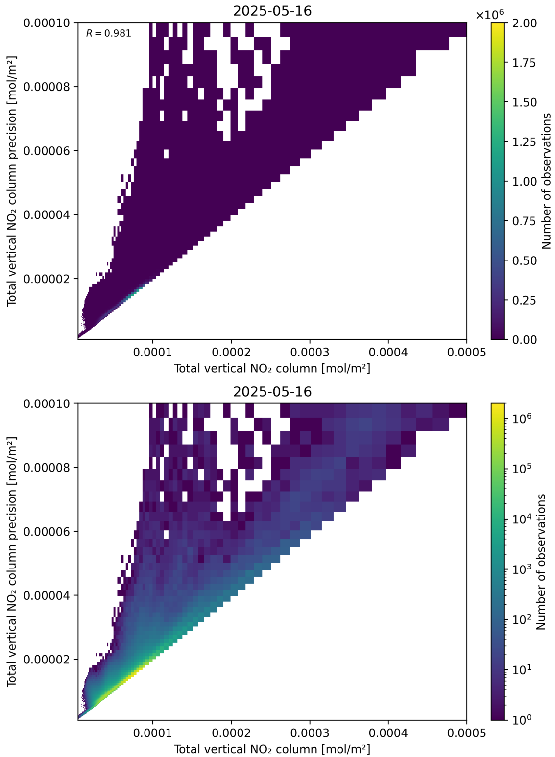
Figure 114: Scatter density plot of “Total vertical NO 2 column” against “Total vertical NO 2 column precision” for 2025-05-15 to 2025-05-17.
