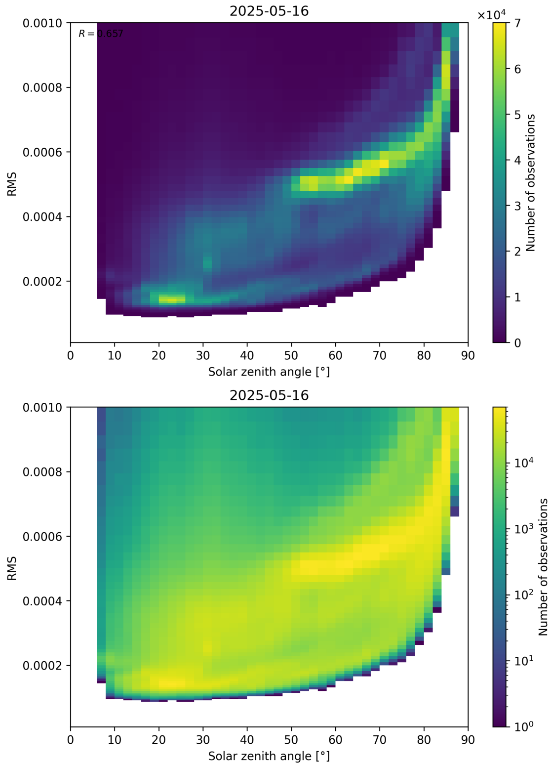
Figure 157: Scatter density plot of “Solar zenith angle” against “RMS” for 2025-05-15 to 2025-05-17.
