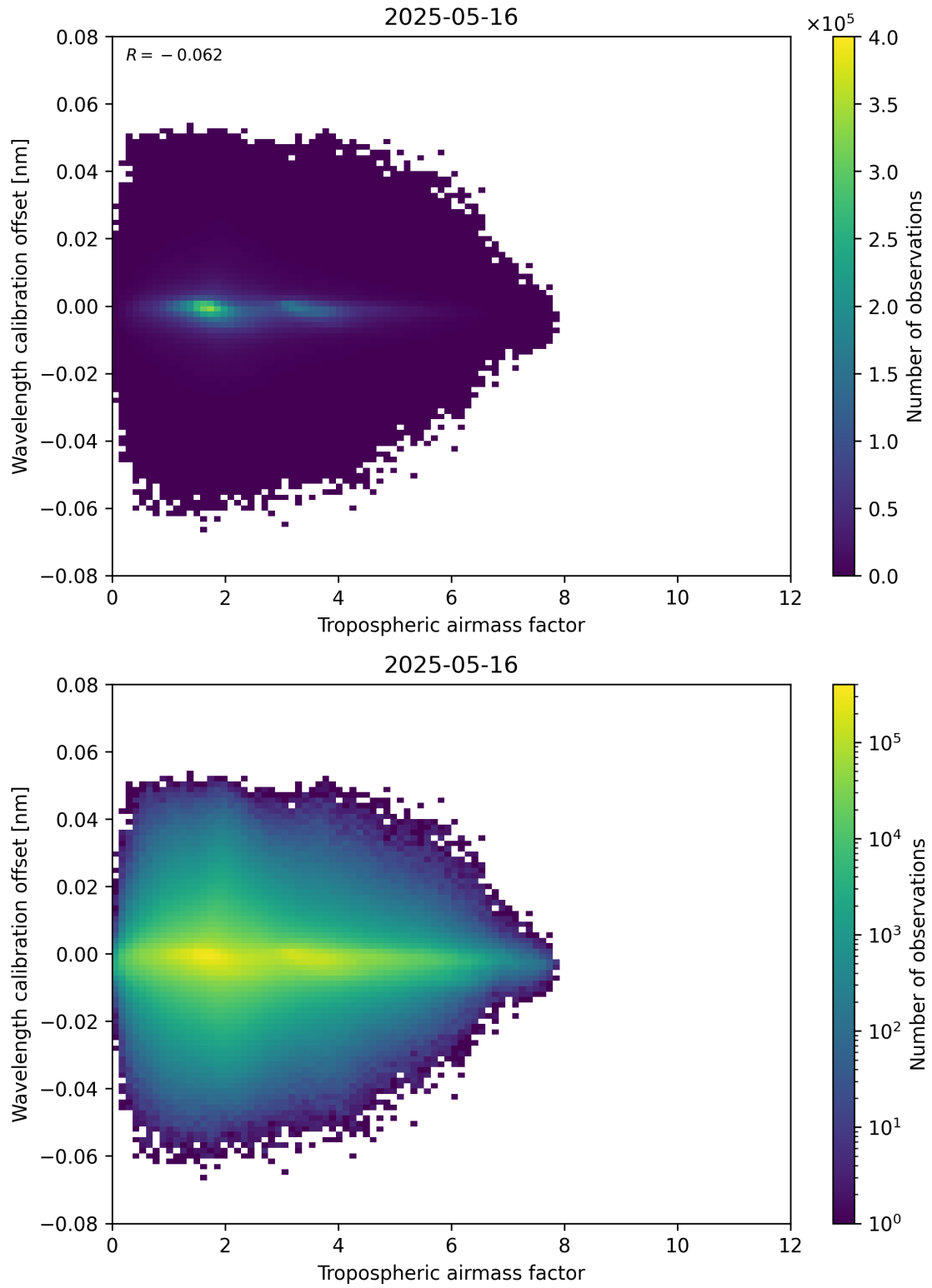
Figure 80: Scatter density plot of “Tropospheric airmass factor” against “Wavelength calibration offset” for 2025-05-15 to 2025-05-17.
