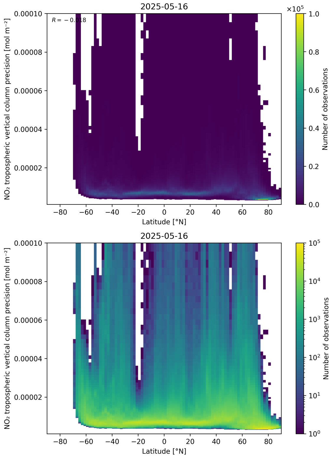
Figure 93: Scatter density plot of “Latitude” against “NO 2 tropospheric vertical column precision” for 2025-05-15 to 2025-05-17.
