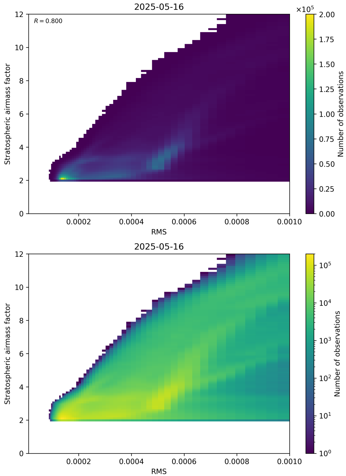
Figure 144: Scatter density plot of “RMS” against “Stratospheric airmass factor” for 2025-05-15 to 2025-05-17.
