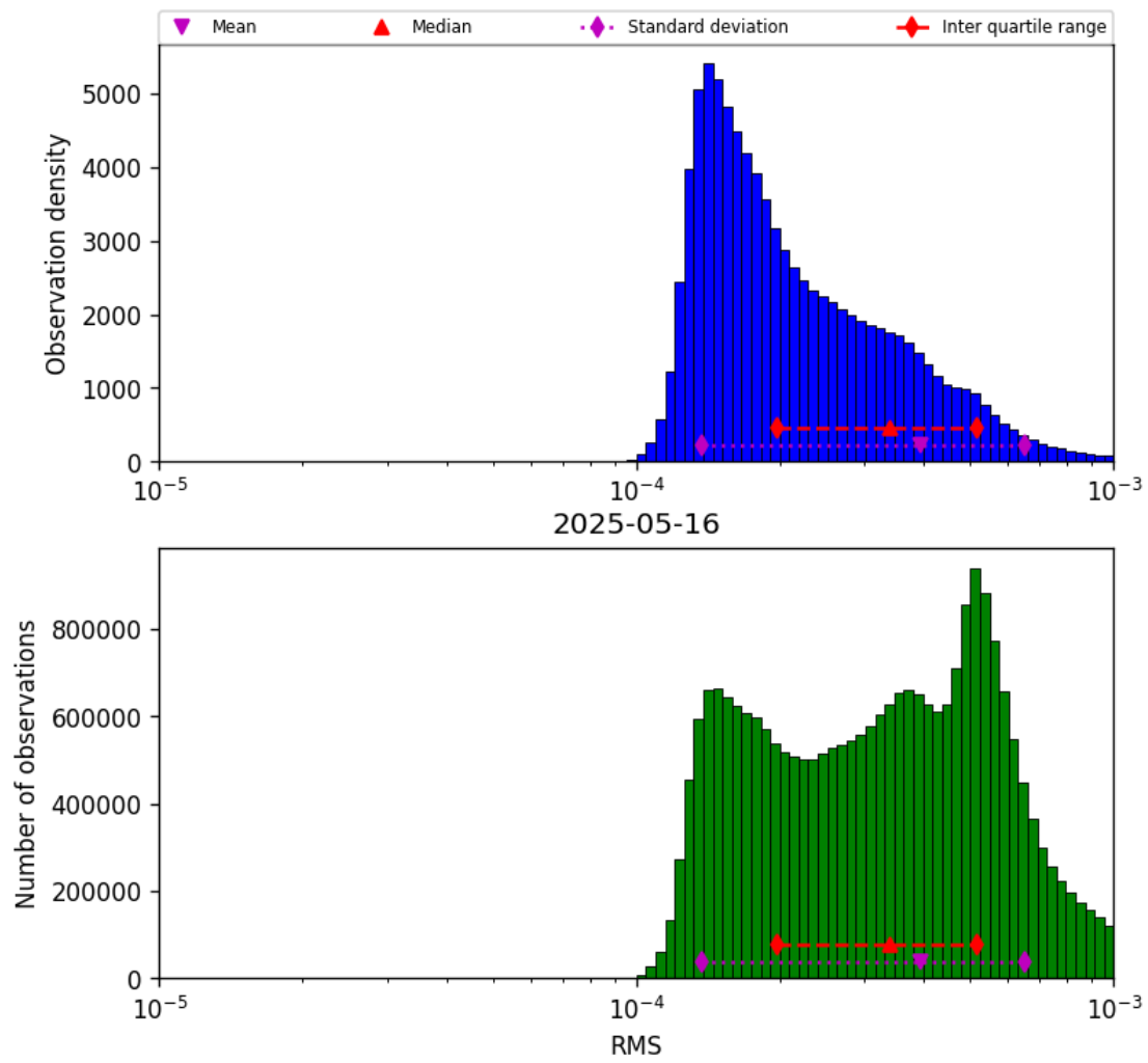
Figure 43: Histogram of “RMS” for 2025-05-15 to 2025-05-17
