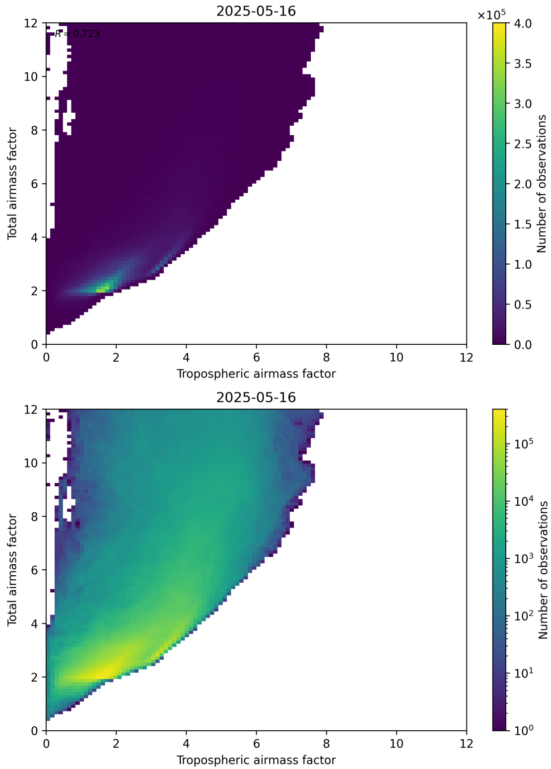
Figure 72: Scatter density plot of “Tropospheric airmass factor” against “Total airmass factor” for 2025-05-15 to 2025-05-17.
