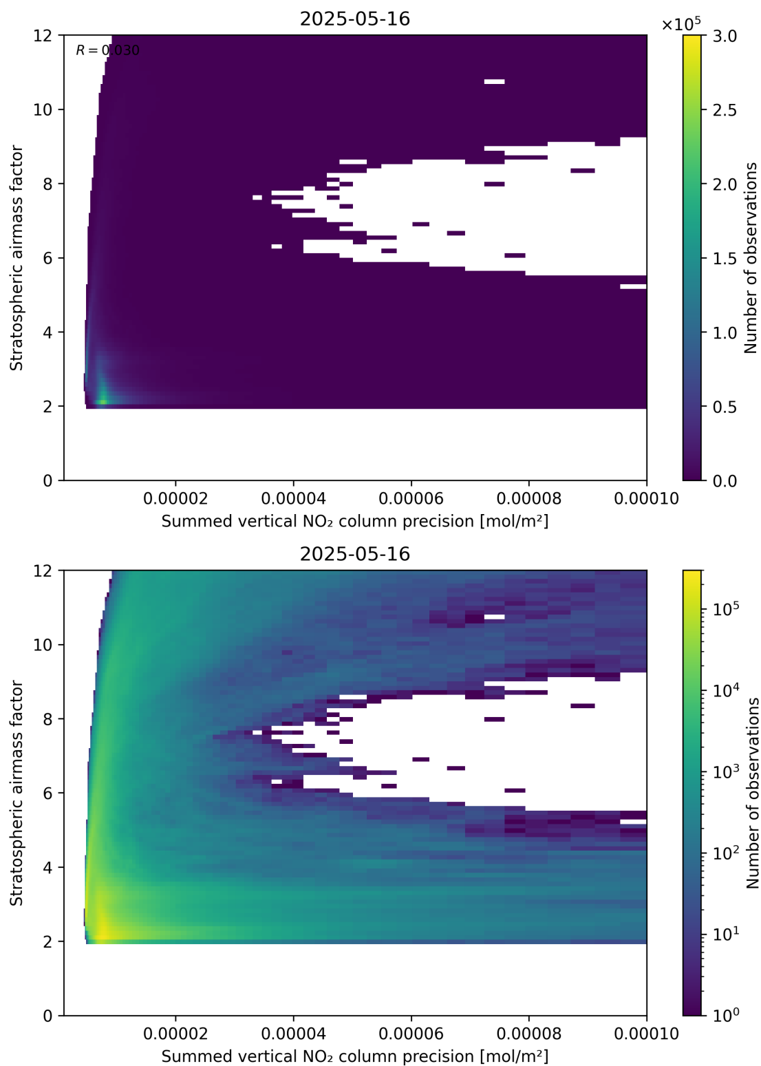
Figure 106: Scatter density plot of “Summed vertical NO 2 column precision” against “Stratospheric airmass factor” for 2025-05-15 to 2025-05-17.
