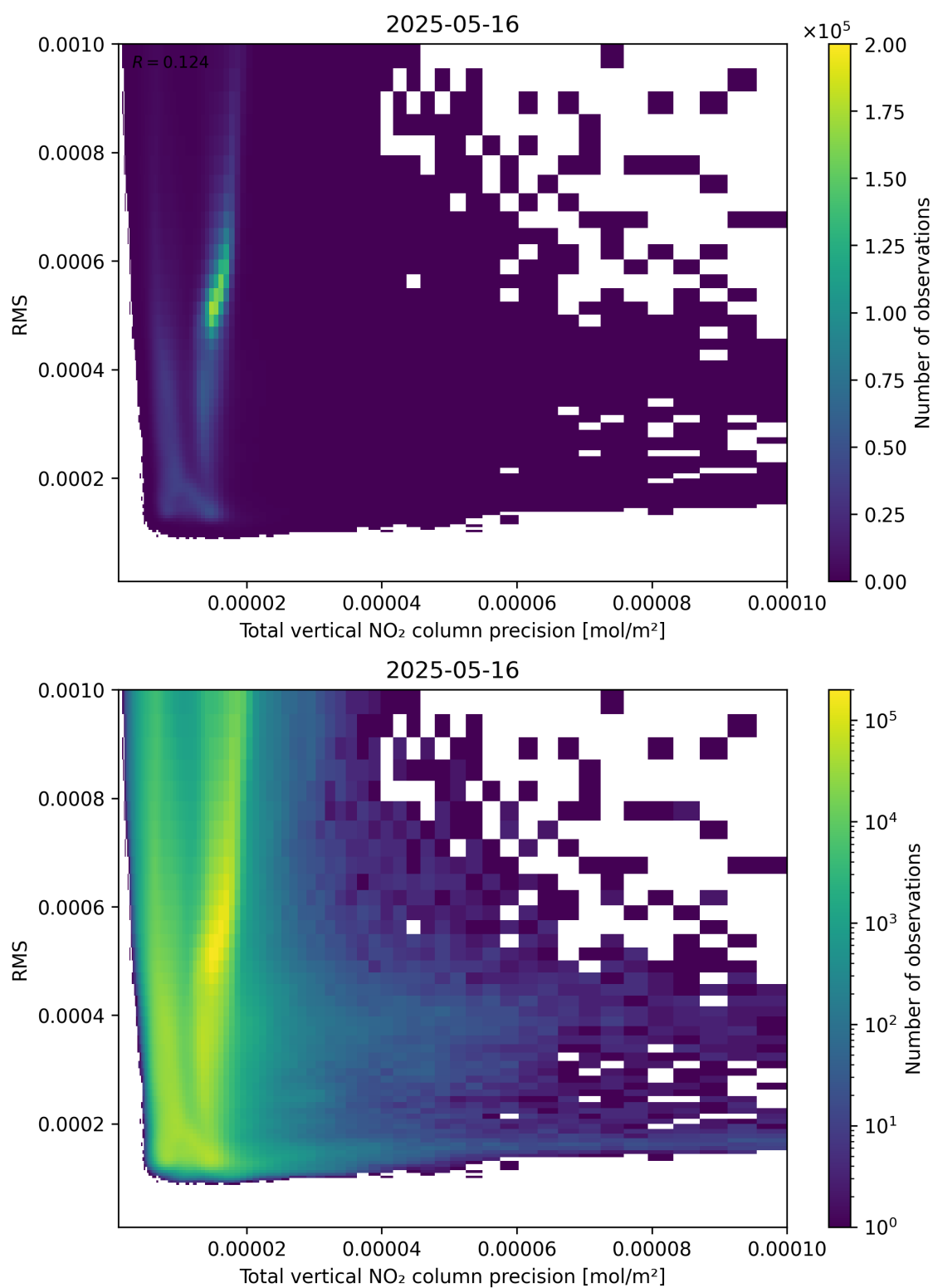
Figure 119: Scatter density plot of “Total vertical NO 2 column precision” against “RMS” for 2025-05-15 to 2025-05-17.
