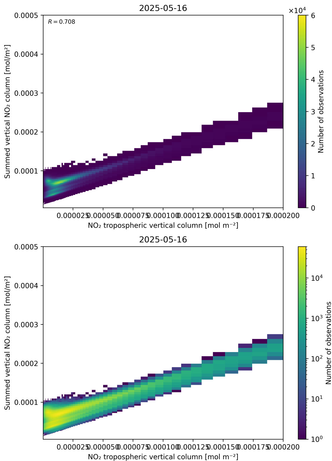
Figure 126: Scatter density plot of “NO 2 tropospheric vertical column” against “Summed vertical NO 2 column” for 2025-05-15 to 2025-05-17.
