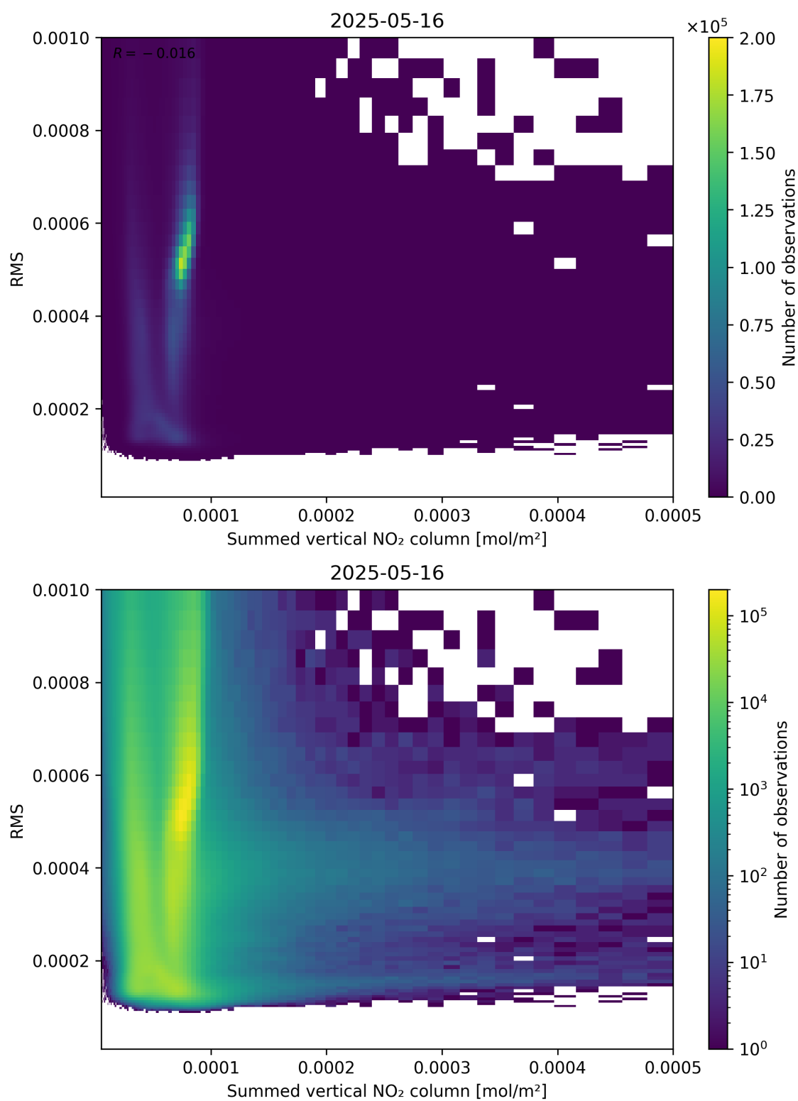
Figure 109: Scatter density plot of “Summed vertical NO 2 column” against “RMS” for 2025-05-15 to 2025-05-17.
