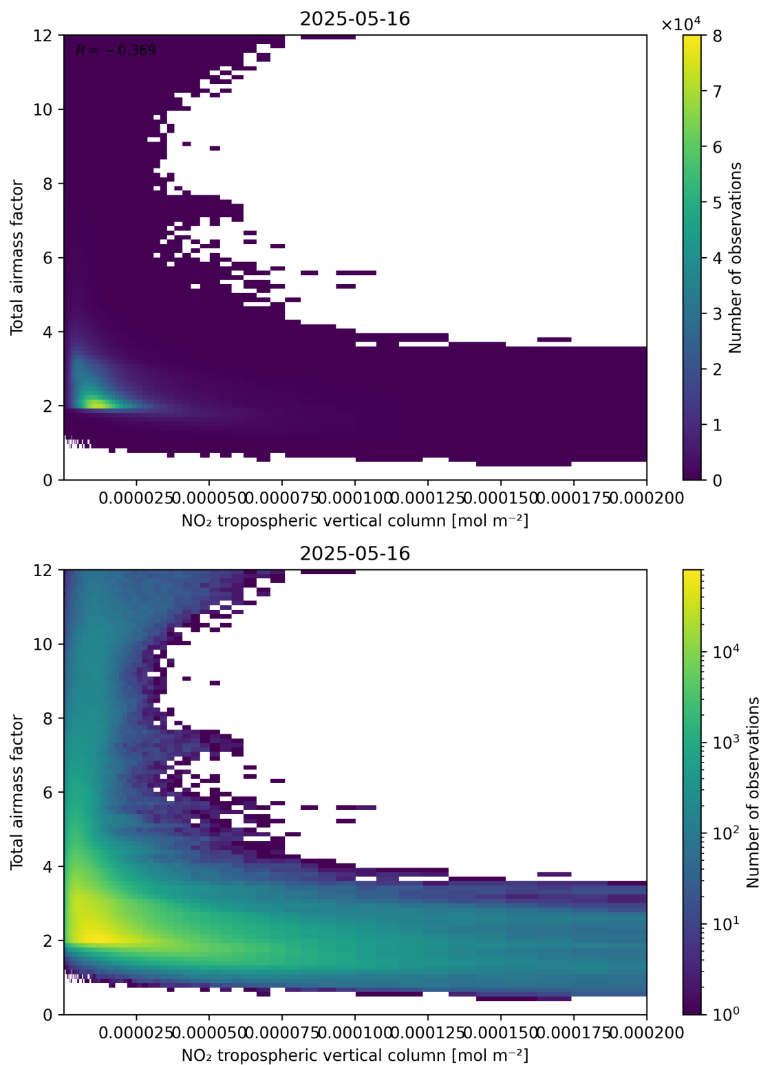
Figure 122: Scatter density plot of “NO 2 tropospheric vertical column” against “Total air mass factor” for 2025-05-15 to 2025-05-17.
