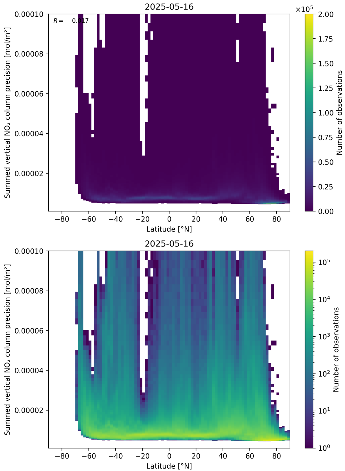
Figure 89: Scatter density plot of “Latitude” against “Summed vertical NO 2 column precision” for 2025-05-15 to 2025-05-17.
