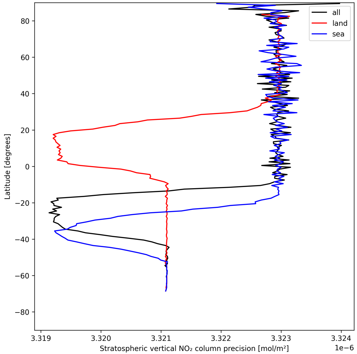
Figure 20: Zonal average of “Stratospheric vertical NO 2 column precision” for 2025-05-15 to 2025-05-17.
