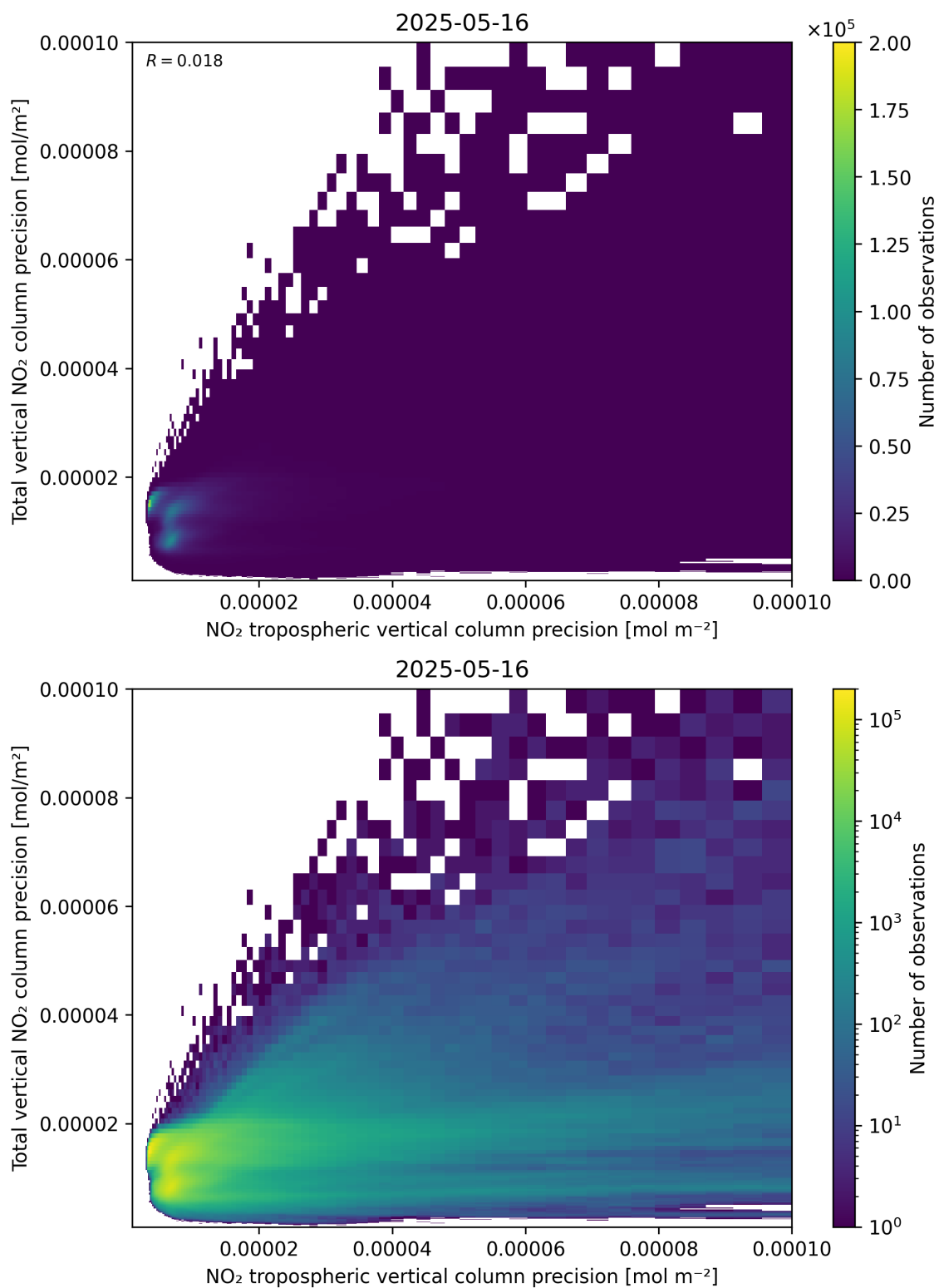
Figure 139: Scatter density plot of “NO 2 tropospheric vertical column precision” against “Total vertical NO 2 column precision” for 2025-05-15 to 2025-05-17.
