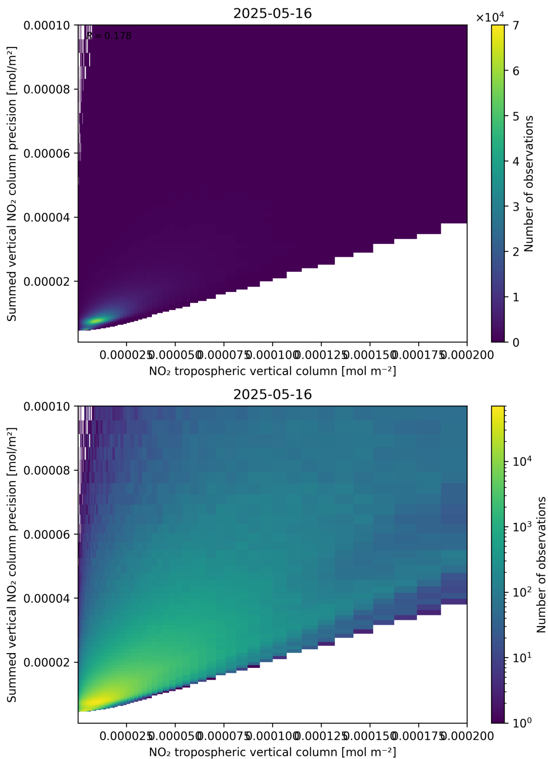
Figure 127: Scatter density plot of “NO 2 tropospheric vertical column” against “Summed vertical NO 2 column precision” for 2025-05-15 to 2025-05-17.
