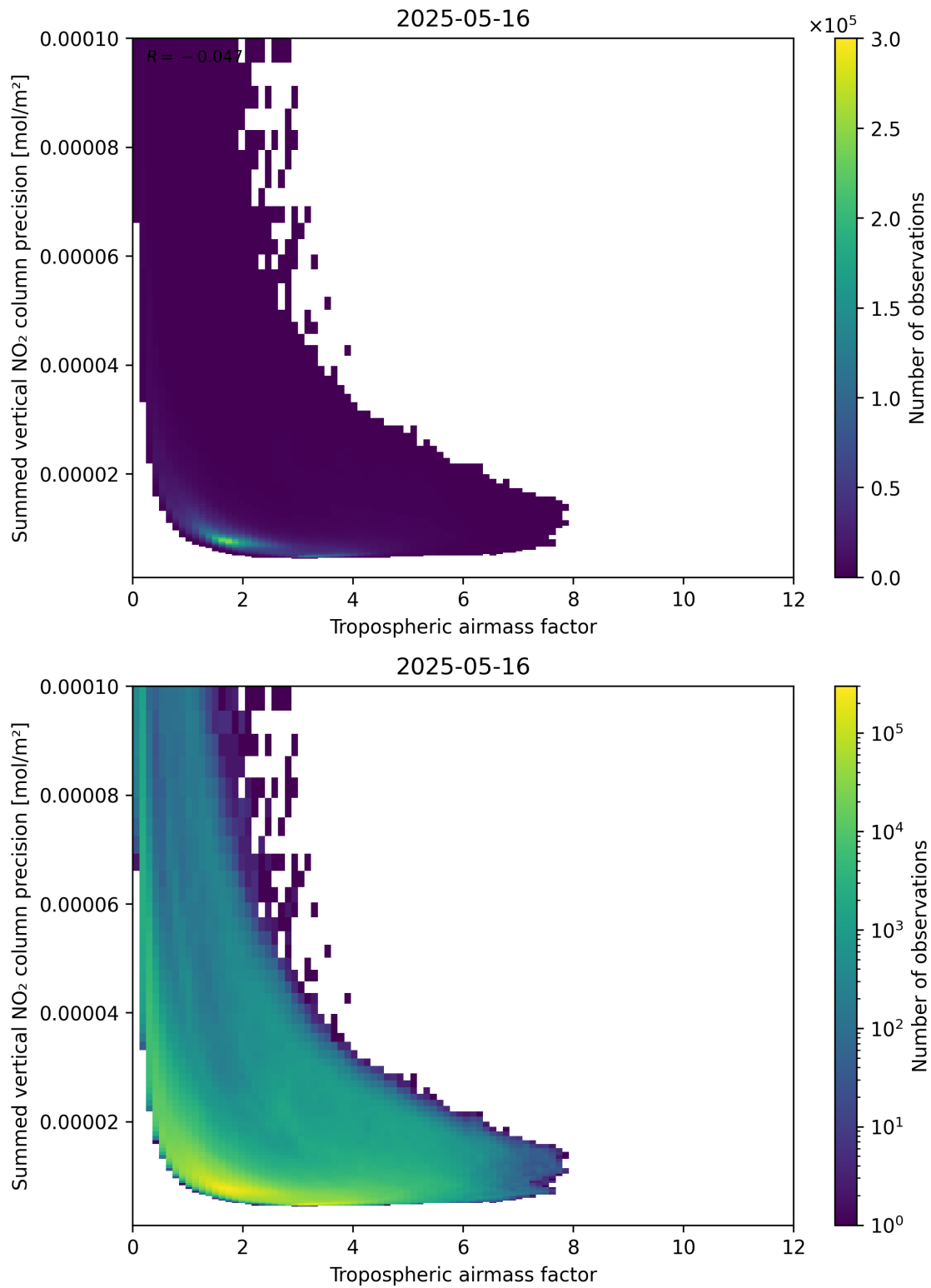
Figure 76: Scatter density plot of “Tropospheric air mass factor” against “Summed vertical NO 2 column precision” for 2025-05-15 to 2025-05-17.
