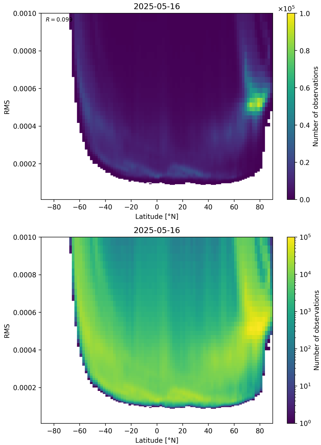
Figure 94: Scatter density plot of “Latitude” against “RMS” for 2025-05-15 to 2025-05-17.
