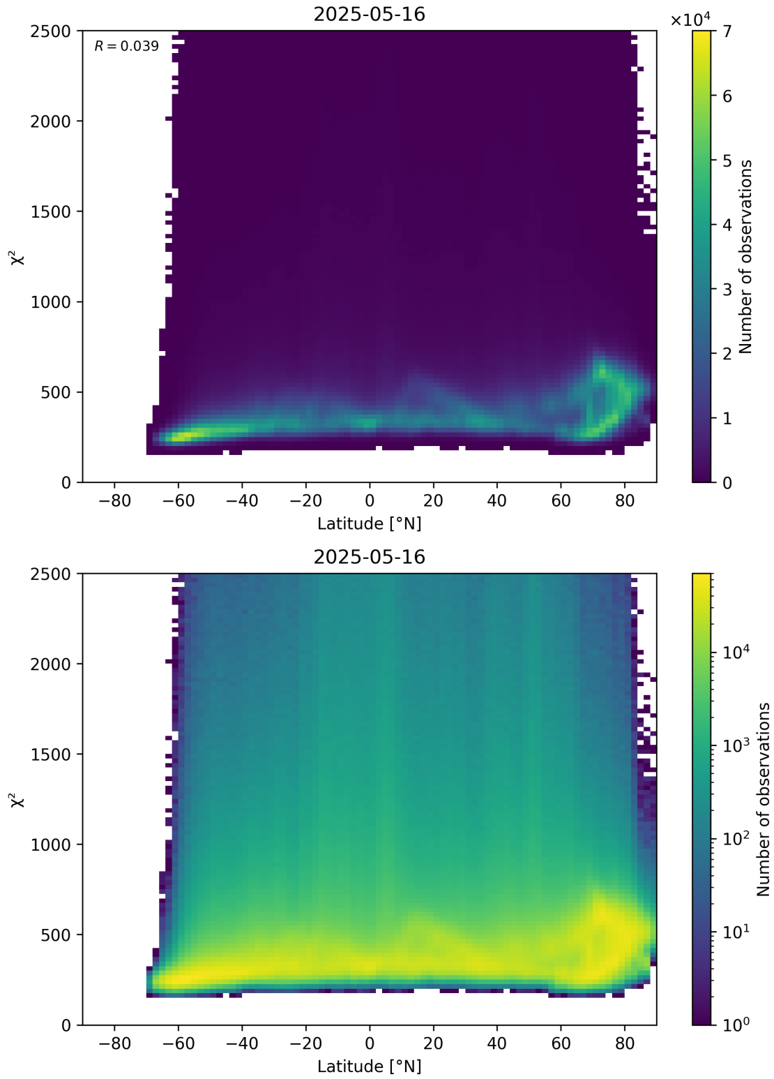
Figure 86: Scatter density plot of “Latitude” against “ \chi^2 ” for 2025-05-15 to 2025-05-17.
