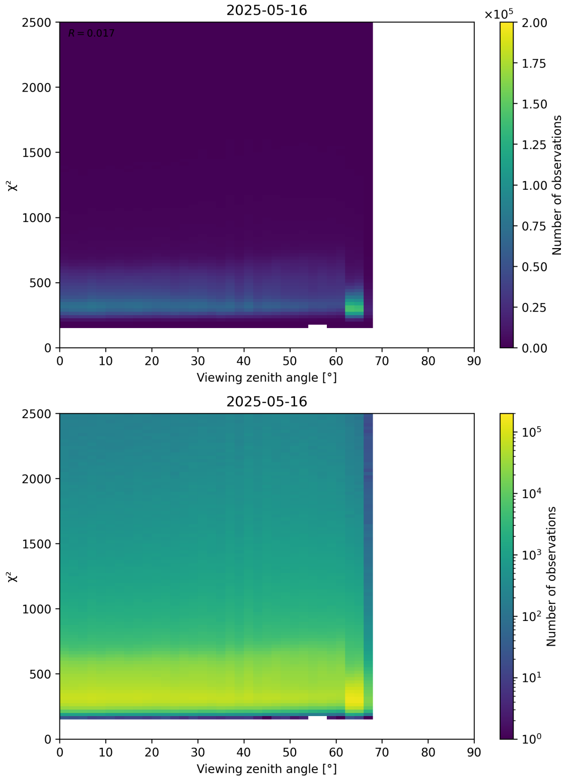
Figure 162: Scatter density plot of “Viewing zenith angle” against “ \chi^2 ” for 2025-05-15 to 2025-05-17.
