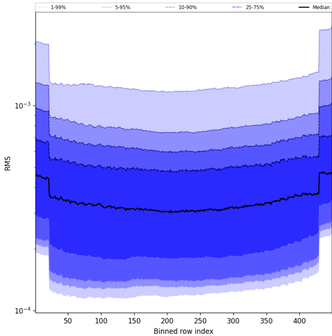
Figure 60: Along track statistics of “RMS” for 2025-05-15 to 2025-05-17
