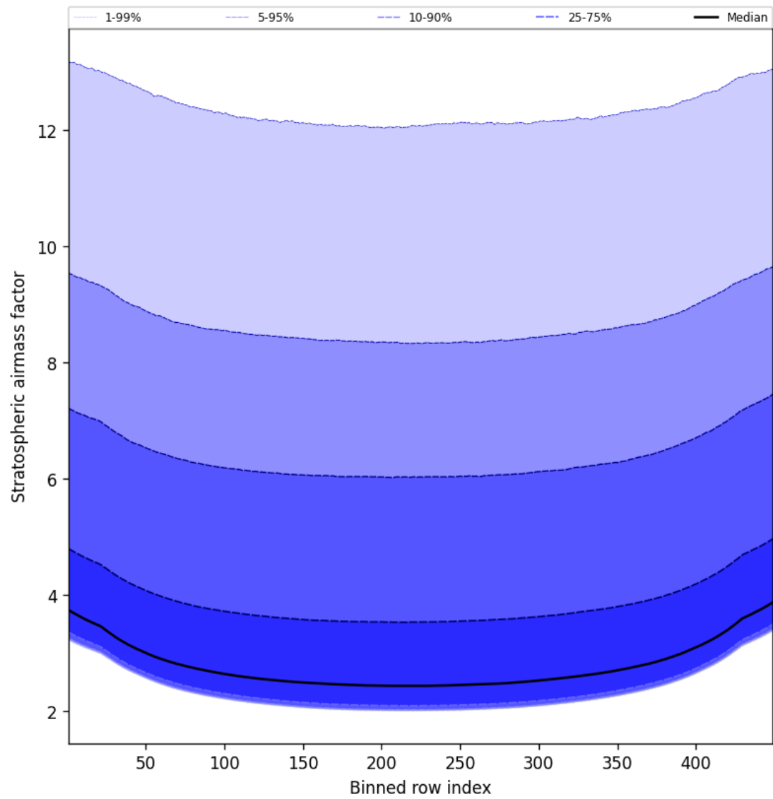
Figure 61: Along track statistics of “Stratospheric airmass factor” for 2025-05-15 to 2025-05-17
