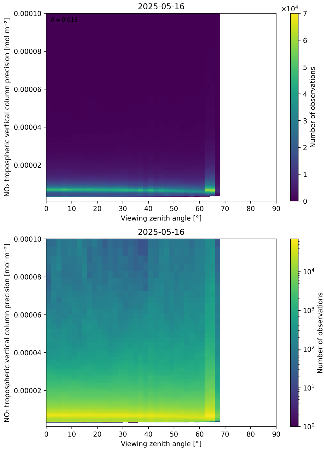
Figure 170: Scatter density plot of “Viewing zenith angle” against “NO 2 tropospheric vertical column precision” for 2025-05-15 to 2025-05-17.
