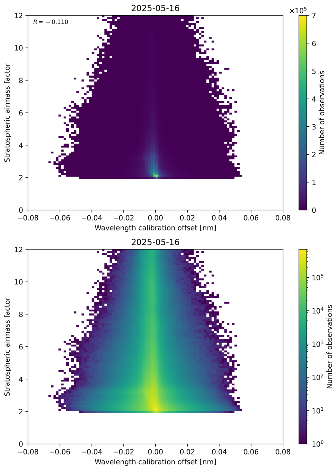
Figure 174: Scatter density plot of “Wavelength calibration offset” against “Stratospheric airmass factor” for 2025-05-15 to 2025-05-17.
