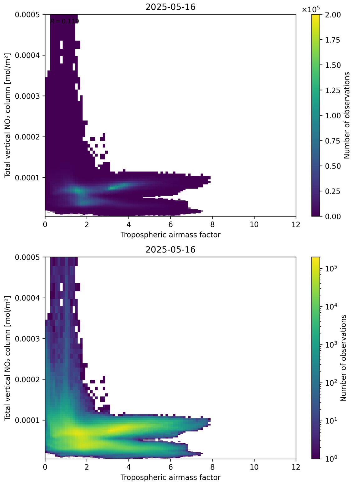
Figure 77: Scatter density plot of “Tropospheric airmass factor” against “Total vertical NO 2 column” for 2025-05-15 to 2025-05-17.
