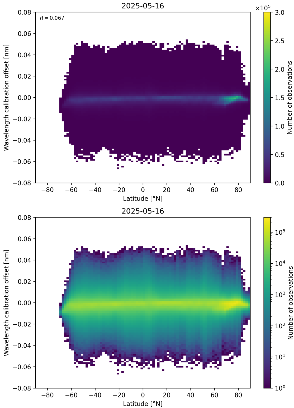
Figure 95: Scatter density plot of “Latitude” against “Wavelength calibration offset” for 2025-05-15 to 2025-05-17.
