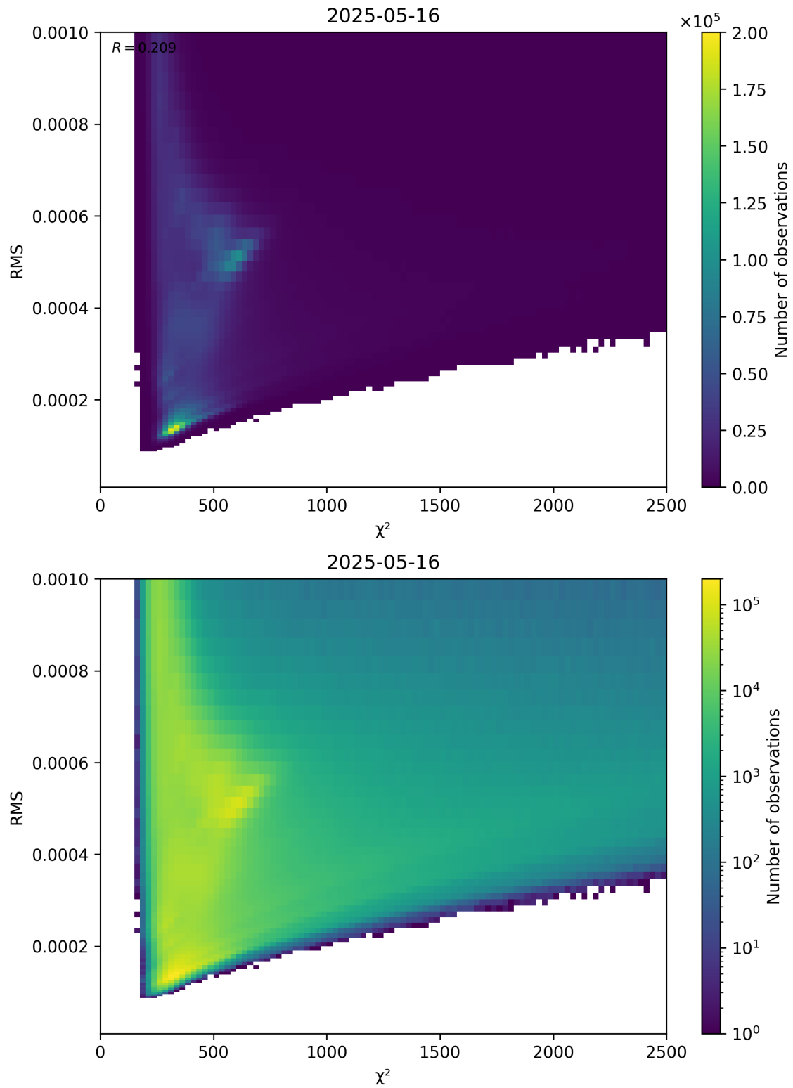
Figure 82: Scatter density plot of “ \chi^2 ” against “RMS” for 2025-05-15 to 2025-05-17.
