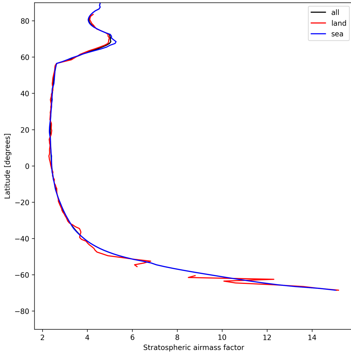
Figure 27: Zonal average of “Stratospheric air mass factor” for 2025-05-15 to 2025-05-17.
