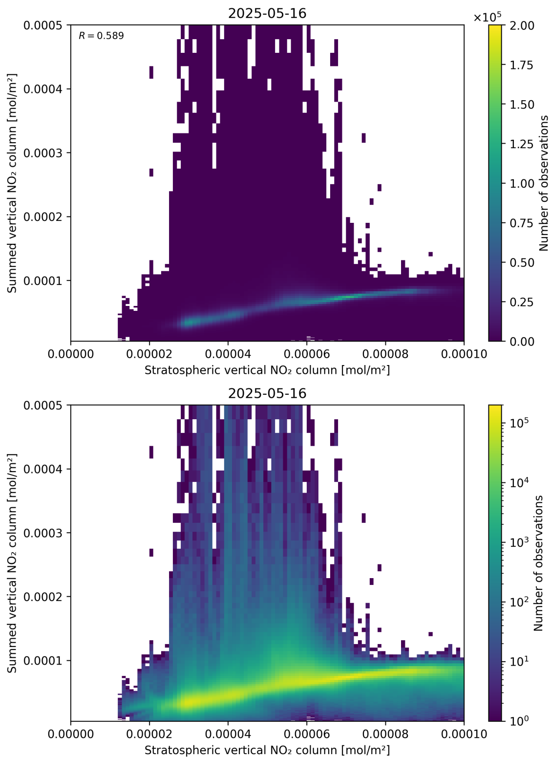
Figure 98: Scatter density plot of “Stratospheric vertical NO 2 column” against “Summed vertical NO 2 column” for 2025-05-15 to 2025-05-17.
