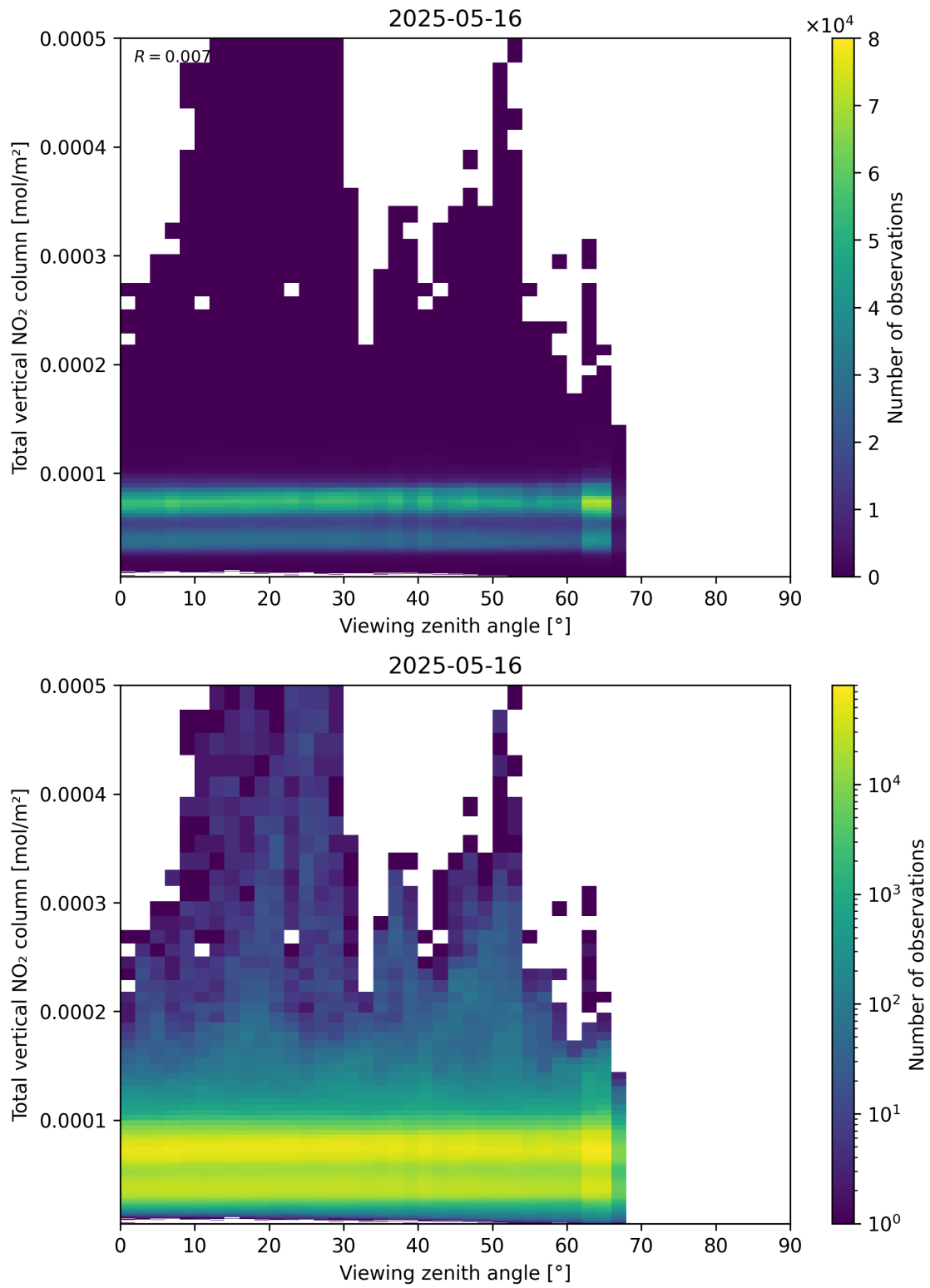
Figure 167: Scatter density plot of “Viewing zenith angle” against “Total vertical NO 2 column” for 2025-05-15 to 2025-05-17.
