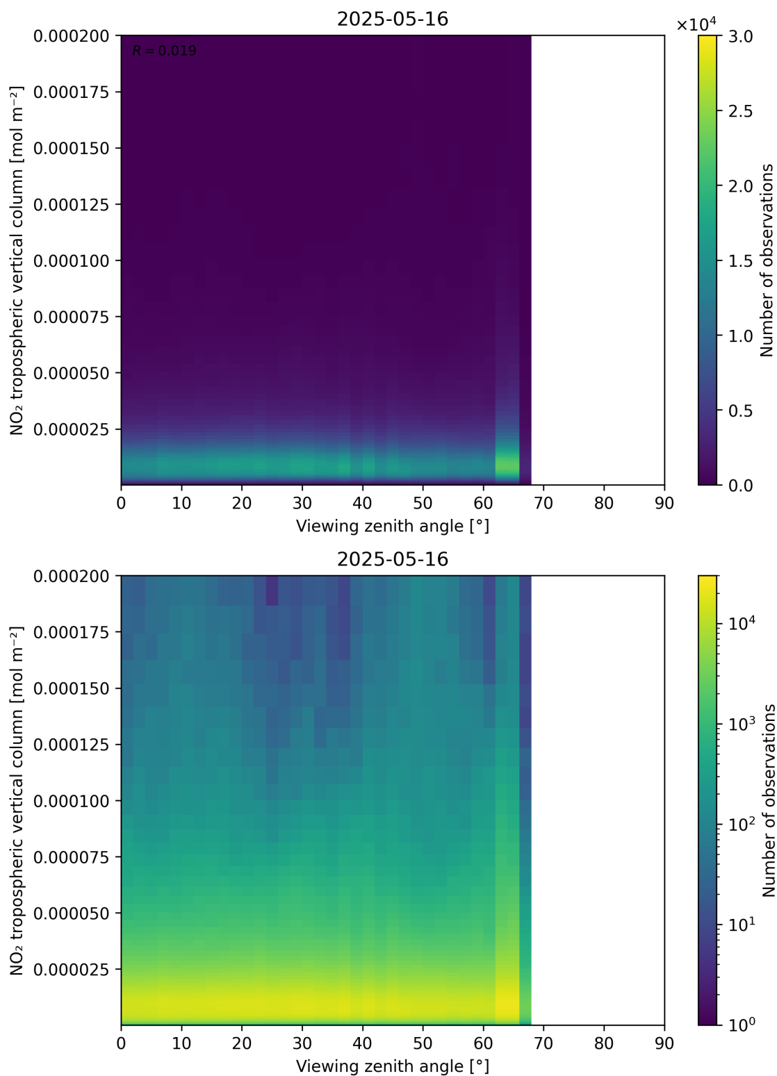
Figure 169: Scatter density plot of “Viewing zenith angle” against “NO 2 tropospheric vertical column” for 2025-05-15 to 2025-05-17.
