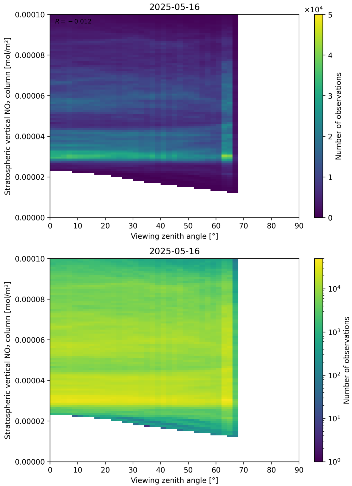
Figure 164: Scatter density plot of “Viewing zenith angle” against “Stratospheric vertical NO 2 column” for 2025-05-15 to 2025-05-17.
