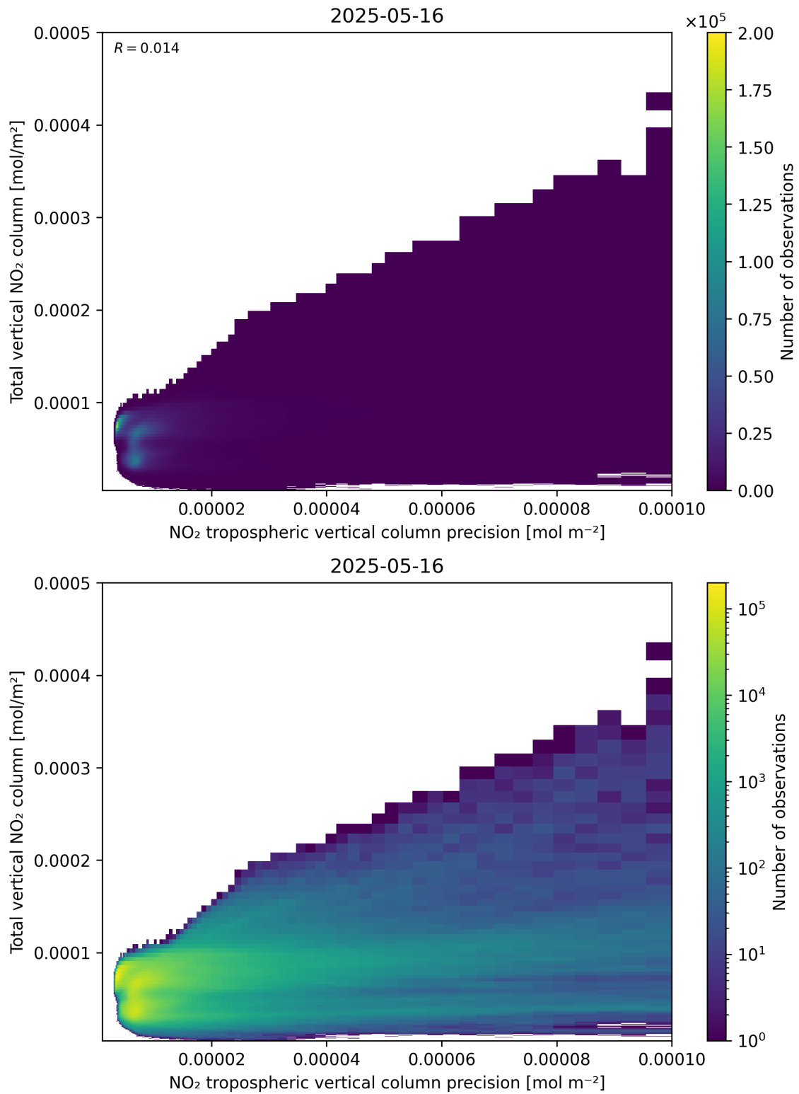
Figure 138: Scatter density plot of “NO 2 tropospheric vertical column precision” against “Total vertical NO 2 column” for 2025-05-15 to 2025-05-17.
