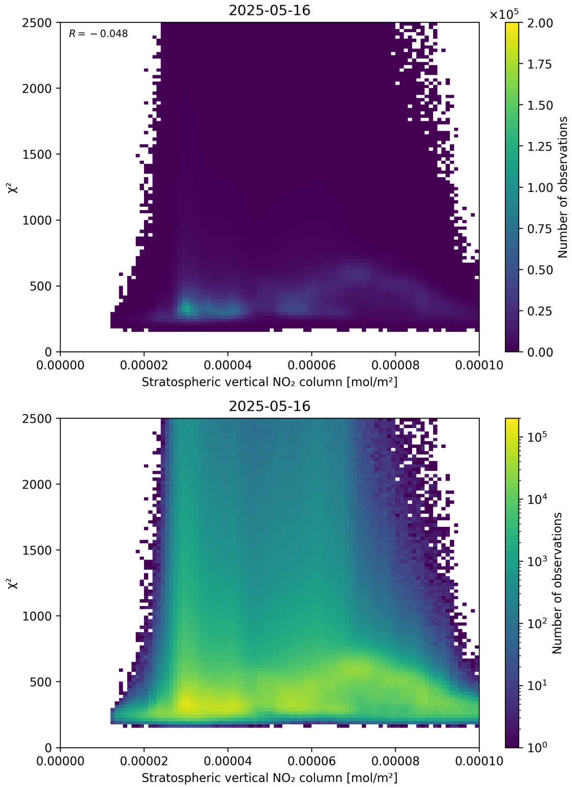
Figure 97: Scatter density plot of “Stratospheric vertical NO 2 column” against “ \chi^2 ” for 2025-05-15 to 2025-05-17.
