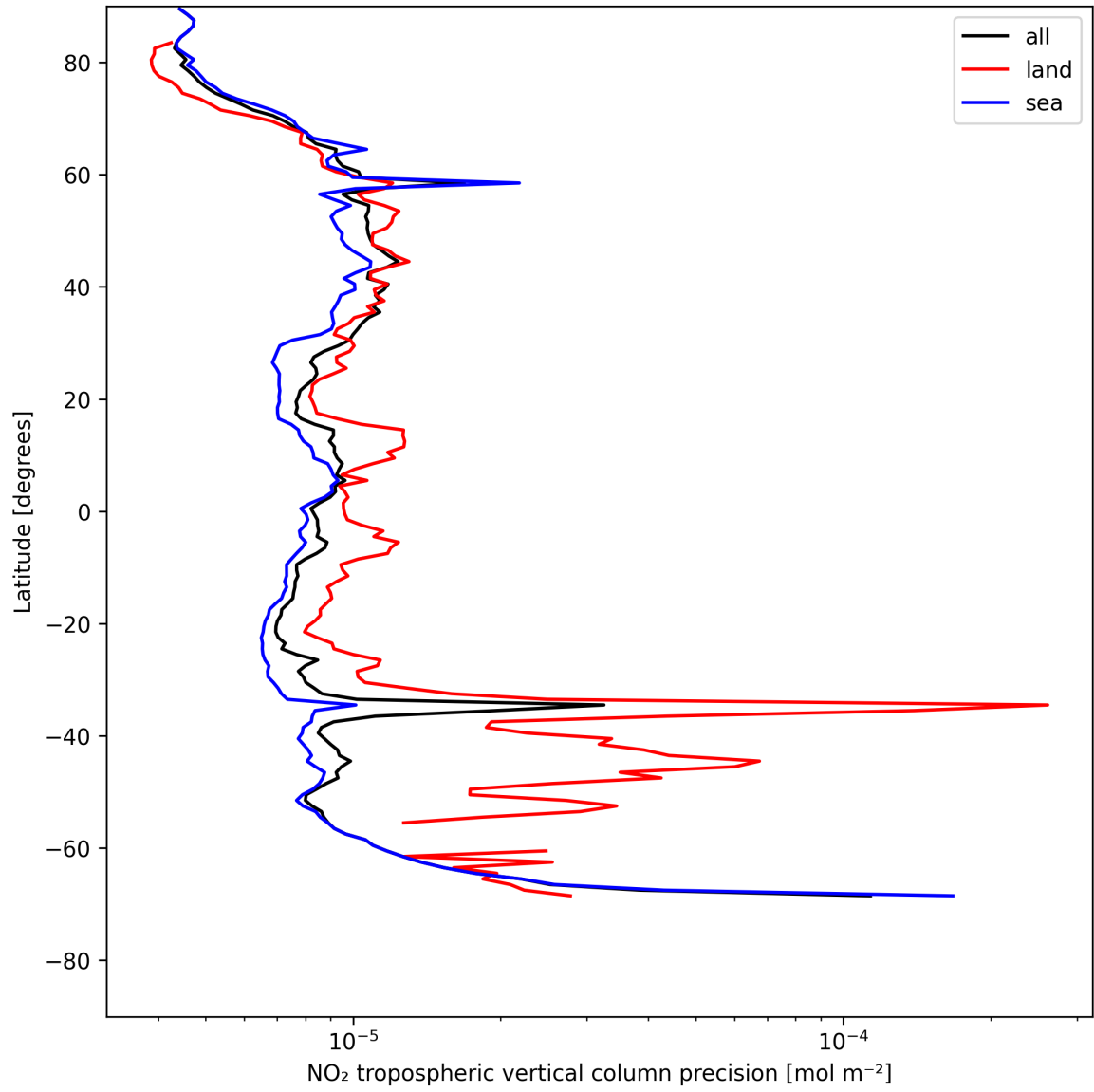
Figure 13: Zonal average of “NO 2 tropospheric vertical column precision” for 2025-05-15 to 2025-05-17.
