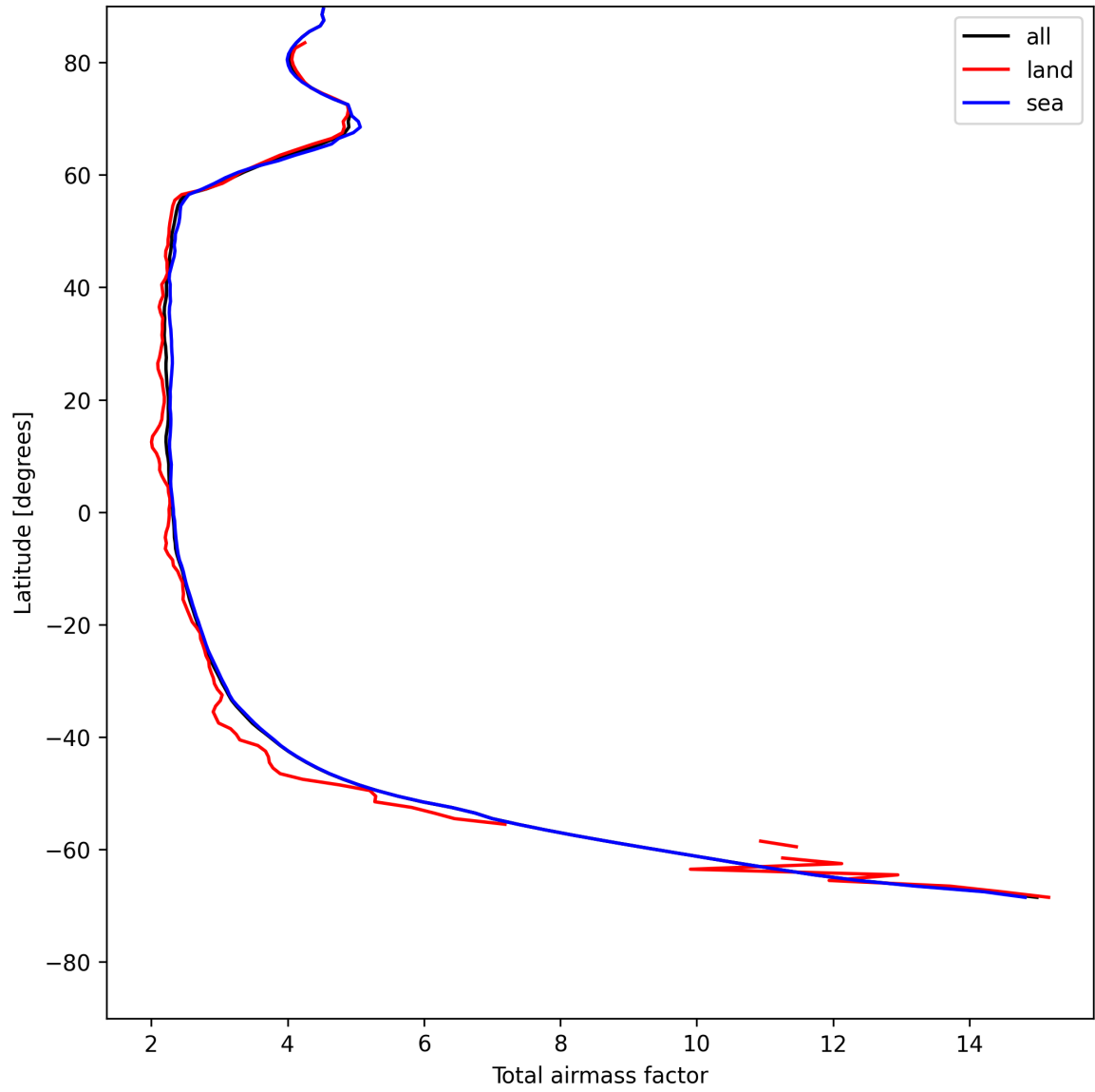
Figure 15: Zonal average of “Total airmass factor” for 2025-05-16 to 2025-05-18.
