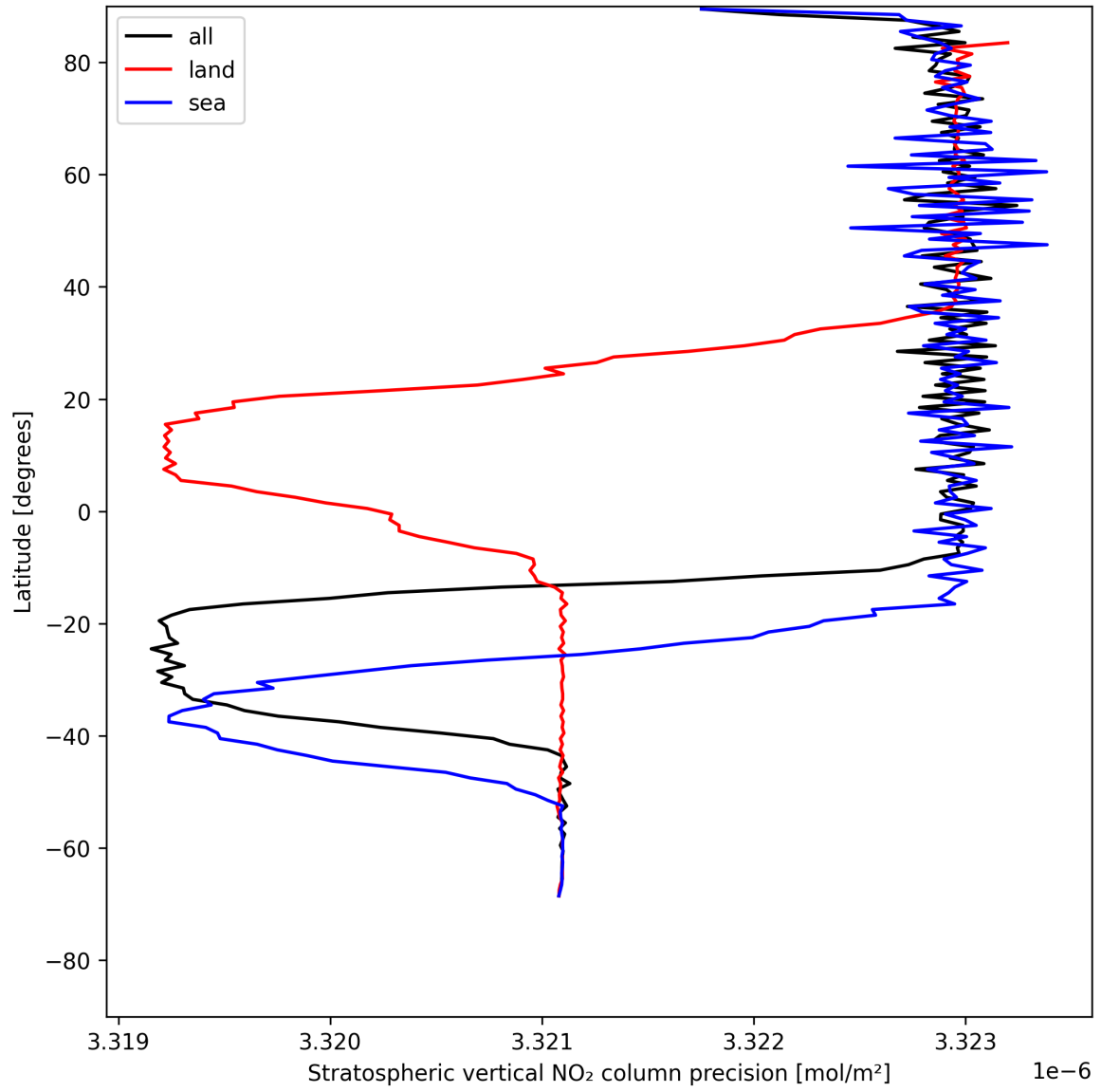
Figure 20: Zonal average of “Stratospheric vertical NO 2 column precision” for 2025-05-16 to 2025-05-18.
