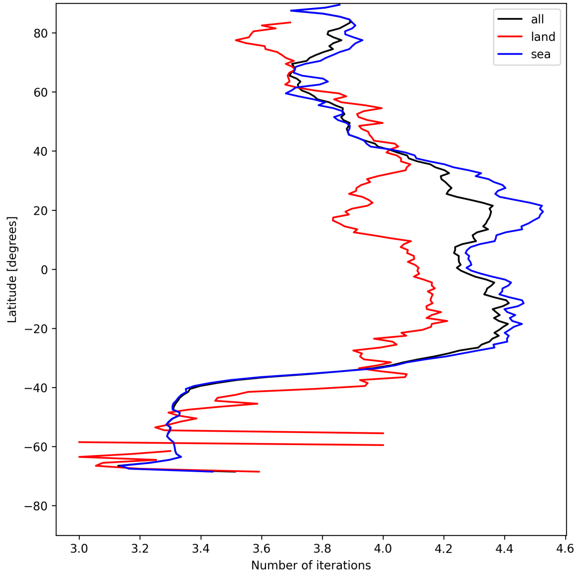
Figure 17: Zonal average of “Number of iterations” for 2025-05-16 to 2025-05-18.
