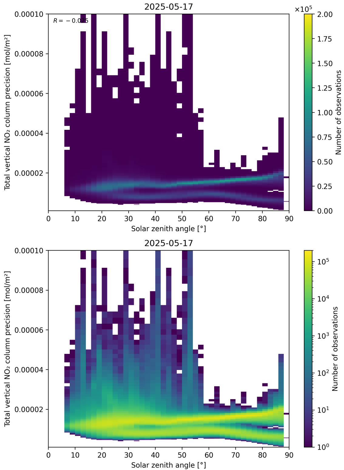
Figure 154: Scatter density plot of “Solar zenith angle” against “Total vertical NO 2 column precision” for 2025-05-16 to 2025-05-18.
