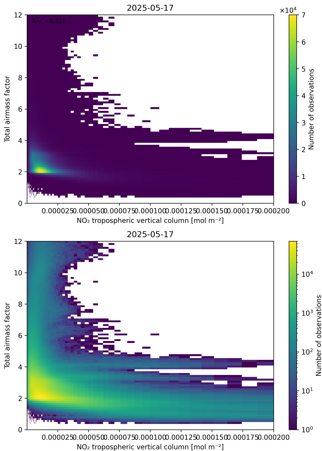
Figure 122: Scatter density plot of “NO 2 tropospheric vertical column” against “Total air mass factor” for 2025-05-16 to 2025-05-18.
