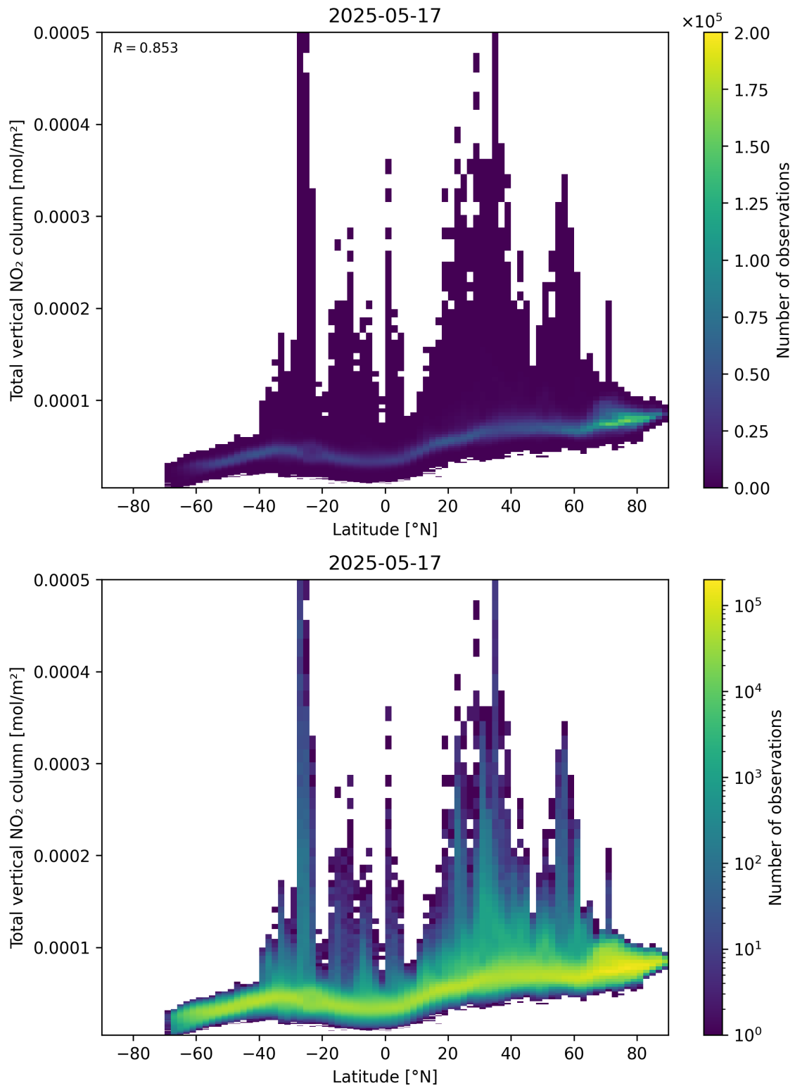
Figure 90: Scatter density plot of “Latitude” against “Total vertical NO 2 column” for 2025-05-16 to 2025-05-18.
