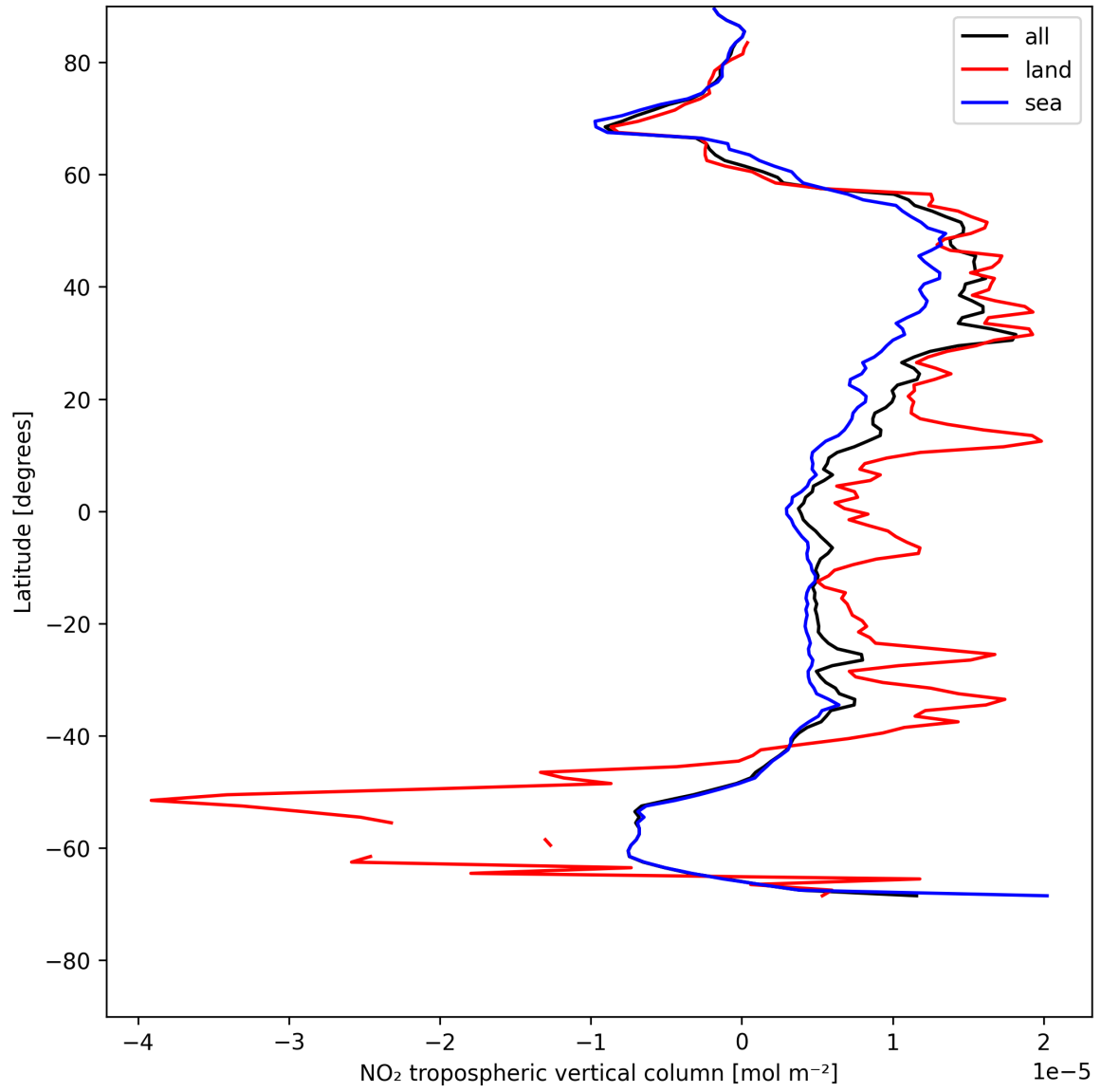
Figure 12: Zonal average of “NO 2 tropospheric vertical column” for 2025-05-16 to 2025-05-18.
