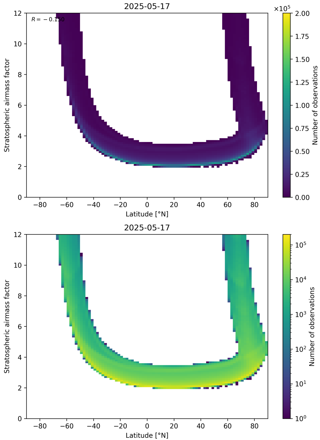
Figure 83: Scatter density plot of “Latitude” against “Stratospheric air mass factor” for 2025-05-16 to 2025-05-18.
