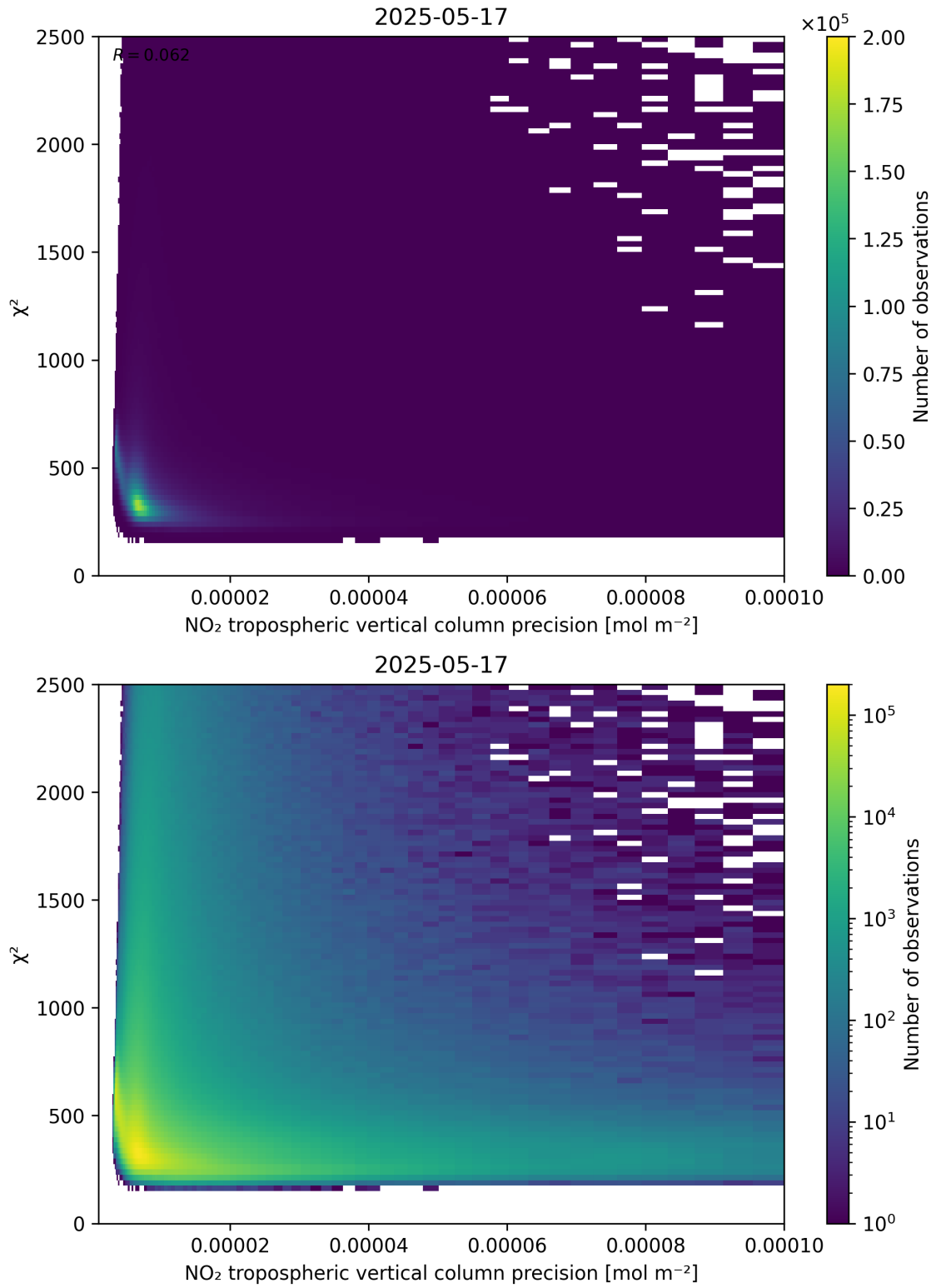
Figure 134: Scatter density plot of “NO 2 tropospheric vertical column precision” against “ \chi^2 ” for 2025-05-16 to 2025-05-18.
