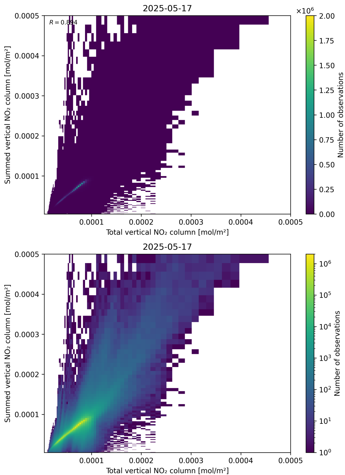
Figure 112: Scatter density plot of “Total vertical NO 2 column” against “Summed vertical NO 2 column” for 2025-05-16 to 2025-05-18.
