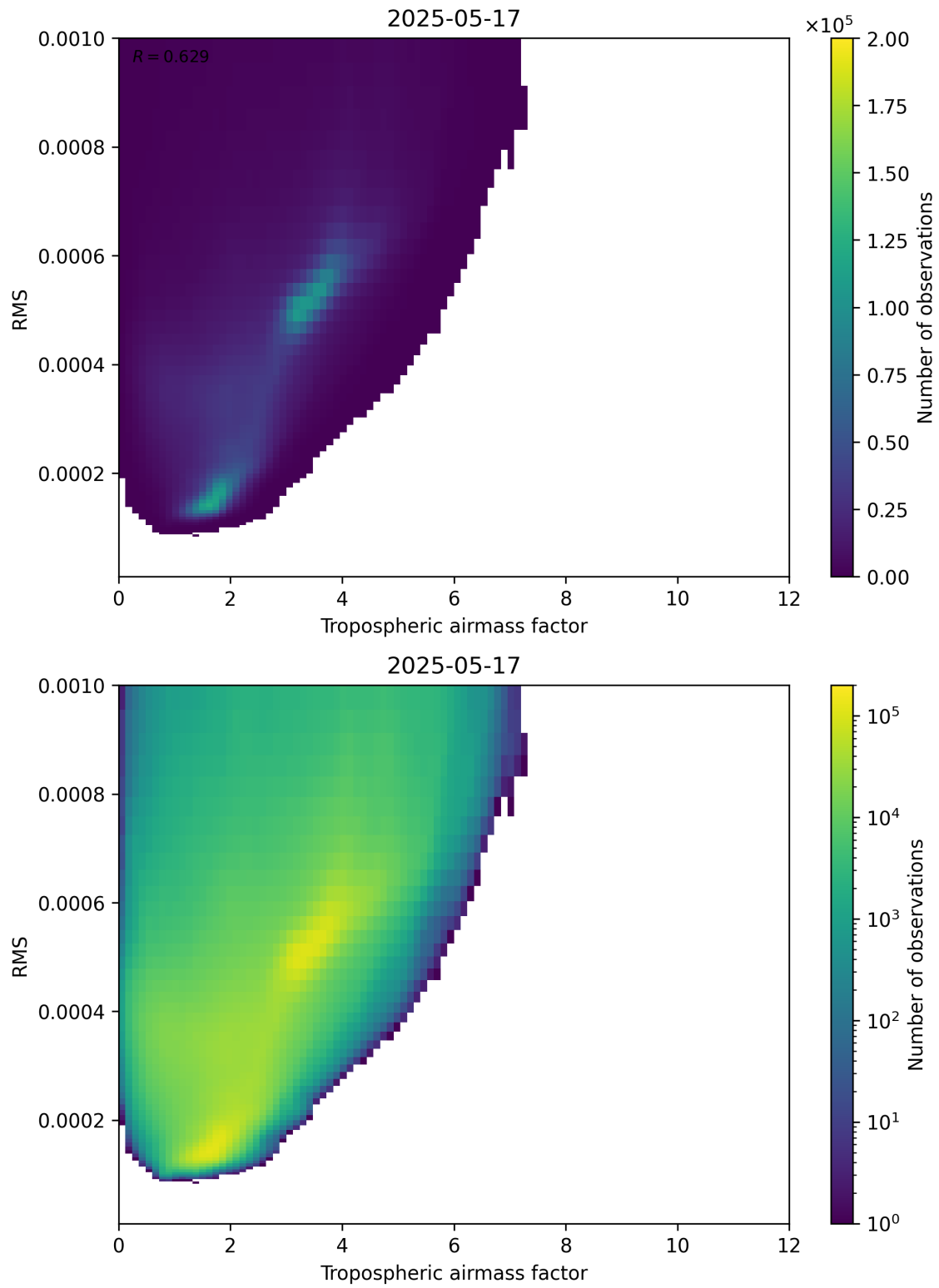
Figure 79: Scatter density plot of “Tropospheric airmass factor” against “RMS” for 2025-05-16 to 2025-05-18.
