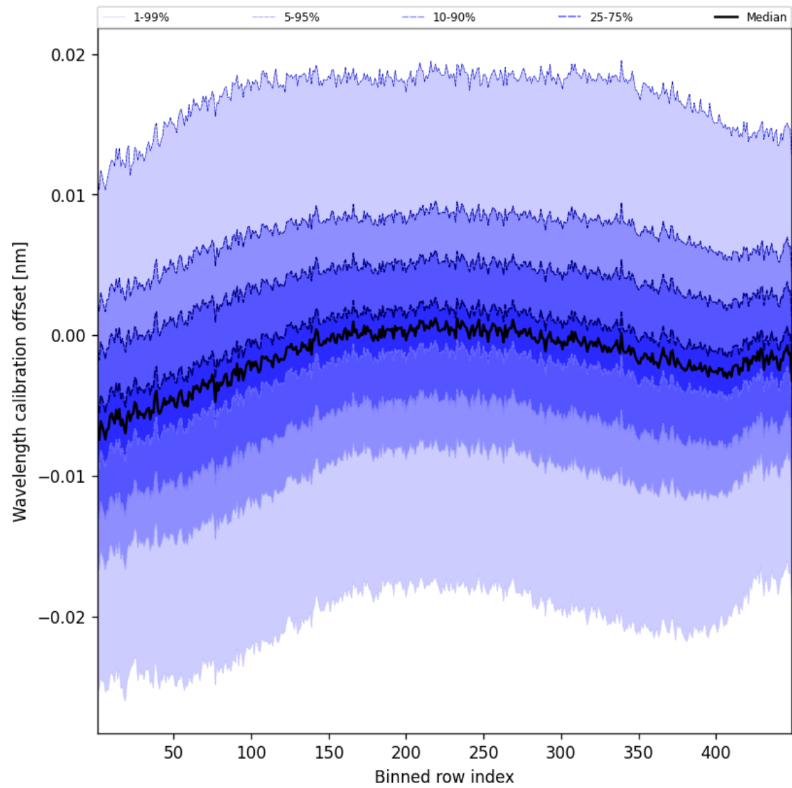
Figure 52: Along track statistics of “Wavelength calibration offset” for 2025-05-16 to 2025-05-18
