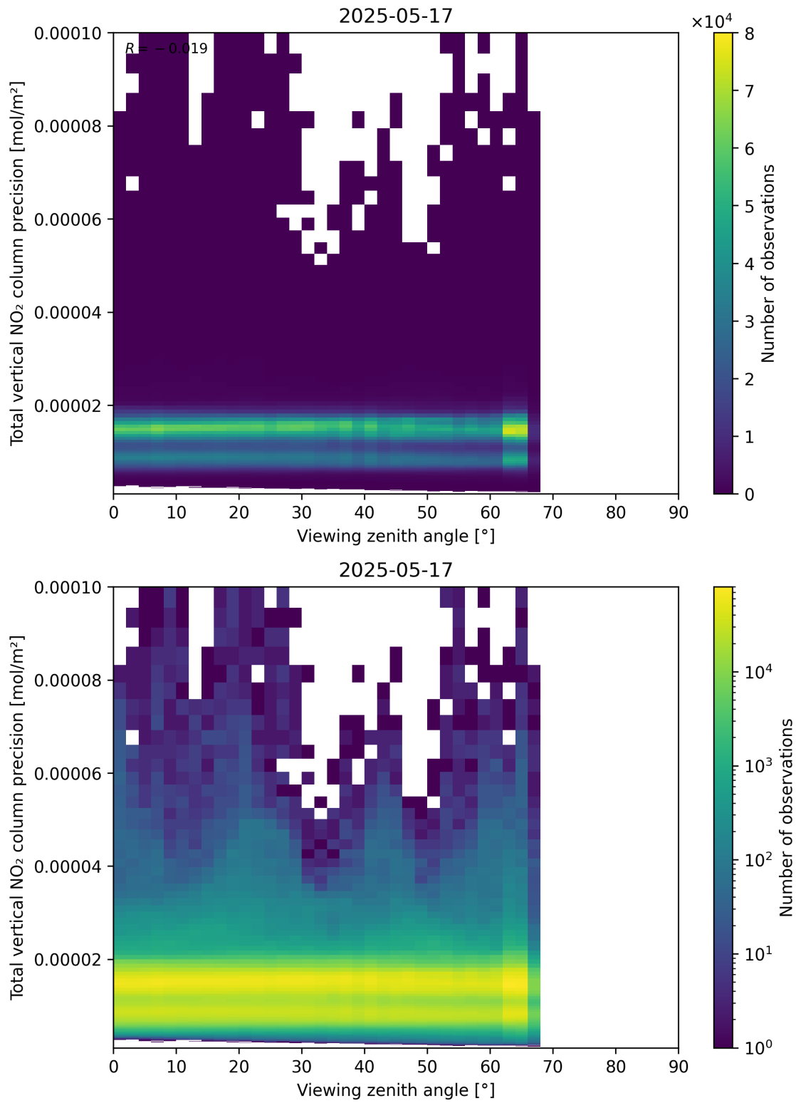
Figure 168: Scatter density plot of “Viewing zenith angle” against “Total vertical NO 2 column precision” for 2025-05-16 to 2025-05-18.
