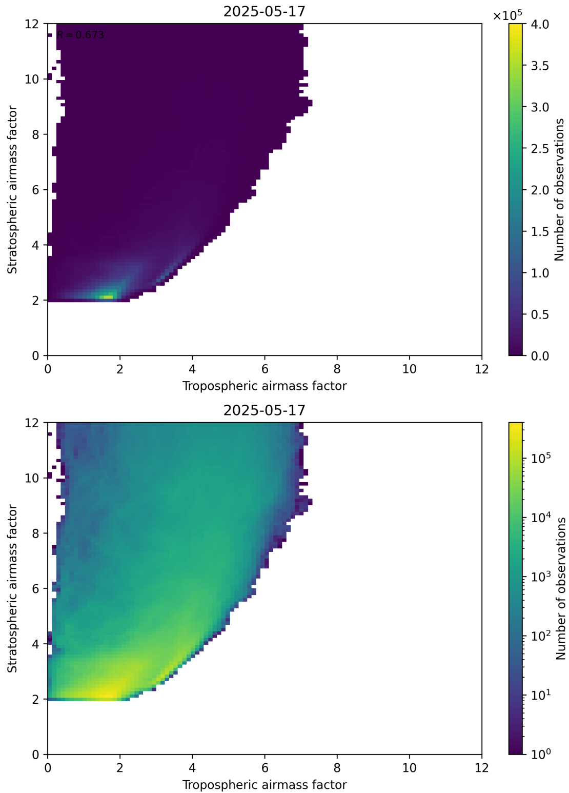
Figure 71: Scatter density plot of “Tropospheric airmass factor” against “Stratospheric airmass factor” for 2025-05-16 to 2025-05-18.
