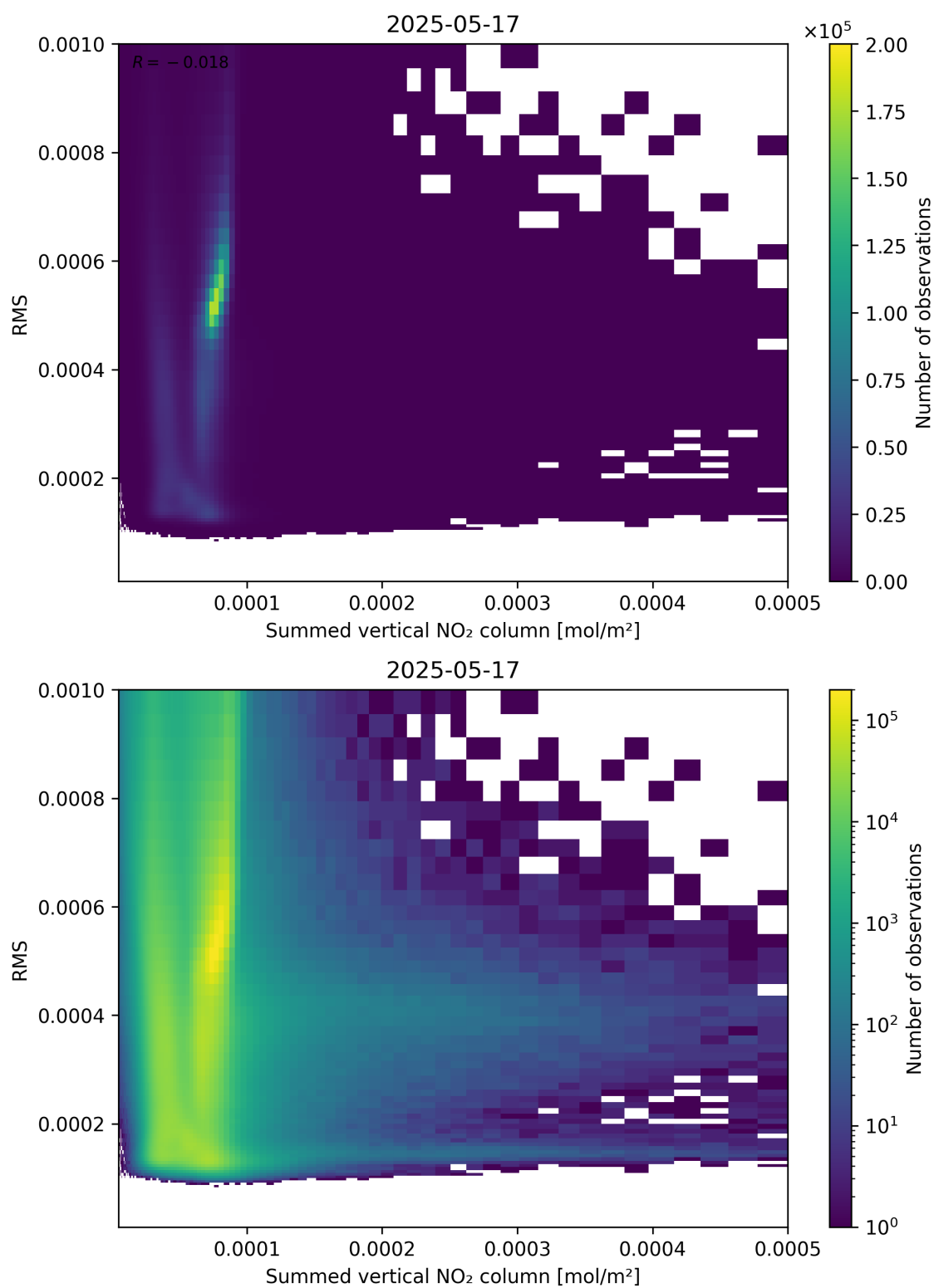
Figure 109: Scatter density plot of “Summed vertical NO 2 column” against “RMS” for 2025-05-16 to 2025-05-18.
