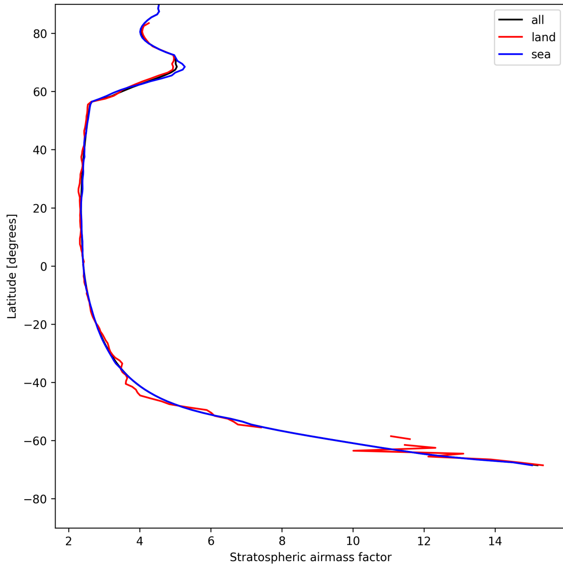
Figure 27: Zonal average of “Stratospheric air mass factor” for 2025-05-16 to 2025-05-18.
