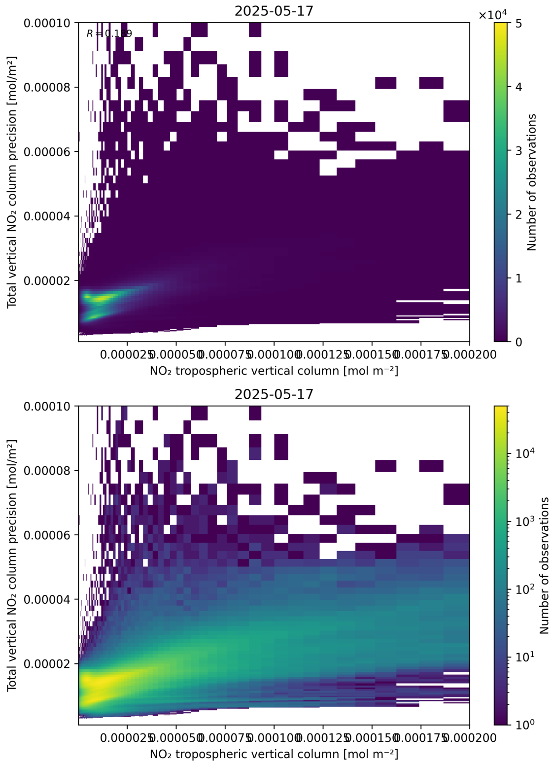
Figure 129: Scatter density plot of “NO 2 tropospheric vertical column” against “Total vertical NO 2 column precision” for 2025-05-16 to 2025-05-18.
