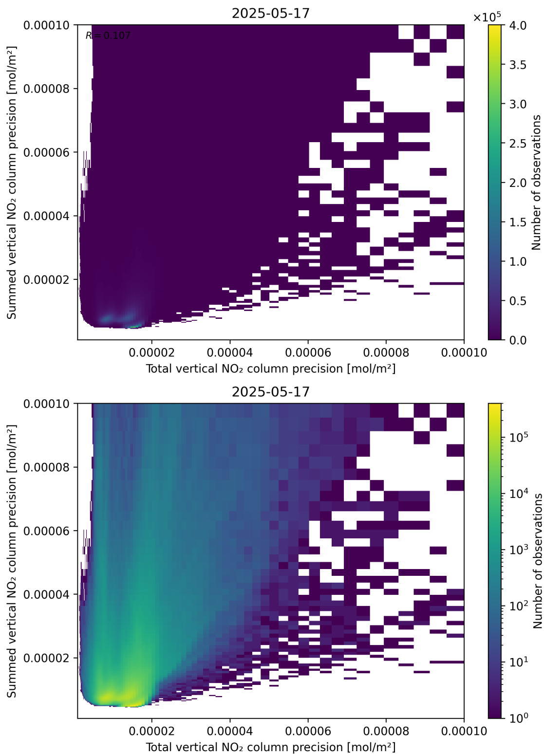
Figure 118: Scatter density plot of “Total vertical NO 2 column precision” against “Summed vertical NO 2 column precision” for 2025-05-16 to 2025-05-18.
