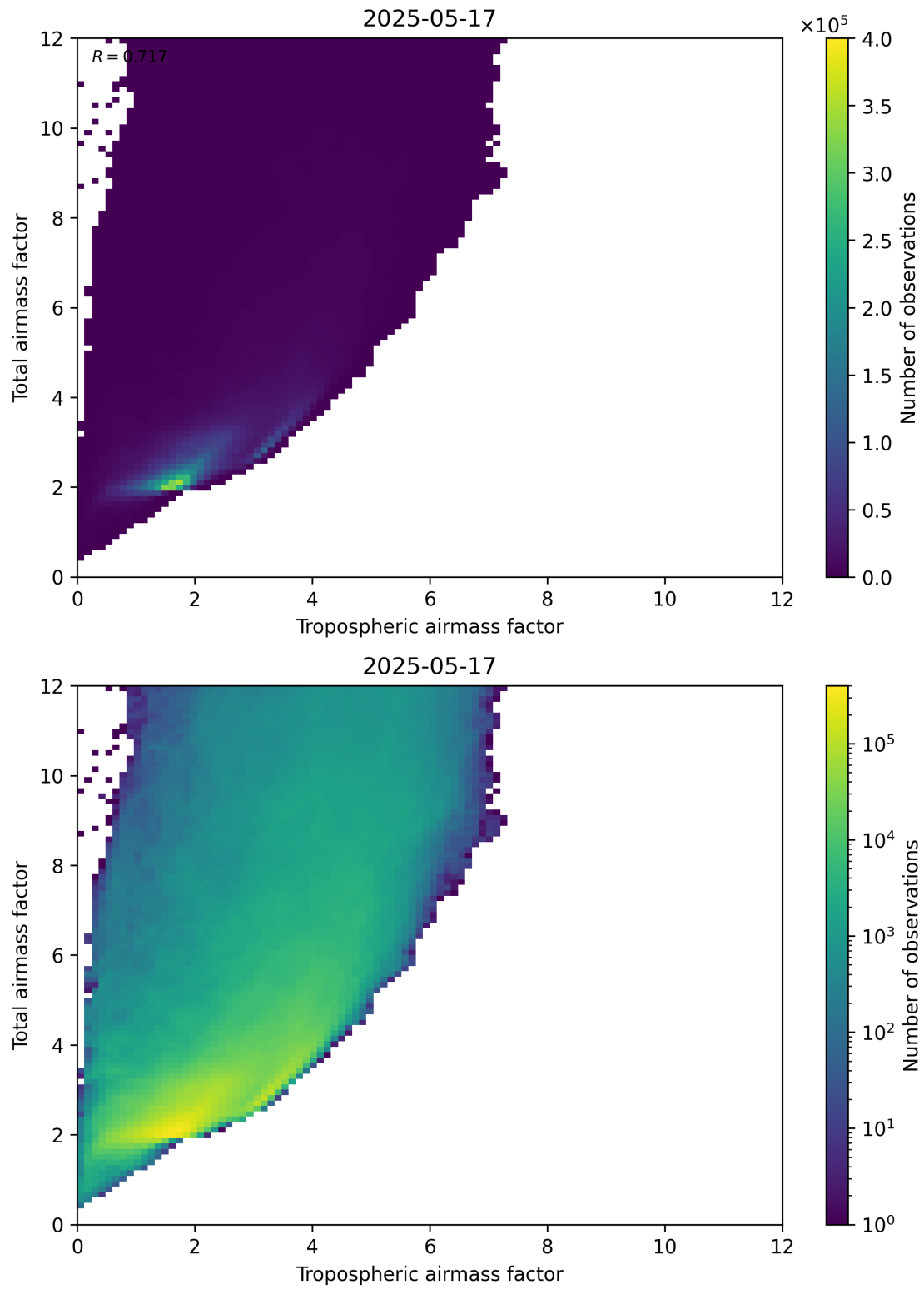
Figure 72: Scatter density plot of “Tropospheric airmass factor” against “Total airmass factor” for 2025-05-16 to 2025-05-18.
