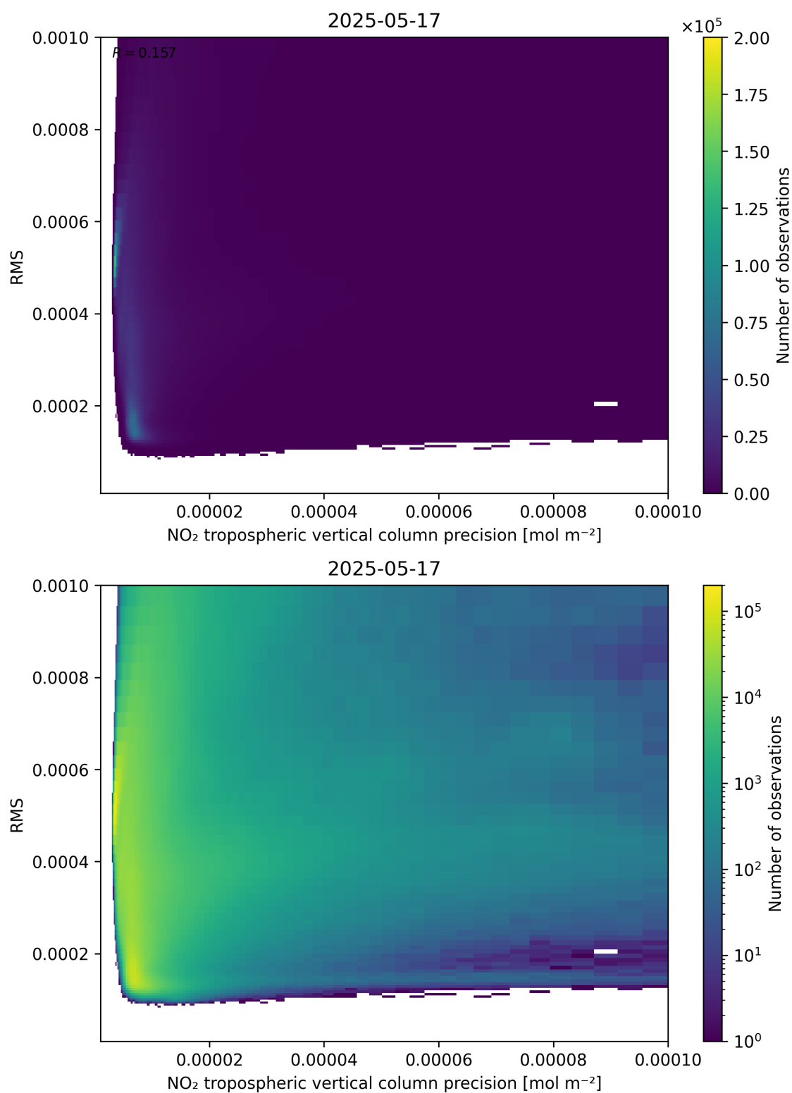
Figure 140: Scatter density plot of “NO 2 tropospheric vertical column precision” against “RMS” for 2025-05-16 to 2025-05-18.
