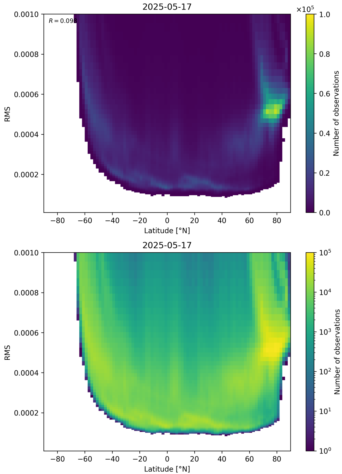
Figure 94: Scatter density plot of “Latitude” against “RMS” for 2025-05-16 to 2025-05-18.
