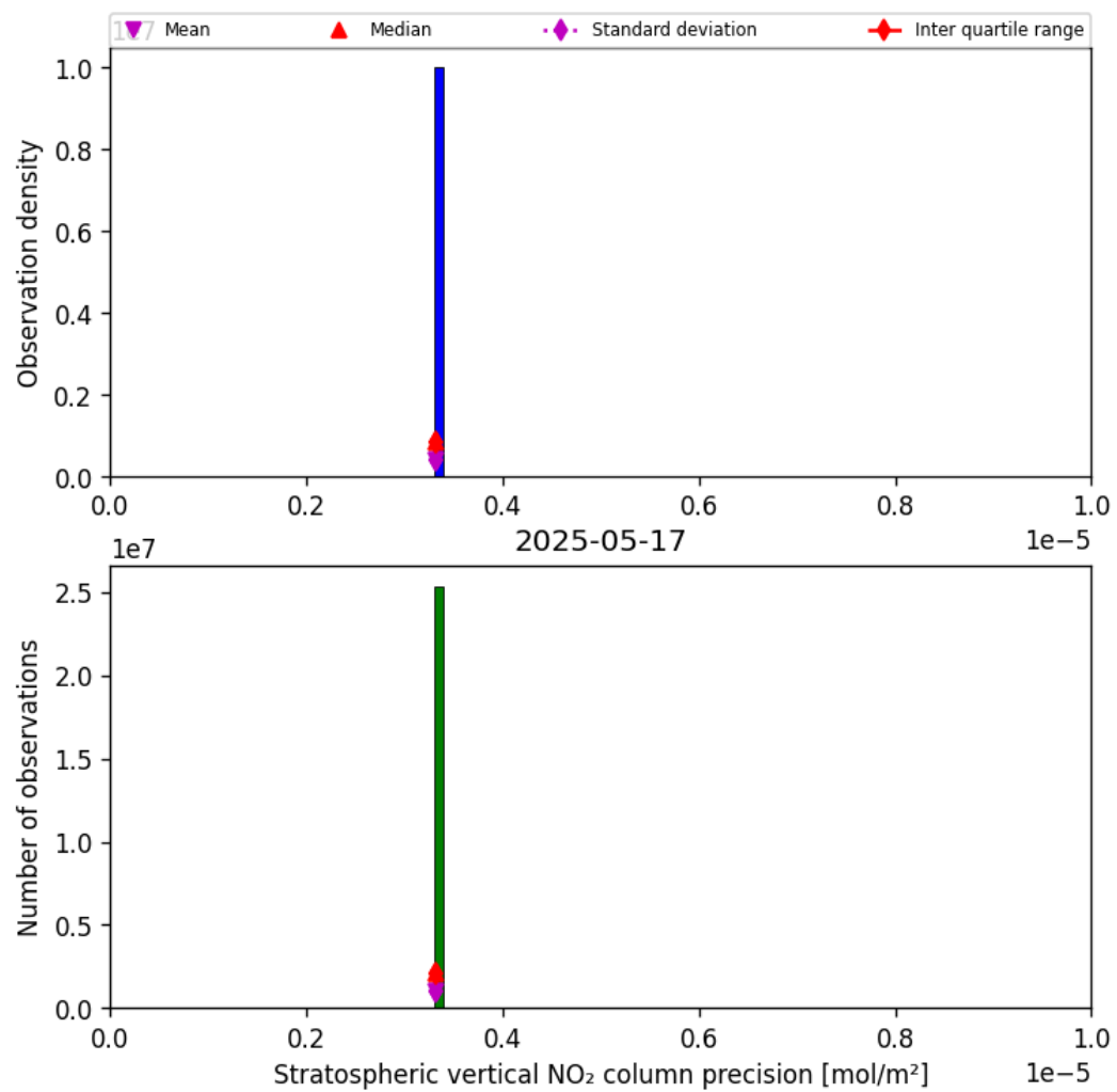
Figure 37: Histogram of “Stratospheric vertical NO 2 column precision” for 2025-05-16 to 2025-05-18
