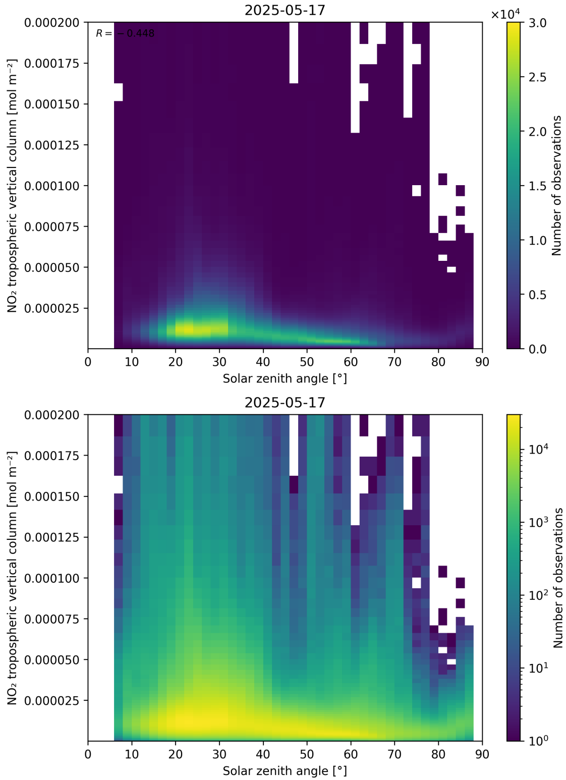
Figure 155: Scatter density plot of “Solar zenith angle” against “NO 2 tropospheric vertical column” for 2025-05-16 to 2025-05-18.
