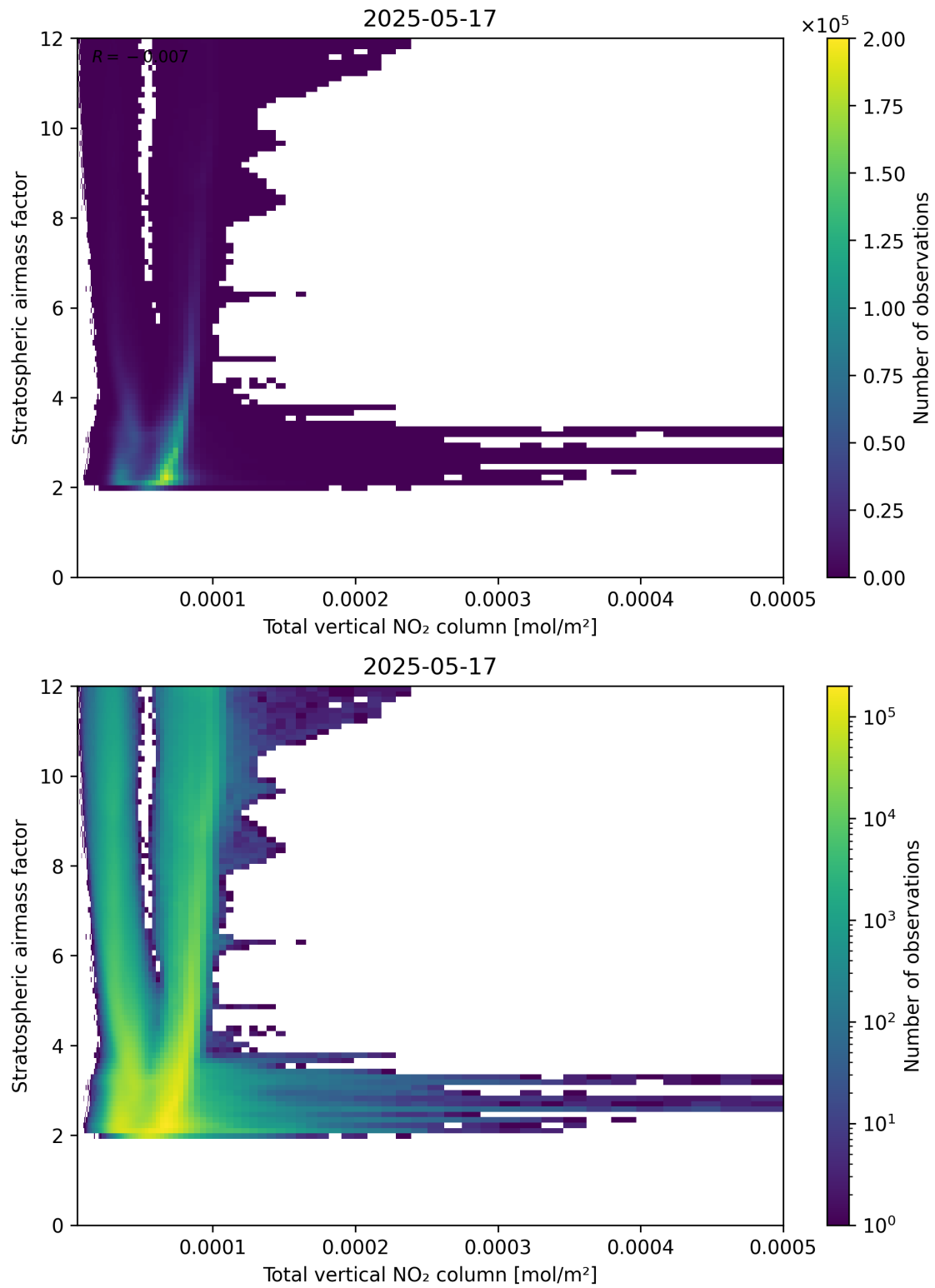
Figure 110: Scatter density plot of “Total vertical NO 2 column” against “Stratospheric airmass factor” for 2025-05-16 to 2025-05-18.
