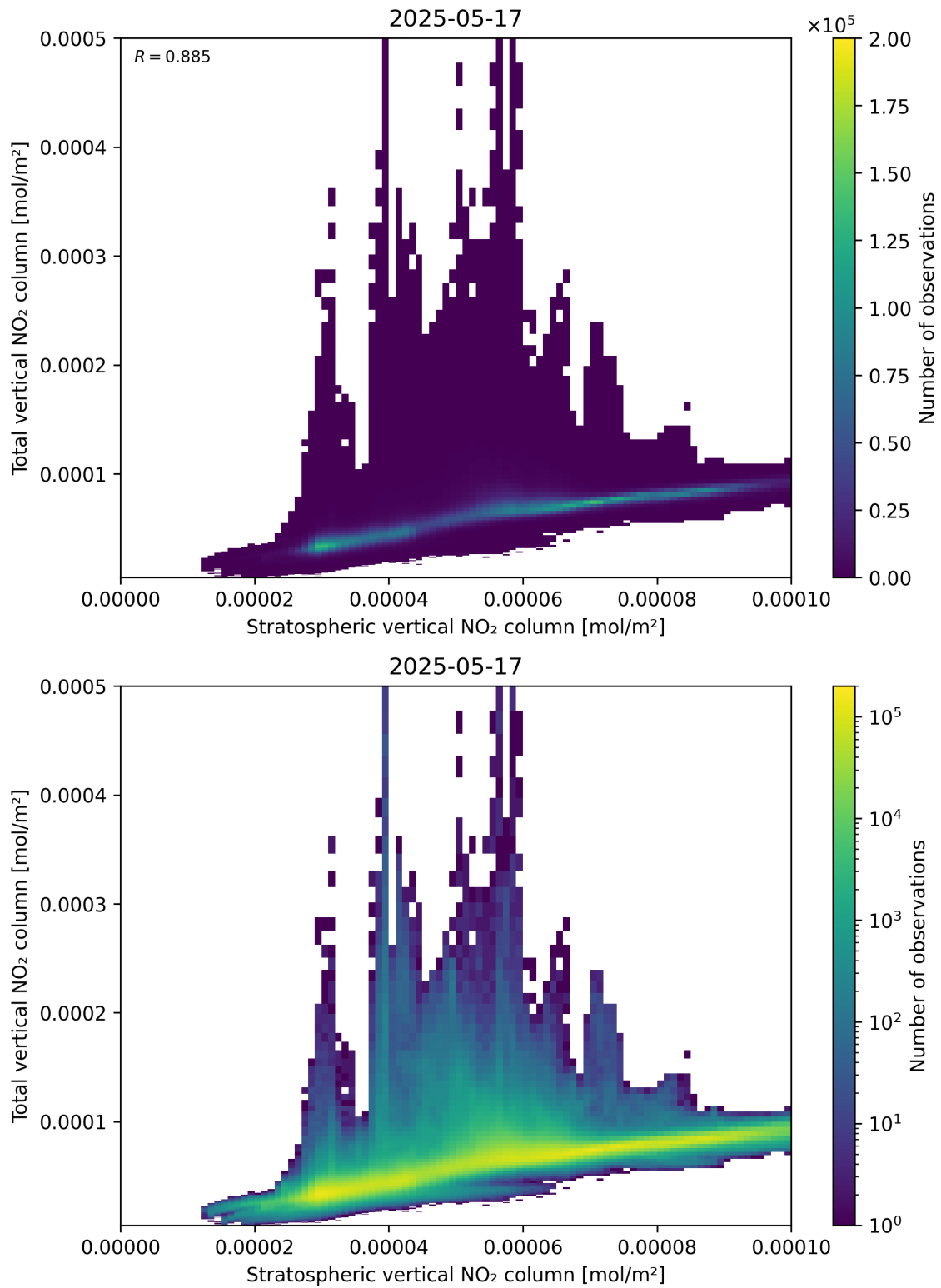
Figure 100: Scatter density plot of “Stratospheric vertical NO 2 column” against “Total vertical NO 2 column” for 2025-05-16 to 2025-05-18.
