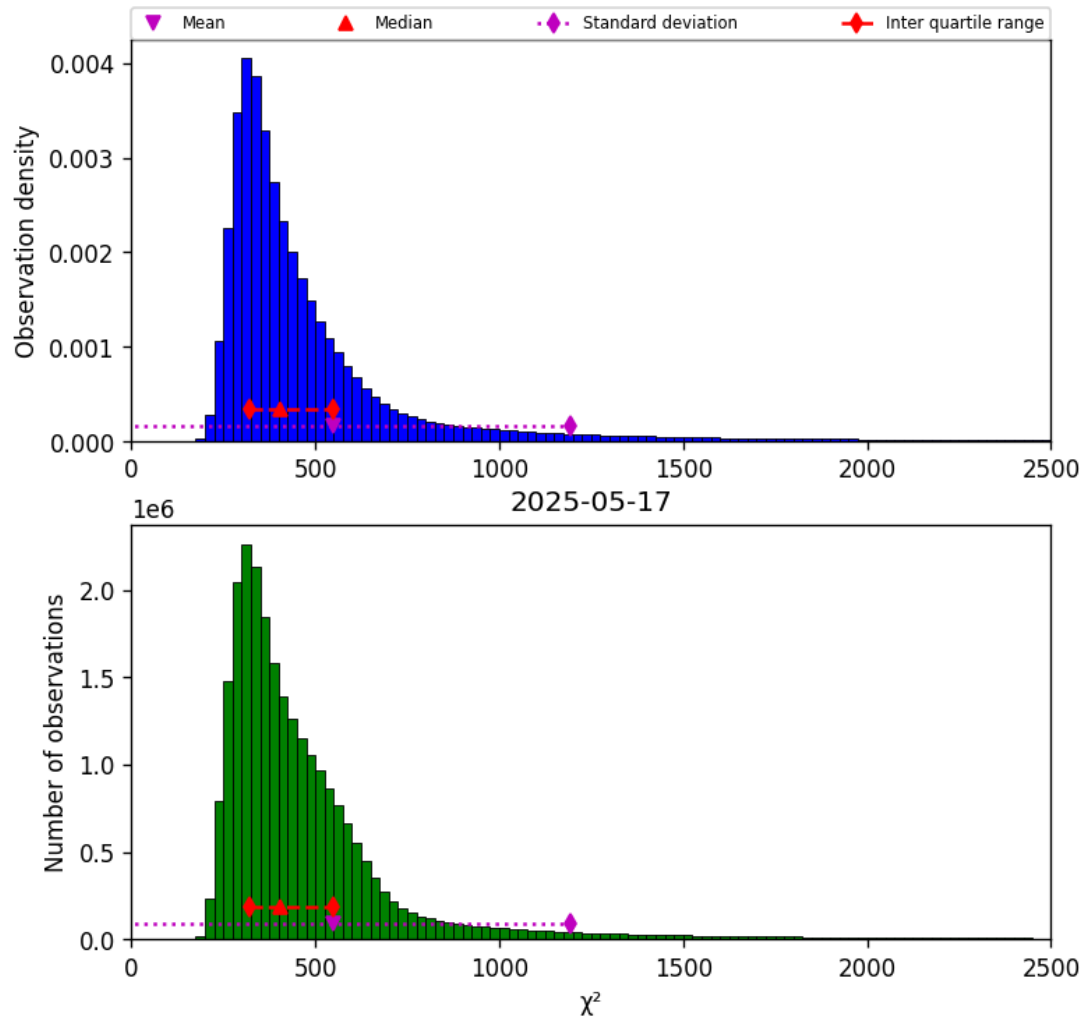
Figure 42: Histogram of “ \chi^2 ” for 2025-05-16 to 2025-05-18
