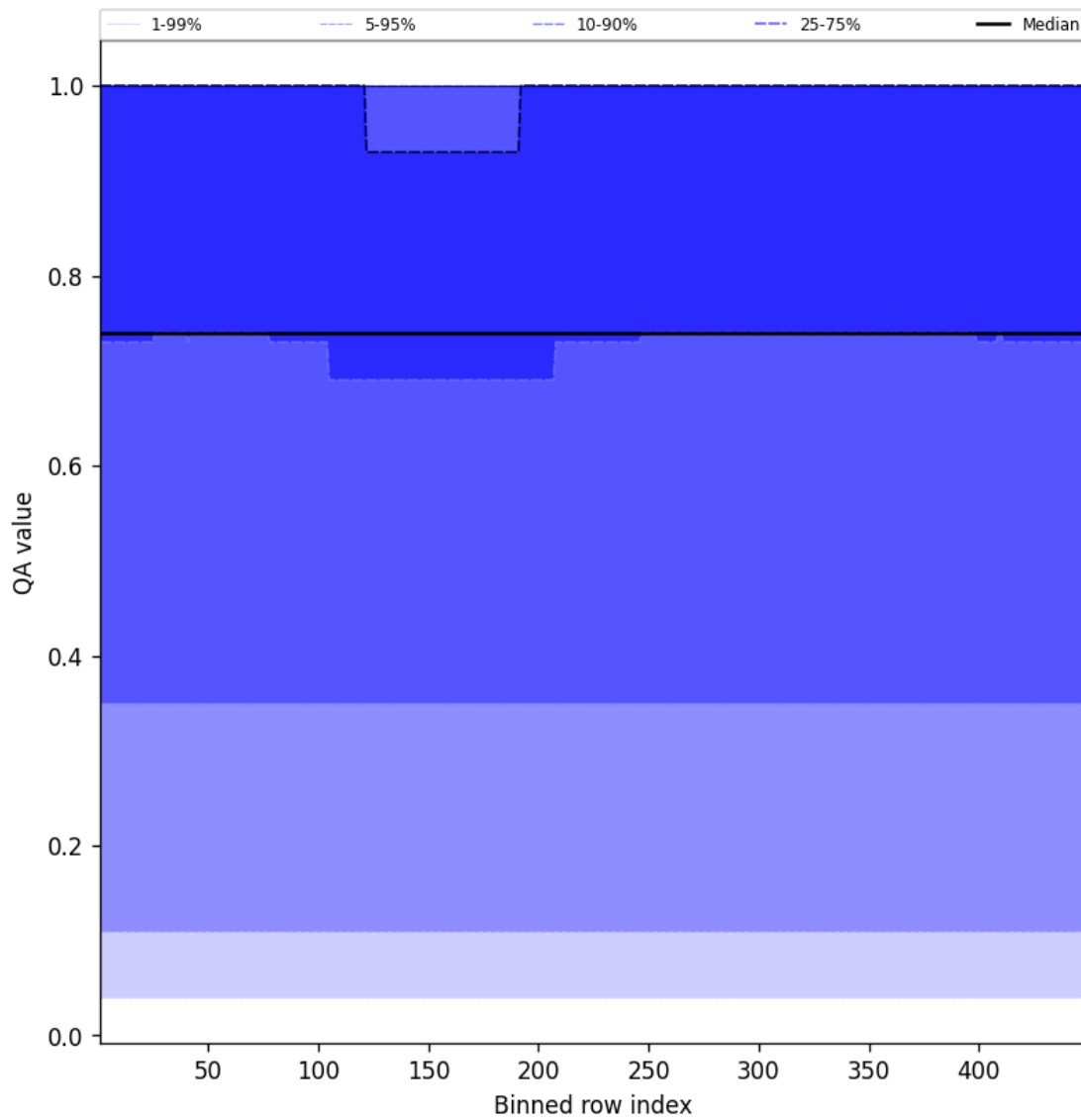
Figure 45: Along track statistics of “QA value” for 2025-05-16 to 2025-05-18
