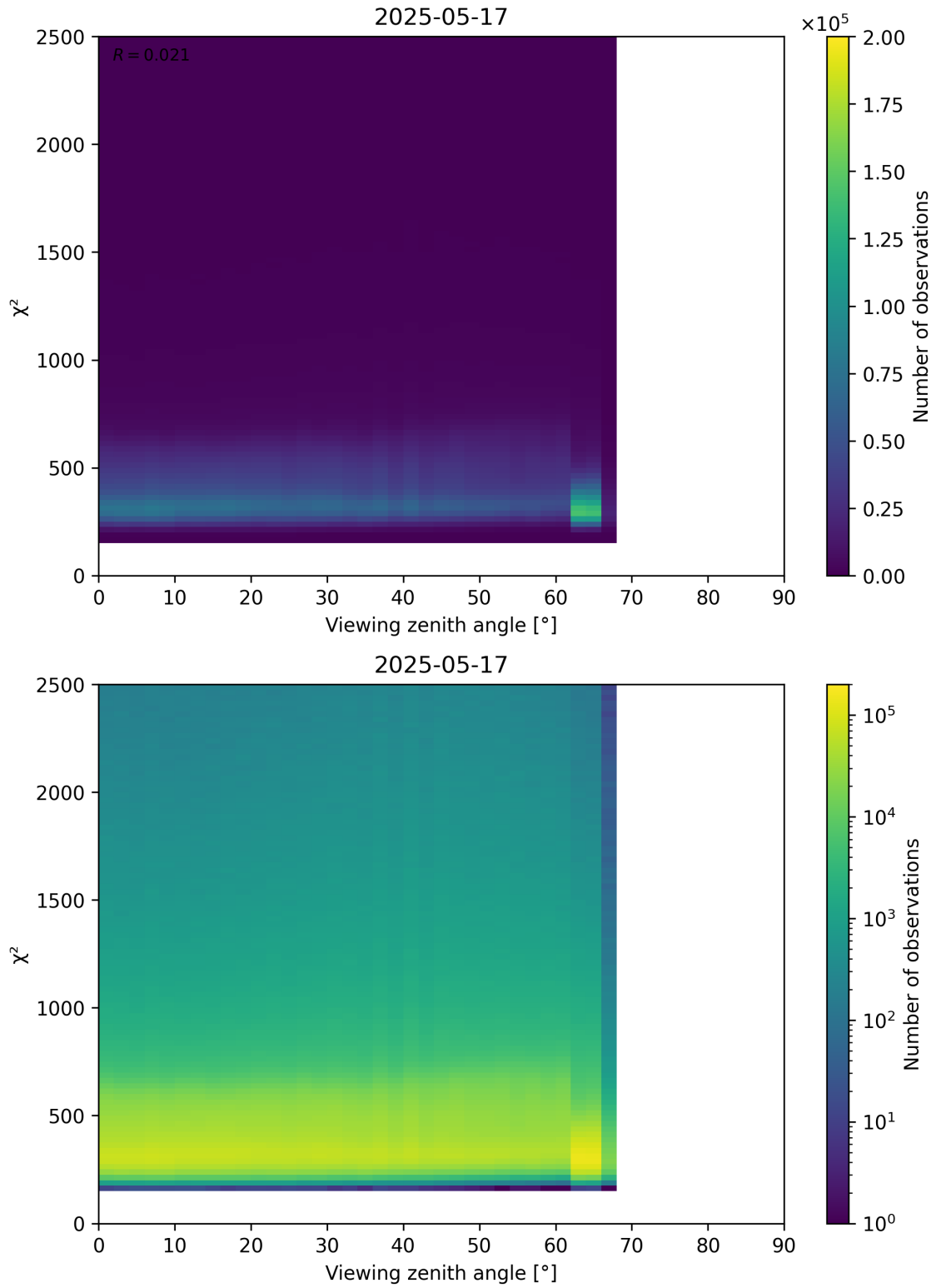
Figure 162: Scatter density plot of “Viewing zenith angle” against “ \chi^2 ” for 2025-05-16 to 2025-05-18.
