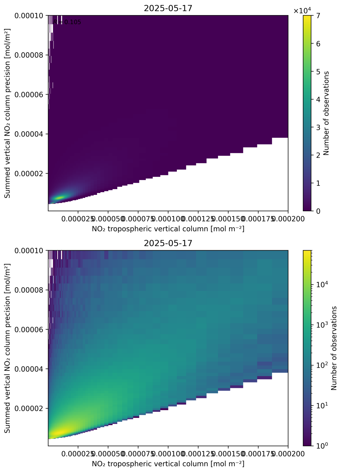
Figure 127: Scatter density plot of “NO 2 tropospheric vertical column” against “Summed vertical NO 2 column precision” for 2025-05-16 to 2025-05-18.
