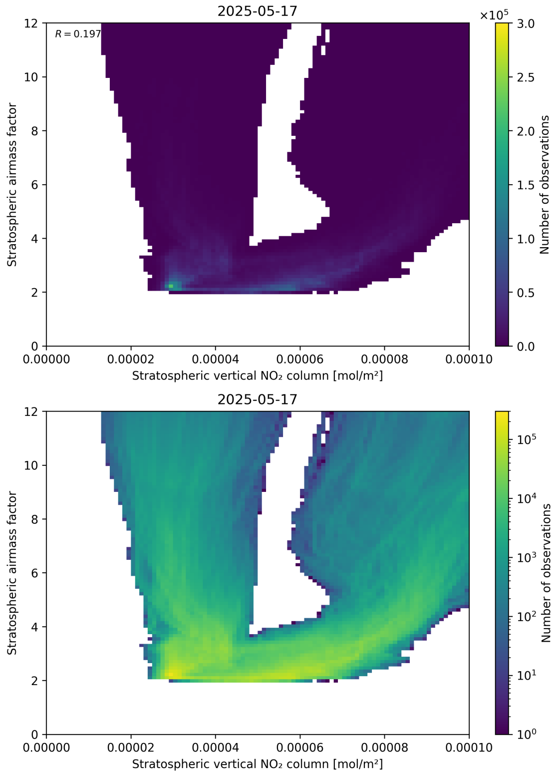
Figure 96: Scatter density plot of “Stratospheric vertical NO 2 column” against “Stratospheric airmass factor” for 2025-05-16 to 2025-05-18.
