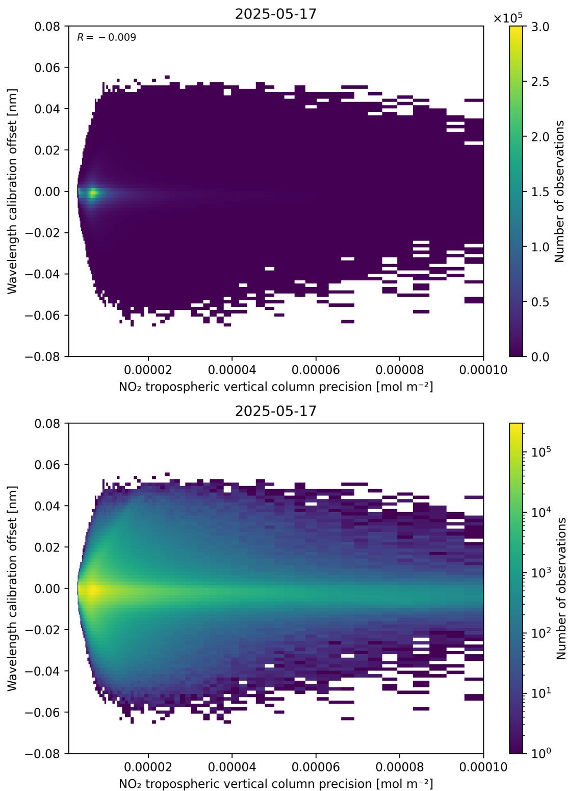
Figure 141: Scatter density plot of “NO 2 tropospheric vertical column precision” against “Wavelength calibration offset” for 2025-05-16 to 2025-05-18.
