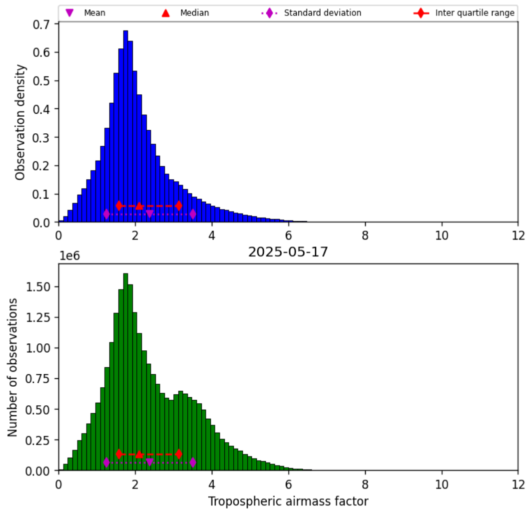
Figure 31: Histogram of “Tropospheric airmass factor” for 2025-05-16 to 2025-05-18
