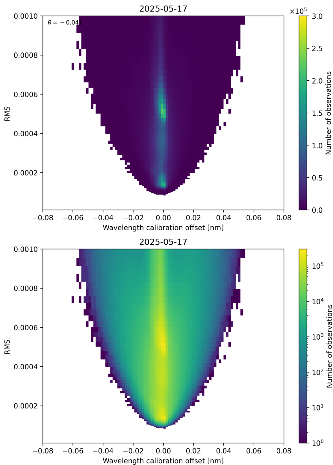
Figure 181: Scatter density plot of “Wavelength calibration offset” against “RMS” for 2025-05-16 to 2025-05-18.
