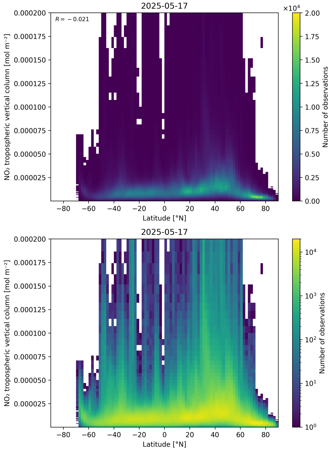
Figure 92: Scatter density plot of “Latitude” against “NO 2 tropospheric vertical column” for 2025-05-16 to 2025-05-18.
