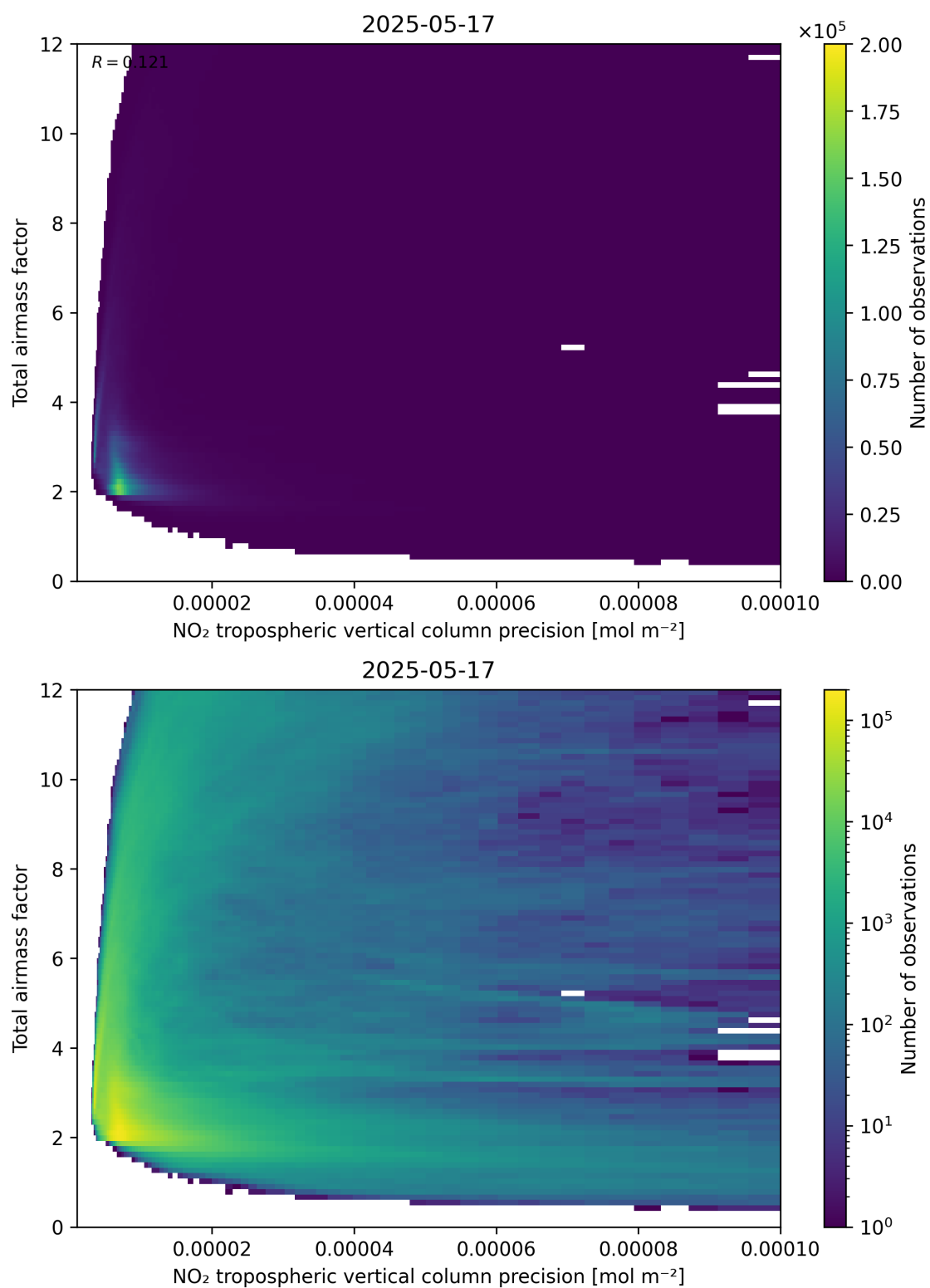
Figure 132: Scatter density plot of “NO 2 tropospheric vertical column precision” against “Total air mass factor” for 2025-05-16 to 2025-05-18.
