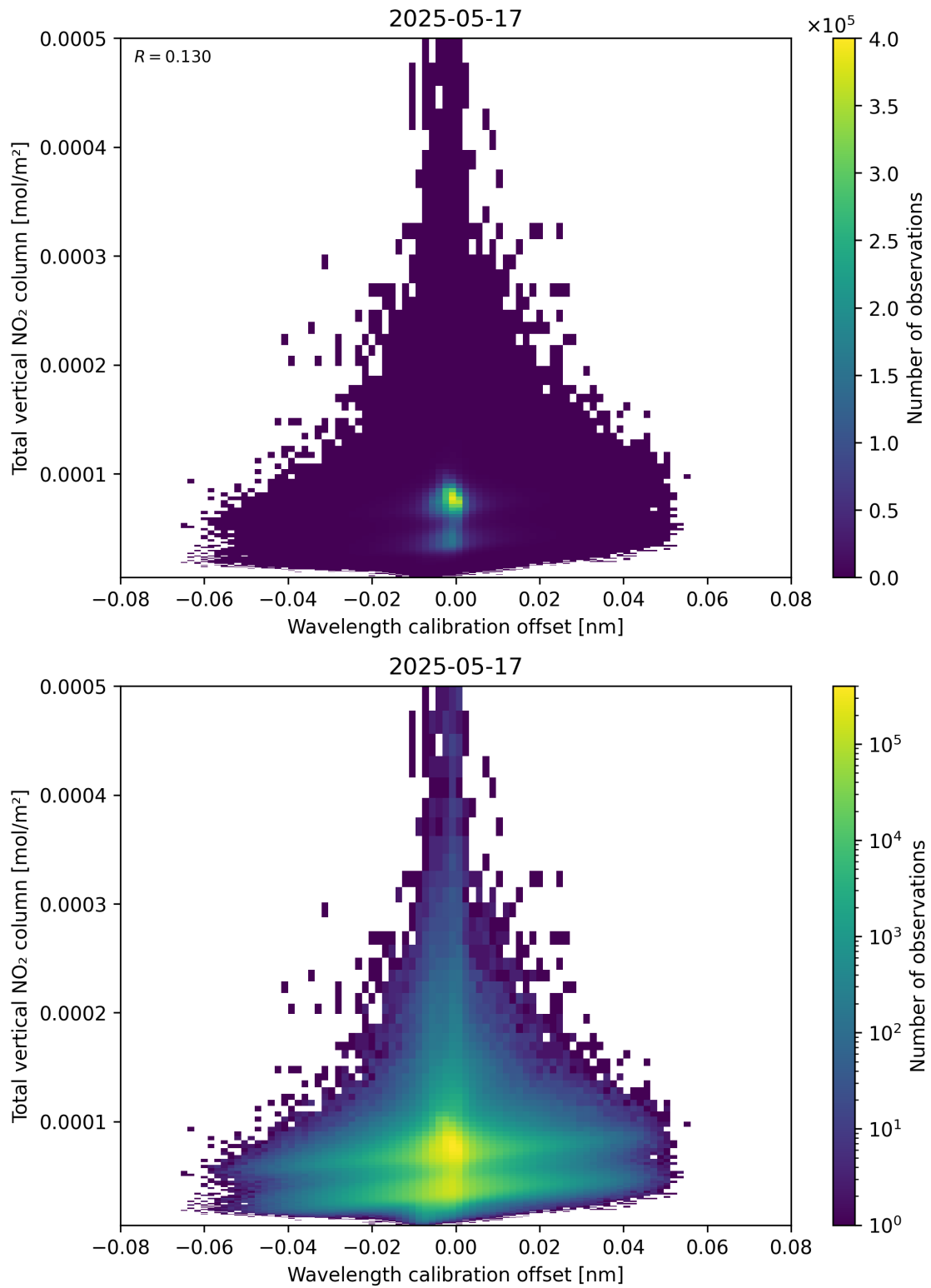
Figure 179: Scatter density plot of “Wavelength calibration offset” against “Total vertical NO 2 column” for 2025-05-16 to 2025-05-18.
