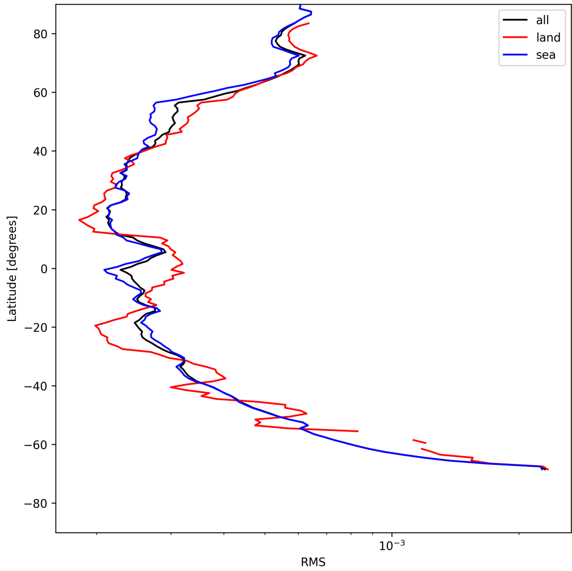
Figure 26: Zonal average of “RMS” for 2025-05-16 to 2025-05-18.
