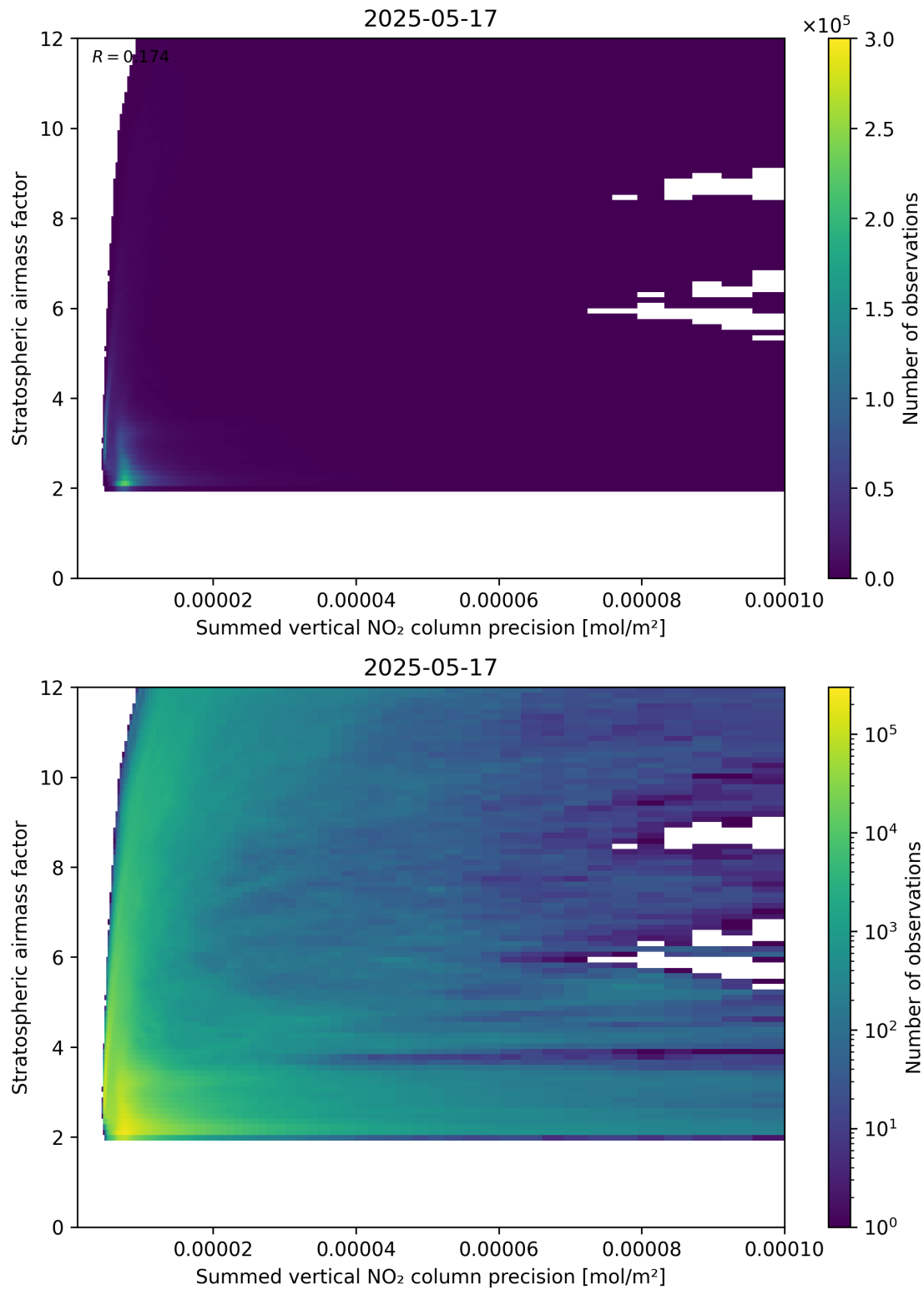
Figure 106: Scatter density plot of “Summed vertical NO 2 column precision” against “Stratospheric airmass factor” for 2025-05-16 to 2025-05-18.
