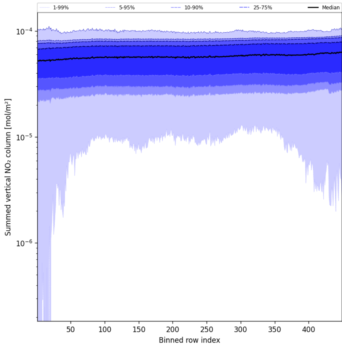
Figure 57: Along track statistics of “Summed vertical NO 2 column” for 2025-05-16 to 2025-05-18
