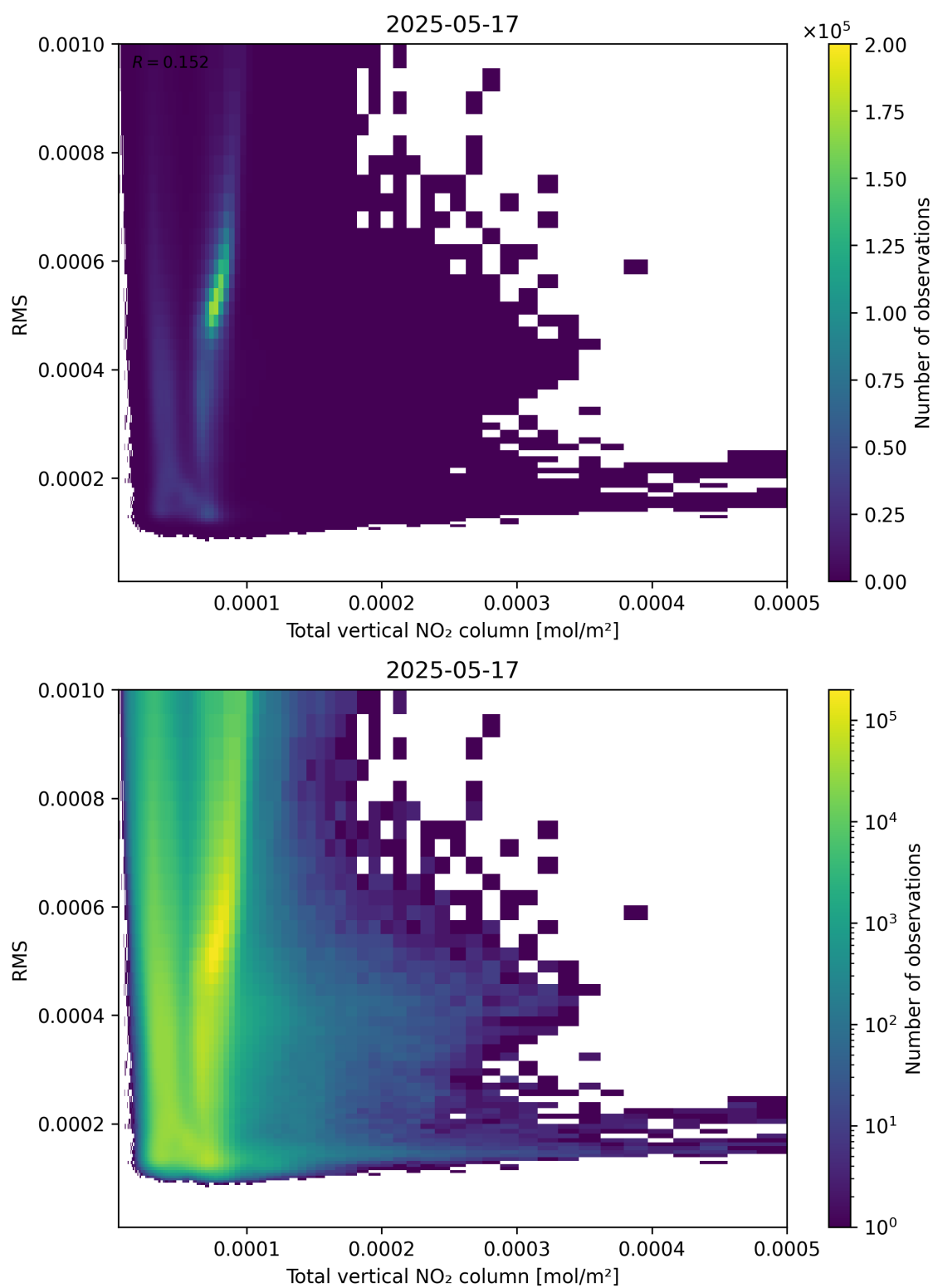
Figure 120: Scatter density plot of “Total vertical NO 2 column” against “RMS” for 2025-05-16 to 2025-05-18.
