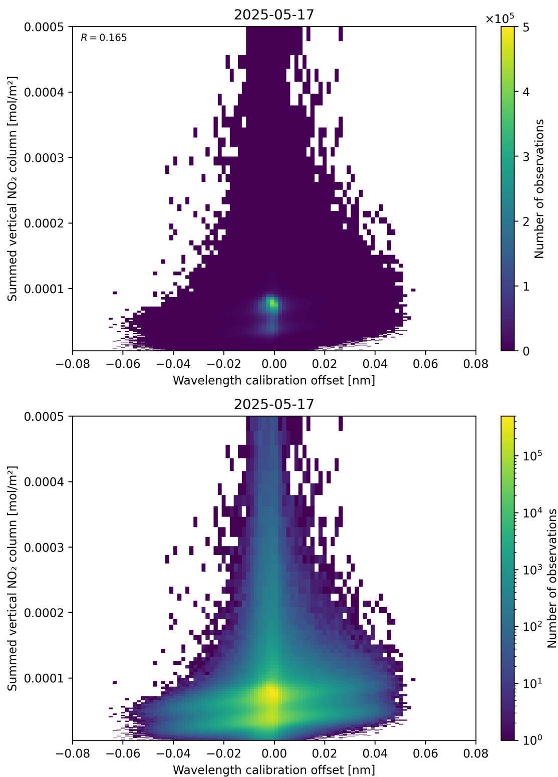
Figure 177: Scatter density plot of “Wavelength calibration offset” against “Summed vertical NO 2 column” for 2025-05-16 to 2025-05-18.
