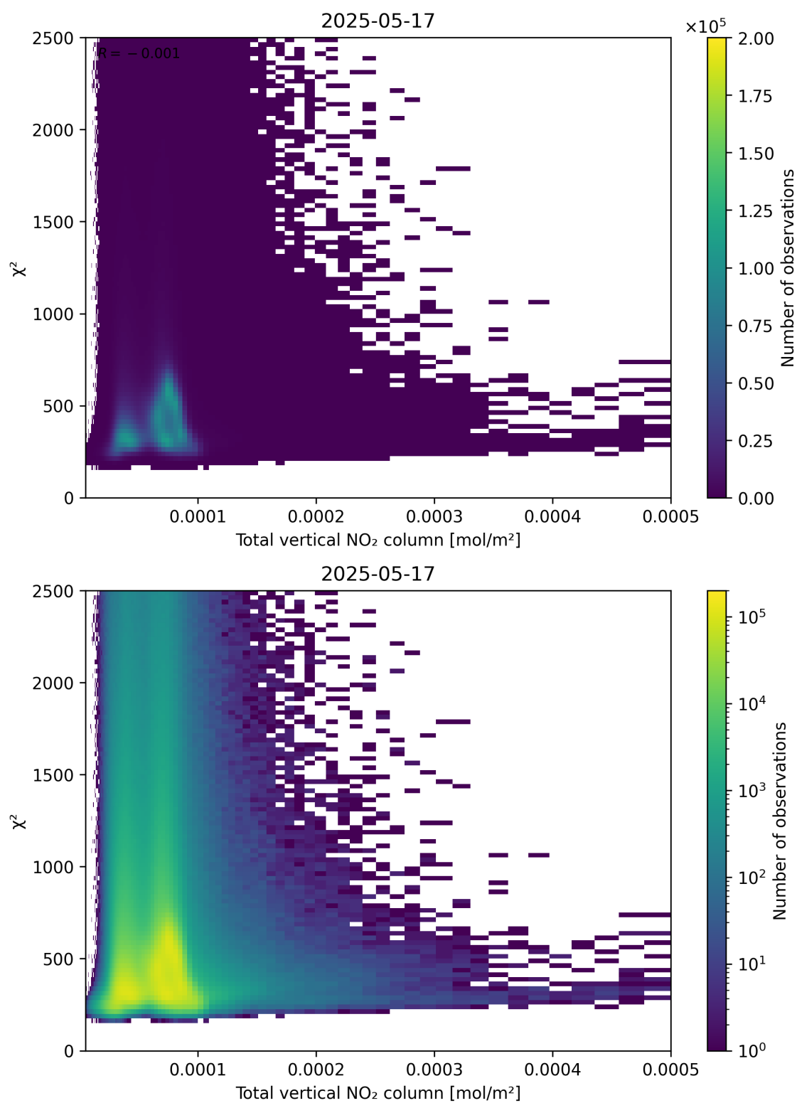
Figure 111: Scatter density plot of “Total vertical NO 2 column” against “ \chi^2 ” for 2025-05-16 to 2025-05-18.
