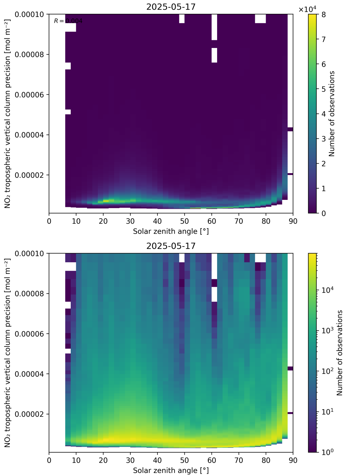
Figure 156: Scatter density plot of “Solar zenith angle” against “NO 2 tropospheric vertical column precision” for 2025-05-16 to 2025-05-18.
