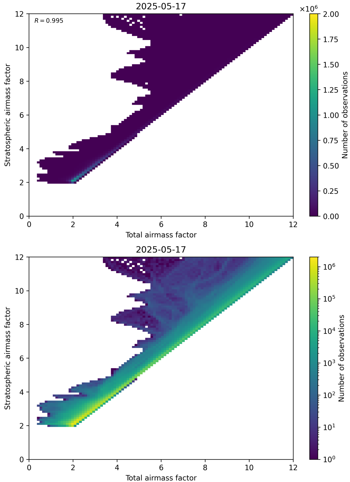
Figure 62: Scatter density plot of “Total airmass factor” against “Stratospheric airmass factor” for 2025-05-16 to 2025-05-18.
