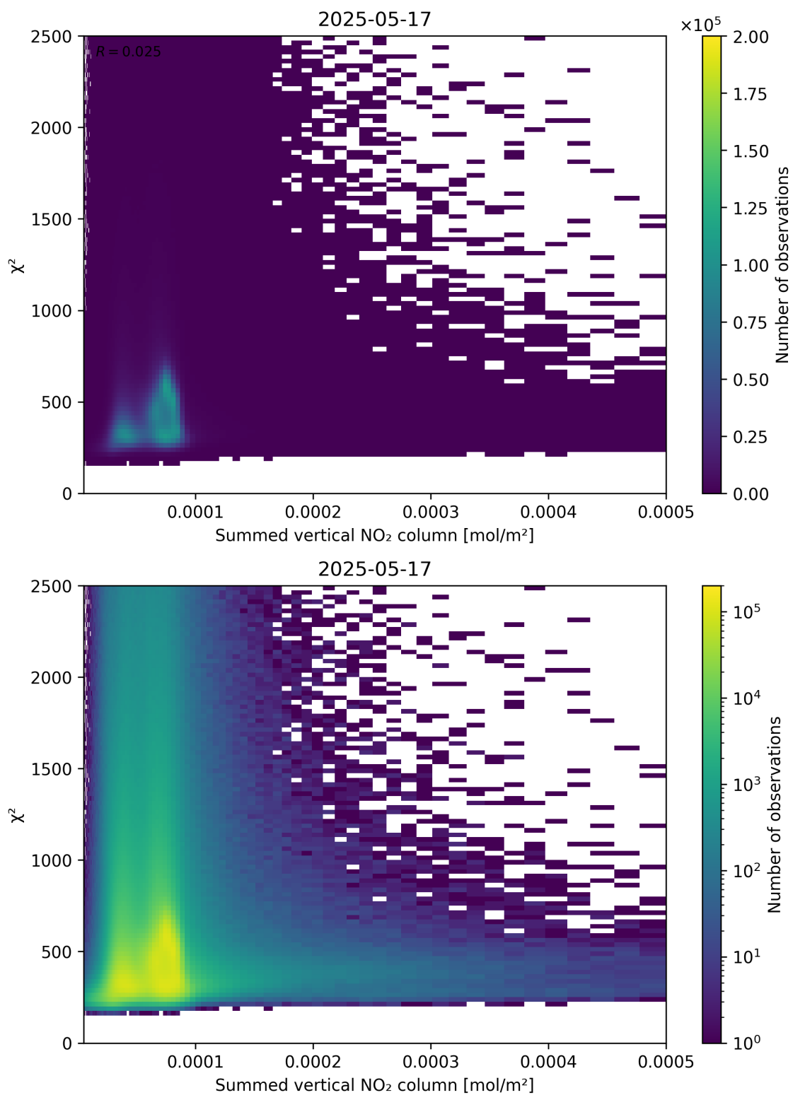
Figure 104: Scatter density plot of “Summed vertical NO 2 column” against “ \chi^2 ” for 2025-05-16 to 2025-05-18.
