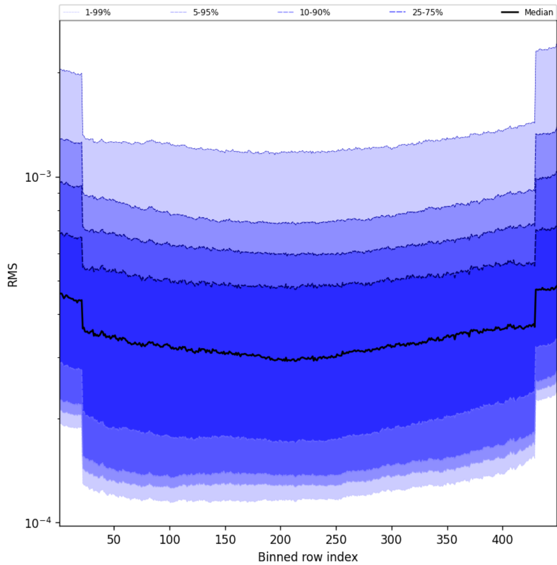
Figure 60: Along track statistics of “RMS” for 2025-05-16 to 2025-05-18
