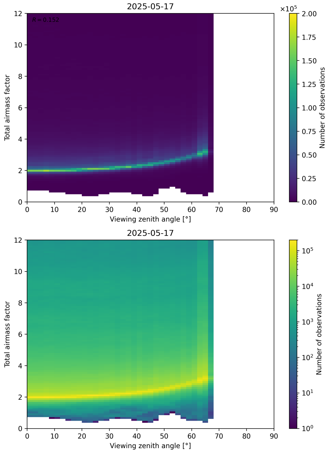
Figure 160: Scatter density plot of “Viewing zenith angle” against “Total airmass factor” for 2025-05-16 to 2025-05-18.
