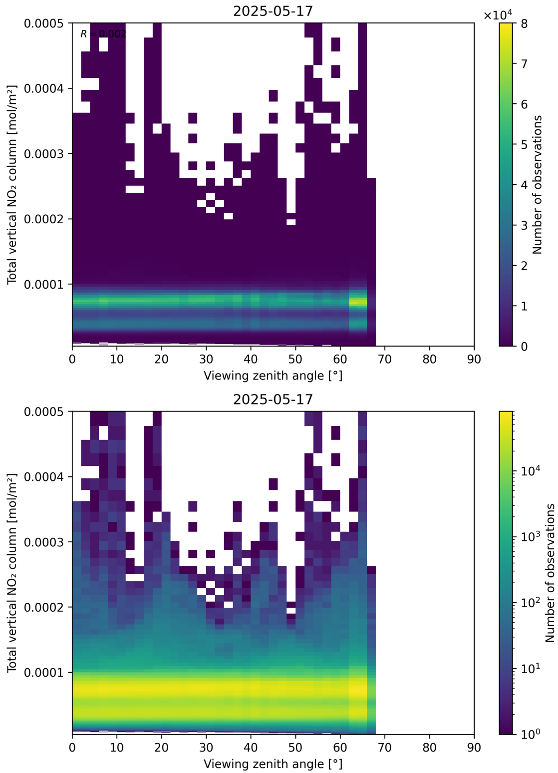
Figure 167: Scatter density plot of “Viewing zenith angle” against “Total vertical NO 2 column” for 2025-05-16 to 2025-05-18.
