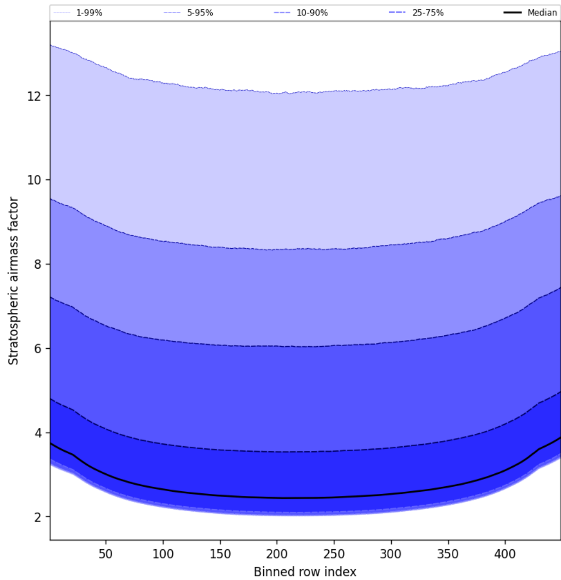
Figure 61: Along track statistics of “Stratospheric airmass factor” for 2025-05-16 to 2025-05-18
