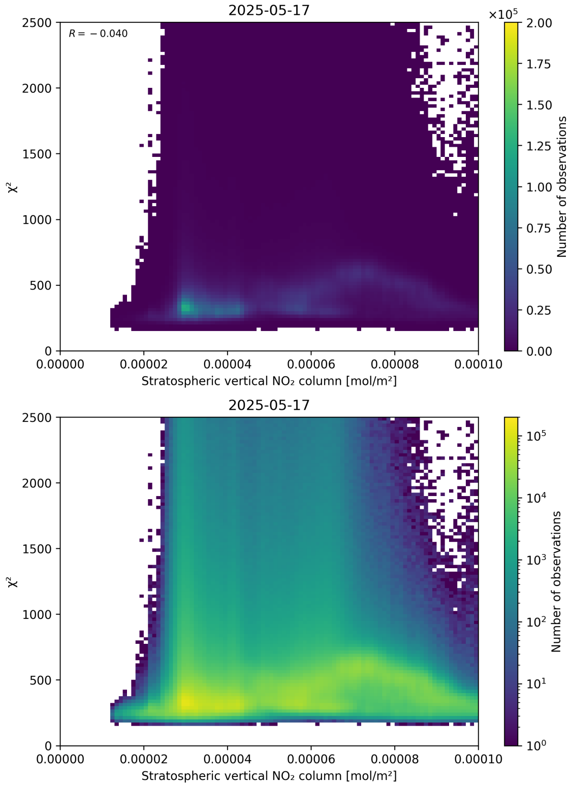
Figure 97: Scatter density plot of “Stratospheric vertical NO 2 column” against “ \chi^2 ” for 2025-05-16 to 2025-05-18.
