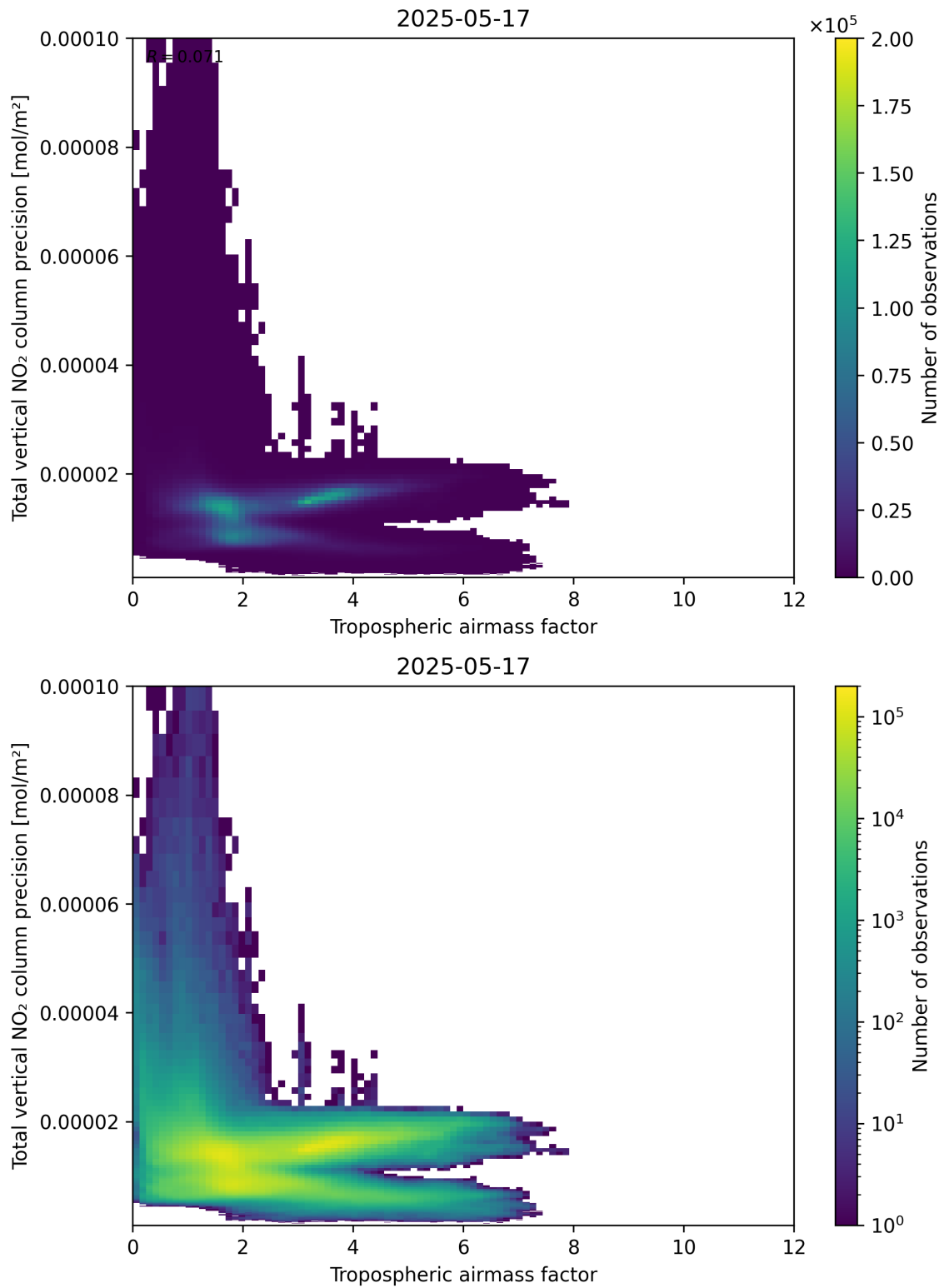
Figure 78: Scatter density plot of “Tropospheric airmass factor” against “Total vertical NO 2 column precision” for 2025-05-16 to 2025-05-18.
