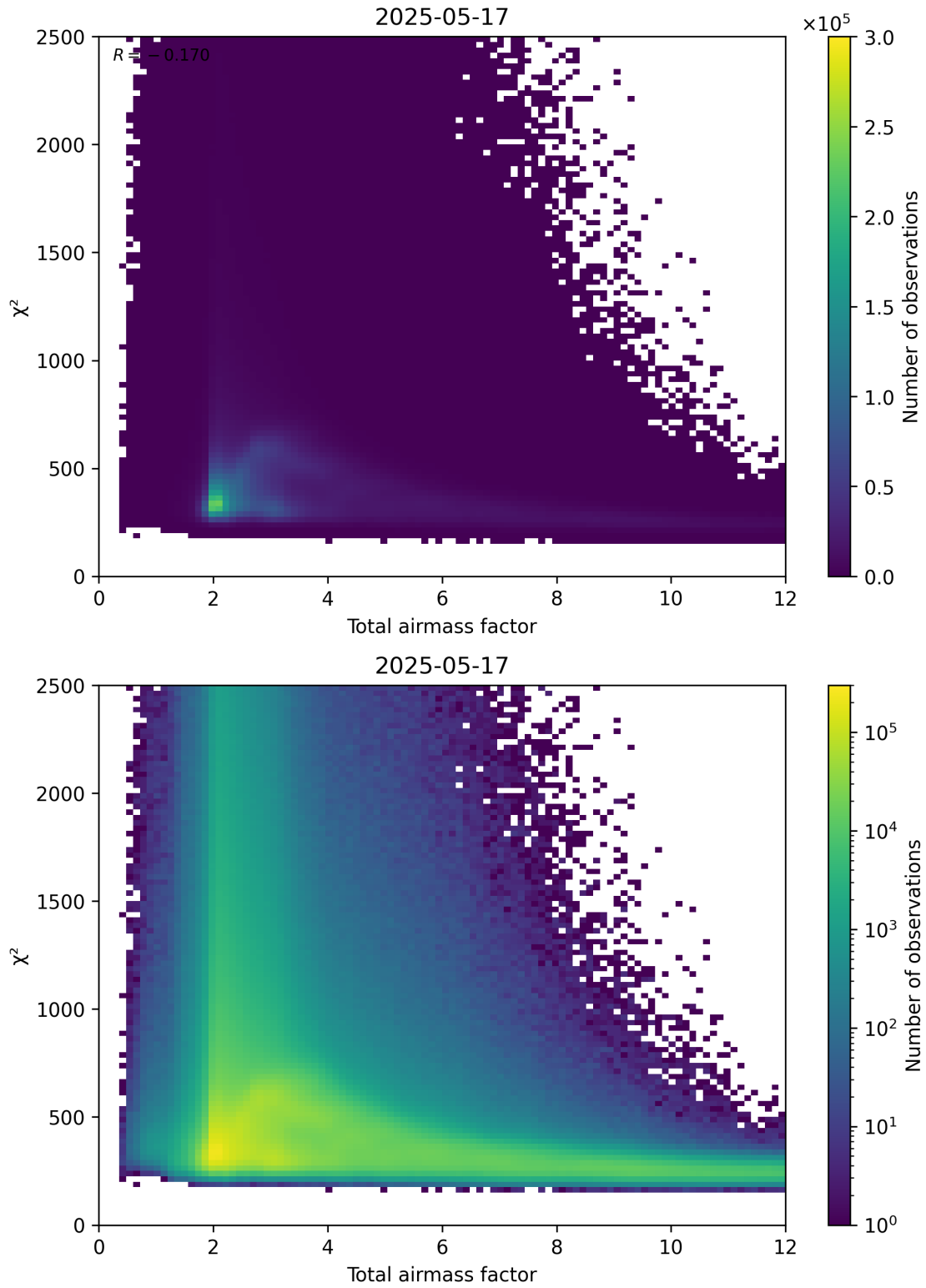
Figure 63: Scatter density plot of “Total airmass factor” against “ \chi^2 ” for 2025-05-16 to 2025-05-18.
