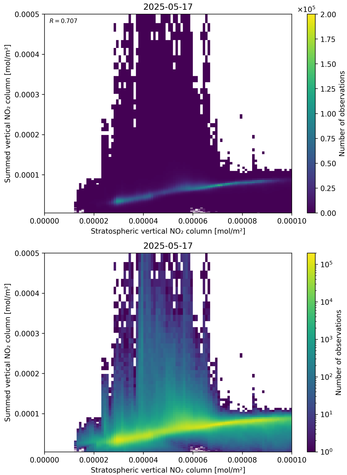
Figure 98: Scatter density plot of “Stratospheric vertical NO 2 column” against “Summed vertical NO 2 column” for 2025-05-16 to 2025-05-18.
