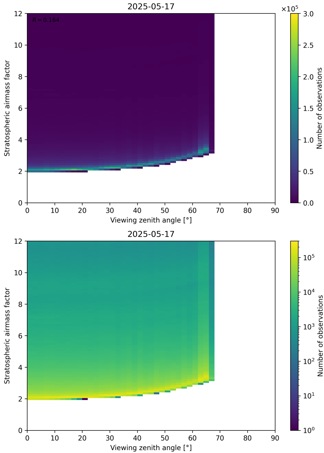
Figure 159: Scatter density plot of “Viewing zenith angle” against “Stratospheric airmass factor” for 2025-05-16 to 2025-05-18.
