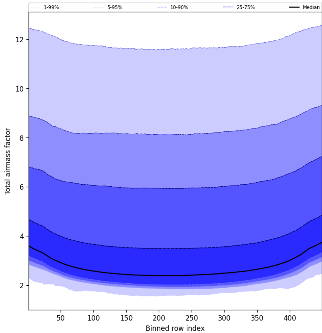
Figure 49: Along track statistics of “Total airmass factor” for 2025-05-16 to 2025-05-18
