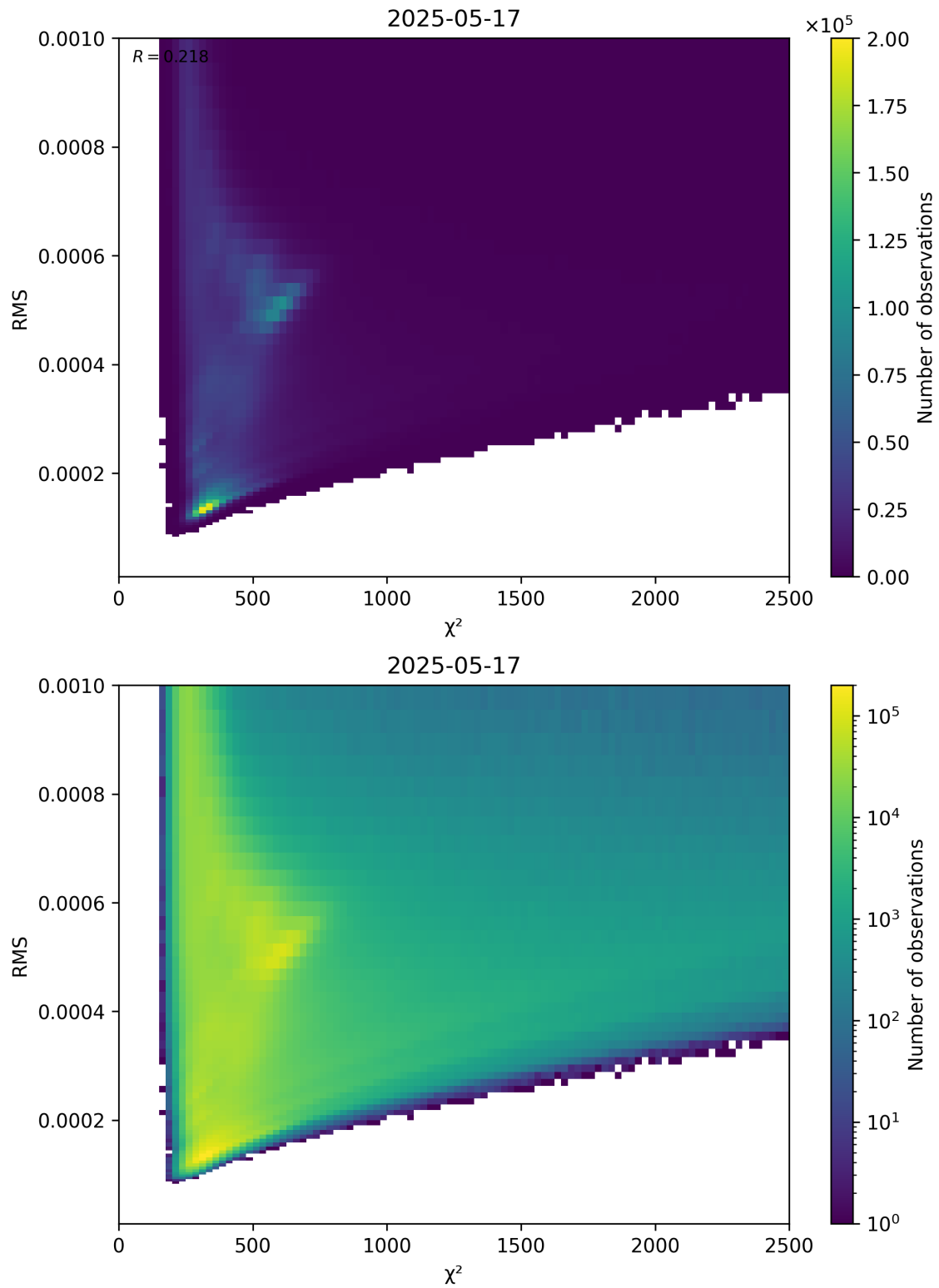
Figure 82: Scatter density plot of “ \chi^2 ” against “RMS” for 2025-05-16 to 2025-05-18.
