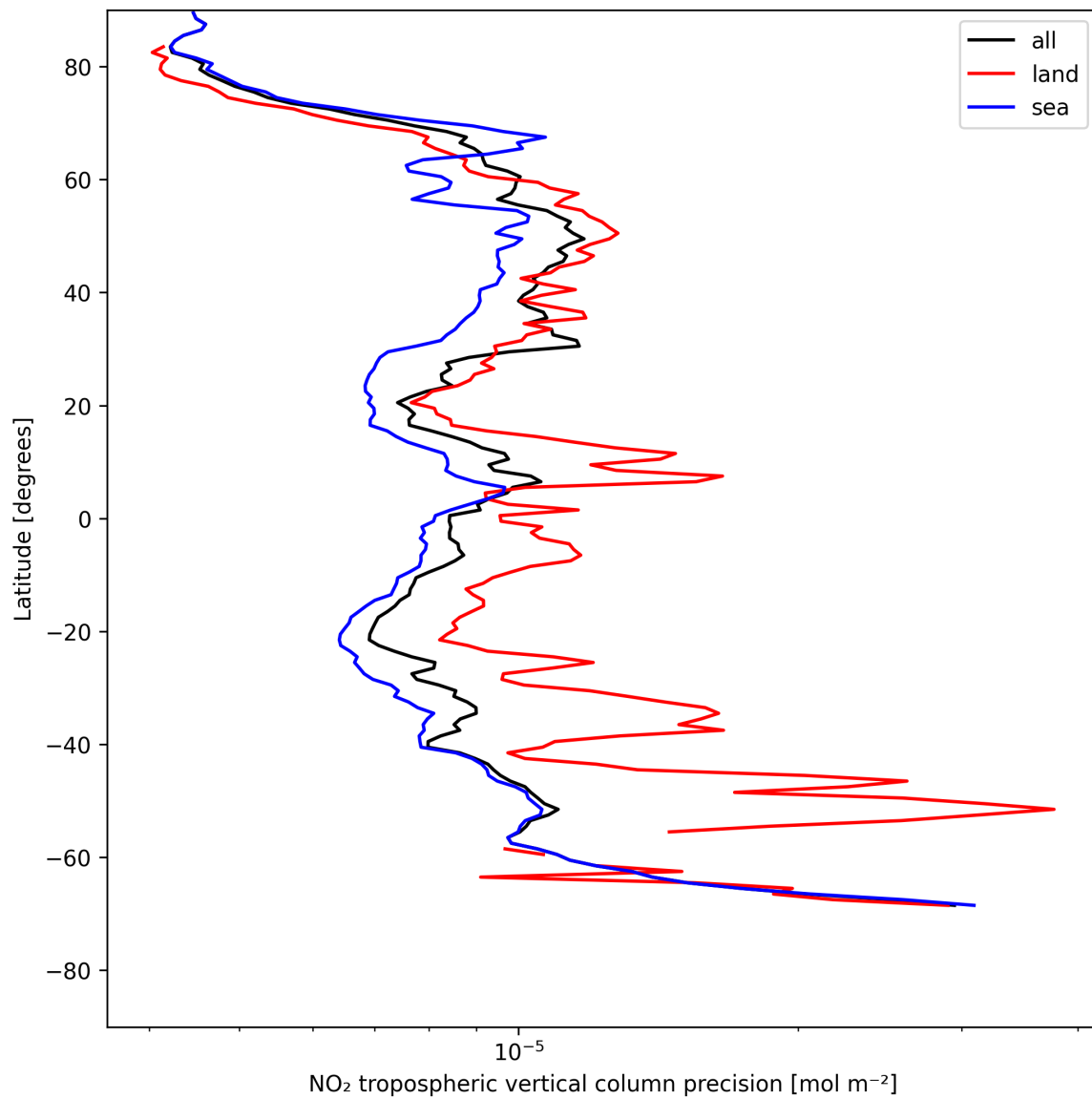
Figure 13: Zonal average of “NO 2 tropospheric vertical column precision” for 2025-05-16 to 2025-05-18.
