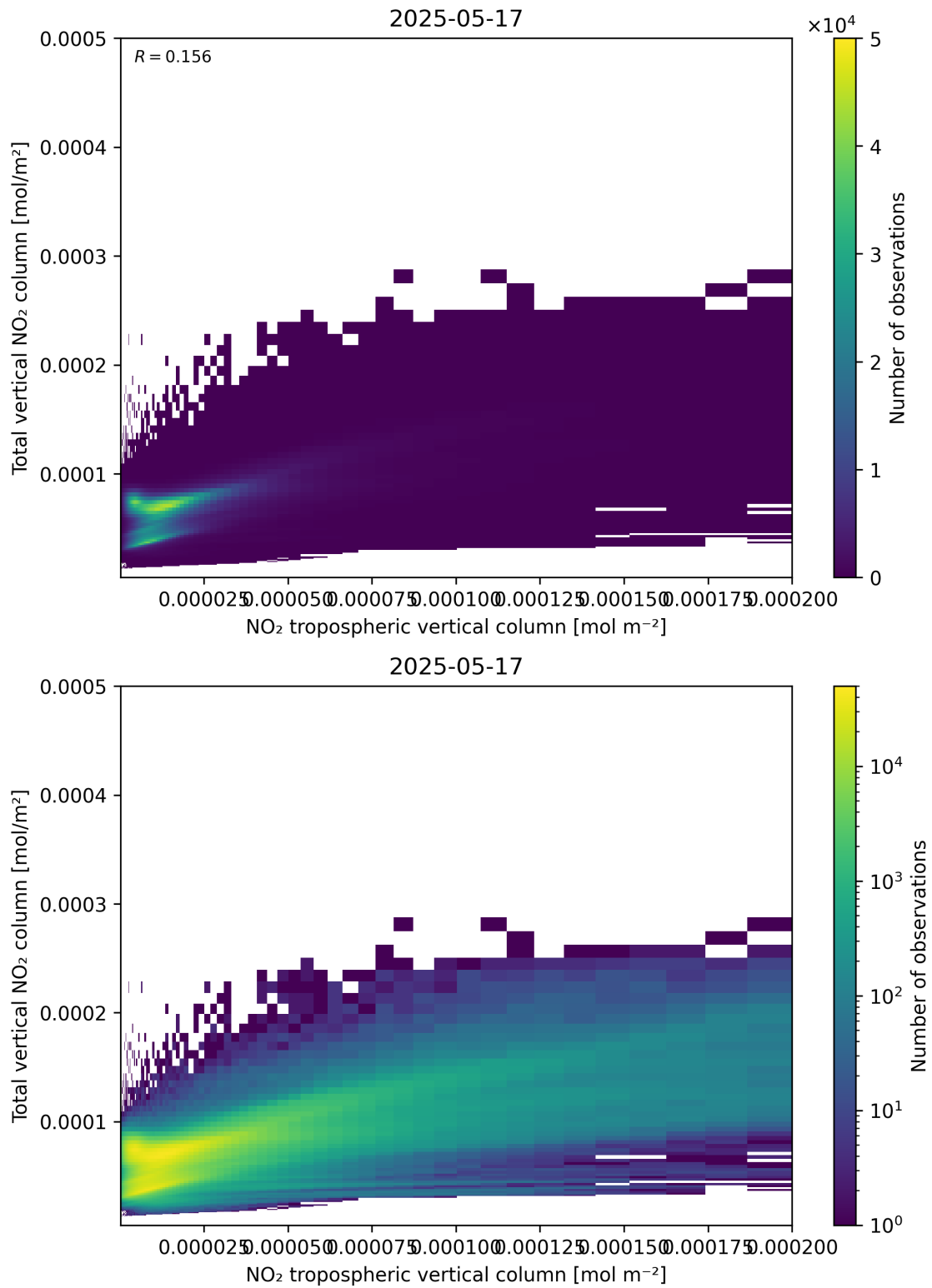
Figure 128: Scatter density plot of “NO 2 tropospheric vertical column” against “Total vertical NO 2 column” for 2025-05-16 to 2025-05-18.
