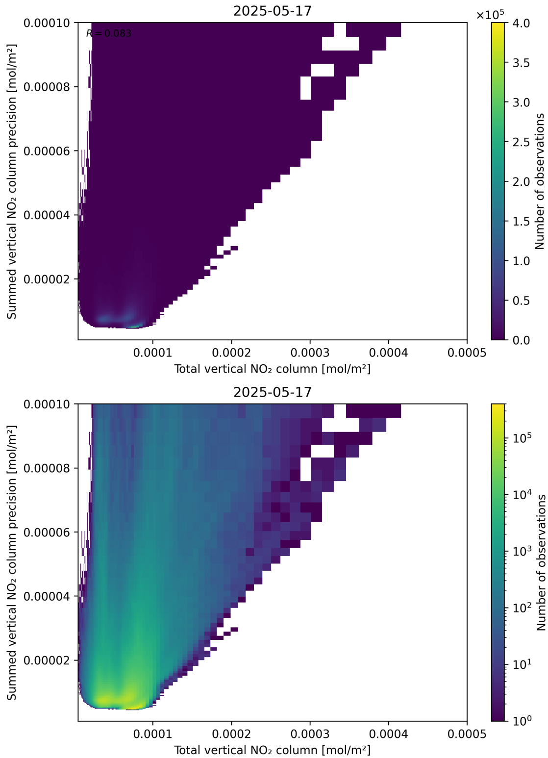
Figure 113: Scatter density plot of “Total vertical NO 2 column” against “Summed vertical NO 2 column precision” for 2025-05-16 to 2025-05-18.
