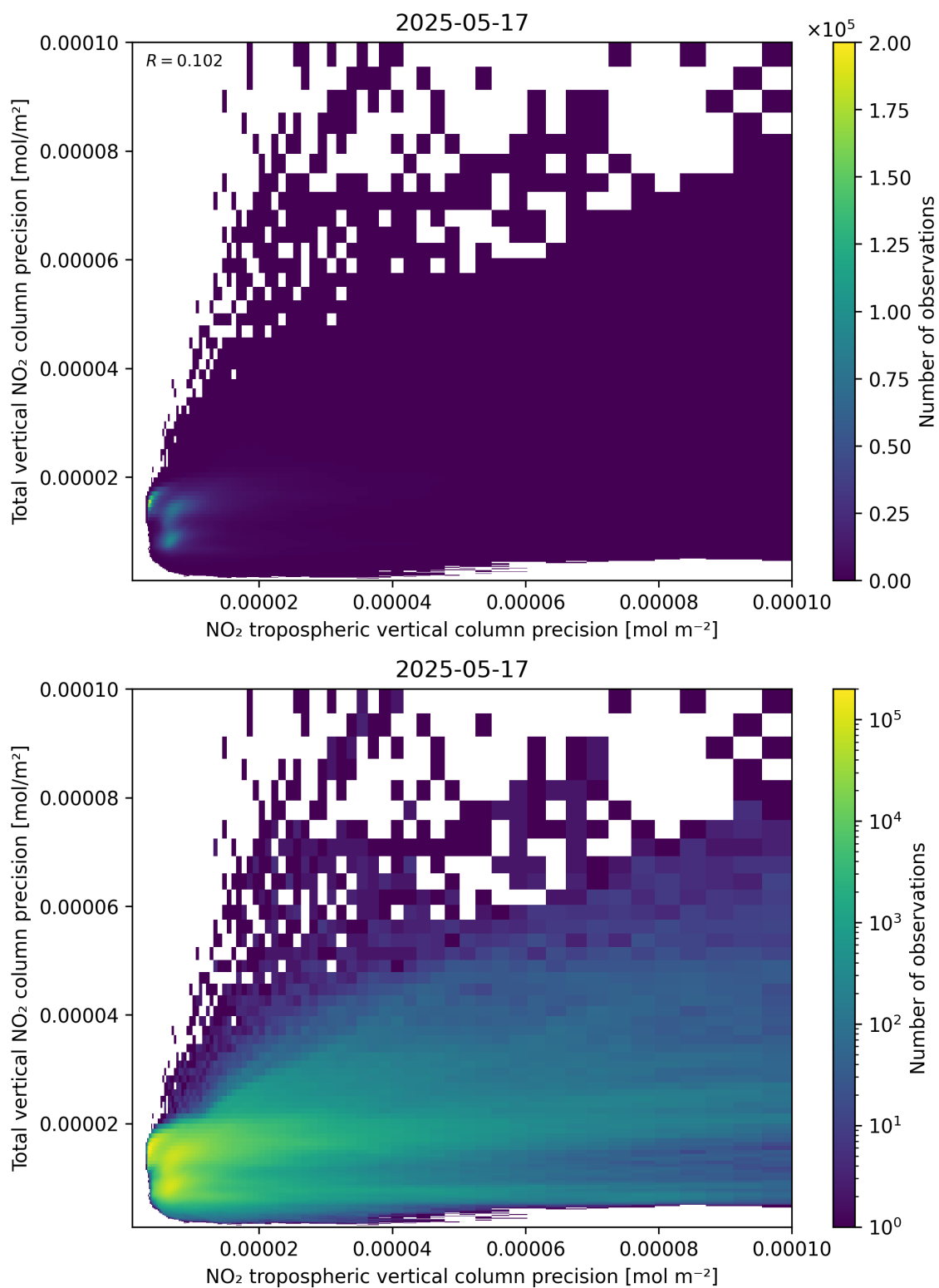
Figure 139: Scatter density plot of “NO 2 tropospheric vertical column precision” against “Total vertical NO 2 column precision” for 2025-05-16 to 2025-05-18.
