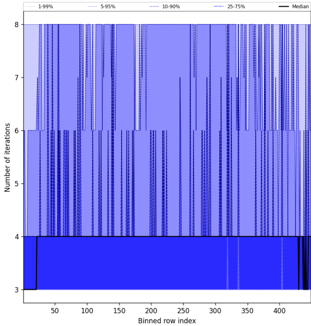
Figure 51: Along track statistics of “Number of iterations” for 2025-05-16 to 2025-05-18
