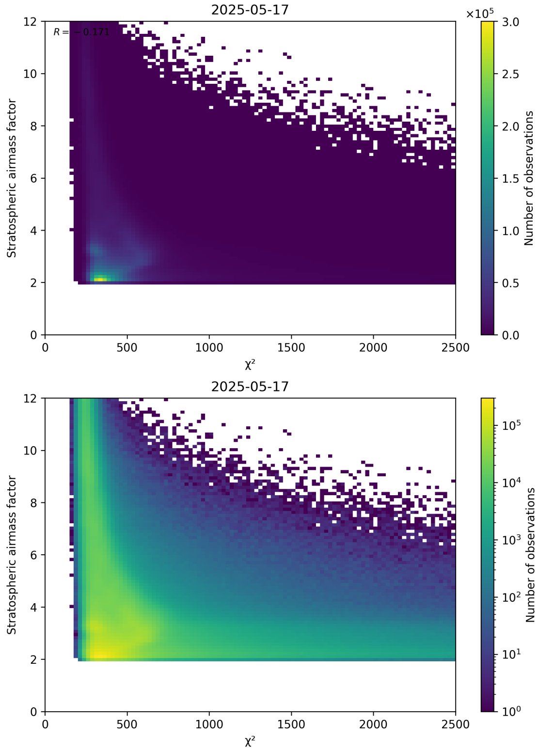
Figure 81: Scatter density plot of “ \chi^2 ” against “Stratospheric airmass factor” for 2025-05-16 to 2025-05-18.
