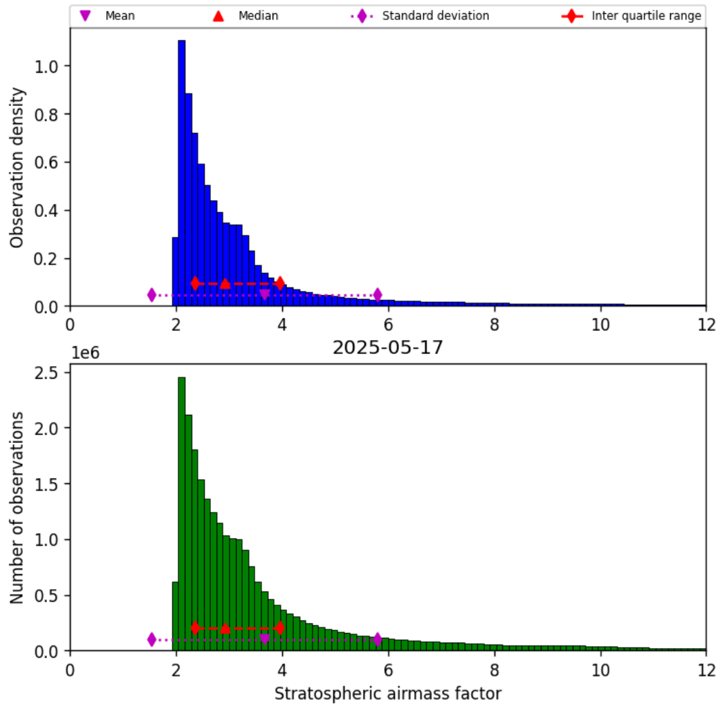
Figure 44: Histogram of “Stratospheric airmass factor” for 2025-05-16 to 2025-05-18
