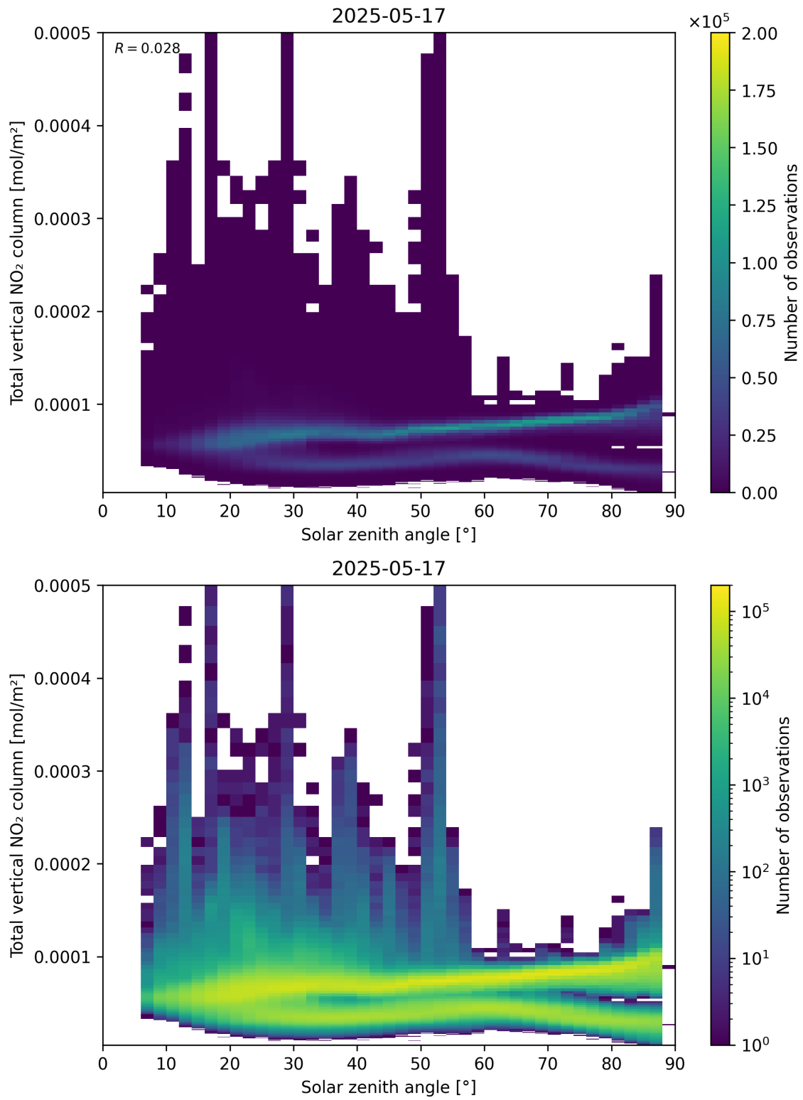
Figure 153: Scatter density plot of “Solar zenith angle” against “Total vertical NO 2 column” for 2025-05-16 to 2025-05-18.
