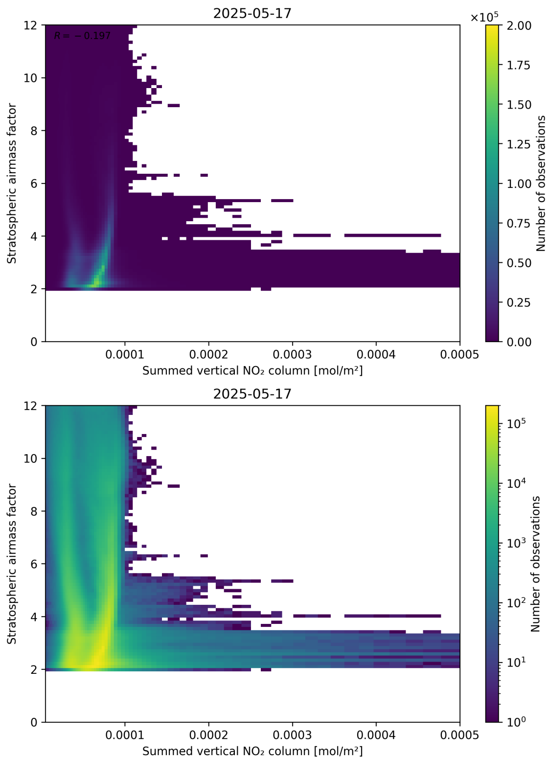
Figure 103: Scatter density plot of “Summed vertical NO 2 column” against “Stratospheric airmass factor” for 2025-05-16 to 2025-05-18.
