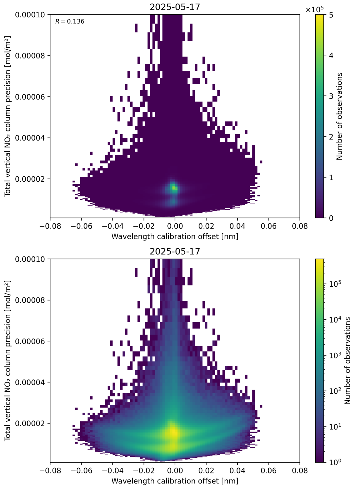
Figure 180: Scatter density plot of “Wavelength calibration offset” against “Total vertical NO 2 column precision” for 2025-05-16 to 2025-05-18.
