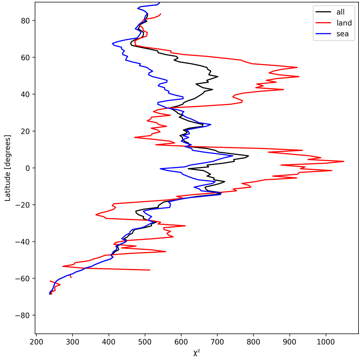
Figure 25: Zonal average of “ \chi^2 ” for 2025-05-16 to 2025-05-18.
