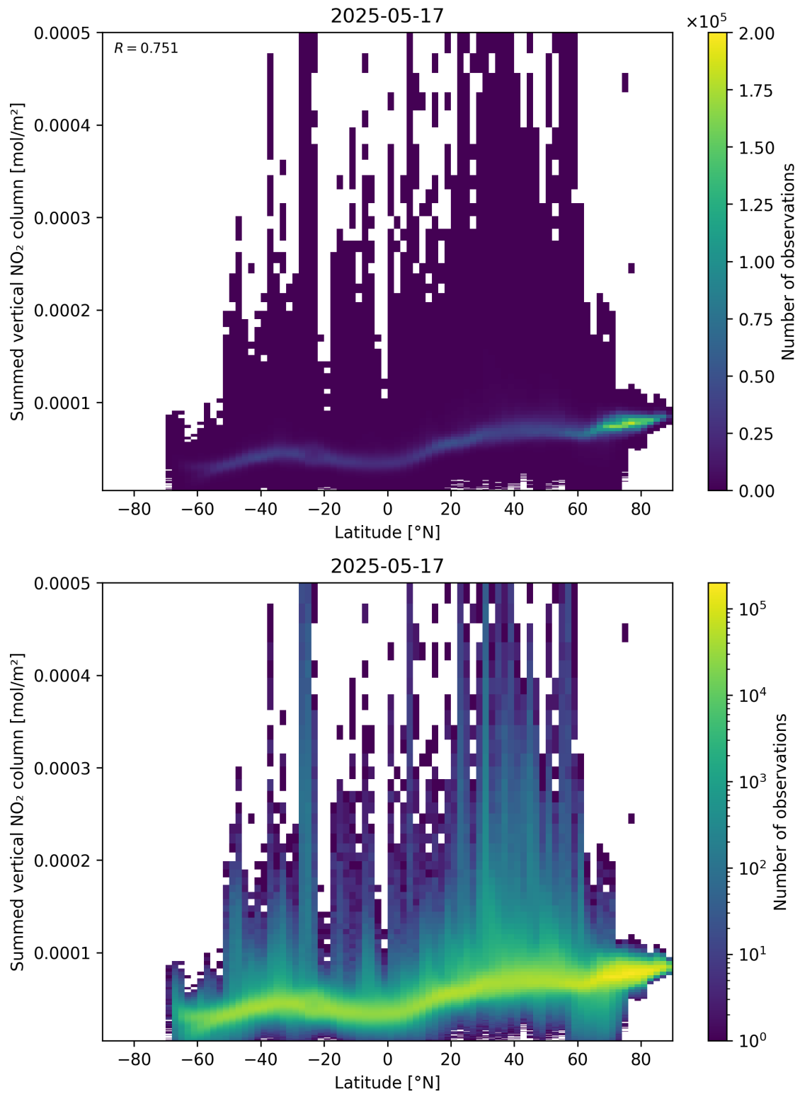
Figure 88: Scatter density plot of “Latitude” against “Summed vertical NO 2 column” for 2025-05-16 to 2025-05-18.
