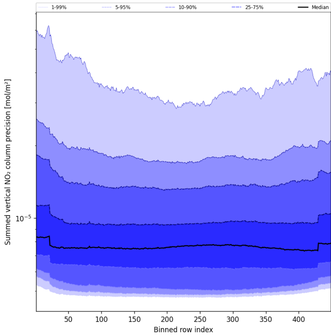
Figure 58: Along track statistics of “Summed vertical NO 2 column precision” for 2025-05-16 to 2025-05-18
