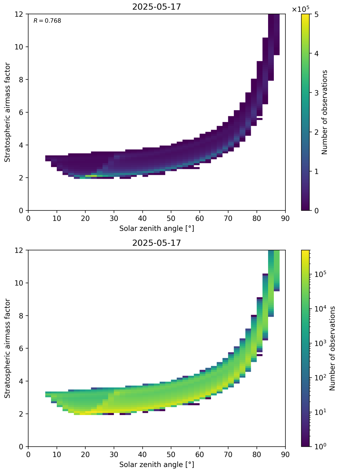
Figure 145: Scatter density plot of “Solar zenith angle” against “Stratospheric airmass factor” for 2025-05-16 to 2025-05-18.
