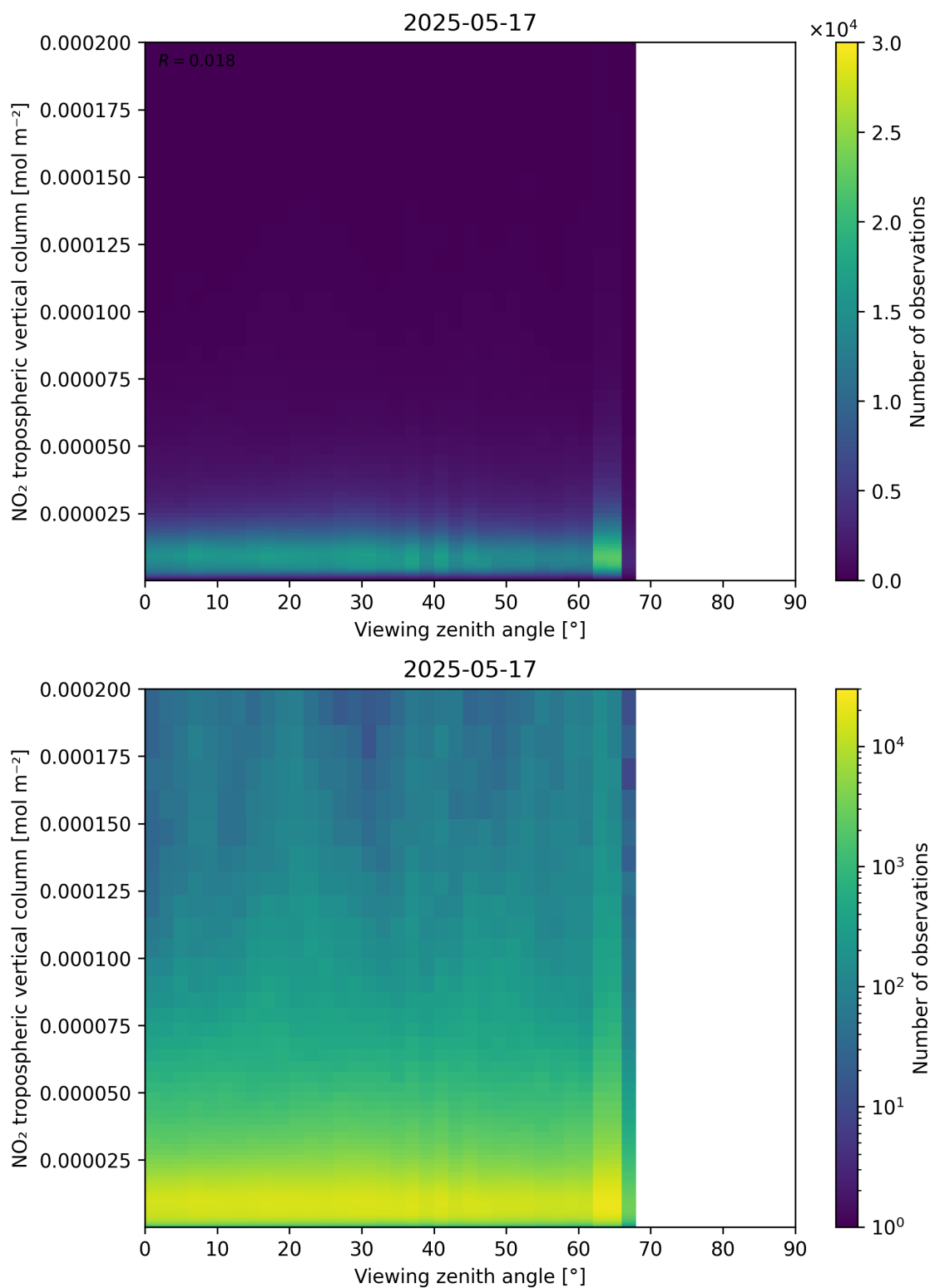
Figure 169: Scatter density plot of “Viewing zenith angle” against “NO 2 tropospheric vertical column” for 2025-05-16 to 2025-05-18.
