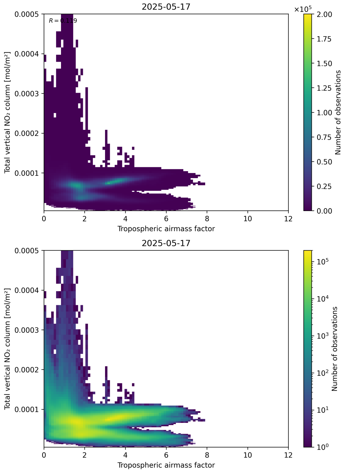
Figure 77: Scatter density plot of “Tropospheric airmass factor” against “Total vertical NO 2 column” for 2025-05-16 to 2025-05-18.
