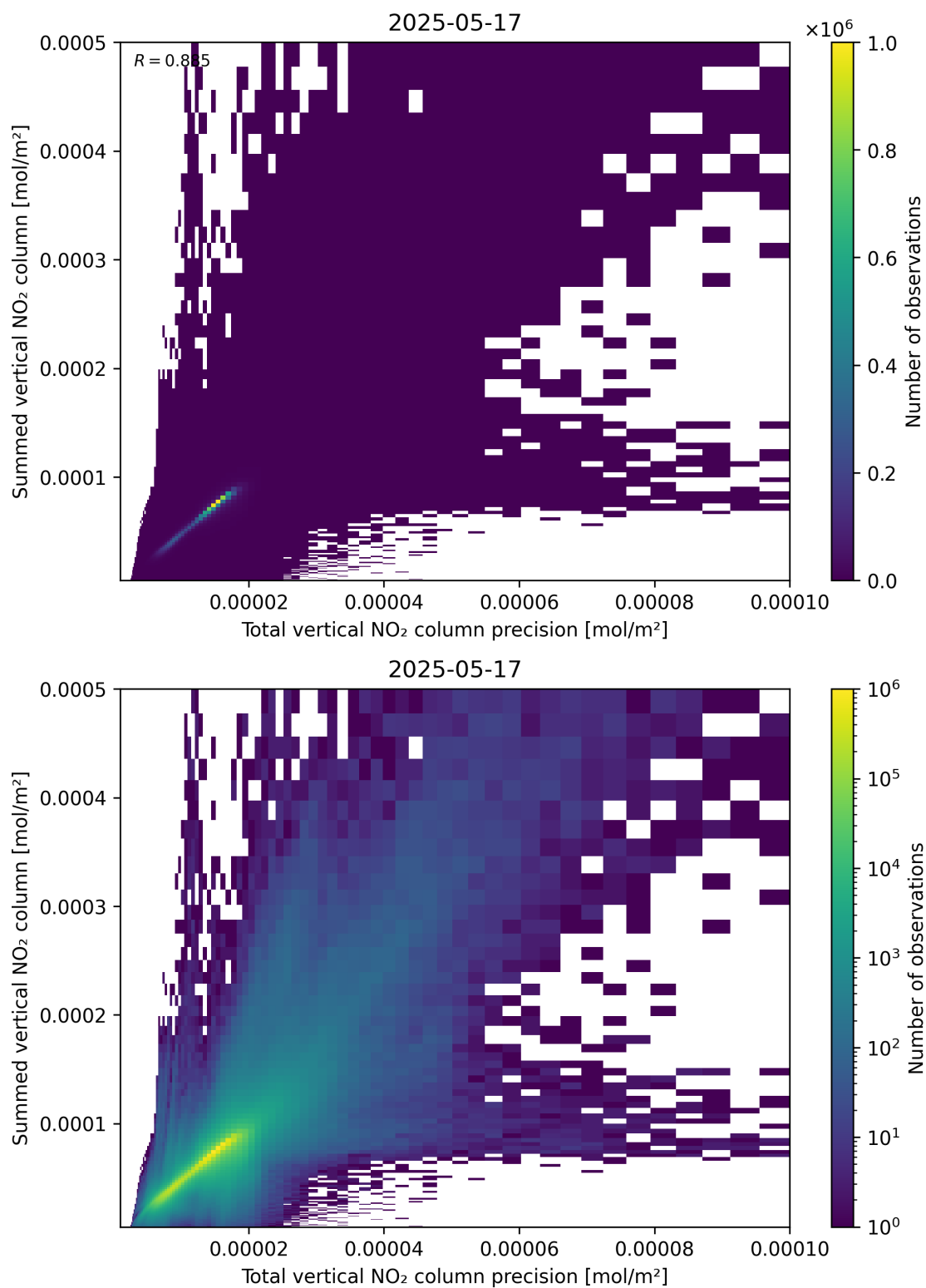
Figure 117: Scatter density plot of “Total vertical NO 2 column precision” against “Summed vertical NO 2 column” for 2025-05-16 to 2025-05-18.
