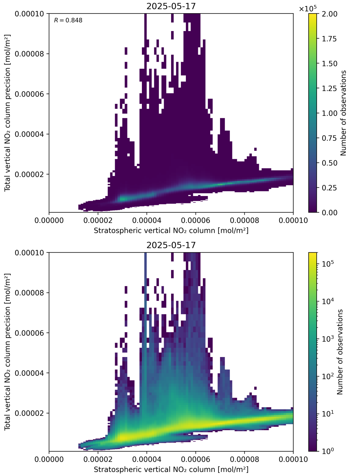
Figure 101: Scatter density plot of “Stratospheric vertical NO 2 column” against “Total vertical NO 2 column precision” for 2025-05-16 to 2025-05-18.
