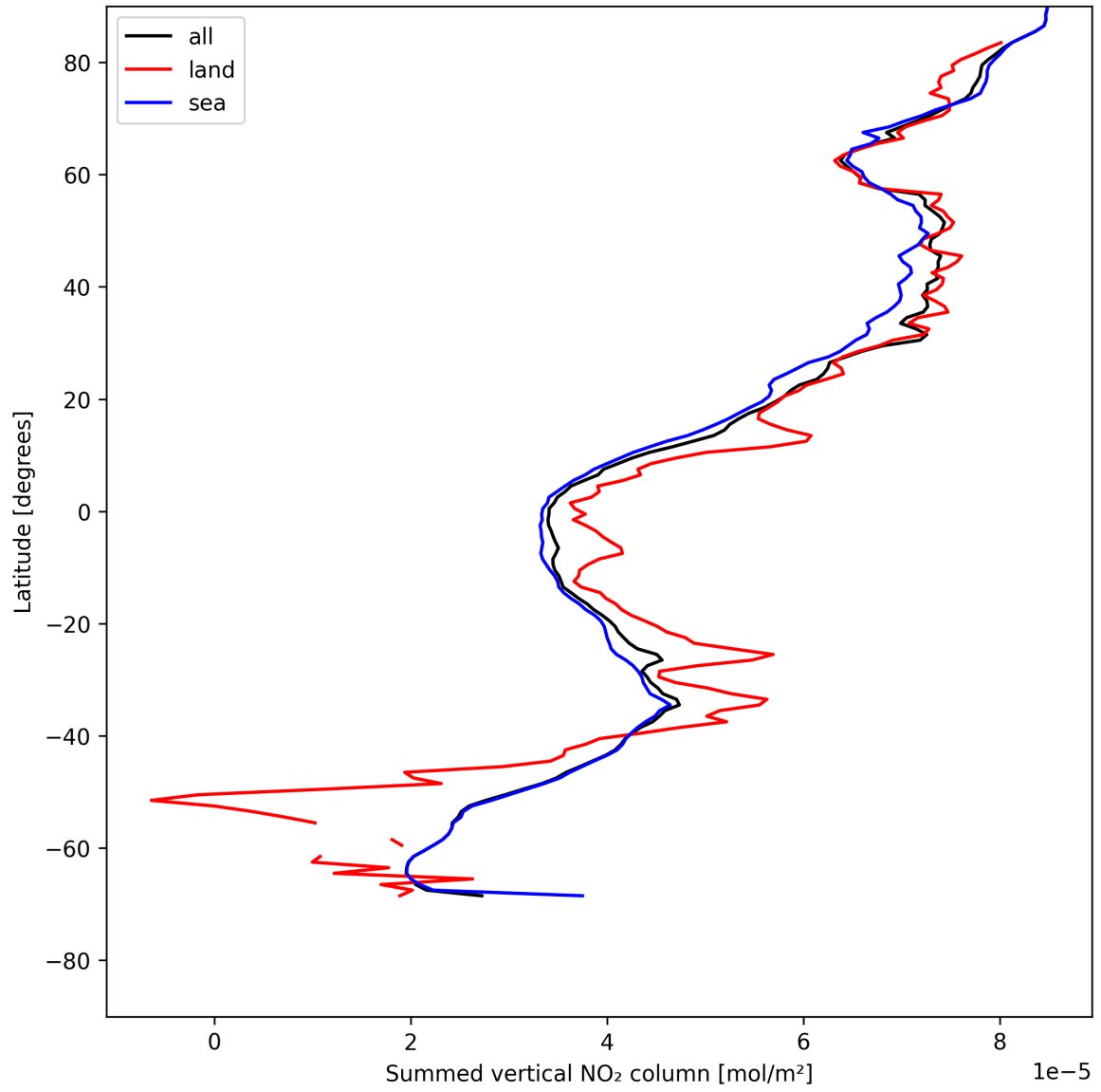
Figure 23: Zonal average of “Summed vertical NO 2 column” for 2025-05-16 to 2025-05-18.
