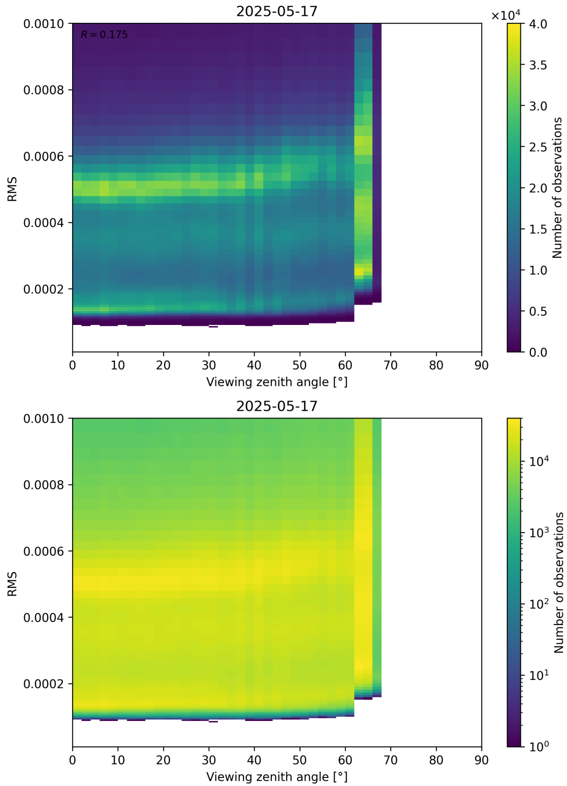
Figure 171: Scatter density plot of “Viewing zenith angle” against “RMS” for 2025-05-16 to 2025-05-18.
