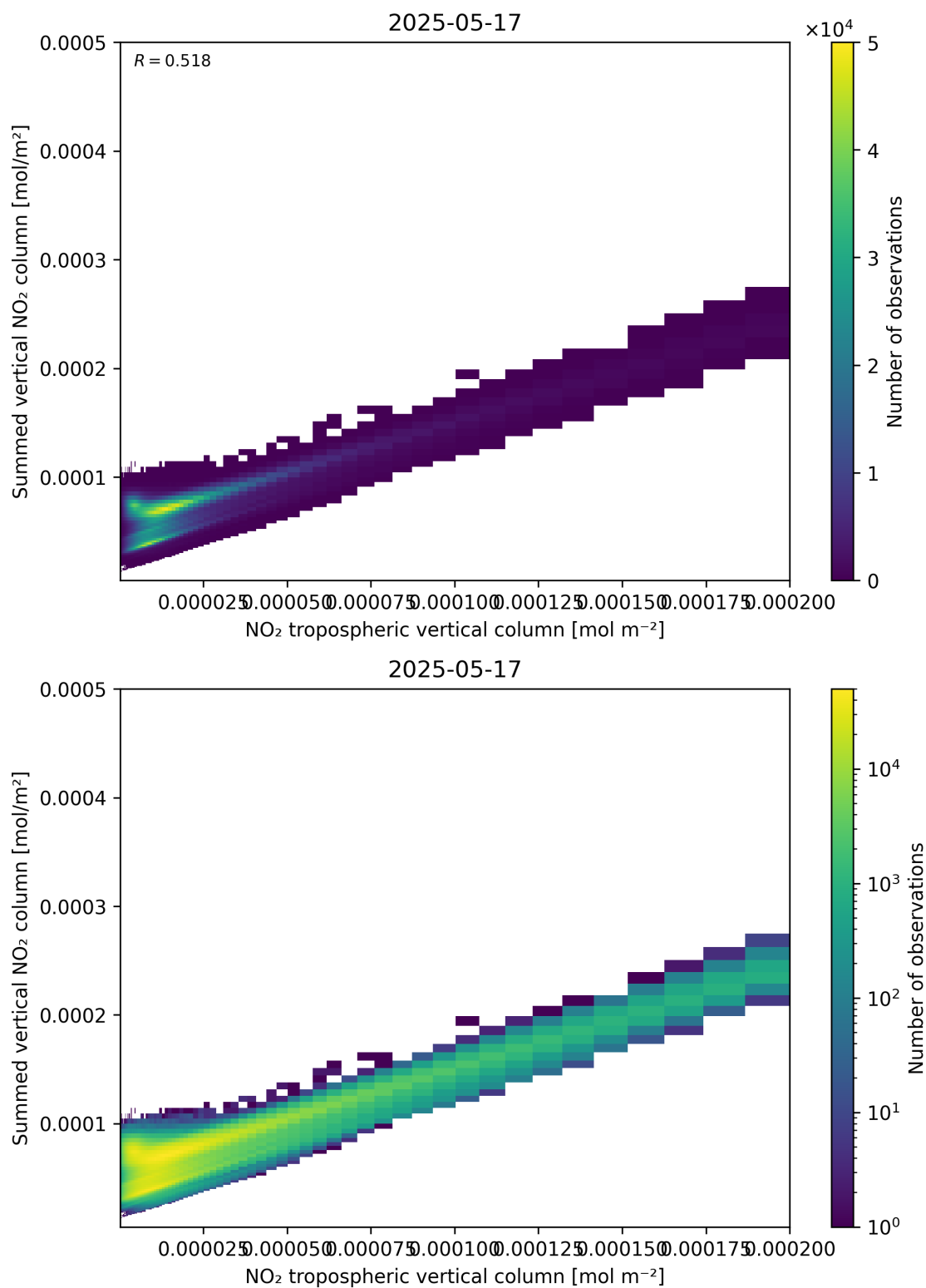
Figure 126: Scatter density plot of “NO 2 tropospheric vertical column” against “Summed vertical NO 2 column” for 2025-05-16 to 2025-05-18.
