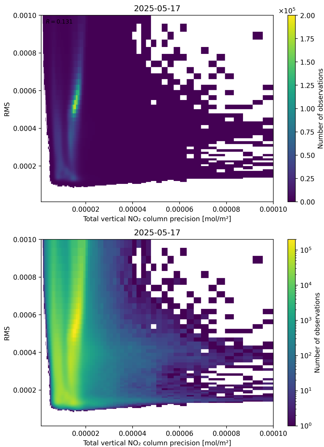
Figure 119: Scatter density plot of “Total vertical NO 2 column precision” against “RMS” for 2025-05-16 to 2025-05-18.
