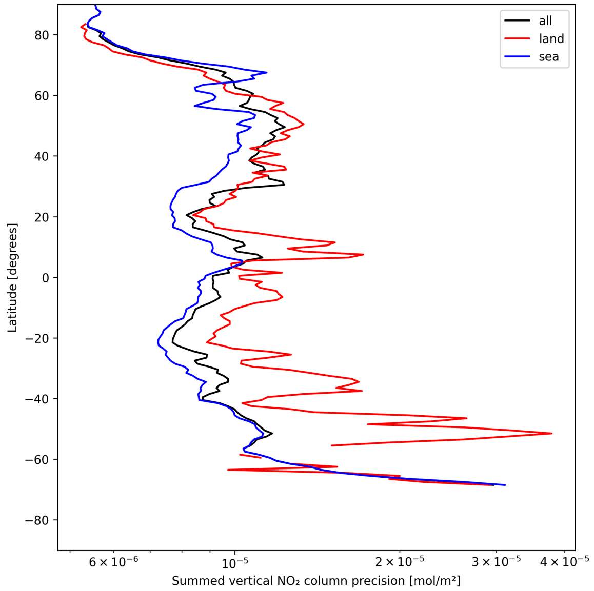
Figure 24: Zonal average of “Summed vertical NO 2 column precision” for 2025-05-16 to 2025-05-18.
