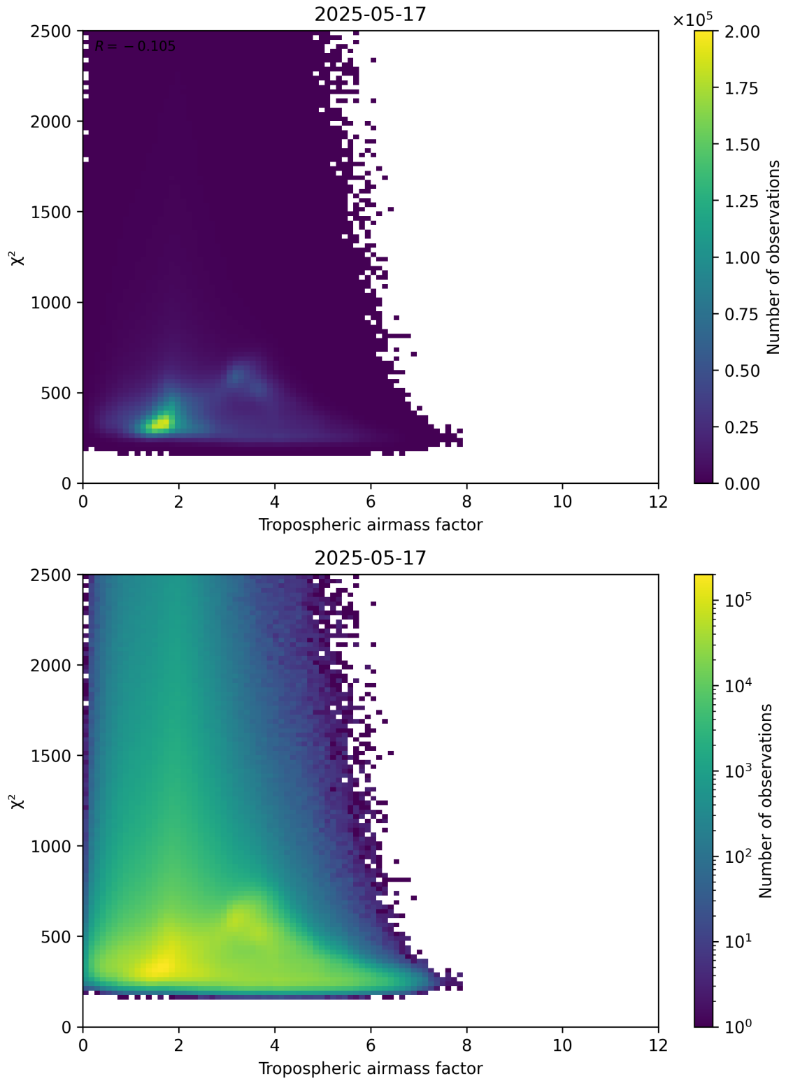
Figure 73: Scatter density plot of “Tropospheric airmass factor” against “ \chi^2 ” for 2025-05-16 to 2025-05-18.
