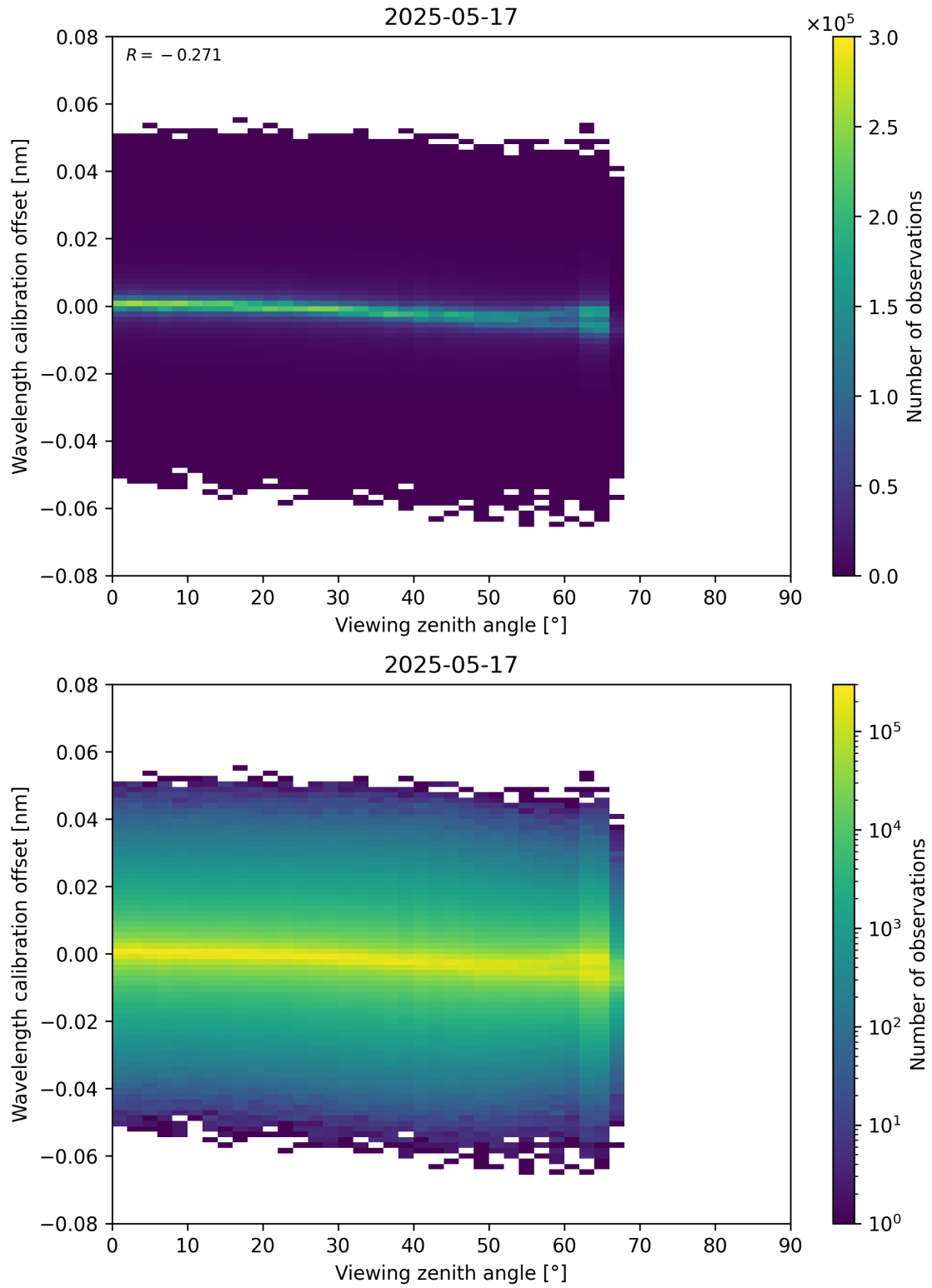
Figure 173: Scatter density plot of “Viewing zenith angle” against “Wavelength calibration offset” for 2025-05-16 to 2025-05-18.
