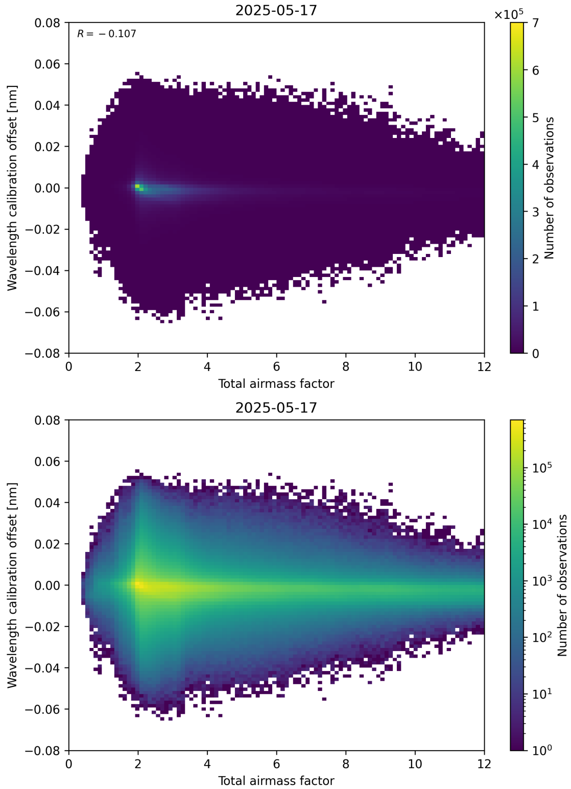
Figure 70: Scatter density plot of “Total airmass factor” against “Wavelength calibration offset” for 2025-05-16 to 2025-05-18.
