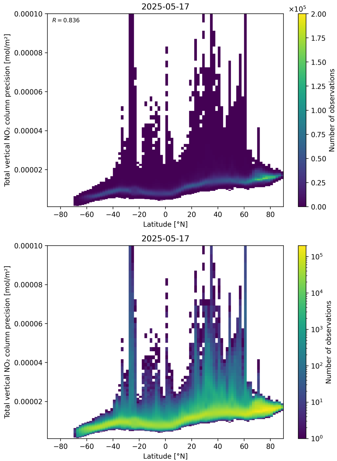
Figure 91: Scatter density plot of “Latitude” against “Total vertical NO 2 column precision” for 2025-05-16 to 2025-05-18.
