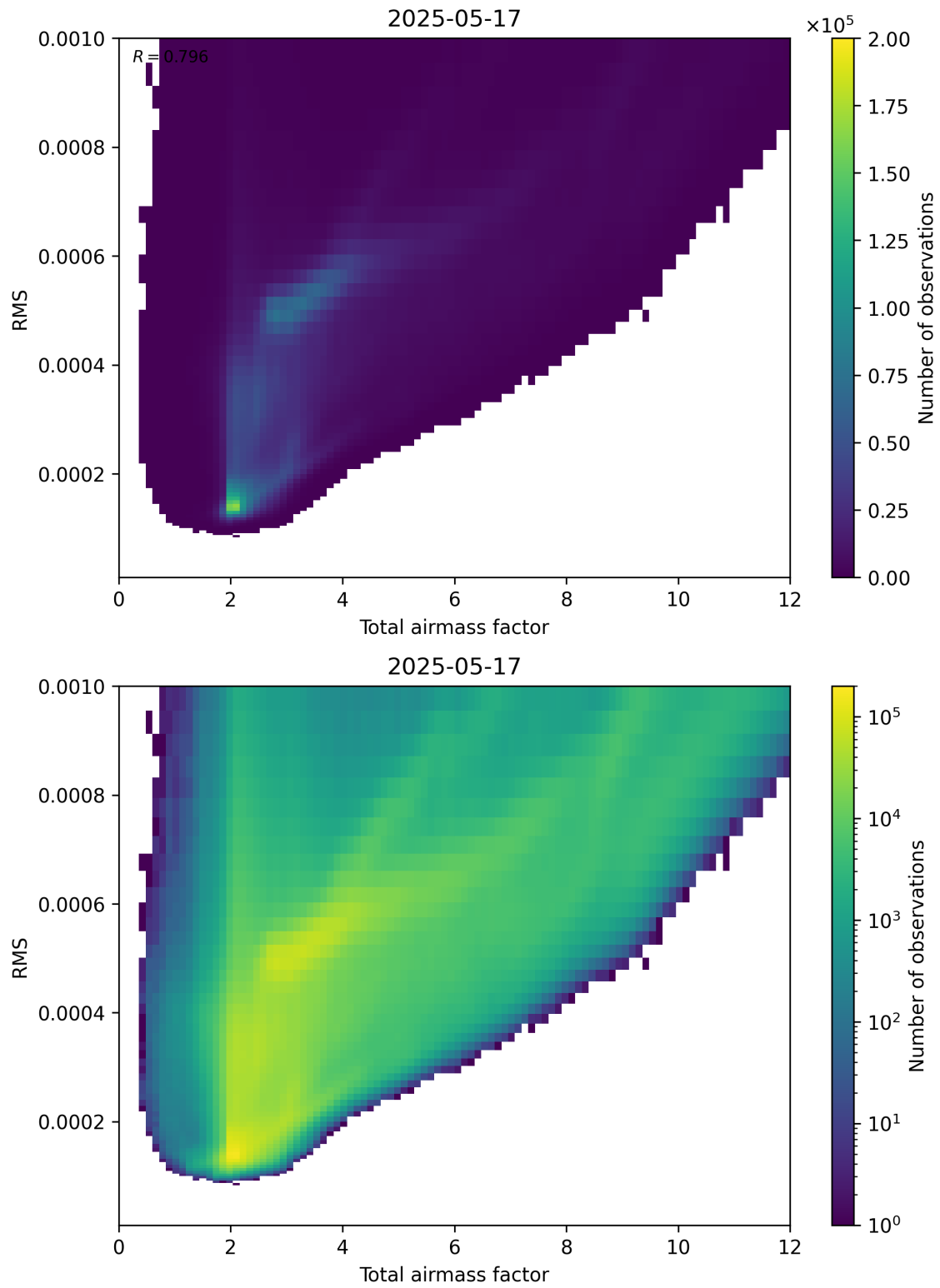
Figure 69: Scatter density plot of “Total airmass factor” against “RMS” for 2025-05-16 to 2025-05-18.
