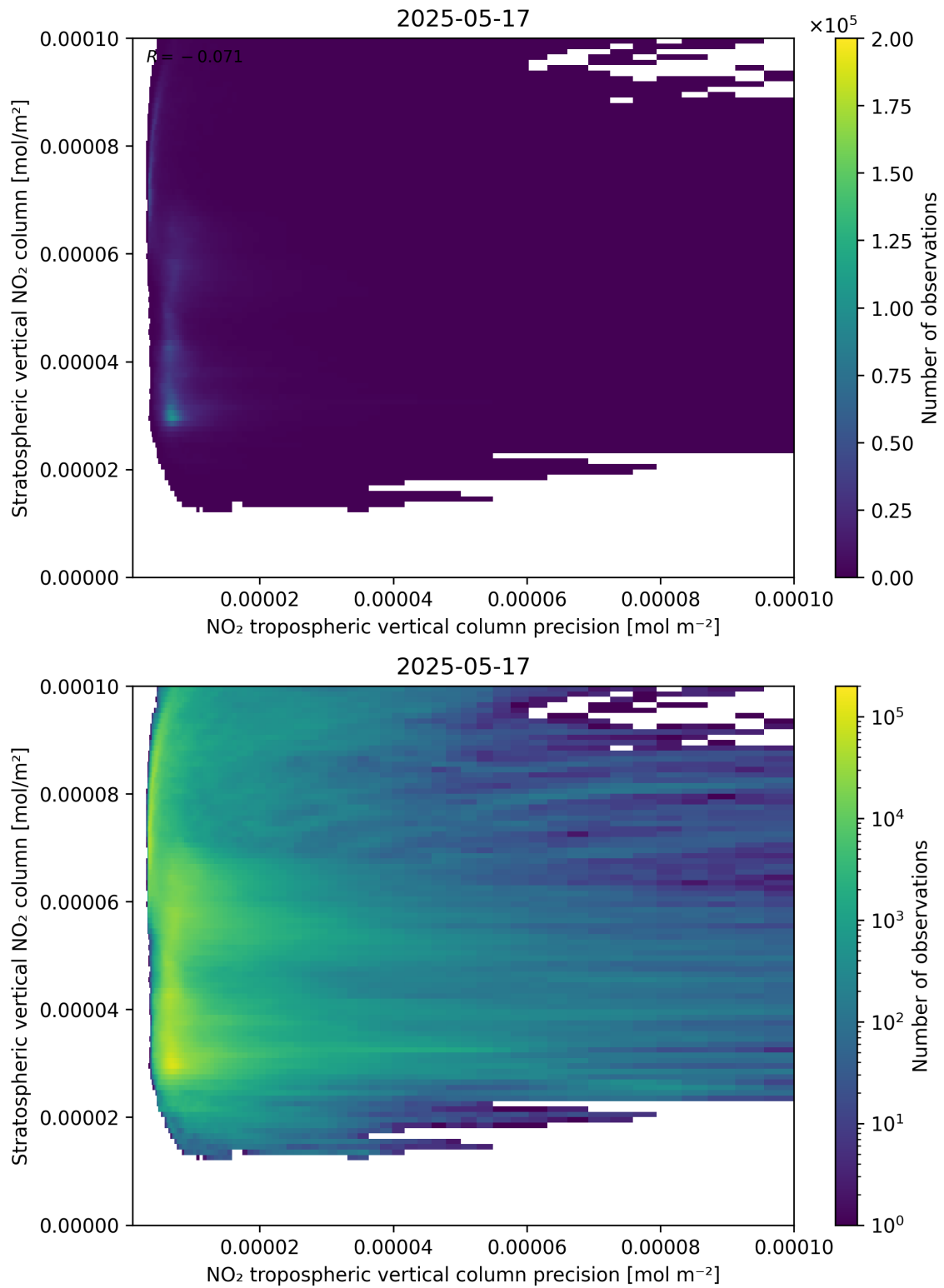
Figure 135: Scatter density plot of “NO 2 tropospheric vertical column precision” against “Stratospheric vertical NO 2 column” for 2025-05-16 to 2025-05-18.
