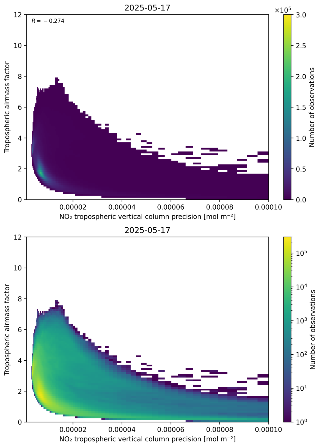
Figure 133: Scatter density plot of “NO 2 tropospheric vertical column precision” against “Tropospheric airmass factor” for 2025-05-16 to 2025-05-18.
