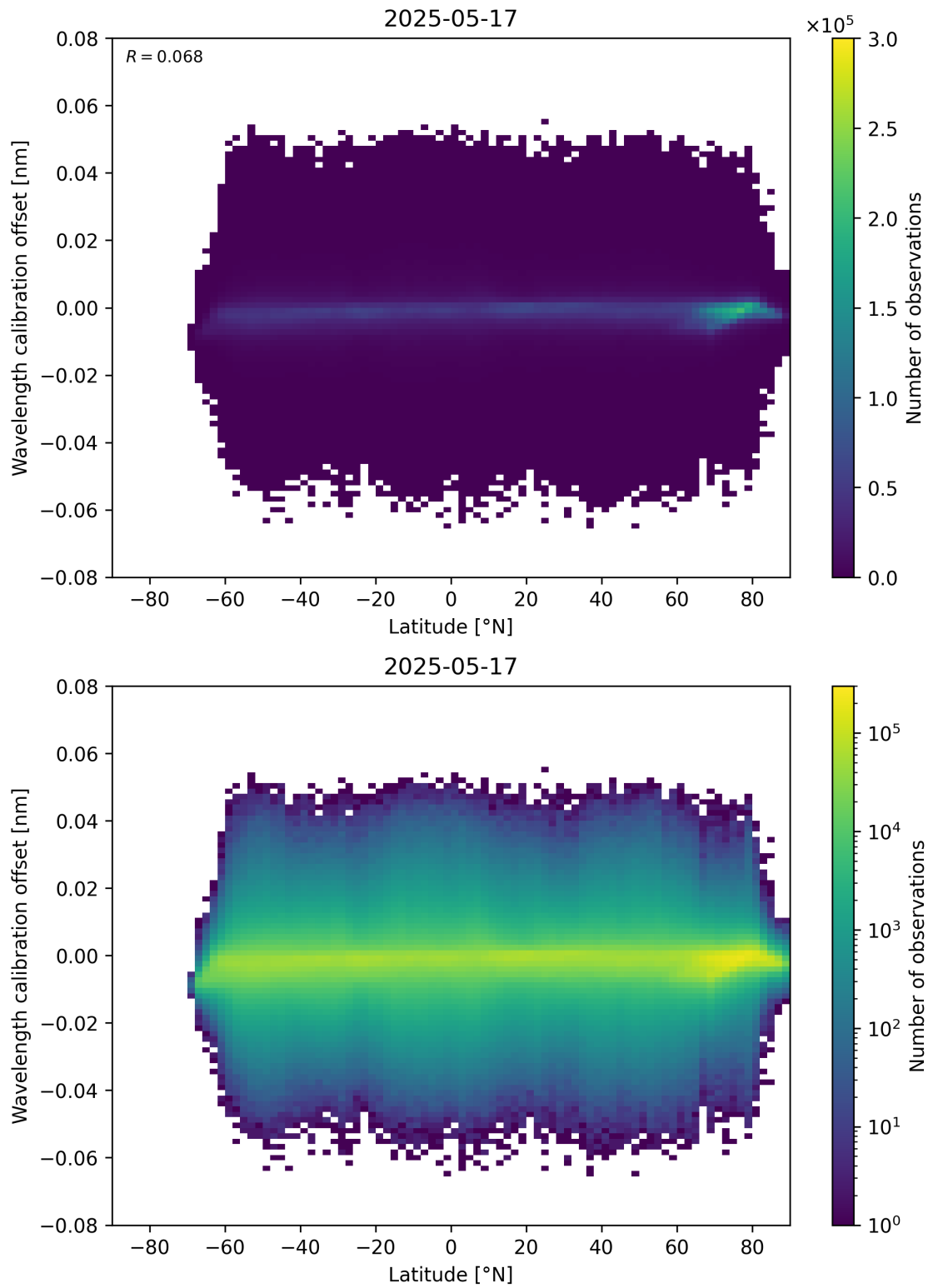
Figure 95: Scatter density plot of “Latitude” against “Wavelength calibration offset” for 2025-05-16 to 2025-05-18.
