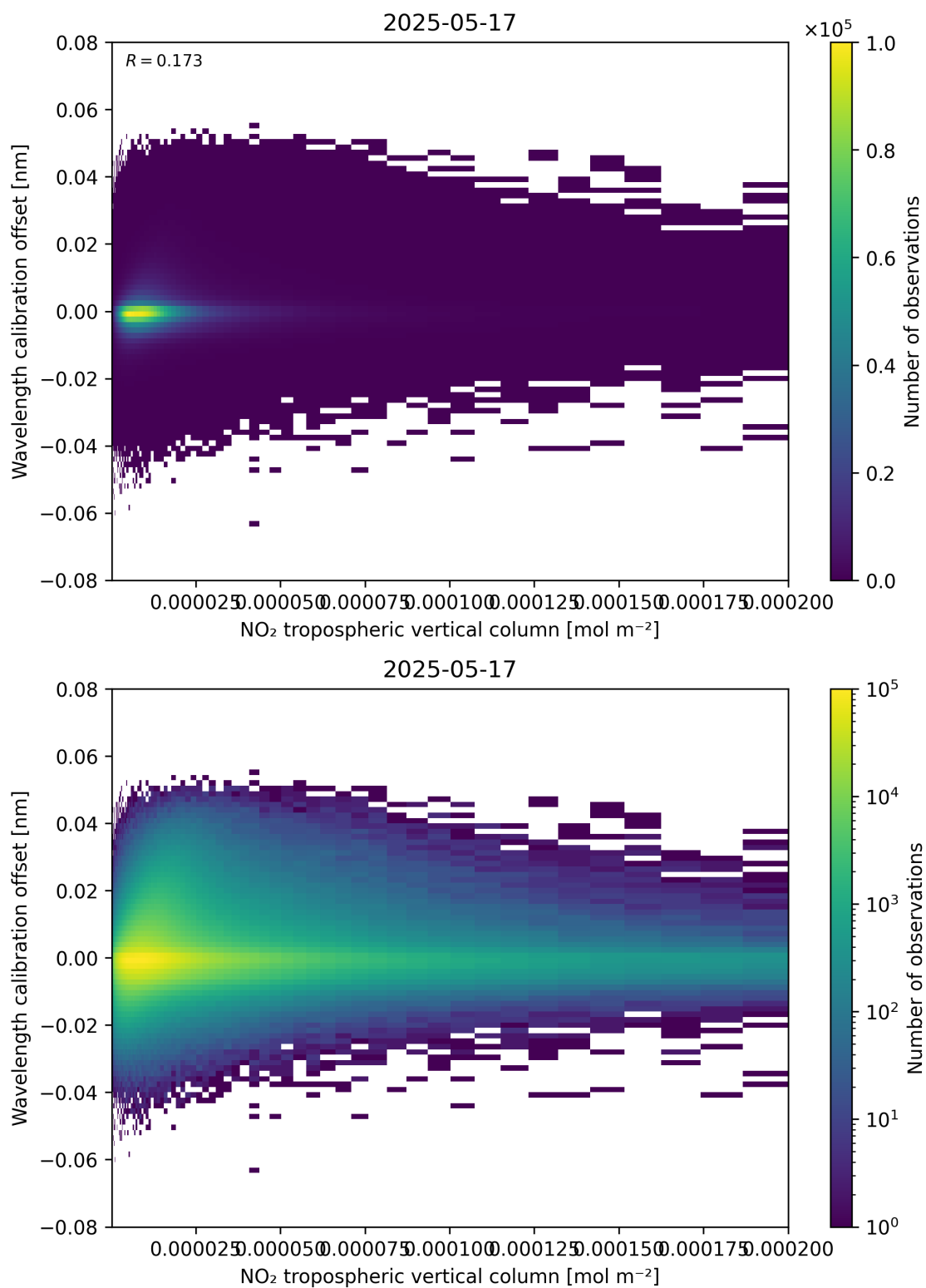
Figure 143: Scatter density plot of “NO 2 tropospheric vertical column” against “Wavelength calibration offset” for 2025-05-16 to 2025-05-18.
