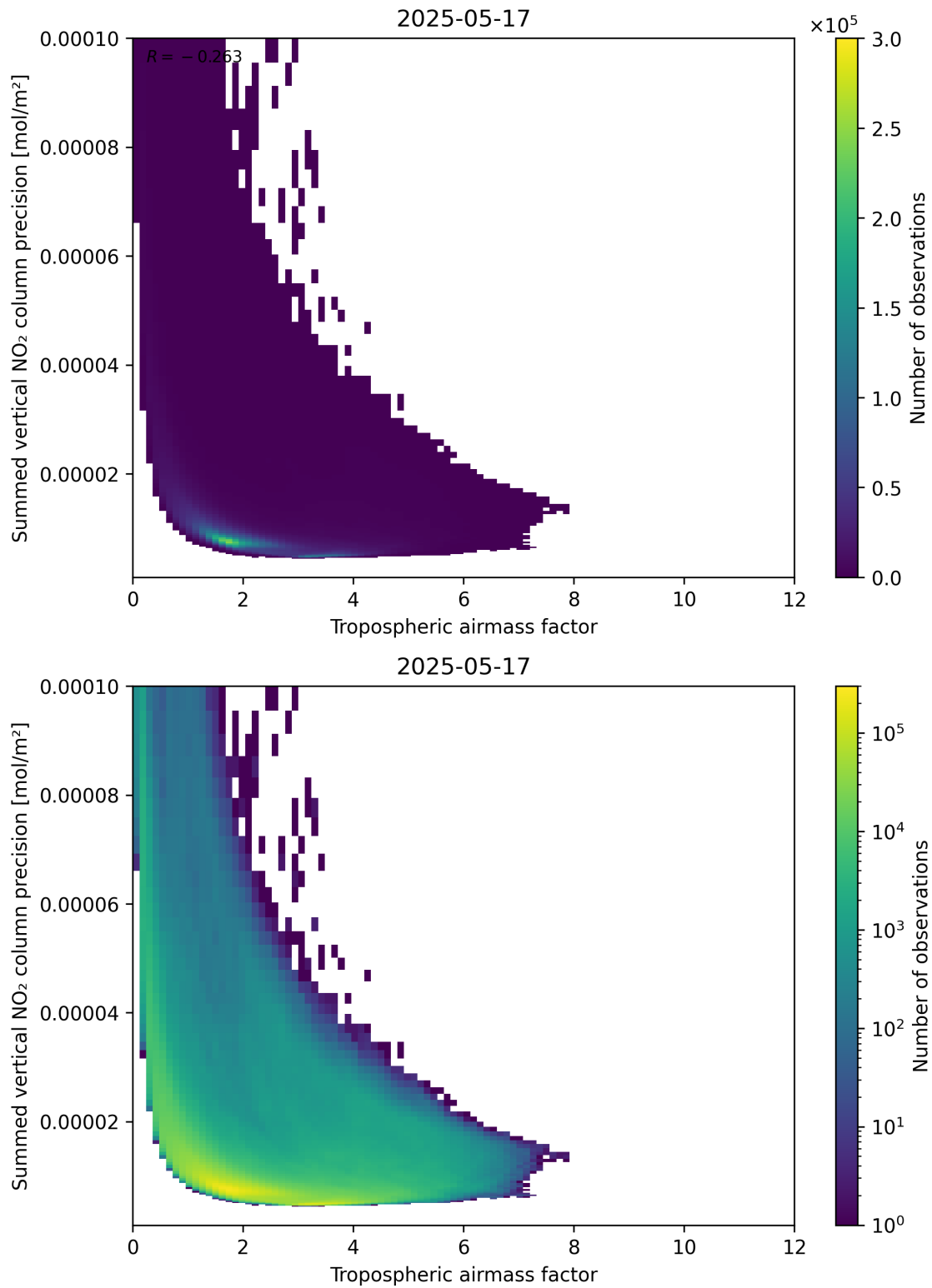
Figure 76: Scatter density plot of “Tropospheric air mass factor” against “Summed vertical NO 2 column precision” for 2025-05-16 to 2025-05-18.
