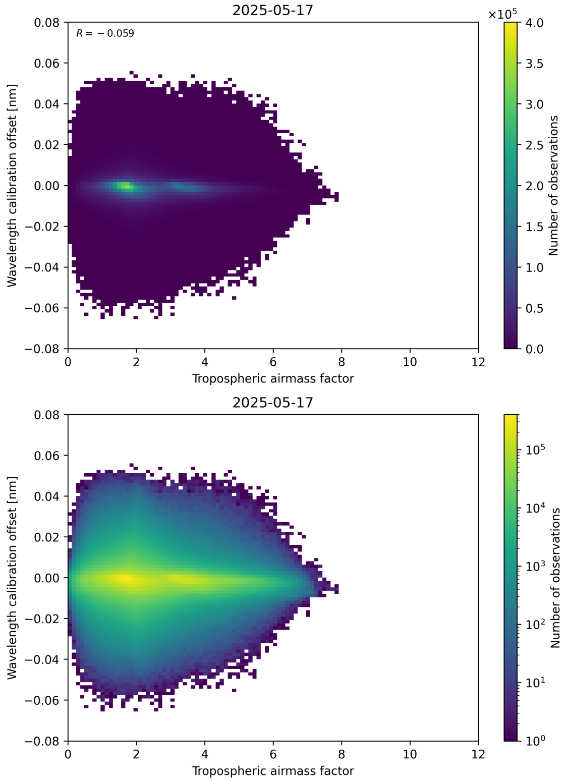
Figure 80: Scatter density plot of “Tropospheric airmass factor” against “Wavelength calibration offset” for 2025-05-16 to 2025-05-18.
