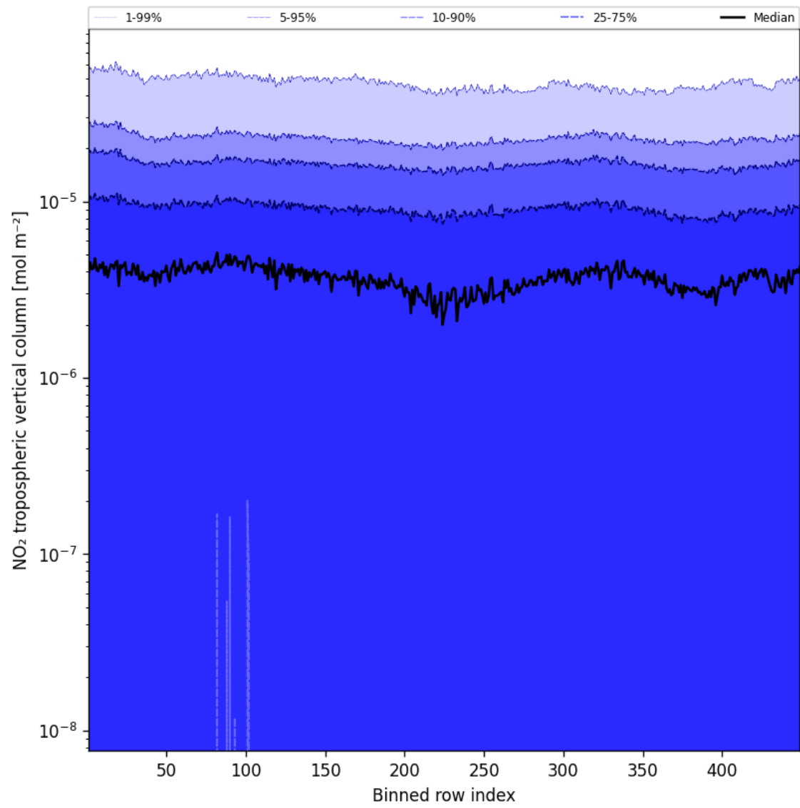
Figure 46: Along track statistics of “NO 2 tropospheric vertical column” for 2025-05-16 to 2025-05-18
