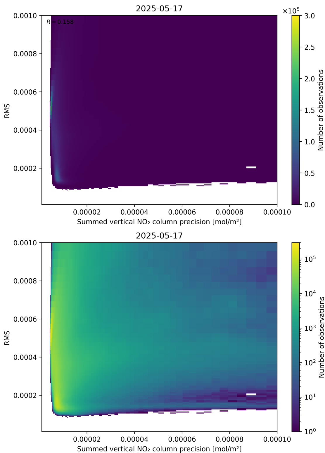
Figure 108: Scatter density plot of “Summed vertical NO 2 column precision” against “RMS” for 2025-05-16 to 2025-05-18.
