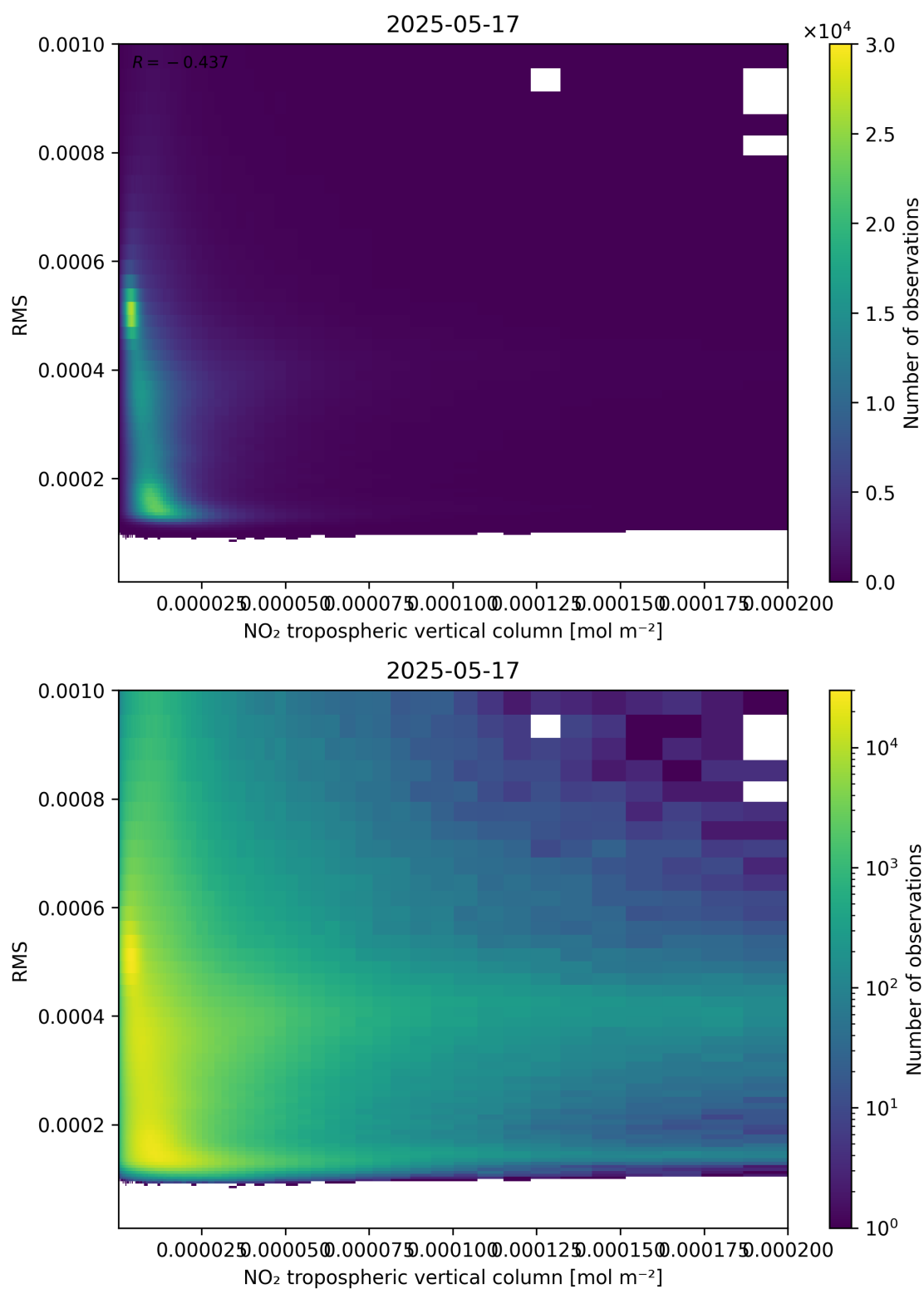
Figure 142: Scatter density plot of “NO 2 tropospheric vertical column” against “RMS” for 2025-05-16 to 2025-05-18.
