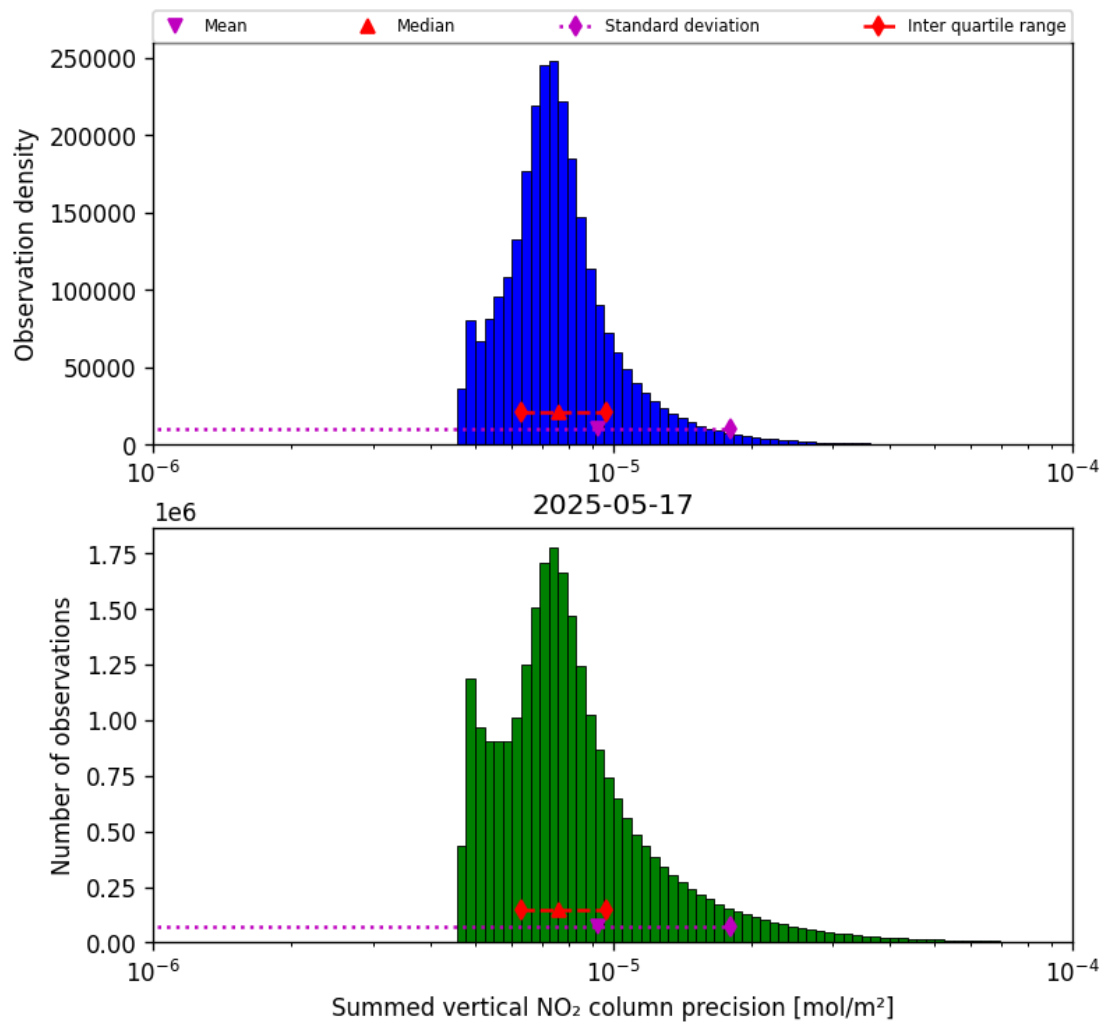
Figure 41: Histogram of "Summed vertical NO 2 column precision" for 2025-05-16 to 2025-05-18
