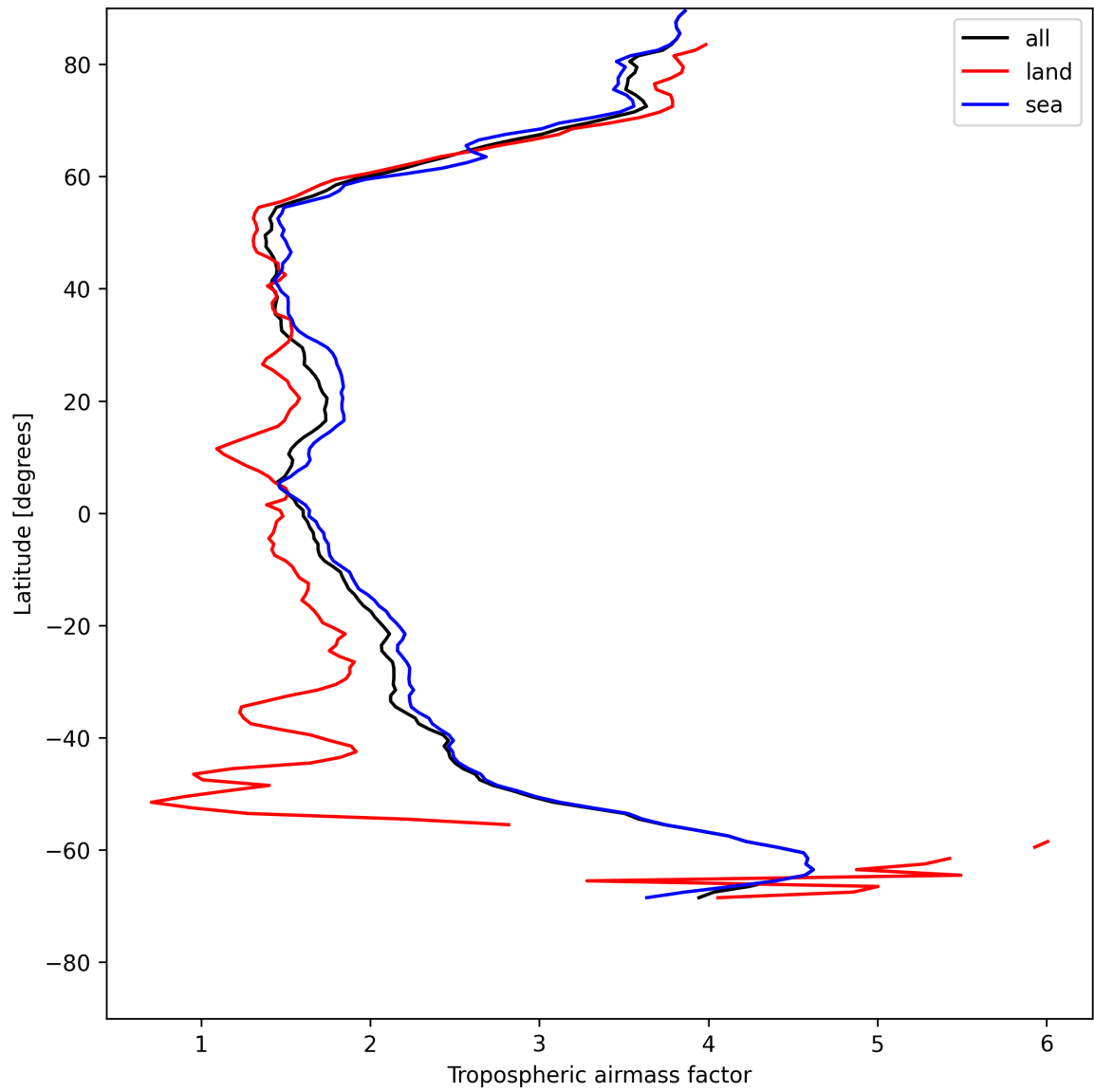
Figure 14: Zonal average of “Tropospheric airmass factor” for 2025-05-16 to 2025-05-18.
