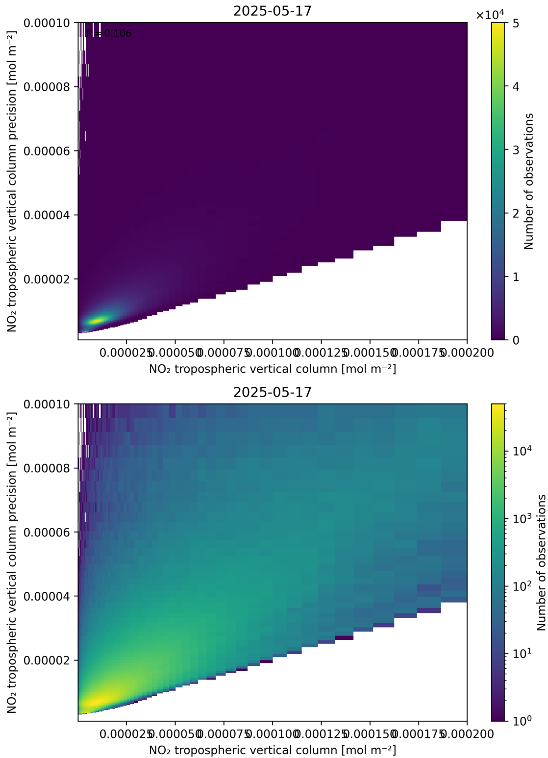
Figure 130: Scatter density plot of “NO 2 tropospheric vertical column” against “NO 2 tropospheric vertical column precision” for 2025-05-16 to 2025-05-18.
