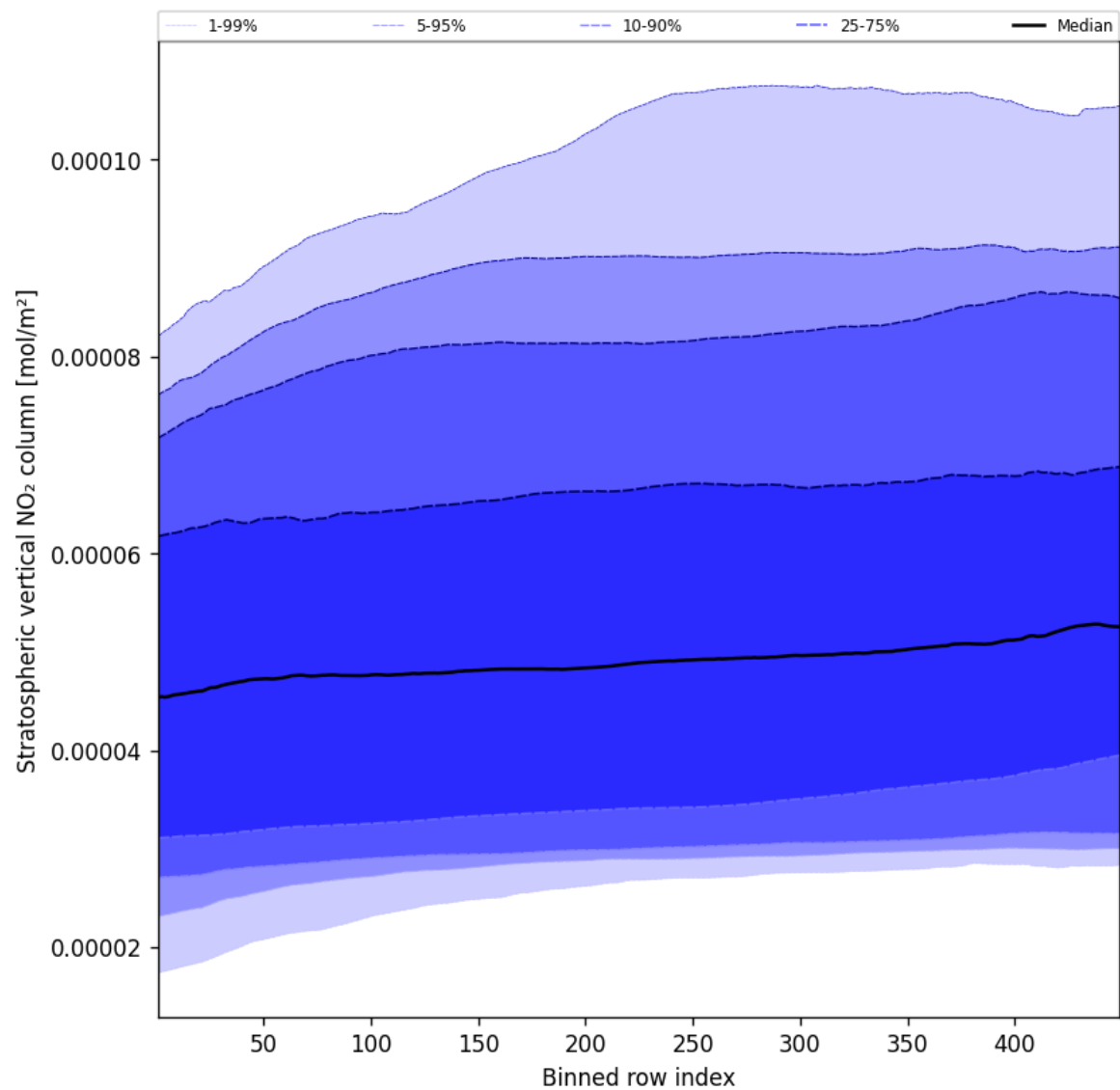
Figure 53: Along track statistics of “Stratospheric vertical NO 2 column” for 2025-05-16 to 2025-05-18
