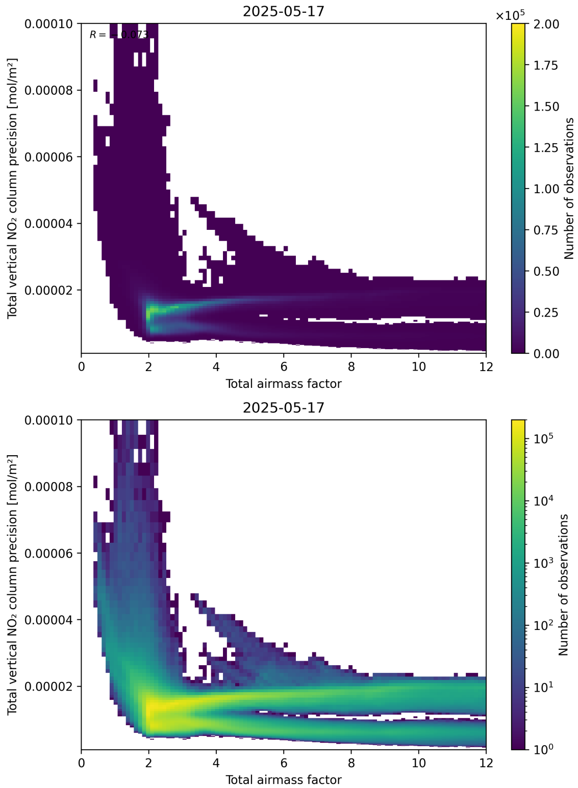
Figure 68: Scatter density plot of “Total airmass factor” against “Total vertical NO 2 column precision” for 2025-05-16 to 2025-05-18.
