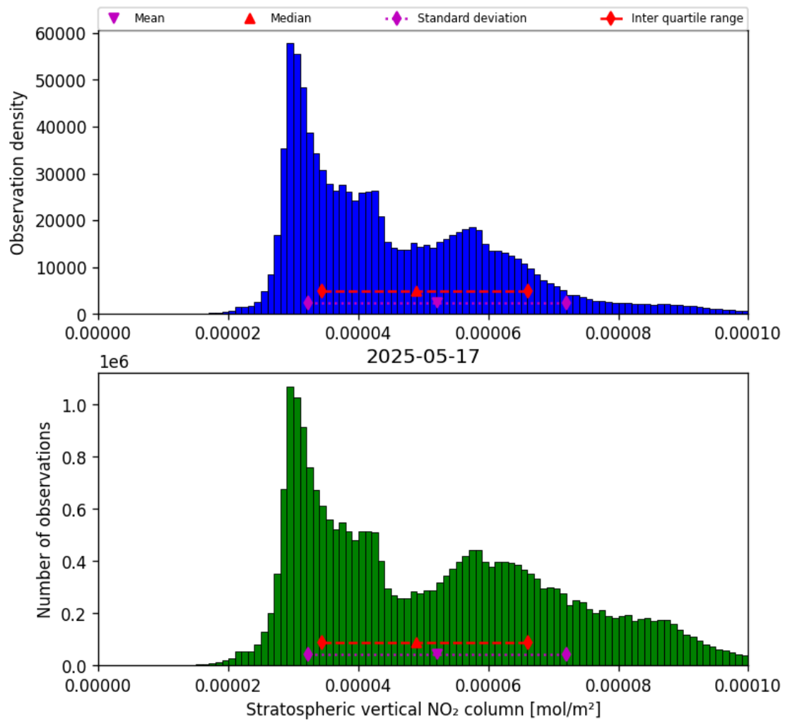
Figure 36: Histogram of “Stratospheric vertical NO 2 column” for 2025-05-16 to 2025-05-18
