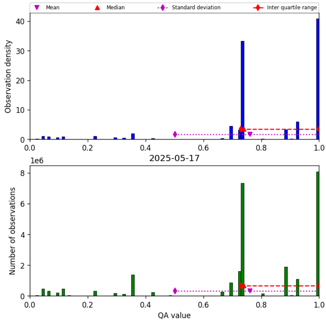
Figure 28: Histogram of “QA value” for 2025-05-16 to 2025-05-18
