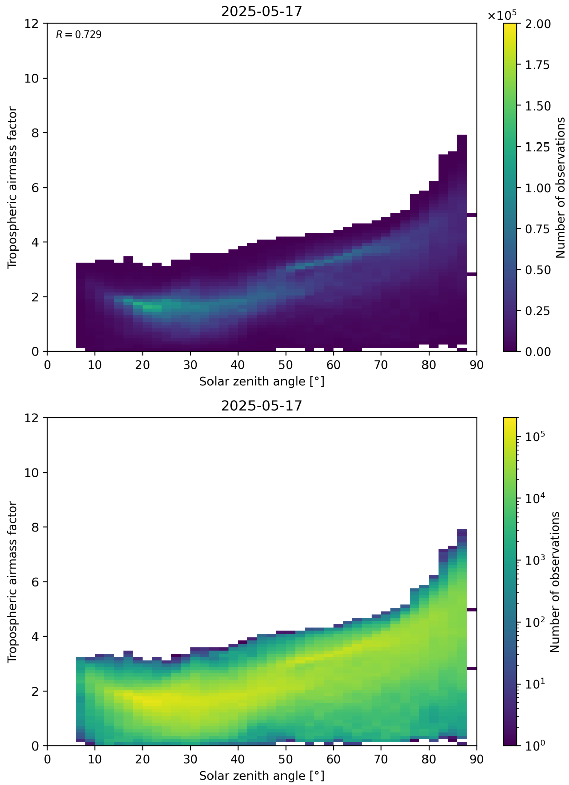
Figure 147: Scatter density plot of “Solar zenith angle” against “Tropospheric airmass factor” for 2025-05-16 to 2025-05-18.
