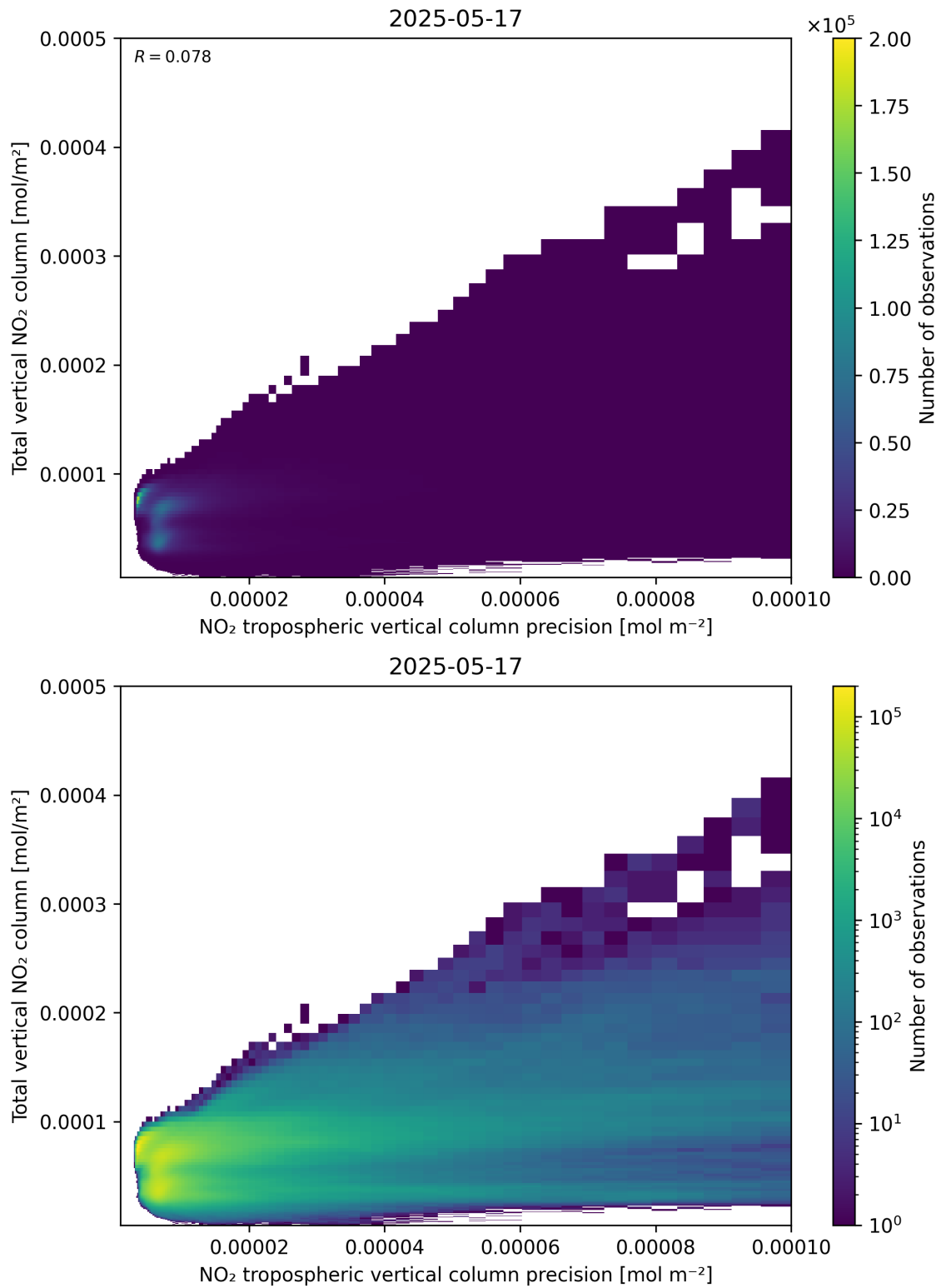
Figure 138: Scatter density plot of “NO 2 tropospheric vertical column precision” against “Total vertical NO 2 column” for 2025-05-16 to 2025-05-18.
