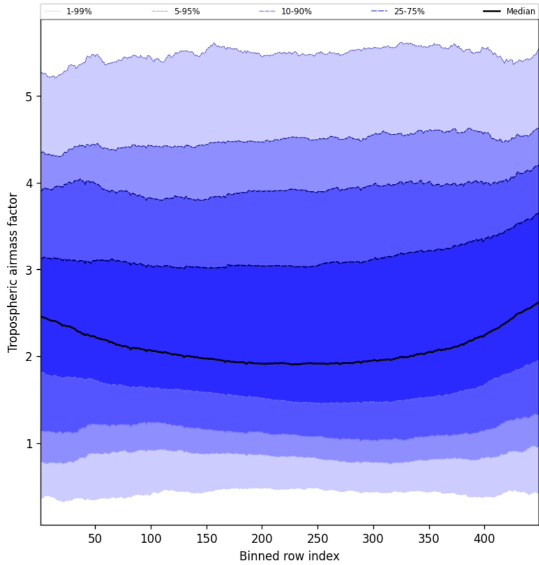
Figure 48: Along track statistics of “Tropospheric airmass factor” for 2025-05-16 to 2025-05-18
