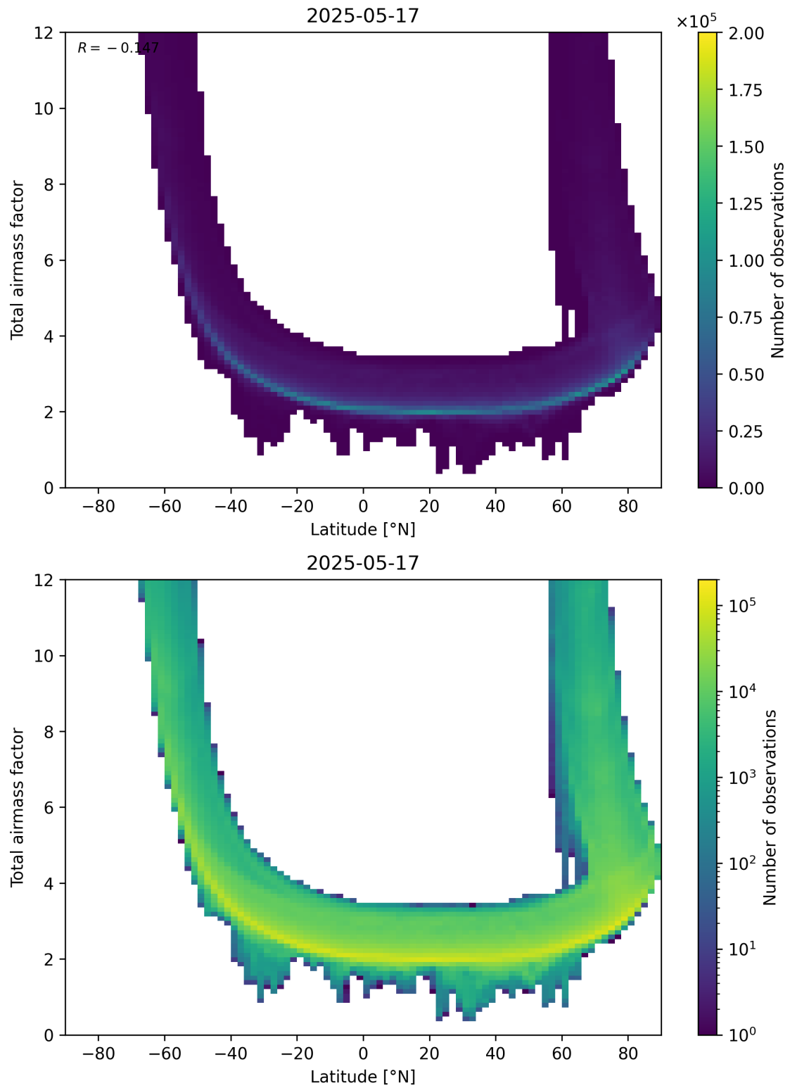
Figure 84: Scatter density plot of “Latitude” against “Total airmass factor” for 2025-05-16 to 2025-05-18.
