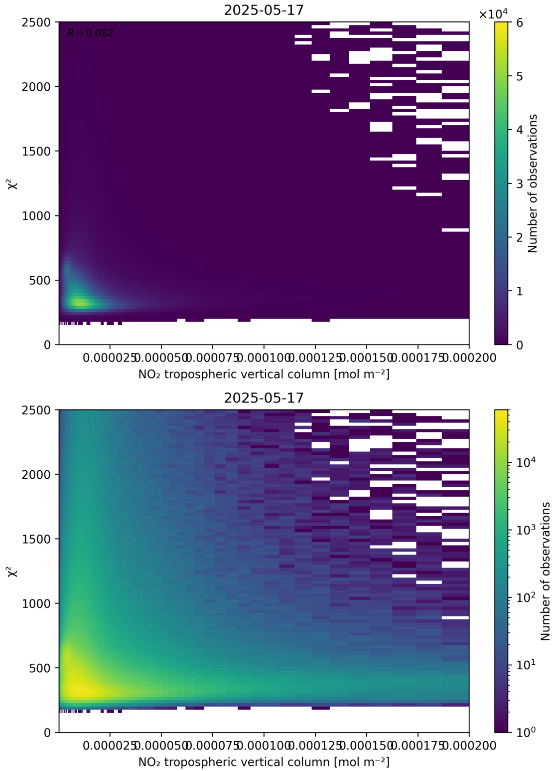
Figure 124: Scatter density plot of “NO 2 tropospheric vertical column” against “ \chi^2 ” for 2025-05-16 to 2025-05-18.
