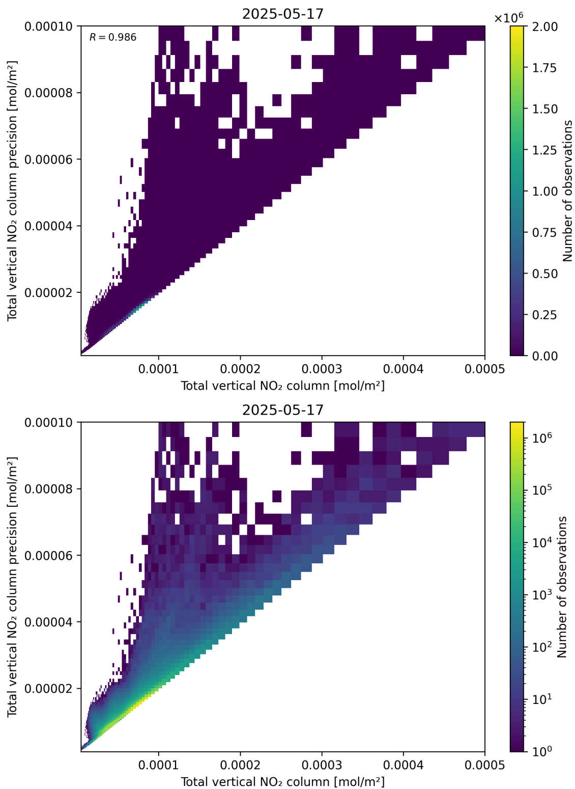
Figure 114: Scatter density plot of “Total vertical NO 2 column” against “Total vertical NO 2 column precision” for 2025-05-16 to 2025-05-18.
