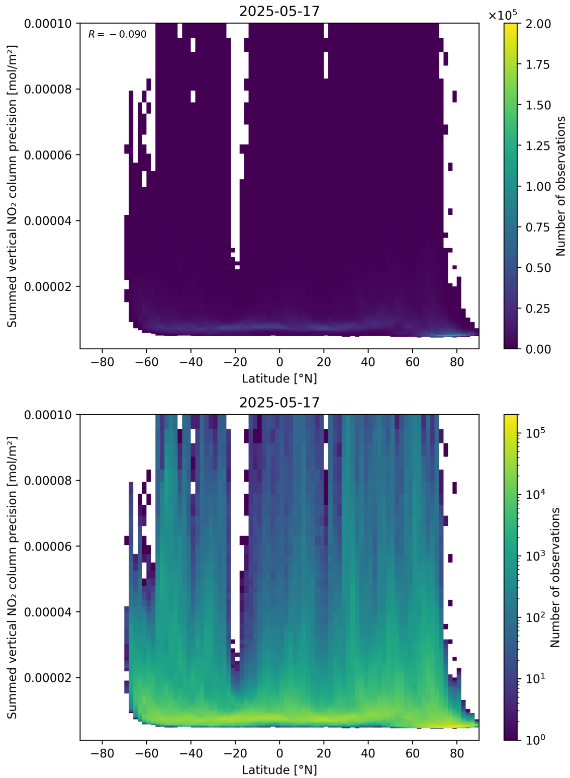
Figure 89: Scatter density plot of “Latitude” against “Summed vertical NO 2 column precision” for 2025-05-16 to 2025-05-18.
