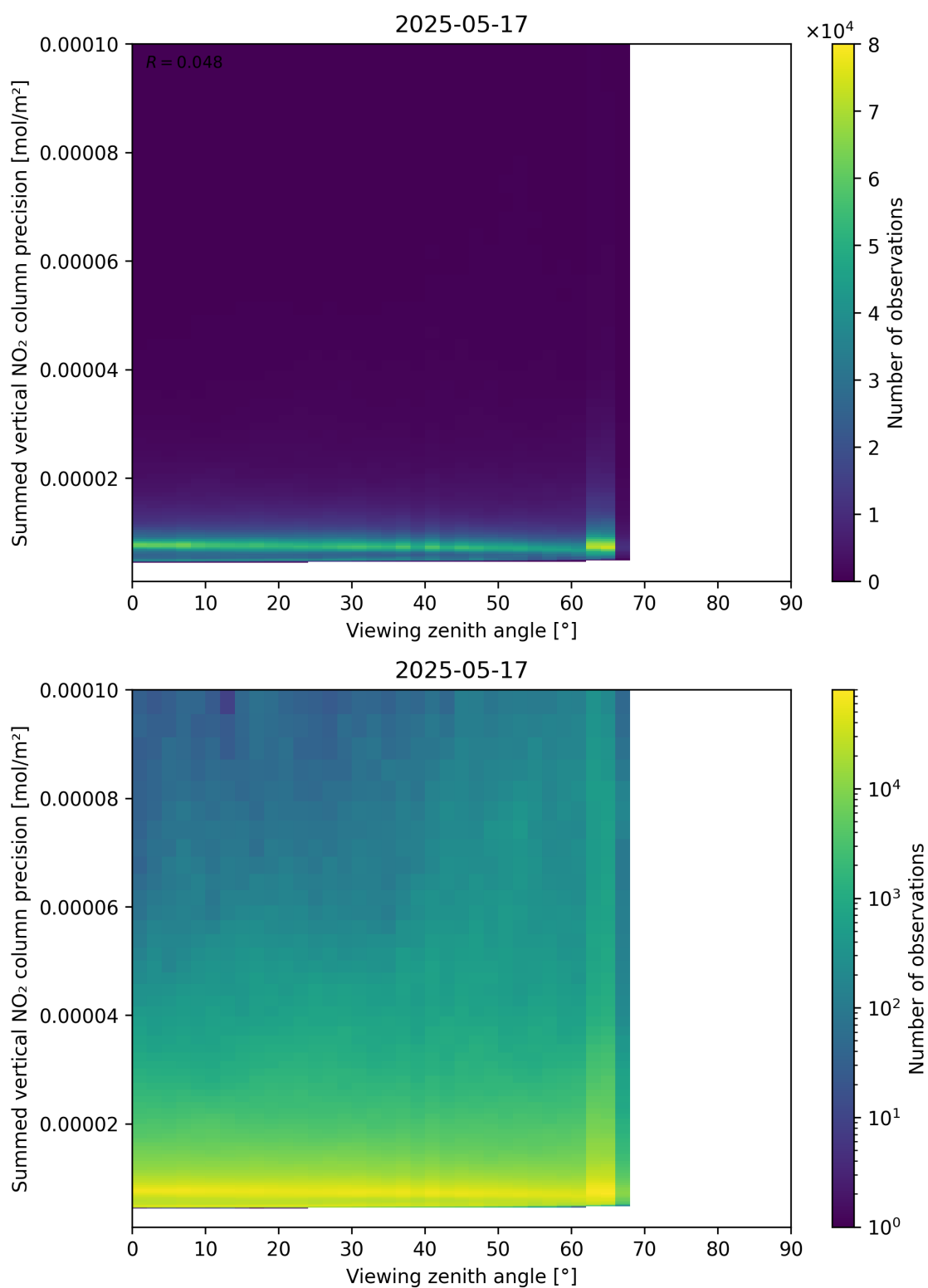
Figure 166: Scatter density plot of “Viewing zenith angle” against “Summed vertical NO 2 column precision” for 2025-05-16 to 2025-05-18.
