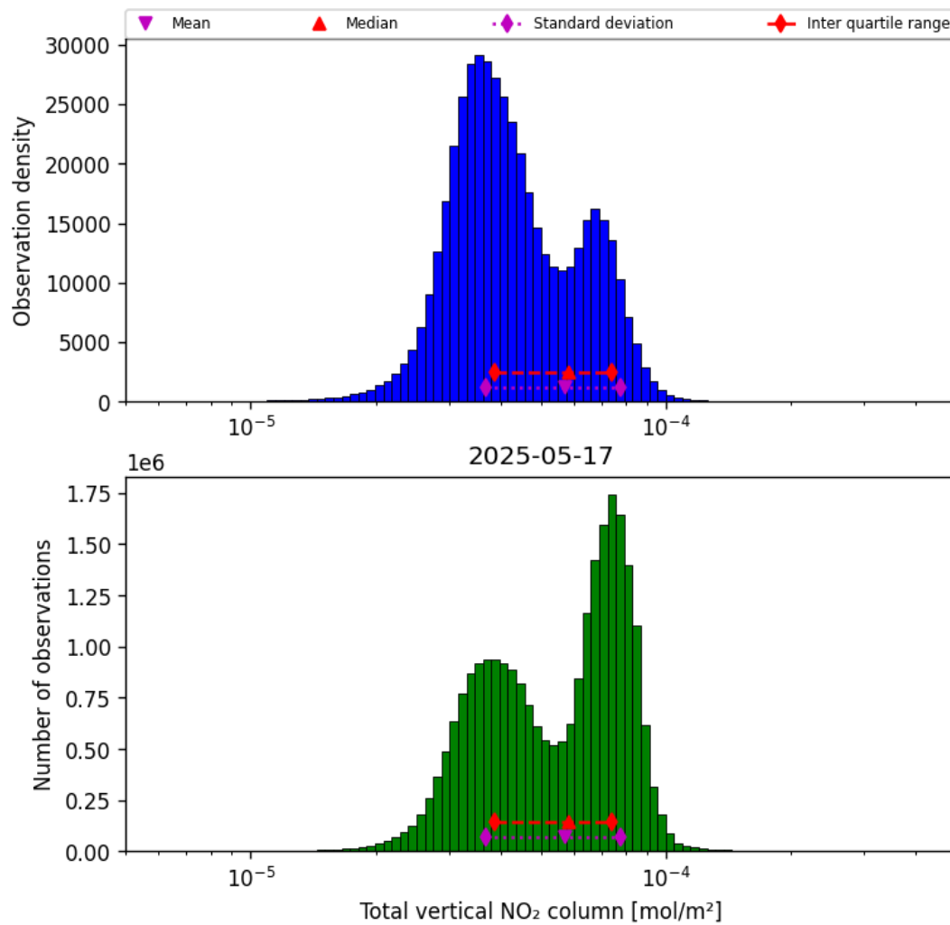
Figure 38: Histogram of "Total vertical NO 2 column" for 2025-05-16 to 2025-05-18
