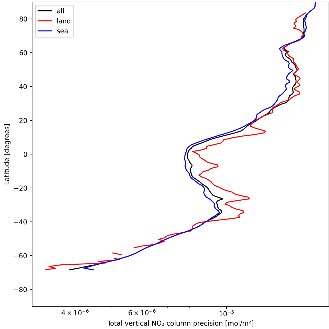
Figure 22: Zonal average of “Total vertical NO 2 column precision” for 2025-05-16 to 2025-05-18.
