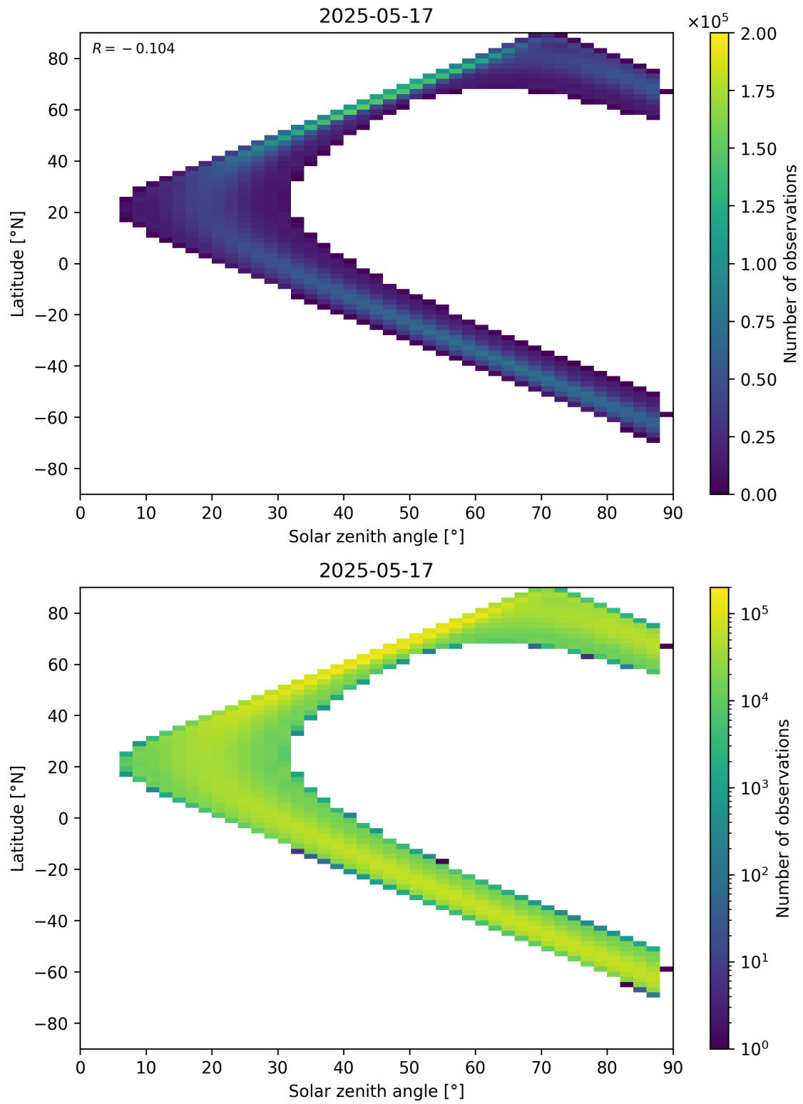
Figure 149: Scatter density plot of “Solar zenith angle” against “Latitude” for 2025-05-16 to 2025-05-18.
