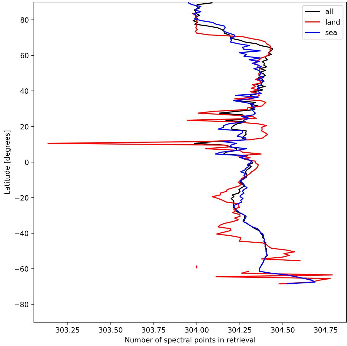
Figure 16: Zonal average of “Number of spectral points in retrieval” for 2025-05-16 to 2025-05-18.
