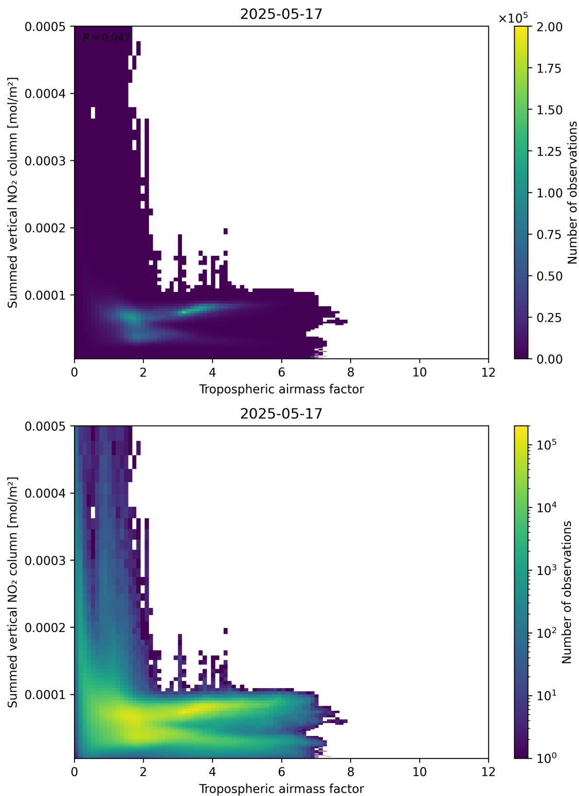
Figure 75: Scatter density plot of “Tropospheric air mass factor” against “Summed vertical NO 2 column” for 2025-05-16 to 2025-05-18.
