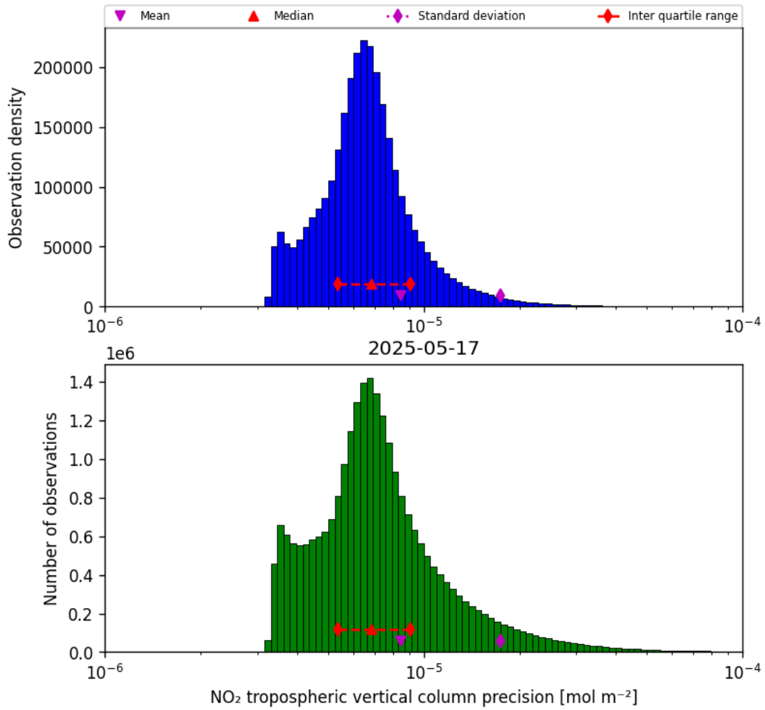
Figure 30: Histogram of “NO 2 tropospheric vertical column precision” for 2025-05-16 to 2025-05-18
