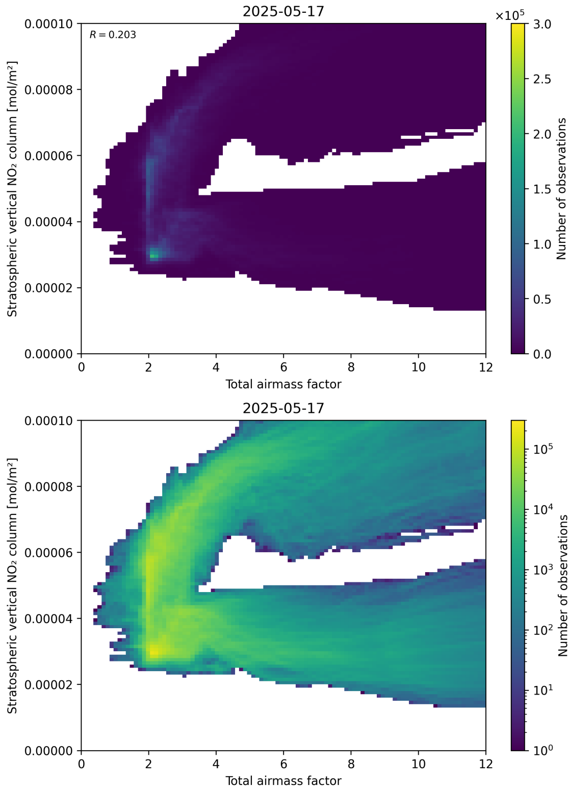
Figure 64: Scatter density plot of “Total airmass factor” against “Stratospheric vertical \text{NO}_2 column” for 2025-05-16 to 2025-05-18.
