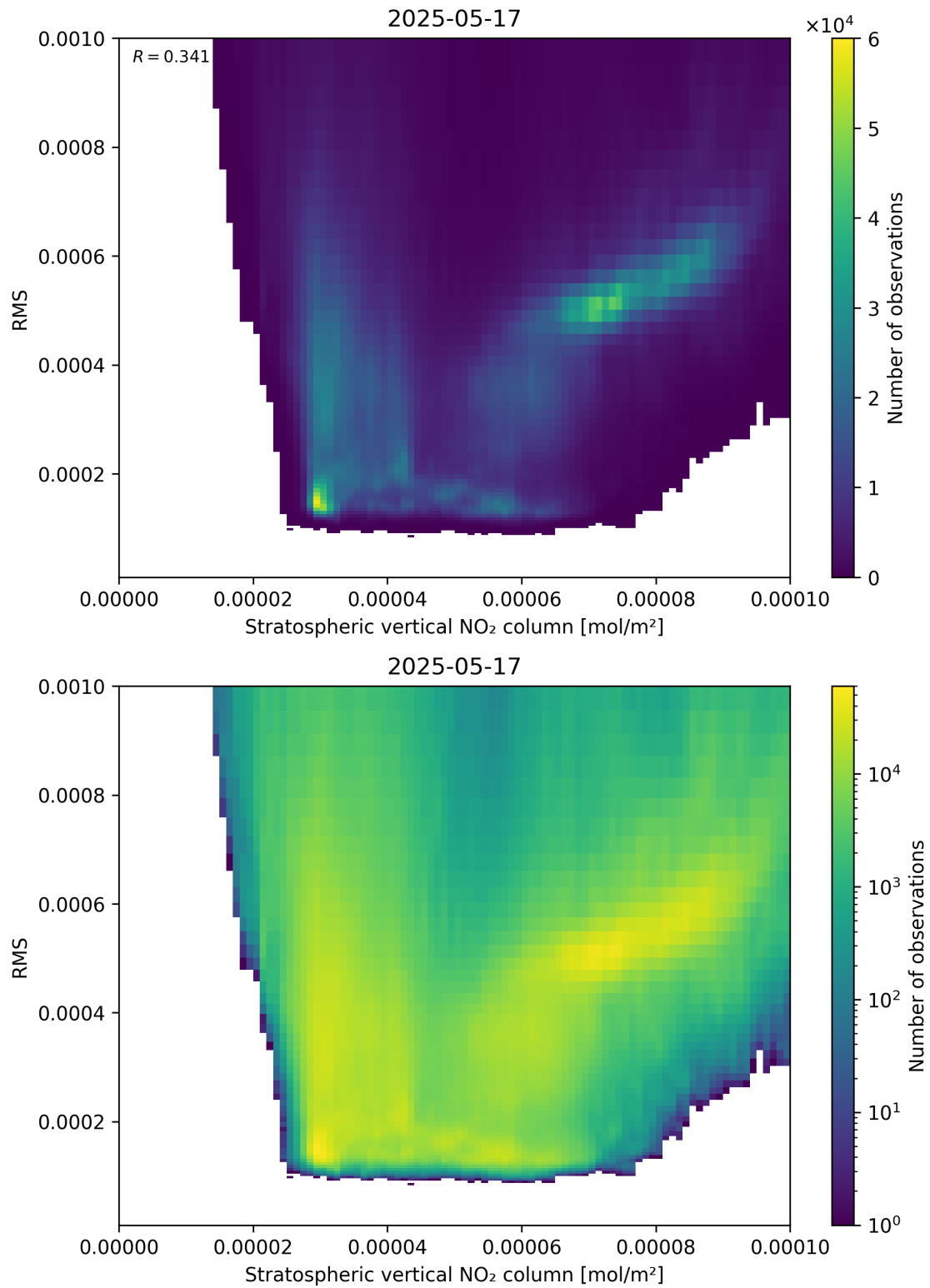
Figure 102: Scatter density plot of “Stratospheric vertical NO 2 column” against “RMS” for 2025-05-16 to 2025-05-18.
