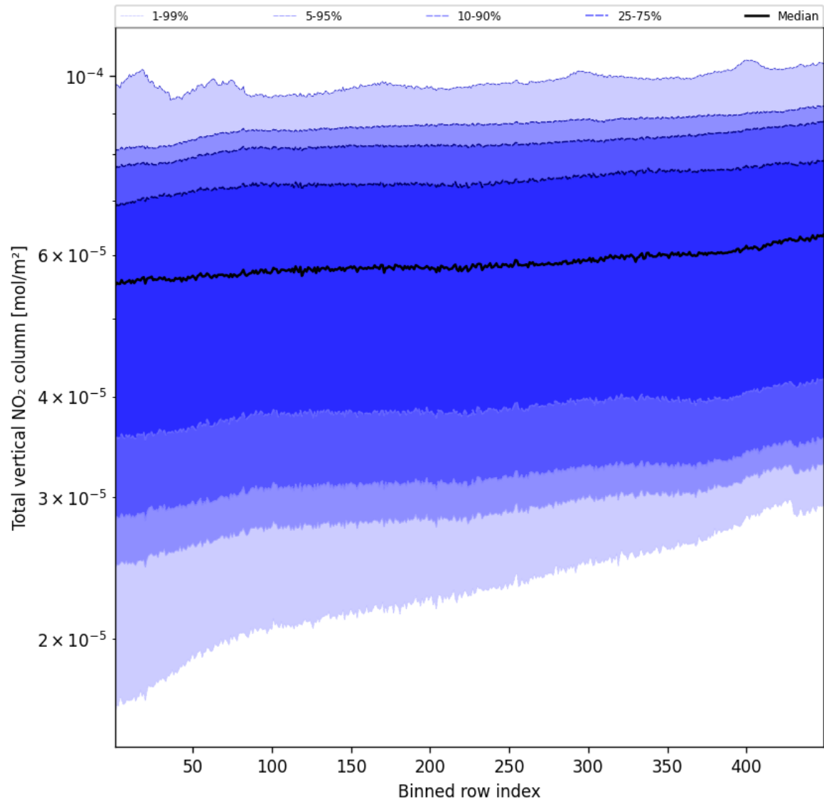
Figure 55: Along track statistics of "Total vertical NO 2 column" for 2025-05-16 to 2025-05-18
