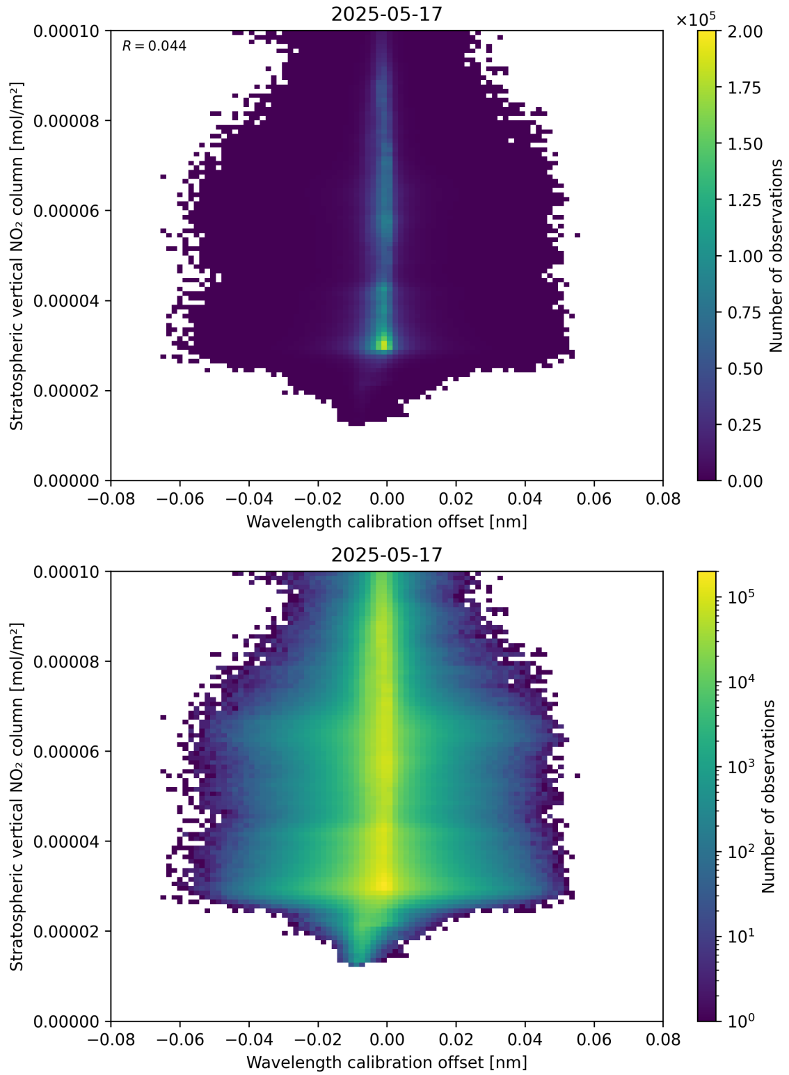
Figure 176: Scatter density plot of “Wavelength calibration offset” against “Stratospheric vertical NO 2 column” for 2025-05-16 to 2025-05-18.
