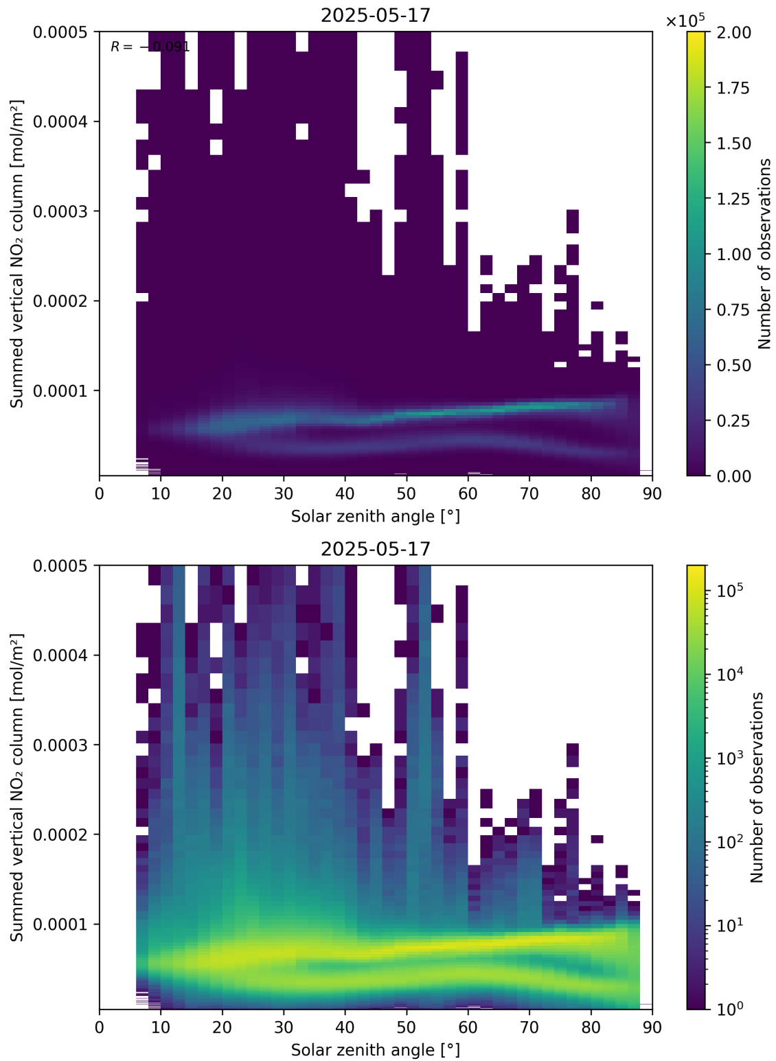
Figure 151: Scatter density plot of “Solar zenith angle” against “Summed vertical NO 2 column” for 2025-05-16 to 2025-05-18.
