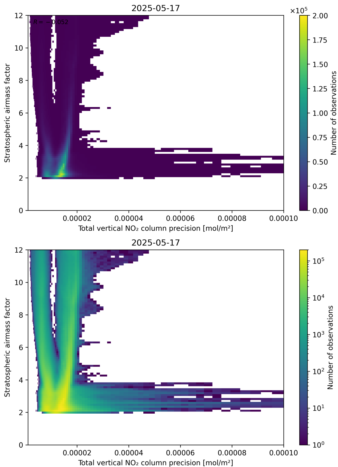
Figure 115: Scatter density plot of “Total vertical NO 2 column precision” against “Stratospheric air mass factor” for 2025-05-16 to 2025-05-18.
