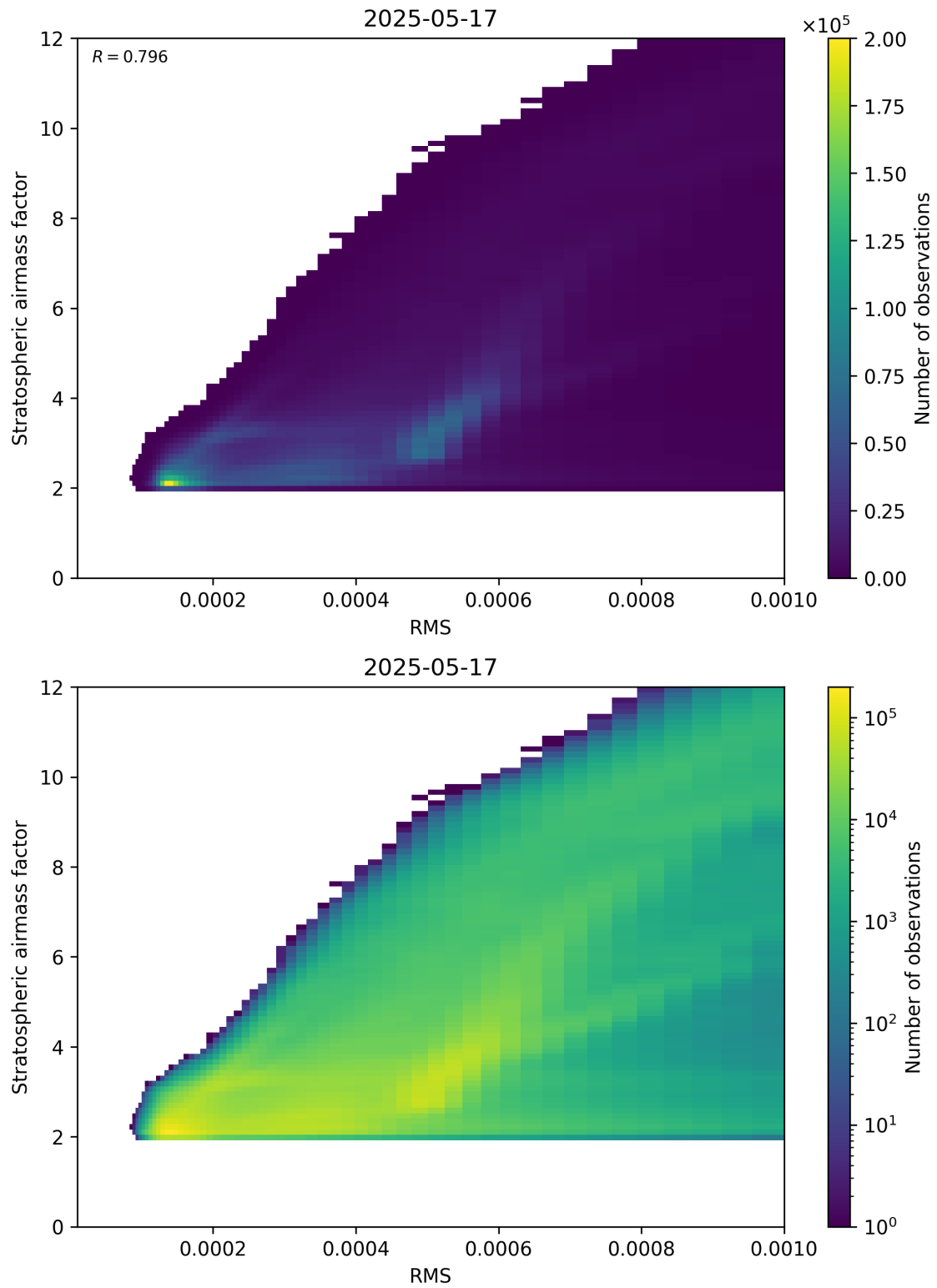
Figure 144: Scatter density plot of “RMS” against “Stratospheric airmass factor” for 2025-05-16 to 2025-05-18.
