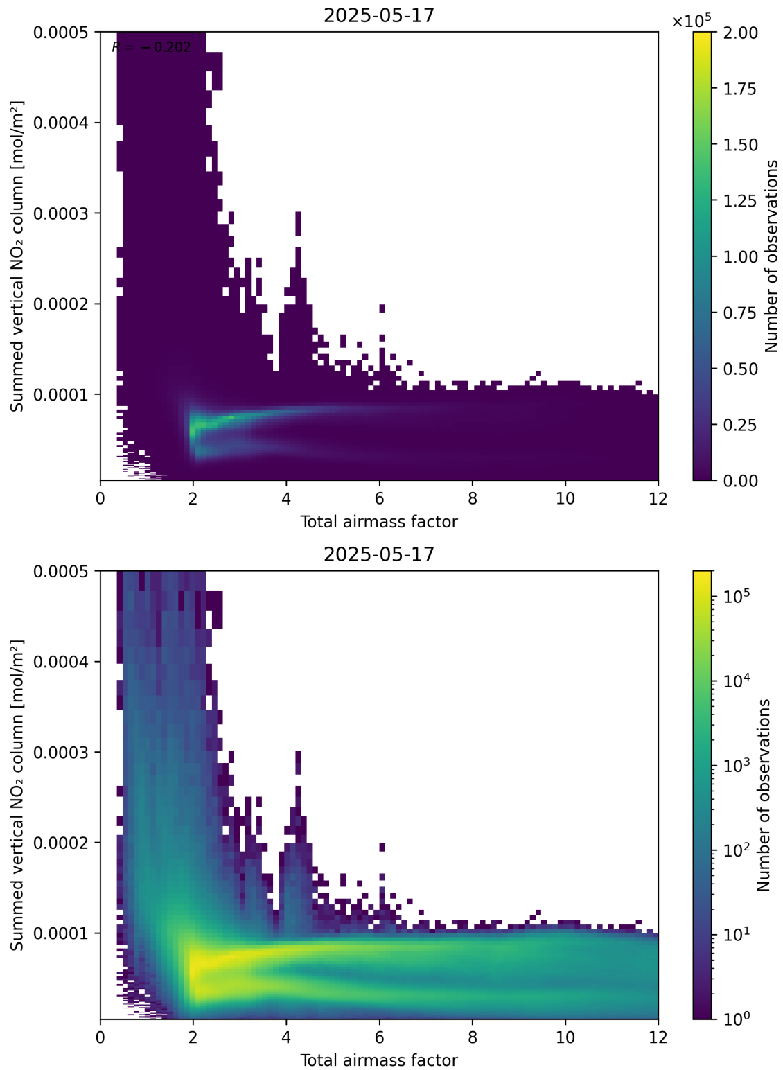
Figure 65: Scatter density plot of “Total airmass factor” against “Summed vertical NO 2 column” for 2025-05-16 to 2025-05-18.
