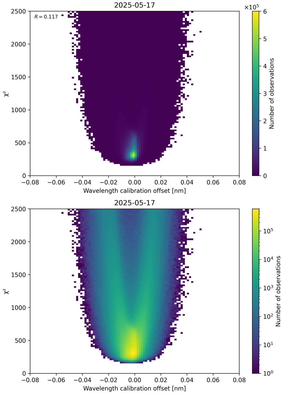
Figure 175: Scatter density plot of “Wavelength calibration offset” against “ \chi^2 ” for 2025-05-16 to 2025-05-18.
