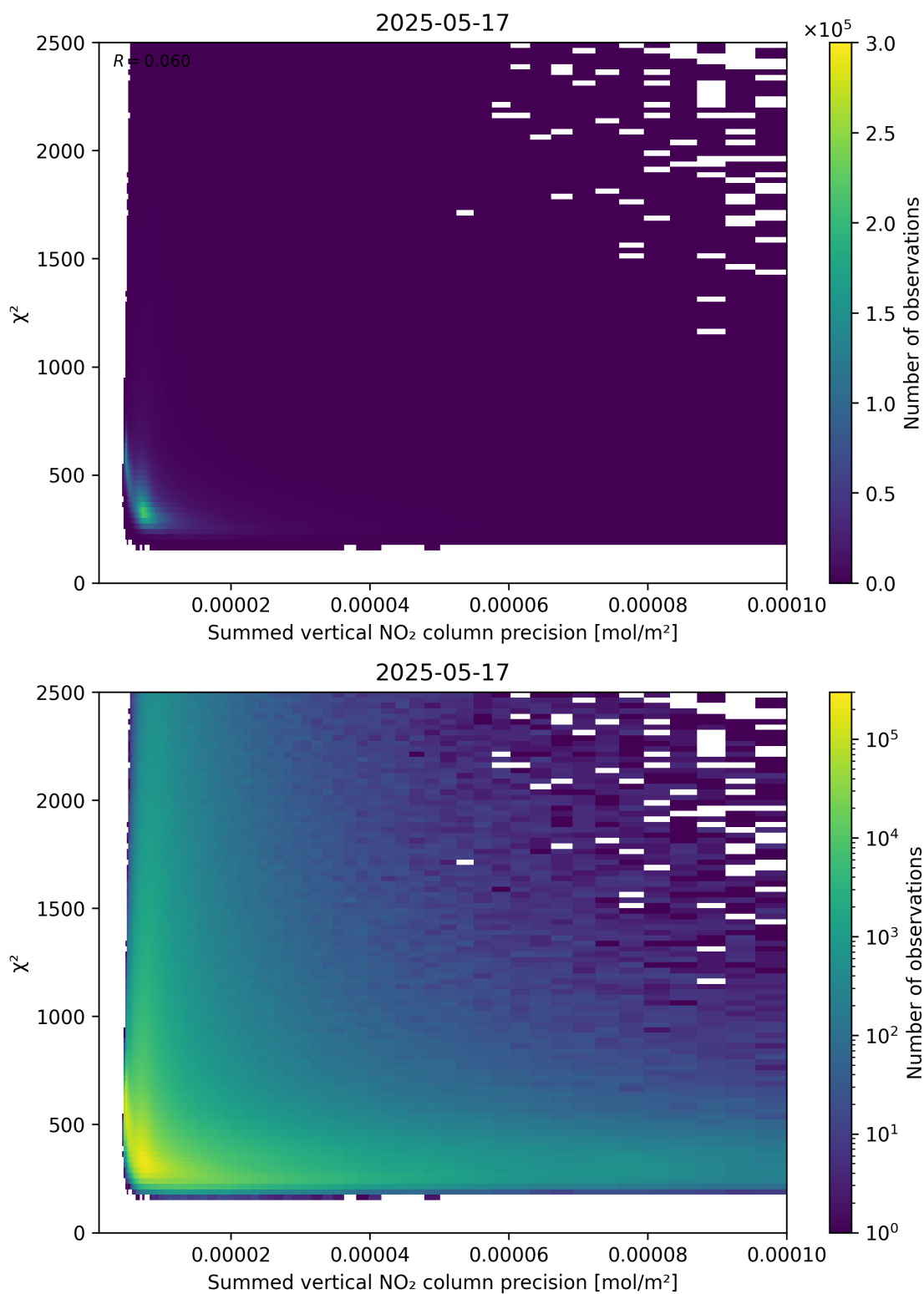
Figure 107: Scatter density plot of “Summed vertical NO 2 column precision” against “ \chi^2 ” for 2025-05-16 to 2025-05-18.
