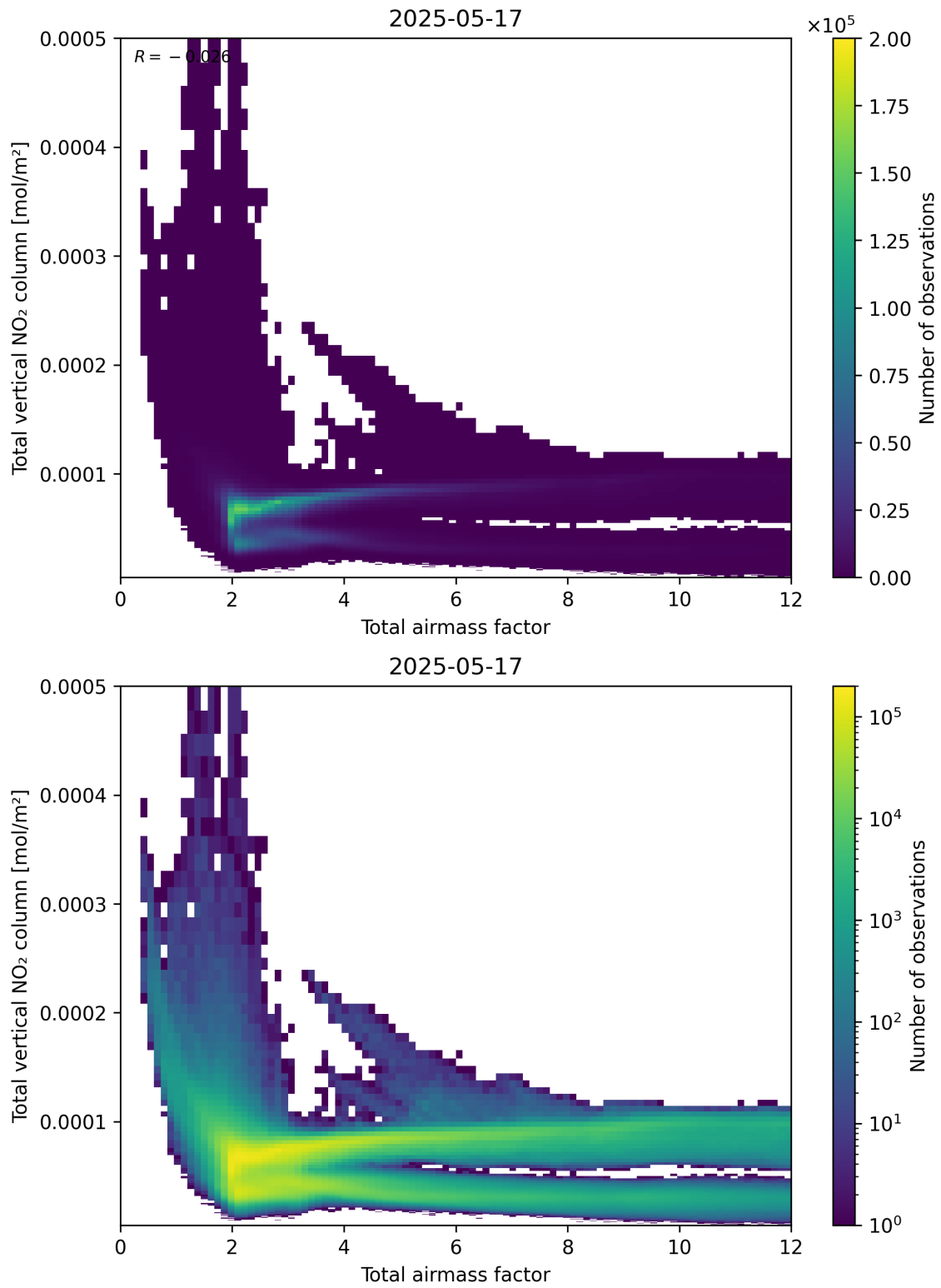
Figure 67: Scatter density plot of “Total airmass factor” against “Total vertical NO 2 column” for 2025-05-16 to 2025-05-18.
