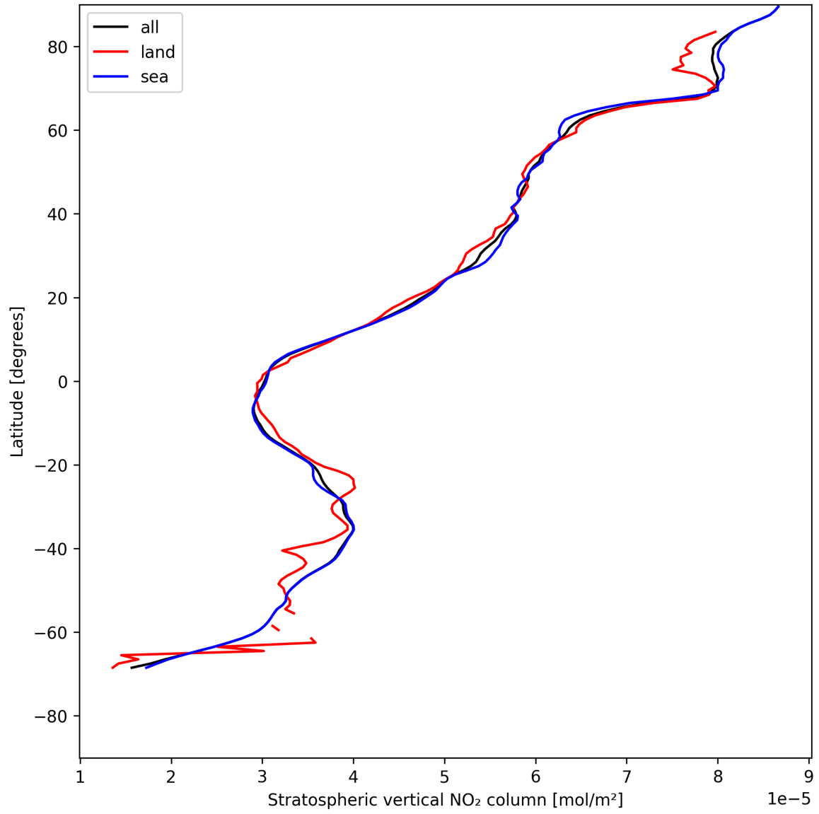
Figure 19: Zonal average of “Stratospheric vertical NO 2 column” for 2025-05-16 to 2025-05-18.
