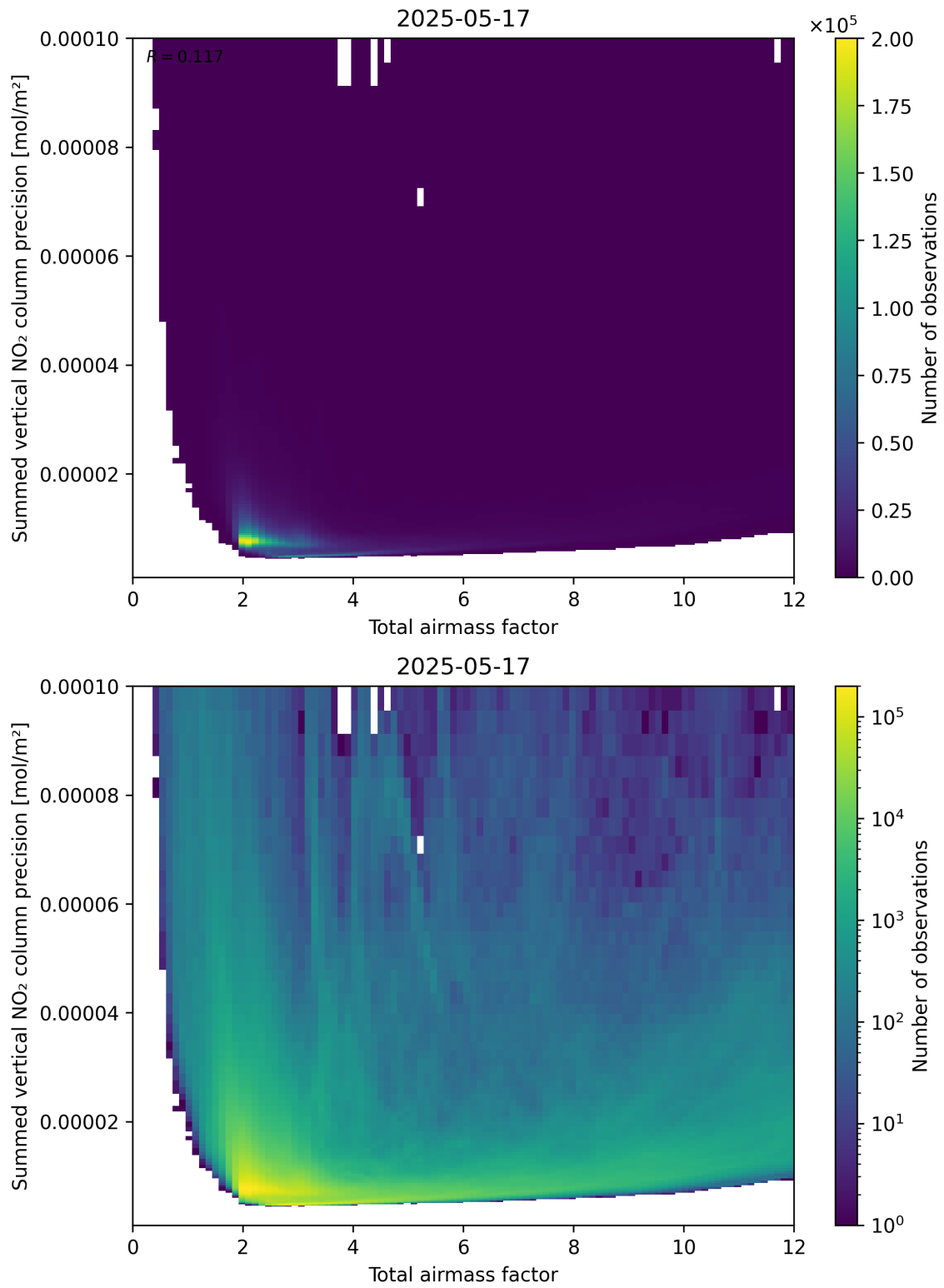
Figure 66: Scatter density plot of “Total airmass factor” against “Summed vertical NO 2 column precision” for 2025-05-16 to 2025-05-18.
