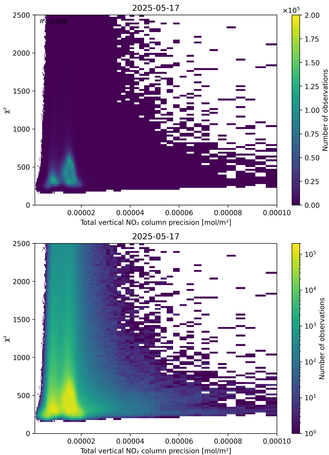
Figure 116: Scatter density plot of “Total vertical NO 2 column precision” against “ \chi^2 ” for 2025-05-16 to 2025-05-18.
