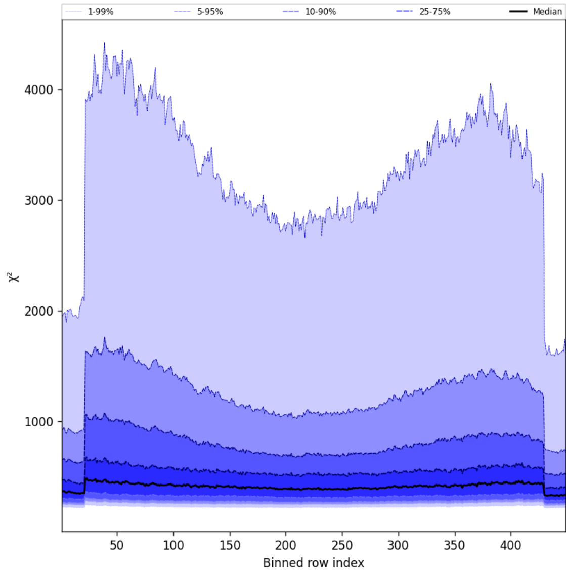
Figure 59: Along track statistics of “ \chi^2 ” for 2025-05-16 to 2025-05-18
