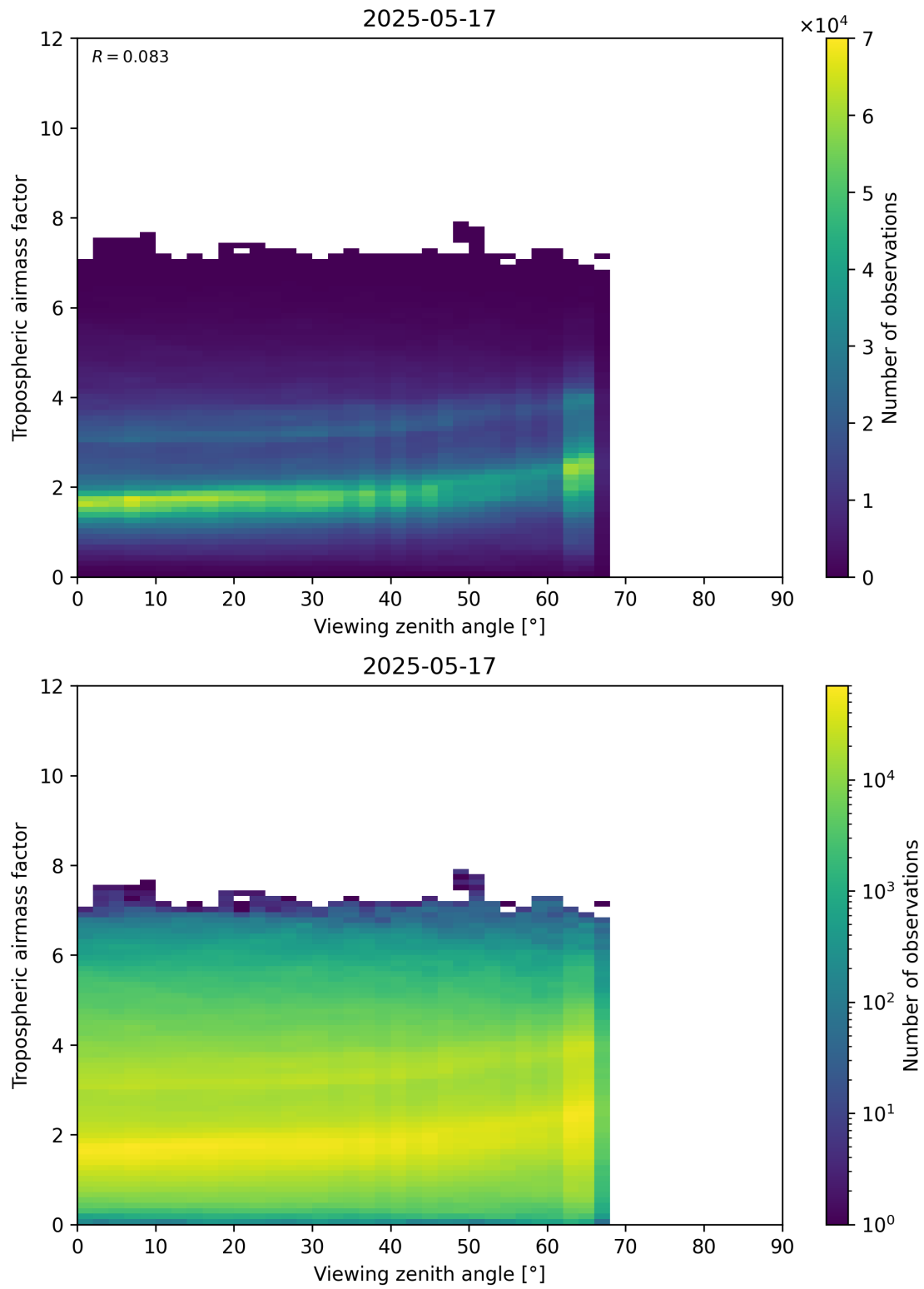
Figure 161: Scatter density plot of “Viewing zenith angle” against “Tropospheric airmass factor” for 2025-05-16 to 2025-05-18.
