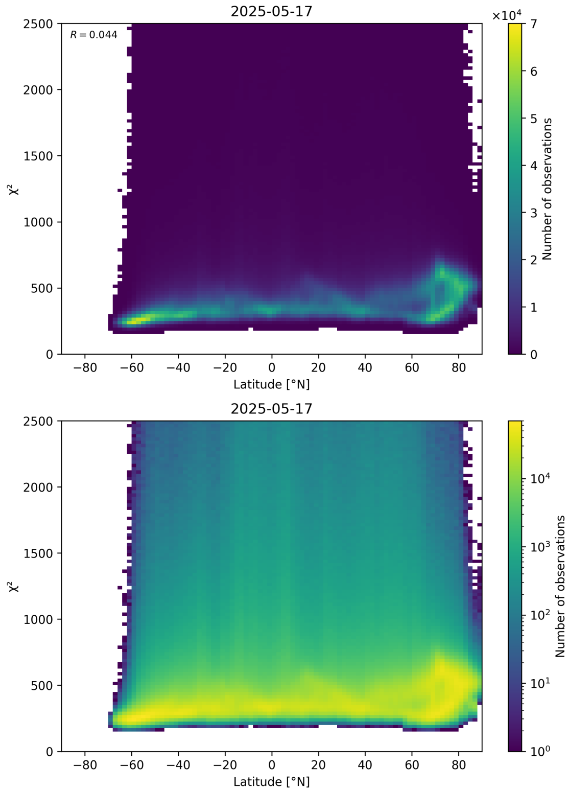
Figure 86: Scatter density plot of “Latitude” against “ \chi^2 ” for 2025-05-16 to 2025-05-18.
