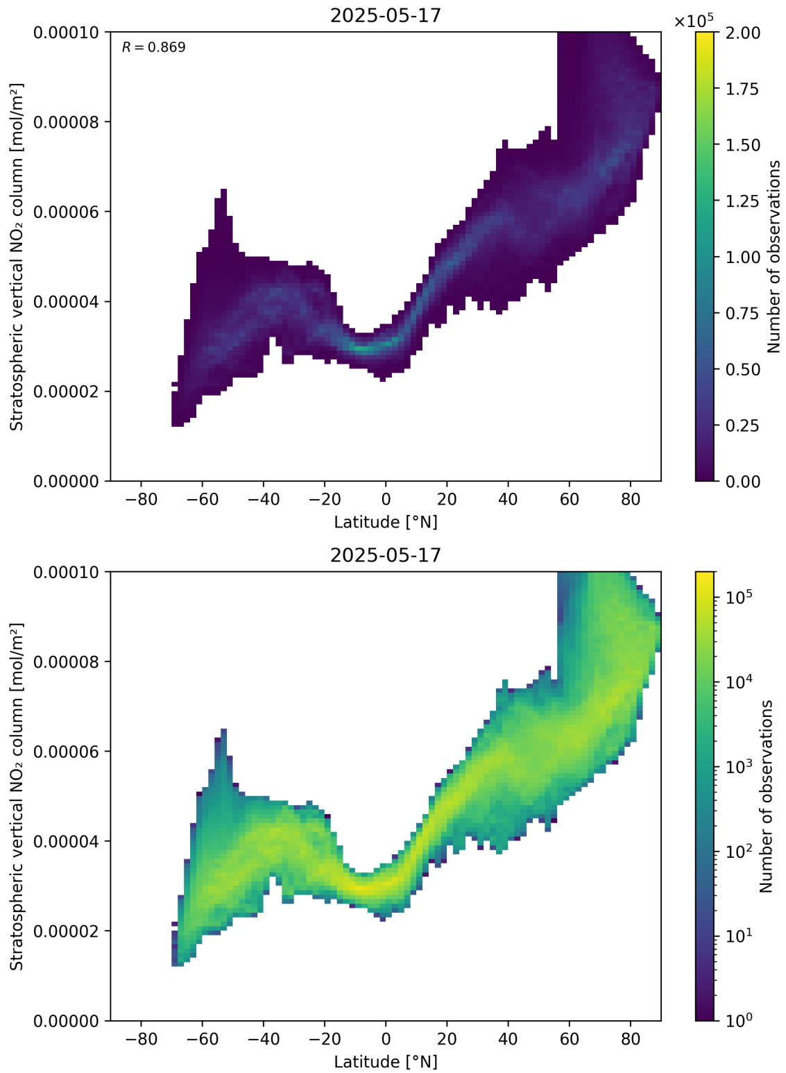
Figure 87: Scatter density plot of “Latitude” against “Stratospheric vertical \text{NO}_2 column” for 2025-05-16 to 2025-05-18.
