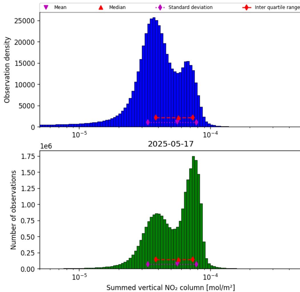
Figure 40: Histogram of “Summed vertical NO 2 column” for 2025-05-16 to 2025-05-18
