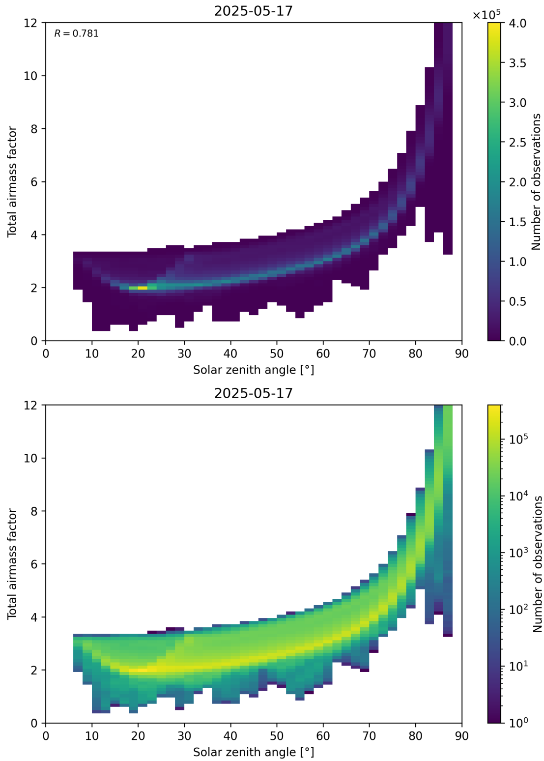
Figure 146: Scatter density plot of “Solar zenith angle” against “Total air mass factor” for 2025-05-16 to 2025-05-18.
