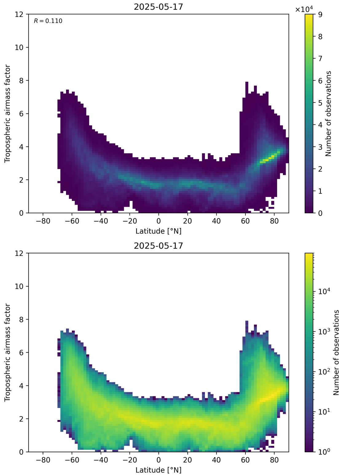
Figure 85: Scatter density plot of “Latitude” against “Tropospheric airmass factor” for 2025-05-16 to 2025-05-18.
