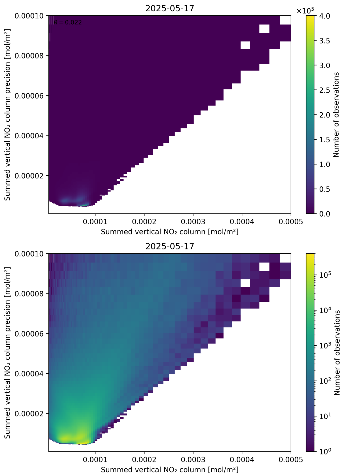
Figure 105: Scatter density plot of “Summed vertical NO 2 column” against “Summed vertical NO 2 column precision” for 2025-05-16 to 2025-05-18.
