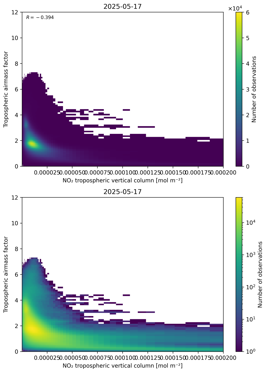
Figure 123: Scatter density plot of “NO 2 tropospheric vertical column” against “Tropospheric air mass factor” for 2025-05-16 to 2025-05-18.
