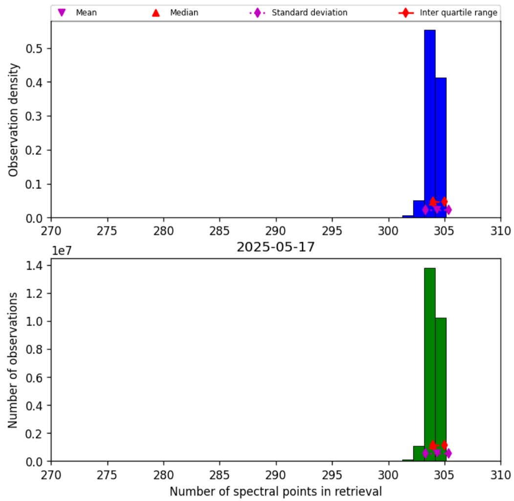
Figure 33: Histogram of “Number of spectral points in retrieval” for 2025-05-16 to 2025-05-18
