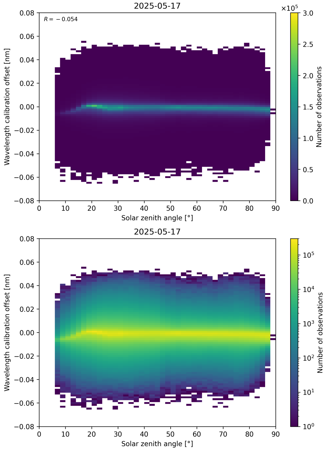
Figure 158: Scatter density plot of “Solar zenith angle” against “Wavelength calibration offset” for 2025-05-16 to 2025-05-18.
