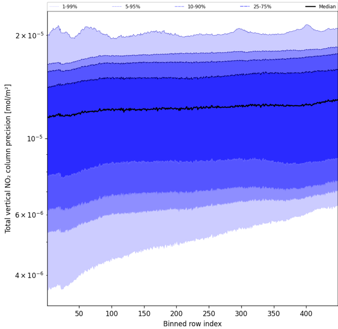
Figure 56: Along track statistics of “Total vertical NO 2 column precision” for 2025-05-16 to 2025-05-18
