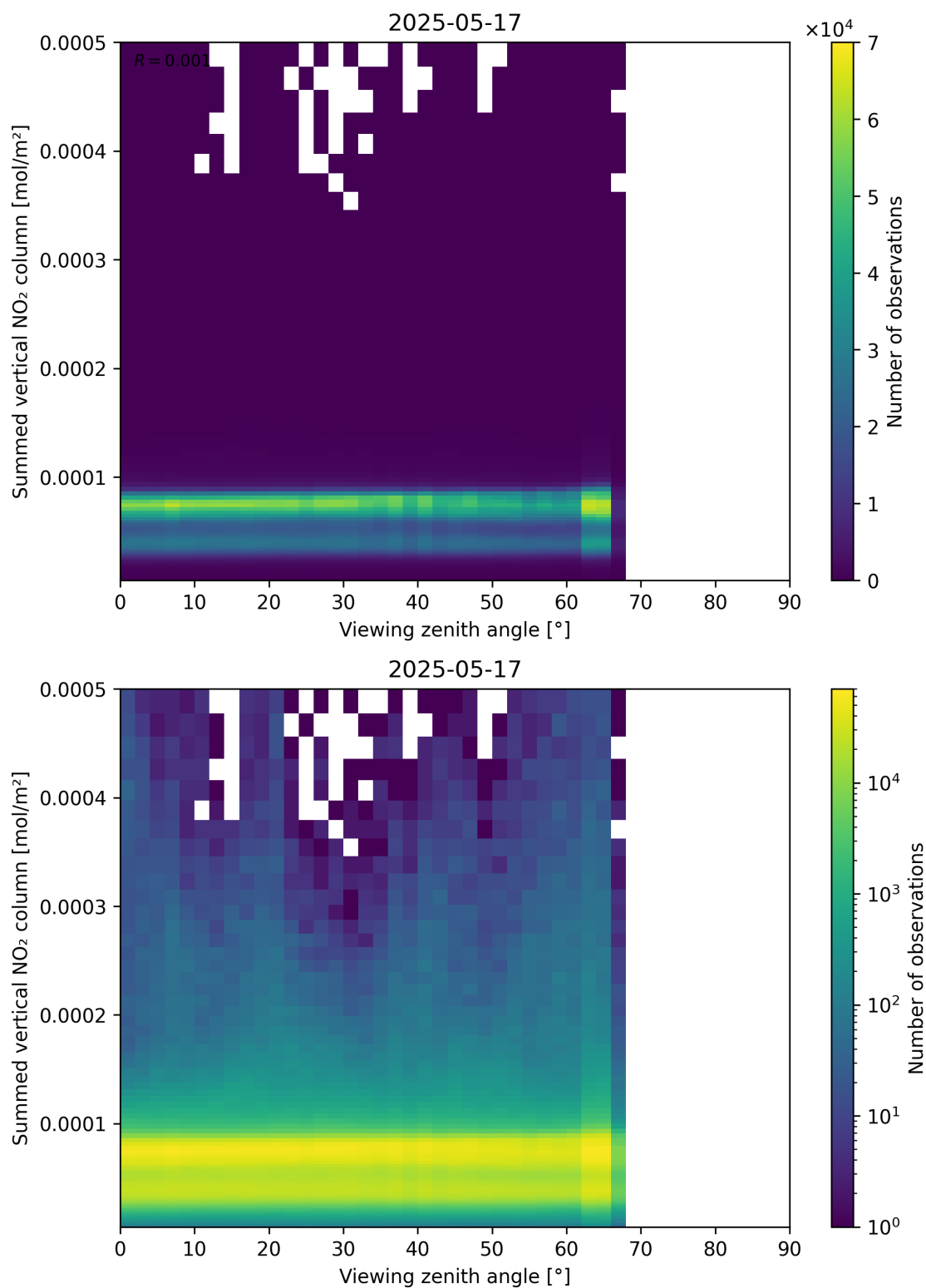
Figure 165: Scatter density plot of “Viewing zenith angle” against “Summed vertical NO 2 column” for 2025-05-16 to 2025-05-18.
