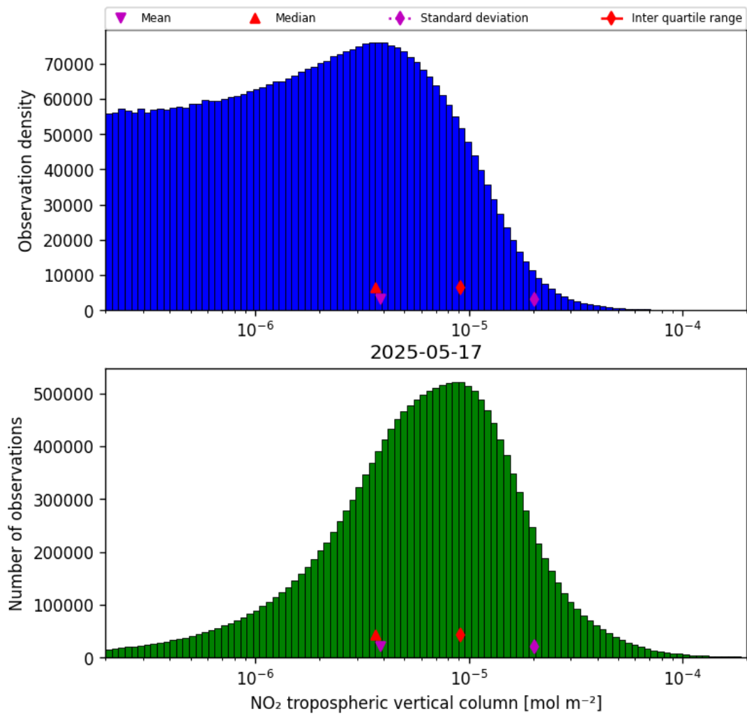
Figure 29: Histogram of “NO 2 tropospheric vertical column” for 2025-05-16 to 2025-05-18
