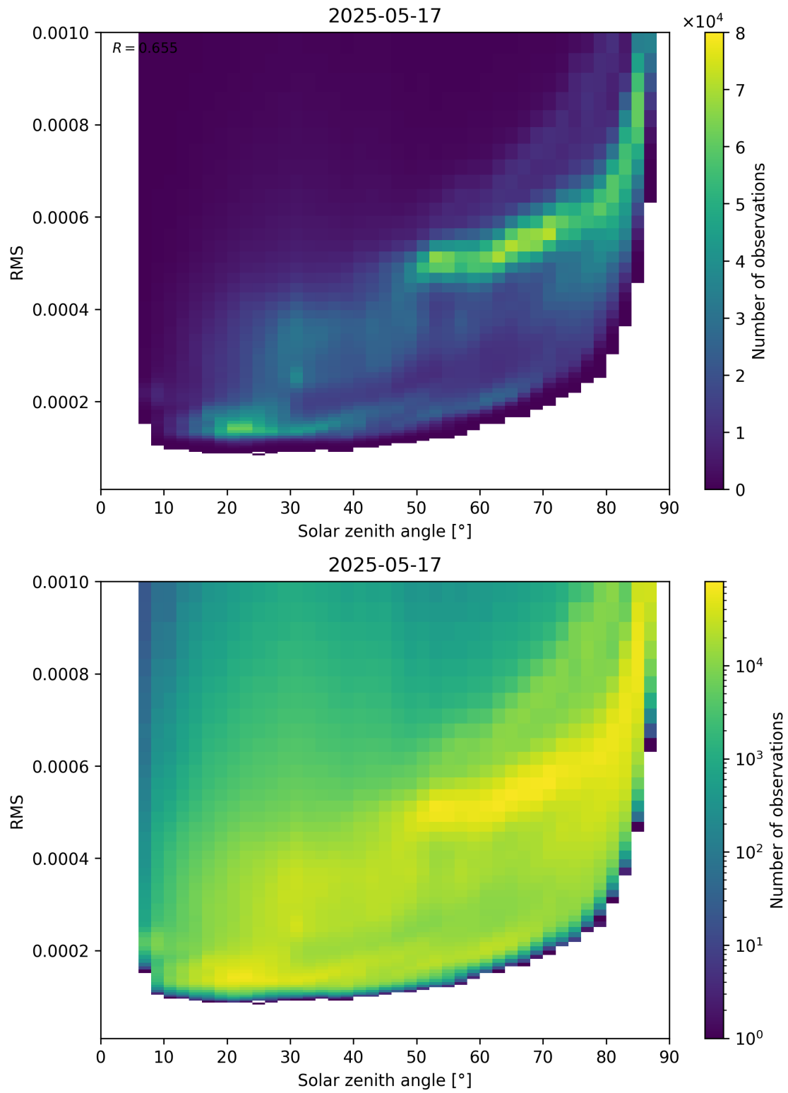
Figure 157: Scatter density plot of “Solar zenith angle” against “RMS” for 2025-05-16 to 2025-05-18.
