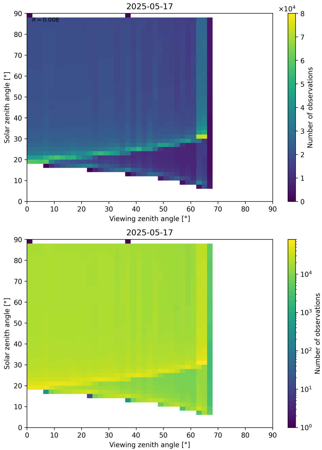
Figure 172: Scatter density plot of “Viewing zenith angle” against “Solar zenith angle” for 2025-05-16 to 2025-05-18.
