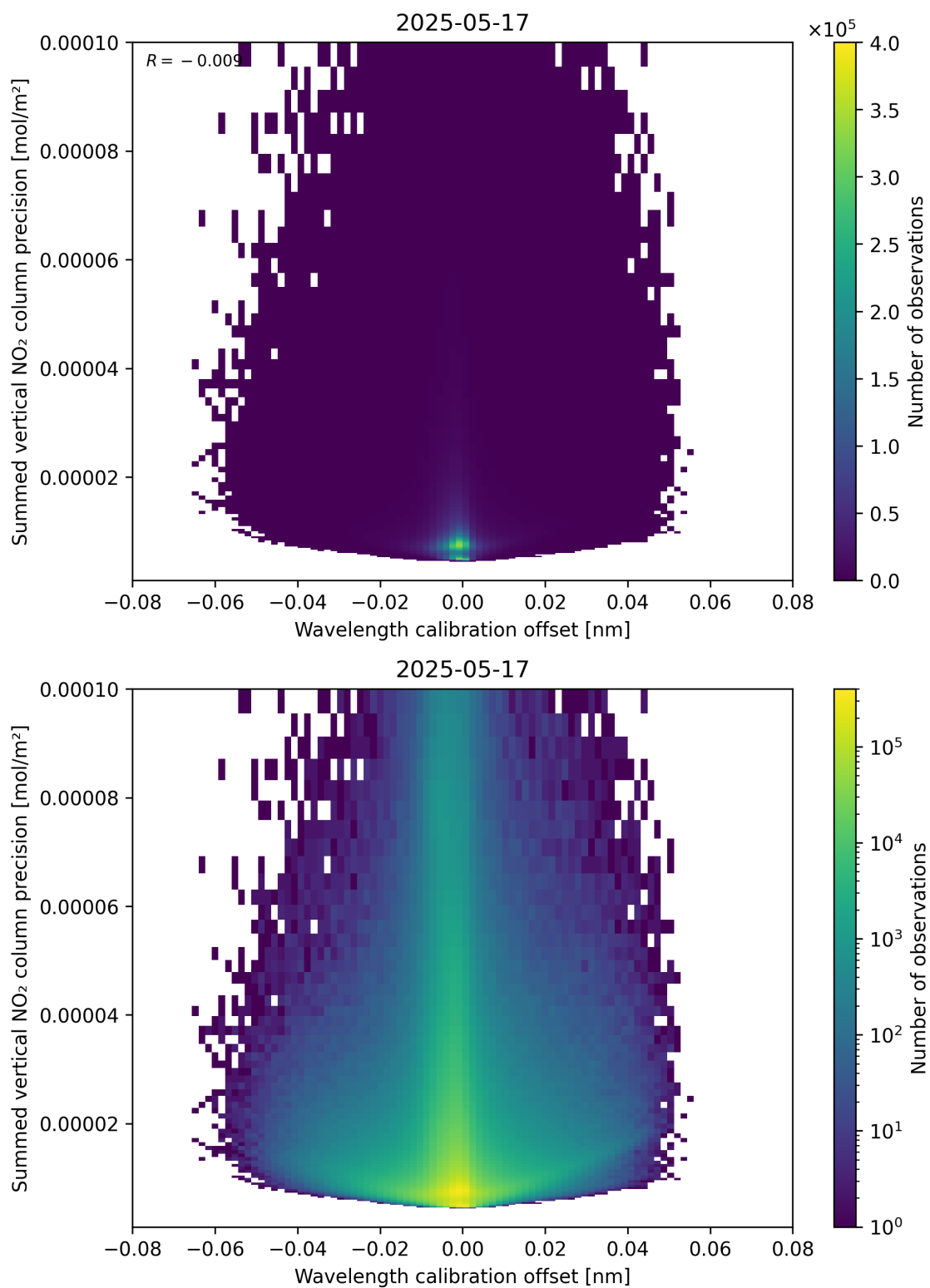
Figure 178: Scatter density plot of “Wavelength calibration offset” against “Summed vertical NO 2 column precision” for 2025-05-16 to 2025-05-18.
