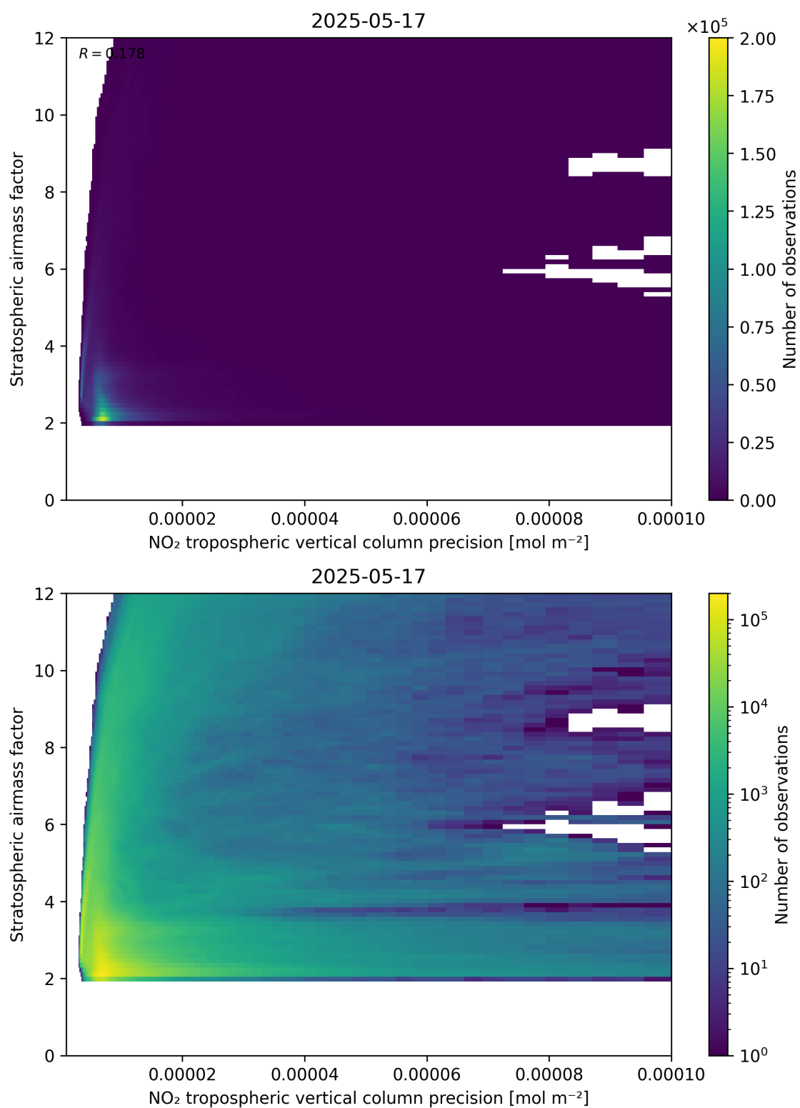
Figure 131: Scatter density plot of “NO 2 tropospheric vertical column precision” against “Stratospheric airmass factor” for 2025-05-16 to 2025-05-18.
