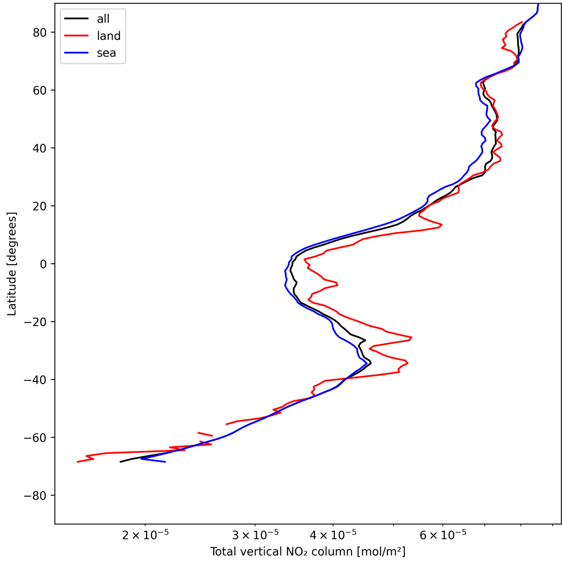
Figure 21: Zonal average of “Total vertical NO 2 column” for 2025-05-16 to 2025-05-18.
