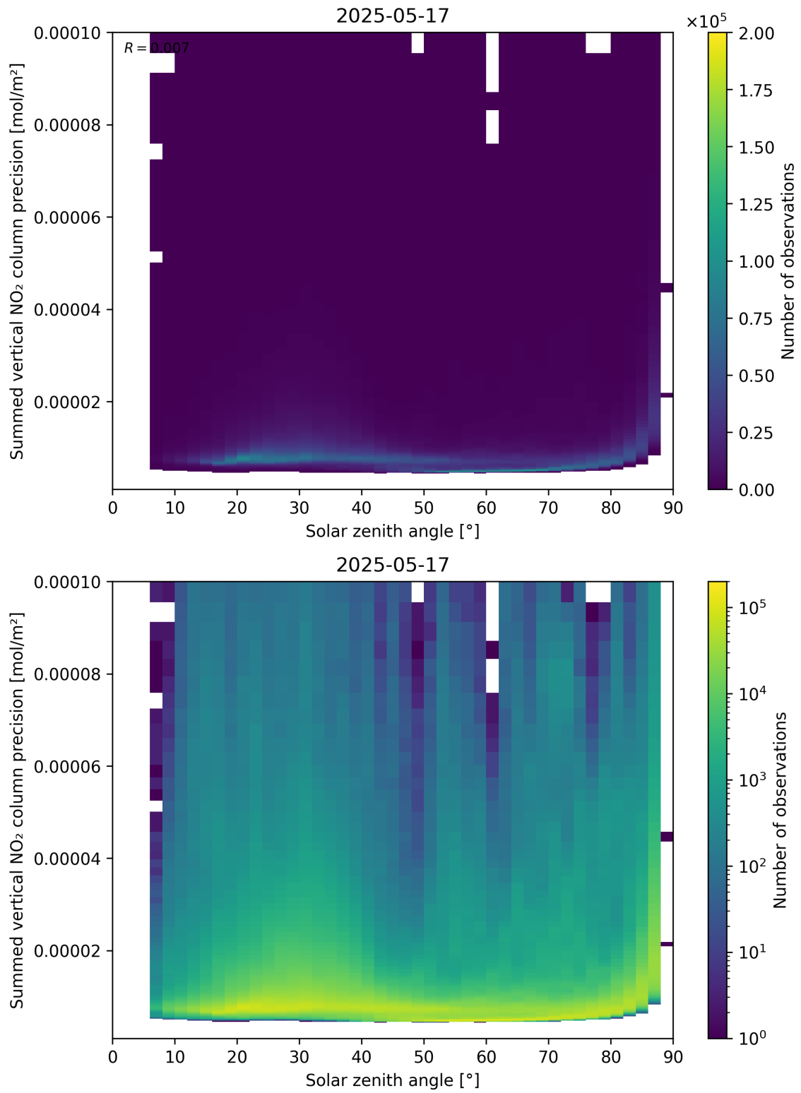
Figure 152: Scatter density plot of “Solar zenith angle” against “Summed vertical NO 2 column precision” for 2025-05-16 to 2025-05-18.
