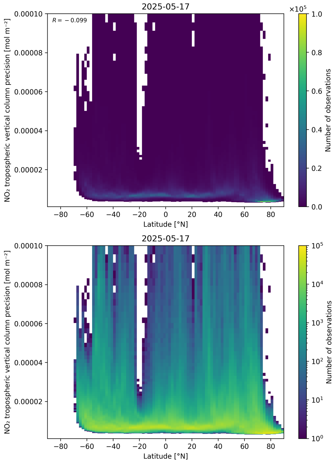
Figure 93: Scatter density plot of “Latitude” against “NO 2 tropospheric vertical column precision” for 2025-05-16 to 2025-05-18.
