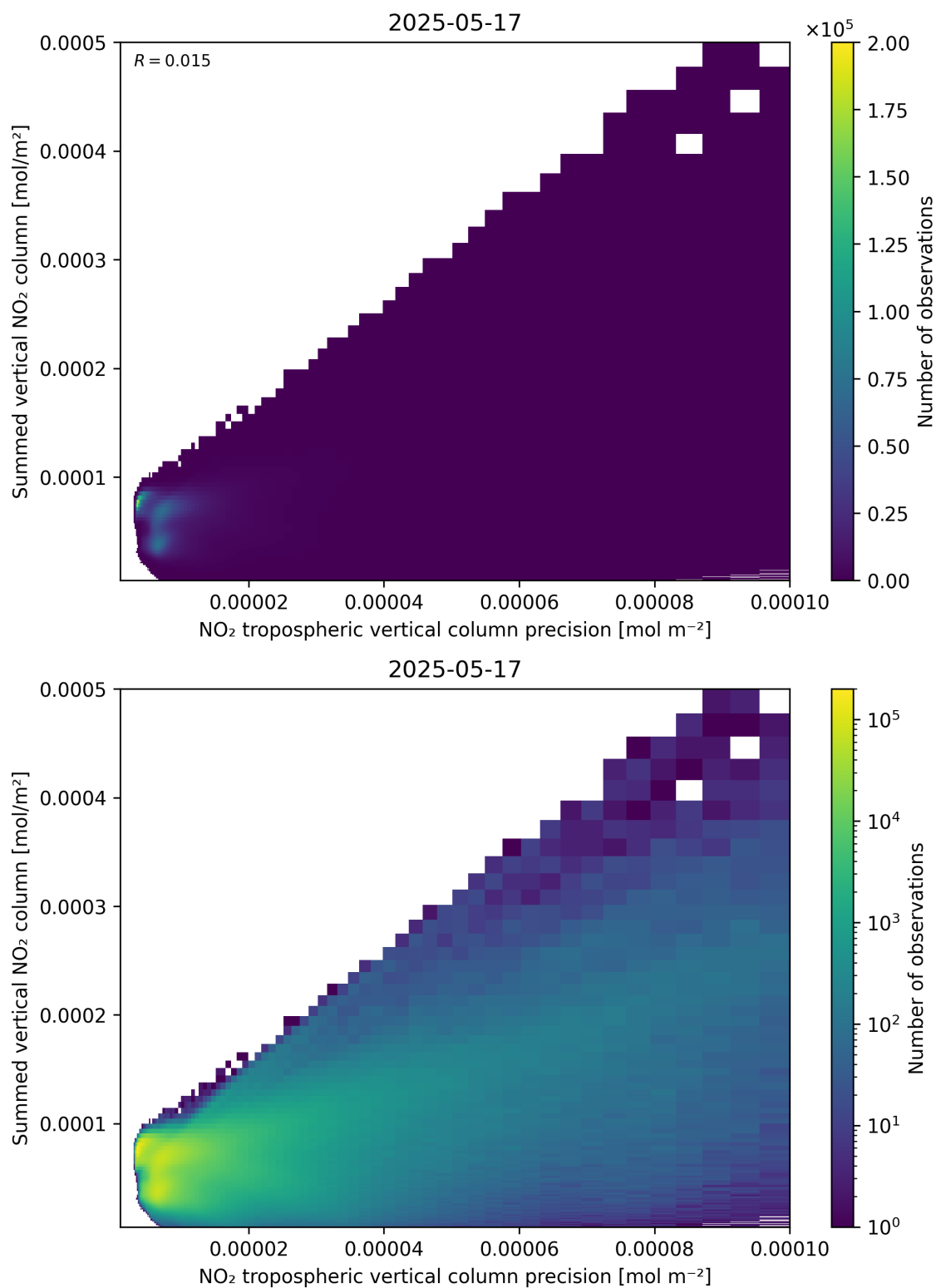
Figure 136: Scatter density plot of “NO 2 tropospheric vertical column precision” against “Summed vertical NO 2 column” for 2025-05-16 to 2025-05-18.
