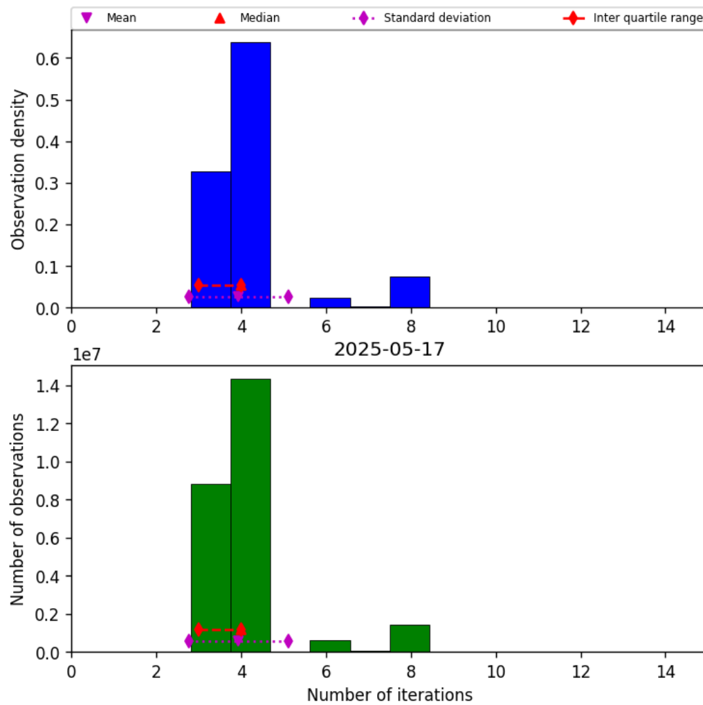
Figure 34: Histogram of “Number of iterations” for 2025-05-16 to 2025-05-18
