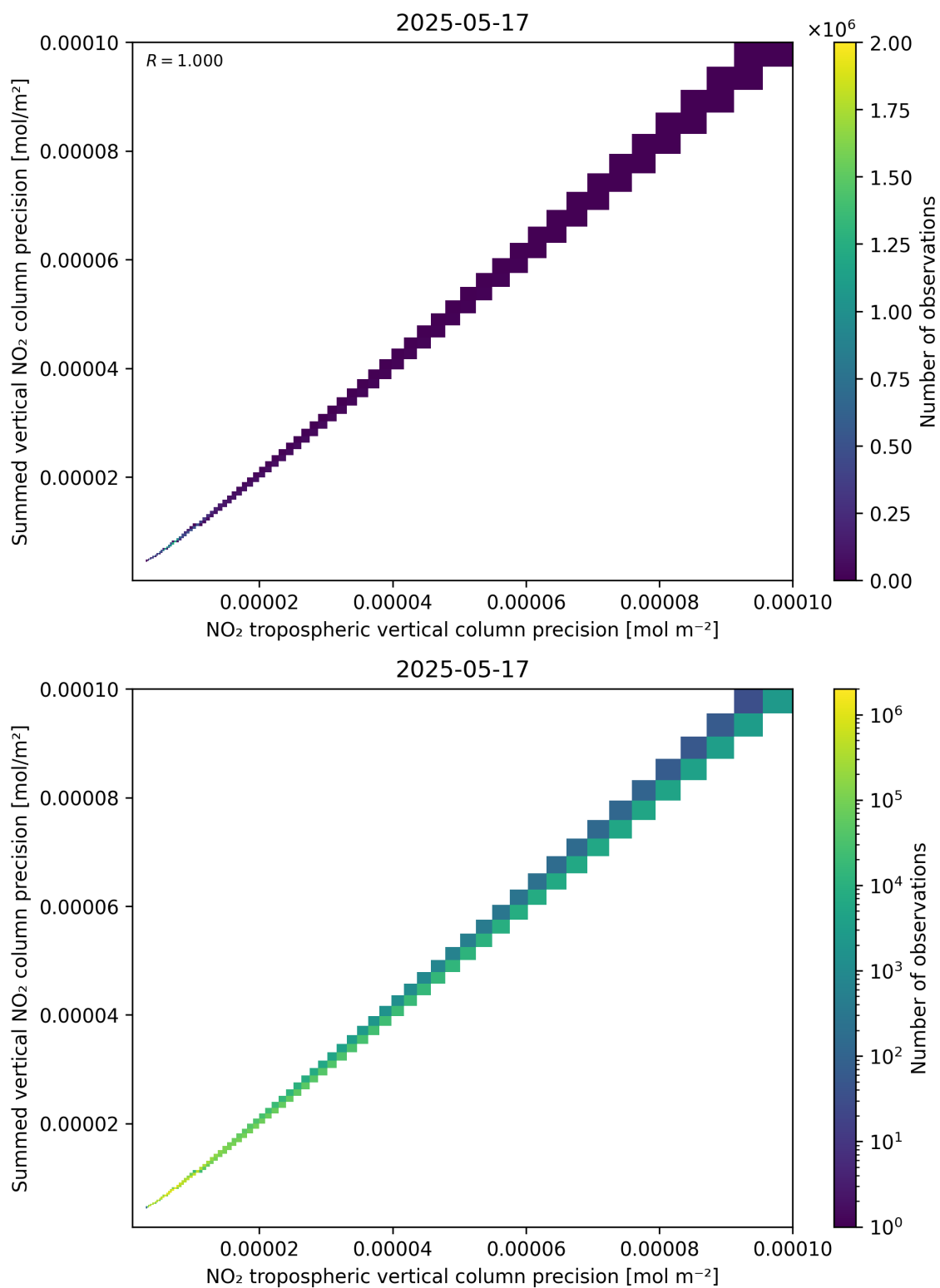
Figure 137: Scatter density plot of “NO 2 tropospheric vertical column precision” against “Summed vertical NO 2 column precision” for 2025-05-16 to 2025-05-18.
