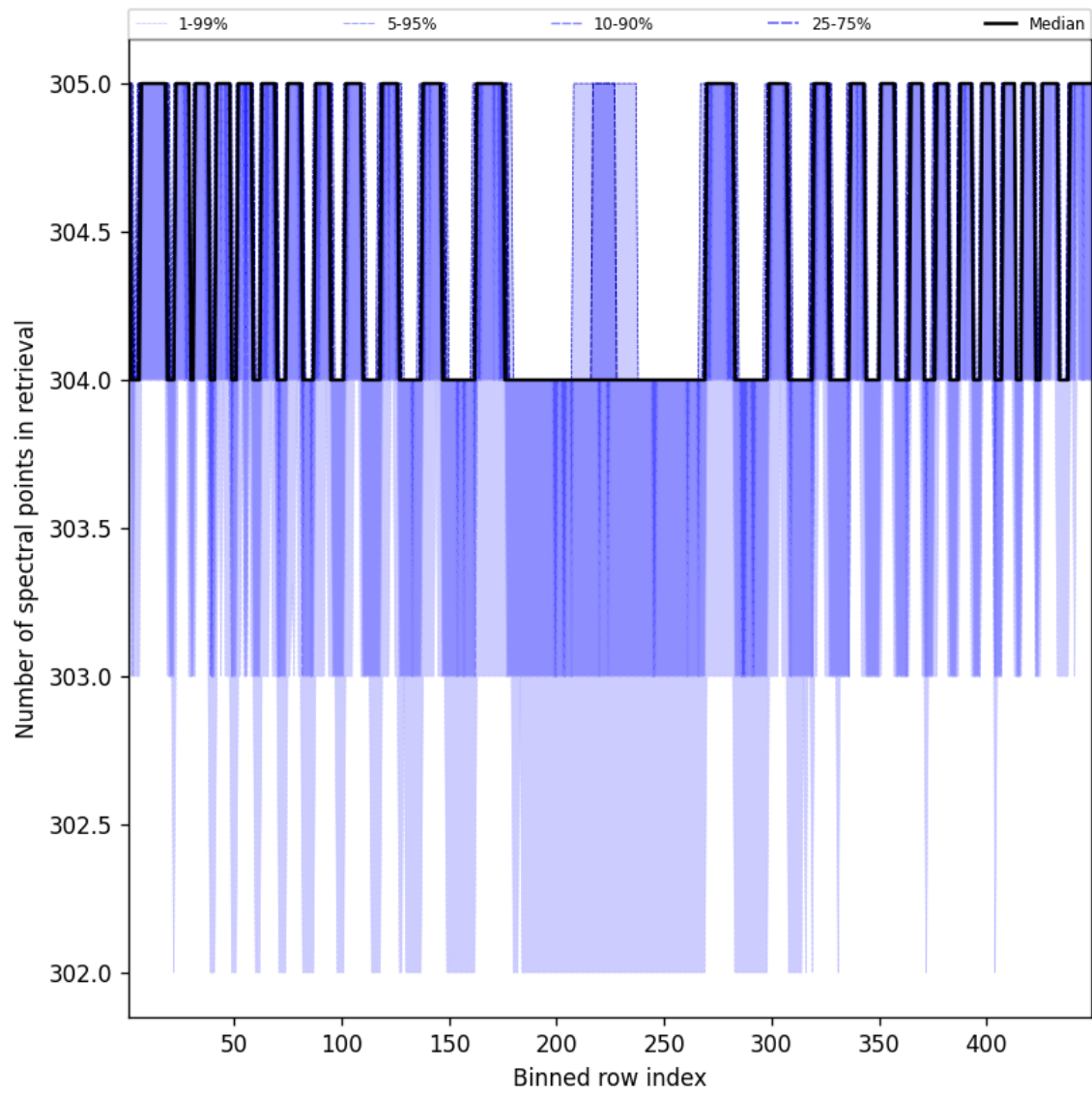
Figure 50: Along track statistics of “Number of spectral points in retrieval” for 2025-05-16 to 2025-05-18
