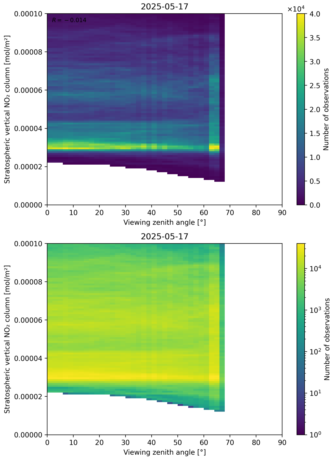
Figure 164: Scatter density plot of “Viewing zenith angle” against “Stratospheric vertical NO 2 column” for 2025-05-16 to 2025-05-18.
