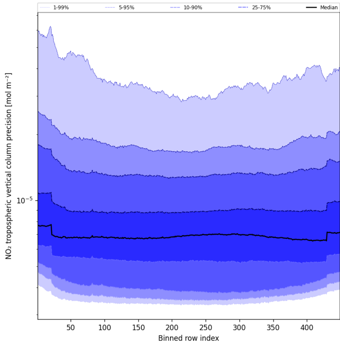
Figure 47: Along track statistics of “NO 2 tropospheric vertical column precision” for 2025-05-16 to 2025-05-18
