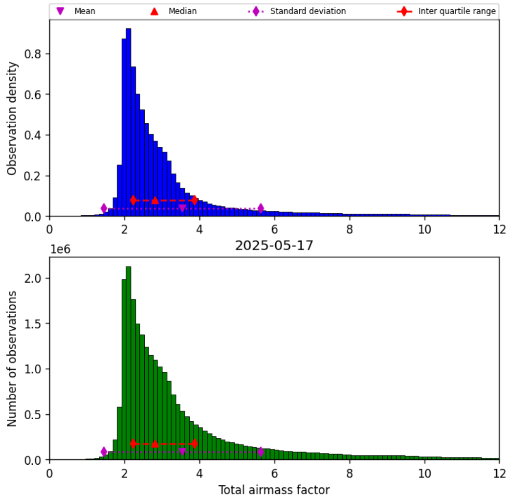
Figure 32: Histogram of “Total airmass factor” for 2025-05-16 to 2025-05-18
