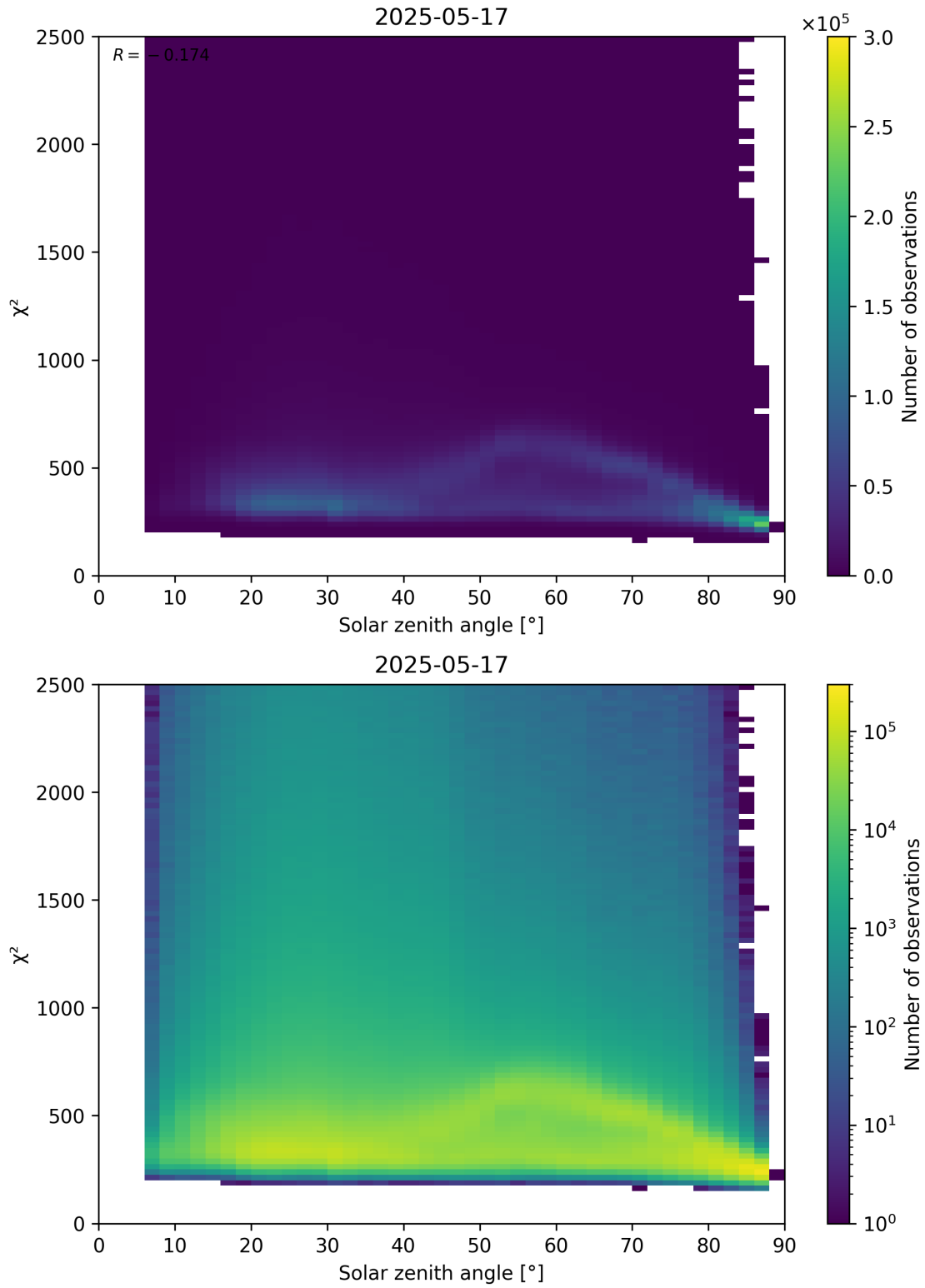
Figure 148: Scatter density plot of “Solar zenith angle” against “ \chi^2 ” for 2025-05-16 to 2025-05-18.
