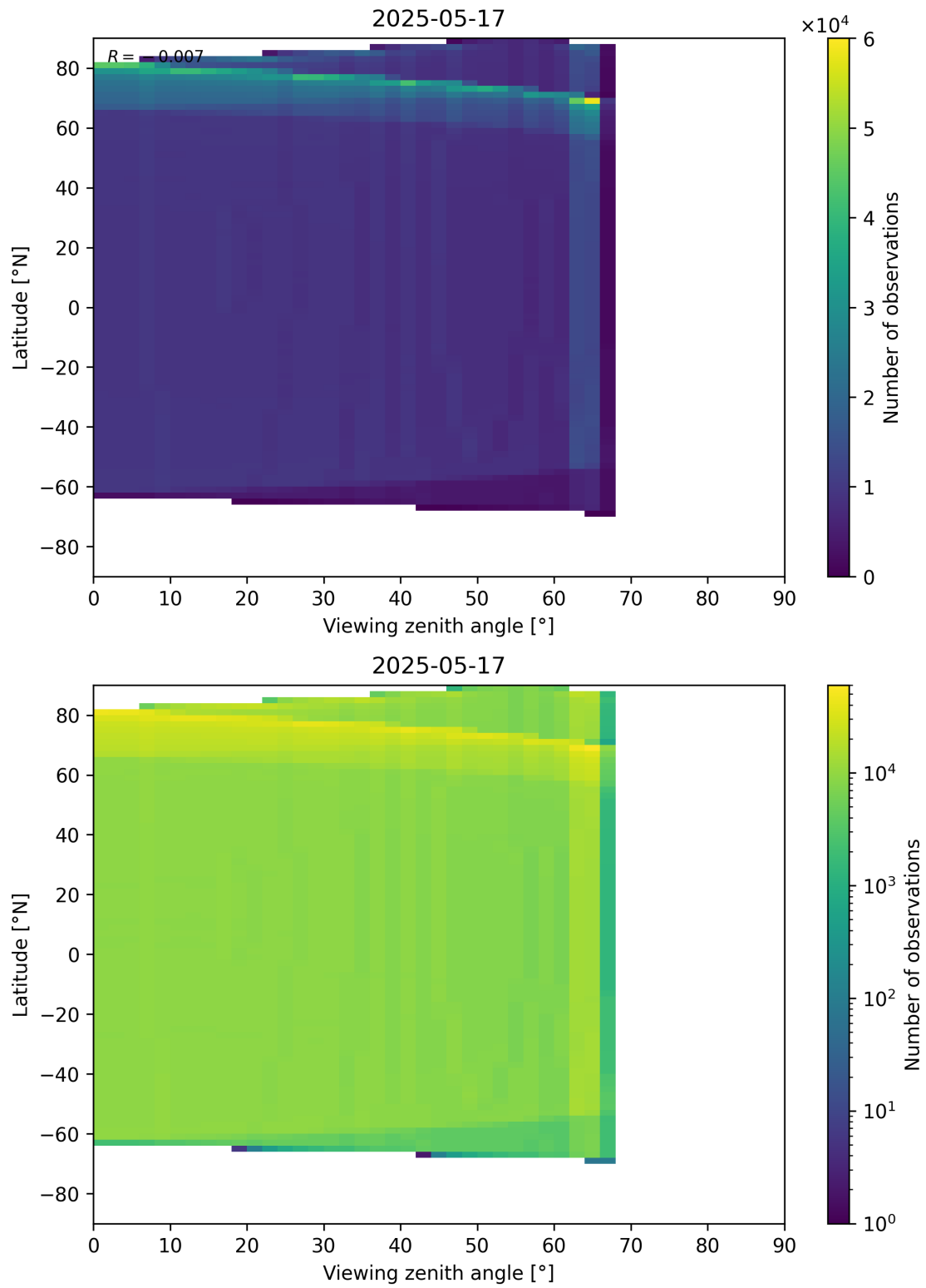
Figure 163: Scatter density plot of “Viewing zenith angle” against “Latitude” for 2025-05-16 to 2025-05-18.
