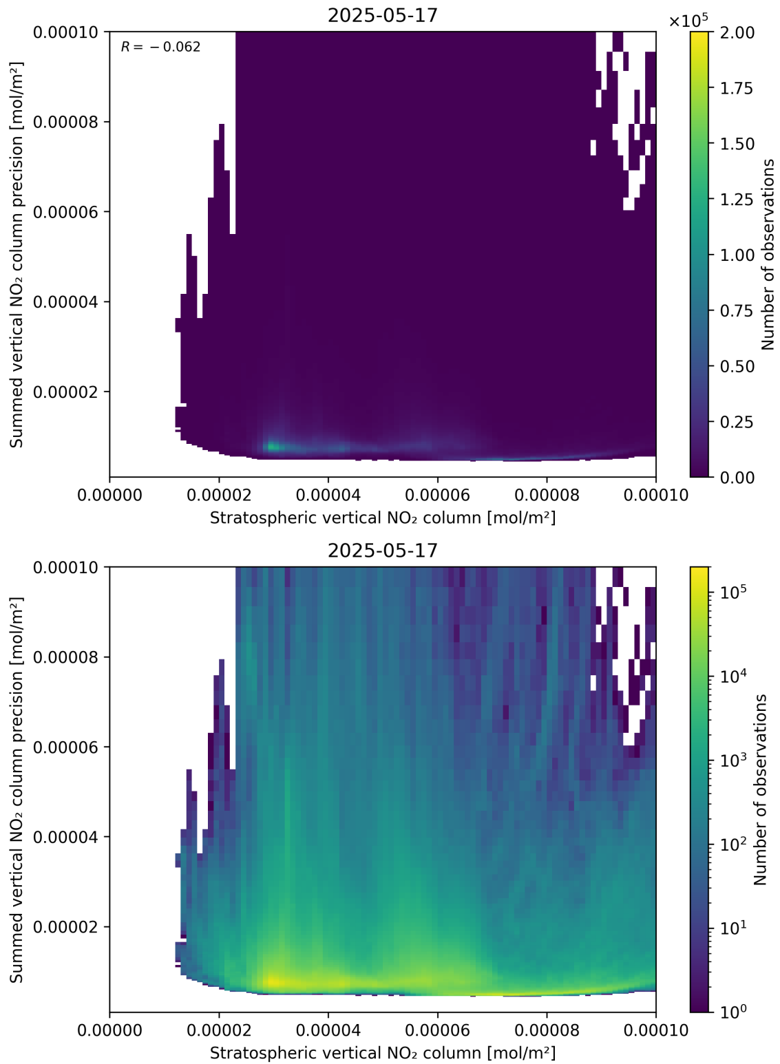
Figure 99: Scatter density plot of “Stratospheric vertical NO 2 column” against “Summed vertical NO 2 column precision” for 2025-05-16 to 2025-05-18.
