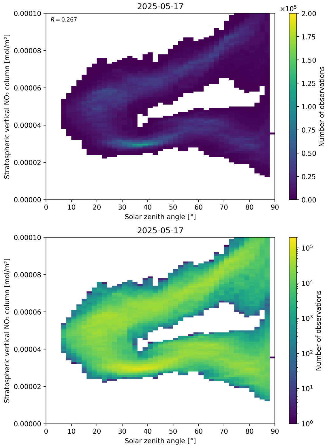
Figure 150: Scatter density plot of “Solar zenith angle” against “Stratospheric vertical \text{NO}_2 column” for 2025-05-16 to 2025-05-18.
