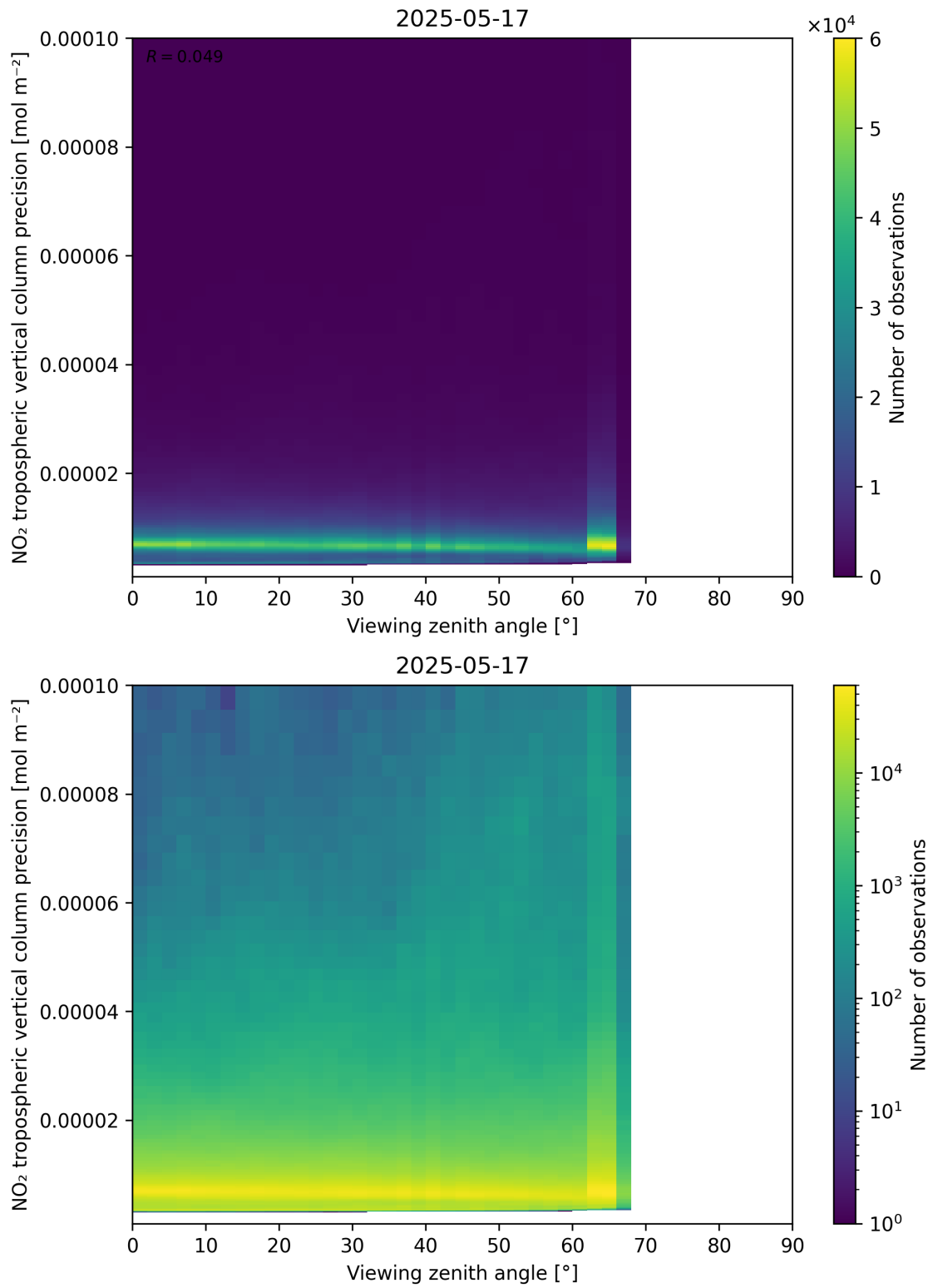
Figure 170: Scatter density plot of “Viewing zenith angle” against “NO 2 tropospheric vertical column precision” for 2025-05-16 to 2025-05-18.
