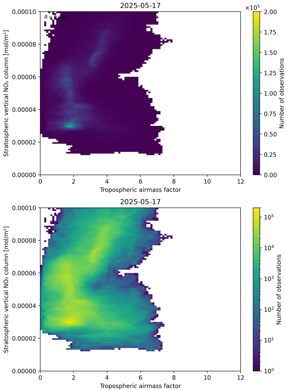
Figure 74: Scatter density plot of “Tropospheric airmass factor” against “Stratospheric vertical NO 2 column” for 2025-05-16 to 2025-05-18.
