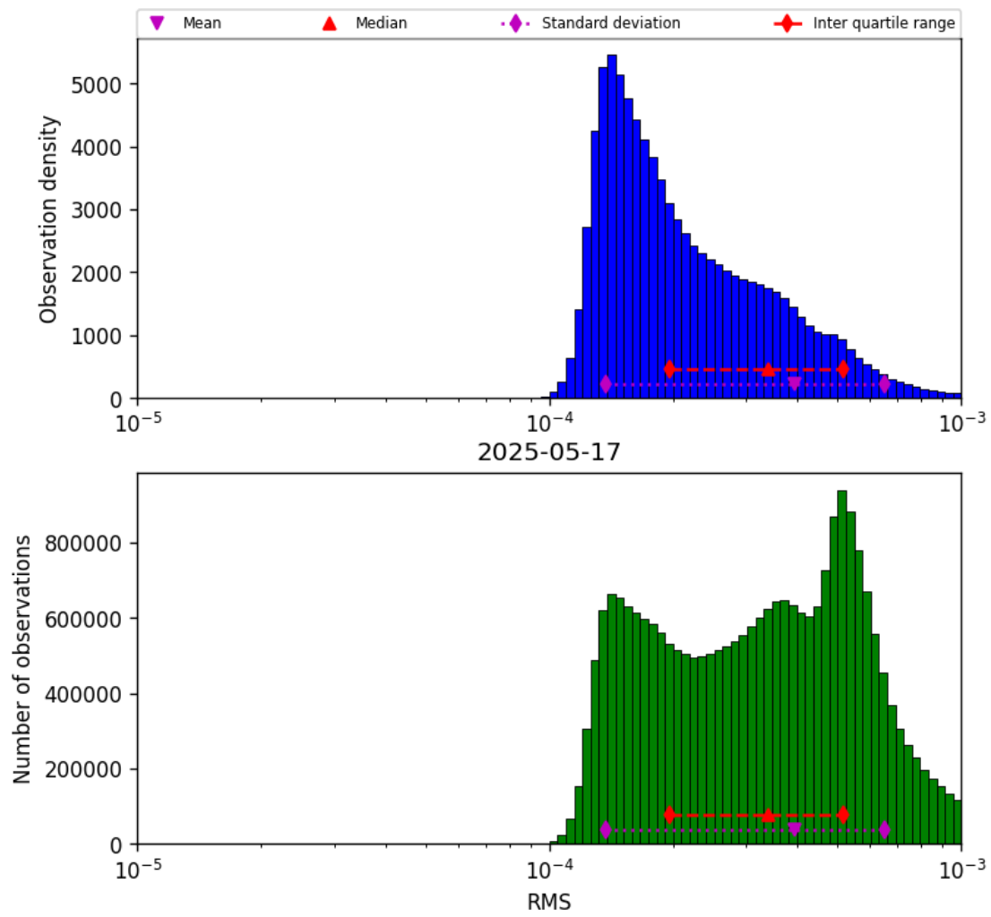
Figure 43: Histogram of “RMS” for 2025-05-16 to 2025-05-18
