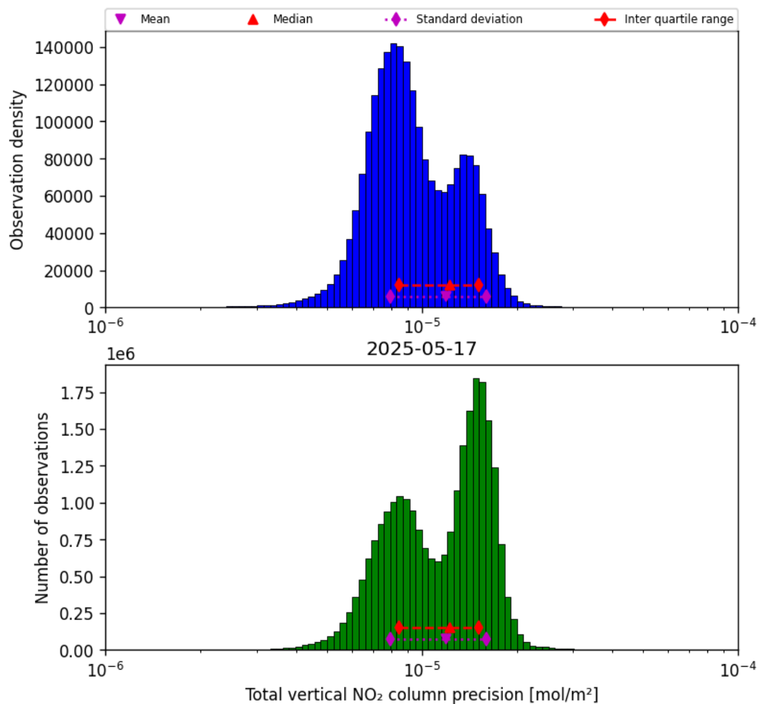
Figure 39: Histogram of “Total vertical NO 2 column precision” for 2025-05-16 to 2025-05-18
