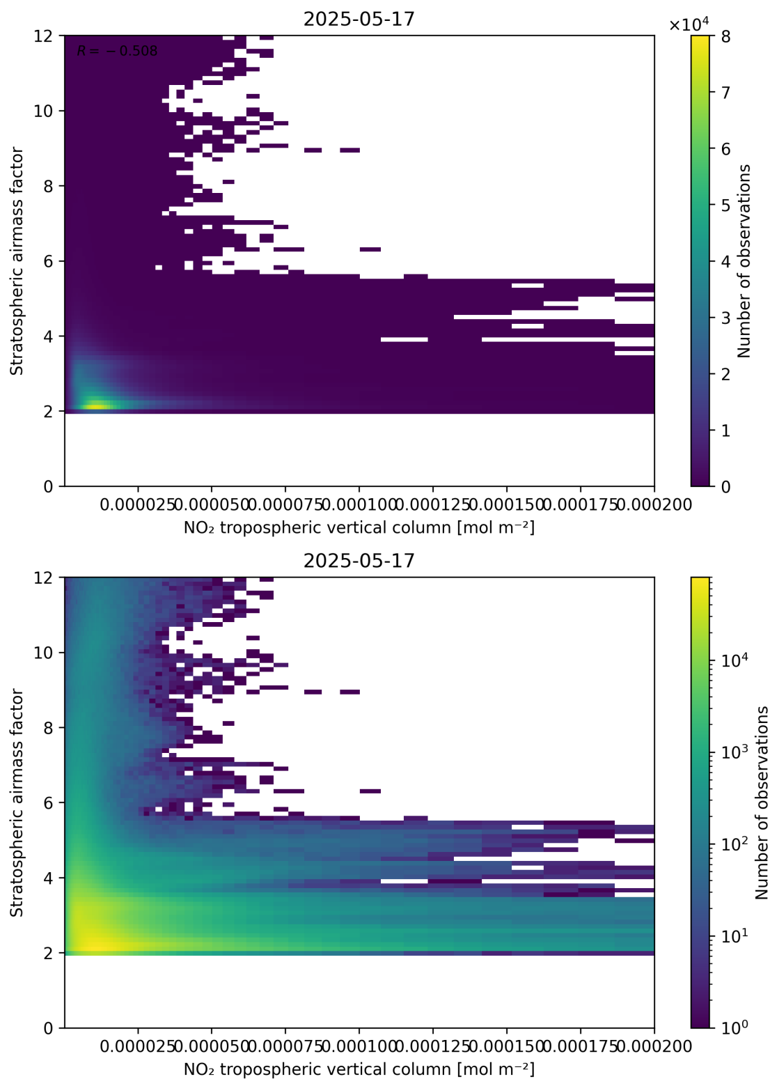
Figure 121: Scatter density plot of “NO 2 tropospheric vertical column” against “Stratospheric air mass factor” for 2025-05-16 to 2025-05-18.
