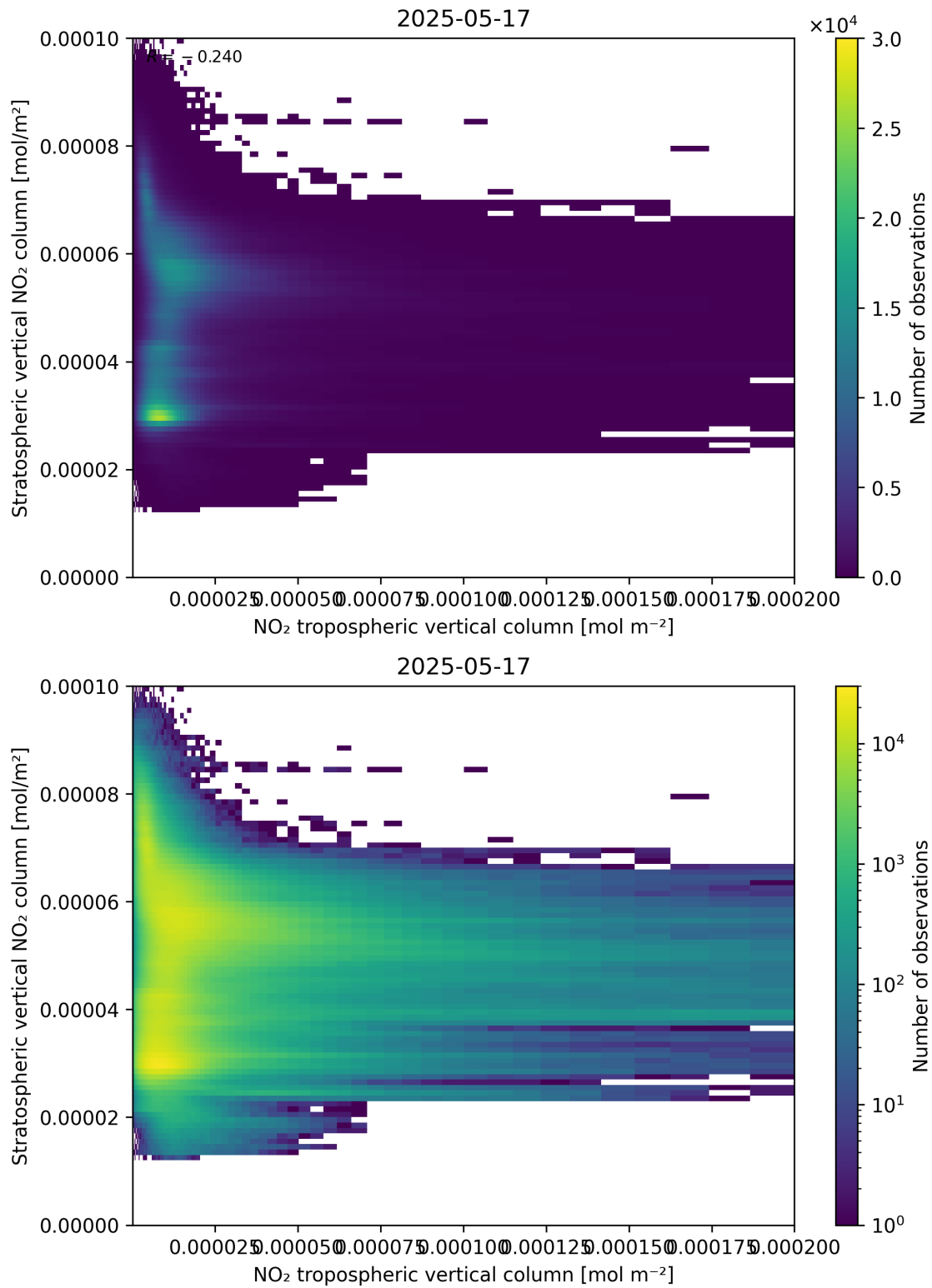
Figure 125: Scatter density plot of “NO 2 tropospheric vertical column” against “Stratospheric vertical NO 2 column” for 2025-05-16 to 2025-05-18.
