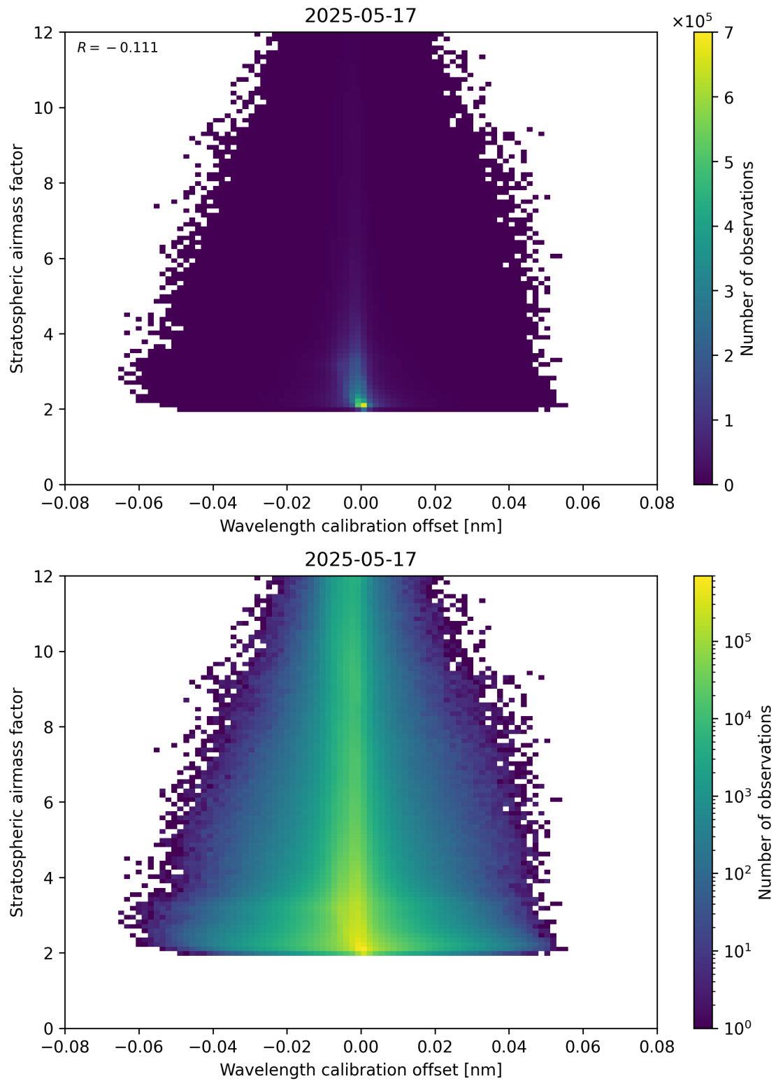
Figure 174: Scatter density plot of “Wavelength calibration offset” against “Stratospheric airmass factor” for 2025-05-16 to 2025-05-18.
