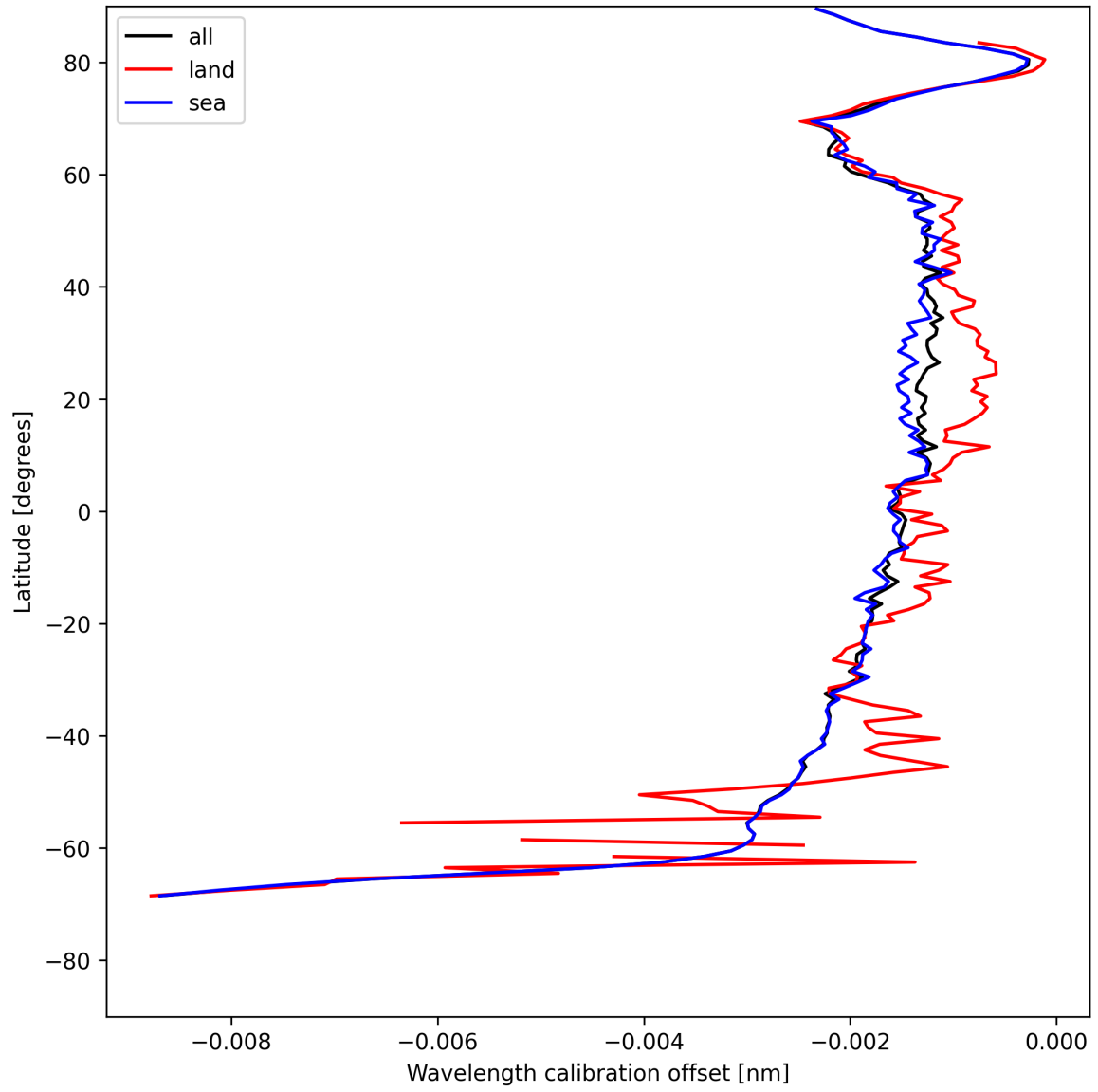
Figure 18: Zonal average of “Wavelength calibration offset” for 2025-05-16 to 2025-05-18.
