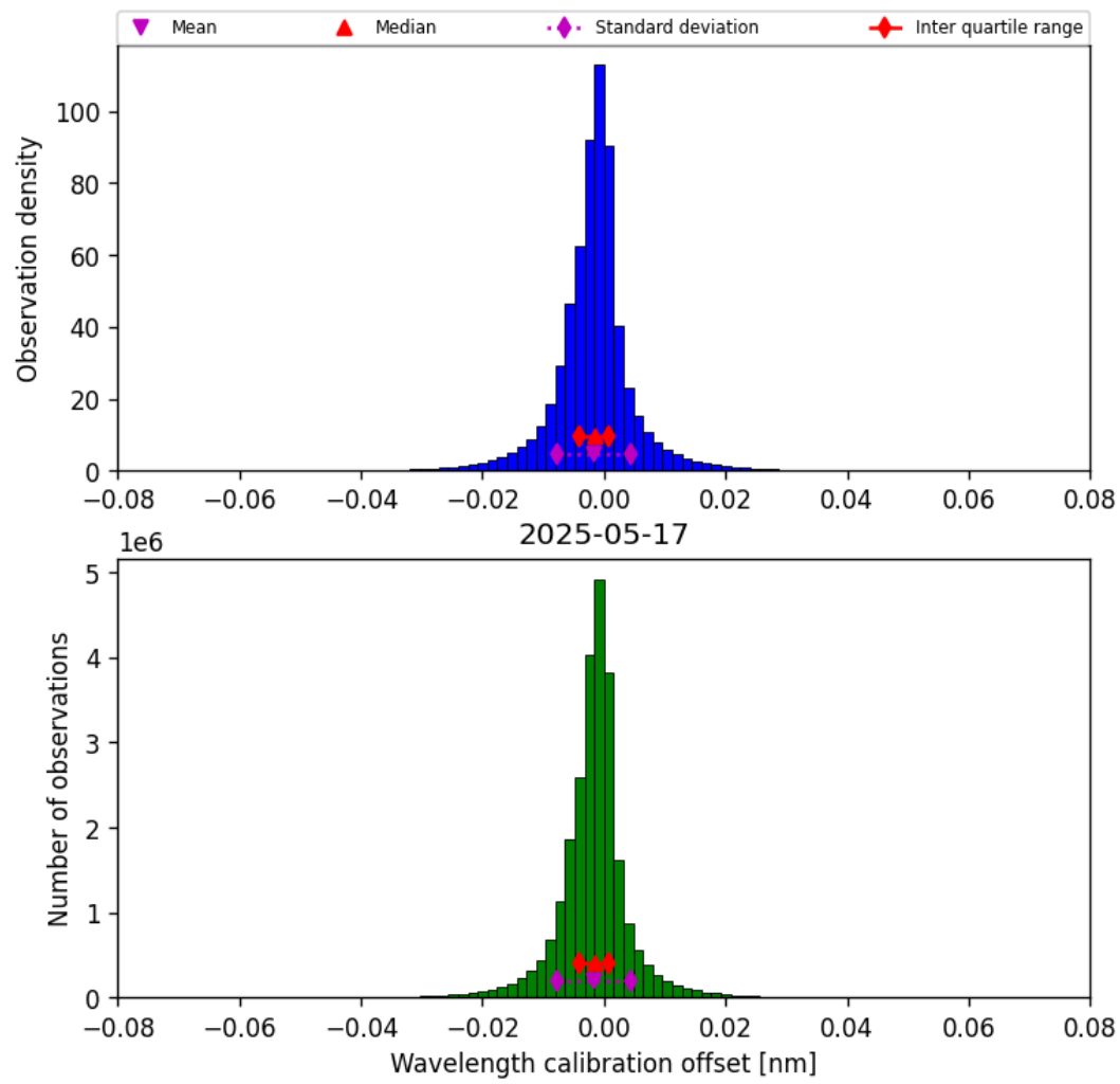
Figure 35: Histogram of “Wavelength calibration offset” for 2025-05-16 to 2025-05-18
