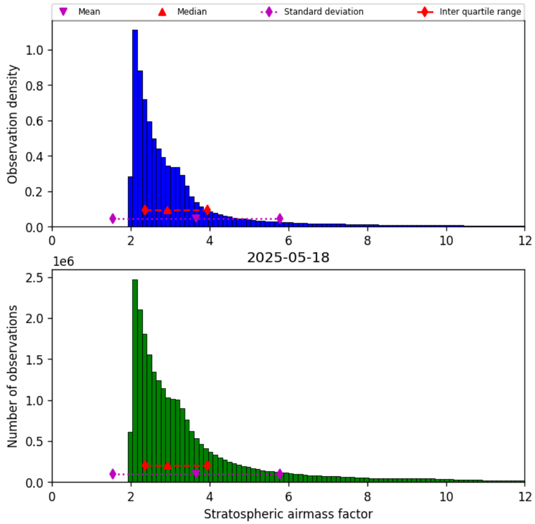
Figure 44: Histogram of “Stratospheric airmass factor” for 2025-05-17 to 2025-05-19
