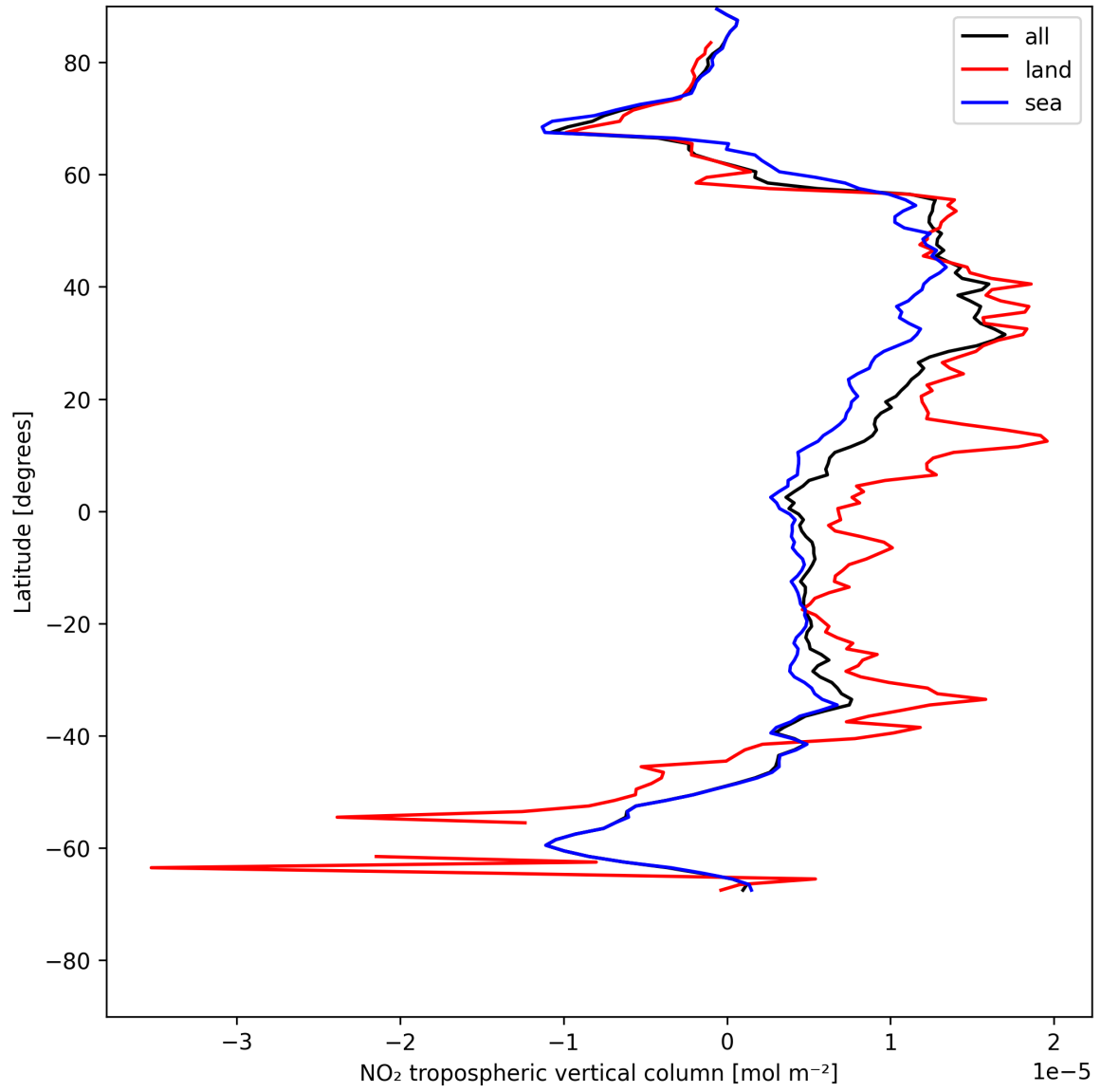
Figure 12: Zonal average of “NO 2 tropospheric vertical column” for 2025-05-17 to 2025-05-19.
