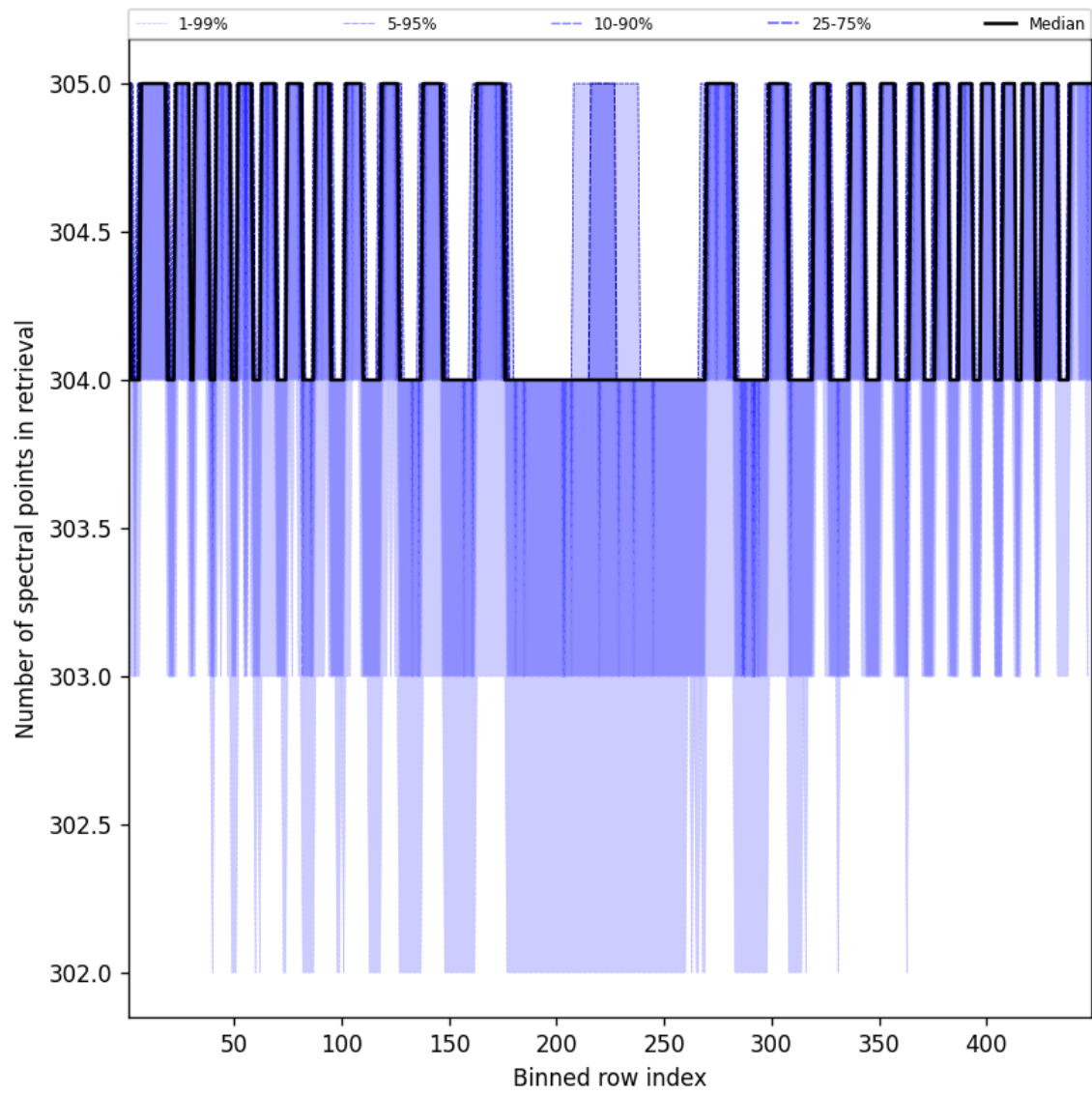
Figure 50: Along track statistics of “Number of spectral points in retrieval” for 2025-05-17 to 2025-05-19
