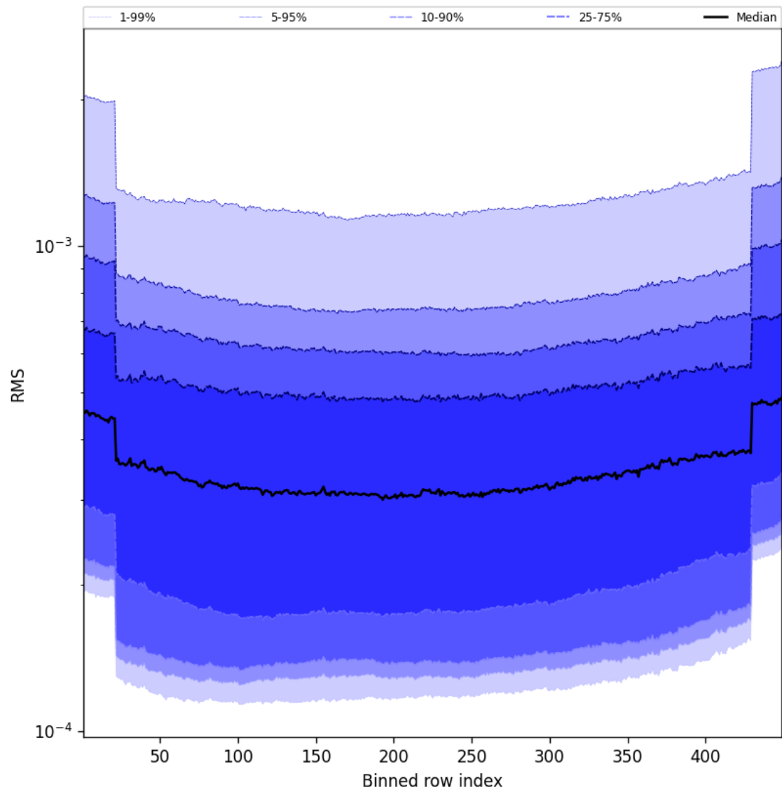
Figure 60: Along track statistics of “RMS” for 2025-05-17 to 2025-05-19
