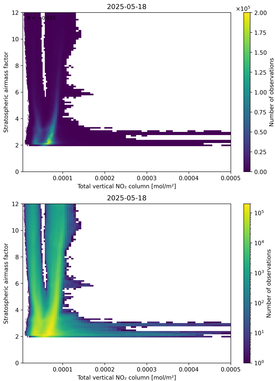
Figure 110: Scatter density plot of “Total vertical NO 2 column” against “Stratospheric airmass factor” for 2025-05-17 to 2025-05-19.
