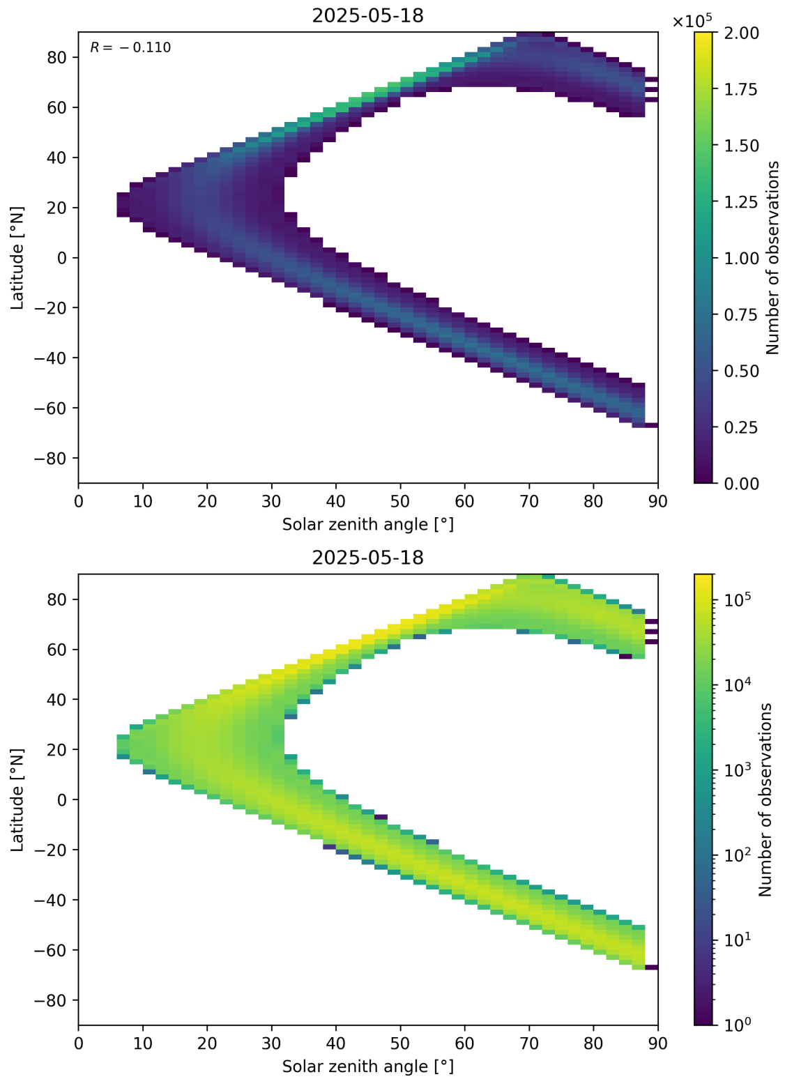
Figure 149: Scatter density plot of “Solar zenith angle” against “Latitude” for 2025-05-17 to 2025-05-19.
