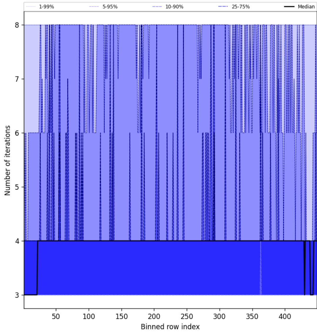
Figure 51: Along track statistics of “Number of iterations” for 2025-05-17 to 2025-05-19
