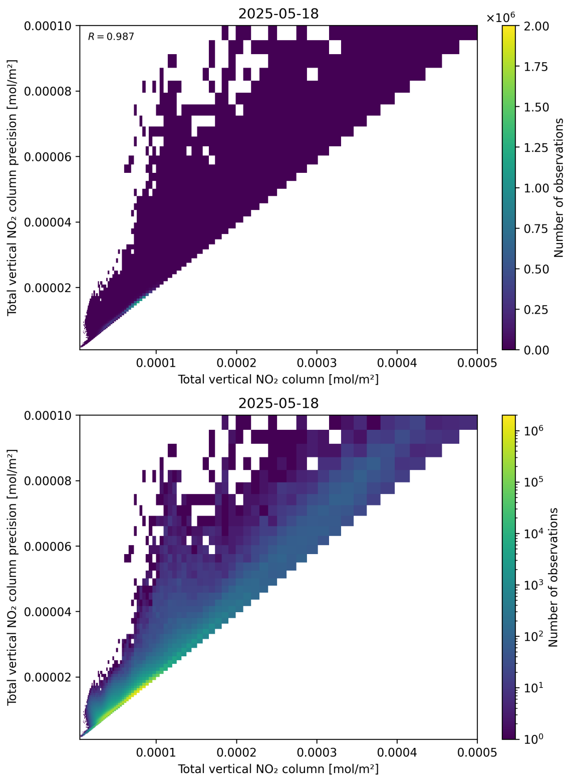
Figure 114: Scatter density plot of “Total vertical NO 2 column” against “Total vertical NO 2 column precision” for 2025-05-17 to 2025-05-19.
