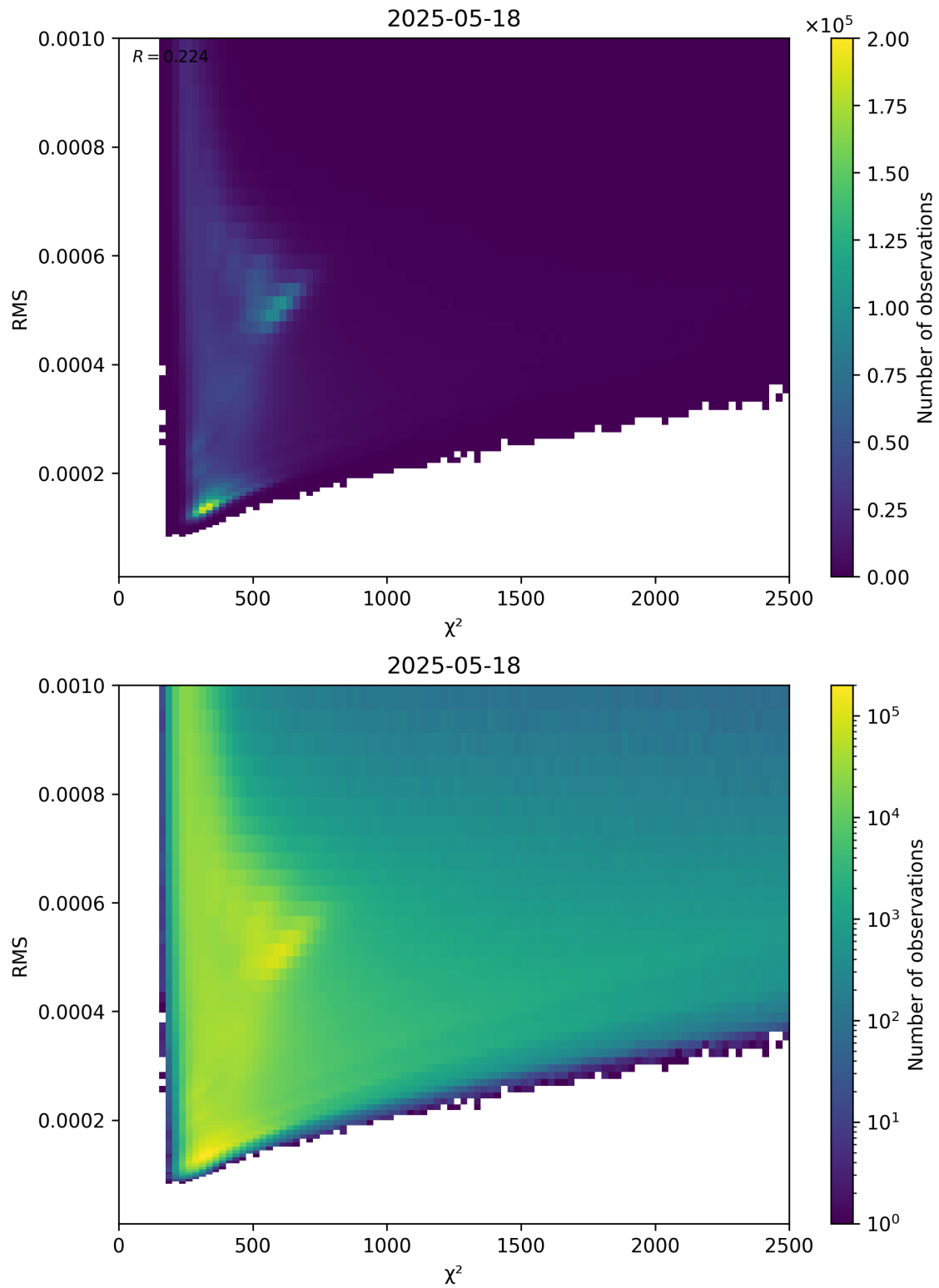
Figure 82: Scatter density plot of “ \chi^2 ” against “RMS” for 2025-05-17 to 2025-05-19.
