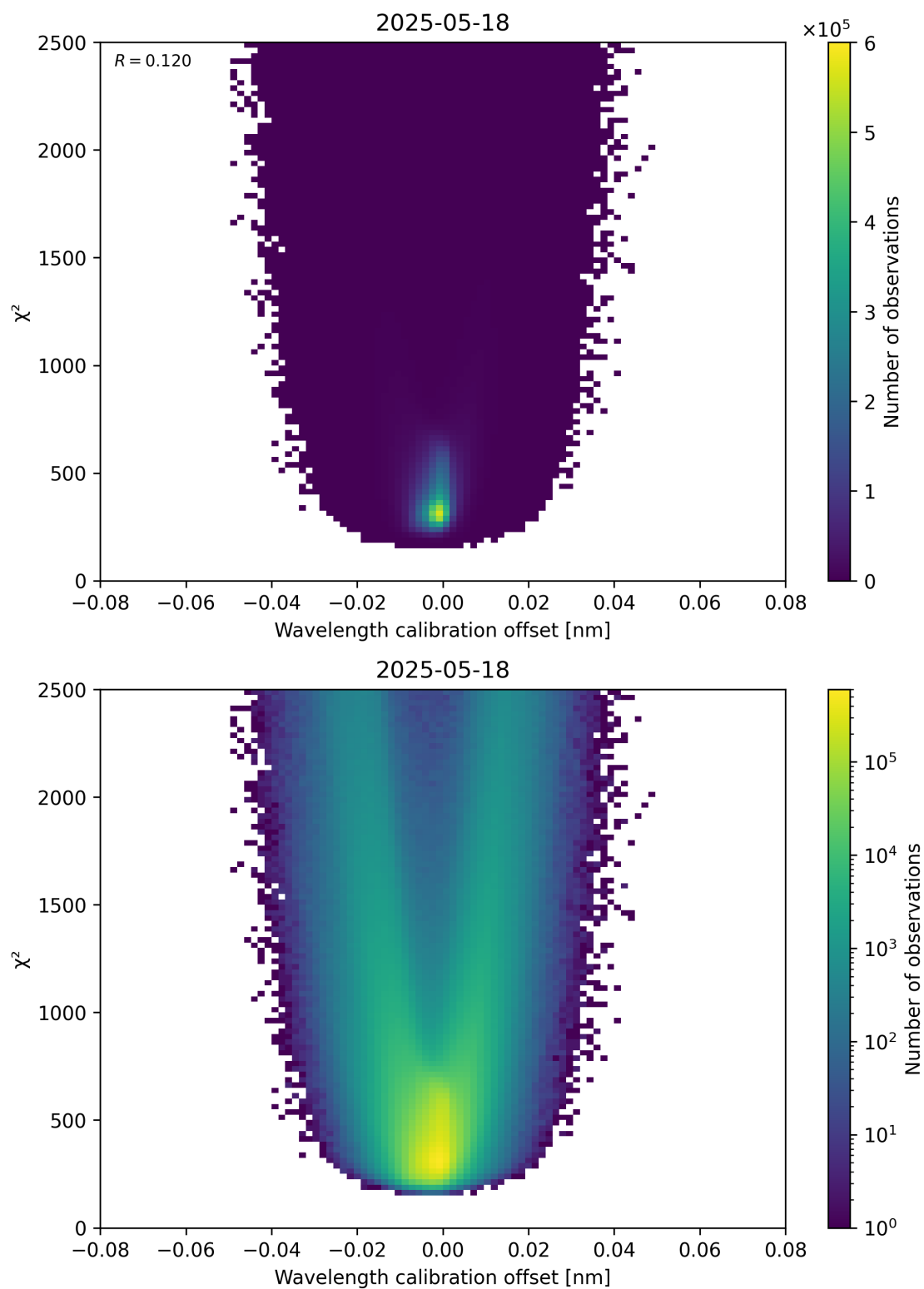
Figure 175: Scatter density plot of “Wavelength calibration offset” against “ \chi^2 ” for 2025-05-17 to 2025-05-19.
