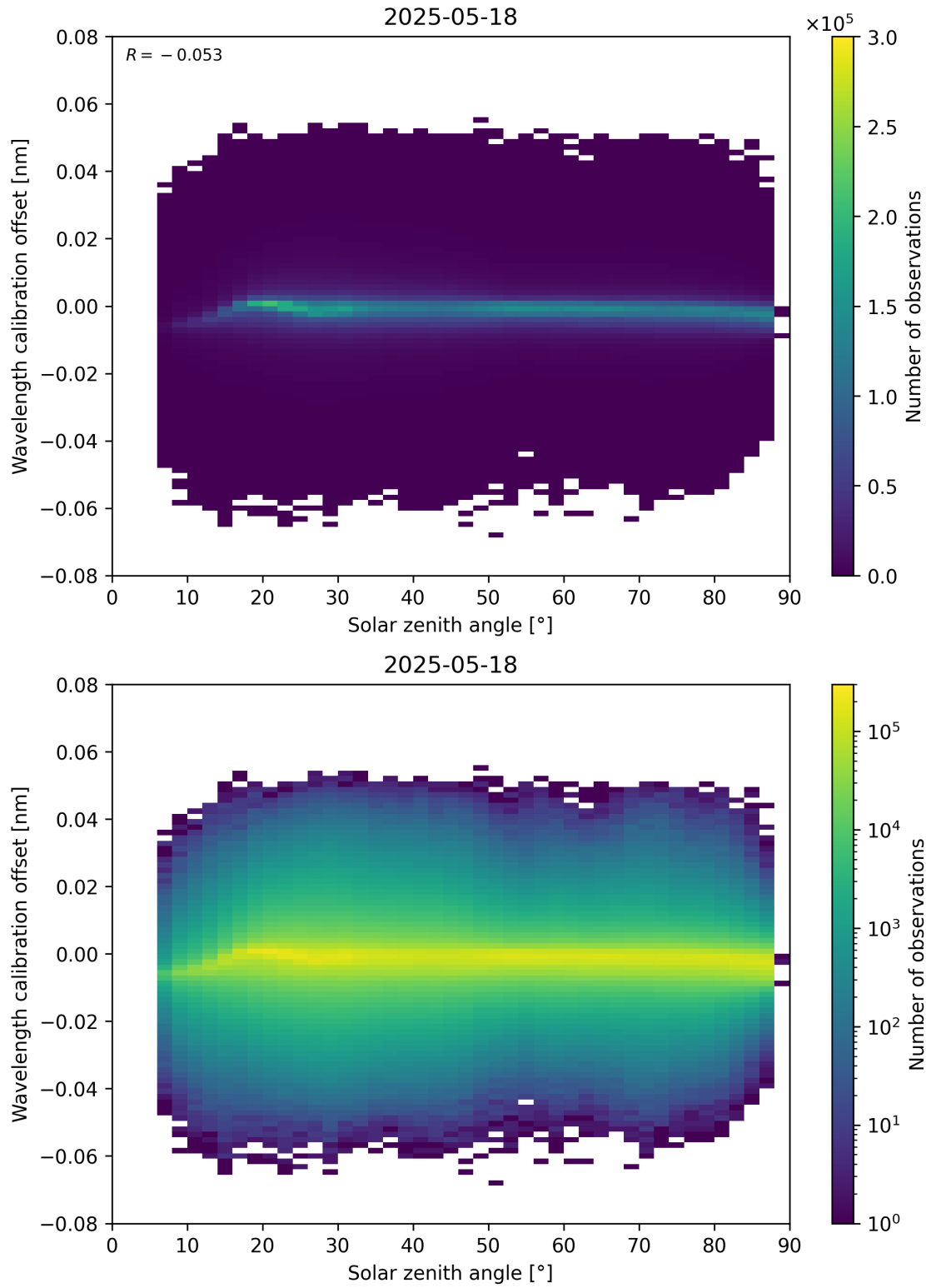
Figure 158: Scatter density plot of “Solar zenith angle” against “Wavelength calibration offset” for 2025-05-17 to 2025-05-19.
