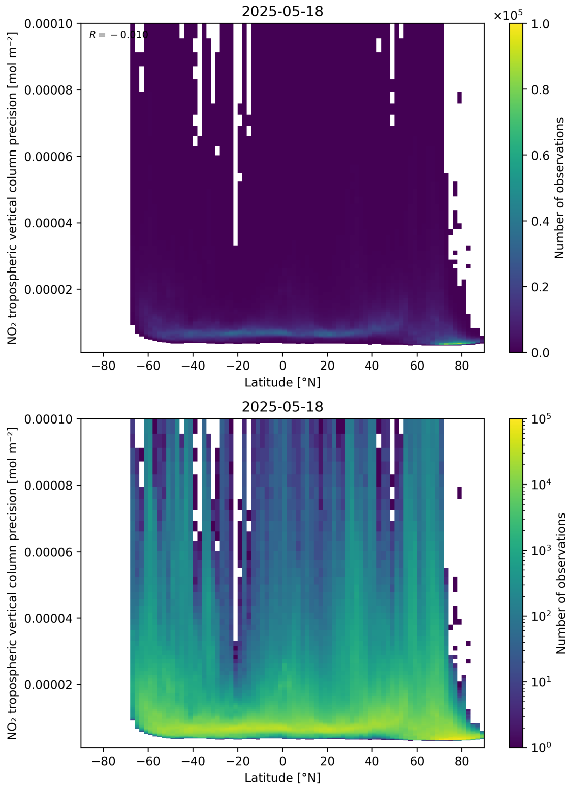
Figure 93: Scatter density plot of “Latitude” against “NO 2 tropospheric vertical column precision” for 2025-05-17 to 2025-05-19.
