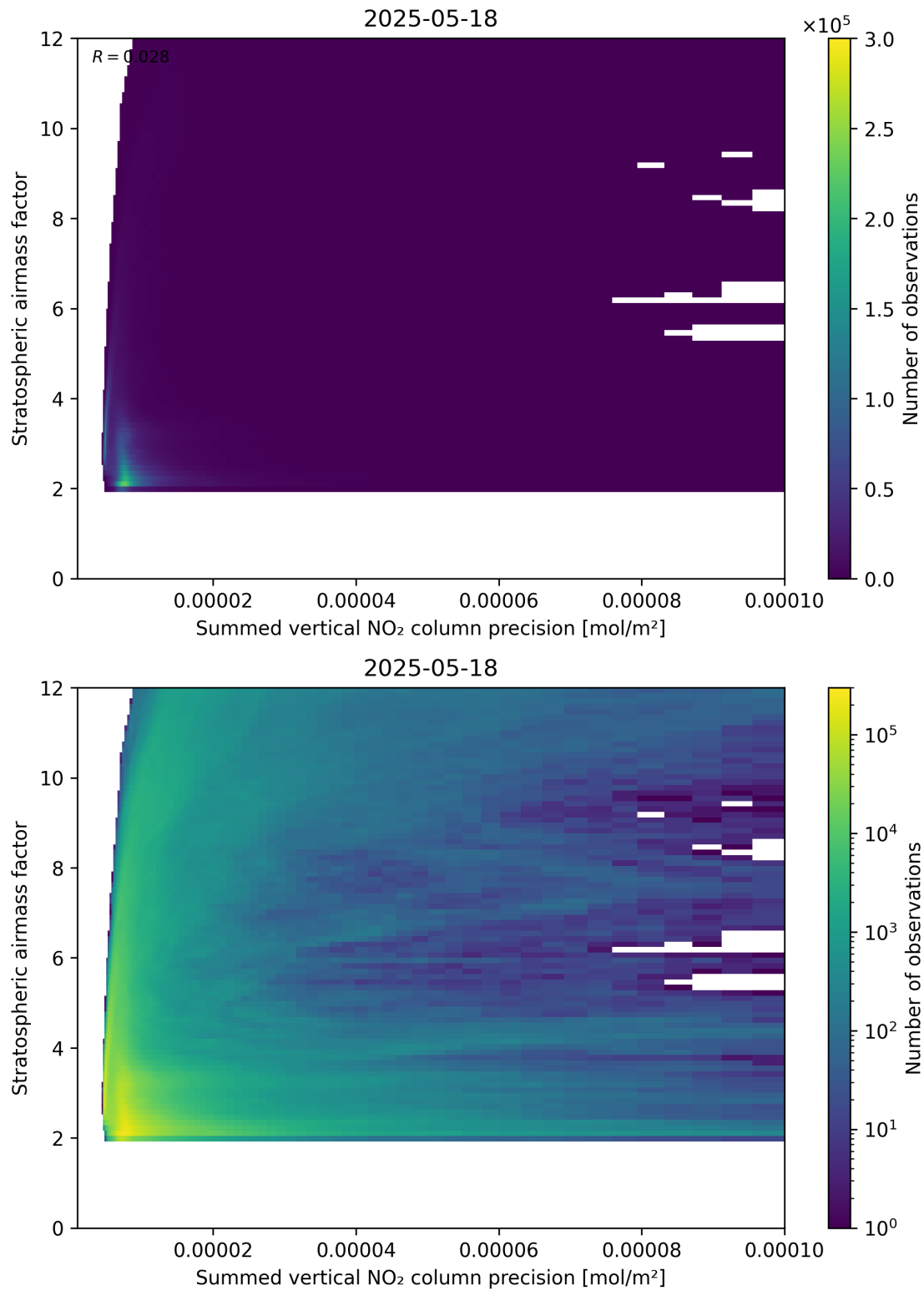
Figure 106: Scatter density plot of “Summed vertical NO 2 column precision” against “Stratospheric airmass factor” for 2025-05-17 to 2025-05-19.
