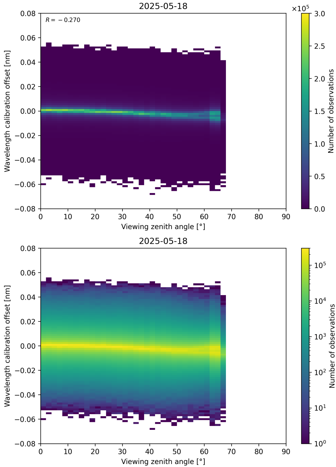
Figure 173: Scatter density plot of “Viewing zenith angle” against “Wavelength calibration offset” for 2025-05-17 to 2025-05-19.
