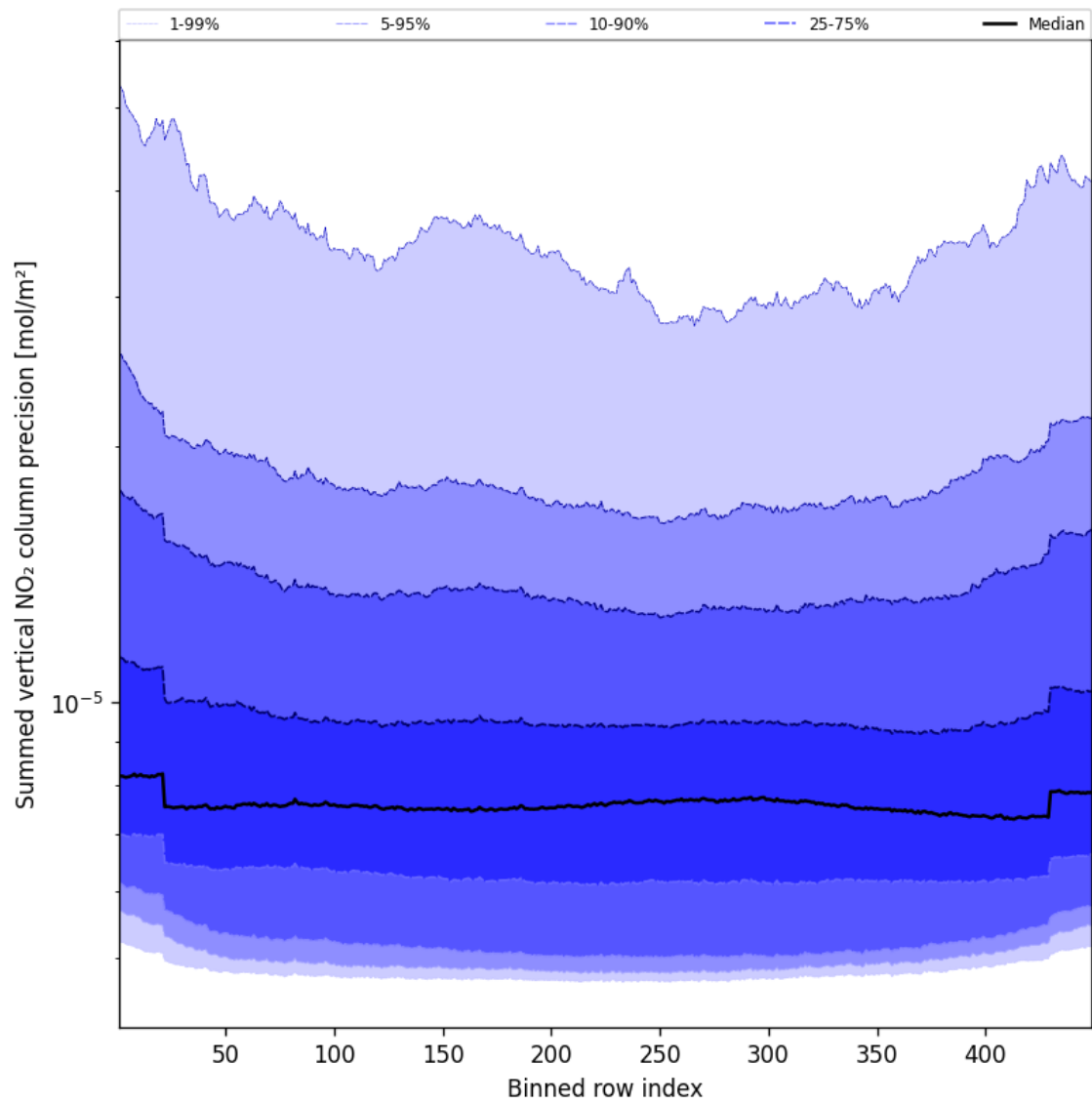
Figure 58: Along track statistics of “Summed vertical NO 2 column precision” for 2025-05-17 to 2025-05-19
