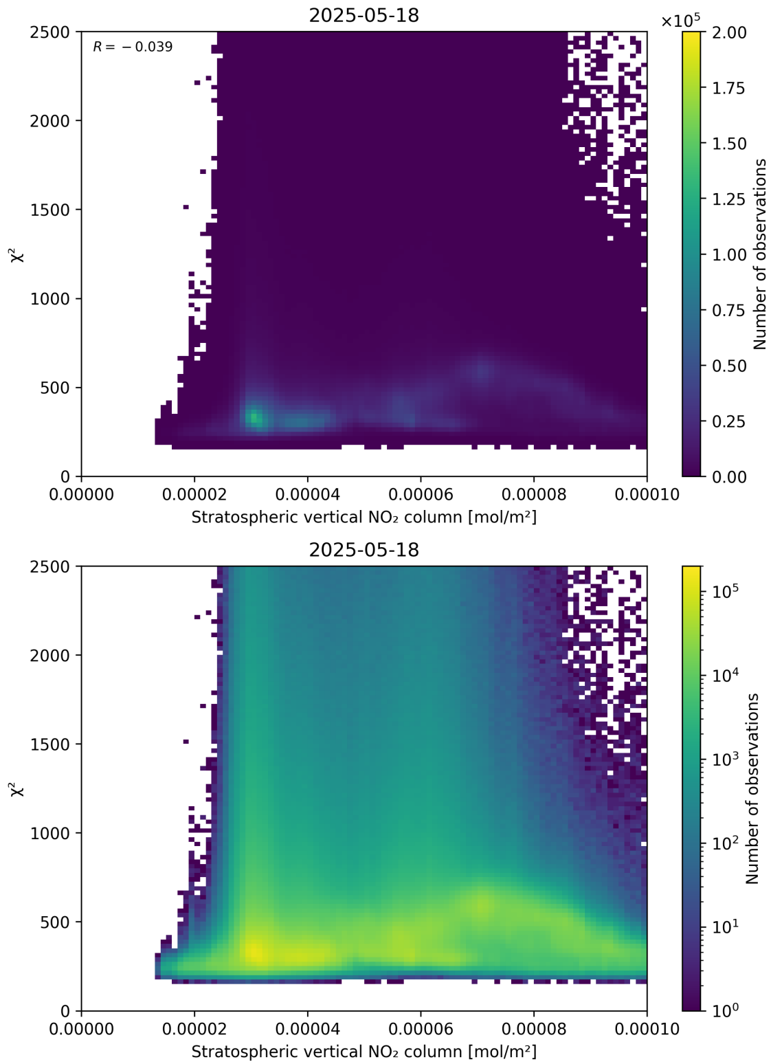
Figure 97: Scatter density plot of “Stratospheric vertical NO 2 column” against “ \chi^2 ” for 2025-05-17 to 2025-05-19.
