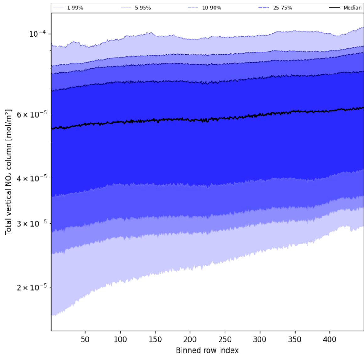
Figure 55: Along track statistics of “Total vertical NO 2 column” for 2025-05-17 to 2025-05-19
