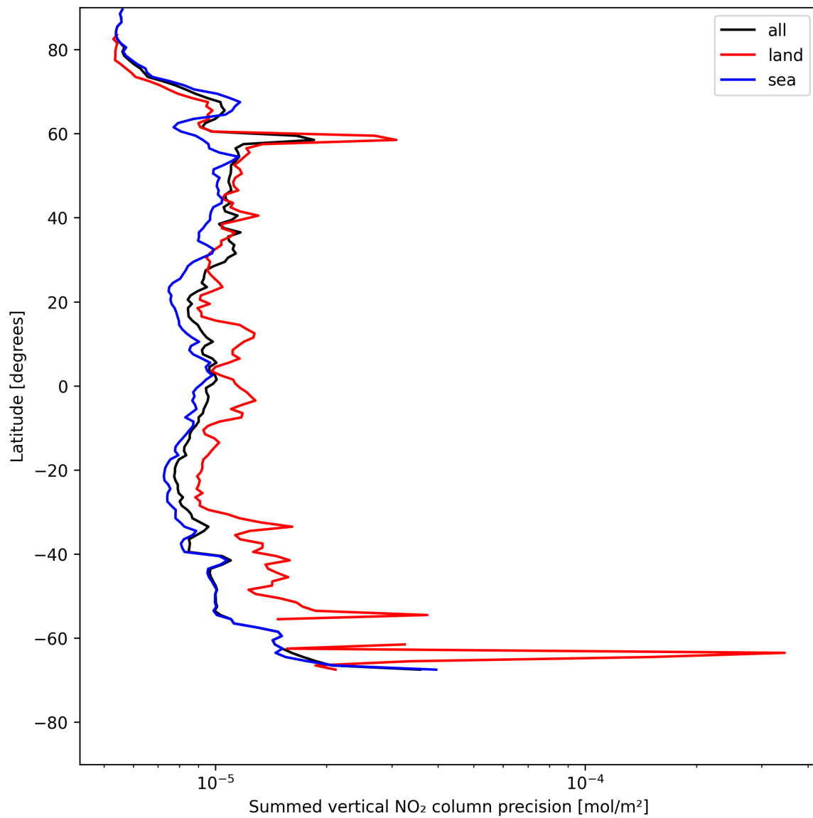
Figure 24: Zonal average of “Summed vertical NO 2 column precision” for 2025-05-17 to 2025-05-19.
