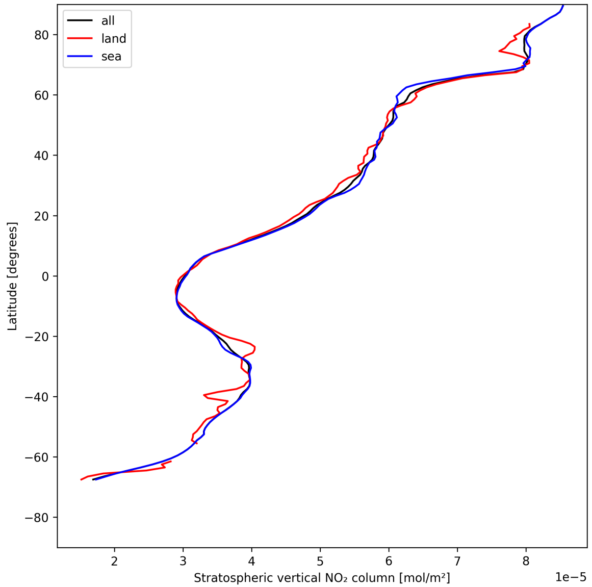
Figure 19: Zonal average of “Stratospheric vertical NO 2 column” for 2025-05-17 to 2025-05-19.
