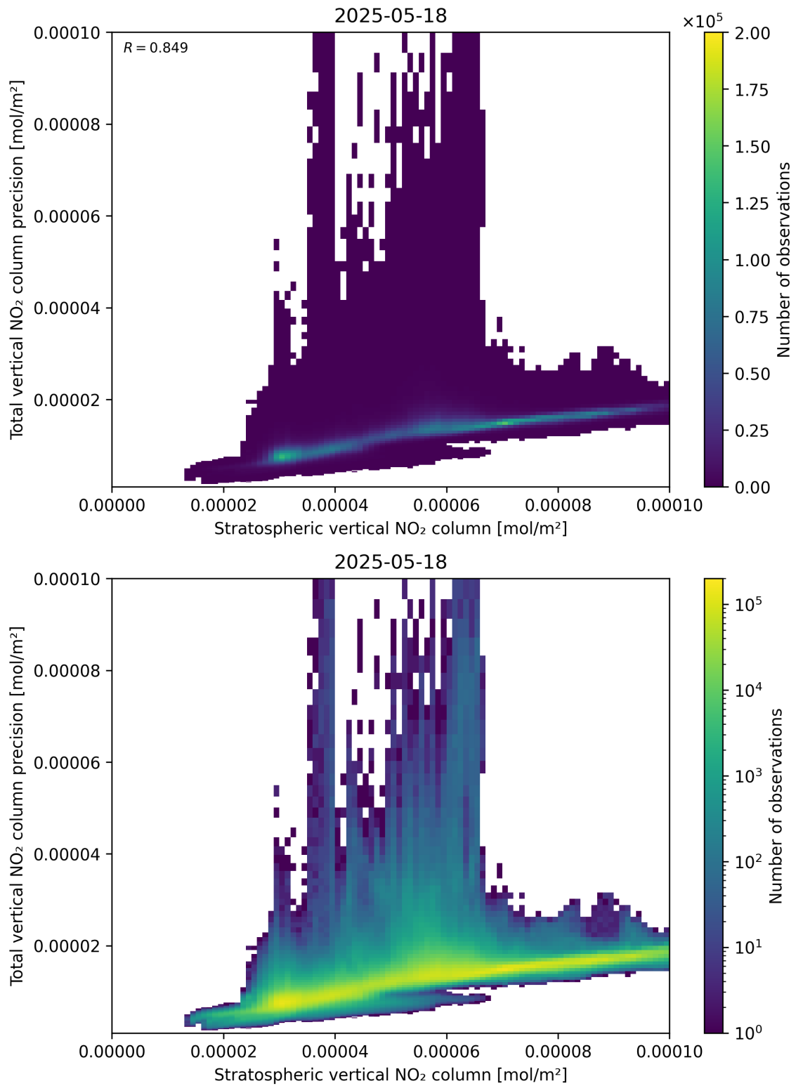
Figure 101: Scatter density plot of “Stratospheric vertical NO 2 column” against “Total vertical NO 2 column precision” for 2025-05-17 to 2025-05-19.
