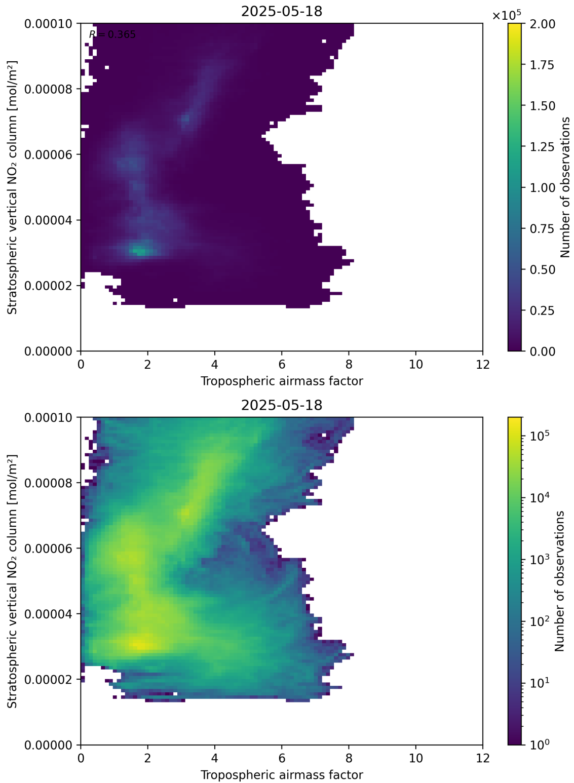
Figure 74: Scatter density plot of “Tropospheric air mass factor” against “Stratospheric vertical NO 2 column” for 2025-05-17 to 2025-05-19.
