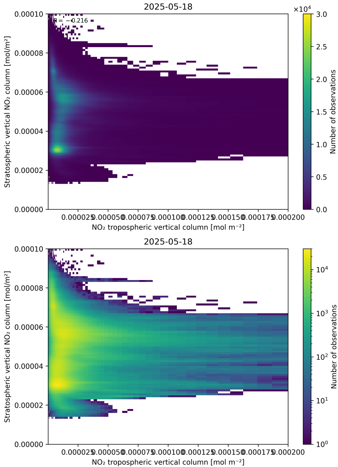
Figure 125: Scatter density plot of “NO 2 tropospheric vertical column” against “Stratospheric vertical NO 2 column” for 2025-05-17 to 2025-05-19.
