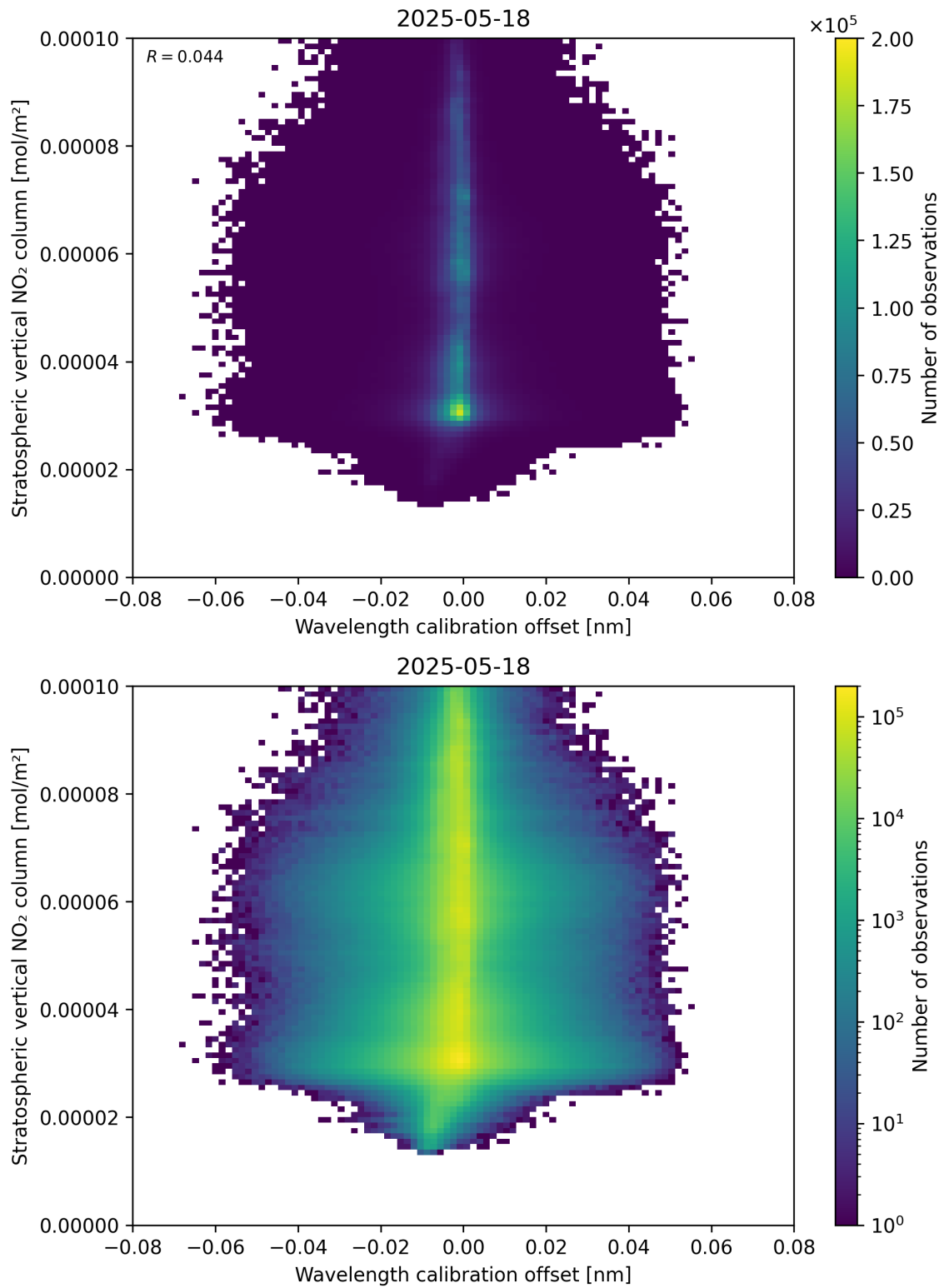
Figure 176: Scatter density plot of “Wavelength calibration offset” against “Stratospheric vertical NO 2 column” for 2025-05-17 to 2025-05-19.
