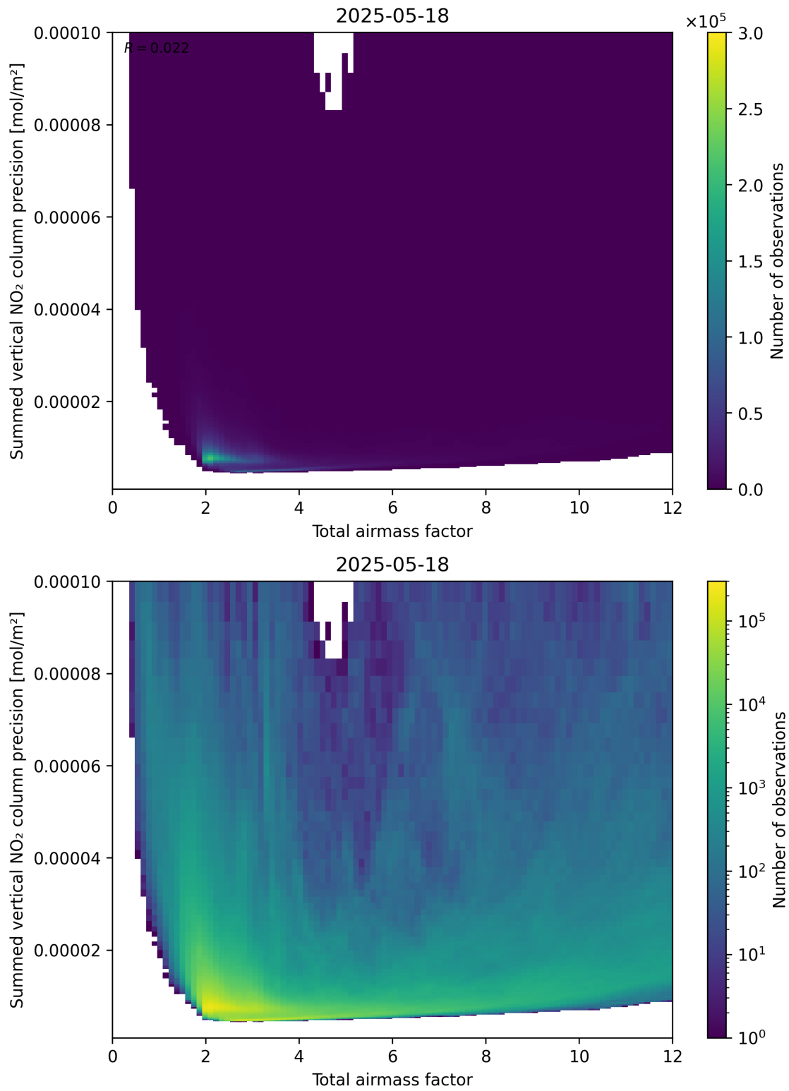
Figure 66: Scatter density plot of “Total airmass factor” against “Summed vertical NO 2 column precision” for 2025-05-17 to 2025-05-19.
