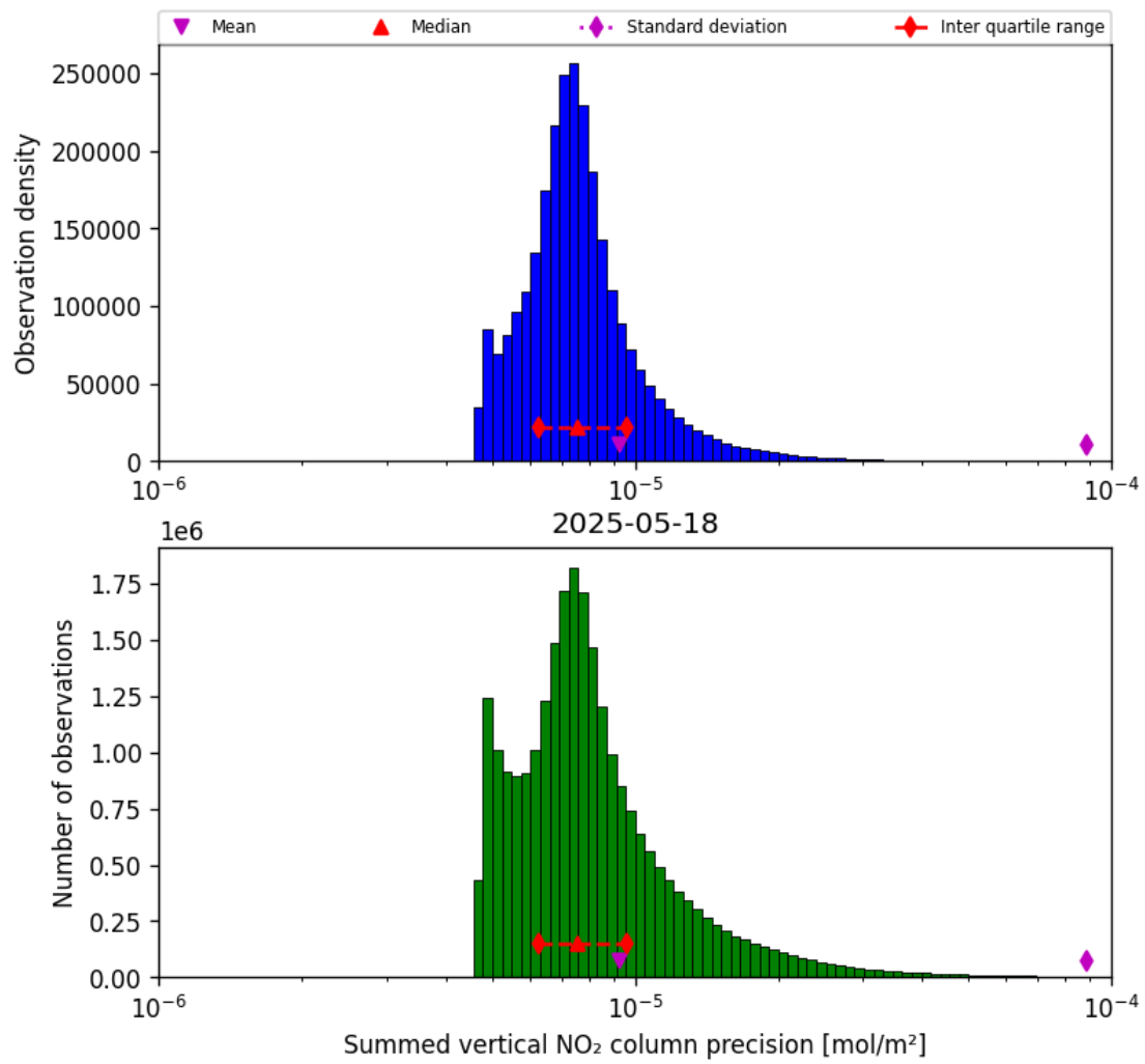
Figure 41: Histogram of "Summed vertical NO 2 column precision" for 2025-05-17 to 2025-05-19
