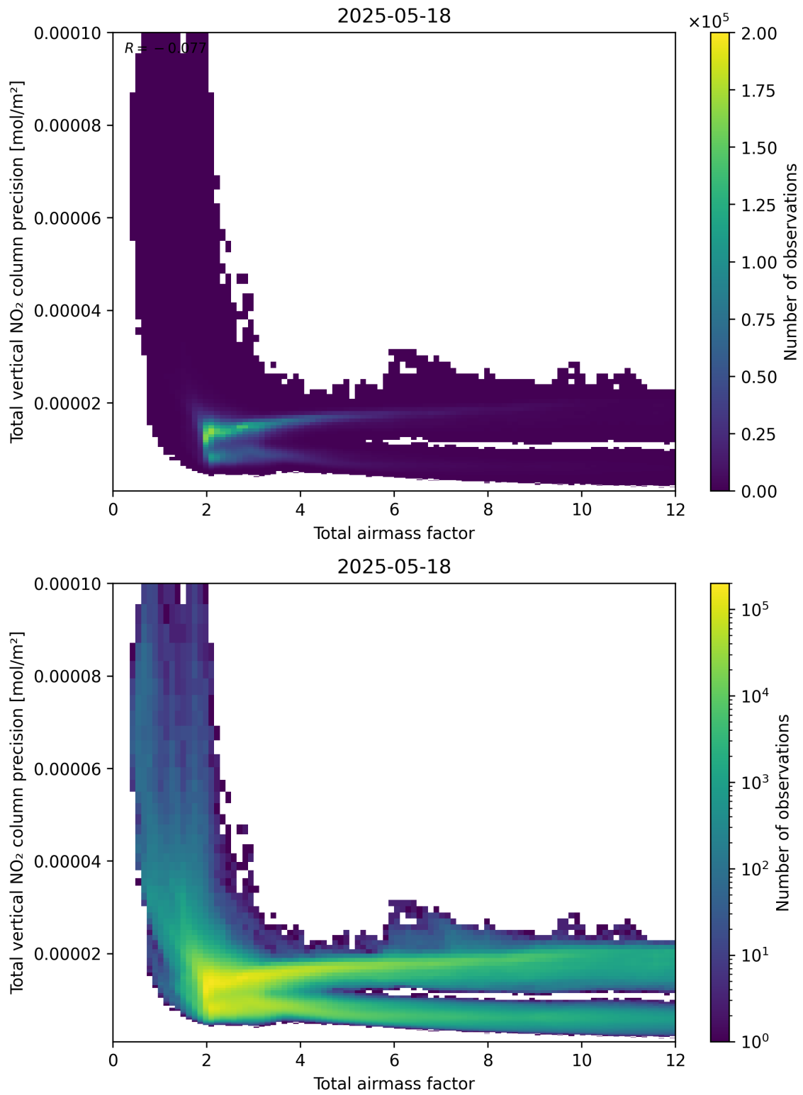
Figure 68: Scatter density plot of “Total airmass factor” against “Total vertical NO 2 column precision” for 2025-05-17 to 2025-05-19.
