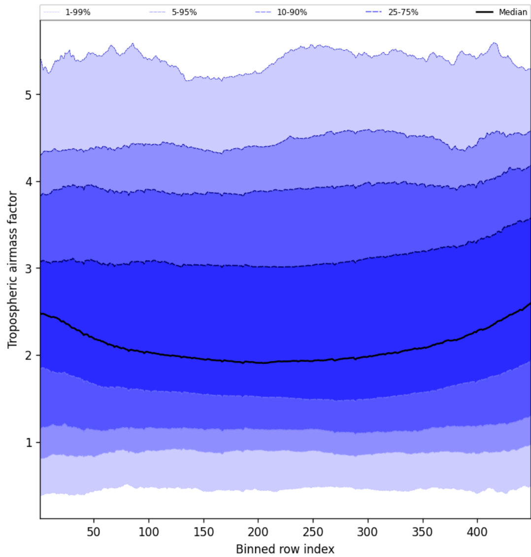
Figure 48: Along track statistics of “Tropospheric airmass factor” for 2025-05-17 to 2025-05-19
