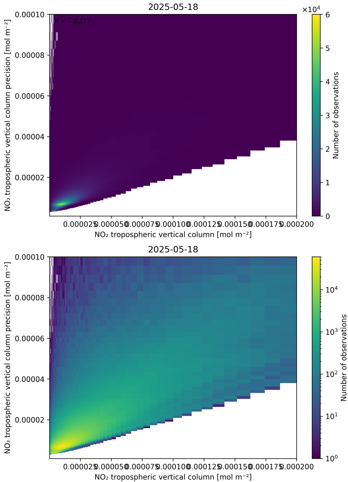
Figure 130: Scatter density plot of “NO 2 tropospheric vertical column” against “NO 2 tropospheric vertical column precision” for 2025-05-17 to 2025-05-19.
