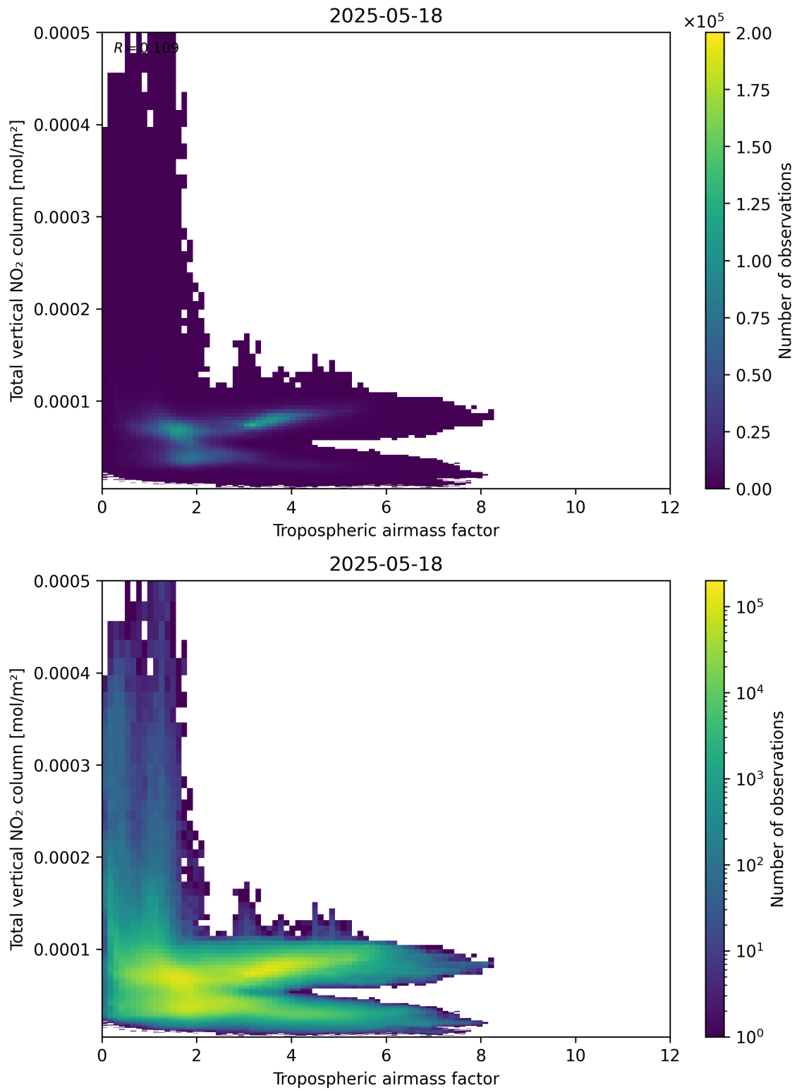
Figure 77: Scatter density plot of “Tropospheric airmass factor” against “Total vertical NO 2 column” for 2025-05-17 to 2025-05-19.
