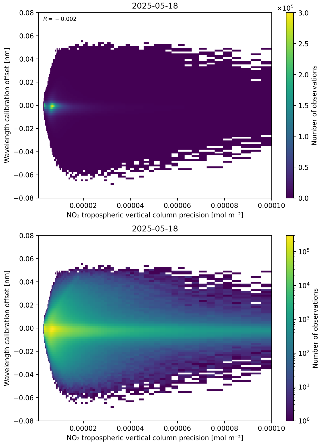
Figure 141: Scatter density plot of “NO 2 tropospheric vertical column precision” against “Wavelength calibration offset” for 2025-05-17 to 2025-05-19.
