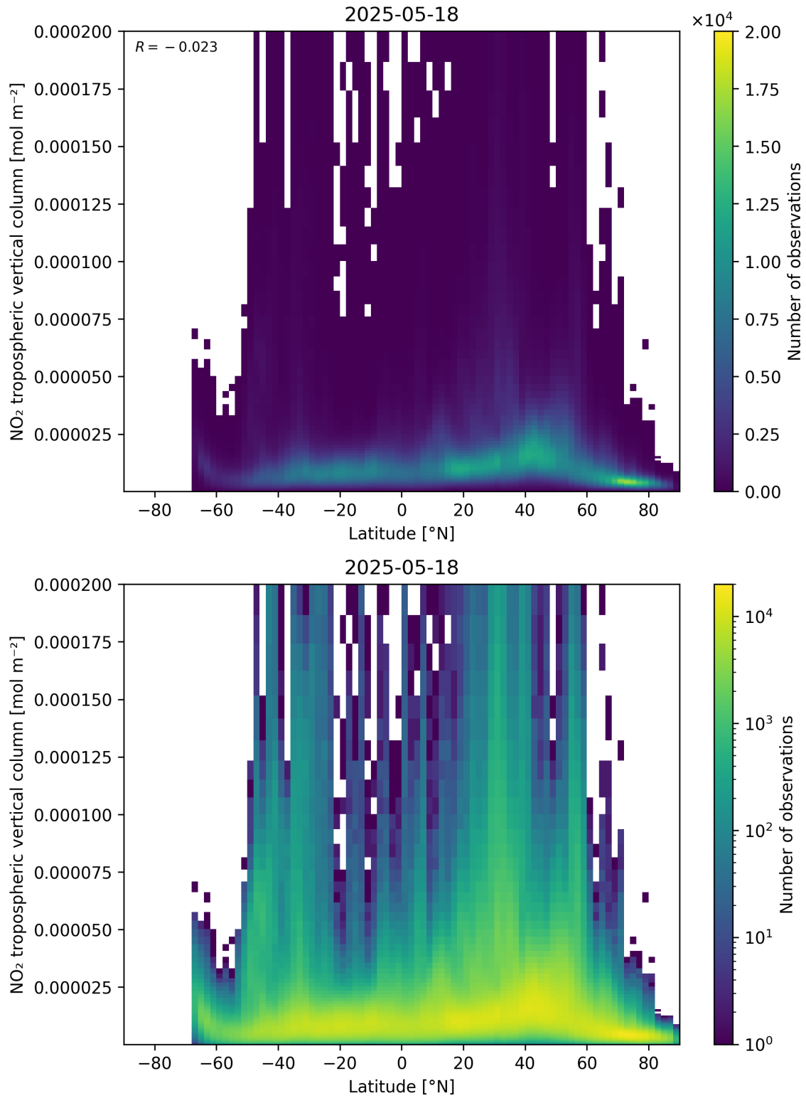
Figure 92: Scatter density plot of “Latitude” against “NO 2 tropospheric vertical column” for 2025-05-17 to 2025-05-19.
