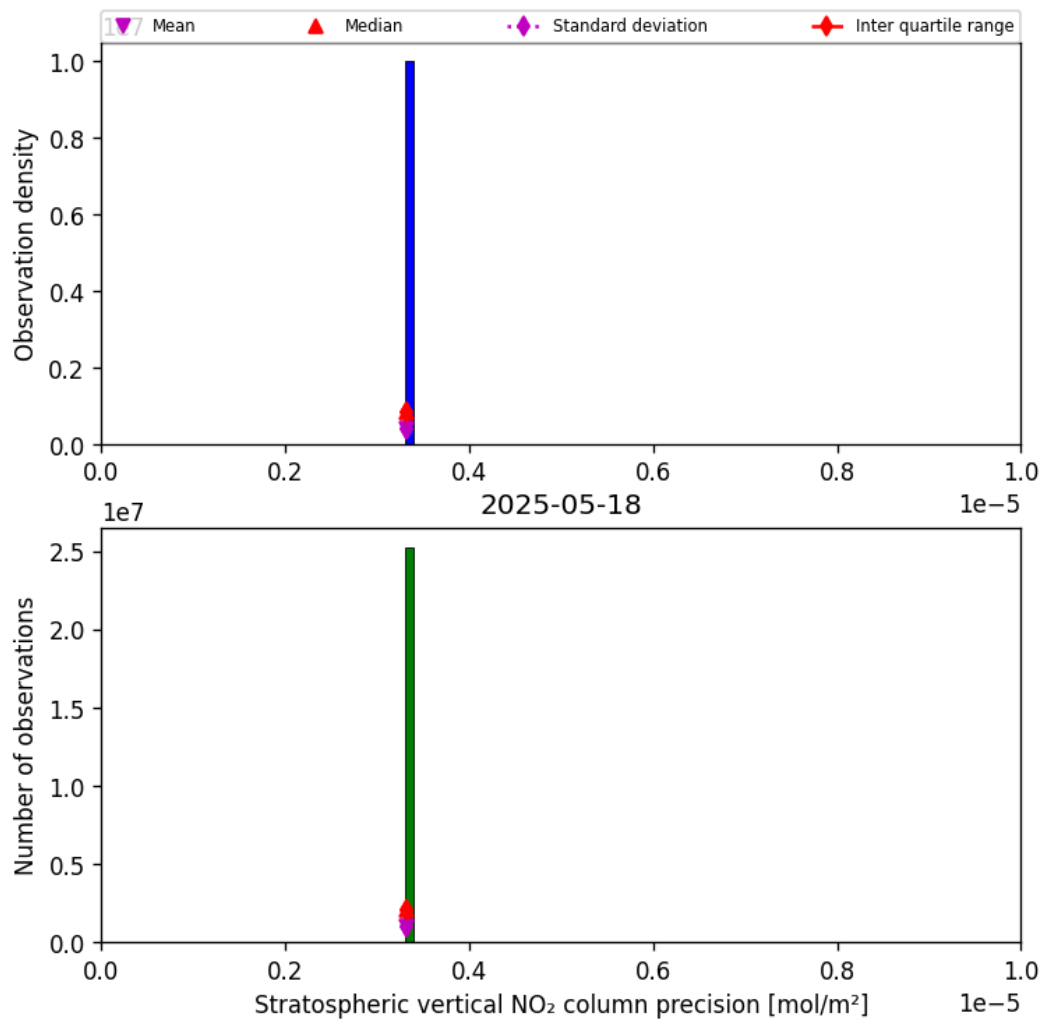
Figure 37: Histogram of “Stratospheric vertical NO 2 column precision” for 2025-05-17 to 2025-05-19
