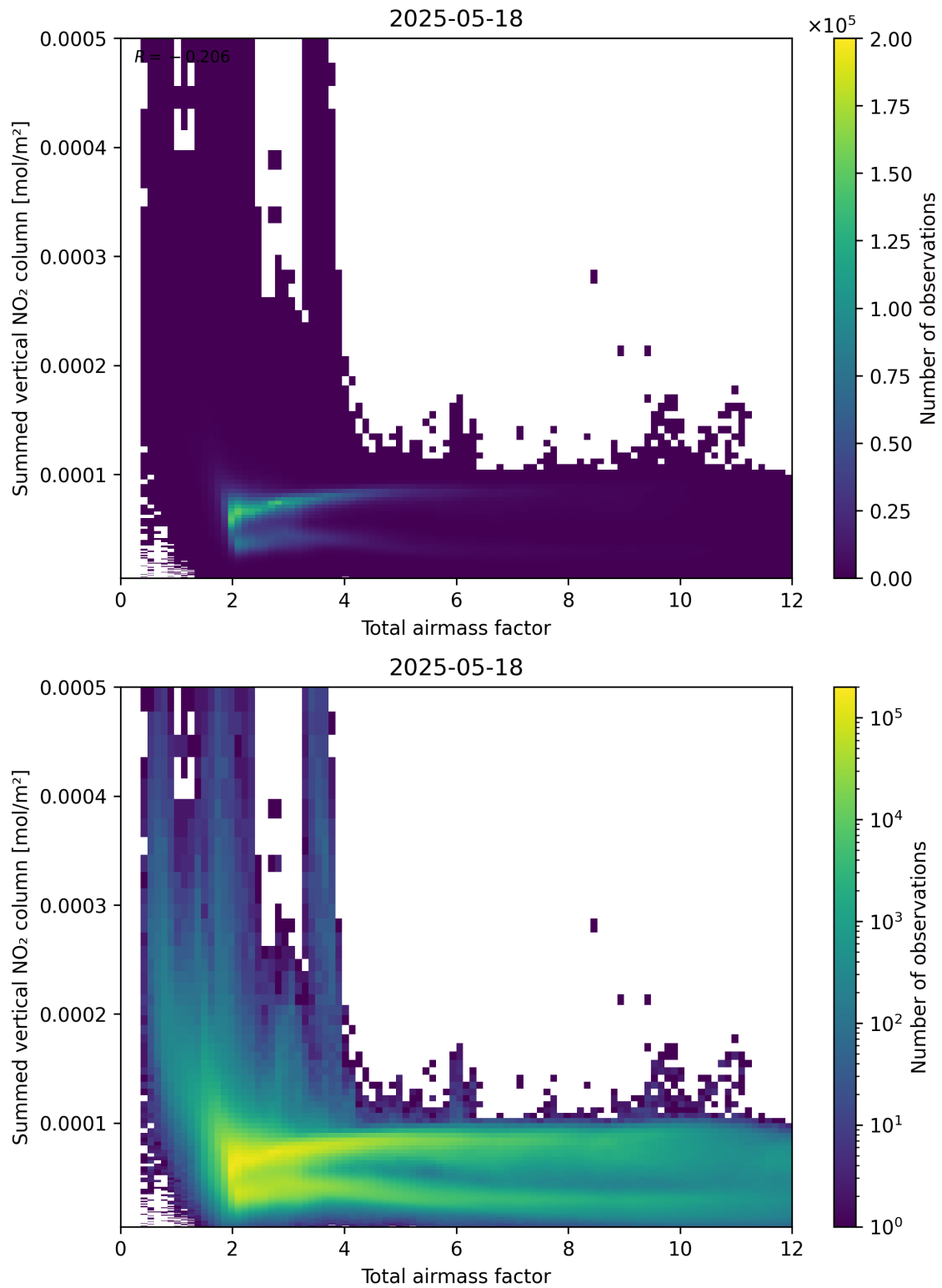
Figure 65: Scatter density plot of “Total airmass factor” against “Summed vertical NO 2 column” for 2025-05-17 to 2025-05-19.
