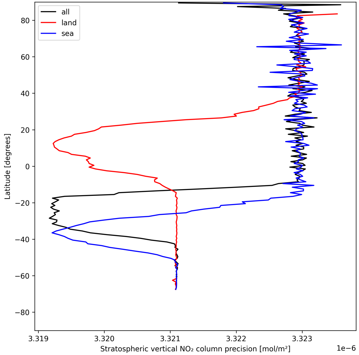
Figure 20: Zonal average of “Stratospheric vertical NO 2 column precision” for 2025-05-17 to 2025-05-19.
