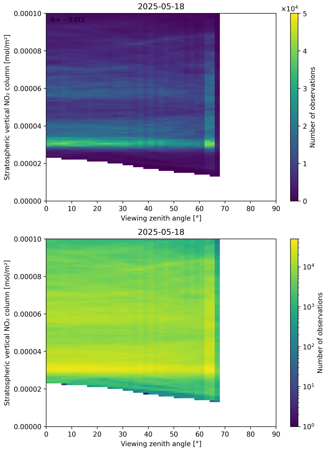
Figure 164: Scatter density plot of “Viewing zenith angle” against “Stratospheric vertical NO 2 column” for 2025-05-17 to 2025-05-19.
