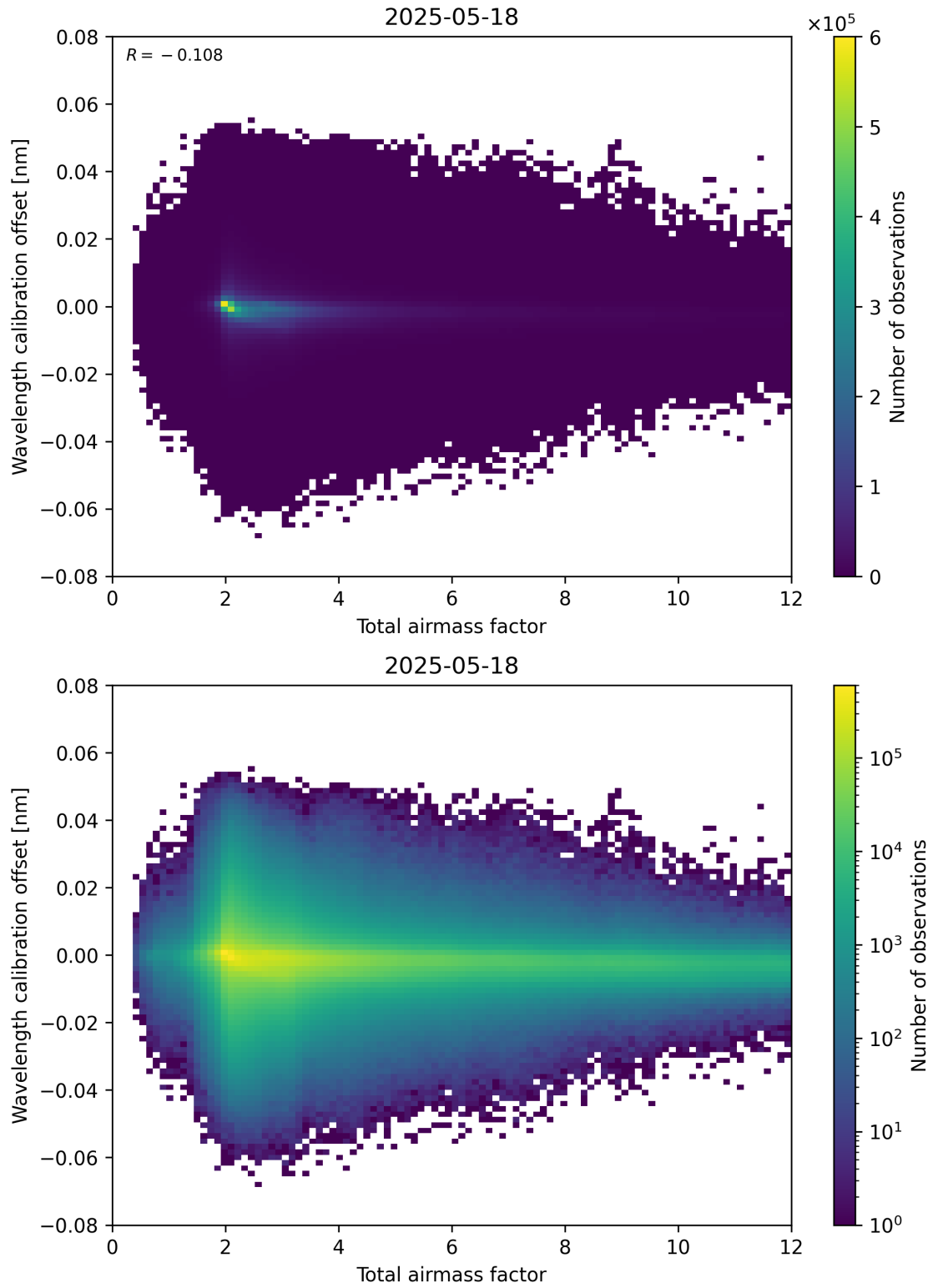
Figure 70: Scatter density plot of “Total airmass factor” against “Wavelength calibration offset” for 2025-05-17 to 2025-05-19.
