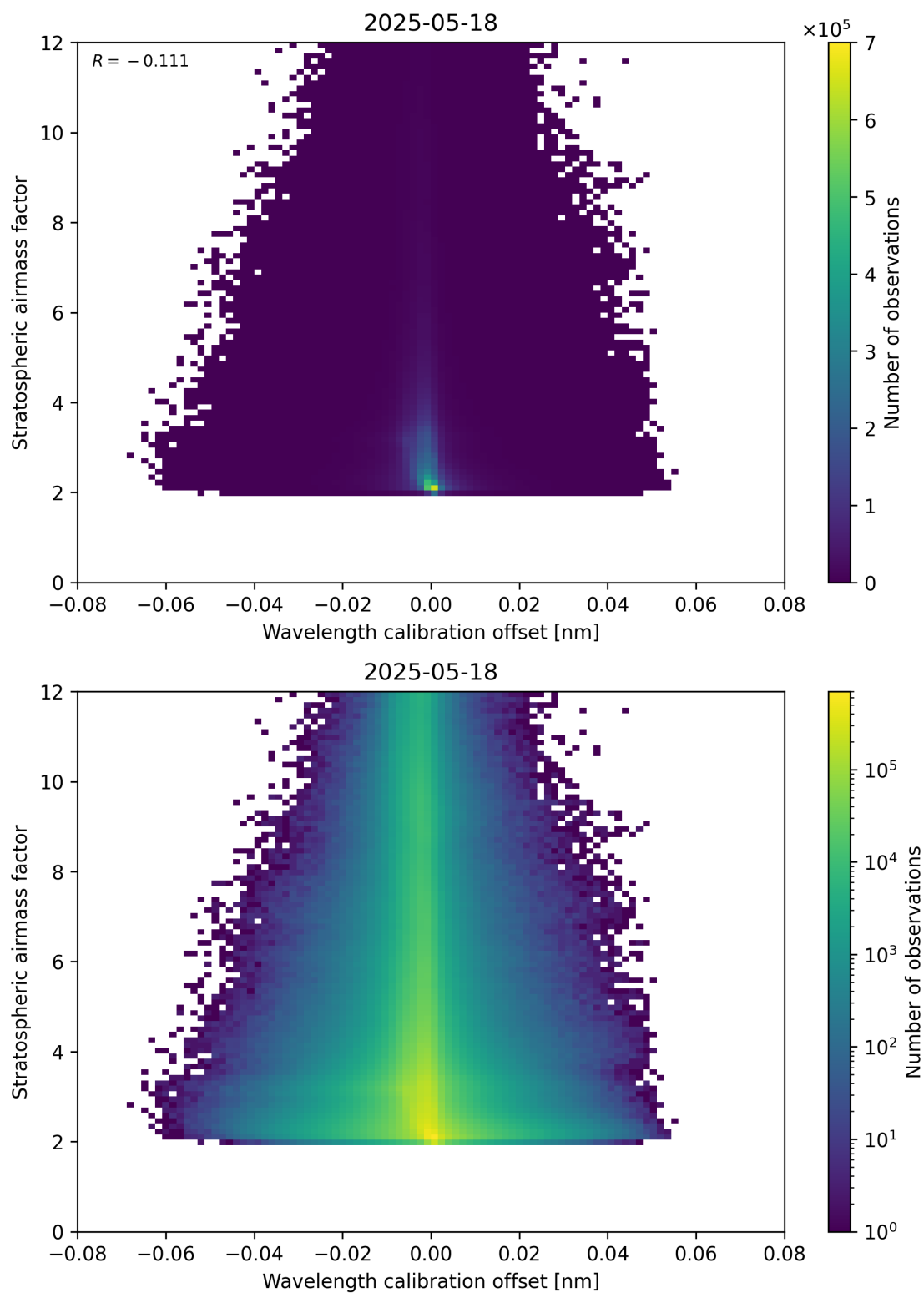
Figure 174: Scatter density plot of “Wavelength calibration offset” against “Stratospheric air mass factor” for 2025-05-17 to 2025-05-19.
