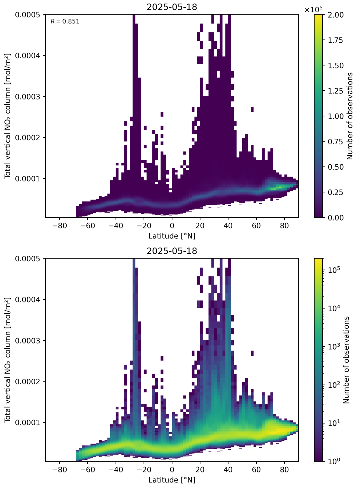
Figure 90: Scatter density plot of “Latitude” against “Total vertical NO 2 column” for 2025-05-17 to 2025-05-19.
