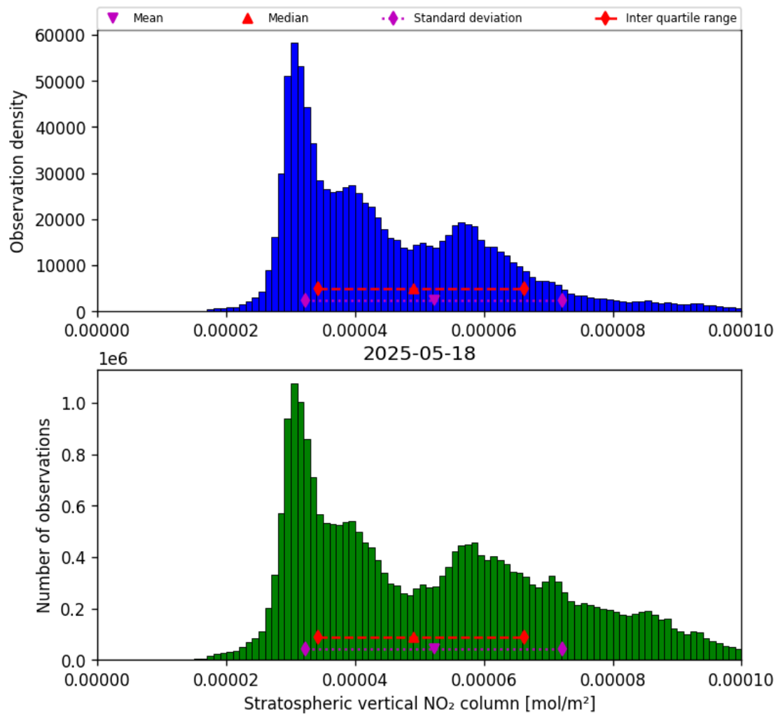
Figure 36: Histogram of “Stratospheric vertical NO 2 column” for 2025-05-17 to 2025-05-19
