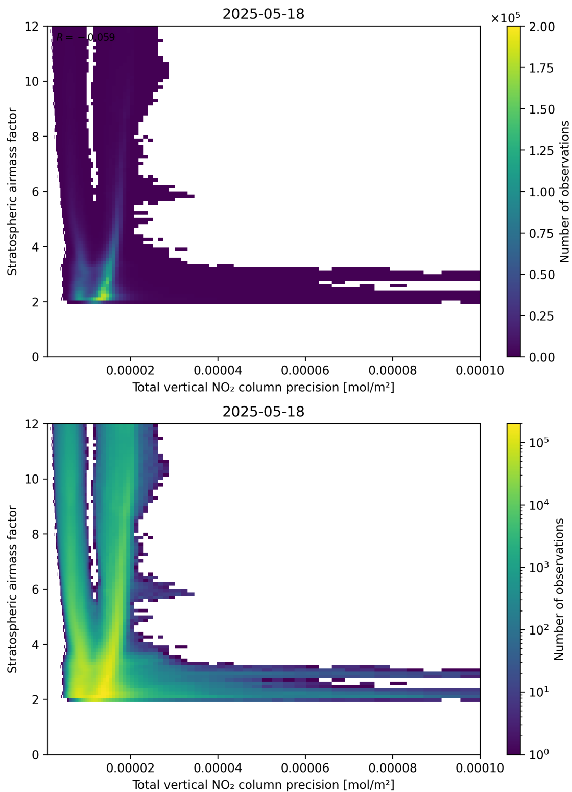
Figure 115: Scatter density plot of “Total vertical NO 2 column precision” against “Stratospheric air mass factor” for 2025-05-17 to 2025-05-19.
