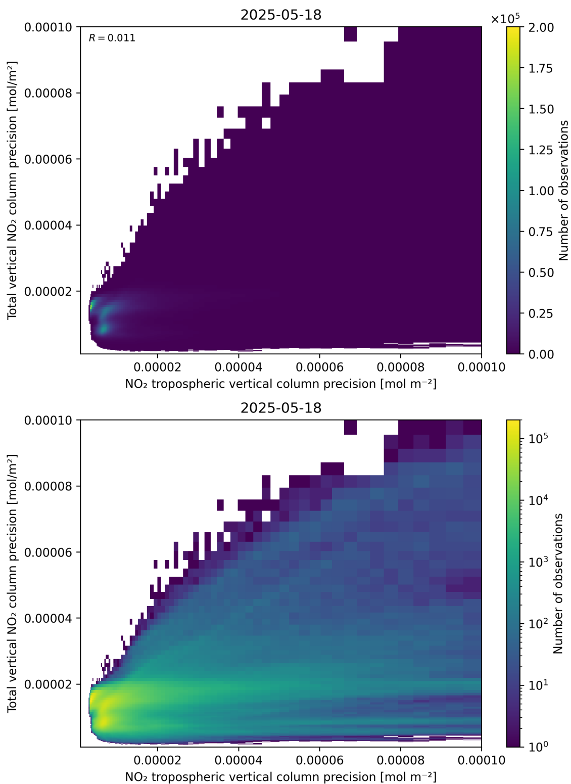
Figure 139: Scatter density plot of “NO 2 tropospheric vertical column precision” against “Total vertical NO 2 column precision” for 2025-05-17 to 2025-05-19.
