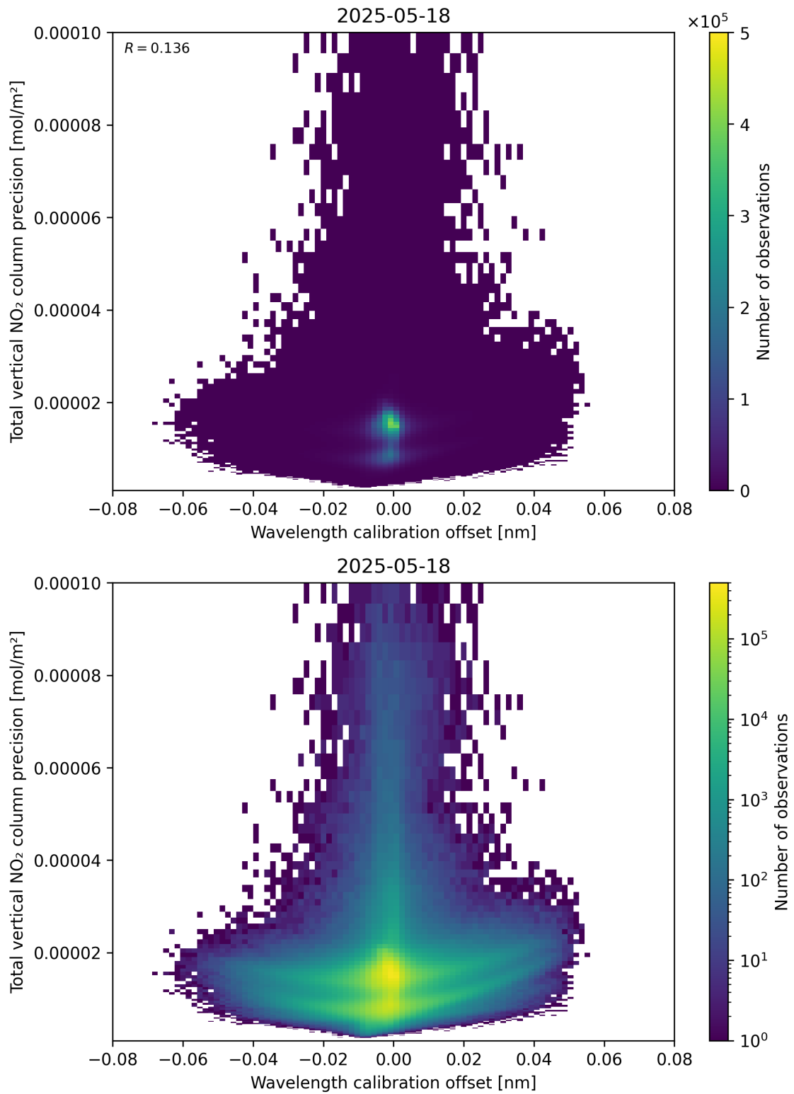
Figure 180: Scatter density plot of “Wavelength calibration offset” against “Total vertical NO 2 column precision” for 2025-05-17 to 2025-05-19.
