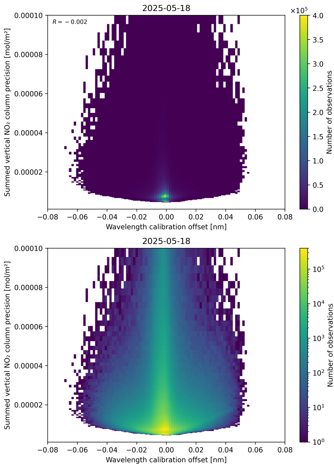
Figure 178: Scatter density plot of “Wavelength calibration offset” against “Summed vertical NO 2 column precision” for 2025-05-17 to 2025-05-19.
