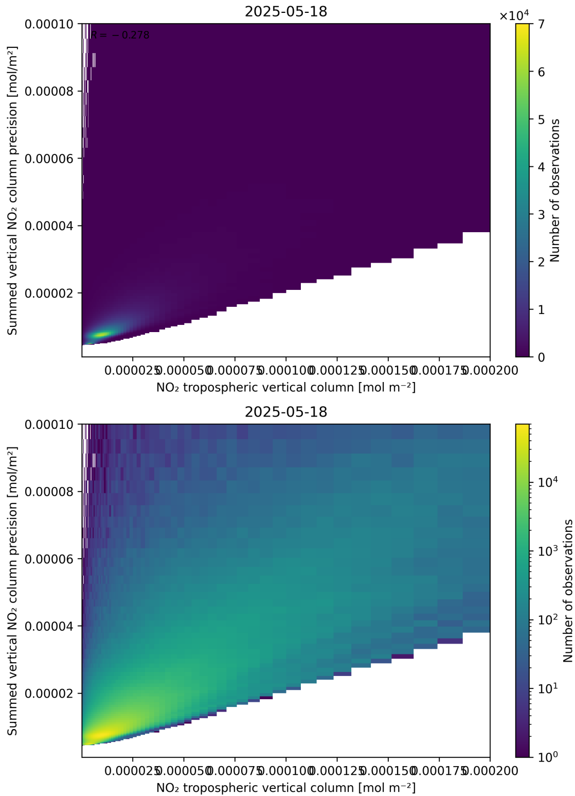
Figure 127: Scatter density plot of “NO 2 tropospheric vertical column” against “Summed vertical NO 2 column precision” for 2025-05-17 to 2025-05-19.
