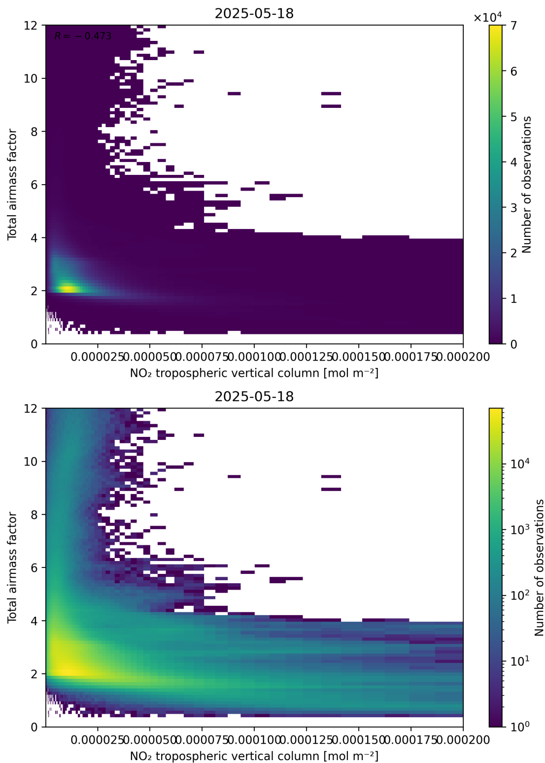
Figure 122: Scatter density plot of “NO 2 tropospheric vertical column” against “Total air mass factor” for 2025-05-17 to 2025-05-19.
