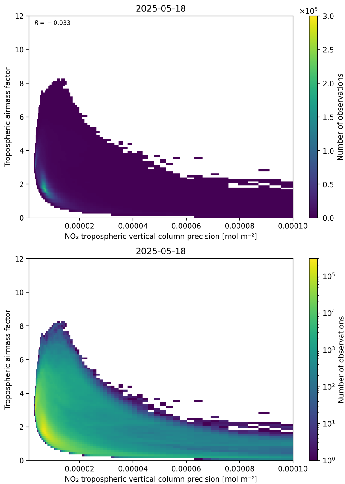
Figure 133: Scatter density plot of “NO 2 tropospheric vertical column precision” against “Tropospheric air mass factor” for 2025-05-17 to 2025-05-19.
