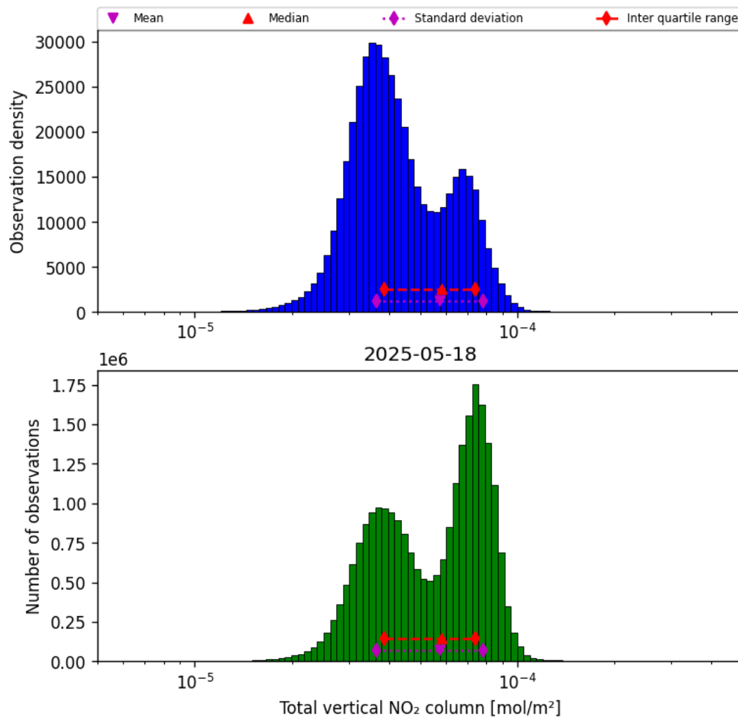
Figure 38: Histogram of “Total vertical NO 2 column” for 2025-05-17 to 2025-05-19
