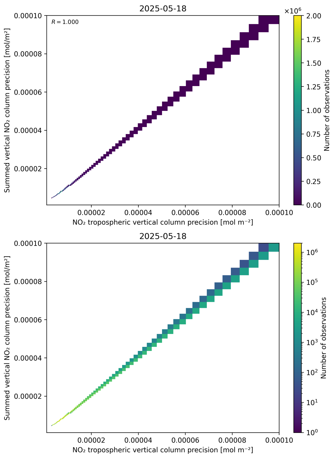
Figure 137: Scatter density plot of “NO 2 tropospheric vertical column precision” against “Summed vertical NO 2 column precision” for 2025-05-17 to 2025-05-19.
