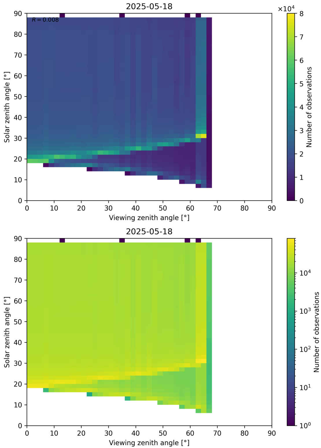
Figure 172: Scatter density plot of “Viewing zenith angle” against “Solar zenith angle” for 2025-05-17 to 2025-05-19.
