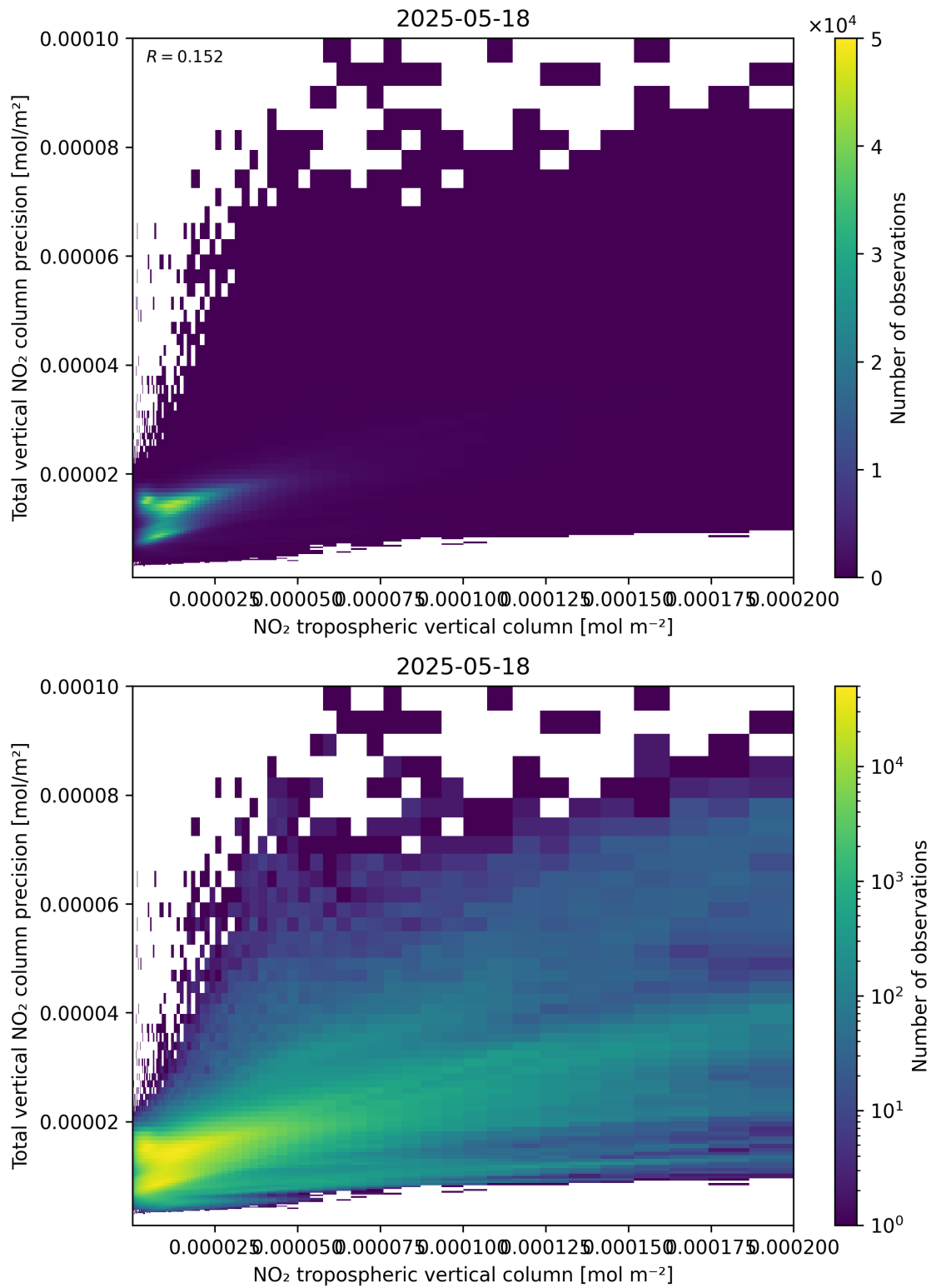
Figure 129: Scatter density plot of “NO 2 tropospheric vertical column” against “Total vertical NO 2 column precision” for 2025-05-17 to 2025-05-19.
