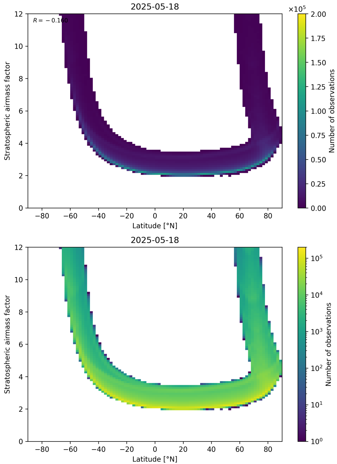
Figure 83: Scatter density plot of “Latitude” against “Stratospheric air mass factor” for 2025-05-17 to 2025-05-19.
