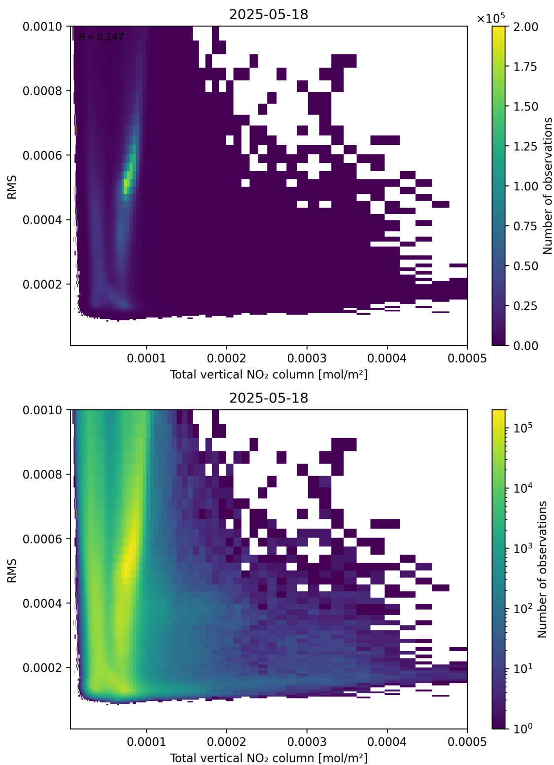
Figure 120: Scatter density plot of “Total vertical NO 2 column” against “RMS” for 2025-05-17 to 2025-05-19.
