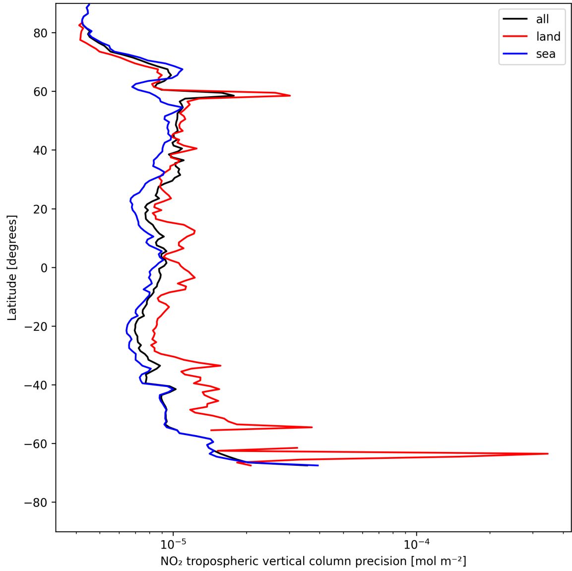
Figure 13: Zonal average of “NO 2 tropospheric vertical column precision” for 2025-05-17 to 2025-05-19.
