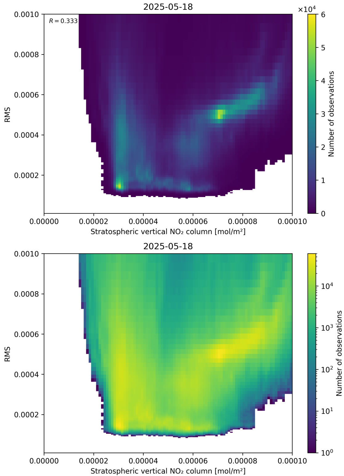
Figure 102: Scatter density plot of “Stratospheric vertical NO 2 column” against “RMS” for 2025-05-17 to 2025-05-19.
