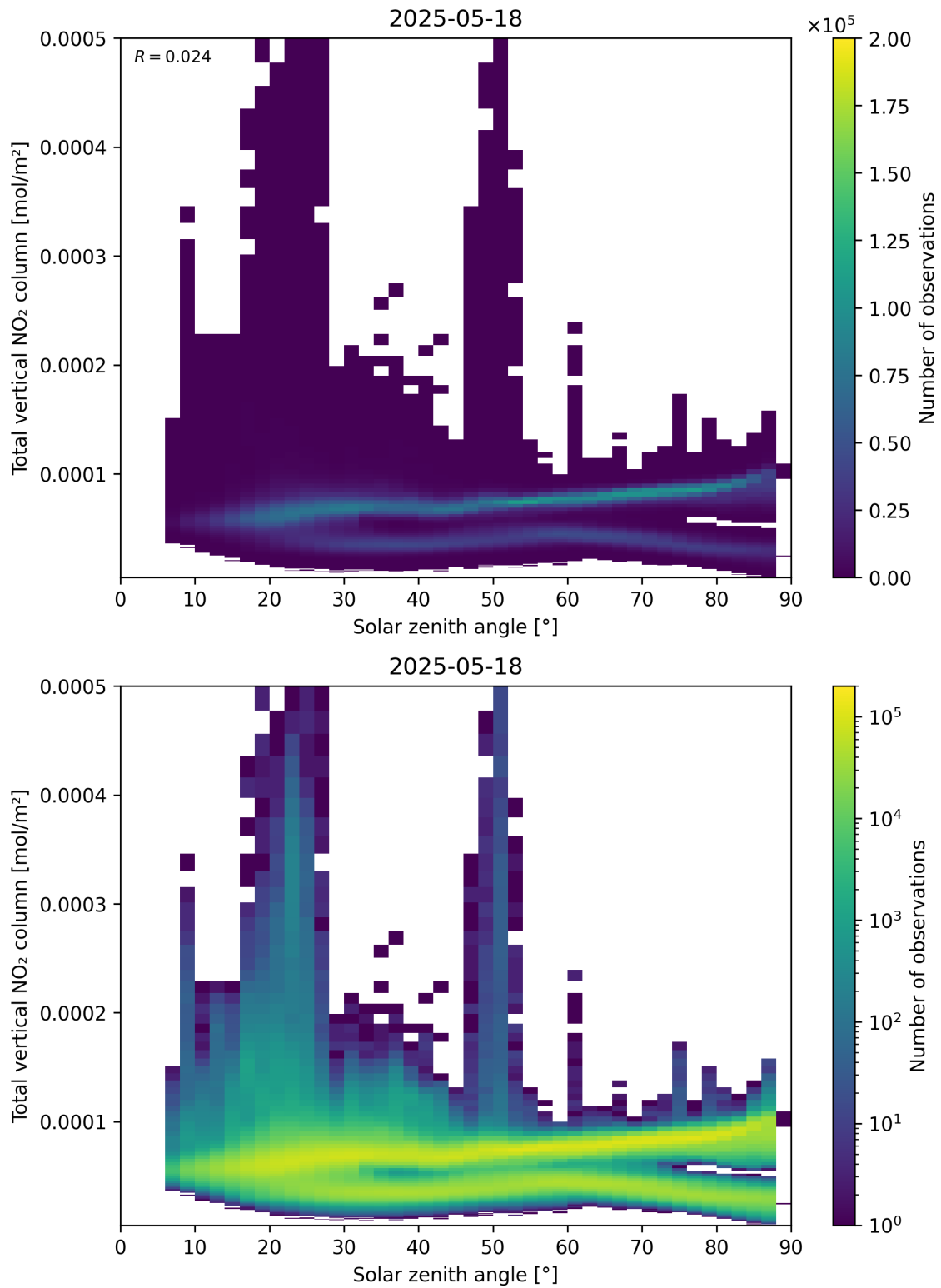
Figure 153: Scatter density plot of “Solar zenith angle” against “Total vertical NO 2 column” for 2025-05-17 to 2025-05-19.
