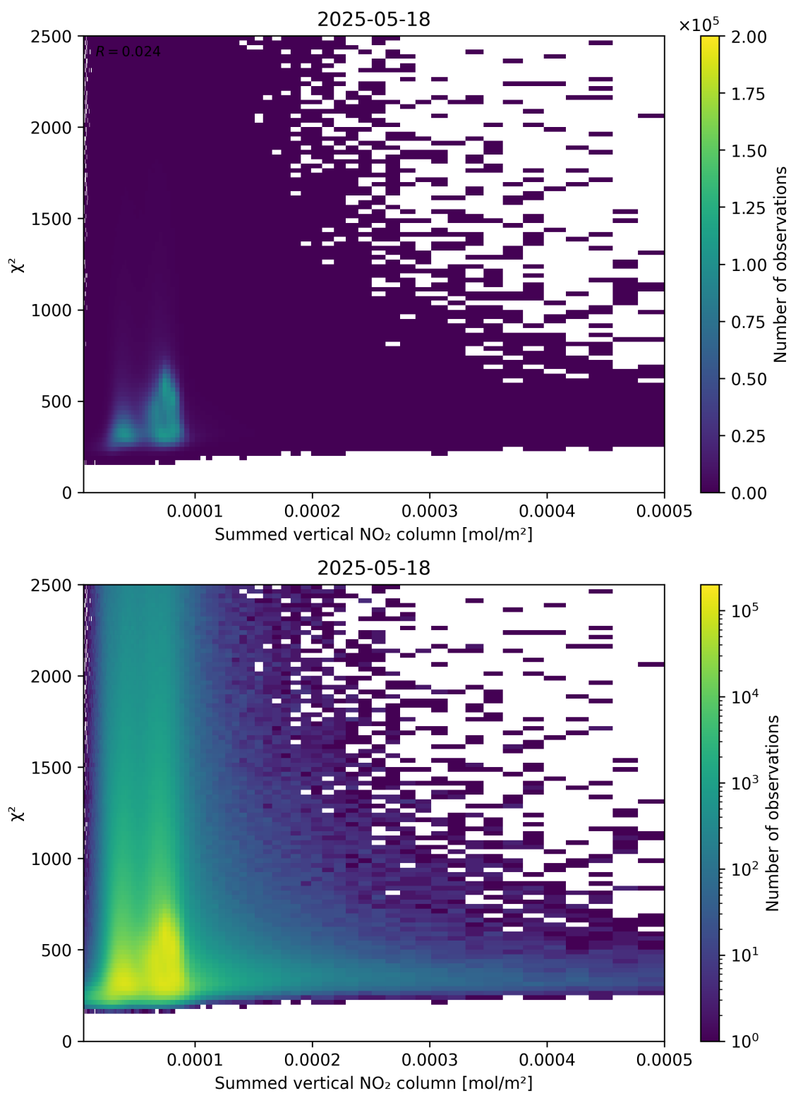
Figure 104: Scatter density plot of “Summed vertical NO 2 column” against “ \chi^2 ” for 2025-05-17 to 2025-05-19.
