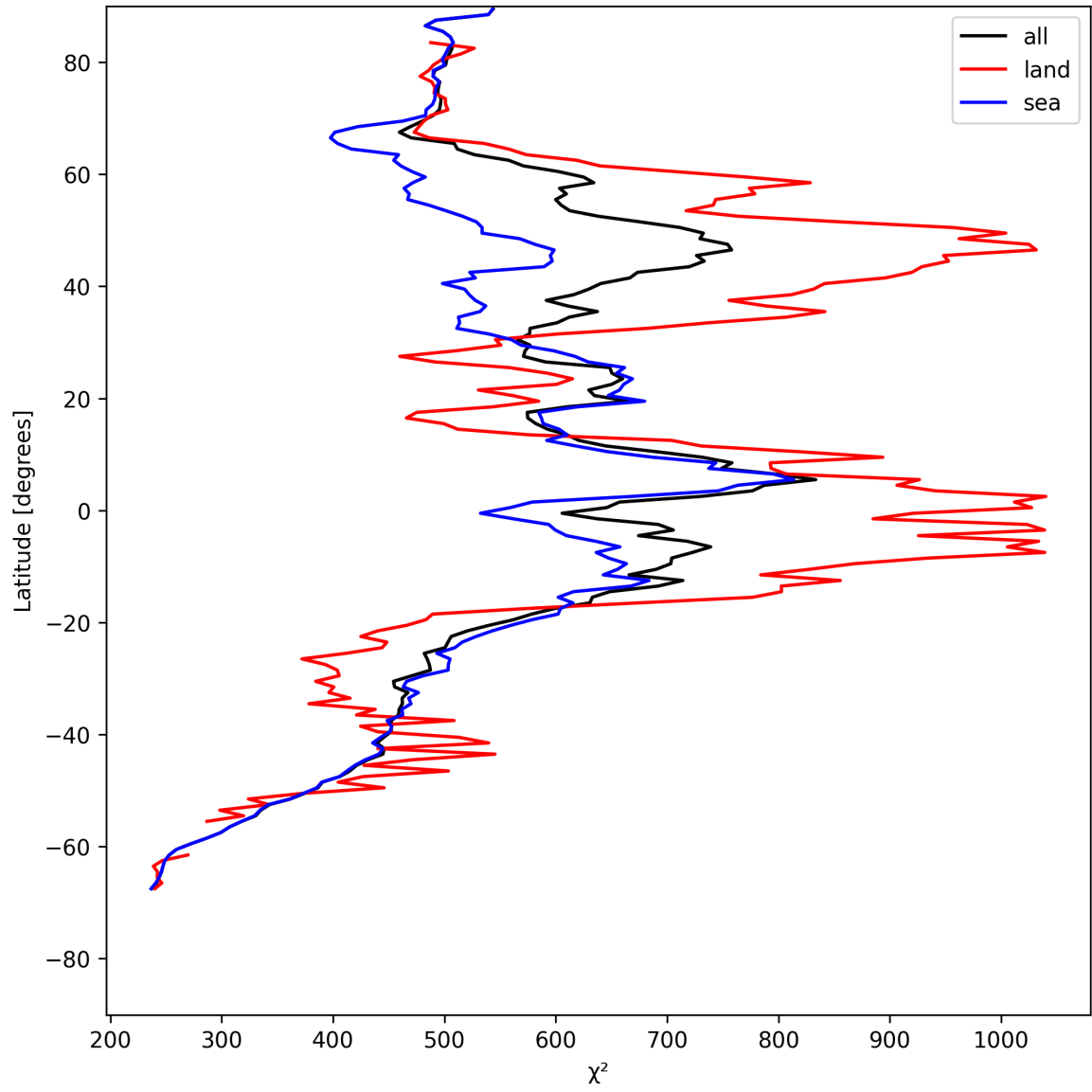
Figure 25: Zonal average of “ \chi^2 ” for 2025-05-17 to 2025-05-19.
