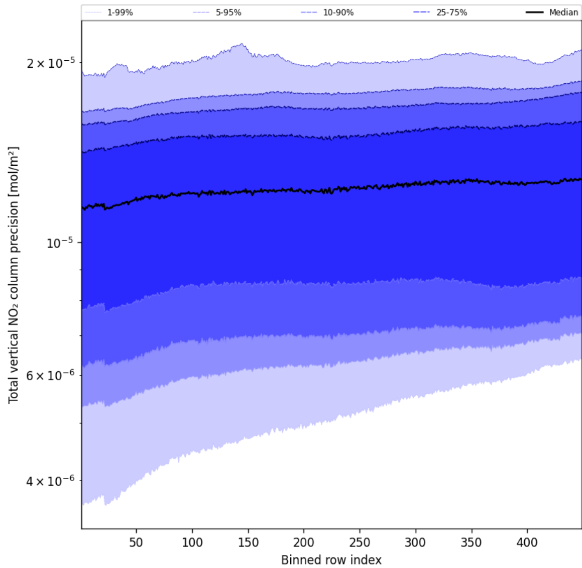
Figure 56: Along track statistics of “Total vertical NO 2 column precision” for 2025-05-17 to 2025-05-19
