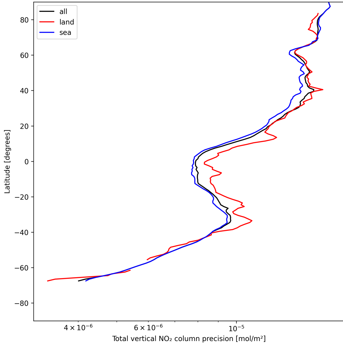
Figure 22: Zonal average of “Total vertical NO 2 column precision” for 2025-05-17 to 2025-05-19.
