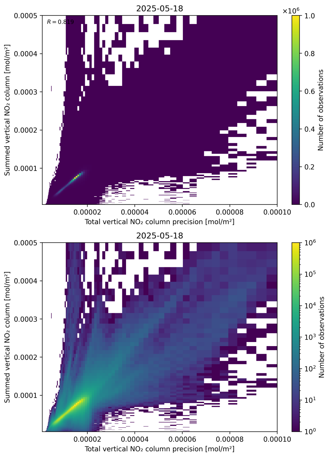
Figure 117: Scatter density plot of “Total vertical NO 2 column precision” against “Summed vertical NO 2 column” for 2025-05-17 to 2025-05-19.
