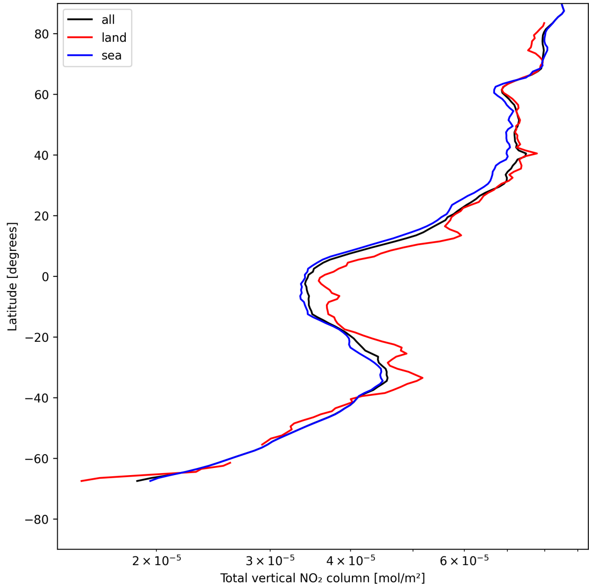
Figure 21: Zonal average of “Total vertical NO 2 column” for 2025-05-17 to 2025-05-19.
