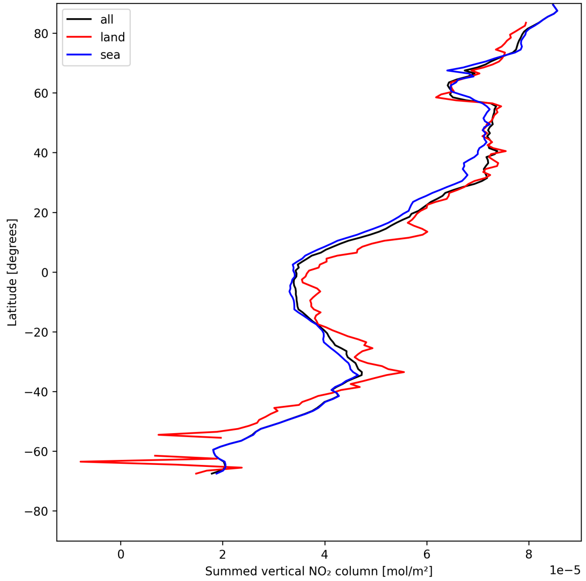
Figure 23: Zonal average of “Summed vertical NO 2 column” for 2025-05-17 to 2025-05-19.
