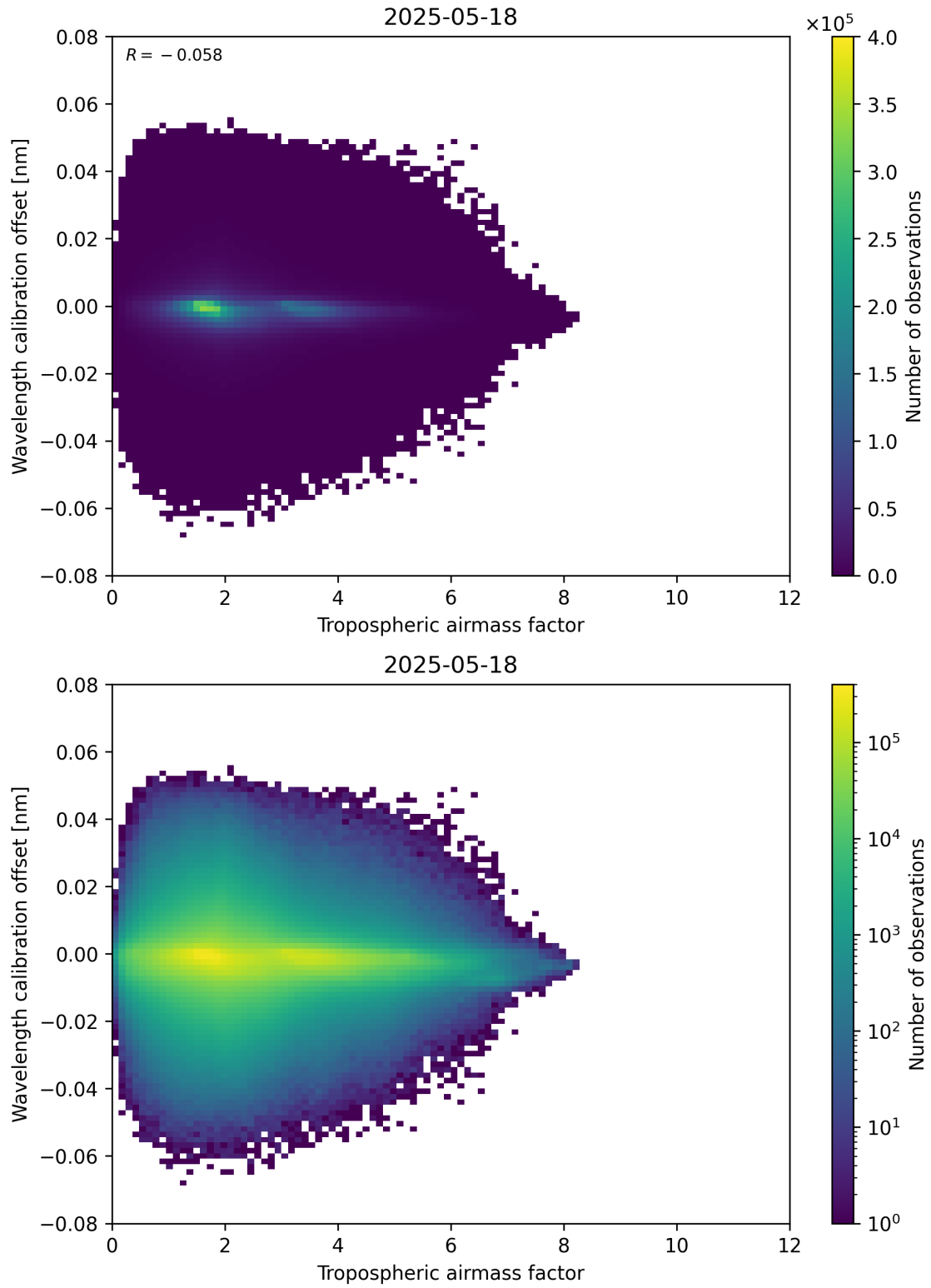
Figure 80: Scatter density plot of “Tropospheric airmass factor” against “Wavelength calibration offset” for 2025-05-17 to 2025-05-19.
