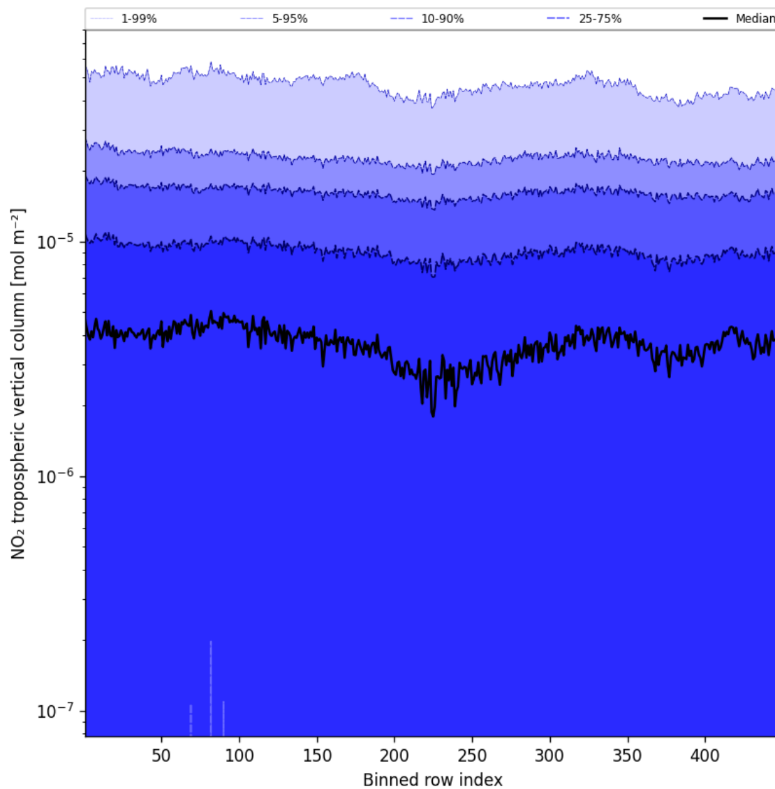
Figure 46: Along track statistics of “NO 2 tropospheric vertical column” for 2025-05-17 to 2025-05-19
