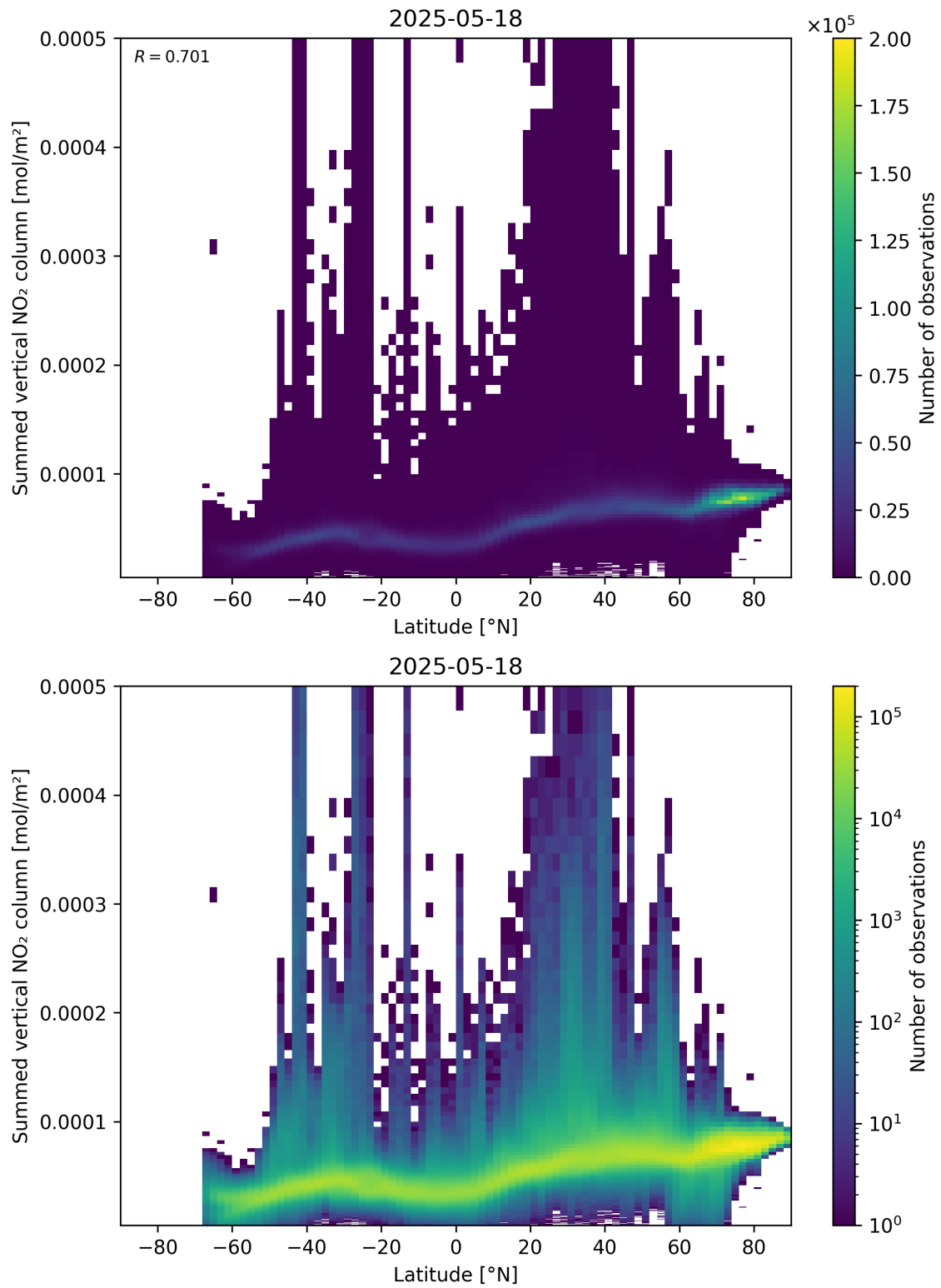
Figure 88: Scatter density plot of “Latitude” against “Summed vertical NO 2 column” for 2025-05-17 to 2025-05-19.
