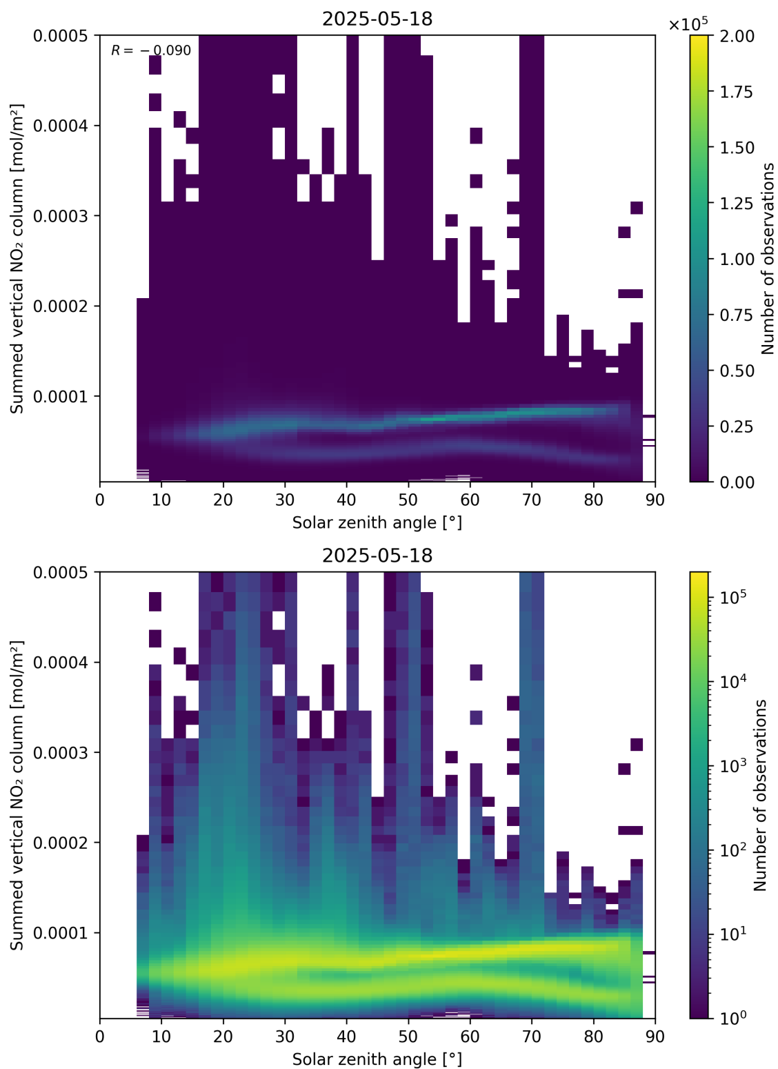
Figure 151: Scatter density plot of “Solar zenith angle” against “Summed vertical NO 2 column” for 2025-05-17 to 2025-05-19.
