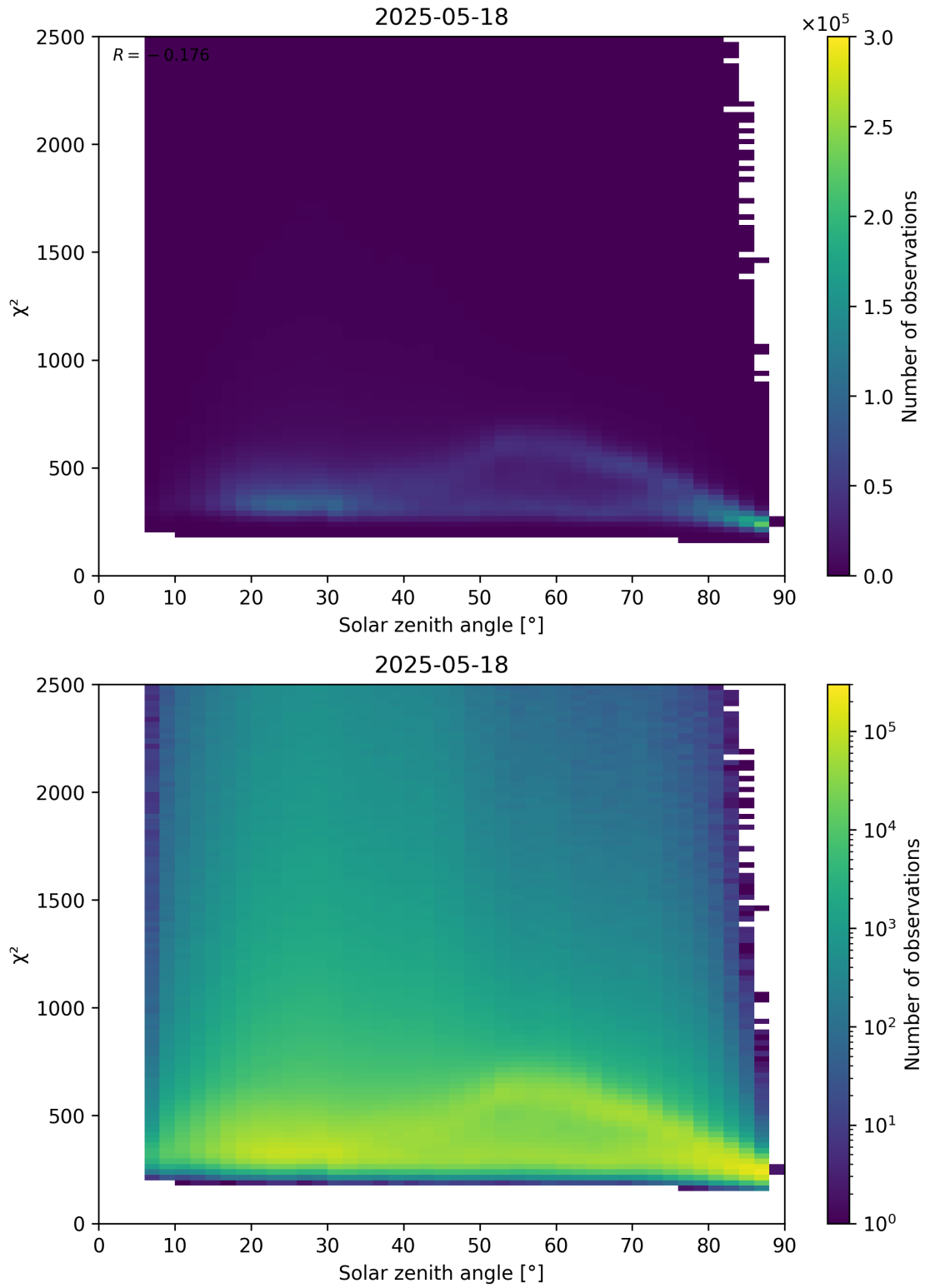
Figure 148: Scatter density plot of “Solar zenith angle” against “ \chi^2 ” for 2025-05-17 to 2025-05-19.
