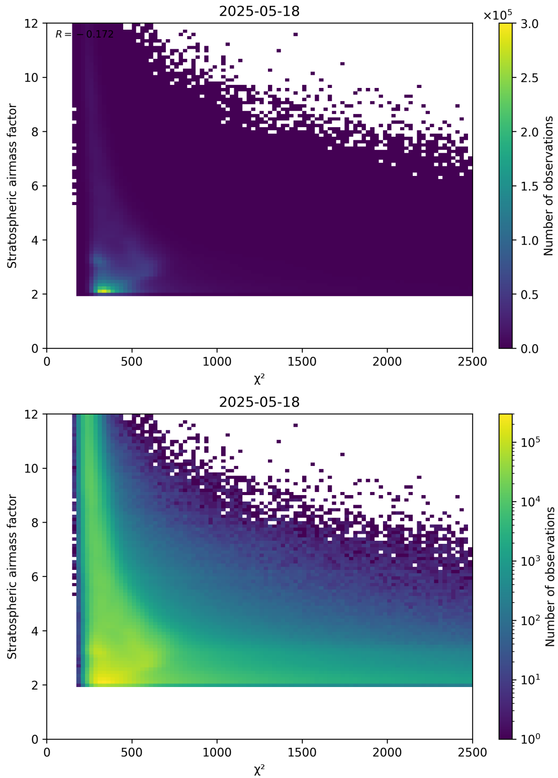
Figure 81: Scatter density plot of “ \chi^2 ” against “Stratospheric airmass factor” for 2025-05-17 to 2025-05-19.
