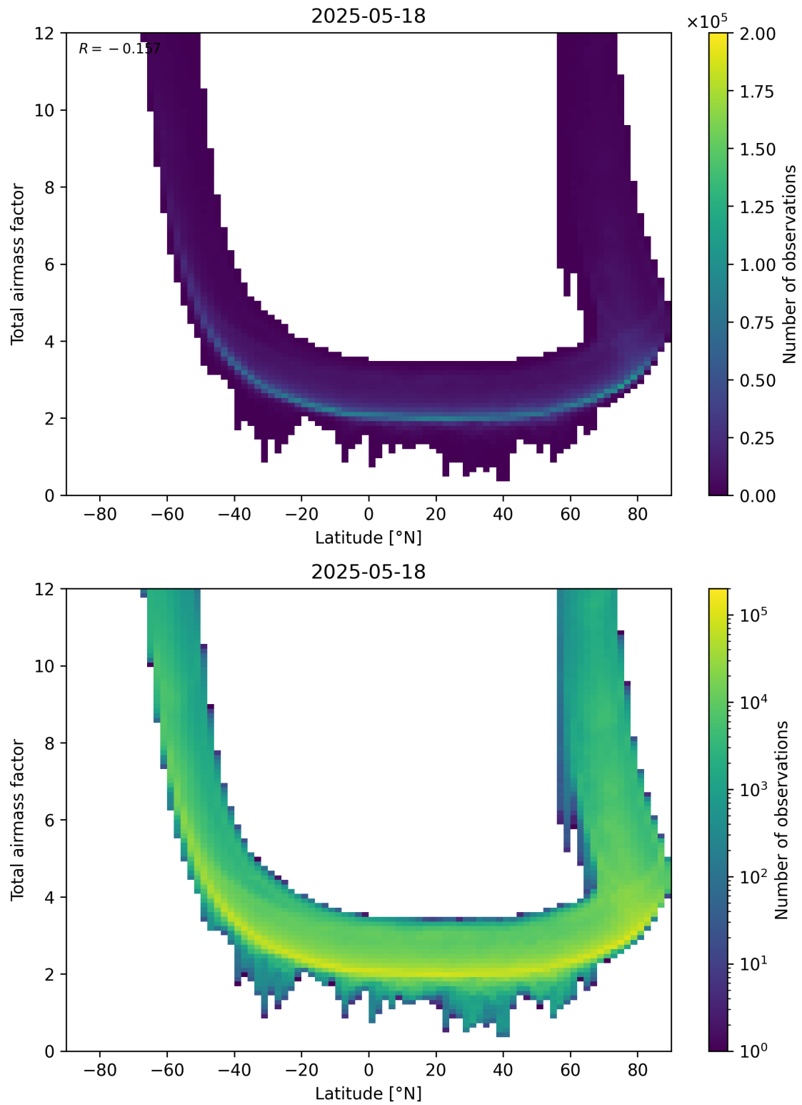
Figure 84: Scatter density plot of “Latitude” against “Total airmass factor” for 2025-05-17 to 2025-05-19.
