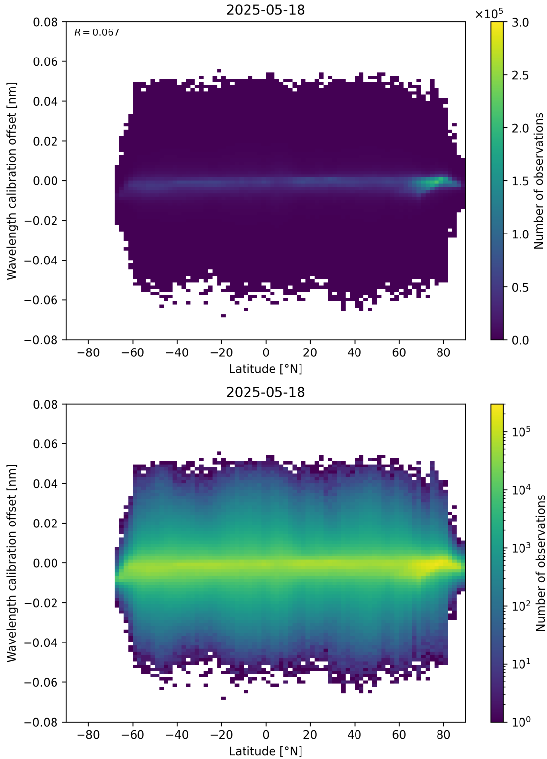
Figure 95: Scatter density plot of “Latitude” against “Wavelength calibration offset” for 2025-05-17 to 2025-05-19.
