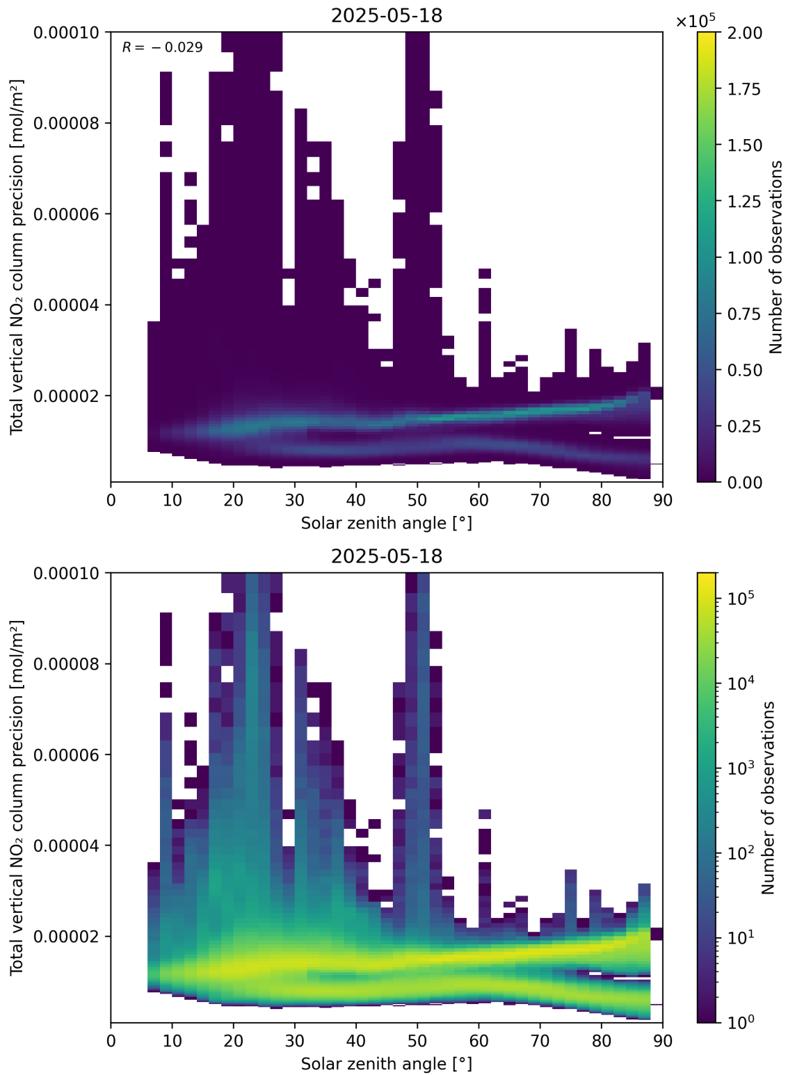
Figure 154: Scatter density plot of “Solar zenith angle” against “Total vertical NO 2 column precision” for 2025-05-17 to 2025-05-19.
