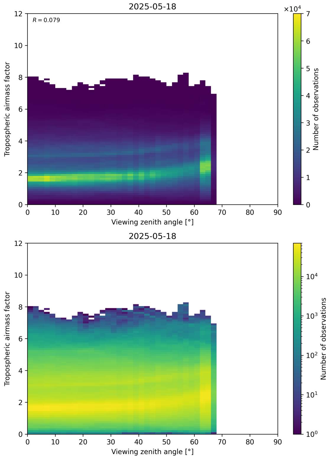
Figure 161: Scatter density plot of “Viewing zenith angle” against “Tropospheric airmass factor” for 2025-05-17 to 2025-05-19.
