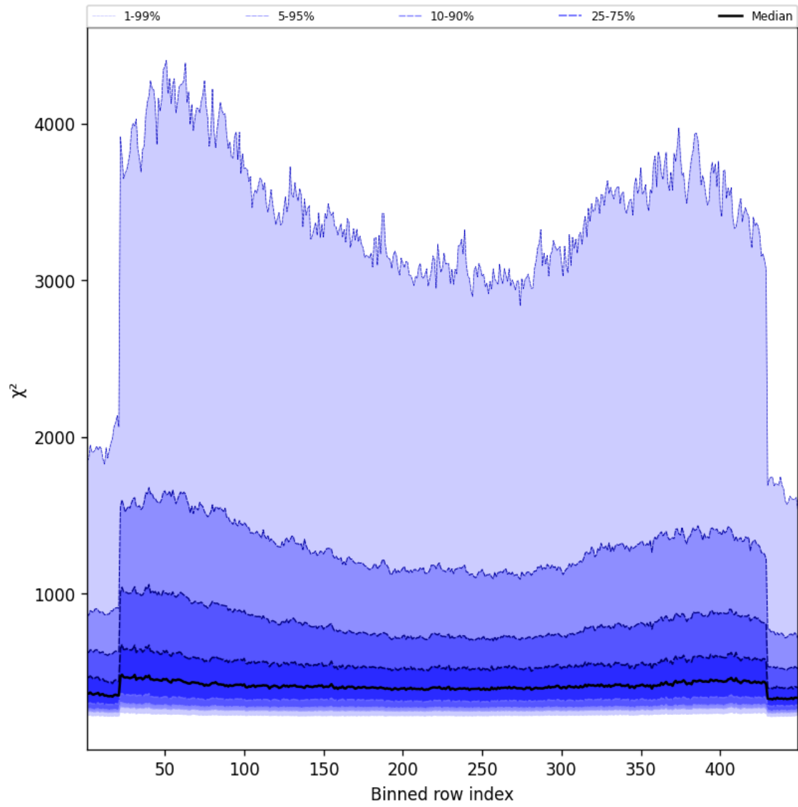
Figure 59: Along track statistics of “ \chi^2 ” for 2025-05-17 to 2025-05-19
