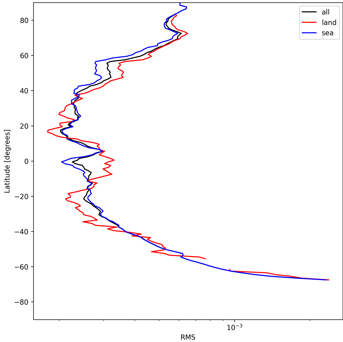
Figure 26: Zonal average of “RMS” for 2025-05-17 to 2025-05-19.
