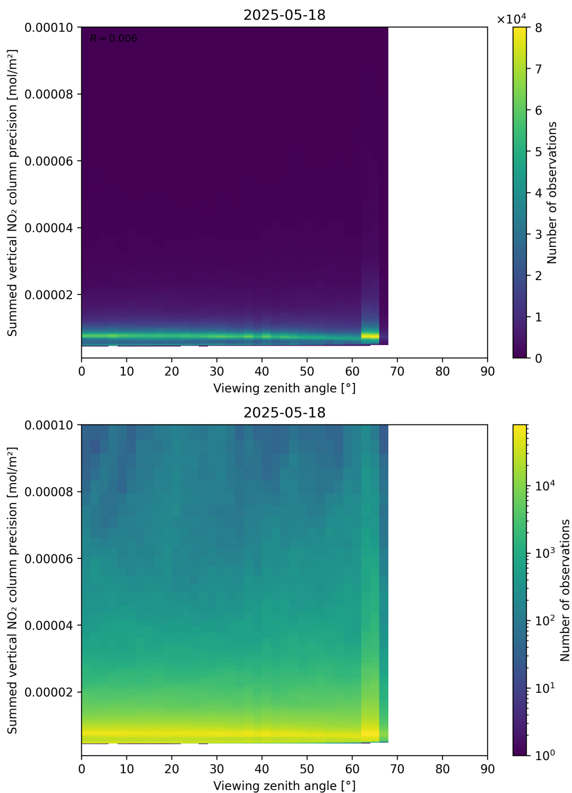
Figure 166: Scatter density plot of “Viewing zenith angle” against “Summed vertical NO 2 column precision” for 2025-05-17 to 2025-05-19.
