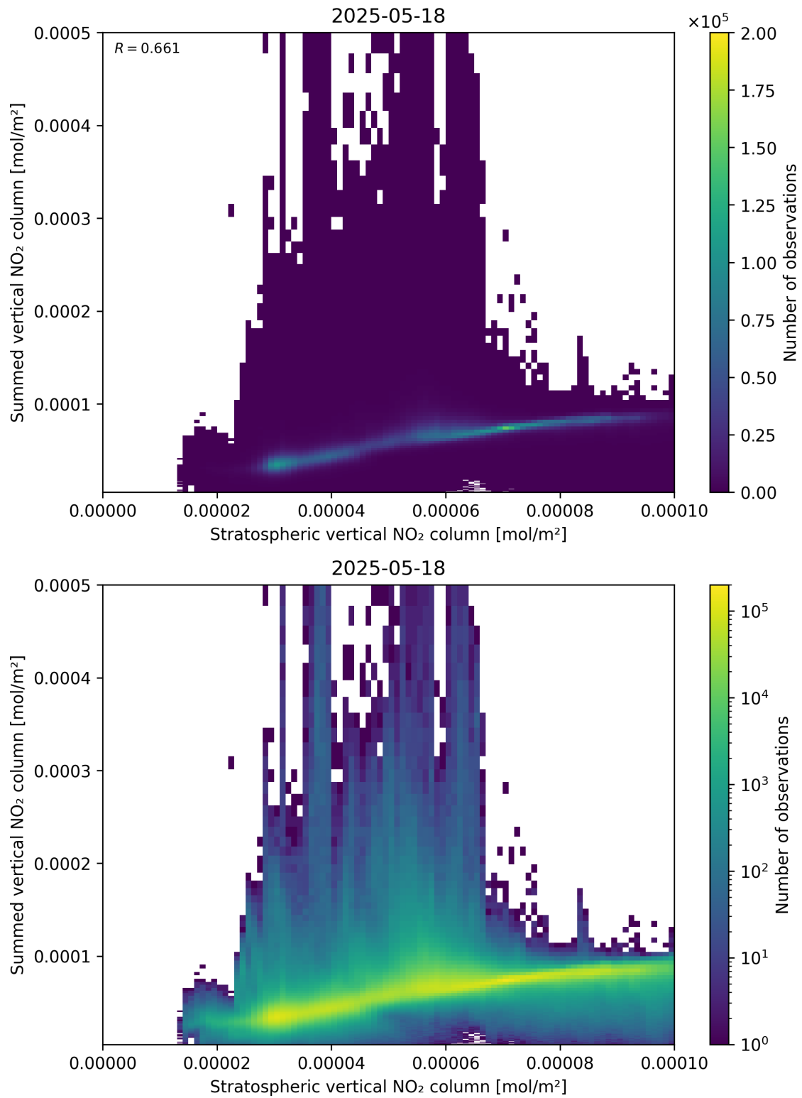
Figure 98: Scatter density plot of “Stratospheric vertical NO 2 column” against “Summed vertical NO 2 column” for 2025-05-17 to 2025-05-19.
