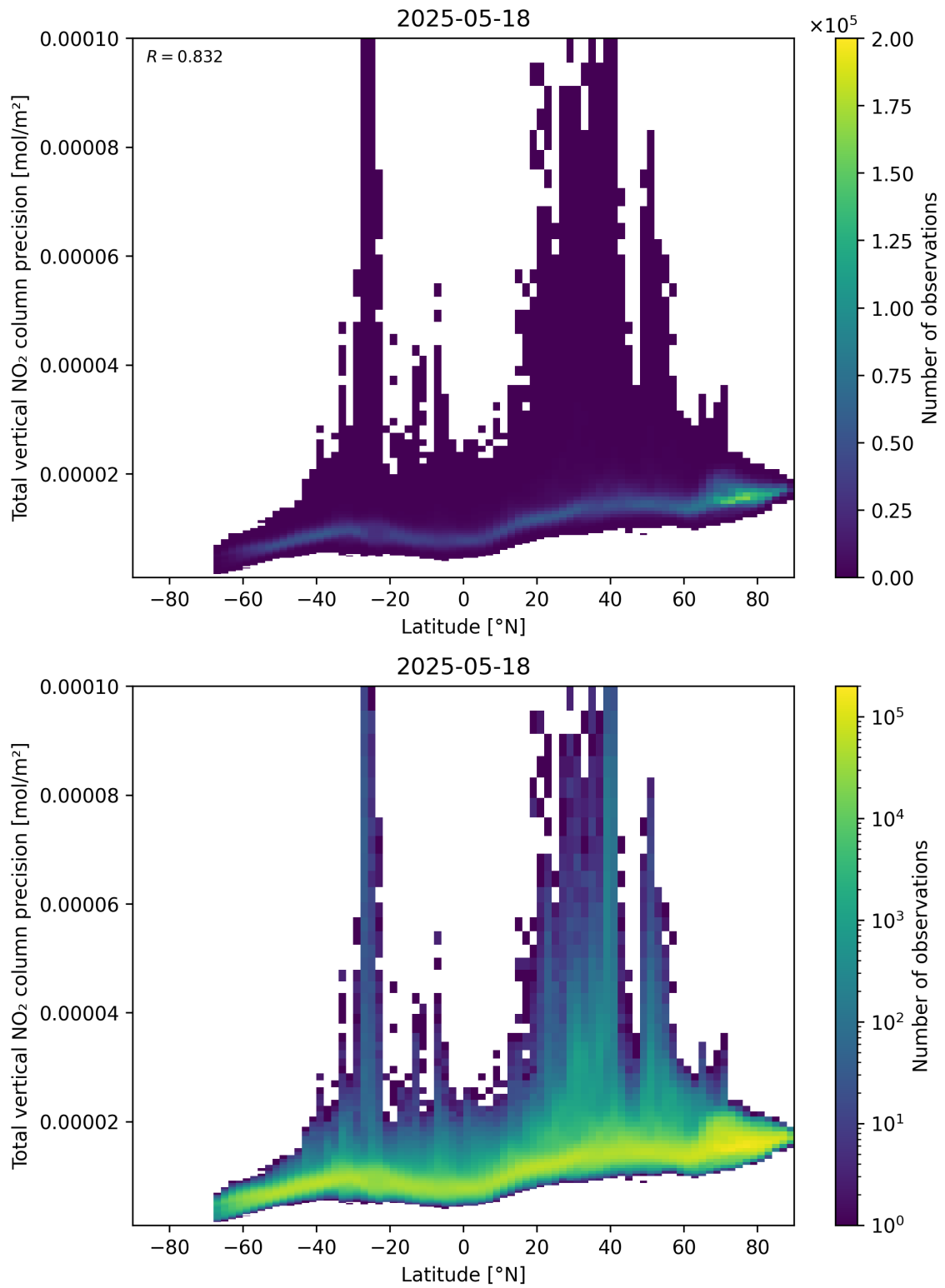
Figure 91: Scatter density plot of “Latitude” against “Total vertical NO 2 column precision” for 2025-05-17 to 2025-05-19.
