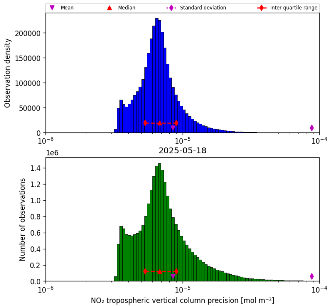
Figure 30: Histogram of “NO 2 tropospheric vertical column precision” for 2025-05-17 to 2025-05-19
