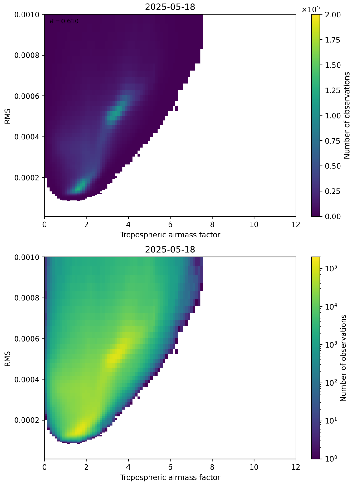
Figure 79: Scatter density plot of “Tropospheric airmass factor” against “RMS” for 2025-05-17 to 2025-05-19.
