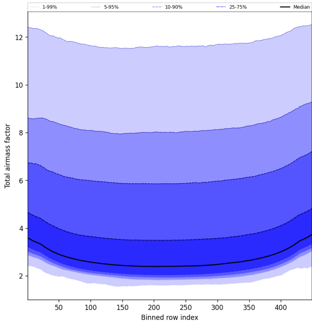
Figure 49: Along track statistics of “Total airmass factor” for 2025-05-17 to 2025-05-19
