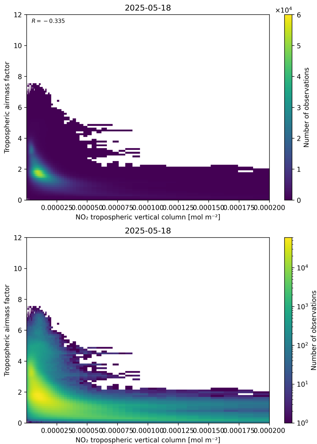
Figure 123: Scatter density plot of “NO 2 tropospheric vertical column” against “Tropospheric air mass factor” for 2025-05-17 to 2025-05-19.
