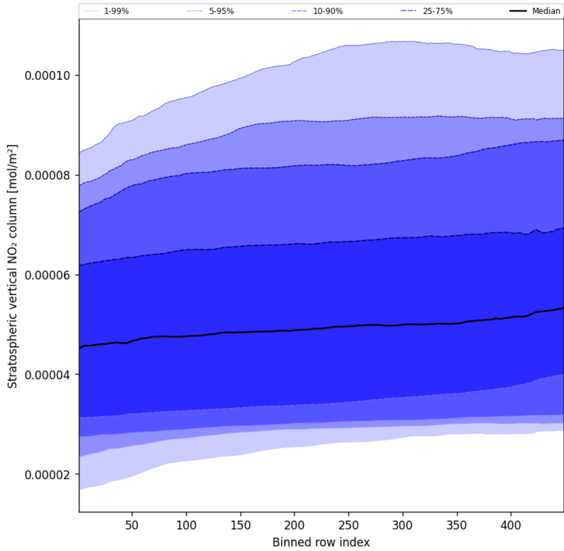
Figure 53: Along track statistics of “Stratospheric vertical NO 2 column” for 2025-05-17 to 2025-05-19
