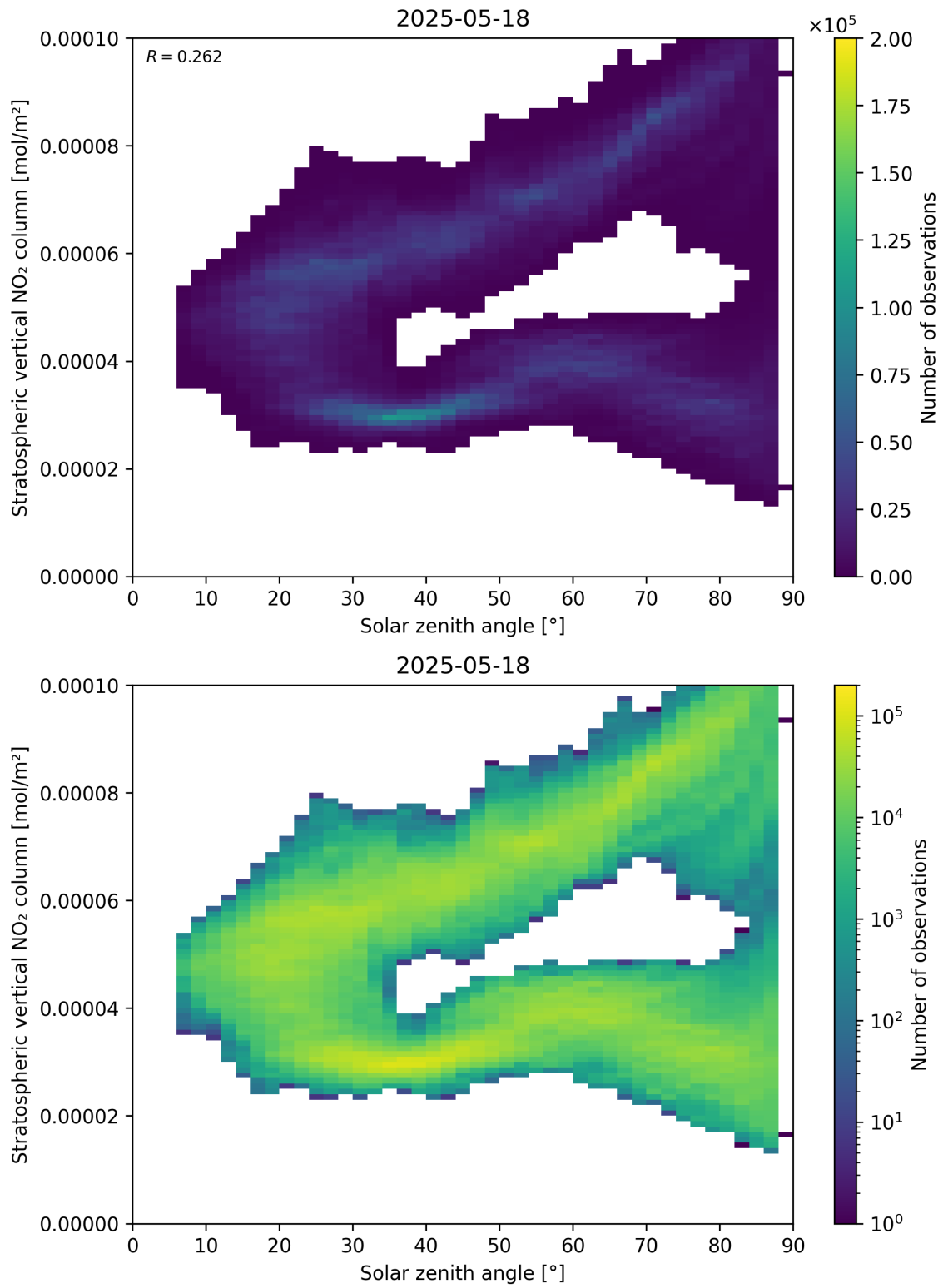
Figure 150: Scatter density plot of “Solar zenith angle” against “Stratospheric vertical NO 2 column” for 2025-05-17 to 2025-05-19.
