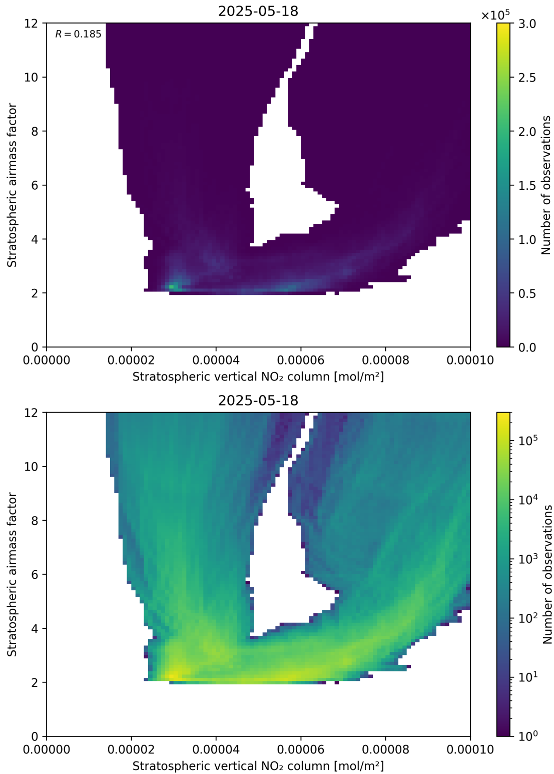
Figure 96: Scatter density plot of “Stratospheric vertical NO 2 column” against “Stratospheric airmass factor” for 2025-05-17 to 2025-05-19.
