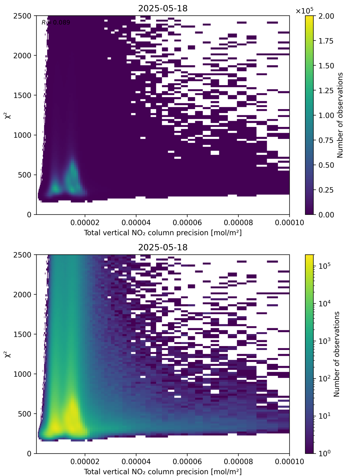
Figure 116: Scatter density plot of “Total vertical NO 2 column precision” against “ \chi^2 ” for 2025-05-17 to 2025-05-19.
