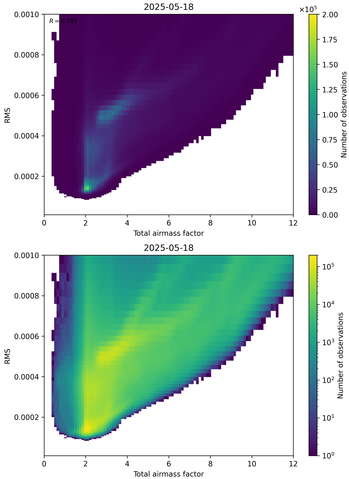
Figure 69: Scatter density plot of “Total airmass factor” against “RMS” for 2025-05-17 to 2025-05-19.
