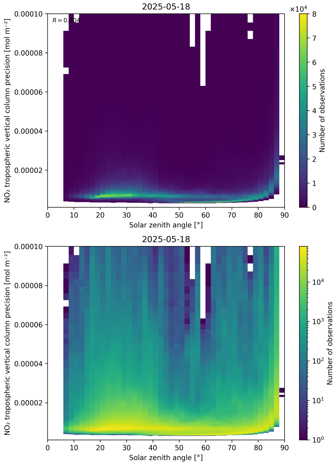
Figure 156: Scatter density plot of “Solar zenith angle” against “NO 2 tropospheric vertical column precision” for 2025-05-17 to 2025-05-19.
