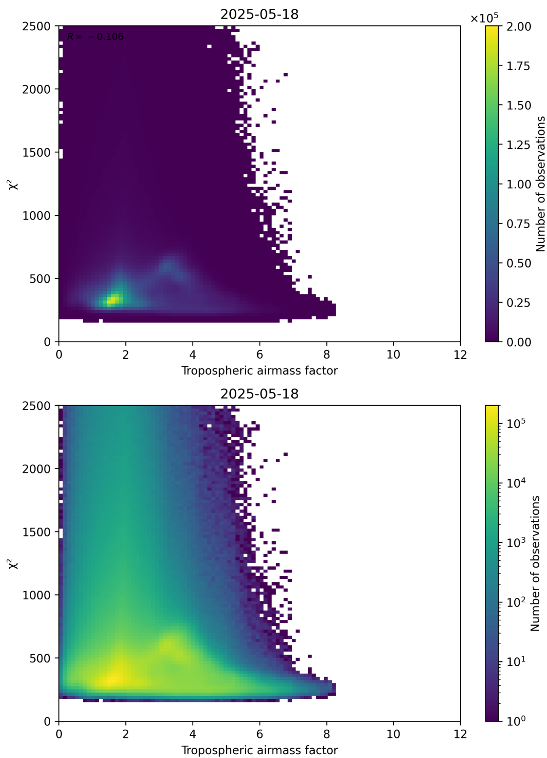
Figure 73: Scatter density plot of “Tropospheric airmass factor” against “ \chi^2 ” for 2025-05-17 to 2025-05-19.
