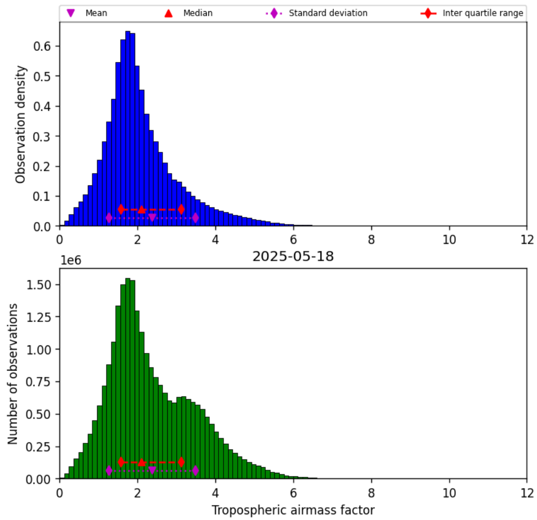
Figure 31: Histogram of “Tropospheric airmass factor” for 2025-05-17 to 2025-05-19
