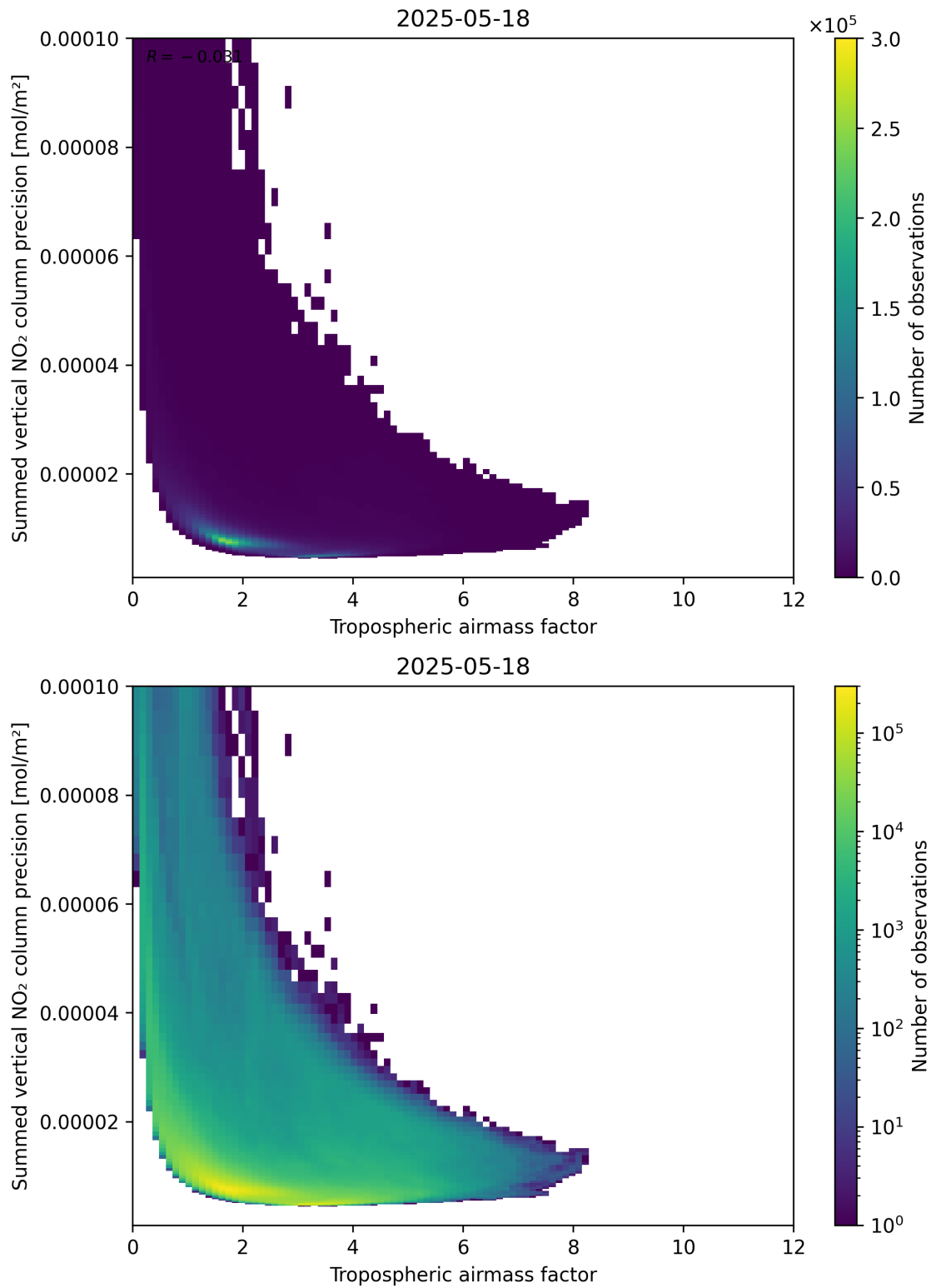
Figure 76: Scatter density plot of “Tropospheric air mass factor” against “Summed vertical NO 2 column precision” for 2025-05-17 to 2025-05-19.
