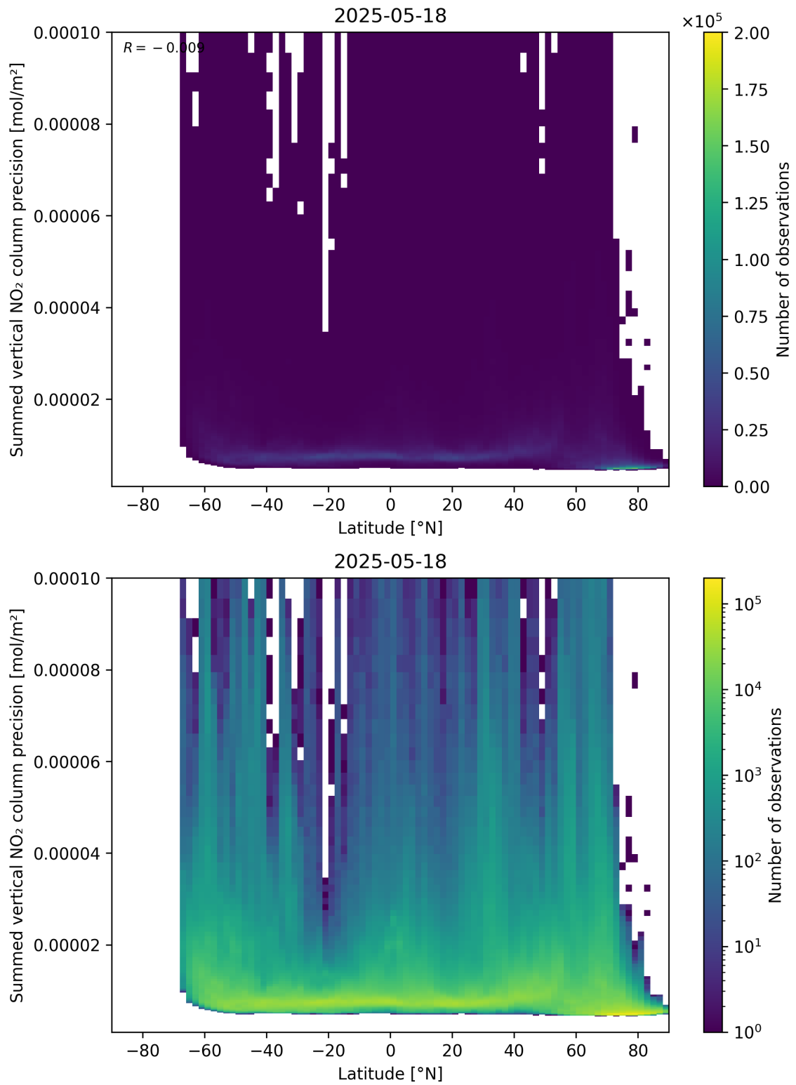
Figure 89: Scatter density plot of “Latitude” against “Summed vertical NO 2 column precision” for 2025-05-17 to 2025-05-19.
