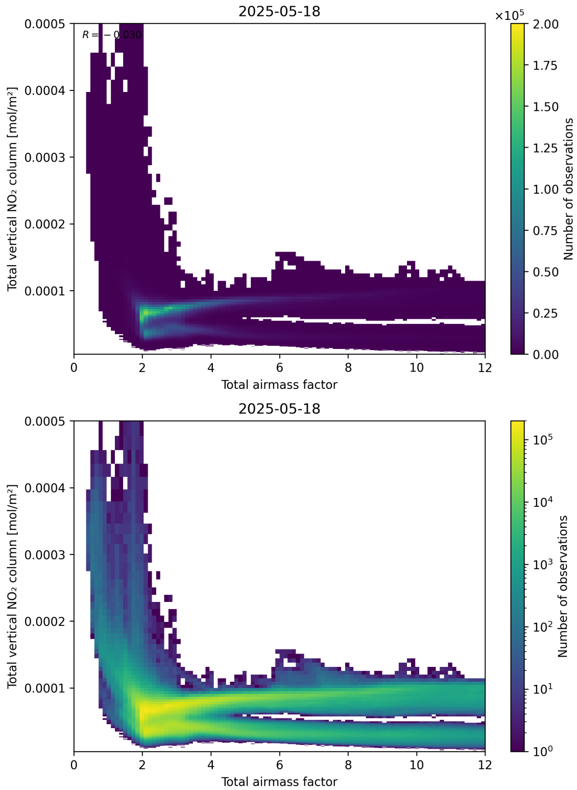
Figure 67: Scatter density plot of “Total airmass factor” against “Total vertical NO 2 column” for 2025-05-17 to 2025-05-19.
