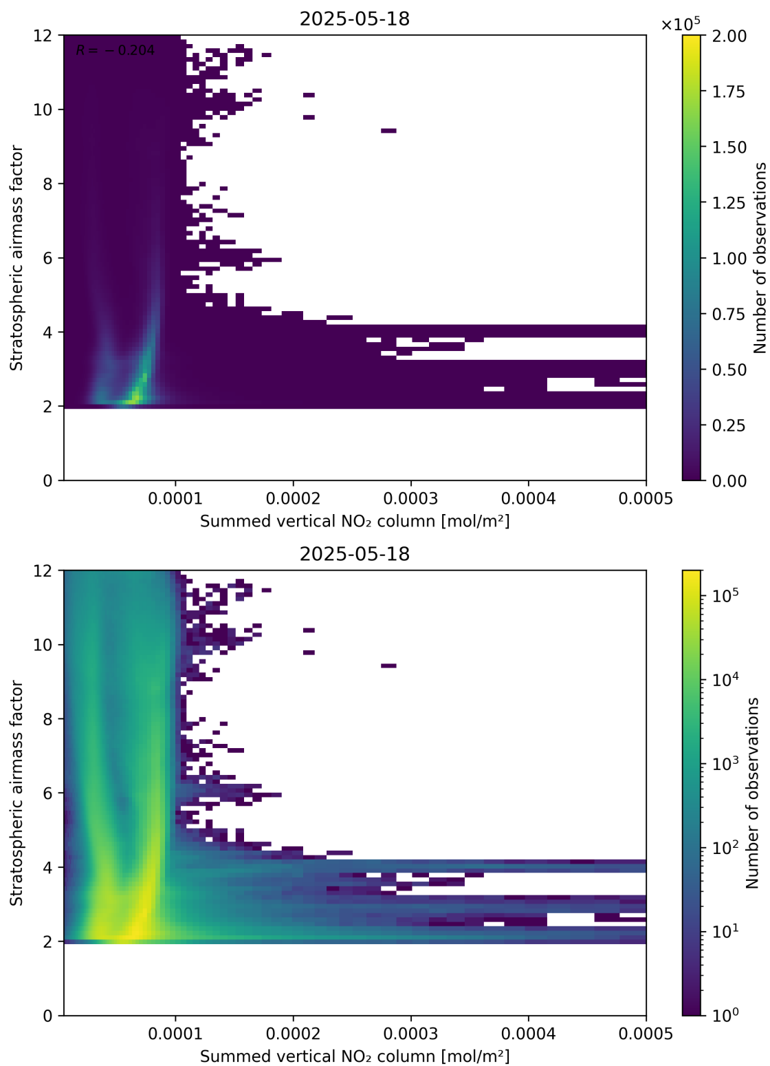
Figure 103: Scatter density plot of “Summed vertical NO 2 column” against “Stratospheric air mass factor” for 2025-05-17 to 2025-05-19.
