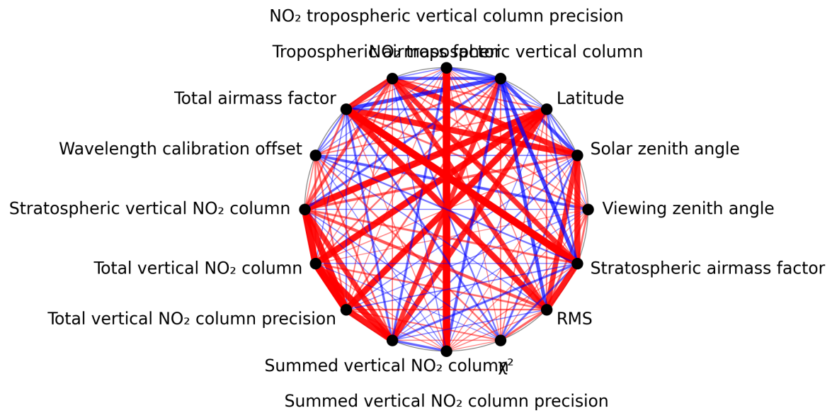
Figure 1: Map of correlation graph for 2025-05-17 to 2025-05-19.
