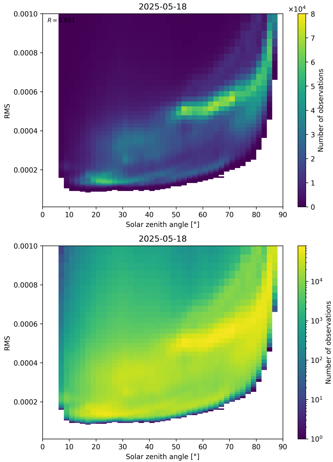
Figure 157: Scatter density plot of “Solar zenith angle” against “RMS” for 2025-05-17 to 2025-05-19.
