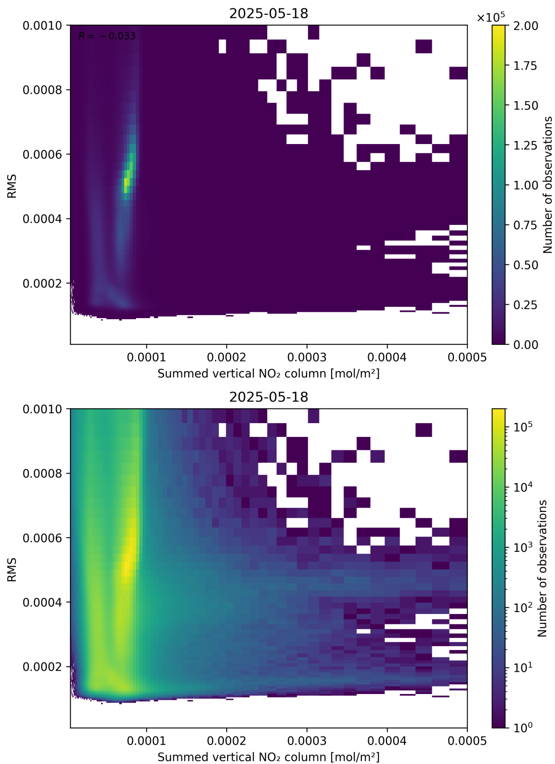
Figure 109: Scatter density plot of “Summed vertical NO 2 column” against “RMS” for 2025-05-17 to 2025-05-19.
