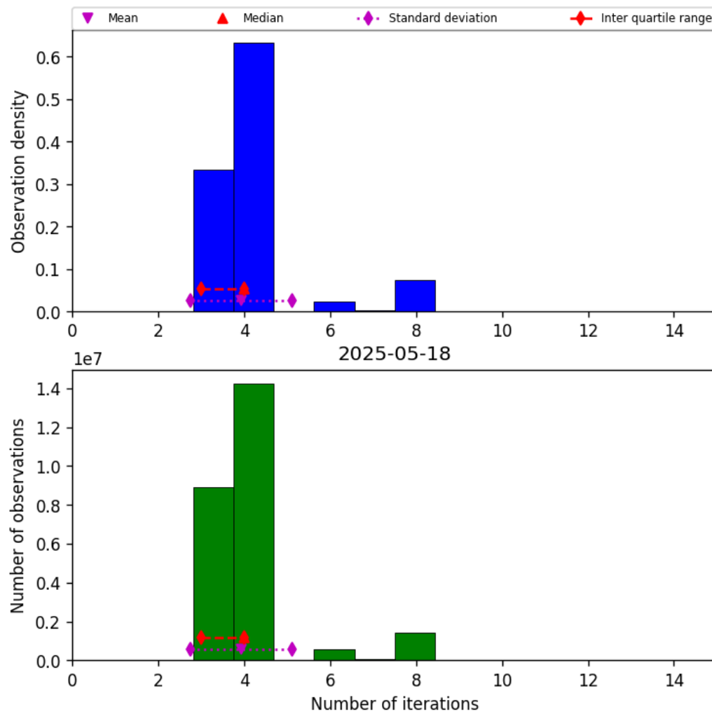
Figure 34: Histogram of “Number of iterations” for 2025-05-17 to 2025-05-19
