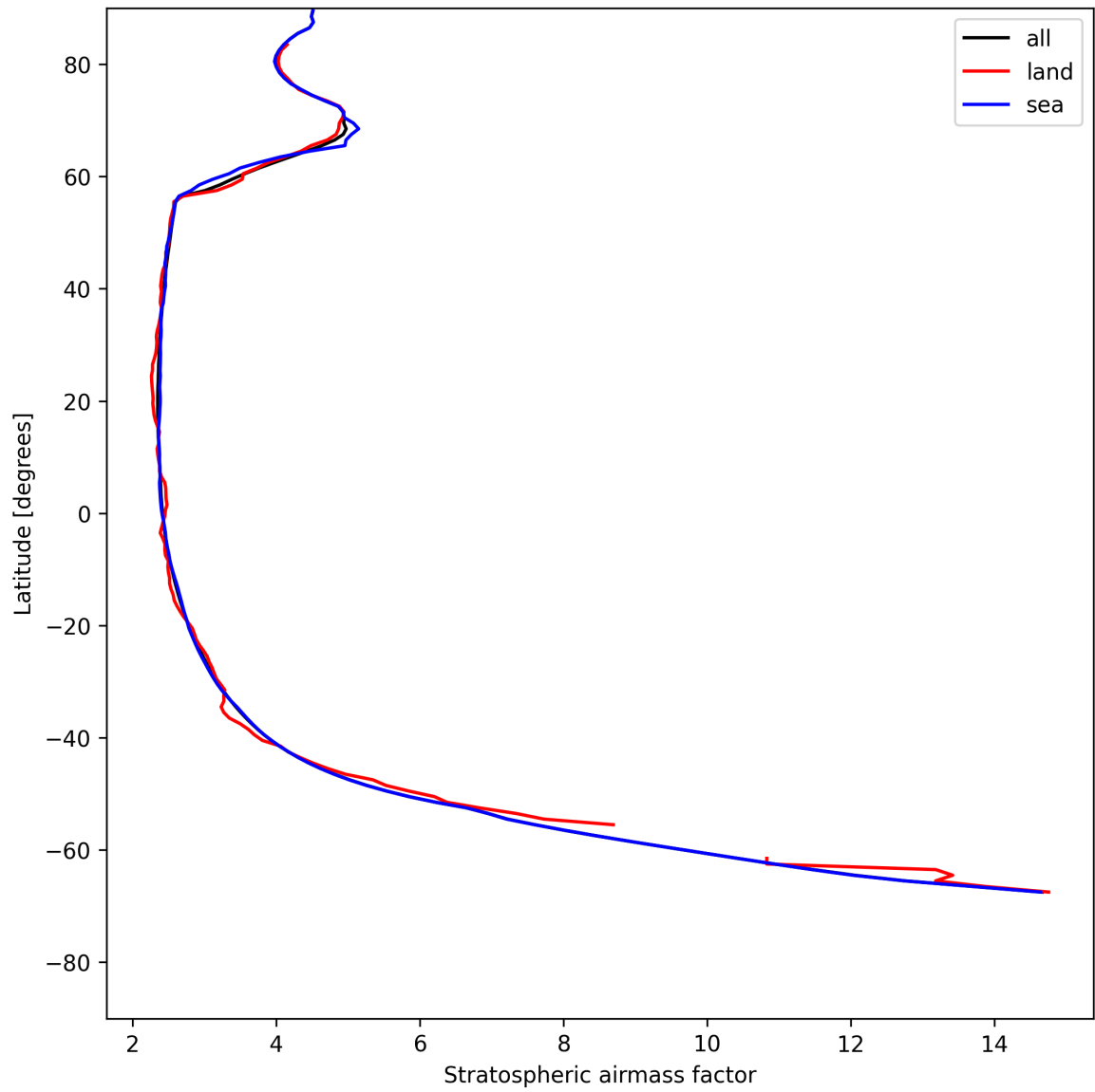
Figure 27: Zonal average of “Stratospheric air mass factor” for 2025-05-17 to 2025-05-19.
