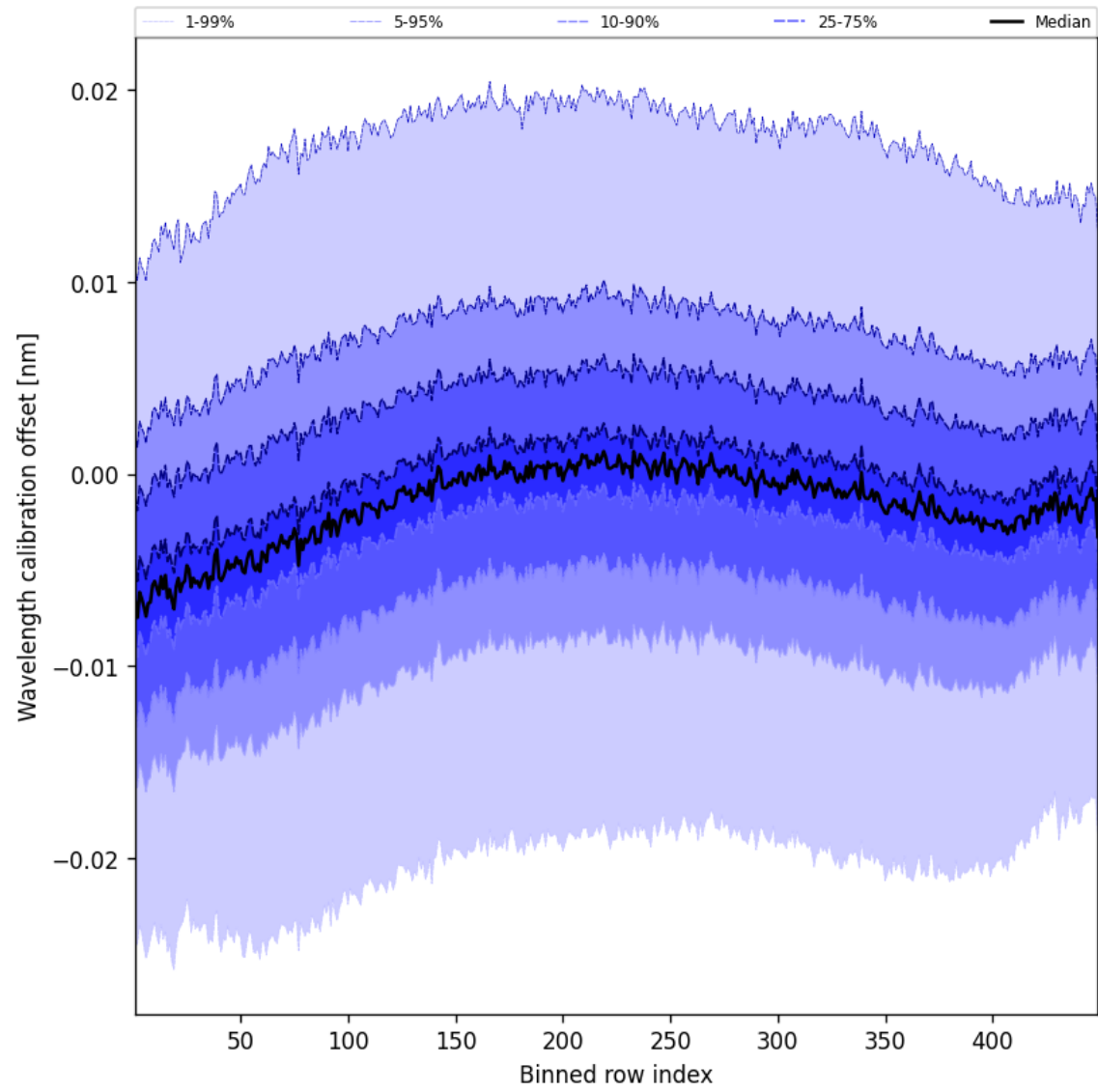
Figure 52: Along track statistics of “Wavelength calibration offset” for 2025-05-17 to 2025-05-19
