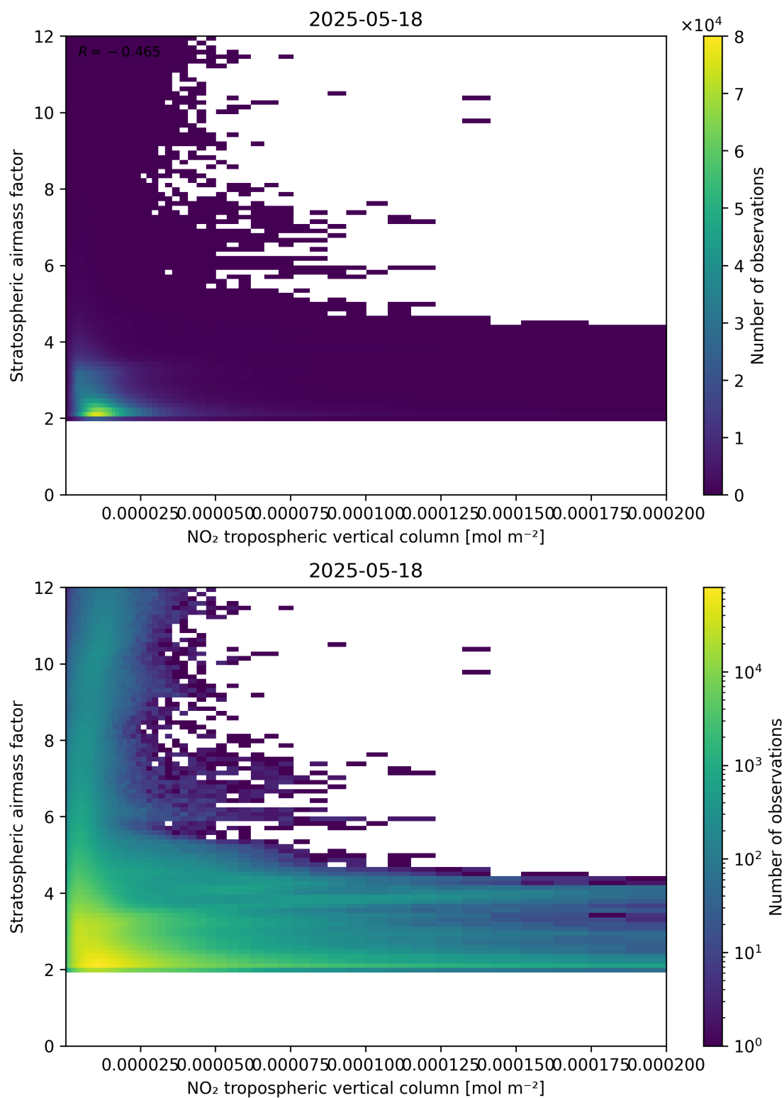
Figure 121: Scatter density plot of “NO 2 tropospheric vertical column” against “Stratospheric air mass factor” for 2025-05-17 to 2025-05-19.
