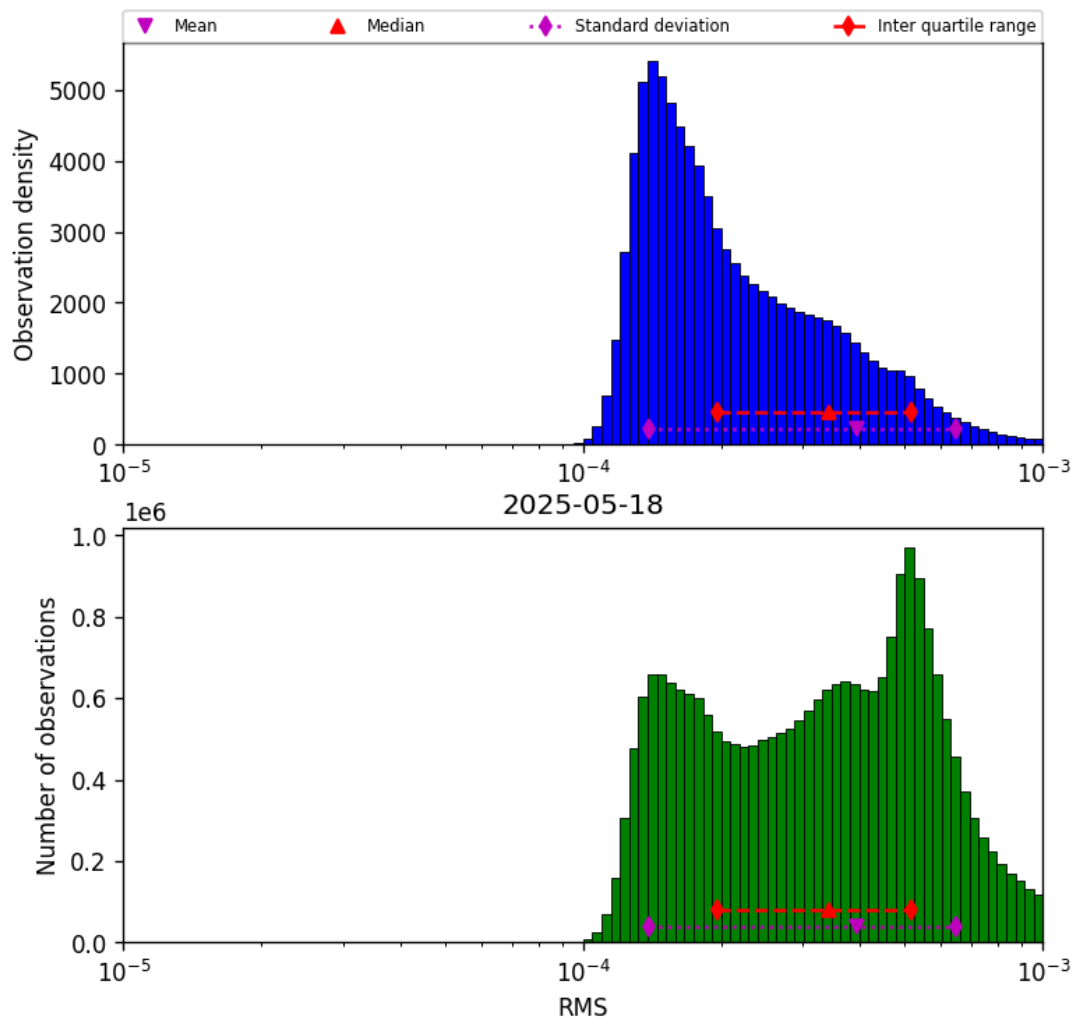
Figure 43: Histogram of “RMS” for 2025-05-17 to 2025-05-19
