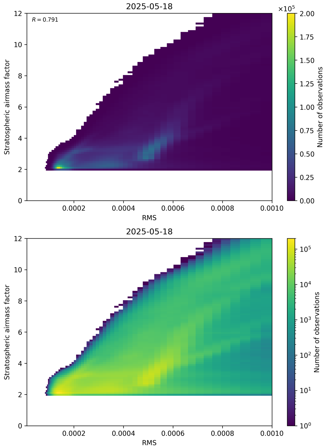
Figure 144: Scatter density plot of “RMS” against “Stratospheric airmass factor” for 2025-05-17 to 2025-05-19.
