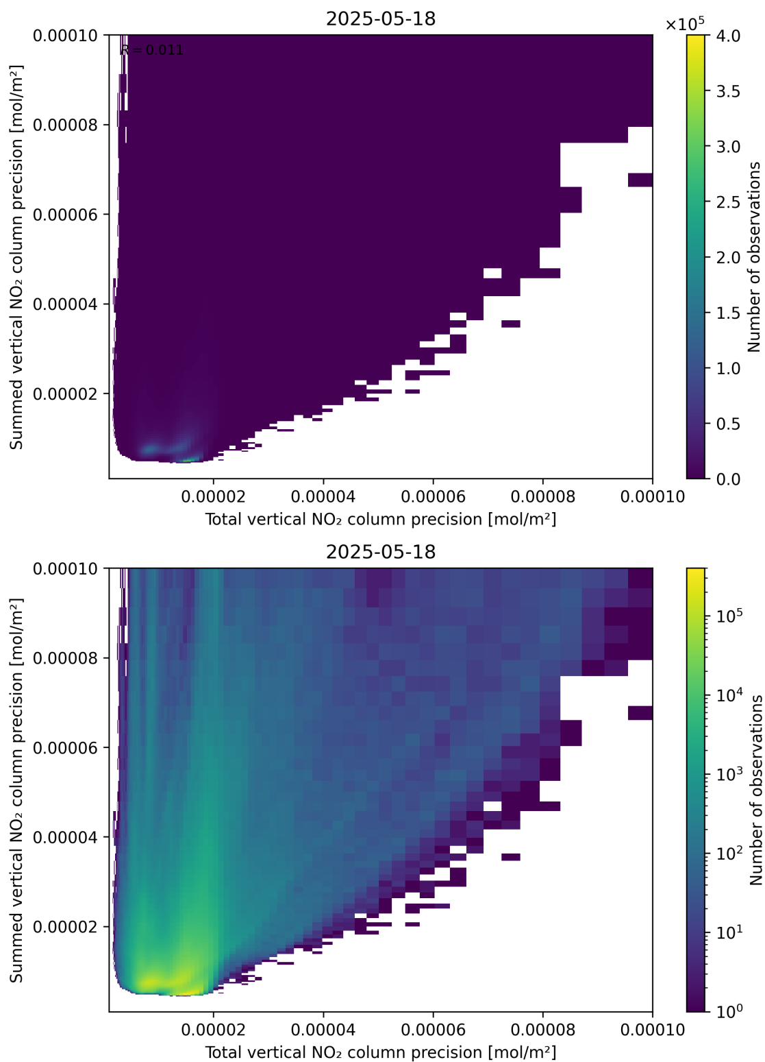
Figure 118: Scatter density plot of “Total vertical NO 2 column precision” against “Summed vertical NO 2 column precision” for 2025-05-17 to 2025-05-19.
