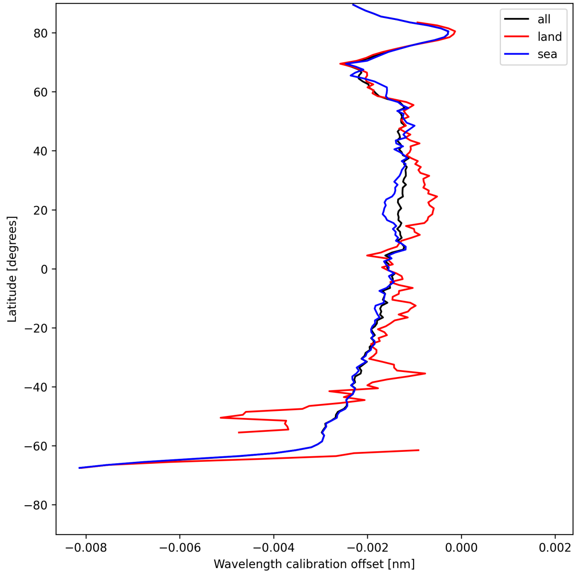
Figure 18: Zonal average of “Wavelength calibration offset” for 2025-05-17 to 2025-05-19.
