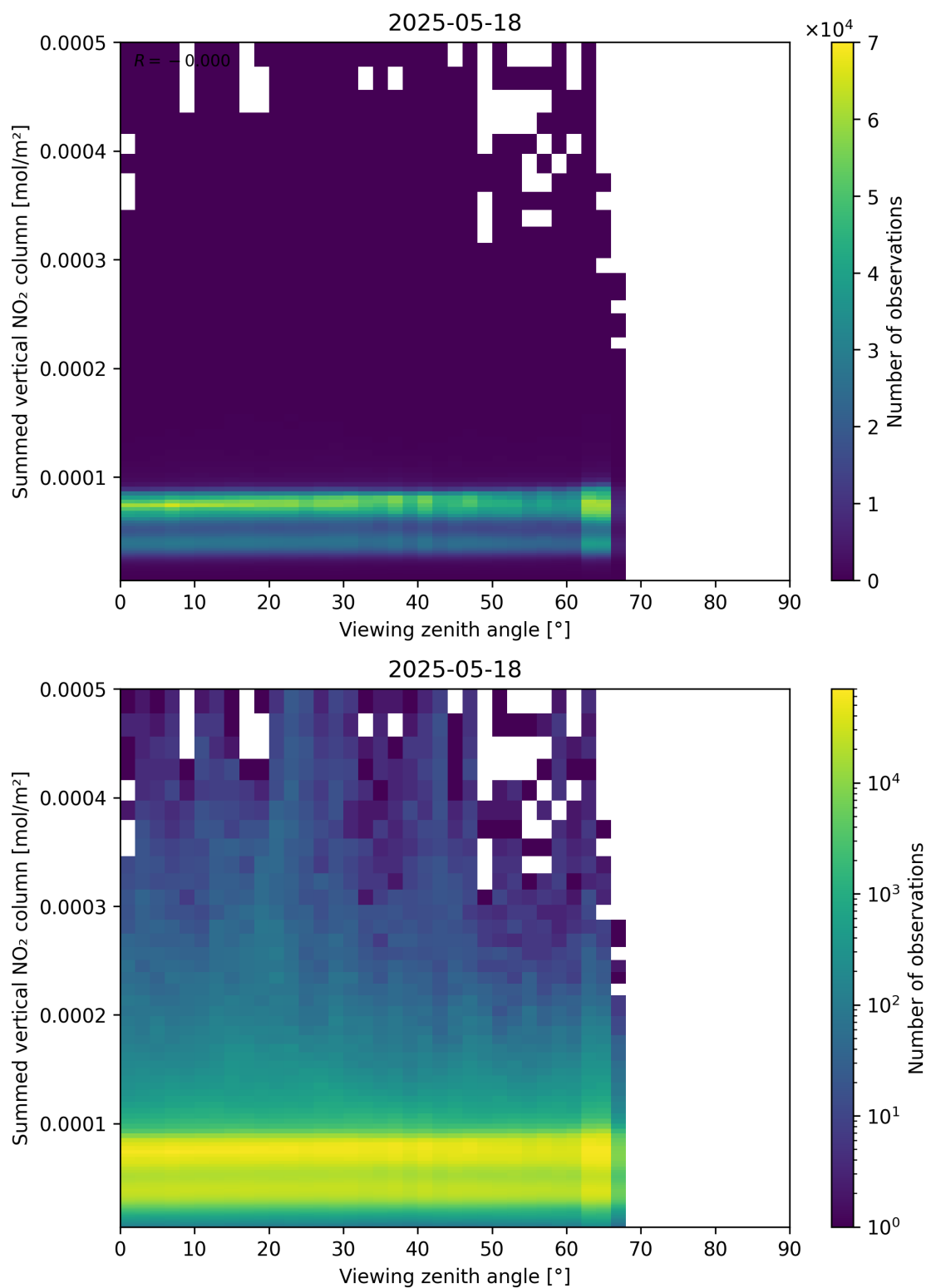
Figure 165: Scatter density plot of “Viewing zenith angle” against “Summed vertical NO 2 column” for 2025-05-17 to 2025-05-19.
