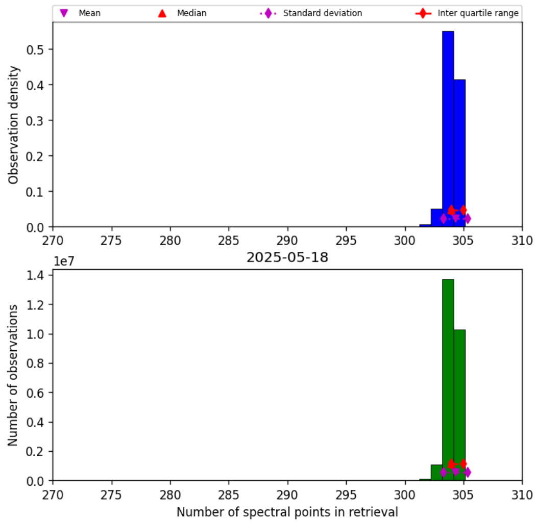
Figure 33: Histogram of “Number of spectral points in retrieval” for 2025-05-17 to 2025-05-19
