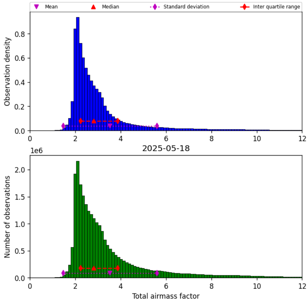
Figure 32: Histogram of “Total airmass factor” for 2025-05-17 to 2025-05-19
