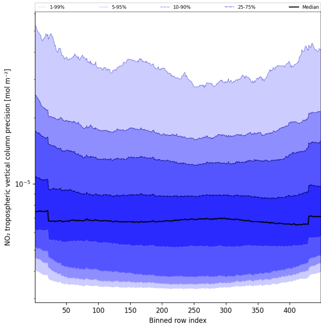
Figure 47: Along track statistics of “NO 2 tropospheric vertical column precision” for 2025-05-17 to 2025-05-19
