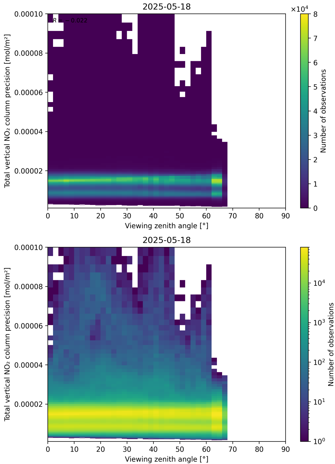
Figure 168: Scatter density plot of “Viewing zenith angle” against “Total vertical NO 2 column precision” for 2025-05-17 to 2025-05-19.
