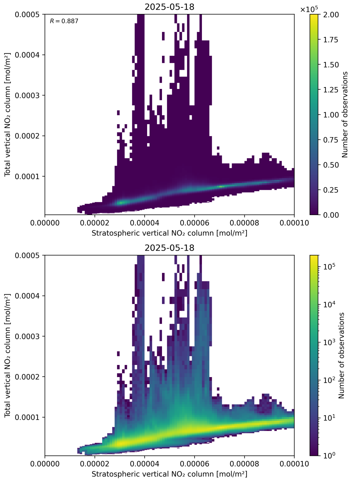
Figure 100: Scatter density plot of “Stratospheric vertical NO 2 column” against “Total vertical NO 2 column” for 2025-05-17 to 2025-05-19.
