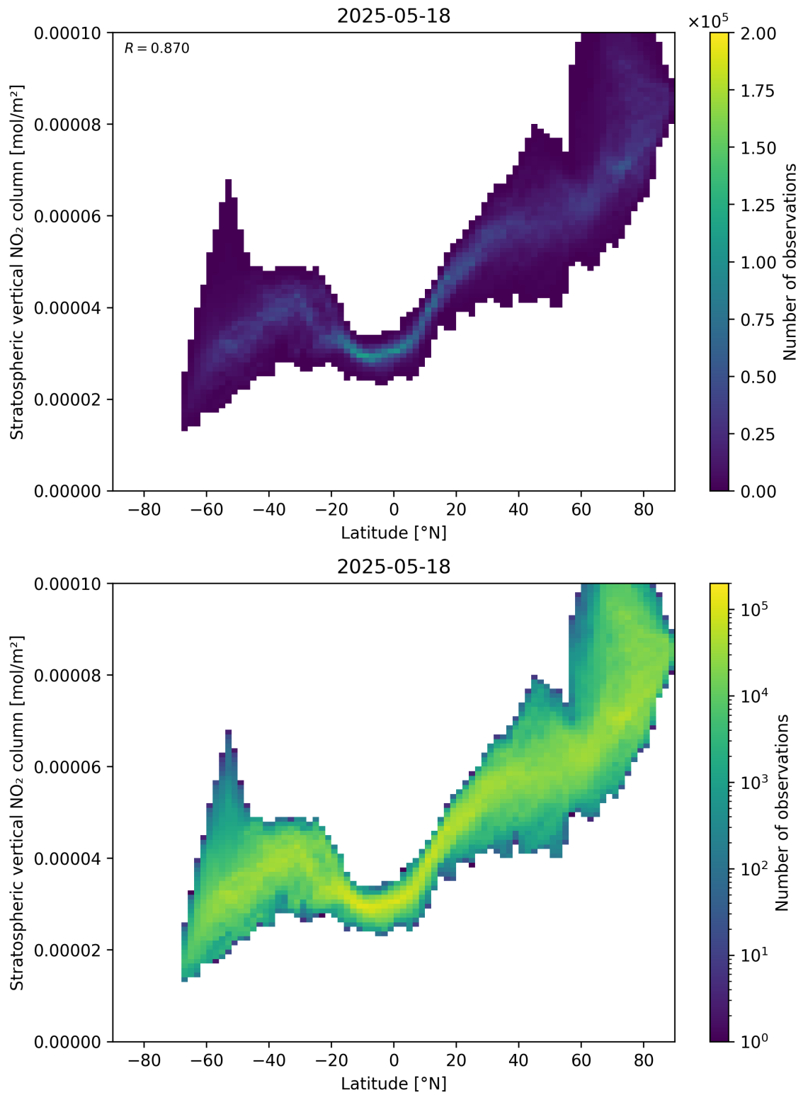
Figure 87: Scatter density plot of “Latitude” against “Stratospheric vertical \text{NO}_2 column” for 2025-05-17 to 2025-05-19.
