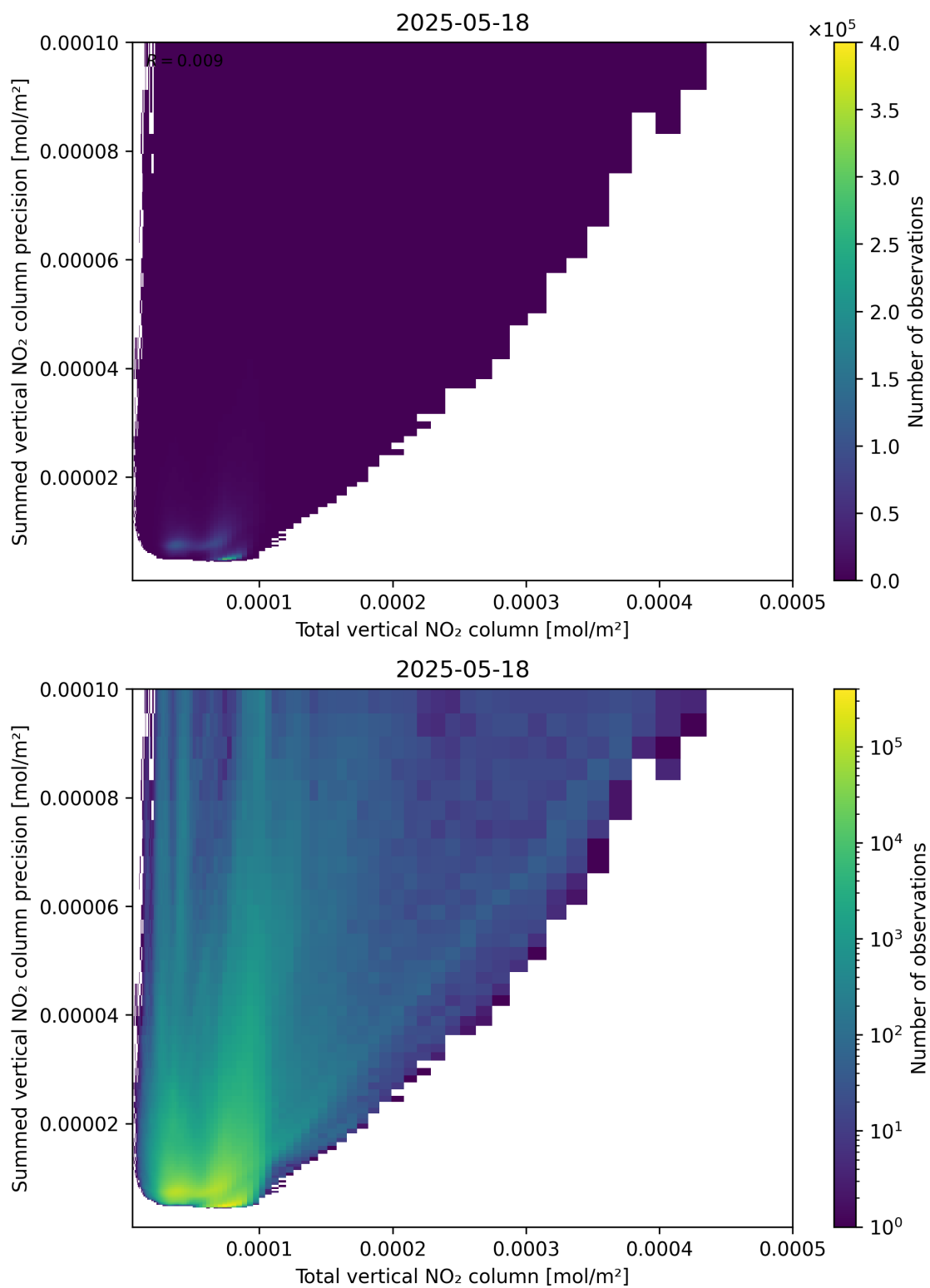
Figure 113: Scatter density plot of “Total vertical NO 2 column” against “Summed vertical NO 2 column precision” for 2025-05-17 to 2025-05-19.
