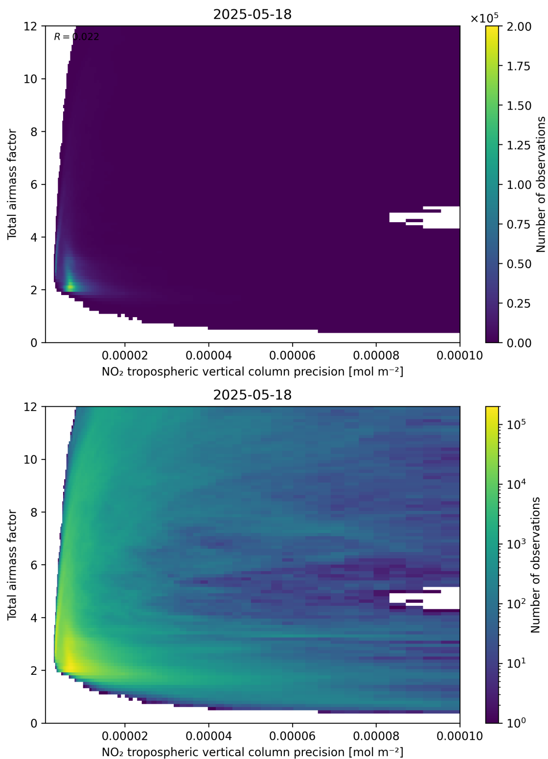
Figure 132: Scatter density plot of “NO 2 tropospheric vertical column precision” against “Total air mass factor” for 2025-05-17 to 2025-05-19.
