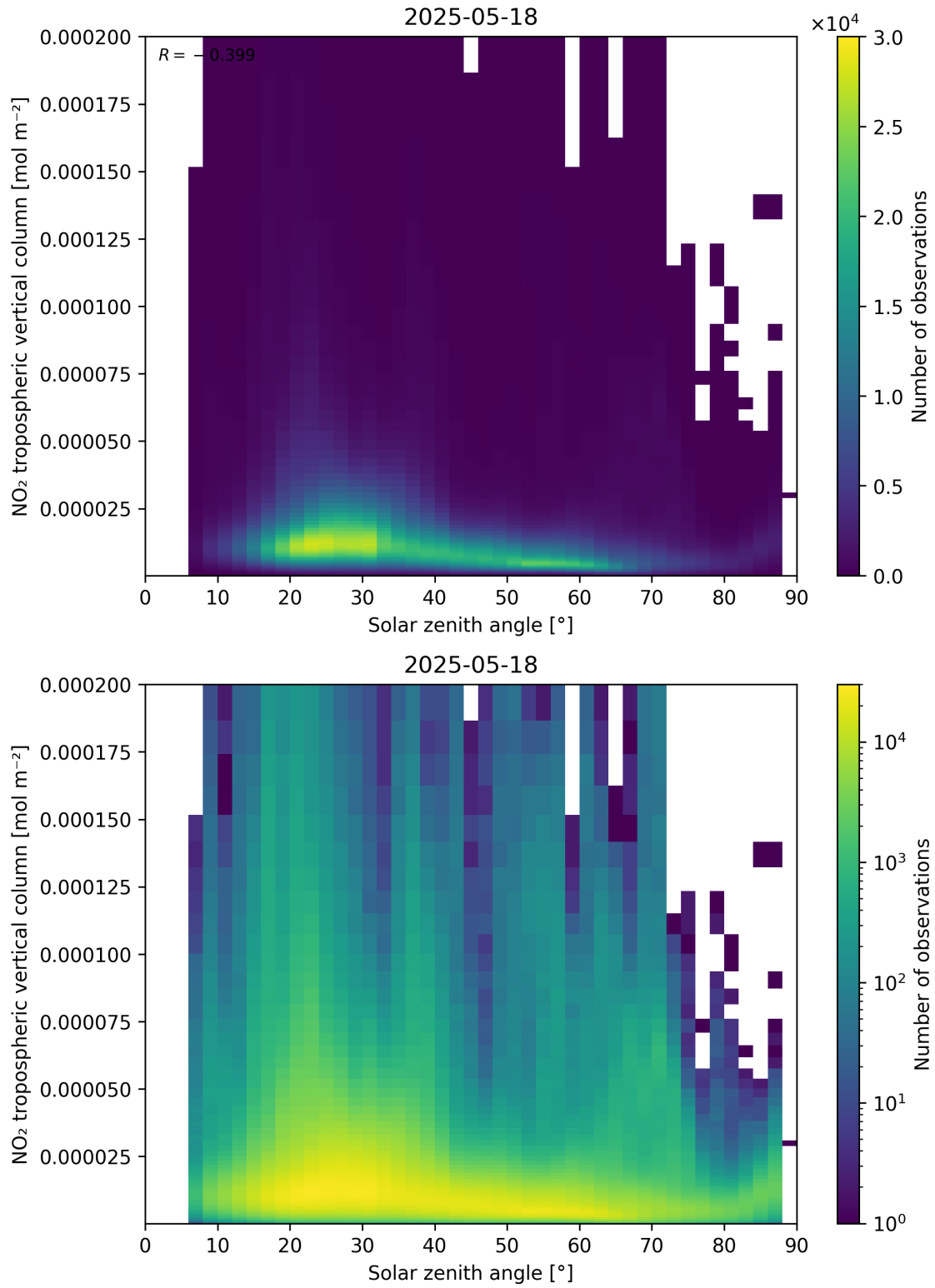
Figure 155: Scatter density plot of “Solar zenith angle” against “NO 2 tropospheric vertical column” for 2025-05-17 to 2025-05-19.
