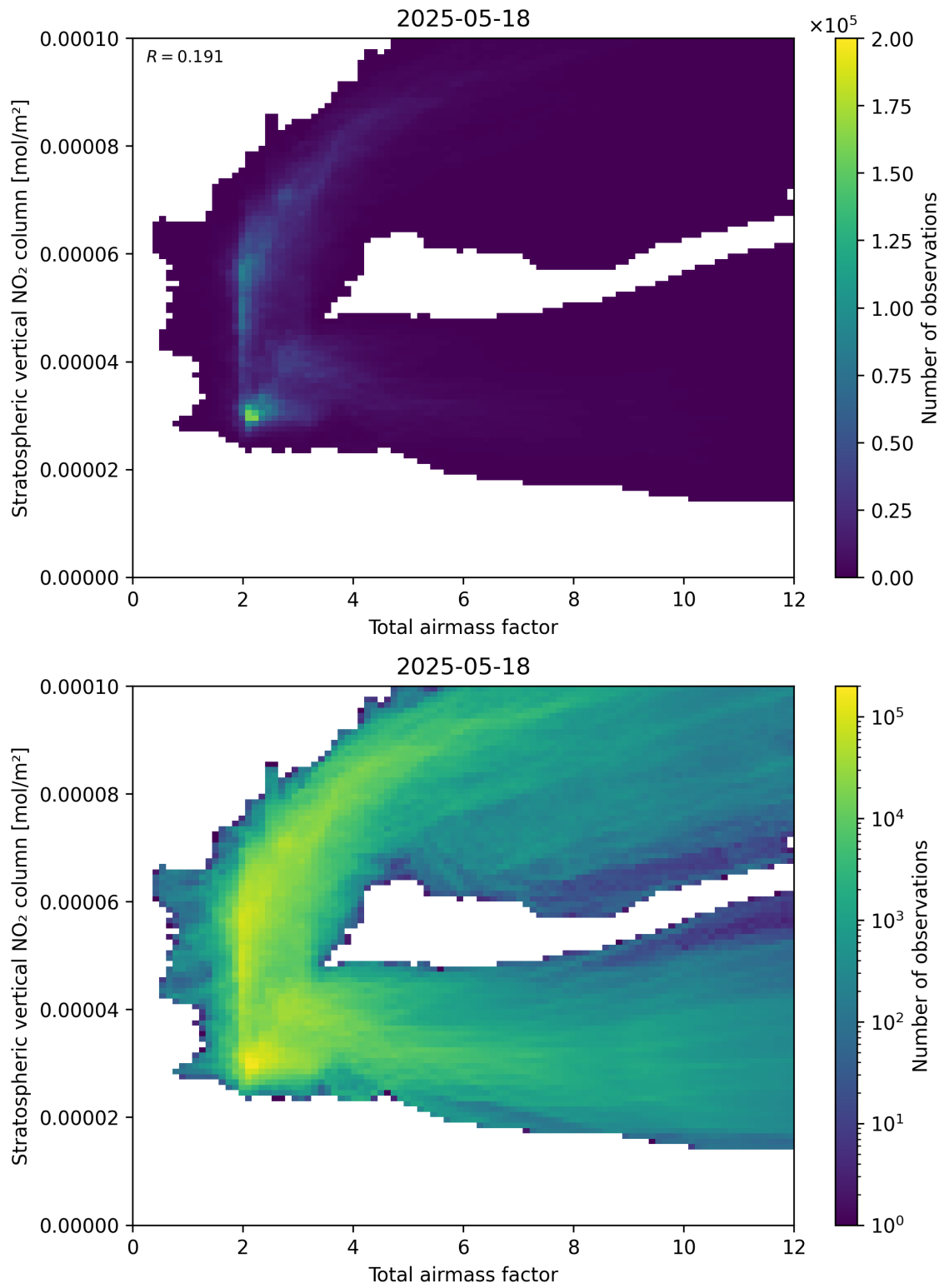
Figure 64: Scatter density plot of “Total airmass factor” against “Stratospheric vertical NO 2 column” for 2025-05-17 to 2025-05-19.
