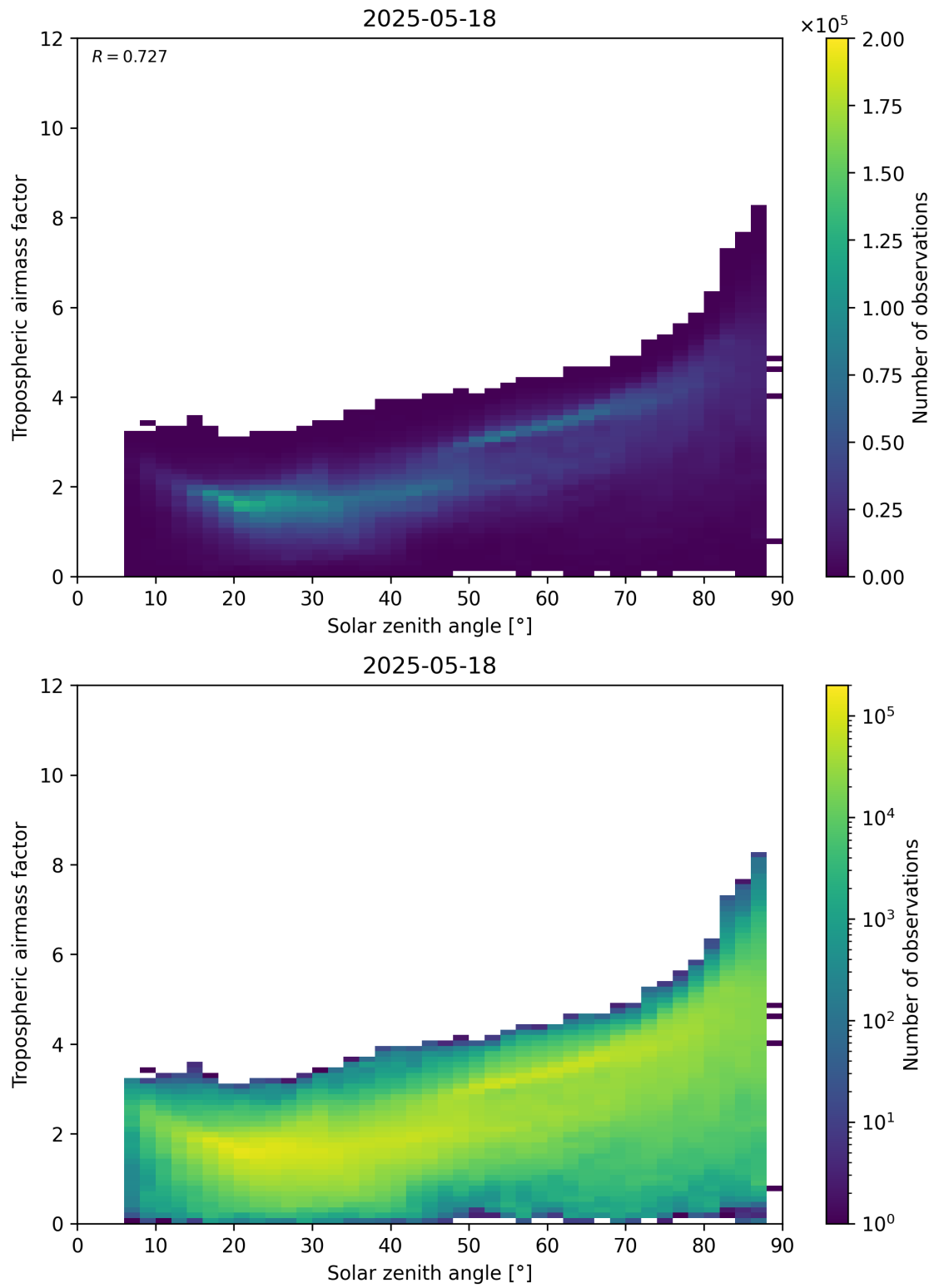
Figure 147: Scatter density plot of “Solar zenith angle” against “Tropospheric airmass factor” for 2025-05-17 to 2025-05-19.
