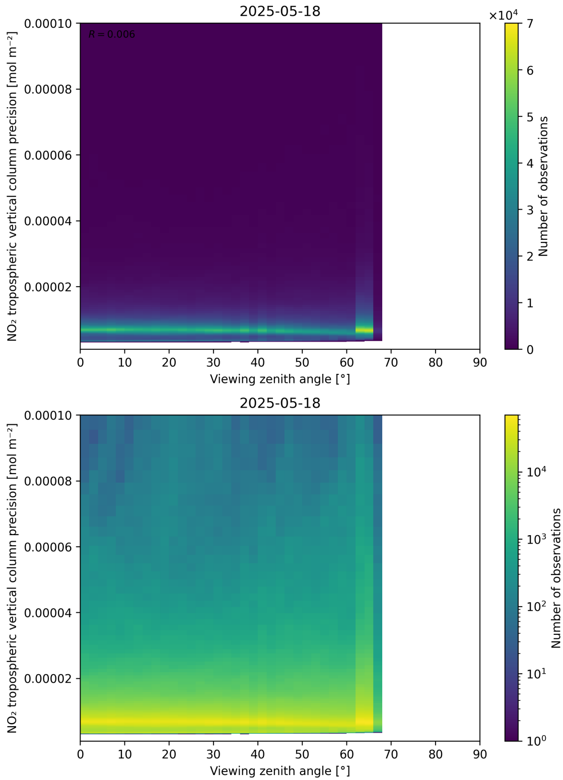
Figure 170: Scatter density plot of “Viewing zenith angle” against “NO 2 tropospheric vertical column precision” for 2025-05-17 to 2025-05-19.
