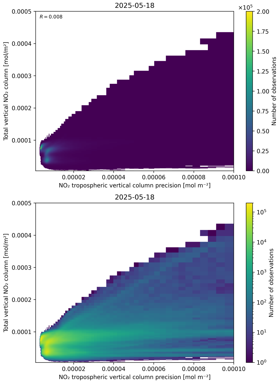
Figure 138: Scatter density plot of “NO 2 tropospheric vertical column precision” against “Total vertical NO 2 column” for 2025-05-17 to 2025-05-19.
