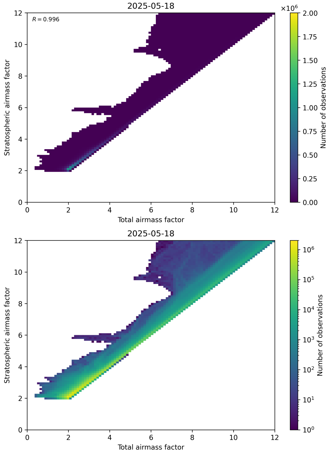
Figure 62: Scatter density plot of “Total airmass factor” against “Stratospheric airmass factor” for 2025-05-17 to 2025-05-19.
