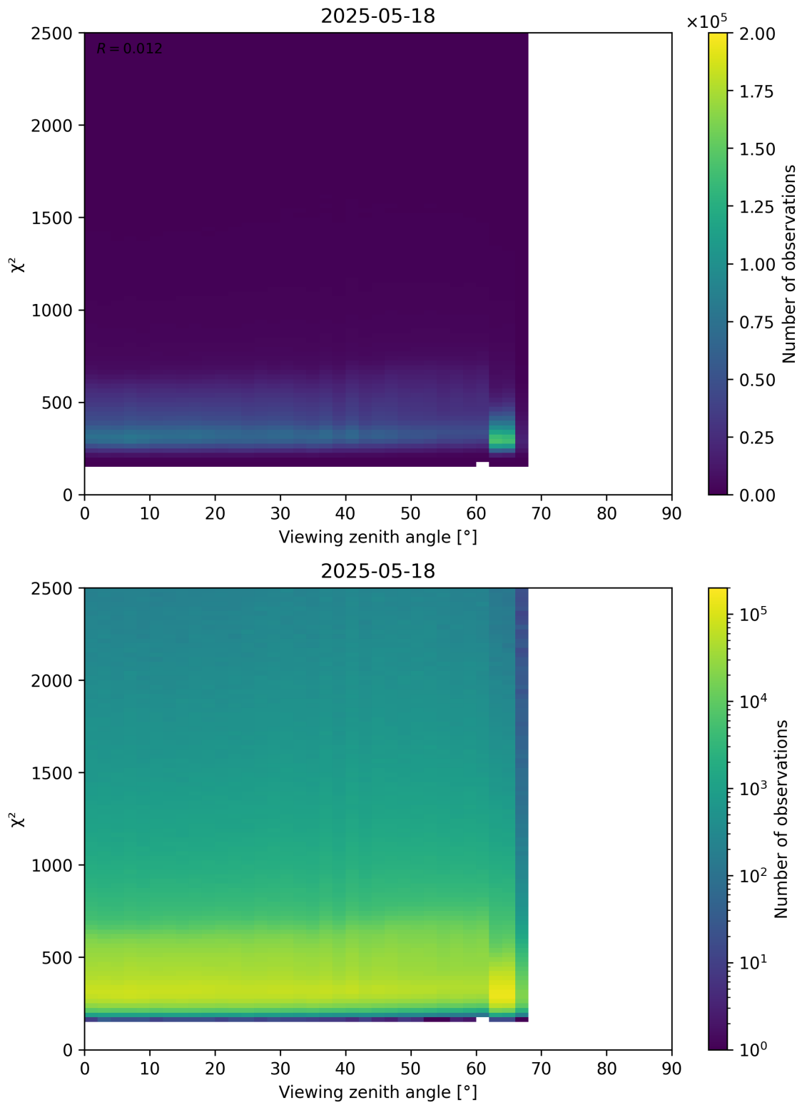
Figure 162: Scatter density plot of “Viewing zenith angle” against “ \chi^2 ” for 2025-05-17 to 2025-05-19.
