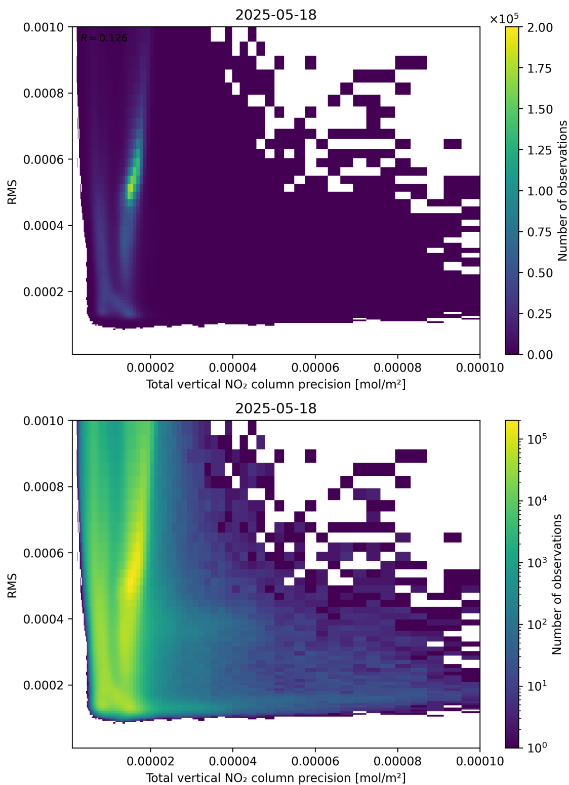
Figure 119: Scatter density plot of “Total vertical NO 2 column precision” against “RMS” for 2025-05-17 to 2025-05-19.
