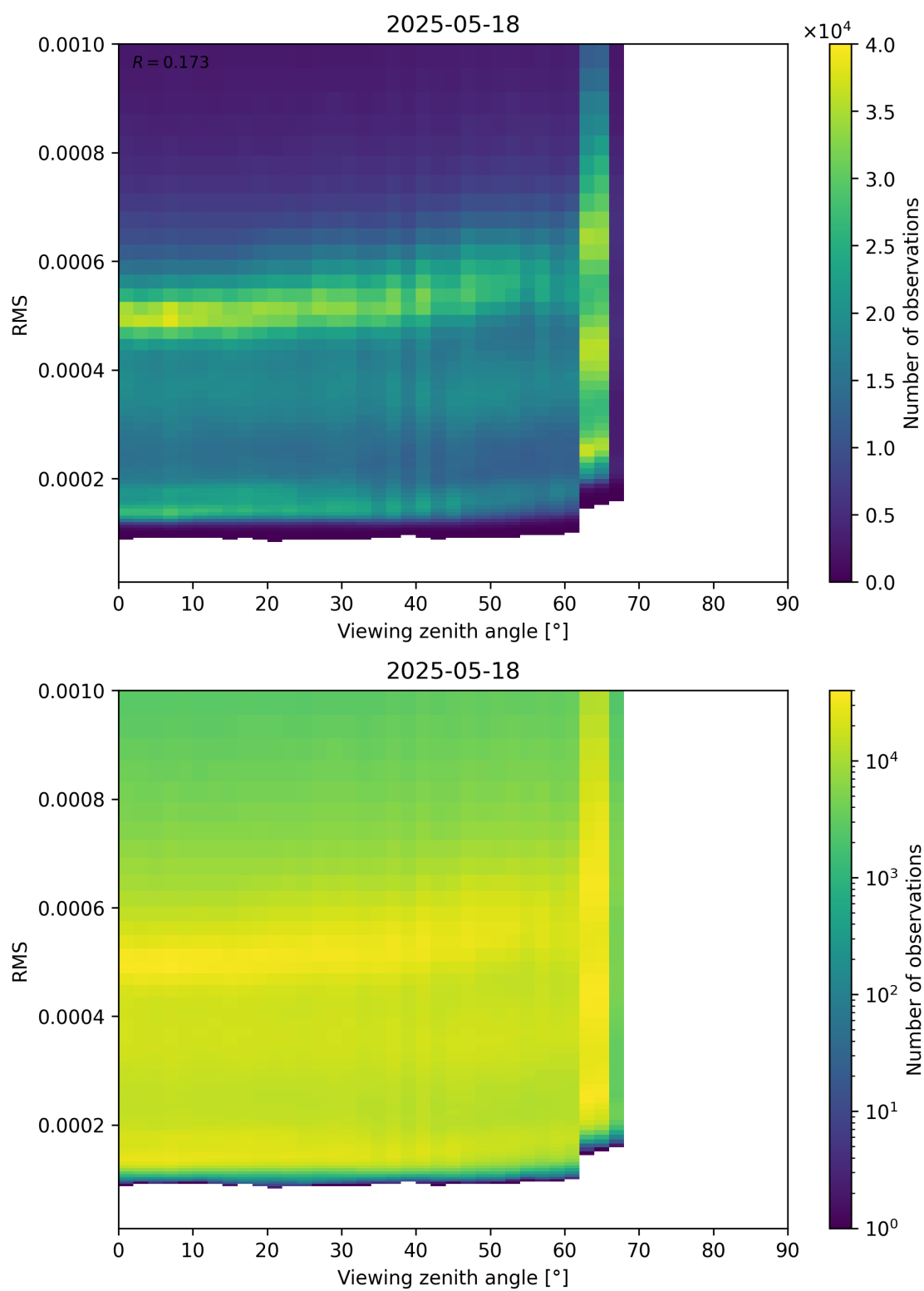
Figure 171: Scatter density plot of “Viewing zenith angle” against “RMS” for 2025-05-17 to 2025-05-19.
