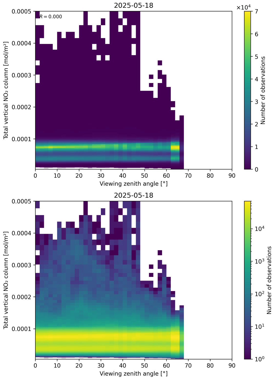
Figure 167: Scatter density plot of “Viewing zenith angle” against “Total vertical NO 2 column” for 2025-05-17 to 2025-05-19.
