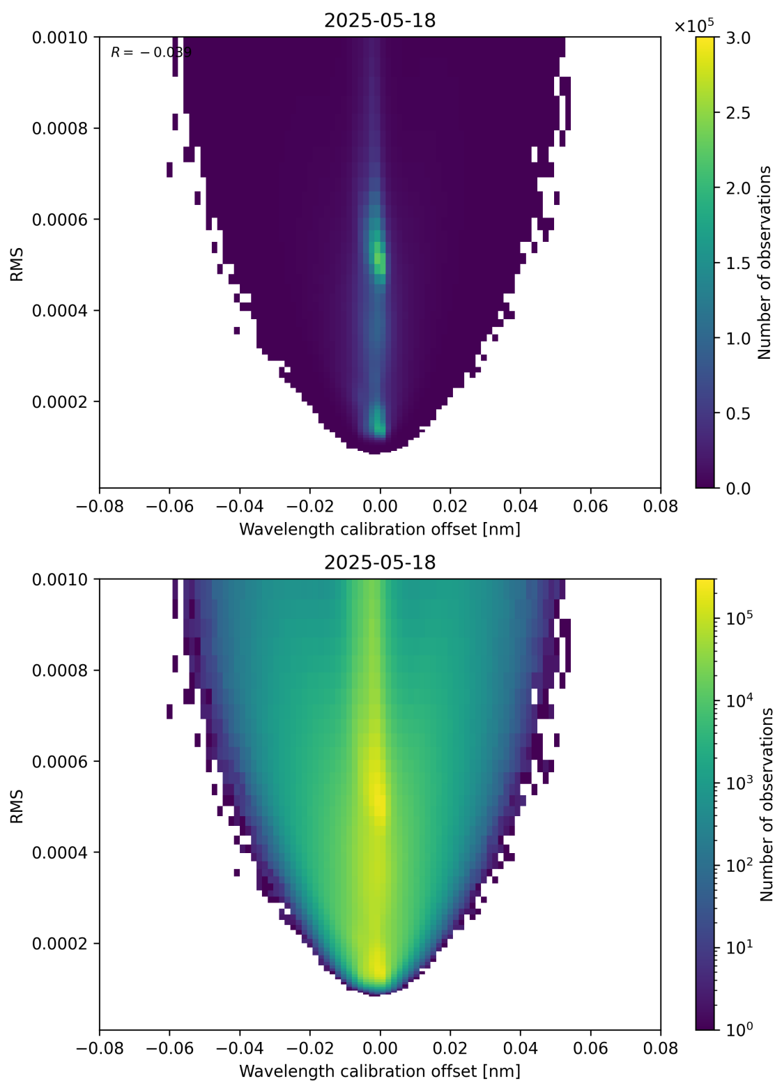
Figure 181: Scatter density plot of “Wavelength calibration offset” against “RMS” for 2025-05-17 to 2025-05-19.
