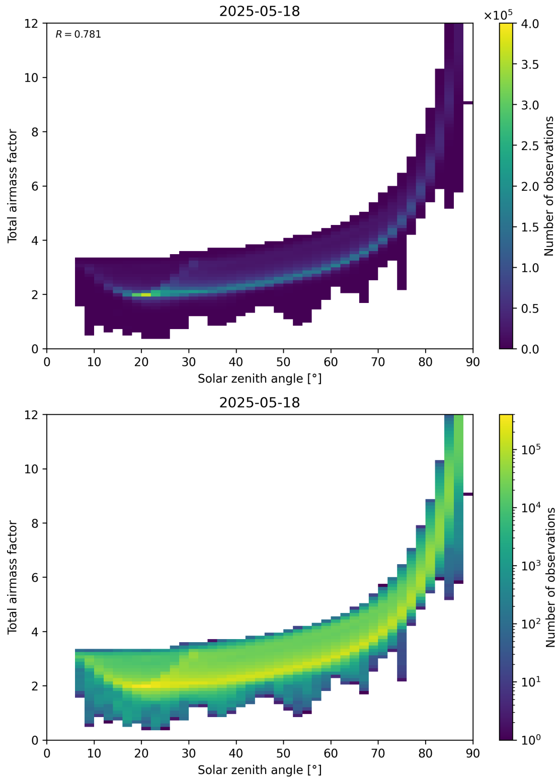
Figure 146: Scatter density plot of “Solar zenith angle” against “Total air mass factor” for 2025-05-17 to 2025-05-19.
