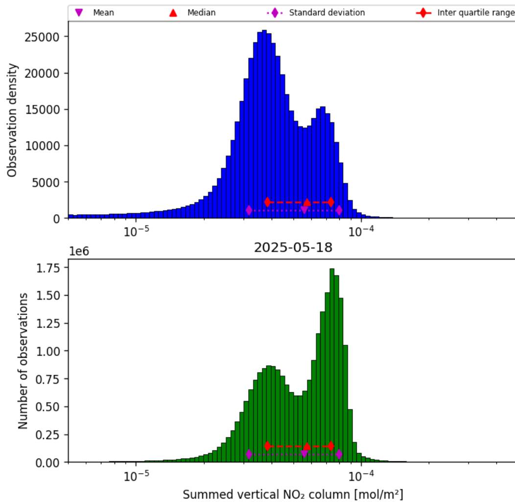
Figure 40: Histogram of “Summed vertical NO 2 column” for 2025-05-17 to 2025-05-19
