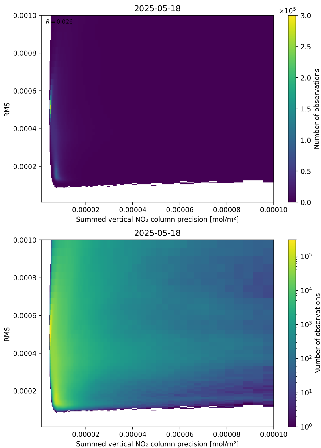
Figure 108: Scatter density plot of “Summed vertical NO 2 column precision” against “RMS” for 2025-05-17 to 2025-05-19.
