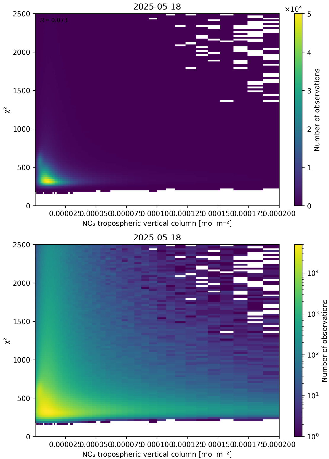
Figure 124: Scatter density plot of “NO 2 tropospheric vertical column” against “ \chi^2 ” for 2025-05-17 to 2025-05-19.
