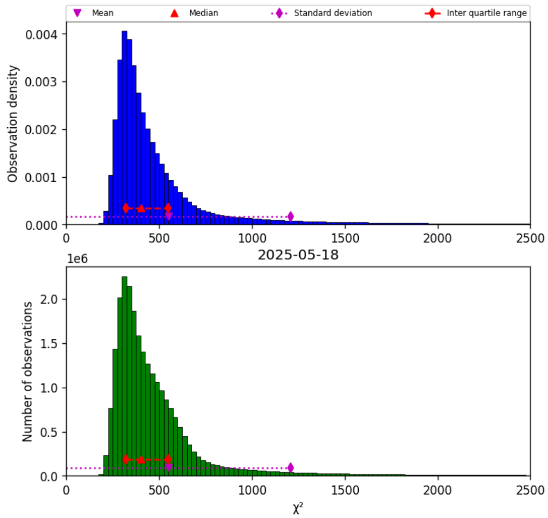
Figure 42: Histogram of “ \chi^2 ” for 2025-05-17 to 2025-05-19
