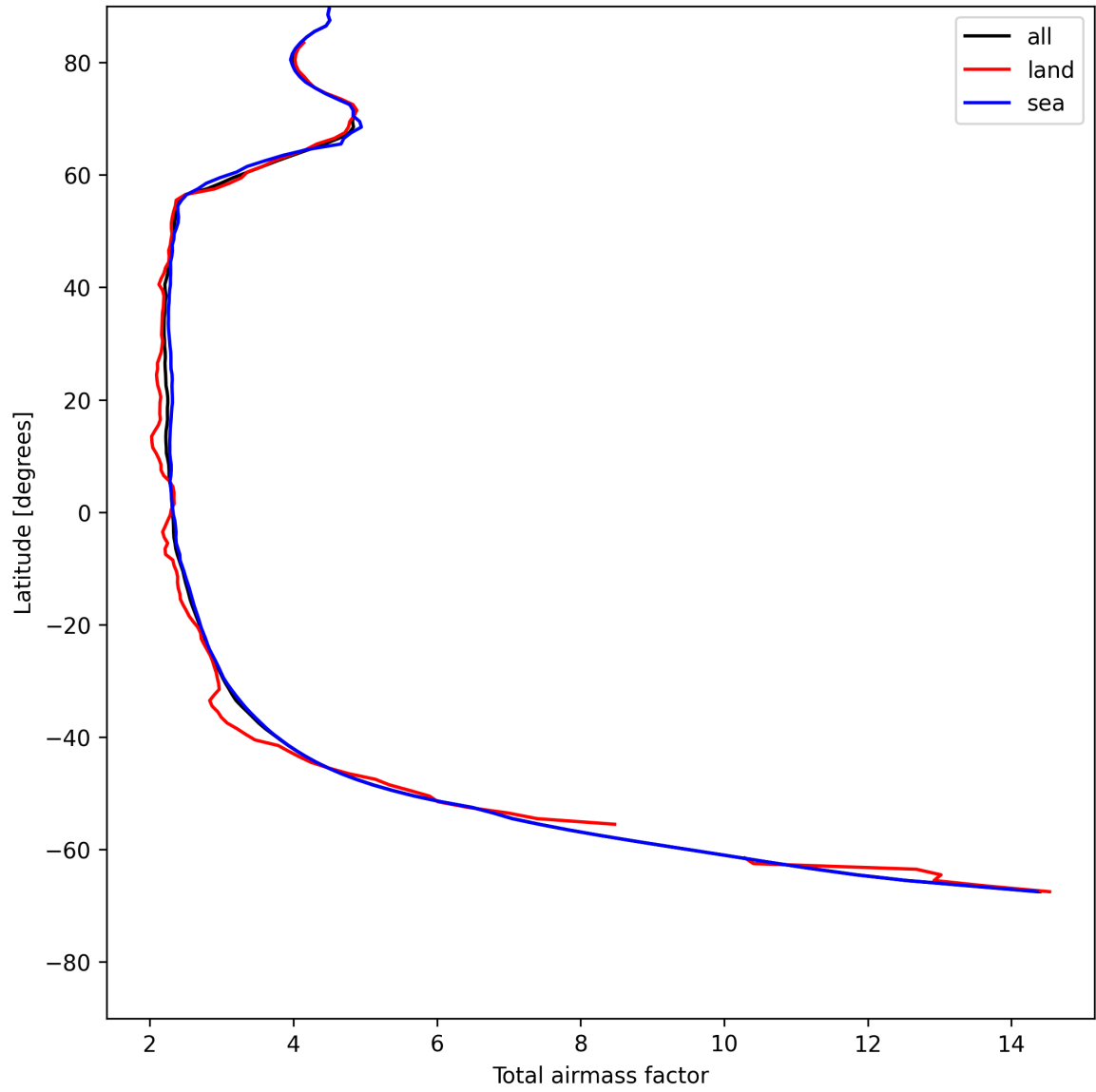
Figure 15: Zonal average of “Total airmass factor” for 2025-05-17 to 2025-05-19.
