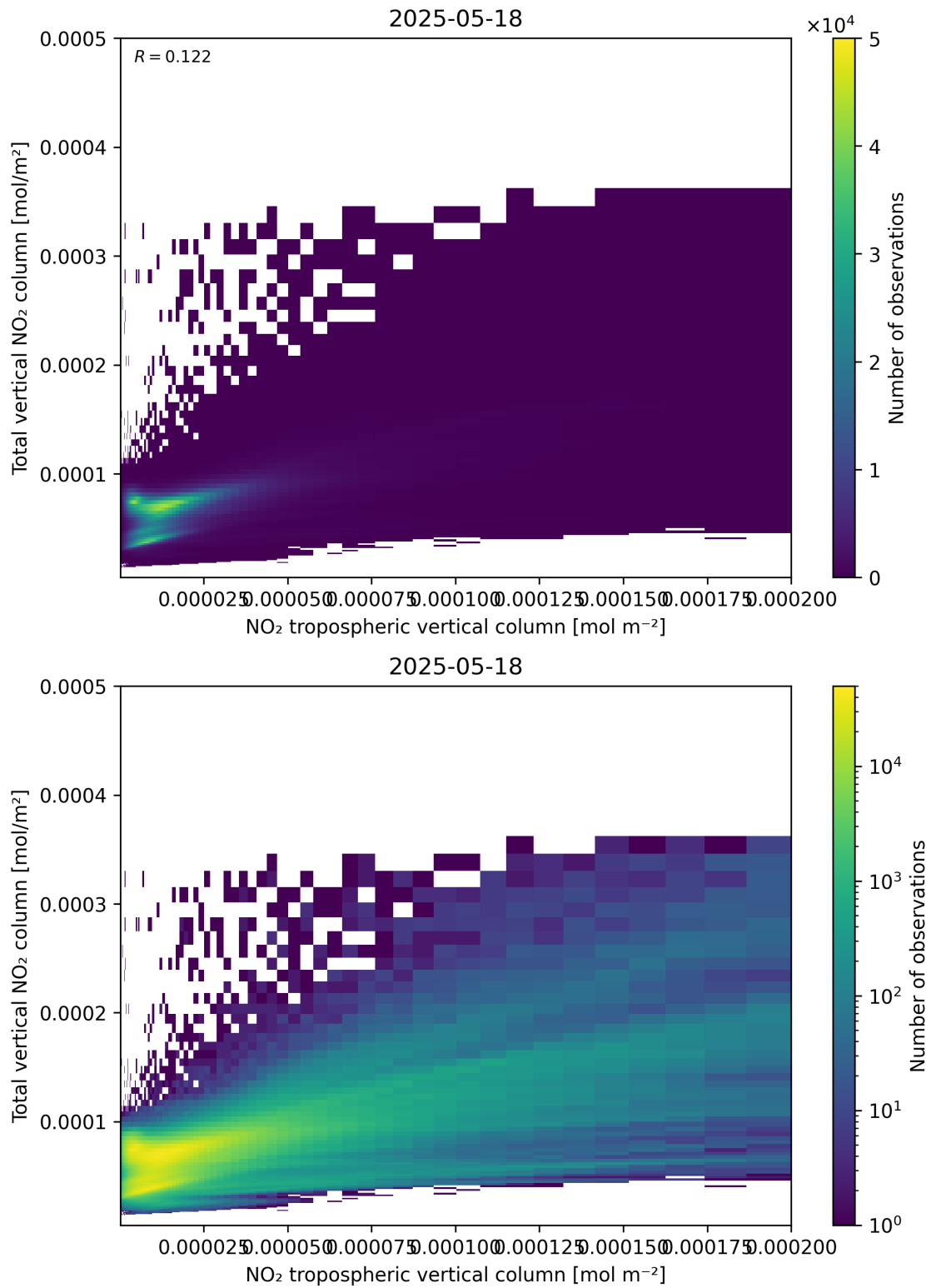
Figure 128: Scatter density plot of “NO 2 tropospheric vertical column” against “Total vertical NO 2 column” for 2025-05-17 to 2025-05-19.
