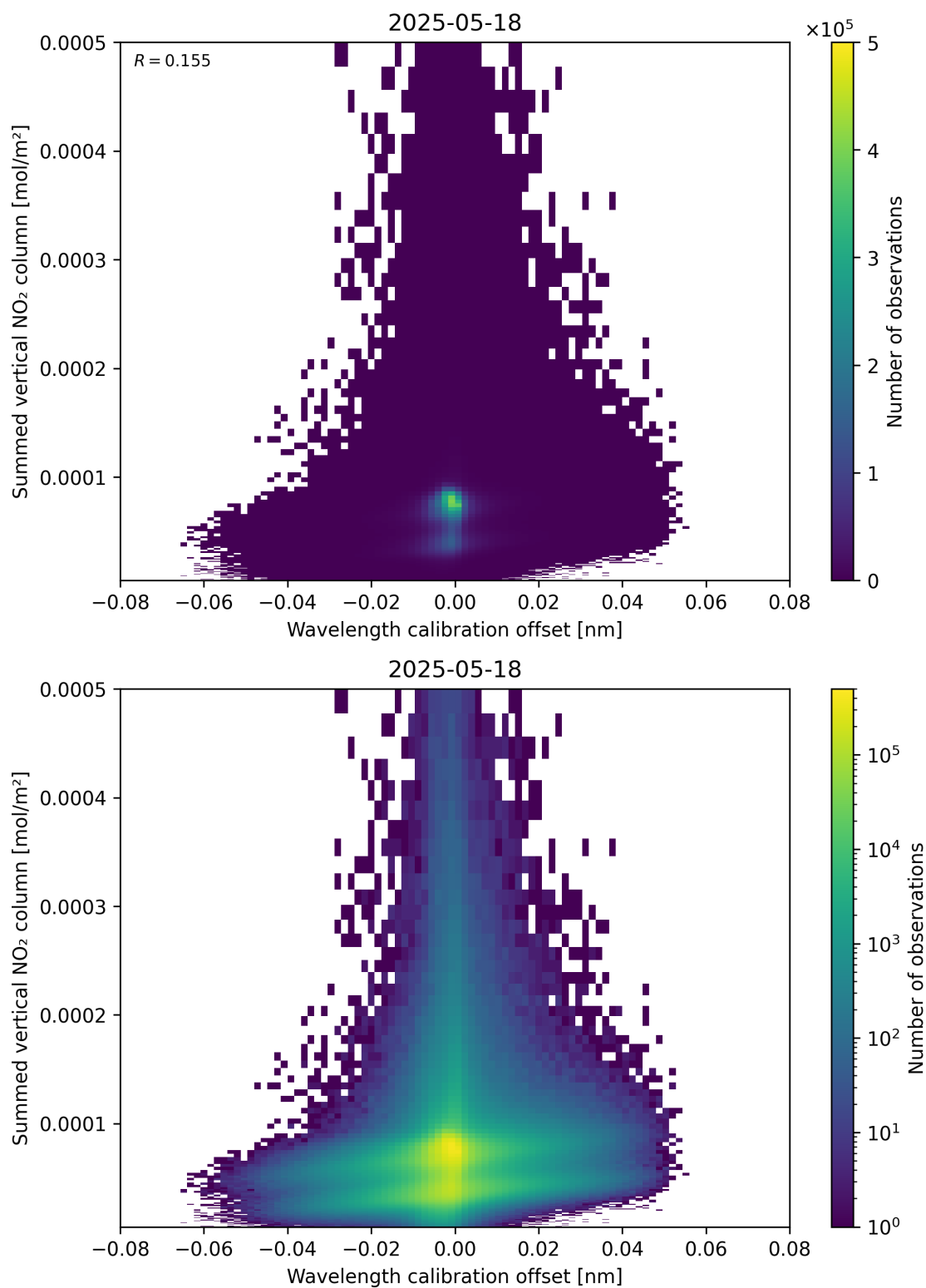
Figure 177: Scatter density plot of “Wavelength calibration offset” against “Summed vertical NO 2 column” for 2025-05-17 to 2025-05-19.
