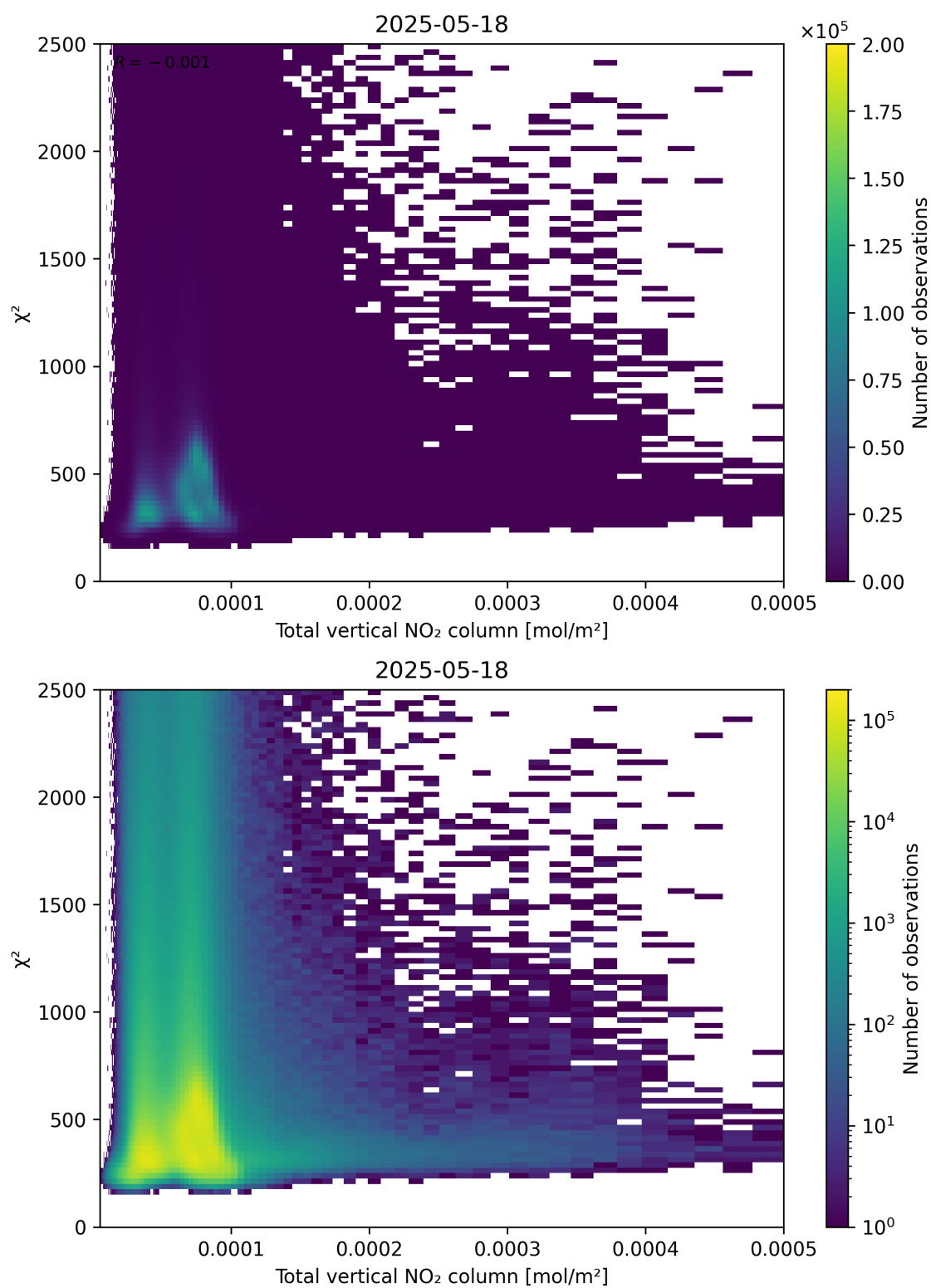
Figure 111: Scatter density plot of “Total vertical NO 2 column” against “ \chi^2 ” for 2025-05-17 to 2025-05-19.
