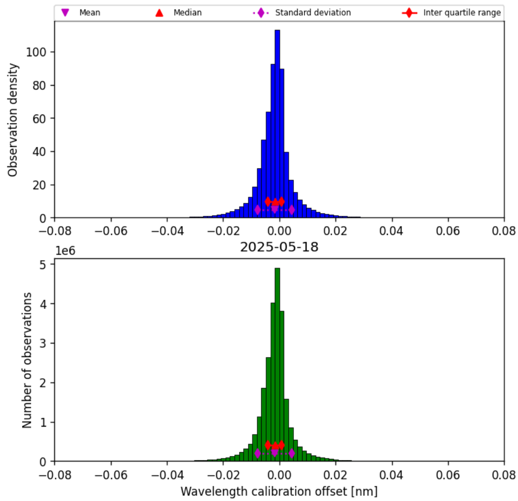
Figure 35: Histogram of “Wavelength calibration offset” for 2025-05-17 to 2025-05-19
