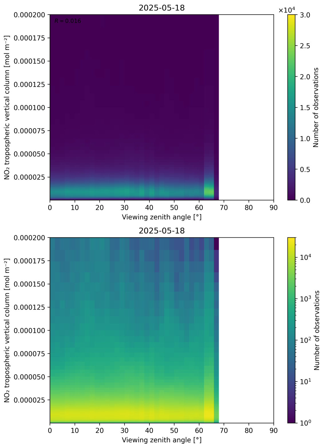
Figure 169: Scatter density plot of “Viewing zenith angle” against “NO 2 tropospheric vertical column” for 2025-05-17 to 2025-05-19.
