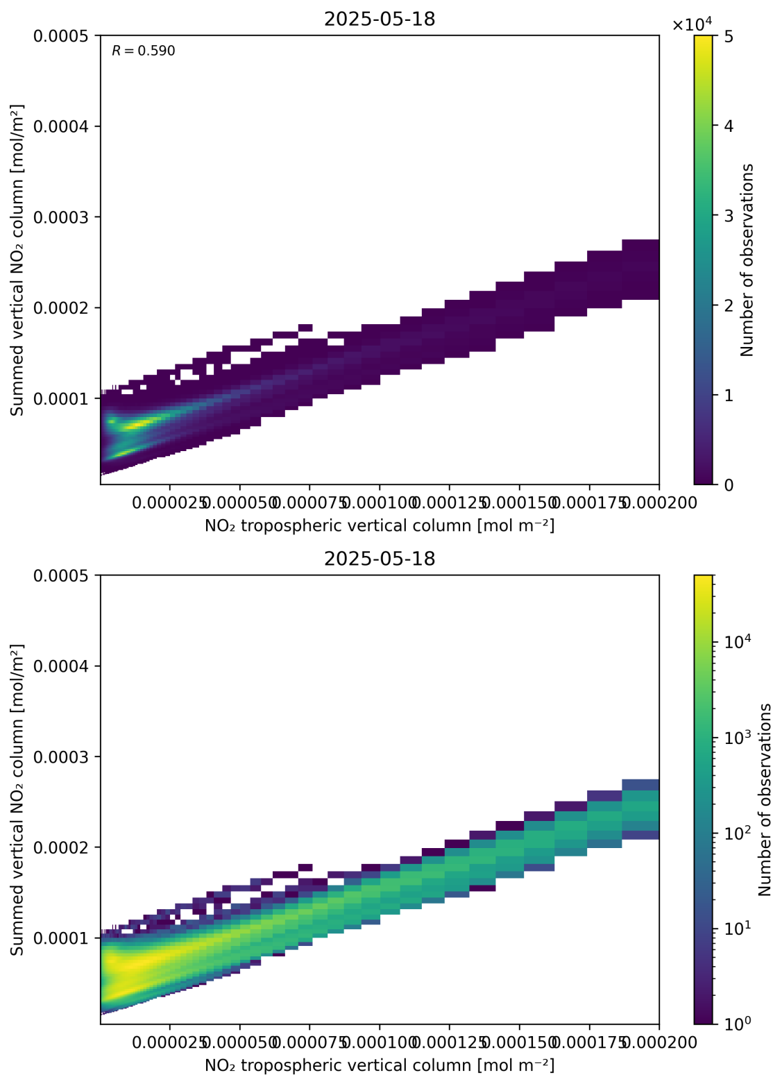
Figure 126: Scatter density plot of “NO 2 tropospheric vertical column” against “Summed vertical NO 2 column” for 2025-05-17 to 2025-05-19.
