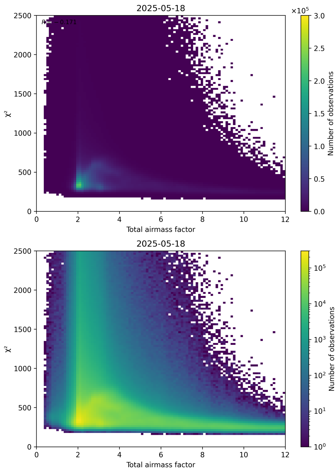
Figure 63: Scatter density plot of “Total airmass factor” against “ \chi^2 ” for 2025-05-17 to 2025-05-19.
