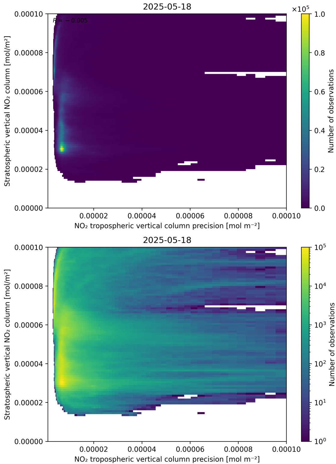
Figure 135: Scatter density plot of “NO 2 tropospheric vertical column precision” against “Stratospheric vertical NO 2 column” for 2025-05-17 to 2025-05-19.
