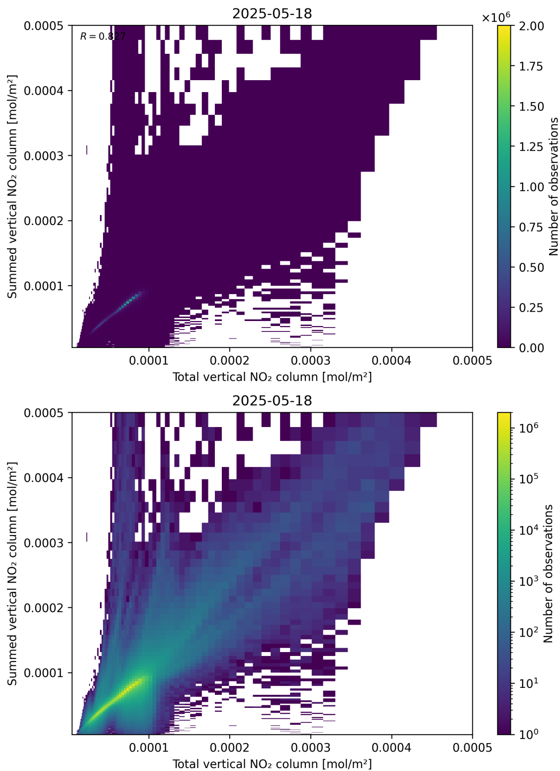
Figure 112: Scatter density plot of “Total vertical NO 2 column” against “Summed vertical NO 2 column” for 2025-05-17 to 2025-05-19.
