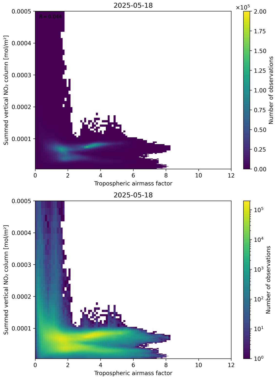
Figure 75: Scatter density plot of “Tropospheric airmass factor” against “Summed vertical NO 2 column” for 2025-05-17 to 2025-05-19.
