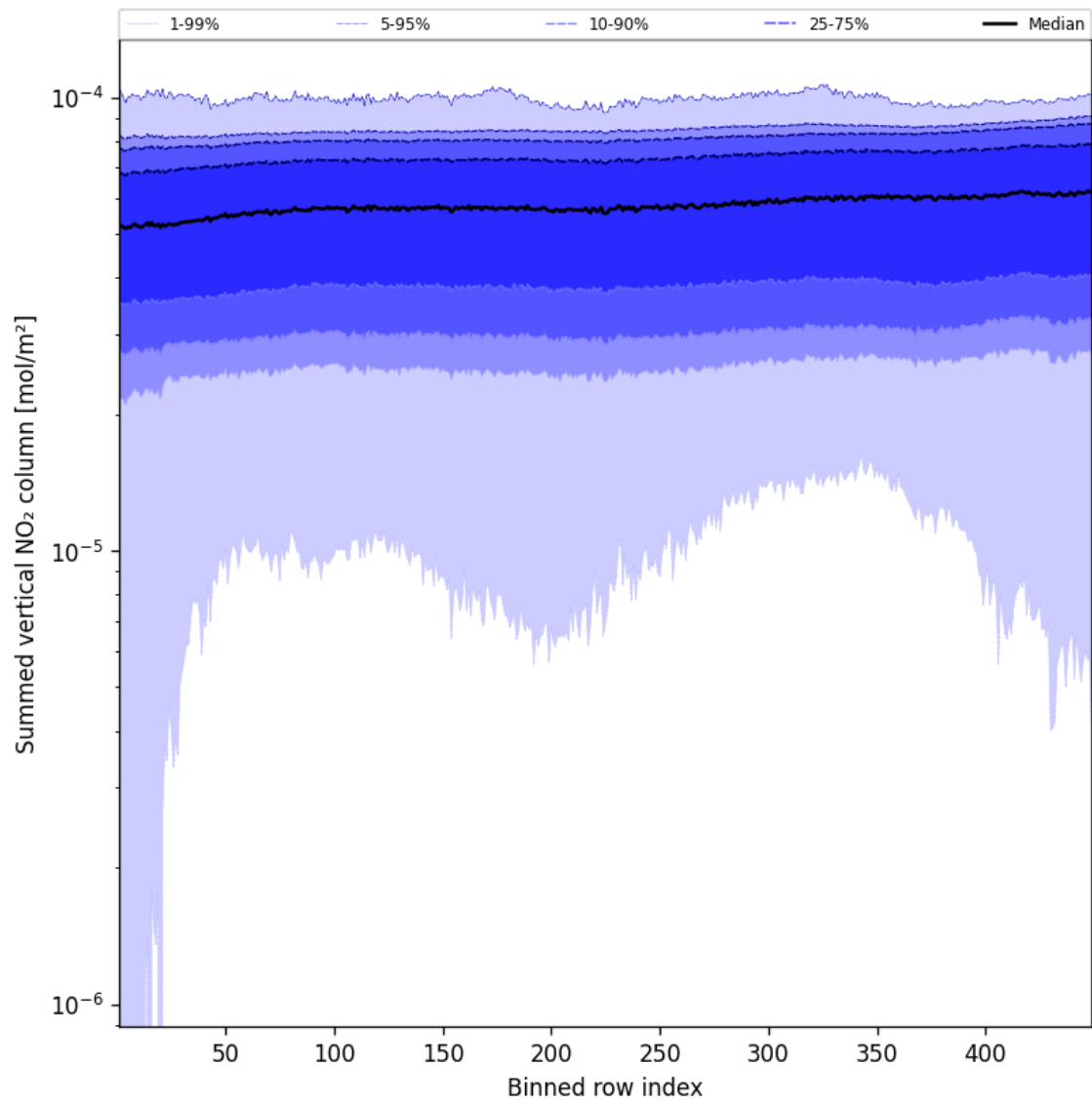
Figure 57: Along track statistics of “Summed vertical NO 2 column” for 2025-05-17 to 2025-05-19
