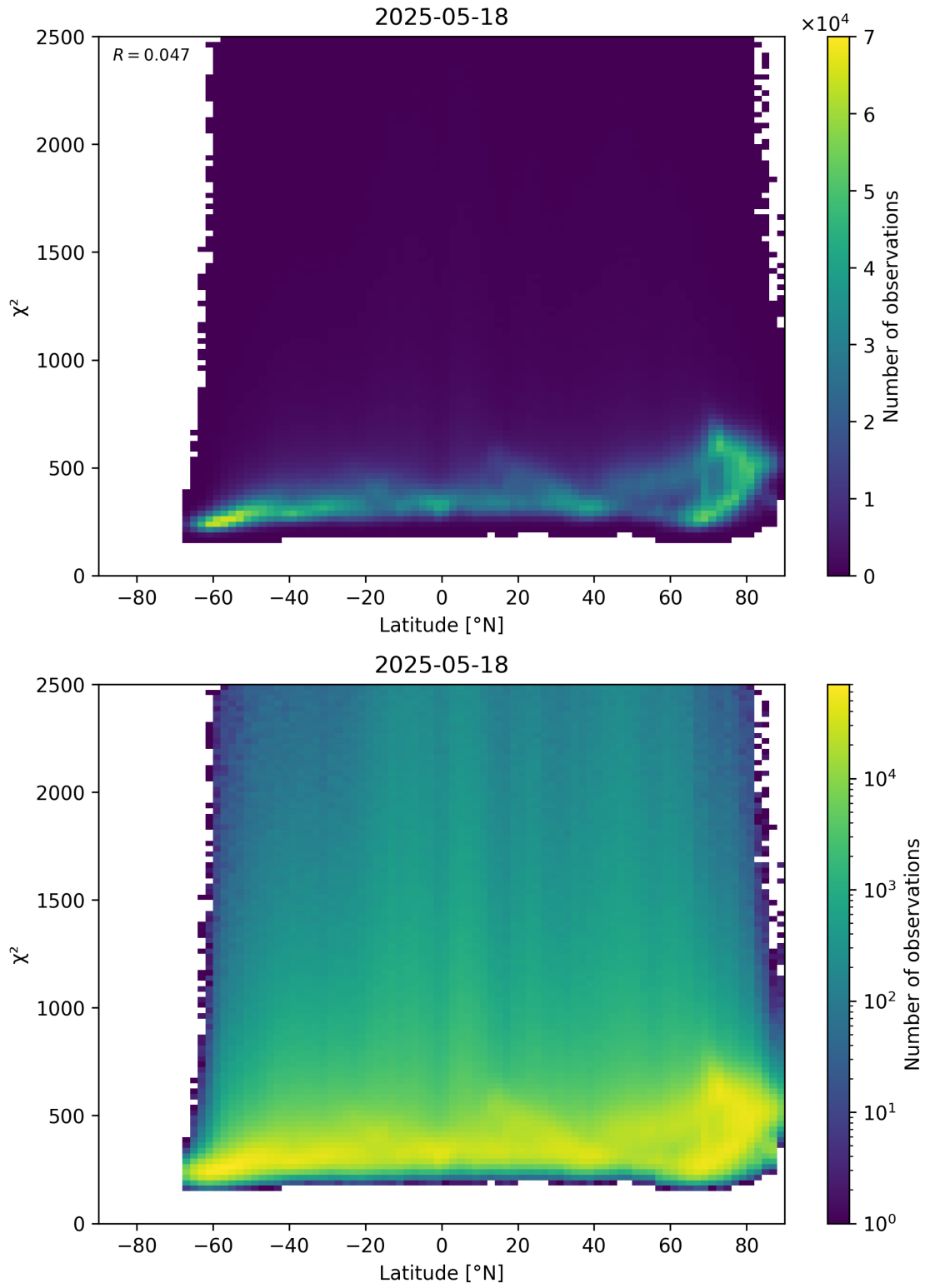
Figure 86: Scatter density plot of “Latitude” against “ \chi^2 ” for 2025-05-17 to 2025-05-19.
