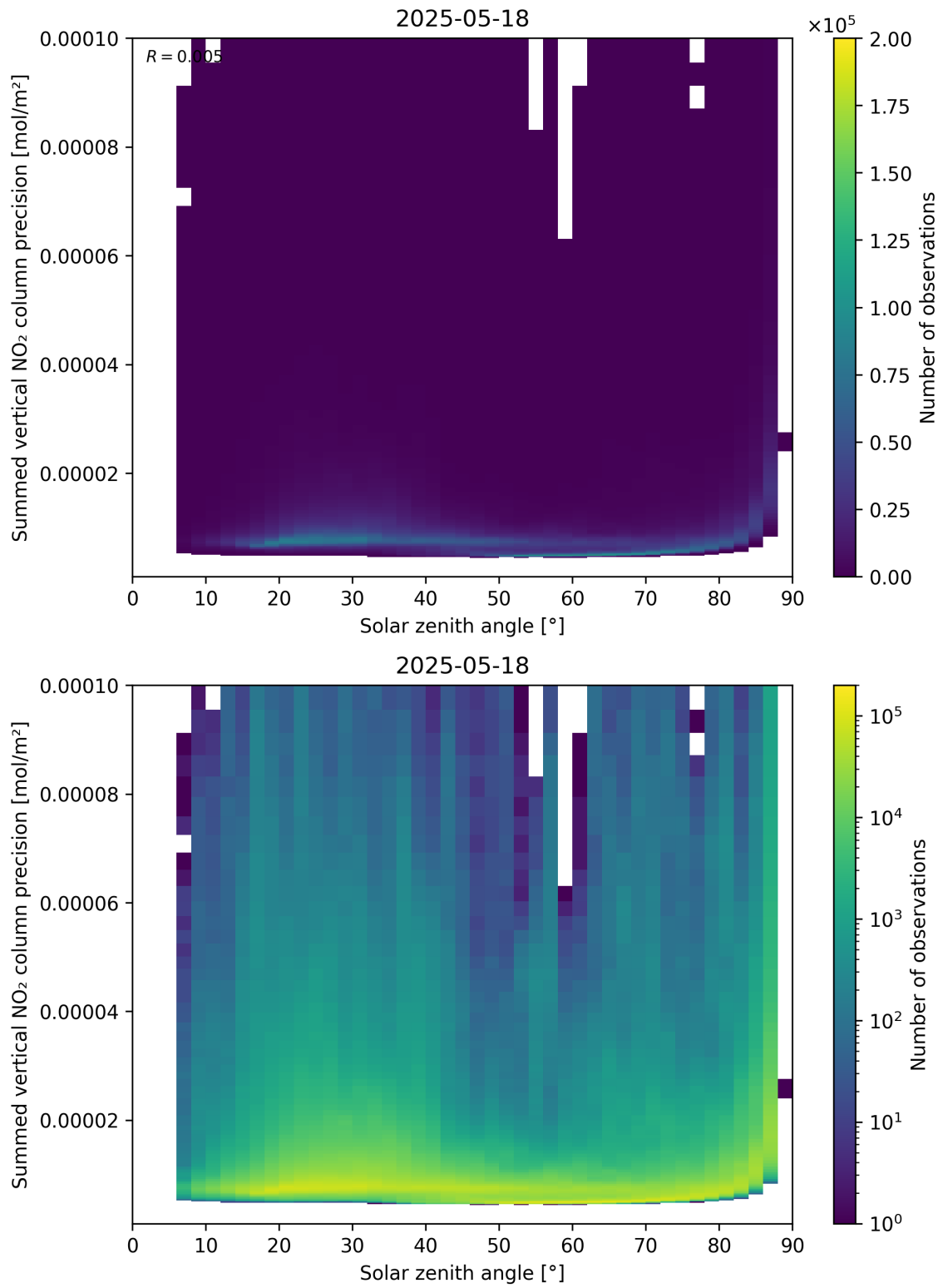
Figure 152: Scatter density plot of “Solar zenith angle” against “Summed vertical NO 2 column precision” for 2025-05-17 to 2025-05-19.
