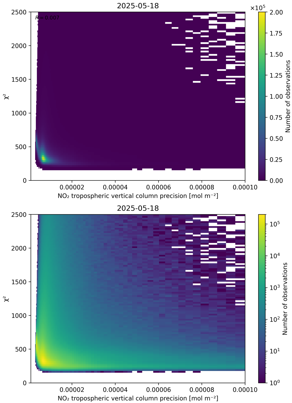
Figure 134: Scatter density plot of “NO 2 tropospheric vertical column precision” against “ \chi^2 ” for 2025-05-17 to 2025-05-19.
