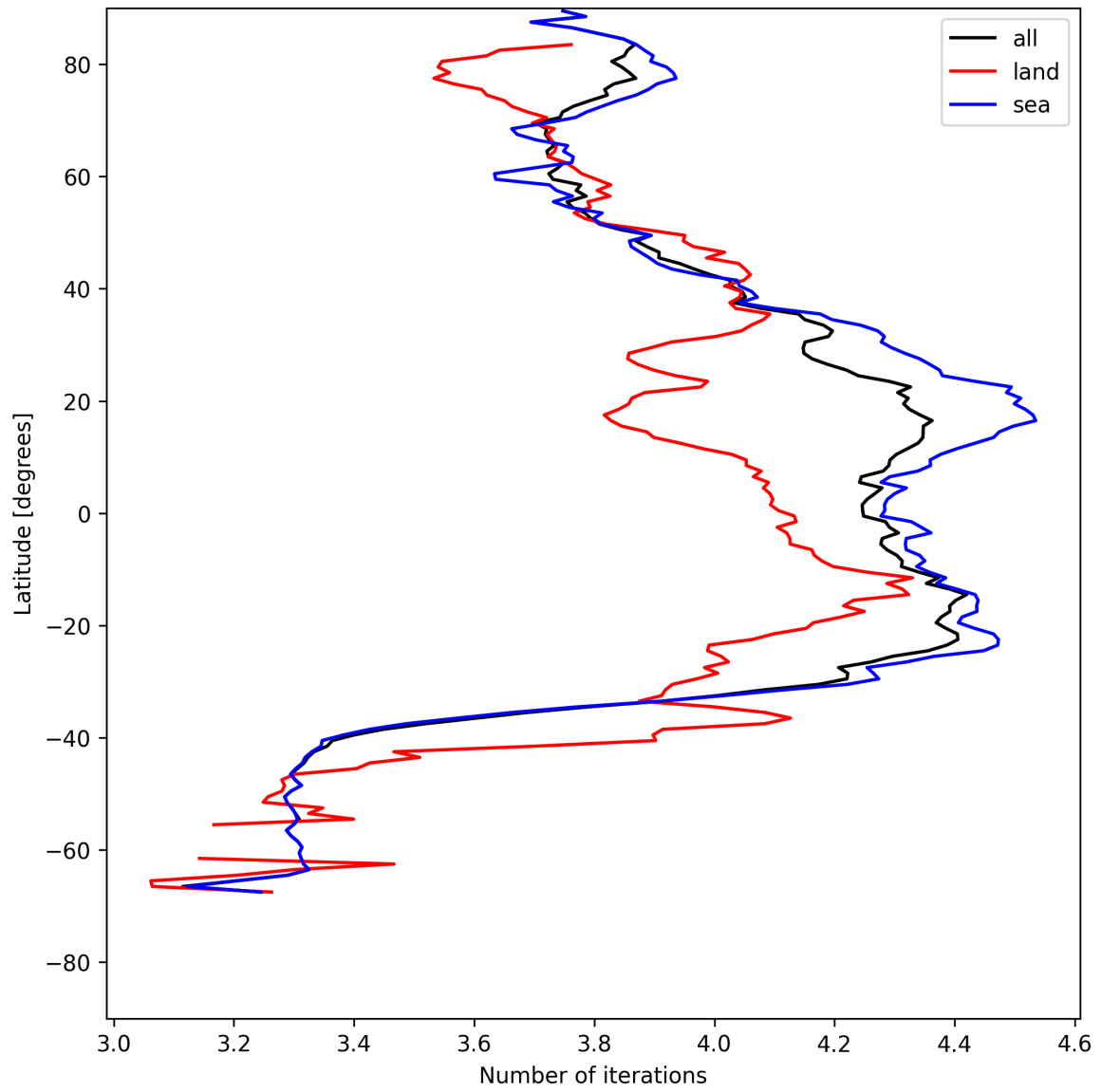
Figure 17: Zonal average of “Number of iterations” for 2025-05-17 to 2025-05-19.
