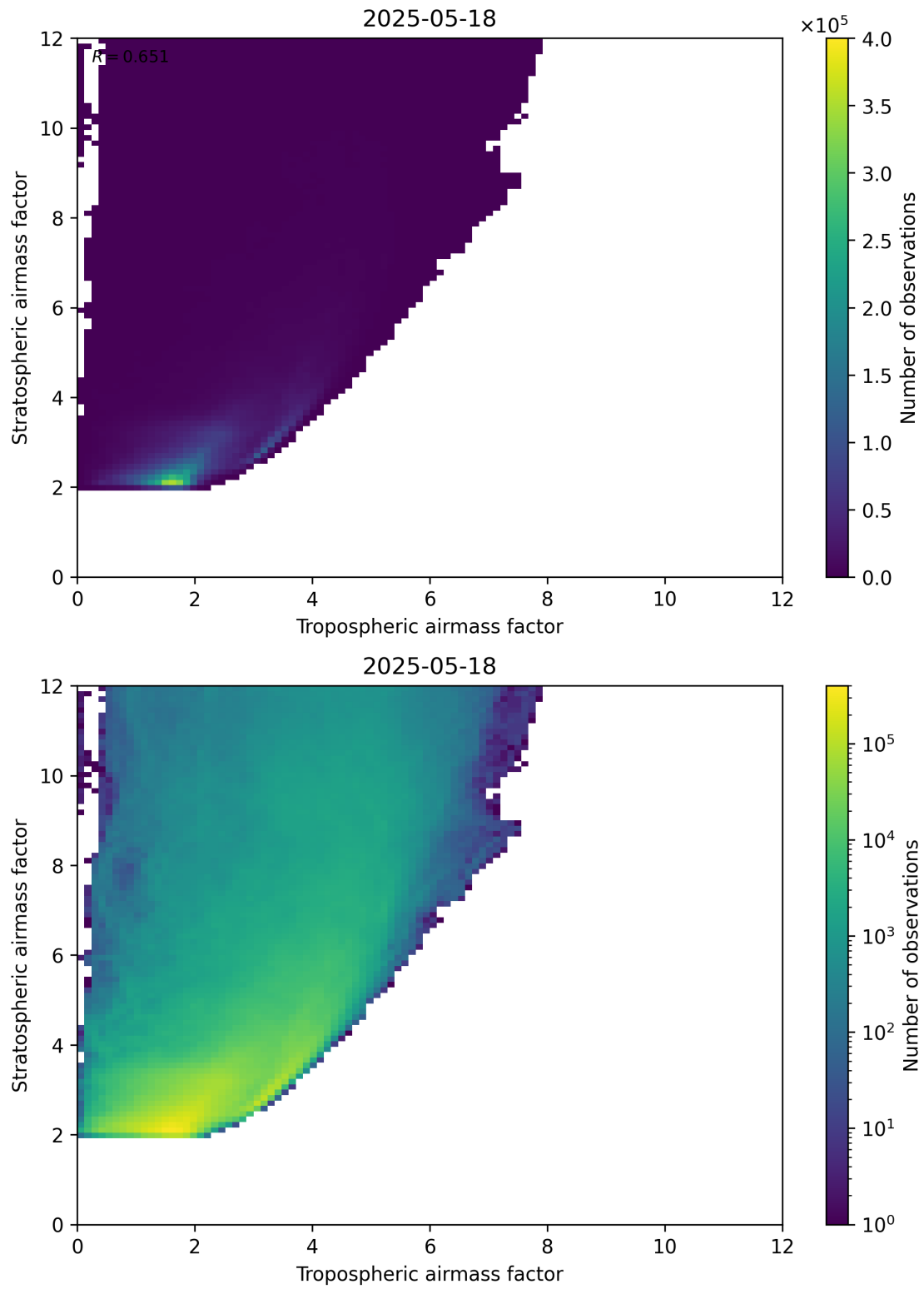
Figure 71: Scatter density plot of “Tropospheric airmass factor” against “Stratospheric airmass factor” for 2025-05-17 to 2025-05-19.
