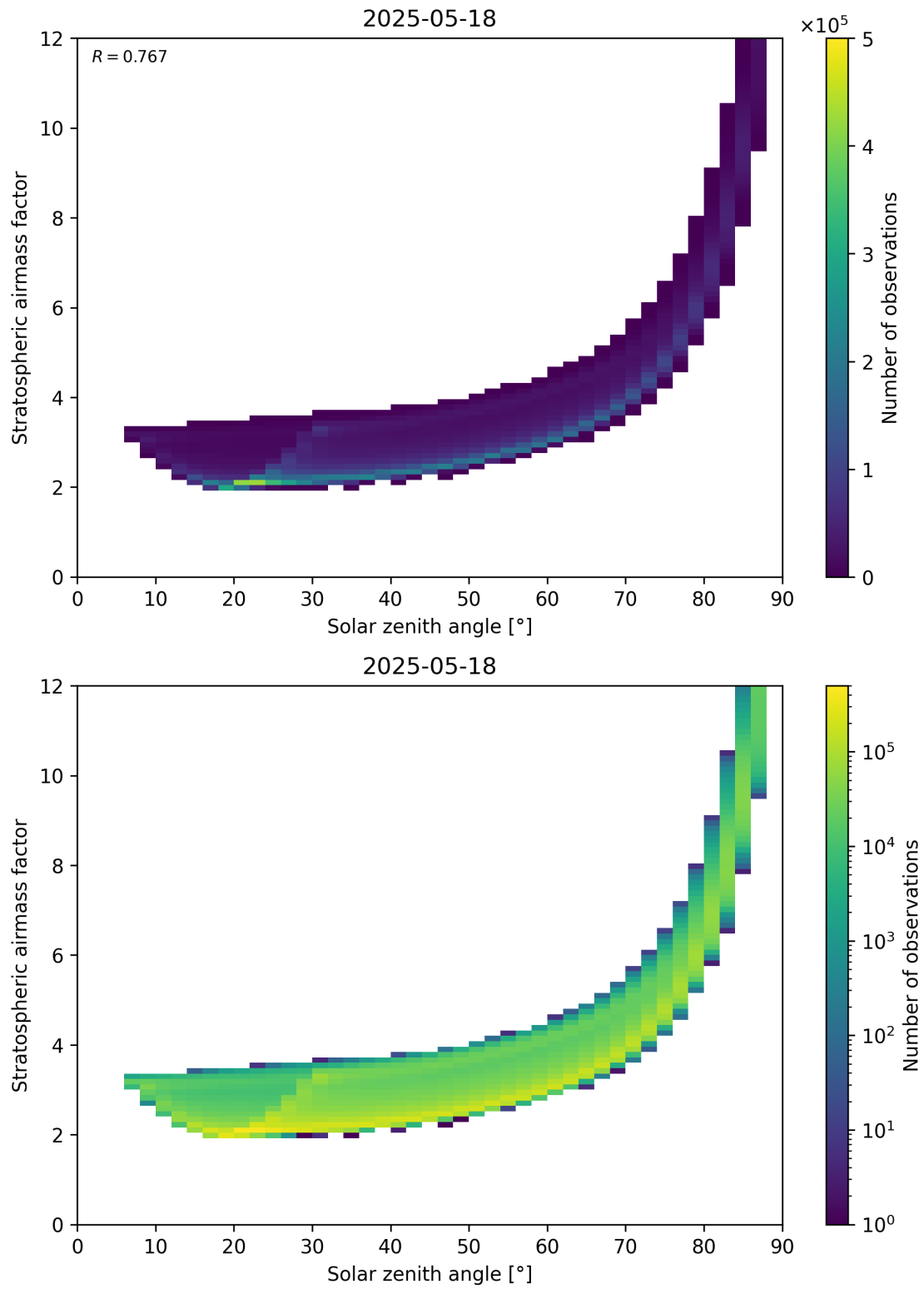
Figure 145: Scatter density plot of “Solar zenith angle” against “Stratospheric airmass factor” for 2025-05-17 to 2025-05-19.
