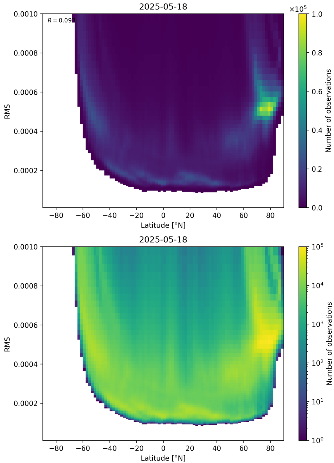
Figure 94: Scatter density plot of “Latitude” against “RMS” for 2025-05-17 to 2025-05-19.
