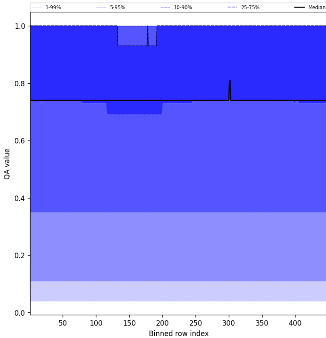
Figure 45: Along track statistics of “QA value” for 2025-05-17 to 2025-05-19
