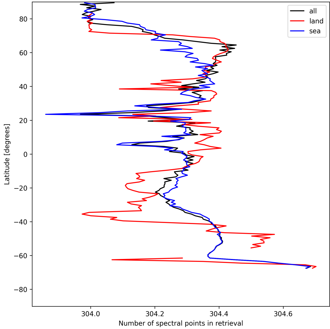
Figure 16: Zonal average of “Number of spectral points in retrieval” for 2025-05-17 to 2025-05-19.
