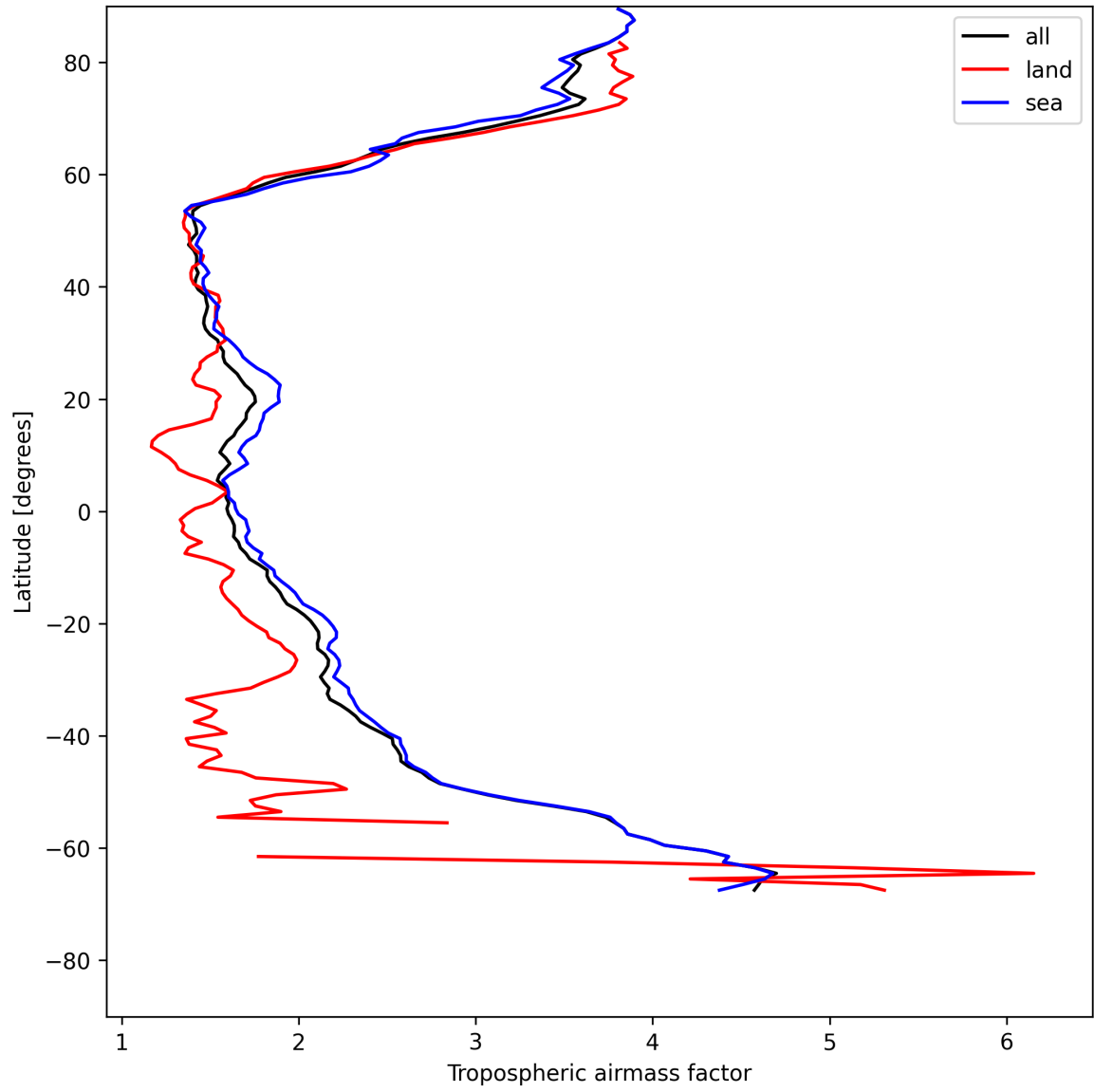
Figure 14: Zonal average of “Tropospheric airmass factor” for 2025-05-17 to 2025-05-19.
