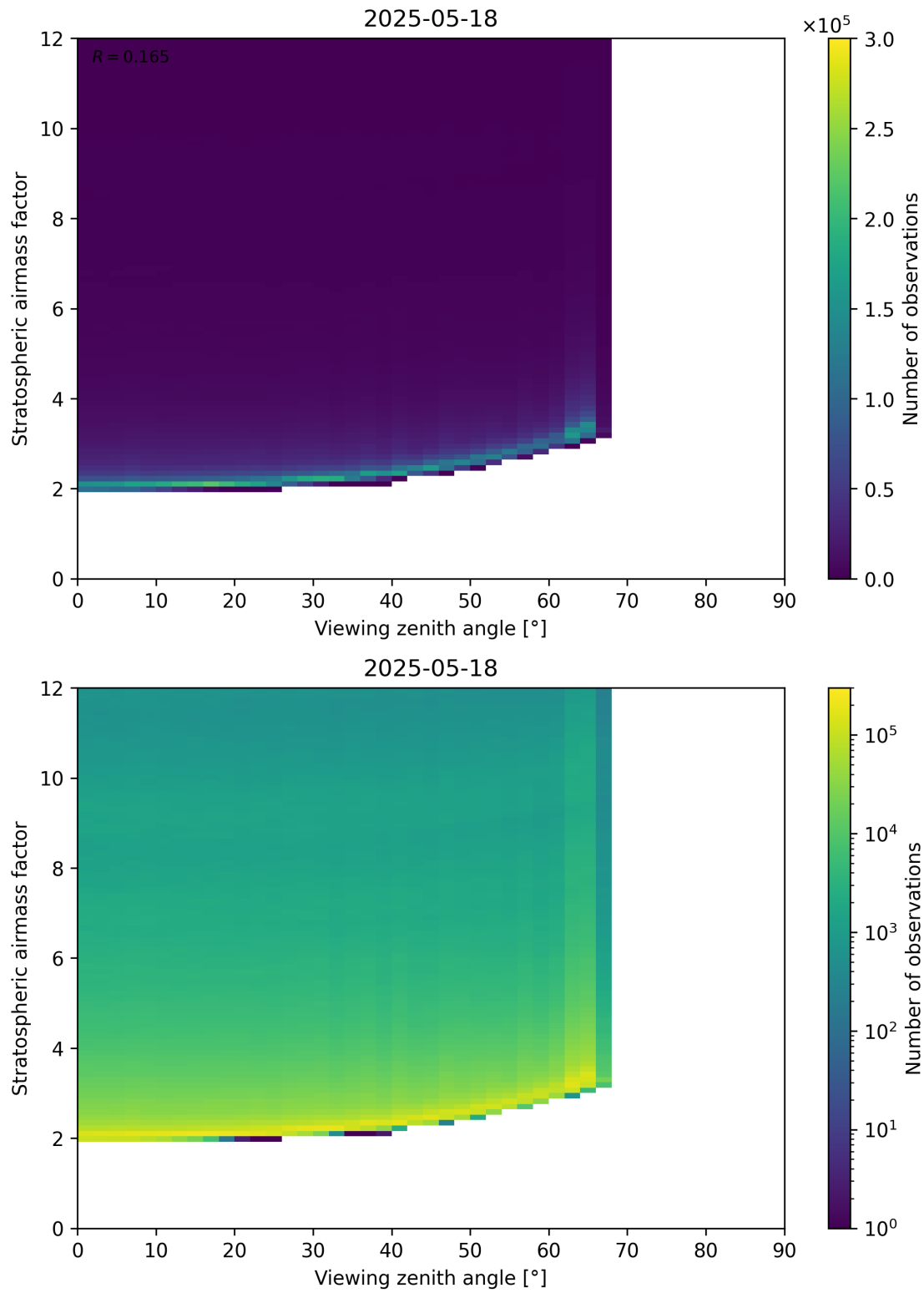
Figure 159: Scatter density plot of “Viewing zenith angle” against “Stratospheric airmass factor” for 2025-05-17 to 2025-05-19.
