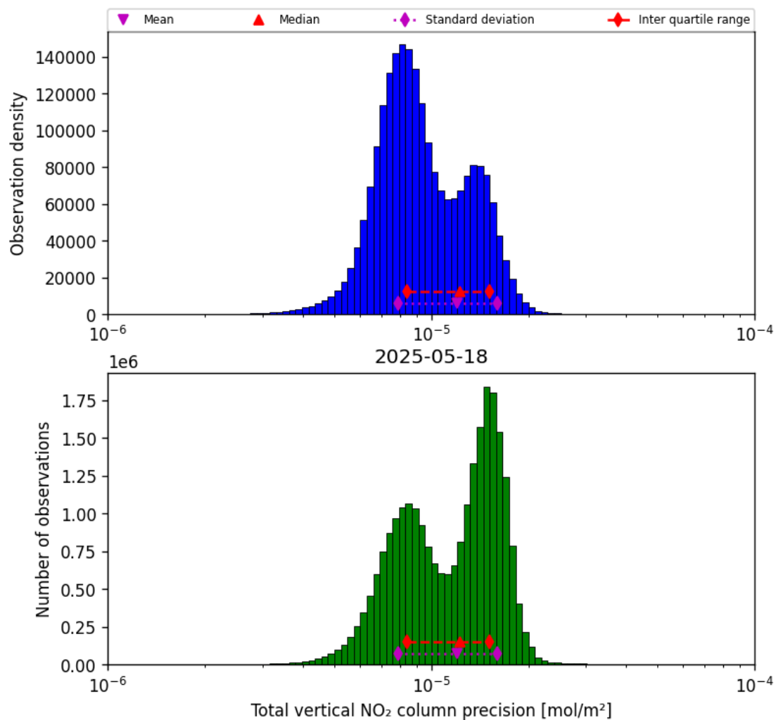
Figure 39: Histogram of “Total vertical NO 2 column precision” for 2025-05-17 to 2025-05-19
