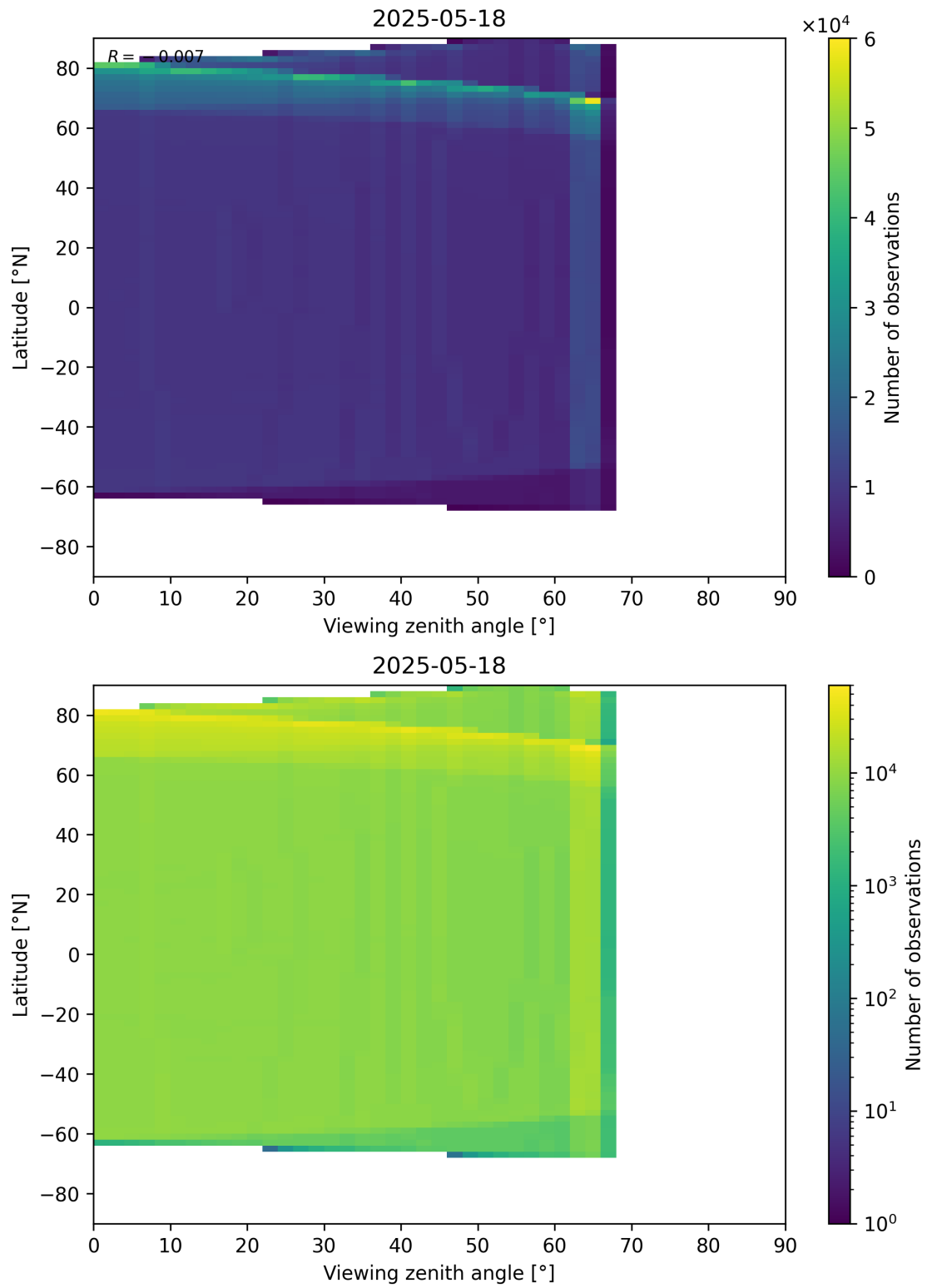
Figure 163: Scatter density plot of “Viewing zenith angle” against “Latitude” for 2025-05-17 to 2025-05-19.
