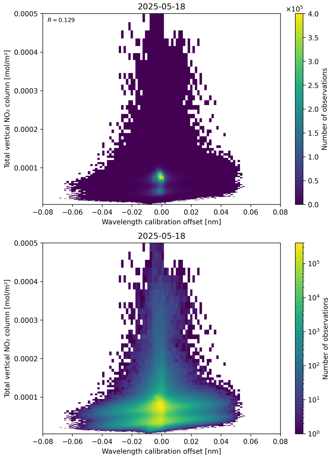
Figure 179: Scatter density plot of “Wavelength calibration offset” against “Total vertical NO 2 column” for 2025-05-17 to 2025-05-19.
