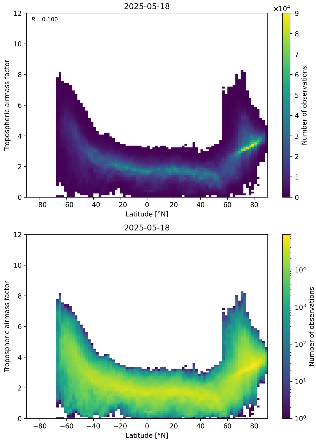
Figure 85: Scatter density plot of “Latitude” against “Tropospheric airmass factor” for 2025-05-17 to 2025-05-19.
