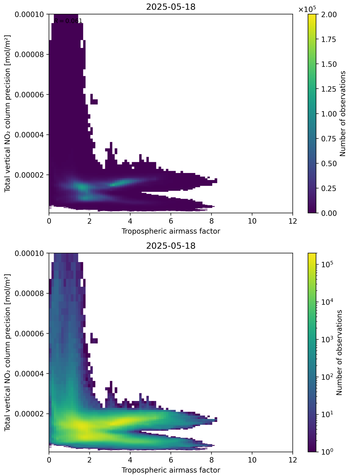
Figure 78: Scatter density plot of “Tropospheric airmass factor” against “Total vertical NO 2 column precision” for 2025-05-17 to 2025-05-19.
