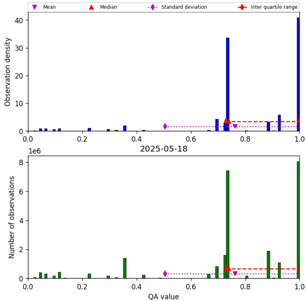
Figure 28: Histogram of “QA value” for 2025-05-17 to 2025-05-19
