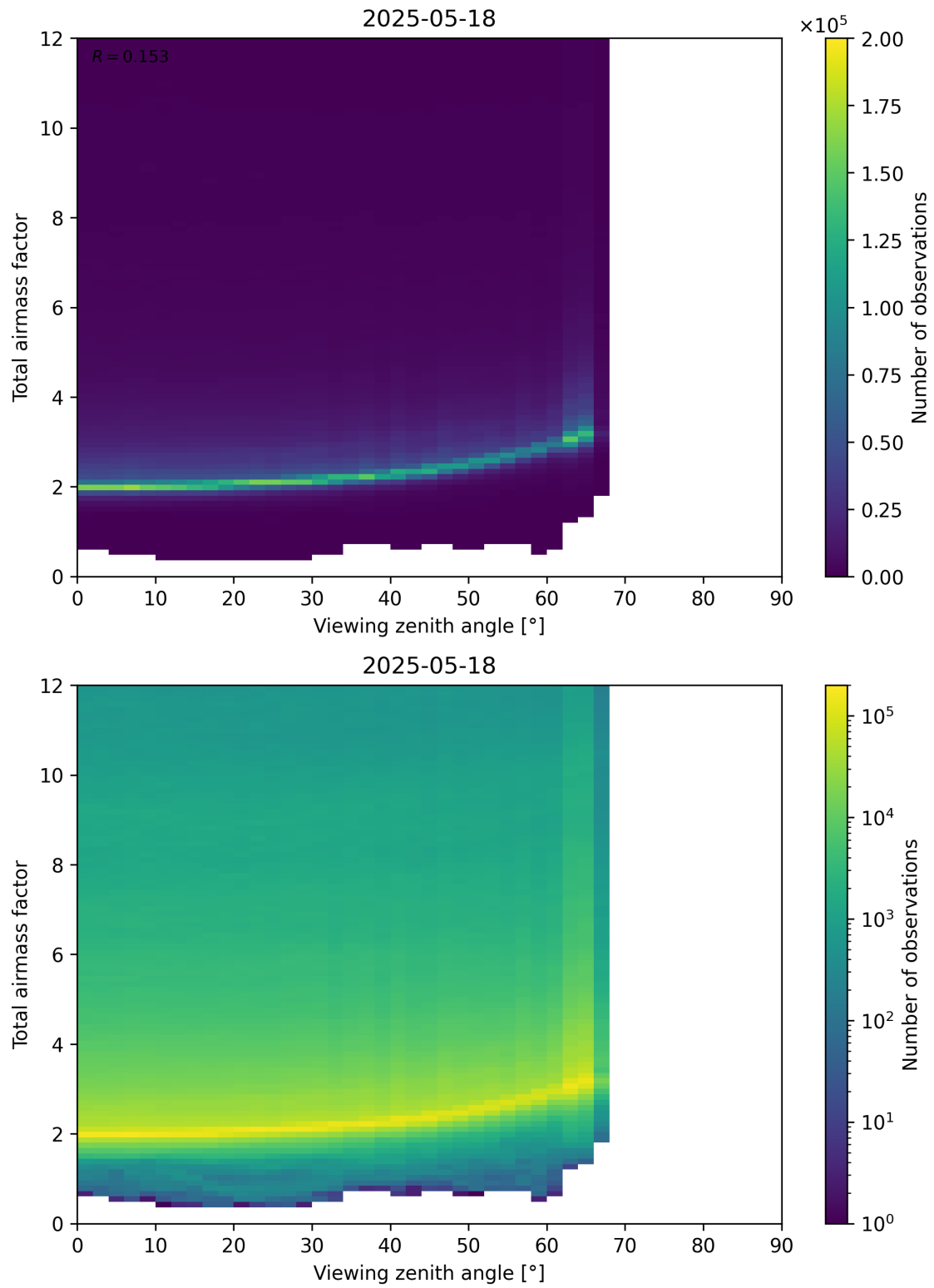
Figure 160: Scatter density plot of “Viewing zenith angle” against “Total airmass factor” for 2025-05-17 to 2025-05-19.
