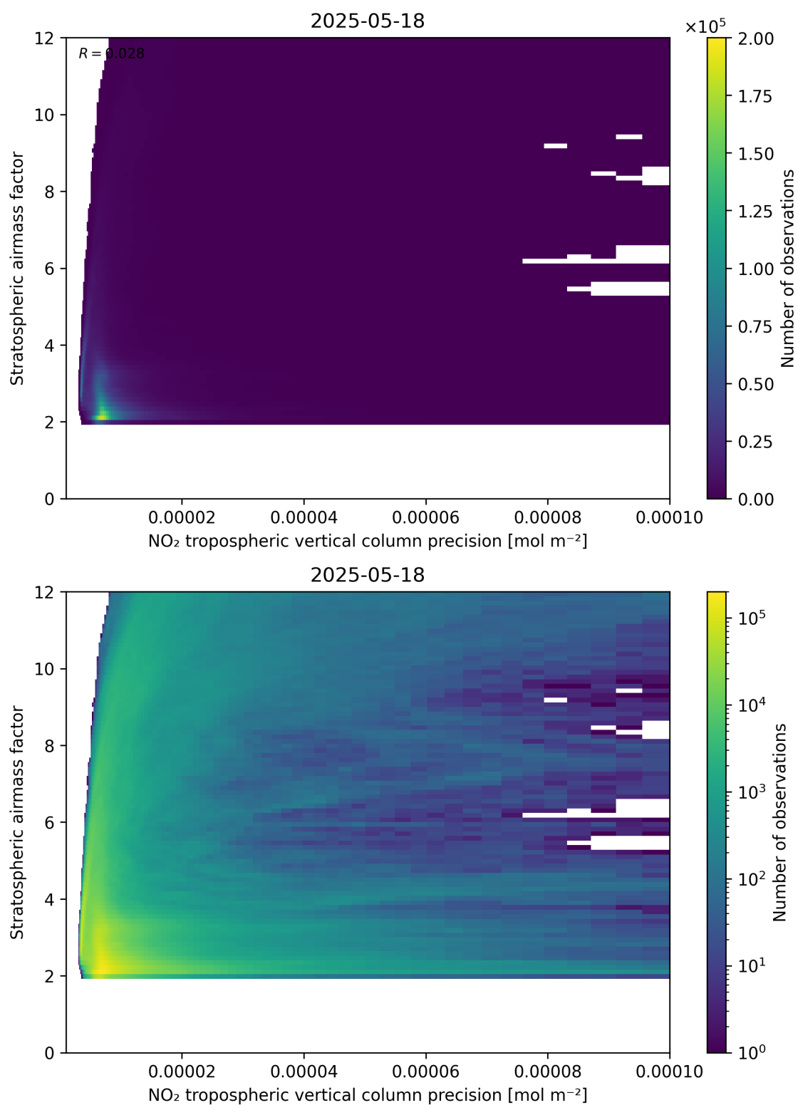
Figure 131: Scatter density plot of “NO 2 tropospheric vertical column precision” against “Stratospheric airmass factor” for 2025-05-17 to 2025-05-19.
