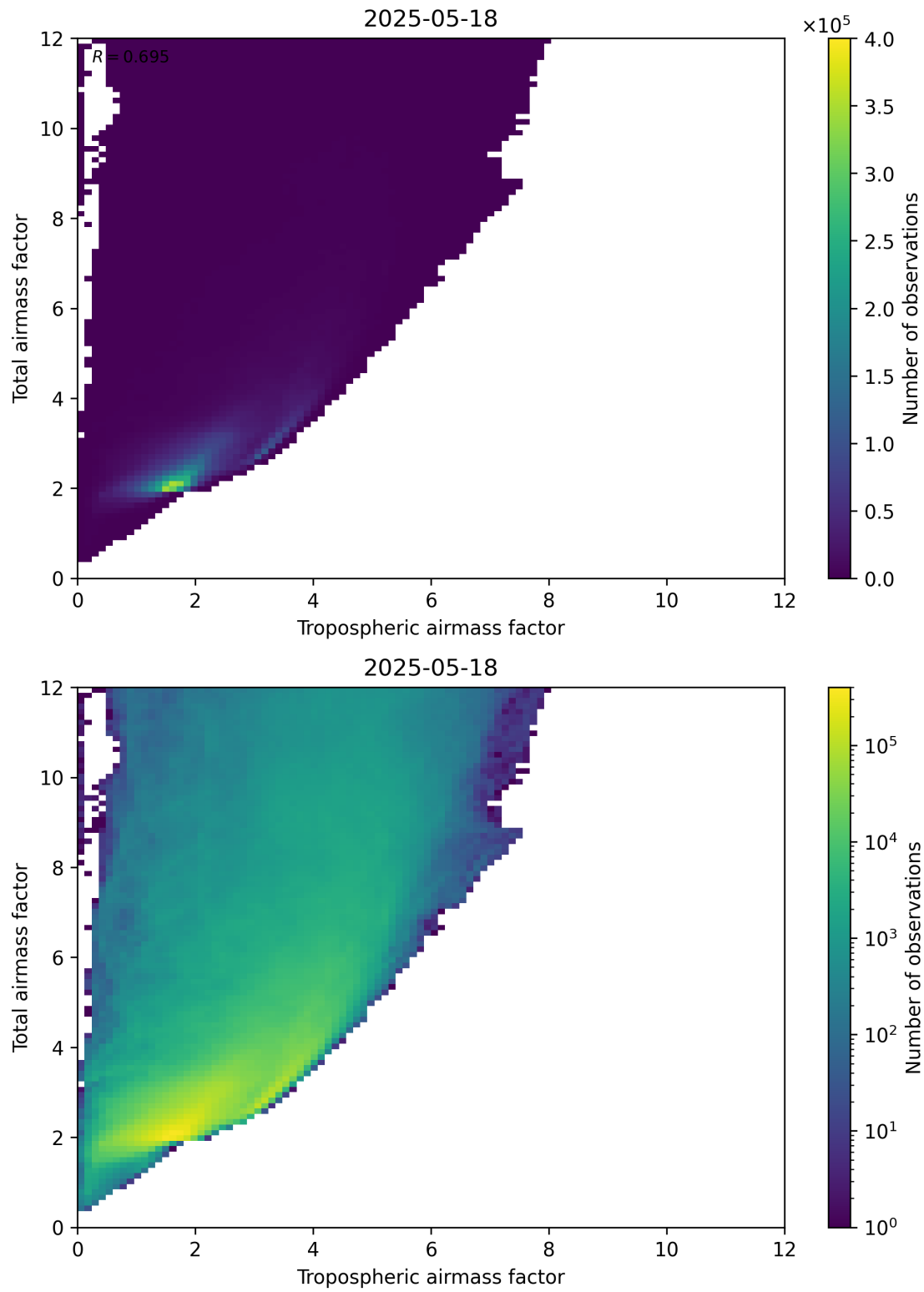
Figure 72: Scatter density plot of “Tropospheric airmass factor” against “Total airmass factor” for 2025-05-17 to 2025-05-19.
