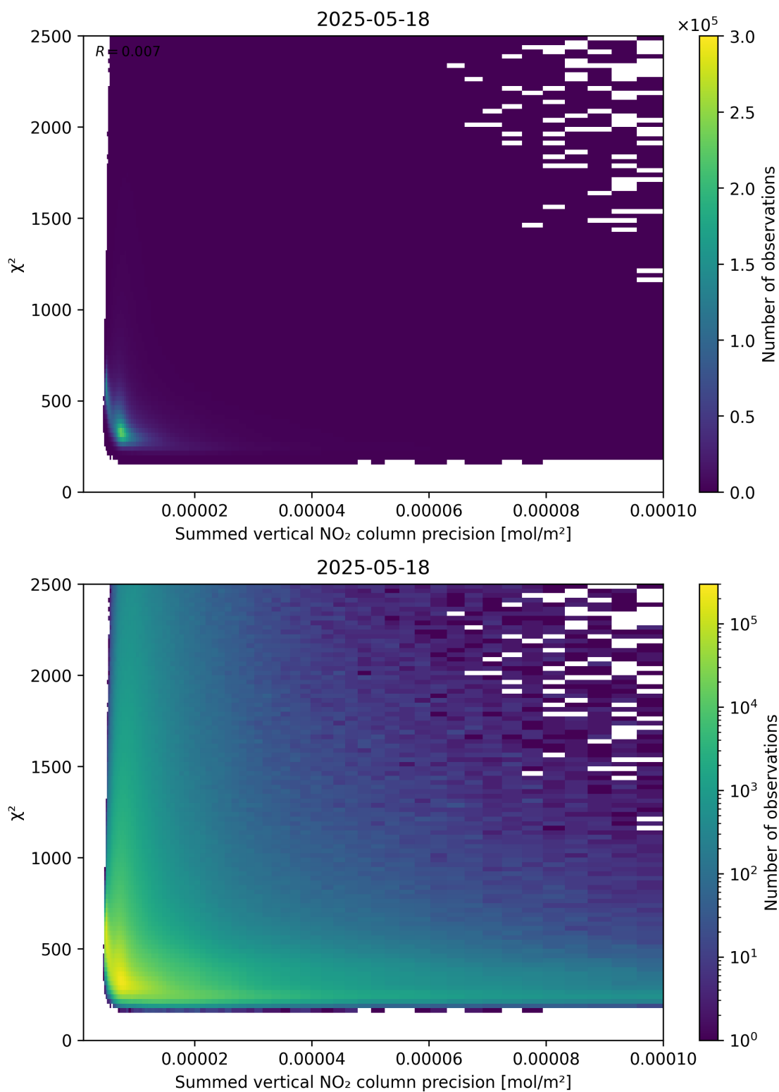
Figure 107: Scatter density plot of “Summed vertical NO 2 column precision” against “ \chi^2 ” for 2025-05-17 to 2025-05-19.
