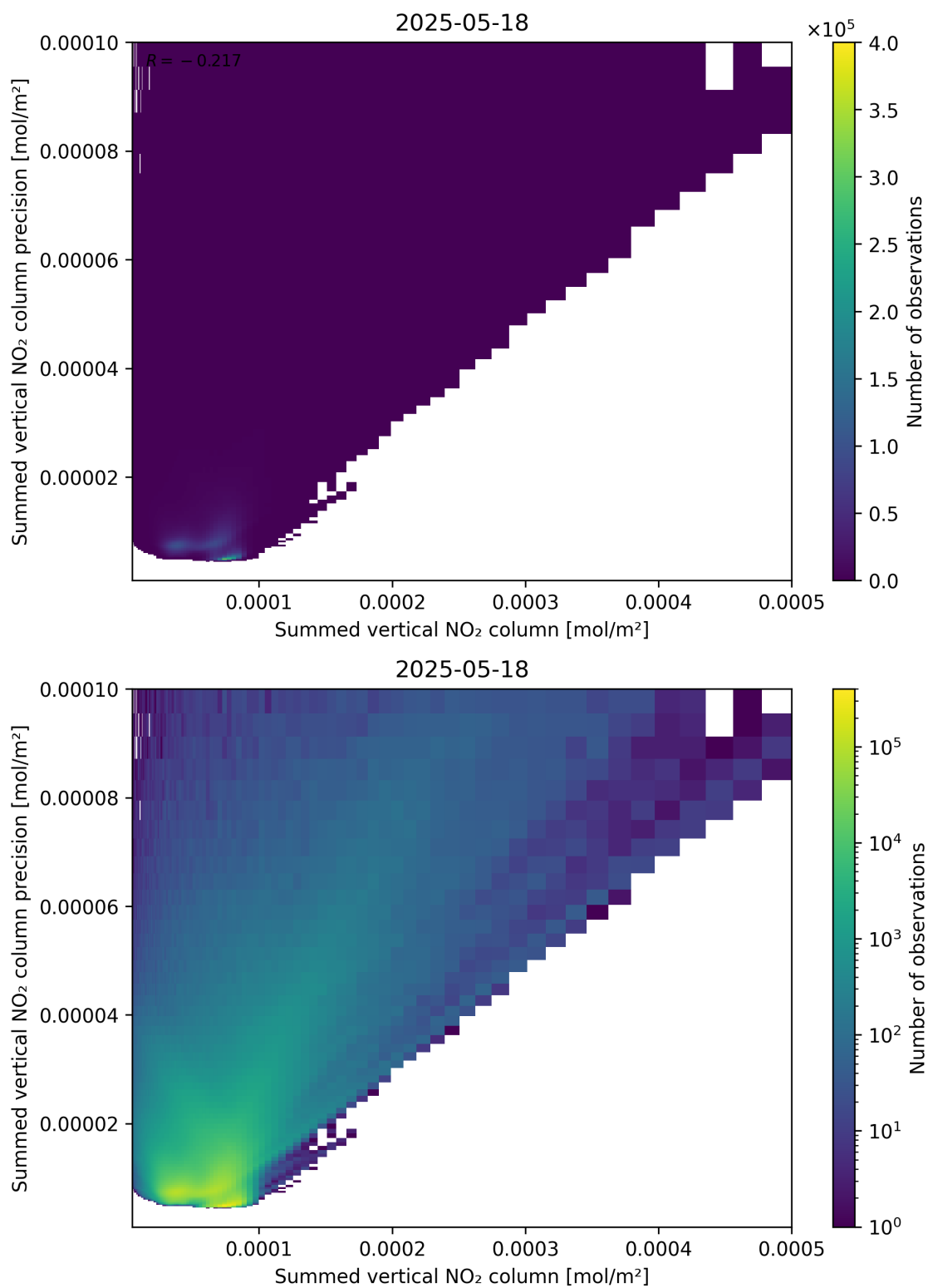
Figure 105: Scatter density plot of “Summed vertical NO 2 column” against “Summed vertical NO 2 column precision” for 2025-05-17 to 2025-05-19.
