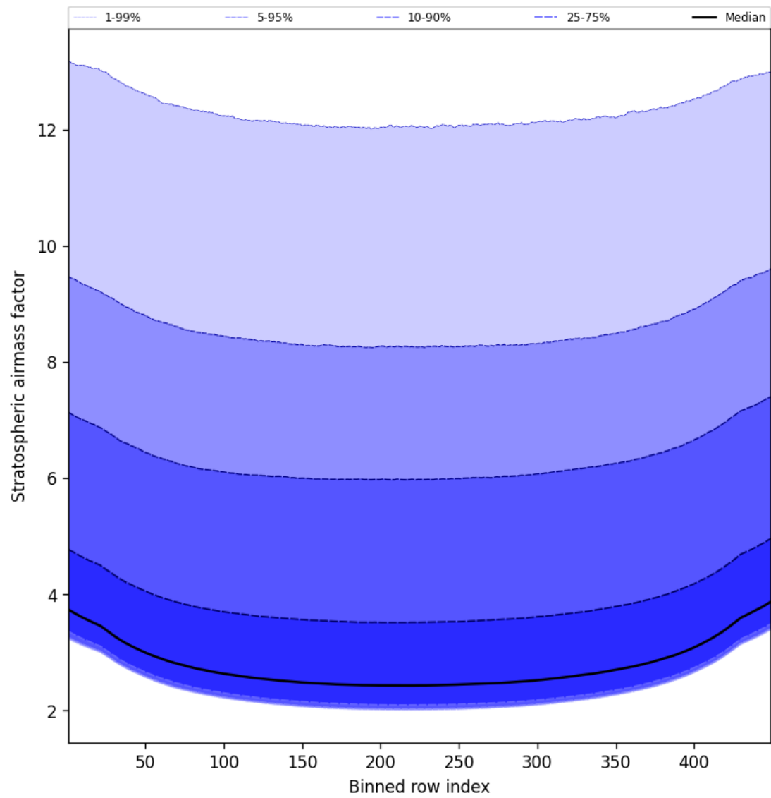
Figure 61: Along track statistics of “Stratospheric airmass factor” for 2025-05-17 to 2025-05-19
