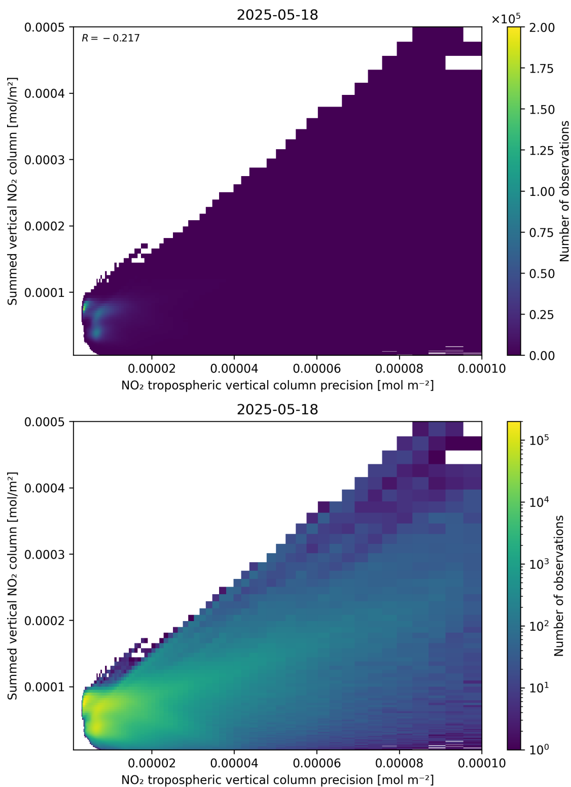
Figure 136: Scatter density plot of “NO 2 tropospheric vertical column precision” against “Summed vertical NO 2 column” for 2025-05-17 to 2025-05-19.
