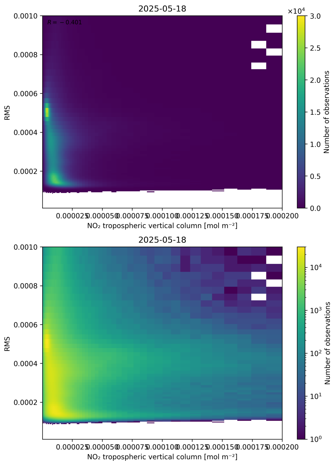
Figure 142: Scatter density plot of “NO 2 tropospheric vertical column” against “RMS” for 2025-05-17 to 2025-05-19.
