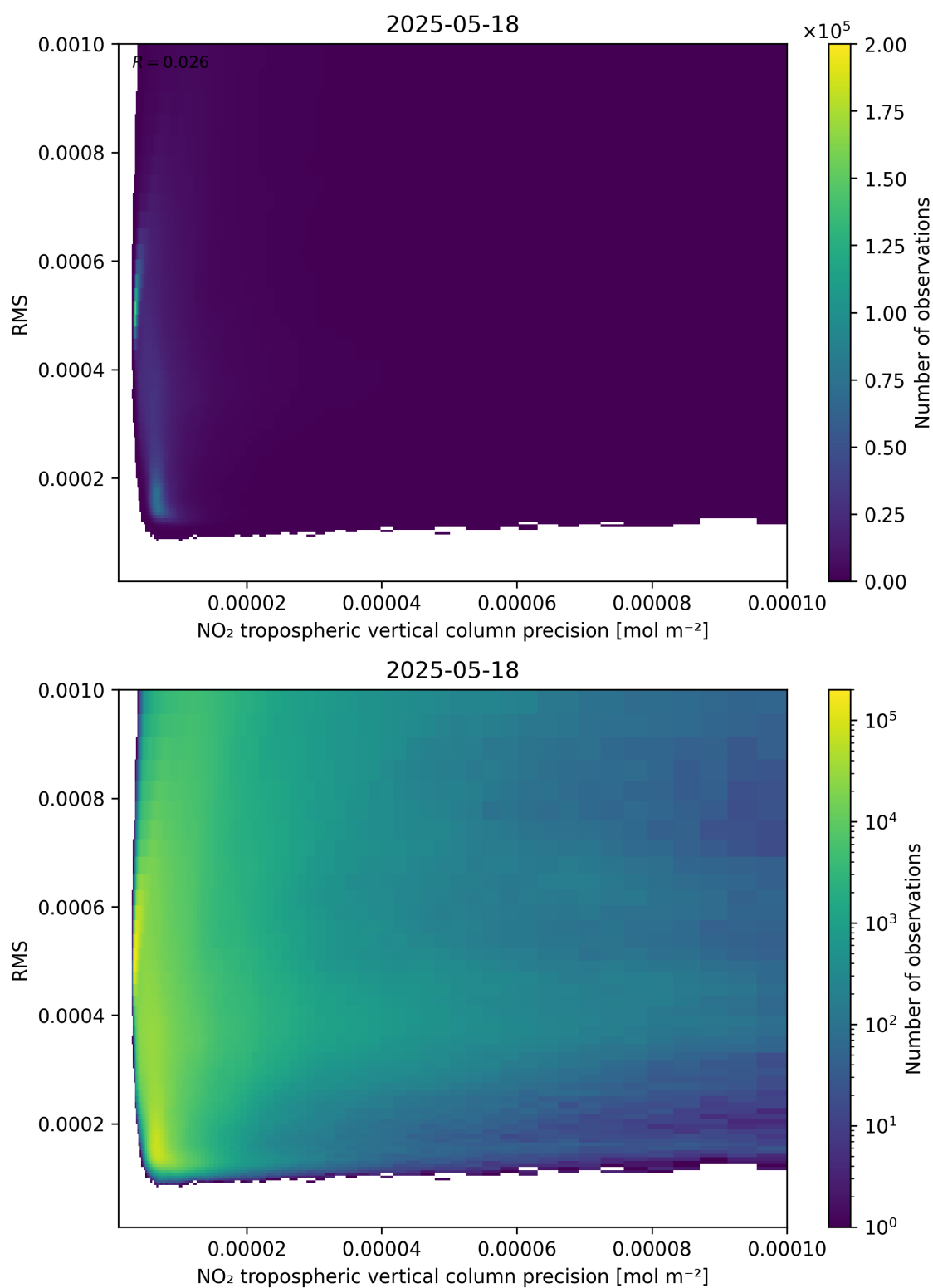
Figure 140: Scatter density plot of “NO 2 tropospheric vertical column precision” against “RMS” for 2025-05-17 to 2025-05-19.
