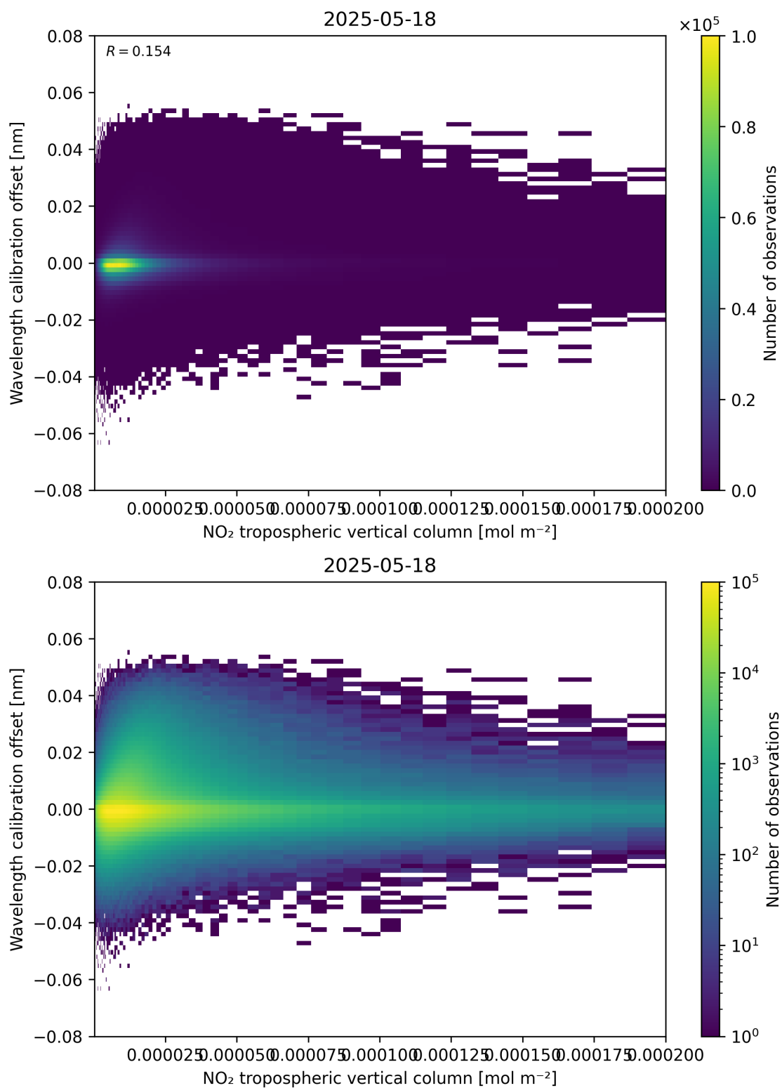
Figure 143: Scatter density plot of “NO 2 tropospheric vertical column” against “Wavelength calibration offset” for 2025-05-17 to 2025-05-19.
