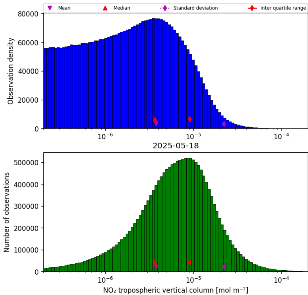
Figure 29: Histogram of “NO 2 tropospheric vertical column” for 2025-05-17 to 2025-05-19
