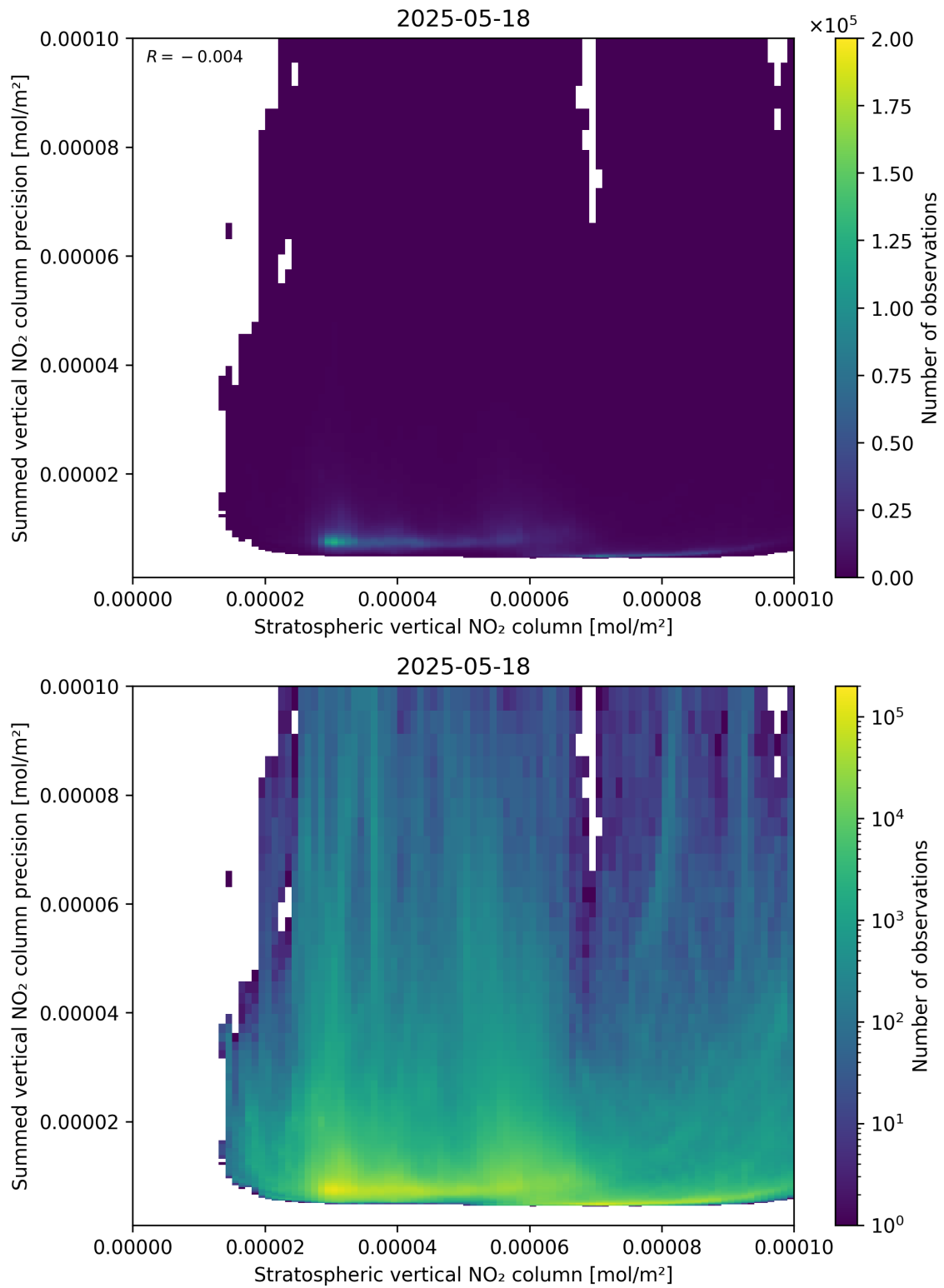
Figure 99: Scatter density plot of “Stratospheric vertical NO 2 column” against “Summed vertical NO 2 column precision” for 2025-05-17 to 2025-05-19.
