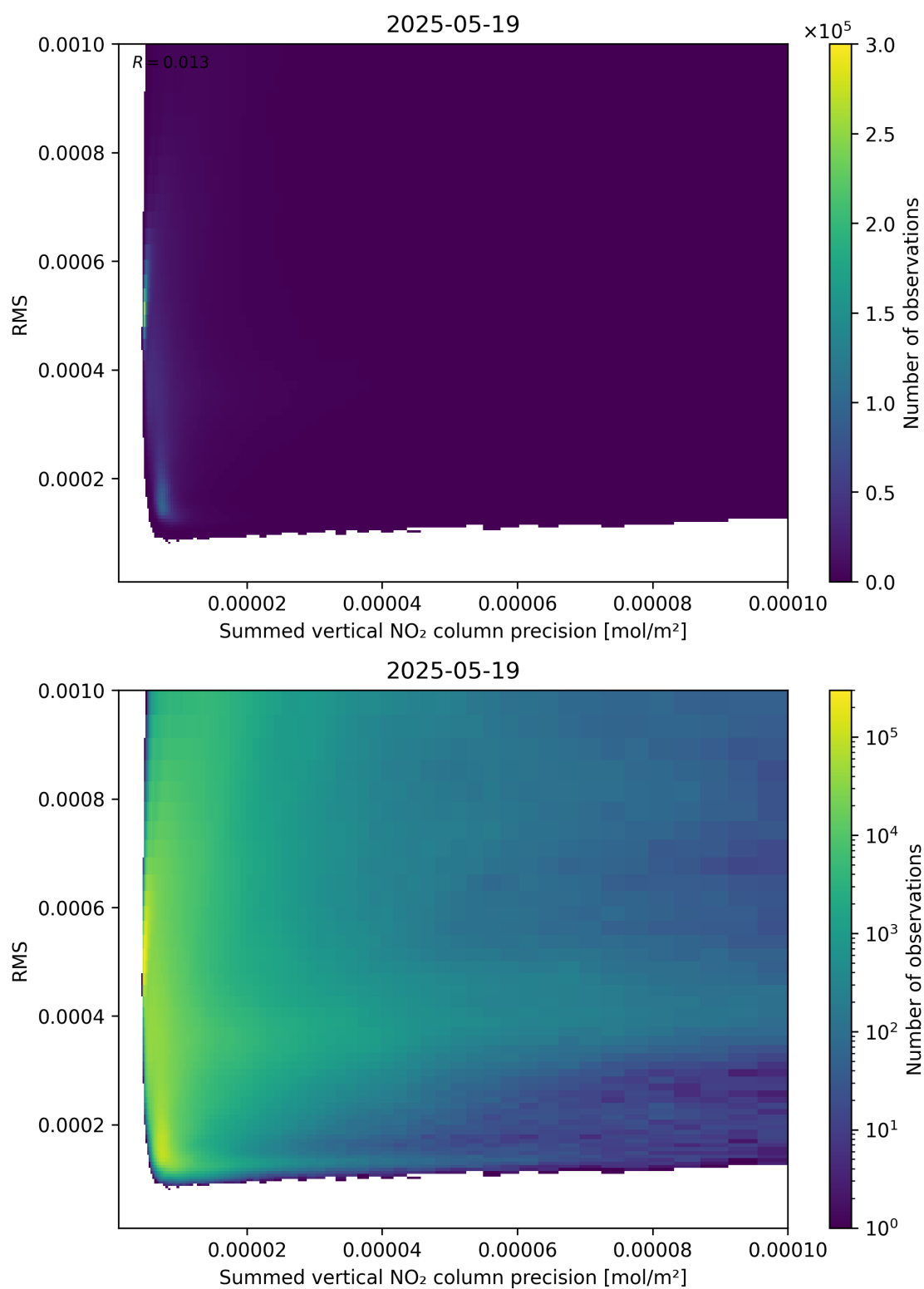
Figure 108: Scatter density plot of “Summed vertical NO 2 column precision” against “RMS” for 2025-05-18 to 2025-05-20.
