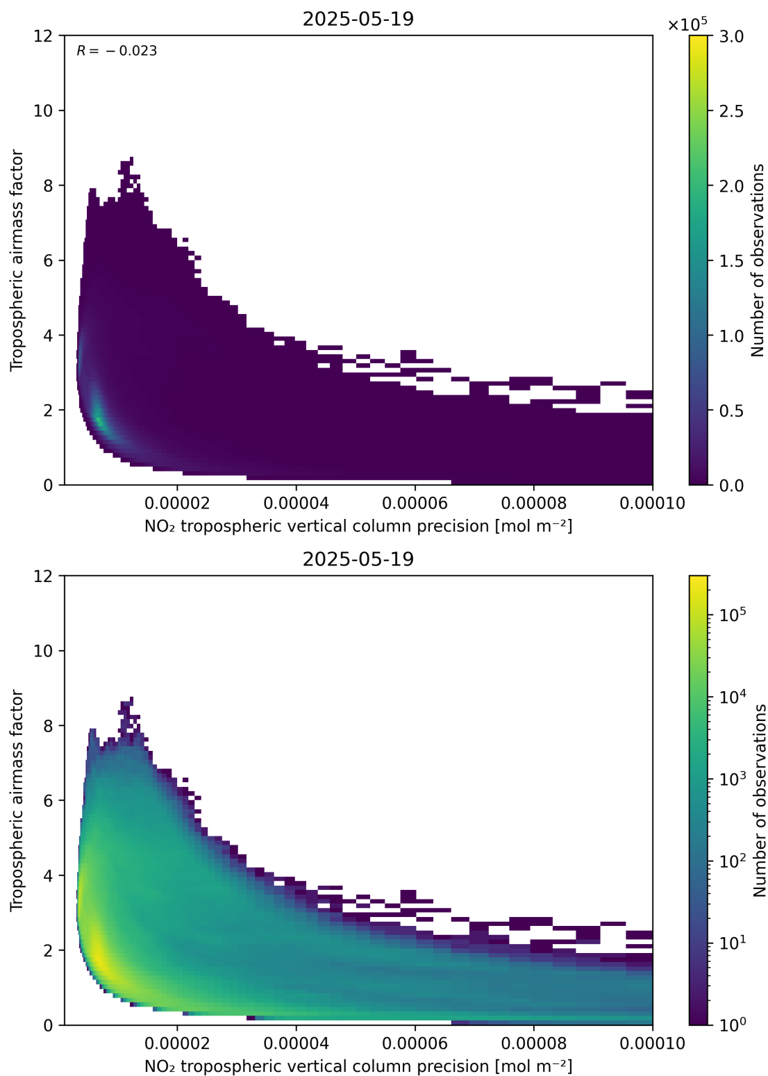
Figure 133: Scatter density plot of “NO 2 tropospheric vertical column precision” against “Tropospheric airmass factor” for 2025-05-18 to 2025-05-20.
