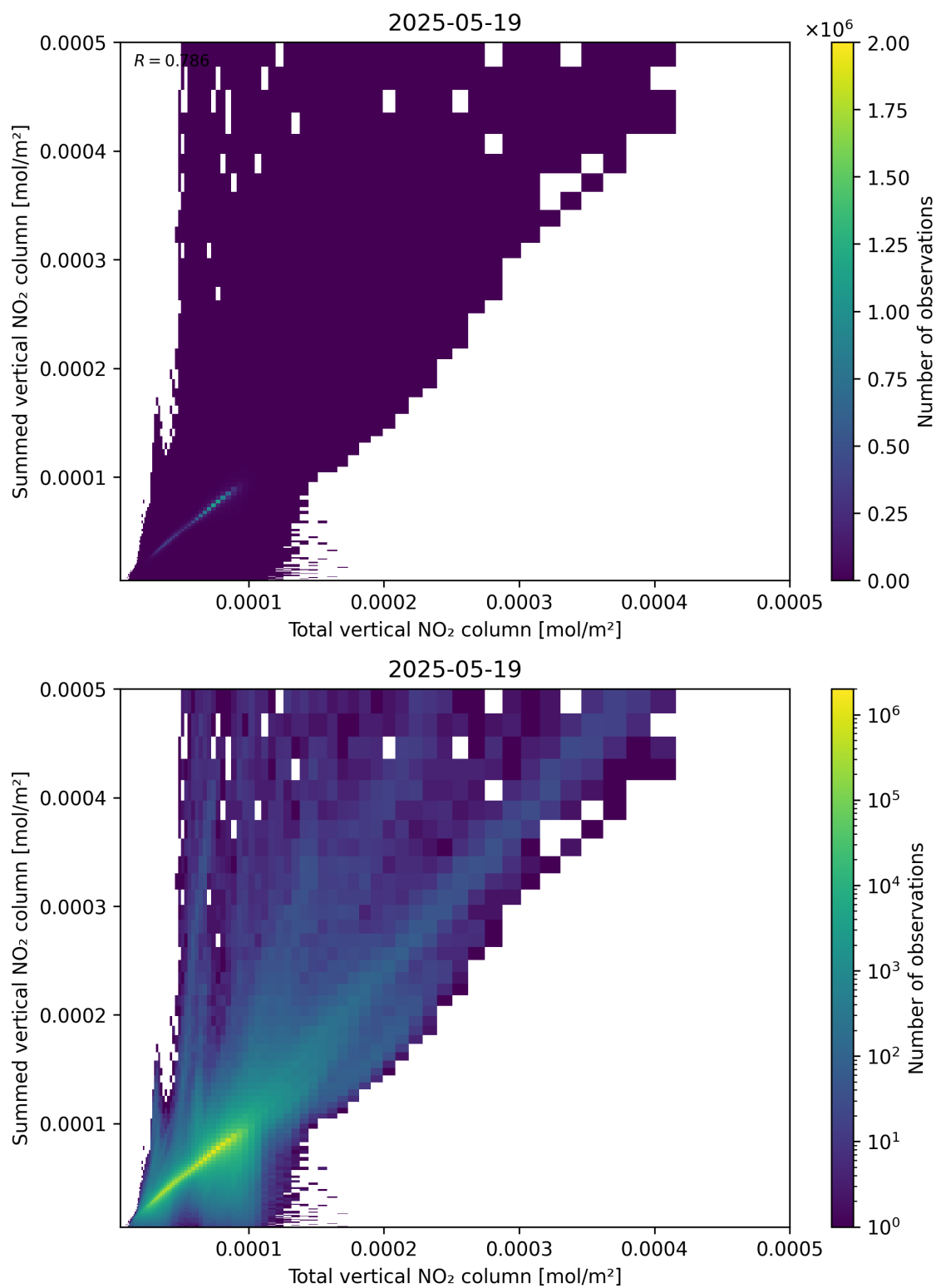
Figure 112: Scatter density plot of “Total vertical NO 2 column” against “Summed vertical NO 2 column” for 2025-05-18 to 2025-05-20.
