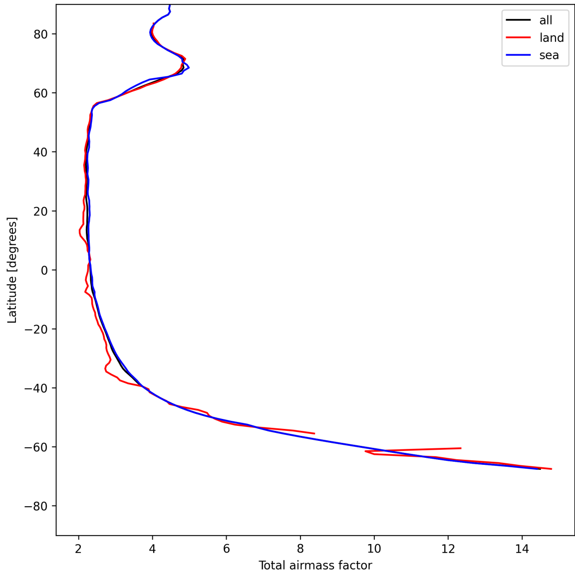
Figure 15: Zonal average of “Total airmass factor” for 2025-05-18 to 2025-05-20.
