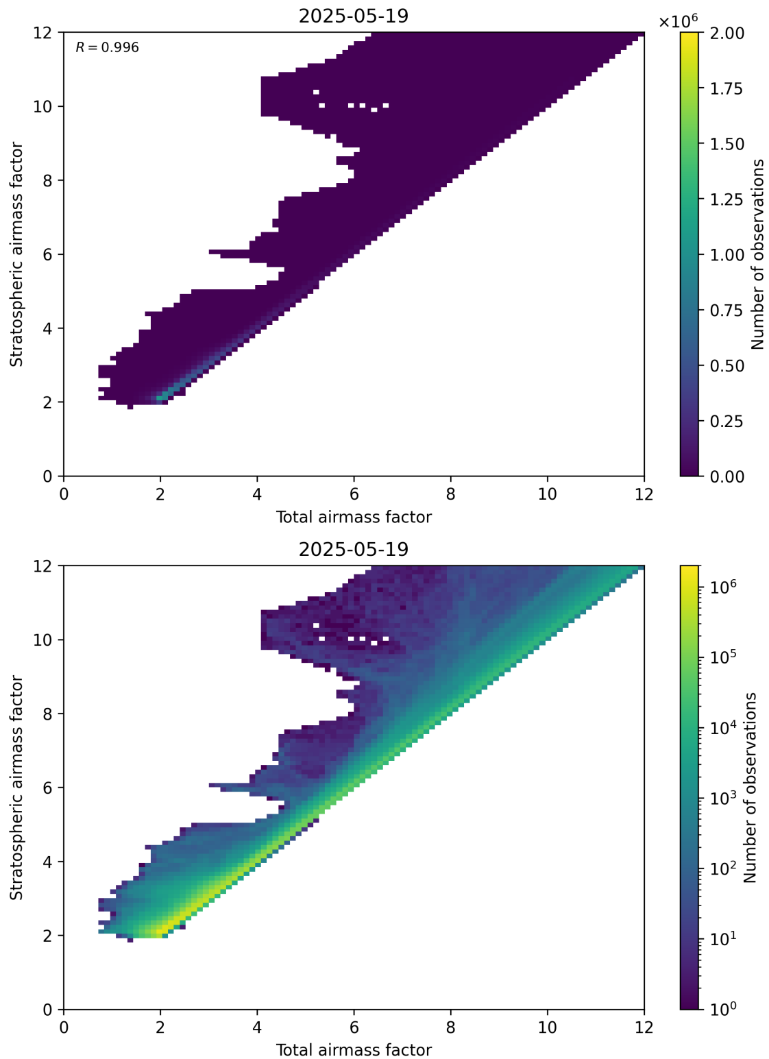
Figure 62: Scatter density plot of “Total airmass factor” against “Stratospheric airmass factor” for 2025-05-18 to 2025-05-20.
