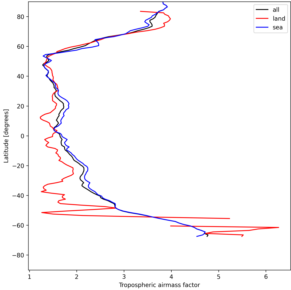
Figure 14: Zonal average of “Tropospheric airmass factor” for 2025-05-18 to 2025-05-20.
