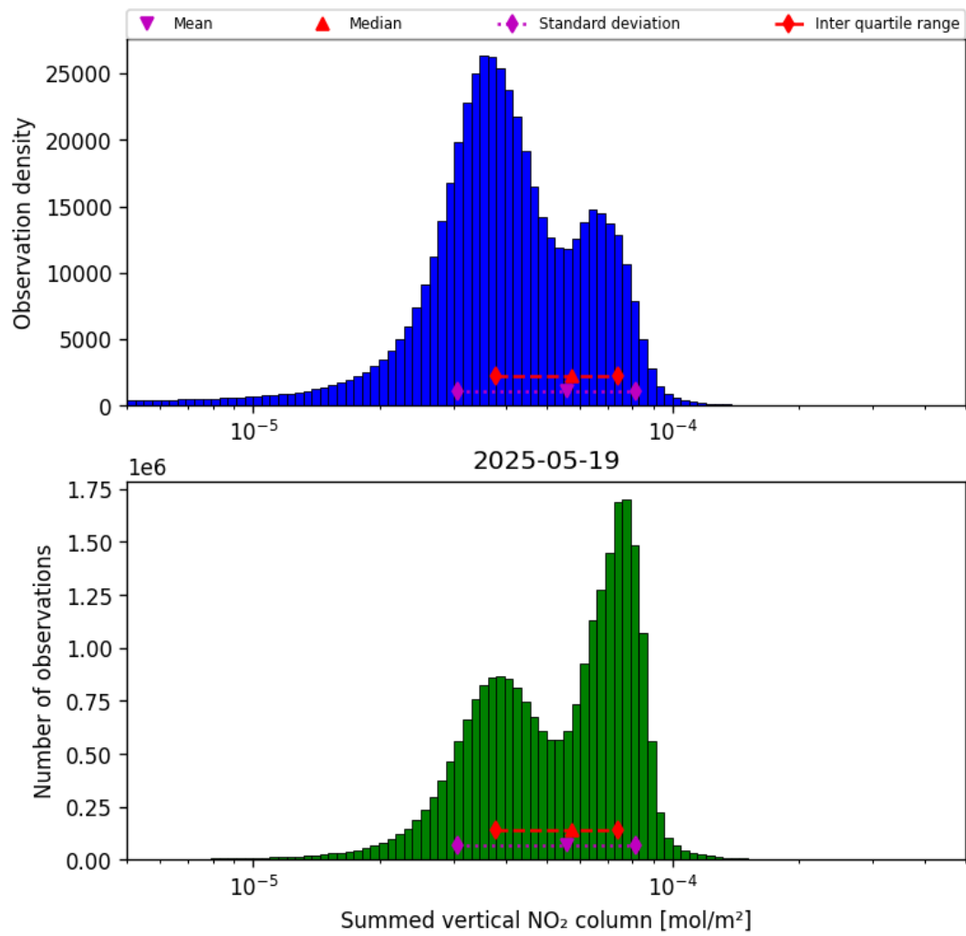
Figure 40: Histogram of “Summed vertical NO 2 column” for 2025-05-18 to 2025-05-20
