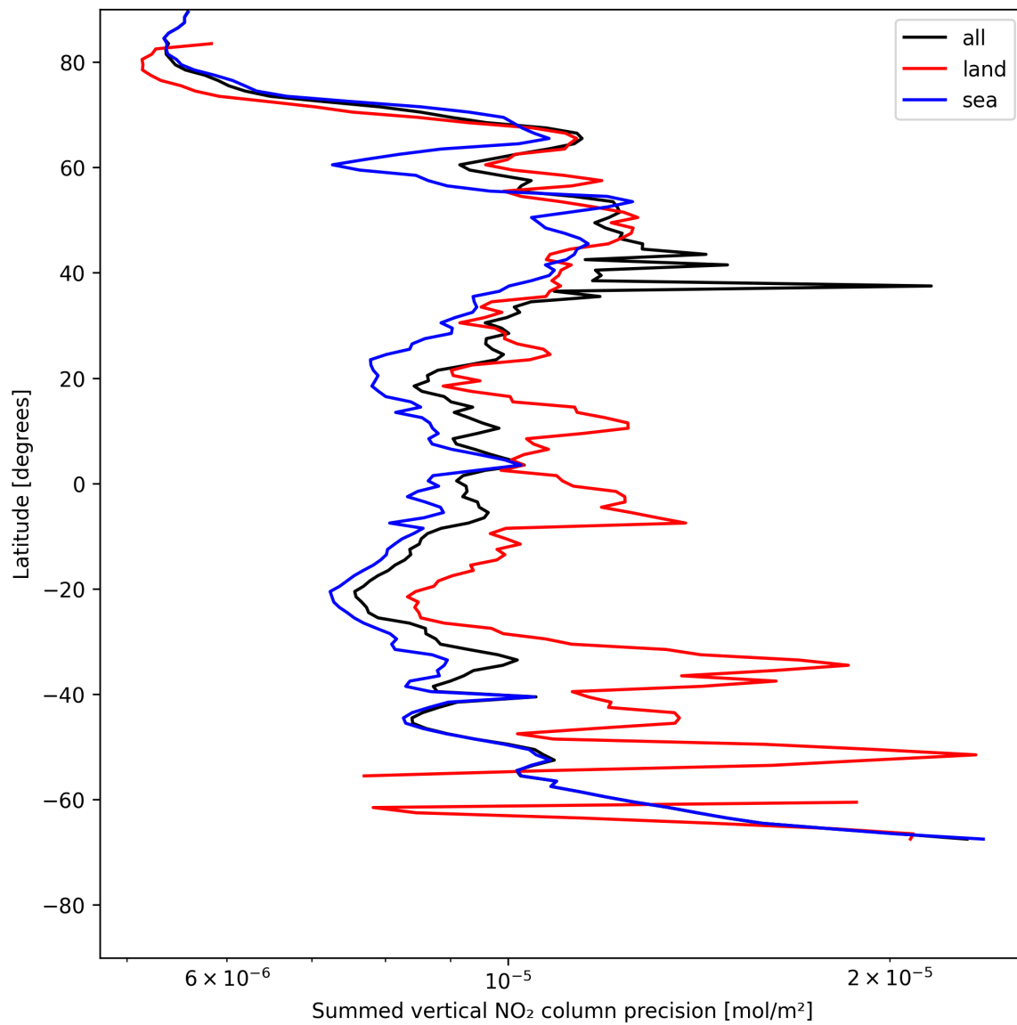
Figure 24: Zonal average of “Summed vertical NO 2 column precision” for 2025-05-18 to 2025-05-20.
