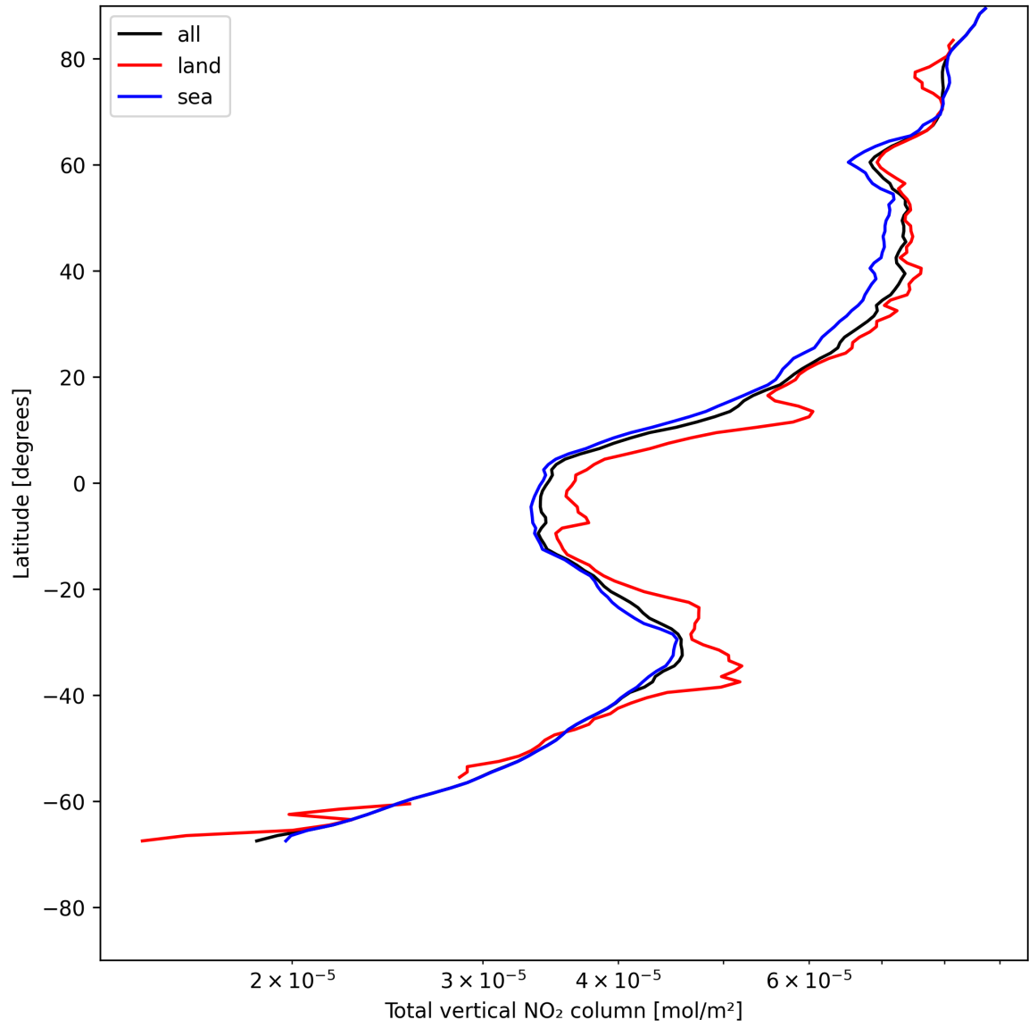
Figure 21: Zonal average of “Total vertical NO 2 column” for 2025-05-18 to 2025-05-20.
