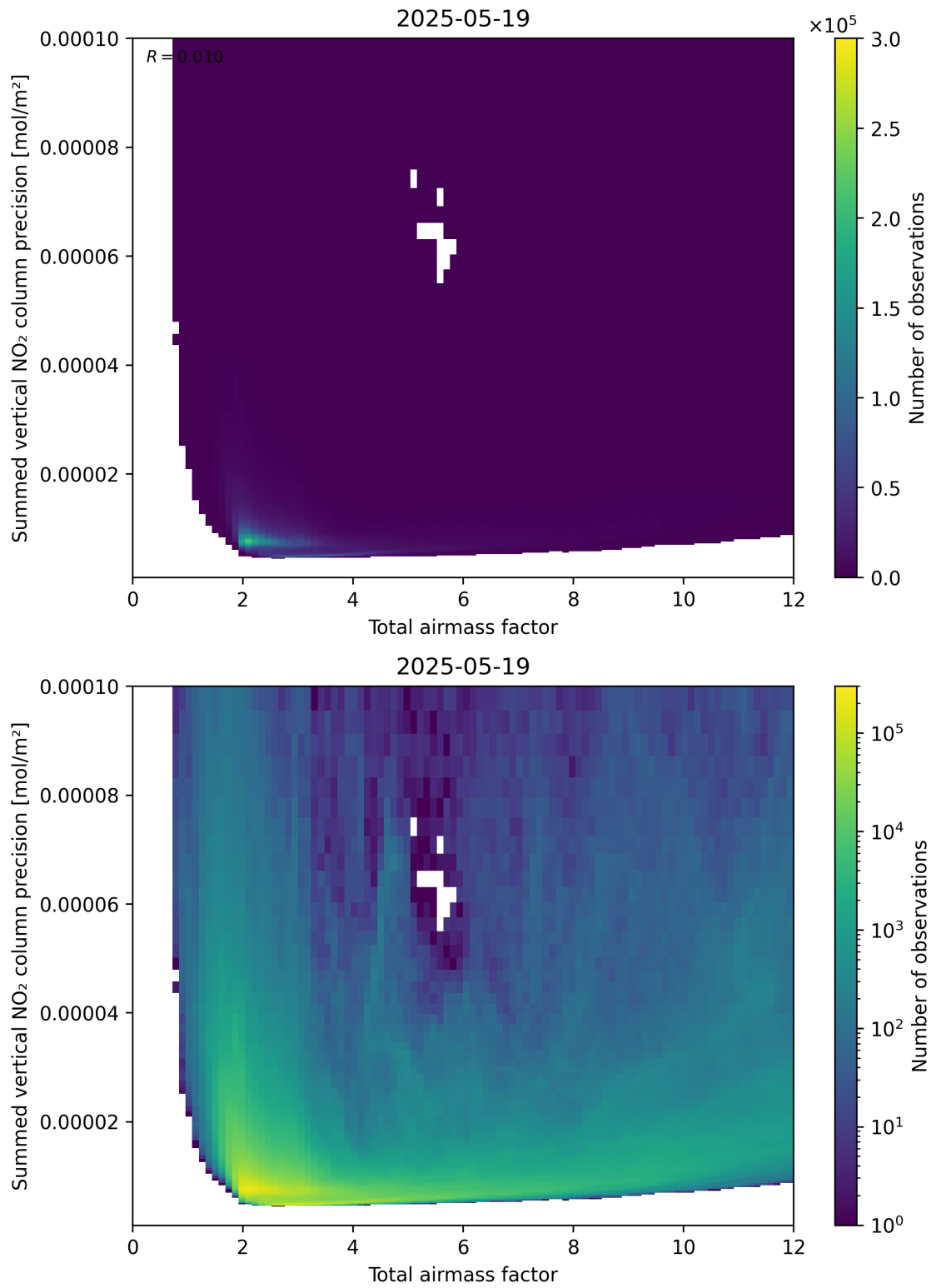
Figure 66: Scatter density plot of “Total airmass factor” against “Summed vertical NO 2 column precision” for 2025-05-18 to 2025-05-20.
