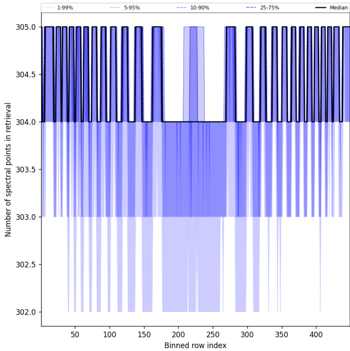
Figure 50: Along track statistics of “Number of spectral points in retrieval” for 2025-05-18 to 2025-05-20
