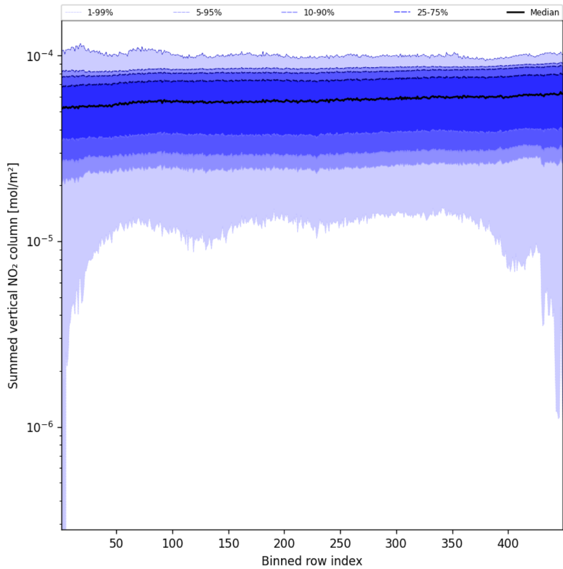
Figure 57: Along track statistics of “Summed vertical NO 2 column” for 2025-05-18 to 2025-05-20
