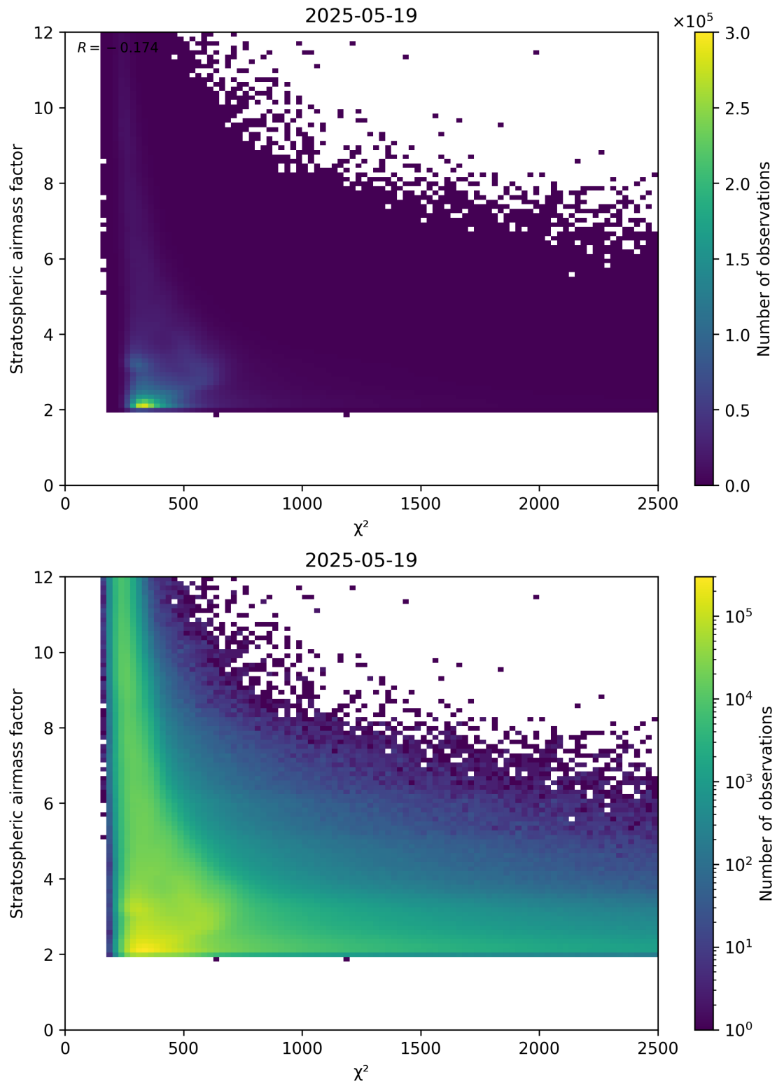
Figure 81: Scatter density plot of “ \chi^2 ” against “Stratospheric airmass factor” for 2025-05-18 to 2025-05-20.
