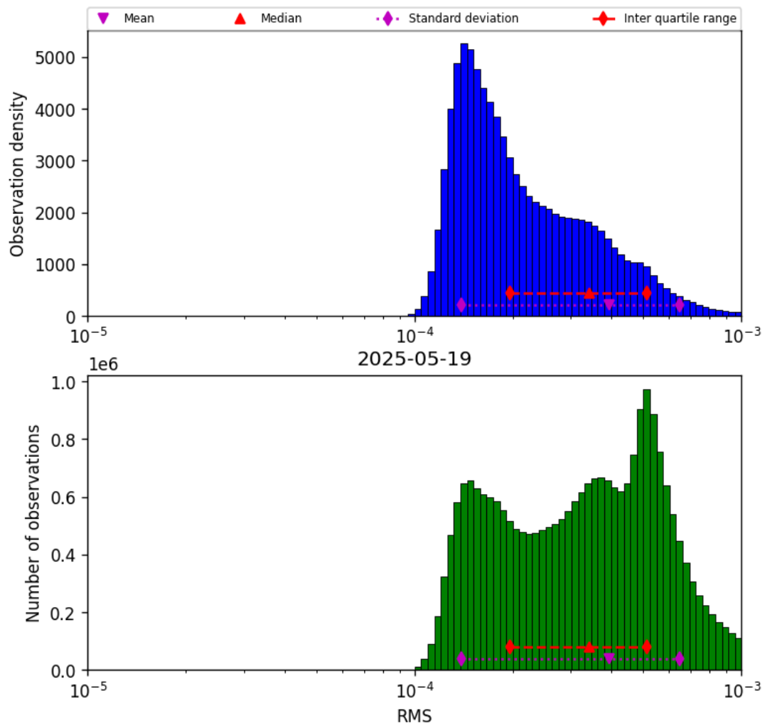
Figure 43: Histogram of “RMS” for 2025-05-18 to 2025-05-20
