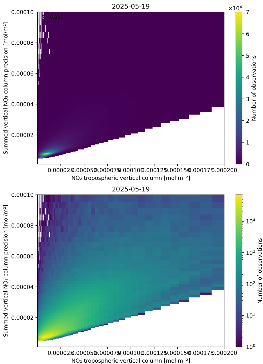
Figure 127: Scatter density plot of “NO 2 tropospheric vertical column” against “Summed vertical NO 2 column precision” for 2025-05-18 to 2025-05-20.
