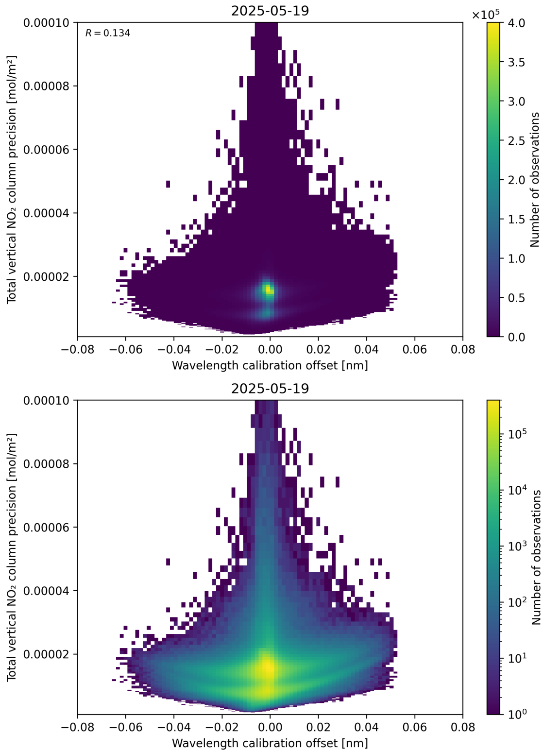
Figure 180: Scatter density plot of “Wavelength calibration offset” against “Total vertical NO 2 column precision” for 2025-05-18 to 2025-05-20.
