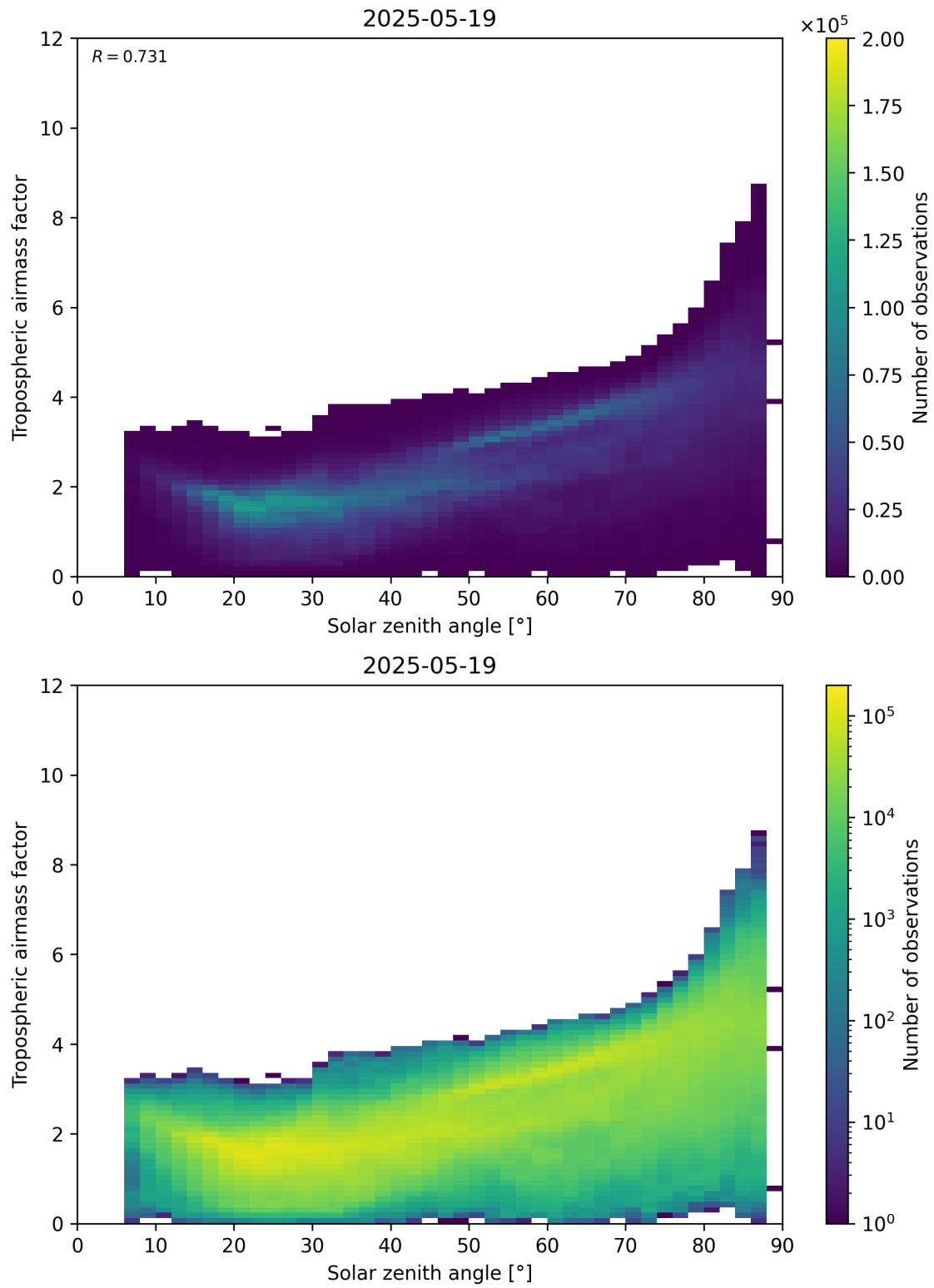
Figure 147: Scatter density plot of “Solar zenith angle” against “Tropospheric airmass factor” for 2025-05-18 to 2025-05-20.
