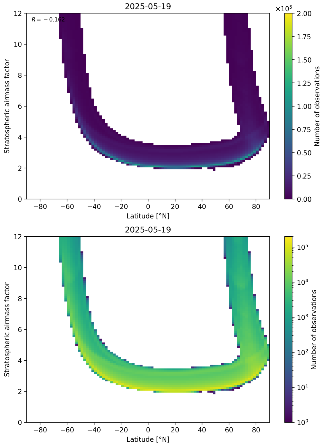
Figure 83: Scatter density plot of “Latitude” against “Stratospheric air mass factor” for 2025-05-18 to 2025-05-20.
