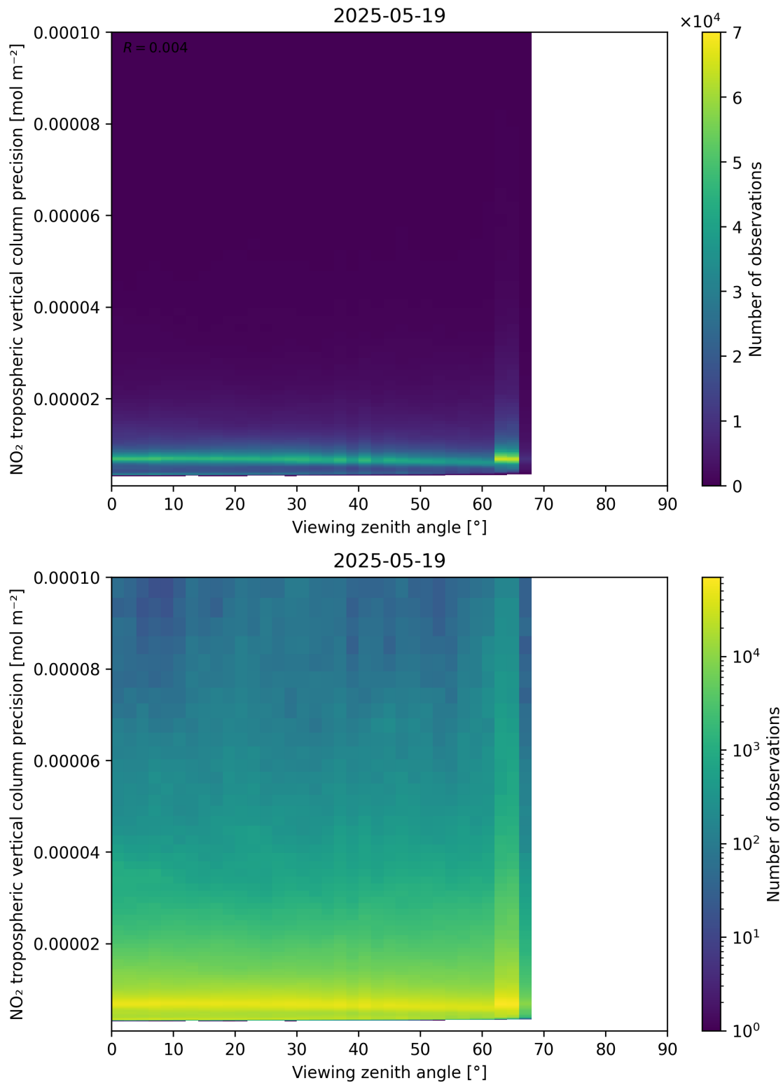
Figure 170: Scatter density plot of “Viewing zenith angle” against “NO 2 tropospheric vertical column precision” for 2025-05-18 to 2025-05-20.
