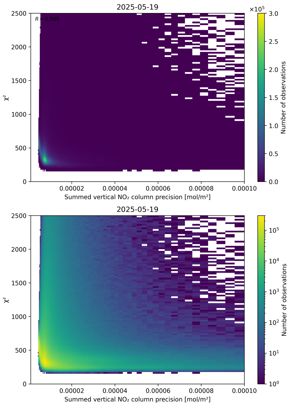
Figure 107: Scatter density plot of “Summed vertical NO 2 column precision” against “ \chi^2 ” for 2025-05-18 to 2025-05-20.
