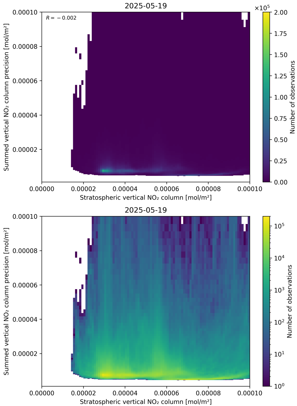
Figure 99: Scatter density plot of “Stratospheric vertical NO 2 column” against “Summed vertical NO 2 column precision” for 2025-05-18 to 2025-05-20.
