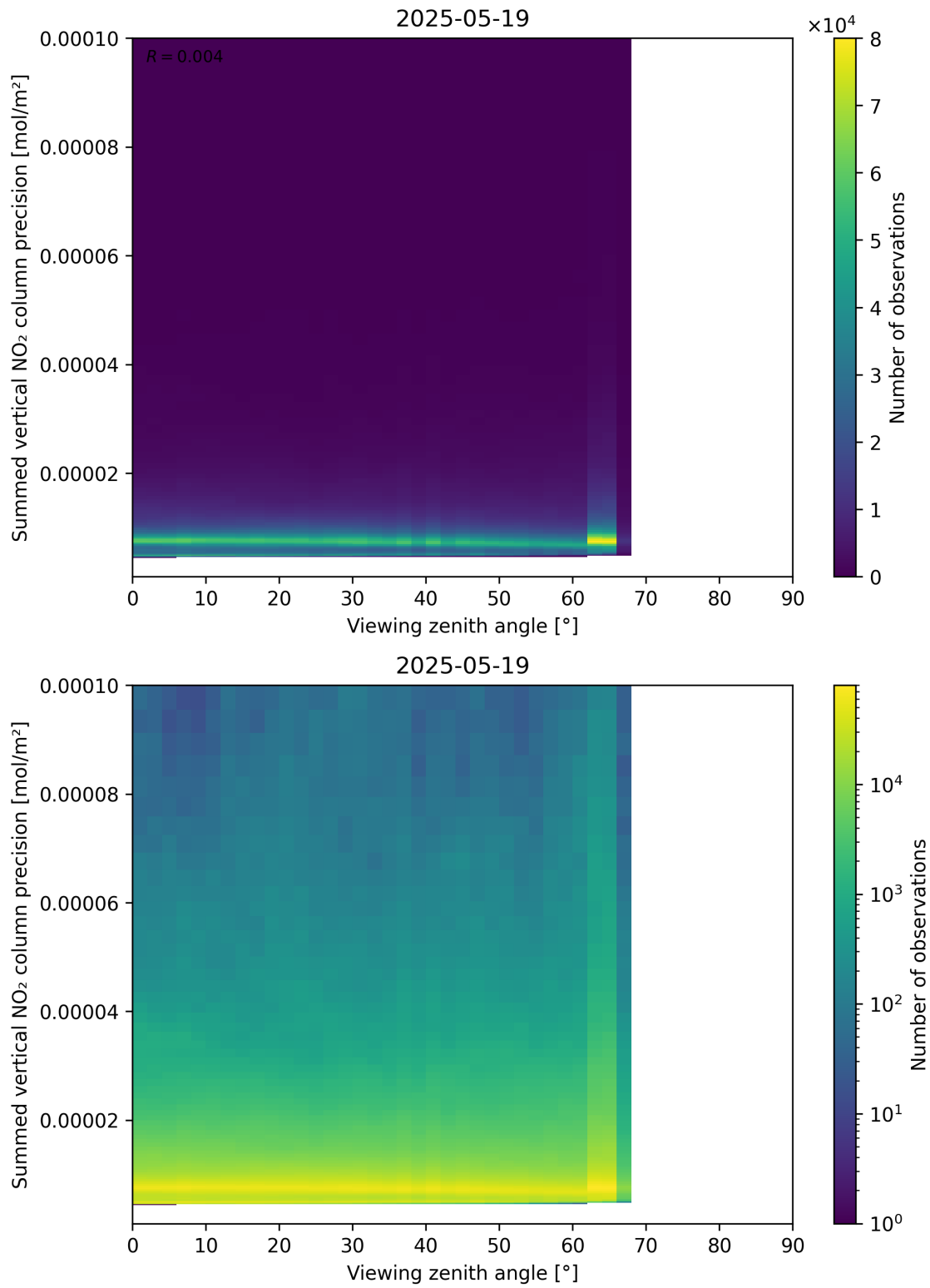
Figure 166: Scatter density plot of “Viewing zenith angle” against “Summed vertical NO 2 column precision” for 2025-05-18 to 2025-05-20.
