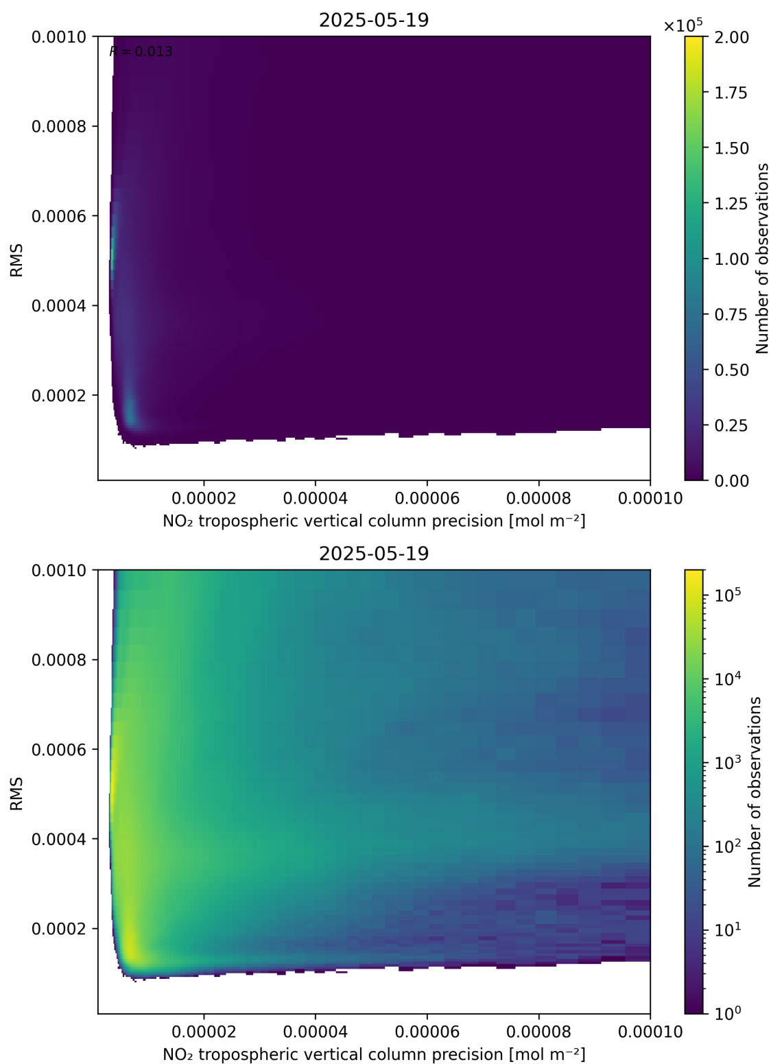
Figure 140: Scatter density plot of “NO 2 tropospheric vertical column precision” against “RMS” for 2025-05-18 to 2025-05-20.
