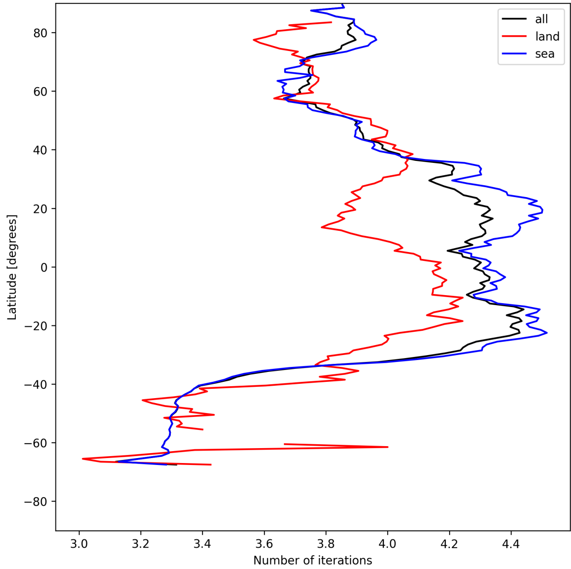
Figure 17: Zonal average of “Number of iterations” for 2025-05-18 to 2025-05-20.
