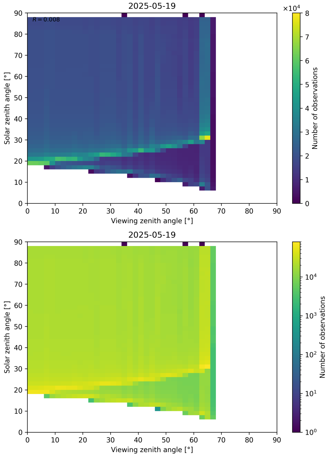
Figure 172: Scatter density plot of “Viewing zenith angle” against “Solar zenith angle” for 2025-05-18 to 2025-05-20.
