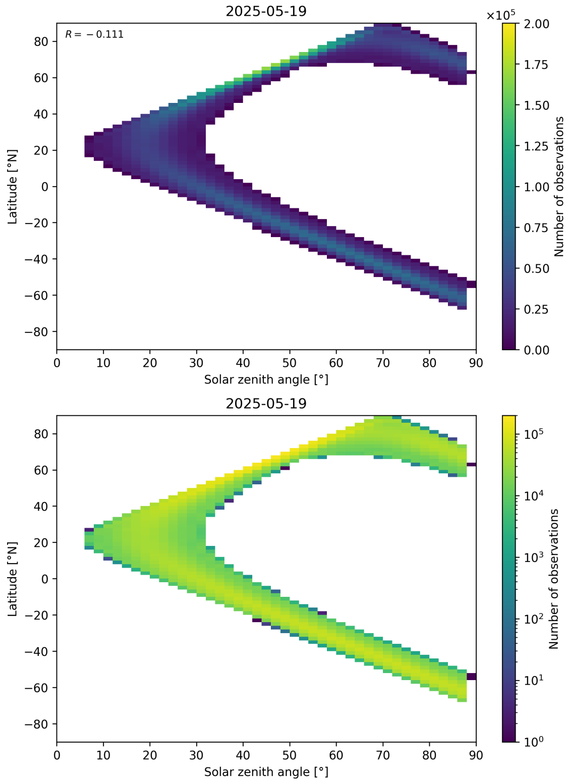
Figure 149: Scatter density plot of “Solar zenith angle” against “Latitude” for 2025-05-18 to 2025-05-20.
