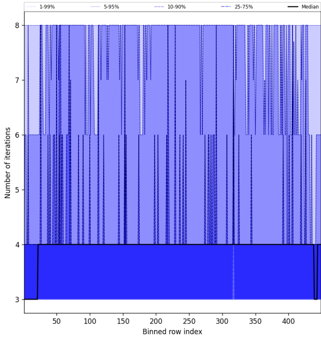
Figure 51: Along track statistics of “Number of iterations” for 2025-05-18 to 2025-05-20
