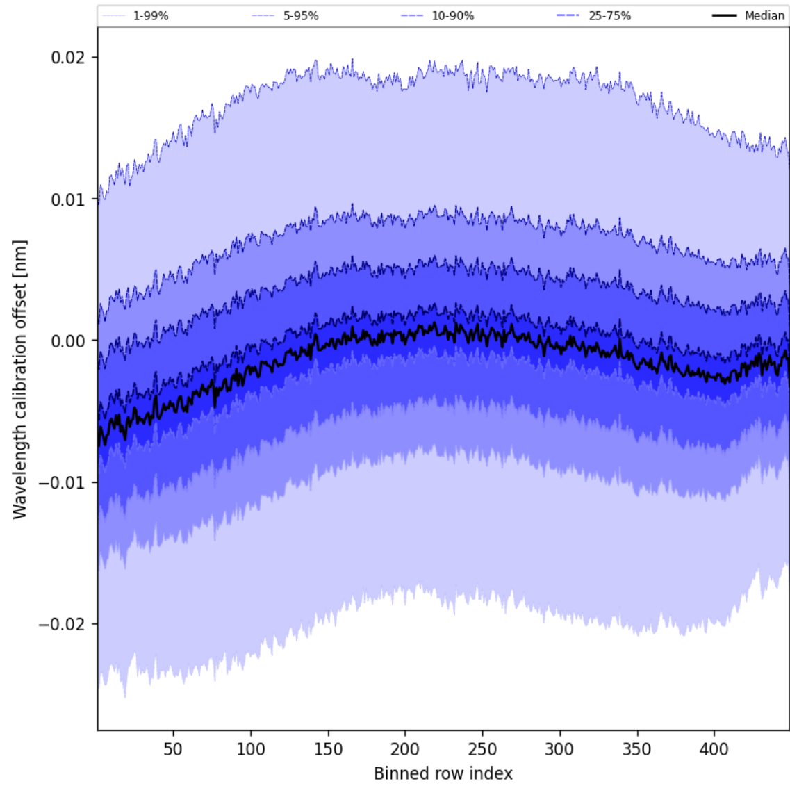
Figure 52: Along track statistics of “Wavelength calibration offset” for 2025-05-18 to 2025-05-20
