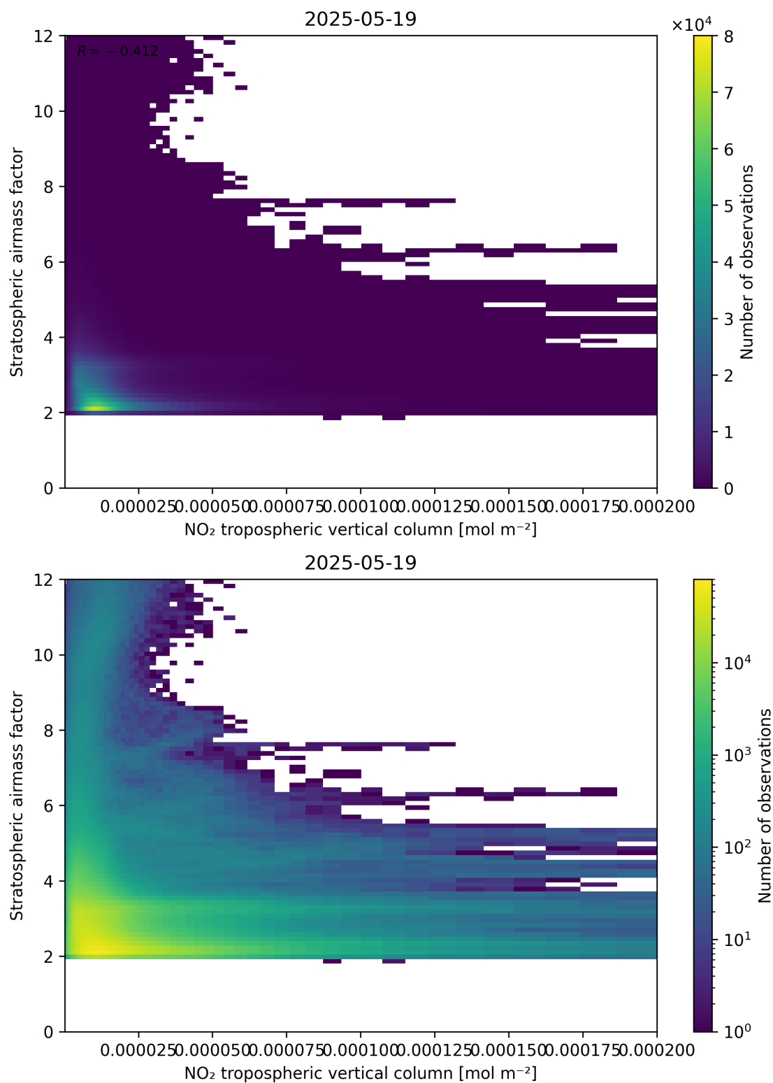
Figure 121: Scatter density plot of “NO 2 tropospheric vertical column” against “Stratospheric air mass factor” for 2025-05-18 to 2025-05-20.
