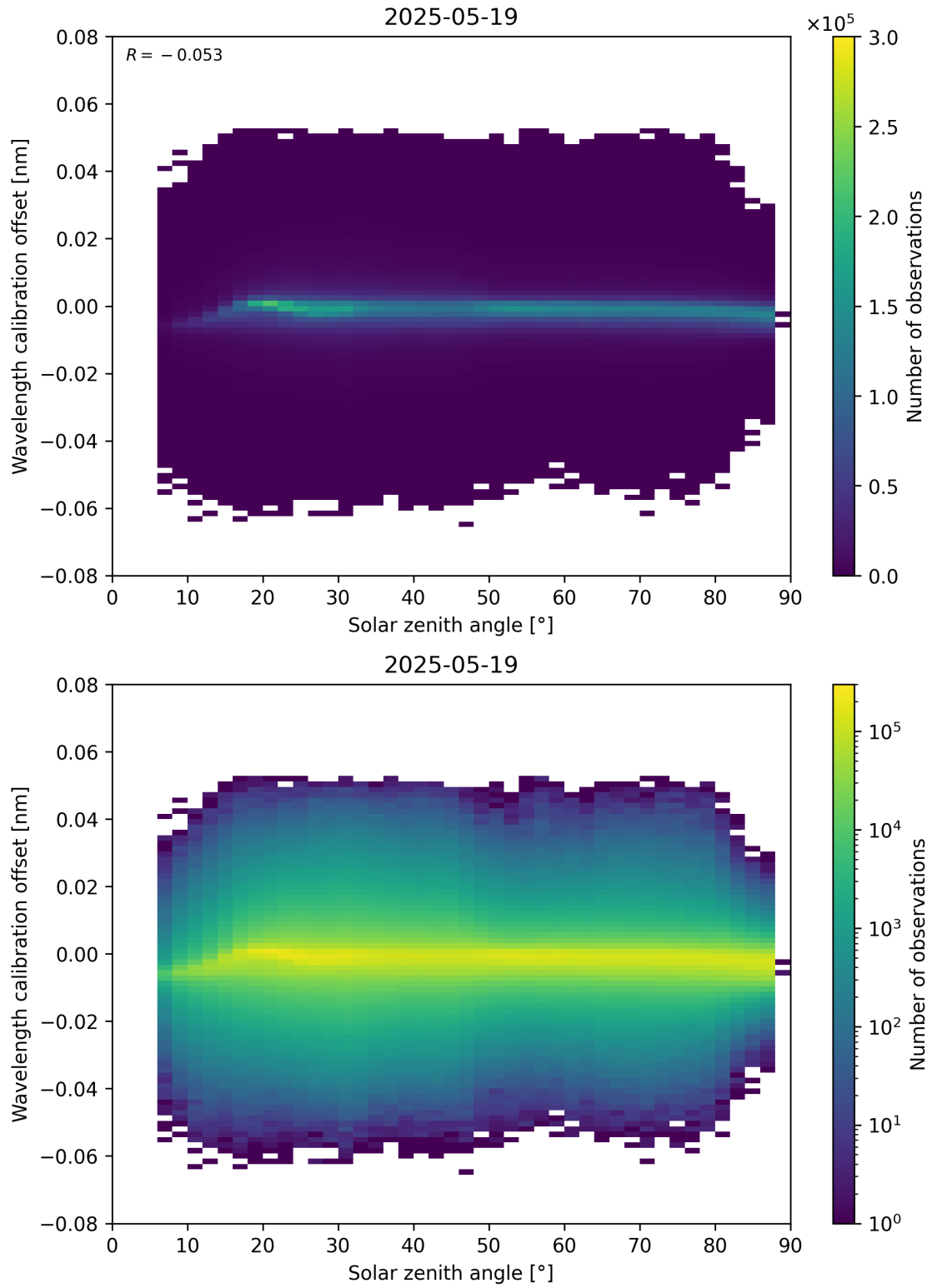
Figure 158: Scatter density plot of “Solar zenith angle” against “Wavelength calibration offset” for 2025-05-18 to 2025-05-20.
