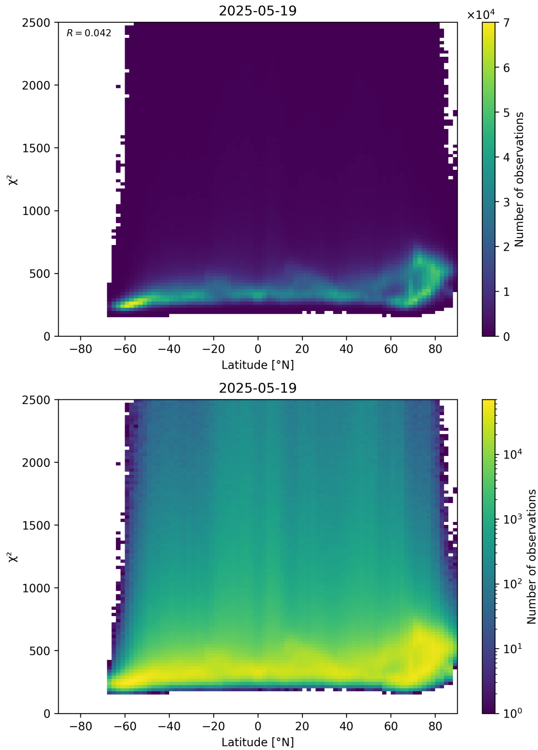
Figure 86: Scatter density plot of “Latitude” against “ \chi^2 ” for 2025-05-18 to 2025-05-20.
