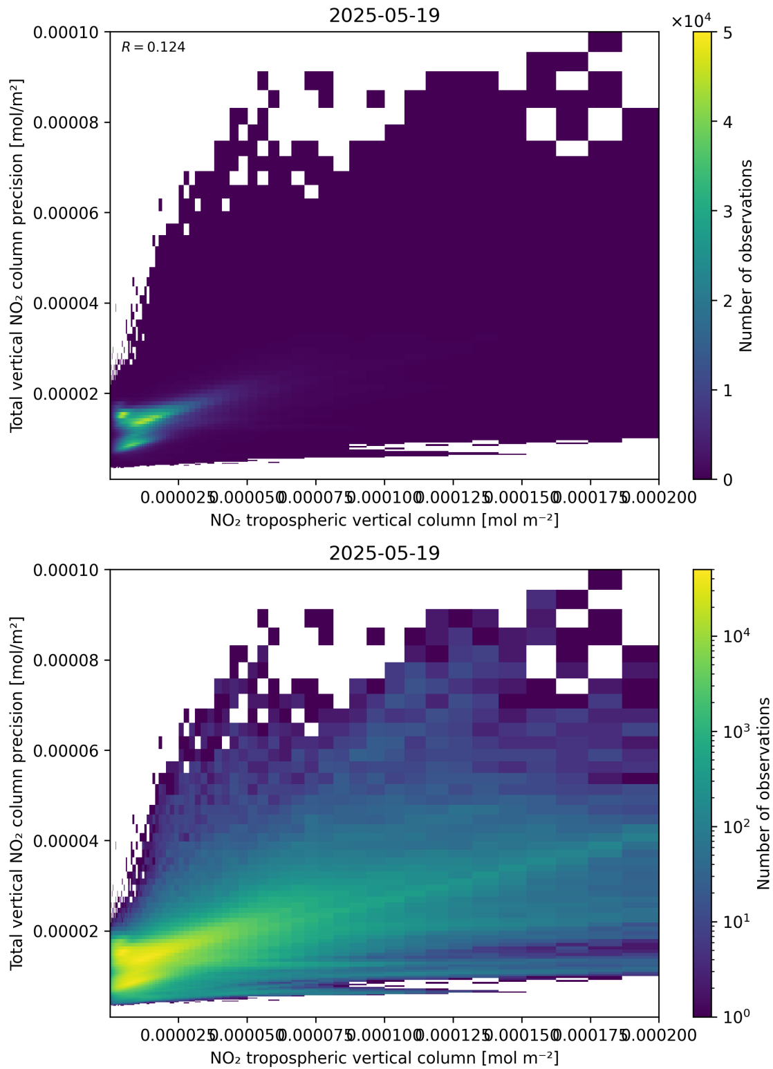
Figure 129: Scatter density plot of “NO 2 tropospheric vertical column” against “Total vertical NO 2 column precision” for 2025-05-18 to 2025-05-20.
