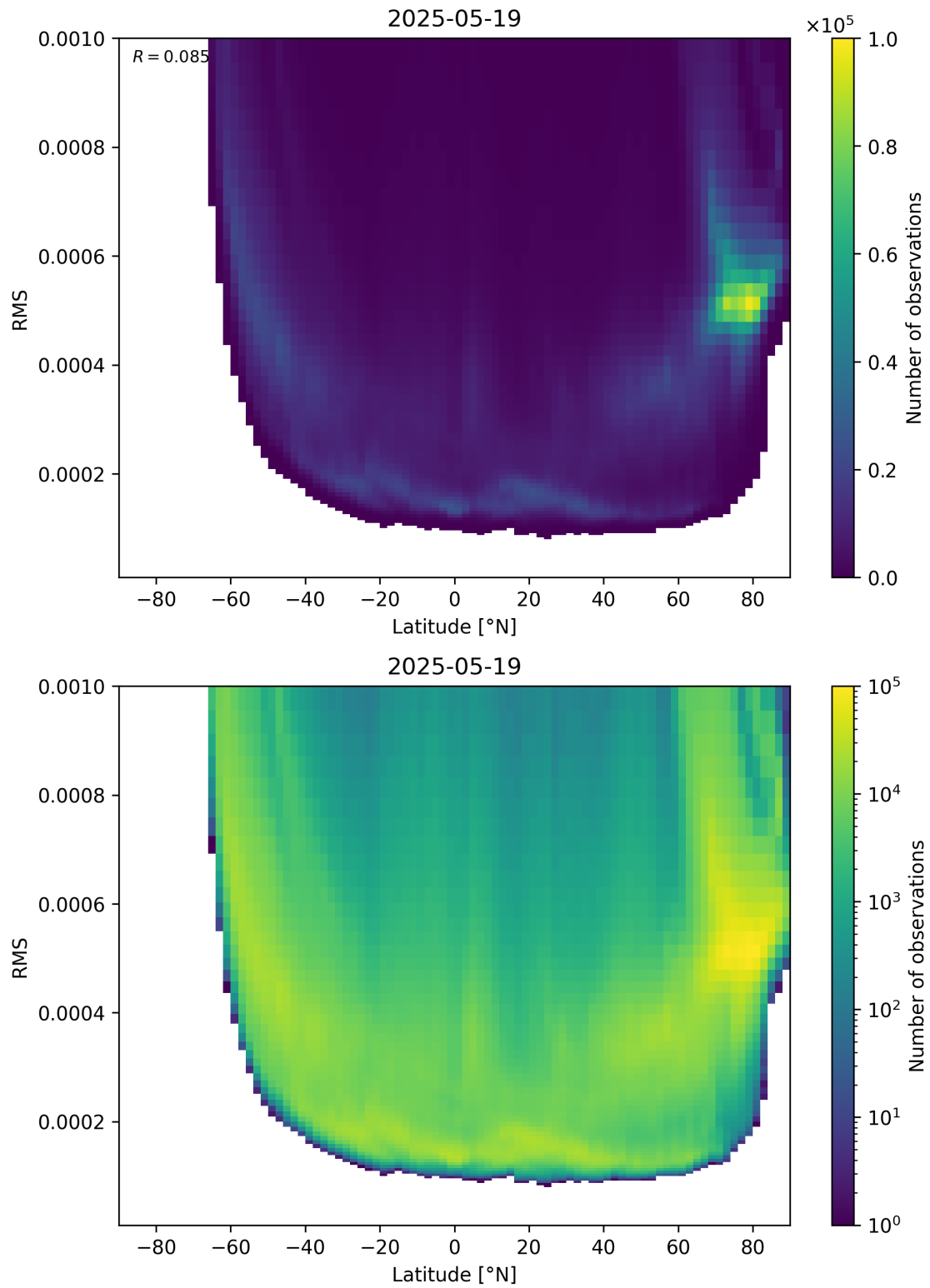
Figure 94: Scatter density plot of “Latitude” against “RMS” for 2025-05-18 to 2025-05-20.
