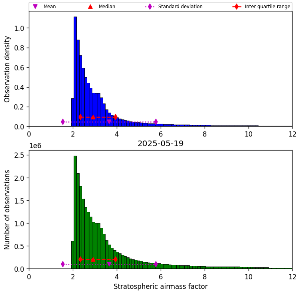
Figure 44: Histogram of “Stratospheric airmass factor” for 2025-05-18 to 2025-05-20
