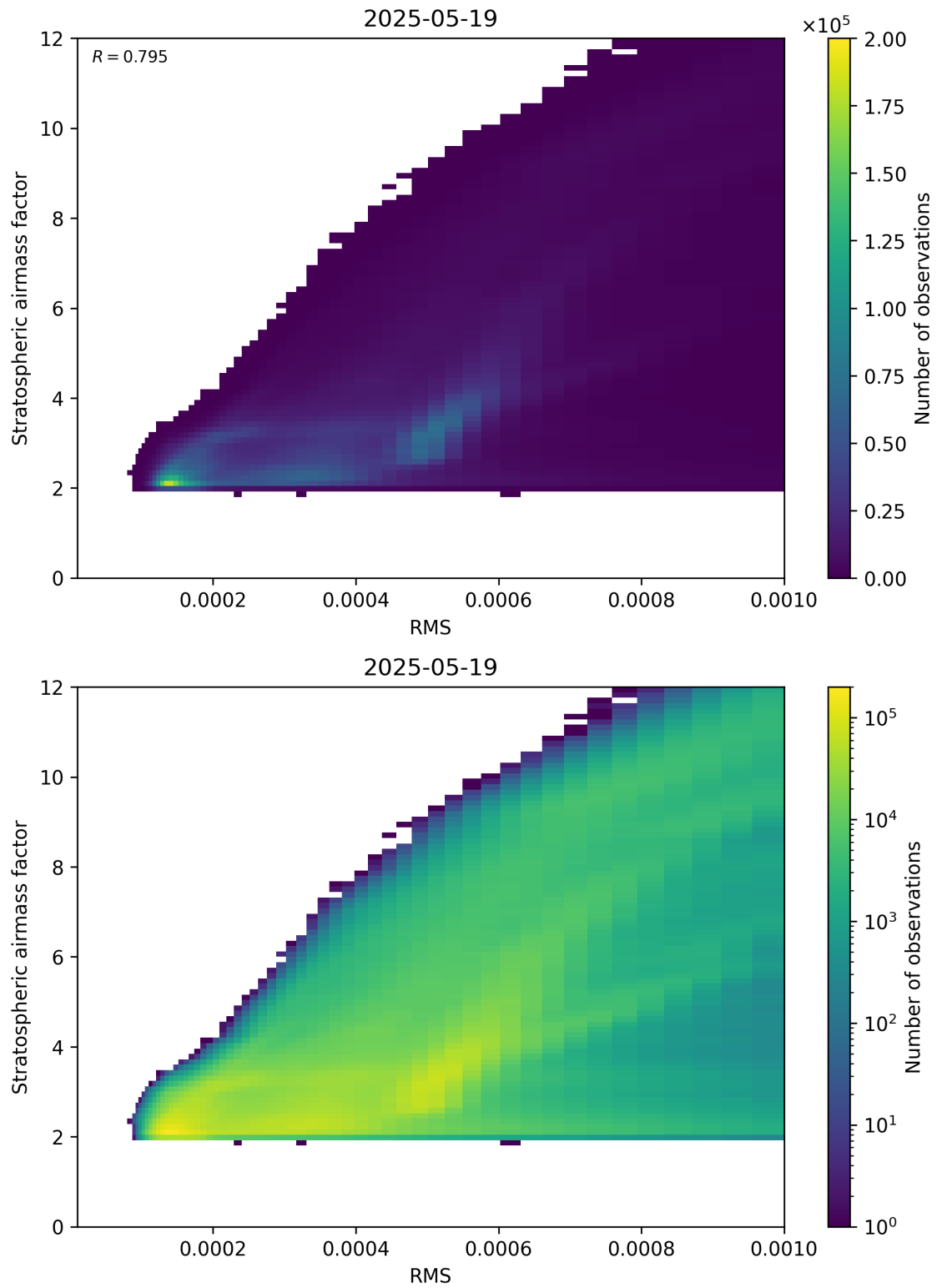
Figure 144: Scatter density plot of “RMS” against “Stratospheric airmass factor” for 2025-05-18 to 2025-05-20.
