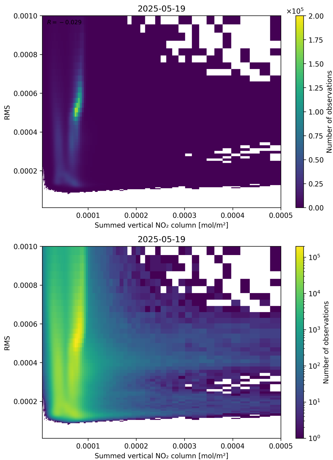
Figure 109: Scatter density plot of “Summed vertical NO 2 column” against “RMS” for 2025-05-18 to 2025-05-20.
