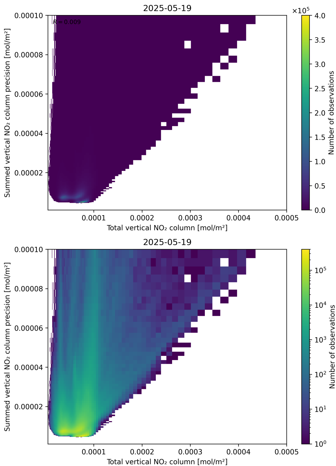
Figure 113: Scatter density plot of “Total vertical NO 2 column” against “Summed vertical NO 2 column precision” for 2025-05-18 to 2025-05-20.
