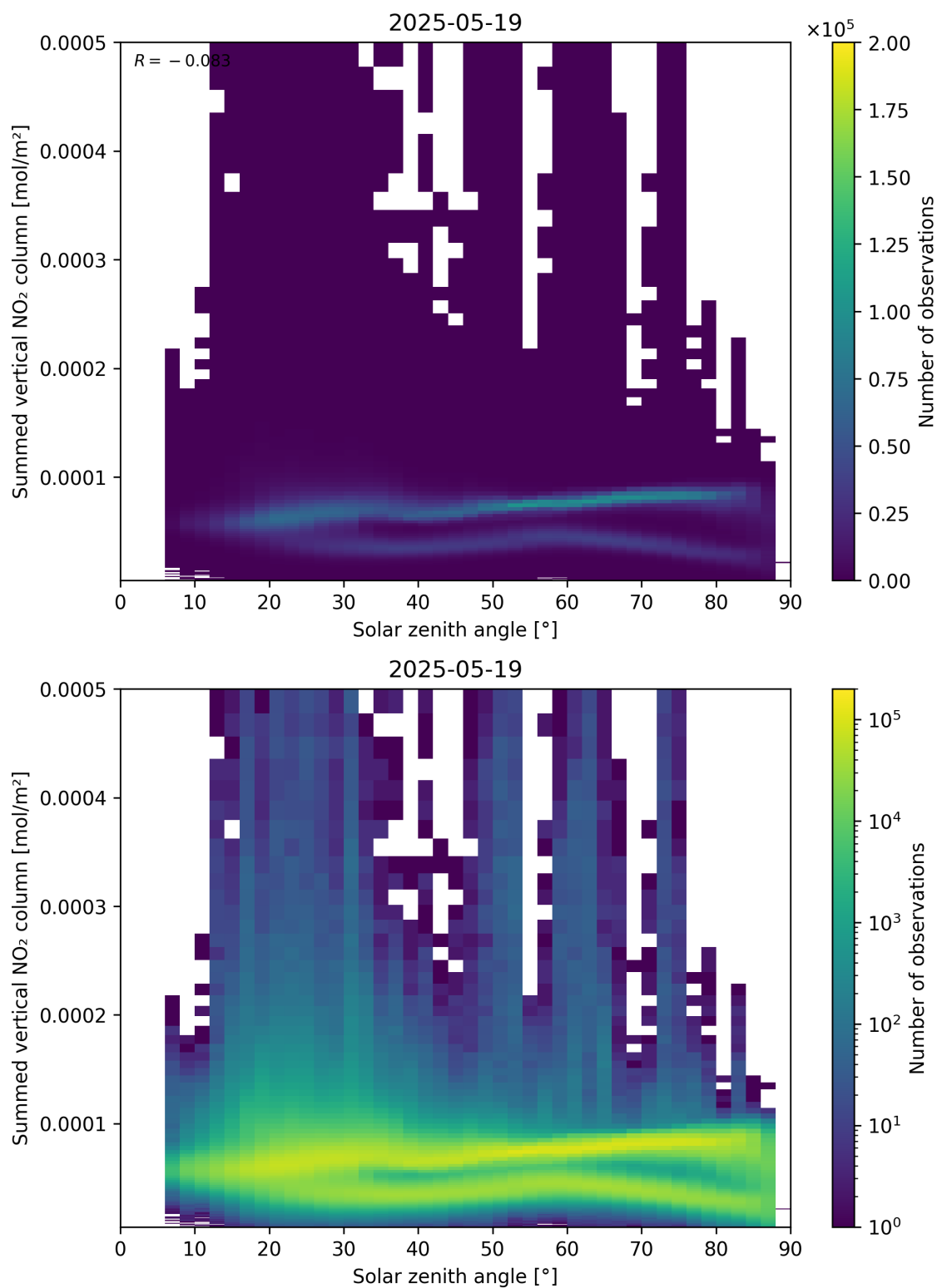
Figure 151: Scatter density plot of “Solar zenith angle” against “Summed vertical NO 2 column” for 2025-05-18 to 2025-05-20.
