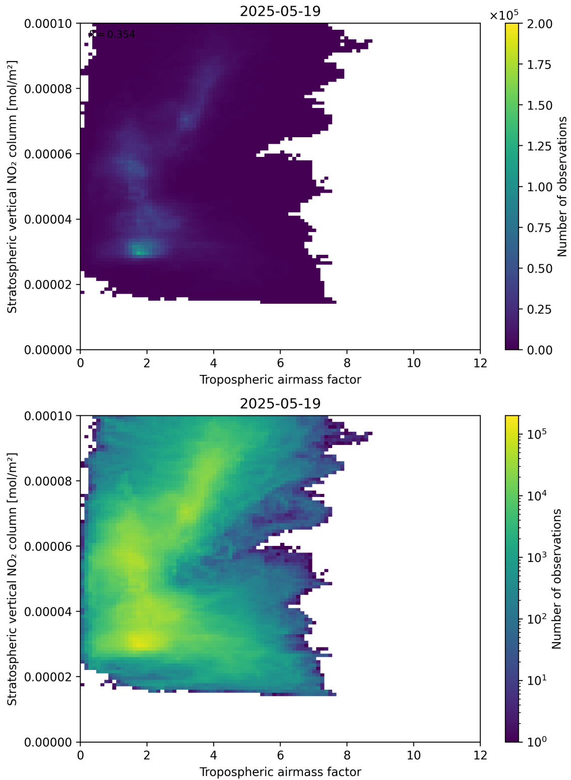
Figure 74: Scatter density plot of “Tropospheric airmass factor” against “Stratospheric vertical NO 2 column” for 2025-05-18 to 2025-05-20.
