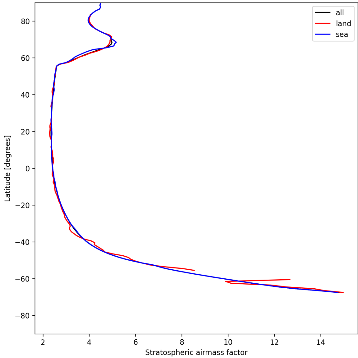
Figure 27: Zonal average of “Stratospheric air mass factor” for 2025-05-18 to 2025-05-20.
