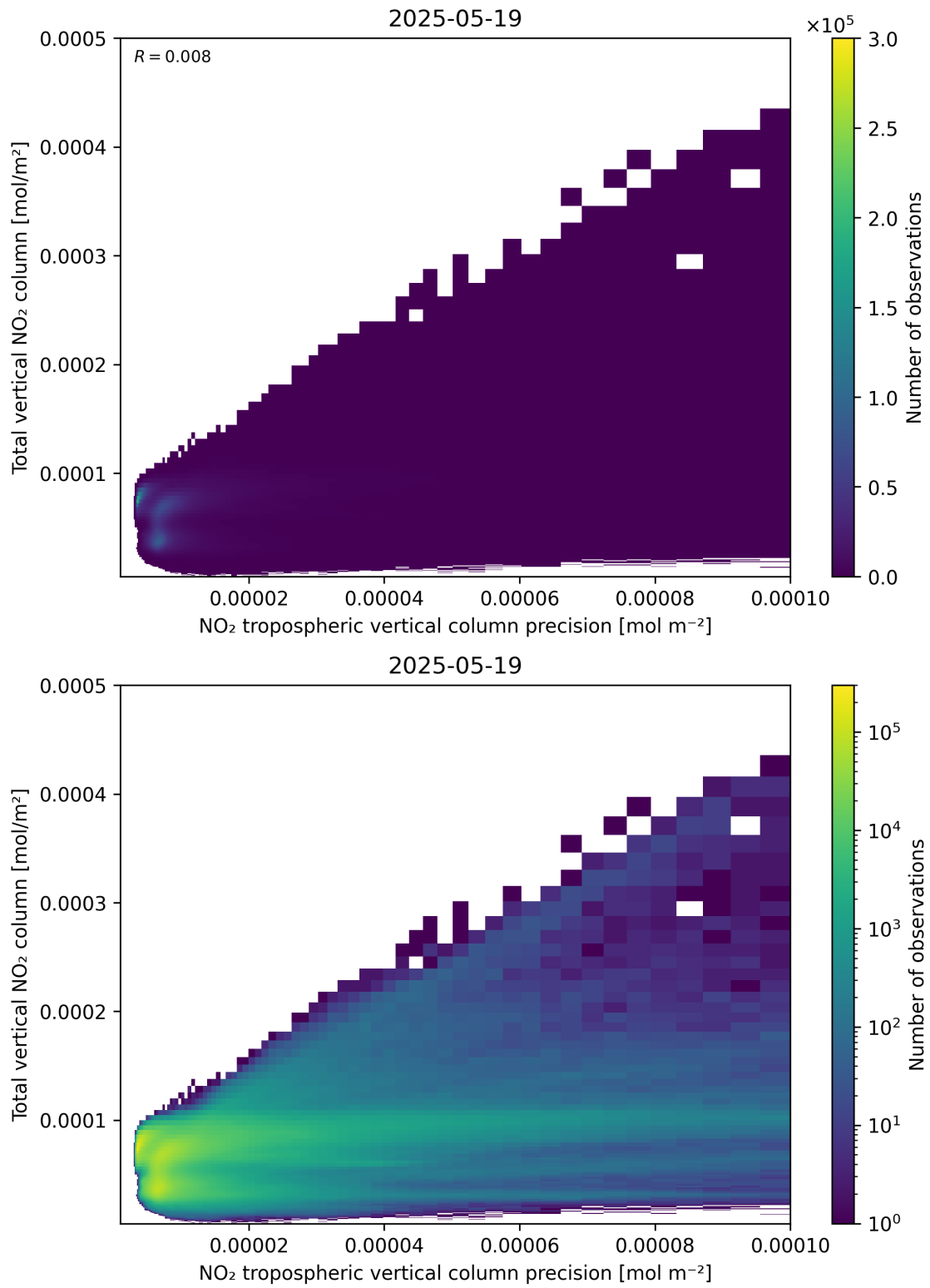
Figure 138: Scatter density plot of “NO 2 tropospheric vertical column precision” against “Total vertical NO 2 column” for 2025-05-18 to 2025-05-20.
