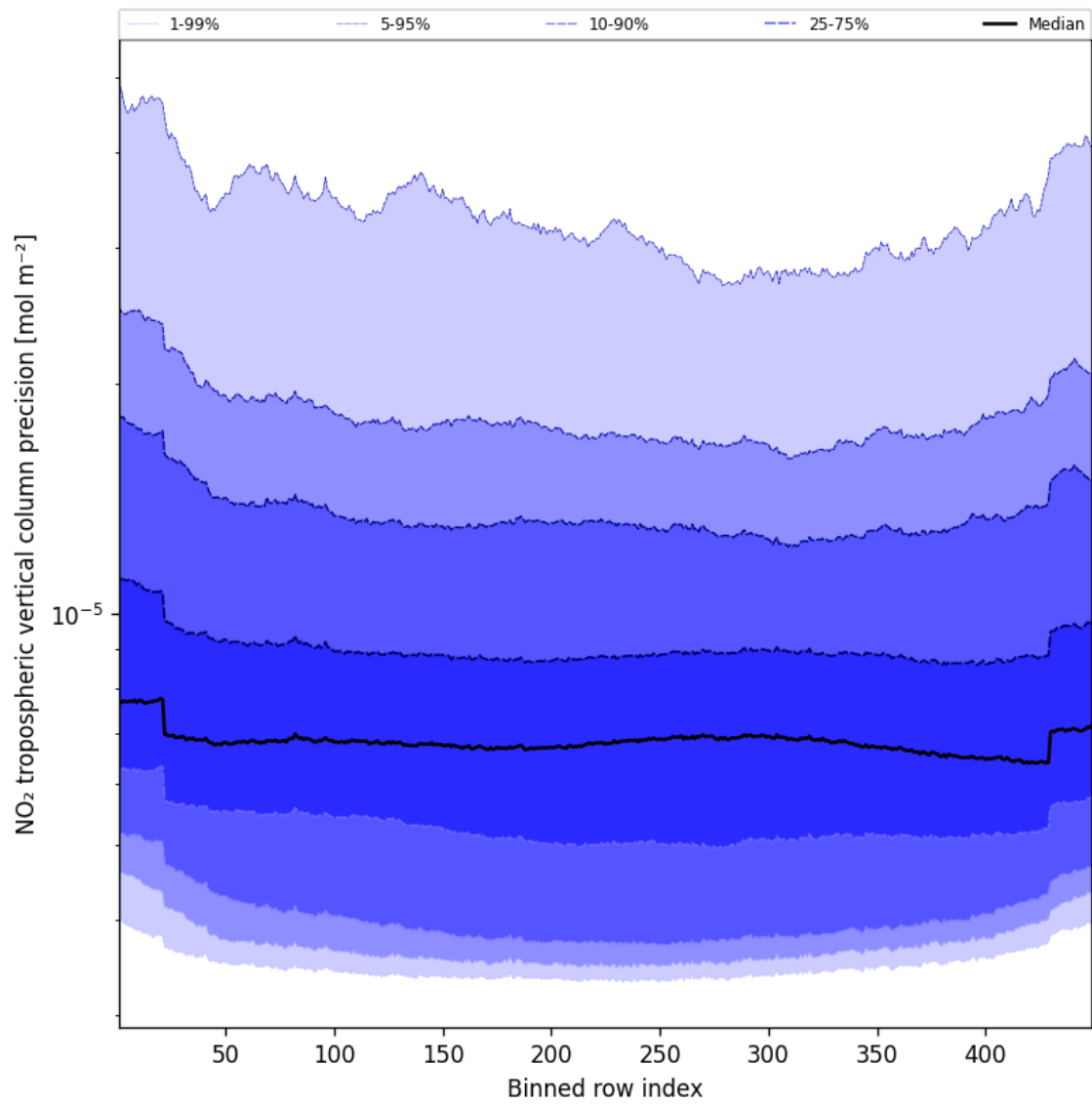
Figure 47: Along track statistics of “NO 2 tropospheric vertical column precision” for 2025-05-18 to 2025-05-20
