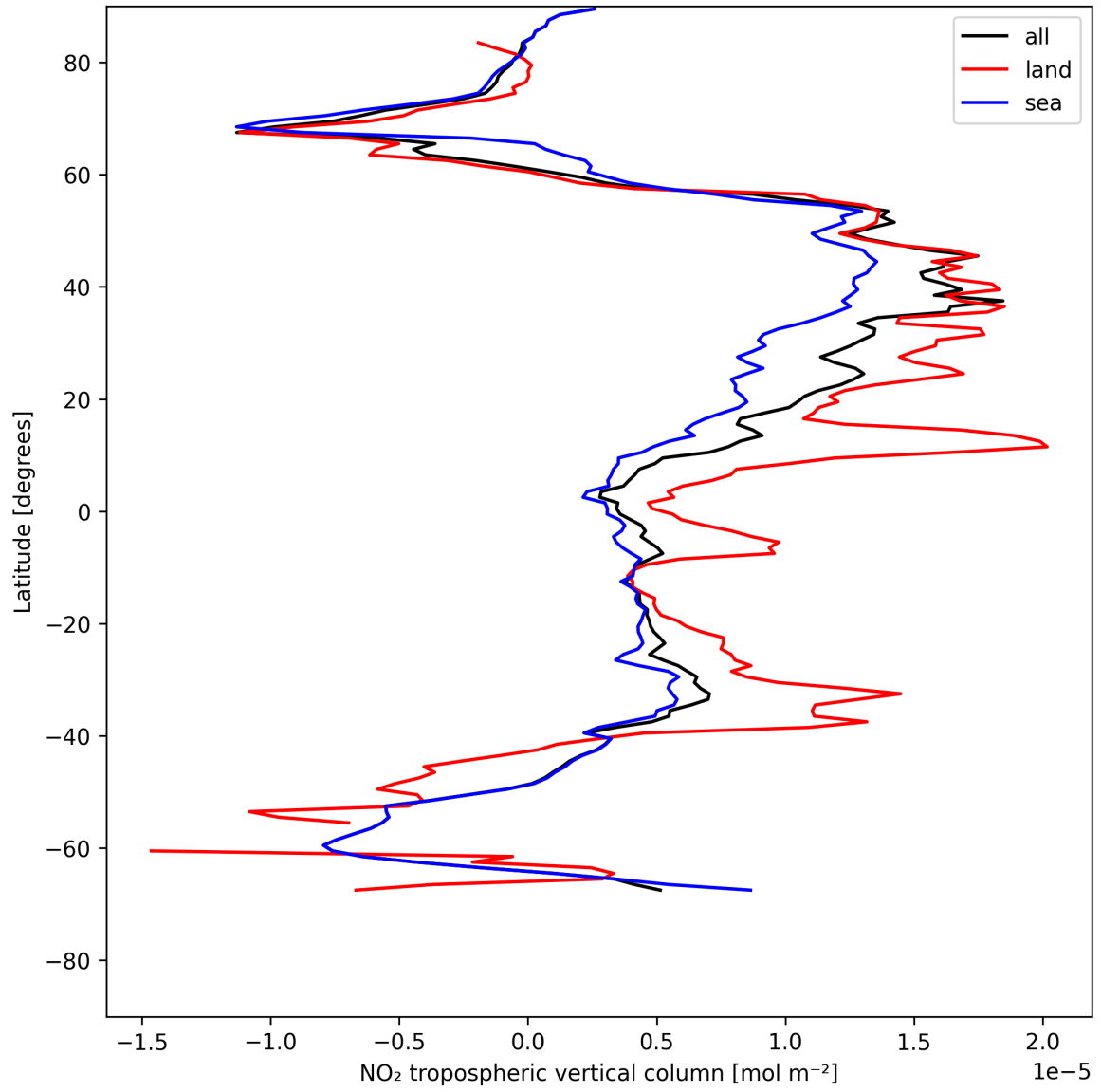
Figure 12: Zonal average of “NO 2 tropospheric vertical column” for 2025-05-18 to 2025-05-20.
