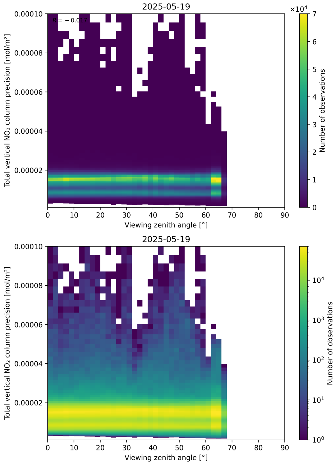
Figure 168: Scatter density plot of “Viewing zenith angle” against “Total vertical NO 2 column precision” for 2025-05-18 to 2025-05-20.
