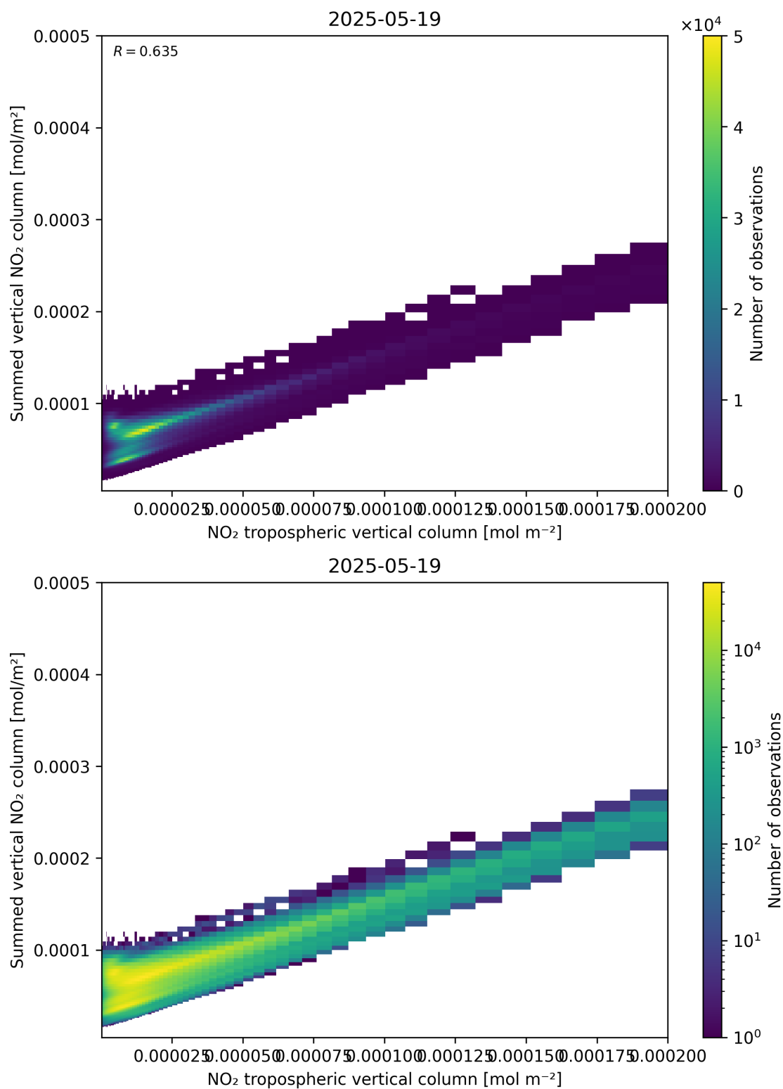
Figure 126: Scatter density plot of “NO 2 tropospheric vertical column” against “Summed vertical NO 2 column” for 2025-05-18 to 2025-05-20.
