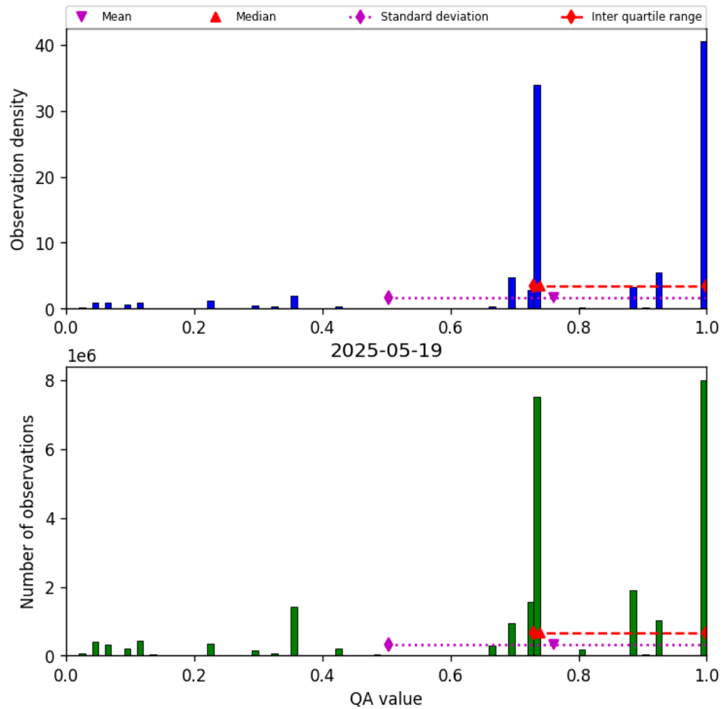
Figure 28: Histogram of “QA value” for 2025-05-18 to 2025-05-20
