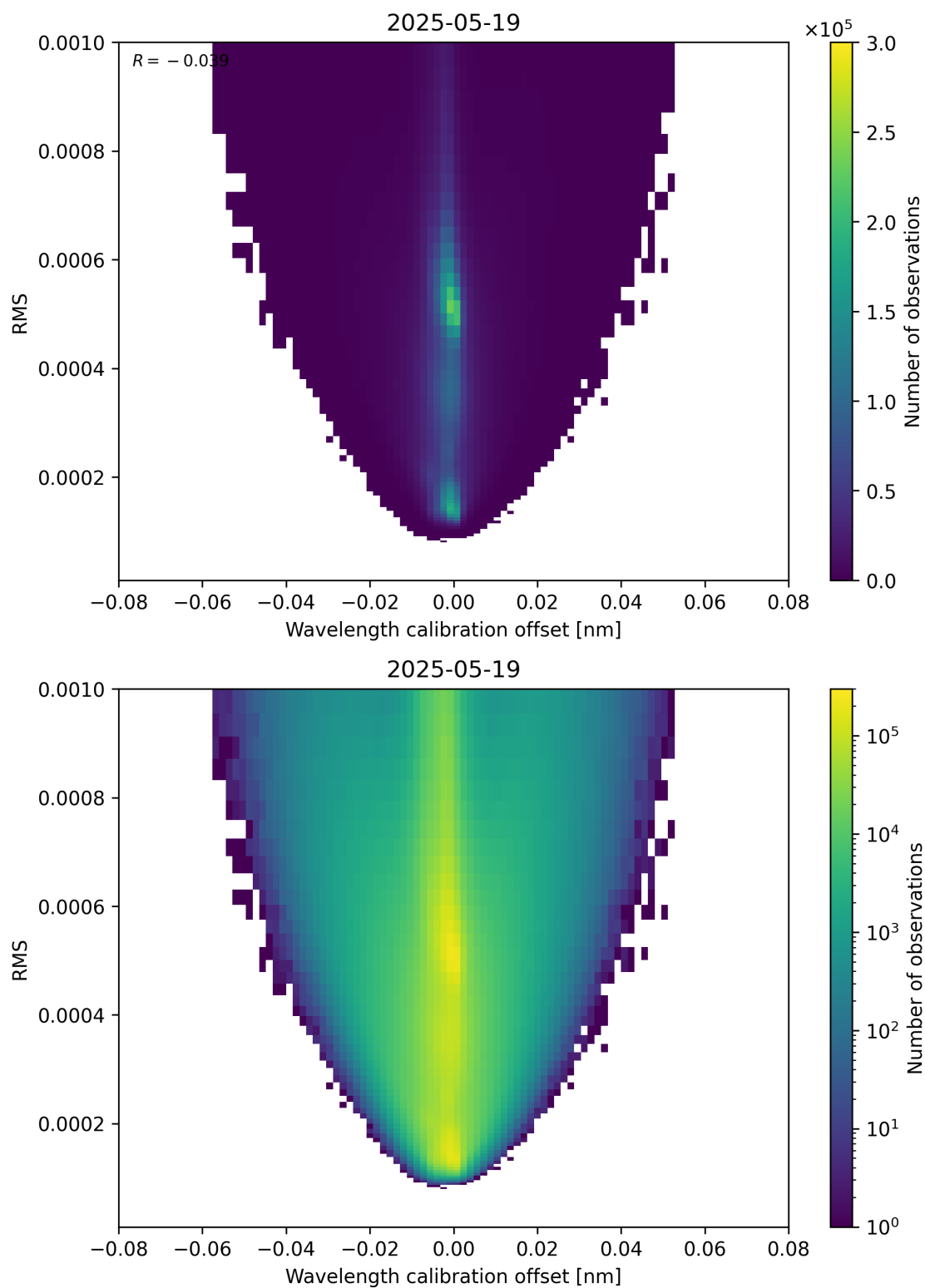
Figure 181: Scatter density plot of “Wavelength calibration offset” against “RMS” for 2025-05-18 to 2025-05-20.
