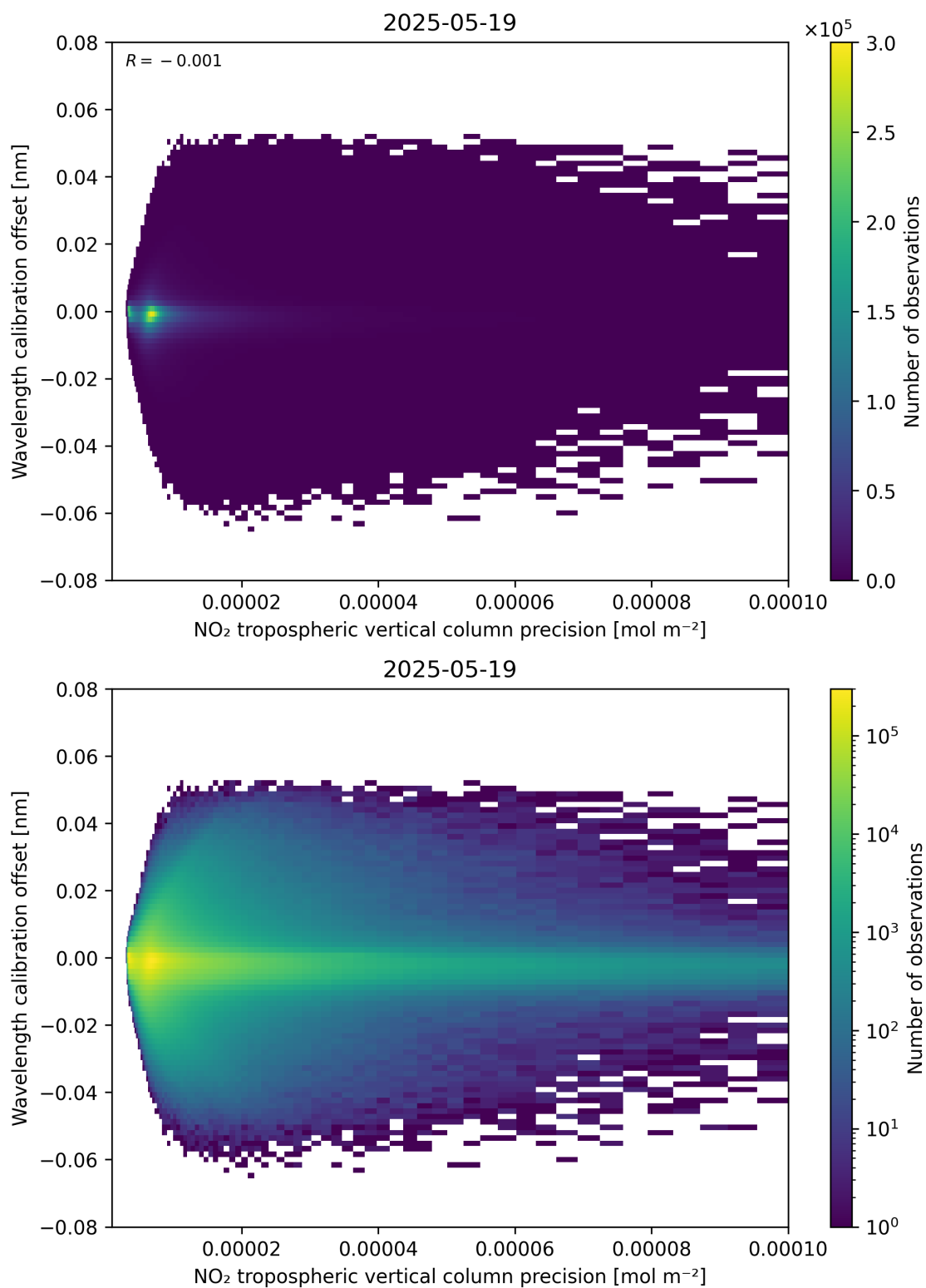
Figure 141: Scatter density plot of “NO 2 tropospheric vertical column precision” against “Wavelength calibration offset” for 2025-05-18 to 2025-05-20.
