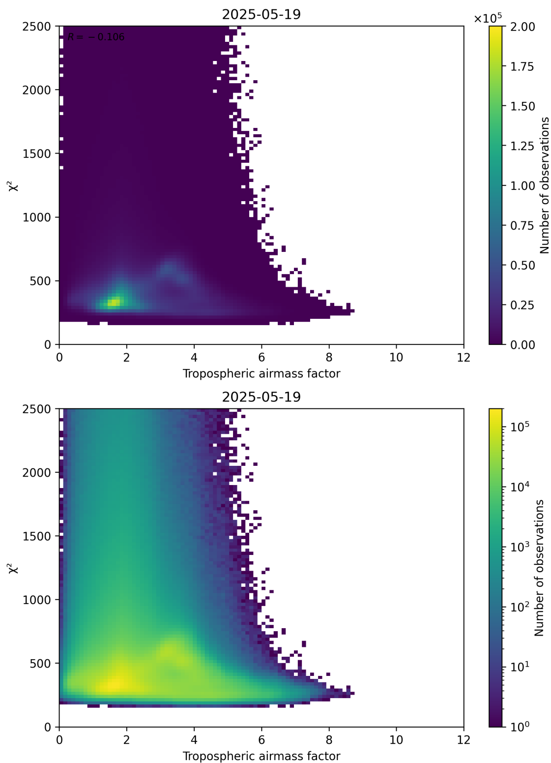
Figure 73: Scatter density plot of “Tropospheric airmass factor” against “ \chi^2 ” for 2025-05-18 to 2025-05-20.
