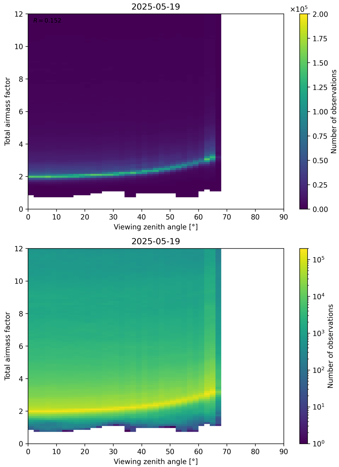
Figure 160: Scatter density plot of “Viewing zenith angle” against “Total airmass factor” for 2025-05-18 to 2025-05-20.
