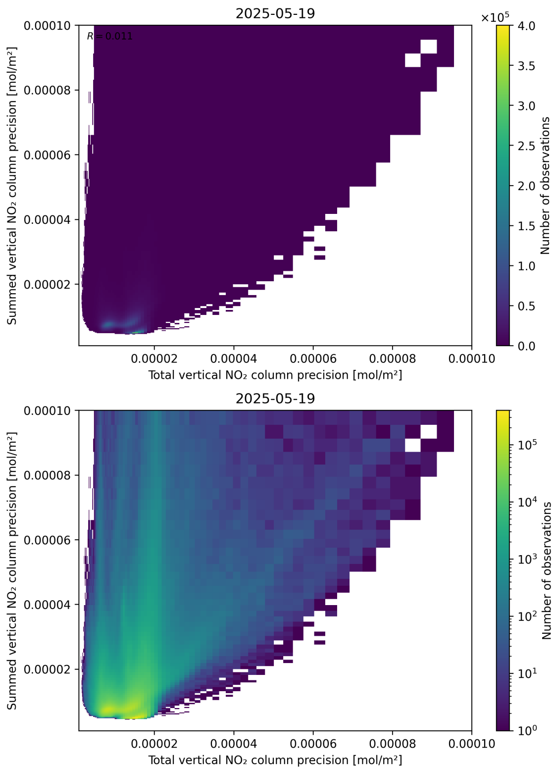
Figure 118: Scatter density plot of “Total vertical NO 2 column precision” against “Summed vertical NO 2 column precision” for 2025-05-18 to 2025-05-20.
