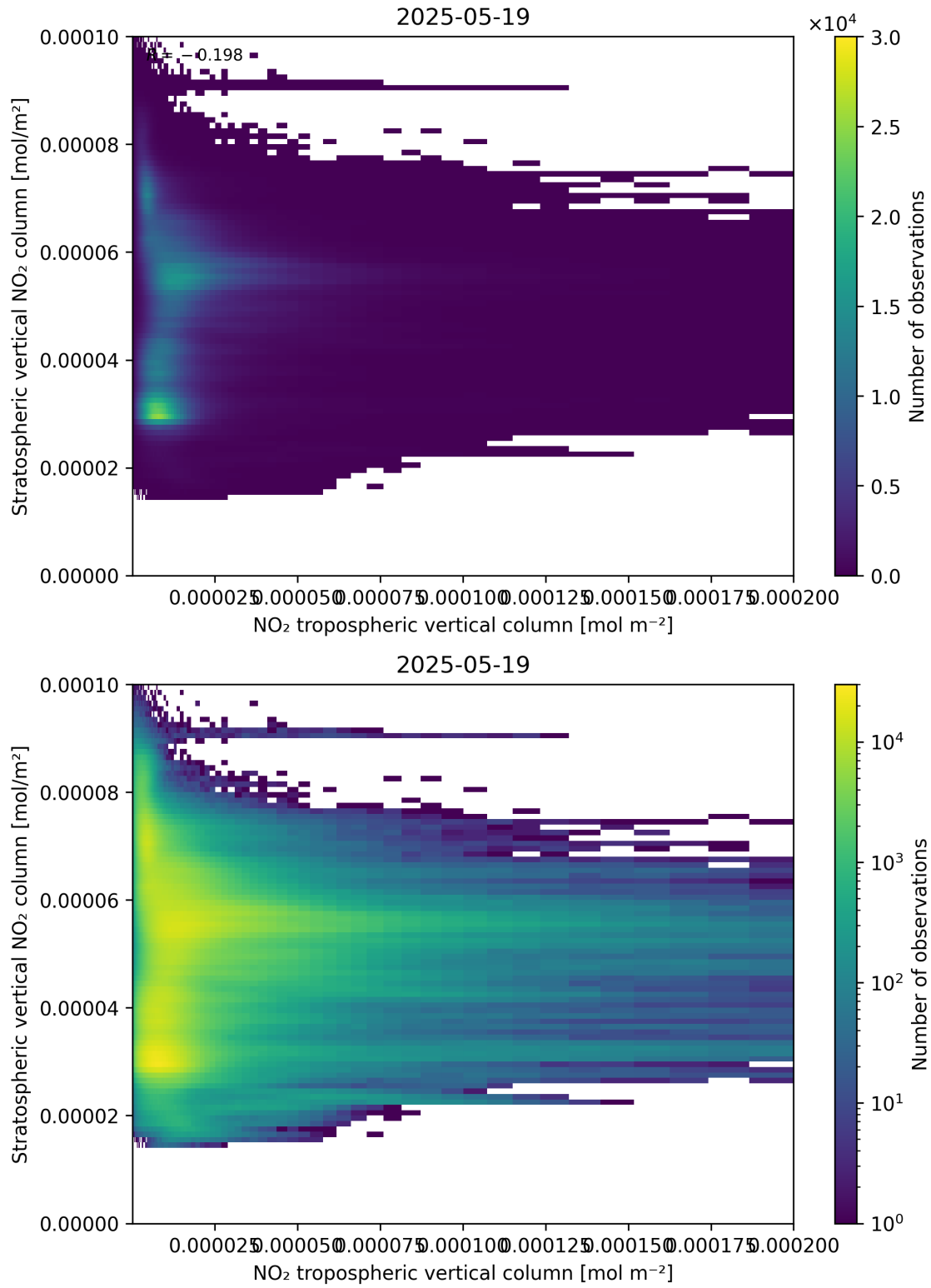
Figure 125: Scatter density plot of “NO 2 tropospheric vertical column” against “Stratospheric vertical NO 2 column” for 2025-05-18 to 2025-05-20.
