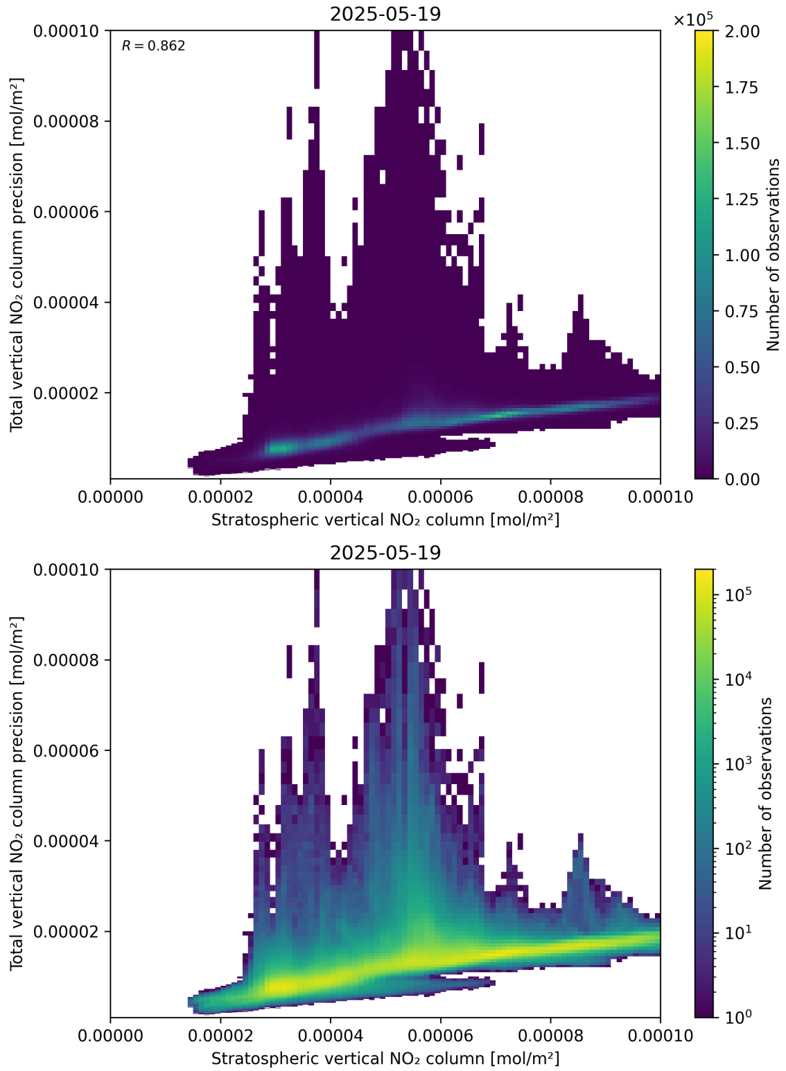
Figure 101: Scatter density plot of “Stratospheric vertical NO 2 column” against “Total vertical NO 2 column precision” for 2025-05-18 to 2025-05-20.
