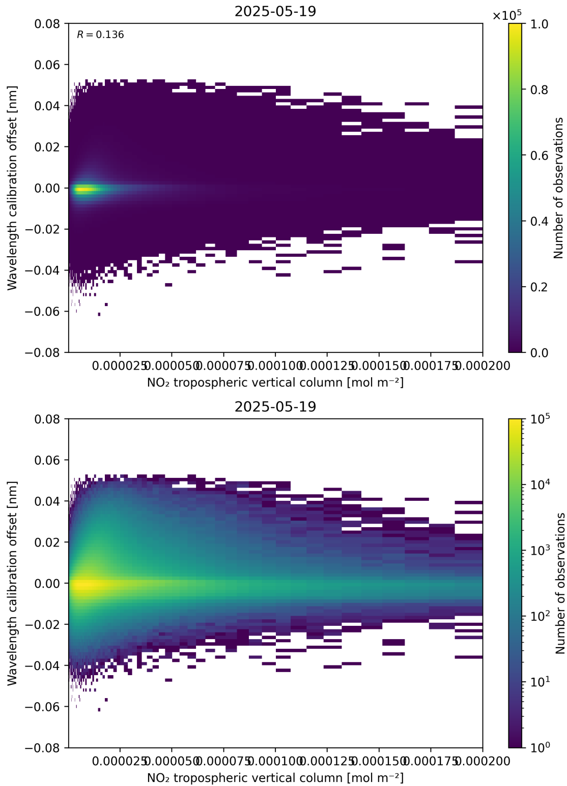
Figure 143: Scatter density plot of “NO 2 tropospheric vertical column” against “Wavelength calibration offset” for 2025-05-18 to 2025-05-20.
