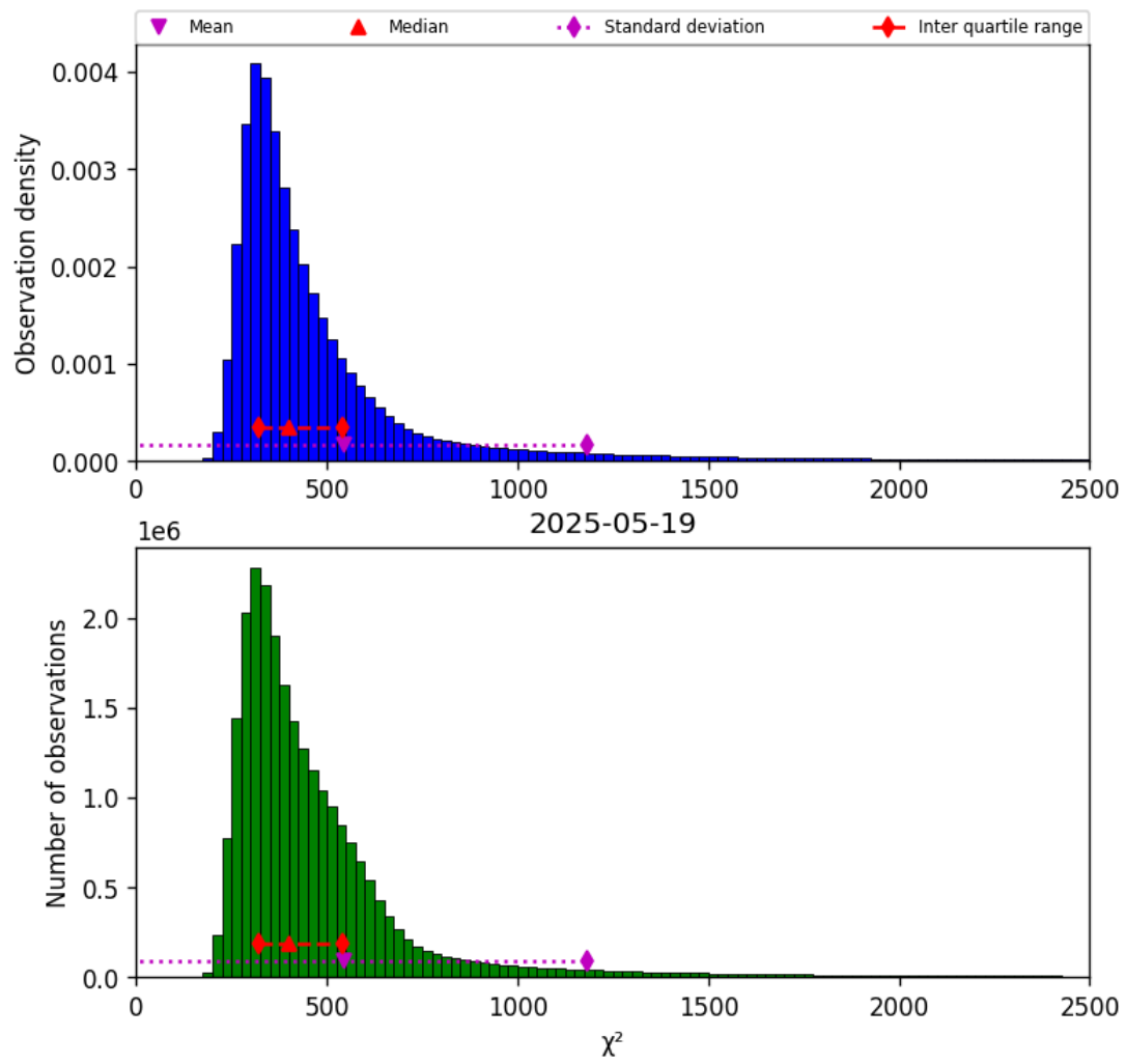
Figure 42: Histogram of “ \chi^2 ” for 2025-05-18 to 2025-05-20
