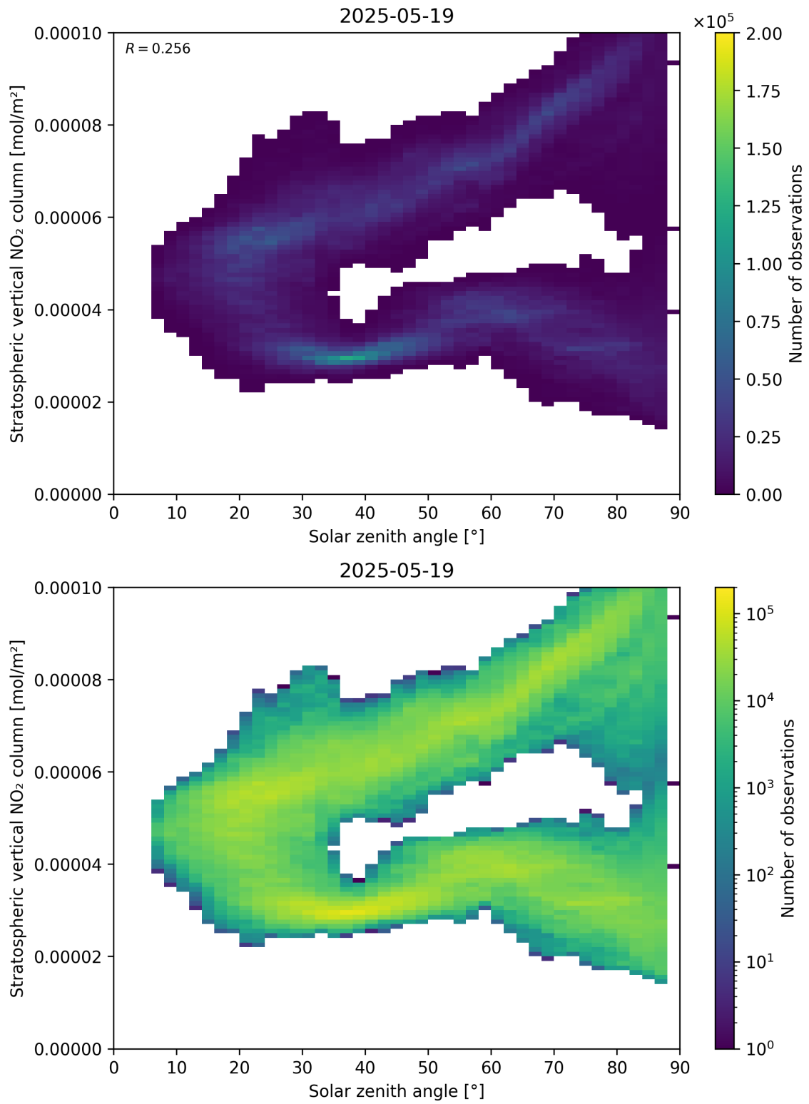
Figure 150: Scatter density plot of “Solar zenith angle” against “Stratospheric vertical NO 2 column” for 2025-05-18 to 2025-05-20.
