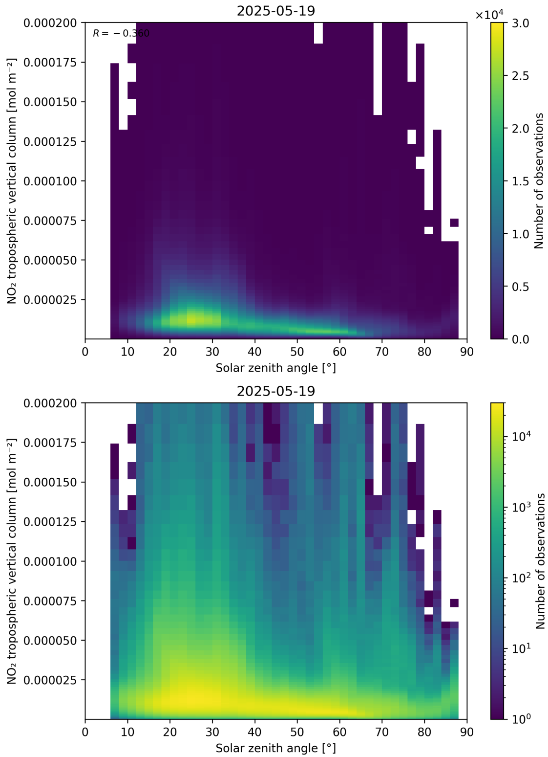
Figure 155: Scatter density plot of “Solar zenith angle” against “NO 2 tropospheric vertical column” for 2025-05-18 to 2025-05-20.
