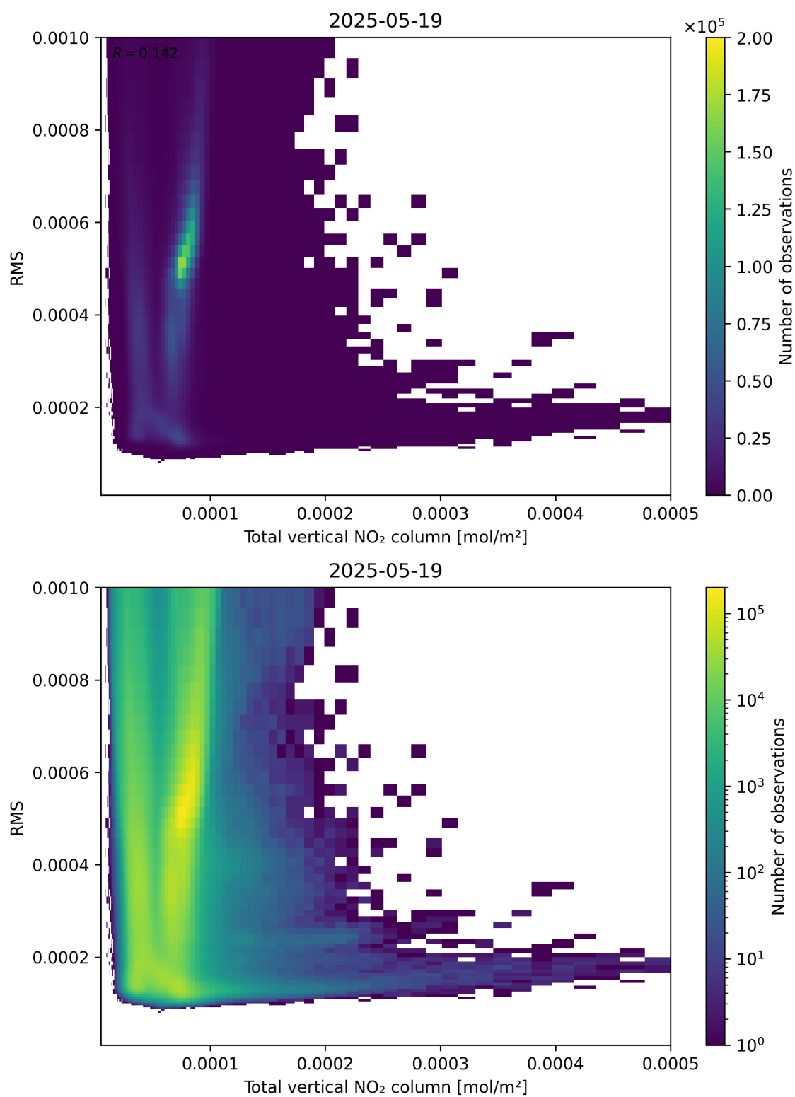
Figure 120: Scatter density plot of “Total vertical NO 2 column” against “RMS” for 2025-05-18 to 2025-05-20.
