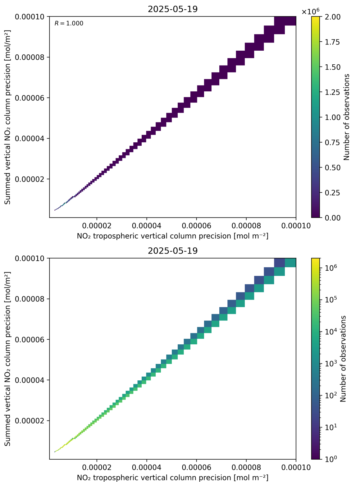
Figure 137: Scatter density plot of “NO 2 tropospheric vertical column precision” against “Summed vertical NO 2 column precision” for 2025-05-18 to 2025-05-20.
