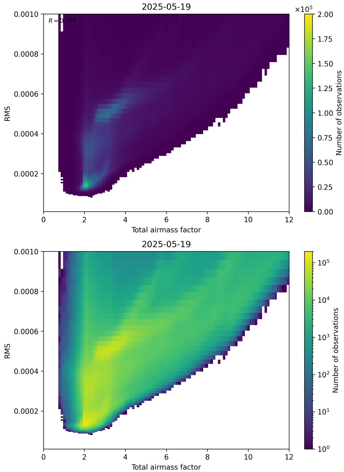
Figure 69: Scatter density plot of “Total airmass factor” against “RMS” for 2025-05-18 to 2025-05-20.
