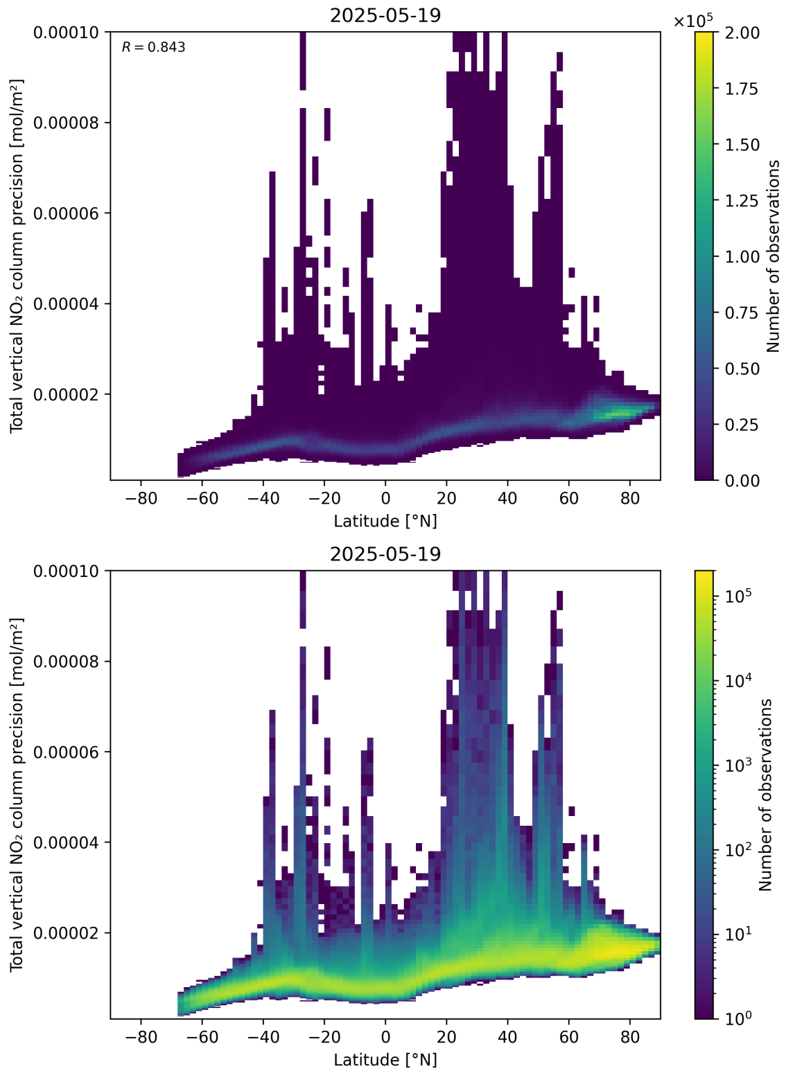
Figure 91: Scatter density plot of “Latitude” against “Total vertical NO 2 column precision” for 2025-05-18 to 2025-05-20.
