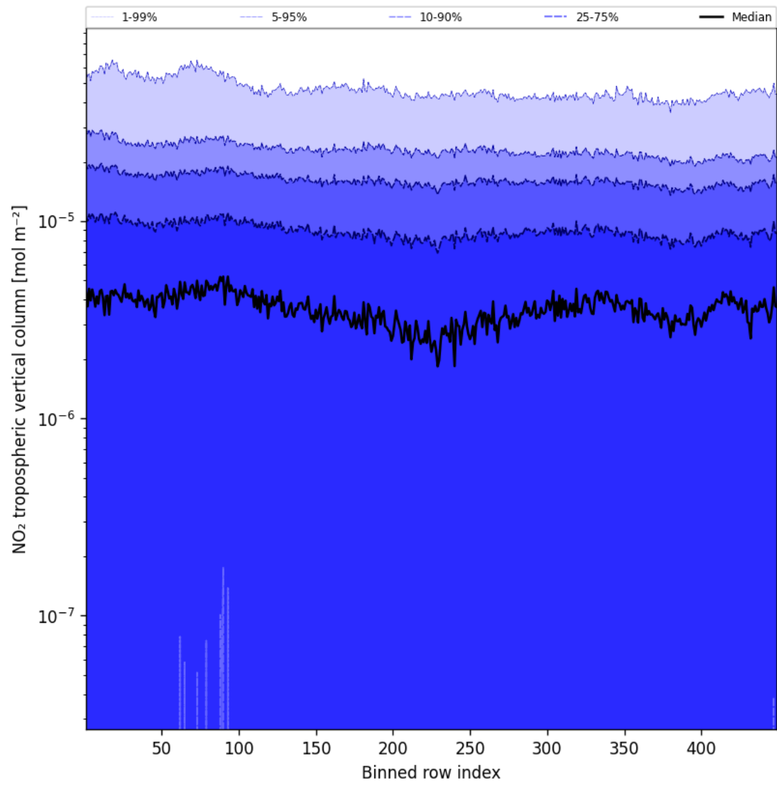
Figure 46: Along track statistics of “NO 2 tropospheric vertical column” for 2025-05-18 to 2025-05-20
