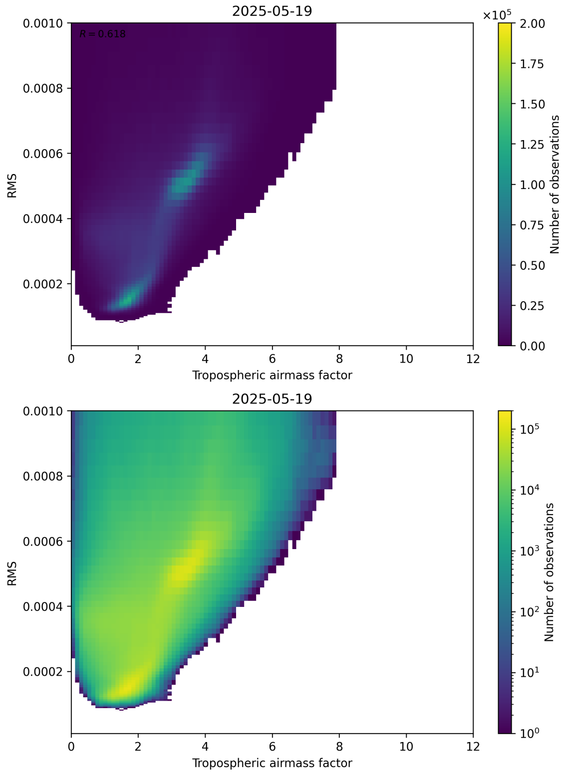
Figure 79: Scatter density plot of “Tropospheric airmass factor” against “RMS” for 2025-05-18 to 2025-05-20.
