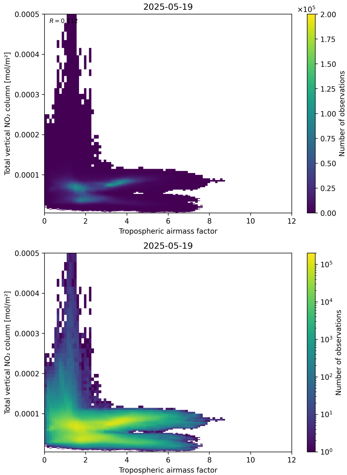
Figure 77: Scatter density plot of “Tropospheric airmass factor” against “Total vertical NO 2 column” for 2025-05-18 to 2025-05-20.
