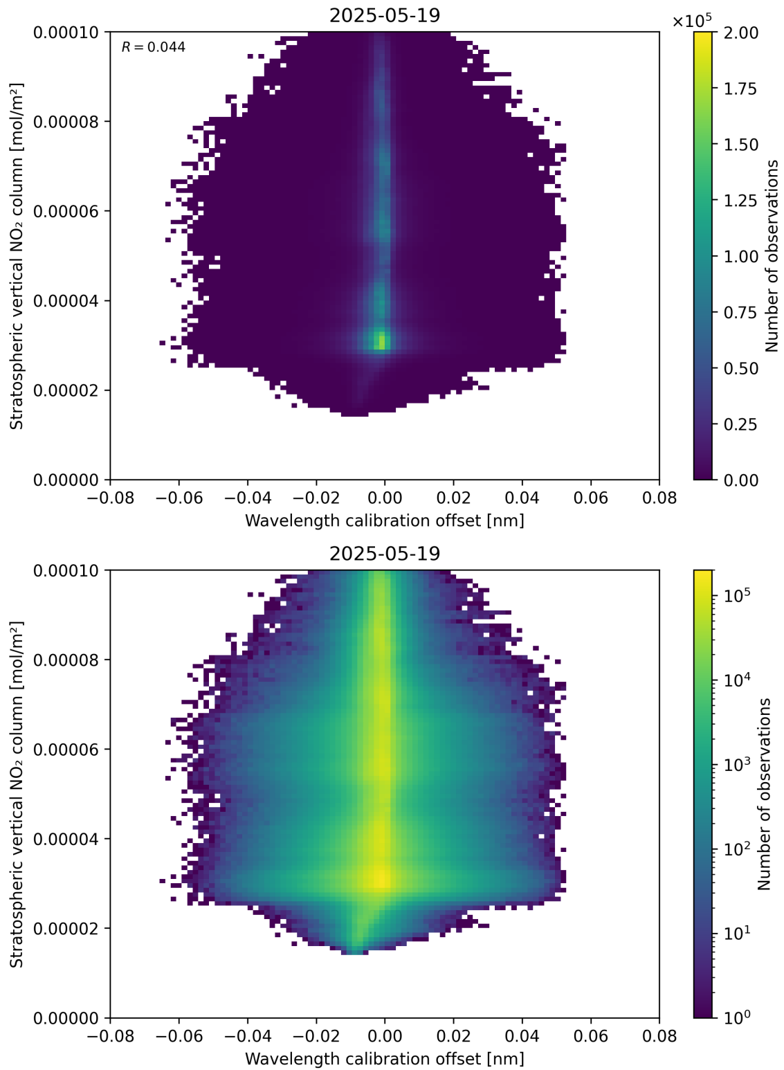
Figure 176: Scatter density plot of “Wavelength calibration offset” against “Stratospheric vertical NO 2 column” for 2025-05-18 to 2025-05-20.
