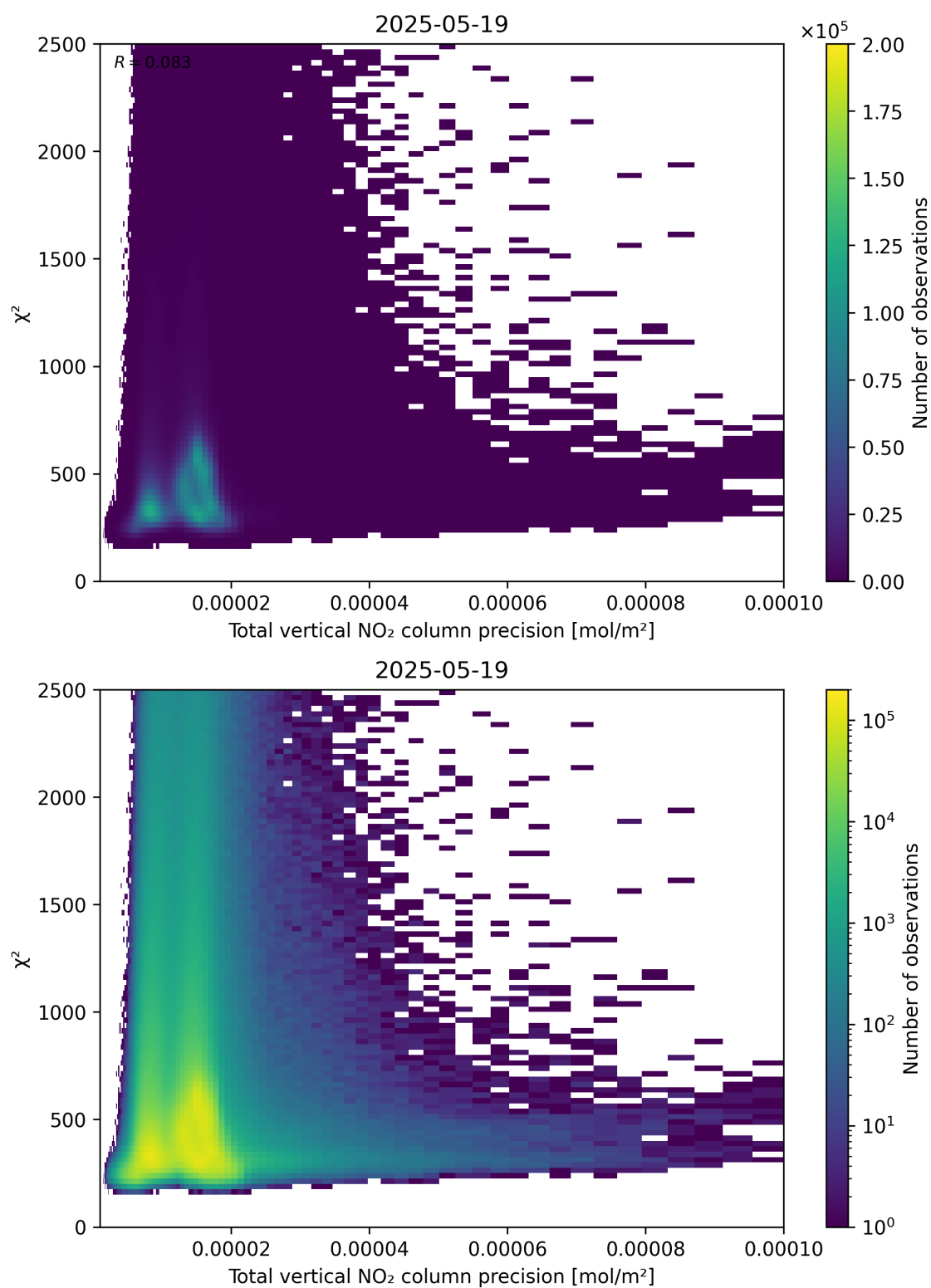
Figure 116: Scatter density plot of “Total vertical NO 2 column precision” against “ \chi^2 ” for 2025-05-18 to 2025-05-20.
