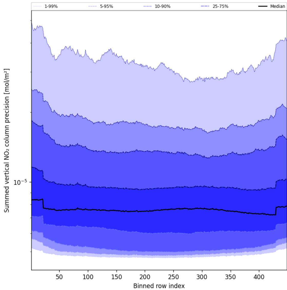
Figure 58: Along track statistics of “Summed vertical NO 2 column precision” for 2025-05-18 to 2025-05-20
