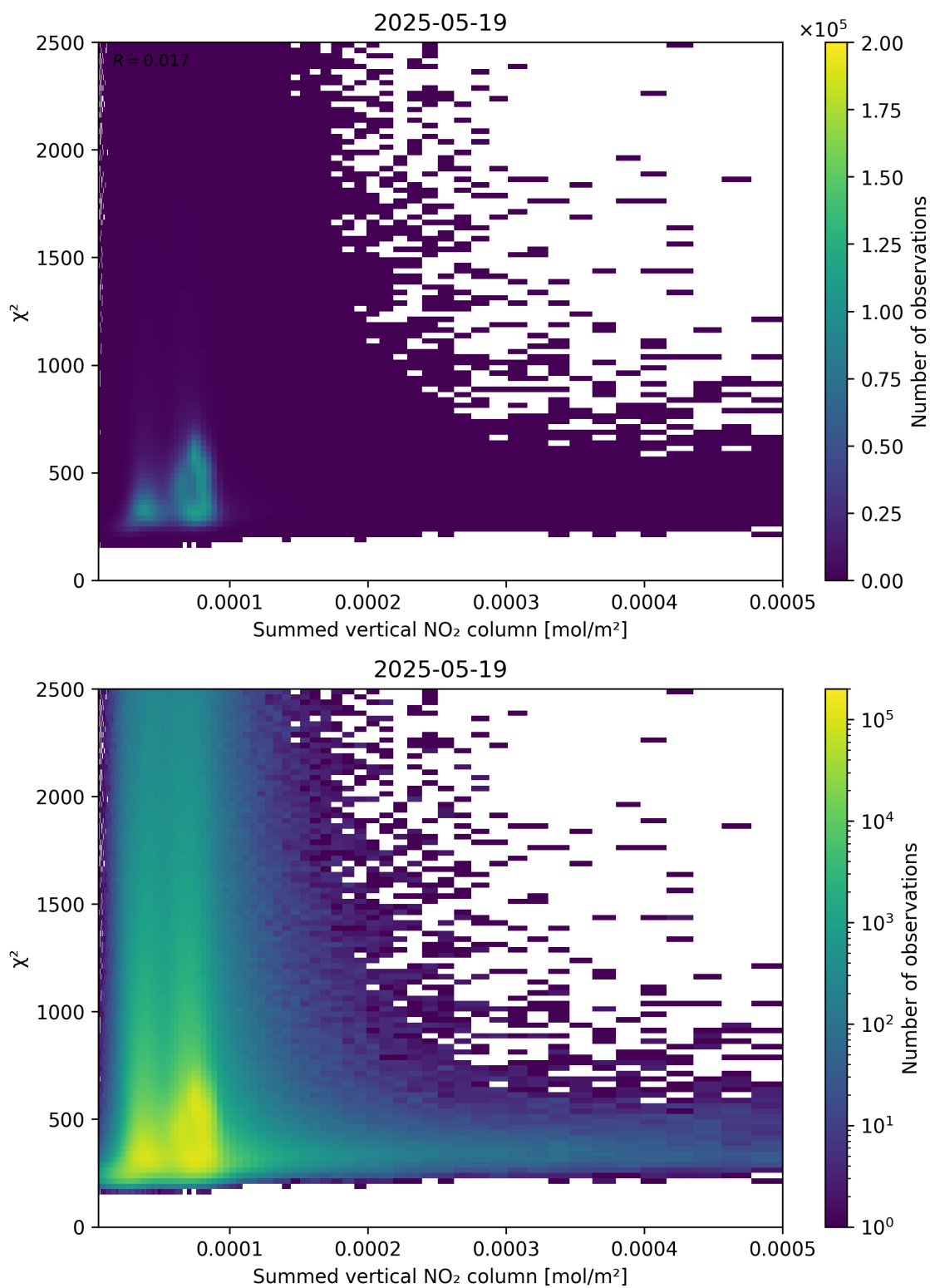
Figure 104: Scatter density plot of “Summed vertical NO 2 column” against “ \chi^2 ” for 2025-05-18 to 2025-05-20.
