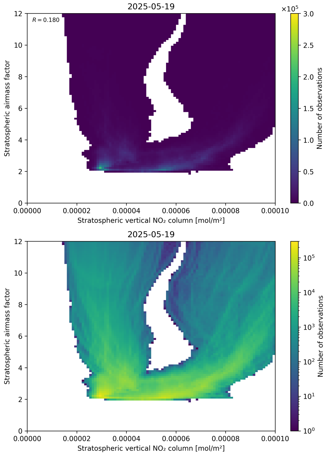
Figure 96: Scatter density plot of “Stratospheric vertical NO 2 column” against “Stratospheric airmass factor” for 2025-05-18 to 2025-05-20.
