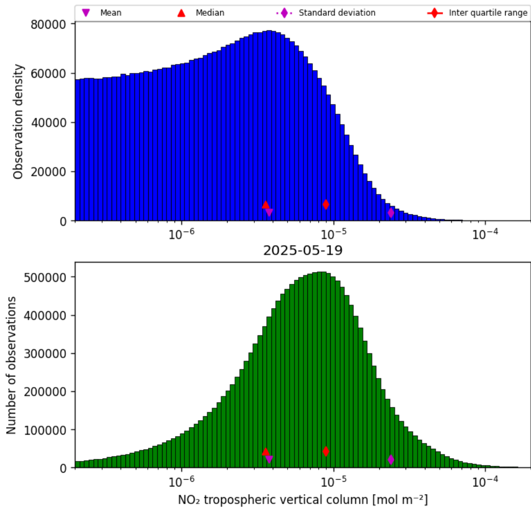
Figure 29: Histogram of “NO 2 tropospheric vertical column” for 2025-05-18 to 2025-05-20
