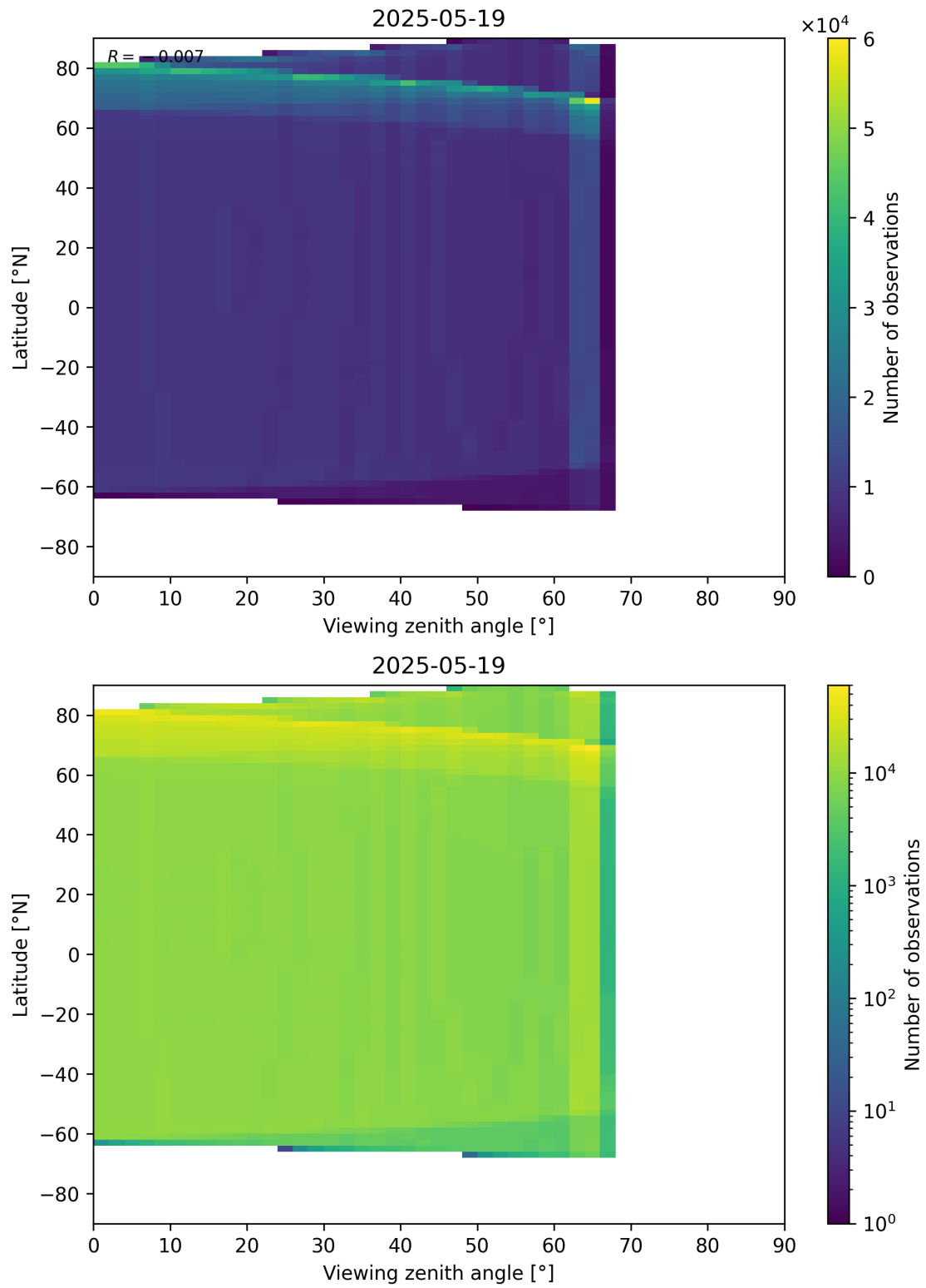
Figure 163: Scatter density plot of “Viewing zenith angle” against “Latitude” for 2025-05-18 to 2025-05-20.
