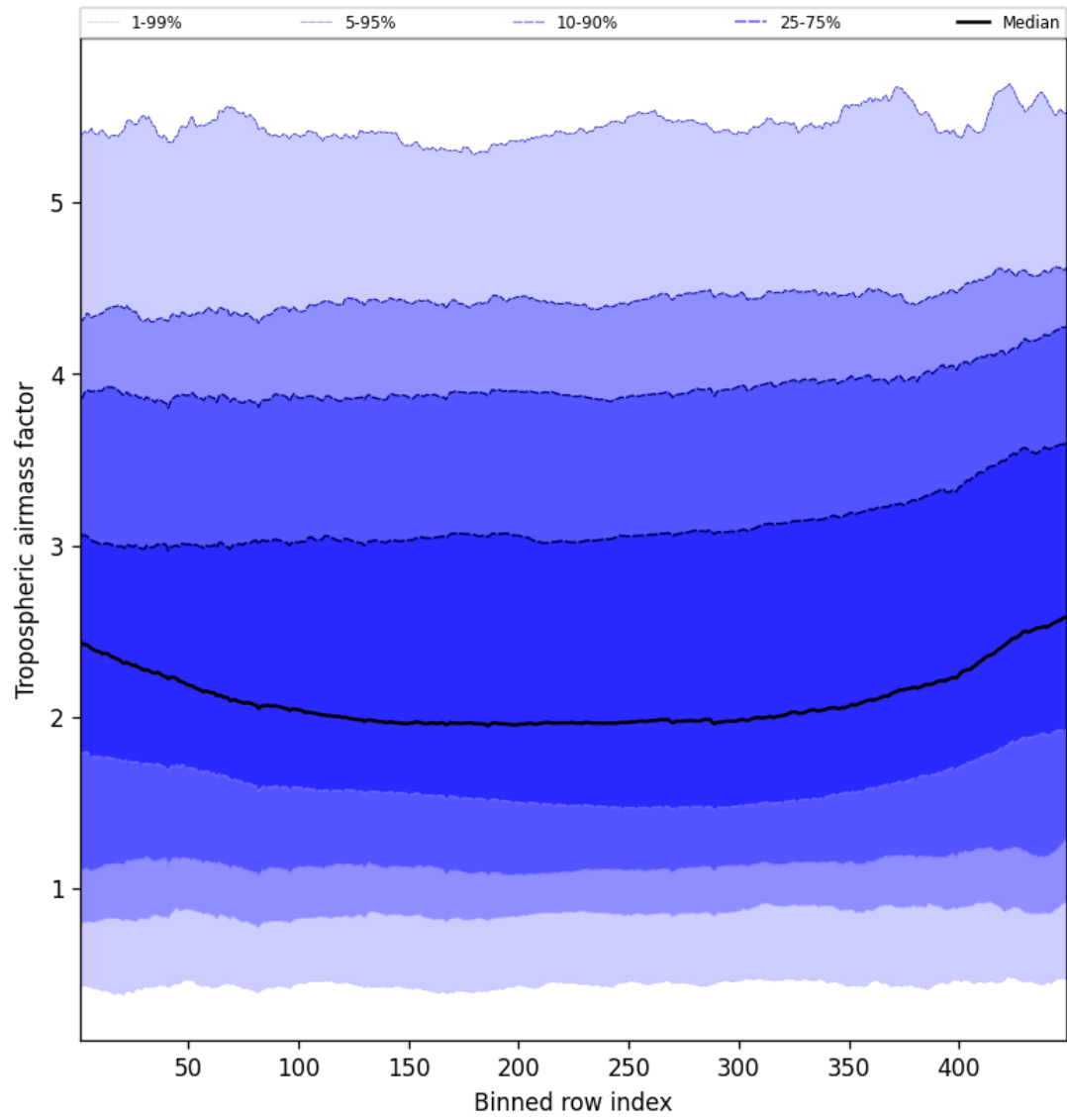
Figure 48: Along track statistics of “Tropospheric airmass factor” for 2025-05-18 to 2025-05-20
