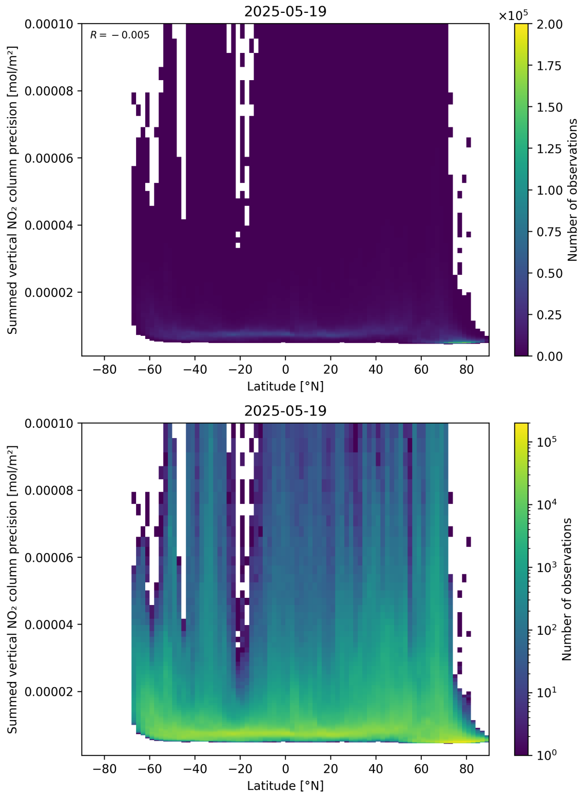
Figure 89: Scatter density plot of “Latitude” against “Summed vertical NO 2 column precision” for 2025-05-18 to 2025-05-20.
