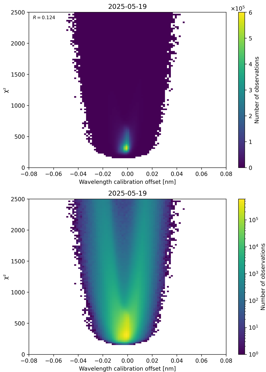
Figure 175: Scatter density plot of “Wavelength calibration offset” against “ \chi^2 ” for 2025-05-18 to 2025-05-20.
