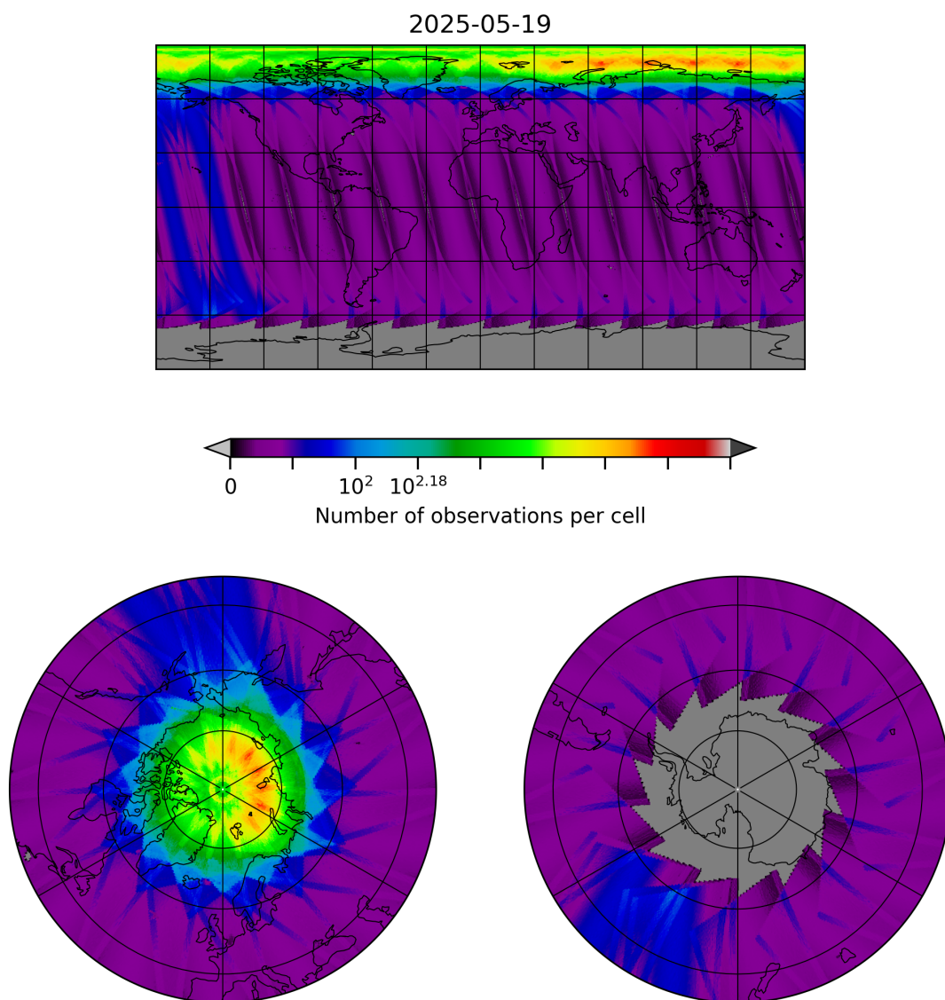
Figure 10: Map of the number of observations for 2025-05-18 to 2025-05-20
