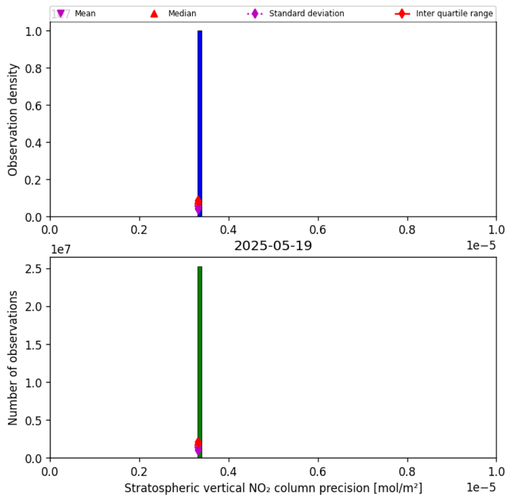
Figure 37: Histogram of “Stratospheric vertical NO 2 column precision” for 2025-05-18 to 2025-05-20
