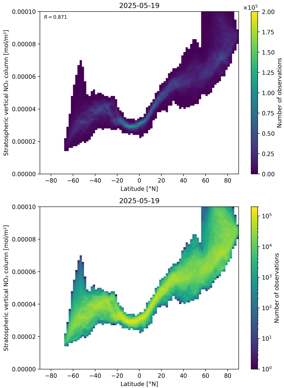
Figure 87: Scatter density plot of “Latitude” against “Stratospheric vertical NO 2 column” for 2025-05-18 to 2025-05-20.
