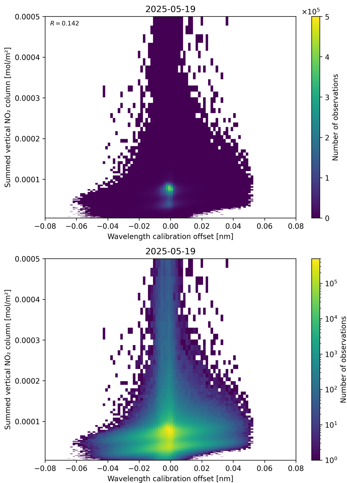
Figure 177: Scatter density plot of “Wavelength calibration offset” against “Summed vertical NO 2 column” for 2025-05-18 to 2025-05-20.
