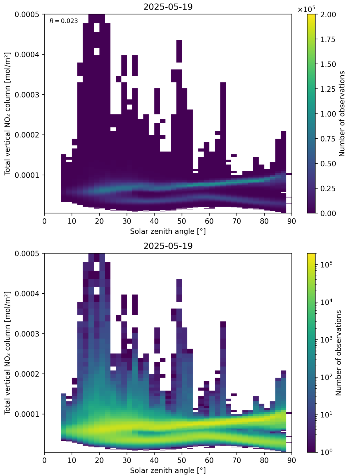
Figure 153: Scatter density plot of “Solar zenith angle” against “Total vertical \text{NO}_2 column” for 2025-05-18 to 2025-05-20.
