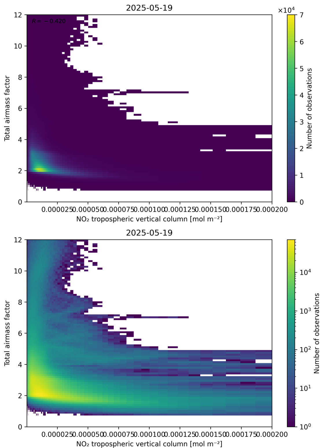
Figure 122: Scatter density plot of “NO 2 tropospheric vertical column” against “Total air mass factor” for 2025-05-18 to 2025-05-20.
