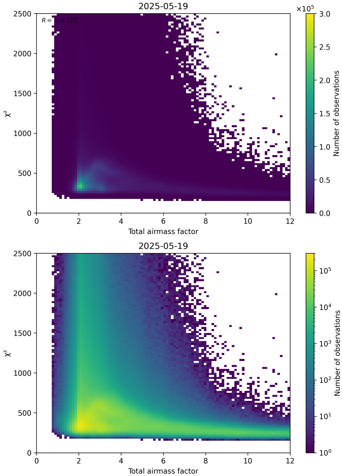
Figure 63: Scatter density plot of “Total airmass factor” against “ \chi^2 ” for 2025-05-18 to 2025-05-20.
