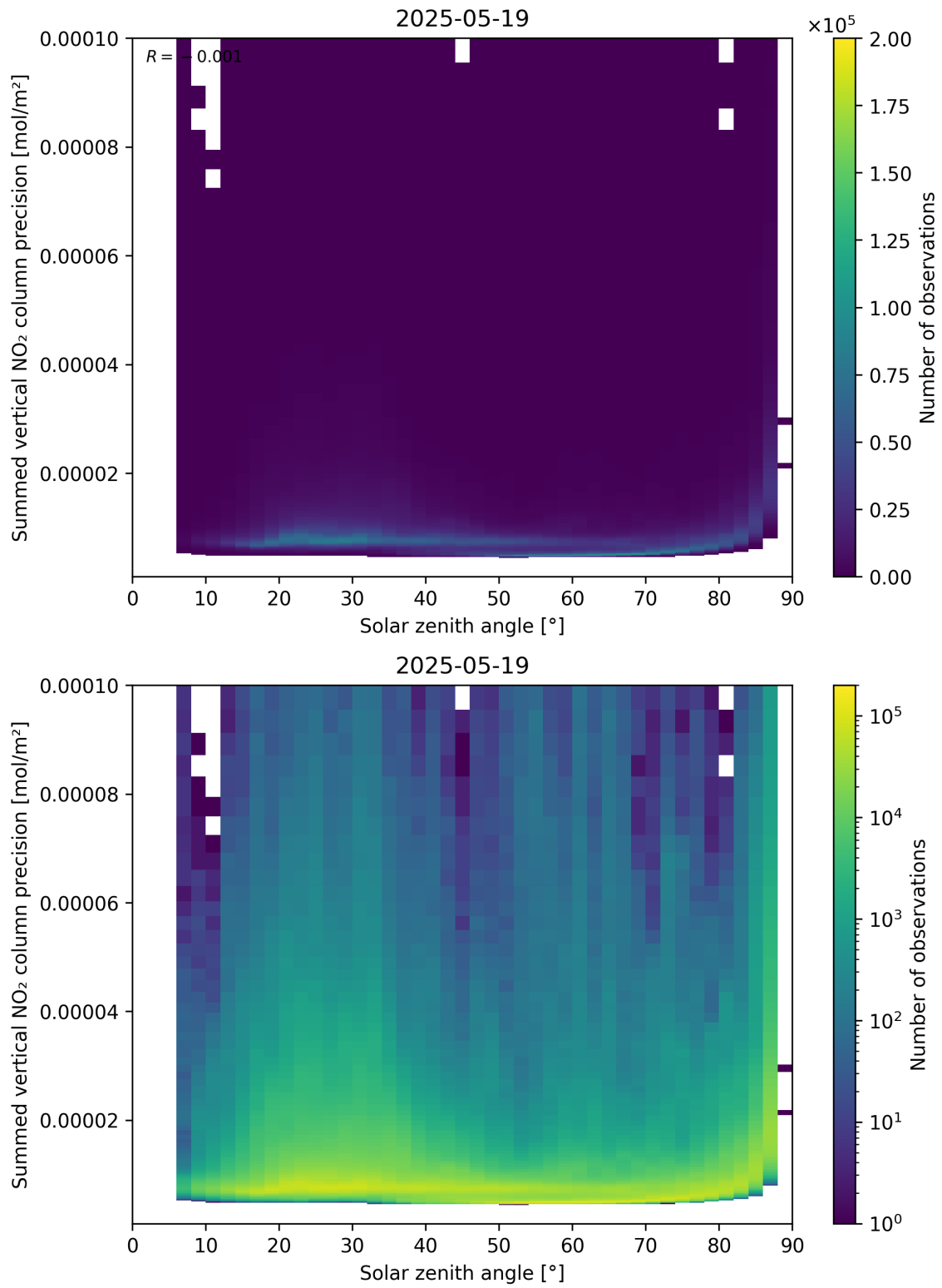
Figure 152: Scatter density plot of “Solar zenith angle” against “Summed vertical NO 2 column precision” for 2025-05-18 to 2025-05-20.
