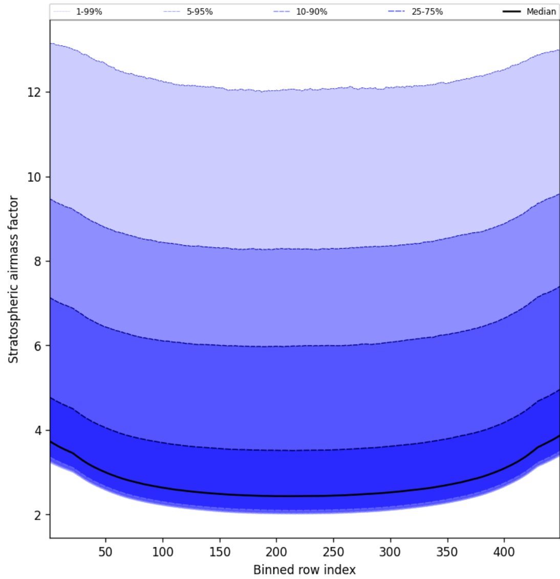
Figure 61: Along track statistics of “Stratospheric airmass factor” for 2025-05-18 to 2025-05-20
