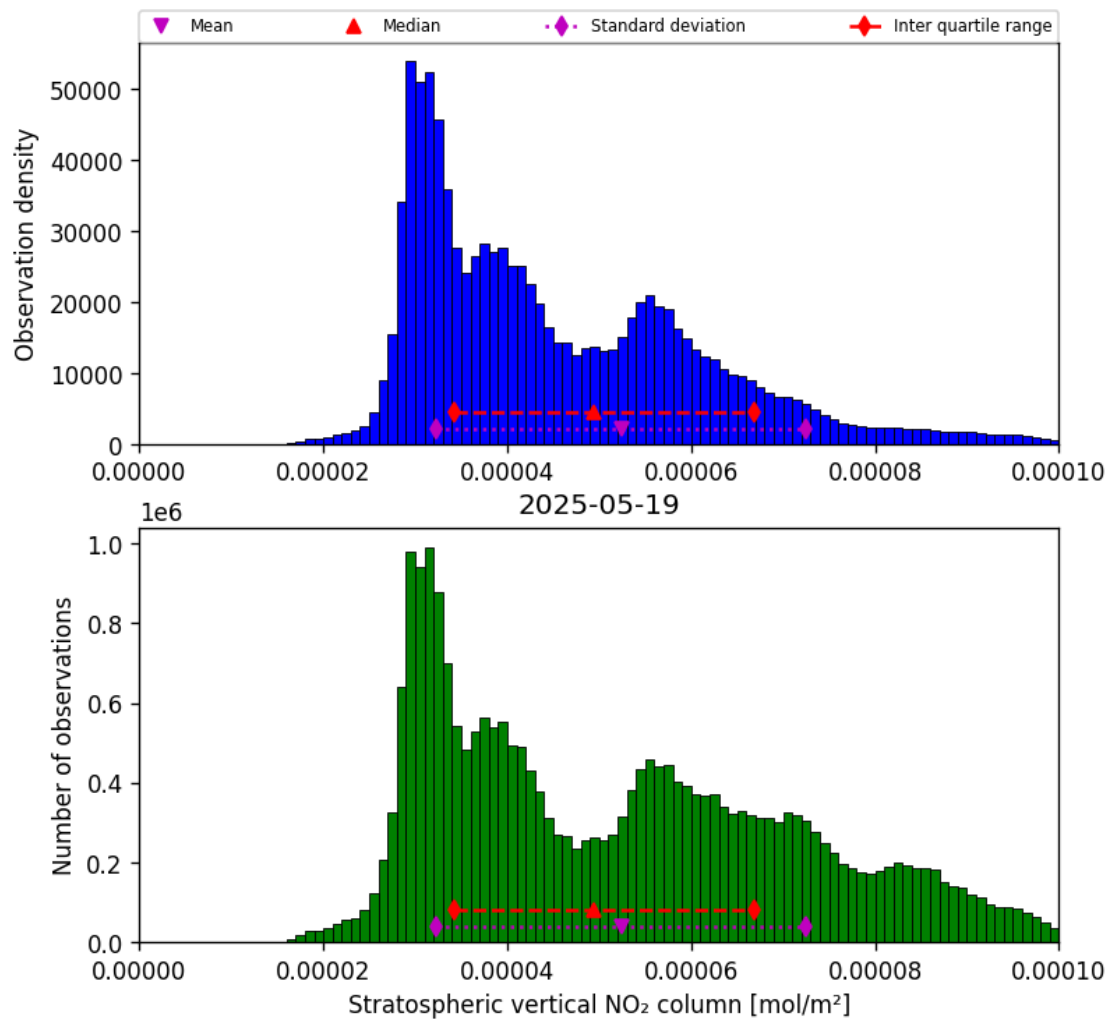
Figure 36: Histogram of “Stratospheric vertical NO 2 column” for 2025-05-18 to 2025-05-20
