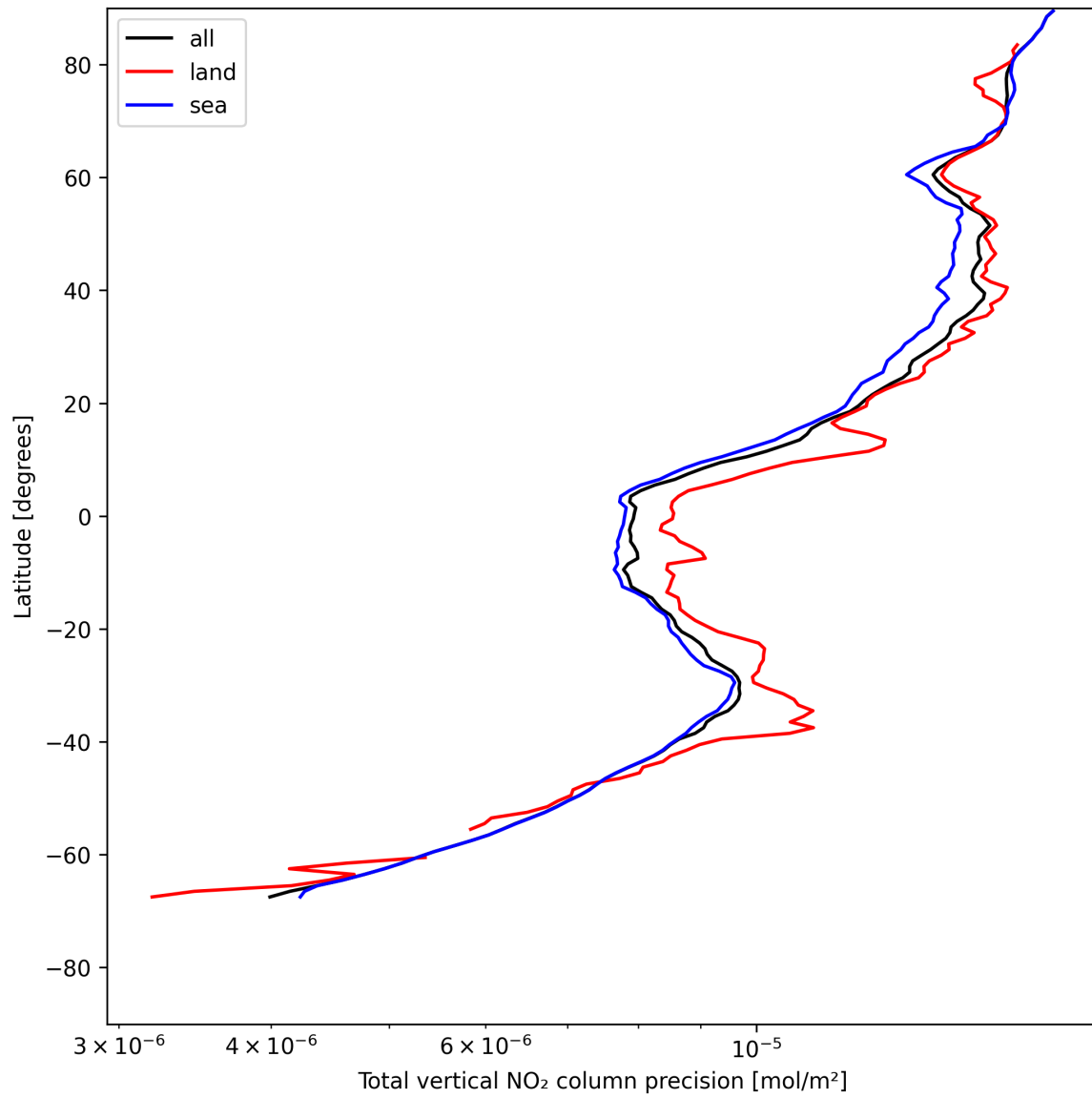
Figure 22: Zonal average of “Total vertical NO 2 column precision” for 2025-05-18 to 2025-05-20.
