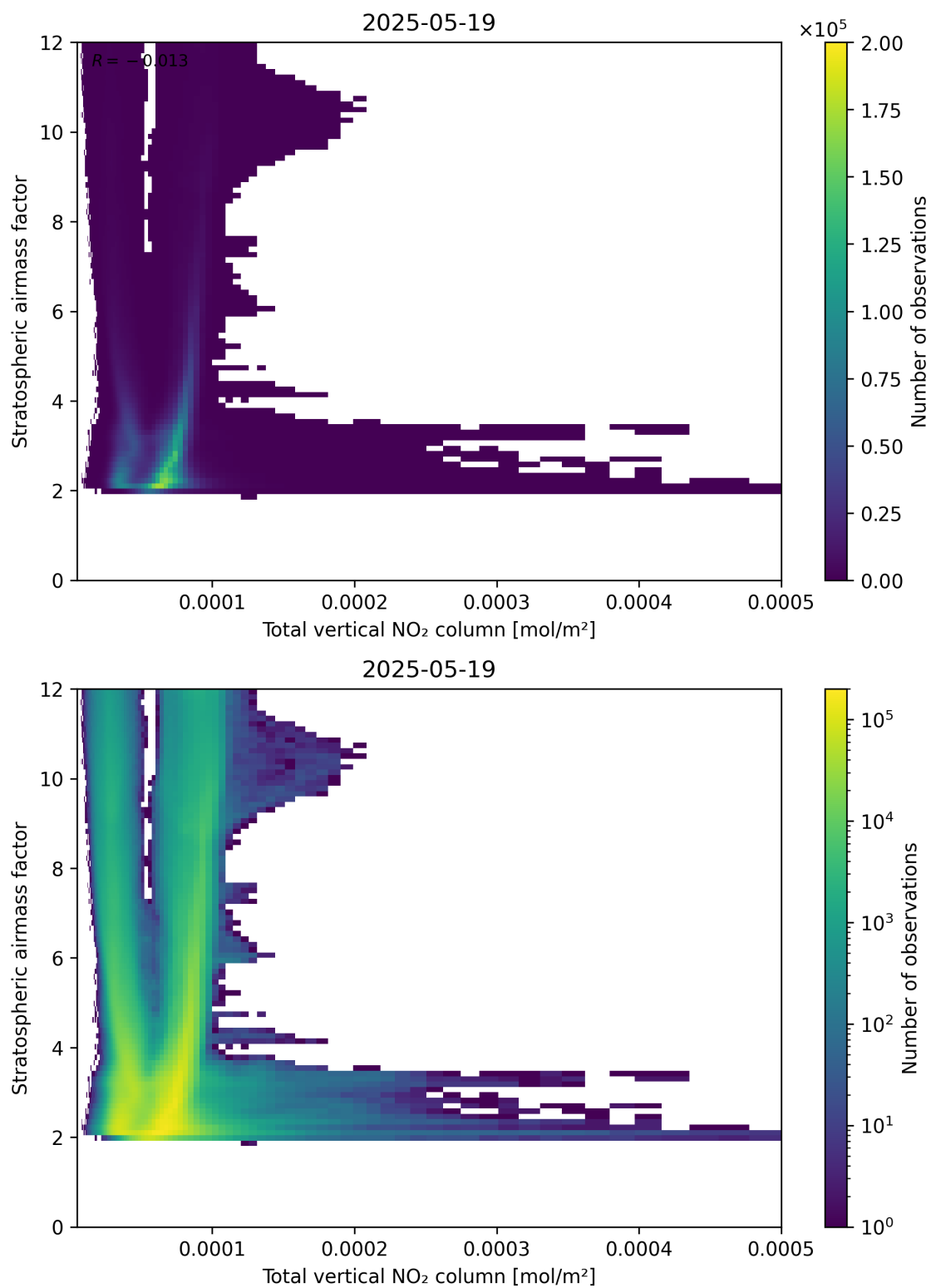
Figure 110: Scatter density plot of “Total vertical NO 2 column” against “Stratospheric airmass factor” for 2025-05-18 to 2025-05-20.
