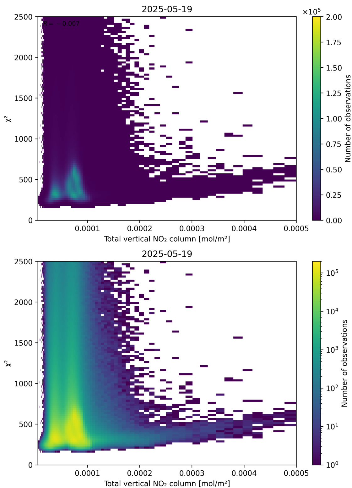
Figure 111: Scatter density plot of “Total vertical NO 2 column” against “ \chi^2 ” for 2025-05-18 to 2025-05-20.
