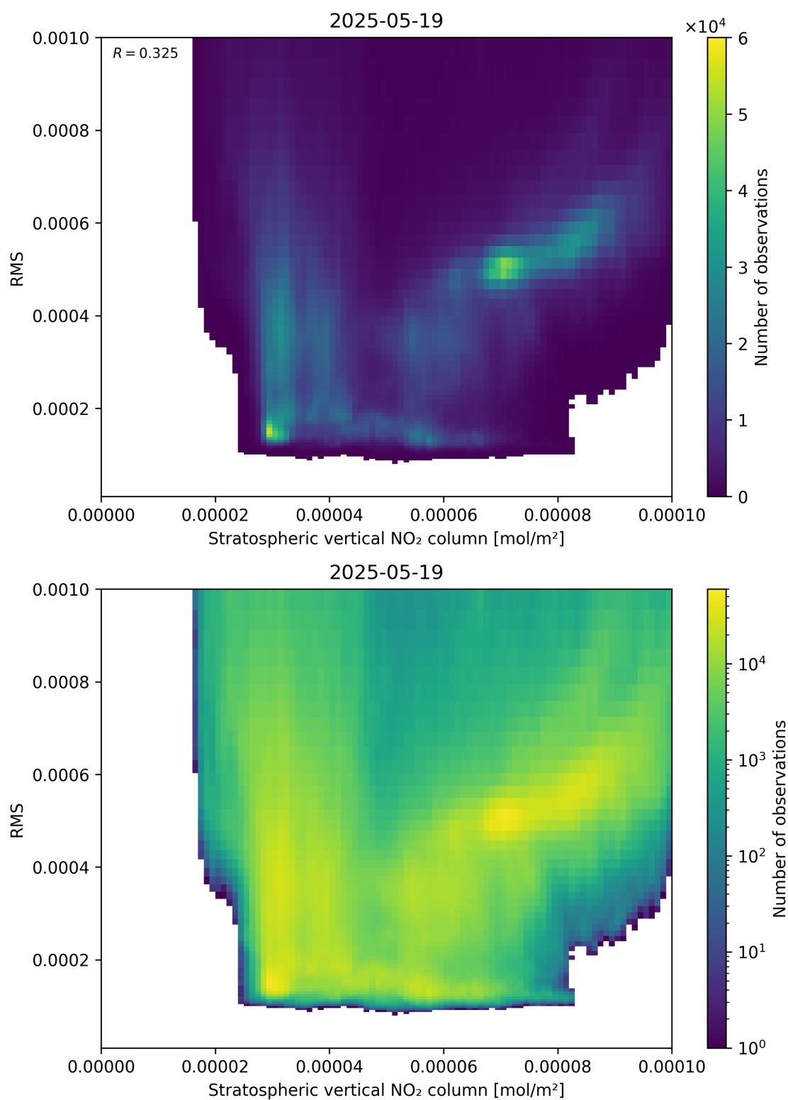
Figure 102: Scatter density plot of “Stratospheric vertical NO 2 column” against “RMS” for 2025-05-18 to 2025-05-20.
