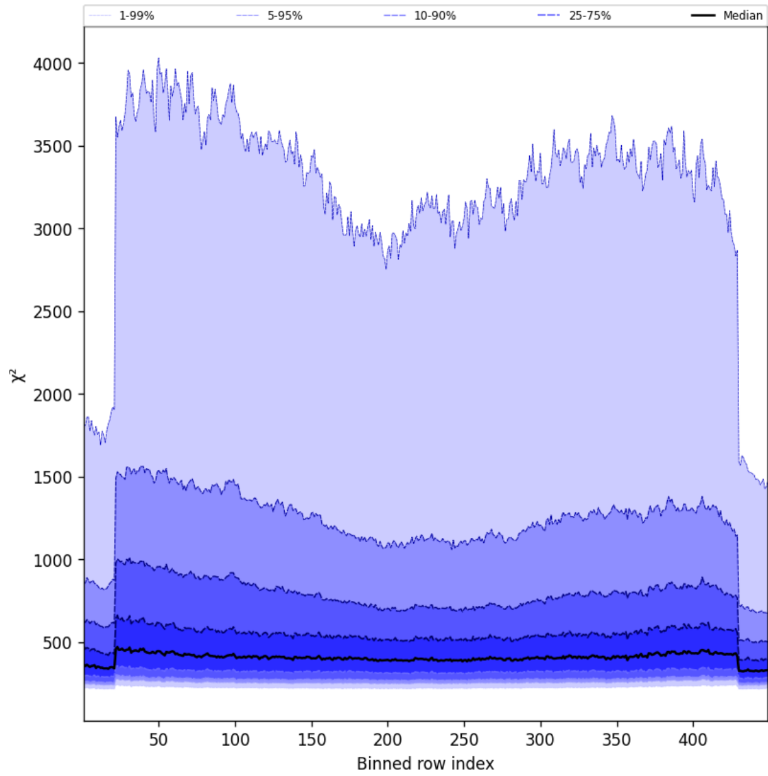
Figure 59: Along track statistics of “ \chi^2 ” for 2025-05-18 to 2025-05-20
