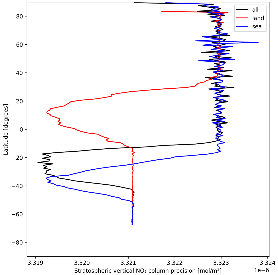
Figure 20: Zonal average of “Stratospheric vertical NO 2 column precision” for 2025-05-18 to 2025-05-20.
