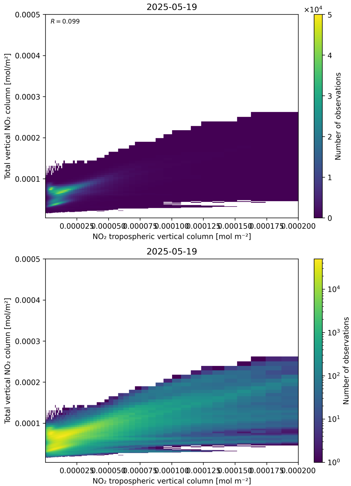
Figure 128: Scatter density plot of “NO 2 tropospheric vertical column” against “Total vertical NO 2 column” for 2025-05-18 to 2025-05-20.
