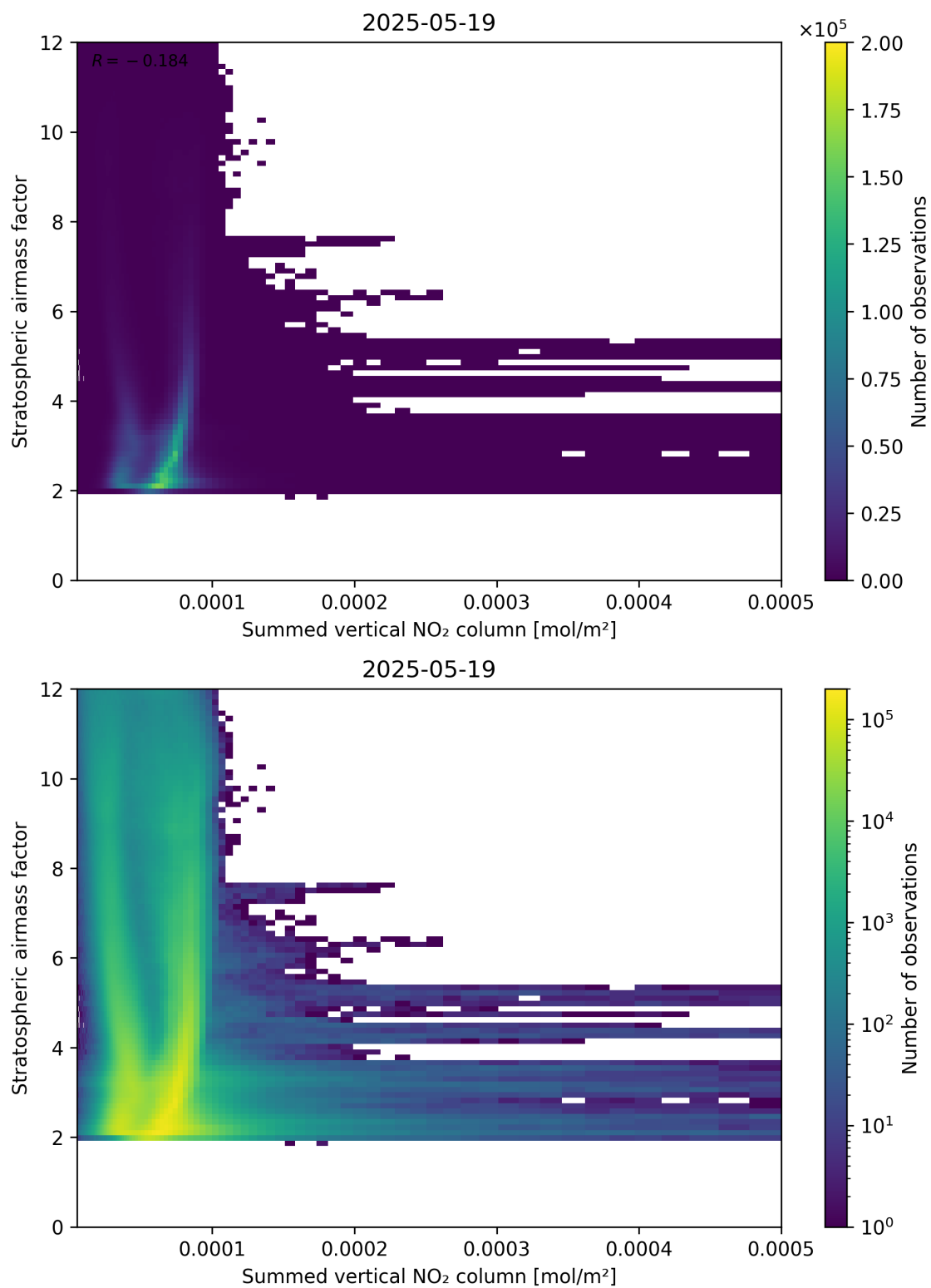
Figure 103: Scatter density plot of “Summed vertical NO 2 column” against “Stratospheric air mass factor” for 2025-05-18 to 2025-05-20.
