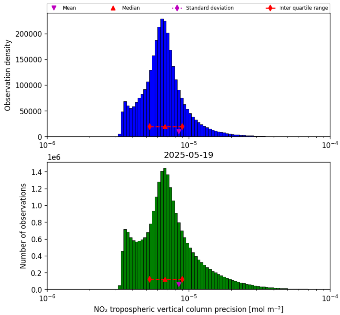
Figure 30: Histogram of “NO 2 tropospheric vertical column precision” for 2025-05-18 to 2025-05-20
