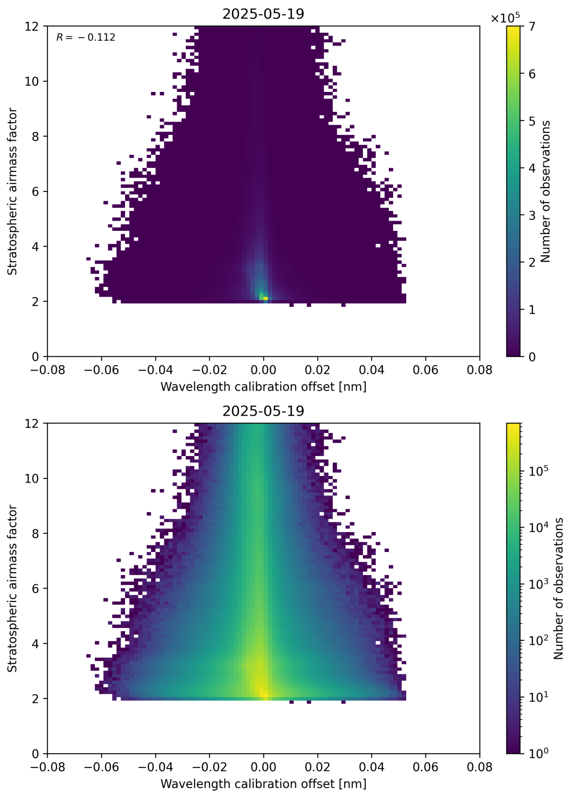
Figure 174: Scatter density plot of “Wavelength calibration offset” against “Stratospheric airmass factor” for 2025-05-18 to 2025-05-20.
