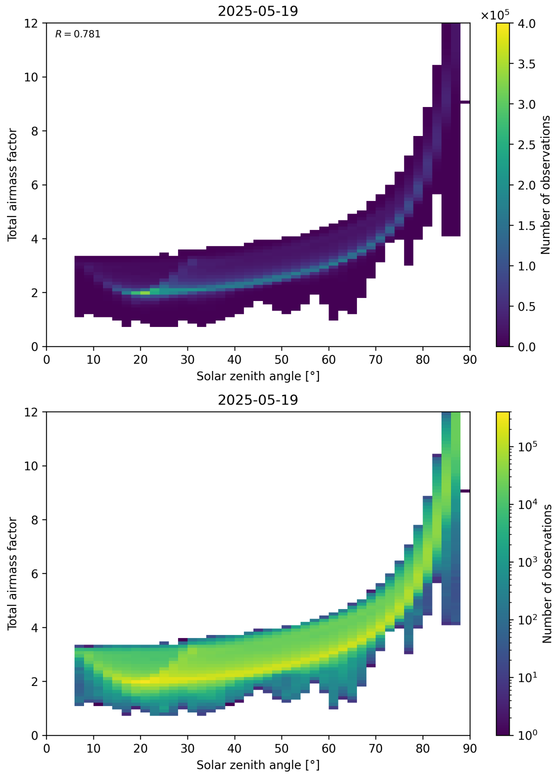
Figure 146: Scatter density plot of “Solar zenith angle” against “Total air mass factor” for 2025-05-18 to 2025-05-20.
