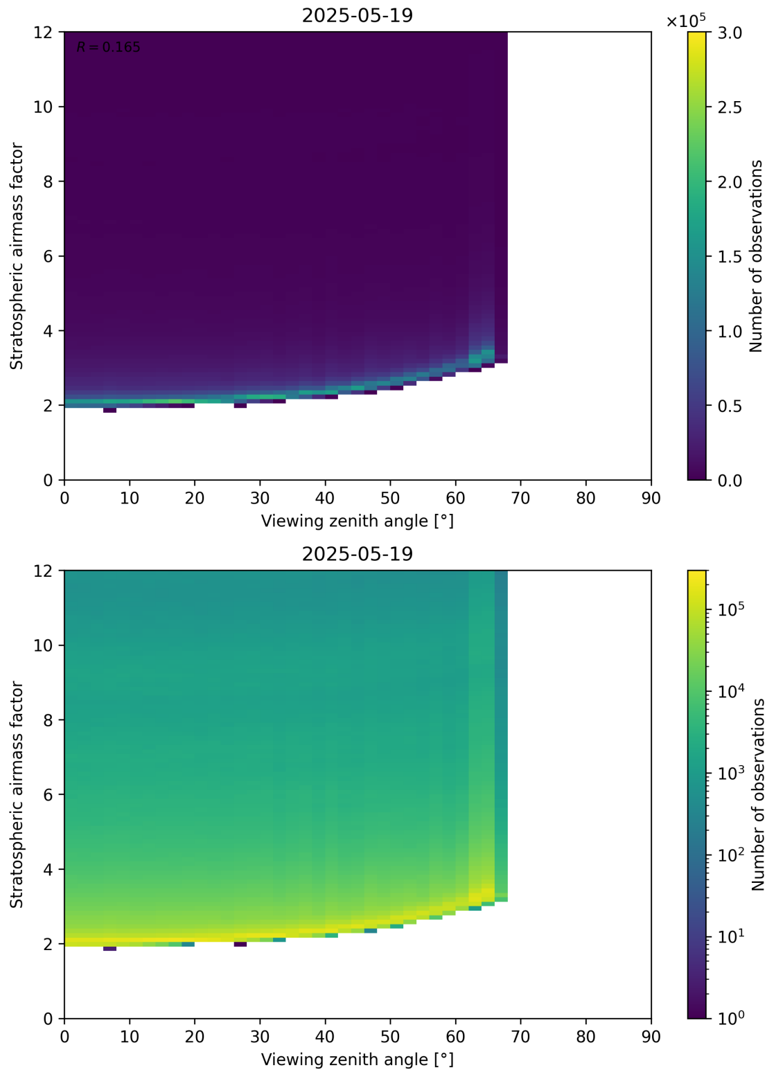
Figure 159: Scatter density plot of “Viewing zenith angle” against “Stratospheric airmass factor” for 2025-05-18 to 2025-05-20.
