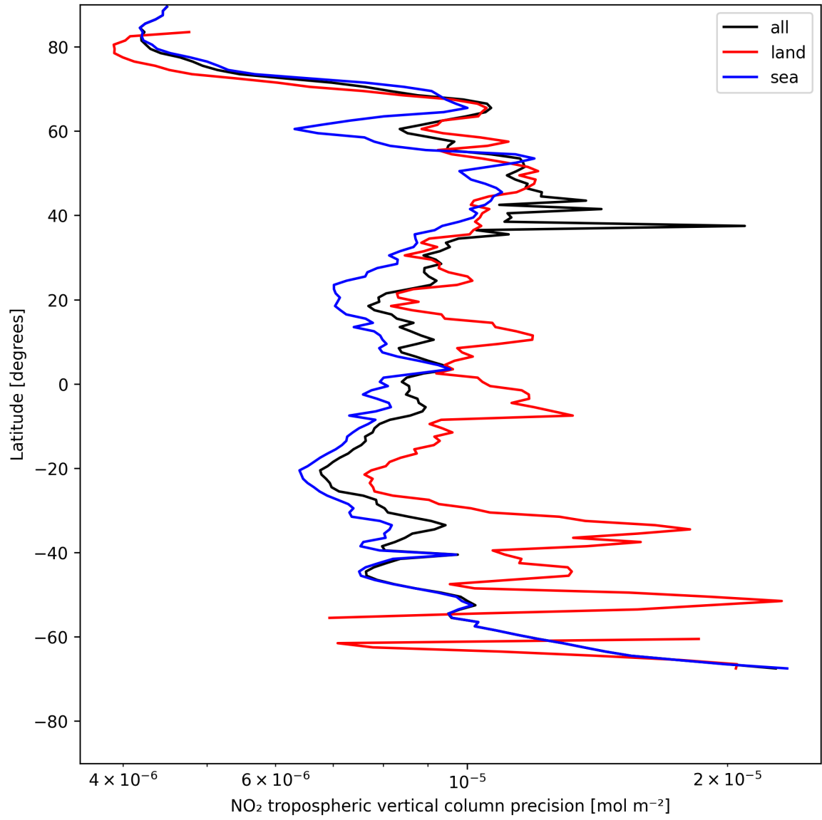
Figure 13: Zonal average of “NO 2 tropospheric vertical column precision” for 2025-05-18 to 2025-05-20.
