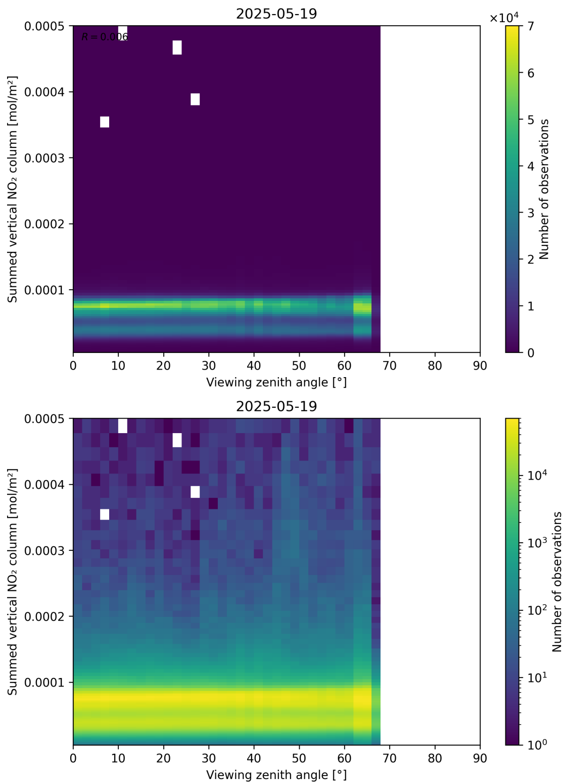
Figure 165: Scatter density plot of “Viewing zenith angle” against “Summed vertical NO 2 column” for 2025-05-18 to 2025-05-20.
