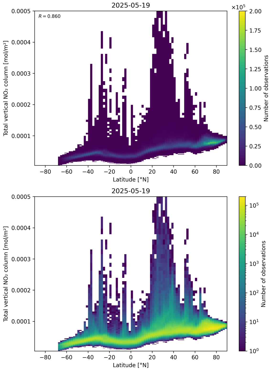
Figure 90: Scatter density plot of “Latitude” against “Total vertical NO 2 column” for 2025-05-18 to 2025-05-20.
