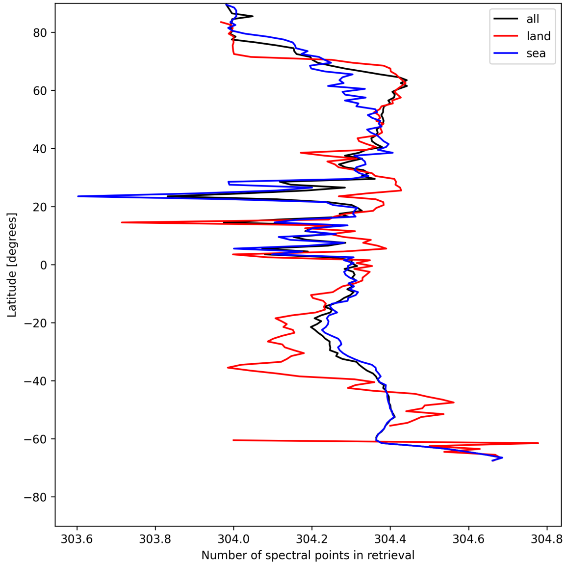
Figure 16: Zonal average of “Number of spectral points in retrieval” for 2025-05-18 to 2025-05-20.
