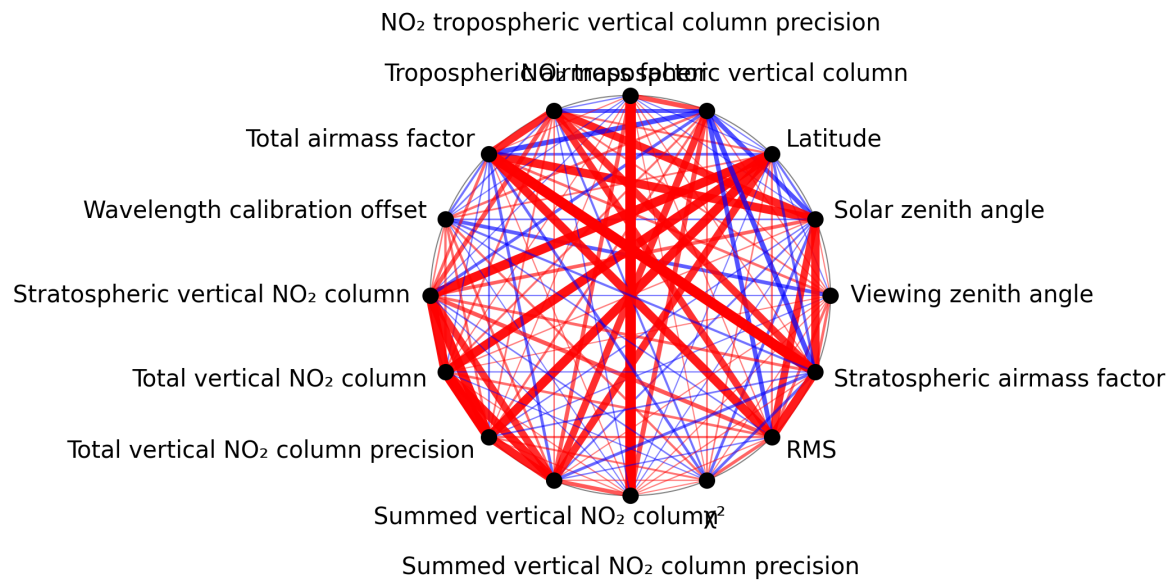
Figure 1: Map of correlation graph for 2025-05-18 to 2025-05-20.
