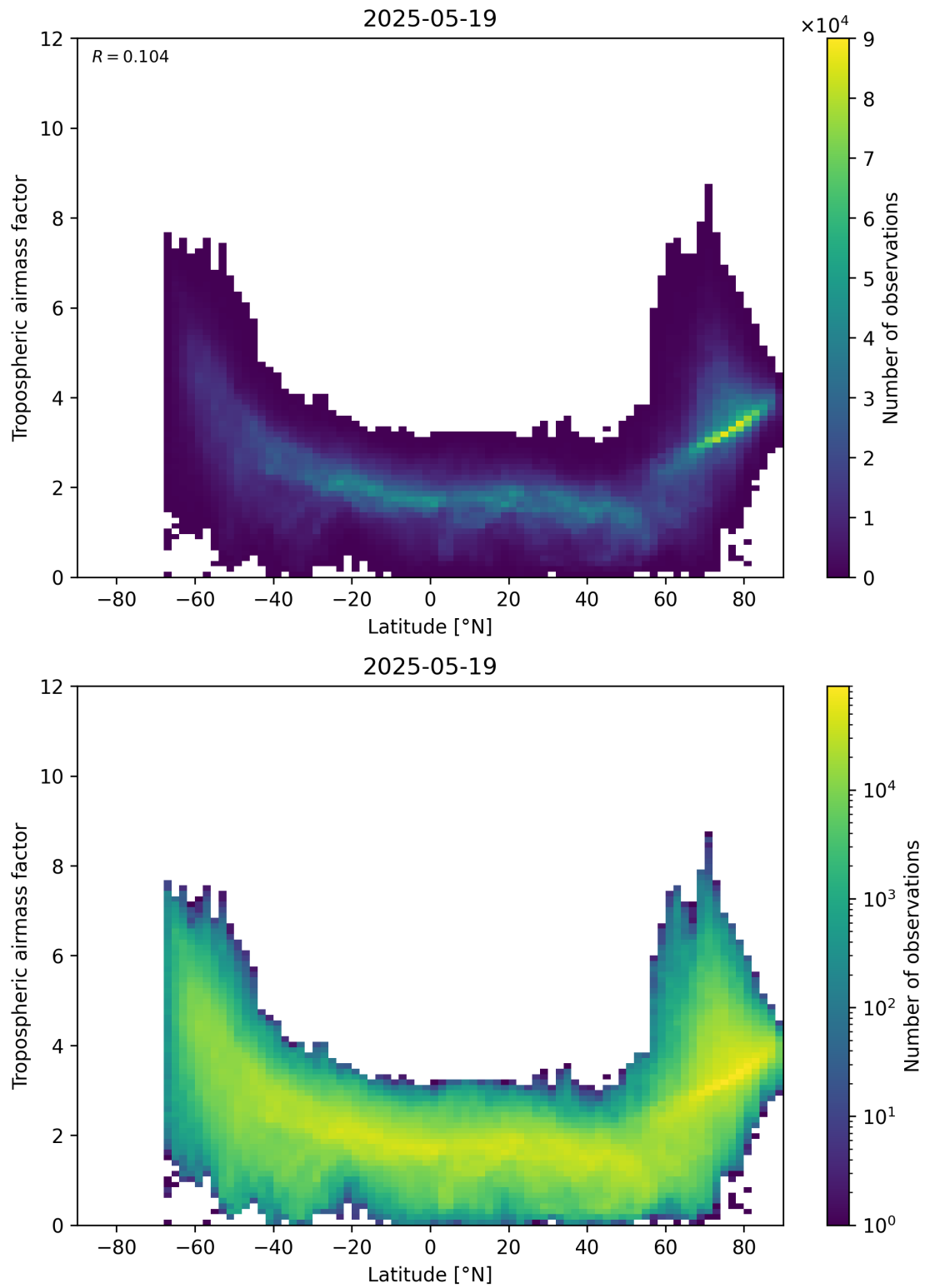
Figure 85: Scatter density plot of “Latitude” against “Tropospheric air mass factor” for 2025-05-18 to 2025-05-20.
