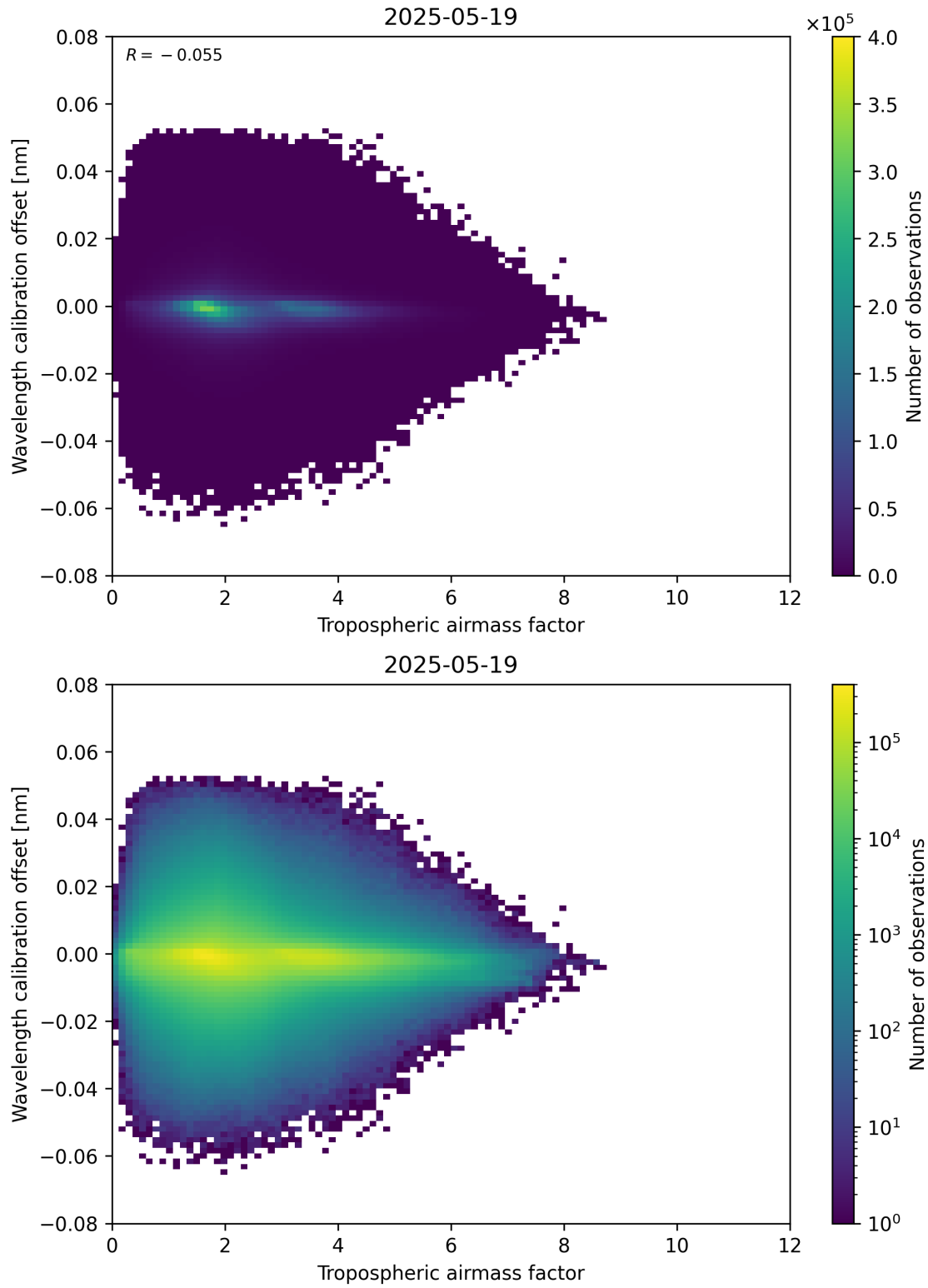
Figure 80: Scatter density plot of “Tropospheric airmass factor” against “Wavelength calibration offset” for 2025-05-18 to 2025-05-20.
