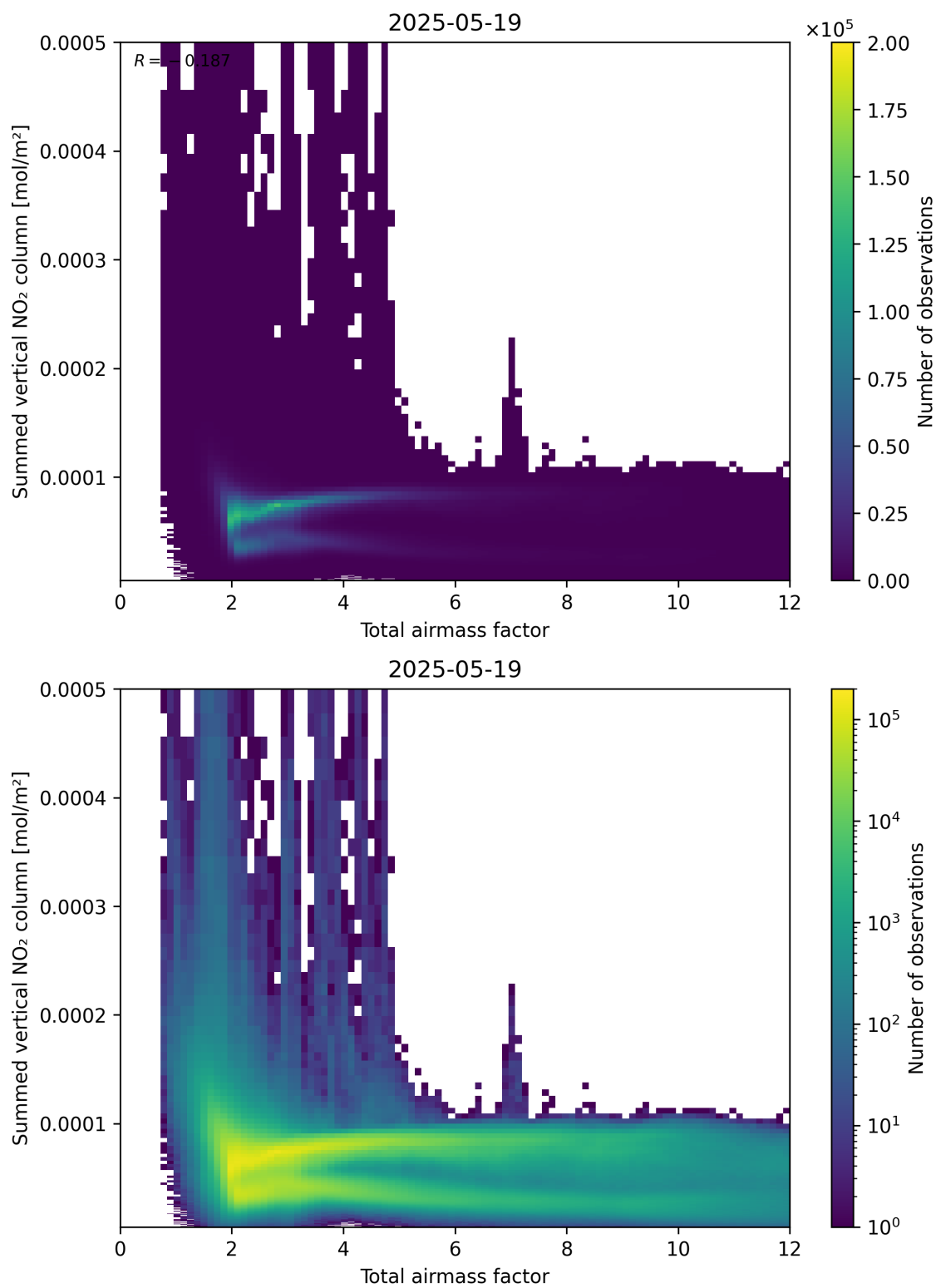
Figure 65: Scatter density plot of “Total airmass factor” against “Summed vertical NO 2 column” for 2025-05-18 to 2025-05-20.
