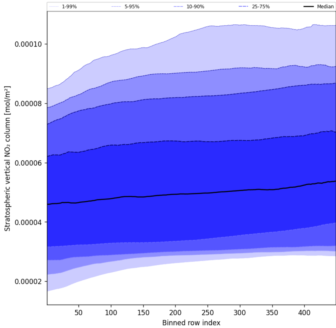
Figure 53: Along track statistics of “Stratospheric vertical NO 2 column” for 2025-05-18 to 2025-05-20
