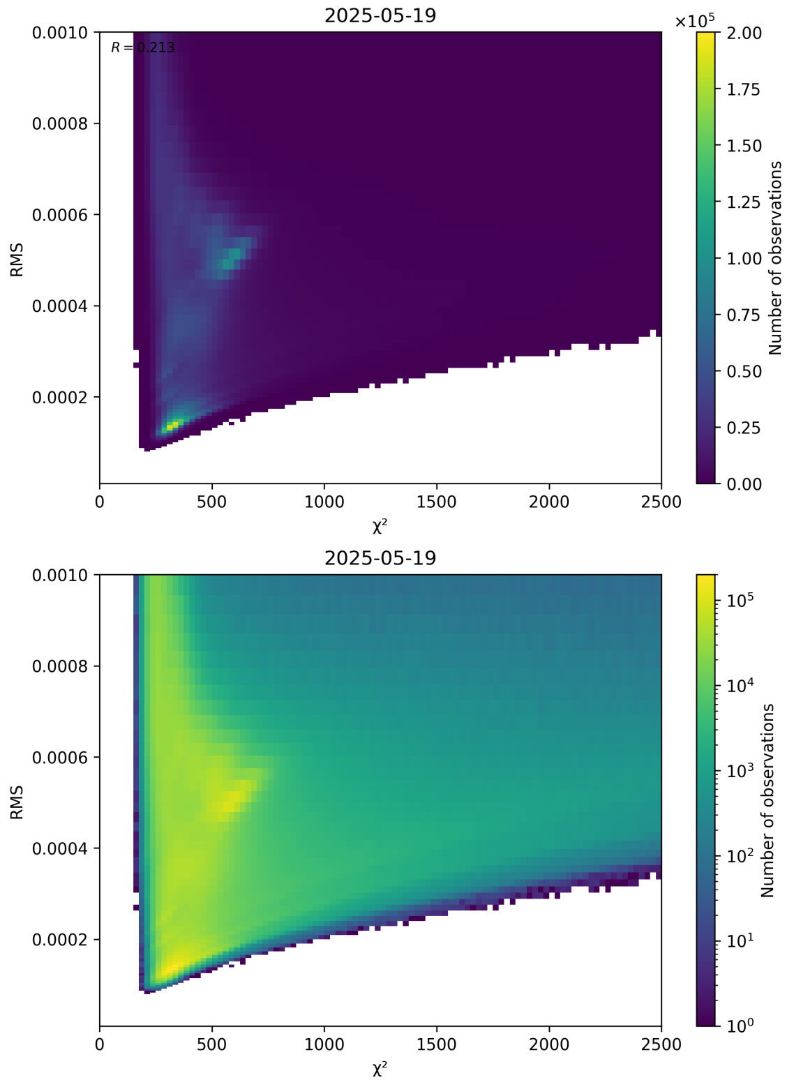
Figure 82: Scatter density plot of “ \chi^2 ” against “RMS” for 2025-05-18 to 2025-05-20.
