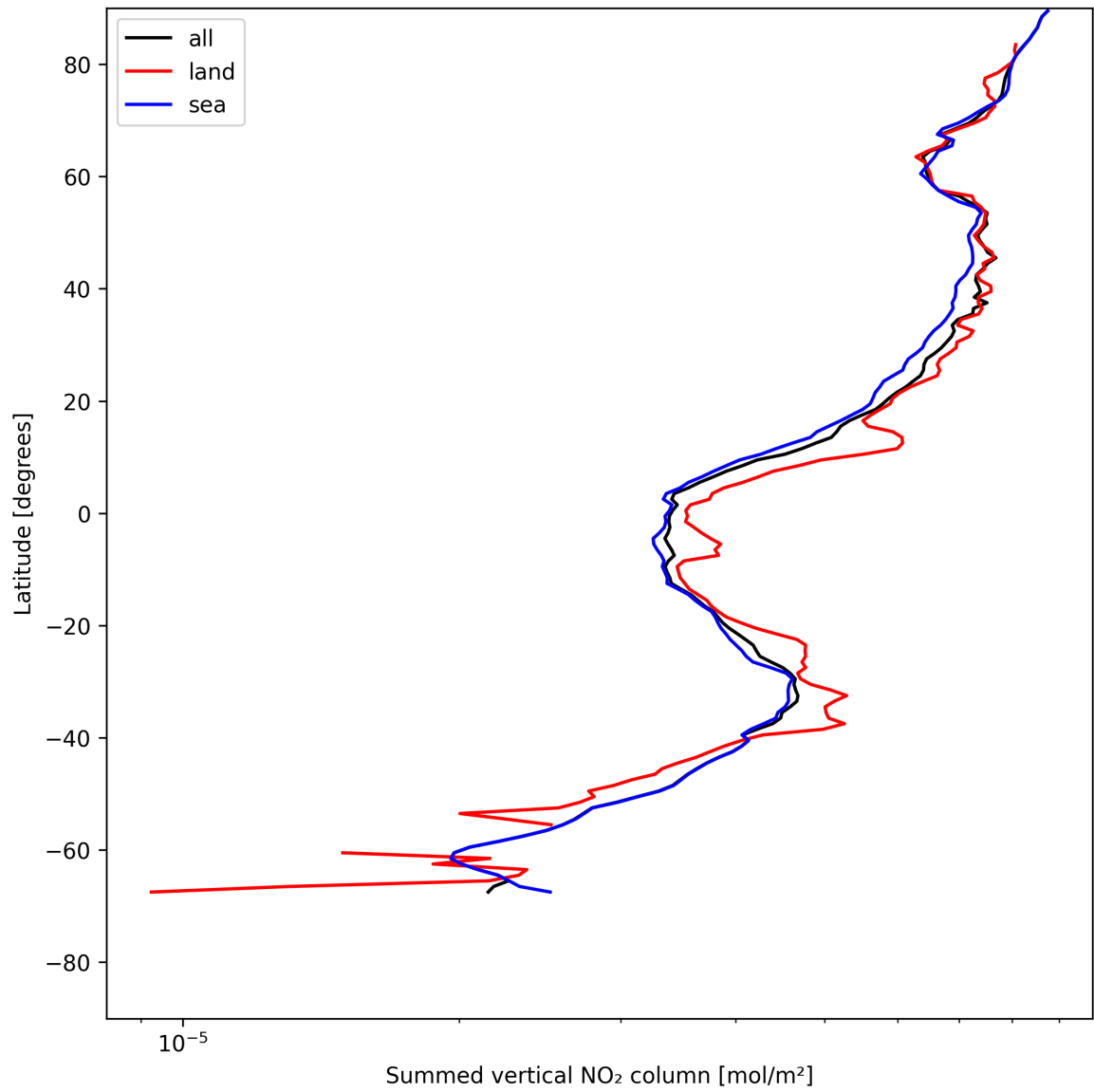
Figure 23: Zonal average of “Summed vertical NO 2 column” for 2025-05-18 to 2025-05-20.
