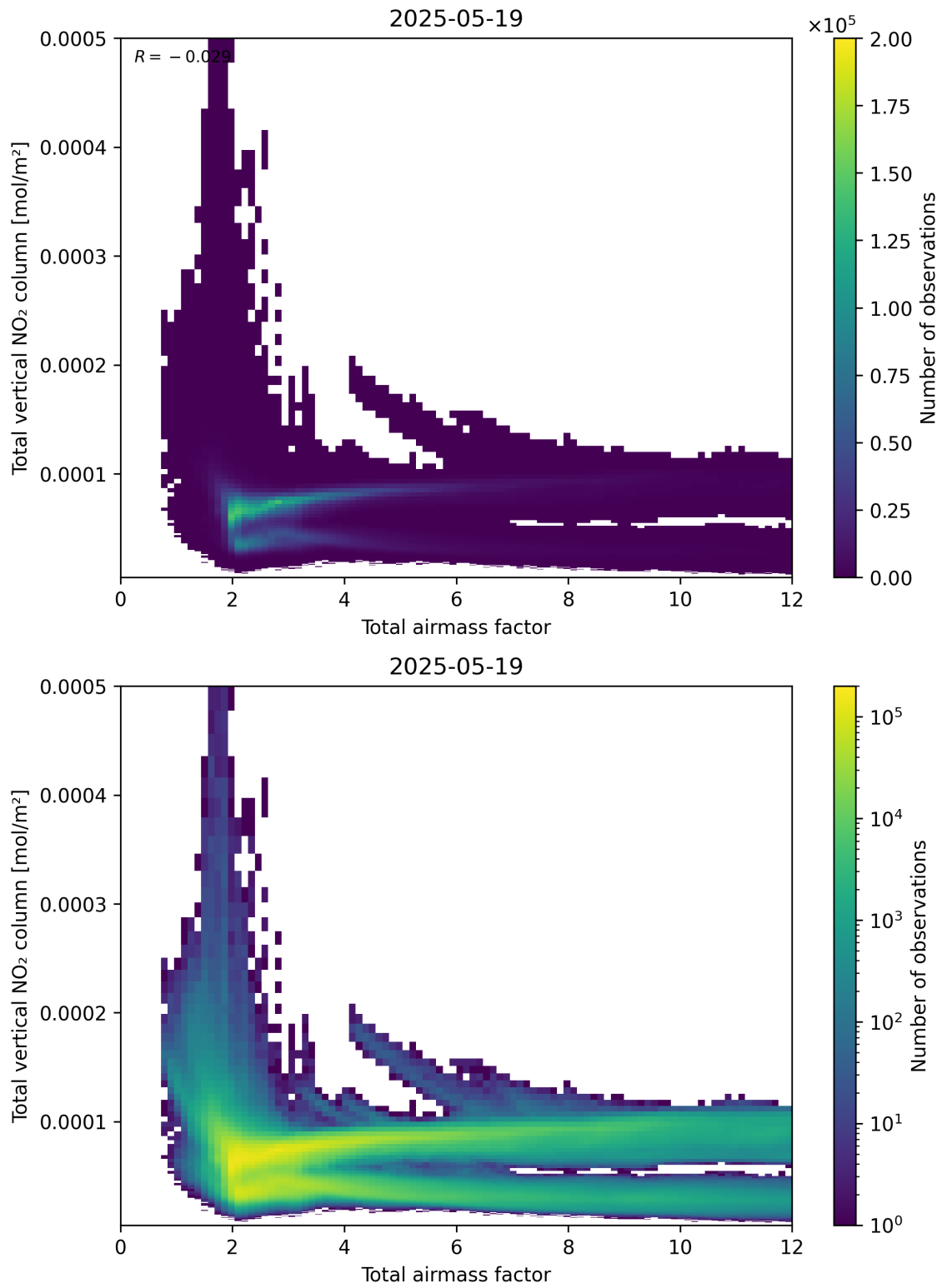
Figure 67: Scatter density plot of “Total airmass factor” against “Total vertical NO 2 column” for 2025-05-18 to 2025-05-20.
