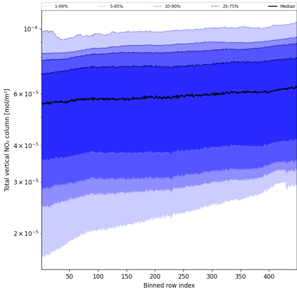
Figure 55: Along track statistics of “Total vertical NO 2 column” for 2025-05-18 to 2025-05-20
