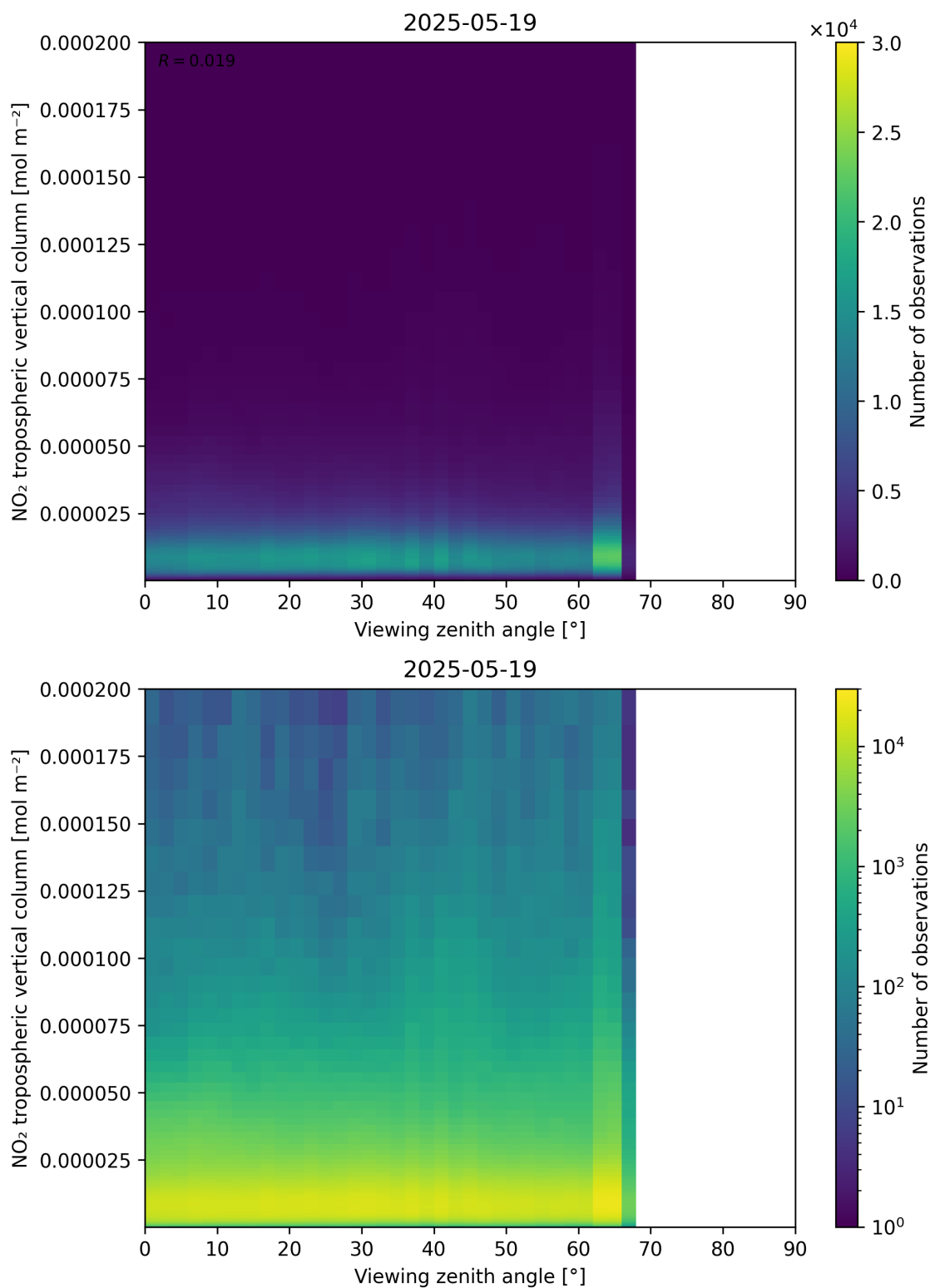
Figure 169: Scatter density plot of “Viewing zenith angle” against “NO 2 tropospheric vertical column” for 2025-05-18 to 2025-05-20.
