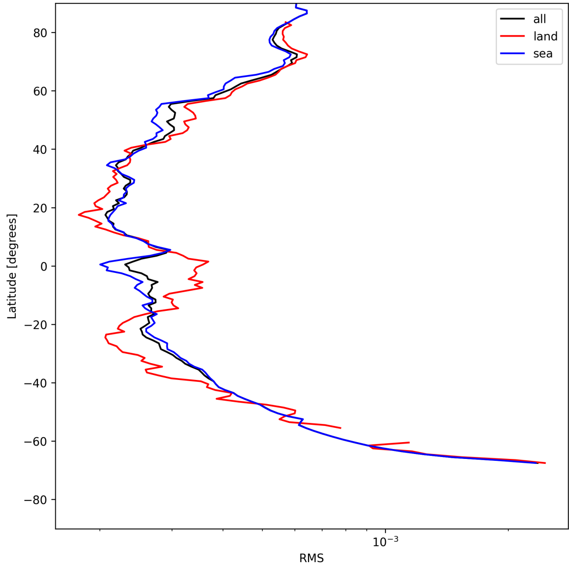
Figure 26: Zonal average of “RMS” for 2025-05-18 to 2025-05-20.
