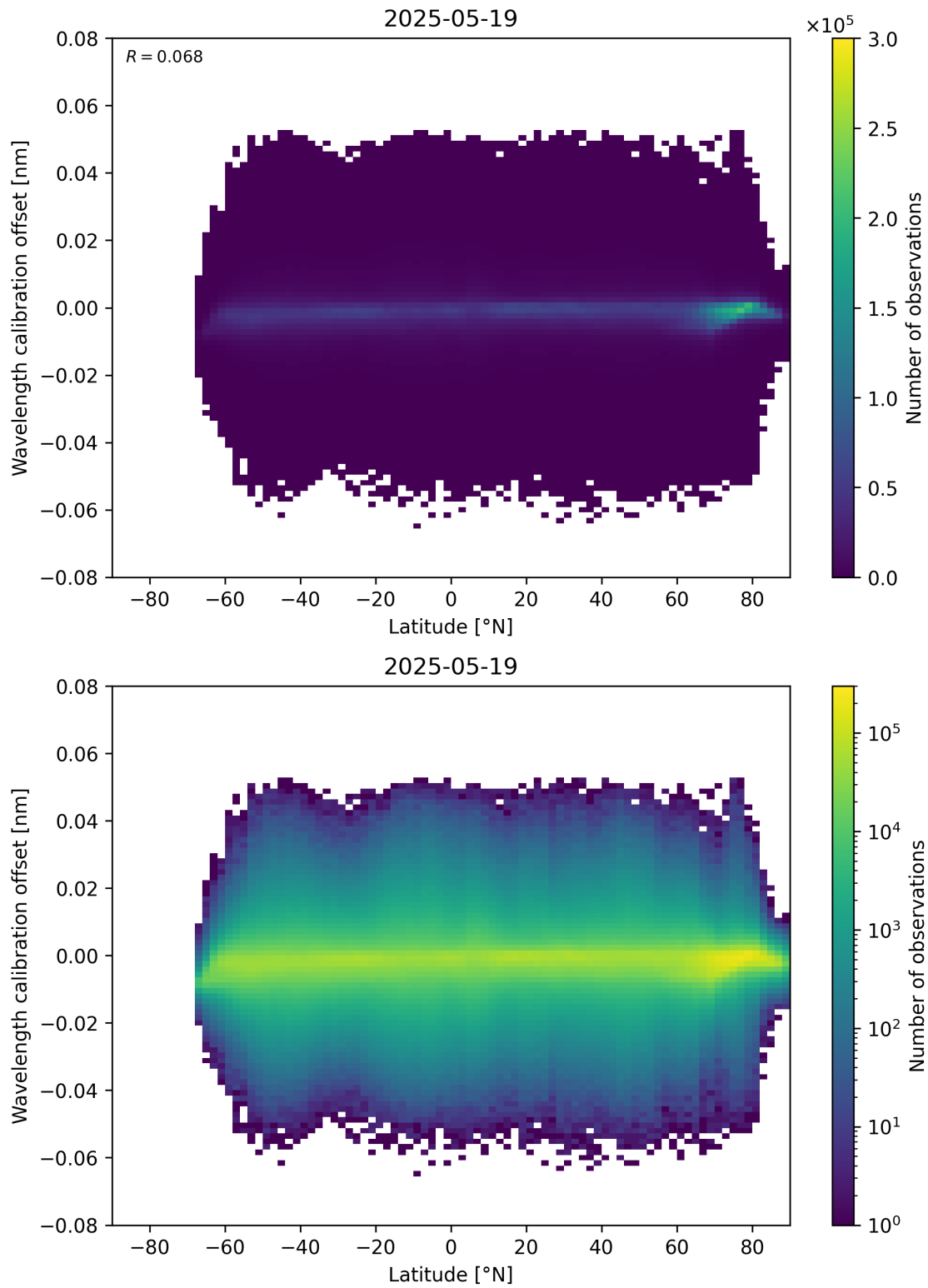
Figure 95: Scatter density plot of “Latitude” against “Wavelength calibration offset” for 2025-05-18 to 2025-05-20.
