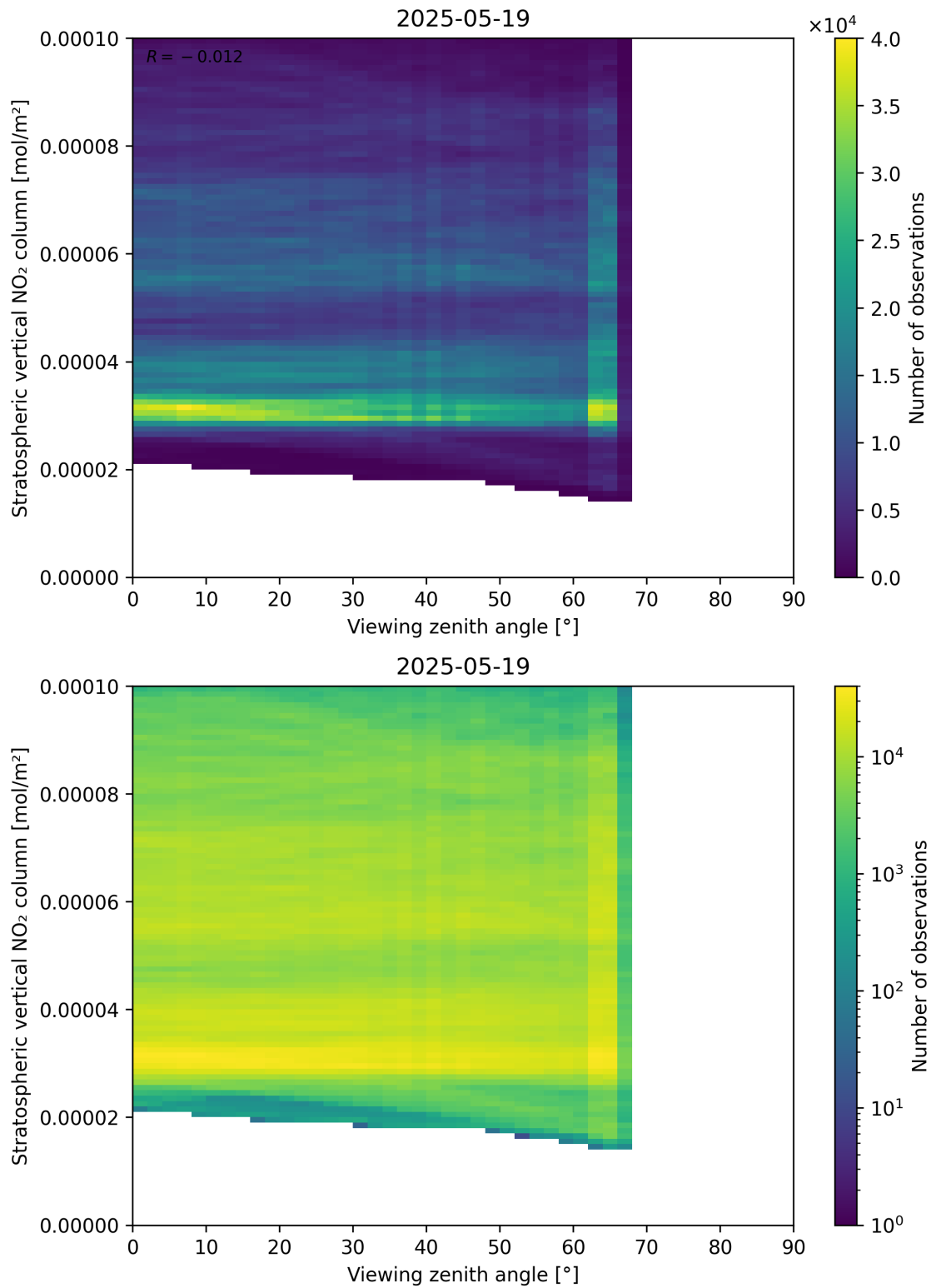
Figure 164: Scatter density plot of “Viewing zenith angle” against “Stratospheric vertical NO 2 column” for 2025-05-18 to 2025-05-20.
