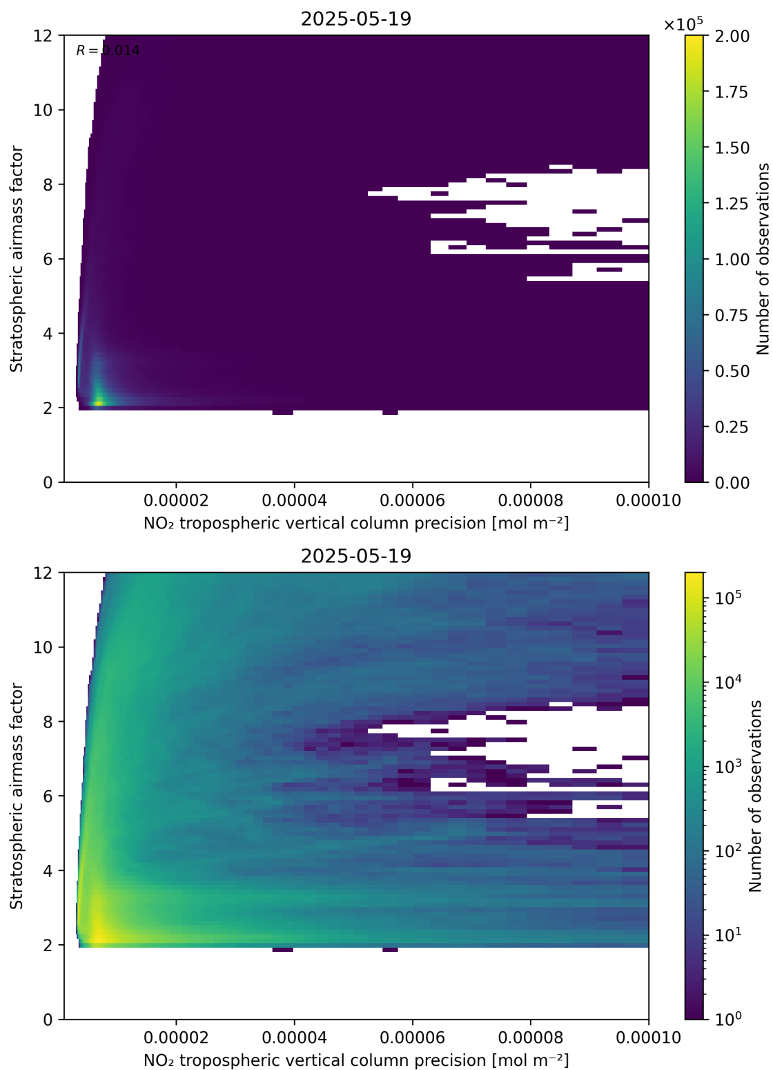
Figure 131: Scatter density plot of “NO 2 tropospheric vertical column precision” against “Stratospheric airmass factor” for 2025-05-18 to 2025-05-20.
