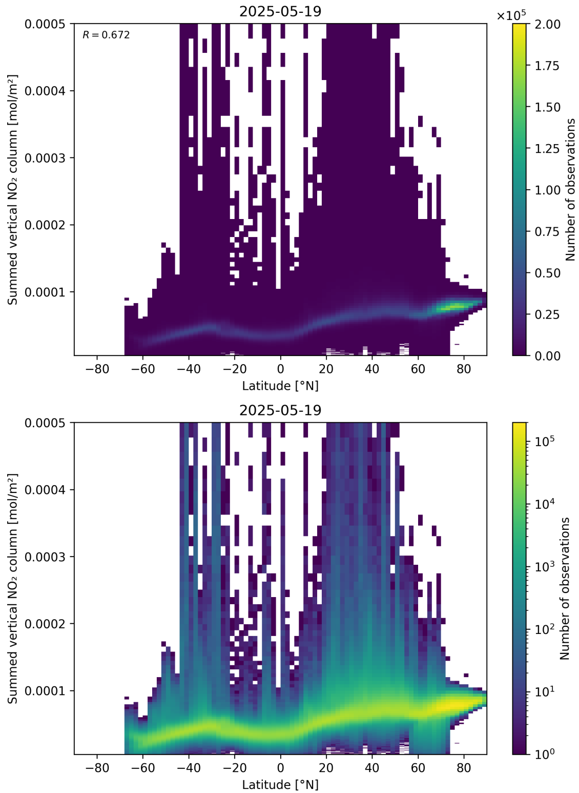
Figure 88: Scatter density plot of “Latitude” against “Summed vertical NO 2 column” for 2025-05-18 to 2025-05-20.
