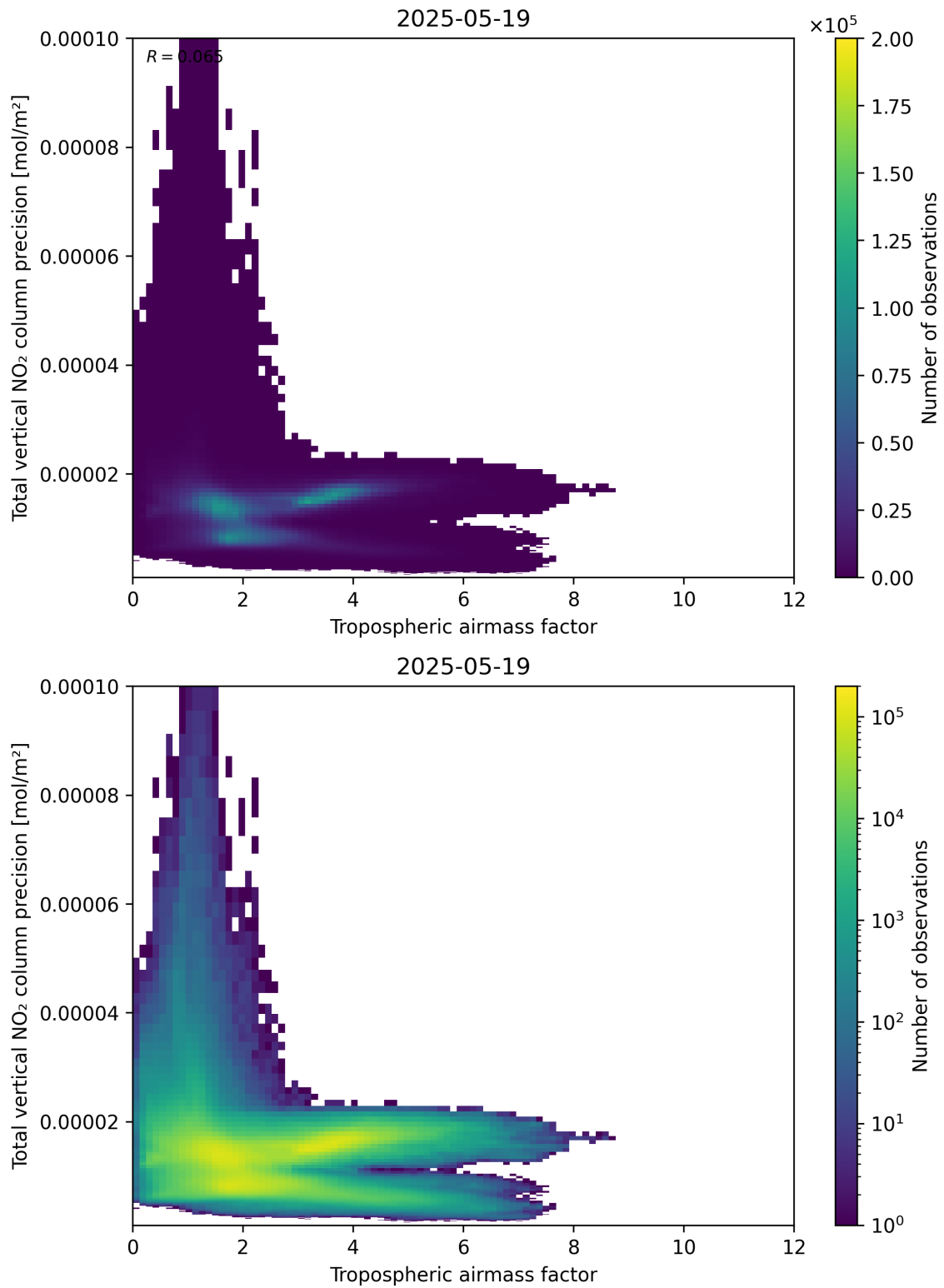
Figure 78: Scatter density plot of “Tropospheric airmass factor” against “Total vertical NO 2 column precision” for 2025-05-18 to 2025-05-20.
