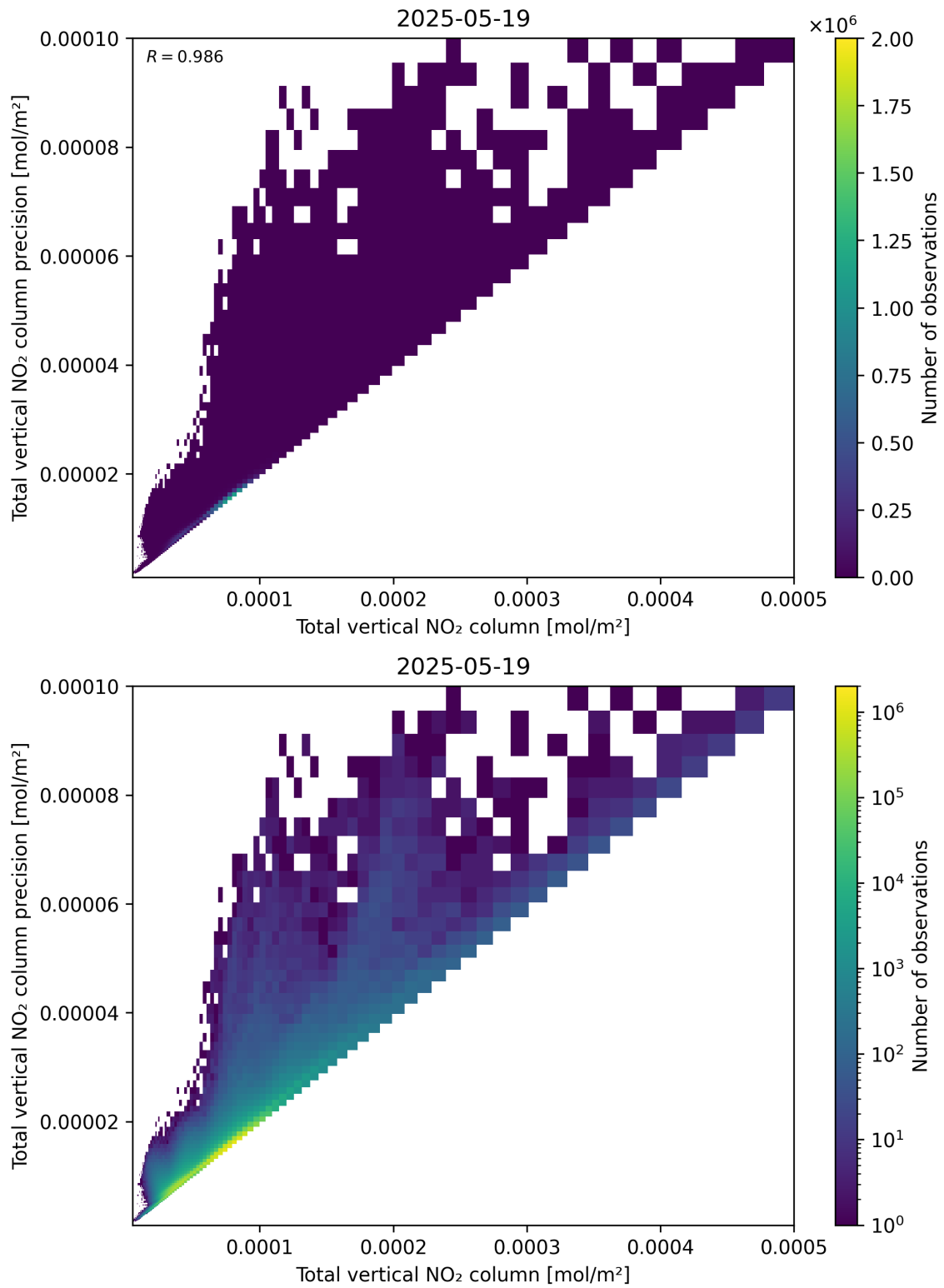
Figure 114: Scatter density plot of “Total vertical NO 2 column” against “Total vertical NO 2 column precision” for 2025-05-18 to 2025-05-20.
