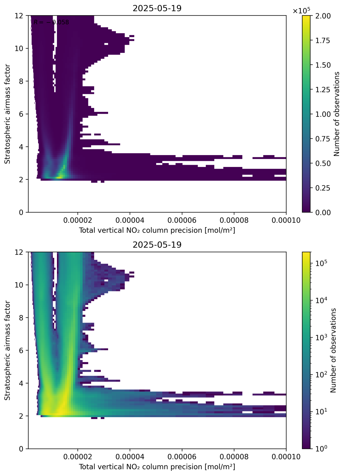
Figure 115: Scatter density plot of “Total vertical NO 2 column precision” against “Stratospheric air mass factor” for 2025-05-18 to 2025-05-20.
