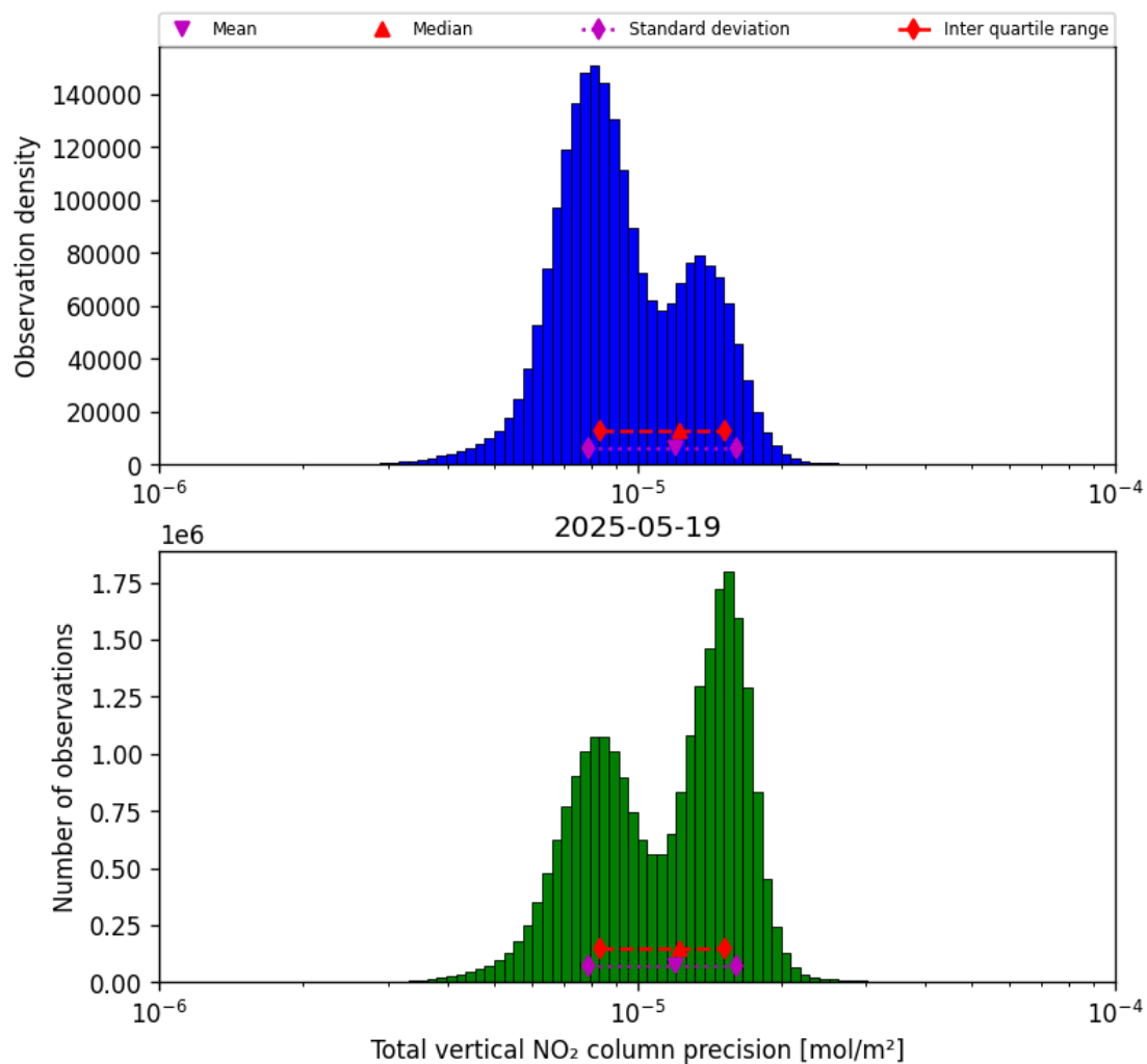
Figure 39: Histogram of “Total vertical NO 2 column precision” for 2025-05-18 to 2025-05-20
