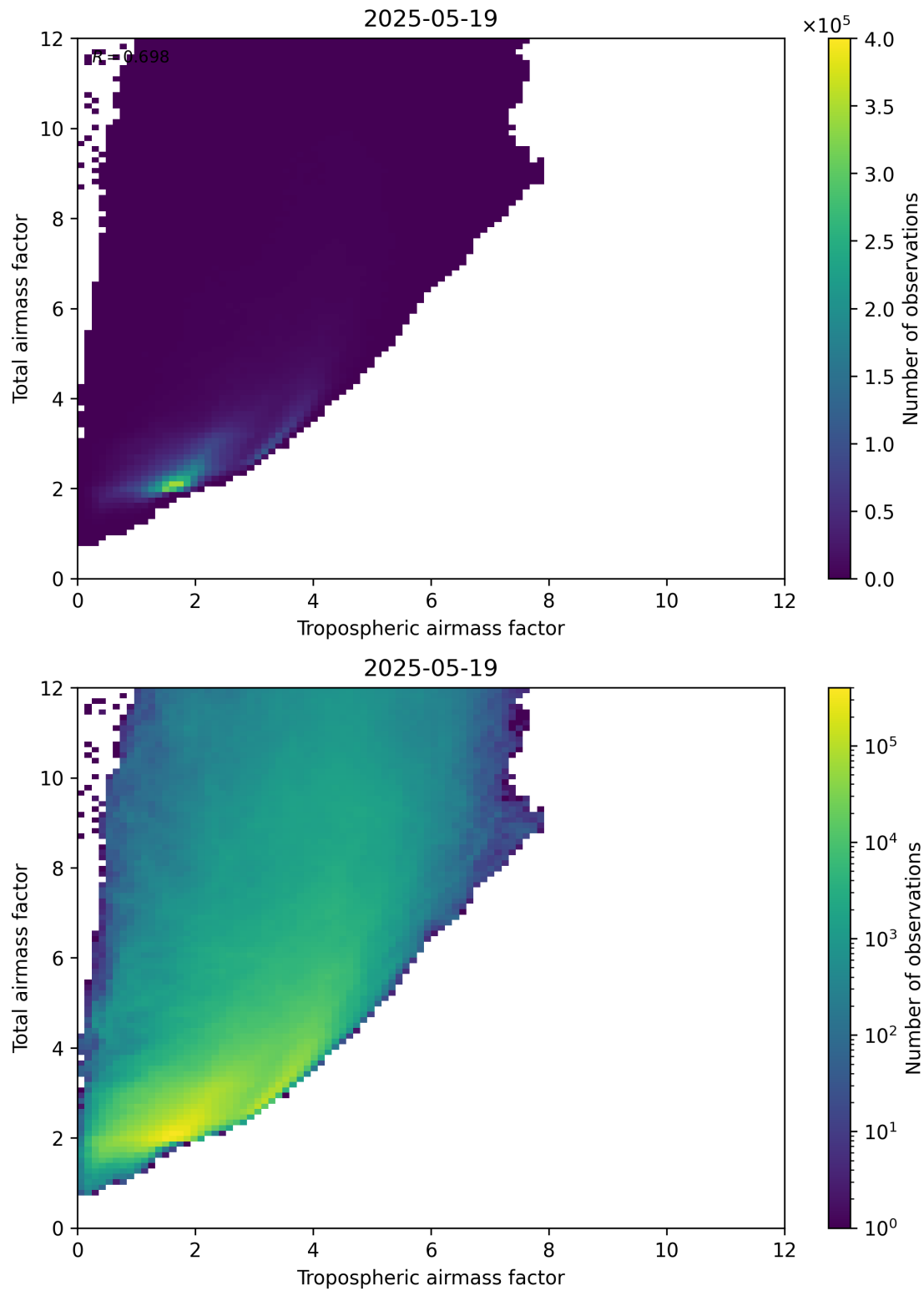
Figure 72: Scatter density plot of “Tropospheric airmass factor” against “Total airmass factor” for 2025-05-18 to 2025-05-20.
