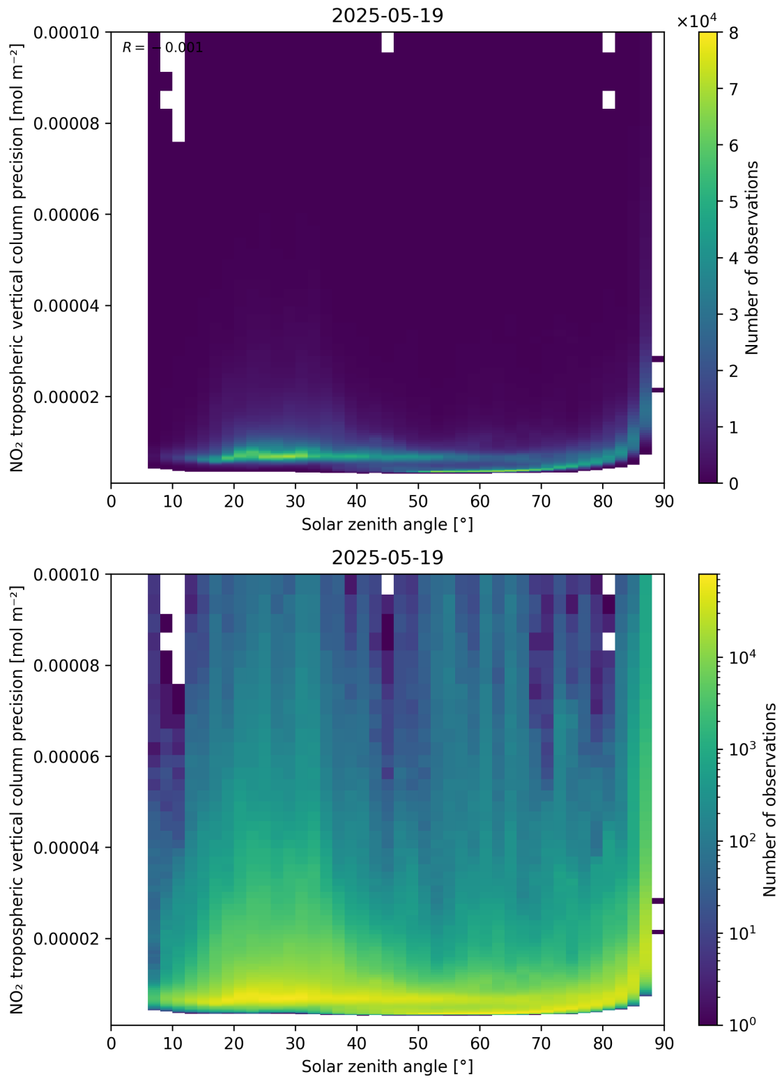
Figure 156: Scatter density plot of “Solar zenith angle” against “NO 2 tropospheric vertical column precision” for 2025-05-18 to 2025-05-20.
