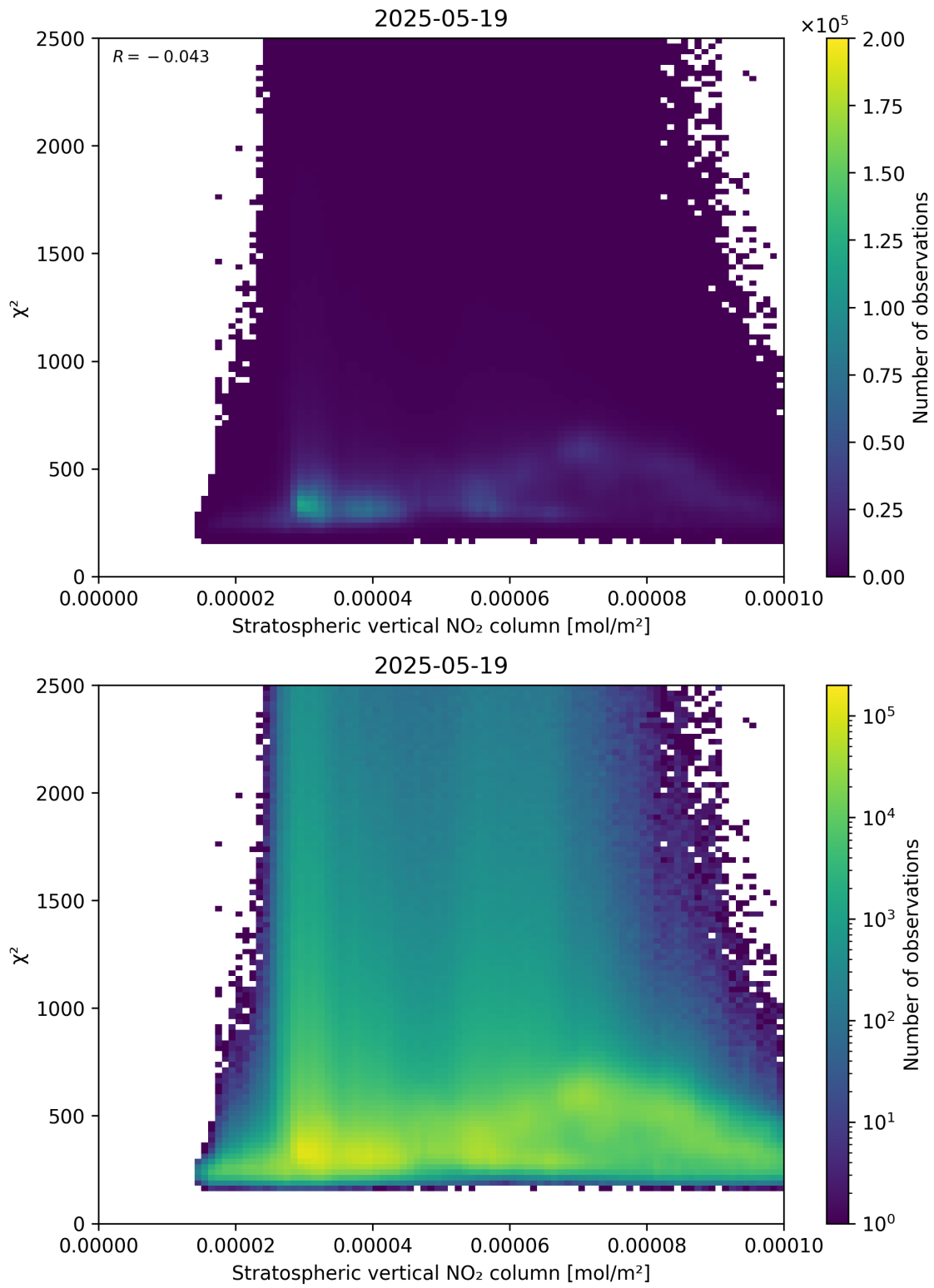
Figure 97: Scatter density plot of “Stratospheric vertical NO 2 column” against “ \chi^2 ” for 2025-05-18 to 2025-05-20.
