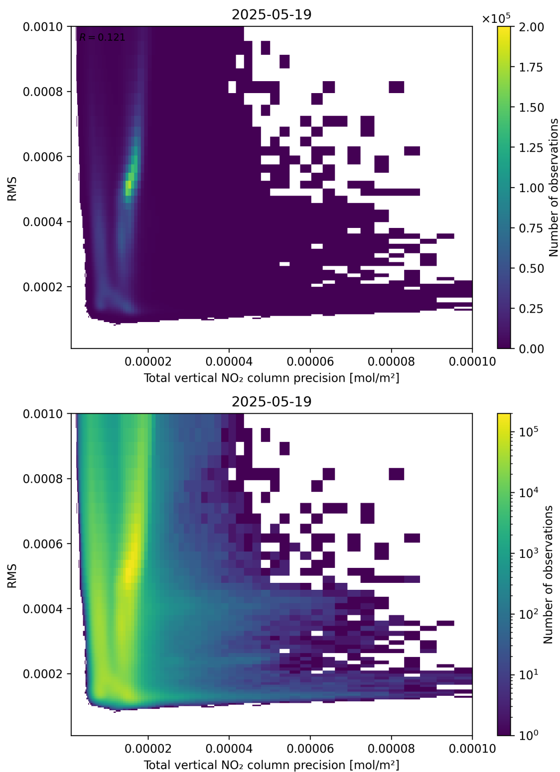
Figure 119: Scatter density plot of “Total vertical NO 2 column precision” against “RMS” for 2025-05-18 to 2025-05-20.
