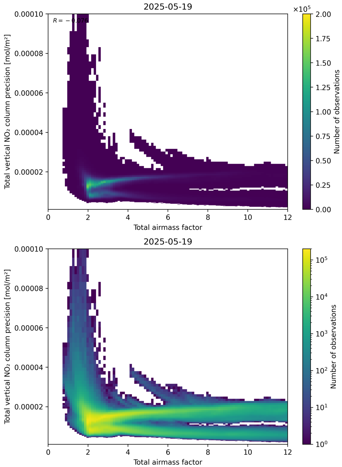
Figure 68: Scatter density plot of “Total airmass factor” against “Total vertical NO 2 column precision” for 2025-05-18 to 2025-05-20.
