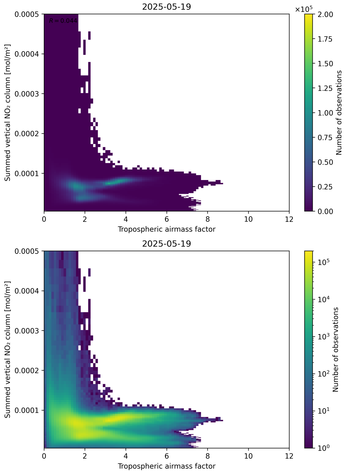
Figure 75: Scatter density plot of “Tropospheric airmass factor” against “Summed vertical NO 2 column” for 2025-05-18 to 2025-05-20.
