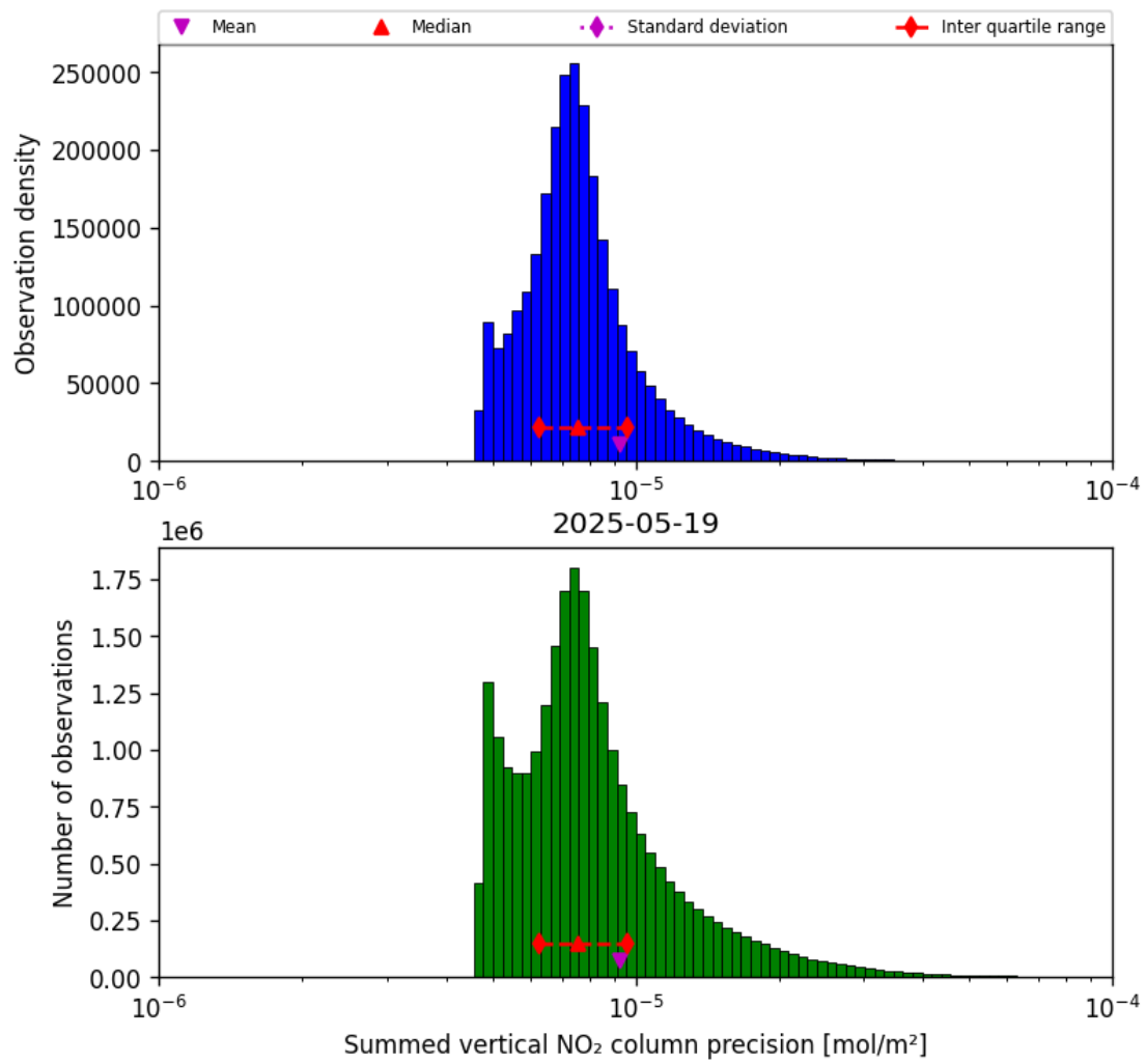
Figure 41: Histogram of “Summed vertical NO 2 column precision” for 2025-05-18 to 2025-05-20
