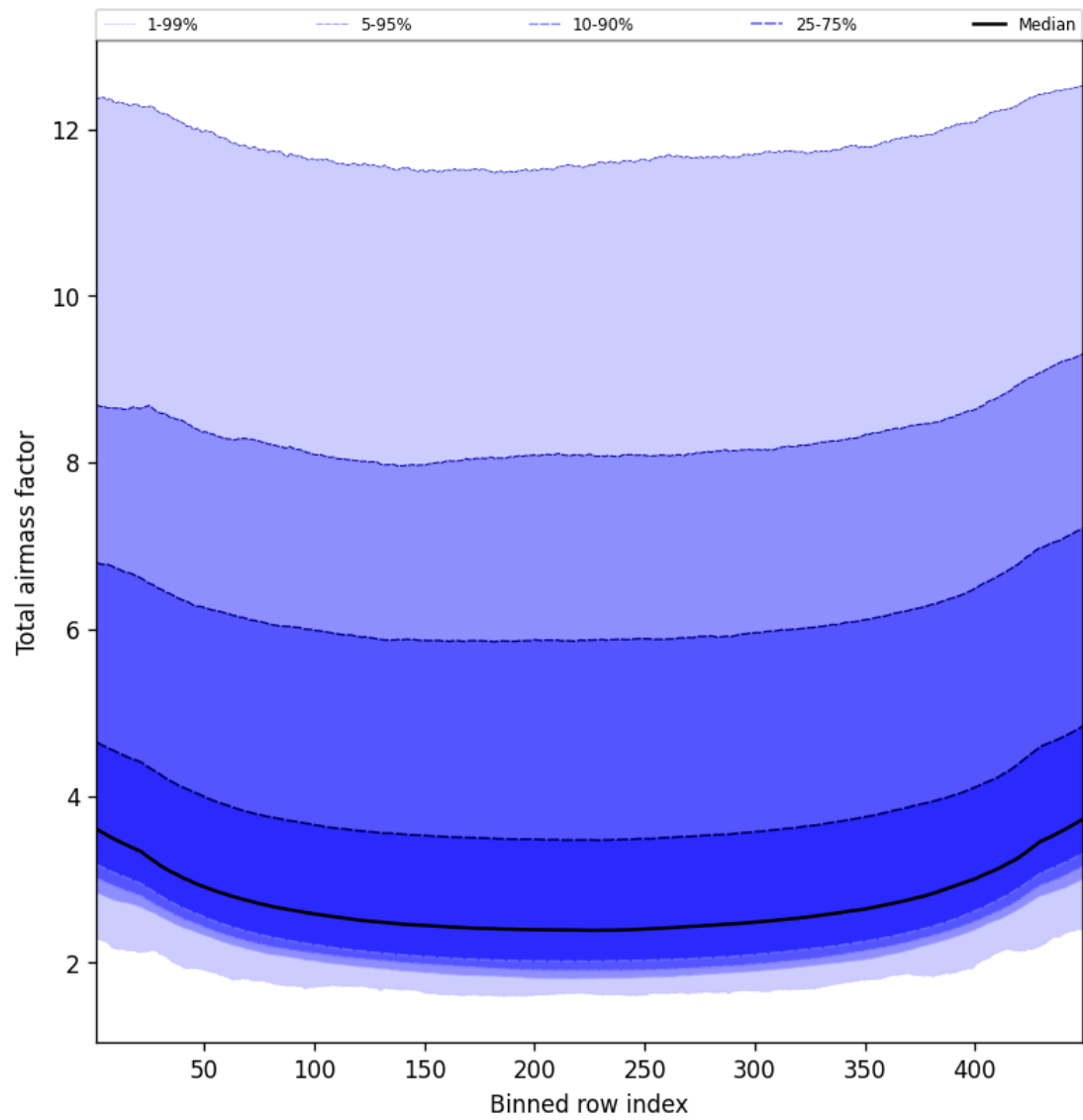
Figure 49: Along track statistics of “Total airmass factor” for 2025-05-18 to 2025-05-20
