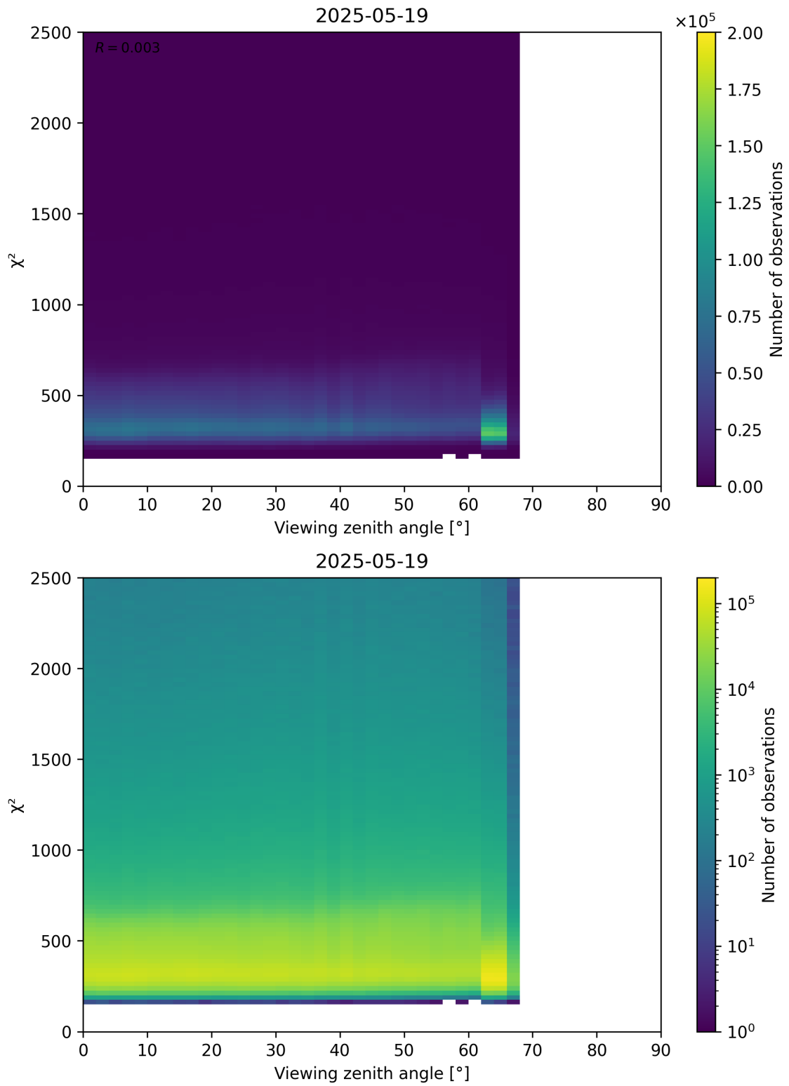
Figure 162: Scatter density plot of “Viewing zenith angle” against “ \chi^2 ” for 2025-05-18 to 2025-05-20.
