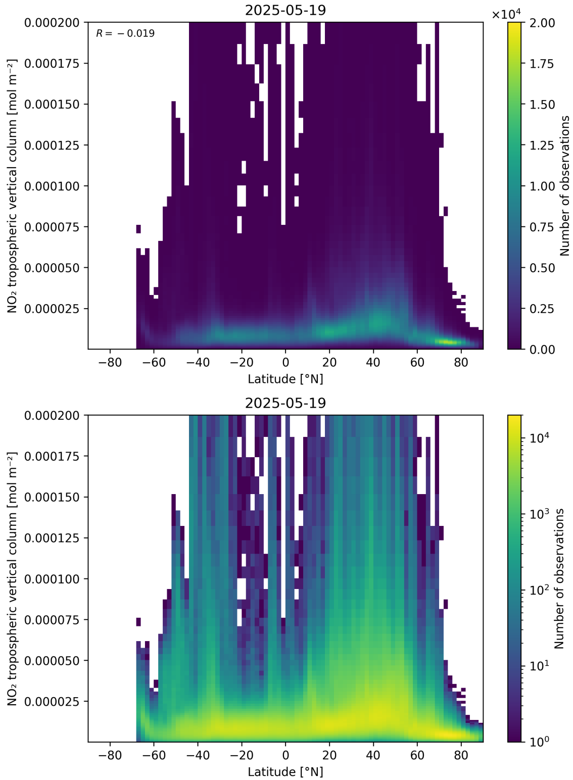
Figure 92: Scatter density plot of “Latitude” against “NO 2 tropospheric vertical column” for 2025-05-18 to 2025-05-20.
