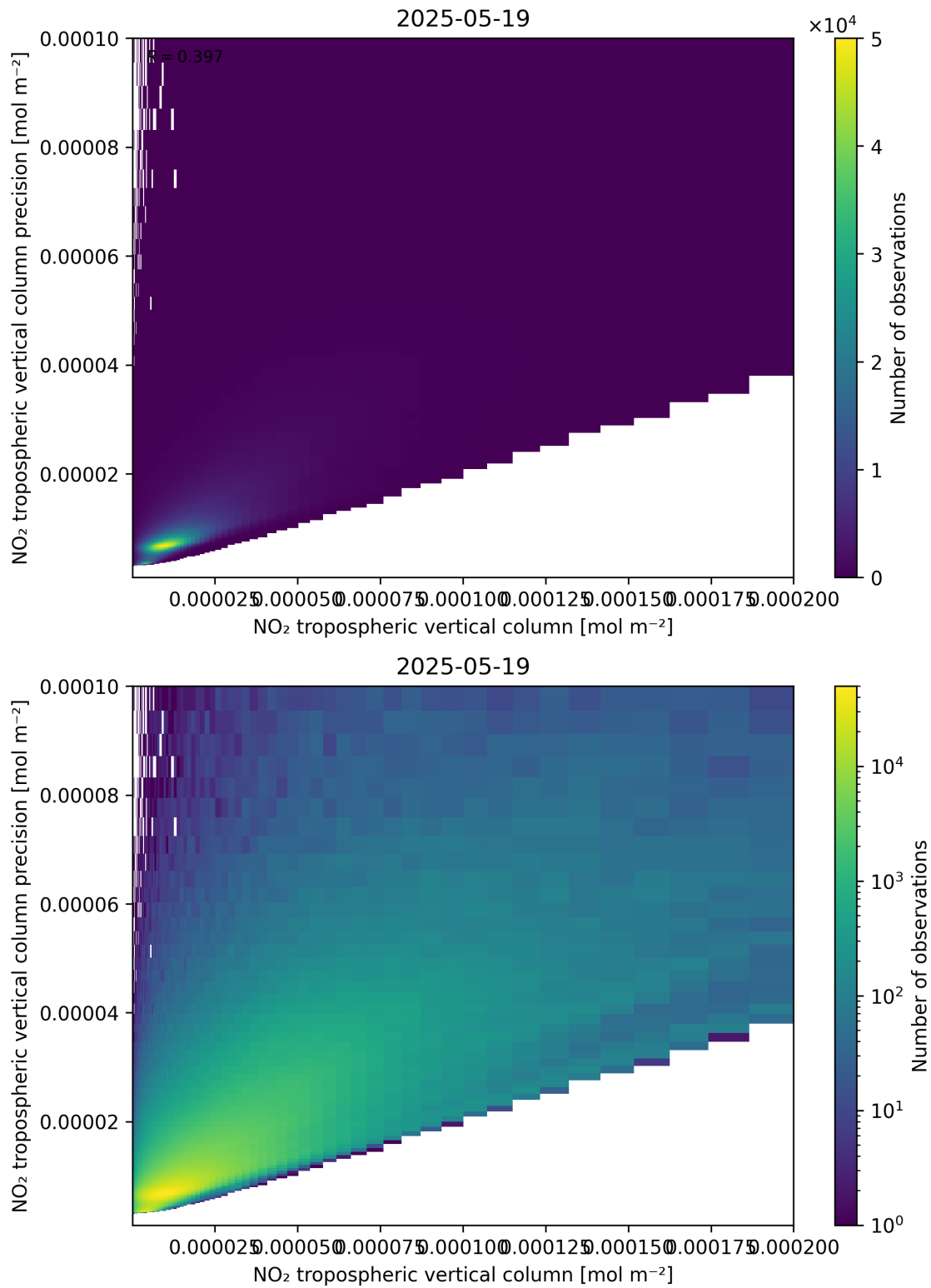
Figure 130: Scatter density plot of “NO 2 tropospheric vertical column” against “NO 2 tropospheric vertical column precision” for 2025-05-18 to 2025-05-20.
