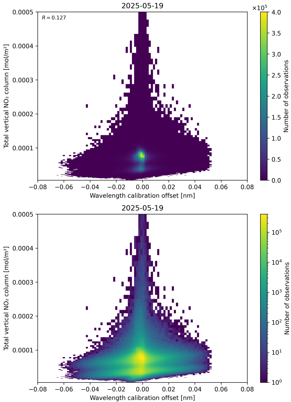
Figure 179: Scatter density plot of “Wavelength calibration offset” against “Total vertical NO 2 column” for 2025-05-18 to 2025-05-20.
