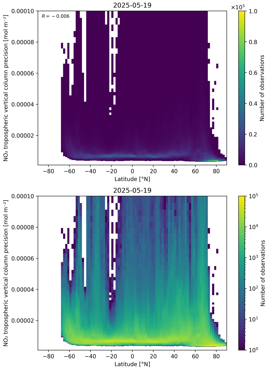
Figure 93: Scatter density plot of “Latitude” against “NO 2 tropospheric vertical column precision” for 2025-05-18 to 2025-05-20.
