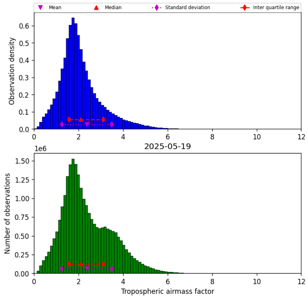
Figure 31: Histogram of “Tropospheric airmass factor” for 2025-05-18 to 2025-05-20
