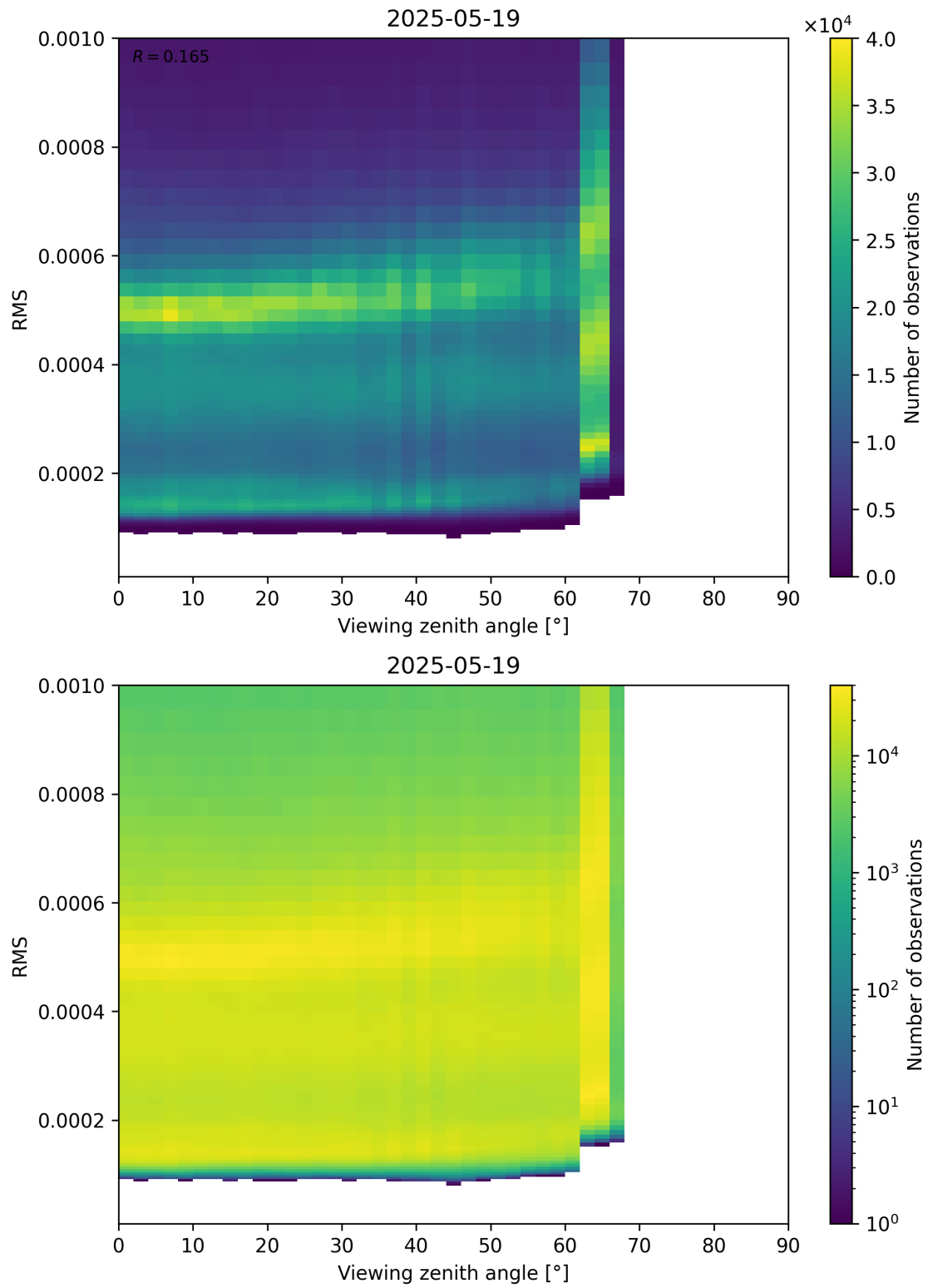
Figure 171: Scatter density plot of “Viewing zenith angle” against “RMS” for 2025-05-18 to 2025-05-20.
