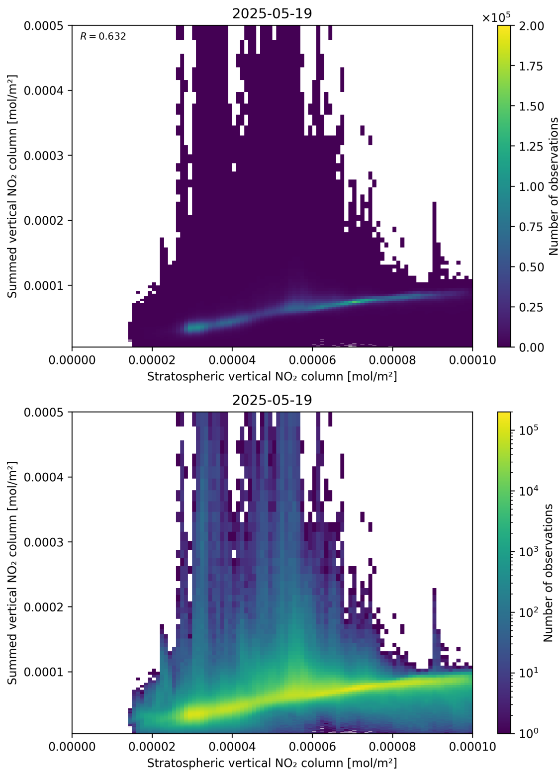
Figure 98: Scatter density plot of “Stratospheric vertical NO 2 column” against “Summed vertical NO 2 column” for 2025-05-18 to 2025-05-20.
