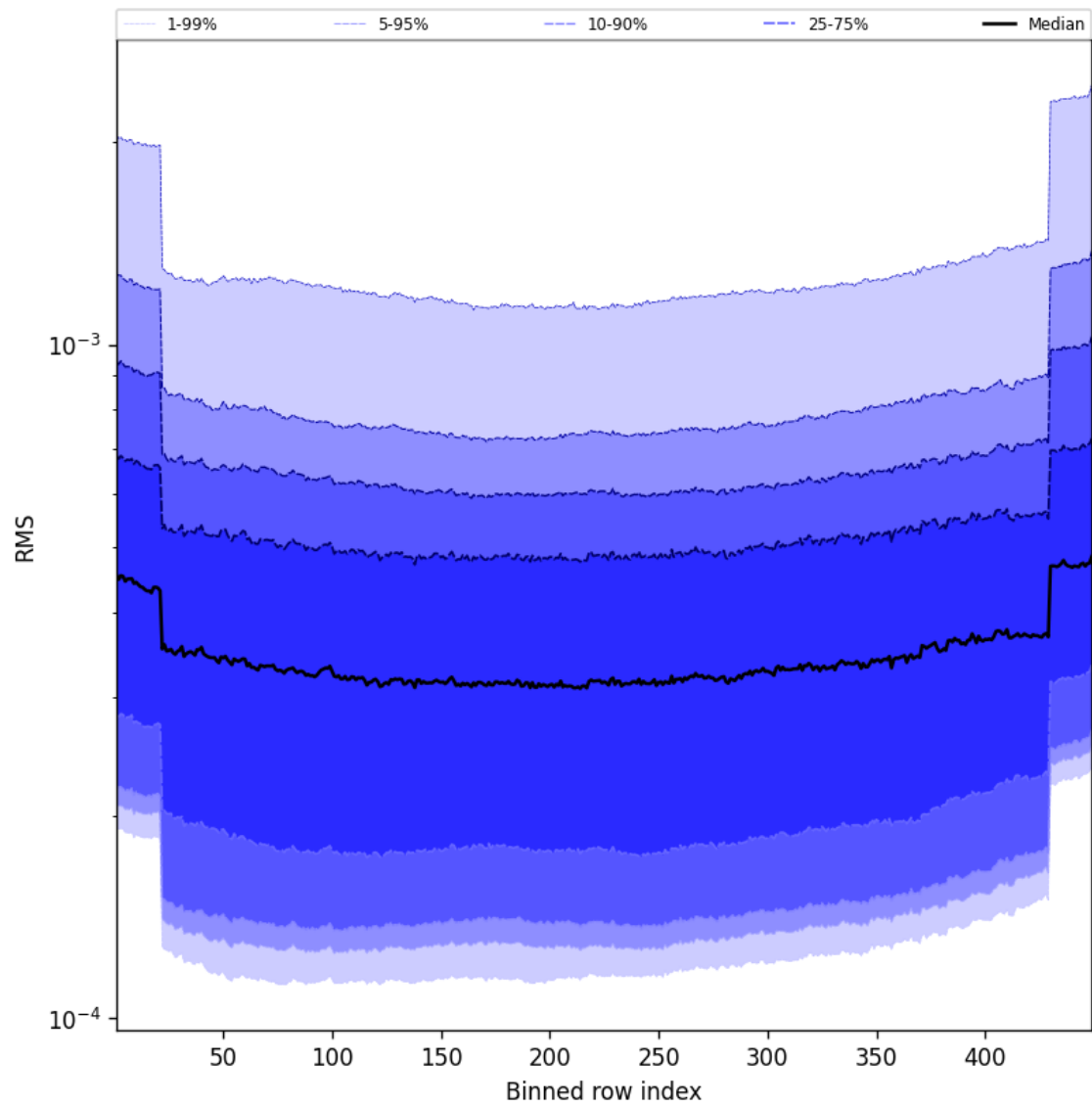
Figure 60: Along track statistics of “RMS” for 2025-05-18 to 2025-05-20
