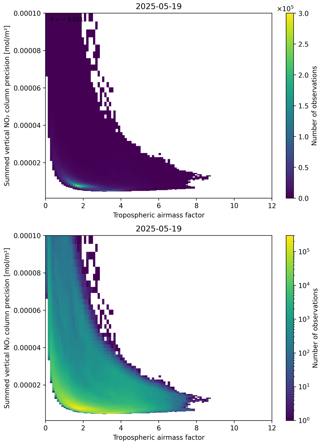
Figure 76: Scatter density plot of “Tropospheric air mass factor” against “Summed vertical NO 2 column precision” for 2025-05-18 to 2025-05-20.
