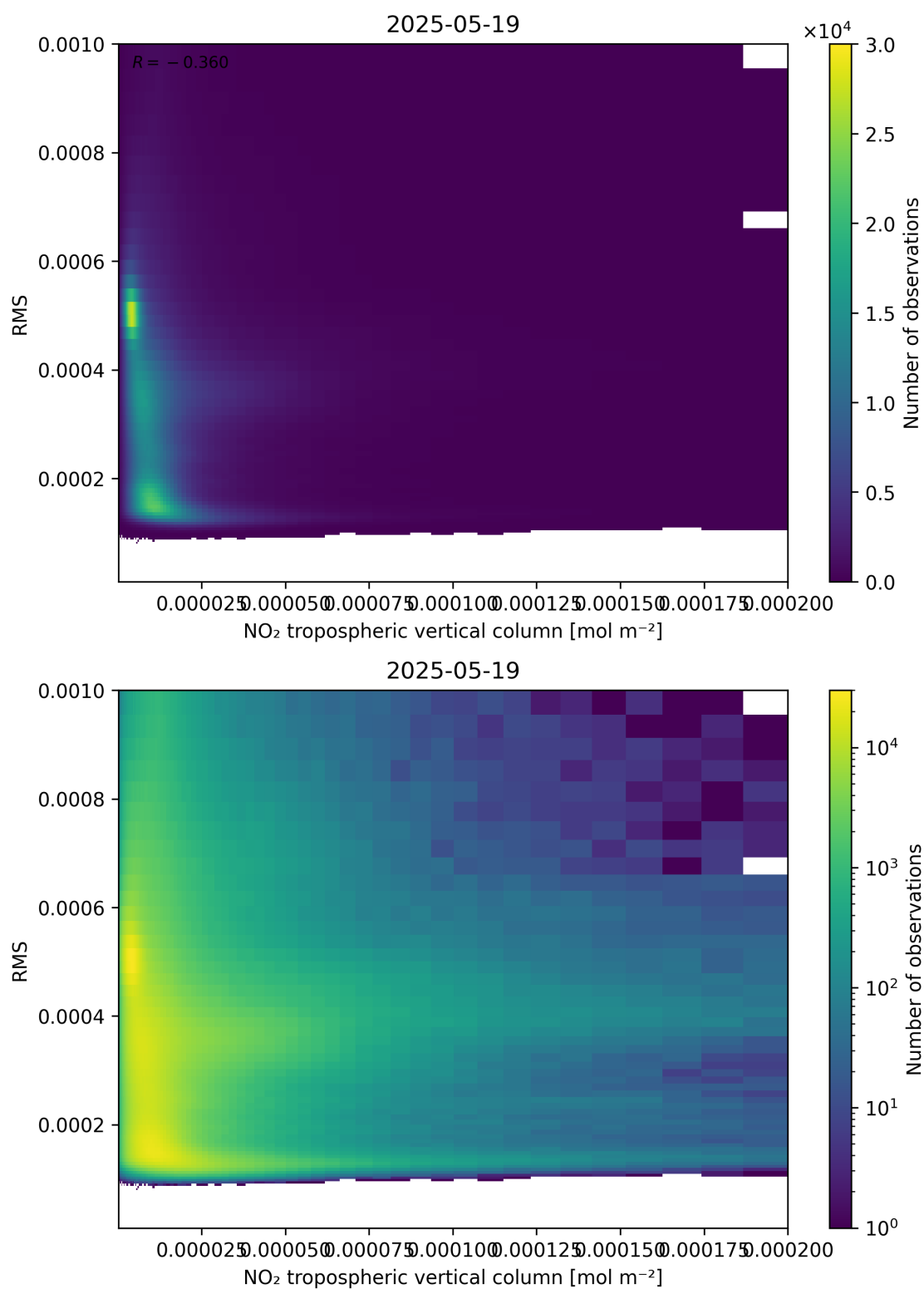
Figure 142: Scatter density plot of “NO 2 tropospheric vertical column” against “RMS” for 2025-05-18 to 2025-05-20.
