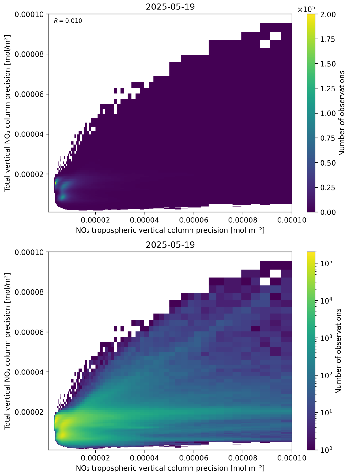
Figure 139: Scatter density plot of “NO 2 tropospheric vertical column precision” against “Total vertical NO 2 column precision” for 2025-05-18 to 2025-05-20.
