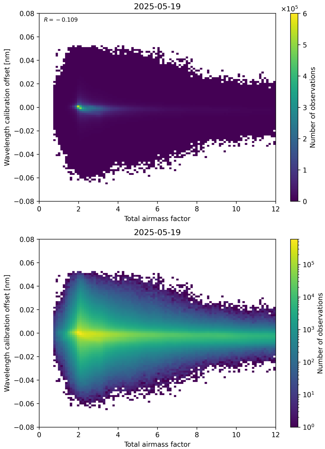
Figure 70: Scatter density plot of “Total airmass factor” against “Wavelength calibration offset” for 2025-05-18 to 2025-05-20.
