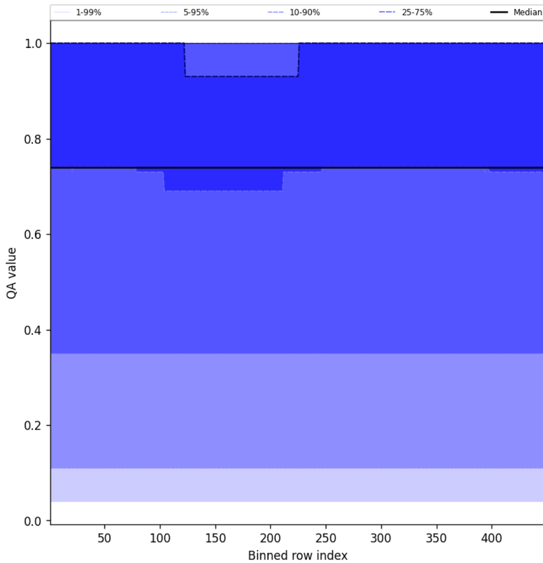
Figure 45: Along track statistics of “QA value” for 2025-05-18 to 2025-05-20
