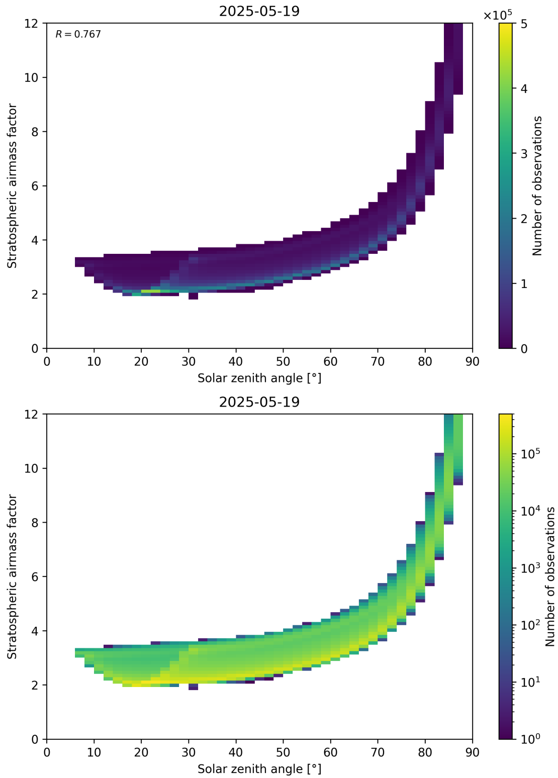
Figure 145: Scatter density plot of “Solar zenith angle” against “Stratospheric airmass factor” for 2025-05-18 to 2025-05-20.
