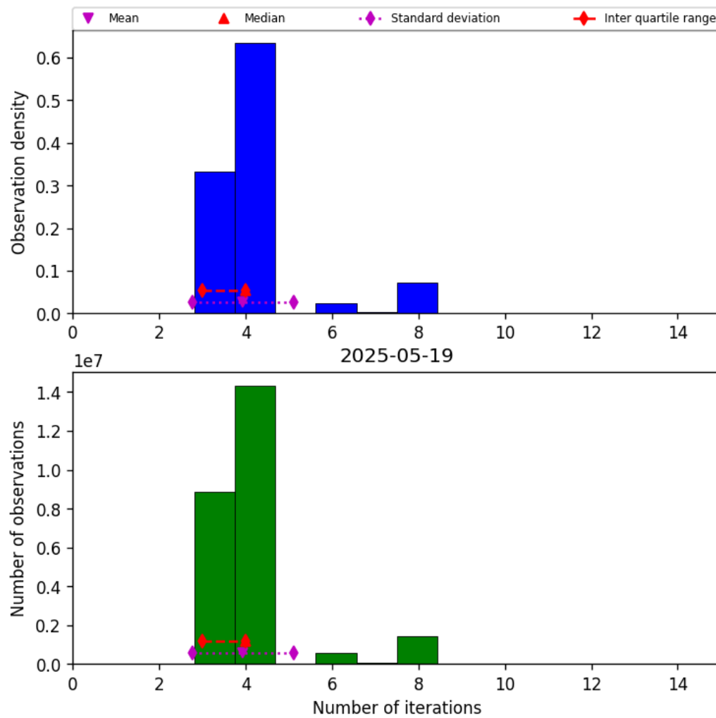
Figure 34: Histogram of “Number of iterations” for 2025-05-18 to 2025-05-20
