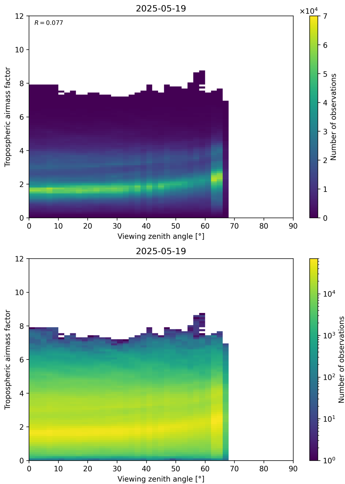
Figure 161: Scatter density plot of “Viewing zenith angle” against “Tropospheric airmass factor” for 2025-05-18 to 2025-05-20.
