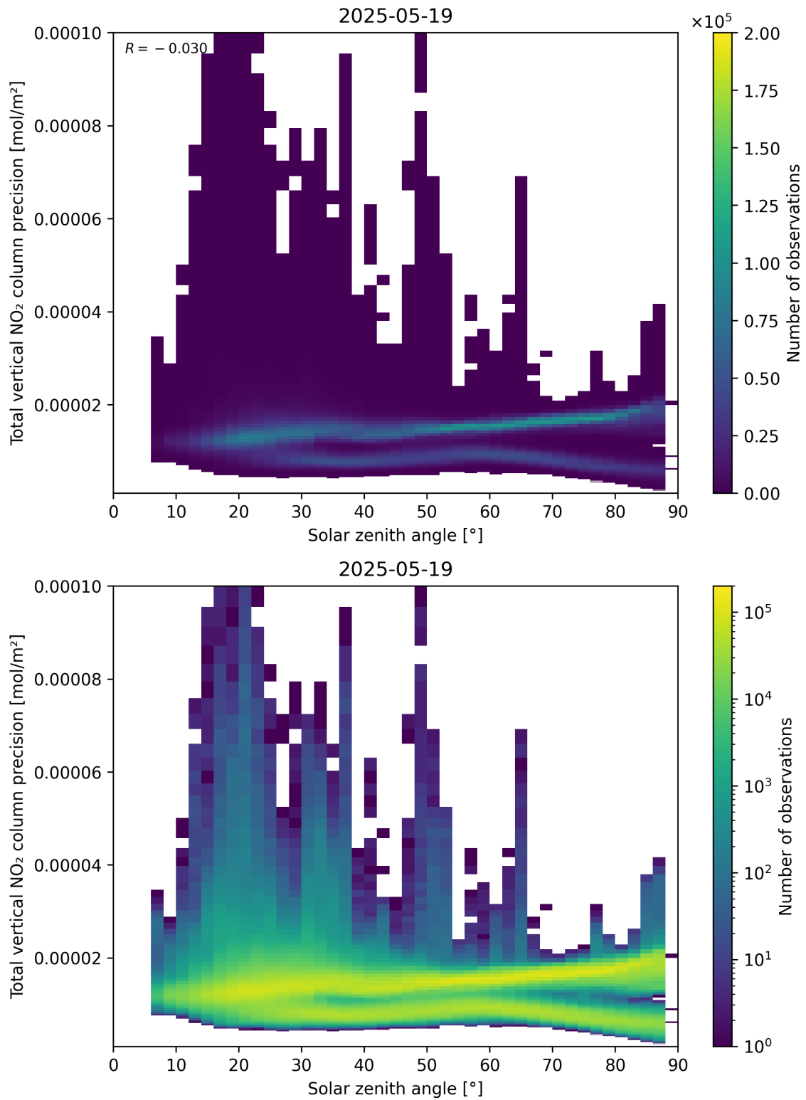
Figure 154: Scatter density plot of “Solar zenith angle” against “Total vertical NO 2 column precision” for 2025-05-18 to 2025-05-20.
