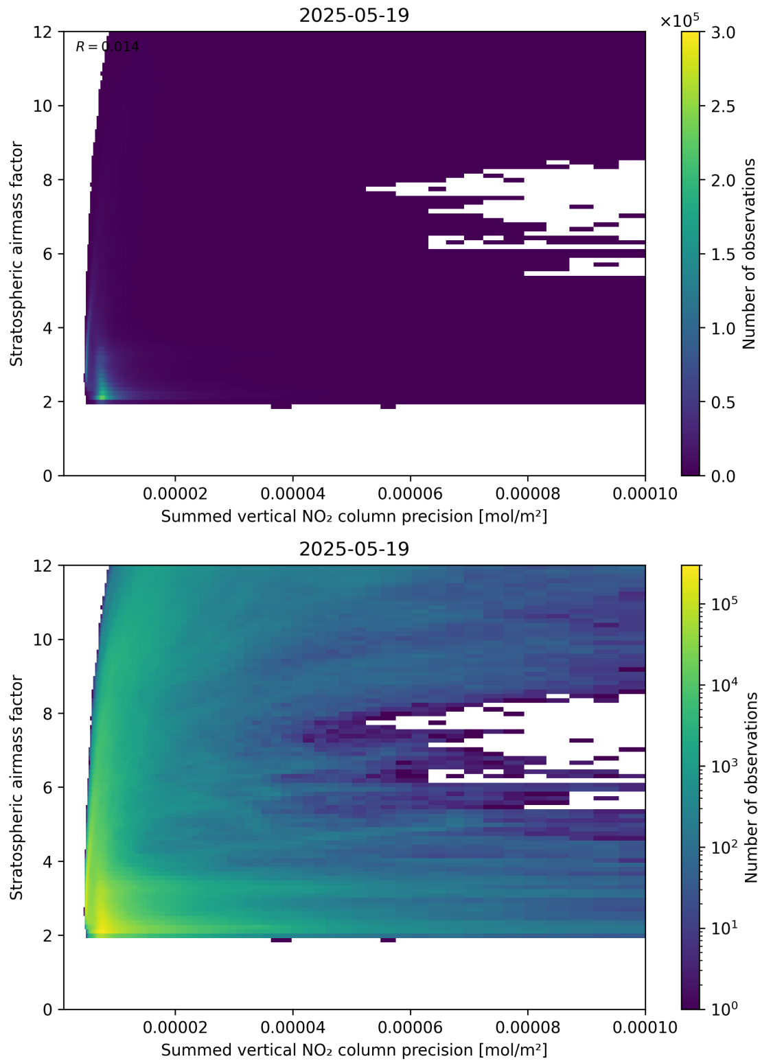
Figure 106: Scatter density plot of “Summed vertical NO 2 column precision” against “Stratospheric airmass factor” for 2025-05-18 to 2025-05-20.
