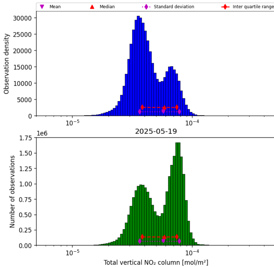
Figure 38: Histogram of “Total vertical NO 2 column” for 2025-05-18 to 2025-05-20
