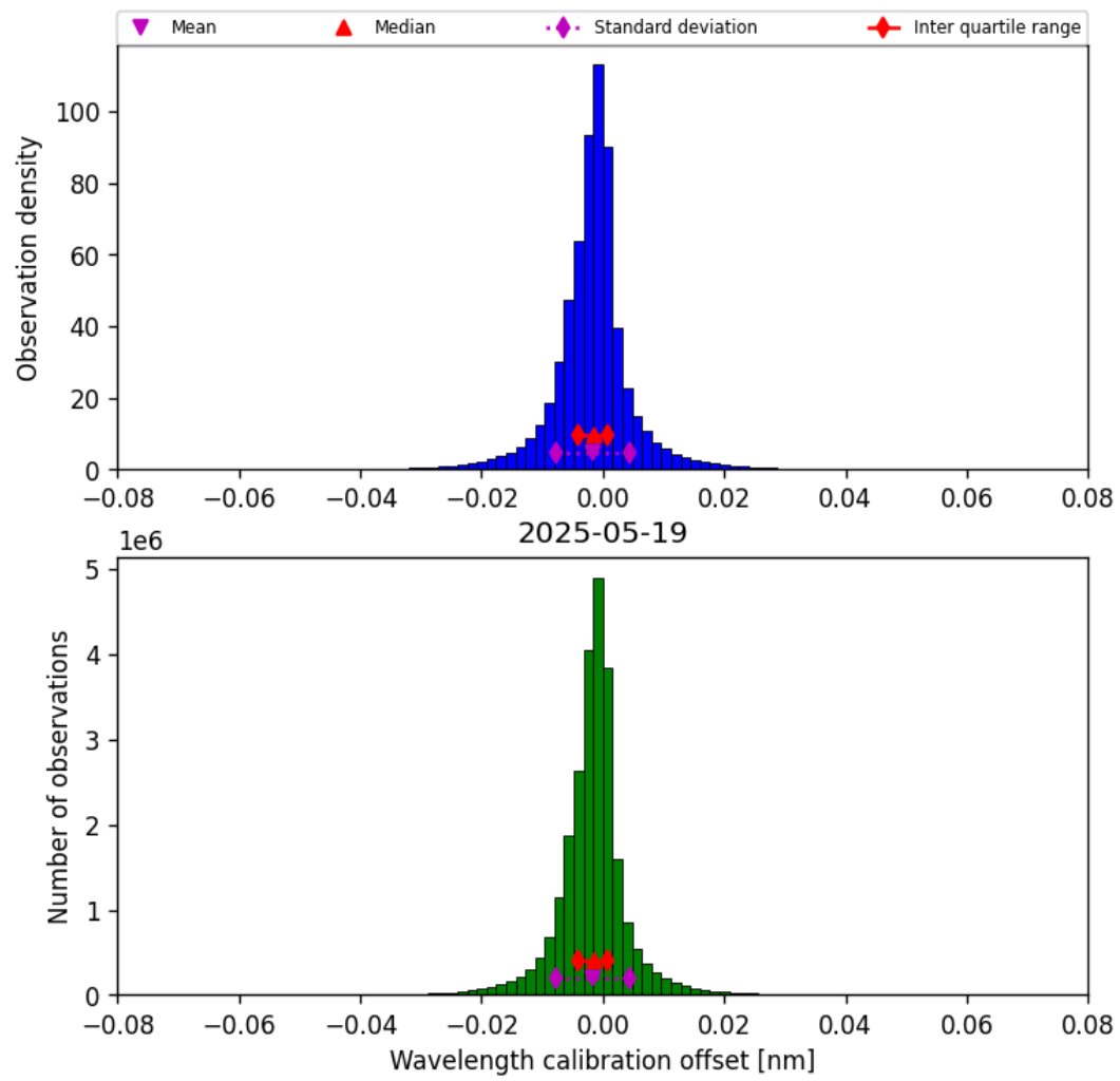
Figure 35: Histogram of “Wavelength calibration offset” for 2025-05-18 to 2025-05-20
