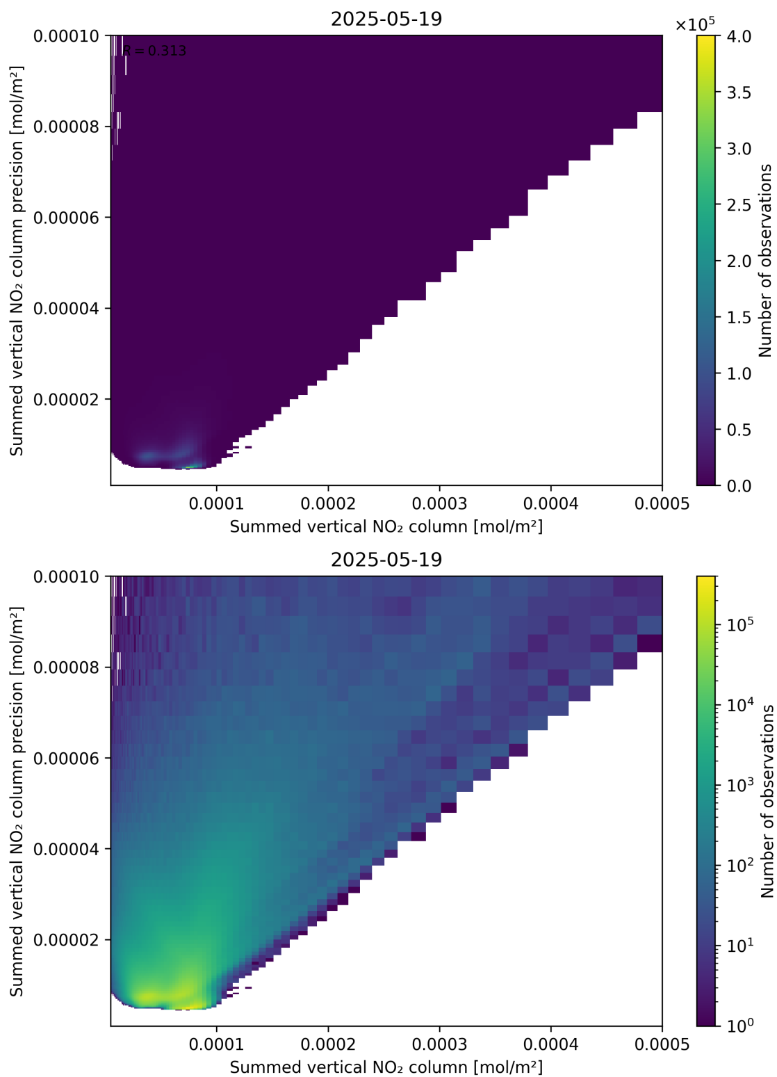
Figure 105: Scatter density plot of “Summed vertical NO 2 column” against “Summed vertical NO 2 column precision” for 2025-05-18 to 2025-05-20.
