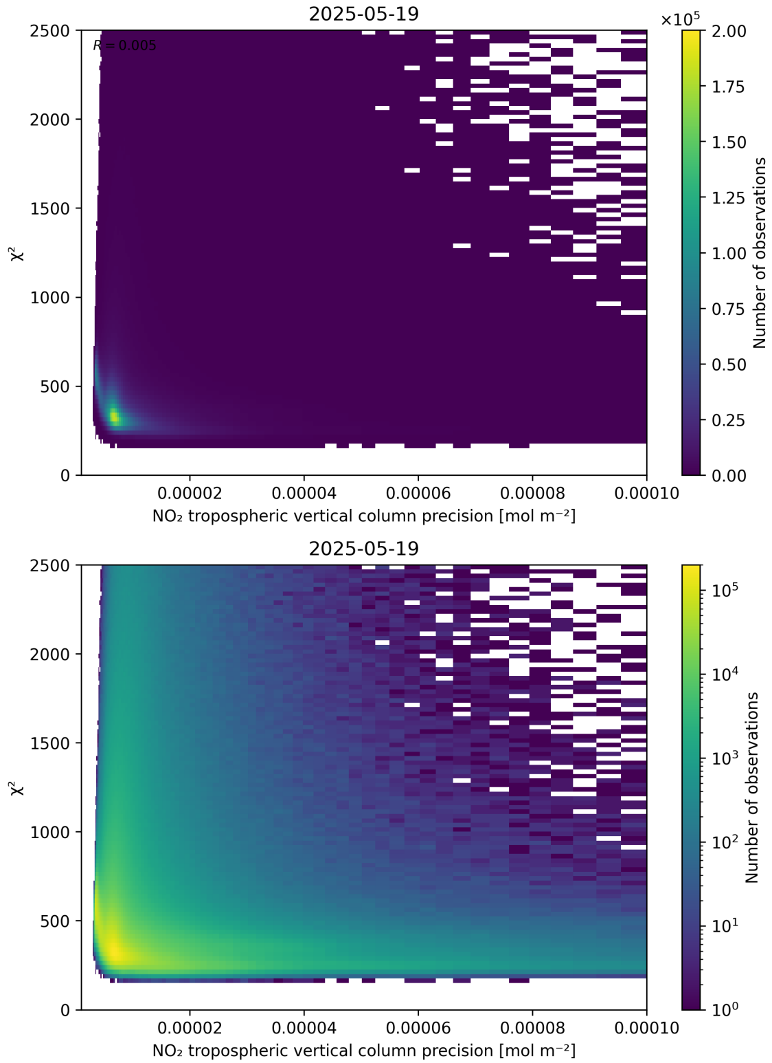
Figure 134: Scatter density plot of “NO 2 tropospheric vertical column precision” against “ \chi^2 ” for 2025-05-18 to 2025-05-20.
