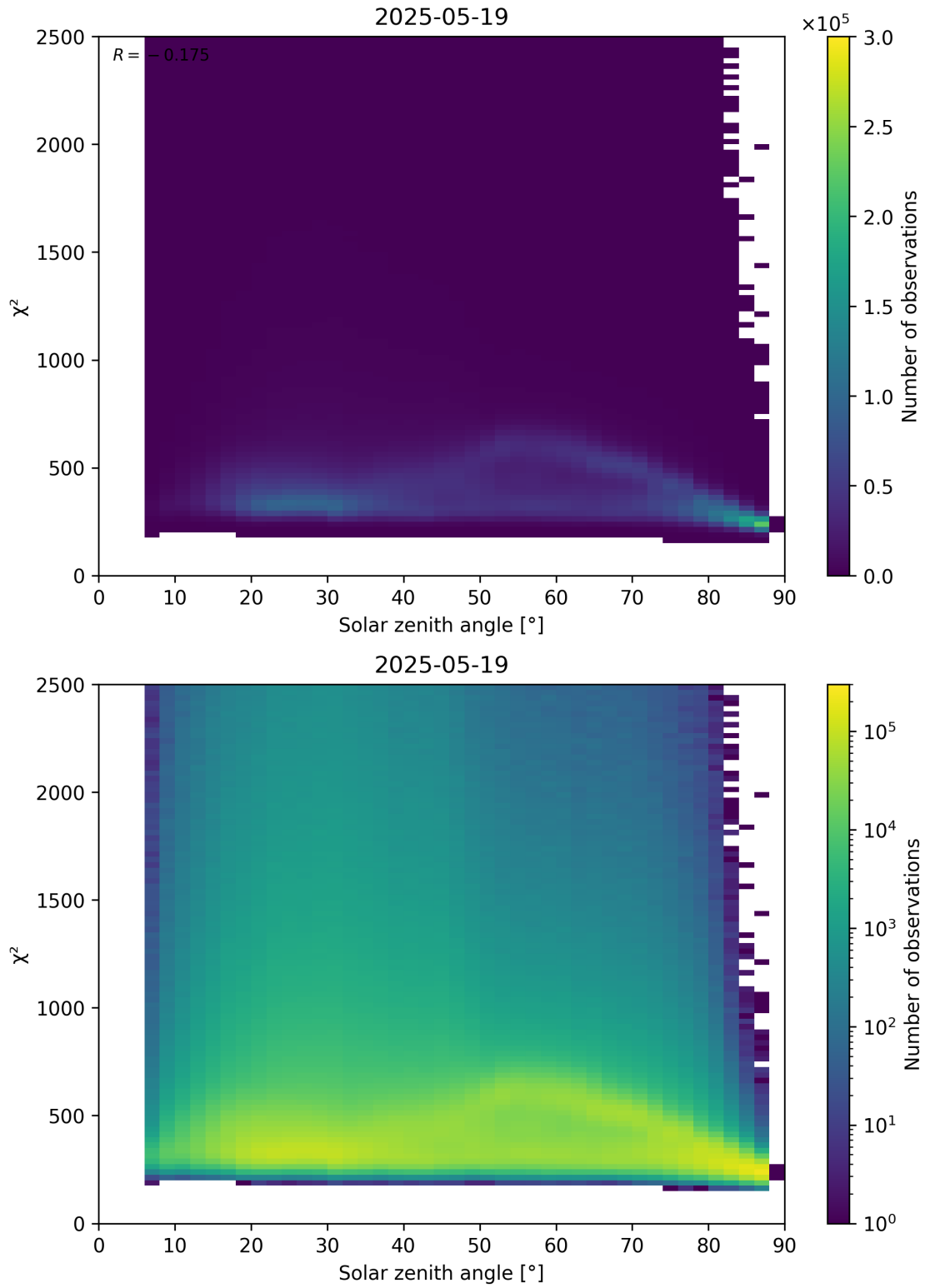
Figure 148: Scatter density plot of “Solar zenith angle” against “ \chi^2 ” for 2025-05-18 to 2025-05-20.
