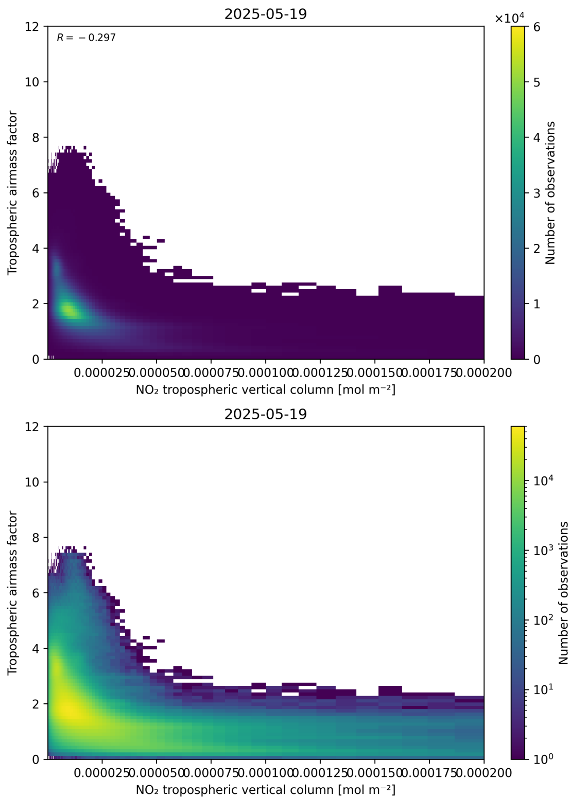
Figure 123: Scatter density plot of “NO 2 tropospheric vertical column” against “Tropospheric air mass factor” for 2025-05-18 to 2025-05-20.
