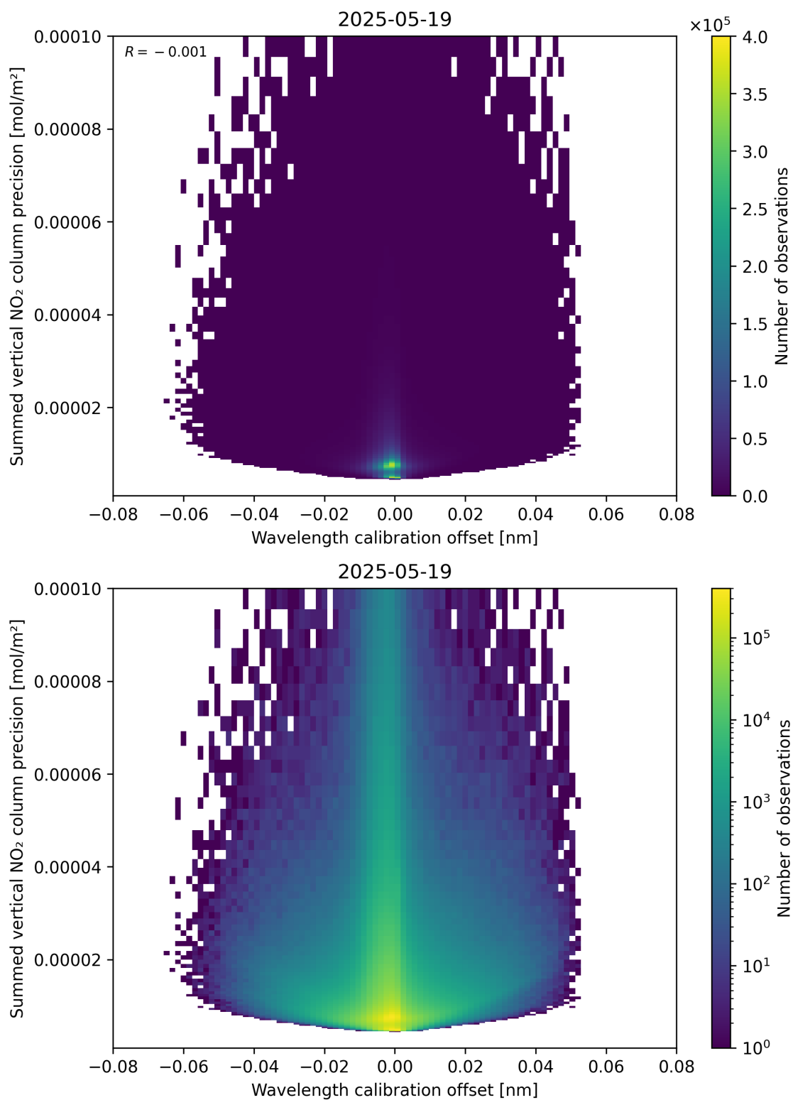
Figure 178: Scatter density plot of “Wavelength calibration offset” against “Summed vertical NO 2 column precision” for 2025-05-18 to 2025-05-20.
