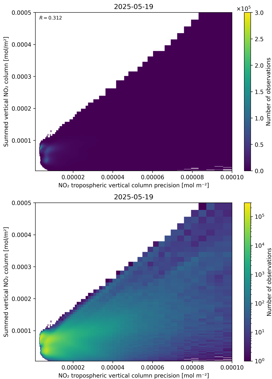
Figure 136: Scatter density plot of “NO 2 tropospheric vertical column precision” against “Summed vertical NO 2 column” for 2025-05-18 to 2025-05-20.
