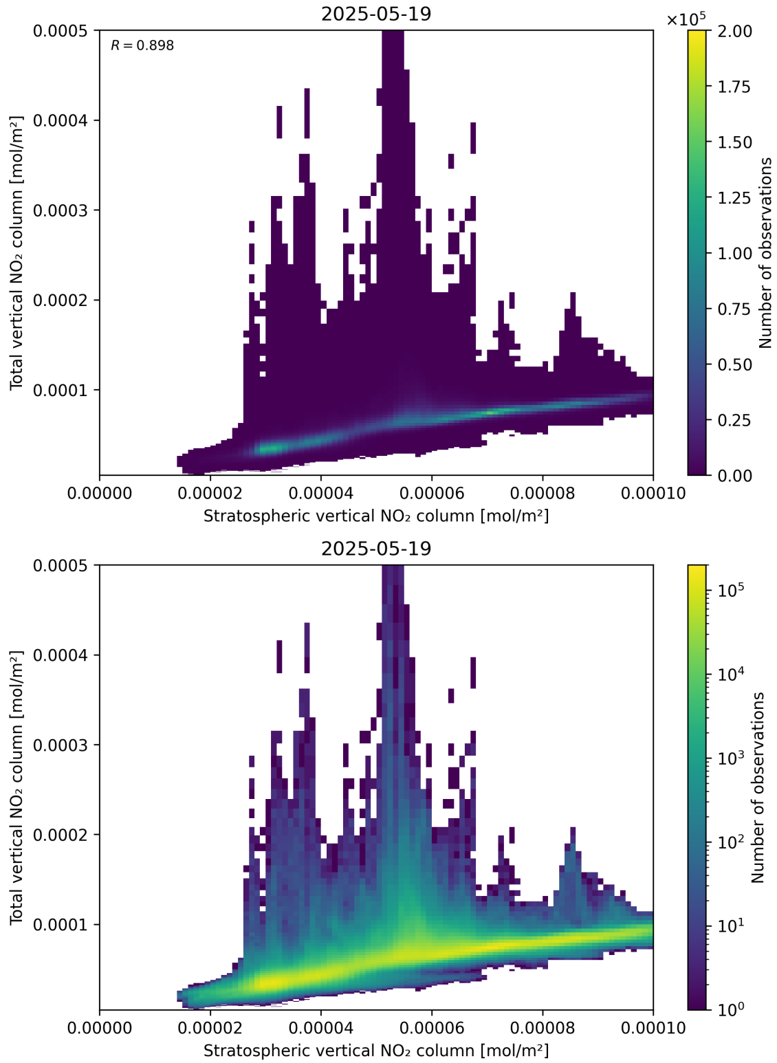
Figure 100: Scatter density plot of “Stratospheric vertical NO 2 column” against “Total vertical NO 2 column” for 2025-05-18 to 2025-05-20.
