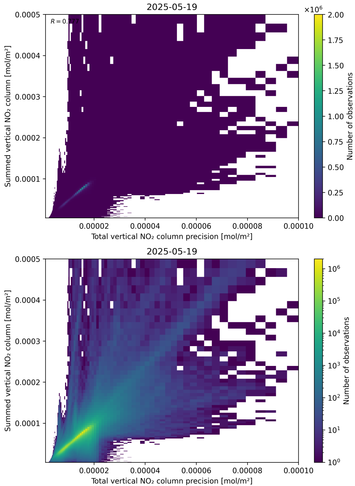
Figure 117: Scatter density plot of “Total vertical NO 2 column precision” against “Summed vertical NO 2 column” for 2025-05-18 to 2025-05-20.
