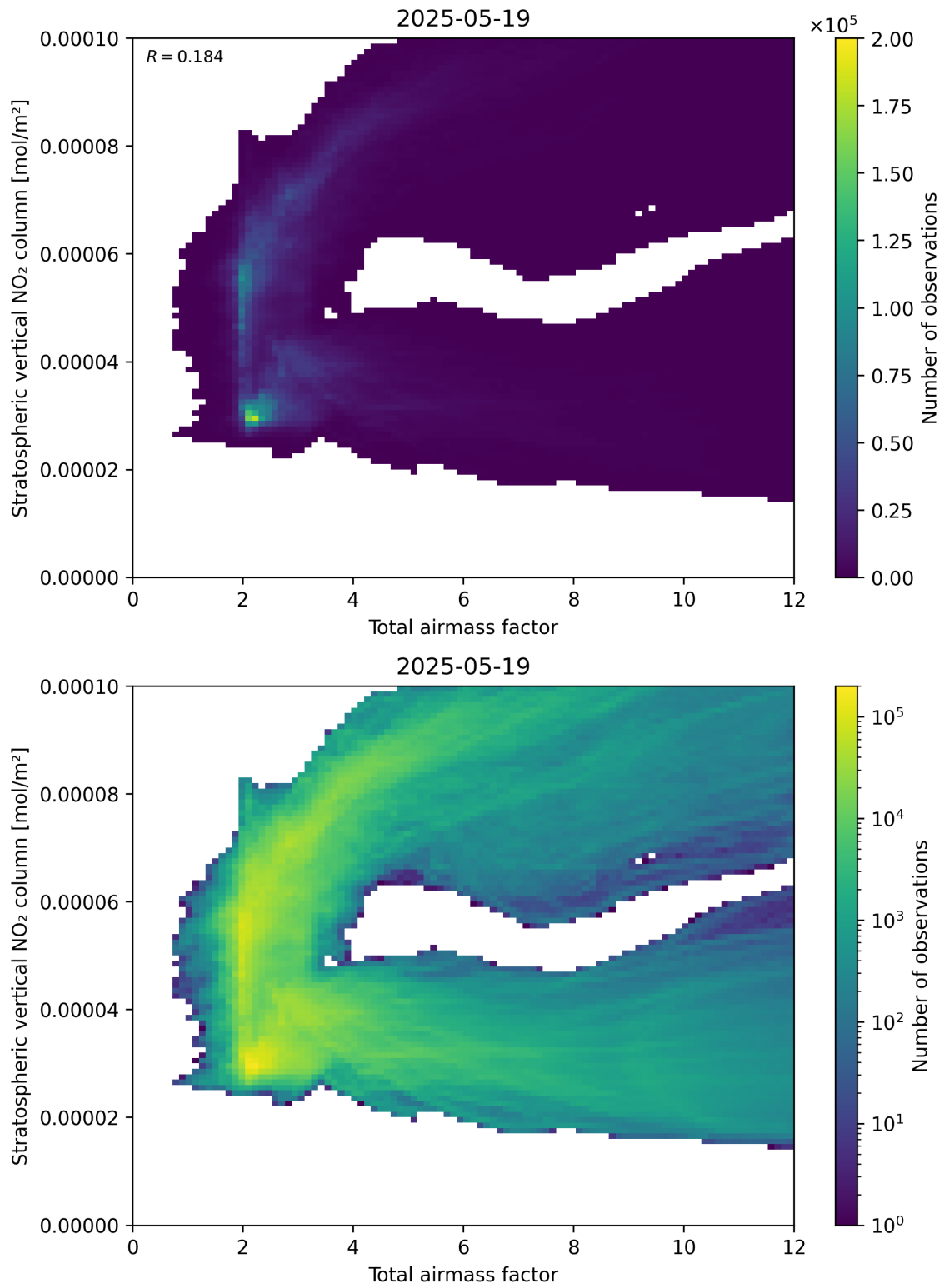
Figure 64: Scatter density plot of “Total airmass factor” against “Stratospheric vertical \text{NO}_2 column” for 2025-05-18 to 2025-05-20.
