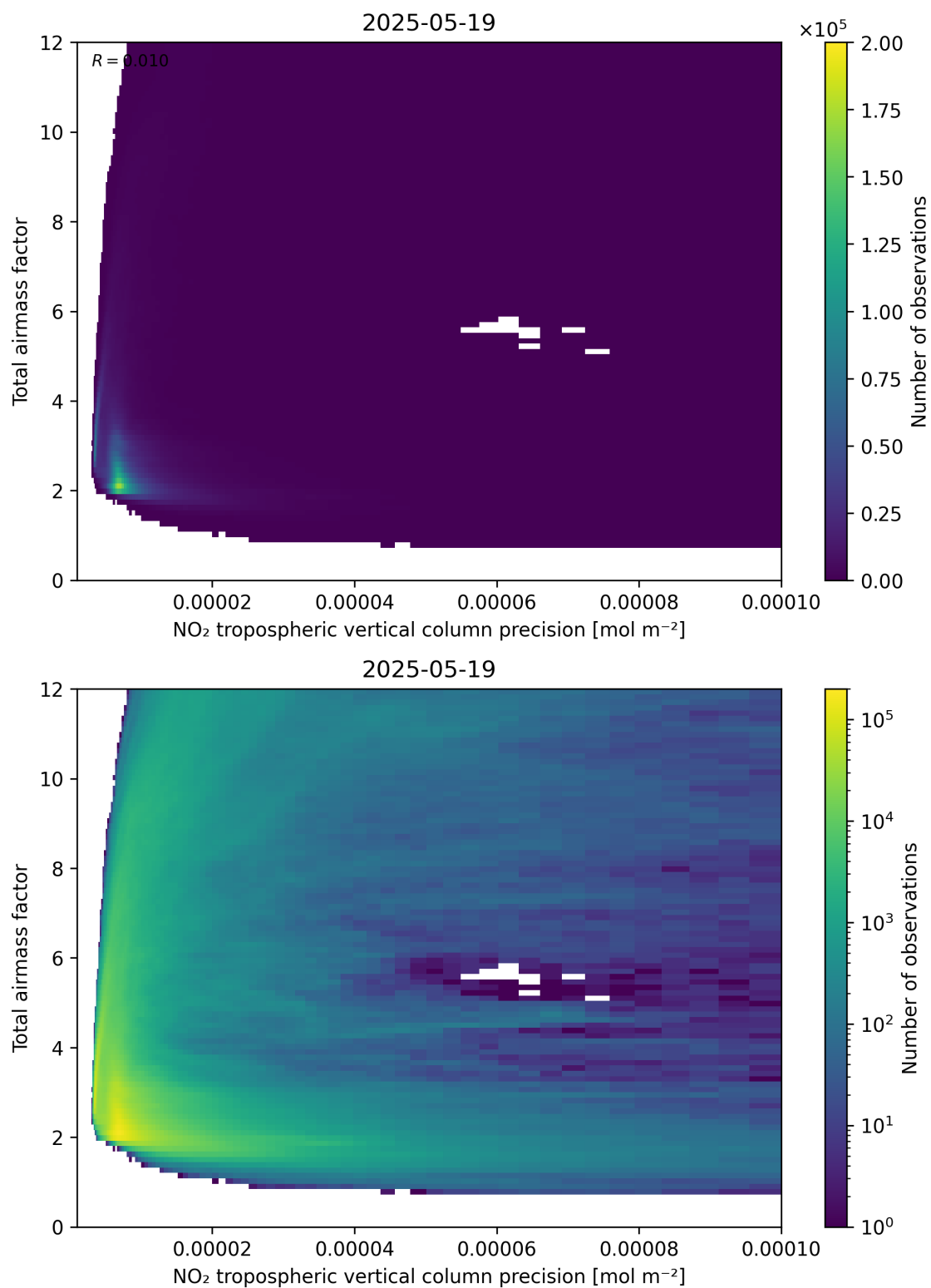
Figure 132: Scatter density plot of “NO 2 tropospheric vertical column precision” against “Total air mass factor” for 2025-05-18 to 2025-05-20.
