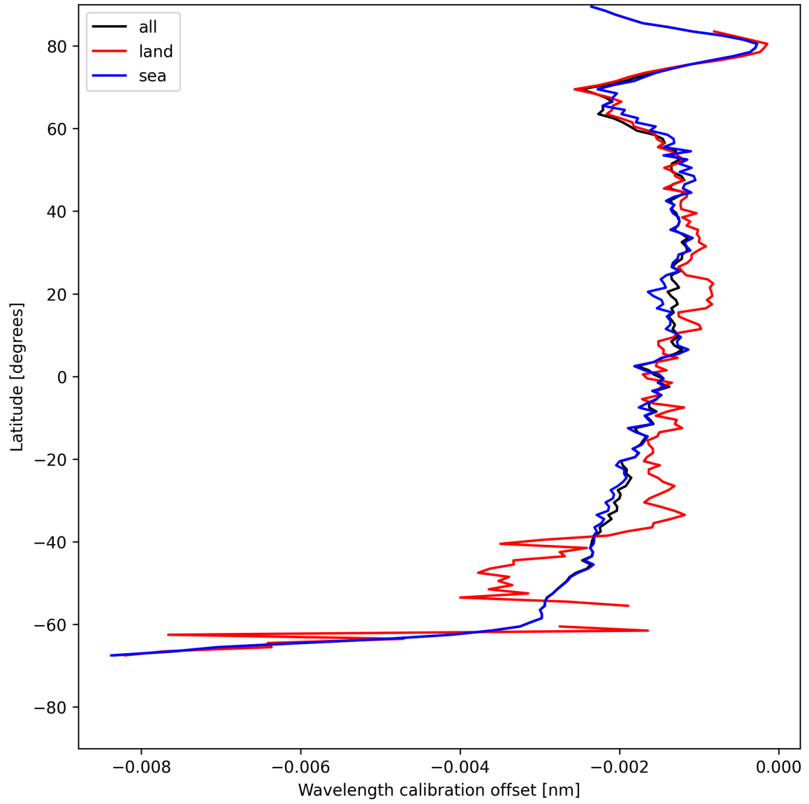
Figure 18: Zonal average of “Wavelength calibration offset” for 2025-05-18 to 2025-05-20.
