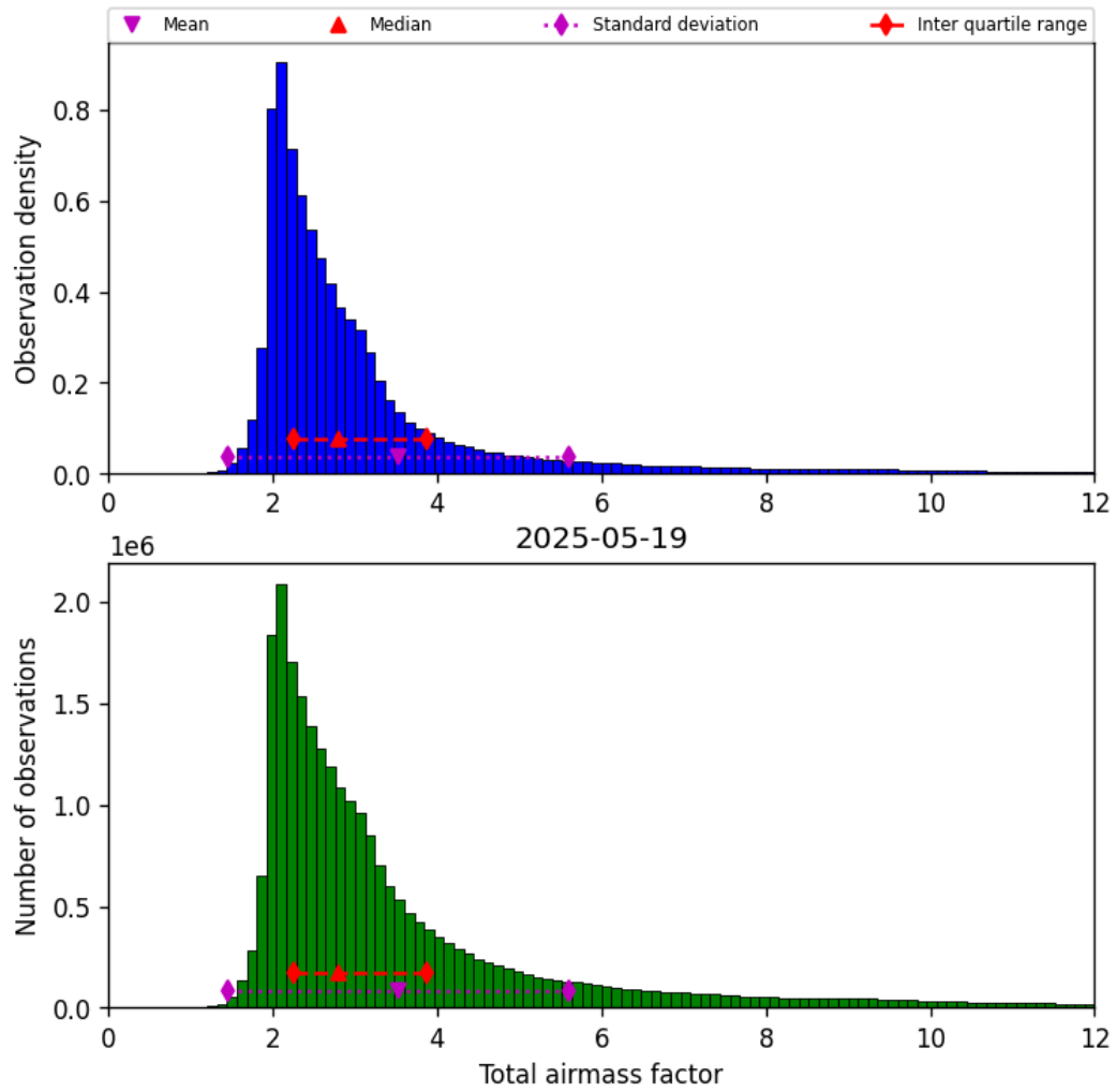
Figure 32: Histogram of “Total airmass factor” for 2025-05-18 to 2025-05-20
