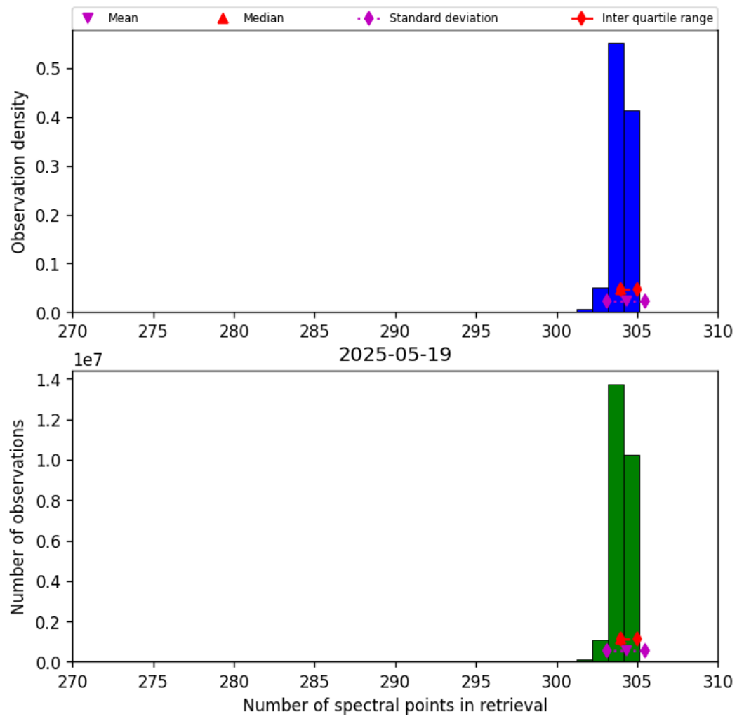
Figure 33: Histogram of “Number of spectral points in retrieval” for 2025-05-18 to 2025-05-20
