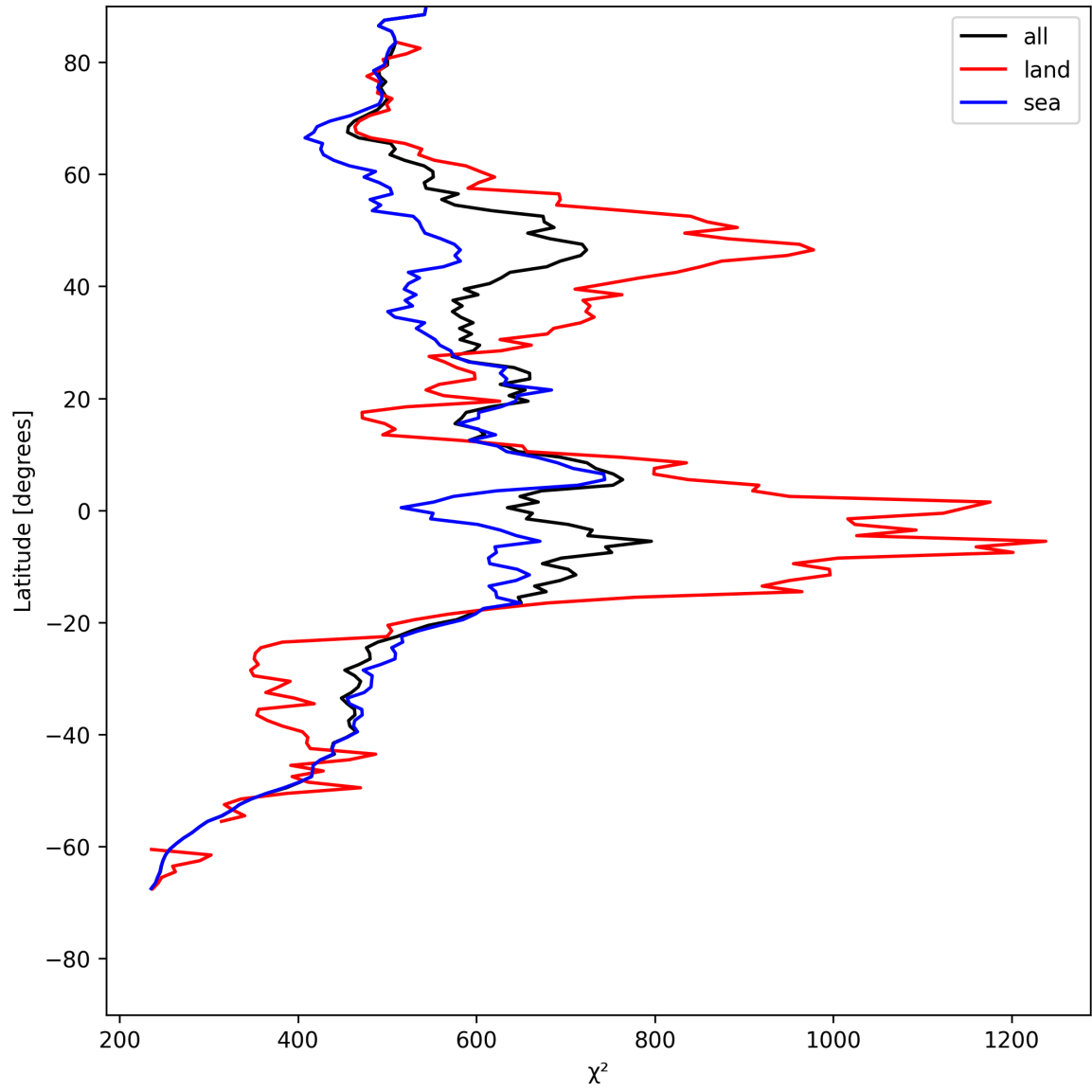
Figure 25: Zonal average of “ \chi^2 ” for 2025-05-18 to 2025-05-20.
