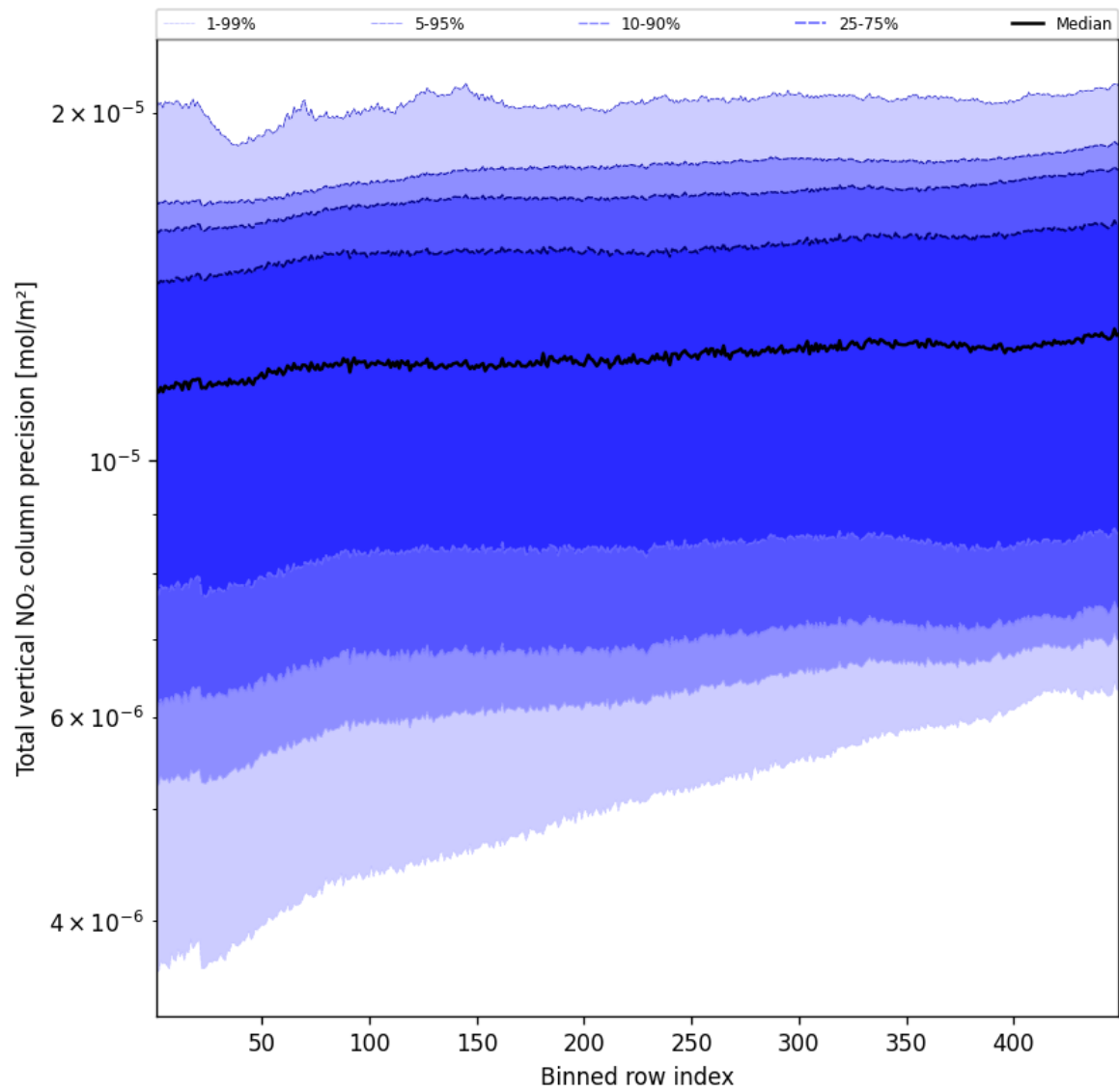
Figure 56: Along track statistics of “Total vertical NO 2 column precision” for 2025-05-18 to 2025-05-20
