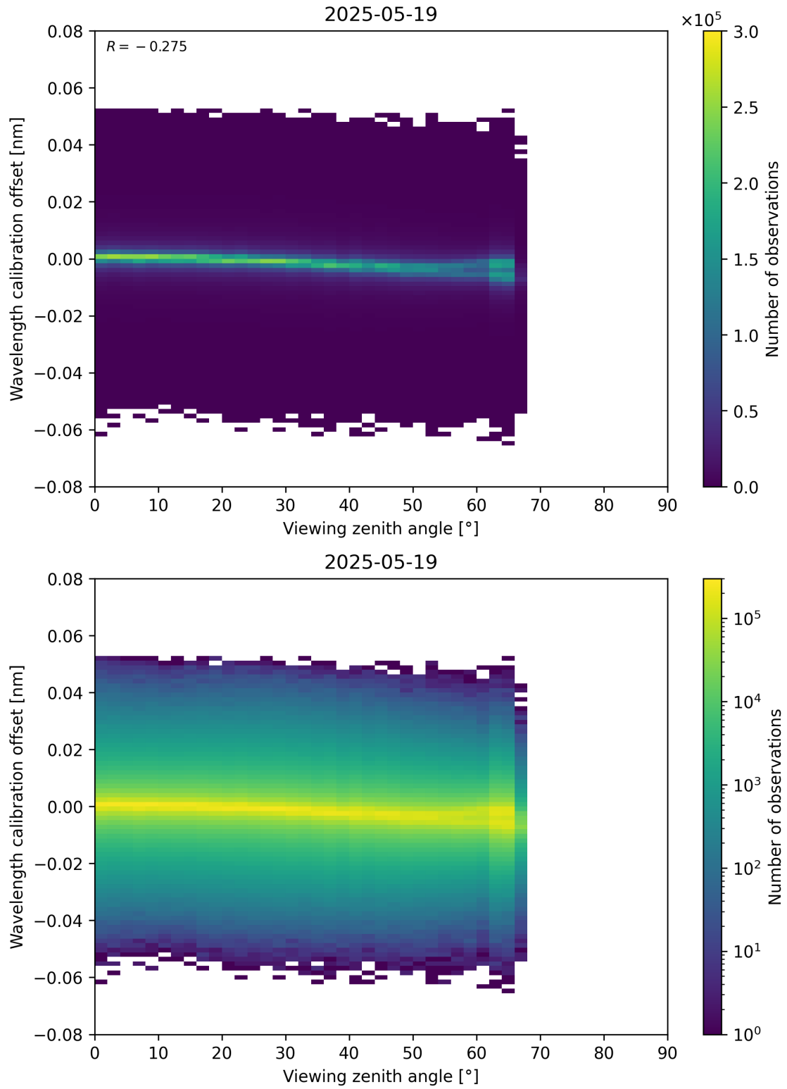
Figure 173: Scatter density plot of “Viewing zenith angle” against “Wavelength calibration offset” for 2025-05-18 to 2025-05-20.
