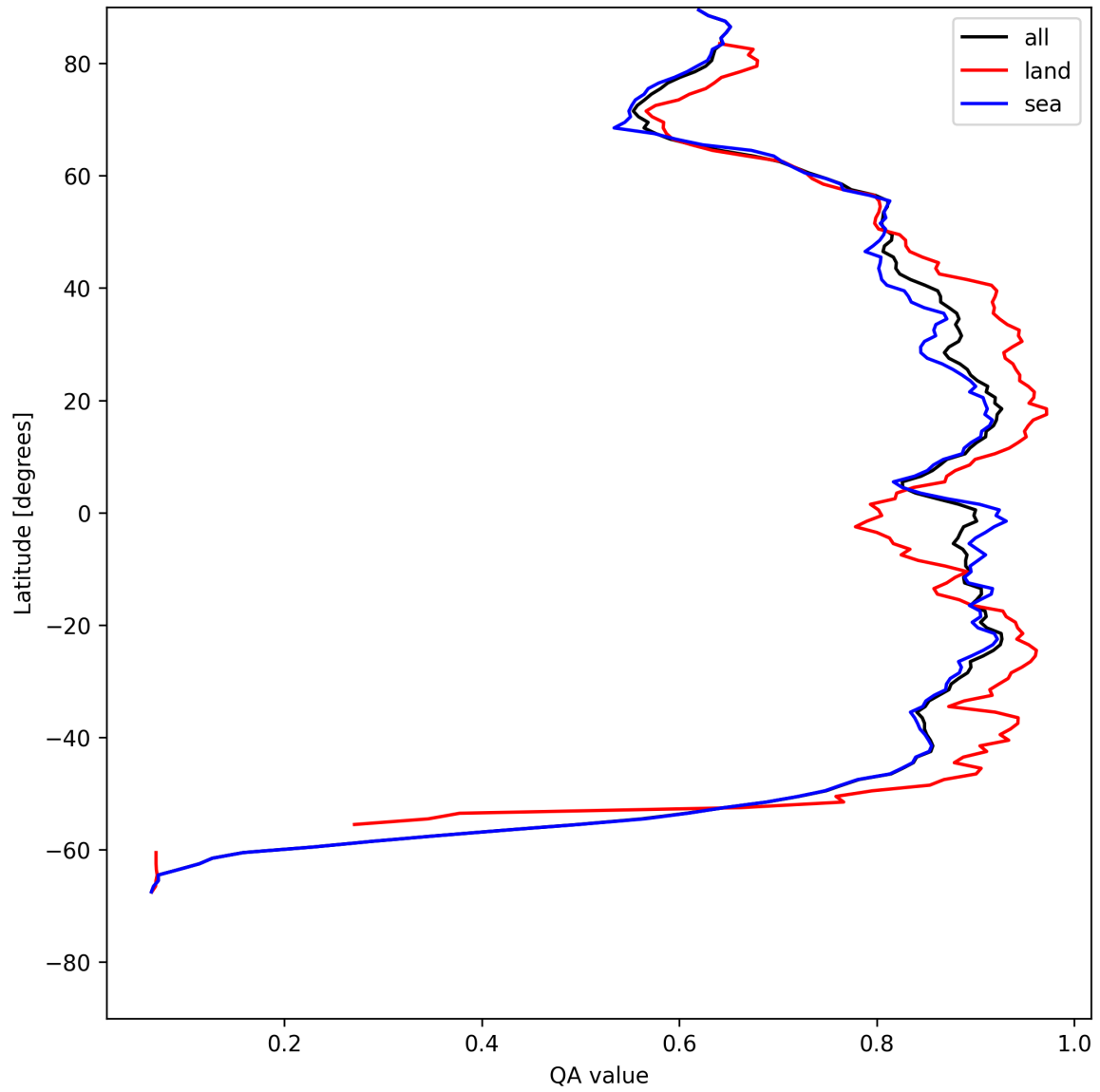
Figure 11: Zonal average of “QA value” for 2025-05-18 to 2025-05-20.
