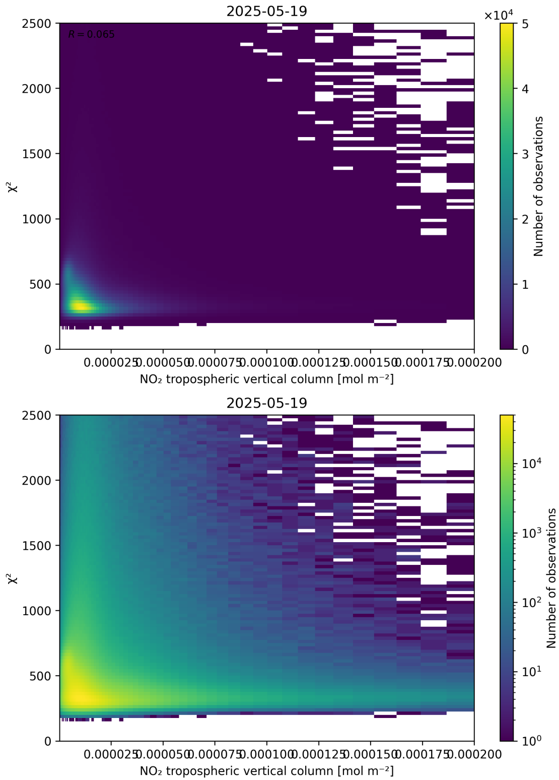
Figure 124: Scatter density plot of “NO 2 tropospheric vertical column” against “ \chi^2 ” for 2025-05-18 to 2025-05-20.
