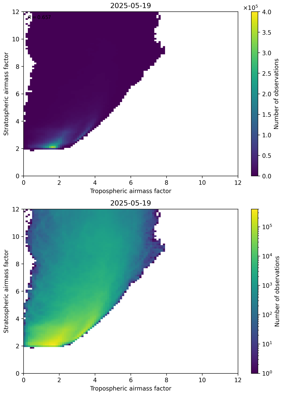
Figure 71: Scatter density plot of “Tropospheric airmass factor” against “Stratospheric airmass factor” for 2025-05-18 to 2025-05-20.
