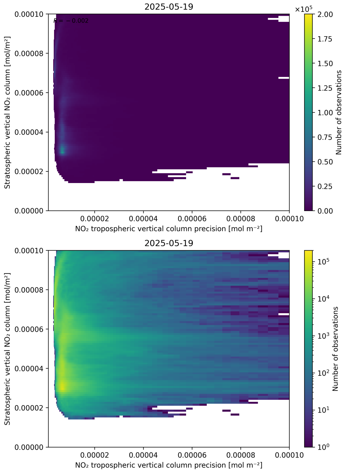
Figure 135: Scatter density plot of “NO 2 tropospheric vertical column precision” against “Stratospheric vertical NO 2 column” for 2025-05-18 to 2025-05-20.
