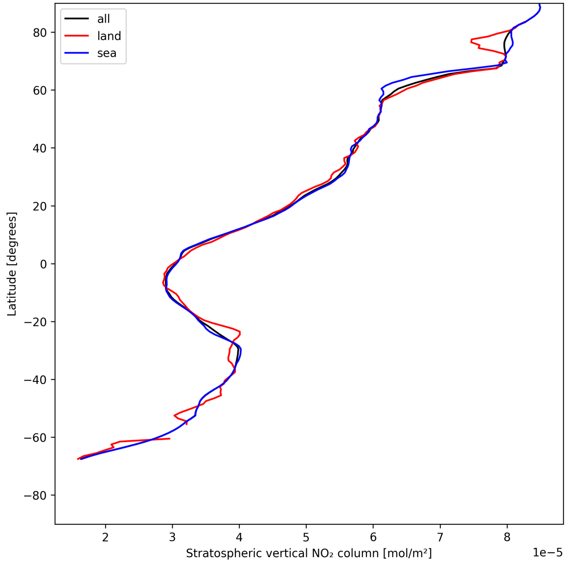
Figure 19: Zonal average of “Stratospheric vertical NO 2 column” for 2025-05-18 to 2025-05-20.
