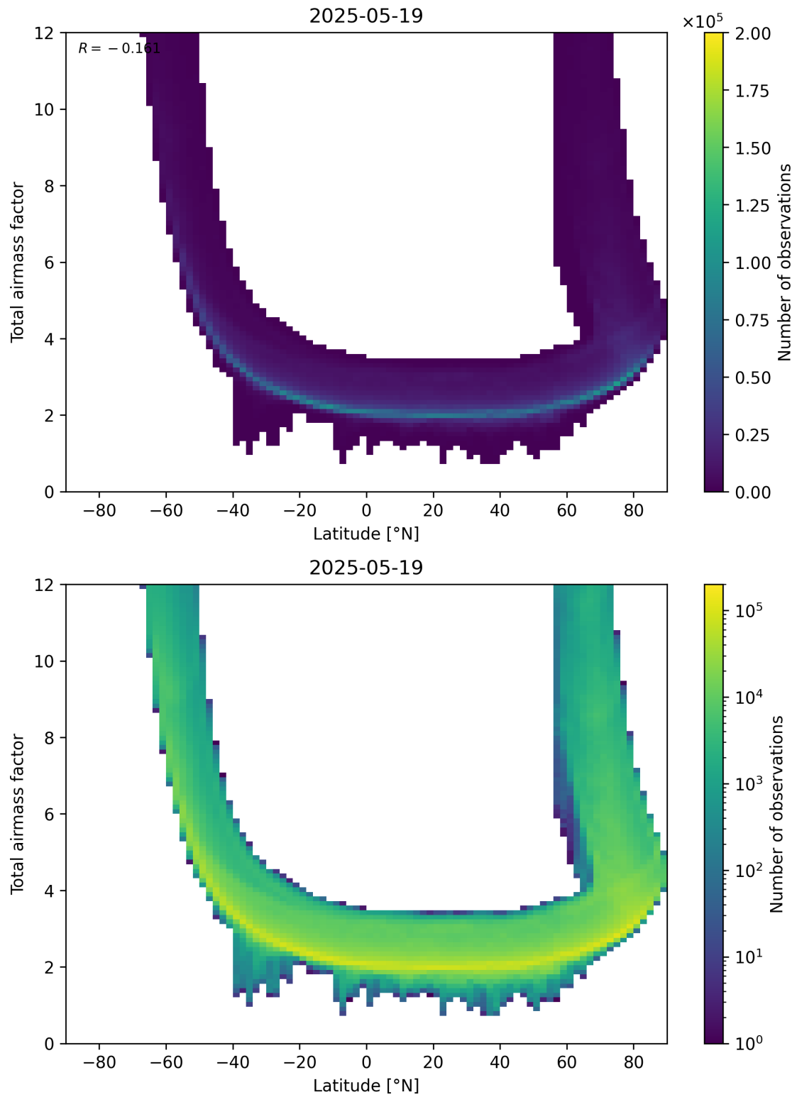
Figure 84: Scatter density plot of “Latitude” against “Total airmass factor” for 2025-05-18 to 2025-05-20.
