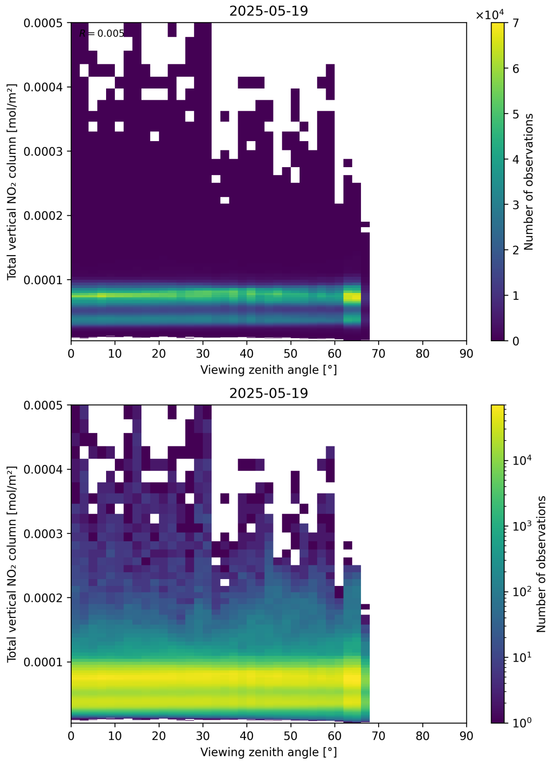
Figure 167: Scatter density plot of “Viewing zenith angle” against “Total vertical NO 2 column” for 2025-05-18 to 2025-05-20.
