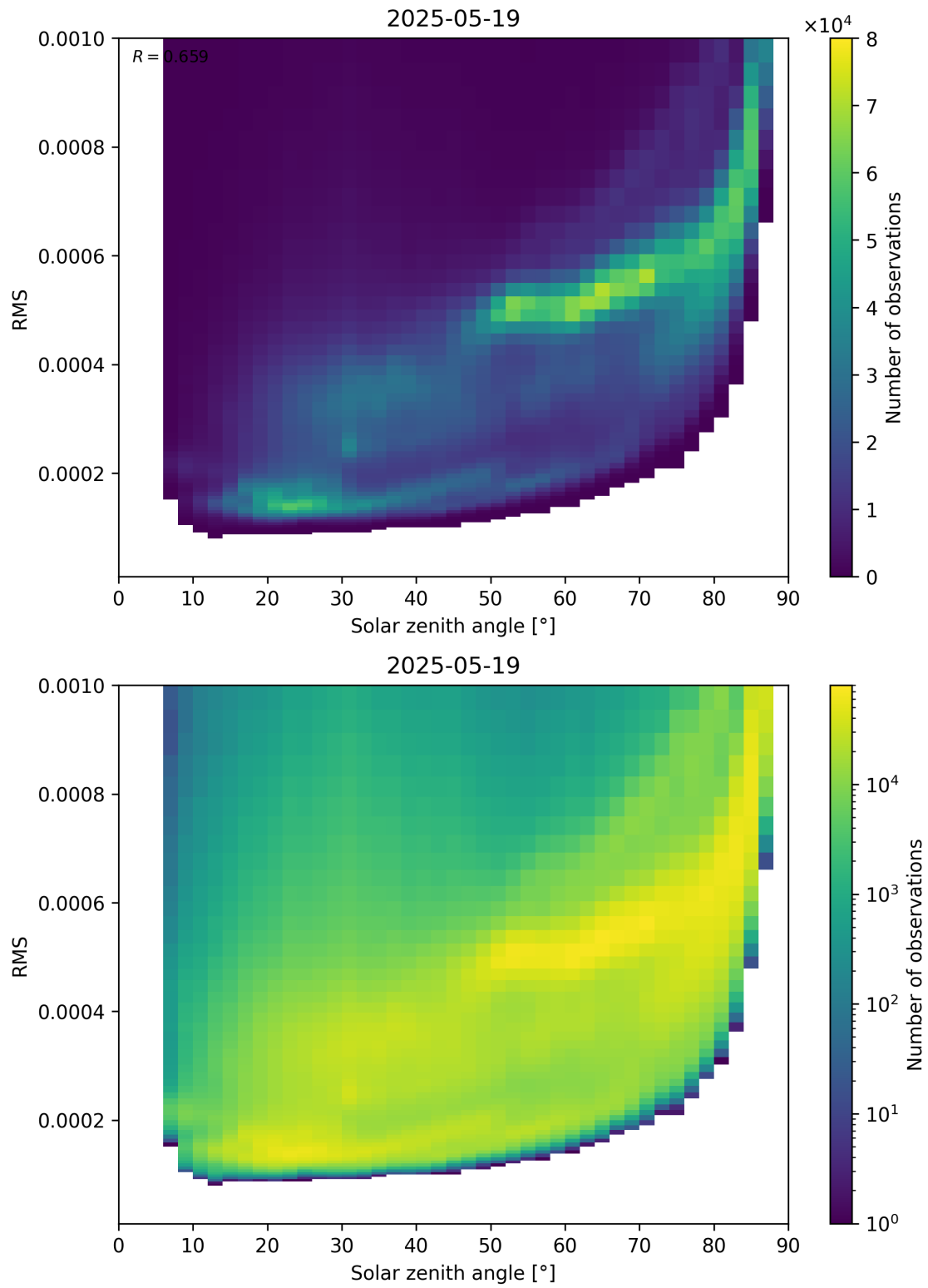
Figure 157: Scatter density plot of “Solar zenith angle” against “RMS” for 2025-05-18 to 2025-05-20.
