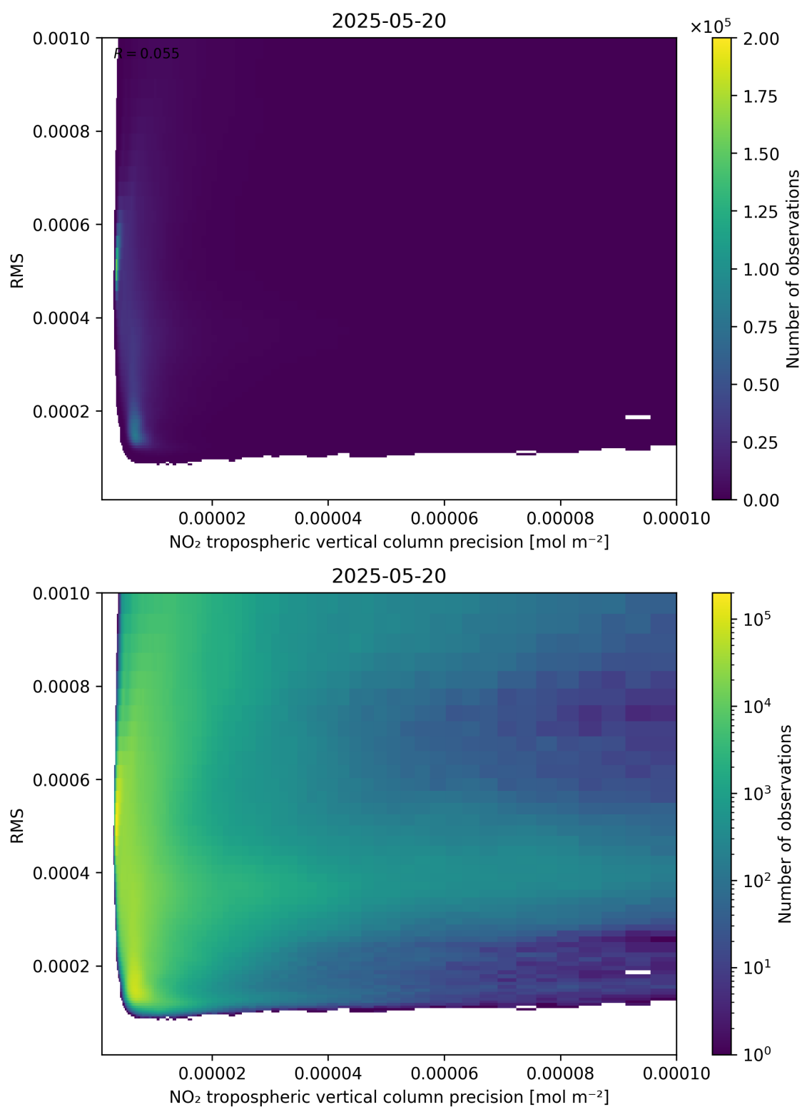
Figure 140: Scatter density plot of “NO 2 tropospheric vertical column precision” against “RMS” for 2025-05-19 to 2025-05-21.
