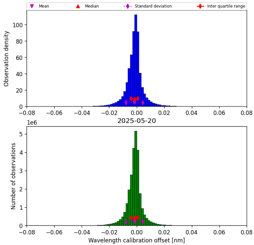
Figure 35: Histogram of “Wavelength calibration offset” for 2025-05-19 to 2025-05-21
