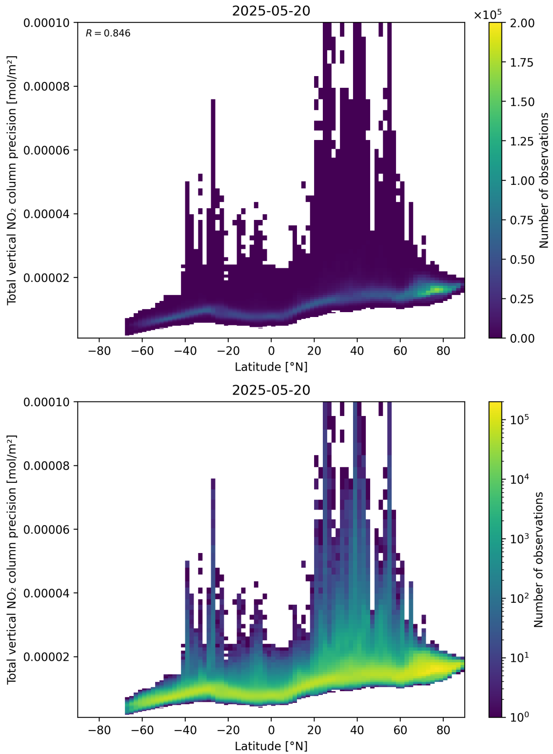
Figure 91: Scatter density plot of “Latitude” against “Total vertical NO 2 column precision” for 2025-05-19 to 2025-05-21.
