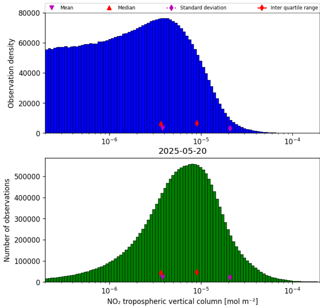
Figure 29: Histogram of “ \text{NO}_2 tropospheric vertical column” for 2025-05-19 to 2025-05-21
