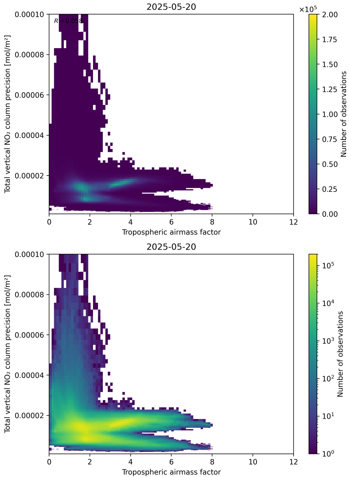
Figure 78: Scatter density plot of “Tropospheric air mass factor” against “Total vertical NO 2 column precision” for 2025-05-19 to 2025-05-21.
