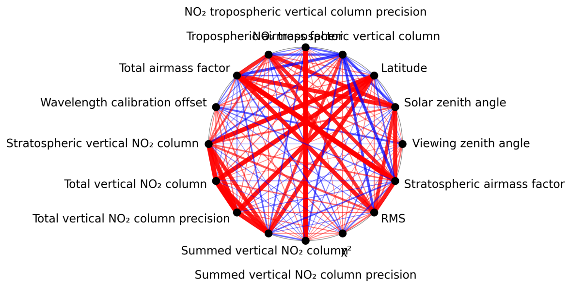
Figure 1: Map of correlation graph for 2025-05-19 to 2025-05-21.
