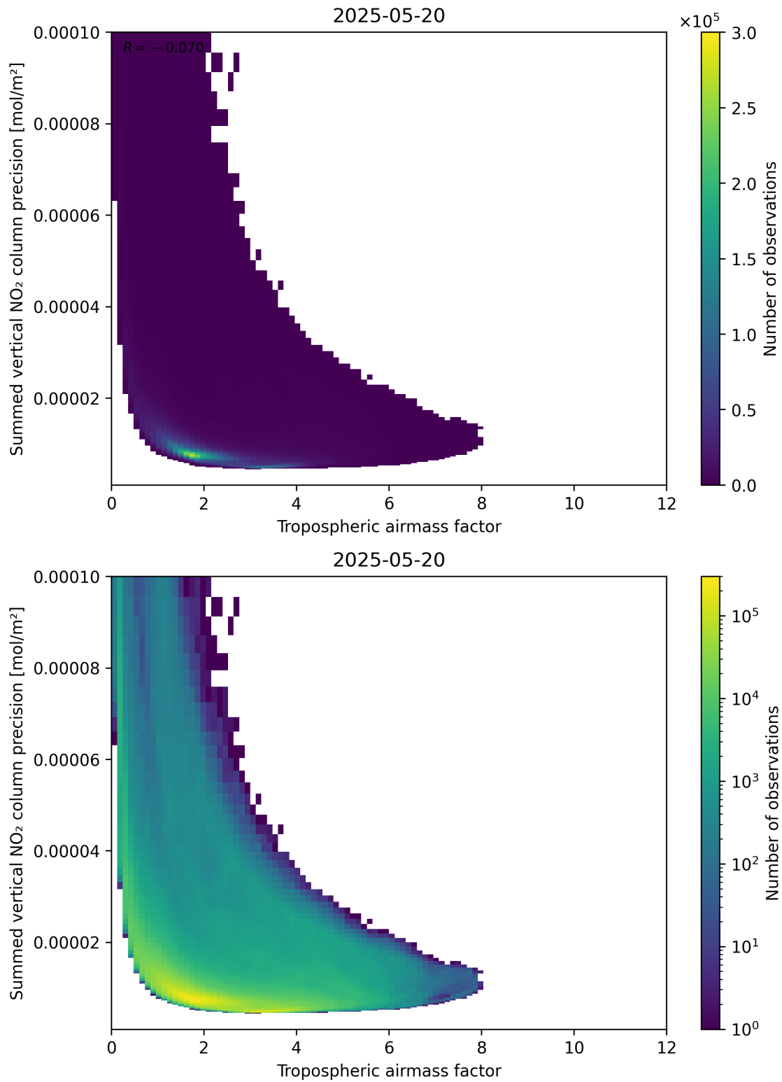
Figure 76: Scatter density plot of “Tropospheric air mass factor” against “Summed vertical NO 2 column precision” for 2025-05-19 to 2025-05-21.
