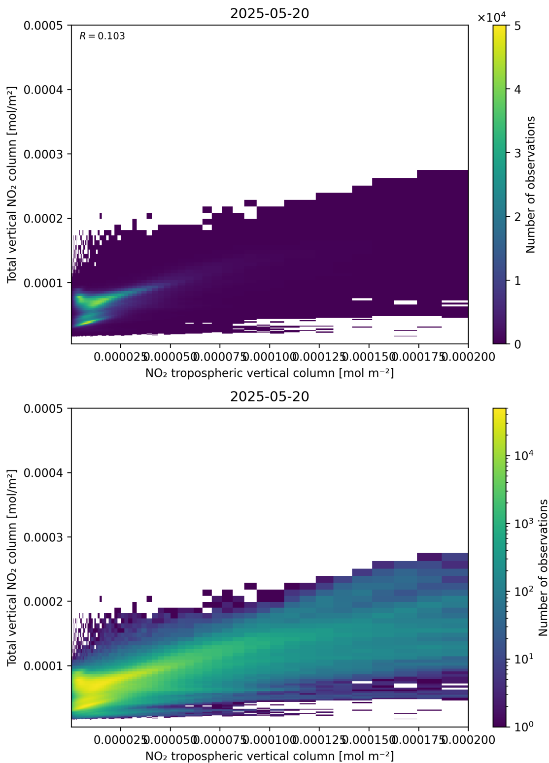
Figure 128: Scatter density plot of “NO 2 tropospheric vertical column” against “Total vertical NO 2 column” for 2025-05-19 to 2025-05-21.
