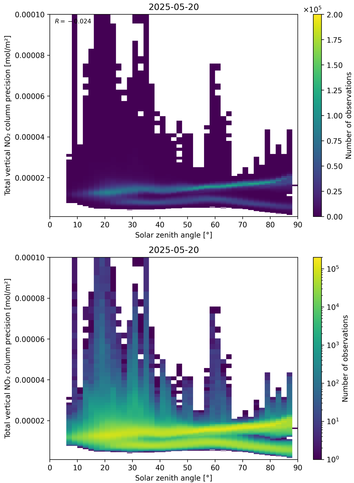
Figure 154: Scatter density plot of “Solar zenith angle” against “Total vertical NO 2 column precision” for 2025-05-19 to 2025-05-21.
