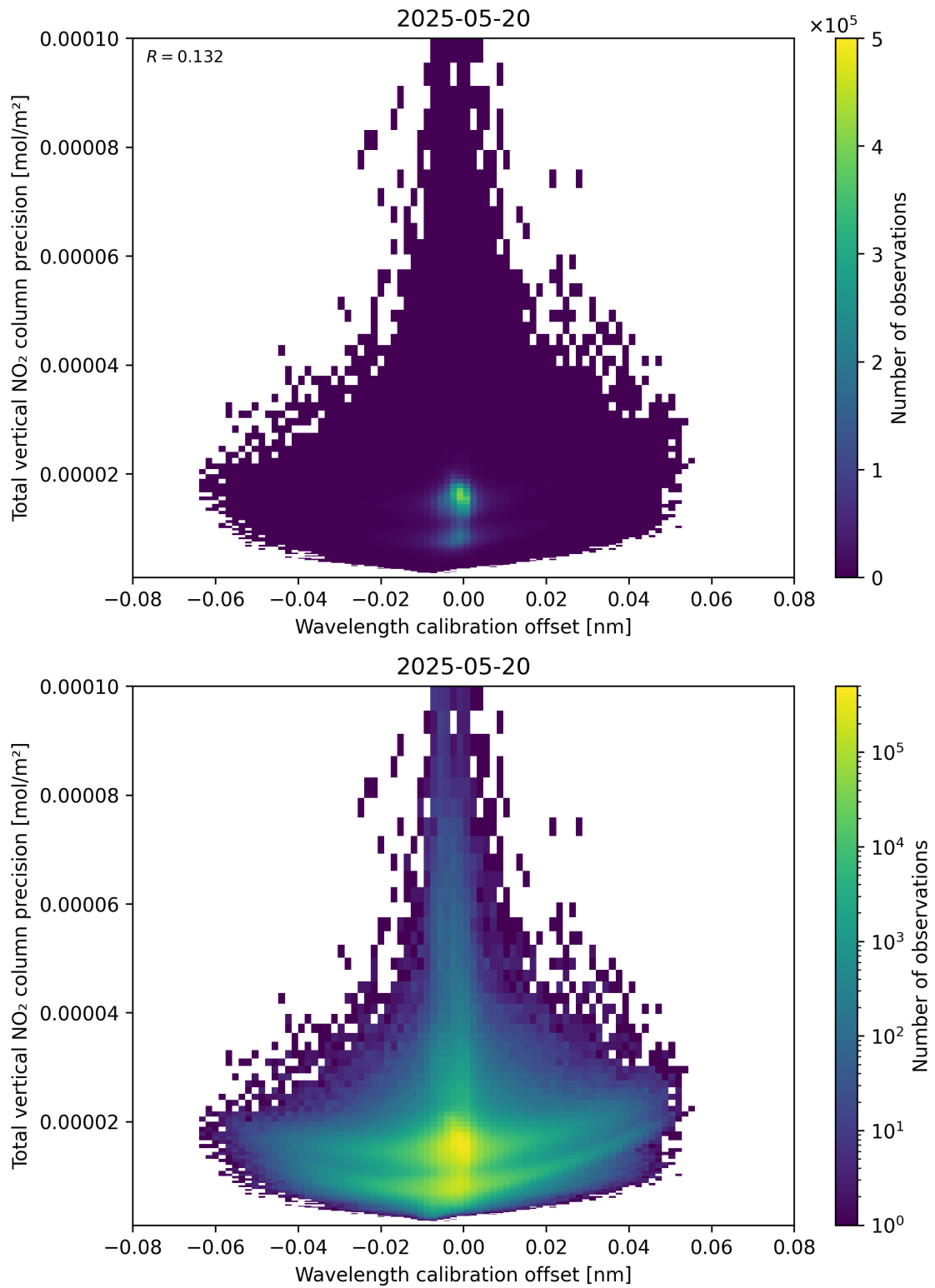
Figure 180: Scatter density plot of “Wavelength calibration offset” against “Total vertical NO 2 column precision” for 2025-05-19 to 2025-05-21.
