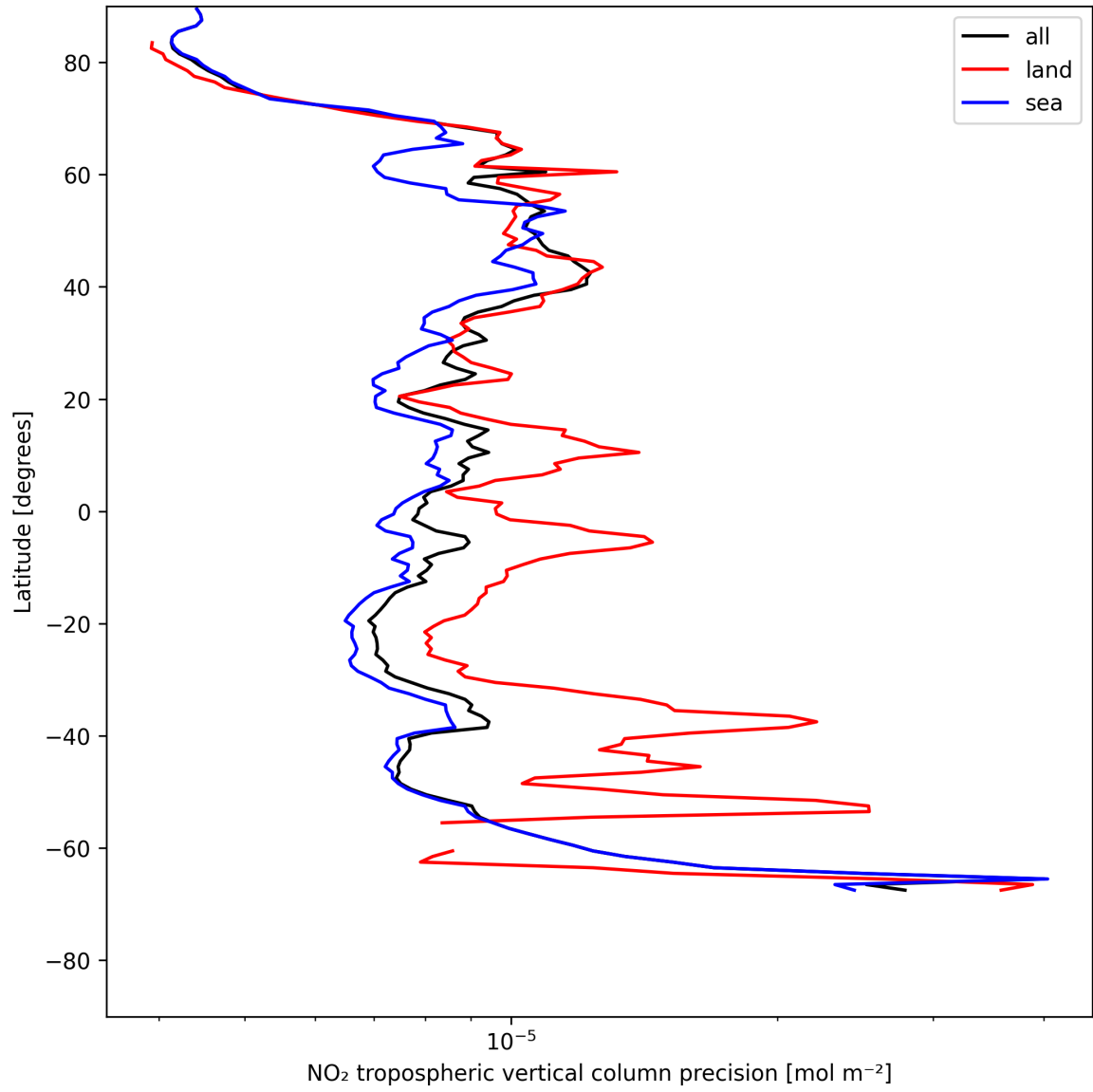
Figure 13: Zonal average of “NO 2 tropospheric vertical column precision” for 2025-05-19 to 2025-05-21.
