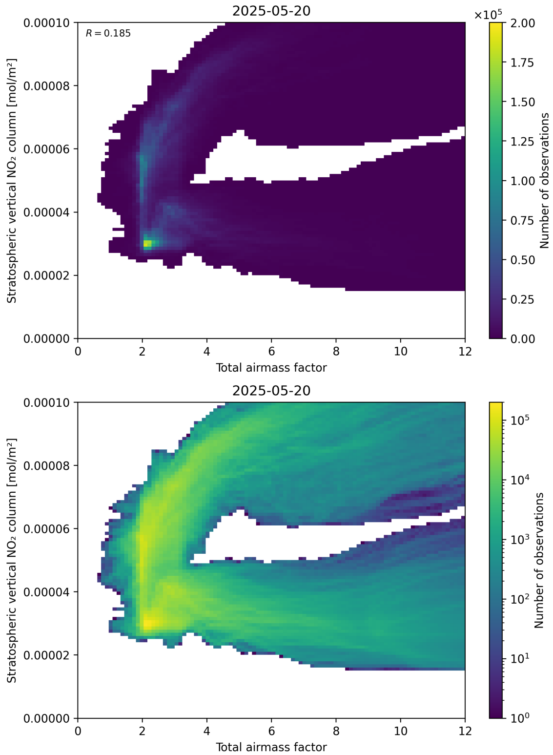
Figure 64: Scatter density plot of “Total airmass factor” against “Stratospheric vertical \text{NO}_2 column” for 2025-05-19 to 2025-05-21.
