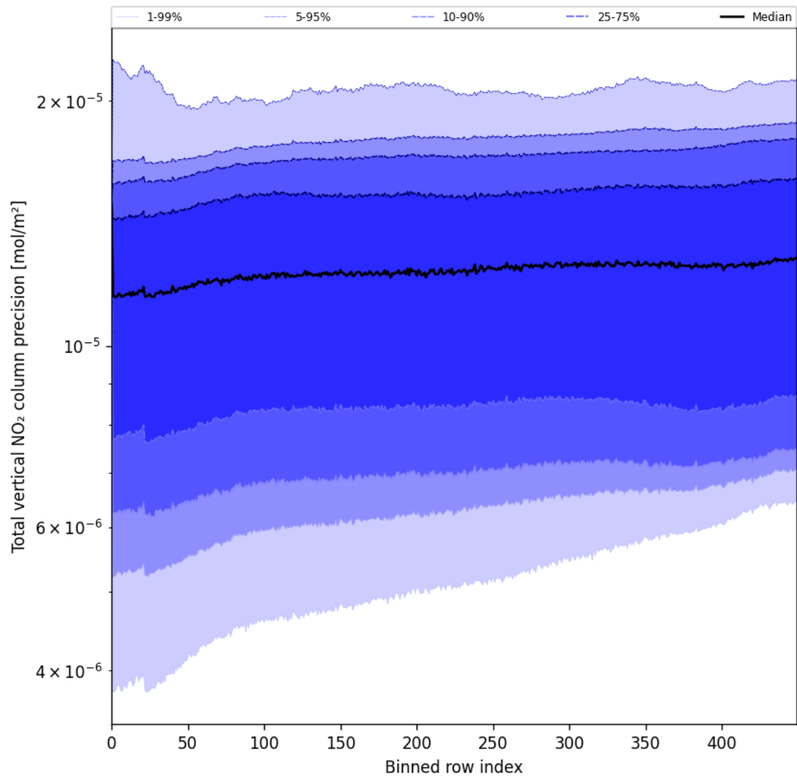
Figure 56: Along track statistics of "Total vertical NO 2 column precision" for 2025-05-19 to 2025-05-21
