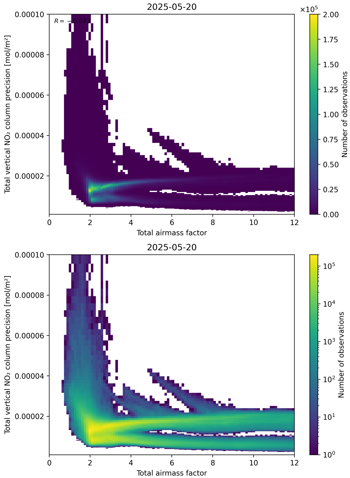
Figure 68: Scatter density plot of “Total airmass factor” against “Total vertical NO 2 column precision” for 2025-05-19 to 2025-05-21.
