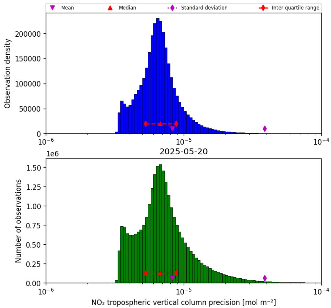
Figure 30: Histogram of “NO 2 tropospheric vertical column precision” for 2025-05-19 to 2025-05-21
