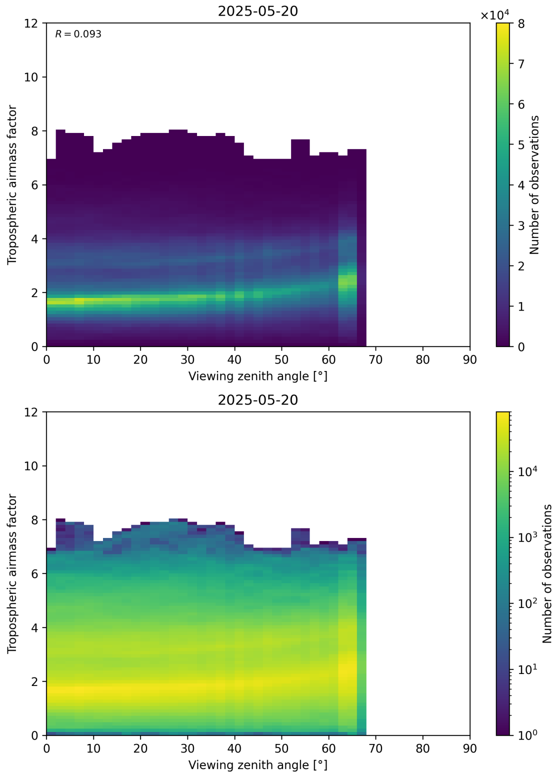
Figure 161: Scatter density plot of “Viewing zenith angle” against “Tropospheric airmass factor” for 2025-05-19 to 2025-05-21.
