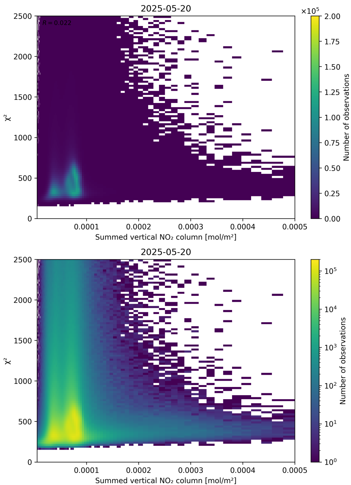
Figure 104: Scatter density plot of “Summed vertical NO 2 column” against “ \chi^2 ” for 2025-05-19 to 2025-05-21.
