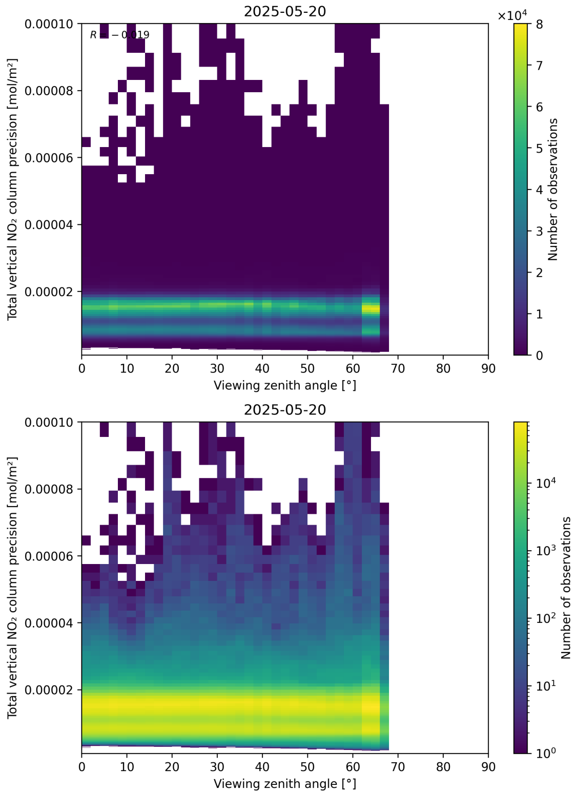
Figure 168: Scatter density plot of “Viewing zenith angle” against “Total vertical NO 2 column precision” for 2025-05-19 to 2025-05-21.
