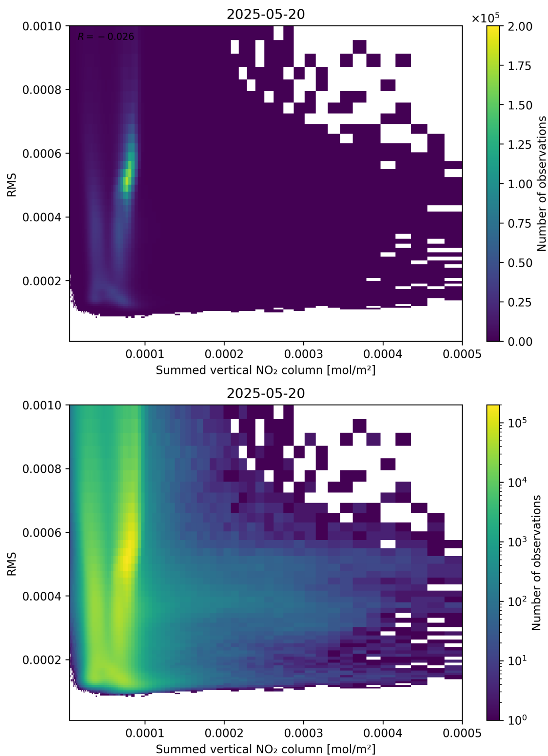
Figure 109: Scatter density plot of “Summed vertical NO 2 column” against “RMS” for 2025-05-19 to 2025-05-21.
