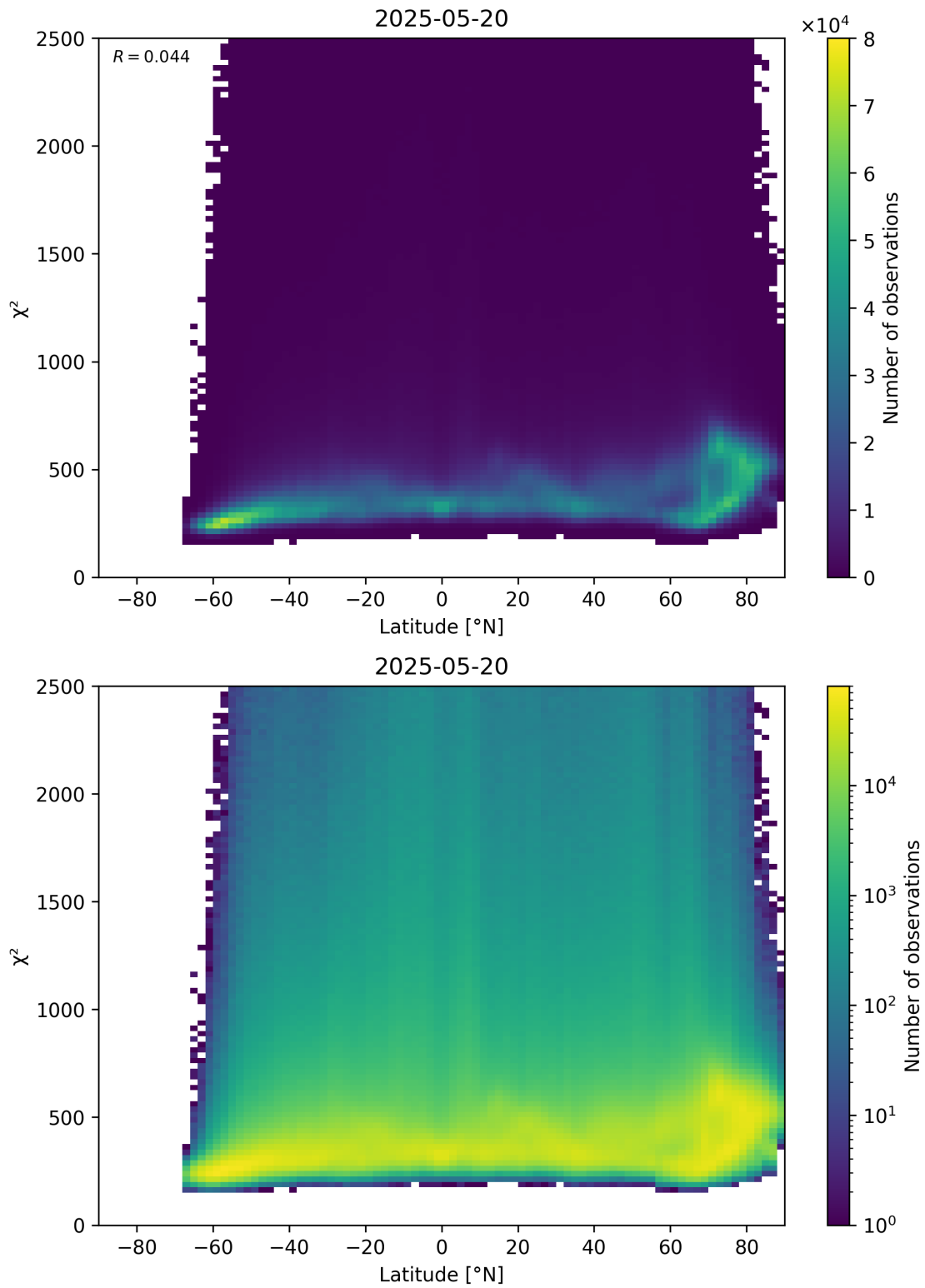
Figure 86: Scatter density plot of “Latitude” against “ \chi^2 ” for 2025-05-19 to 2025-05-21.
