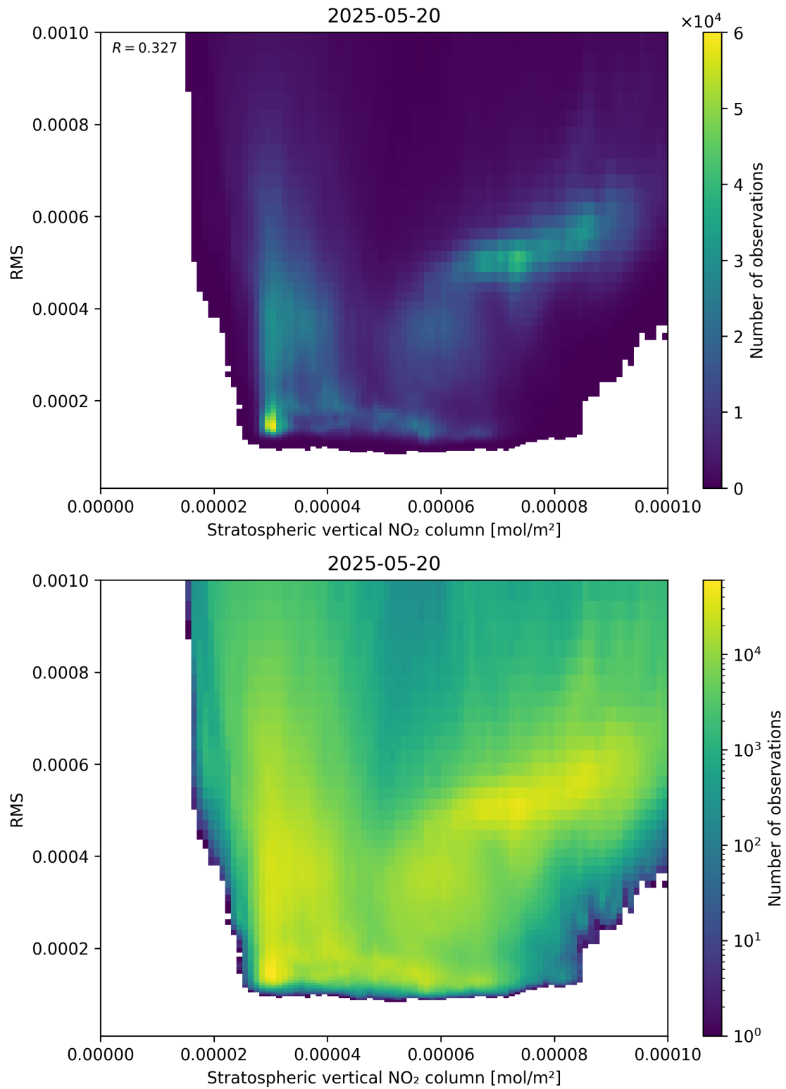
Figure 102: Scatter density plot of “Stratospheric vertical NO 2 column” against “RMS” for 2025-05-19 to 2025-05-21.
