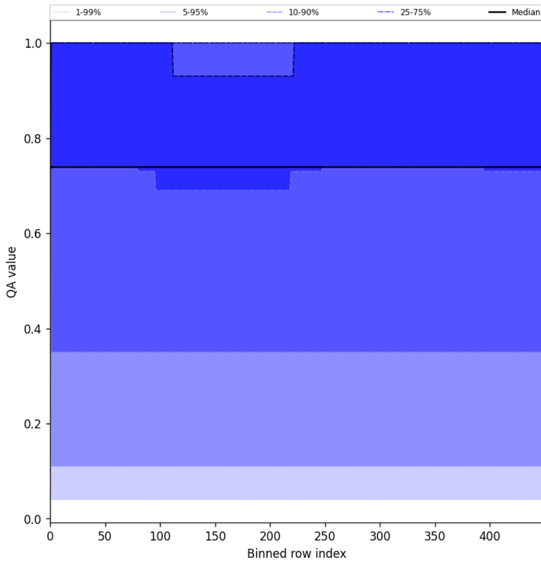
Figure 45: Along track statistics of “QA value” for 2025-05-19 to 2025-05-21
