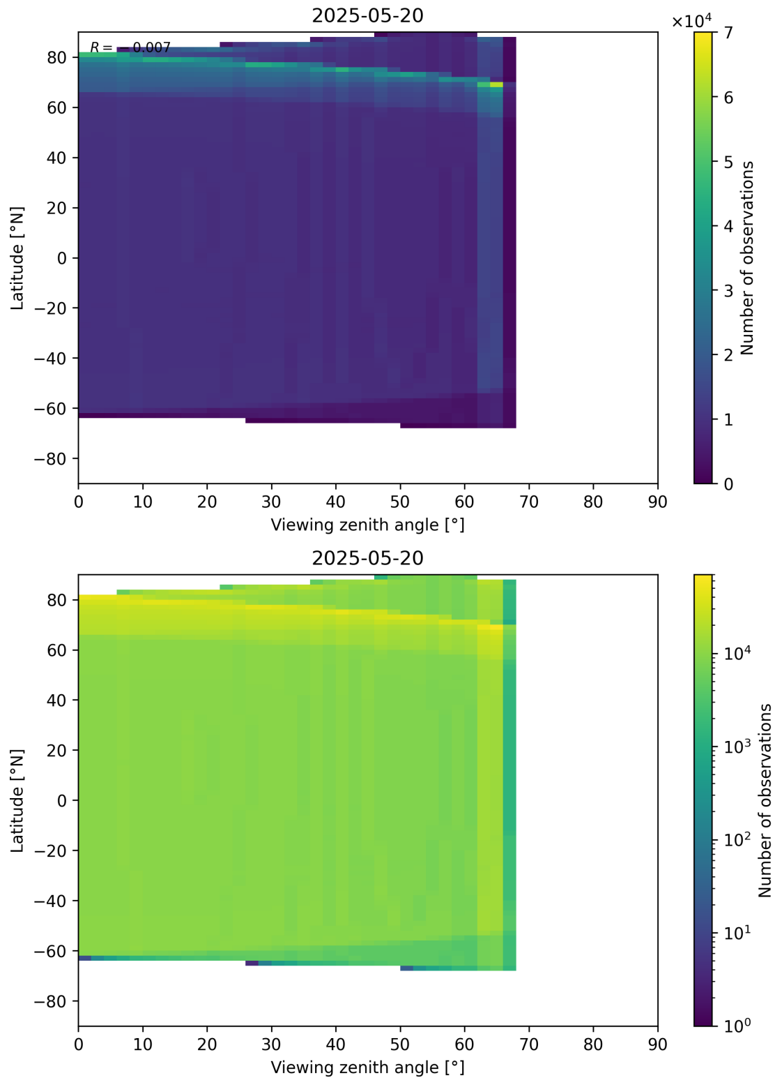
Figure 163: Scatter density plot of “Viewing zenith angle” against “Latitude” for 2025-05-19 to 2025-05-21.
