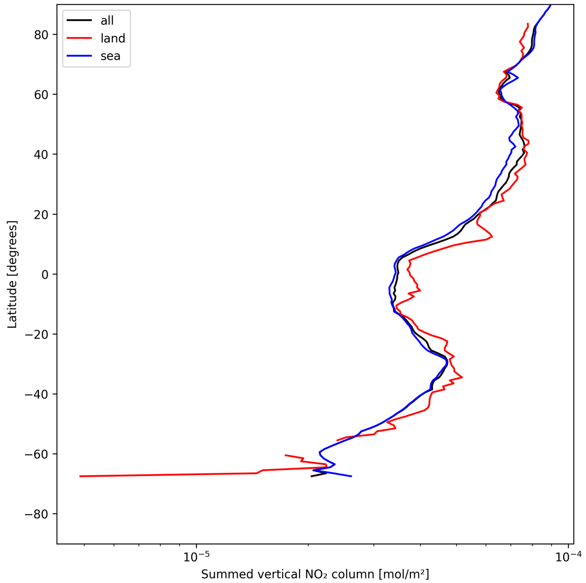
Figure 23: Zonal average of “Summed vertical NO 2 column” for 2025-05-19 to 2025-05-21.
