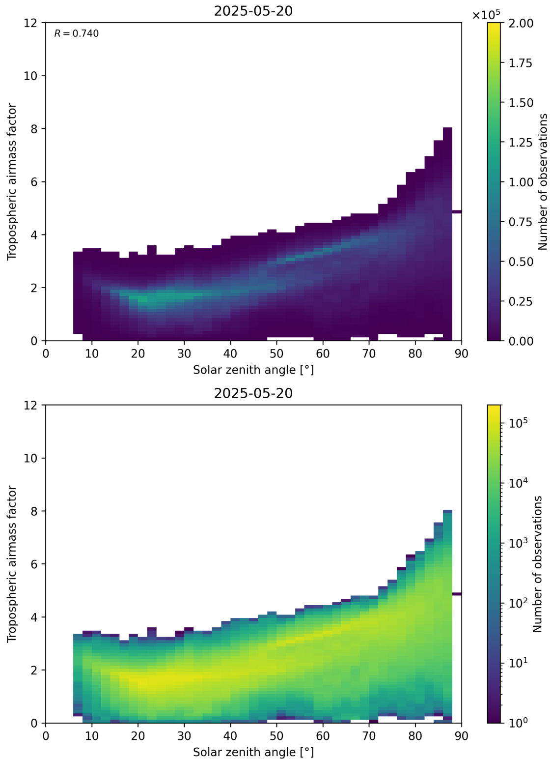
Figure 147: Scatter density plot of “Solar zenith angle” against “Tropospheric airmass factor” for 2025-05-19 to 2025-05-21.
