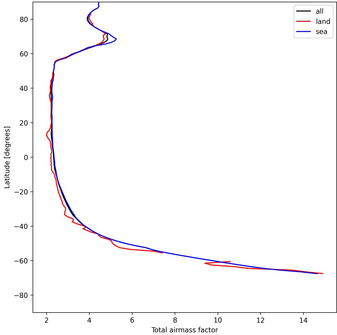
Figure 15: Zonal average of “Total airmass factor” for 2025-05-19 to 2025-05-21.
