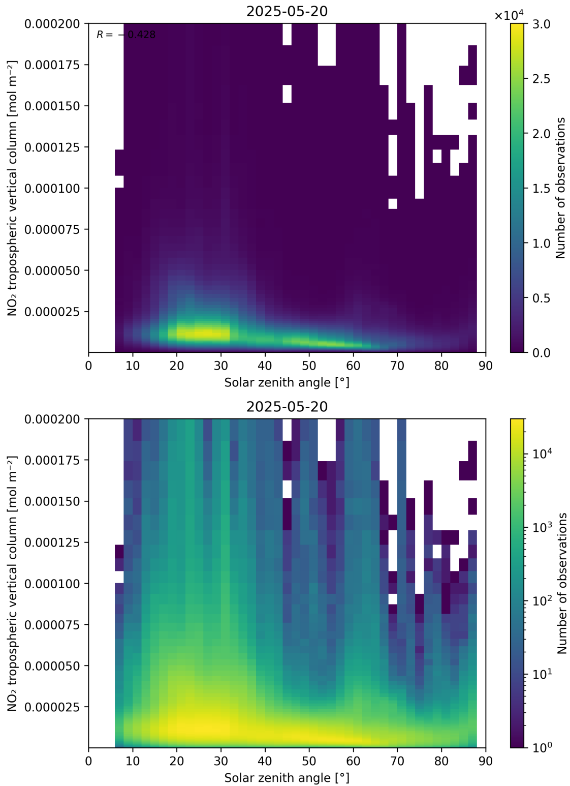
Figure 155: Scatter density plot of “Solar zenith angle” against “NO 2 tropospheric vertical column” for 2025-05-19 to 2025-05-21.
