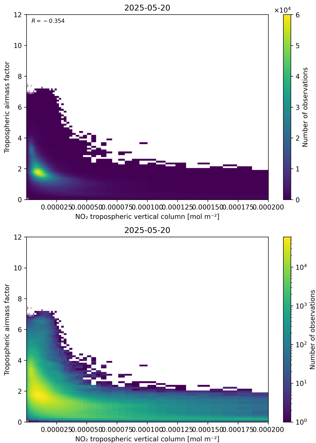
Figure 123: Scatter density plot of “NO 2 tropospheric vertical column” against “Tropospheric air mass factor” for 2025-05-19 to 2025-05-21.
