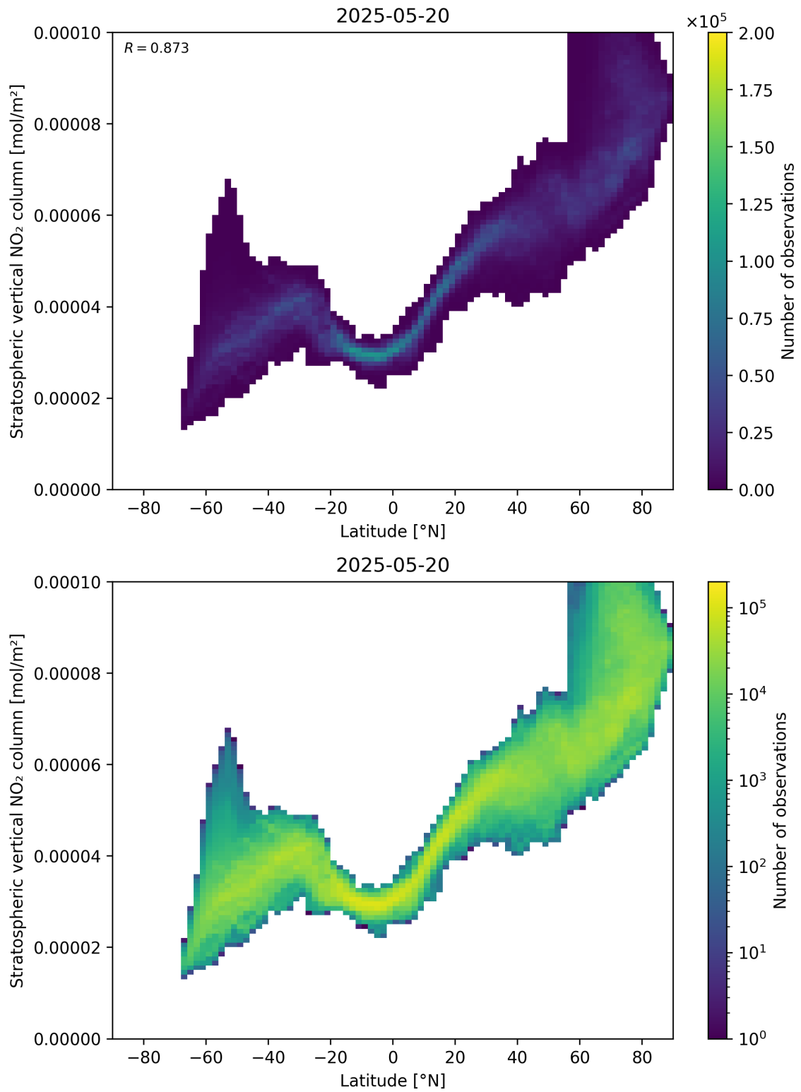
Figure 87: Scatter density plot of “Latitude” against “Stratospheric vertical NO 2 column” for 2025-05-19 to 2025-05-21.
