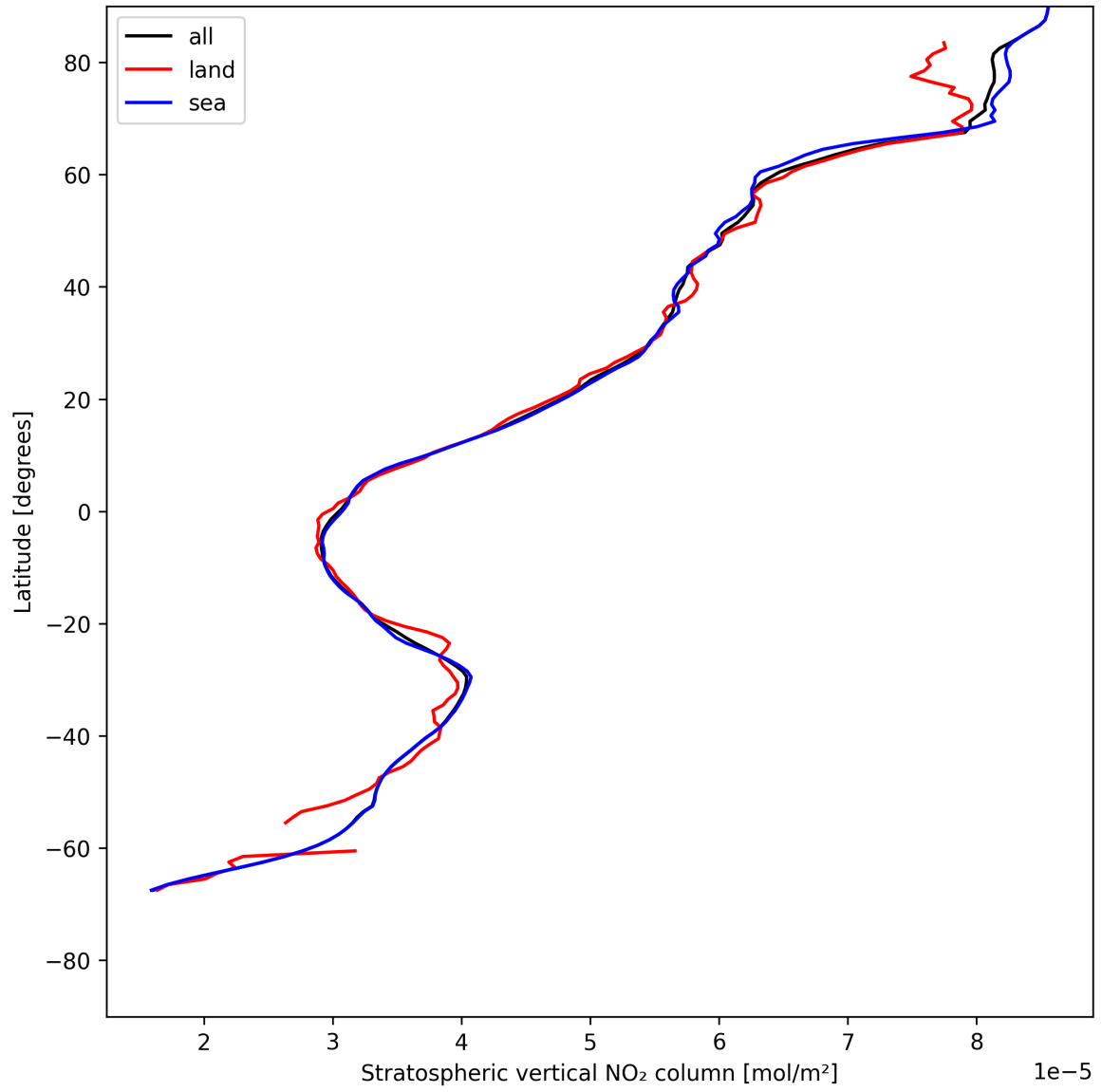
Figure 19: Zonal average of “Stratospheric vertical NO 2 column” for 2025-05-19 to 2025-05-21.
