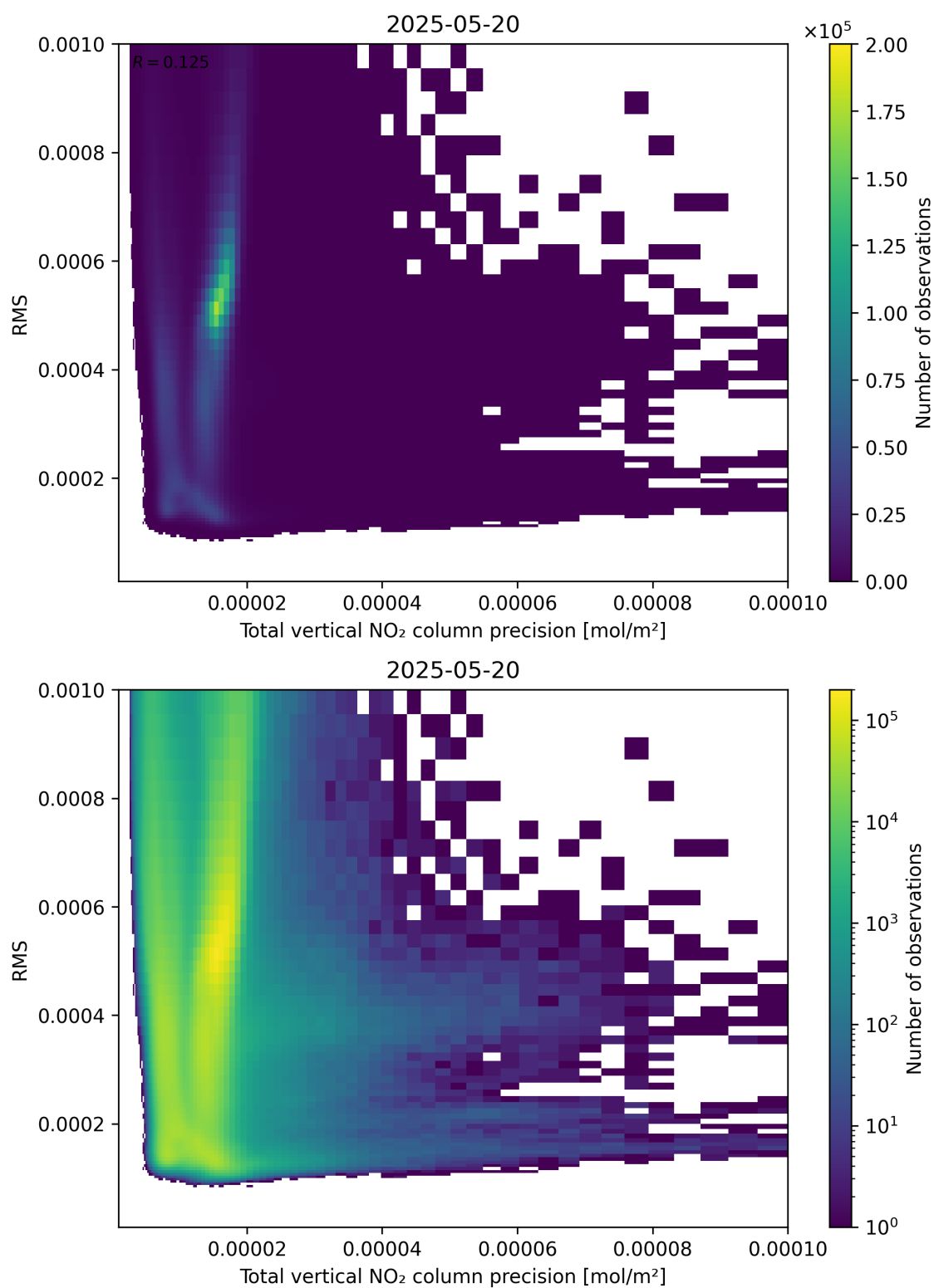
Figure 119: Scatter density plot of “Total vertical NO 2 column precision” against “RMS” for 2025-05-19 to 2025-05-21.
