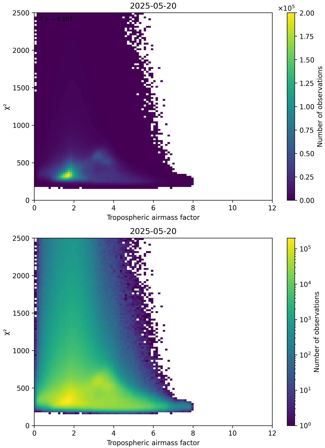
Figure 73: Scatter density plot of “Tropospheric airmass factor” against “ \chi^2 ” for 2025-05-19 to 2025-05-21.
