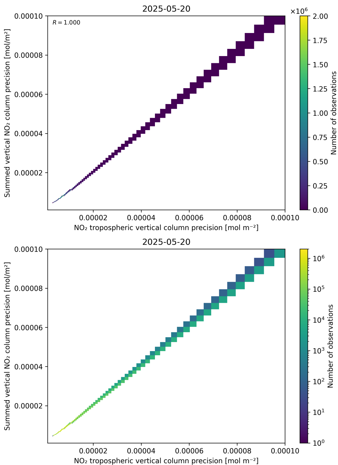
Figure 137: Scatter density plot of “NO 2 tropospheric vertical column precision” against “Summed vertical NO 2 column precision” for 2025-05-19 to 2025-05-21.
