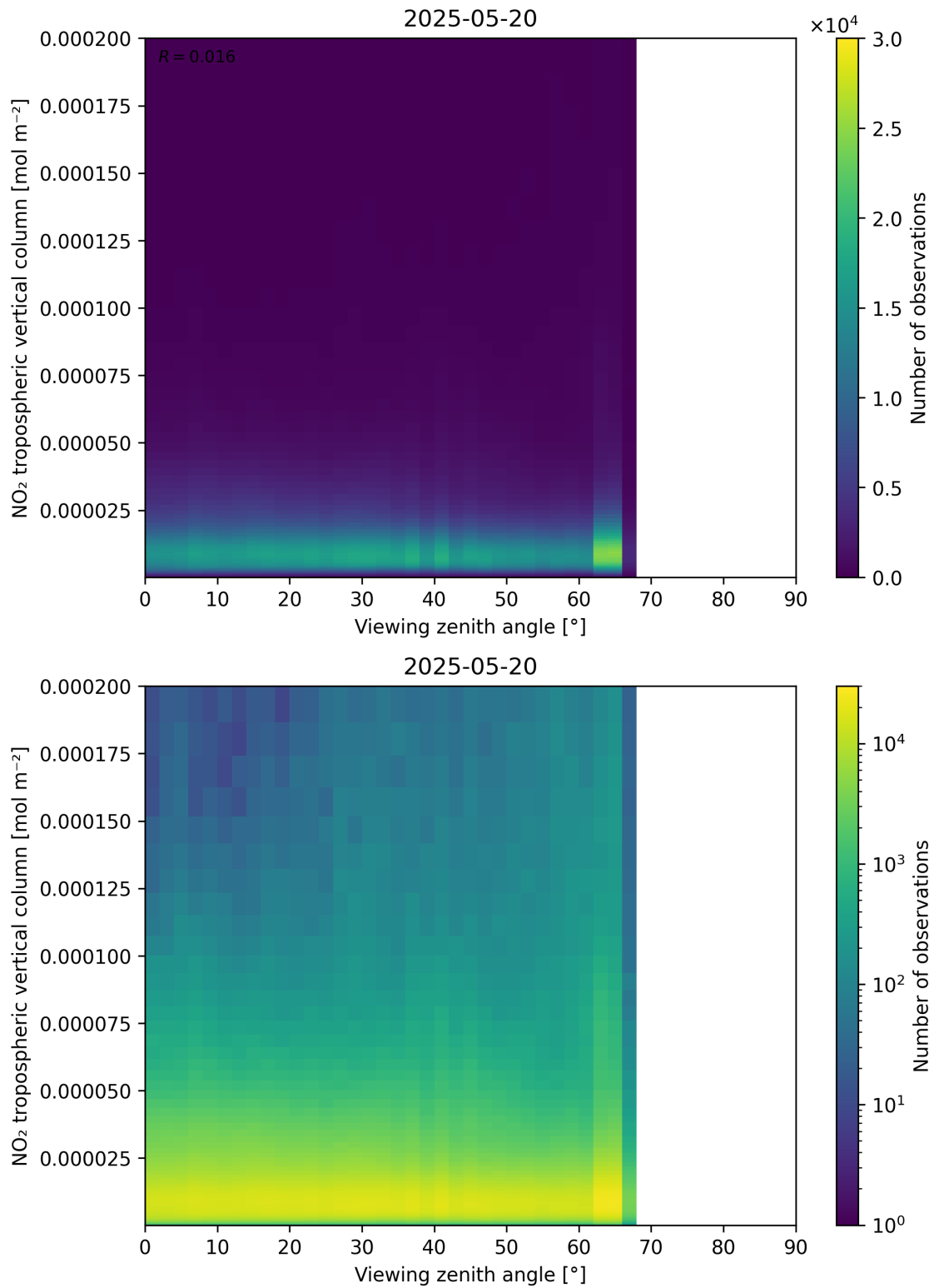
Figure 169: Scatter density plot of “Viewing zenith angle” against “NO 2 tropospheric vertical column” for 2025-05-19 to 2025-05-21.
