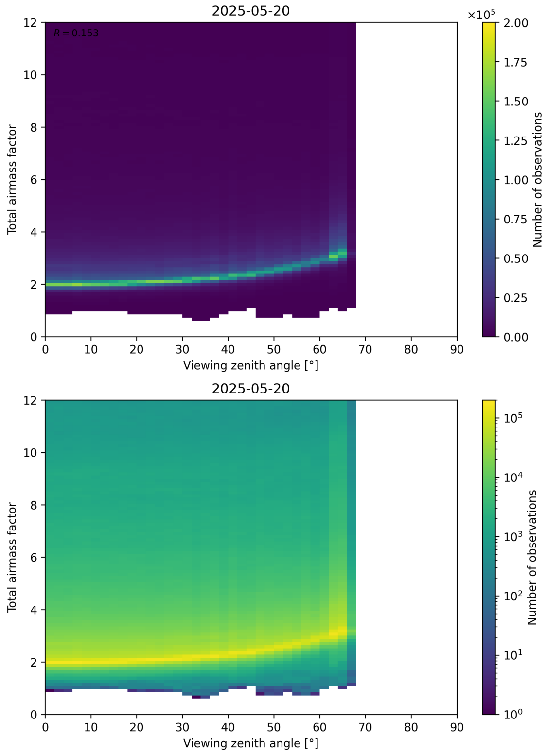
Figure 160: Scatter density plot of “Viewing zenith angle” against “Total airmass factor” for 2025-05-19 to 2025-05-21.
