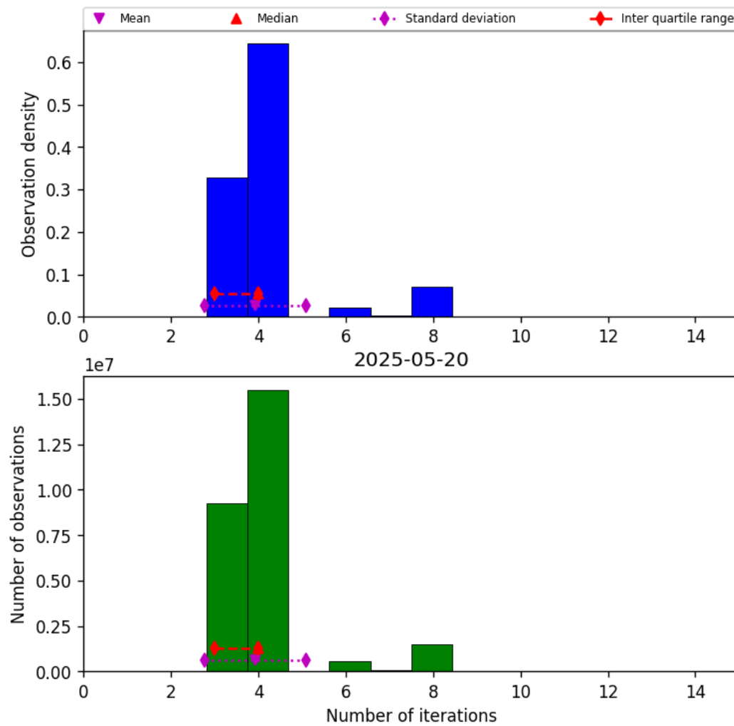
Figure 34: Histogram of “Number of iterations” for 2025-05-19 to 2025-05-21
