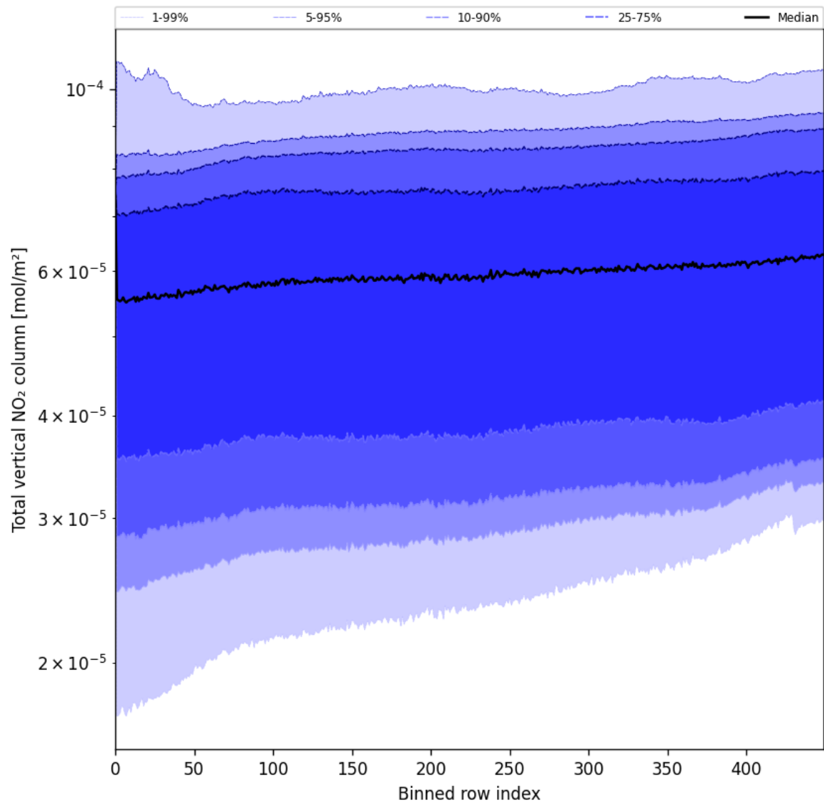
Figure 55: Along track statistics of “Total vertical NO 2 column” for 2025-05-19 to 2025-05-21
