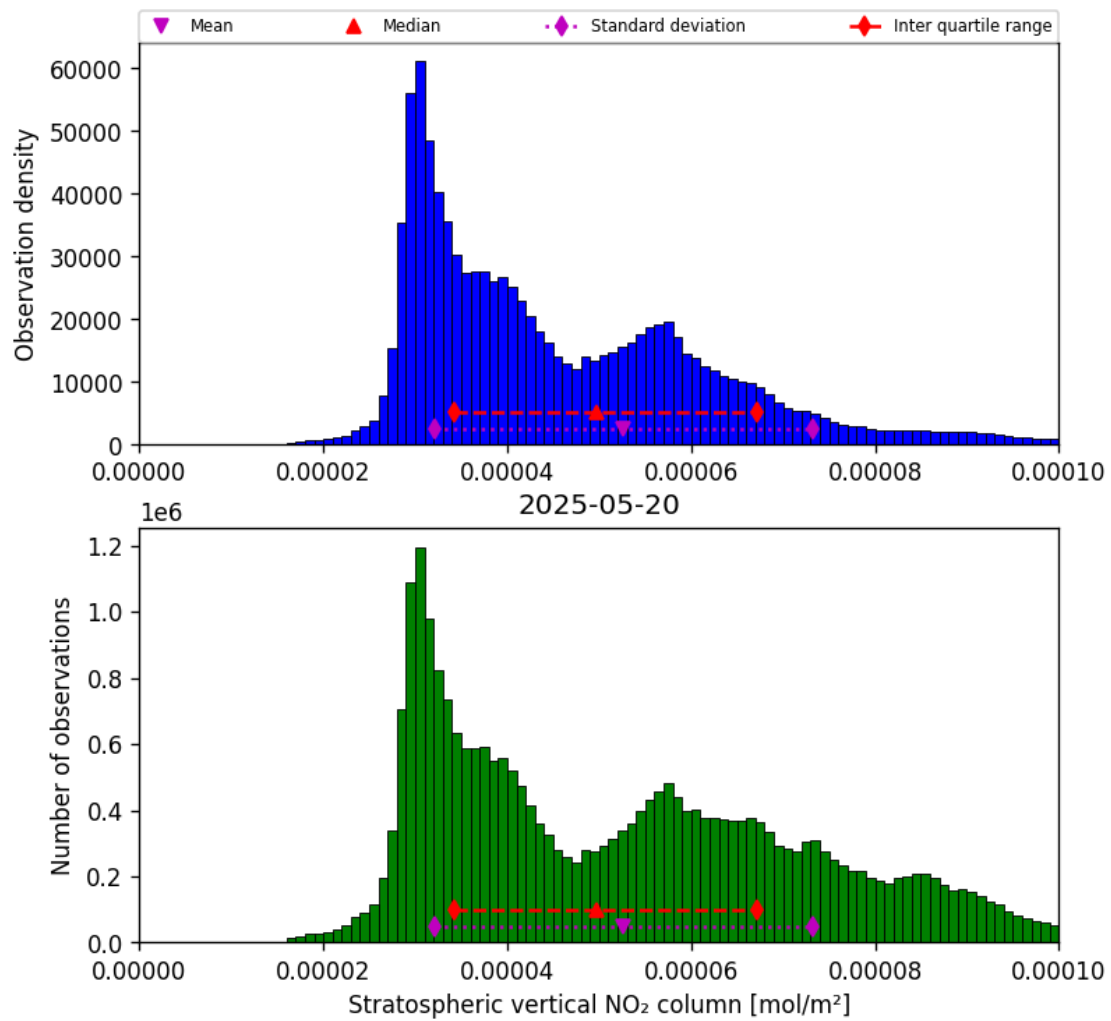
Figure 36: Histogram of “Stratospheric vertical NO 2 column” for 2025-05-19 to 2025-05-21
