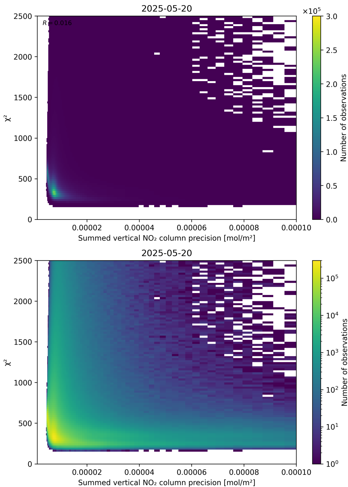
Figure 107: Scatter density plot of “Summed vertical NO 2 column precision” against “ \chi^2 ” for 2025-05-19 to 2025-05-21.
