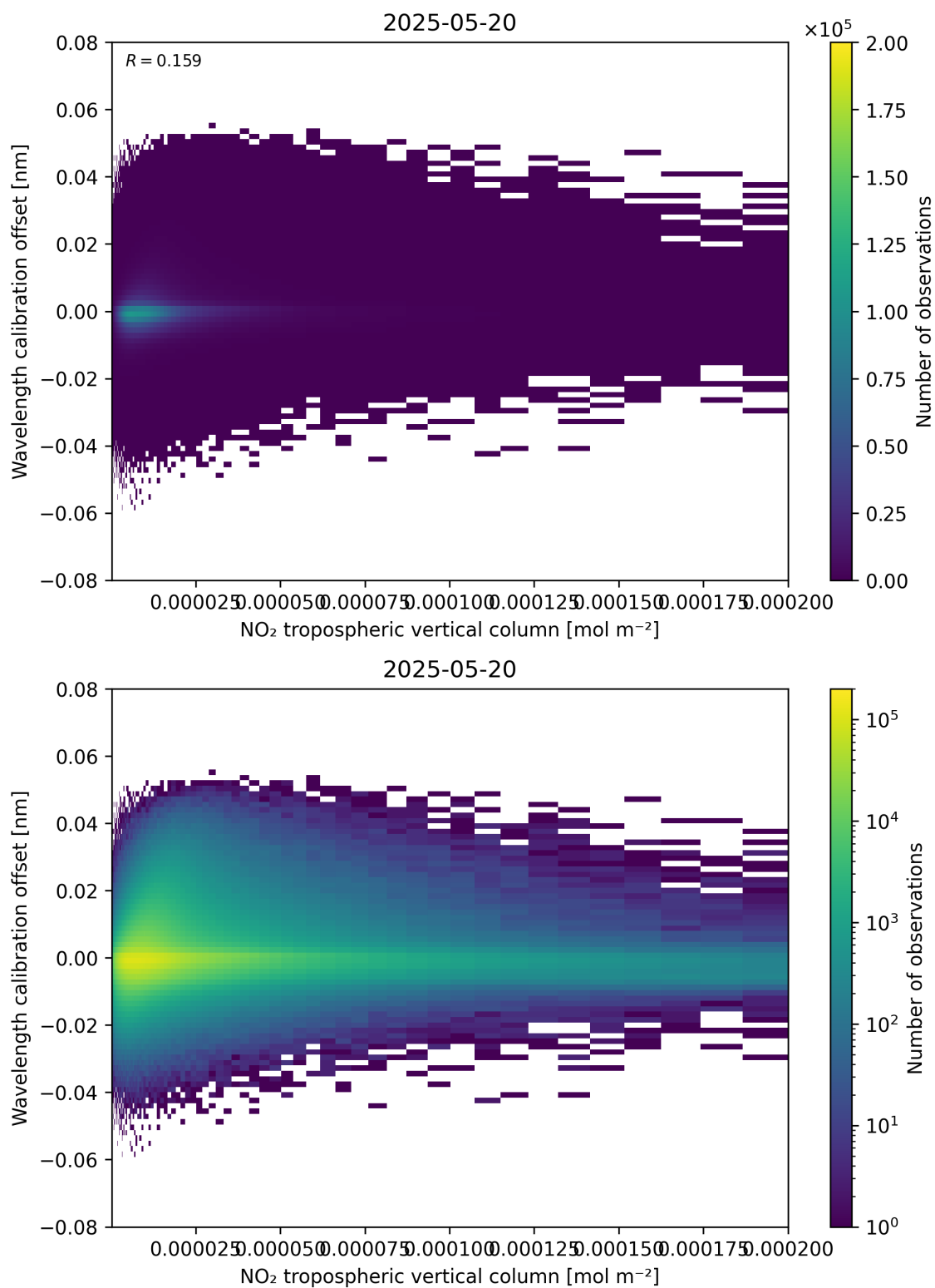
Figure 143: Scatter density plot of “NO 2 tropospheric vertical column” against “Wavelength calibration offset” for 2025-05-19 to 2025-05-21.
