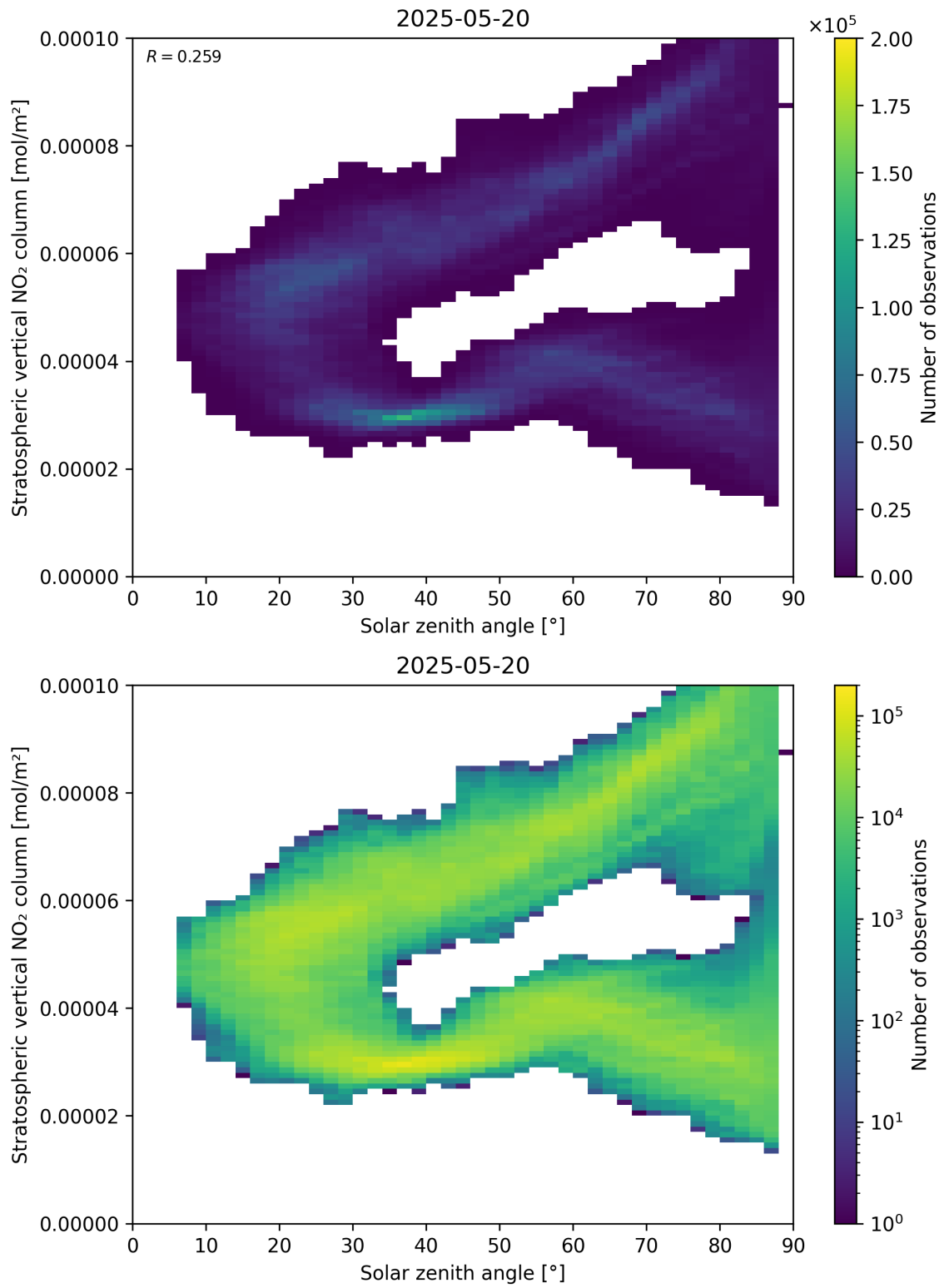
Figure 150: Scatter density plot of “Solar zenith angle” against “Stratospheric vertical \text{NO}_2 column” for 2025-05-19 to 2025-05-21.
