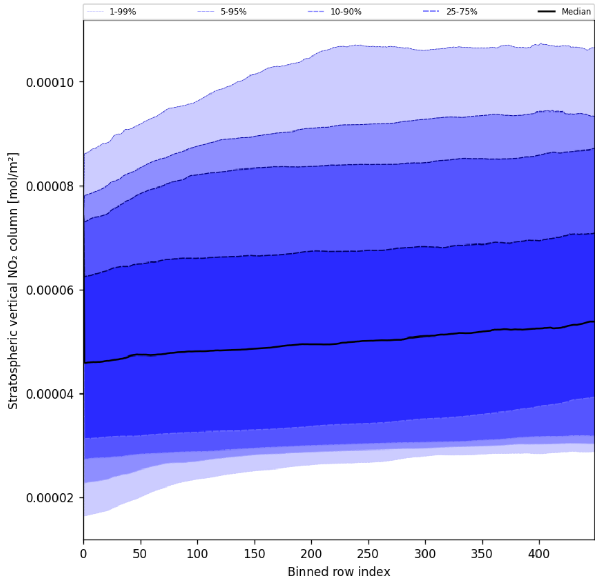
Figure 53: Along track statistics of “Stratospheric vertical NO 2 column” for 2025-05-19 to 2025-05-21
