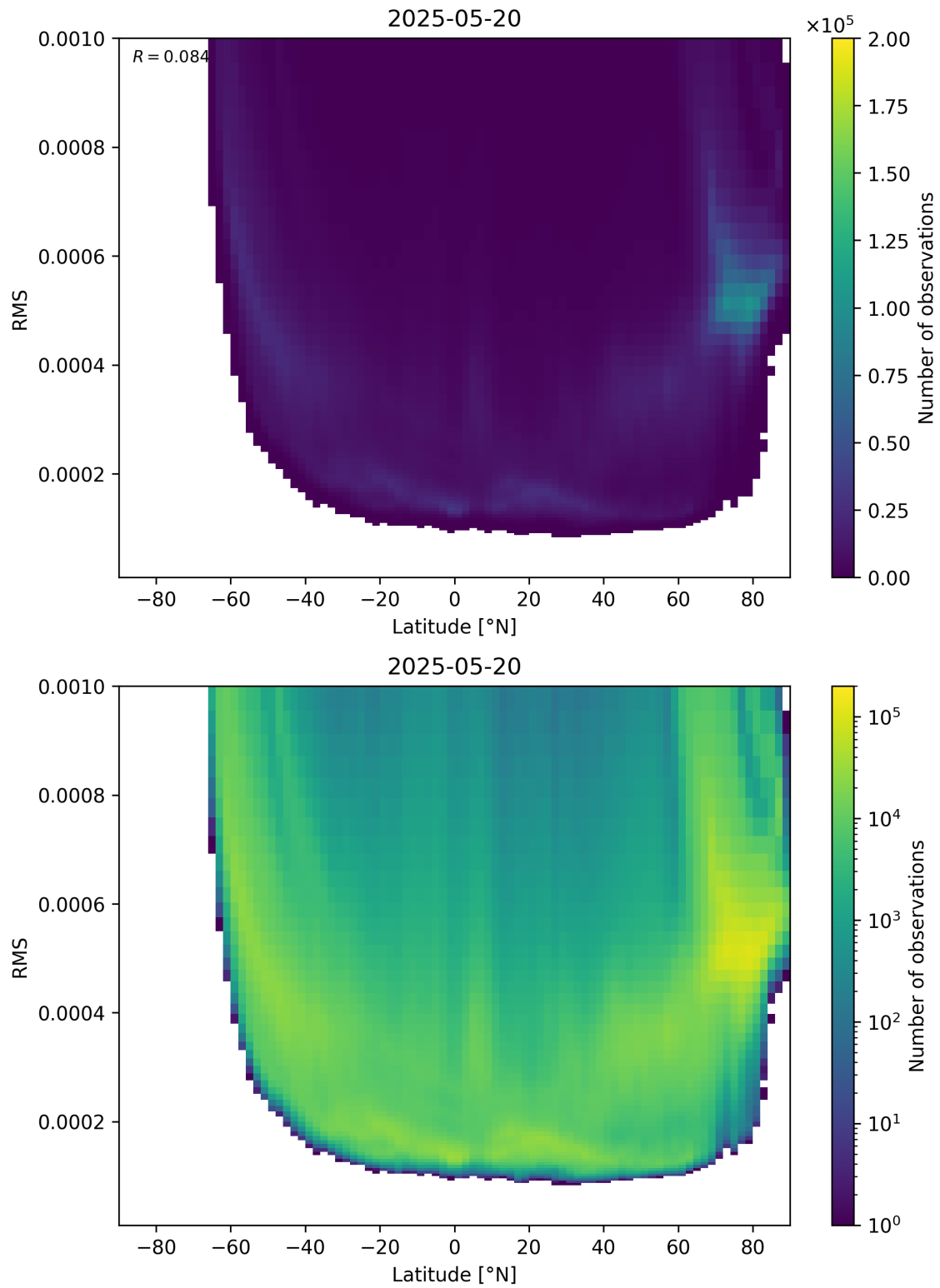
Figure 94: Scatter density plot of “Latitude” against “RMS” for 2025-05-19 to 2025-05-21.
