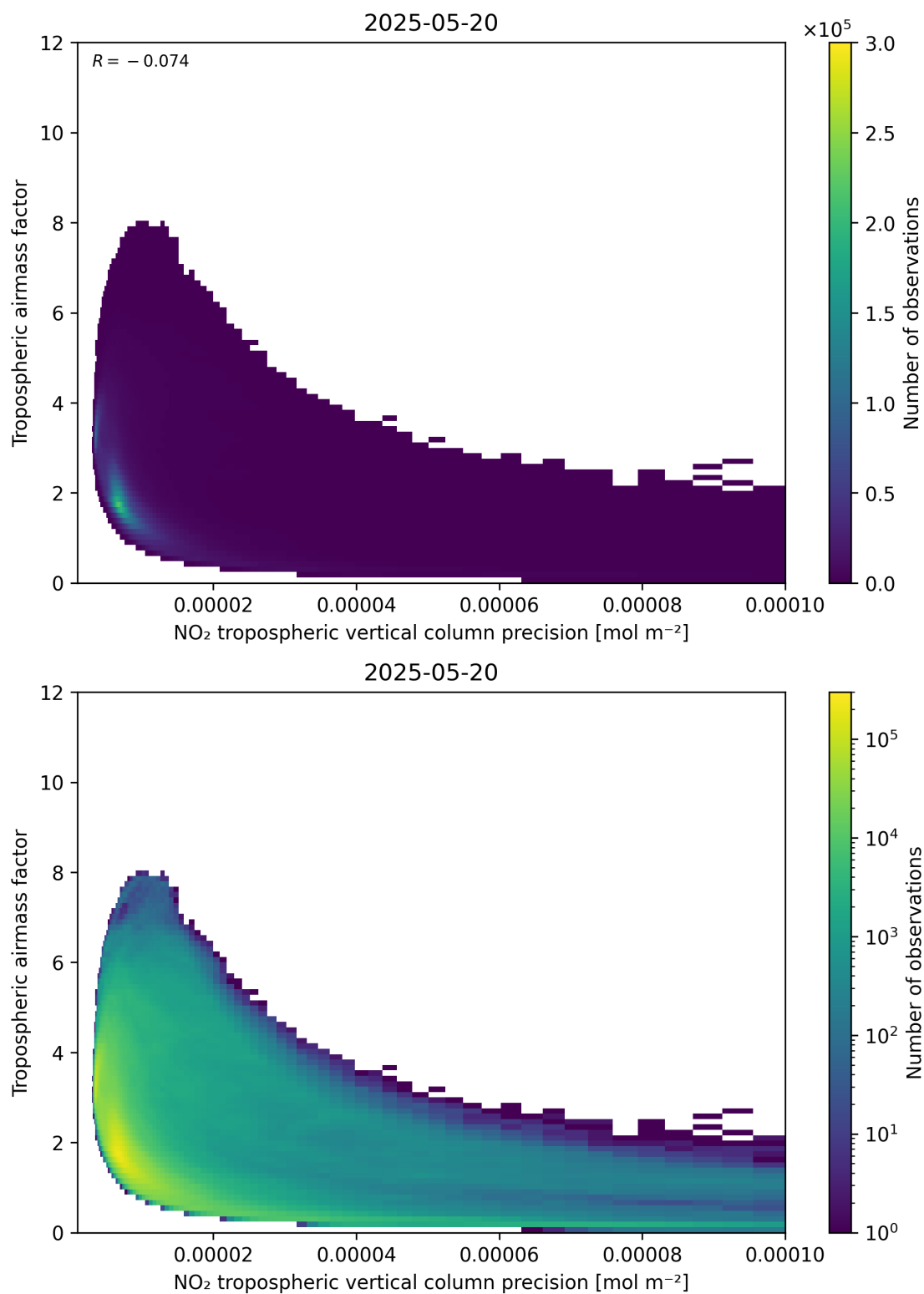
Figure 133: Scatter density plot of “NO 2 tropospheric vertical column precision” against “Tropospheric airmass factor” for 2025-05-19 to 2025-05-21.
