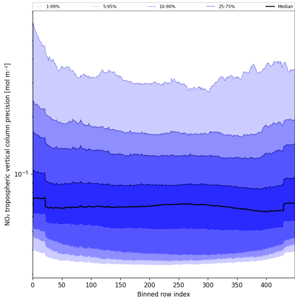
Figure 47: Along track statistics of “NO 2 tropospheric vertical column precision” for 2025-05-19 to 2025-05-21
