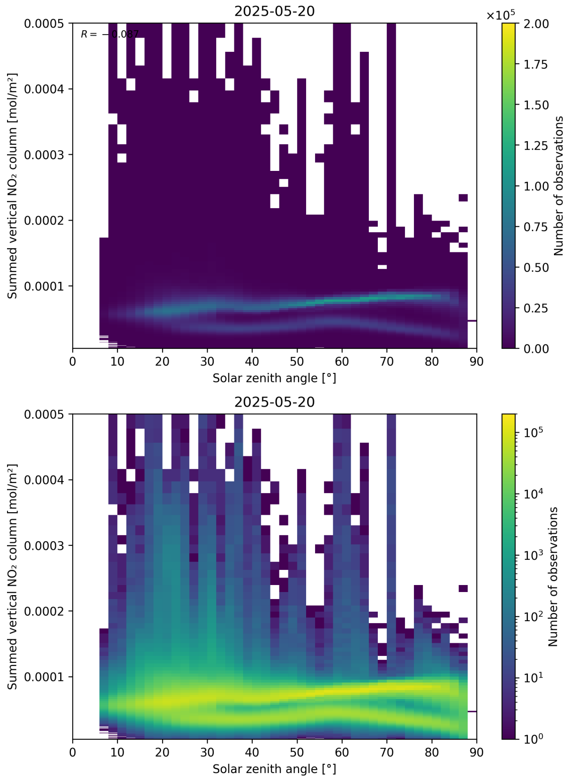
Figure 151: Scatter density plot of “Solar zenith angle” against “Summed vertical NO 2 column” for 2025-05-19 to 2025-05-21.
