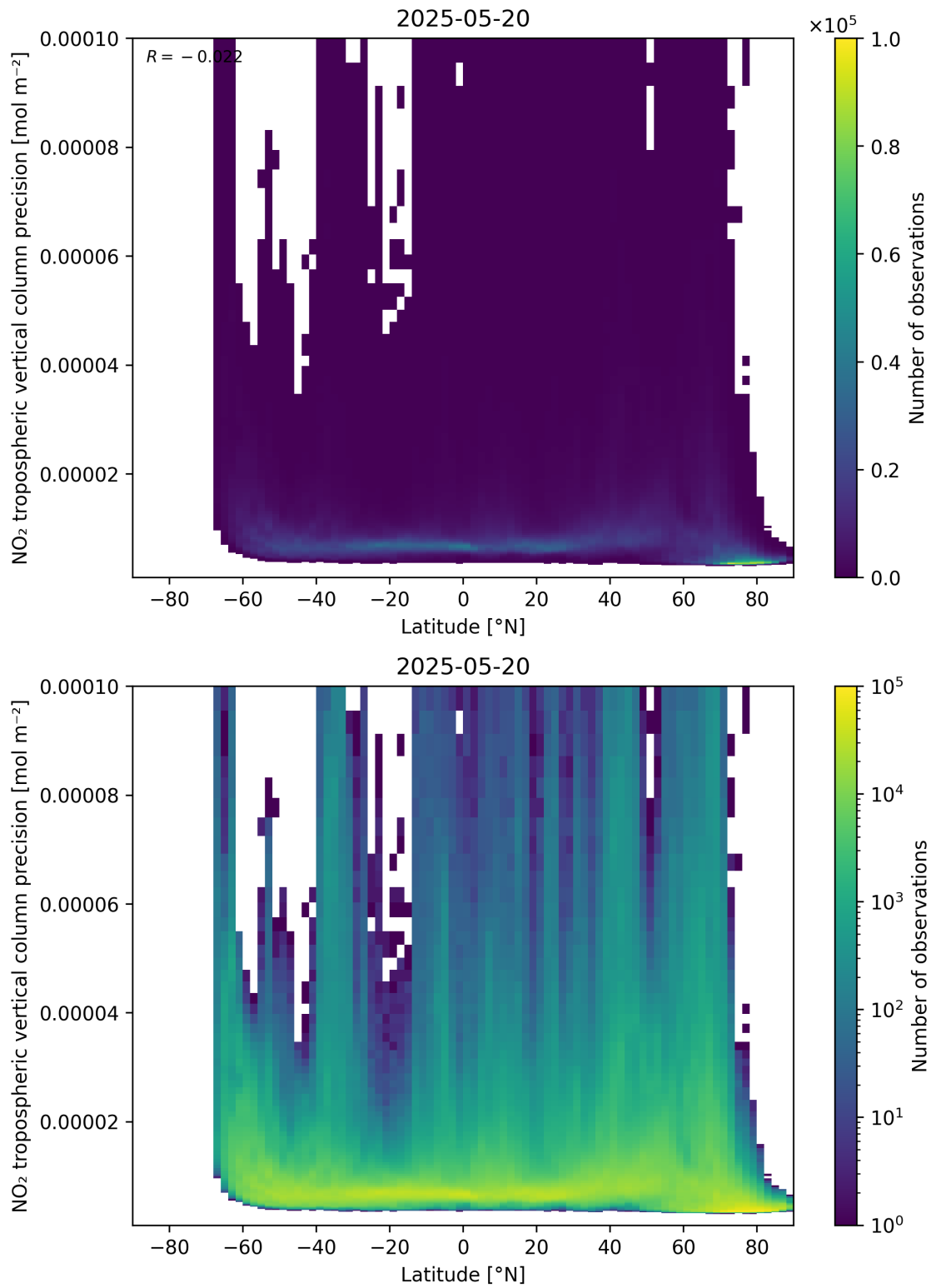
Figure 93: Scatter density plot of “Latitude” against “NO 2 tropospheric vertical column precision” for 2025-05-19 to 2025-05-21.
