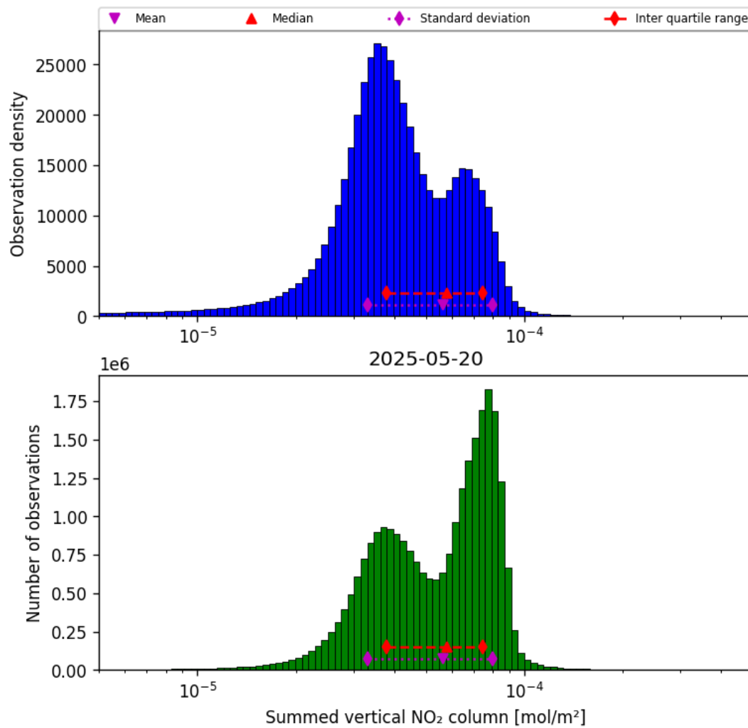
Figure 40: Histogram of “Summed vertical NO 2 column” for 2025-05-19 to 2025-05-21
