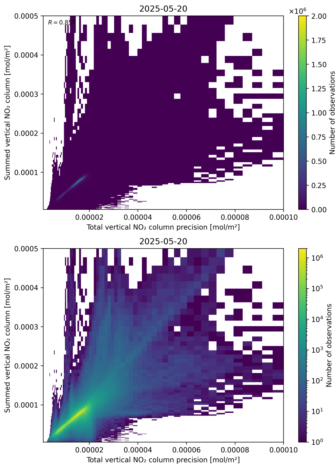
Figure 117: Scatter density plot of “Total vertical NO 2 column precision” against “Summed vertical NO 2 column” for 2025-05-19 to 2025-05-21.
