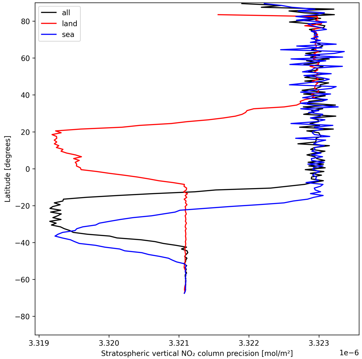
Figure 20: Zonal average of “Stratospheric vertical NO 2 column precision” for 2025-05-19 to 2025-05-21.
