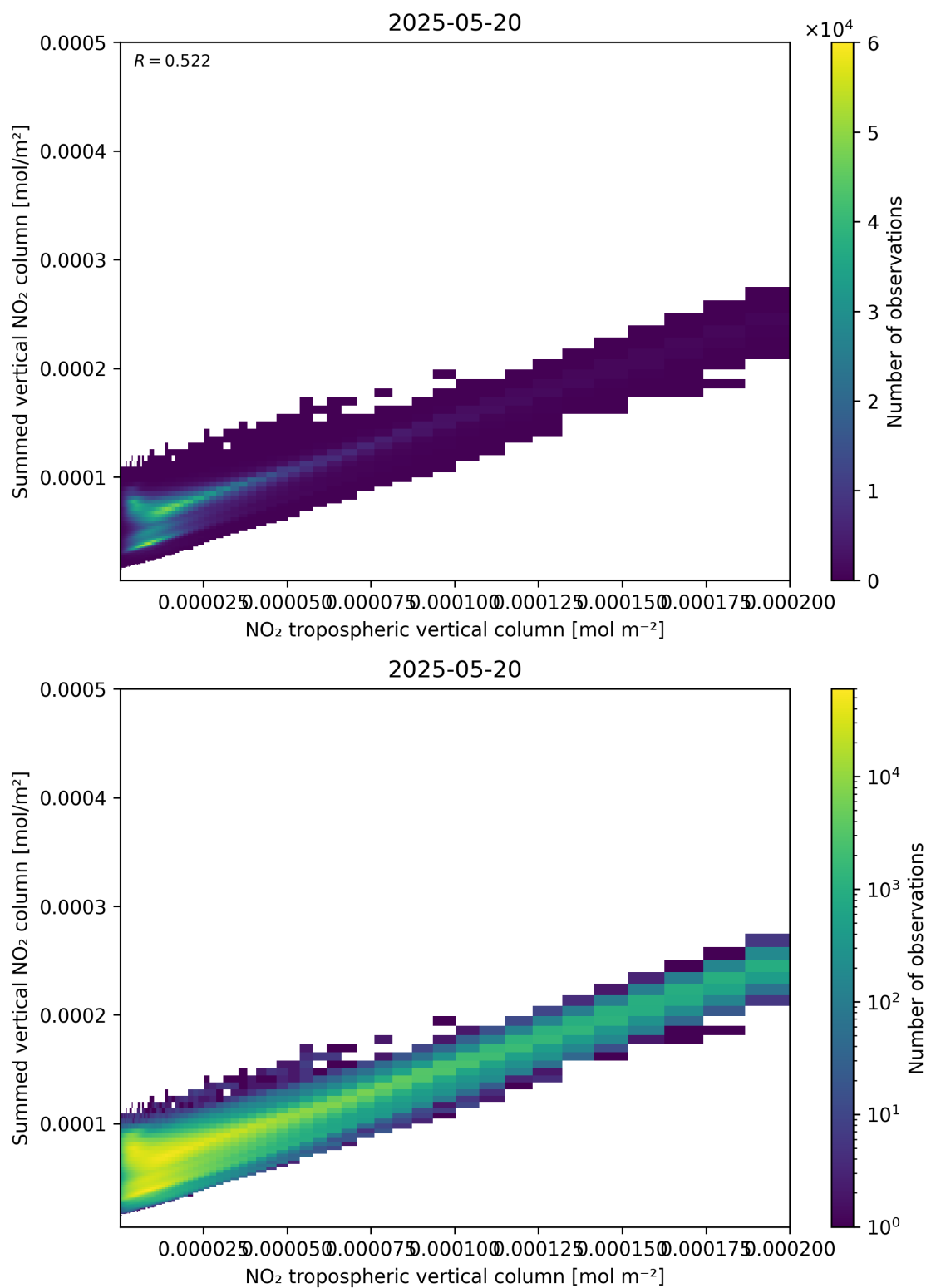
Figure 126: Scatter density plot of “NO 2 tropospheric vertical column” against “Summed vertical NO 2 column” for 2025-05-19 to 2025-05-21.
