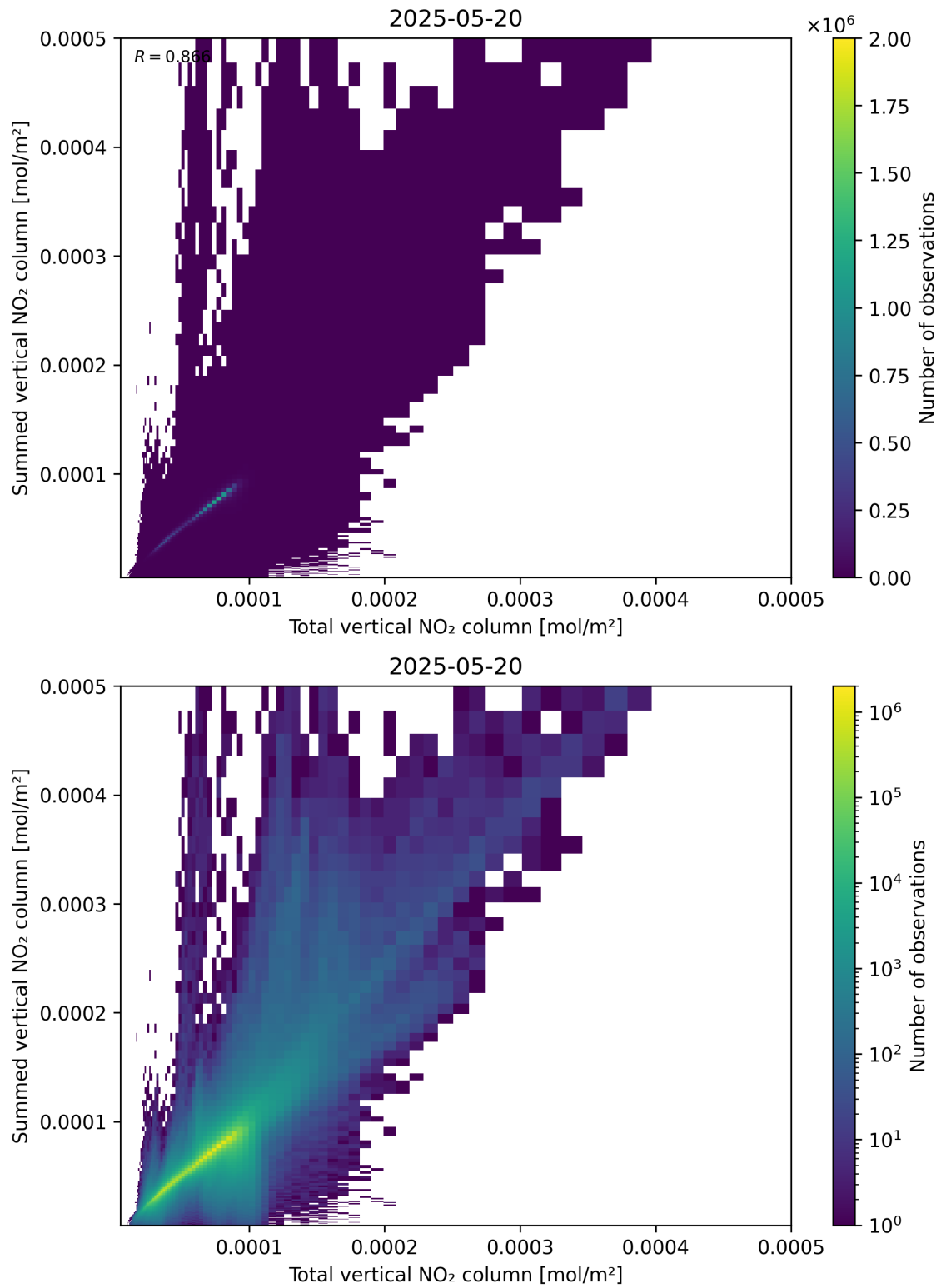
Figure 112: Scatter density plot of “Total vertical NO 2 column” against “Summed vertical NO 2 column” for 2025-05-19 to 2025-05-21.
