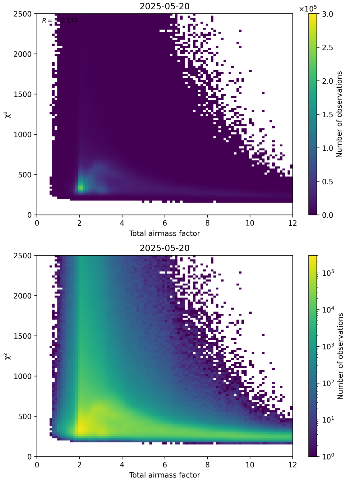
Figure 63: Scatter density plot of “Total airmass factor” against “ \chi^2 ” for 2025-05-19 to 2025-05-21.
