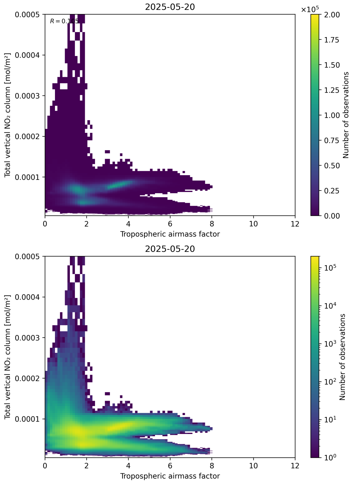
Figure 77: Scatter density plot of “Tropospheric airmass factor” against “Total vertical NO 2 column” for 2025-05-19 to 2025-05-21.
