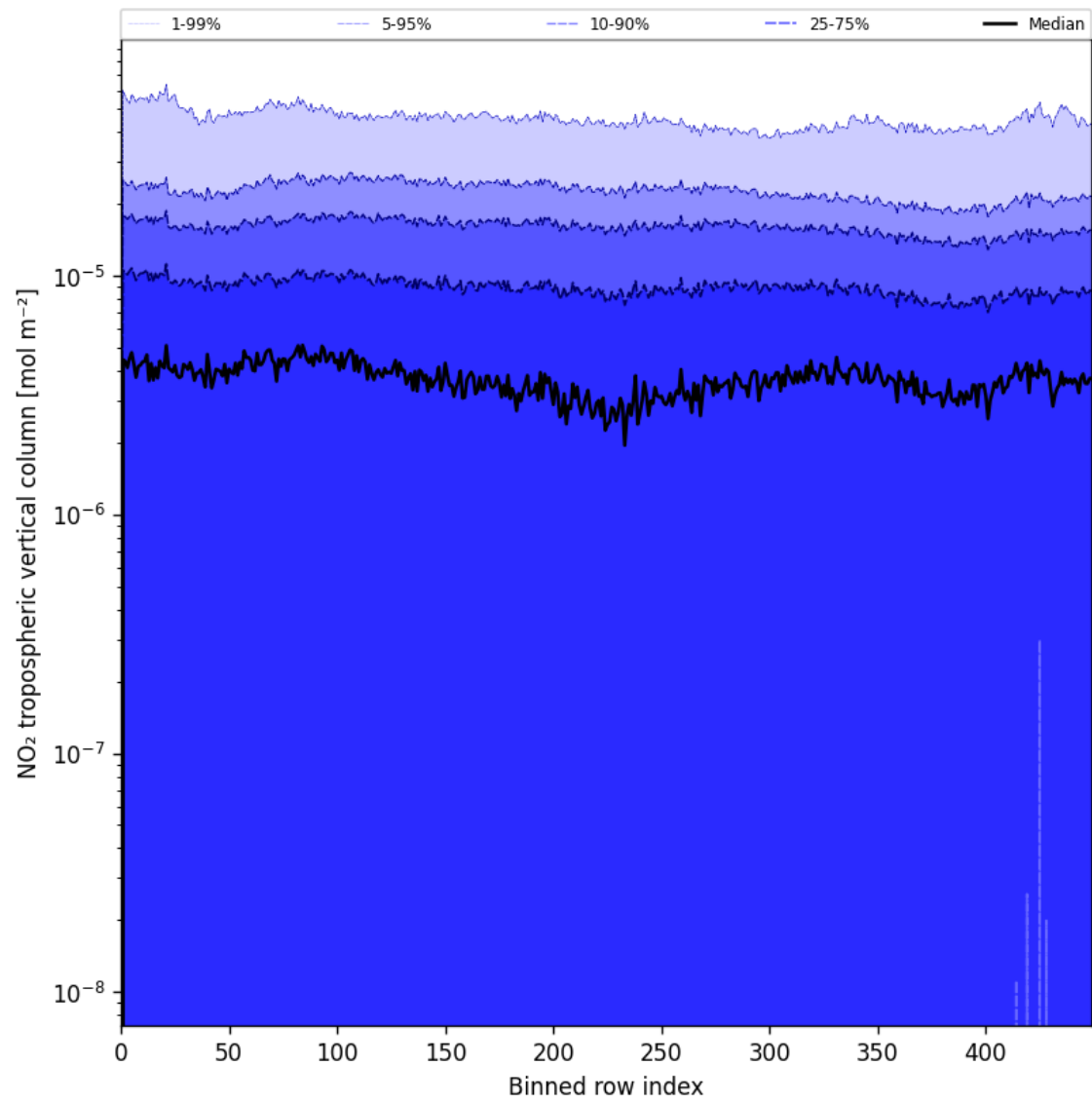
Figure 46: Along track statistics of “NO 2 tropospheric vertical column” for 2025-05-19 to 2025-05-21
