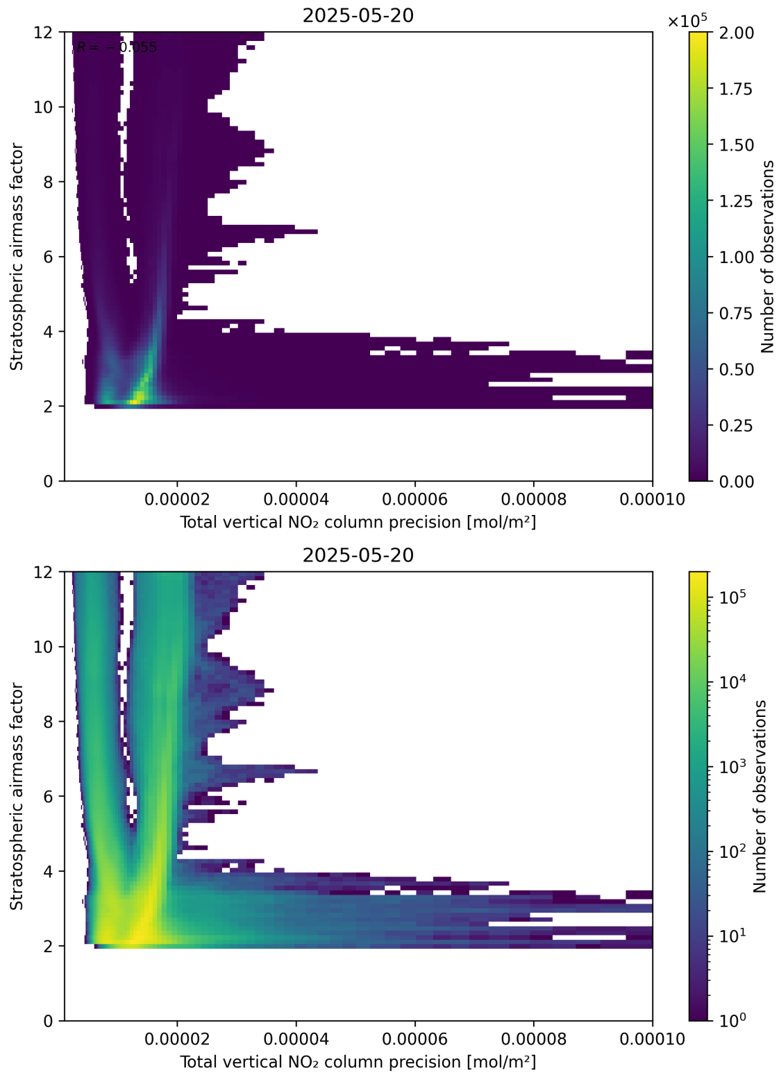
Figure 115: Scatter density plot of “Total vertical NO 2 column precision” against “Stratospheric air mass factor” for 2025-05-19 to 2025-05-21.
