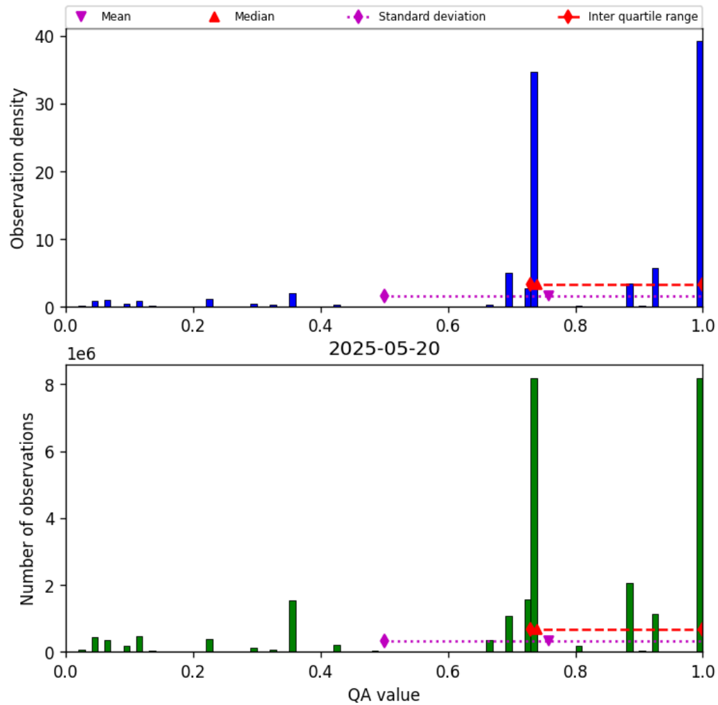
Figure 28: Histogram of “QA value” for 2025-05-19 to 2025-05-21
