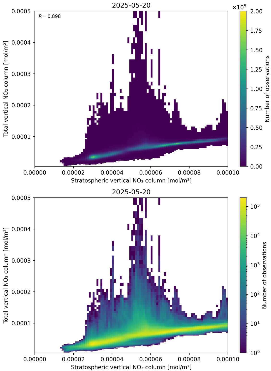
Figure 100: Scatter density plot of “Stratospheric vertical NO 2 column” against “Total vertical NO 2 column” for 2025-05-19 to 2025-05-21.
