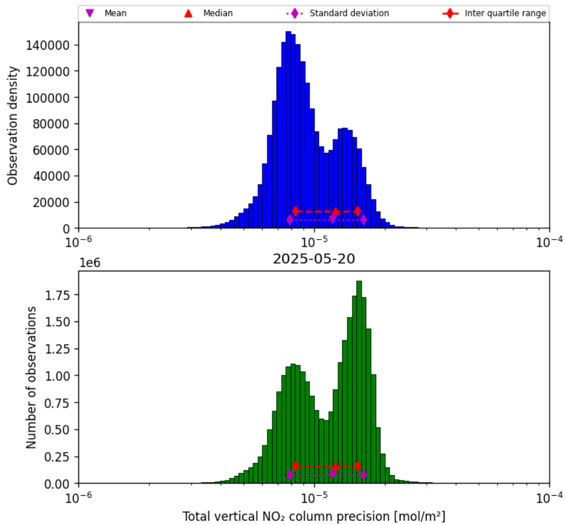
Figure 39: Histogram of “Total vertical NO 2 column precision” for 2025-05-19 to 2025-05-21
