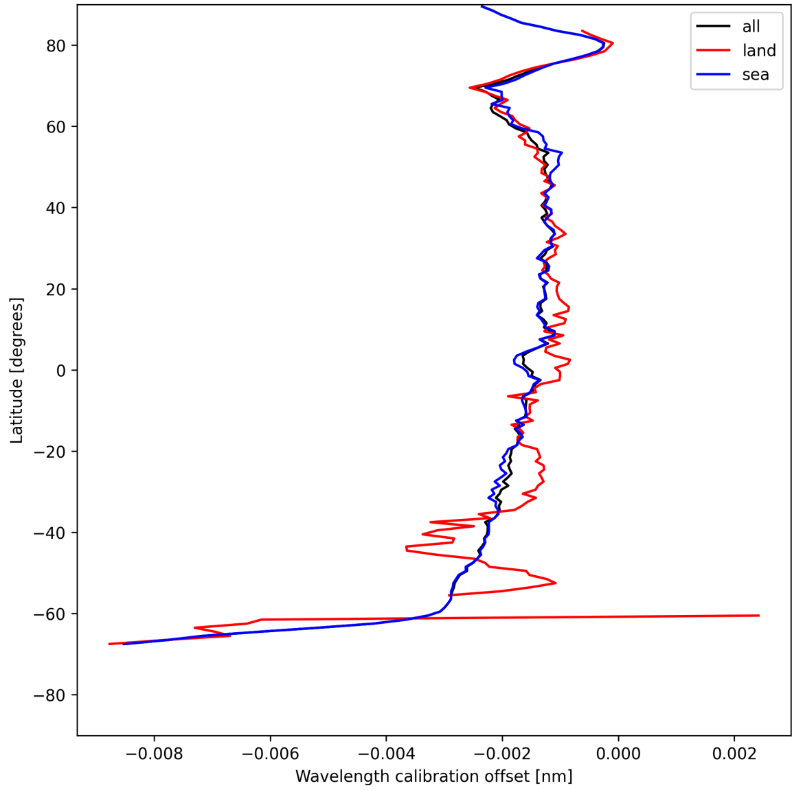
Figure 18: Zonal average of “Wavelength calibration offset” for 2025-05-19 to 2025-05-21.
