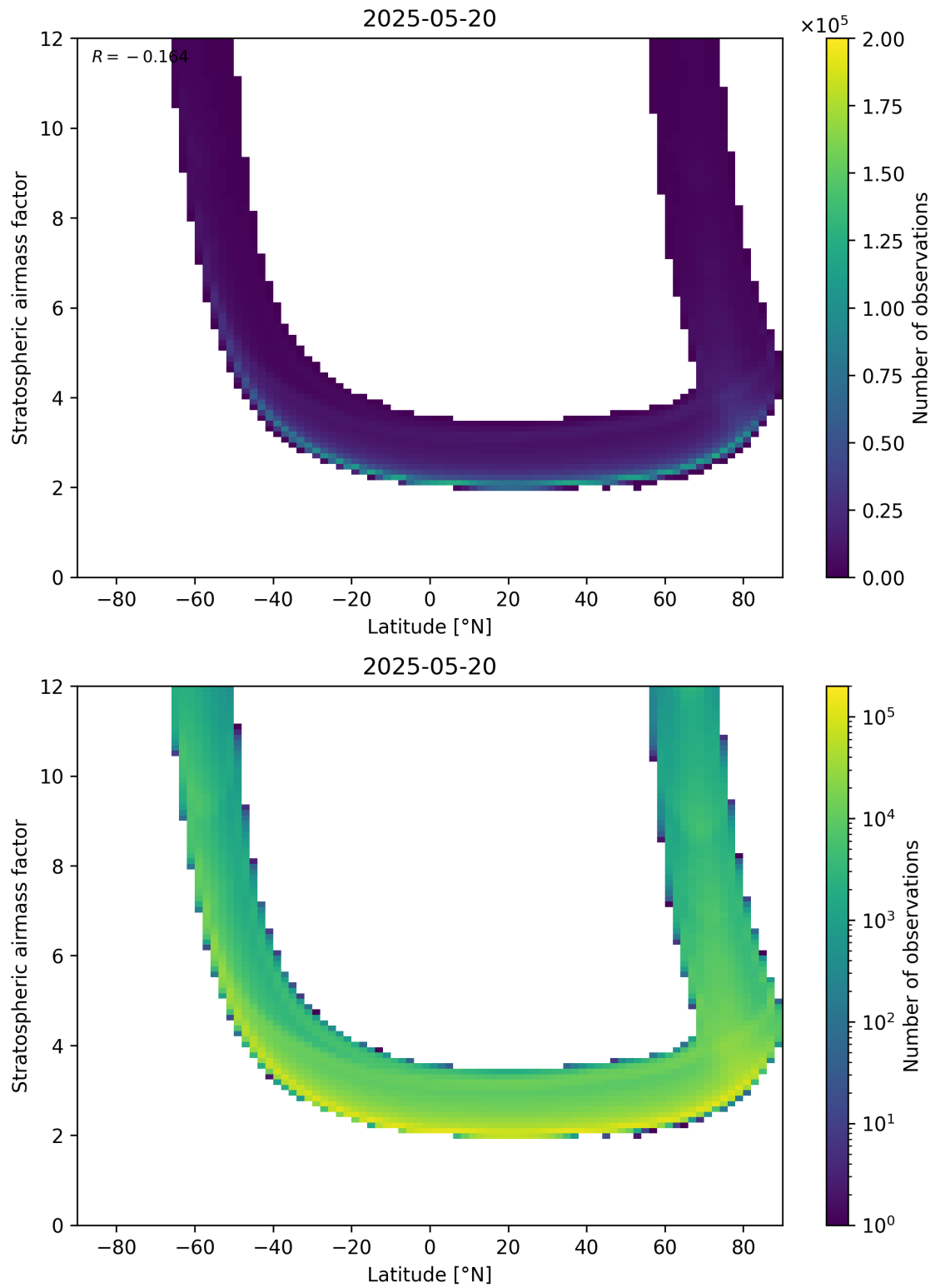
Figure 83: Scatter density plot of “Latitude” against “Stratospheric air mass factor” for 2025-05-19 to 2025-05-21.
