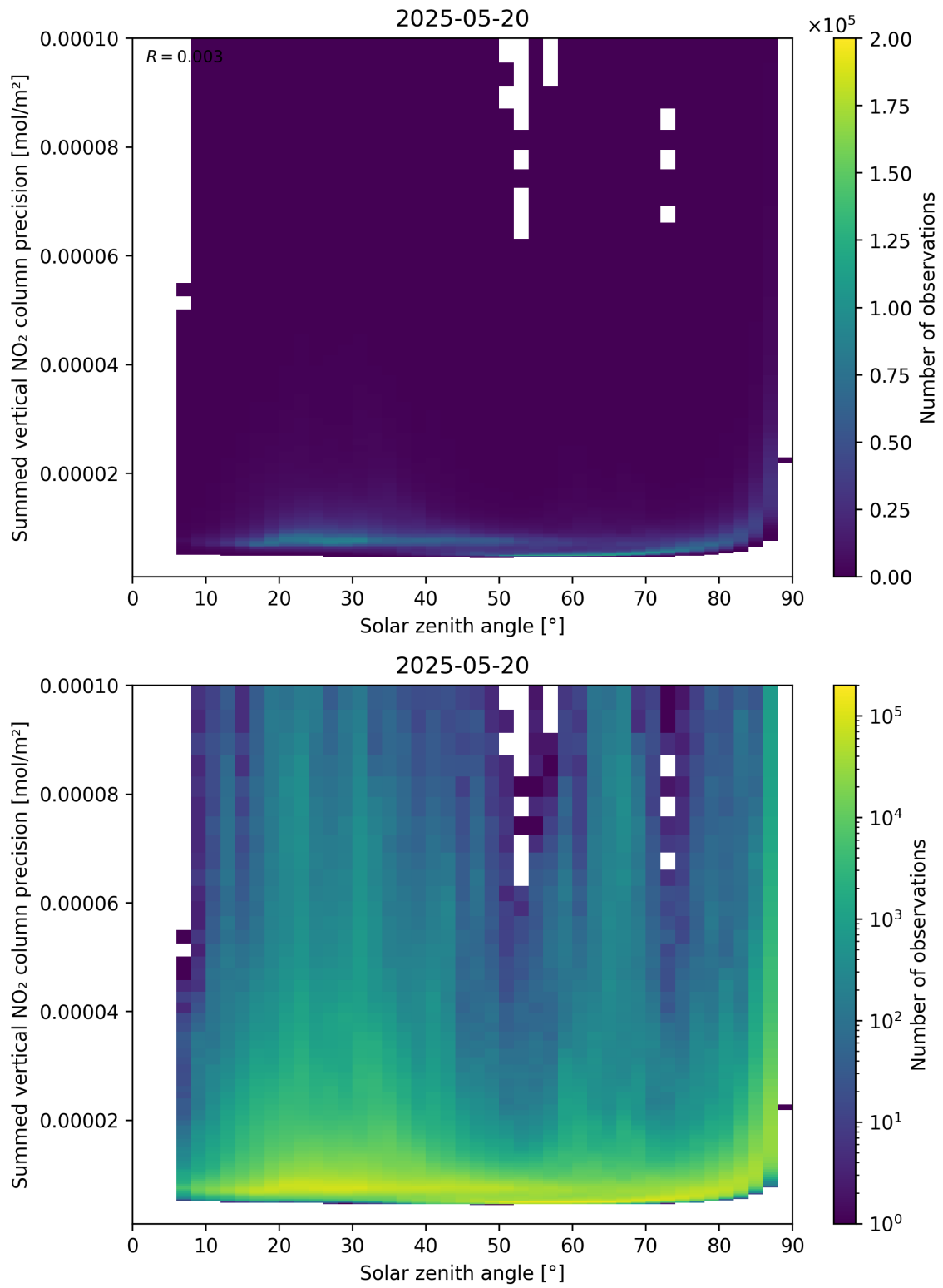
Figure 152: Scatter density plot of “Solar zenith angle” against “Summed vertical NO 2 column precision” for 2025-05-19 to 2025-05-21.
