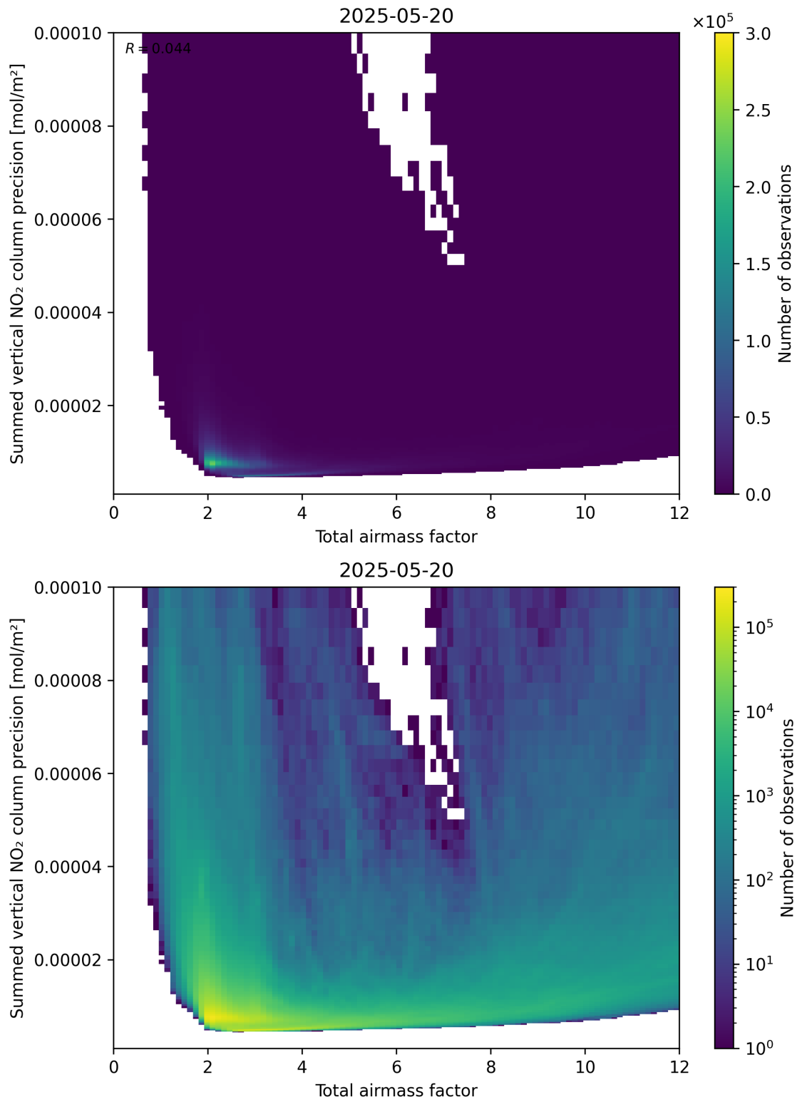
Figure 66: Scatter density plot of “Total airmass factor” against “Summed vertical NO 2 column precision” for 2025-05-19 to 2025-05-21.
