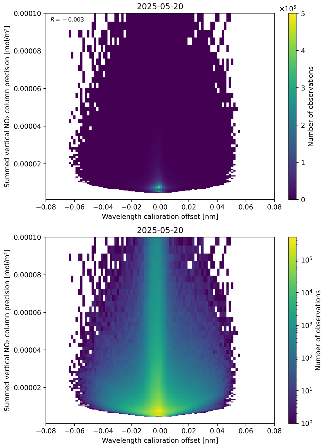
Figure 178: Scatter density plot of “Wavelength calibration offset” against “Summed vertical NO 2 column precision” for 2025-05-19 to 2025-05-21.
