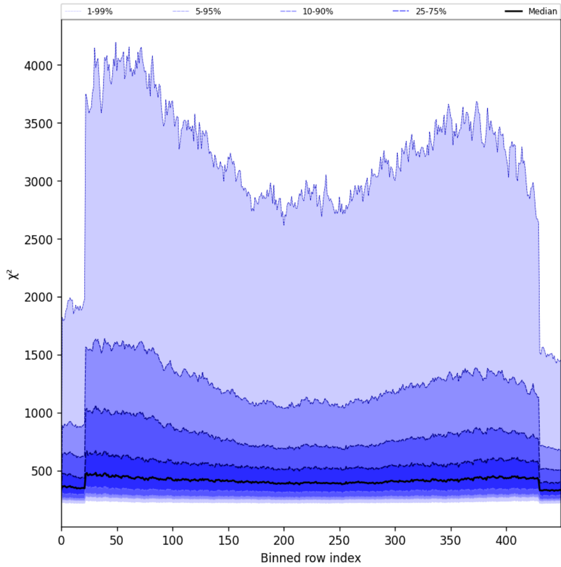
Figure 59: Along track statistics of “ \chi^2 ” for 2025-05-19 to 2025-05-21
