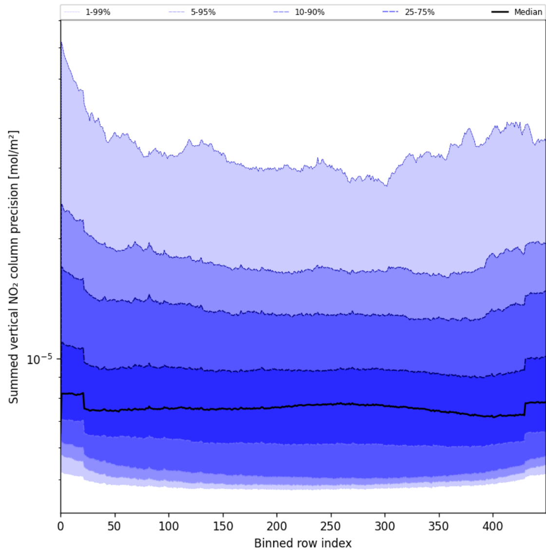
Figure 58: Along track statistics of “Summed vertical NO 2 column precision” for 2025-05-19 to 2025-05-21
