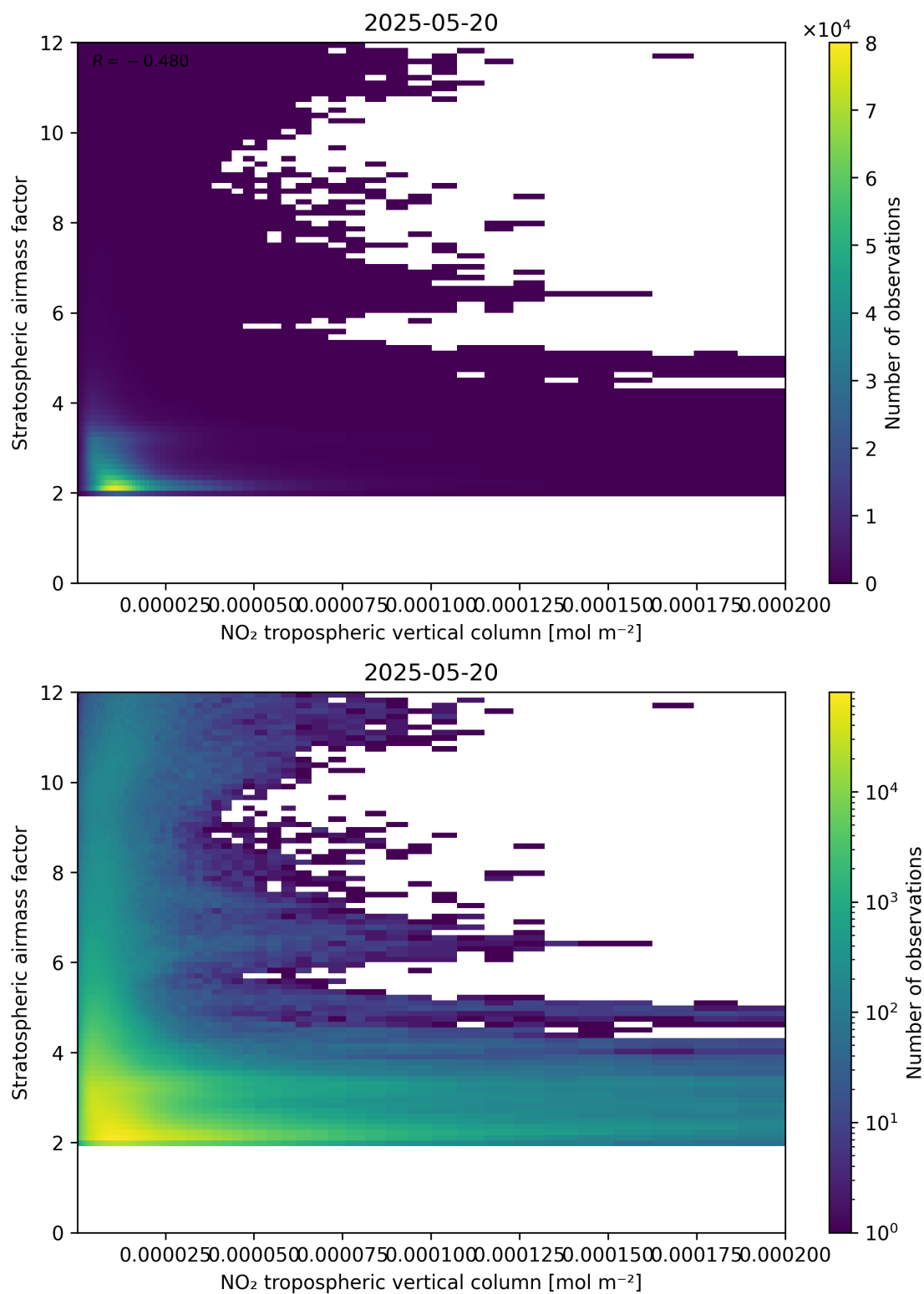
Figure 121: Scatter density plot of “NO 2 tropospheric vertical column” against “Stratospheric air mass factor” for 2025-05-19 to 2025-05-21.
