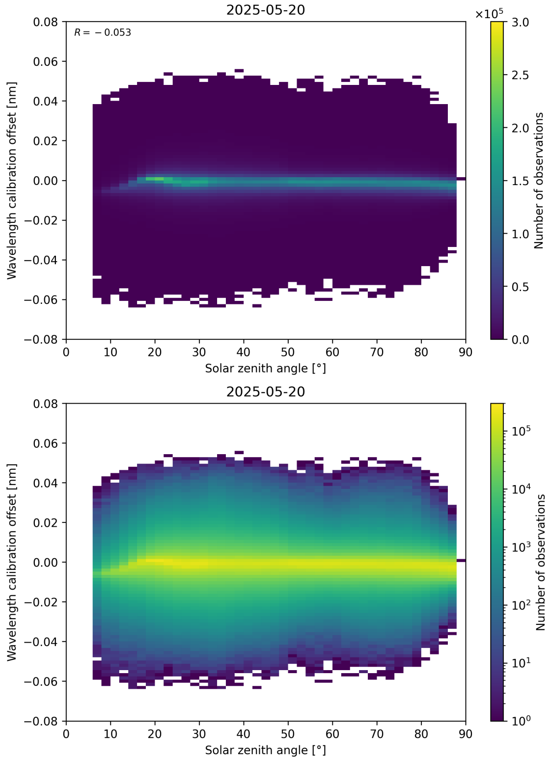
Figure 158: Scatter density plot of “Solar zenith angle” against “Wavelength calibration offset” for 2025-05-19 to 2025-05-21.
