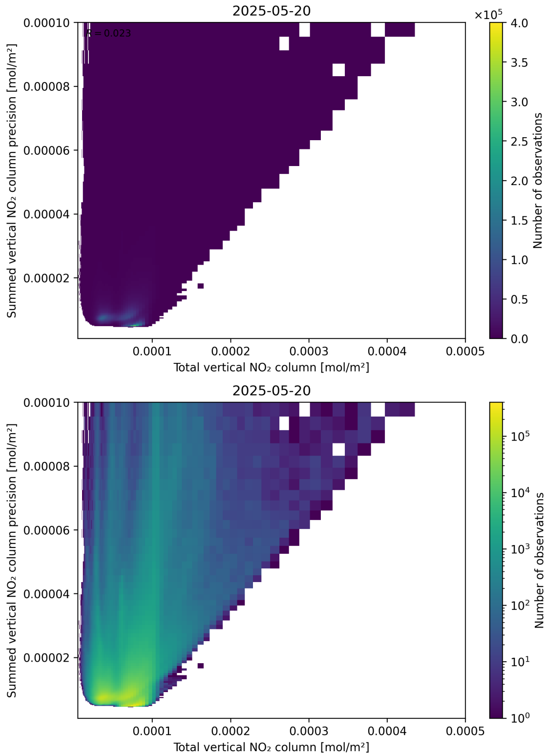
Figure 113: Scatter density plot of “Total vertical NO 2 column” against “Summed vertical NO 2 column precision” for 2025-05-19 to 2025-05-21.
