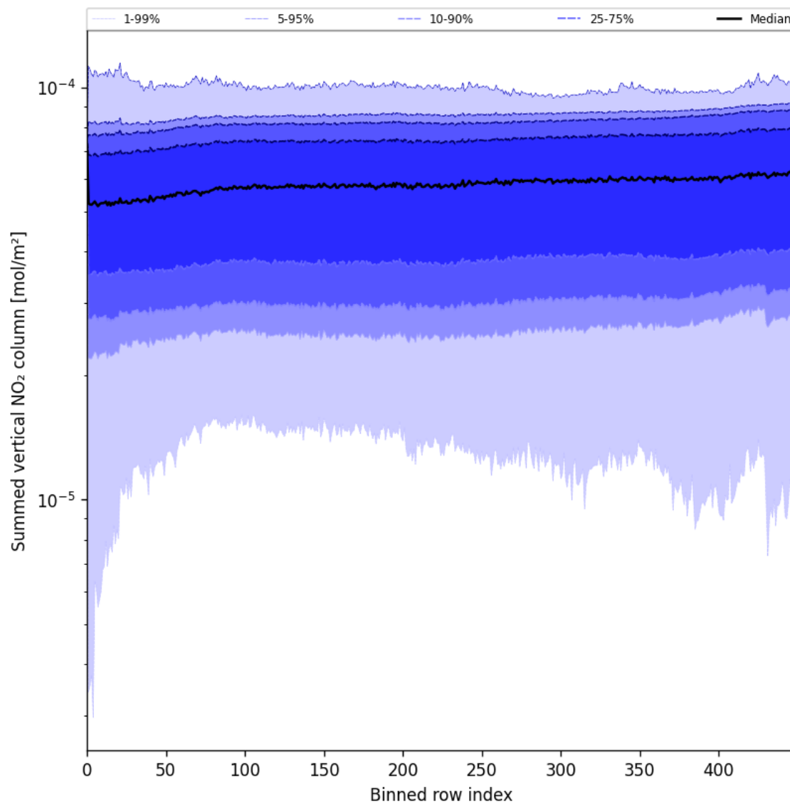
Figure 57: Along track statistics of “Summed vertical NO 2 column” for 2025-05-19 to 2025-05-21
