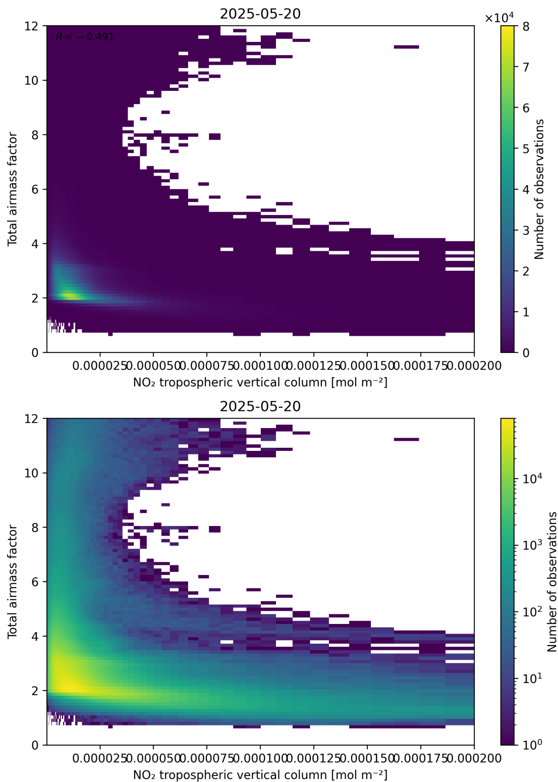
Figure 122: Scatter density plot of “NO 2 tropospheric vertical column” against “Total air mass factor” for 2025-05-19 to 2025-05-21.
