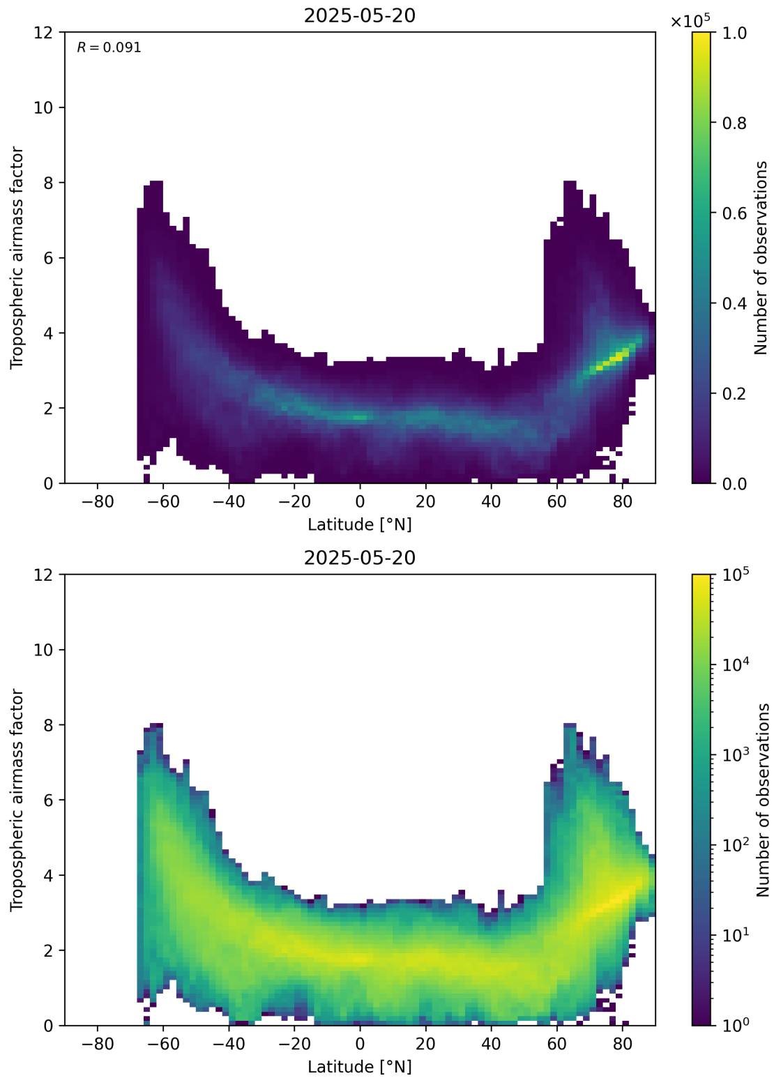
Figure 85: Scatter density plot of “Latitude” against “Tropospheric air mass factor” for 2025-05-19 to 2025-05-21.
