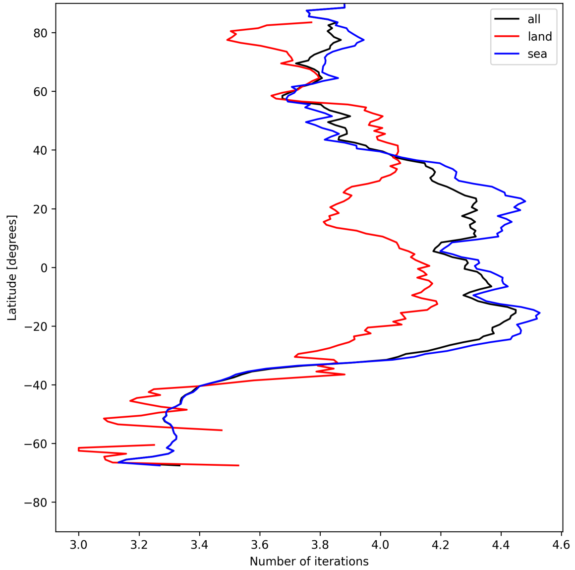
Figure 17: Zonal average of “Number of iterations” for 2025-05-19 to 2025-05-21.
