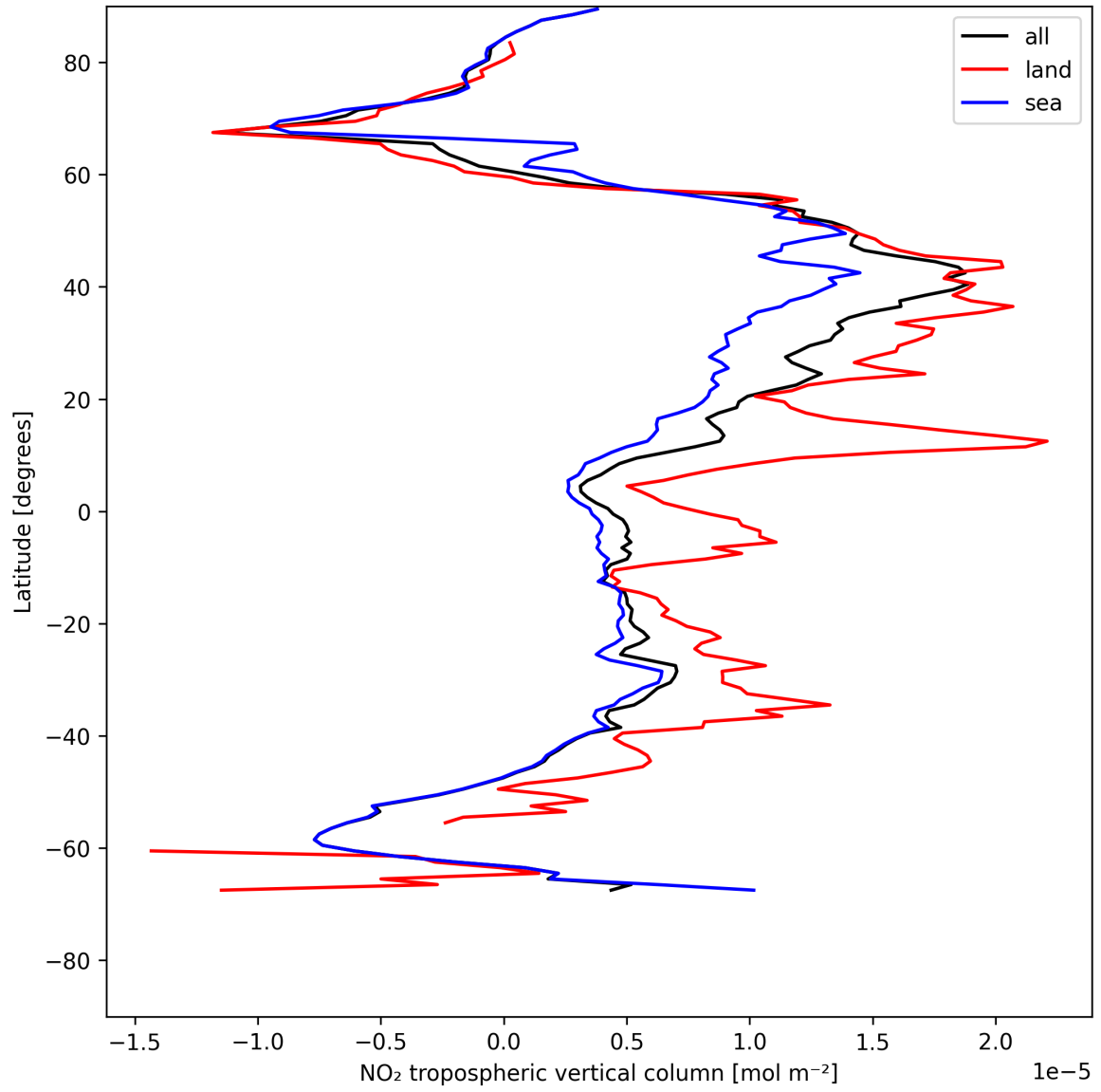
Figure 12: Zonal average of “NO 2 tropospheric vertical column” for 2025-05-19 to 2025-05-21.
