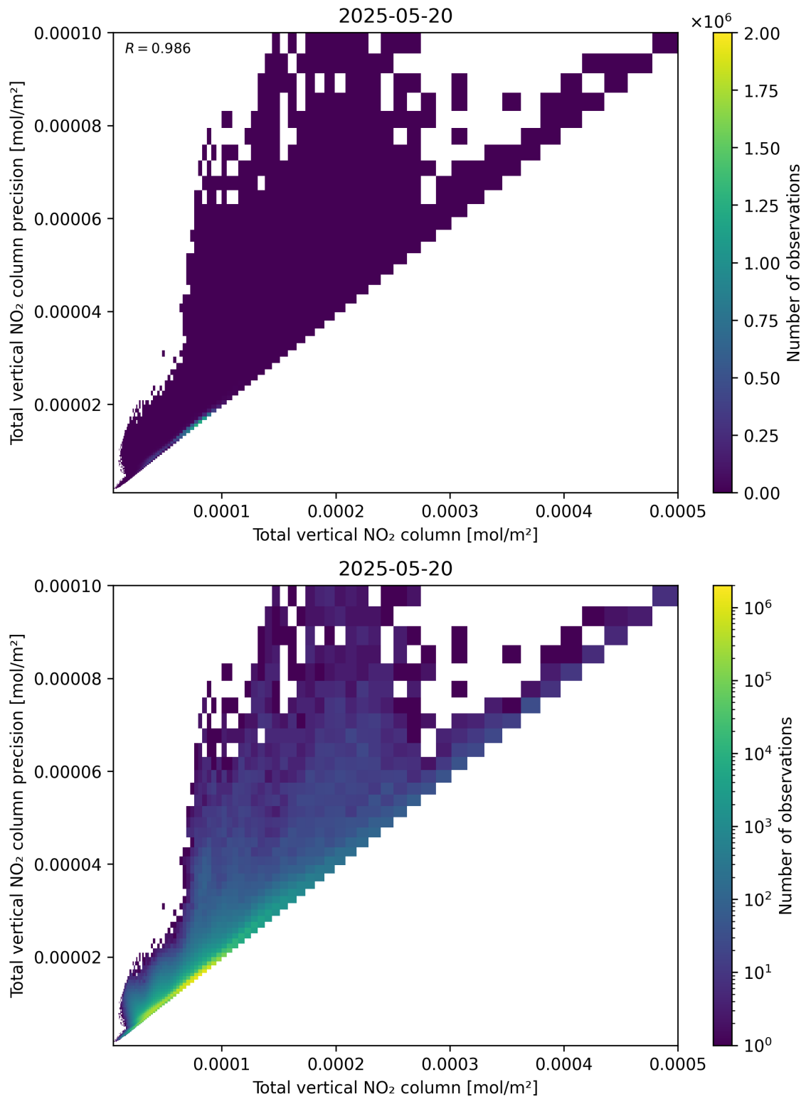
Figure 114: Scatter density plot of “Total vertical NO 2 column” against “Total vertical NO 2 column precision” for 2025-05-19 to 2025-05-21.
