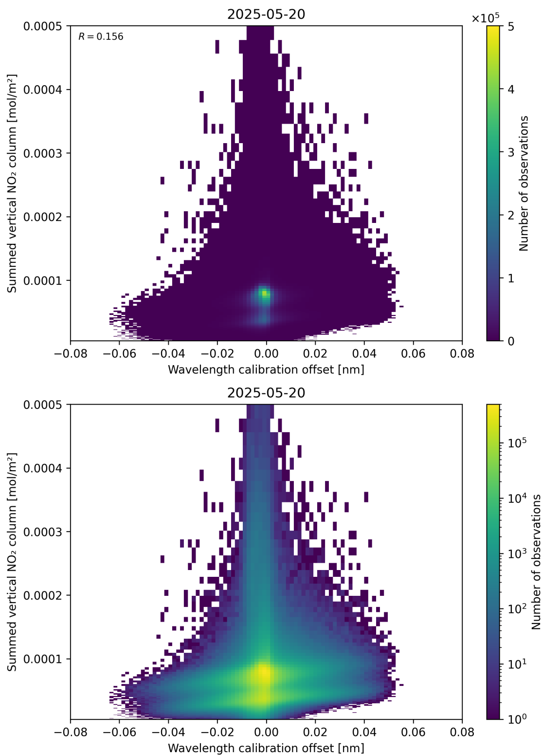
Figure 177: Scatter density plot of “Wavelength calibration offset” against “Summed vertical NO 2 column” for 2025-05-19 to 2025-05-21.
