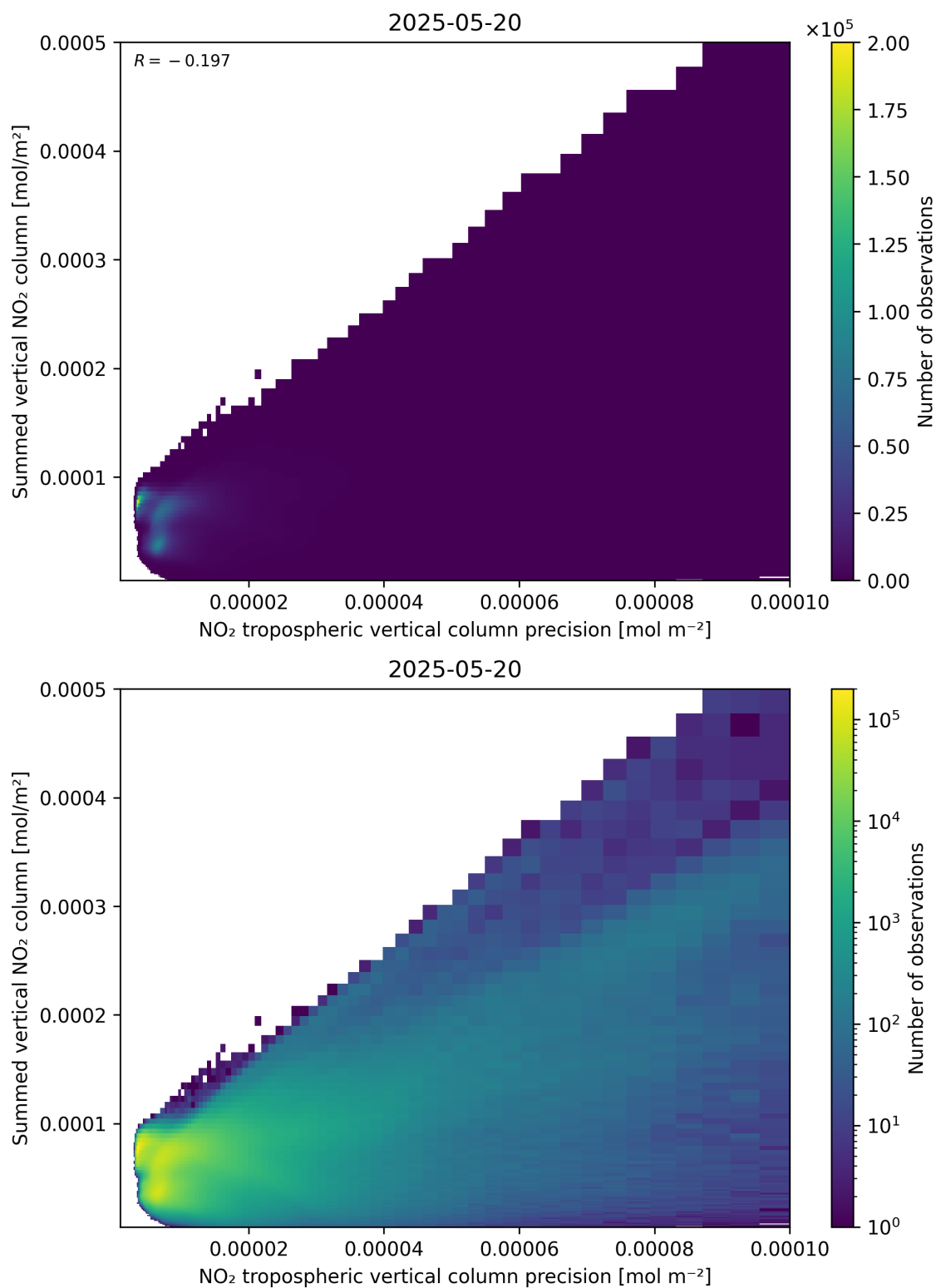
Figure 136: Scatter density plot of “NO 2 tropospheric vertical column precision” against “Summed vertical NO 2 column” for 2025-05-19 to 2025-05-21.
