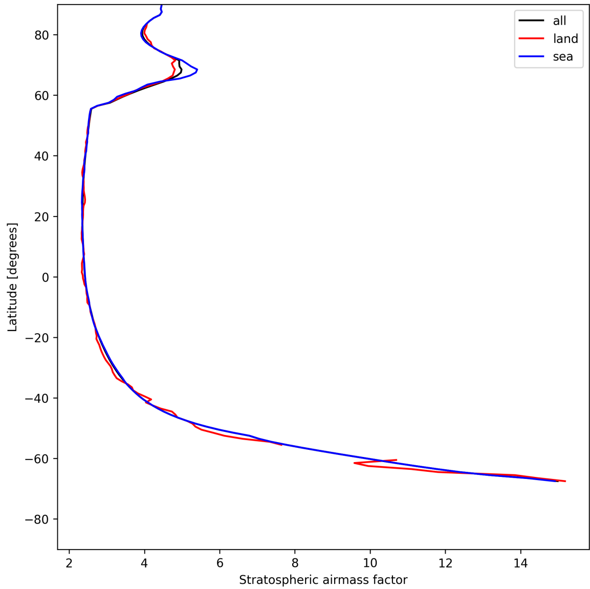
Figure 27: Zonal average of “Stratospheric airmass factor” for 2025-05-19 to 2025-05-21.
