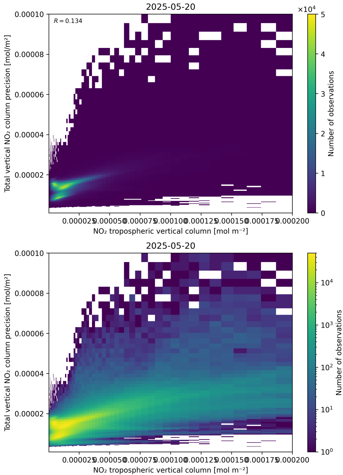
Figure 129: Scatter density plot of “NO 2 tropospheric vertical column” against “Total vertical NO 2 column precision” for 2025-05-19 to 2025-05-21.
