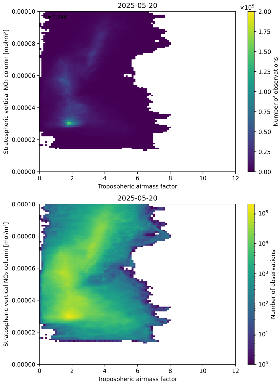
Figure 74: Scatter density plot of “Tropospheric air mass factor” against “Stratospheric vertical NO 2 column” for 2025-05-19 to 2025-05-21.
