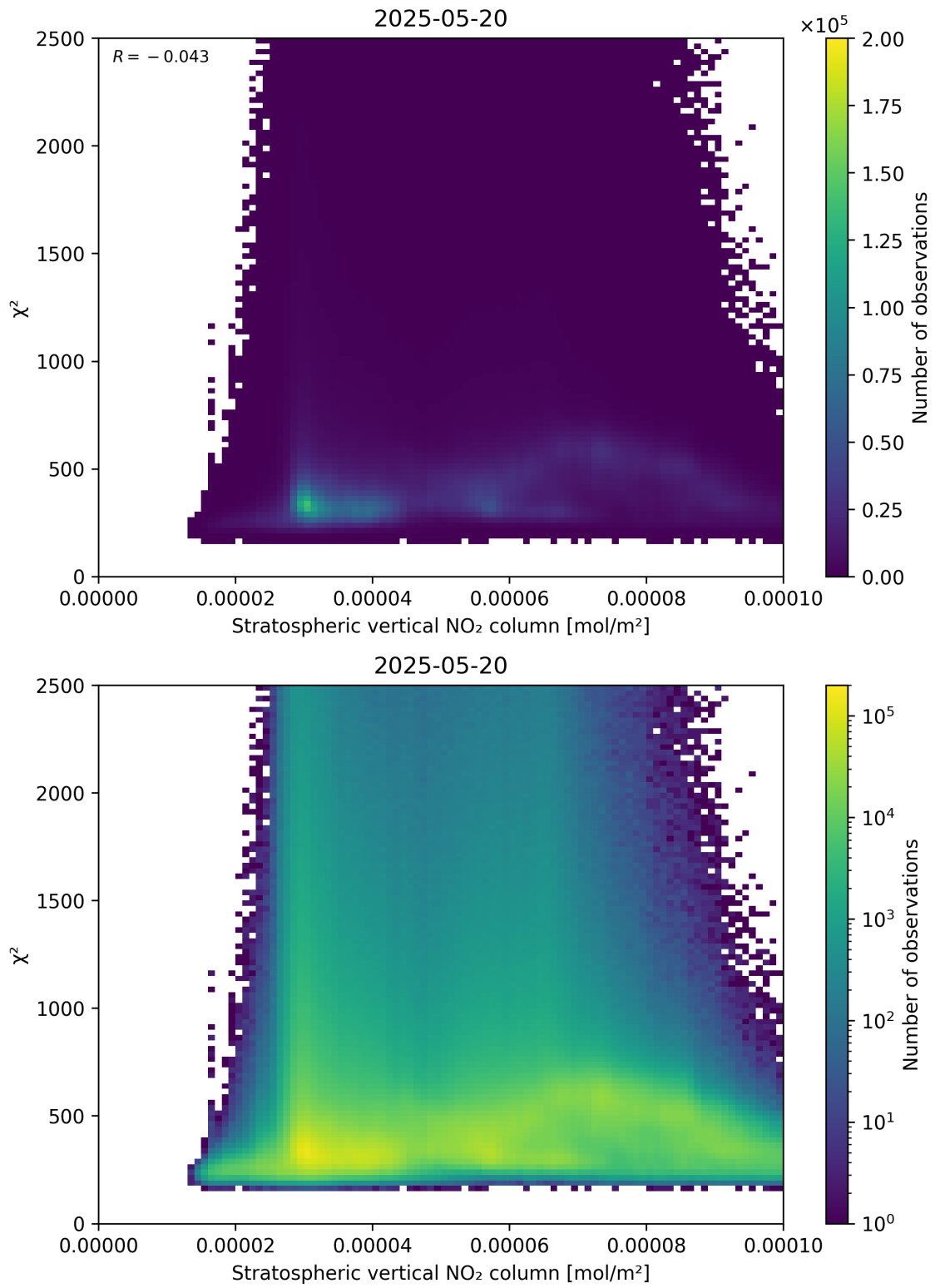
Figure 97: Scatter density plot of “Stratospheric vertical NO 2 column” against “ \chi^2 ” for 2025-05-19 to 2025-05-21.
