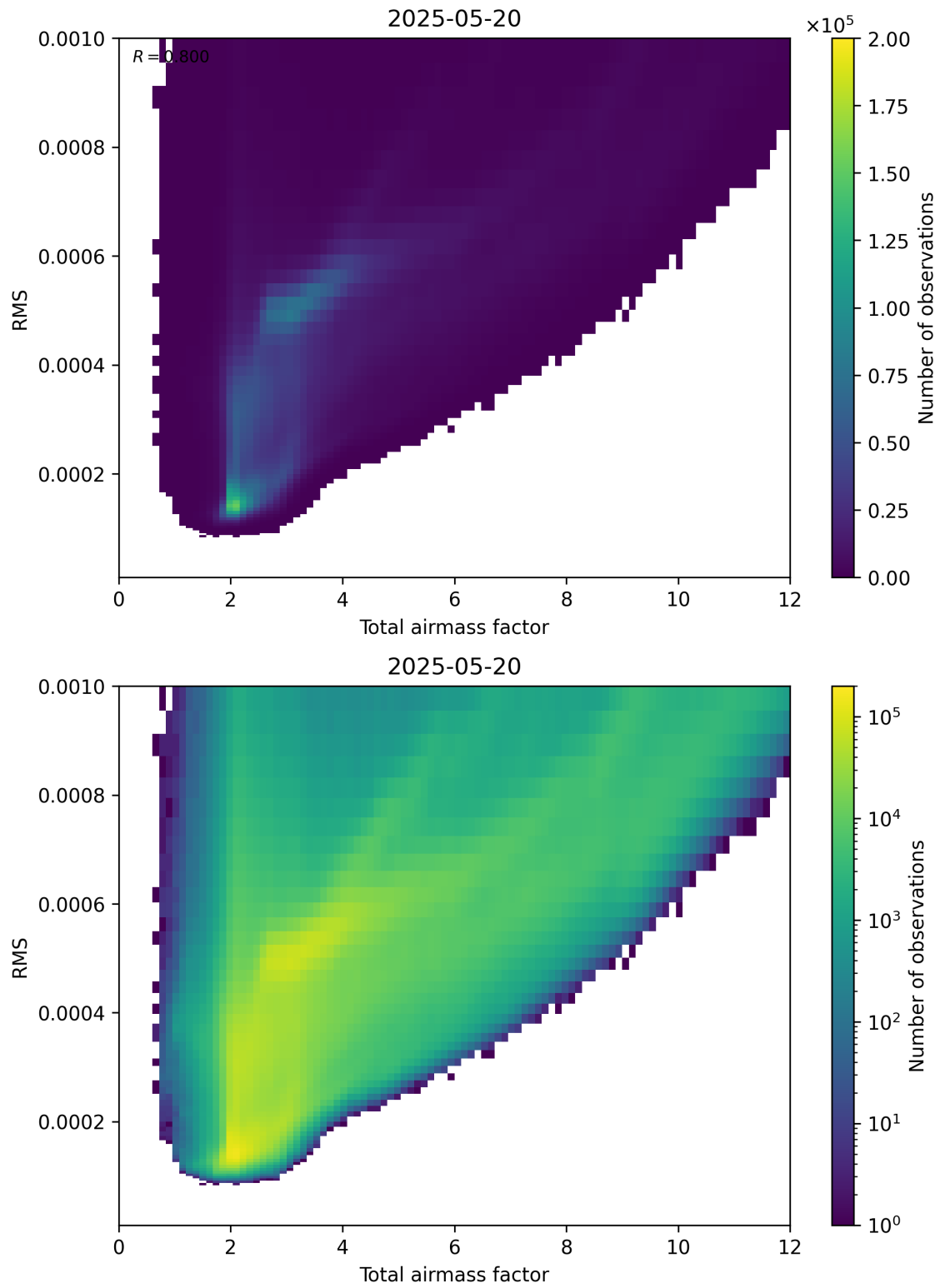
Figure 69: Scatter density plot of “Total airmass factor” against “RMS” for 2025-05-19 to 2025-05-21.
