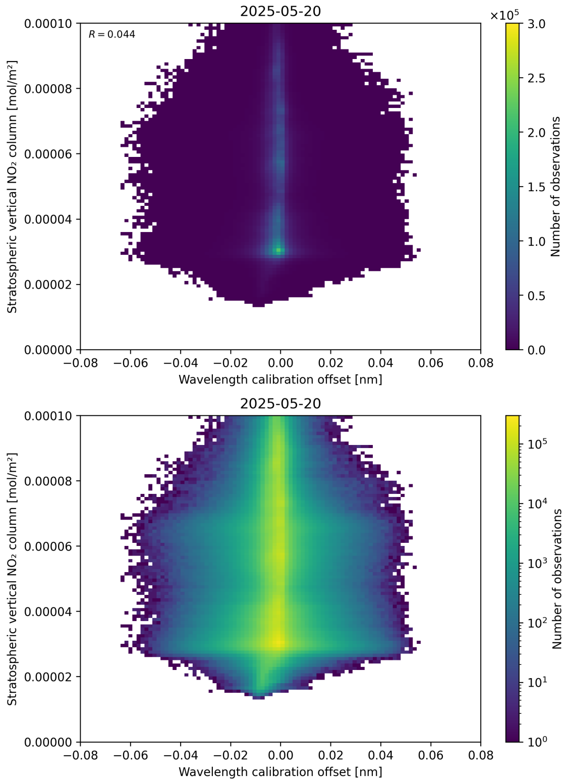
Figure 176: Scatter density plot of “Wavelength calibration offset” against “Stratospheric vertical NO 2 column” for 2025-05-19 to 2025-05-21.
