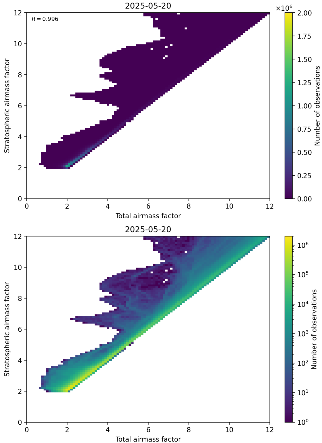
Figure 62: Scatter density plot of “Total airmass factor” against “Stratospheric airmass factor” for 2025-05-19 to 2025-05-21.
