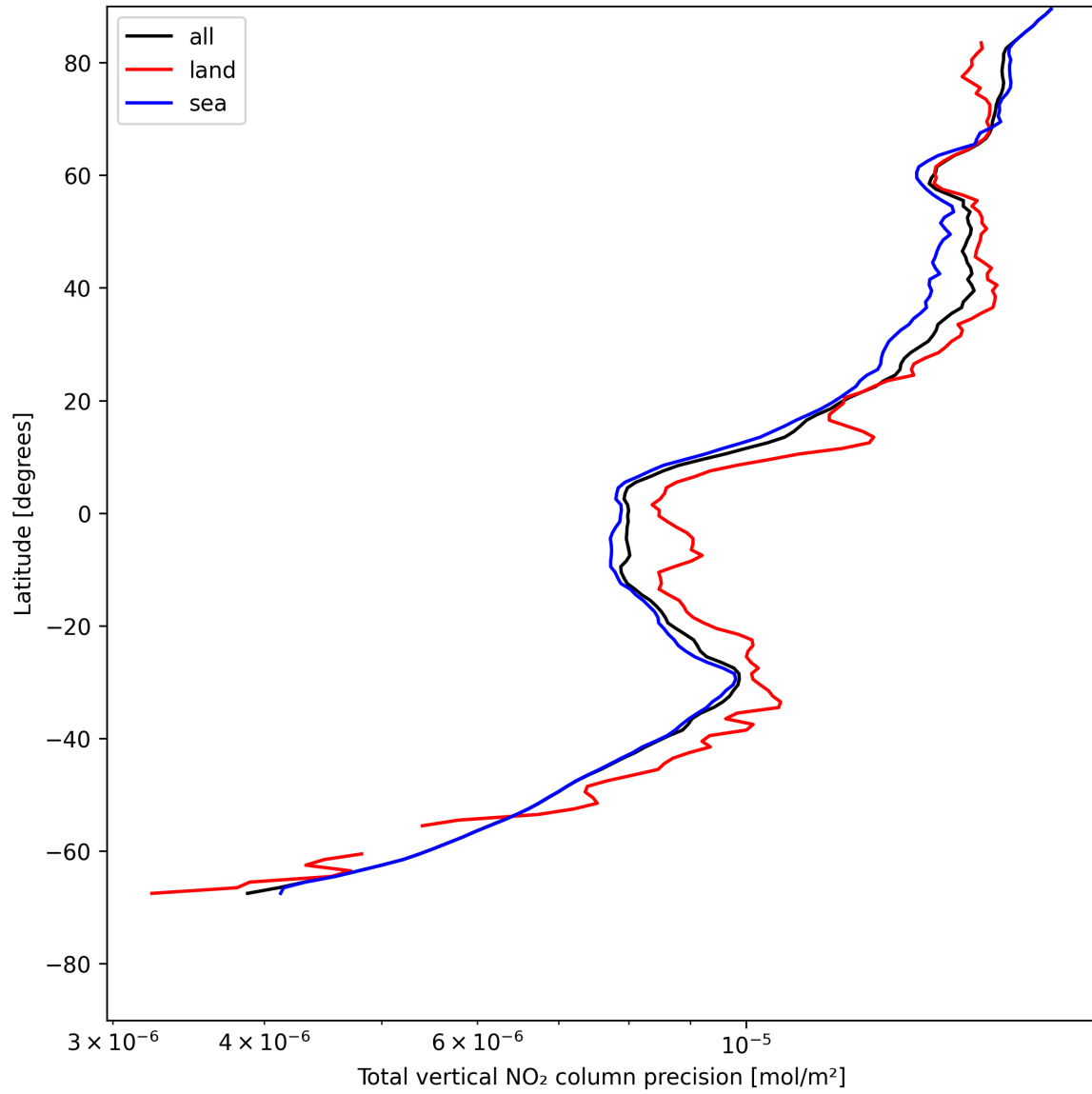
Figure 22: Zonal average of “Total vertical NO 2 column precision” for 2025-05-19 to 2025-05-21.
