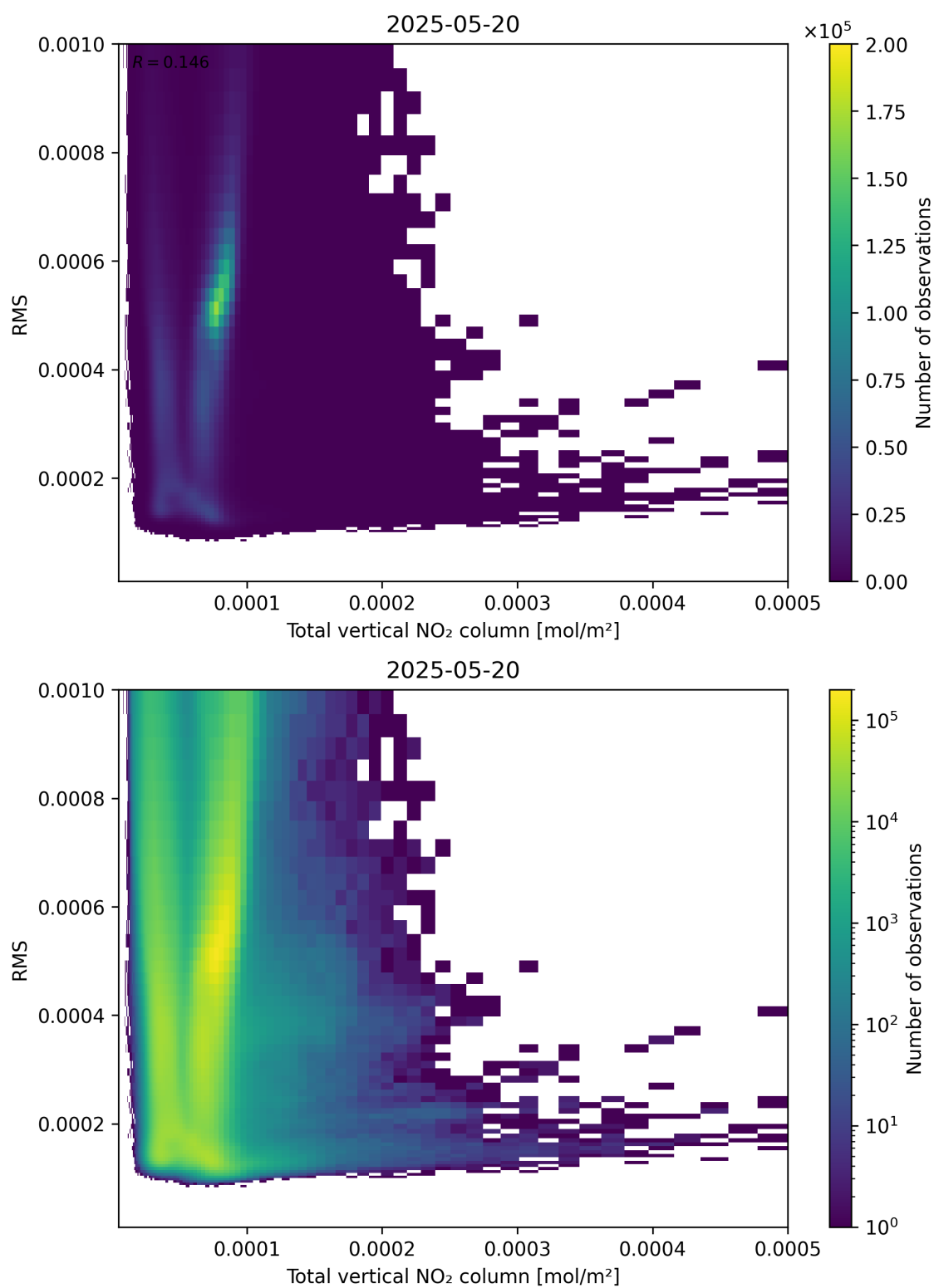
Figure 120: Scatter density plot of “Total vertical NO 2 column” against “RMS” for 2025-05-19 to 2025-05-21.
