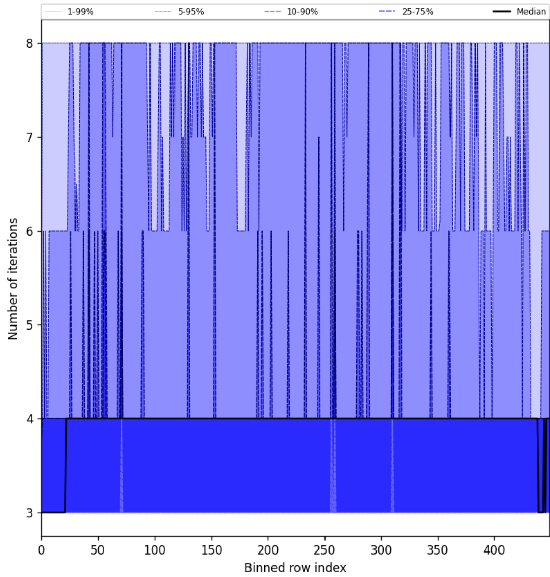
Figure 51: Along track statistics of “Number of iterations” for 2025-05-19 to 2025-05-21
