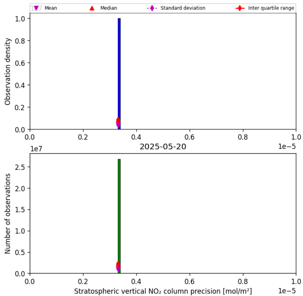
Figure 37: Histogram of “Stratospheric vertical NO 2 column precision” for 2025-05-19 to 2025-05-21
