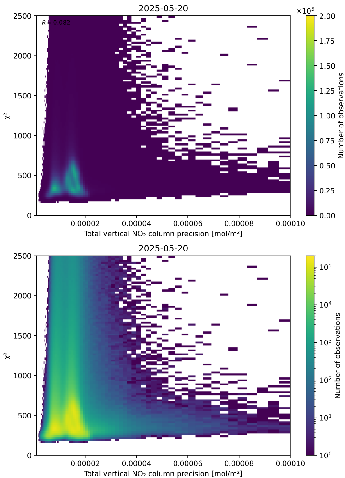
Figure 116: Scatter density plot of “Total vertical NO 2 column precision” against “ \chi^2 ” for 2025-05-19 to 2025-05-21.
