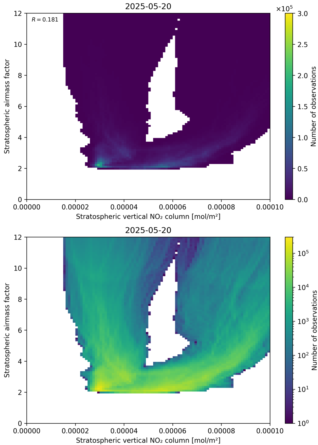
Figure 96: Scatter density plot of “Stratospheric vertical NO 2 column” against “Stratospheric airmass factor” for 2025-05-19 to 2025-05-21.
