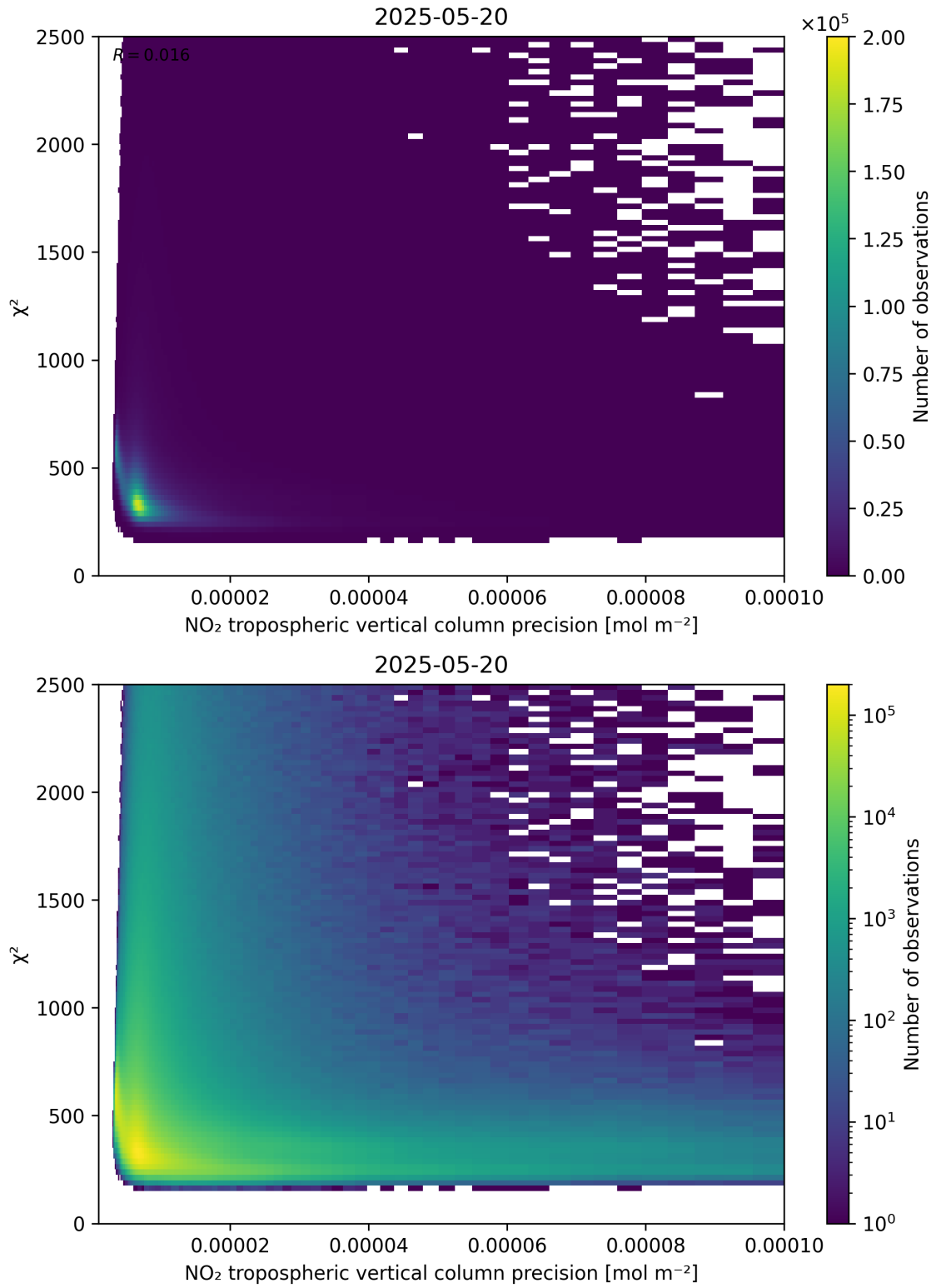
Figure 134: Scatter density plot of “NO 2 tropospheric vertical column precision” against “ \chi^2 ” for 2025-05-19 to 2025-05-21.
