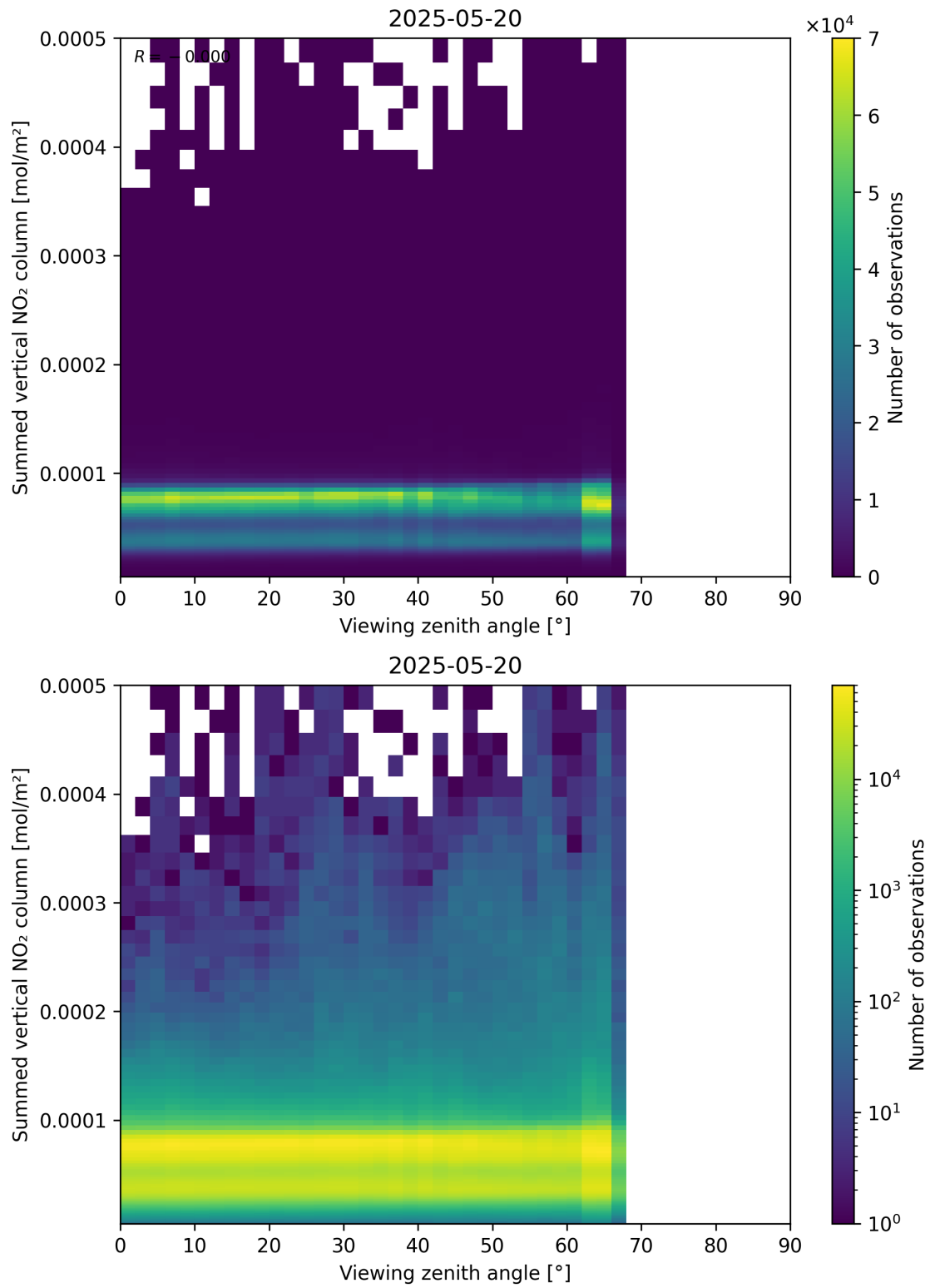
Figure 165: Scatter density plot of “Viewing zenith angle” against “Summed vertical NO 2 column” for 2025-05-19 to 2025-05-21.
