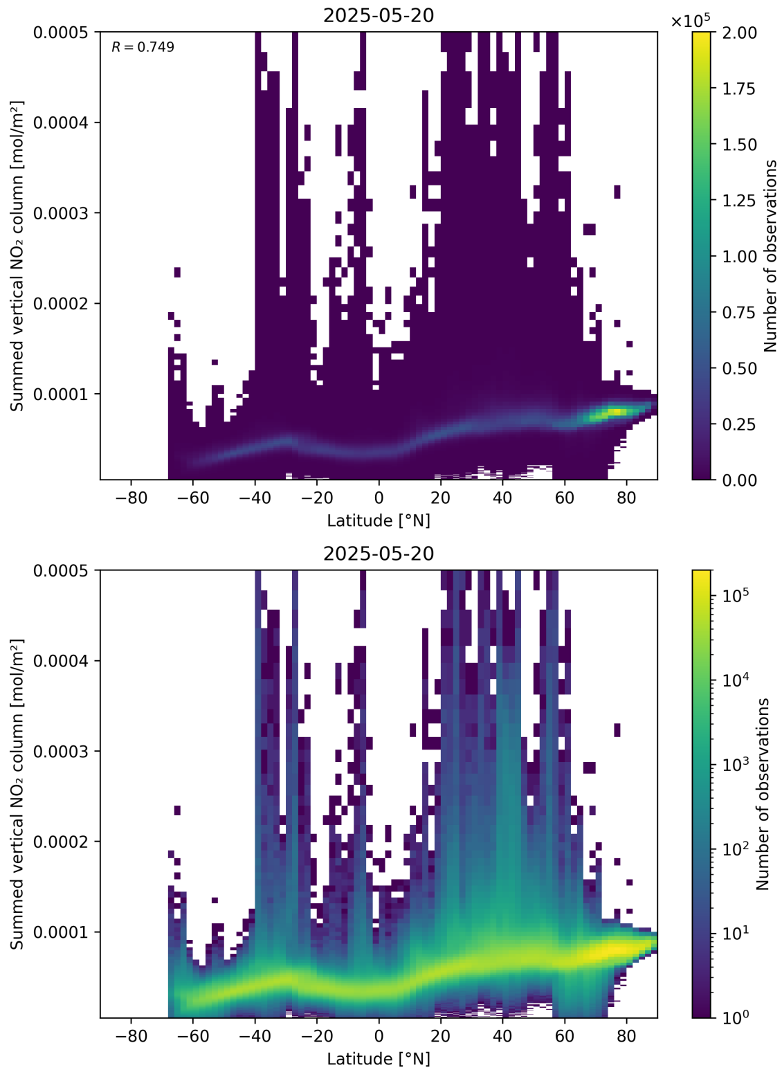
Figure 88: Scatter density plot of “Latitude” against “Summed vertical NO 2 column” for 2025-05-19 to 2025-05-21.
