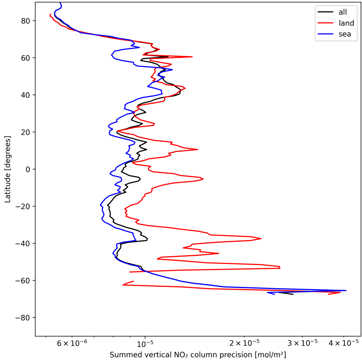
Figure 24: Zonal average of “Summed vertical NO 2 column precision” for 2025-05-19 to 2025-05-21.
