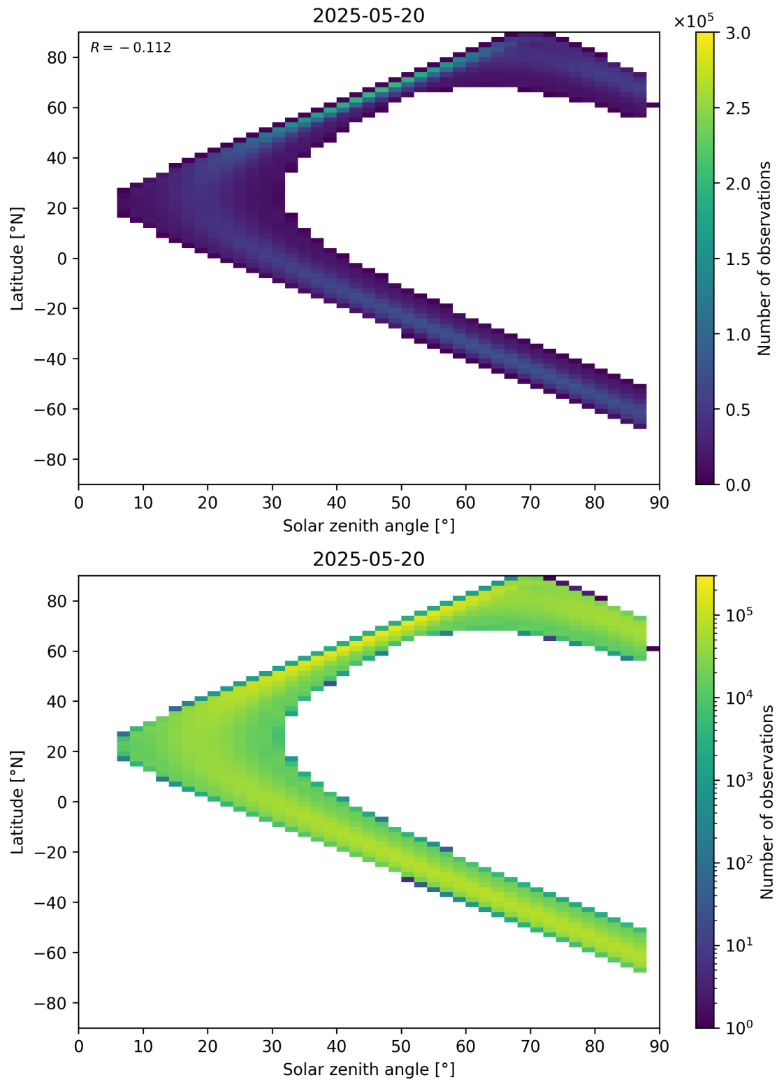
Figure 149: Scatter density plot of “Solar zenith angle” against “Latitude” for 2025-05-19 to 2025-05-21.
