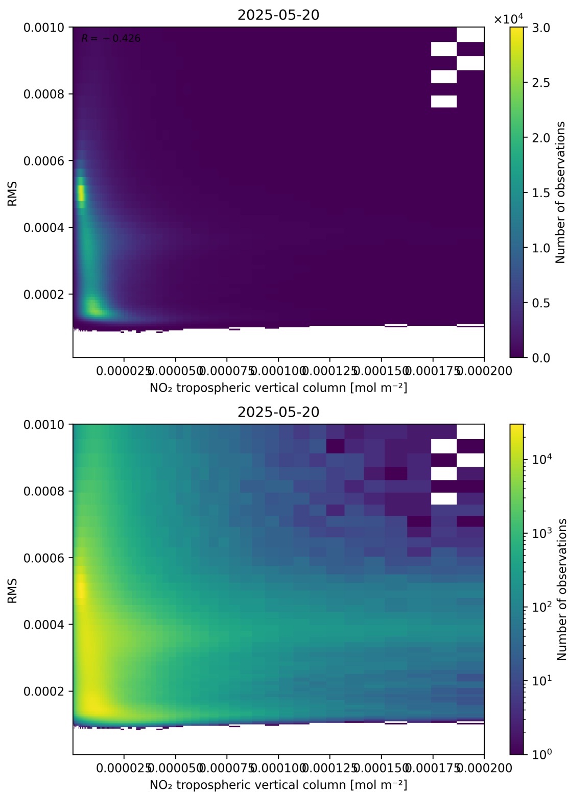
Figure 142: Scatter density plot of “NO 2 tropospheric vertical column” against “RMS” for 2025-05-19 to 2025-05-21.
