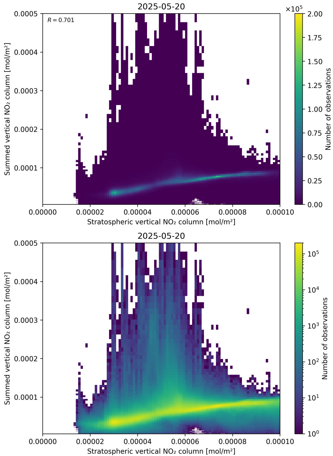
Figure 98: Scatter density plot of “Stratospheric vertical NO 2 column” against “Summed vertical NO 2 column” for 2025-05-19 to 2025-05-21.
