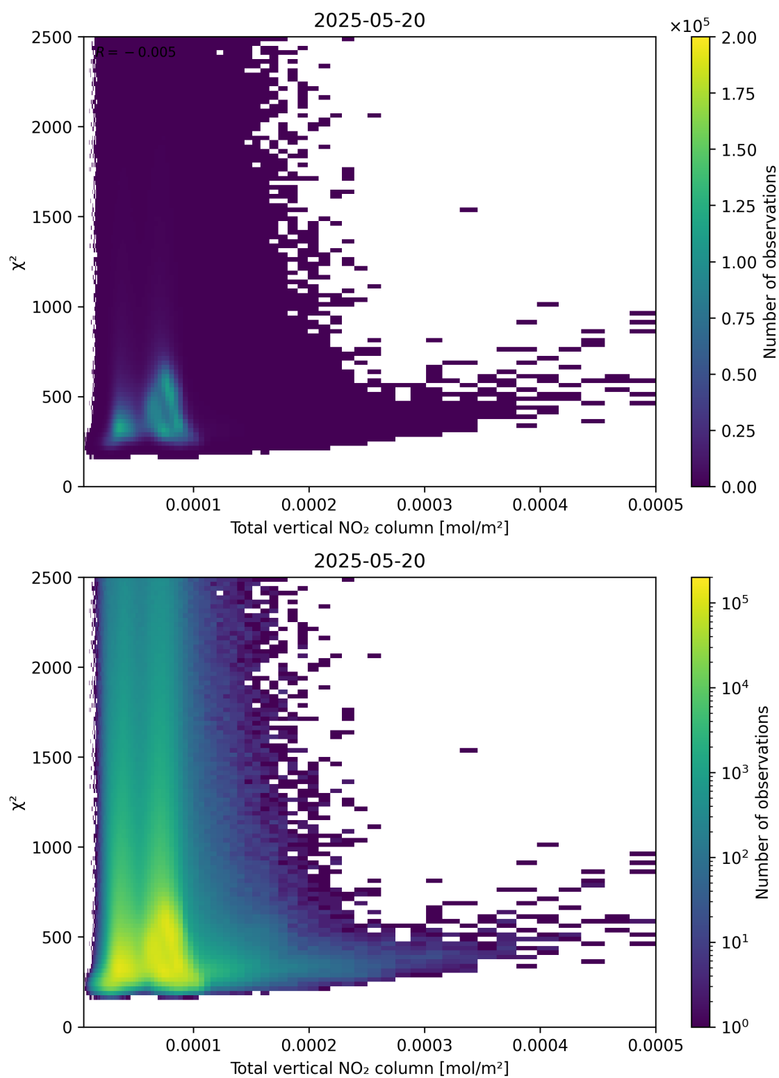
Figure 111: Scatter density plot of “Total vertical NO 2 column” against “ \chi^2 ” for 2025-05-19 to 2025-05-21.
