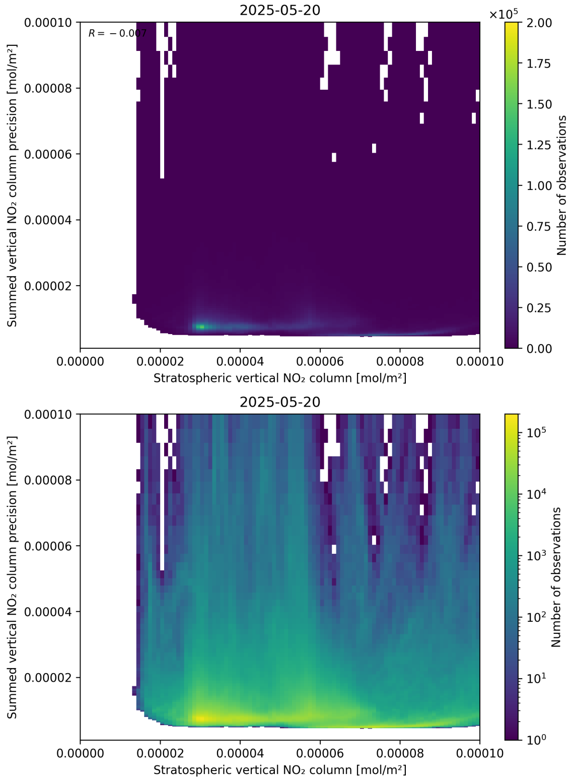
Figure 99: Scatter density plot of “Stratospheric vertical NO 2 column” against “Summed vertical NO 2 column precision” for 2025-05-19 to 2025-05-21.
