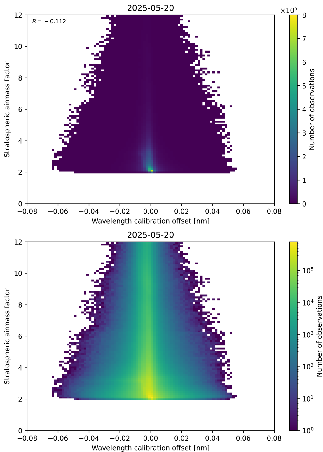
Figure 174: Scatter density plot of “Wavelength calibration offset” against “Stratospheric air mass factor” for 2025-05-19 to 2025-05-21.
