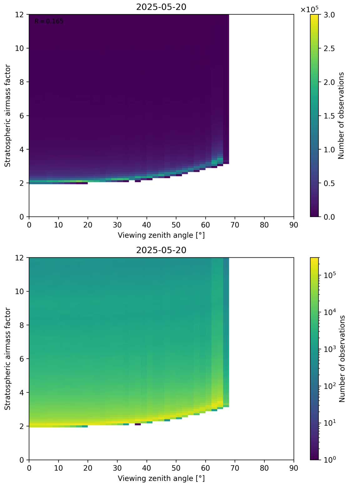
Figure 159: Scatter density plot of “Viewing zenith angle” against “Stratospheric airmass factor” for 2025-05-19 to 2025-05-21.
