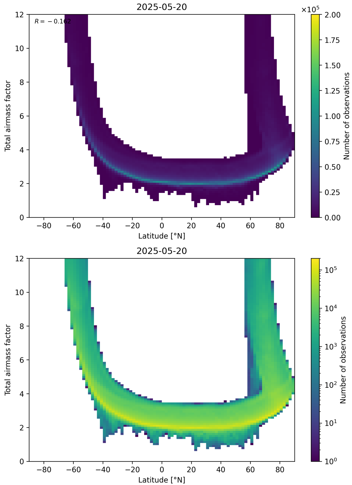
Figure 84: Scatter density plot of “Latitude” against “Total airmass factor” for 2025-05-19 to 2025-05-21.
