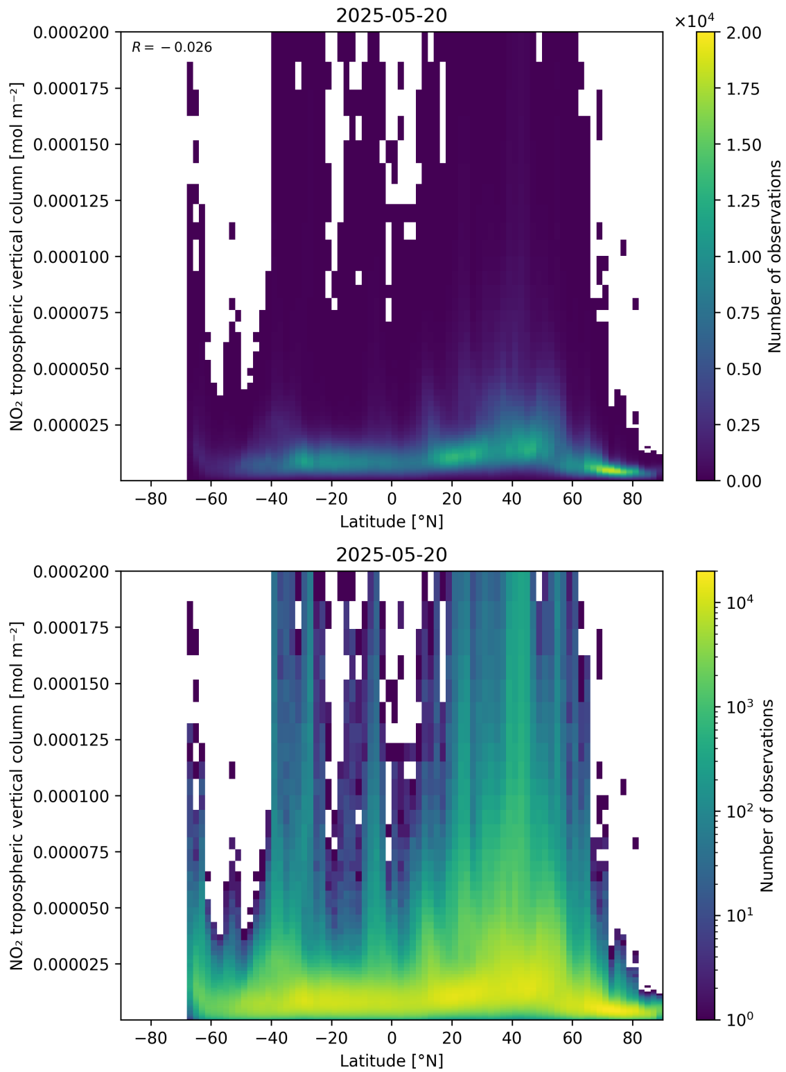
Figure 92: Scatter density plot of “Latitude” against “NO 2 tropospheric vertical column” for 2025-05-19 to 2025-05-21.
