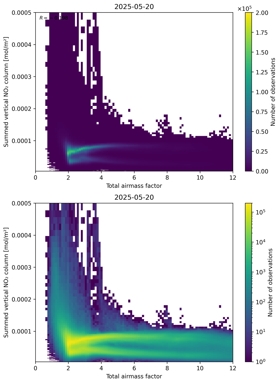
Figure 65: Scatter density plot of “Total airmass factor” against “Summed vertical NO 2 column” for 2025-05-19 to 2025-05-21.
