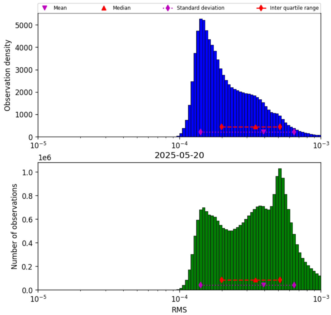
Figure 43: Histogram of “RMS” for 2025-05-19 to 2025-05-21
