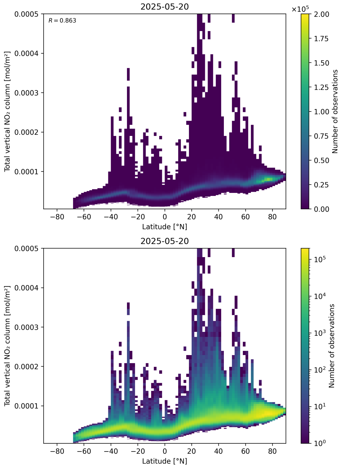
Figure 90: Scatter density plot of “Latitude” against “Total vertical NO 2 column” for 2025-05-19 to 2025-05-21.
