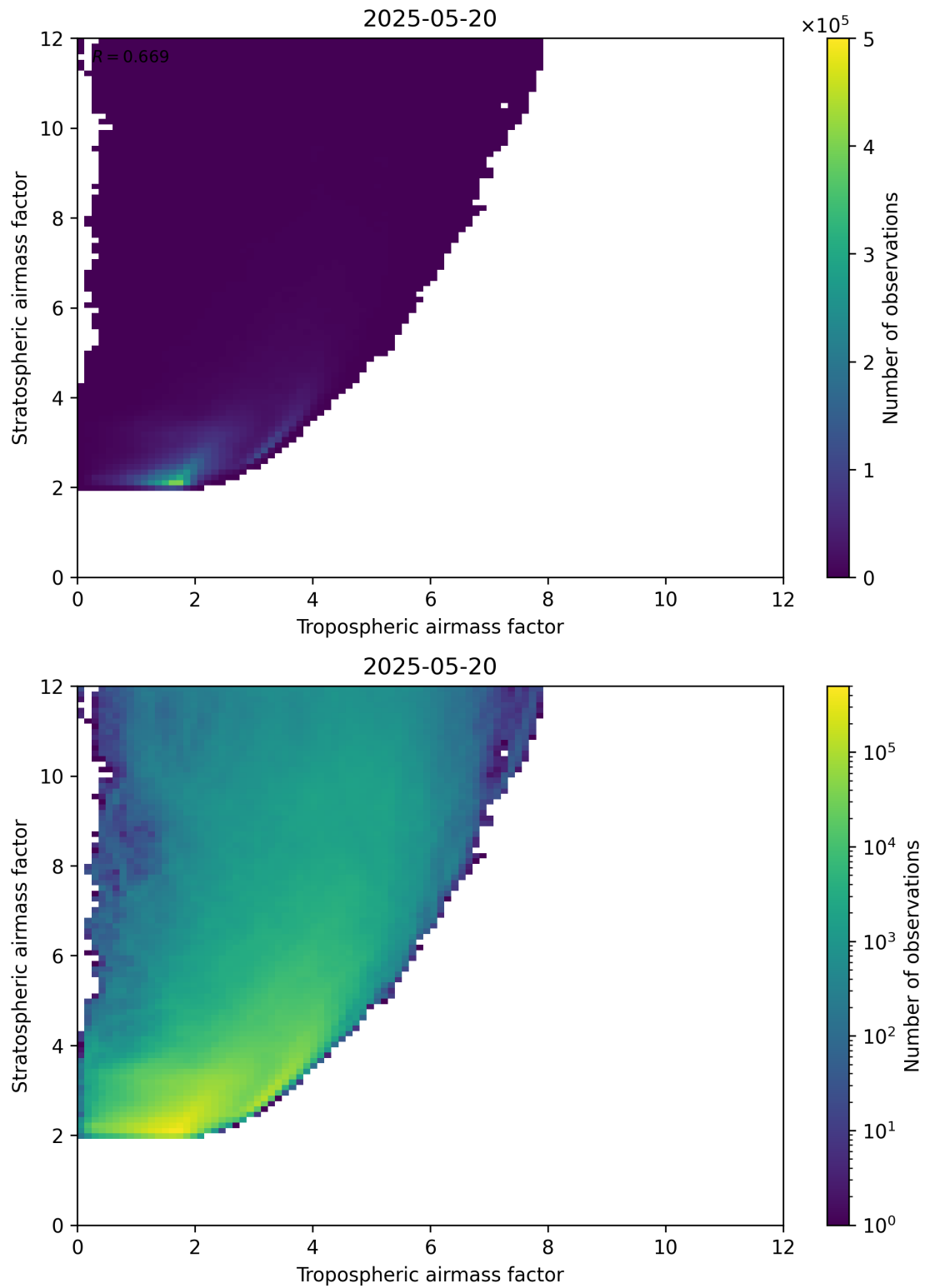
Figure 71: Scatter density plot of “Tropospheric airmass factor” against “Stratospheric airmass factor” for 2025-05-19 to 2025-05-21.
