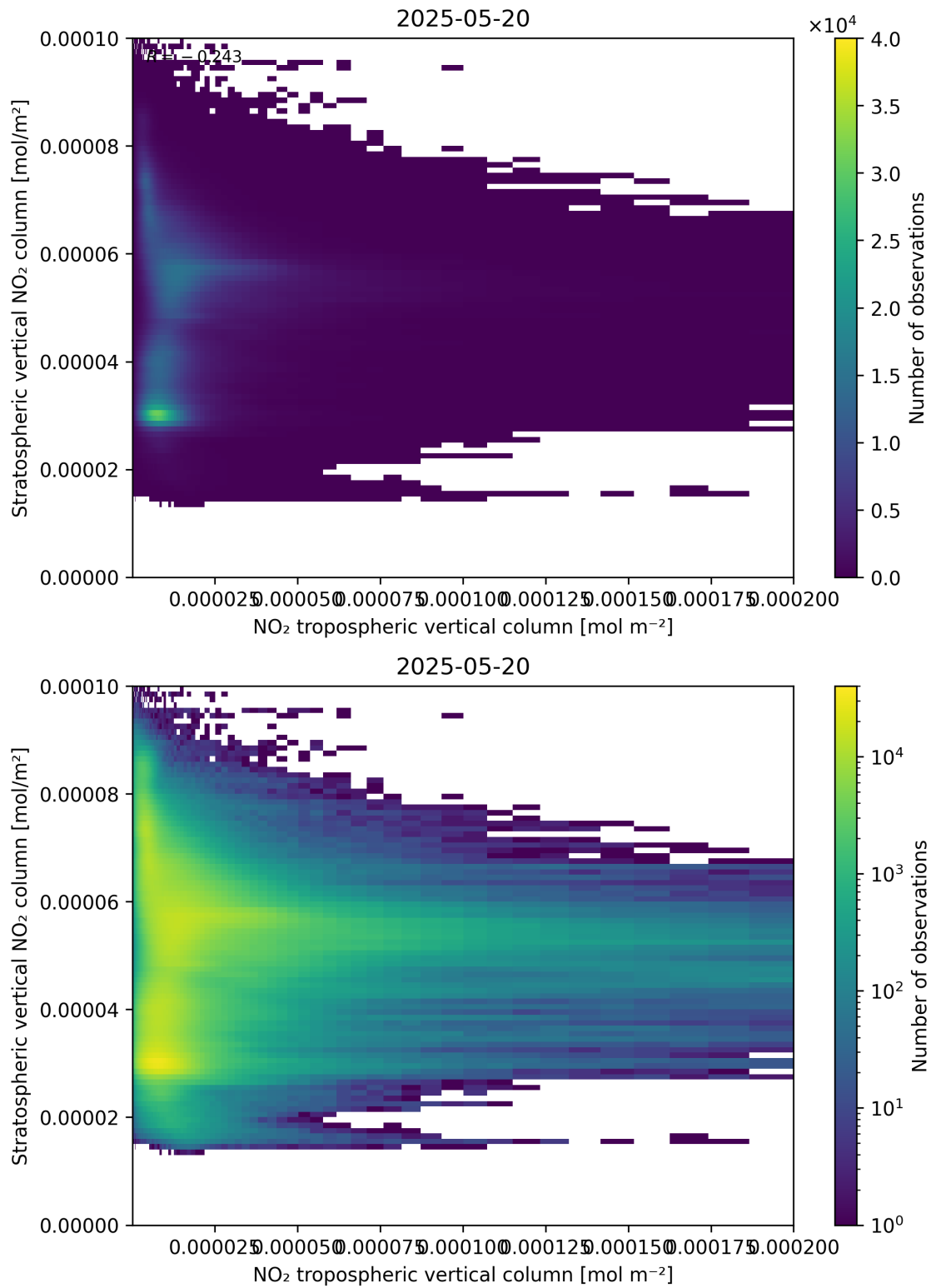
Figure 125: Scatter density plot of “NO 2 tropospheric vertical column” against “Stratospheric vertical NO 2 column” for 2025-05-19 to 2025-05-21.
