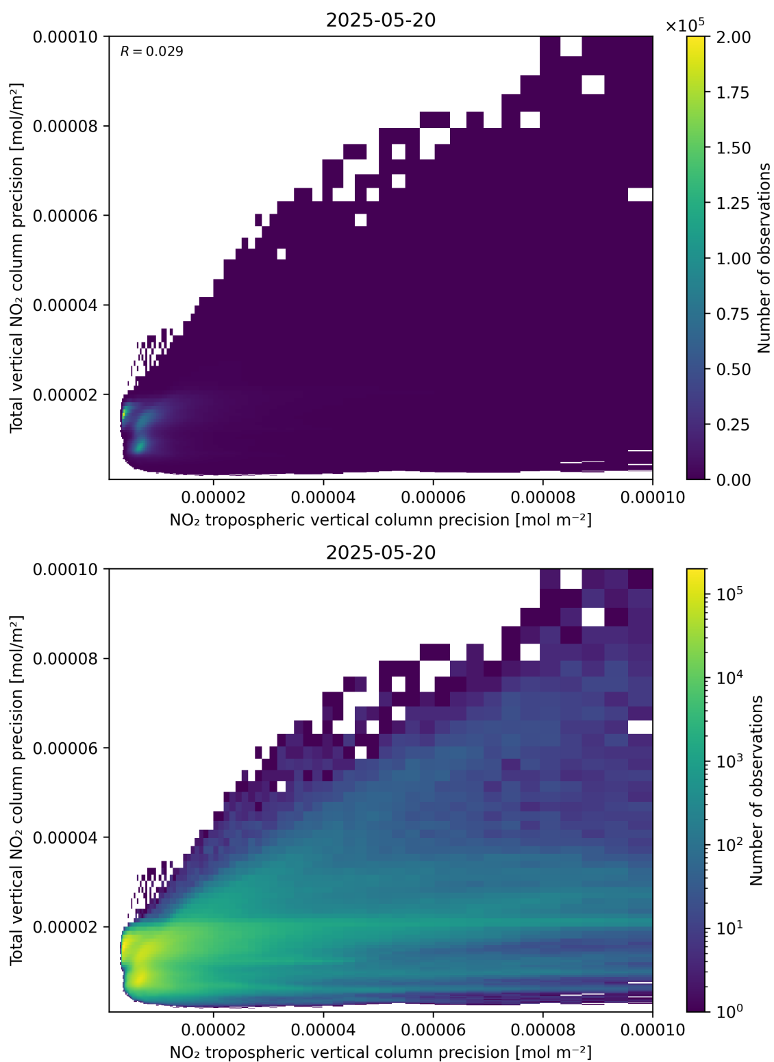
Figure 139: Scatter density plot of “NO 2 tropospheric vertical column precision” against “Total vertical NO 2 column precision” for 2025-05-19 to 2025-05-21.
