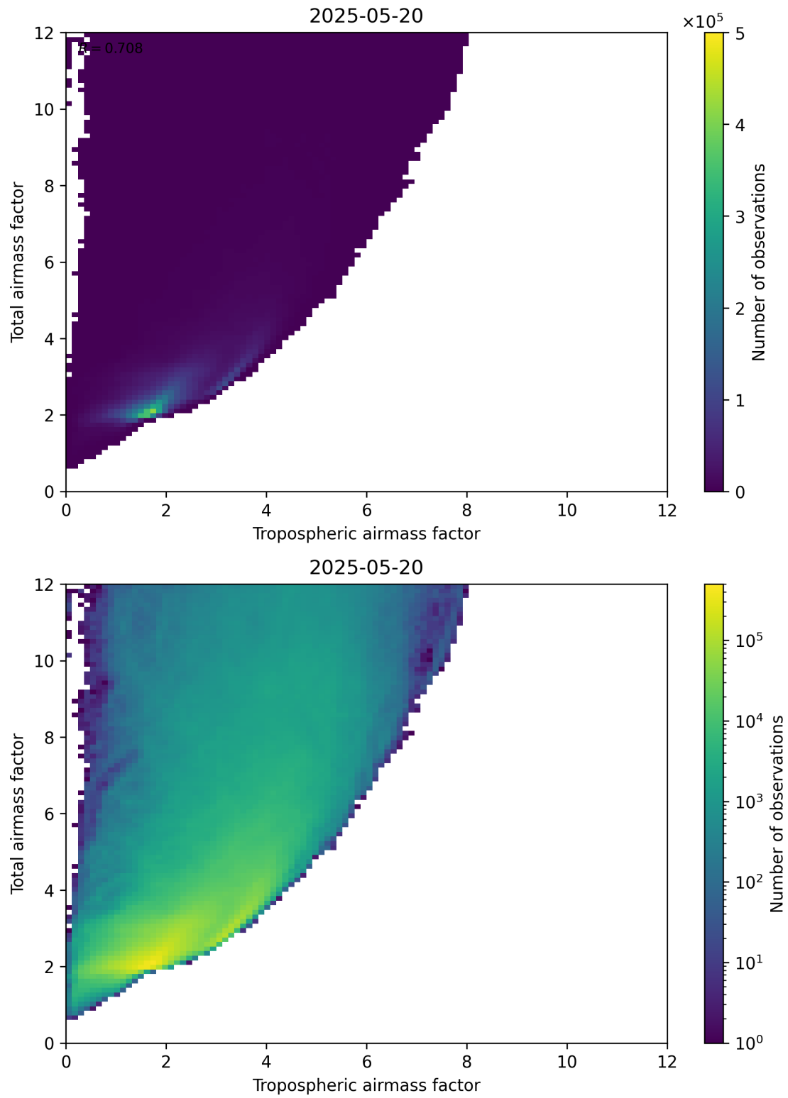
Figure 72: Scatter density plot of “Tropospheric airmass factor” against “Total airmass factor” for 2025-05-19 to 2025-05-21.
