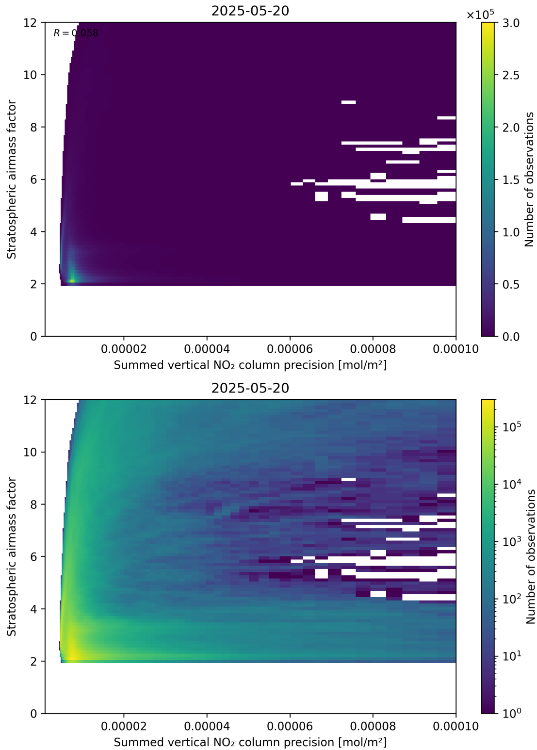
Figure 106: Scatter density plot of “Summed vertical NO 2 column precision” against “Stratospheric airmass factor” for 2025-05-19 to 2025-05-21.
