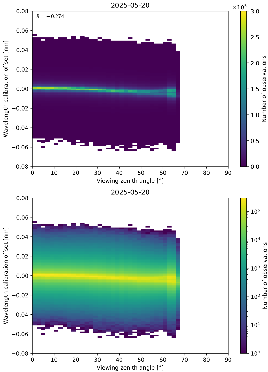
Figure 173: Scatter density plot of “Viewing zenith angle” against “Wavelength calibration offset” for 2025-05-19 to 2025-05-21.
