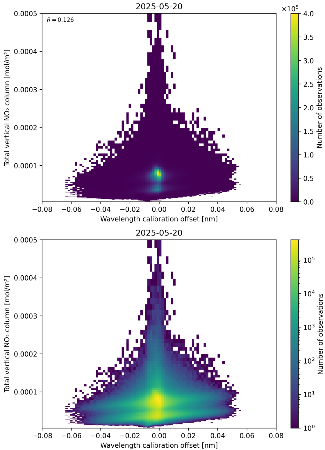
Figure 179: Scatter density plot of “Wavelength calibration offset” against “Total vertical NO 2 column” for 2025-05-19 to 2025-05-21.
