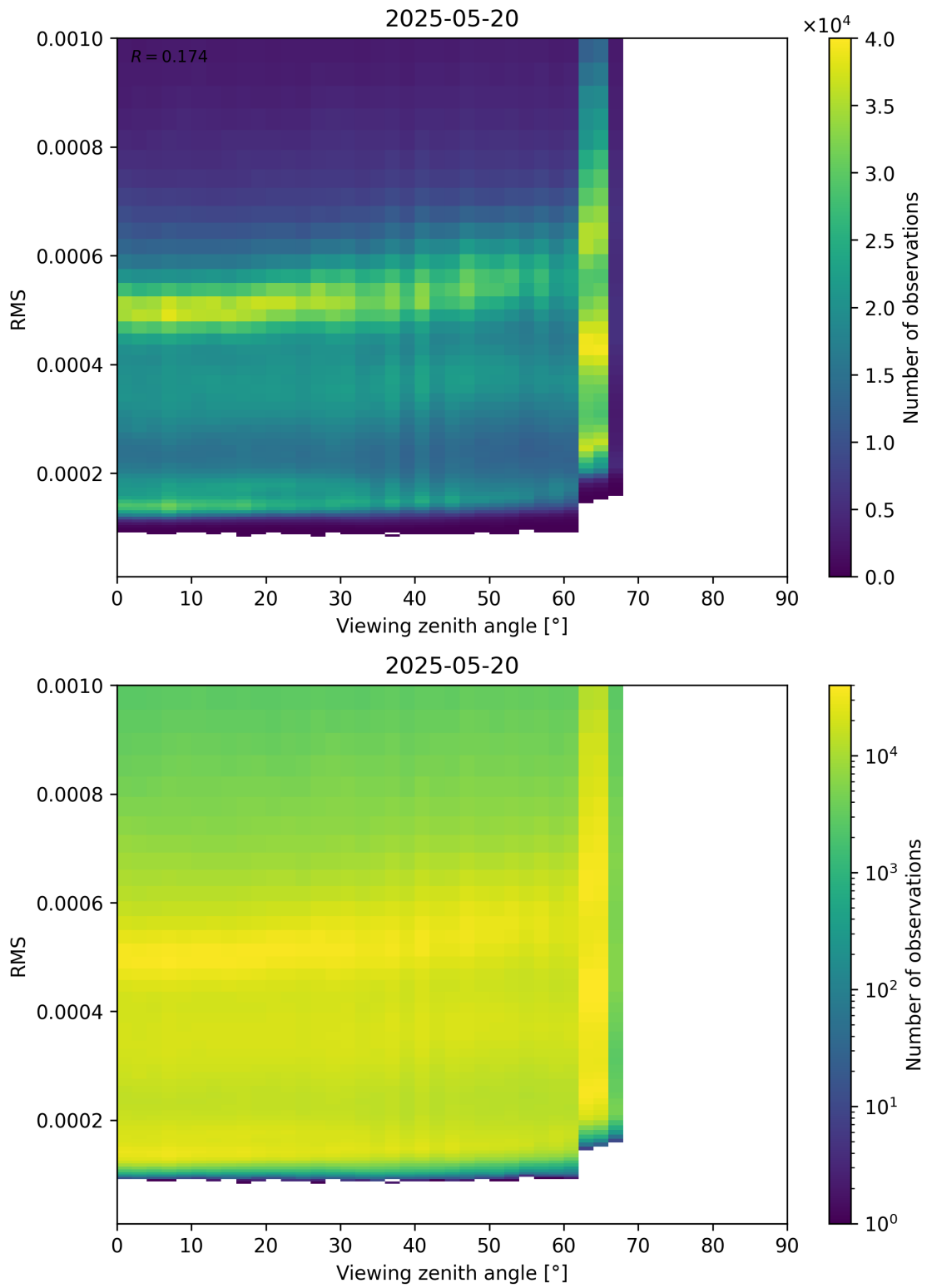
Figure 171: Scatter density plot of “Viewing zenith angle” against “RMS” for 2025-05-19 to 2025-05-21.
