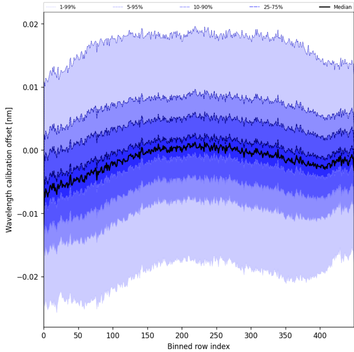
Figure 52: Along track statistics of “Wavelength calibration offset” for 2025-05-19 to 2025-05-21
