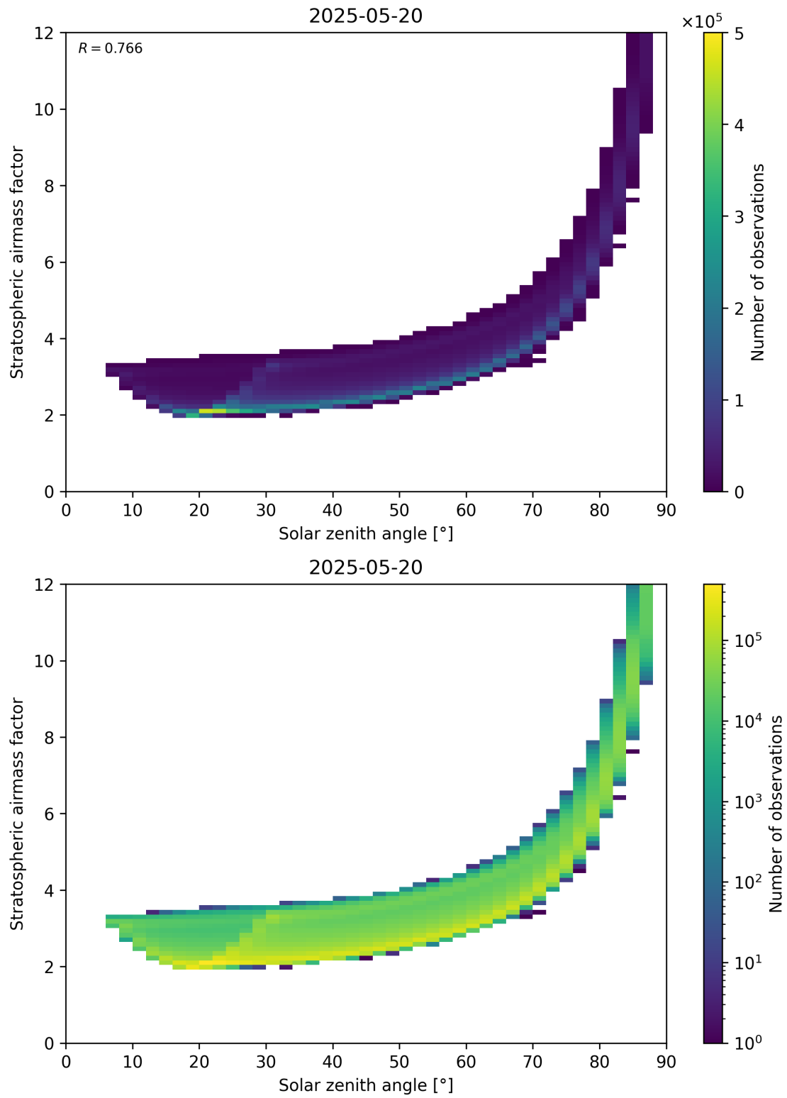
Figure 145: Scatter density plot of “Solar zenith angle” against “Stratospheric airmass factor” for 2025-05-19 to 2025-05-21.
