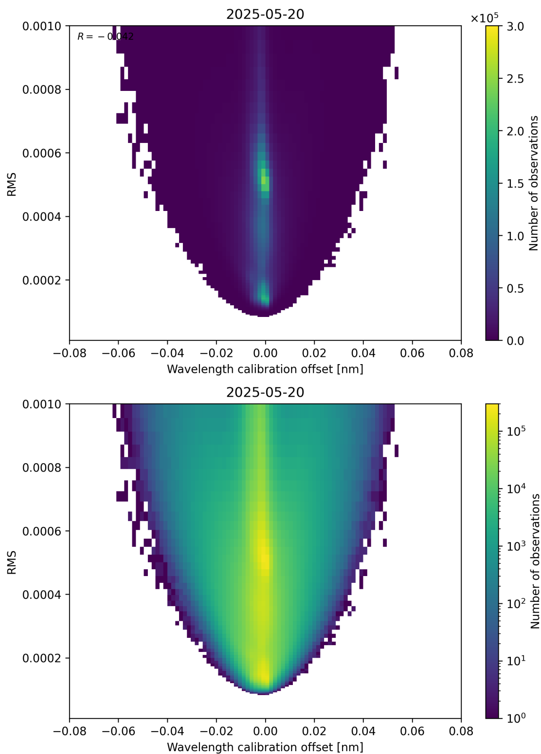
Figure 181: Scatter density plot of “Wavelength calibration offset” against “RMS” for 2025-05-19 to 2025-05-21.
