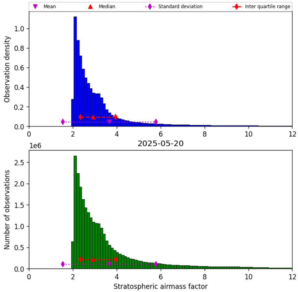
Figure 44: Histogram of “Stratospheric airmass factor” for 2025-05-19 to 2025-05-21
