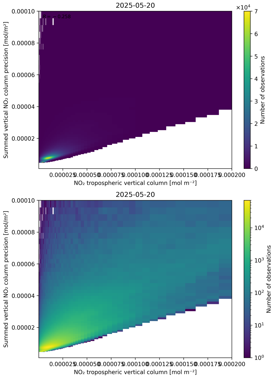
Figure 127: Scatter density plot of “NO 2 tropospheric vertical column” against “Summed vertical NO 2 column precision” for 2025-05-19 to 2025-05-21.
