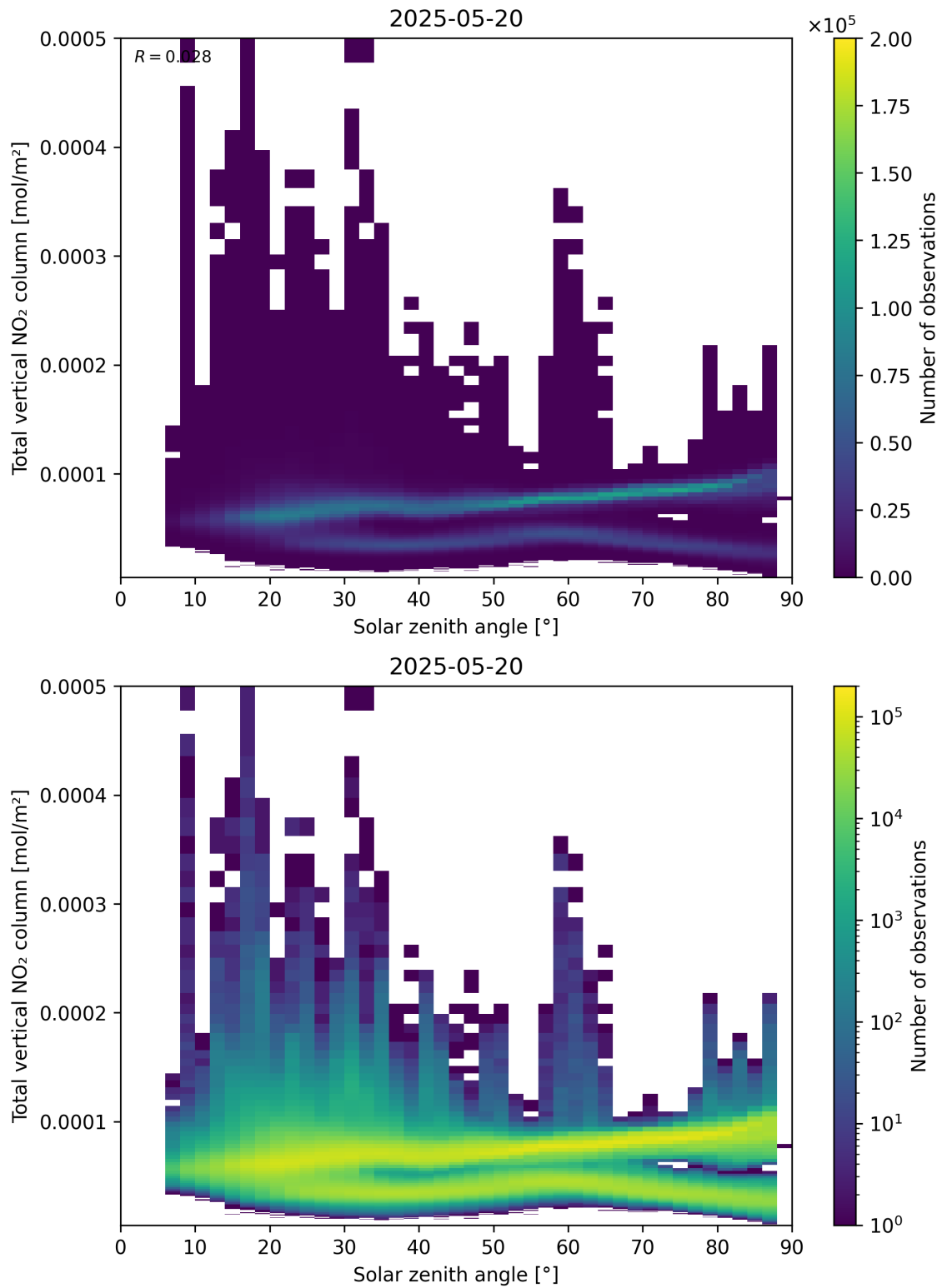
Figure 153: Scatter density plot of “Solar zenith angle” against “Total vertical NO 2 column” for 2025-05-19 to 2025-05-21.
