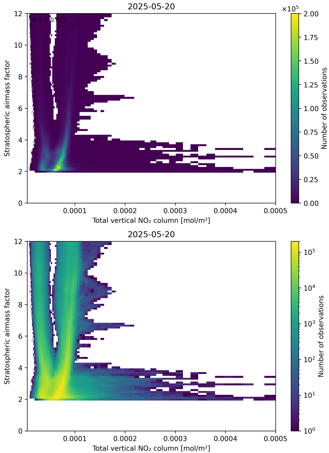
Figure 110: Scatter density plot of “Total vertical NO 2 column” against “Stratospheric airmass factor” for 2025-05-19 to 2025-05-21.
