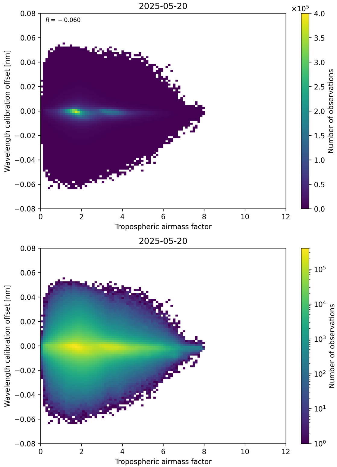
Figure 80: Scatter density plot of “Tropospheric airmass factor” against “Wavelength calibration offset” for 2025-05-19 to 2025-05-21.
