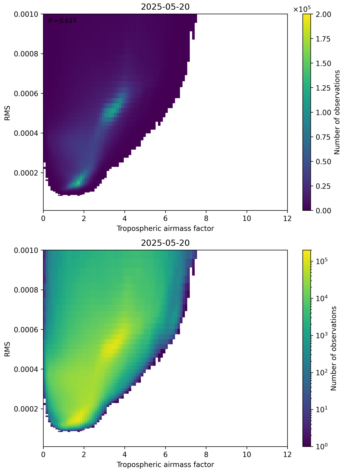
Figure 79: Scatter density plot of “Tropospheric airmass factor” against “RMS” for 2025-05-19 to 2025-05-21.
