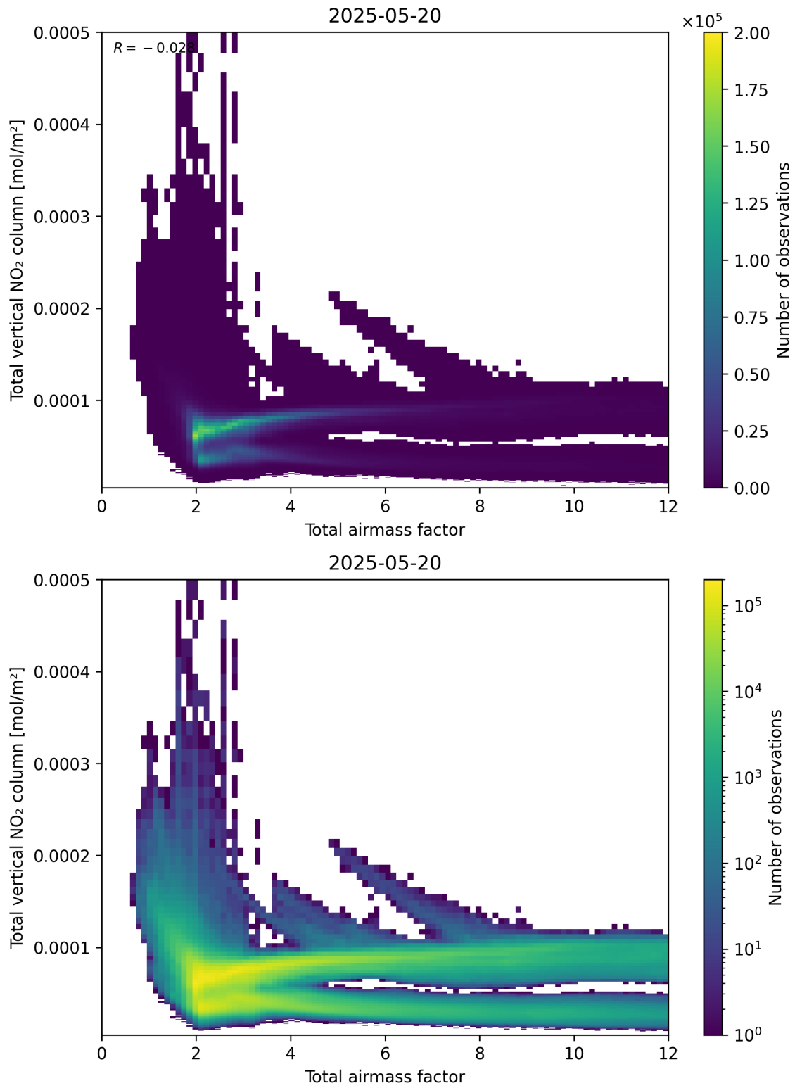
Figure 67: Scatter density plot of “Total airmass factor” against “Total vertical NO 2 column” for 2025-05-19 to 2025-05-21.
