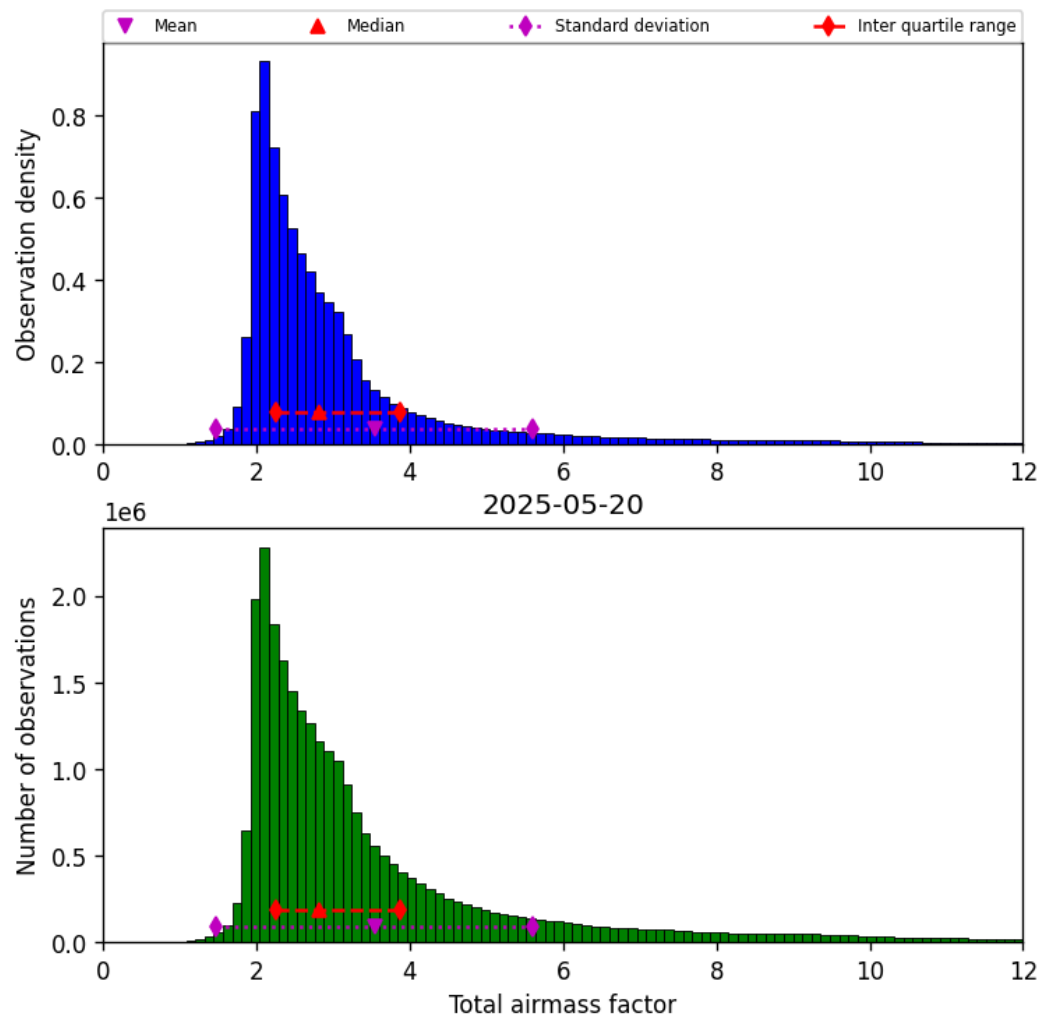
Figure 32: Histogram of “Total airmass factor” for 2025-05-19 to 2025-05-21
