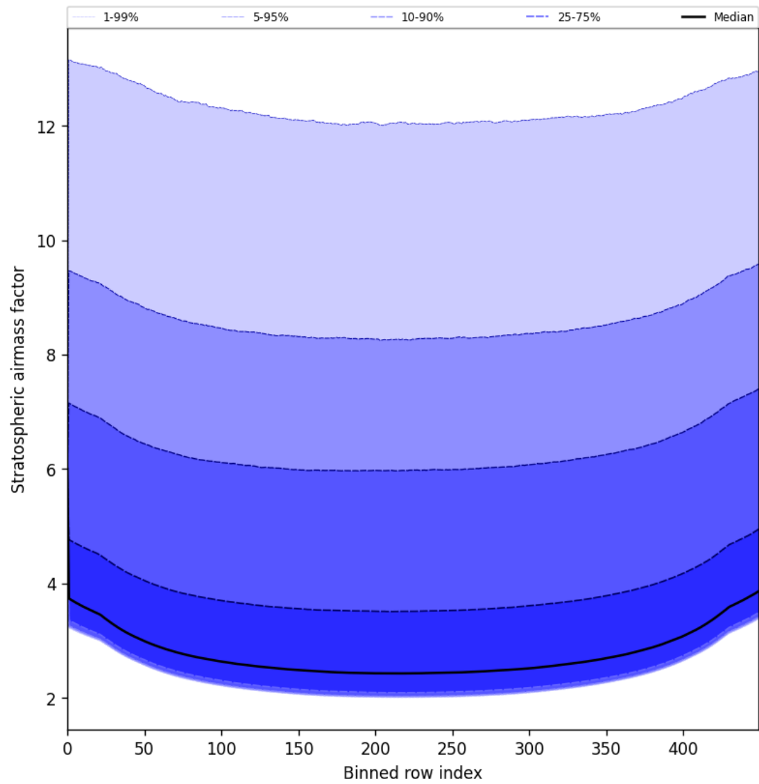
Figure 61: Along track statistics of “Stratospheric airmass factor” for 2025-05-19 to 2025-05-21
