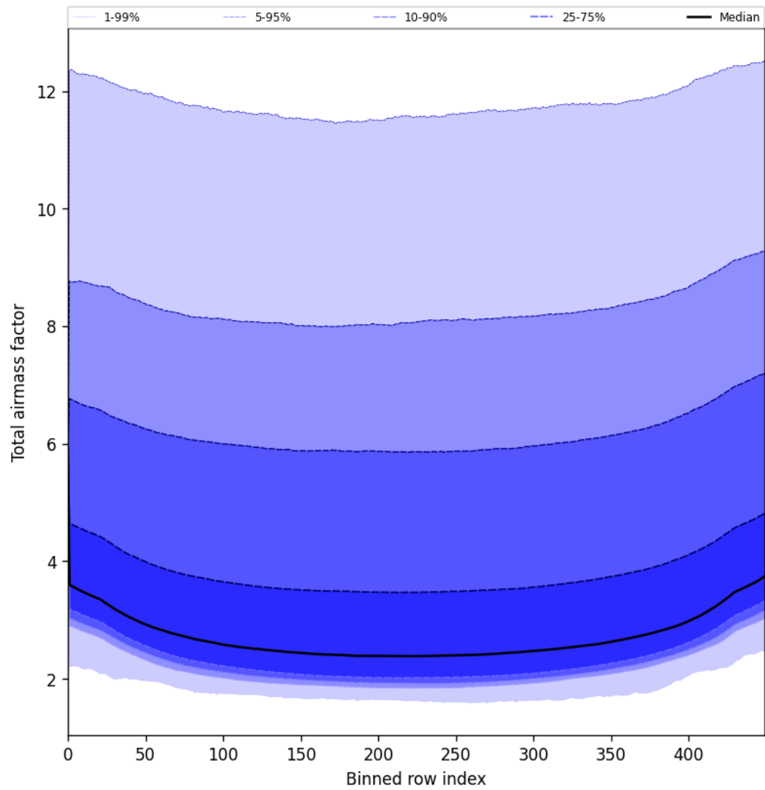
Figure 49: Along track statistics of “Total airmass factor” for 2025-05-19 to 2025-05-21
