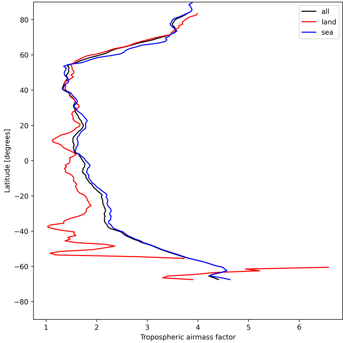
Figure 14: Zonal average of “Tropospheric air mass factor” for 2025-05-19 to 2025-05-21.
