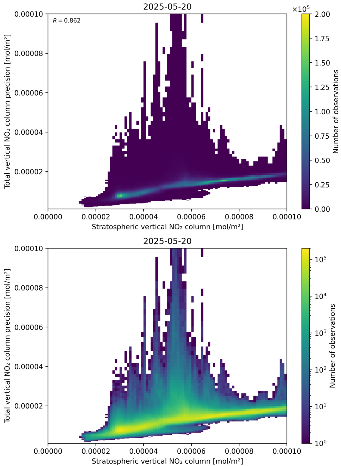
Figure 101: Scatter density plot of “Stratospheric vertical NO 2 column” against “Total vertical NO 2 column precision” for 2025-05-19 to 2025-05-21.
