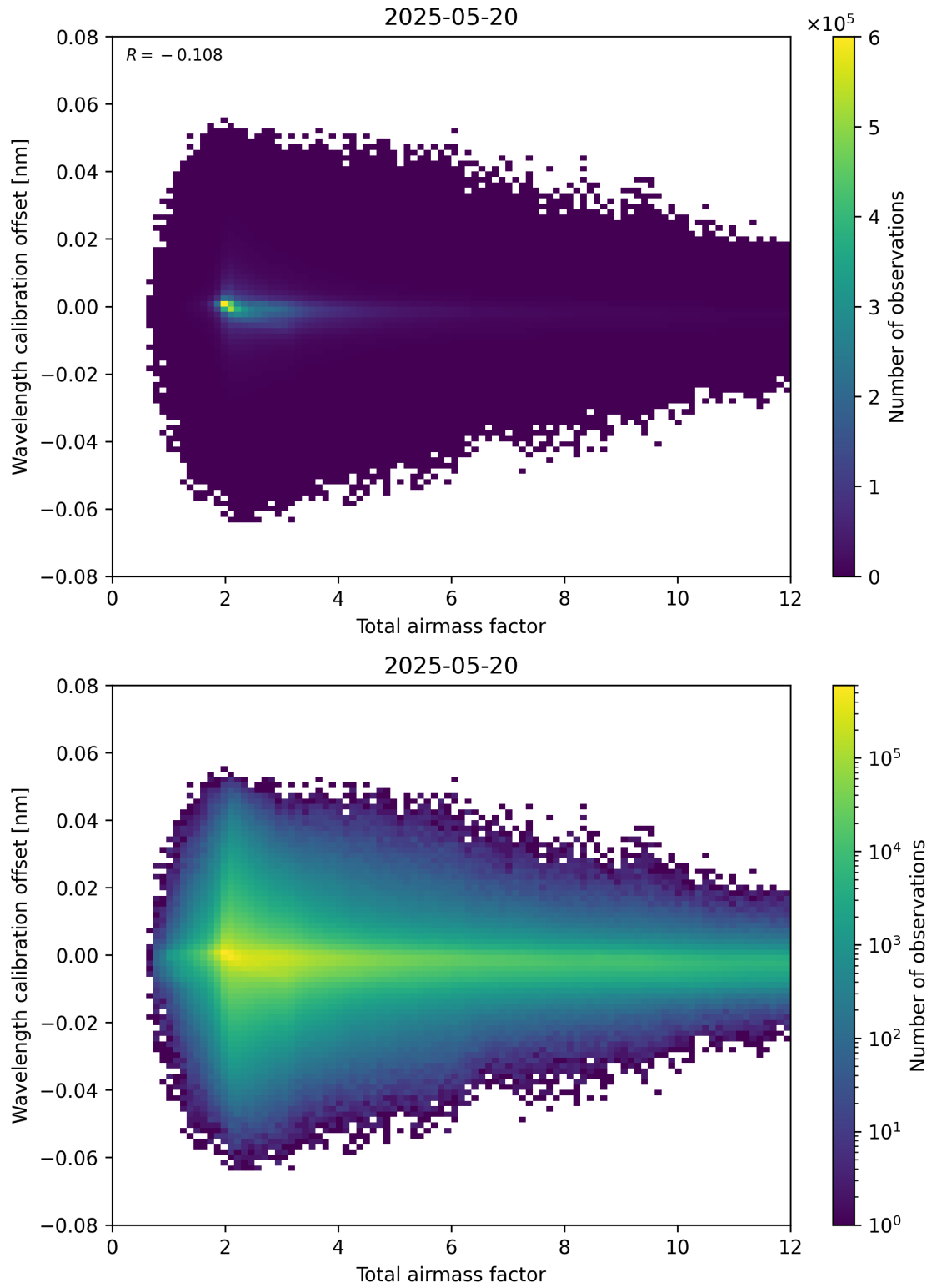
Figure 70: Scatter density plot of “Total airmass factor” against “Wavelength calibration offset” for 2025-05-19 to 2025-05-21.
