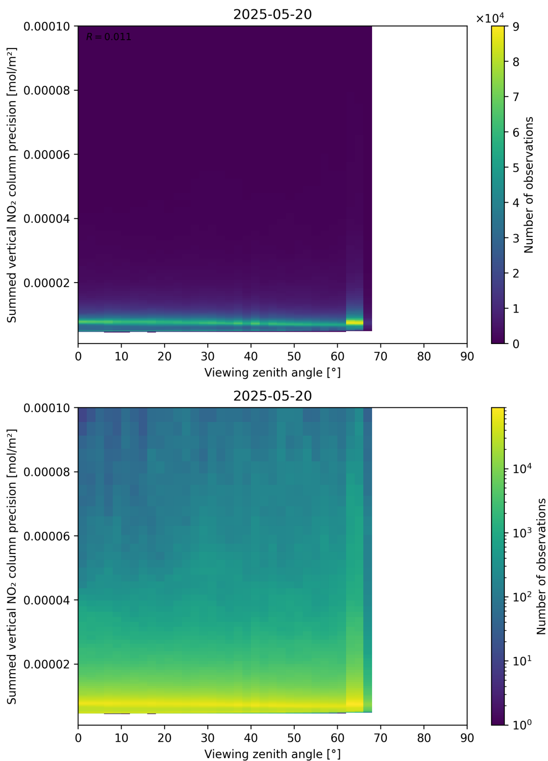
Figure 166: Scatter density plot of “Viewing zenith angle” against “Summed vertical NO 2 column precision” for 2025-05-19 to 2025-05-21.
