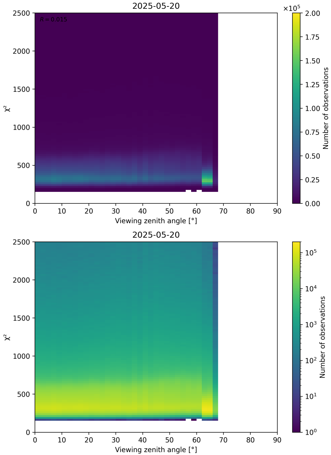
Figure 162: Scatter density plot of “Viewing zenith angle” against “ \chi^2 ” for 2025-05-19 to 2025-05-21.
