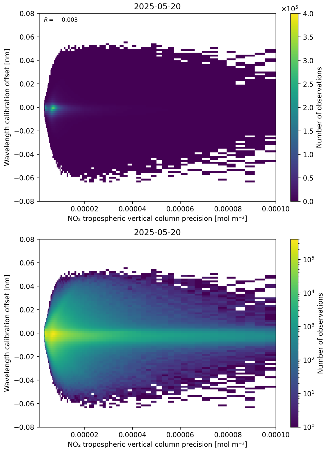
Figure 141: Scatter density plot of “NO 2 tropospheric vertical column precision” against “Wavelength calibration offset” for 2025-05-19 to 2025-05-21.
