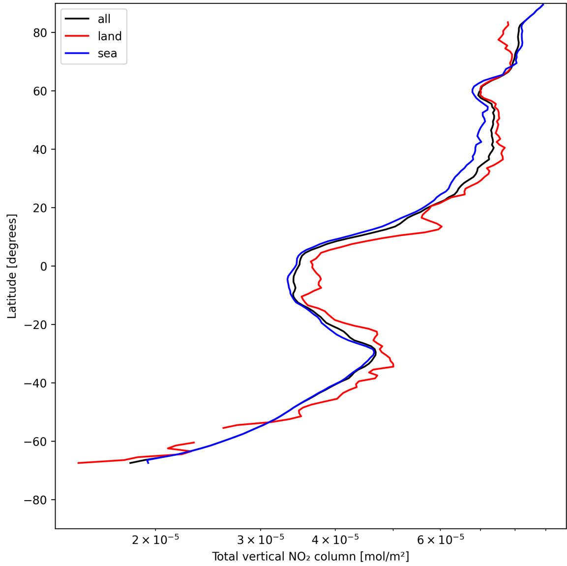
Figure 21: Zonal average of “Total vertical NO 2 column” for 2025-05-19 to 2025-05-21.
