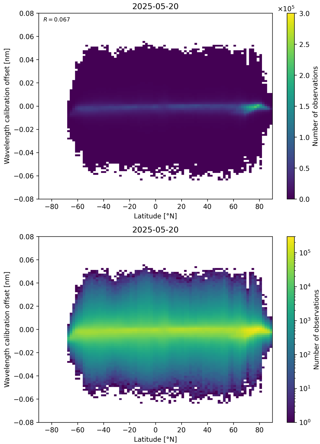
Figure 95: Scatter density plot of “Latitude” against “Wavelength calibration offset” for 2025-05-19 to 2025-05-21.
