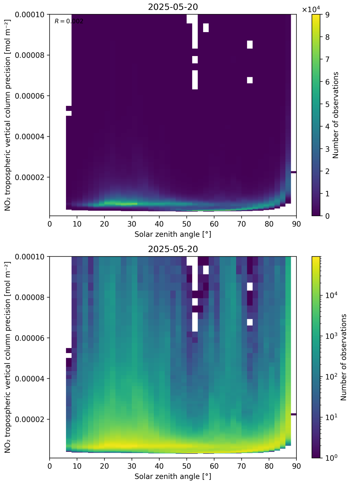
Figure 156: Scatter density plot of “Solar zenith angle” against “NO 2 tropospheric vertical column precision” for 2025-05-19 to 2025-05-21.
