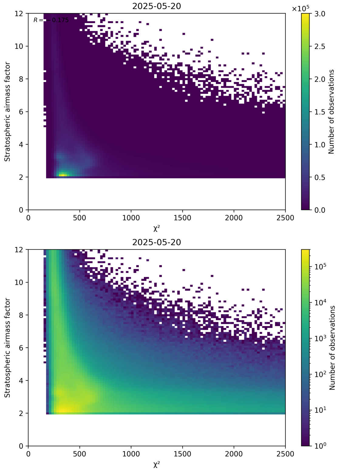
Figure 81: Scatter density plot of “ \chi^2 ” against “Stratospheric airmass factor” for 2025-05-19 to 2025-05-21.
