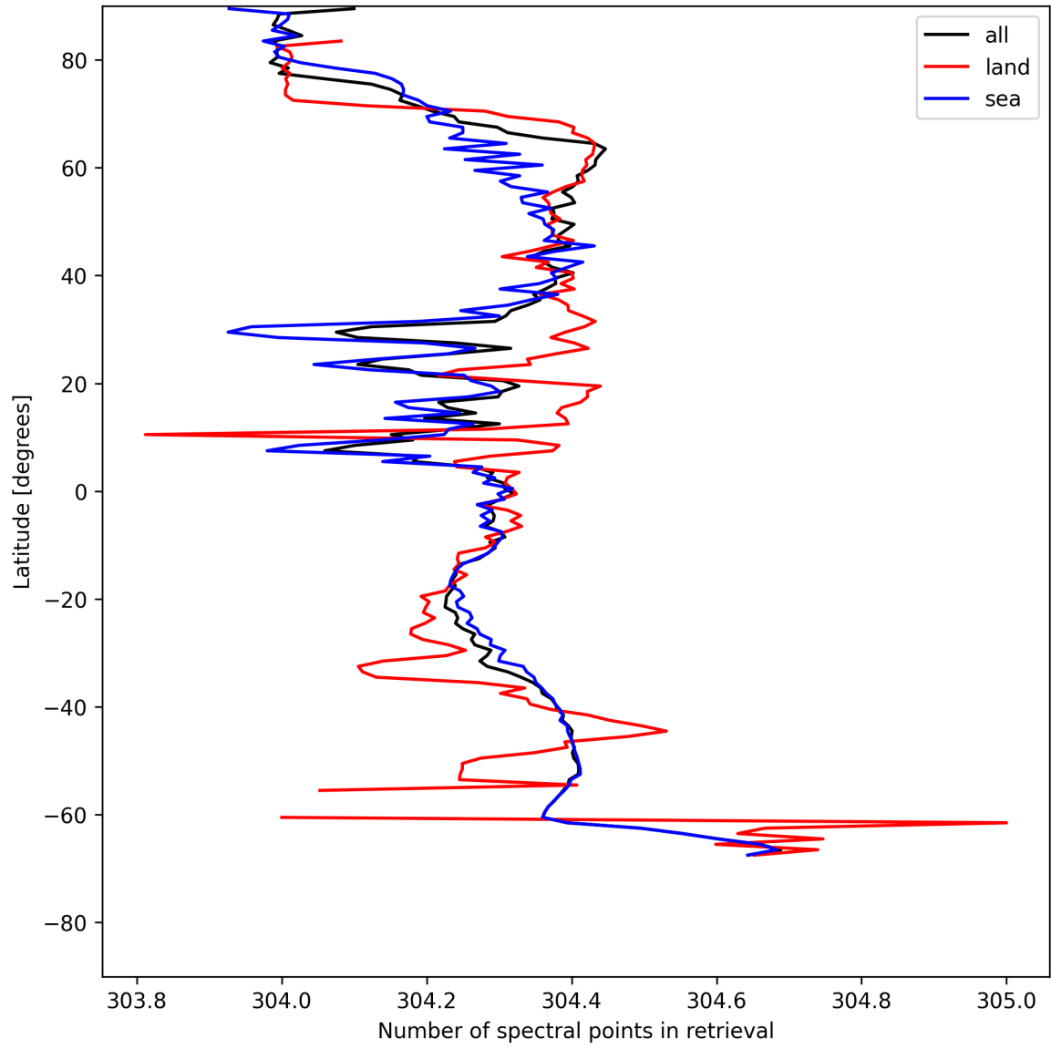
Figure 16: Zonal average of “Number of spectral points in retrieval” for 2025-05-19 to 2025-05-21.
