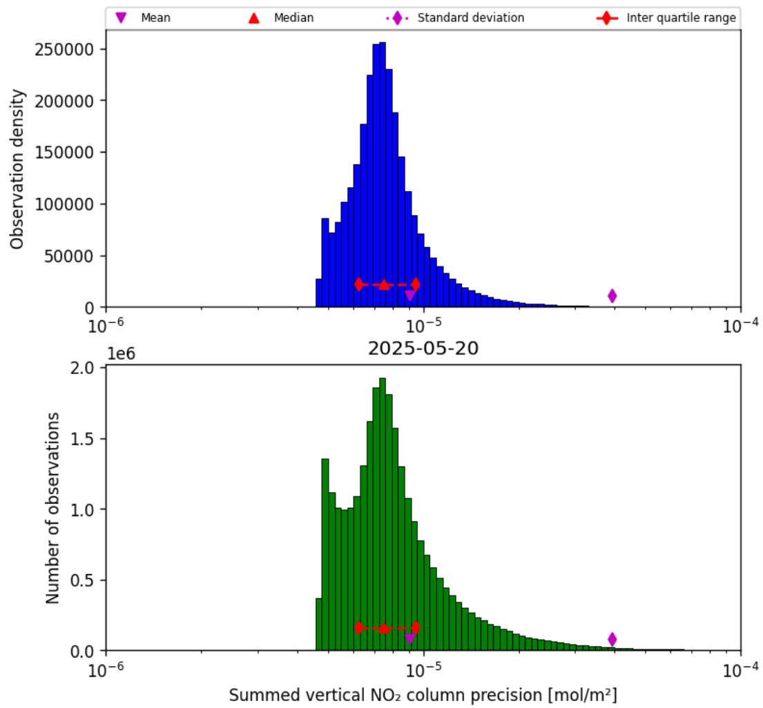
Figure 41: Histogram of "Summed vertical NO 2 column precision" for 2025-05-19 to 2025-05-21
