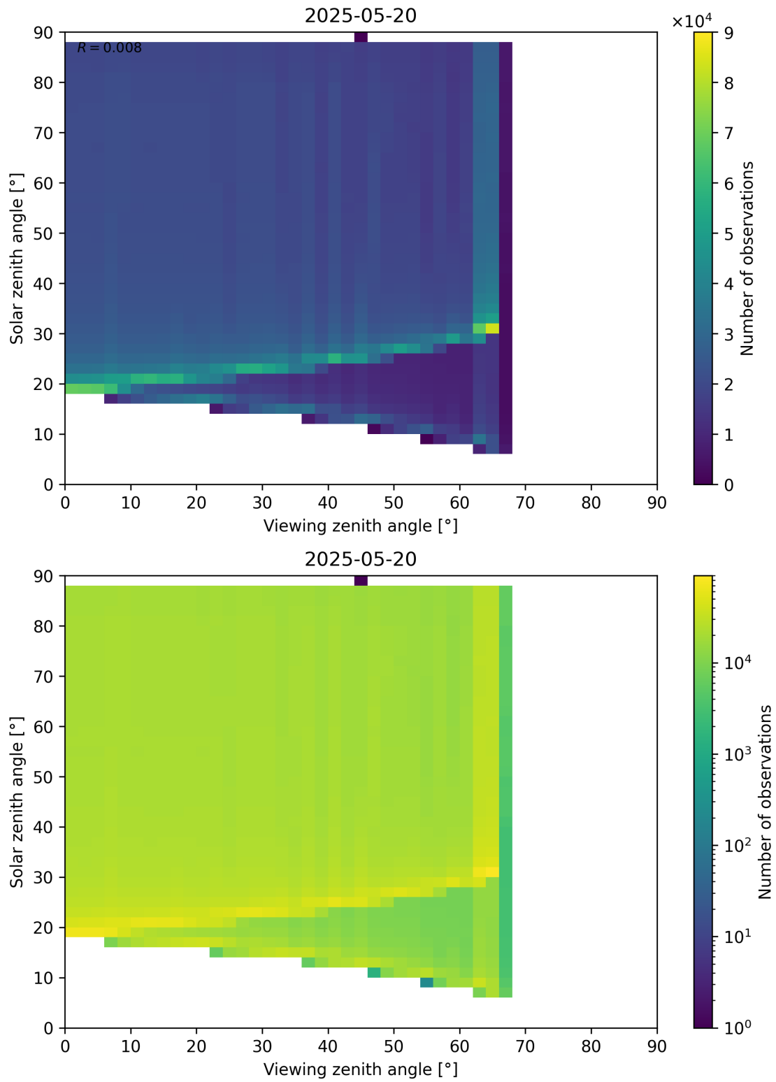
Figure 172: Scatter density plot of “Viewing zenith angle” against “Solar zenith angle” for 2025-05-19 to 2025-05-21.
