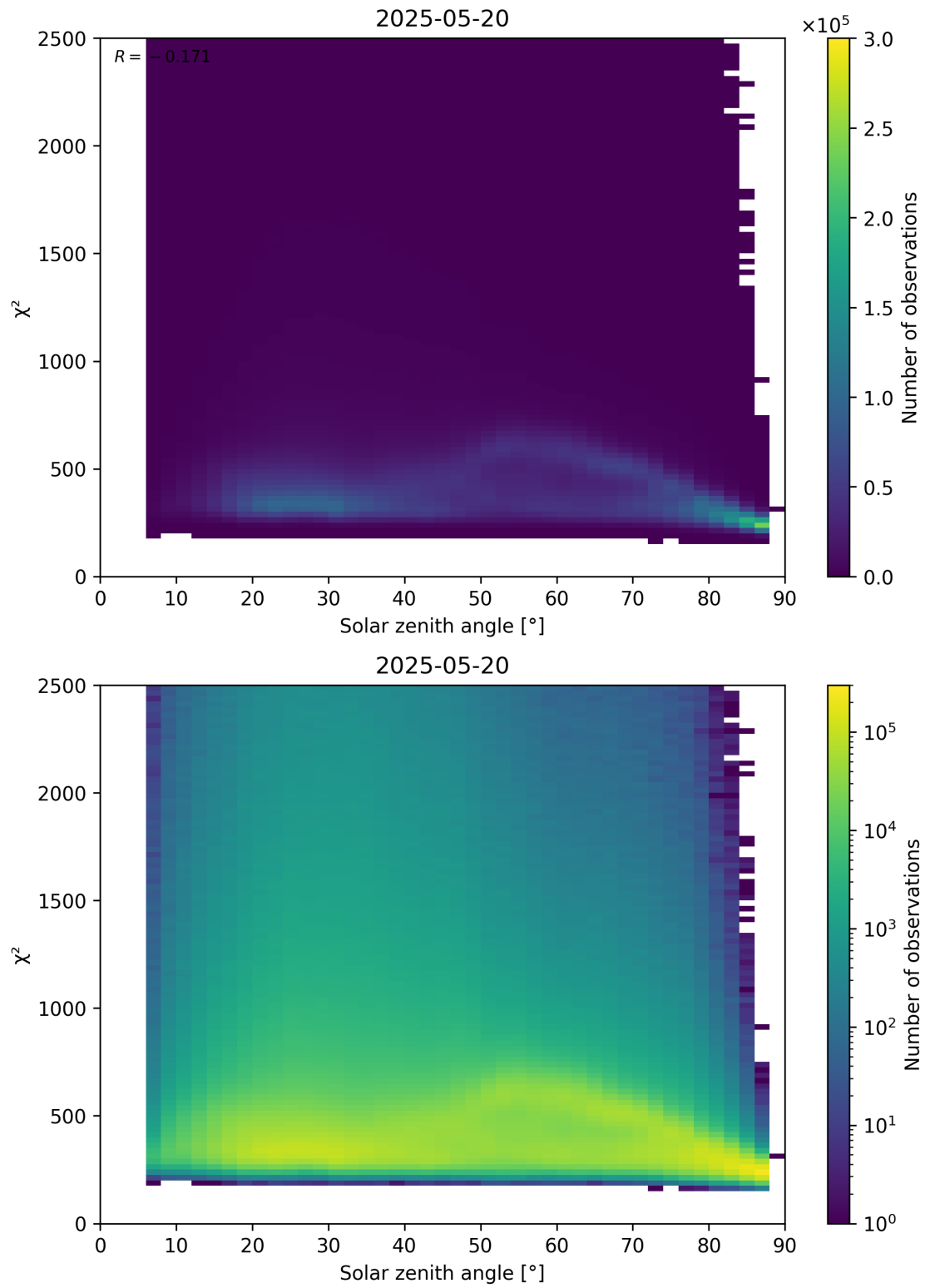
Figure 148: Scatter density plot of “Solar zenith angle” against “ \chi^2 ” for 2025-05-19 to 2025-05-21.
