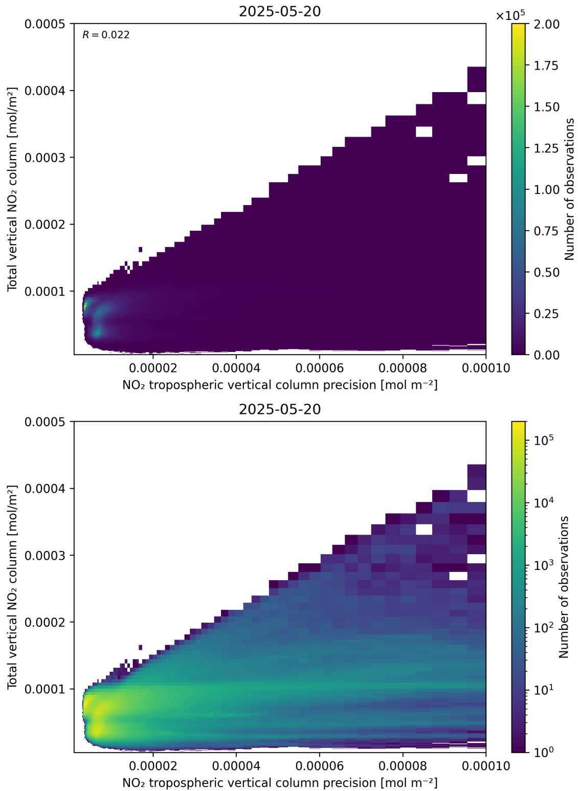
Figure 138: Scatter density plot of “NO 2 tropospheric vertical column precision” against “Total vertical NO 2 column” for 2025-05-19 to 2025-05-21.
