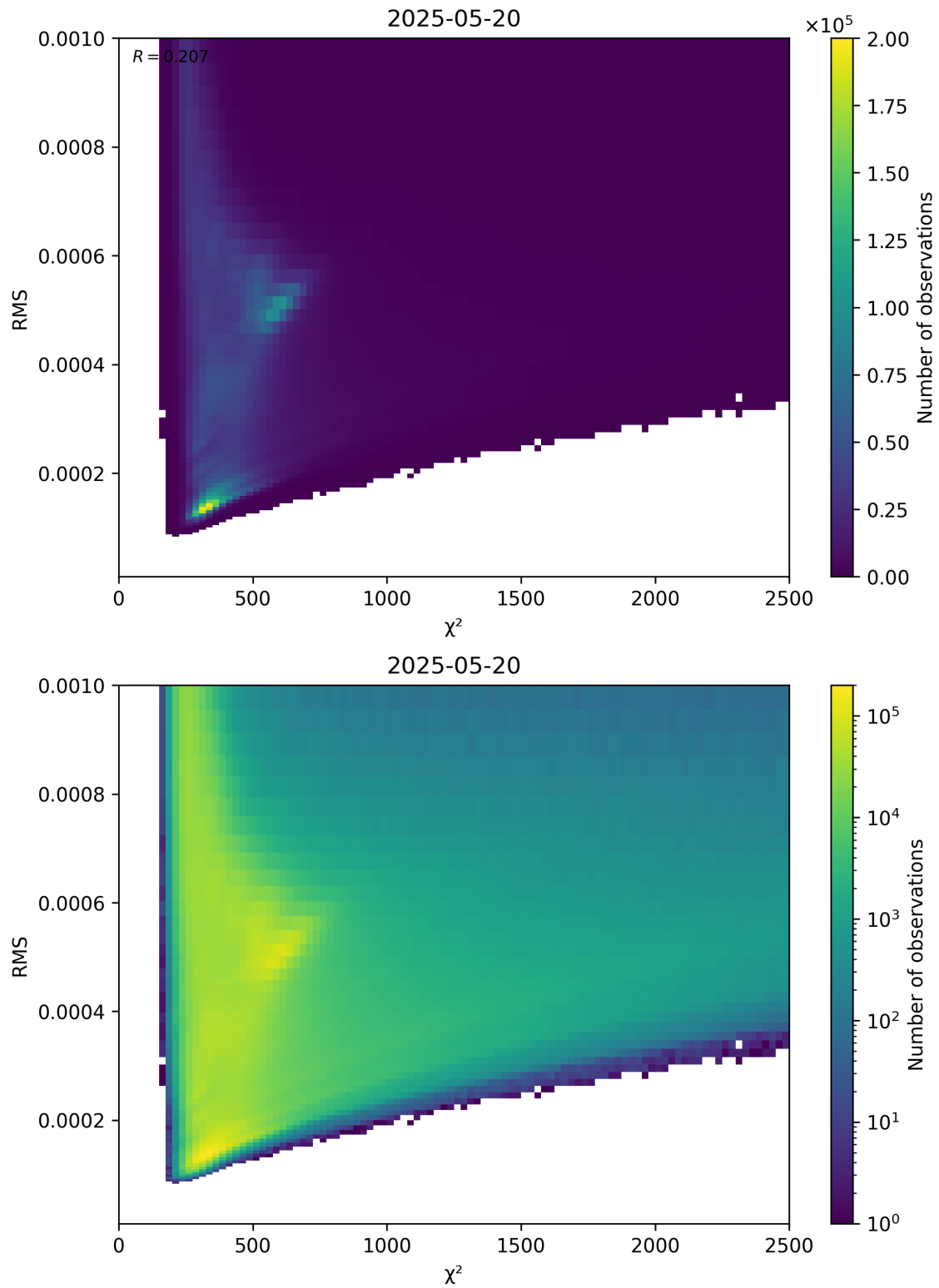
Figure 82: Scatter density plot of “ \chi^2 ” against “RMS” for 2025-05-19 to 2025-05-21.
