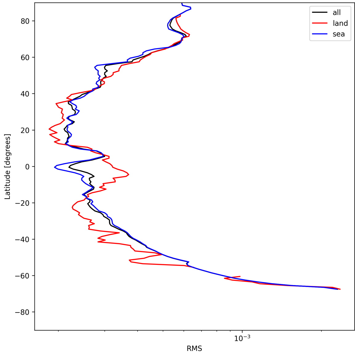
Figure 26: Zonal average of “RMS” for 2025-05-19 to 2025-05-21.
