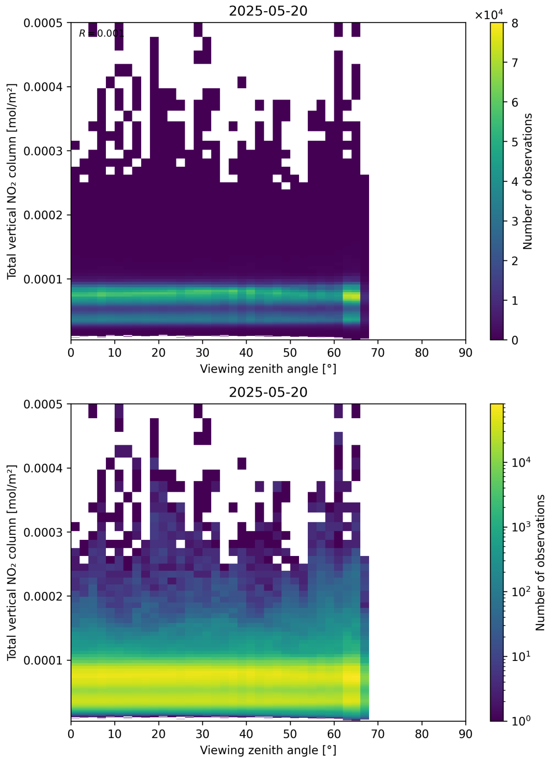
Figure 167: Scatter density plot of “Viewing zenith angle” against “Total vertical NO 2 column” for 2025-05-19 to 2025-05-21.
