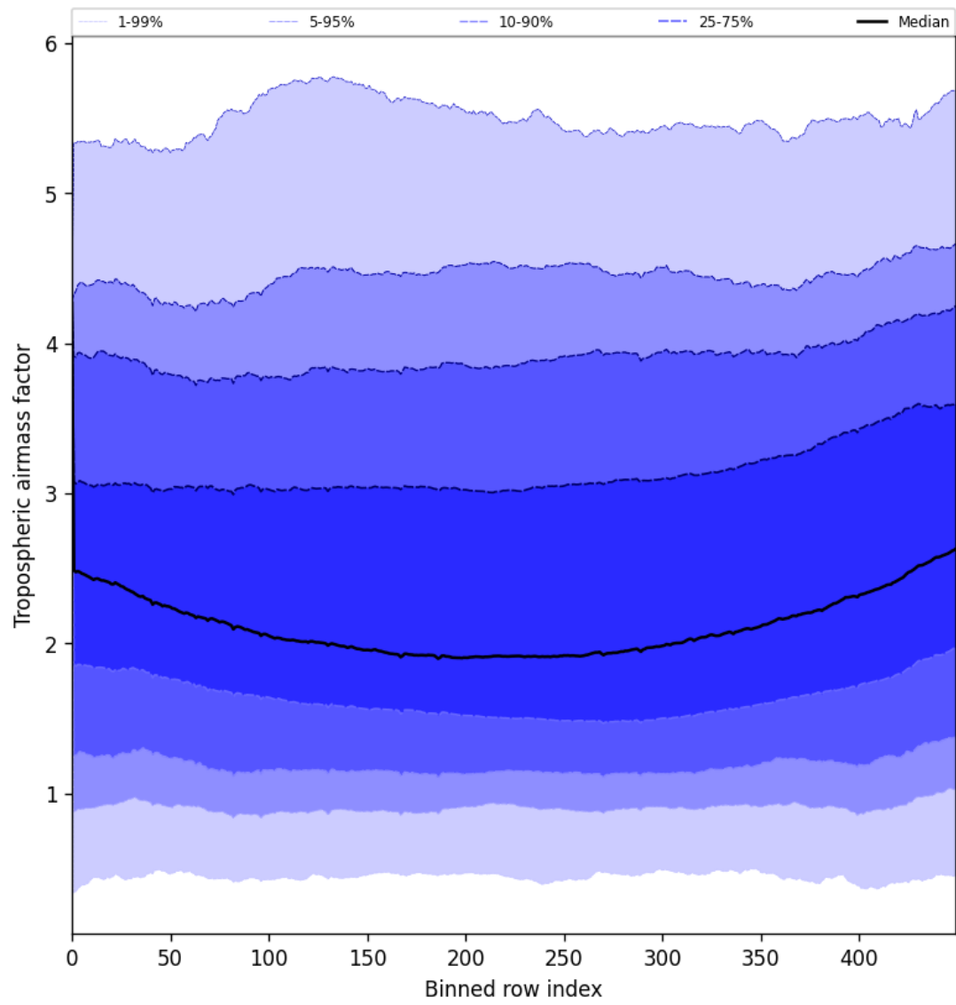
Figure 48: Along track statistics of “Tropospheric airmass factor” for 2025-05-19 to 2025-05-21
