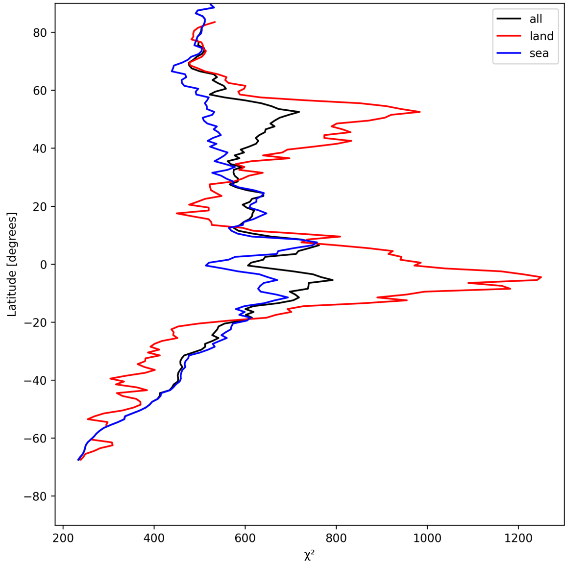
Figure 25: Zonal average of “ \chi^2 ” for 2025-05-19 to 2025-05-21.
