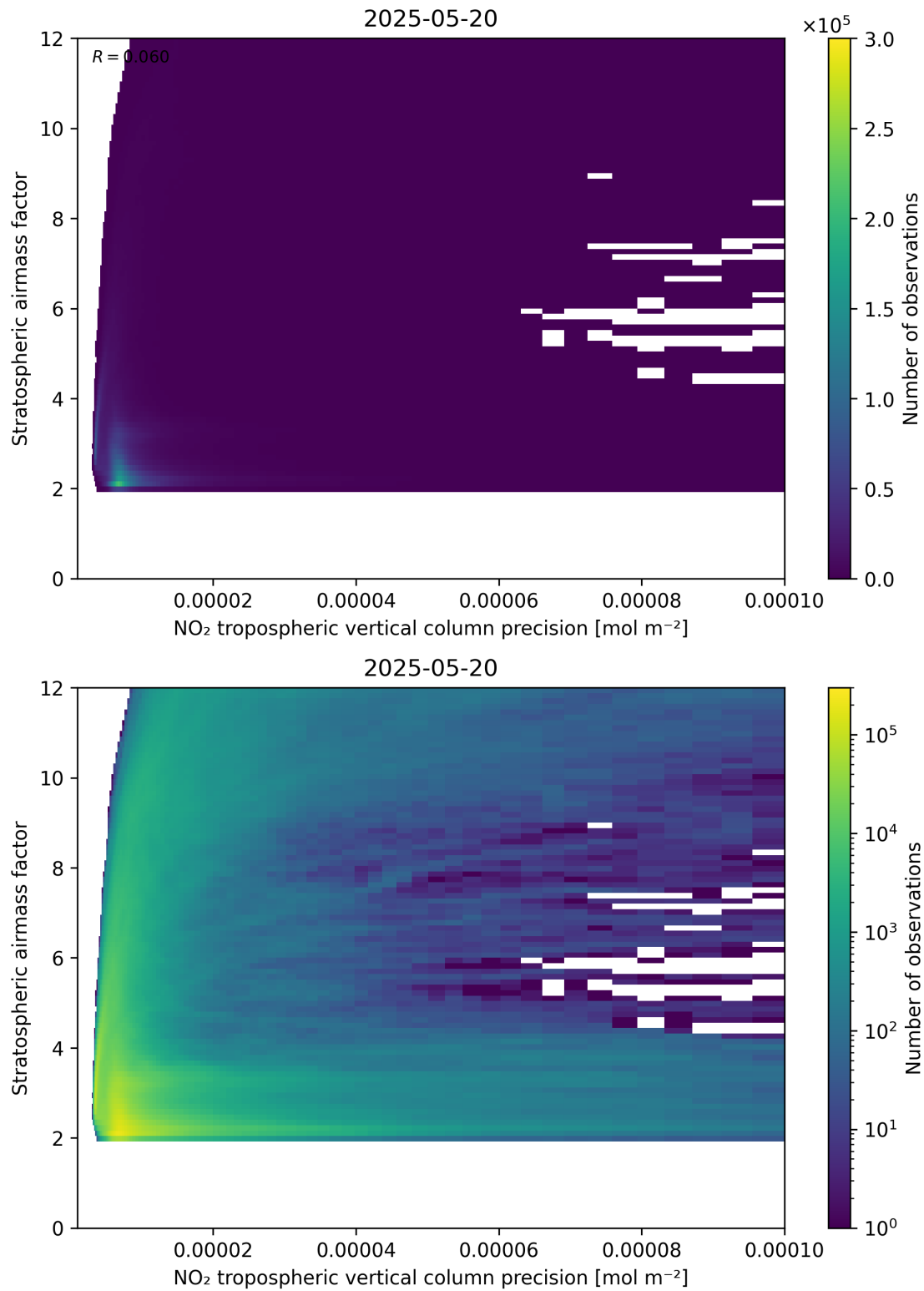
Figure 131: Scatter density plot of “NO 2 tropospheric vertical column precision” against “Stratospheric airmass factor” for 2025-05-19 to 2025-05-21.
