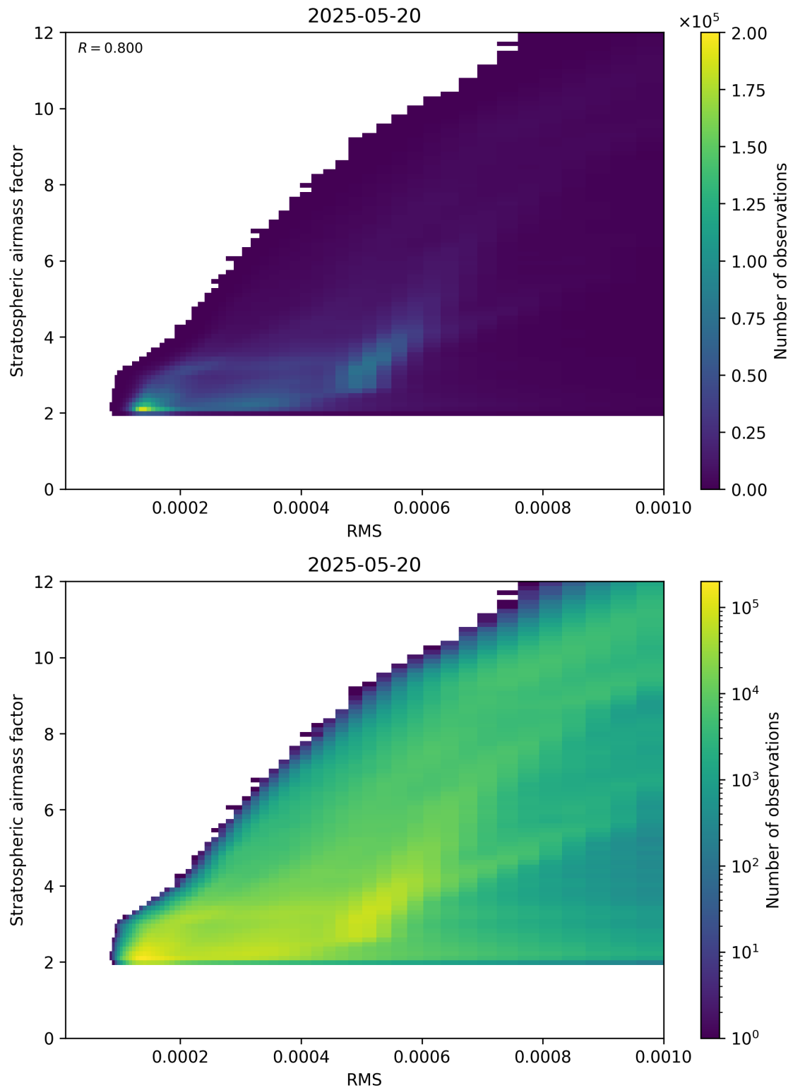
Figure 144: Scatter density plot of “RMS” against “Stratospheric airmass factor” for 2025-05-19 to 2025-05-21.
