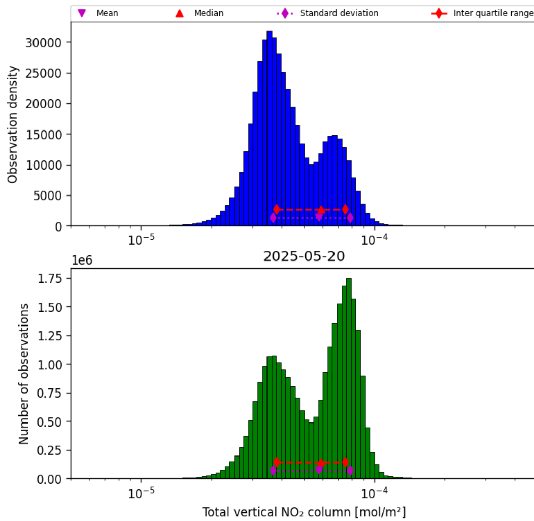
Figure 38: Histogram of "Total vertical NO 2 column" for 2025-05-19 to 2025-05-21
