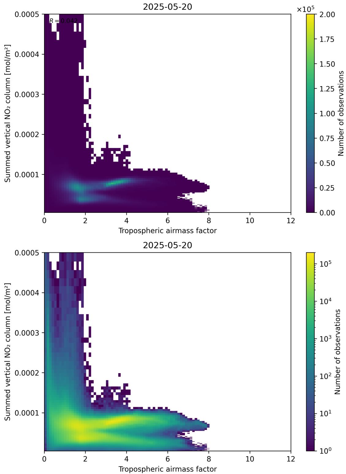
Figure 75: Scatter density plot of “Tropospheric airmass factor” against “Summed vertical NO 2 column” for 2025-05-19 to 2025-05-21.
