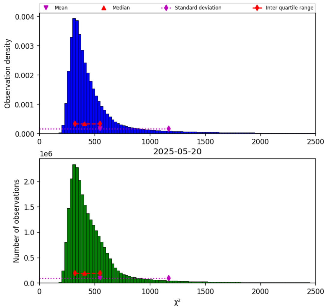
Figure 42: Histogram of “ \chi^2 ” for 2025-05-19 to 2025-05-21
