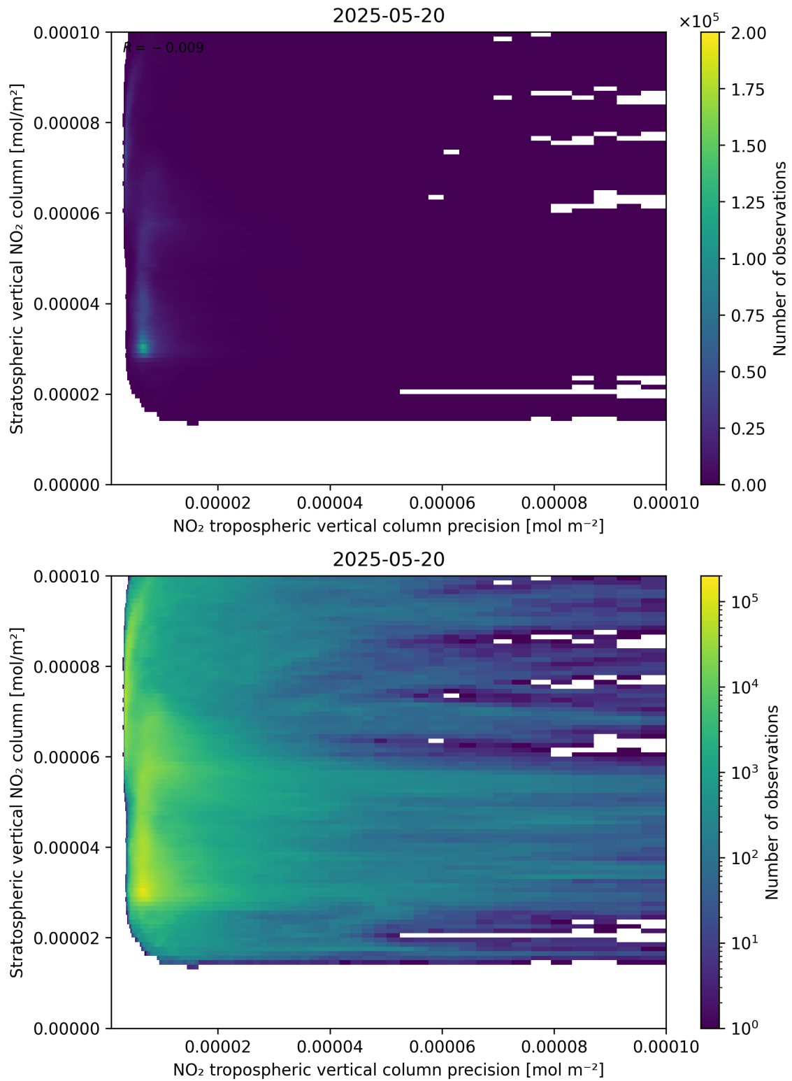
Figure 135: Scatter density plot of “NO 2 tropospheric vertical column precision” against “Stratospheric vertical NO 2 column” for 2025-05-19 to 2025-05-21.
