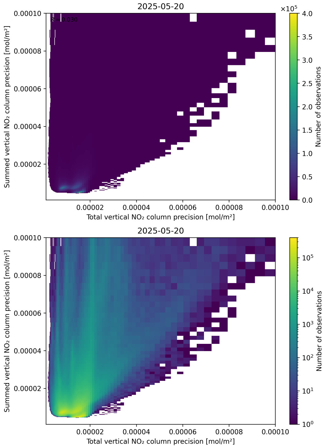
Figure 118: Scatter density plot of “Total vertical NO 2 column precision” against “Summed vertical NO 2 column precision” for 2025-05-19 to 2025-05-21.
