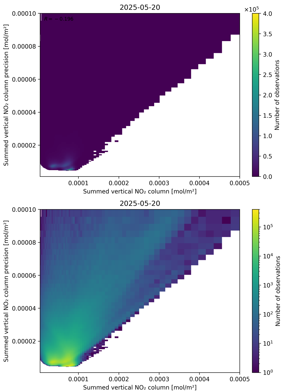
Figure 105: Scatter density plot of “Summed vertical NO 2 column” against “Summed vertical NO 2 column precision” for 2025-05-19 to 2025-05-21.
