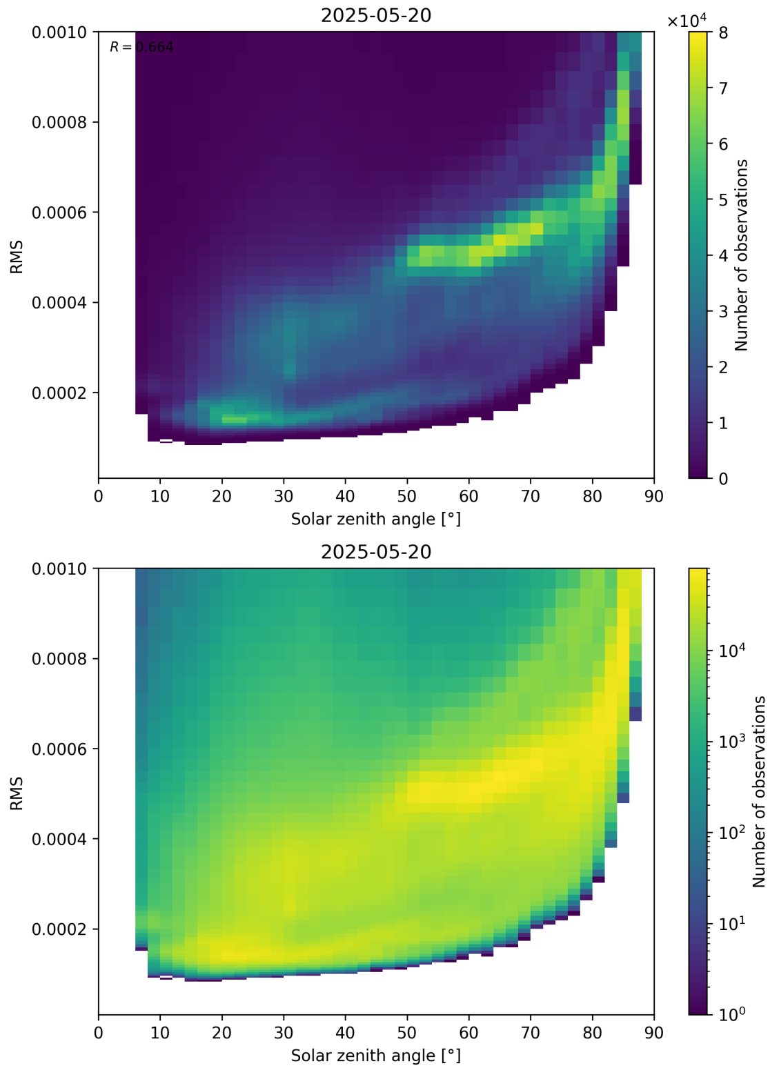
Figure 157: Scatter density plot of “Solar zenith angle” against “RMS” for 2025-05-19 to 2025-05-21.
