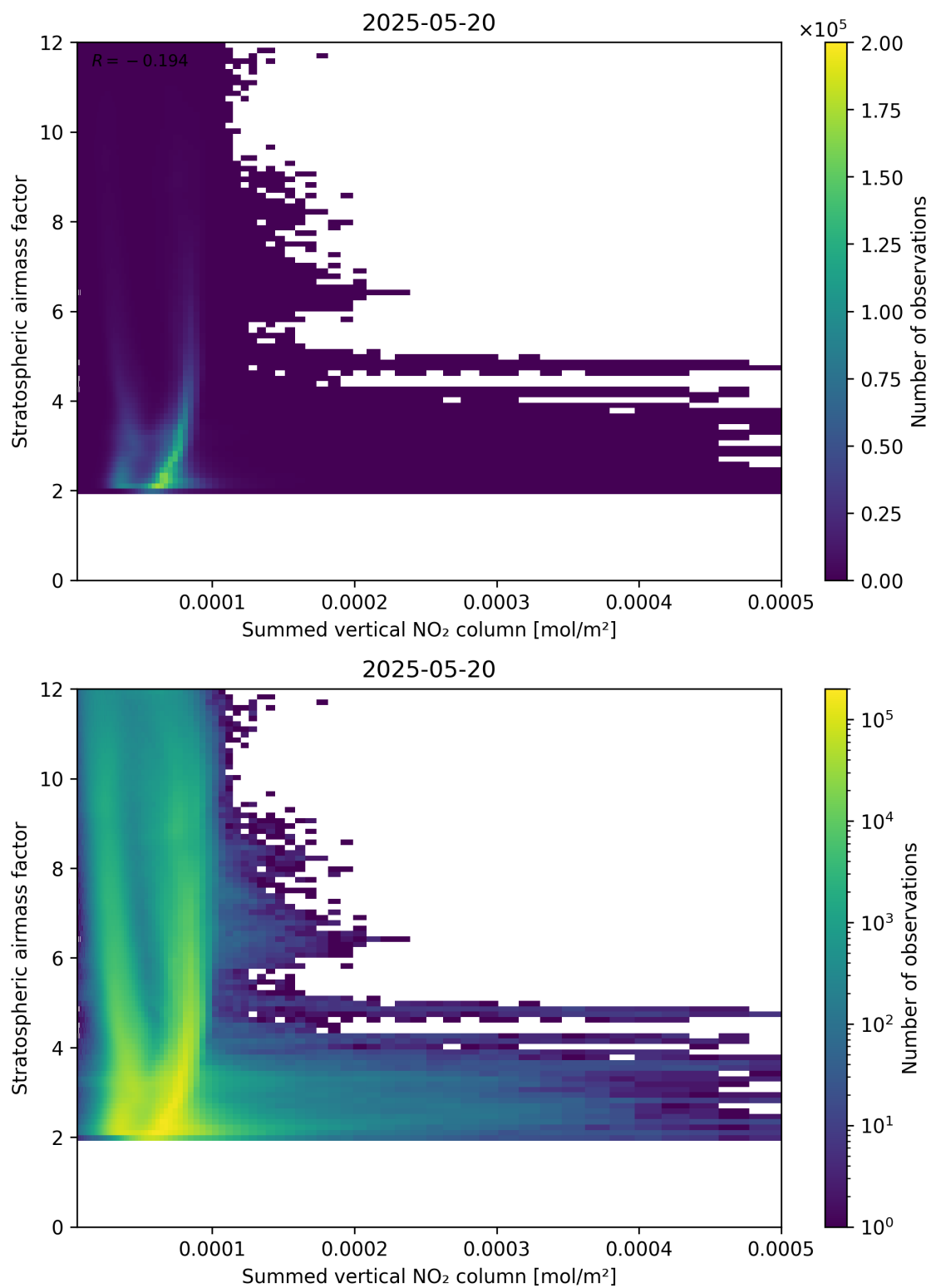
Figure 103: Scatter density plot of “Summed vertical NO 2 column” against “Stratospheric air mass factor” for 2025-05-19 to 2025-05-21.
