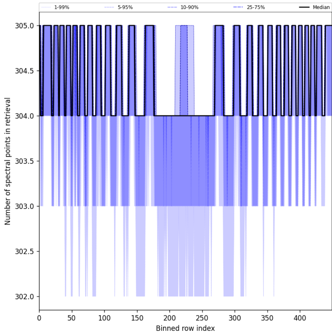
Figure 50: Along track statistics of “Number of spectral points in retrieval” for 2025-05-19 to 2025-05-21
