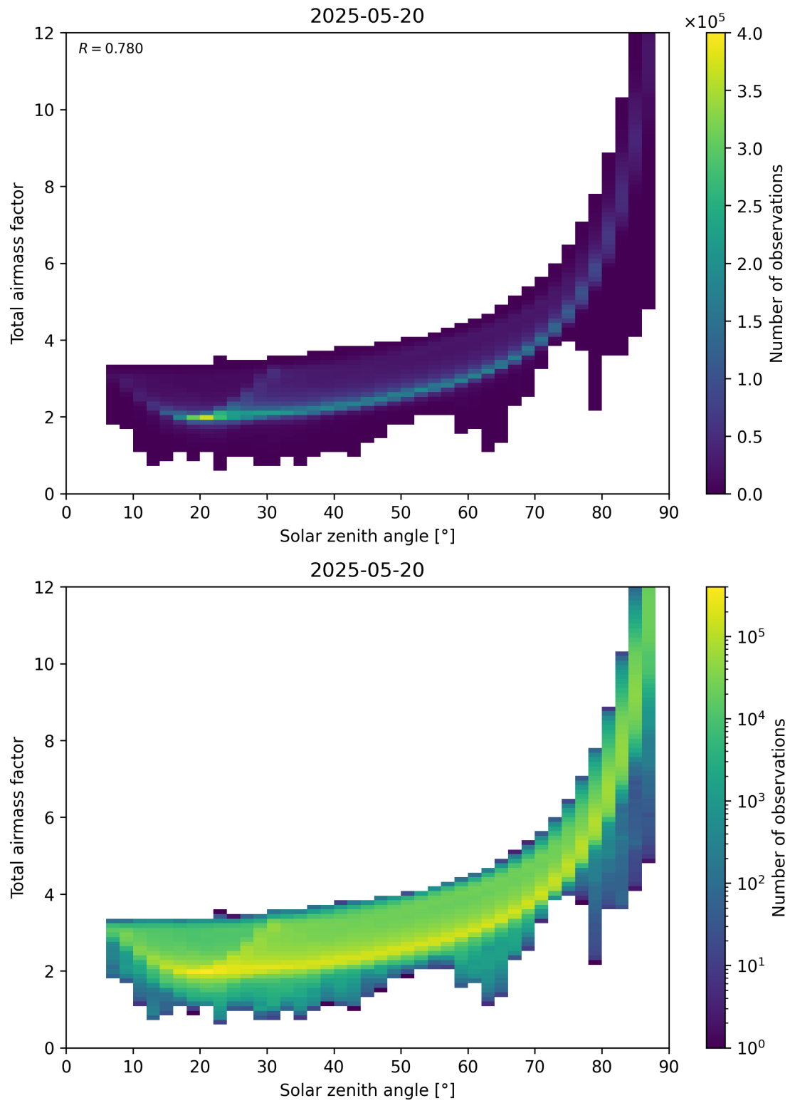
Figure 146: Scatter density plot of “Solar zenith angle” against “Total air mass factor” for 2025-05-19 to 2025-05-21.
