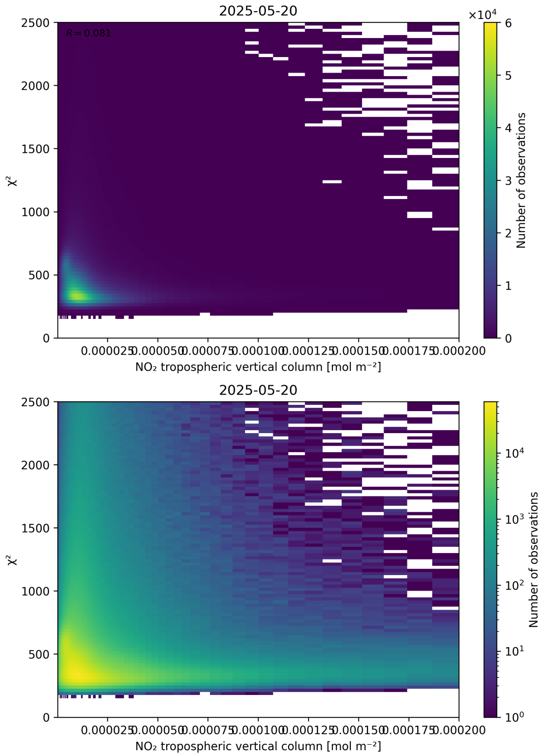
Figure 124: Scatter density plot of “NO 2 tropospheric vertical column” against “ \chi^2 ” for 2025-05-19 to 2025-05-21.
