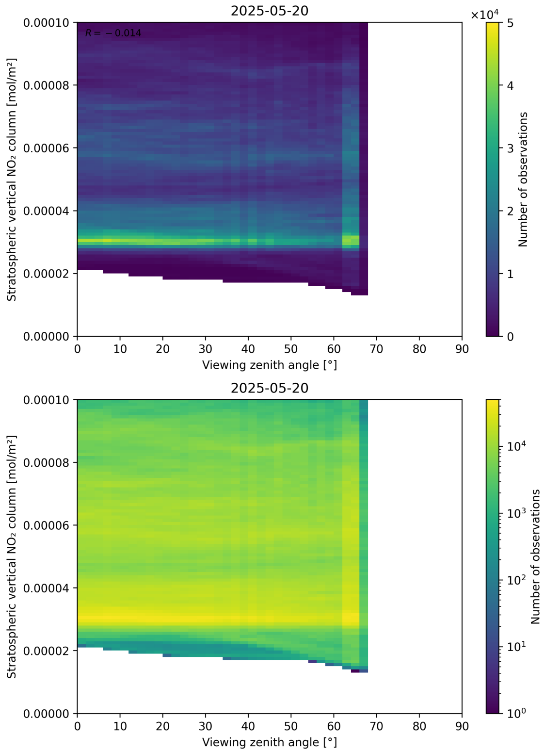
Figure 164: Scatter density plot of “Viewing zenith angle” against “Stratospheric vertical NO 2 column” for 2025-05-19 to 2025-05-21.
