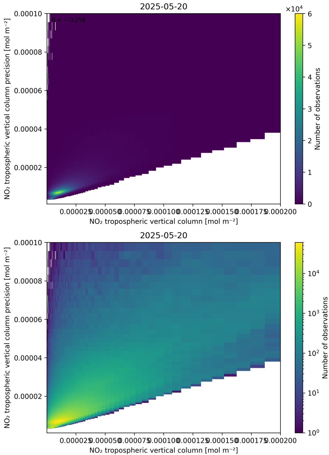
Figure 130: Scatter density plot of “NO 2 tropospheric vertical column” against “NO 2 tropospheric vertical column precision” for 2025-05-19 to 2025-05-21.
