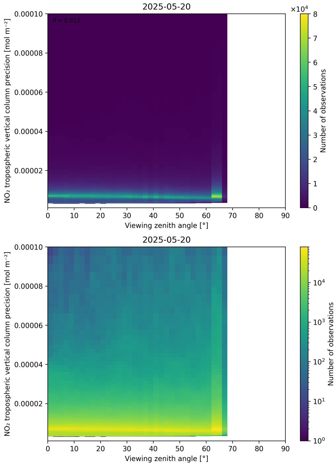
Figure 170: Scatter density plot of “Viewing zenith angle” against “NO 2 tropospheric vertical column precision” for 2025-05-19 to 2025-05-21.
