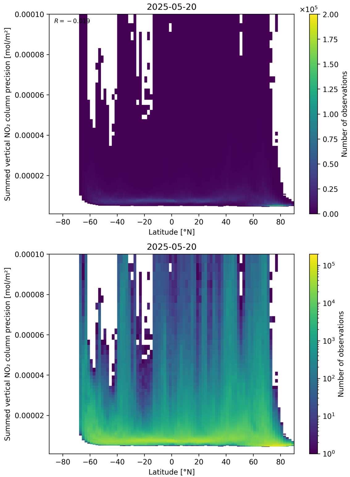
Figure 89: Scatter density plot of “Latitude” against “Summed vertical NO 2 column precision” for 2025-05-19 to 2025-05-21.
