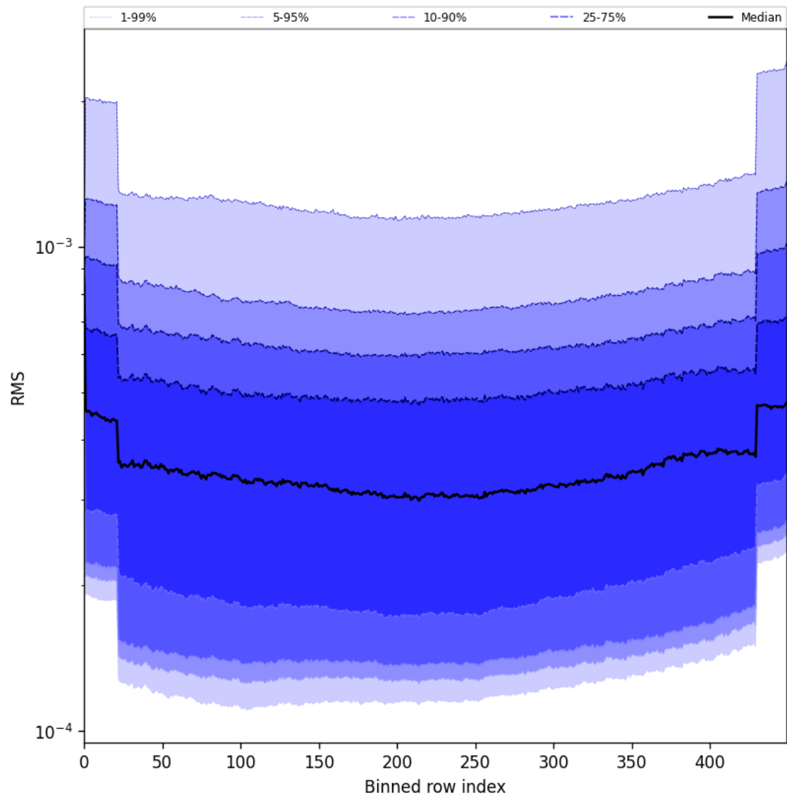
Figure 60: Along track statistics of “RMS” for 2025-05-19 to 2025-05-21
