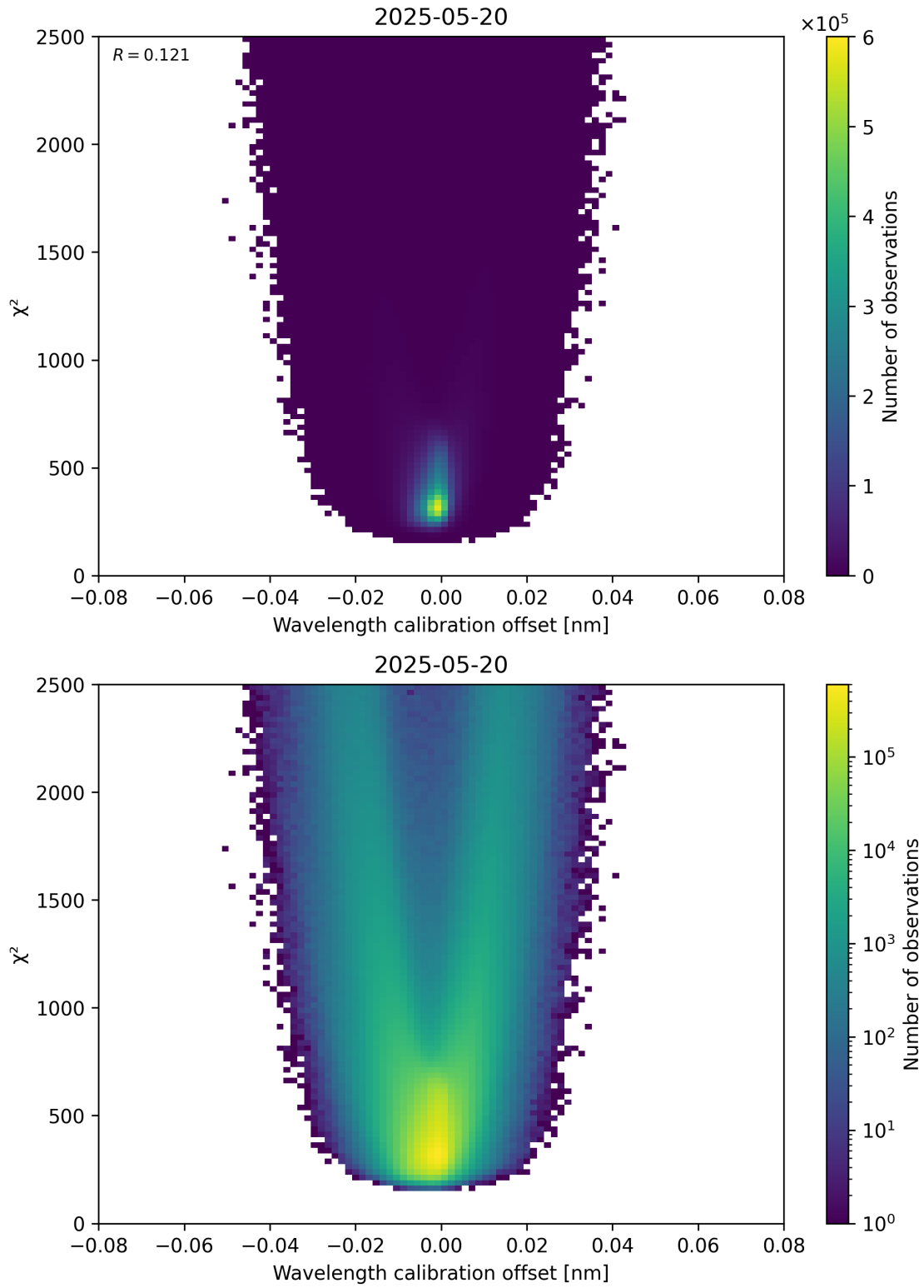
Figure 175: Scatter density plot of “Wavelength calibration offset” against “ \chi^2 ” for 2025-05-19 to 2025-05-21.
