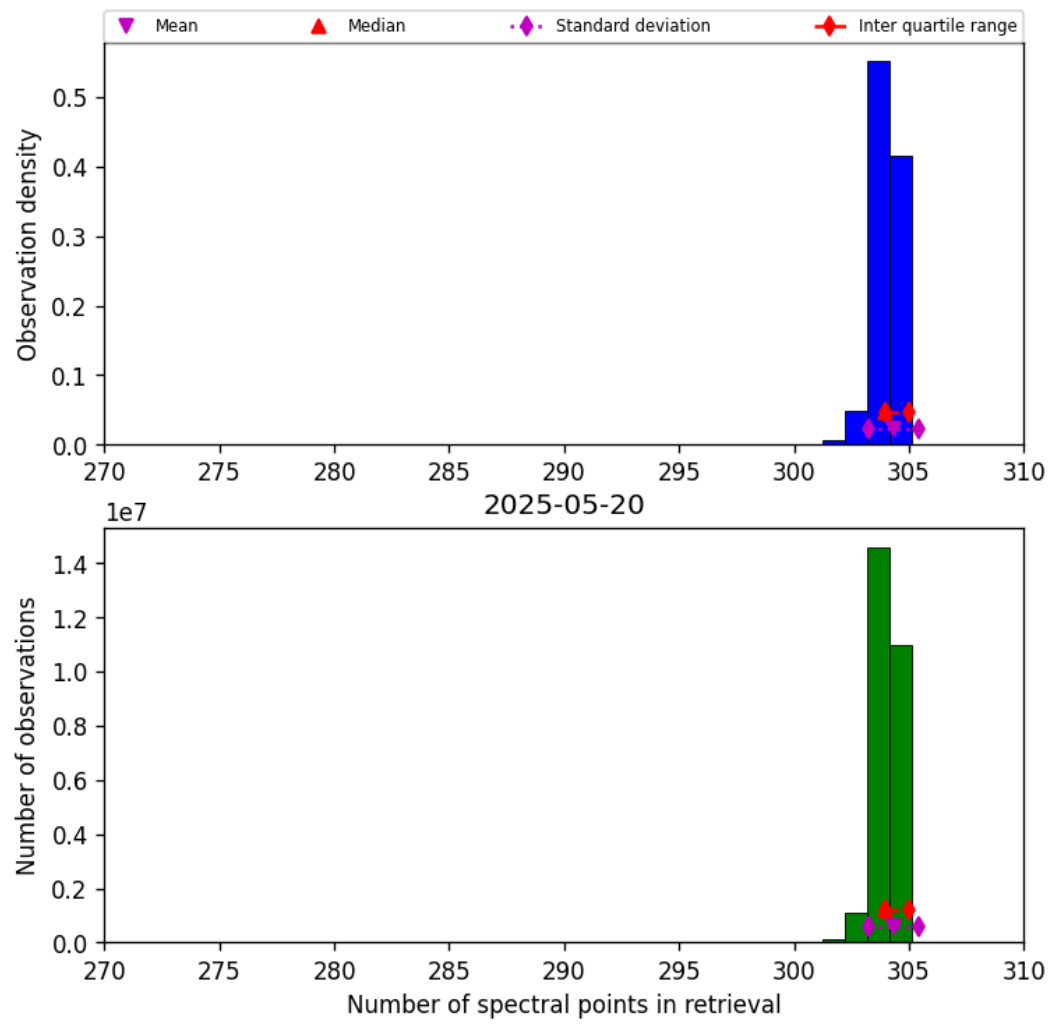
Figure 33: Histogram of “Number of spectral points in retrieval” for 2025-05-19 to 2025-05-21
