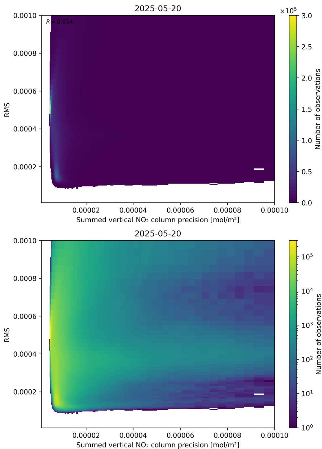
Figure 108: Scatter density plot of “Summed vertical NO 2 column precision” against “RMS” for 2025-05-19 to 2025-05-21.
