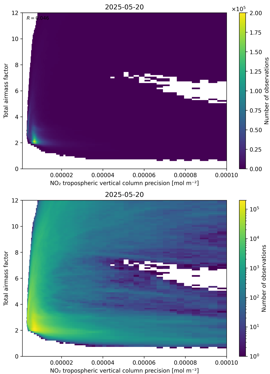
Figure 132: Scatter density plot of “NO 2 tropospheric vertical column precision” against “Total air mass factor” for 2025-05-19 to 2025-05-21.
