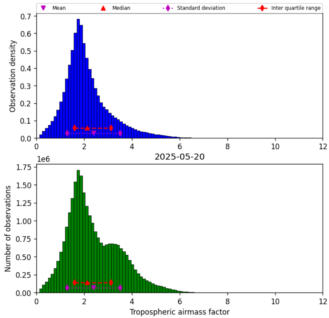
Figure 31: Histogram of “Tropospheric airmass factor” for 2025-05-19 to 2025-05-21
