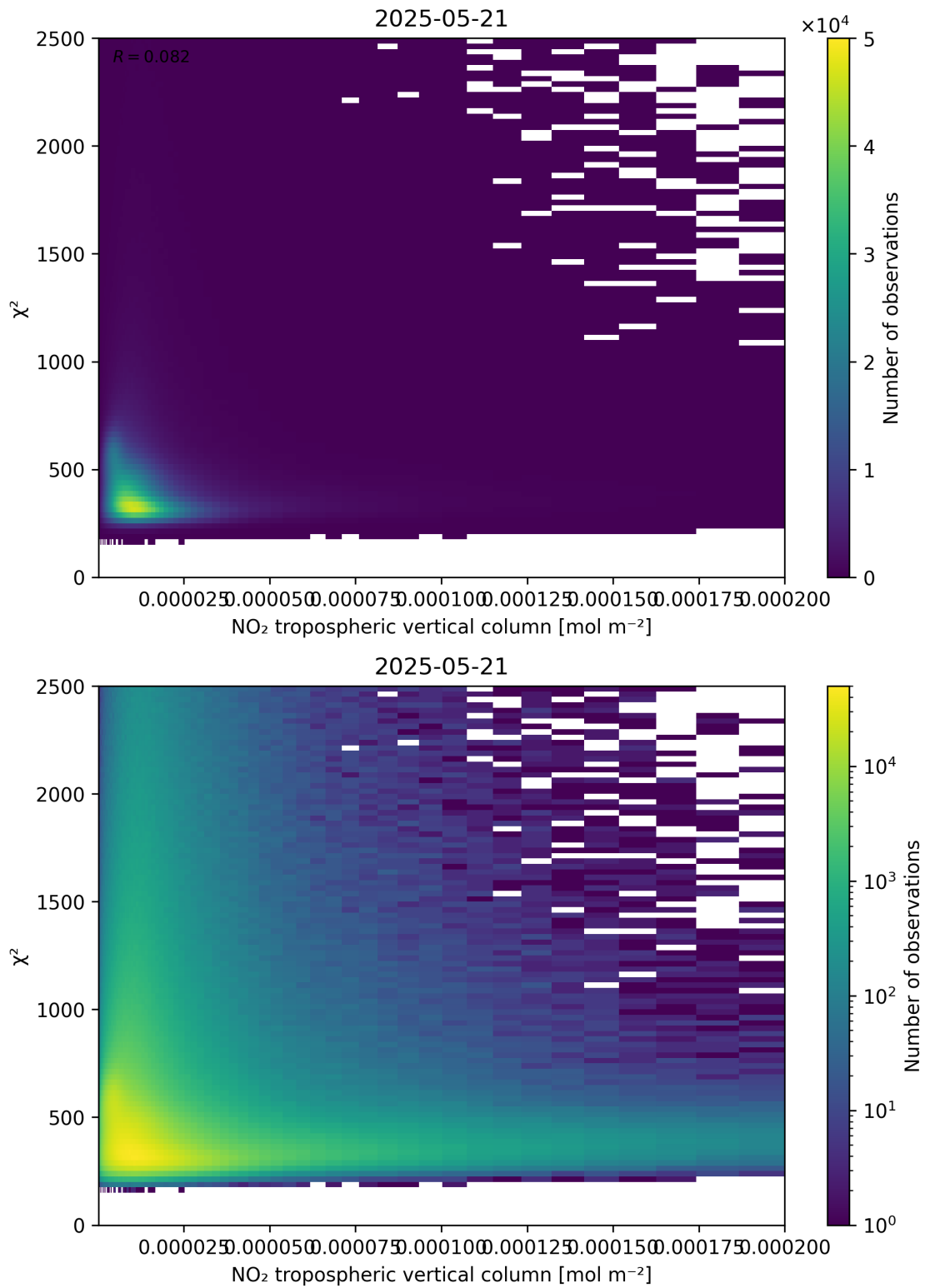
Figure 124: Scatter density plot of “NO 2 tropospheric vertical column” against “ \chi^2 ” for 2025-05-21 to 2025-05-22.
