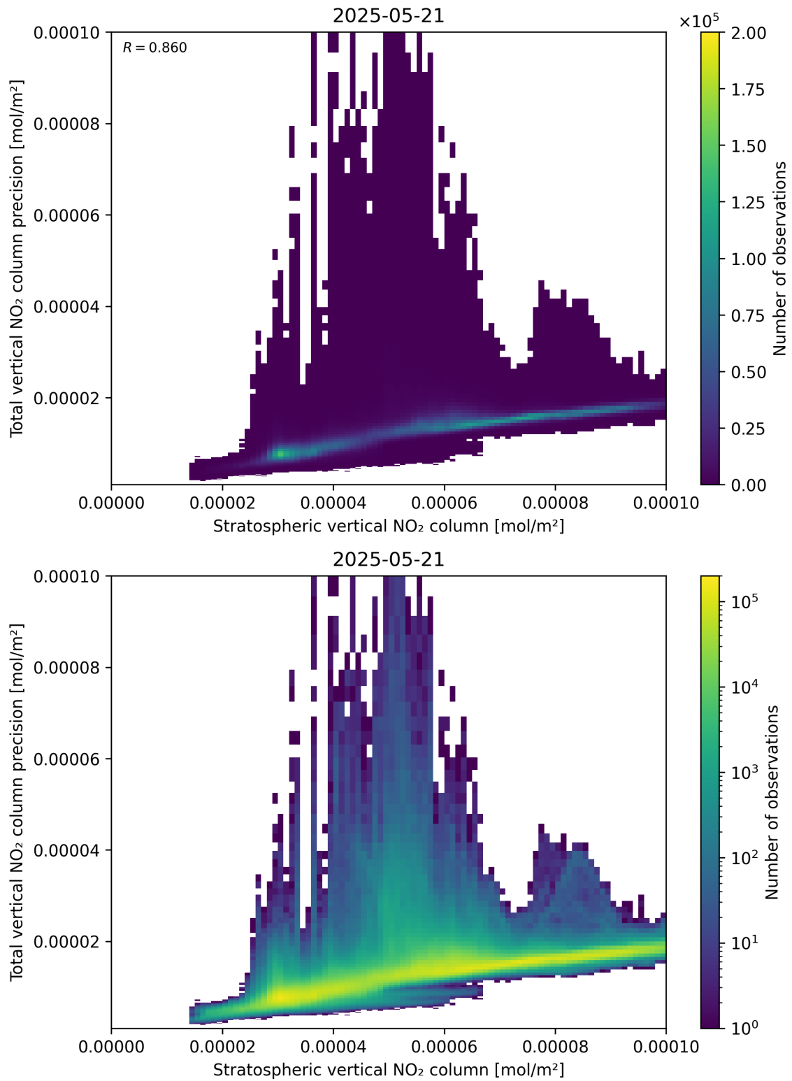
Figure 101: Scatter density plot of “Stratospheric vertical NO 2 column” against “Total vertical NO 2 column precision” for 2025-05-21 to 2025-05-22.
