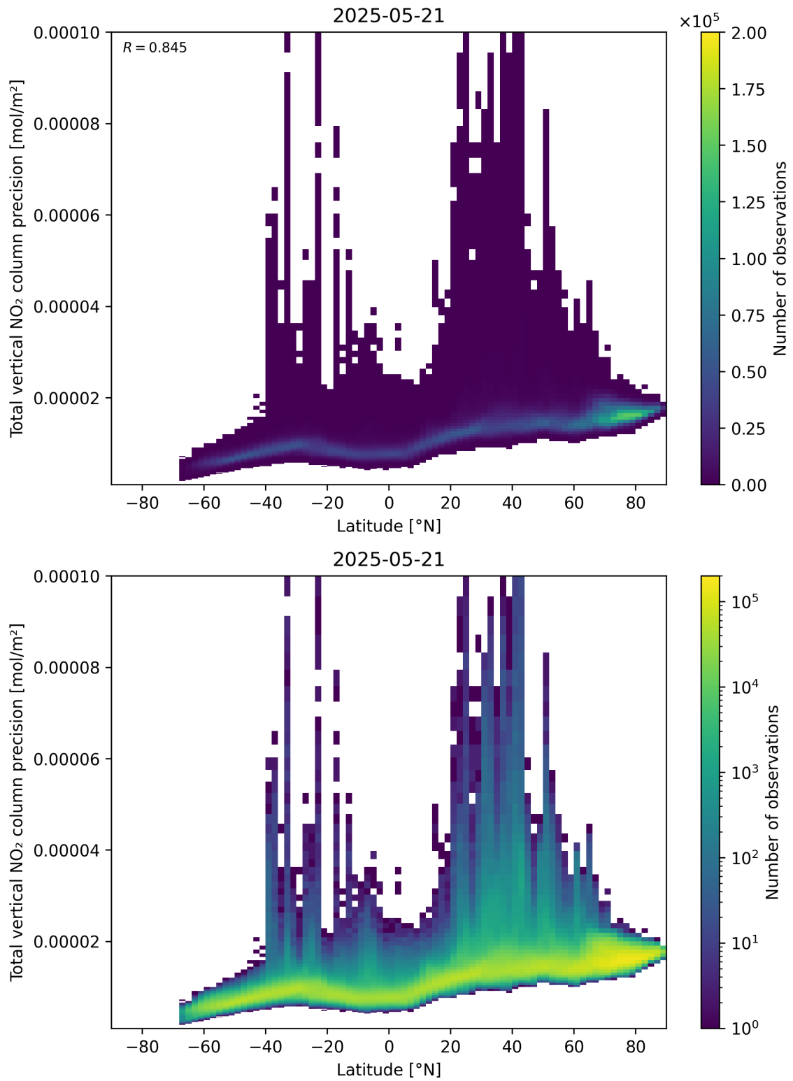
Figure 91: Scatter density plot of “Latitude” against “Total vertical NO 2 column precision” for 2025-05-21 to 2025-05-22.
