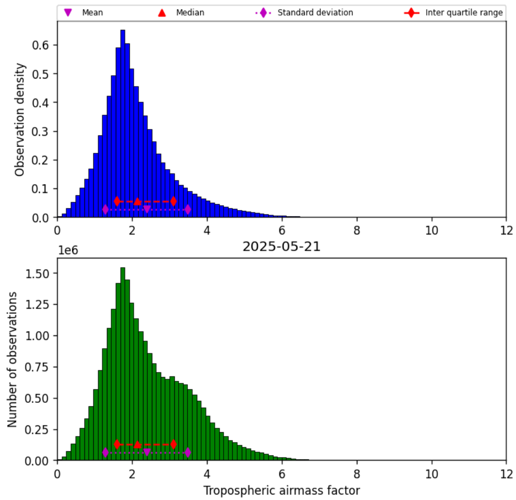
Figure 31: Histogram of “Tropospheric airmass factor” for 2025-05-21 to 2025-05-22
