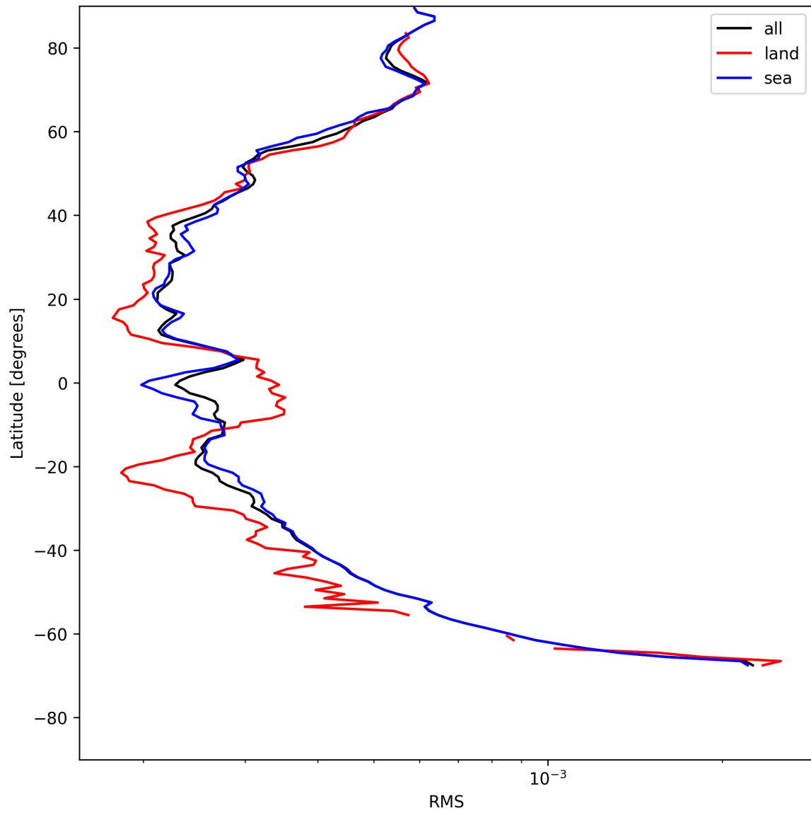
Figure 26: Zonal average of “RMS” for 2025-05-21 to 2025-05-22.
