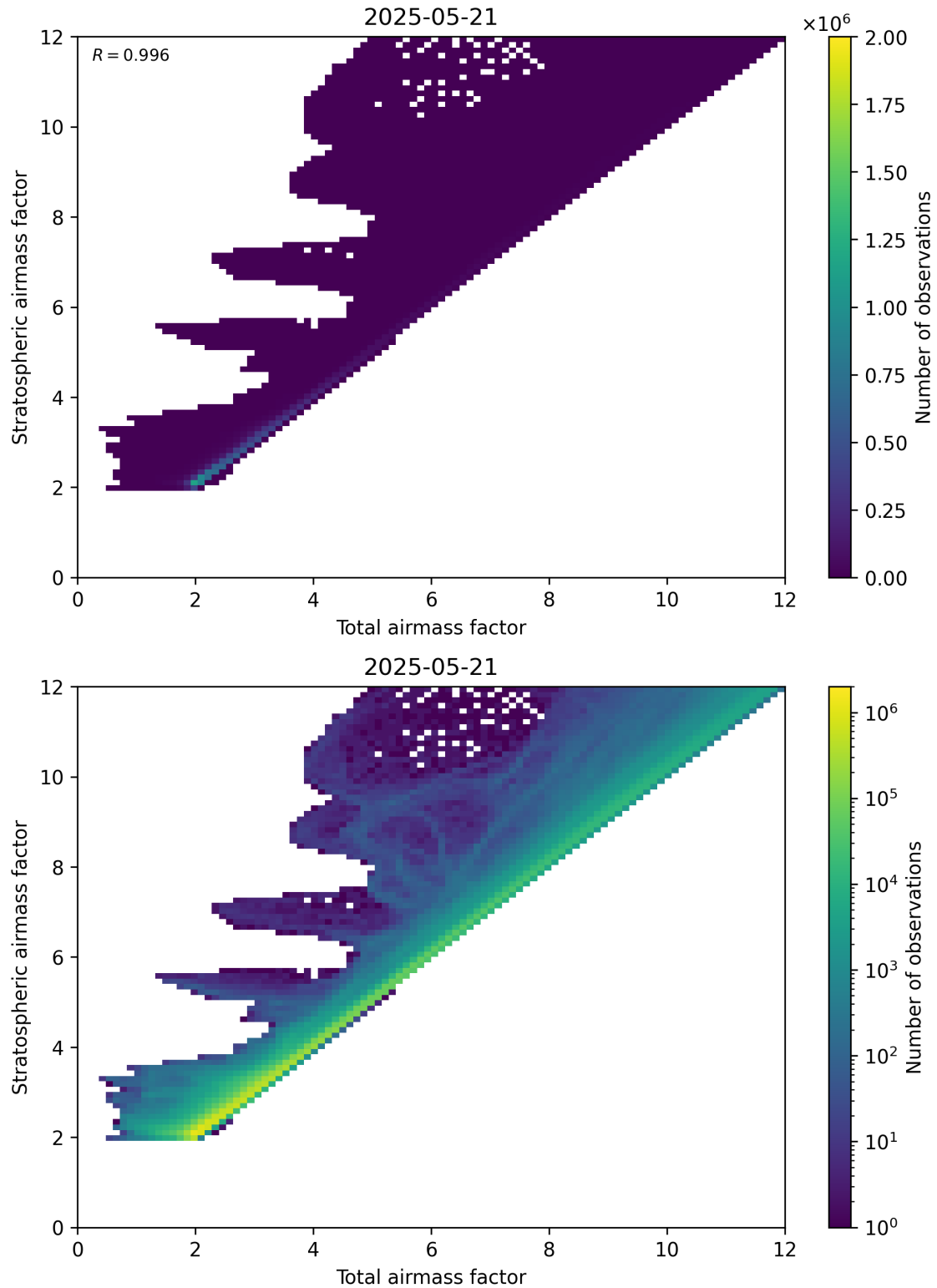
Figure 62: Scatter density plot of “Total airmass factor” against “Stratospheric airmass factor” for 2025-05-21 to 2025-05-22.
