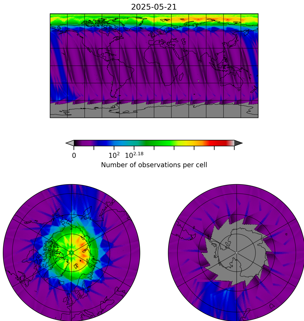
Figure 10: Map of the number of observations for 2025-05-21 to 2025-05-22
