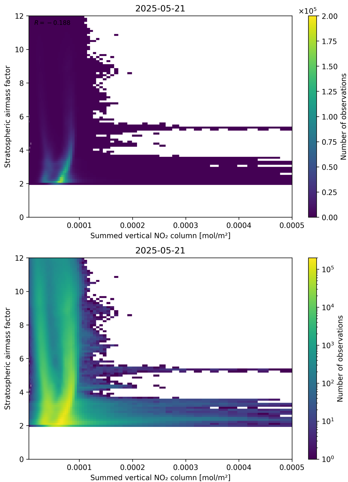
Figure 103: Scatter density plot of “Summed vertical NO 2 column” against “Stratospheric air mass factor” for 2025-05-21 to 2025-05-22.
