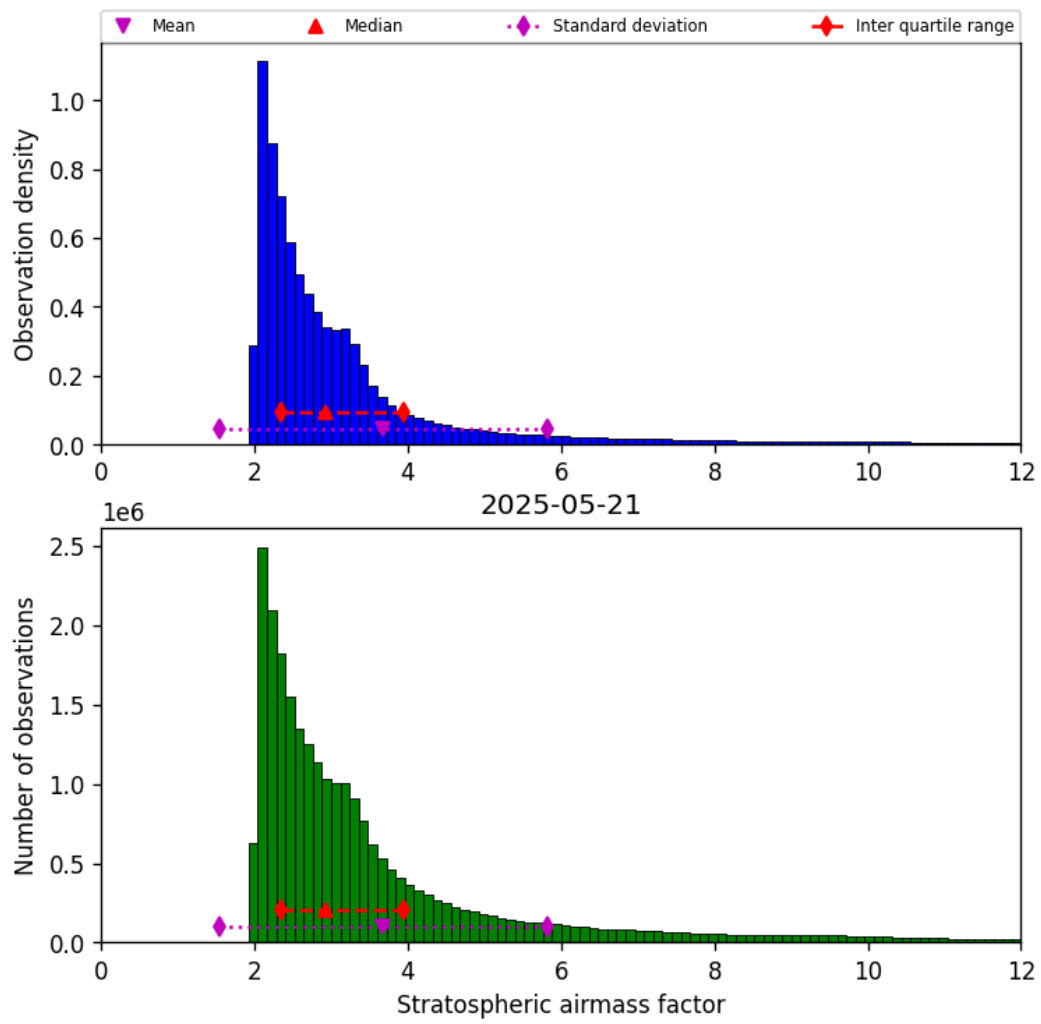
Figure 44: Histogram of “Stratospheric airmass factor” for 2025-05-21 to 2025-05-22
