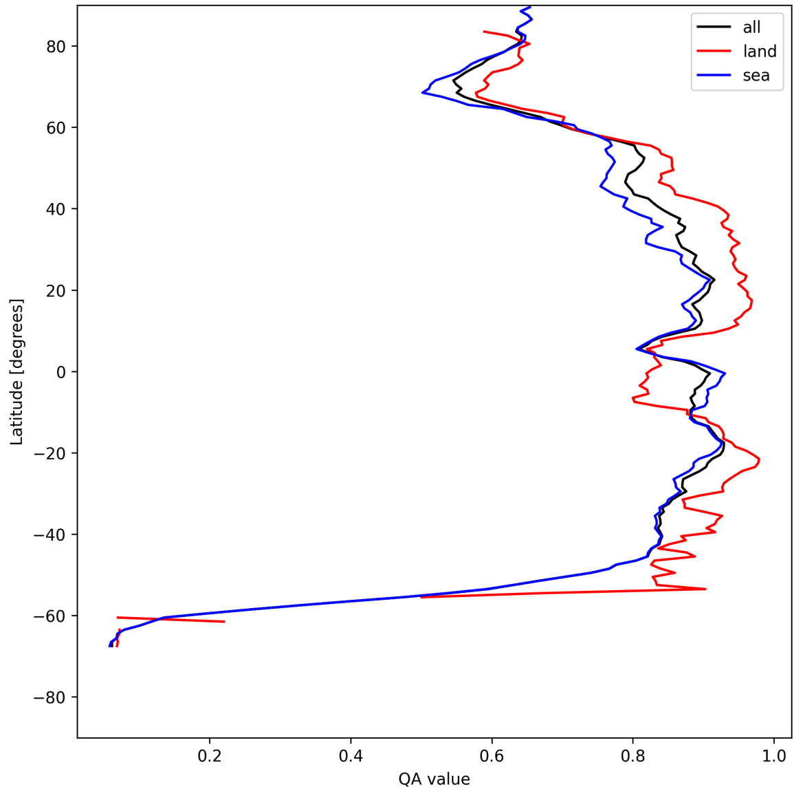
Figure 11: Zonal average of “QA value” for 2025-05-21 to 2025-05-22.
