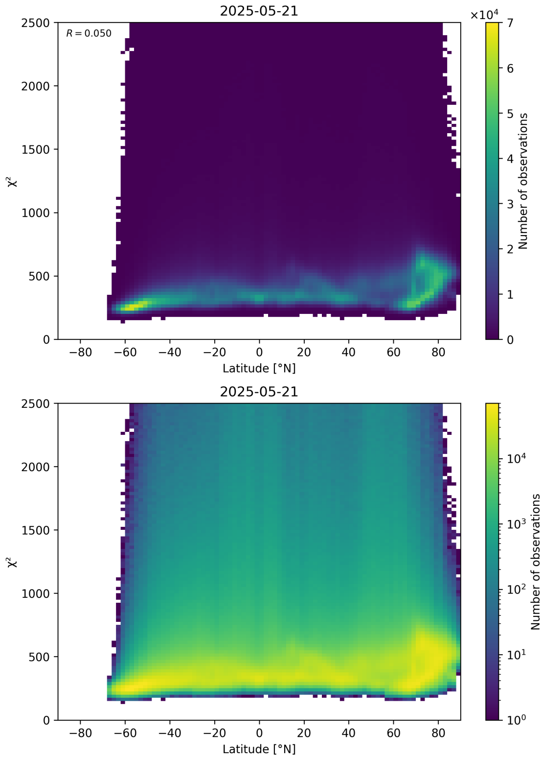
Figure 86: Scatter density plot of “Latitude” against “ \chi^2 ” for 2025-05-21 to 2025-05-22.
