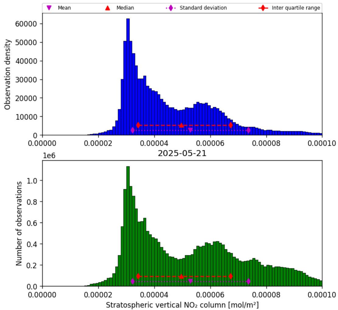
Figure 36: Histogram of “Stratospheric vertical NO 2 column” for 2025-05-21 to 2025-05-22
