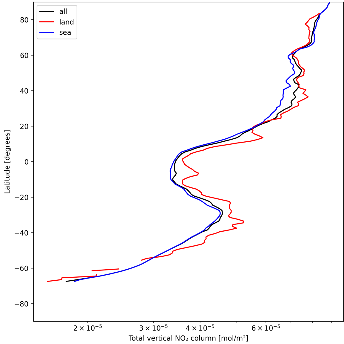
Figure 21: Zonal average of “Total vertical NO 2 column” for 2025-05-21 to 2025-05-22.
