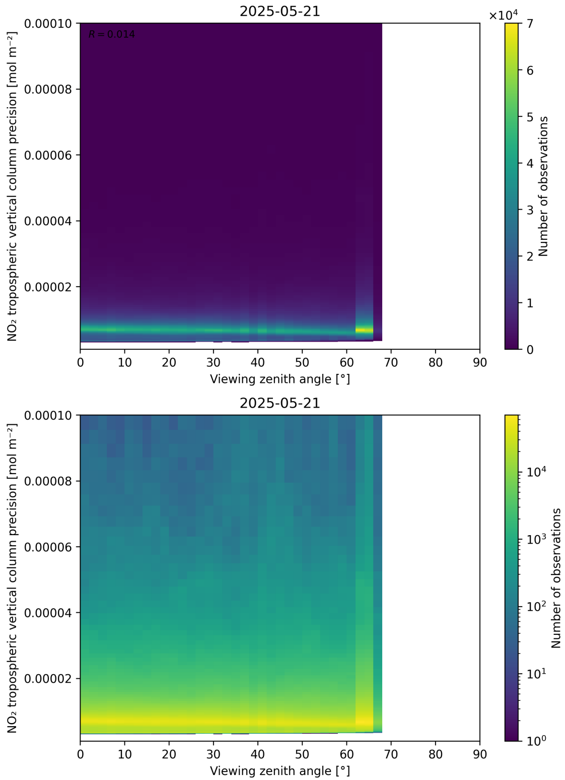
Figure 170: Scatter density plot of “Viewing zenith angle” against “NO 2 tropospheric vertical column precision” for 2025-05-21 to 2025-05-22.
