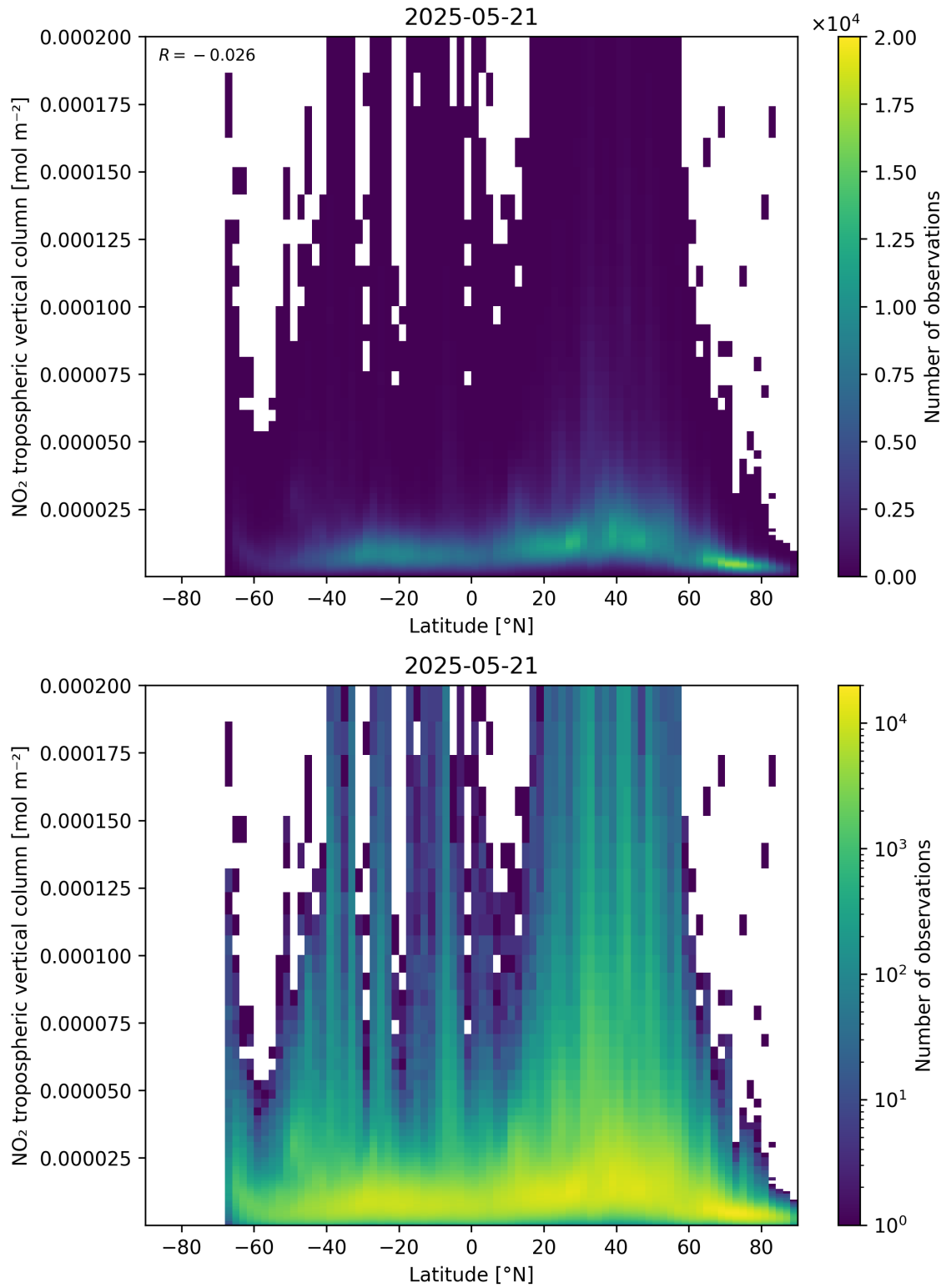
Figure 92: Scatter density plot of “Latitude” against “NO 2 tropospheric vertical column” for 2025-05-21 to 2025-05-22.
