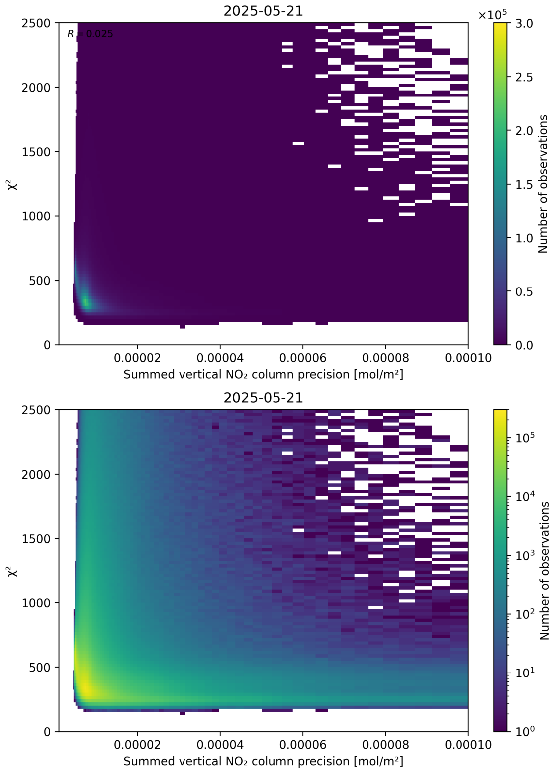
Figure 107: Scatter density plot of “Summed vertical NO 2 column precision” against “ \chi^2 ” for 2025-05-21 to 2025-05-22.
