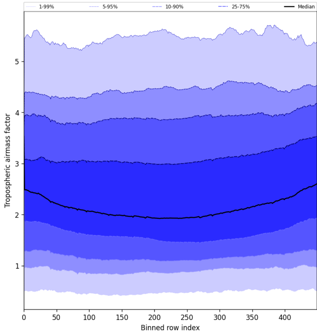
Figure 48: Along track statistics of “Tropospheric airmass factor” for 2025-05-21 to 2025-05-22
