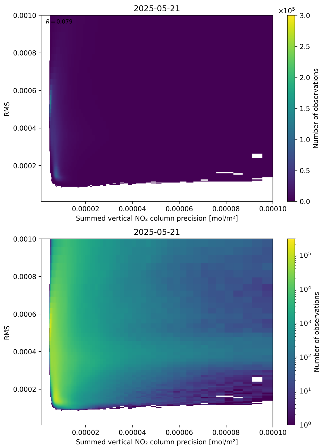
Figure 108: Scatter density plot of “Summed vertical NO 2 column precision” against “RMS” for 2025-05-21 to 2025-05-22.
