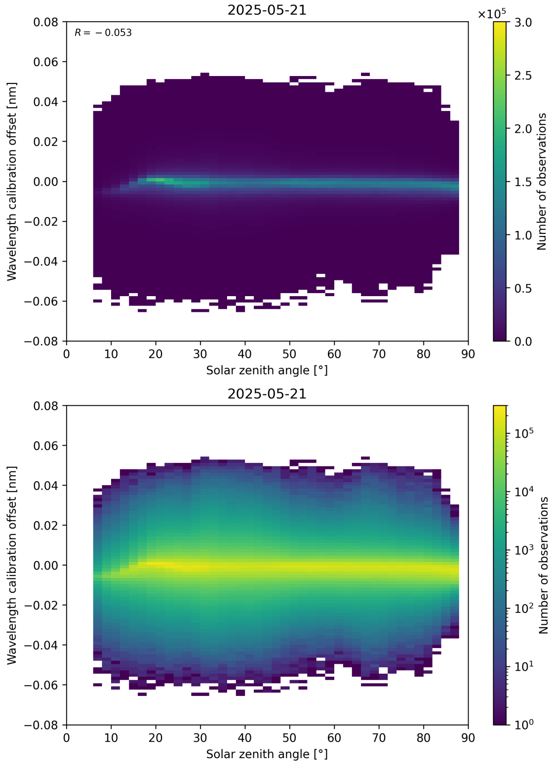
Figure 158: Scatter density plot of “Solar zenith angle” against “Wavelength calibration offset” for 2025-05-21 to 2025-05-22.
