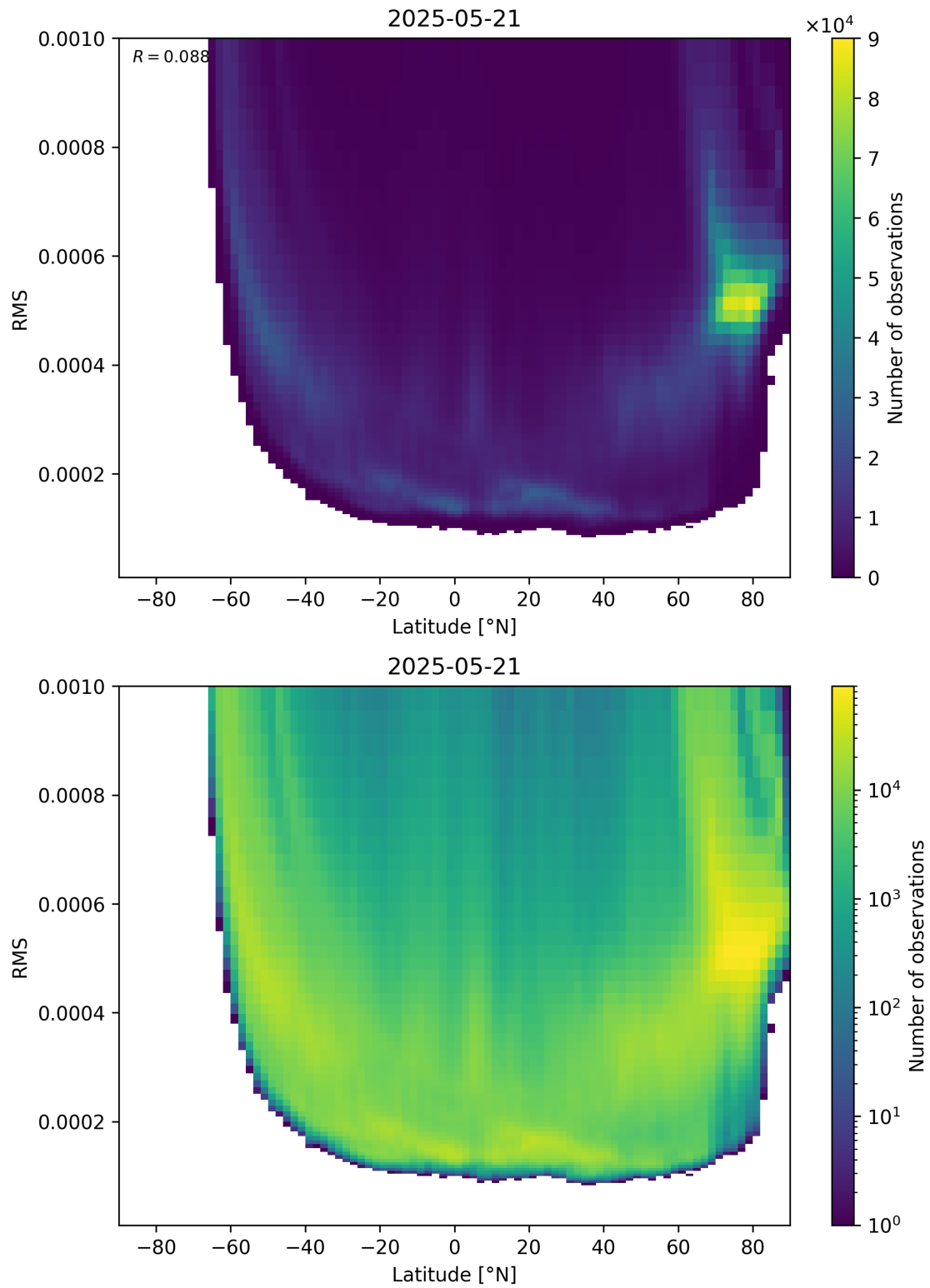
Figure 94: Scatter density plot of “Latitude” against “RMS” for 2025-05-21 to 2025-05-22.
