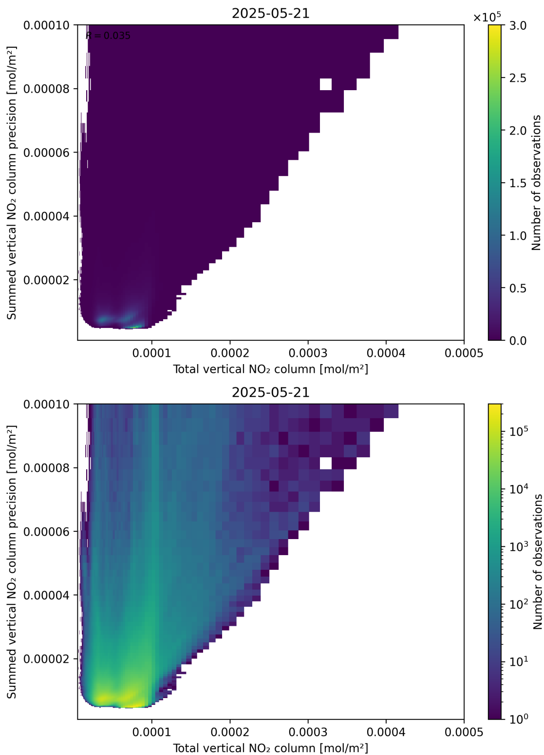
Figure 113: Scatter density plot of “Total vertical NO 2 column” against “Summed vertical NO 2 column precision” for 2025-05-21 to 2025-05-22.
