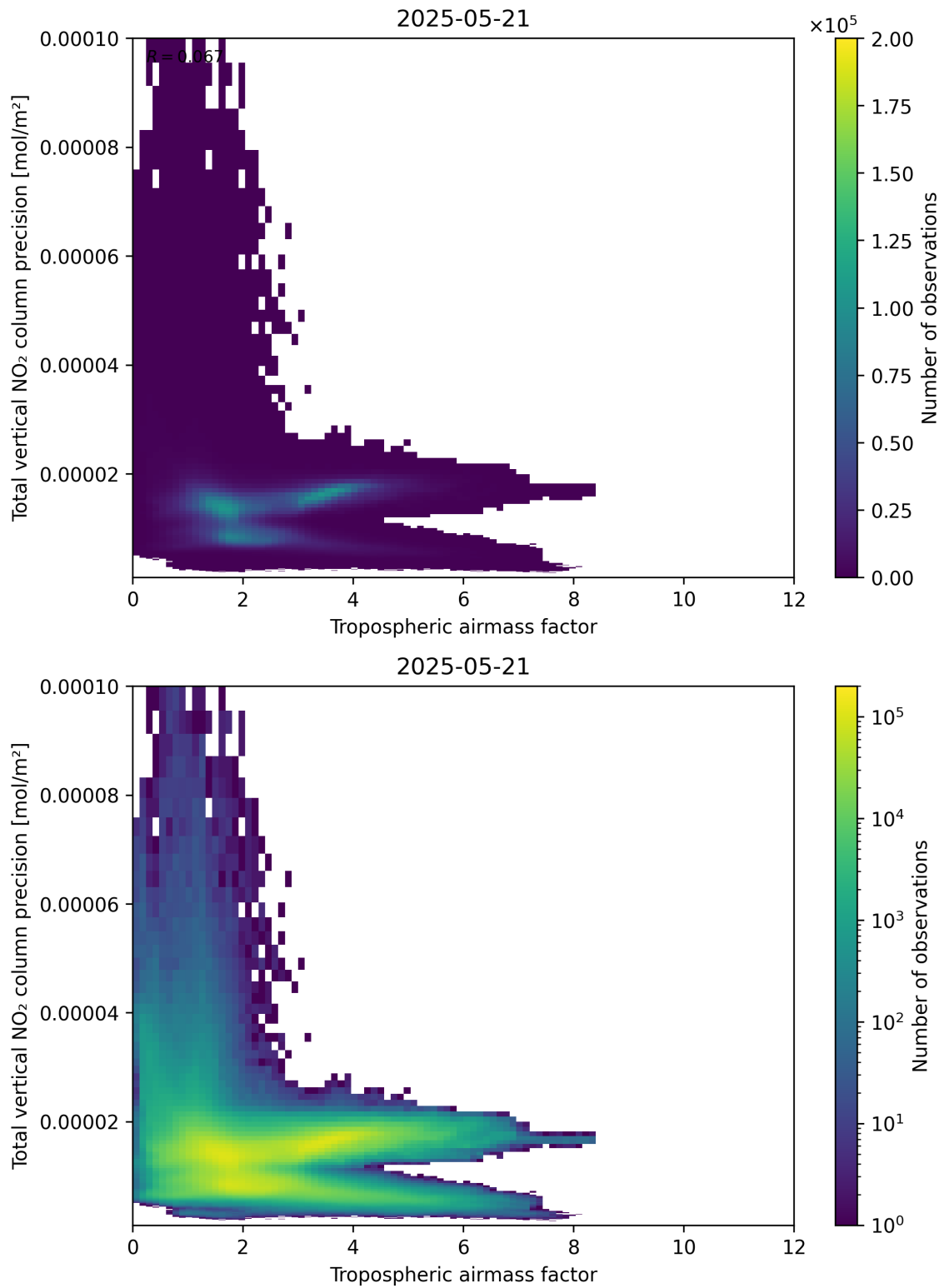
Figure 78: Scatter density plot of “Tropospheric air mass factor” against “Total vertical NO 2 column precision” for 2025-05-21 to 2025-05-22.
