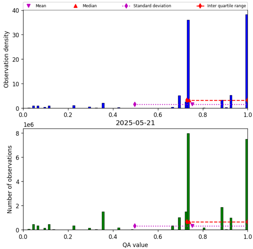
Figure 28: Histogram of “QA value” for 2025-05-21 to 2025-05-22
