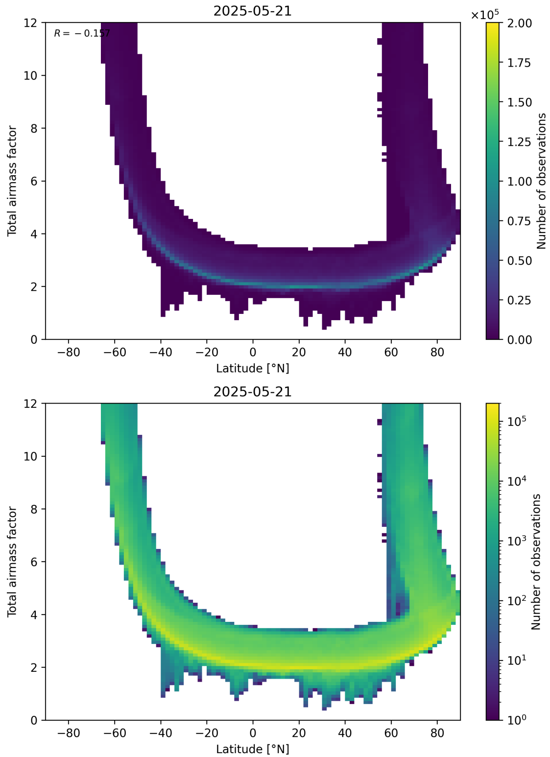
Figure 84: Scatter density plot of “Latitude” against “Total airmass factor” for 2025-05-21 to 2025-05-22.
