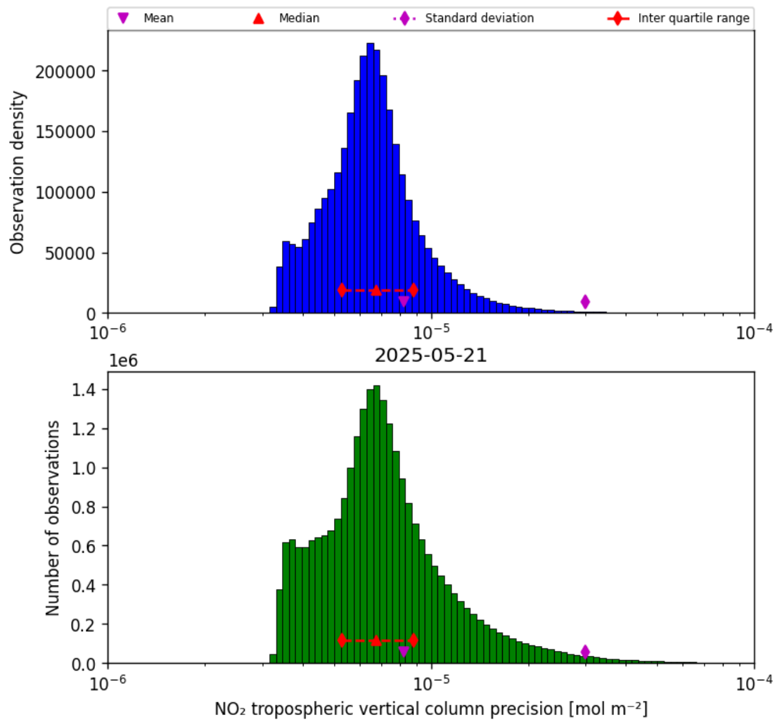
Figure 30: Histogram of “NO 2 tropospheric vertical column precision” for 2025-05-21 to 2025-05-22
