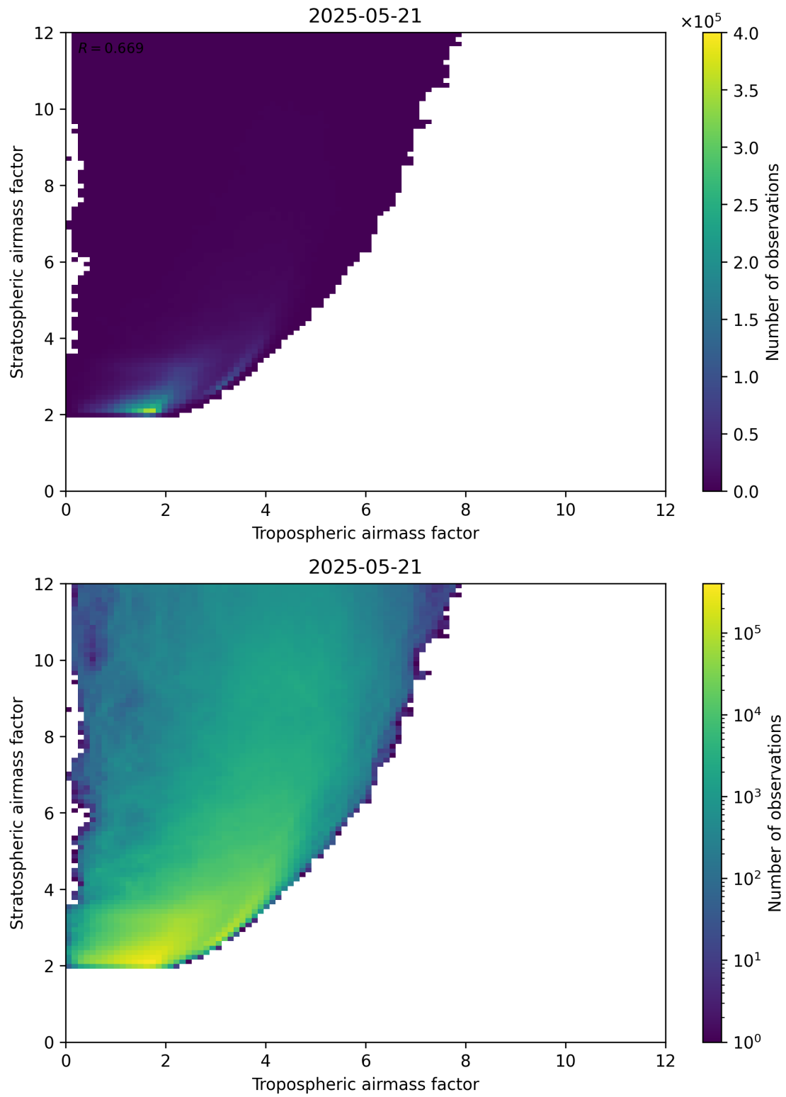
Figure 71: Scatter density plot of “Tropospheric airmass factor” against “Stratospheric airmass factor” for 2025-05-21 to 2025-05-22.
