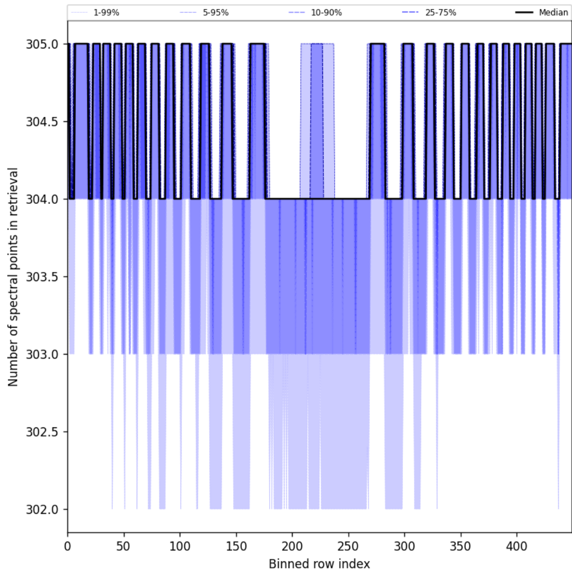
Figure 50: Along track statistics of “Number of spectral points in retrieval” for 2025-05-21 to 2025-05-22
