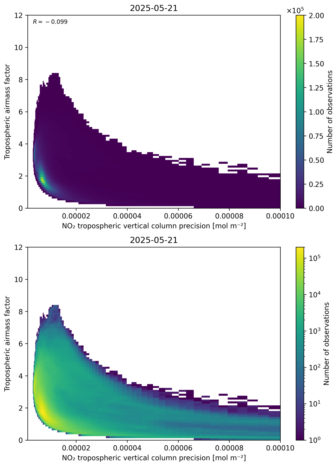
Figure 133: Scatter density plot of “NO 2 tropospheric vertical column precision” against “Tropospheric airmass factor” for 2025-05-21 to 2025-05-22.
