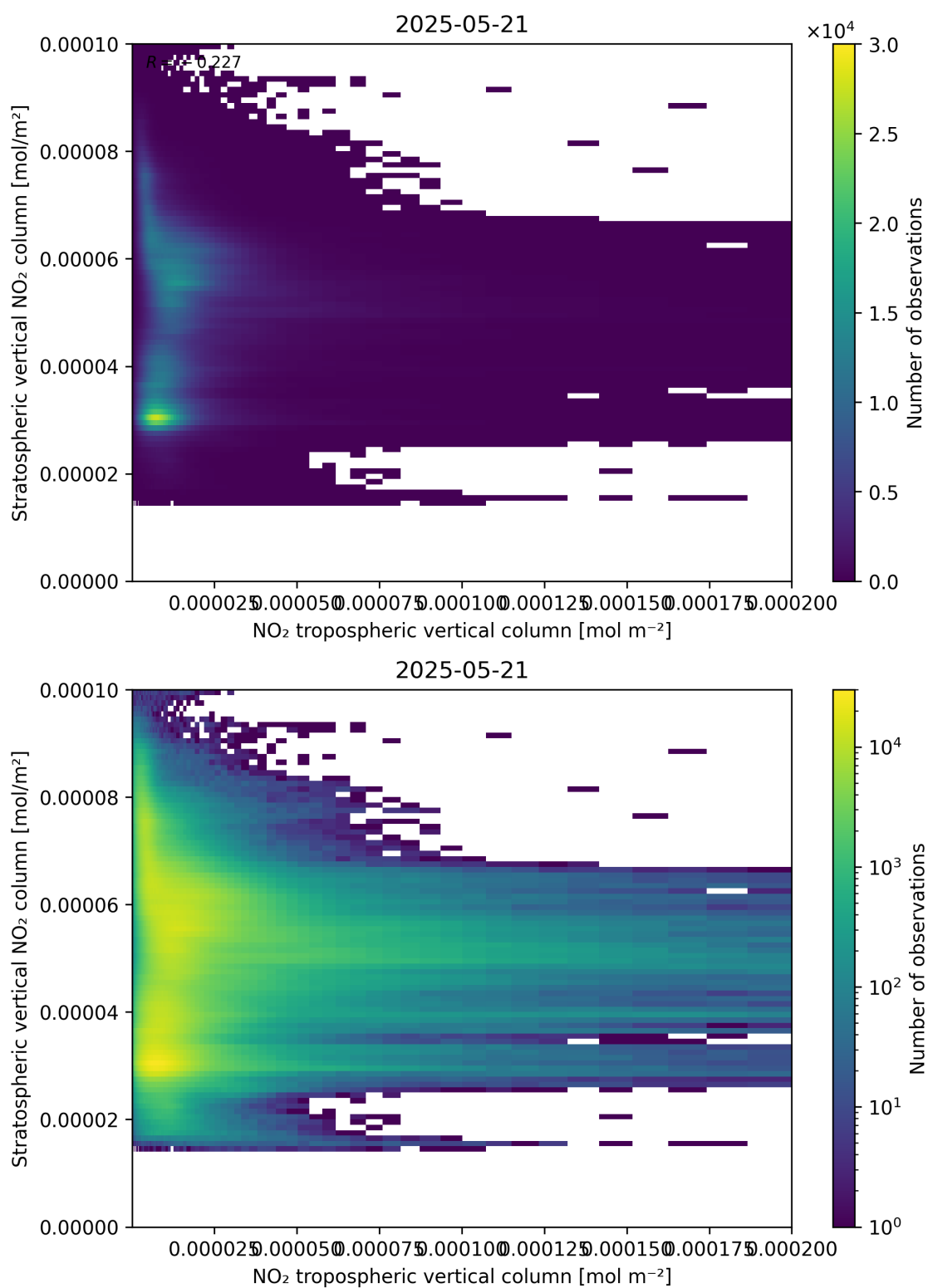
Figure 125: Scatter density plot of “NO 2 tropospheric vertical column” against “Stratospheric vertical NO 2 column” for 2025-05-21 to 2025-05-22.
