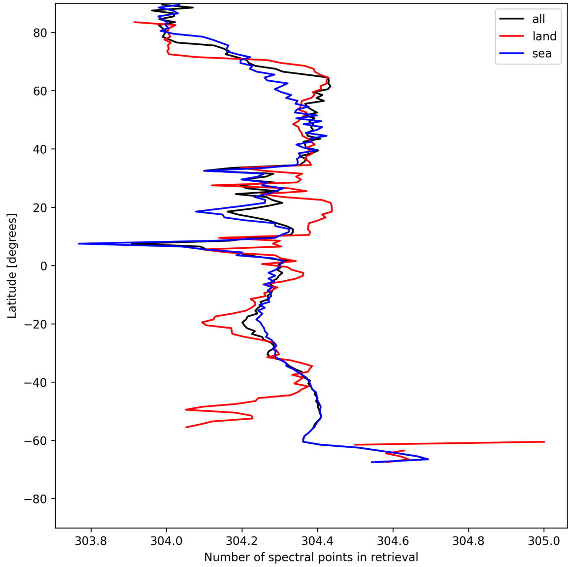
Figure 16: Zonal average of “Number of spectral points in retrieval” for 2025-05-21 to 2025-05-22.
