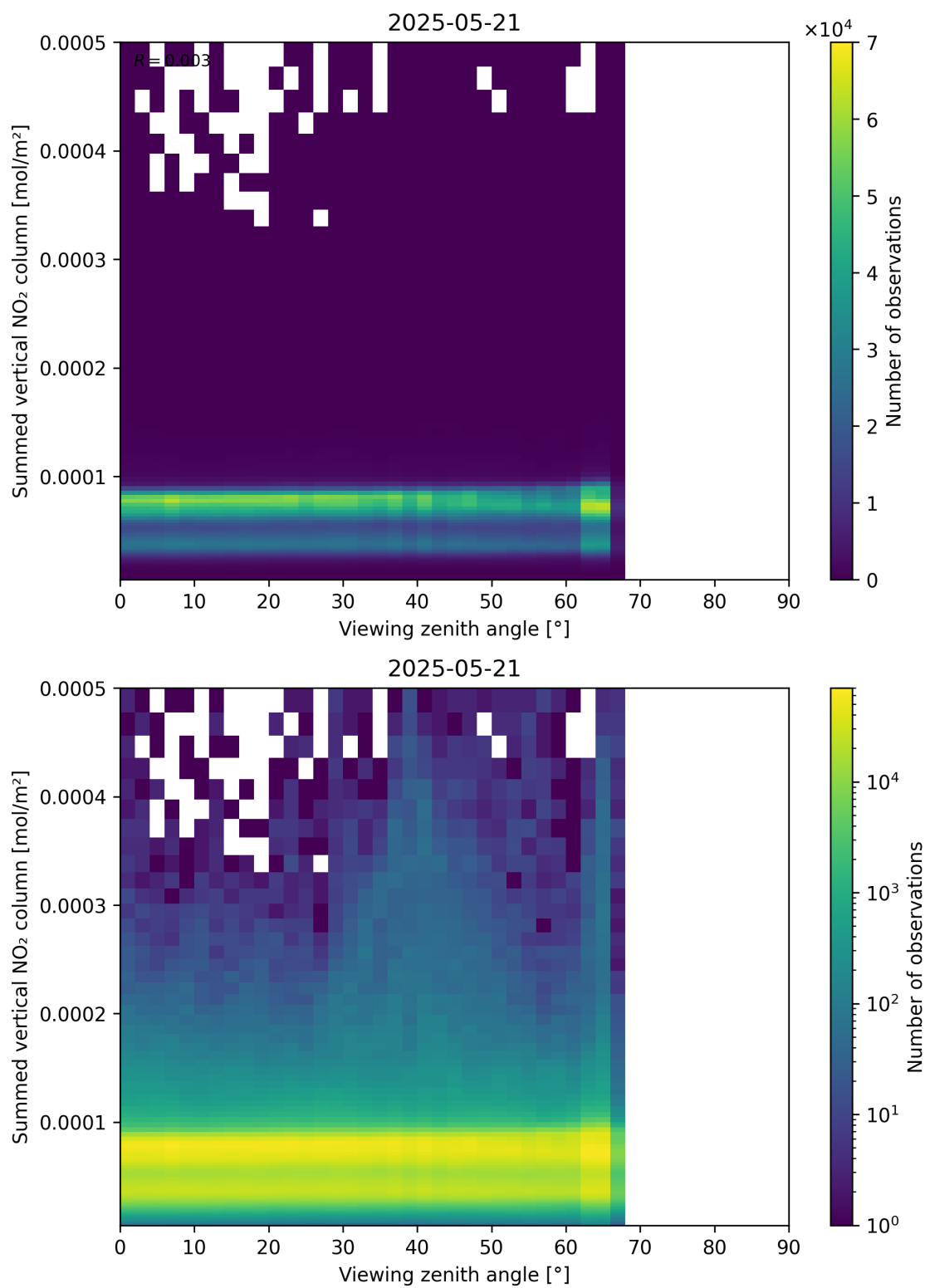
Figure 165: Scatter density plot of “Viewing zenith angle” against “Summed vertical NO 2 column” for 2025-05-21 to 2025-05-22.
