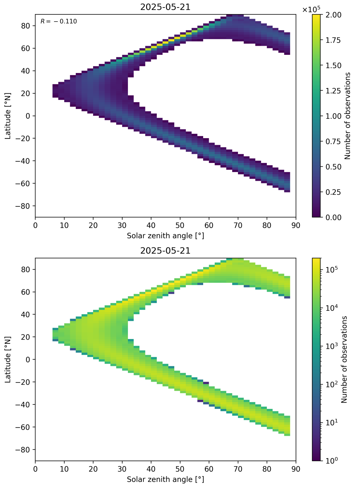
Figure 149: Scatter density plot of “Solar zenith angle” against “Latitude” for 2025-05-21 to 2025-05-22.
