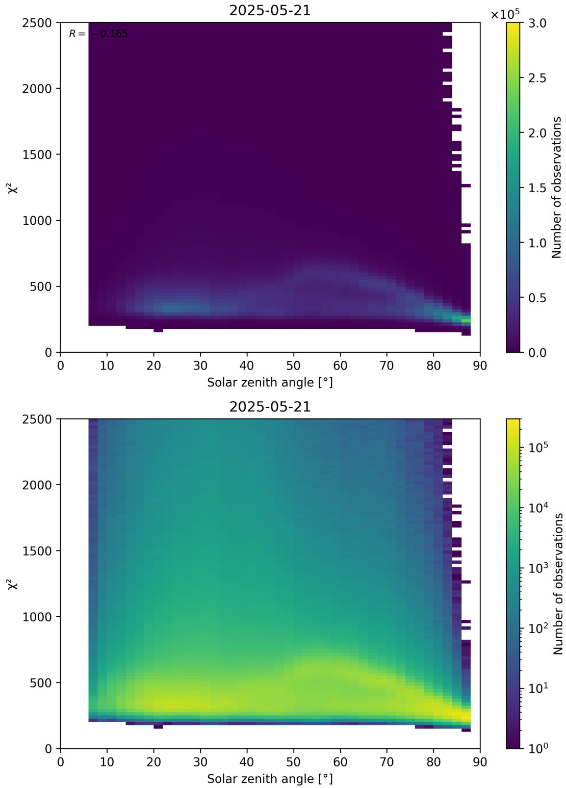
Figure 148: Scatter density plot of “Solar zenith angle” against “ \chi^2 ” for 2025-05-21 to 2025-05-22.
