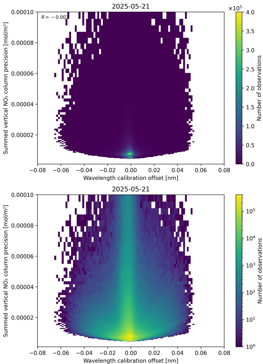
Figure 178: Scatter density plot of “Wavelength calibration offset” against “Summed vertical NO 2 column precision” for 2025-05-21 to 2025-05-22.
