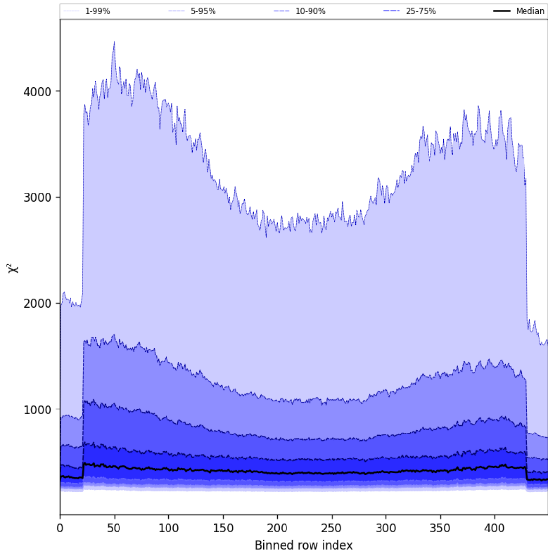
Figure 59: Along track statistics of “ \chi^2 ” for 2025-05-21 to 2025-05-22
