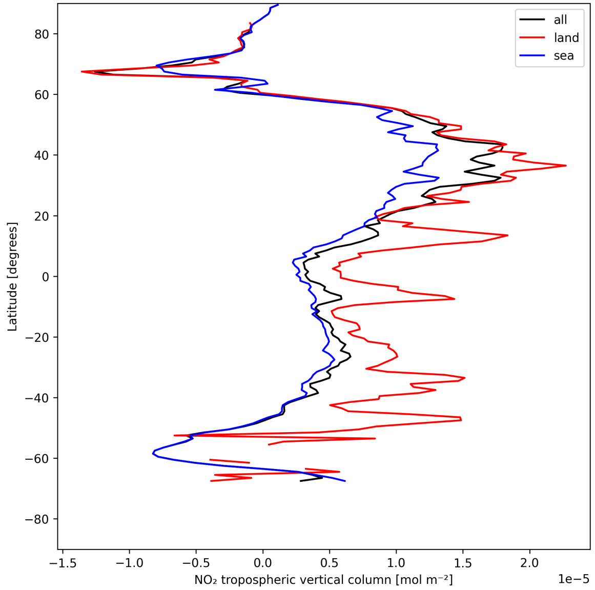
Figure 12: Zonal average of “NO 2 tropospheric vertical column” for 2025-05-21 to 2025-05-22.
