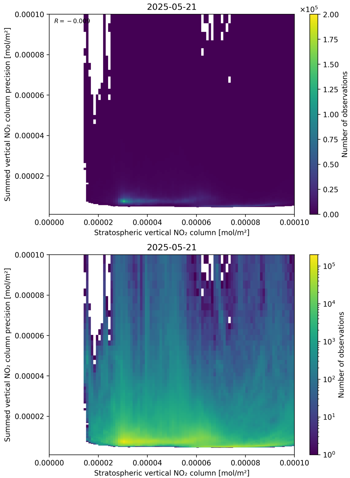
Figure 99: Scatter density plot of “Stratospheric vertical NO 2 column” against “Summed vertical NO 2 column precision” for 2025-05-21 to 2025-05-22.
