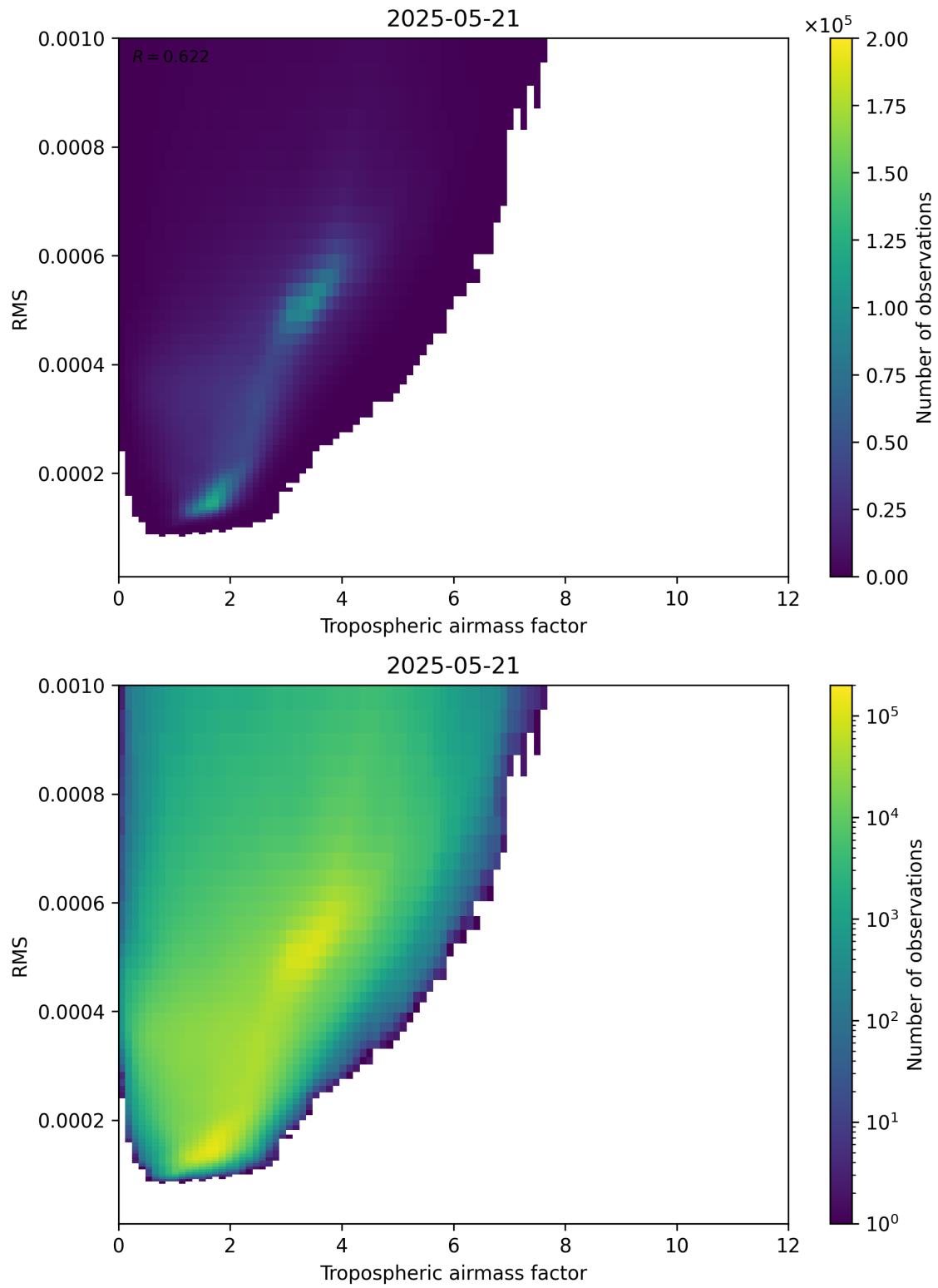
Figure 79: Scatter density plot of “Tropospheric airmass factor” against “RMS” for 2025-05-21 to 2025-05-22.
