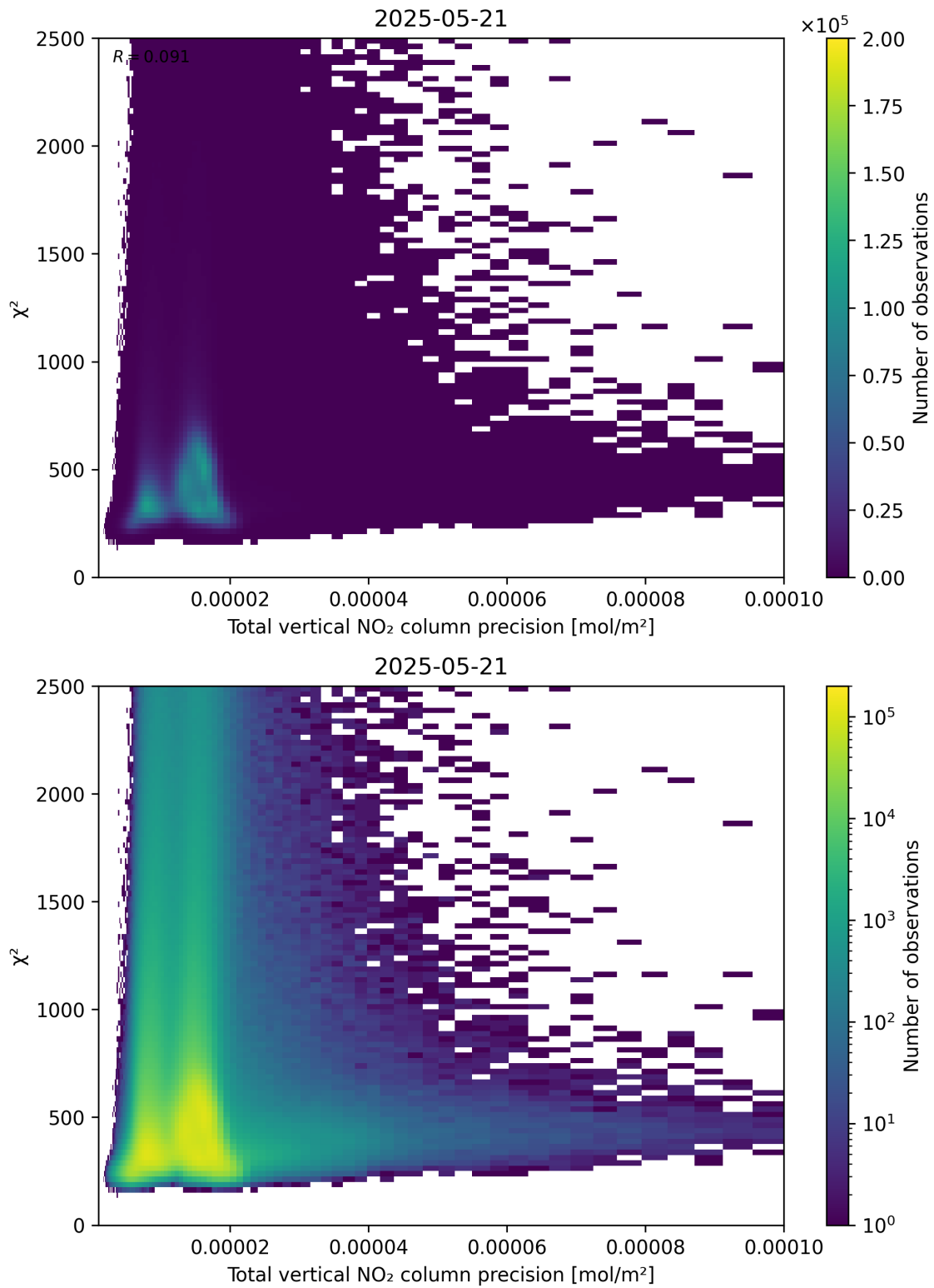
Figure 116: Scatter density plot of “Total vertical NO 2 column precision” against “ \chi^2 ” for 2025-05-21 to 2025-05-22.
