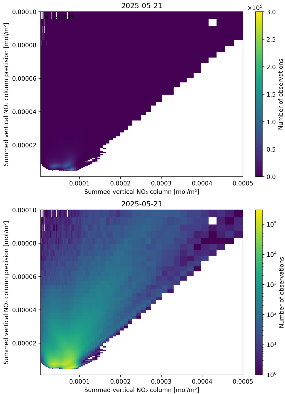
Figure 105: Scatter density plot of “Summed vertical NO 2 column” against “Summed vertical NO 2 column precision” for 2025-05-21 to 2025-05-22.
