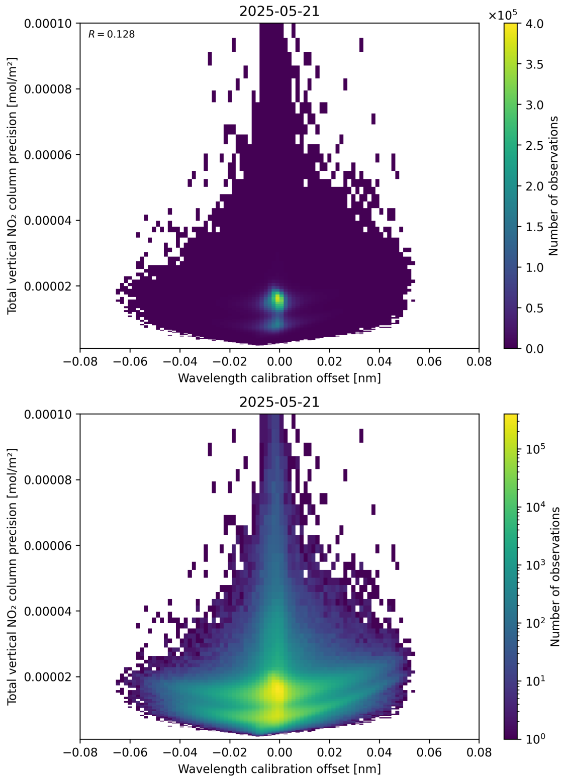
Figure 180: Scatter density plot of “Wavelength calibration offset” against “Total vertical NO 2 column precision” for 2025-05-21 to 2025-05-22.
