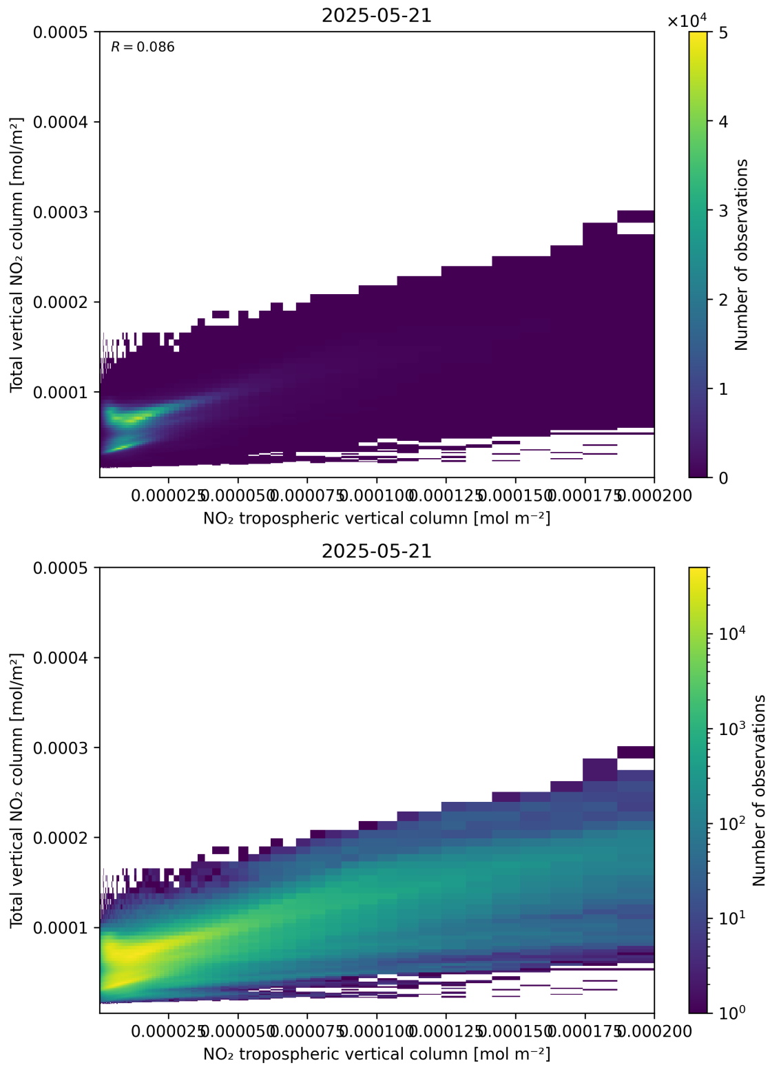
Figure 128: Scatter density plot of “NO 2 tropospheric vertical column” against “Total vertical NO 2 column” for 2025-05-21 to 2025-05-22.
