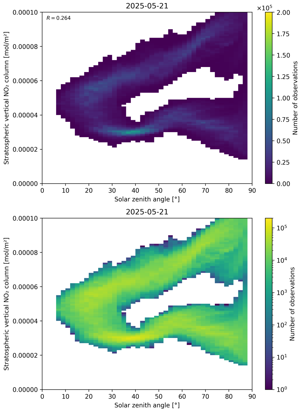
Figure 150: Scatter density plot of “Solar zenith angle” against “Stratospheric vertical NO 2 column” for 2025-05-21 to 2025-05-22.
