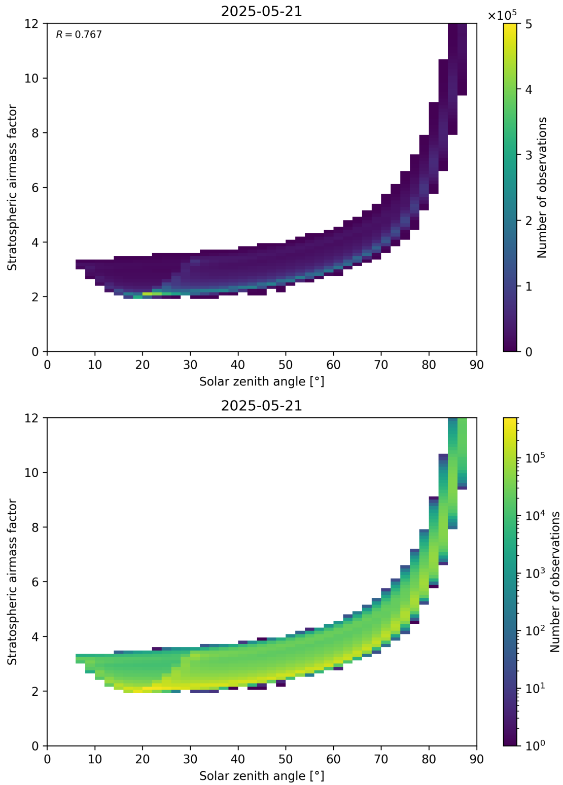
Figure 145: Scatter density plot of “Solar zenith angle” against “Stratospheric airmass factor” for 2025-05-21 to 2025-05-22.
