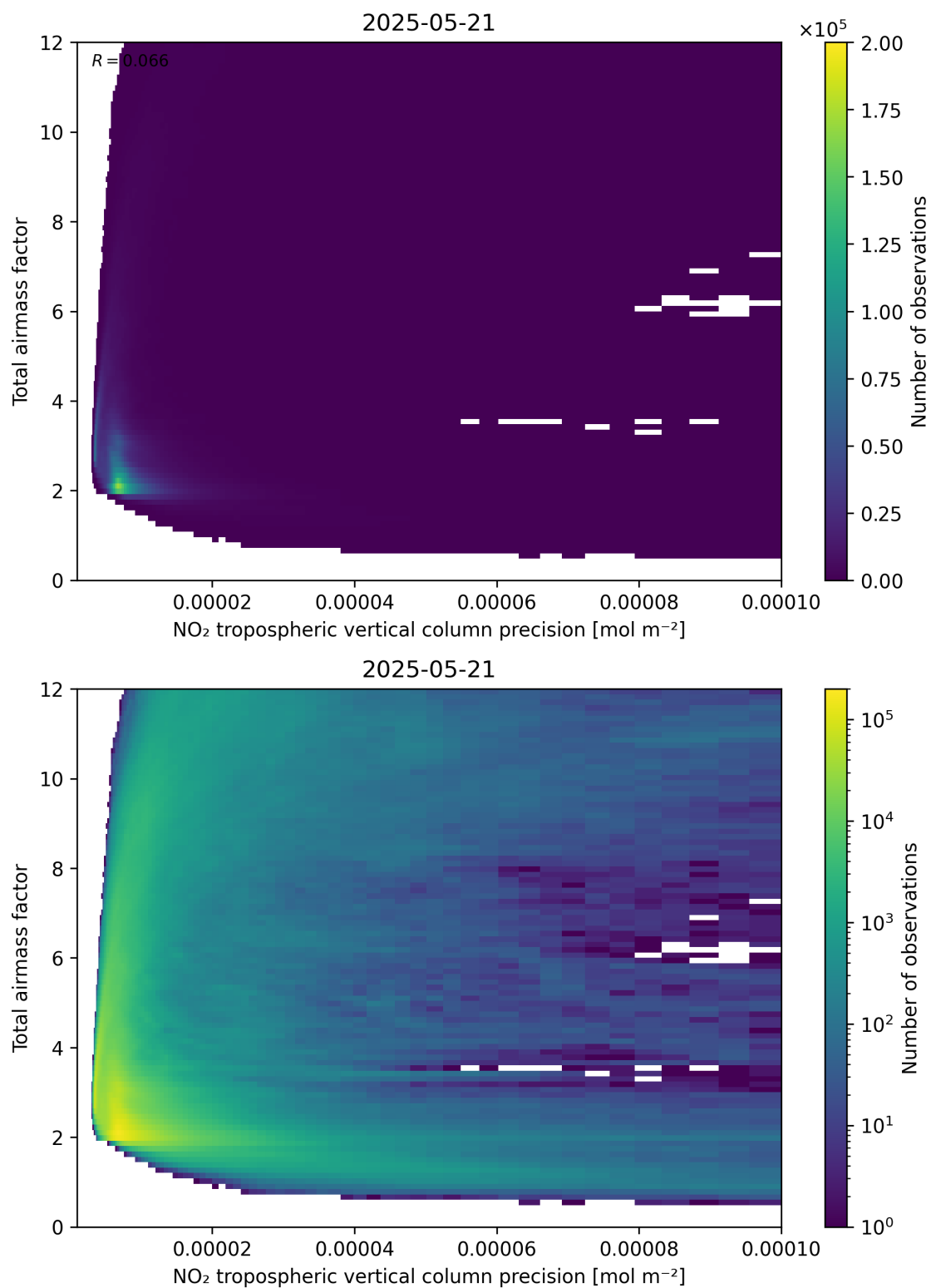
Figure 132: Scatter density plot of “NO 2 tropospheric vertical column precision” against “Total air mass factor” for 2025-05-21 to 2025-05-22.
