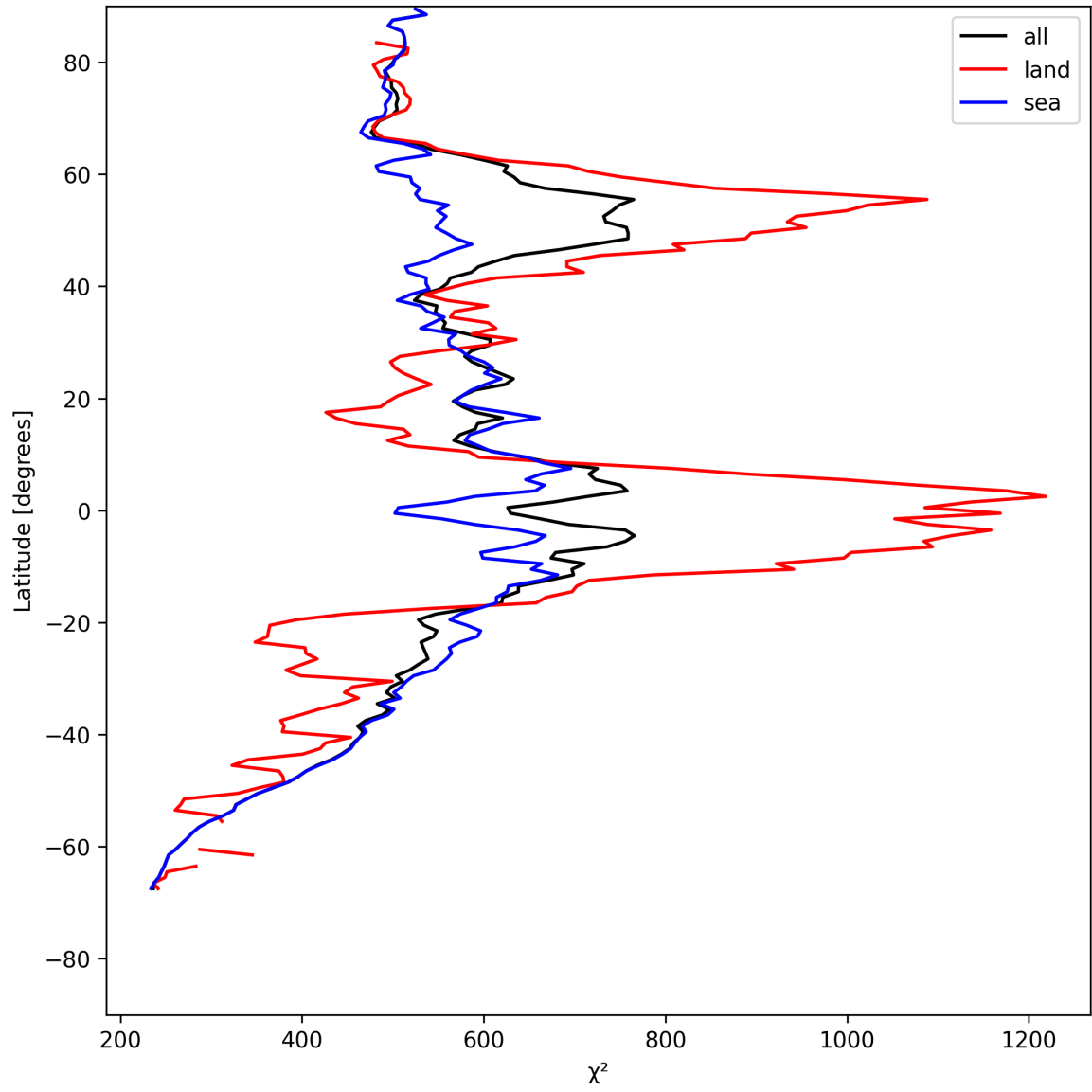
Figure 25: Zonal average of “ \chi^2 ” for 2025-05-21 to 2025-05-22.
