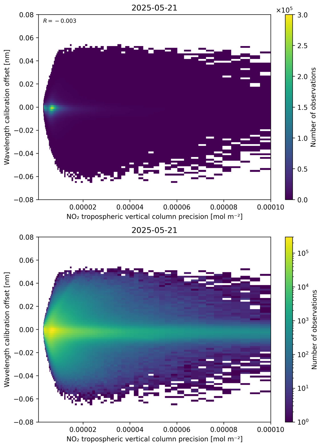
Figure 141: Scatter density plot of “NO 2 tropospheric vertical column precision” against “Wavelength calibration offset” for 2025-05-21 to 2025-05-22.
