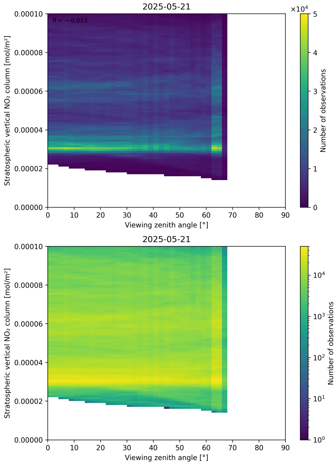
Figure 164: Scatter density plot of “Viewing zenith angle” against “Stratospheric vertical NO 2 column” for 2025-05-21 to 2025-05-22.
