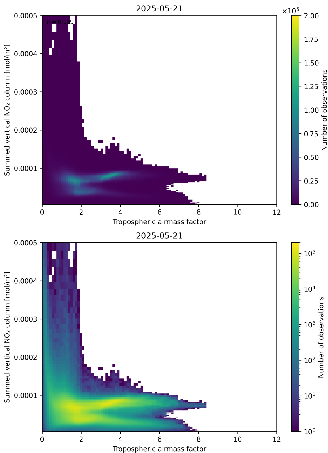
Figure 75: Scatter density plot of “Tropospheric airmass factor” against “Summed vertical NO 2 column” for 2025-05-21 to 2025-05-22.
