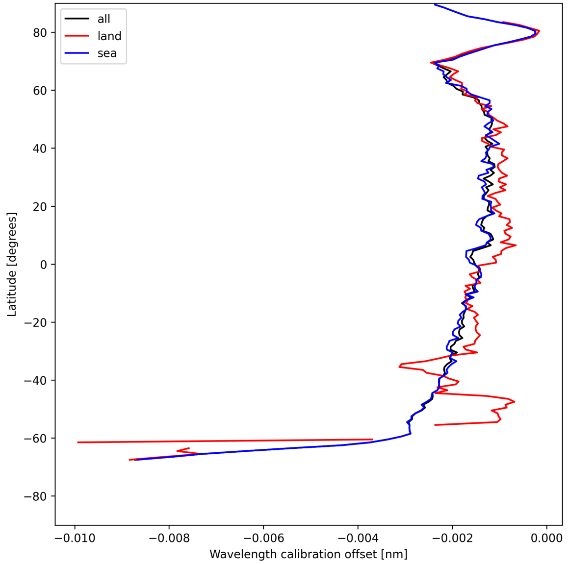
Figure 18: Zonal average of “Wavelength calibration offset” for 2025-05-21 to 2025-05-22.
