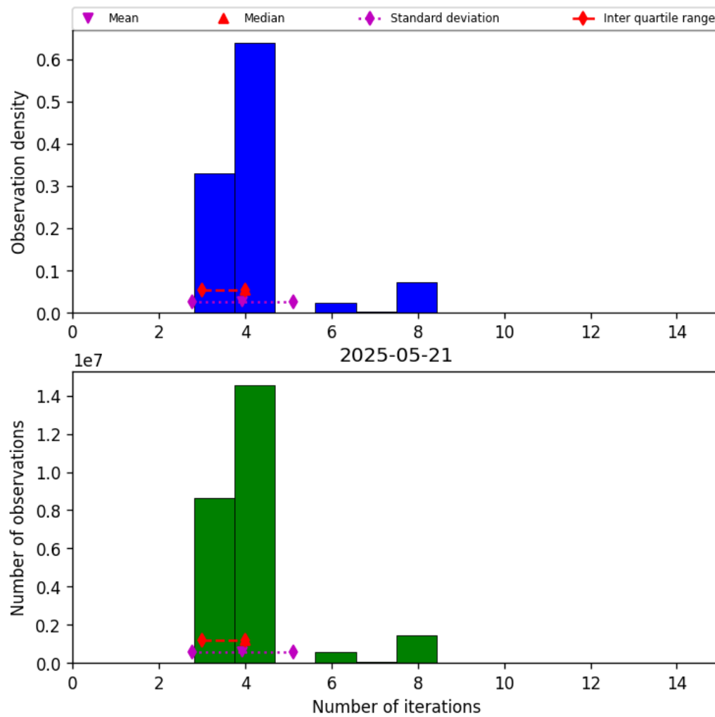
Figure 34: Histogram of “Number of iterations” for 2025-05-21 to 2025-05-22
