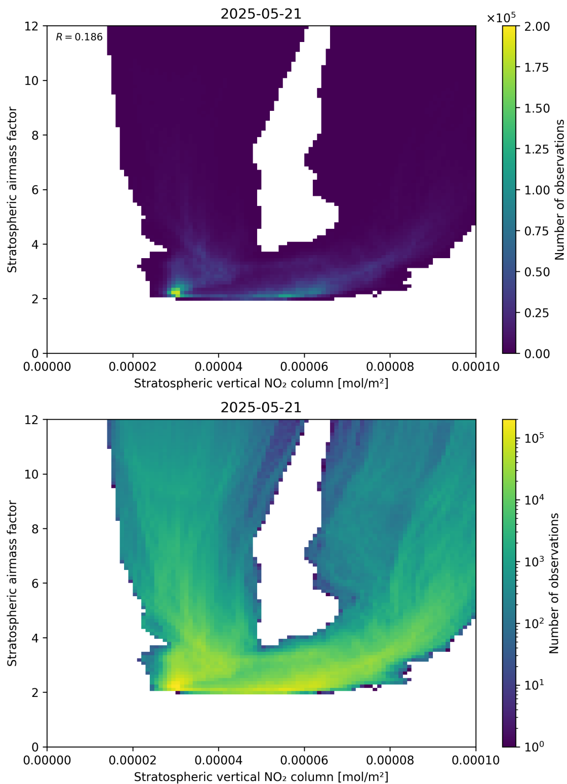
Figure 96: Scatter density plot of “Stratospheric vertical NO 2 column” against “Stratospheric airmass factor” for 2025-05-21 to 2025-05-22.
