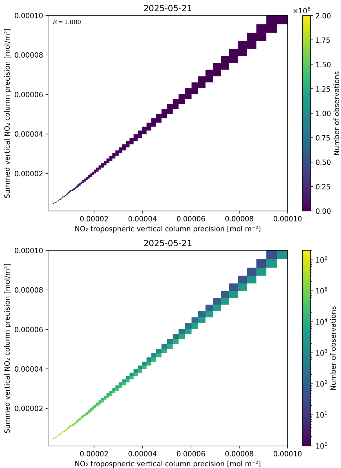
Figure 137: Scatter density plot of “NO 2 tropospheric vertical column precision” against “Summed vertical NO 2 column precision” for 2025-05-21 to 2025-05-22.
