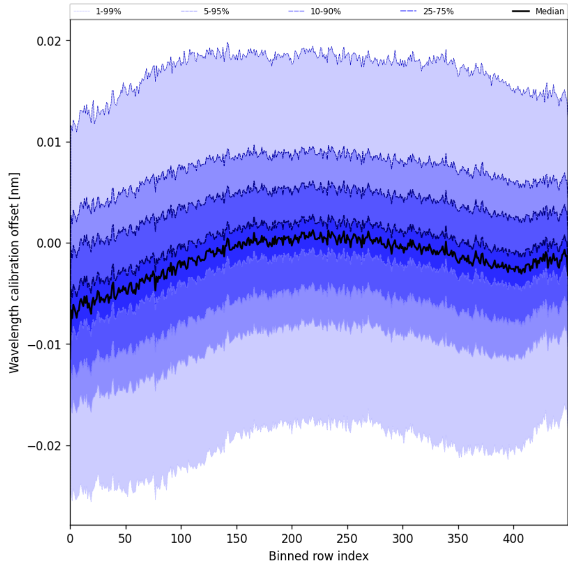
Figure 52: Along track statistics of “Wavelength calibration offset” for 2025-05-21 to 2025-05-22
