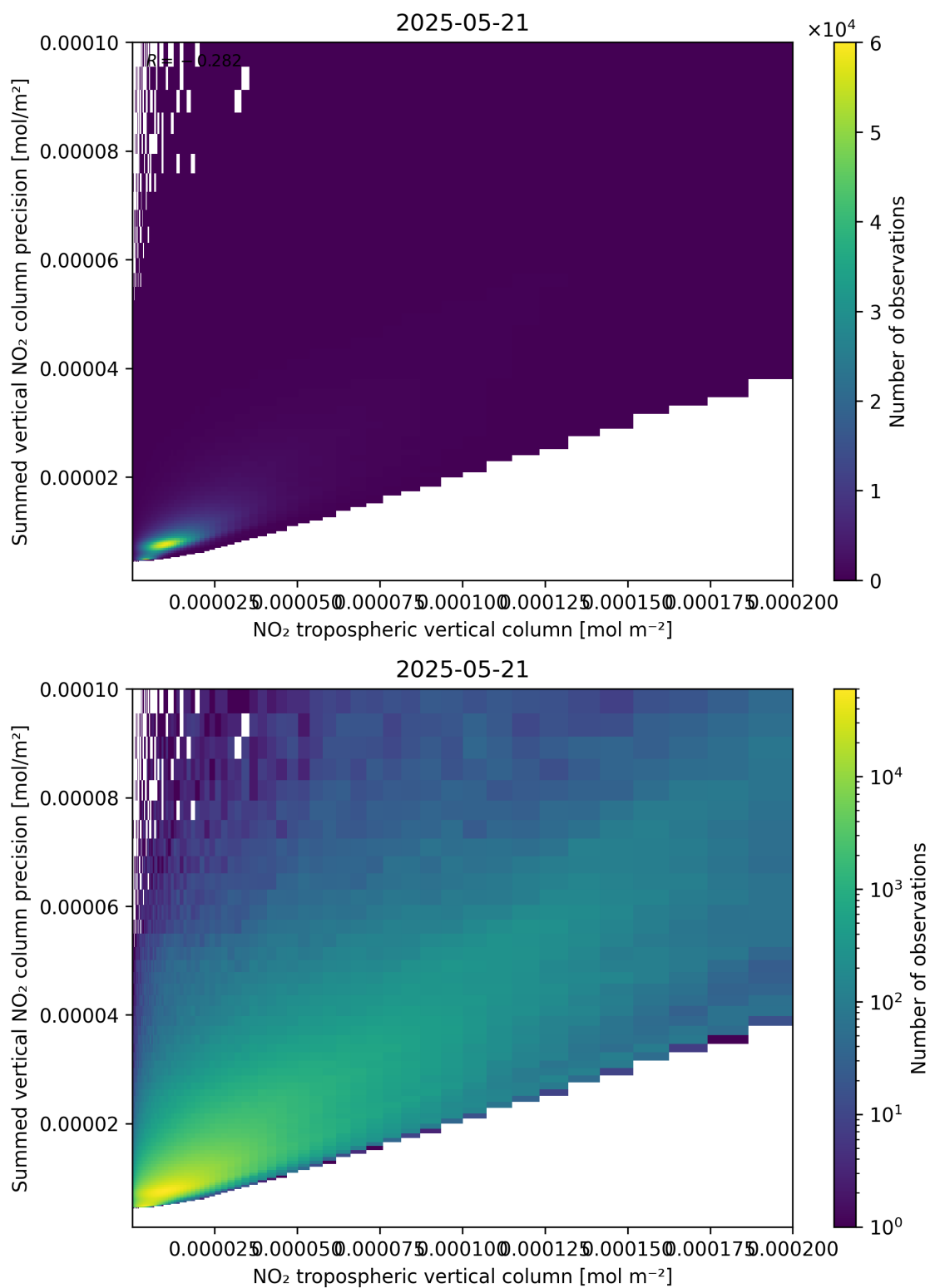
Figure 127: Scatter density plot of “NO 2 tropospheric vertical column” against “Summed vertical NO 2 column precision” for 2025-05-21 to 2025-05-22.
