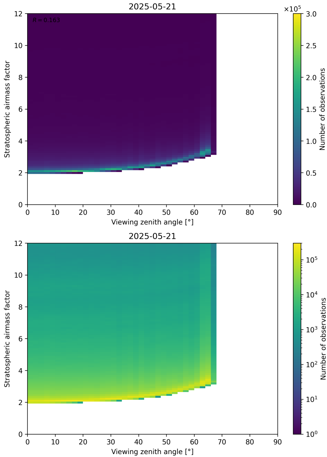
Figure 159: Scatter density plot of “Viewing zenith angle” against “Stratospheric airmass factor” for 2025-05-21 to 2025-05-22.
