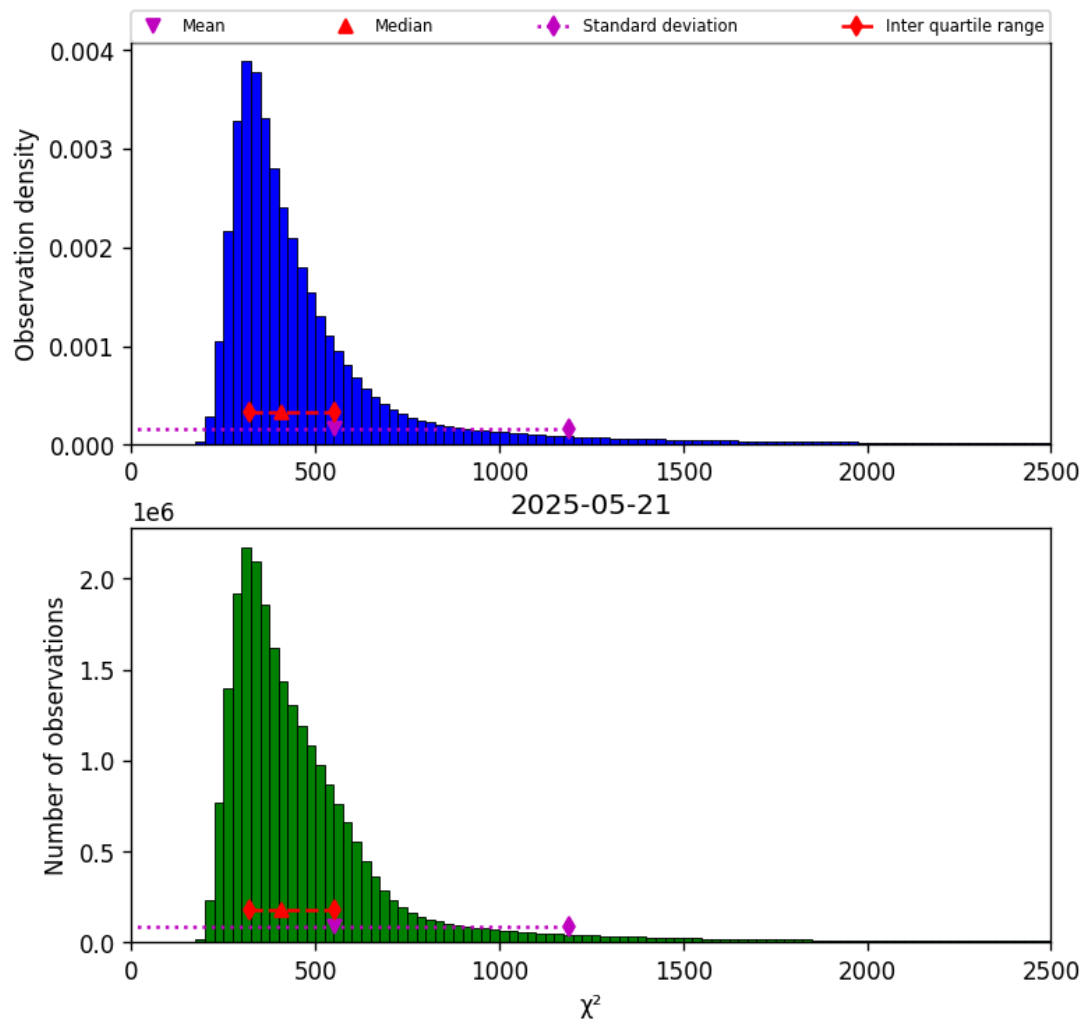
Figure 42: Histogram of “ \chi^2 ” for 2025-05-21 to 2025-05-22
