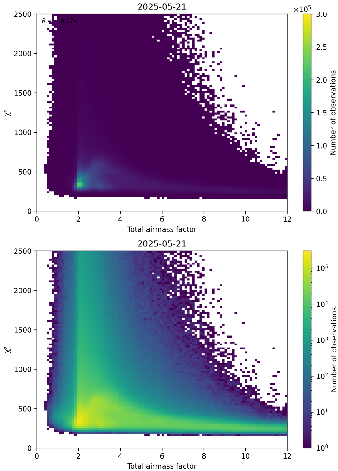
Figure 63: Scatter density plot of “Total airmass factor” against “ \chi^2 ” for 2025-05-21 to 2025-05-22.
