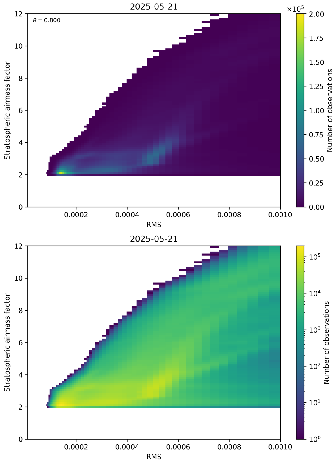
Figure 144: Scatter density plot of “RMS” against “Stratospheric airmass factor” for 2025-05-21 to 2025-05-22.
