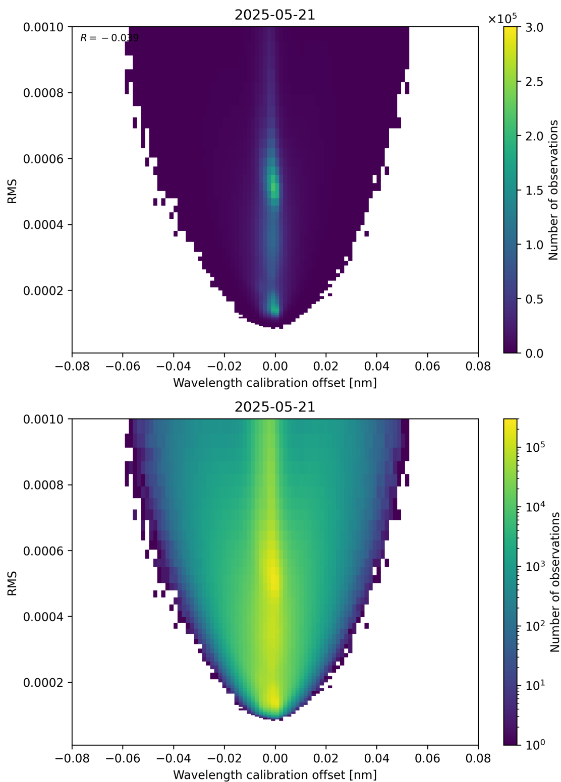
Figure 181: Scatter density plot of “Wavelength calibration offset” against “RMS” for 2025-05-21 to 2025-05-22.
