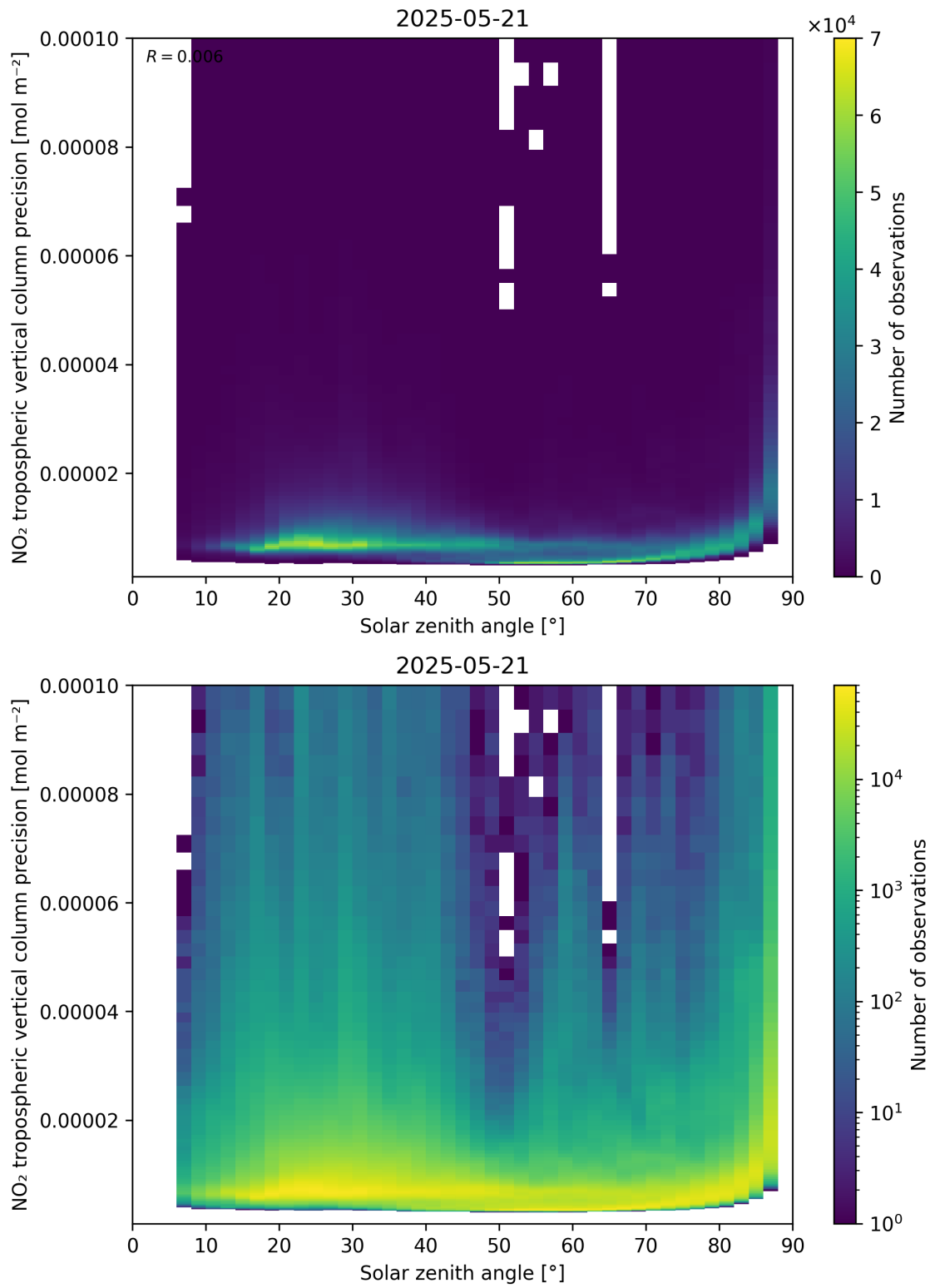
Figure 156: Scatter density plot of “Solar zenith angle” against “NO 2 tropospheric vertical column precision” for 2025-05-21 to 2025-05-22.
