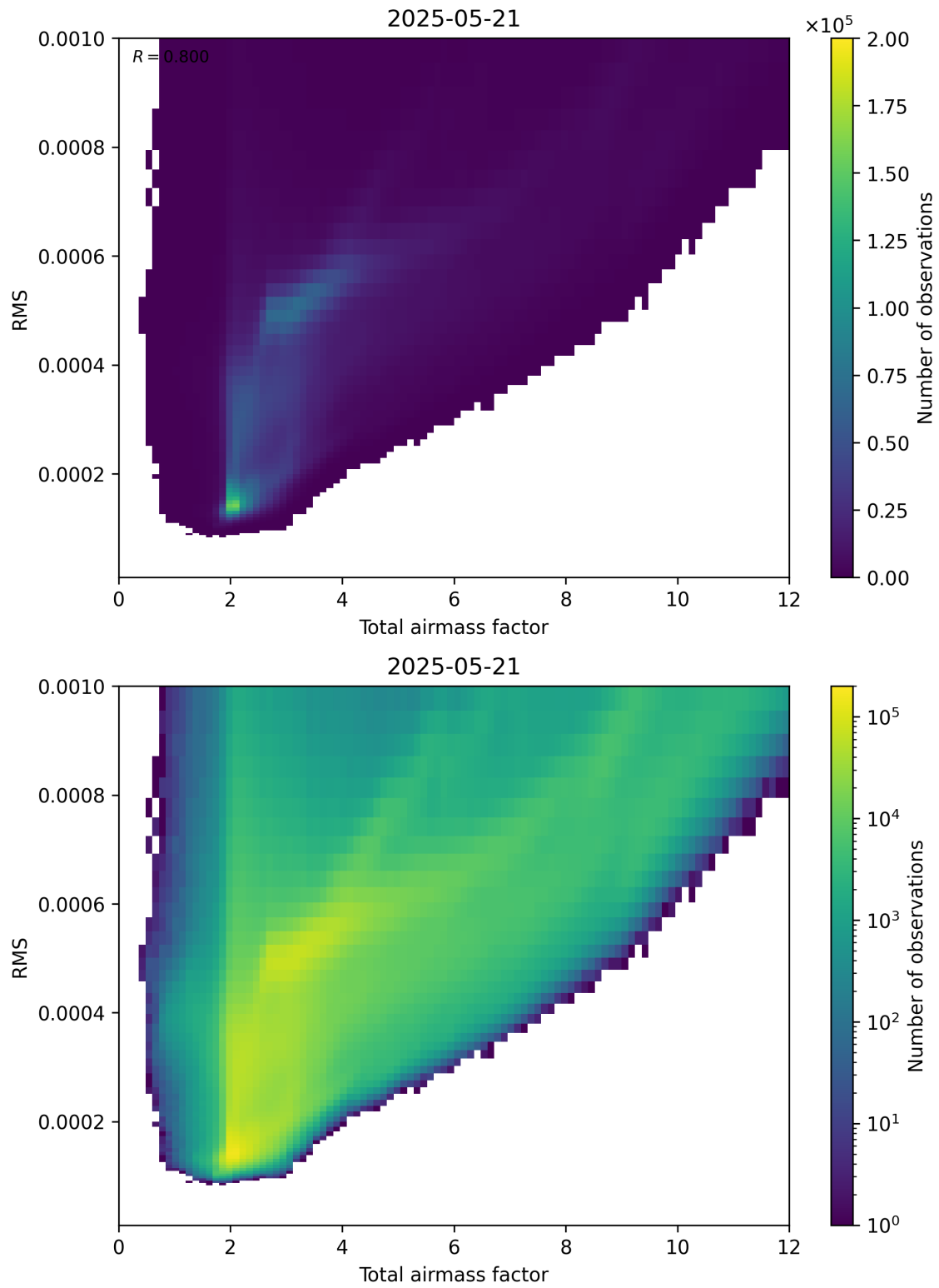
Figure 69: Scatter density plot of “Total airmass factor” against “RMS” for 2025-05-21 to 2025-05-22.
