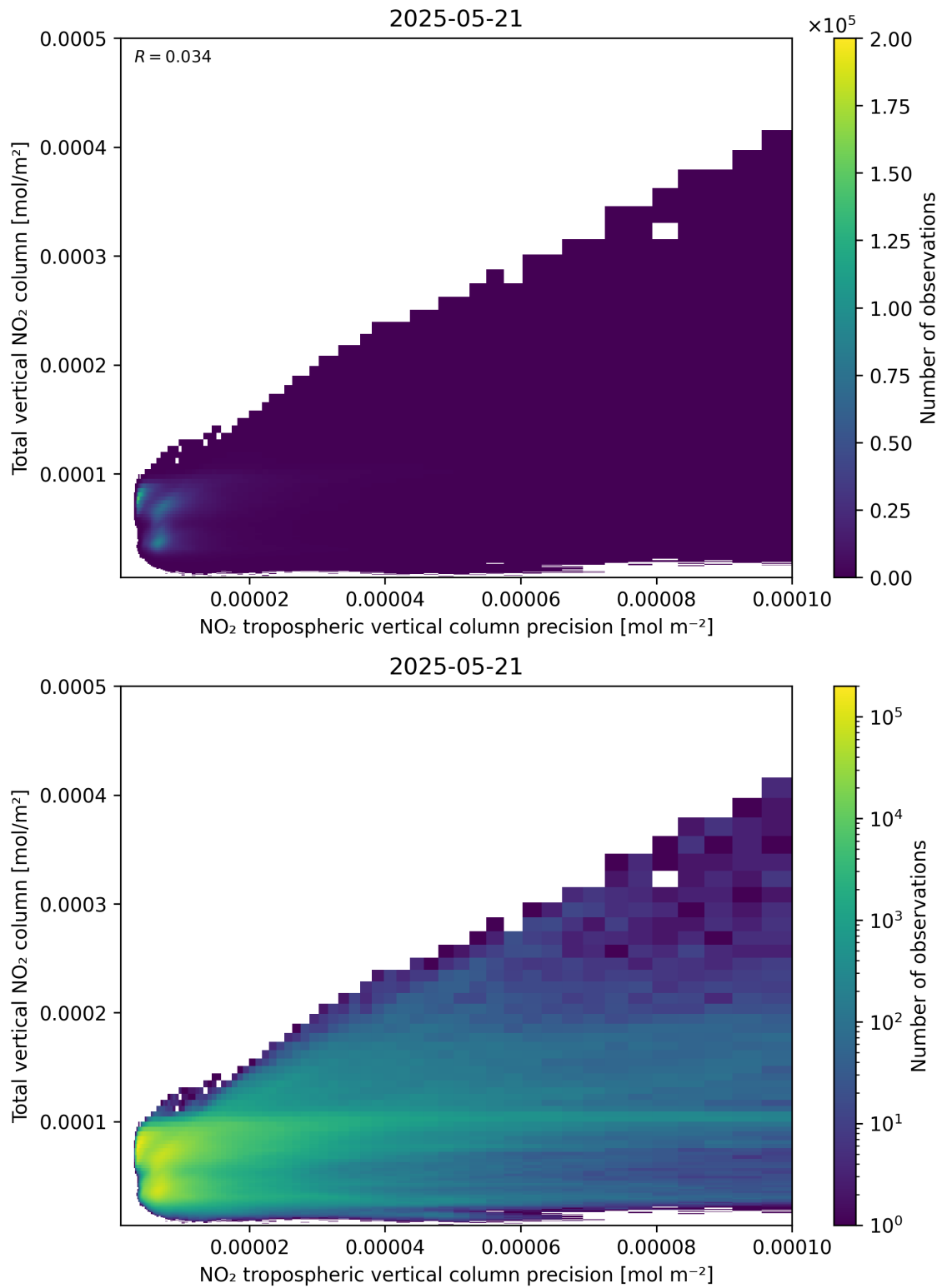
Figure 138: Scatter density plot of “NO 2 tropospheric vertical column precision” against “Total vertical NO 2 column” for 2025-05-21 to 2025-05-22.
