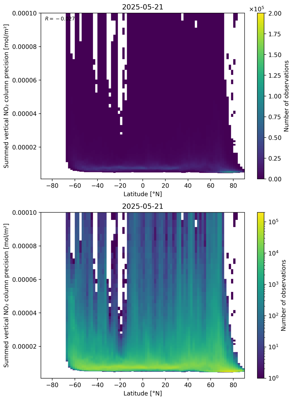
Figure 89: Scatter density plot of “Latitude” against “Summed vertical NO 2 column precision” for 2025-05-21 to 2025-05-22.
