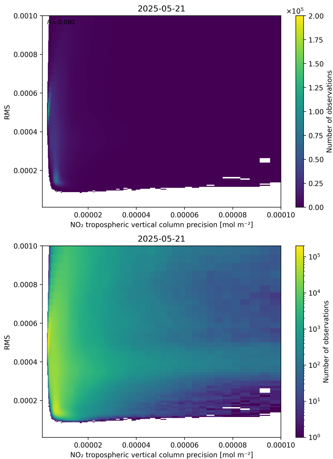
Figure 140: Scatter density plot of “NO 2 tropospheric vertical column precision” against “RMS” for 2025-05-21 to 2025-05-22.
