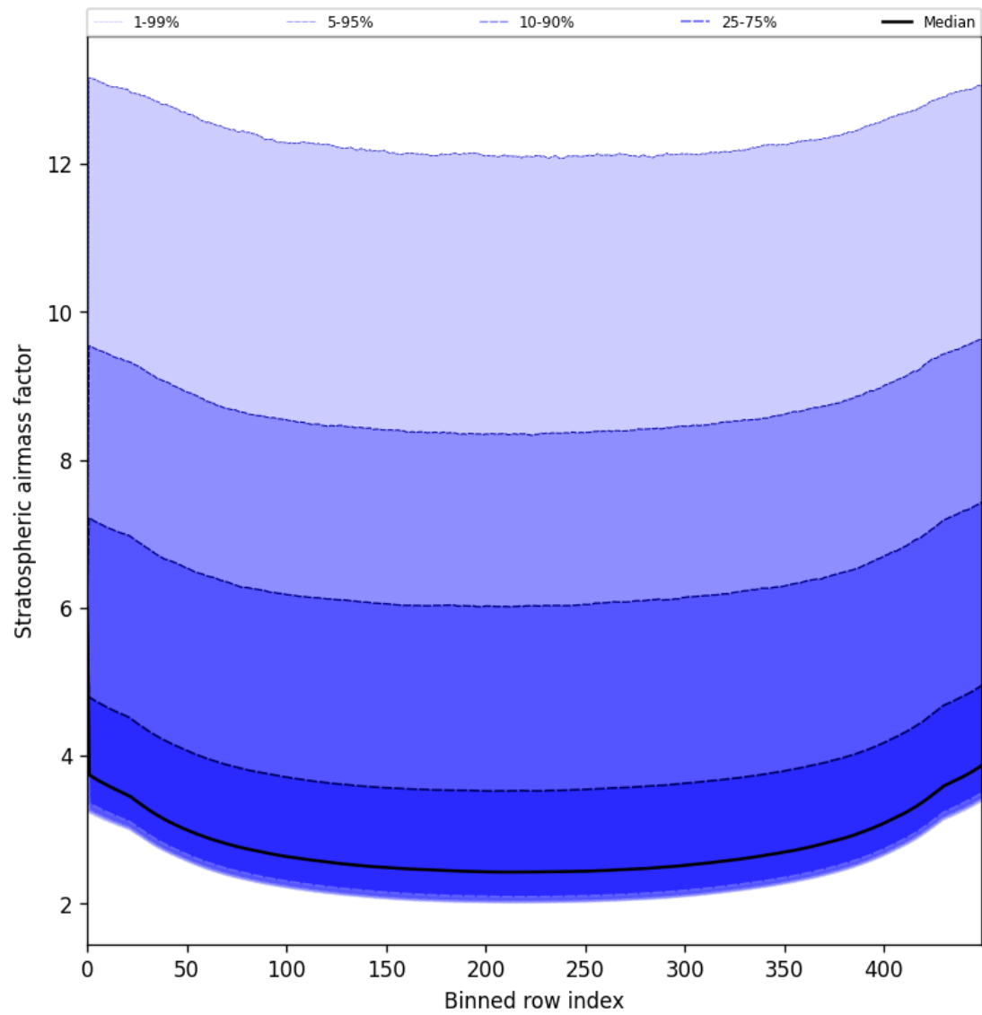
Figure 61: Along track statistics of “Stratospheric airmass factor” for 2025-05-21 to 2025-05-22
