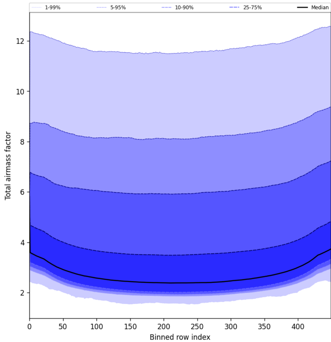
Figure 49: Along track statistics of “Total airmass factor” for 2025-05-21 to 2025-05-22
