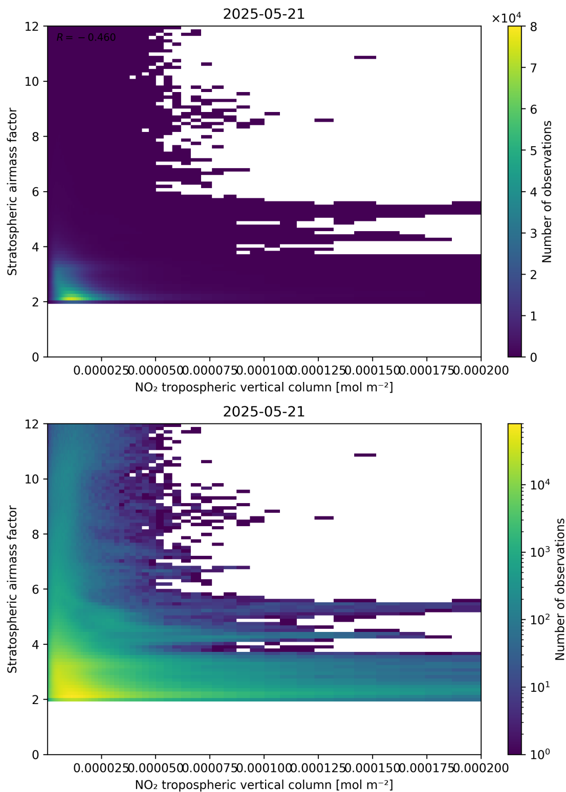
Figure 121: Scatter density plot of “NO 2 tropospheric vertical column” against “Stratospheric air mass factor” for 2025-05-21 to 2025-05-22.
