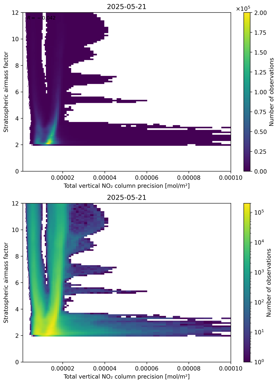
Figure 115: Scatter density plot of “Total vertical NO 2 column precision” against “Stratospheric airmass factor” for 2025-05-21 to 2025-05-22.
