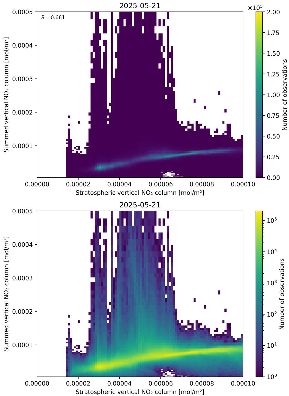
Figure 98: Scatter density plot of “Stratospheric vertical NO 2 column” against “Summed vertical NO 2 column” for 2025-05-21 to 2025-05-22.
