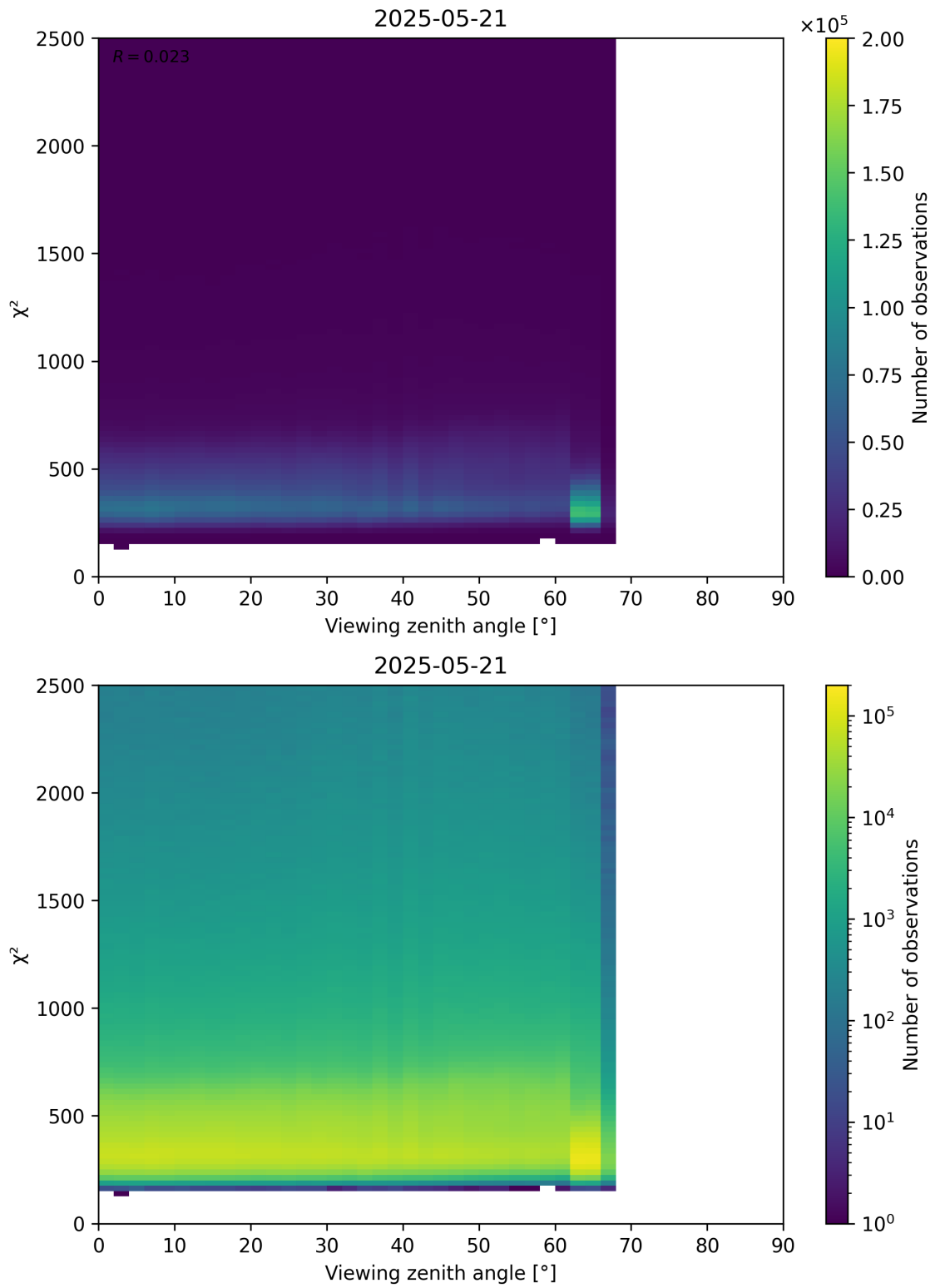
Figure 162: Scatter density plot of “Viewing zenith angle” against “ \chi^2 ” for 2025-05-21 to 2025-05-22.
