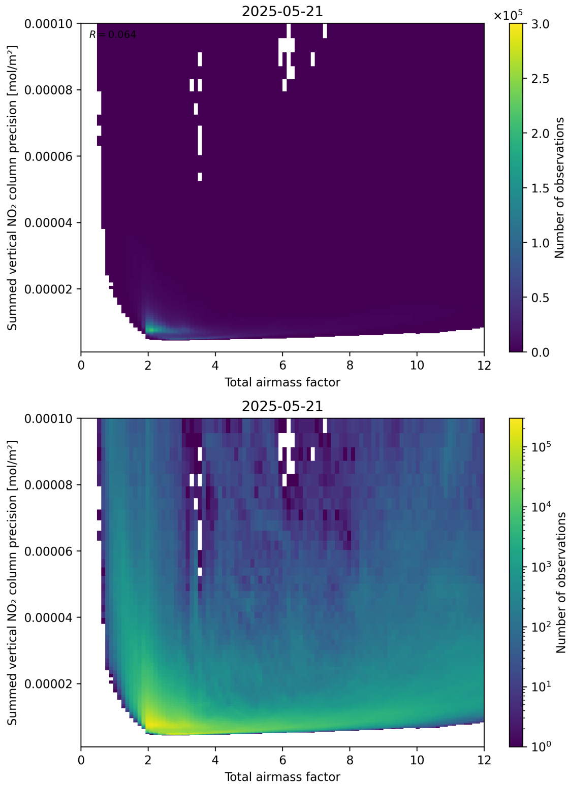
Figure 66: Scatter density plot of “Total airmass factor” against “Summed vertical NO 2 column precision” for 2025-05-21 to 2025-05-22.
