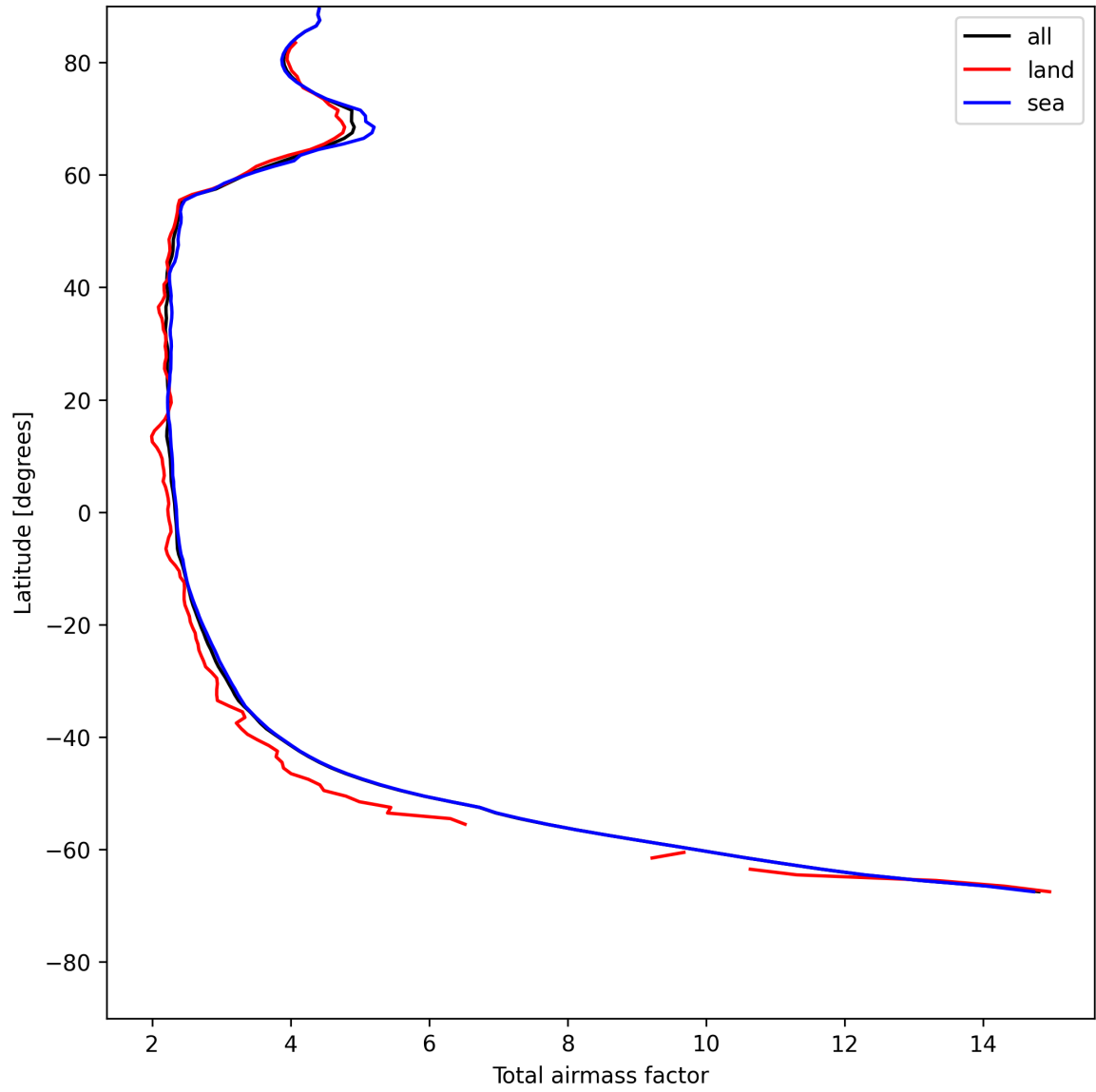
Figure 15: Zonal average of “Total airmass factor” for 2025-05-21 to 2025-05-22.
