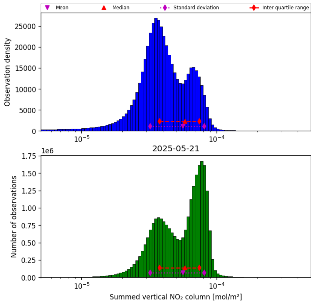
Figure 40: Histogram of “Summed vertical NO 2 column” for 2025-05-21 to 2025-05-22
