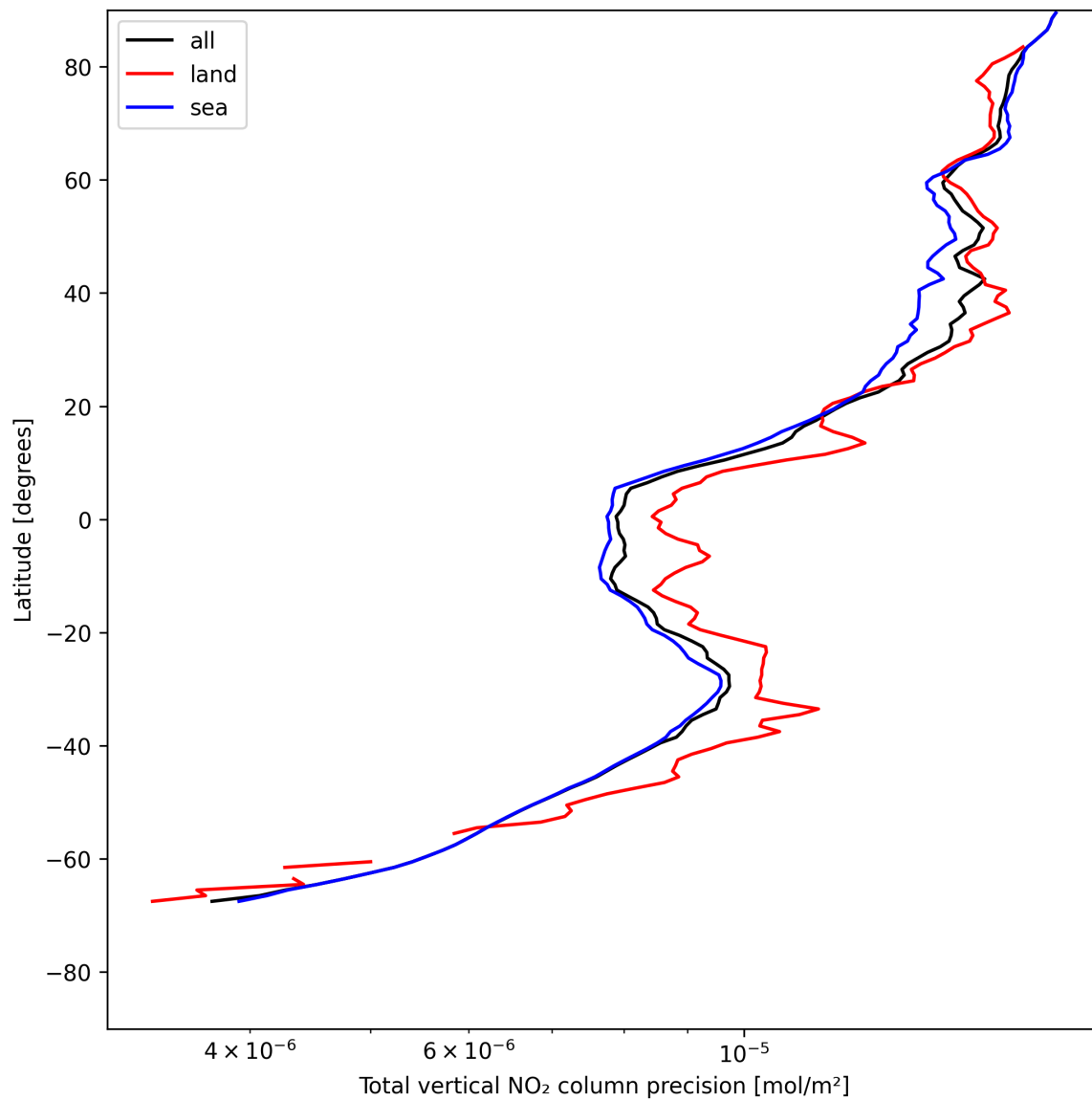
Figure 22: Zonal average of “Total vertical NO 2 column precision” for 2025-05-21 to 2025-05-22.
