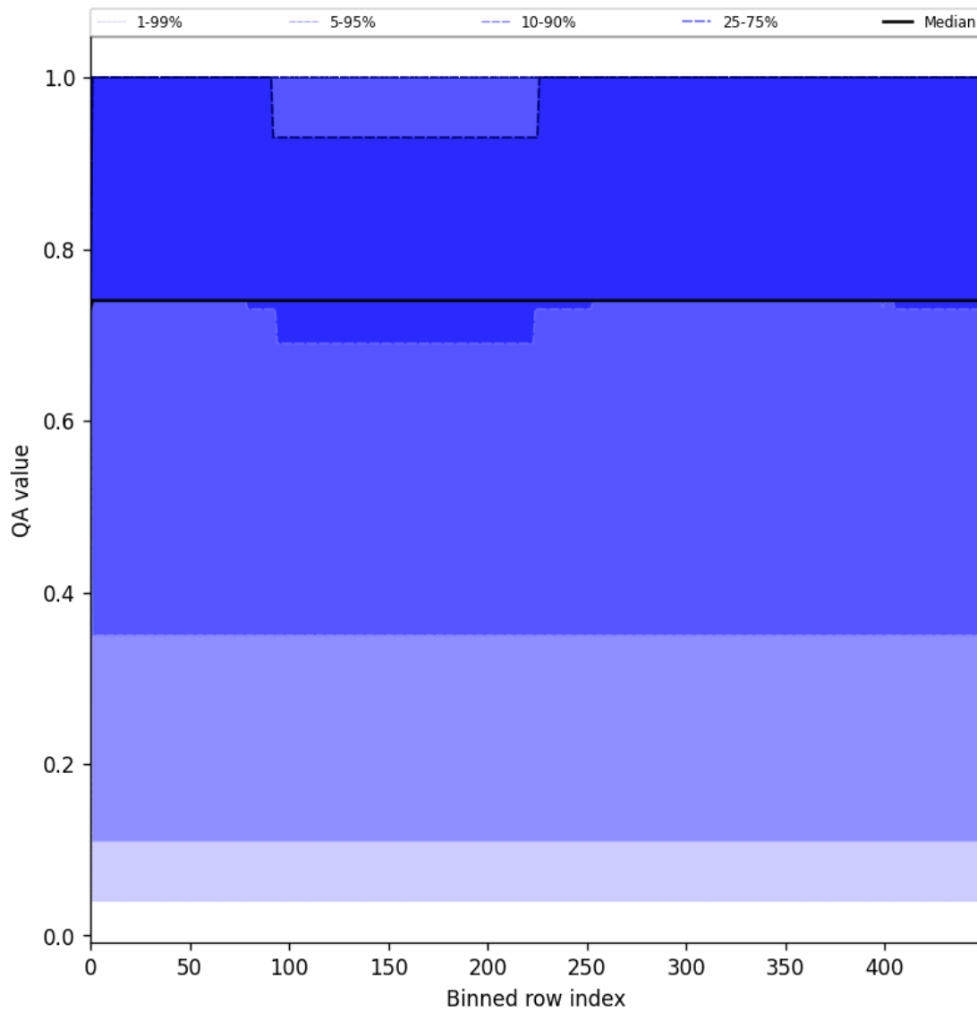
Figure 45: Along track statistics of “QA value” for 2025-05-21 to 2025-05-22
