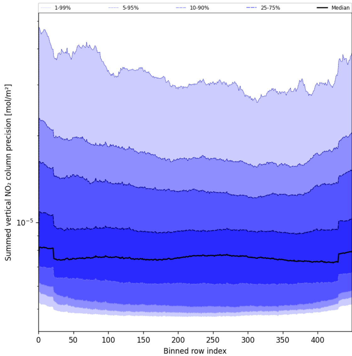
Figure 58: Along track statistics of “Summed vertical NO 2 column precision” for 2025-05-21 to 2025-05-22
