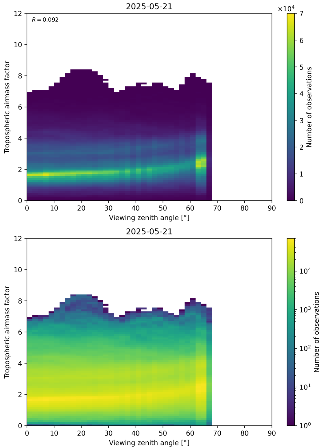
Figure 161: Scatter density plot of “Viewing zenith angle” against “Tropospheric airmass factor” for 2025-05-21 to 2025-05-22.
