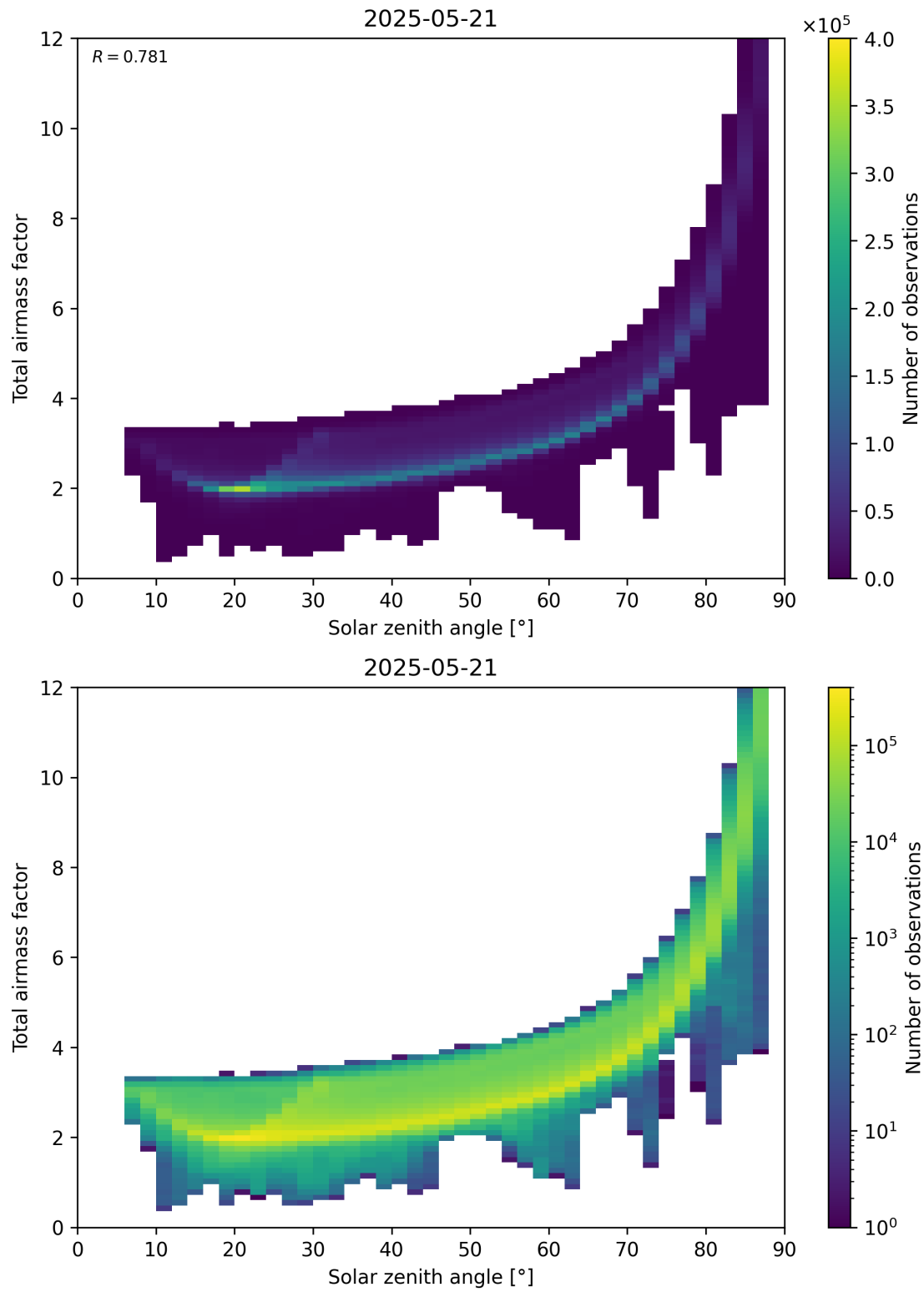
Figure 146: Scatter density plot of “Solar zenith angle” against “Total air mass factor” for 2025-05-21 to 2025-05-22.
