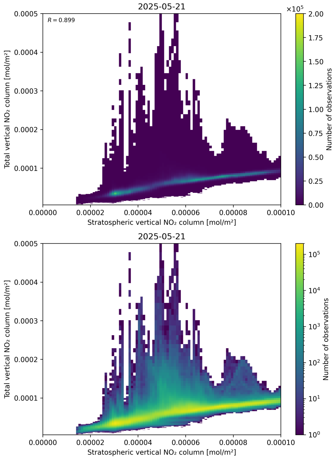
Figure 100: Scatter density plot of “Stratospheric vertical NO 2 column” against “Total vertical NO 2 column” for 2025-05-21 to 2025-05-22.
