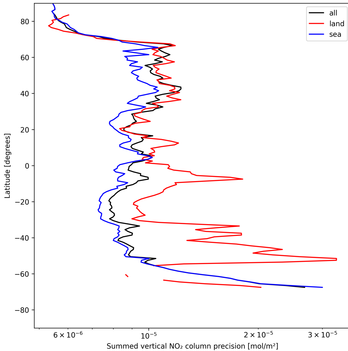
Figure 24: Zonal average of “Summed vertical NO 2 column precision” for 2025-05-21 to 2025-05-22.
