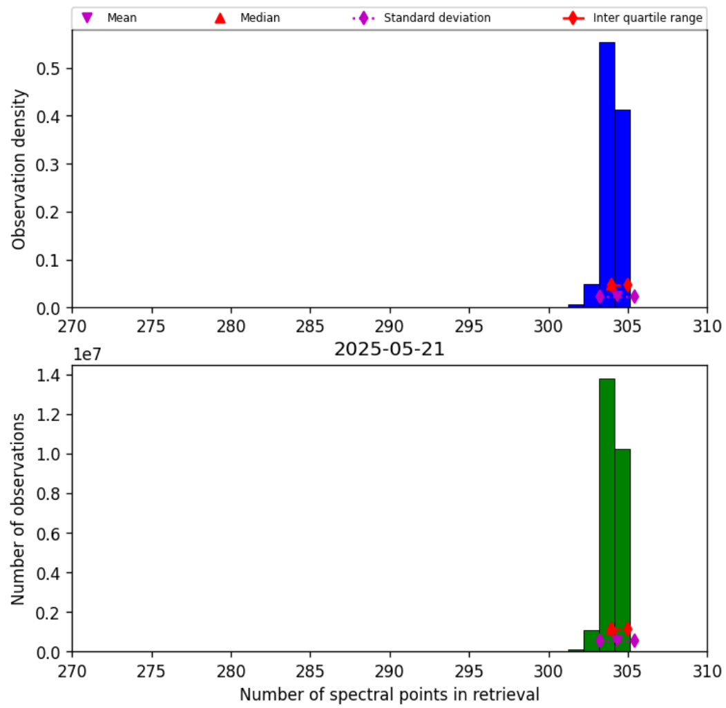
Figure 33: Histogram of “Number of spectral points in retrieval” for 2025-05-21 to 2025-05-22
