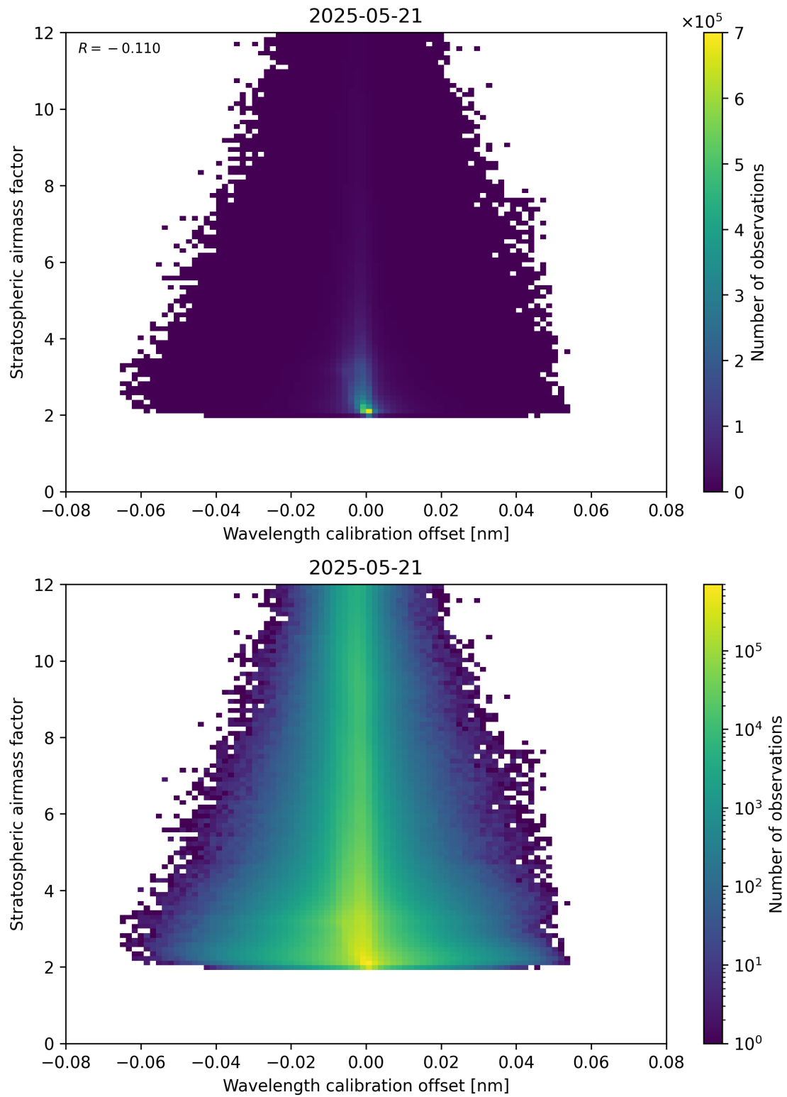
Figure 174: Scatter density plot of “Wavelength calibration offset” against “Stratospheric airmass factor” for 2025-05-21 to 2025-05-22.
