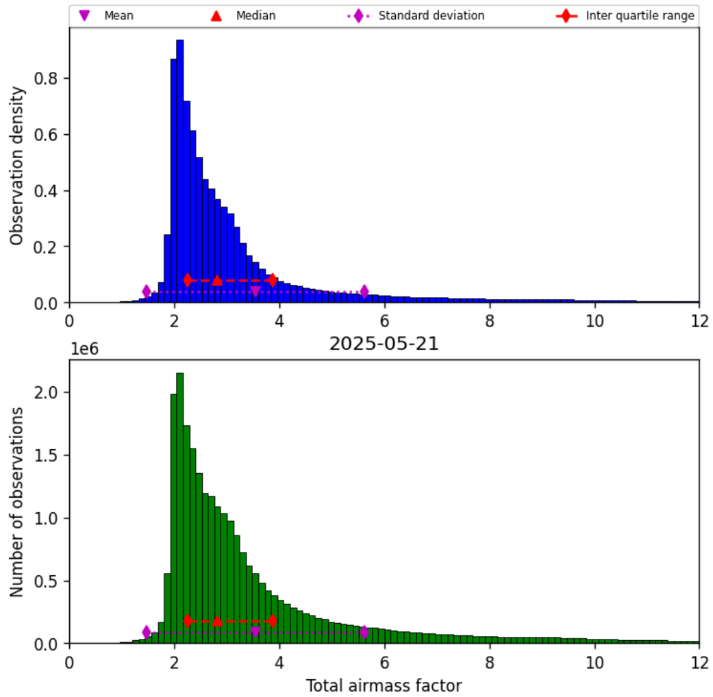
Figure 32: Histogram of “Total airmass factor” for 2025-05-21 to 2025-05-22
