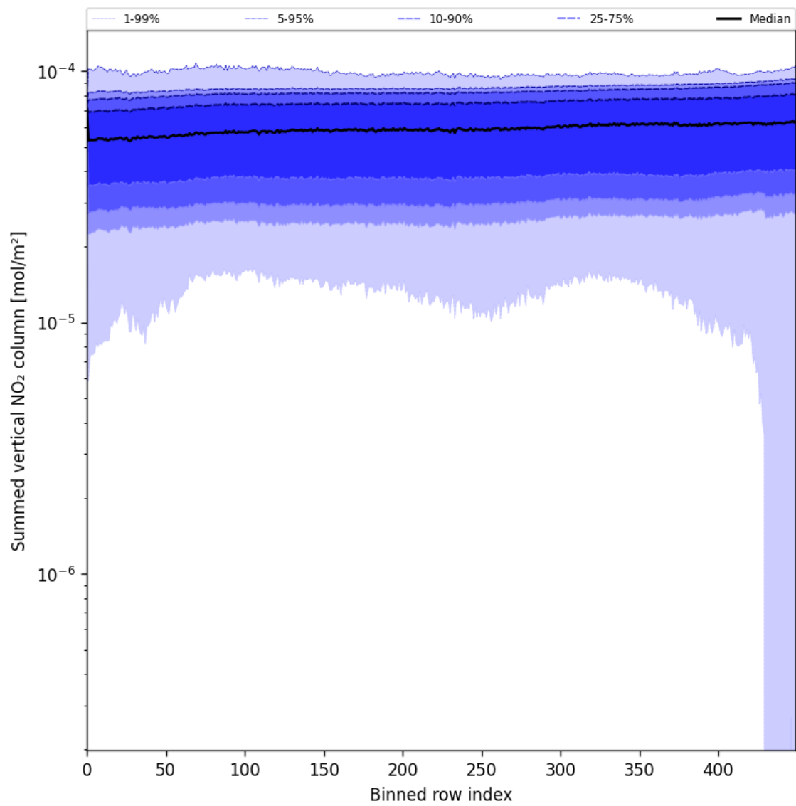
Figure 57: Along track statistics of “Summed vertical NO 2 column” for 2025-05-21 to 2025-05-22
