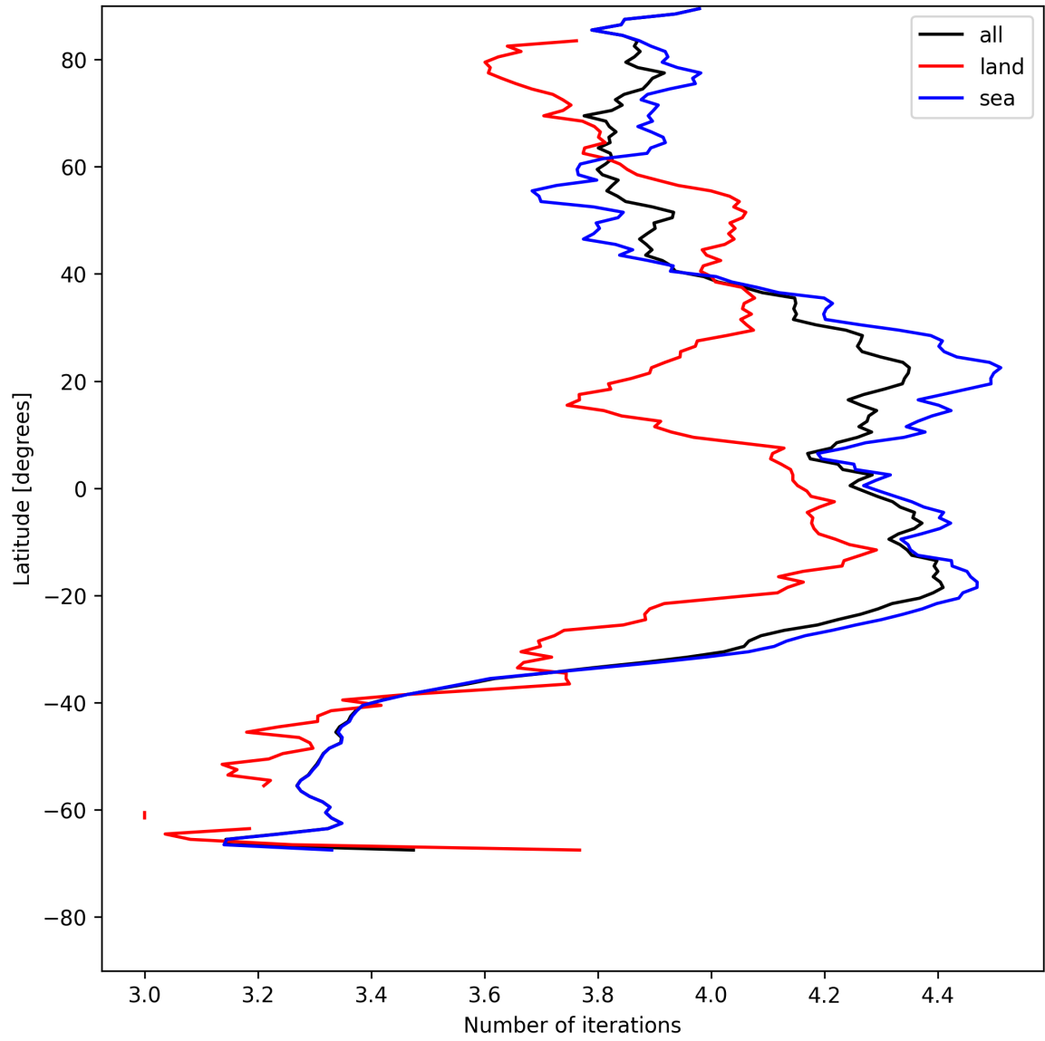
Figure 17: Zonal average of “Number of iterations” for 2025-05-21 to 2025-05-22.
