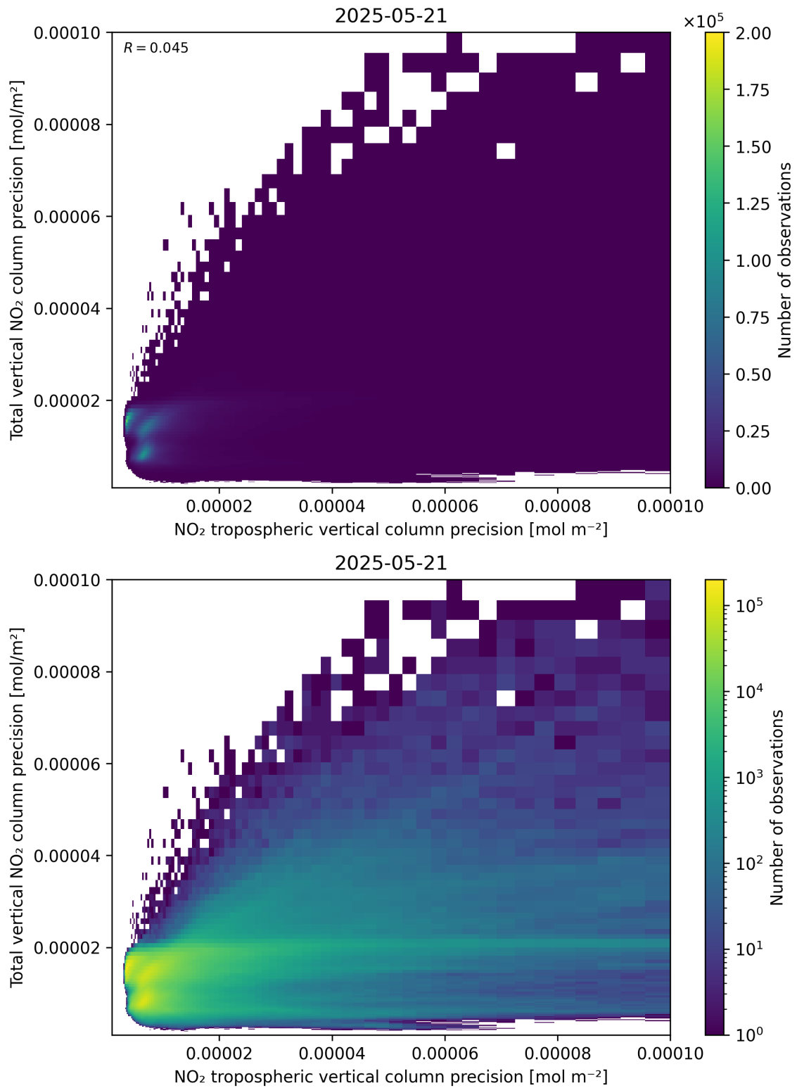
Figure 139: Scatter density plot of “NO 2 tropospheric vertical column precision” against “Total vertical NO 2 column precision” for 2025-05-21 to 2025-05-22.
