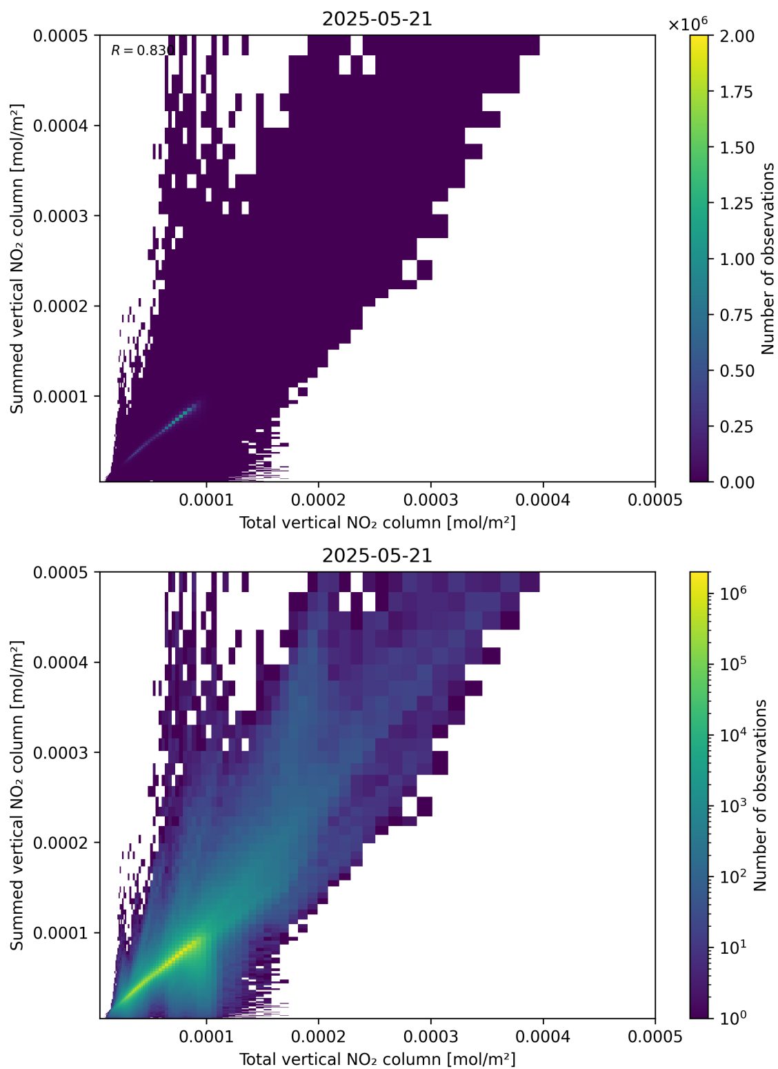
Figure 112: Scatter density plot of “Total vertical NO 2 column” against “Summed vertical NO 2 column” for 2025-05-21 to 2025-05-22.
