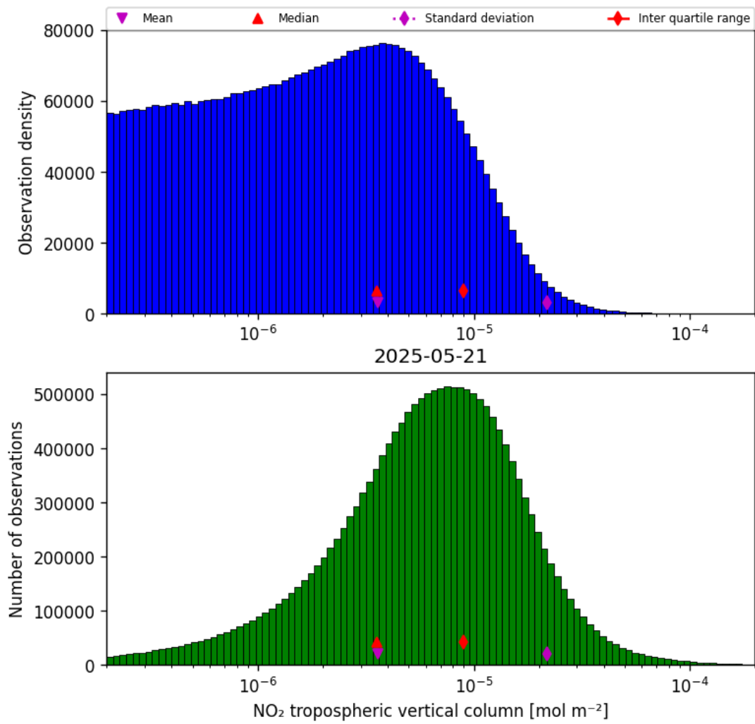
Figure 29: Histogram of “NO 2 tropospheric vertical column” for 2025-05-21 to 2025-05-22
