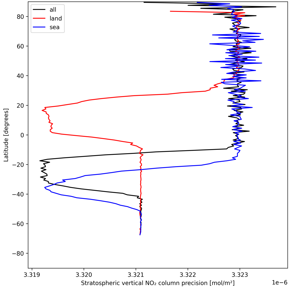
Figure 20: Zonal average of “Stratospheric vertical NO 2 column precision” for 2025-05-21 to 2025-05-22.
