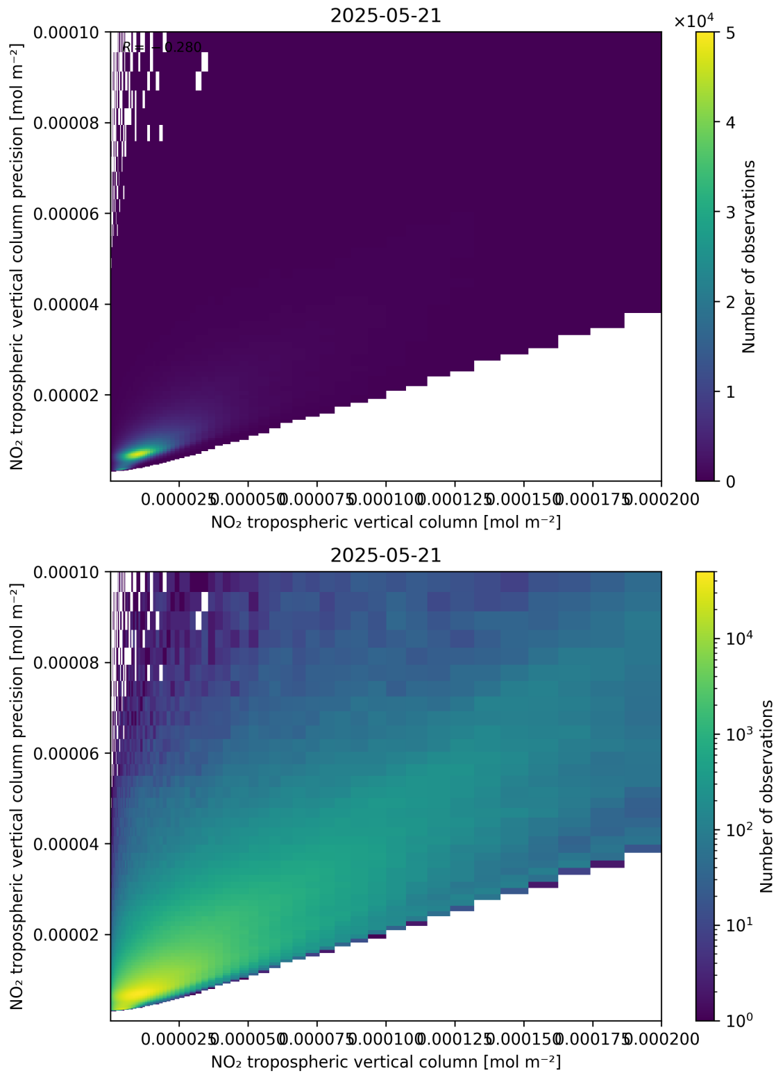
Figure 130: Scatter density plot of “NO 2 tropospheric vertical column” against “NO 2 tropospheric vertical column precision” for 2025-05-21 to 2025-05-22.
