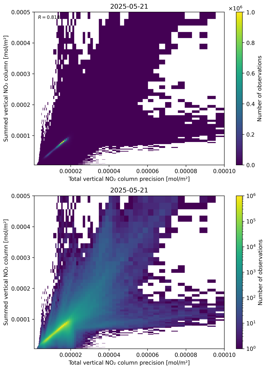
Figure 117: Scatter density plot of “Total vertical NO 2 column precision” against “Summed vertical NO 2 column” for 2025-05-21 to 2025-05-22.
