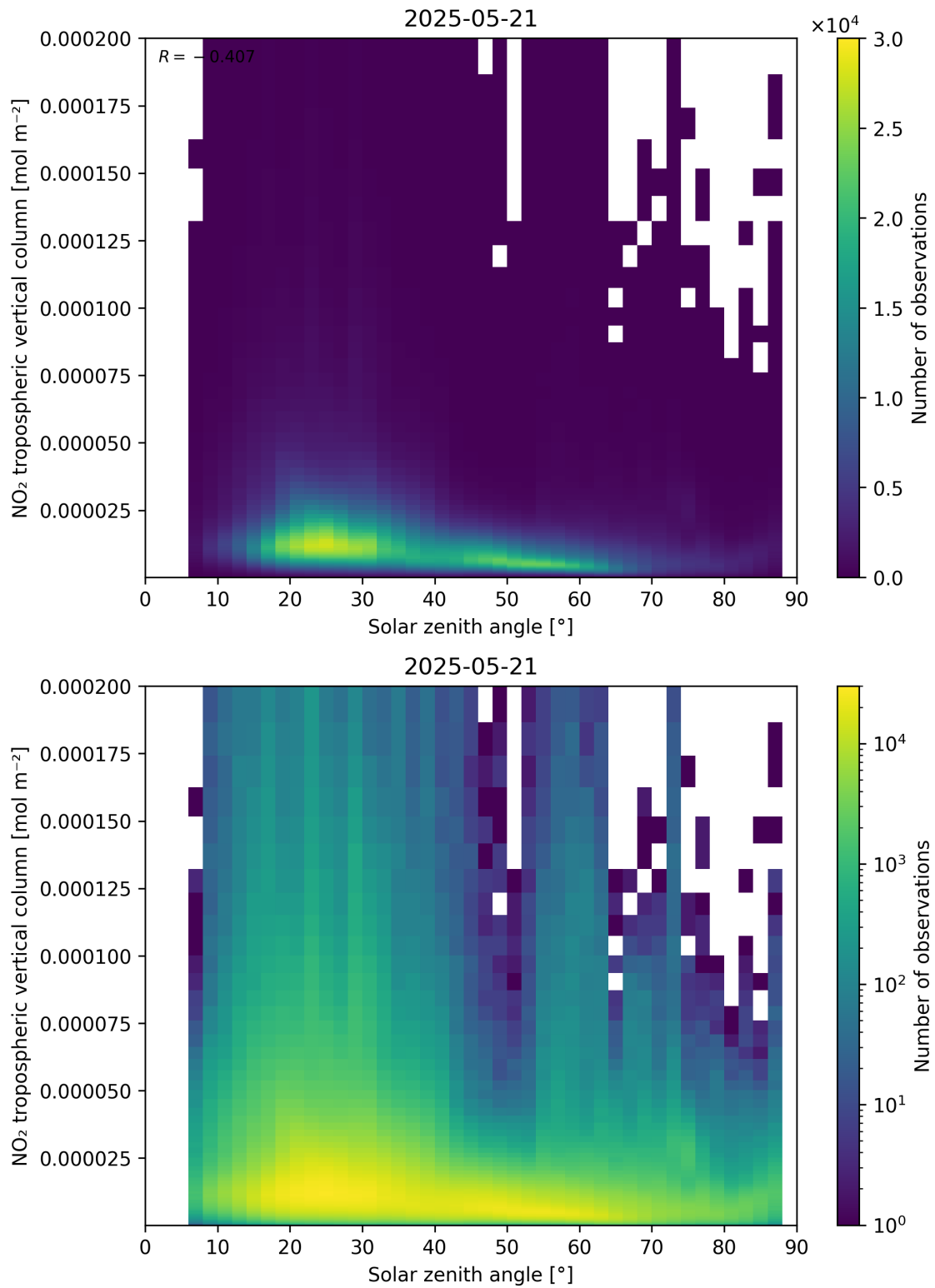
Figure 155: Scatter density plot of “Solar zenith angle” against “NO 2 tropospheric vertical column” for 2025-05-21 to 2025-05-22.
