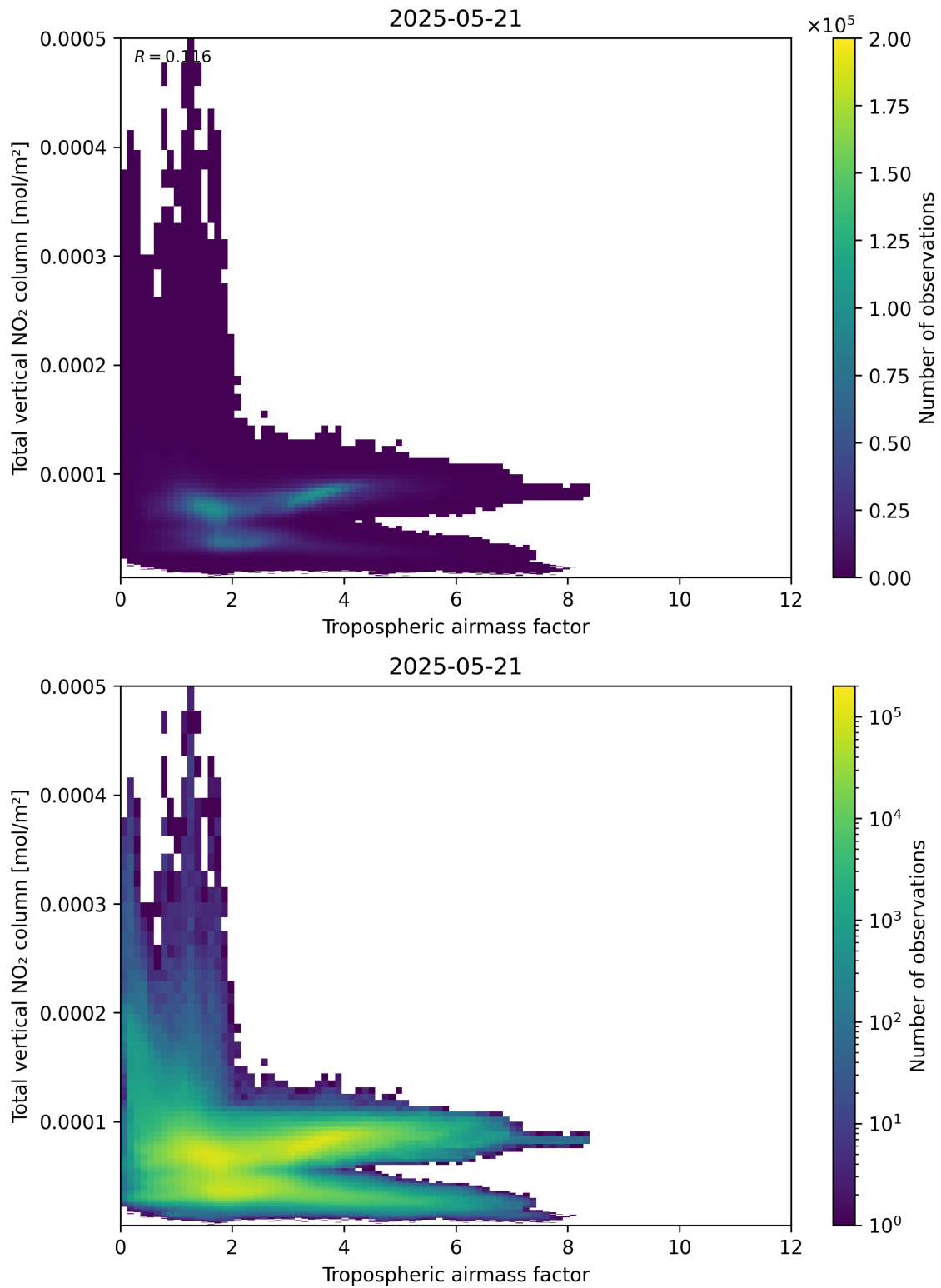
Figure 77: Scatter density plot of “Tropospheric airmass factor” against “Total vertical NO 2 column” for 2025-05-21 to 2025-05-22.
