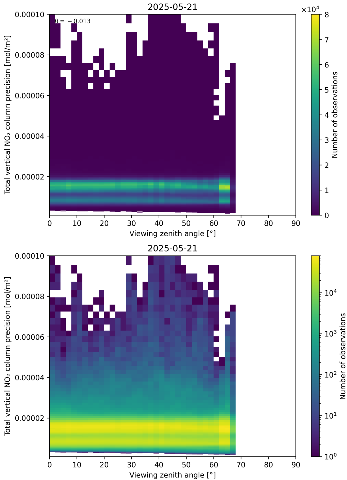
Figure 168: Scatter density plot of “Viewing zenith angle” against “Total vertical NO 2 column precision” for 2025-05-21 to 2025-05-22.
