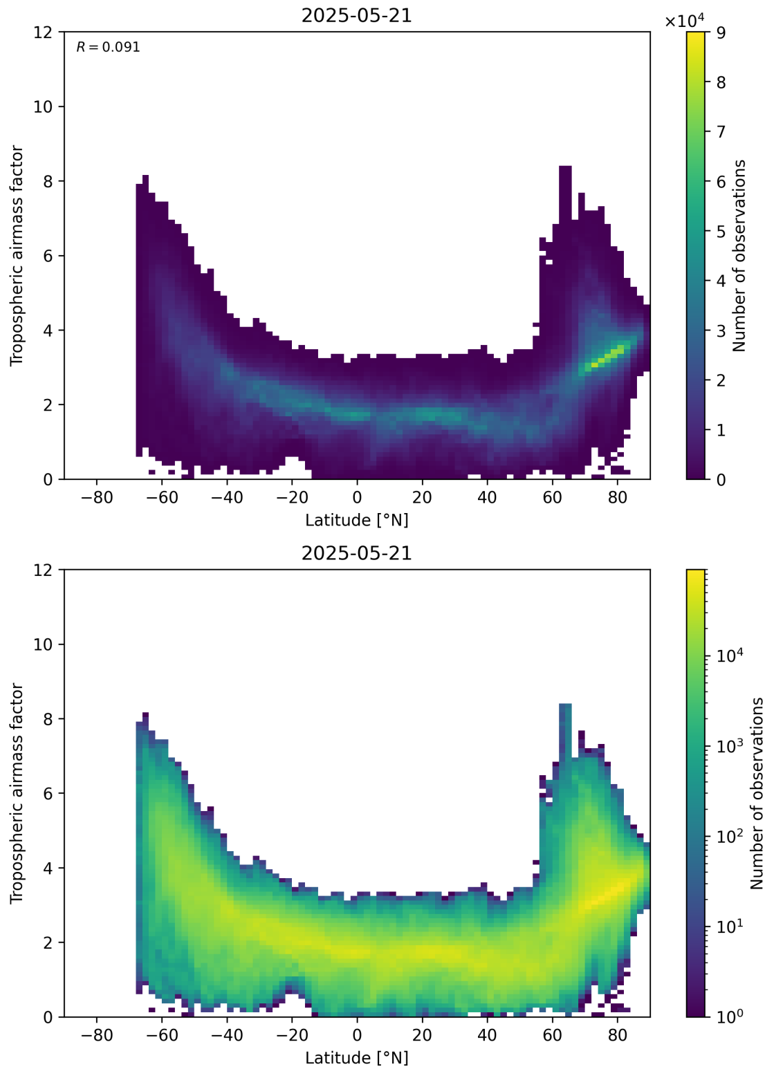
Figure 85: Scatter density plot of “Latitude” against “Tropospheric air mass factor” for 2025-05-21 to 2025-05-22.
