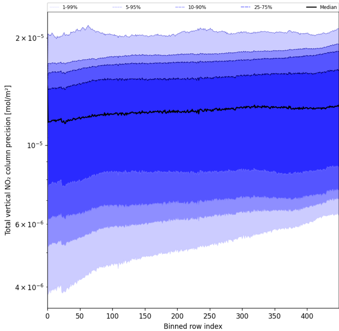
Figure 56: Along track statistics of “Total vertical NO 2 column precision” for 2025-05-21 to 2025-05-22
