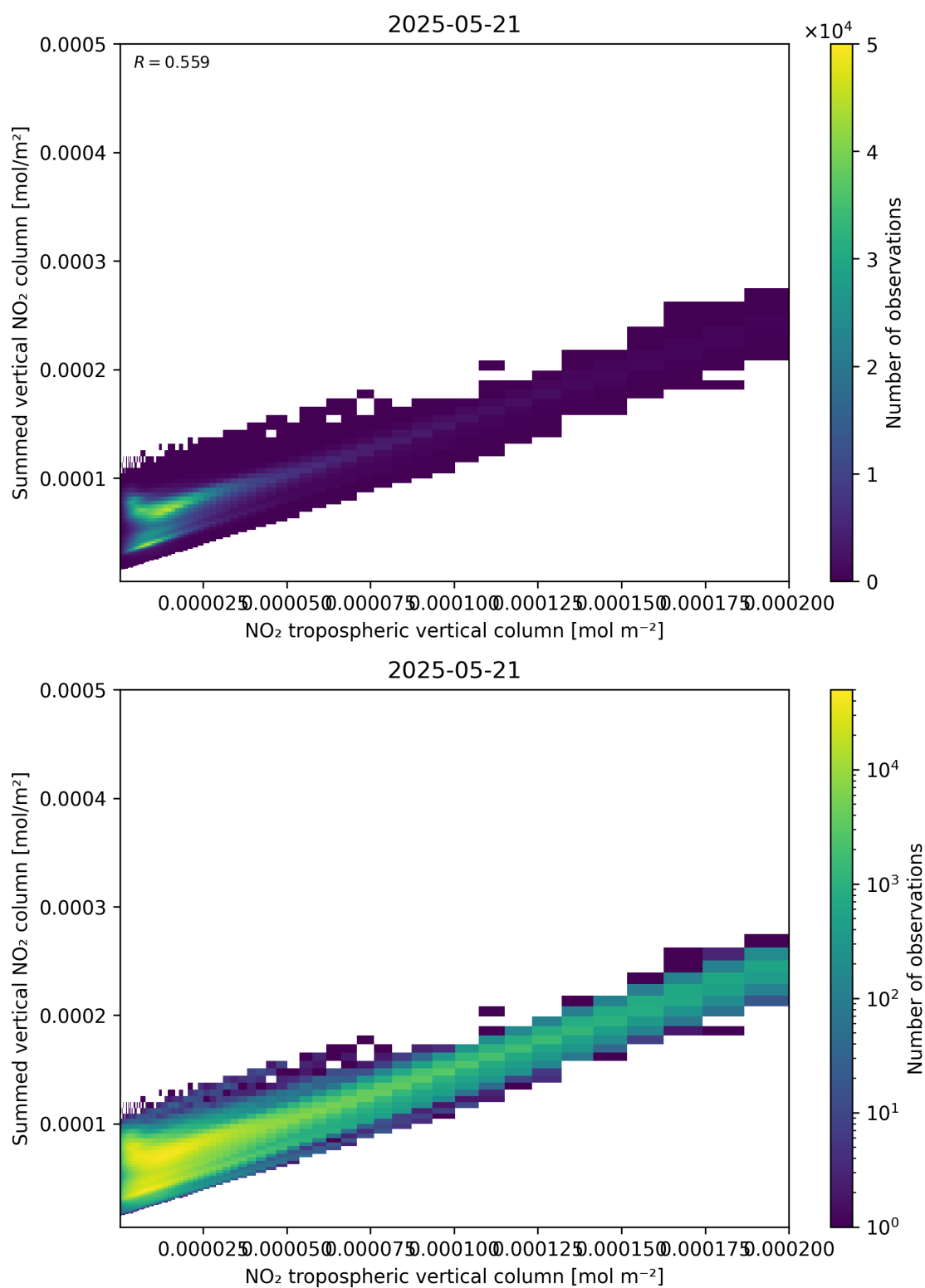
Figure 126: Scatter density plot of “NO 2 tropospheric vertical column” against “Summed vertical NO 2 column” for 2025-05-21 to 2025-05-22.
