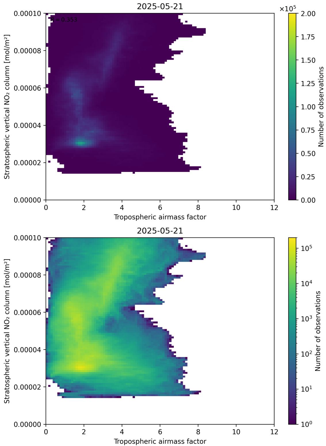
Figure 74: Scatter density plot of “Tropospheric airmass factor” against “Stratospheric vertical NO 2 column” for 2025-05-21 to 2025-05-22.
