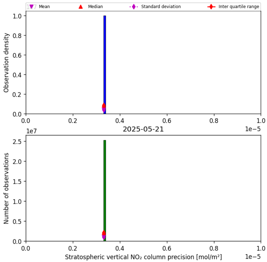
Figure 37: Histogram of “Stratospheric vertical NO 2 column precision” for 2025-05-21 to 2025-05-22
