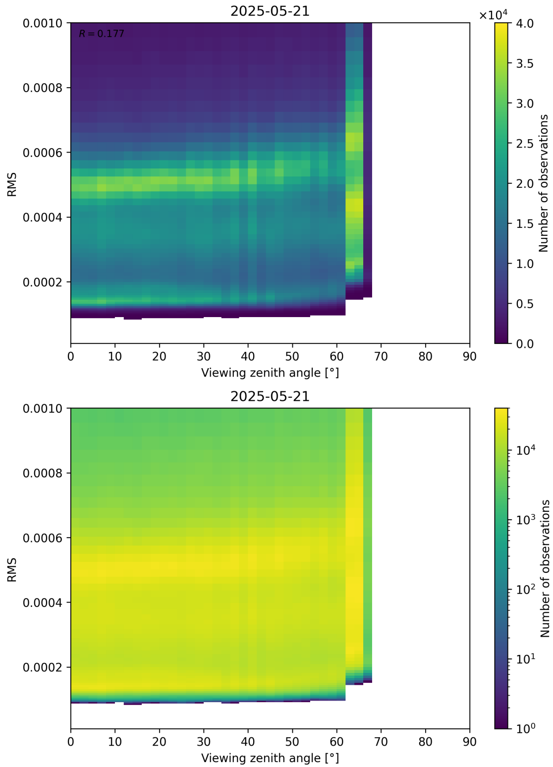
Figure 171: Scatter density plot of “Viewing zenith angle” against “RMS” for 2025-05-21 to 2025-05-22.
