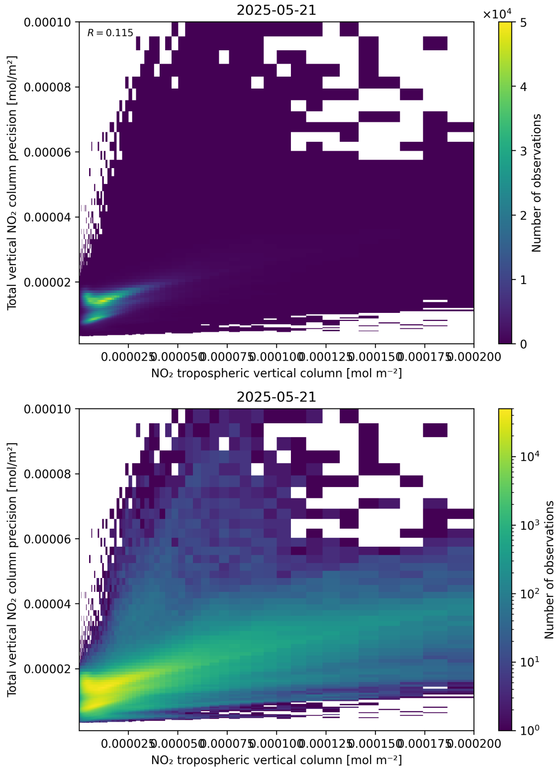
Figure 129: Scatter density plot of “NO 2 tropospheric vertical column” against “Total vertical NO 2 column precision” for 2025-05-21 to 2025-05-22.
