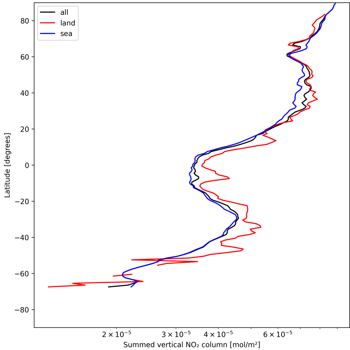
Figure 23: Zonal average of “Summed vertical NO 2 column” for 2025-05-21 to 2025-05-22.
