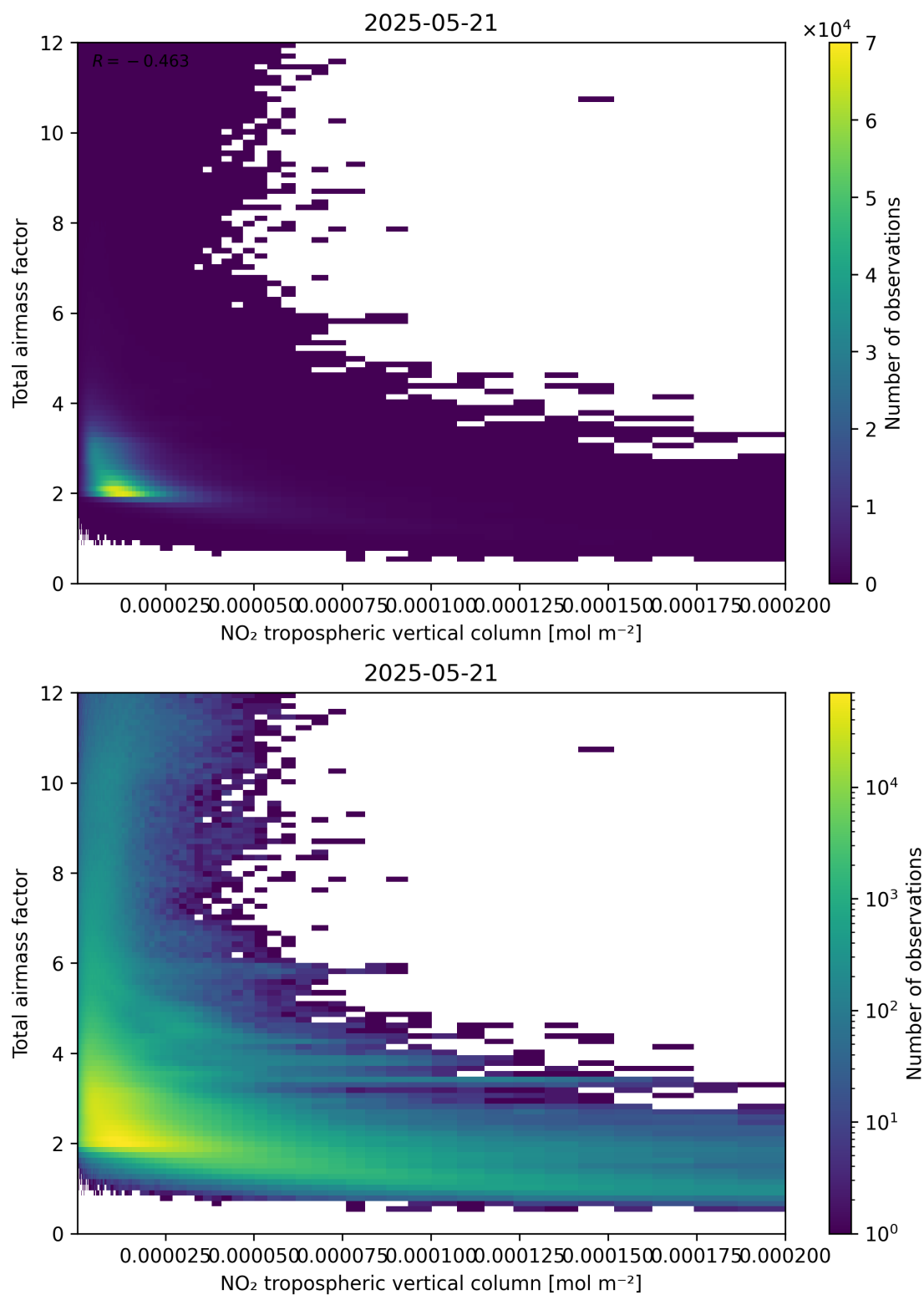
Figure 122: Scatter density plot of “NO 2 tropospheric vertical column” against “Total air mass factor” for 2025-05-21 to 2025-05-22.
