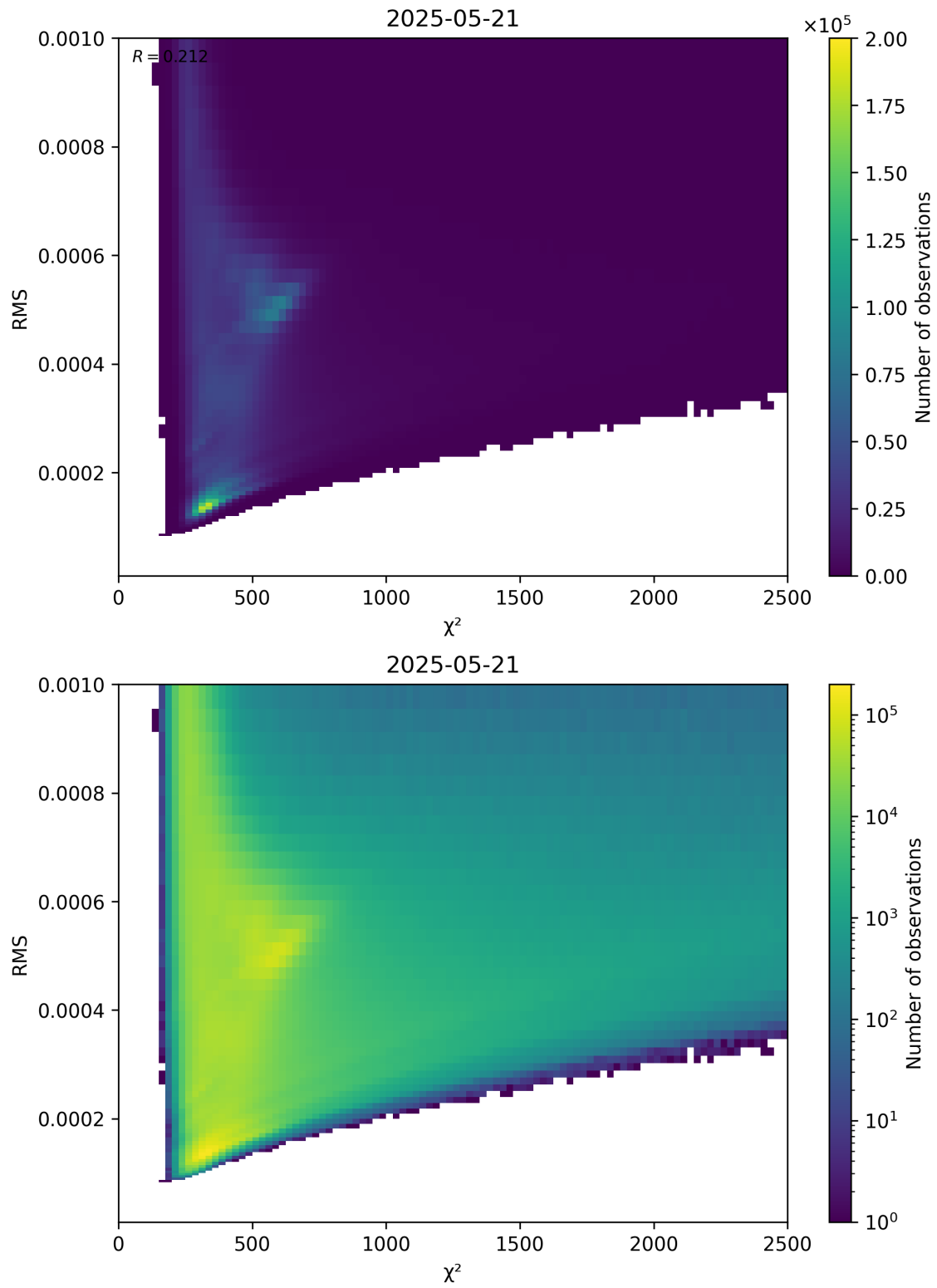
Figure 82: Scatter density plot of “ \chi^2 ” against “RMS” for 2025-05-21 to 2025-05-22.
