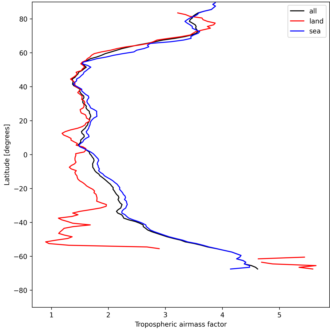
Figure 14: Zonal average of “Tropospheric air mass factor” for 2025-05-21 to 2025-05-22.
