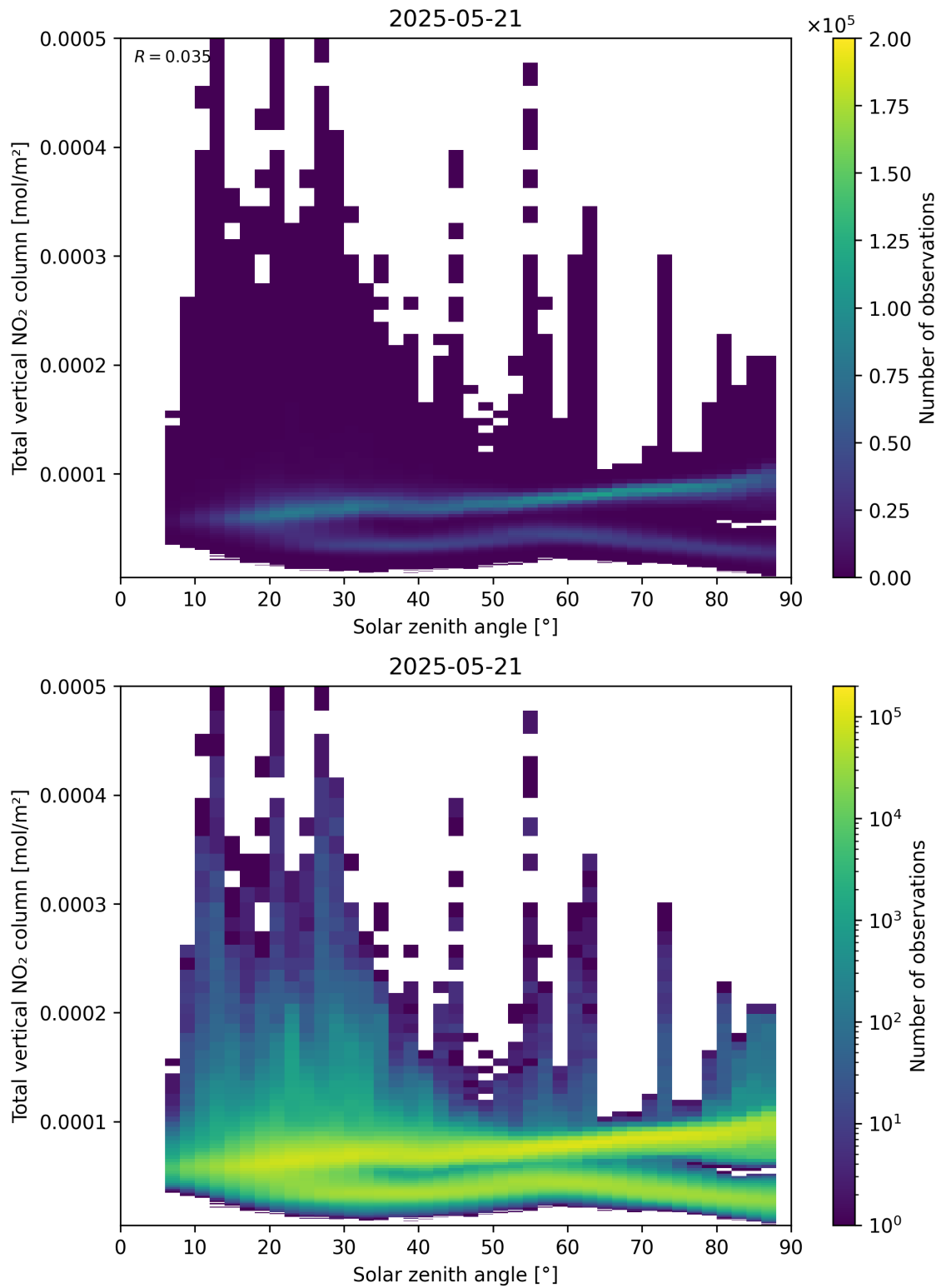
Figure 153: Scatter density plot of “Solar zenith angle” against “Total vertical NO 2 column” for 2025-05-21 to 2025-05-22.
