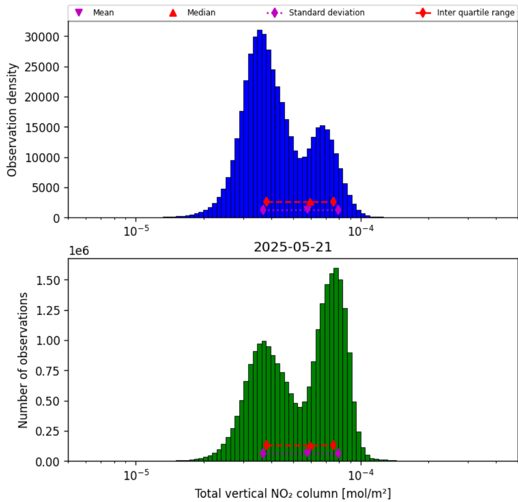
Figure 38: Histogram of “Total vertical NO 2 column” for 2025-05-21 to 2025-05-22
