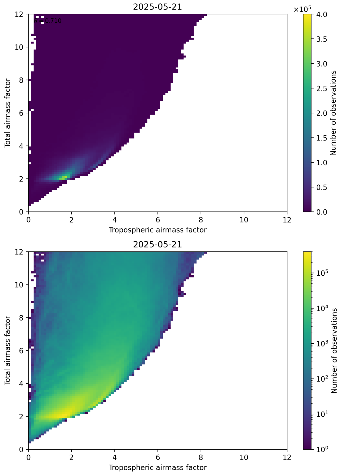
Figure 72: Scatter density plot of “Tropospheric airmass factor” against “Total airmass factor” for 2025-05-21 to 2025-05-22.
