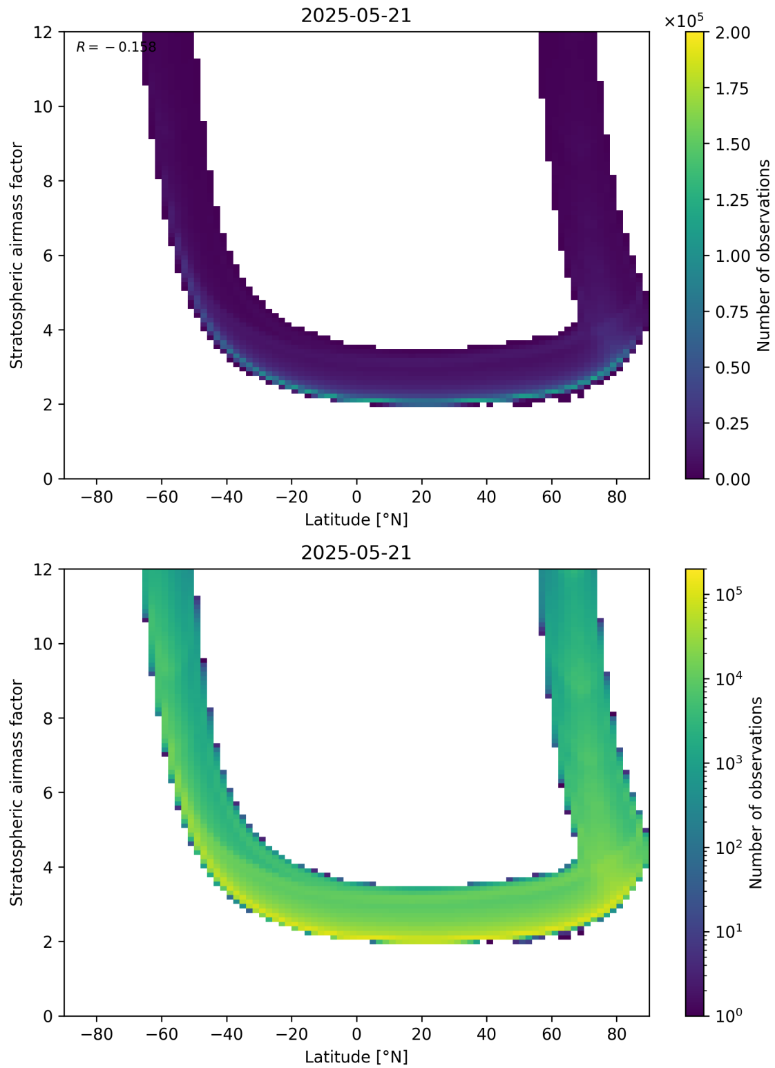
Figure 83: Scatter density plot of “Latitude” against “Stratospheric air mass factor” for 2025-05-21 to 2025-05-22.
