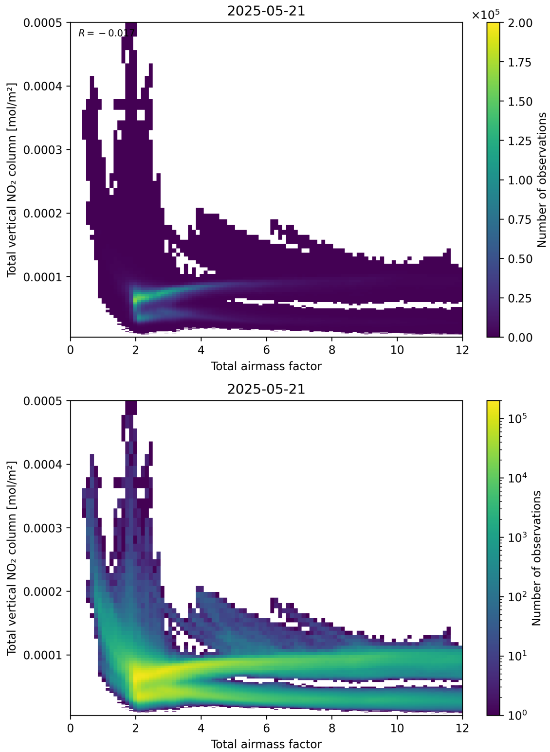
Figure 67: Scatter density plot of “Total airmass factor” against “Total vertical NO 2 column” for 2025-05-21 to 2025-05-22.
