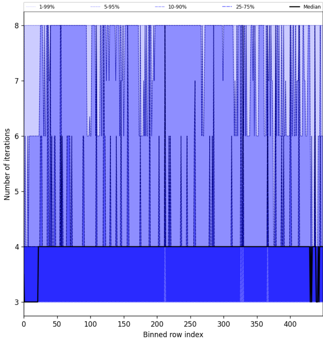
Figure 51: Along track statistics of “Number of iterations” for 2025-05-21 to 2025-05-22
