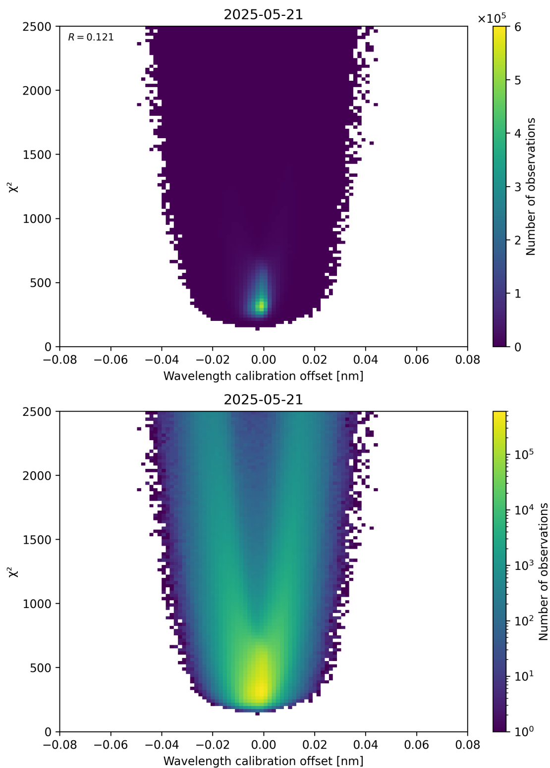
Figure 175: Scatter density plot of “Wavelength calibration offset” against “ \chi^2 ” for 2025-05-21 to 2025-05-22.
