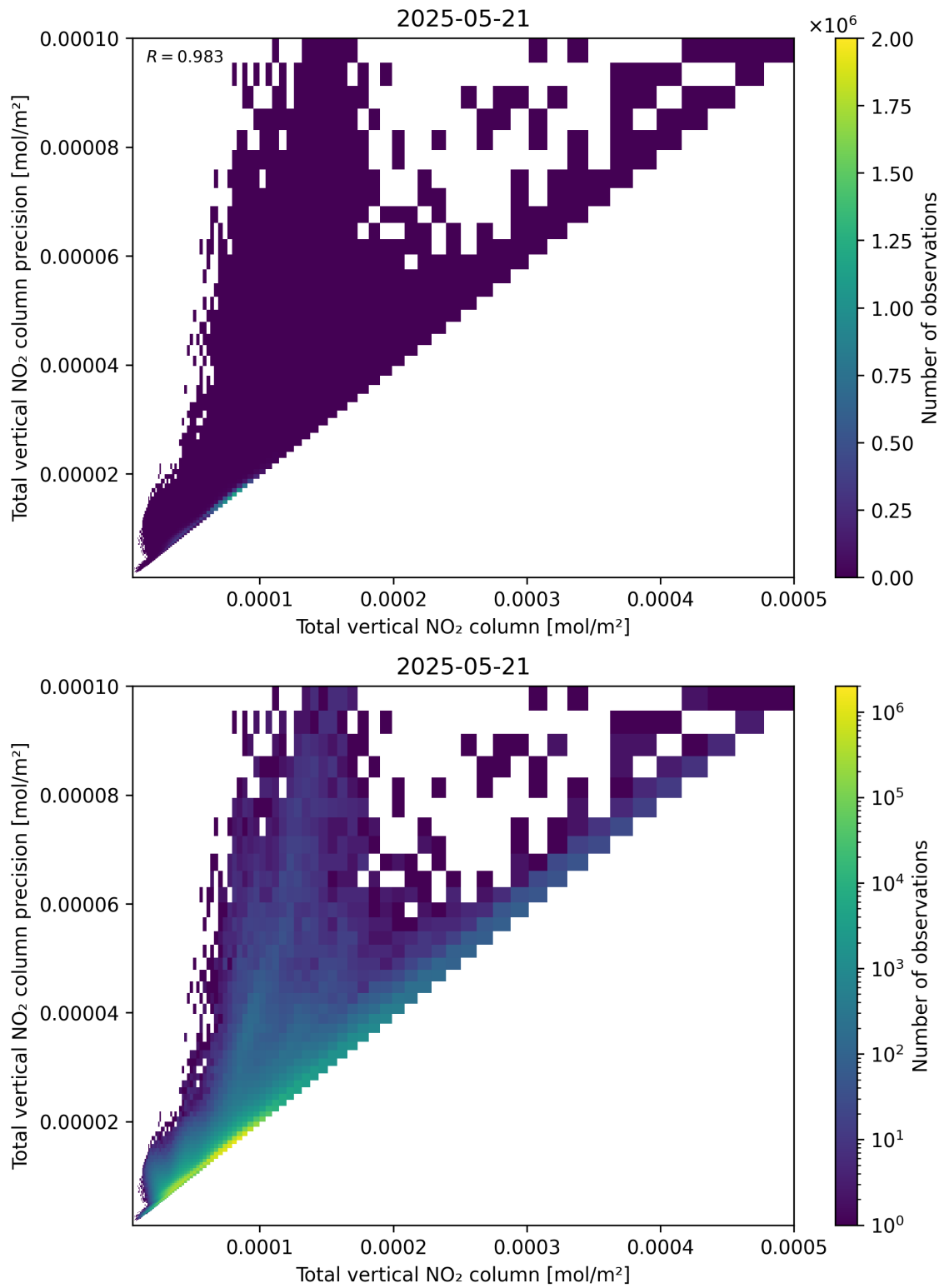
Figure 114: Scatter density plot of “Total vertical NO 2 column” against “Total vertical NO 2 column precision” for 2025-05-21 to 2025-05-22.
