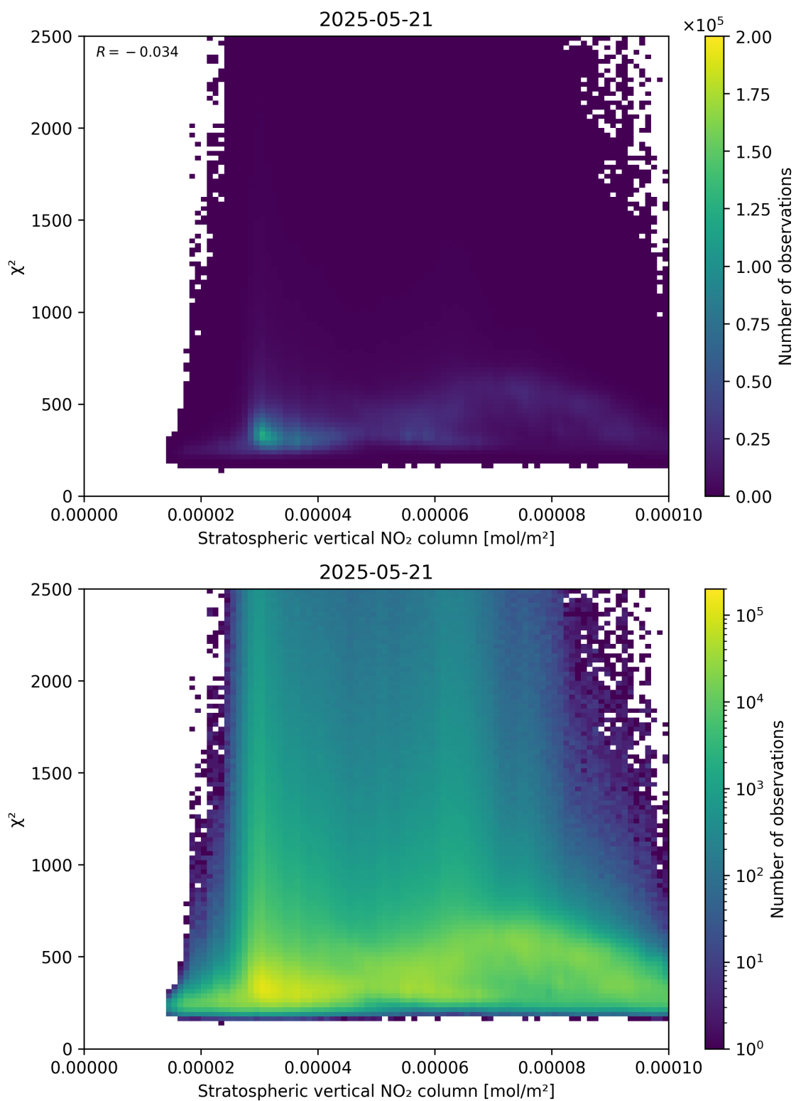
Figure 97: Scatter density plot of “Stratospheric vertical NO 2 column” against “ \chi^2 ” for 2025-05-21 to 2025-05-22.
