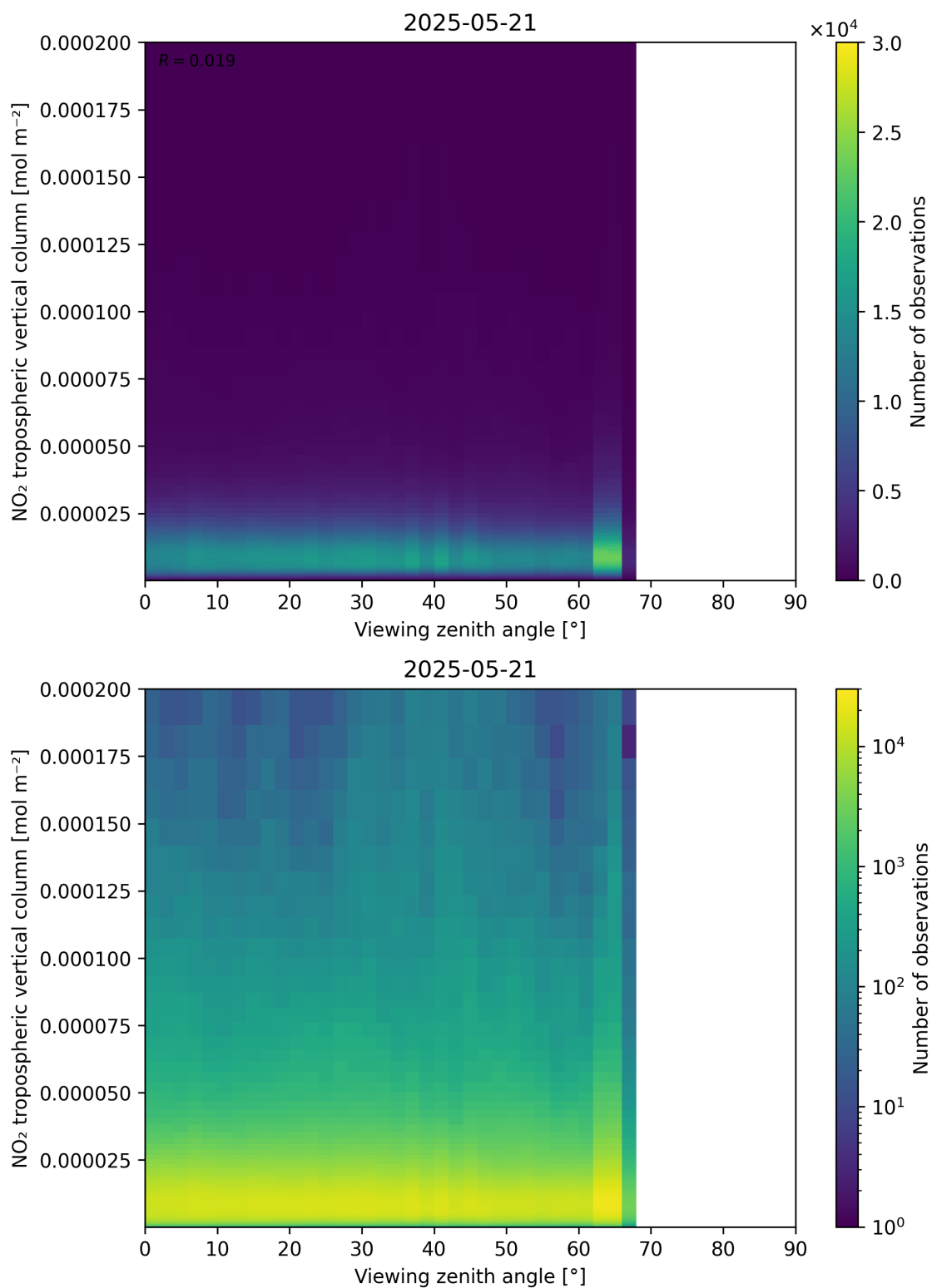
Figure 169: Scatter density plot of “Viewing zenith angle” against “NO 2 tropospheric vertical column” for 2025-05-21 to 2025-05-22.
