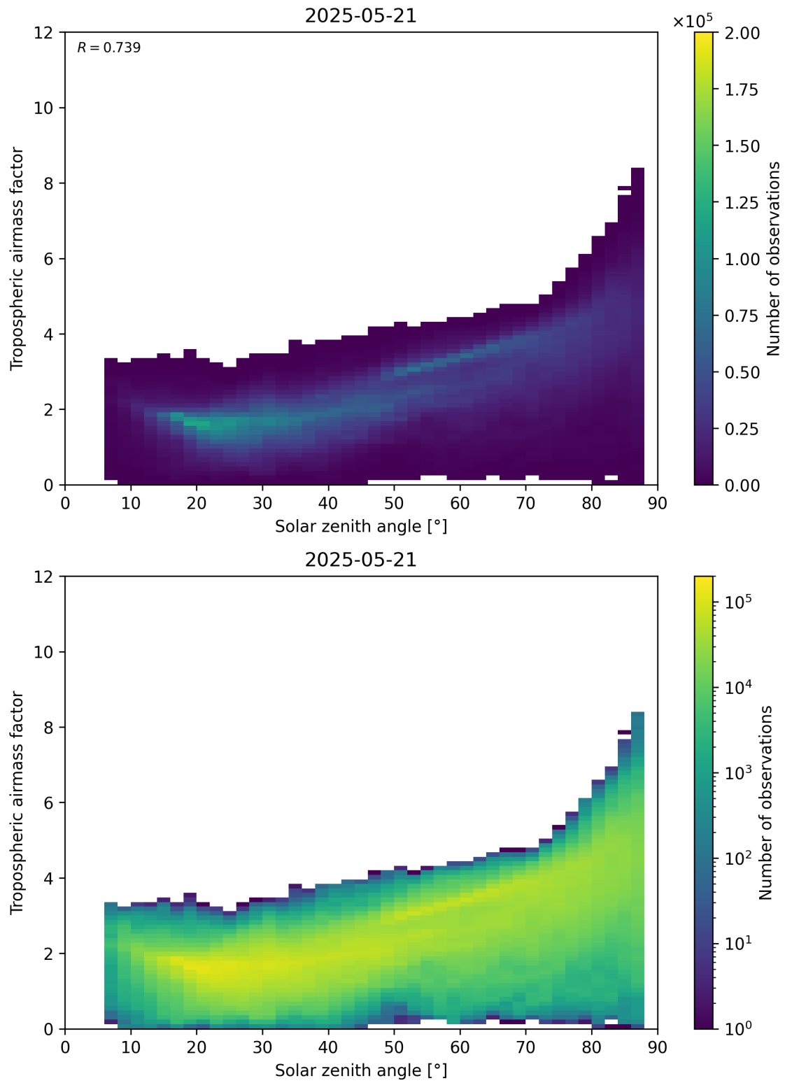
Figure 147: Scatter density plot of “Solar zenith angle” against “Tropospheric airmass factor” for 2025-05-21 to 2025-05-22.
