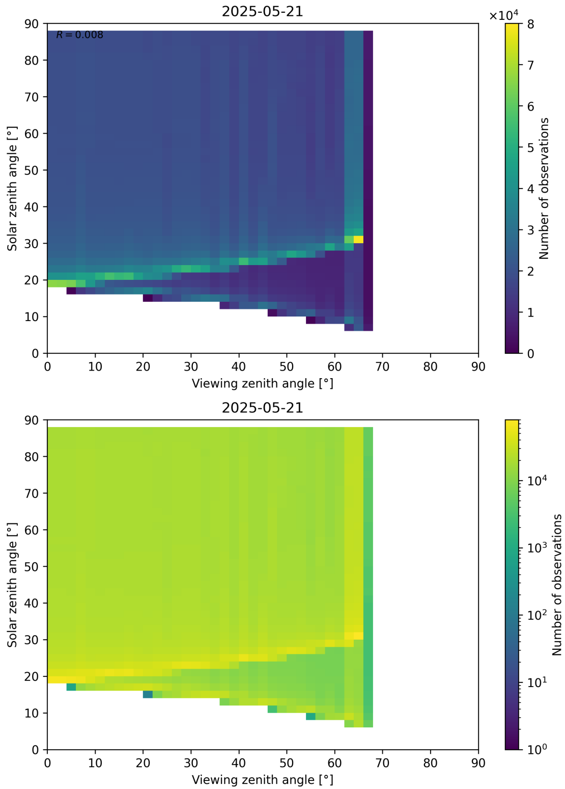
Figure 172: Scatter density plot of “Viewing zenith angle” against “Solar zenith angle” for 2025-05-21 to 2025-05-22.
