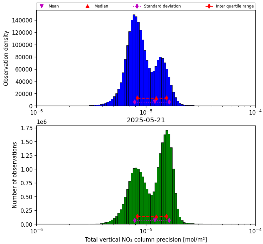
Figure 39: Histogram of “Total vertical NO 2 column precision” for 2025-05-21 to 2025-05-22
