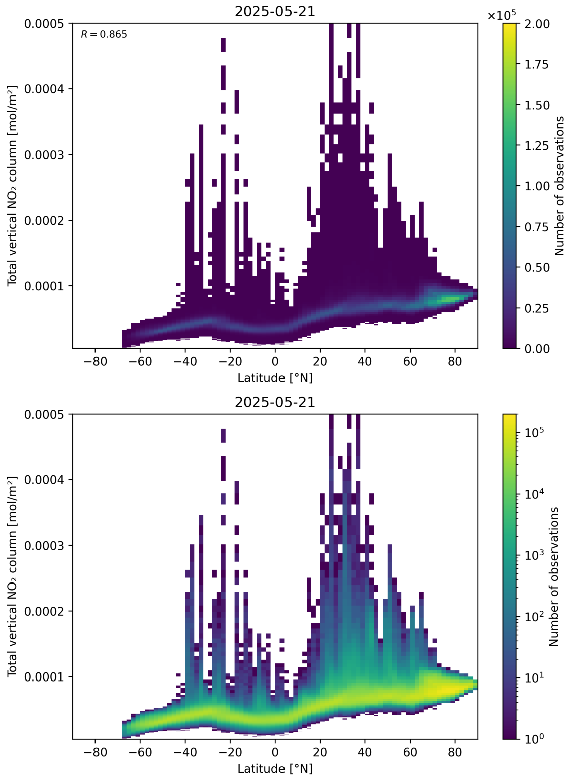
Figure 90: Scatter density plot of “Latitude” against “Total vertical NO 2 column” for 2025-05-21 to 2025-05-22.
