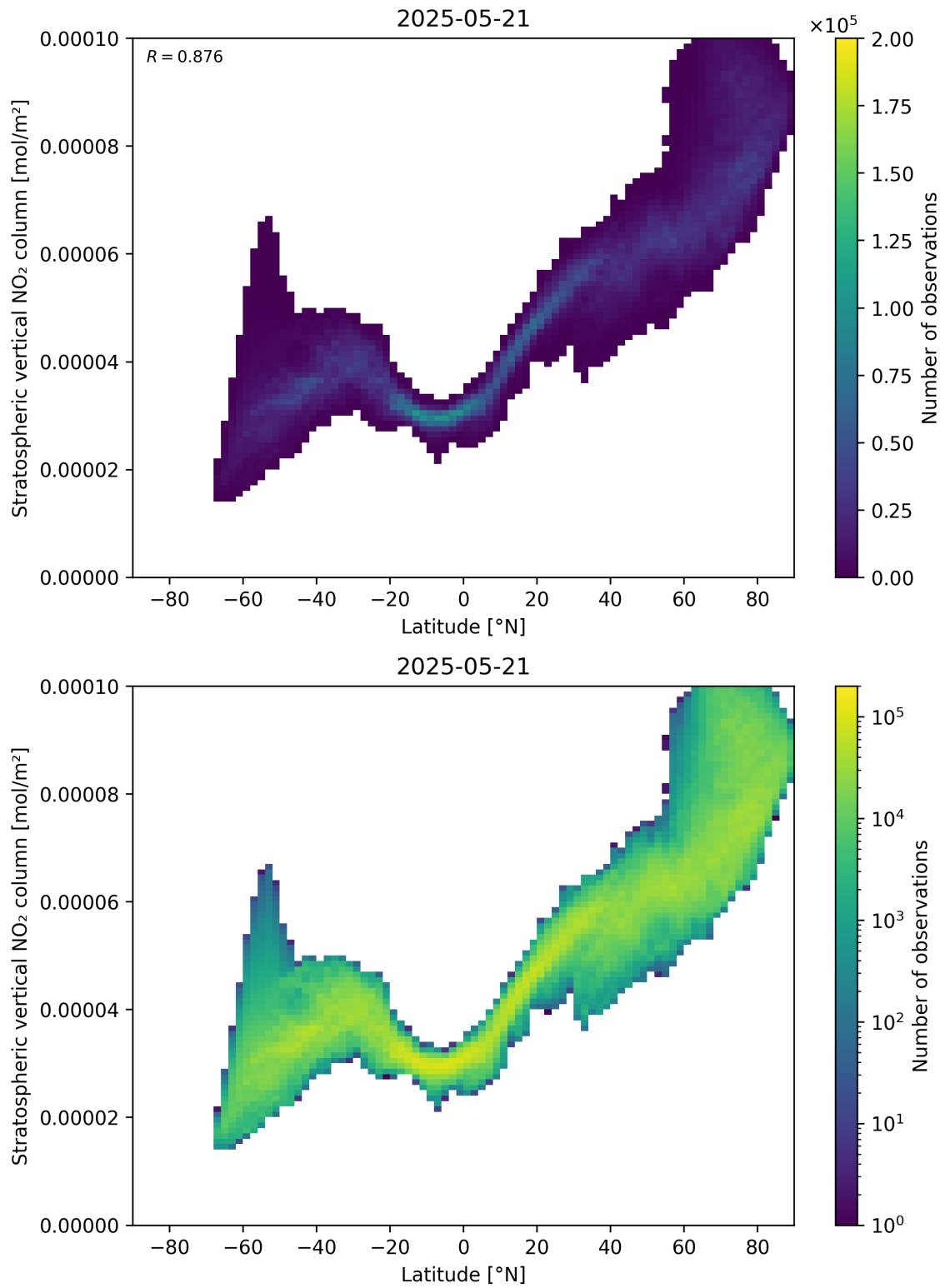
Figure 87: Scatter density plot of “Latitude” against “Stratospheric vertical NO 2 column” for 2025-05-21 to 2025-05-22.
