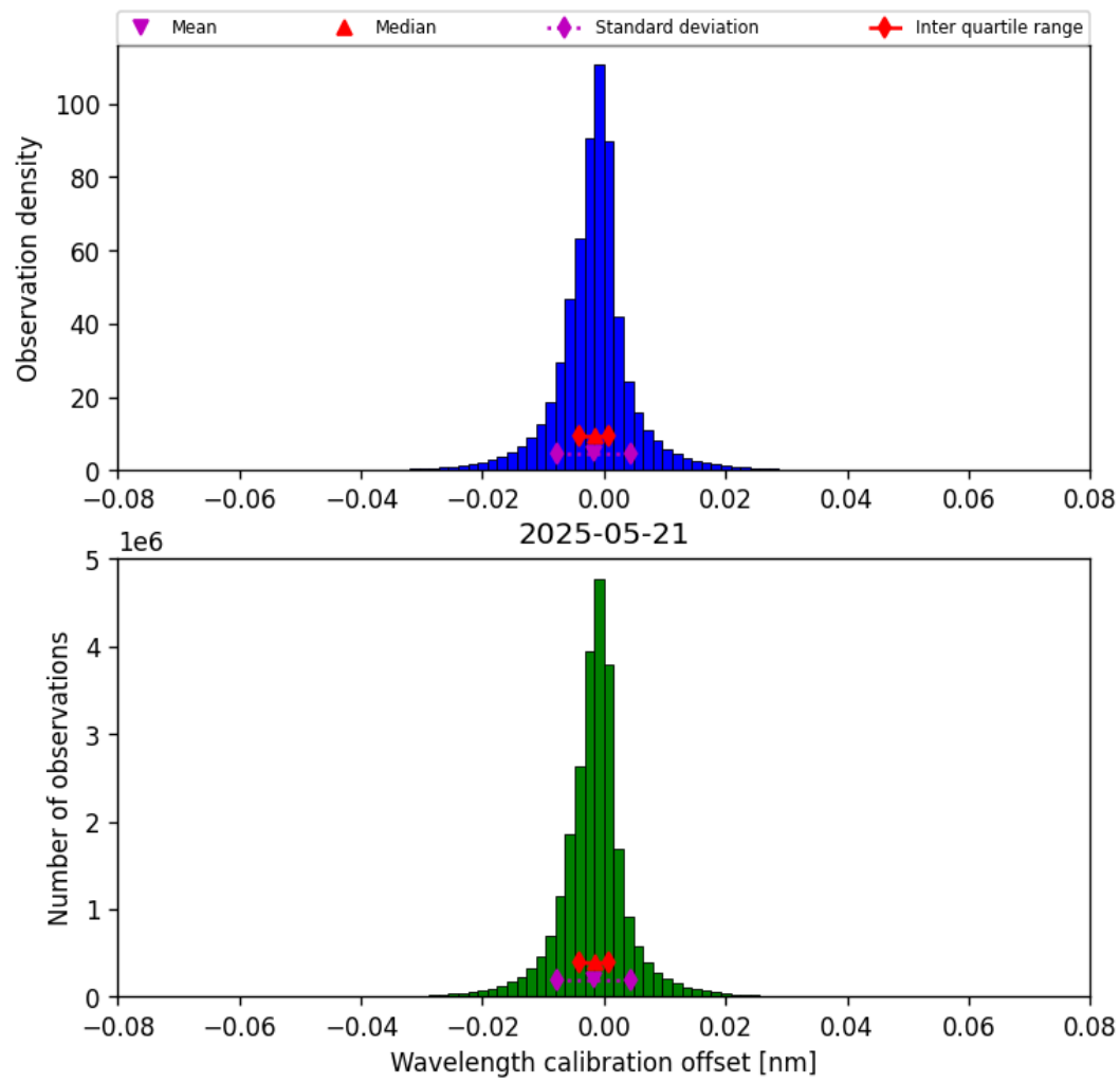
Figure 35: Histogram of “Wavelength calibration offset” for 2025-05-21 to 2025-05-22
