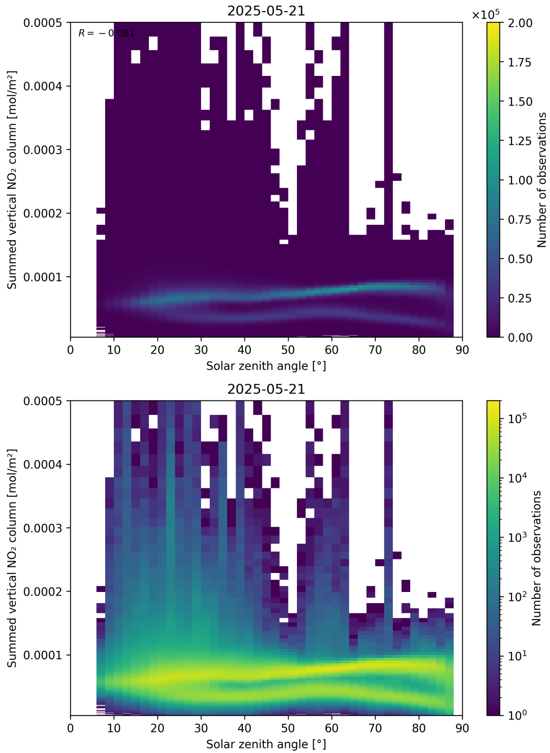
Figure 151: Scatter density plot of “Solar zenith angle” against “Summed vertical NO 2 column” for 2025-05-21 to 2025-05-22.
