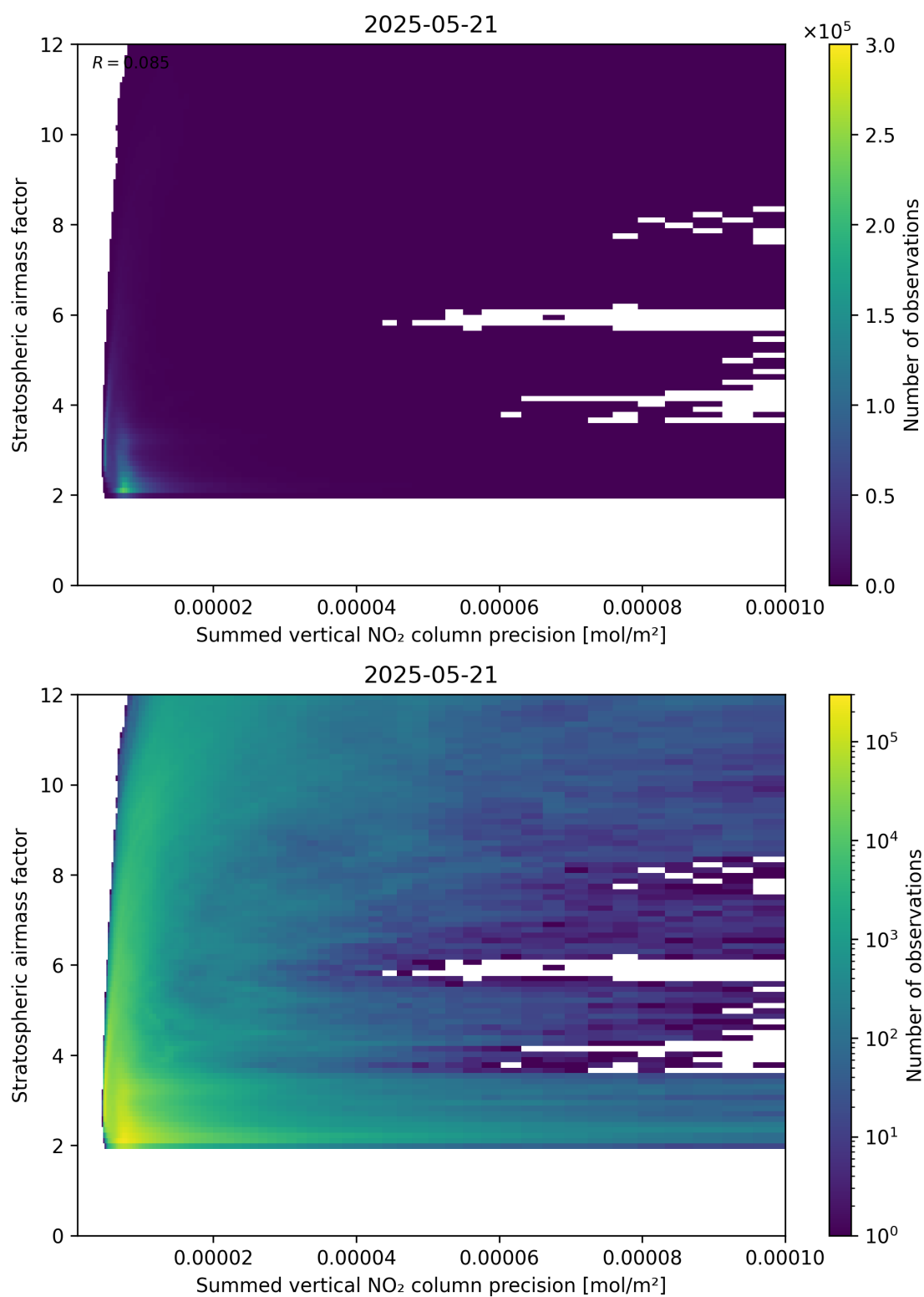
Figure 106: Scatter density plot of “Summed vertical NO 2 column precision” against “Stratospheric airmass factor” for 2025-05-21 to 2025-05-22.
