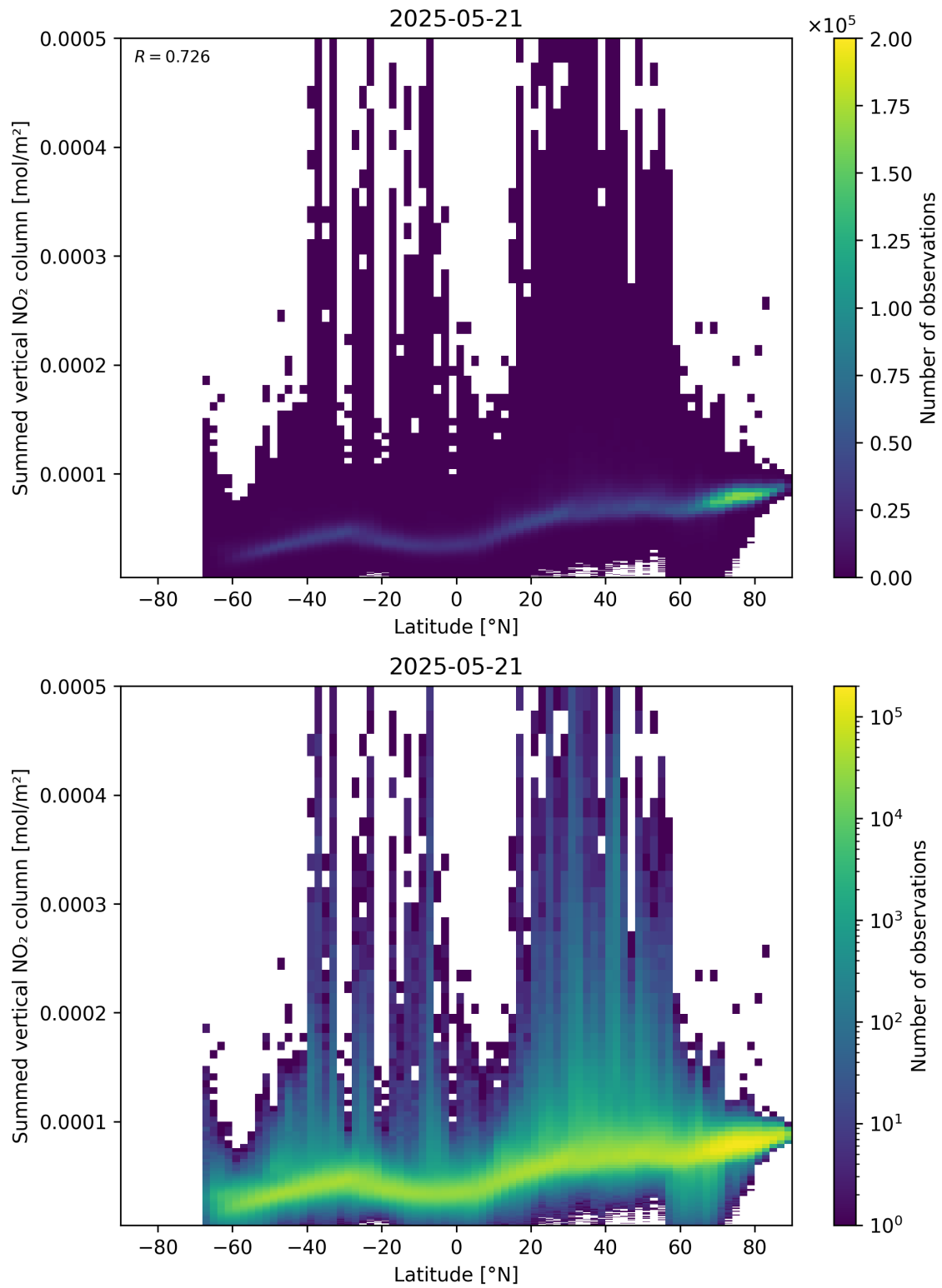
Figure 88: Scatter density plot of “Latitude” against “Summed vertical NO 2 column” for 2025-05-21 to 2025-05-22.
