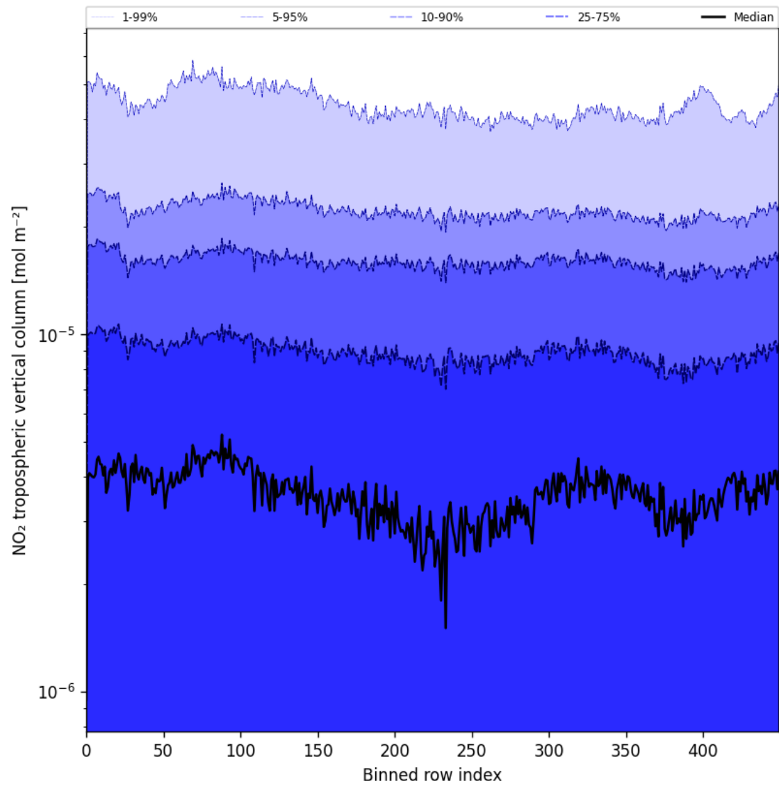
Figure 46: Along track statistics of “NO 2 tropospheric vertical column” for 2025-05-21 to 2025-05-22
