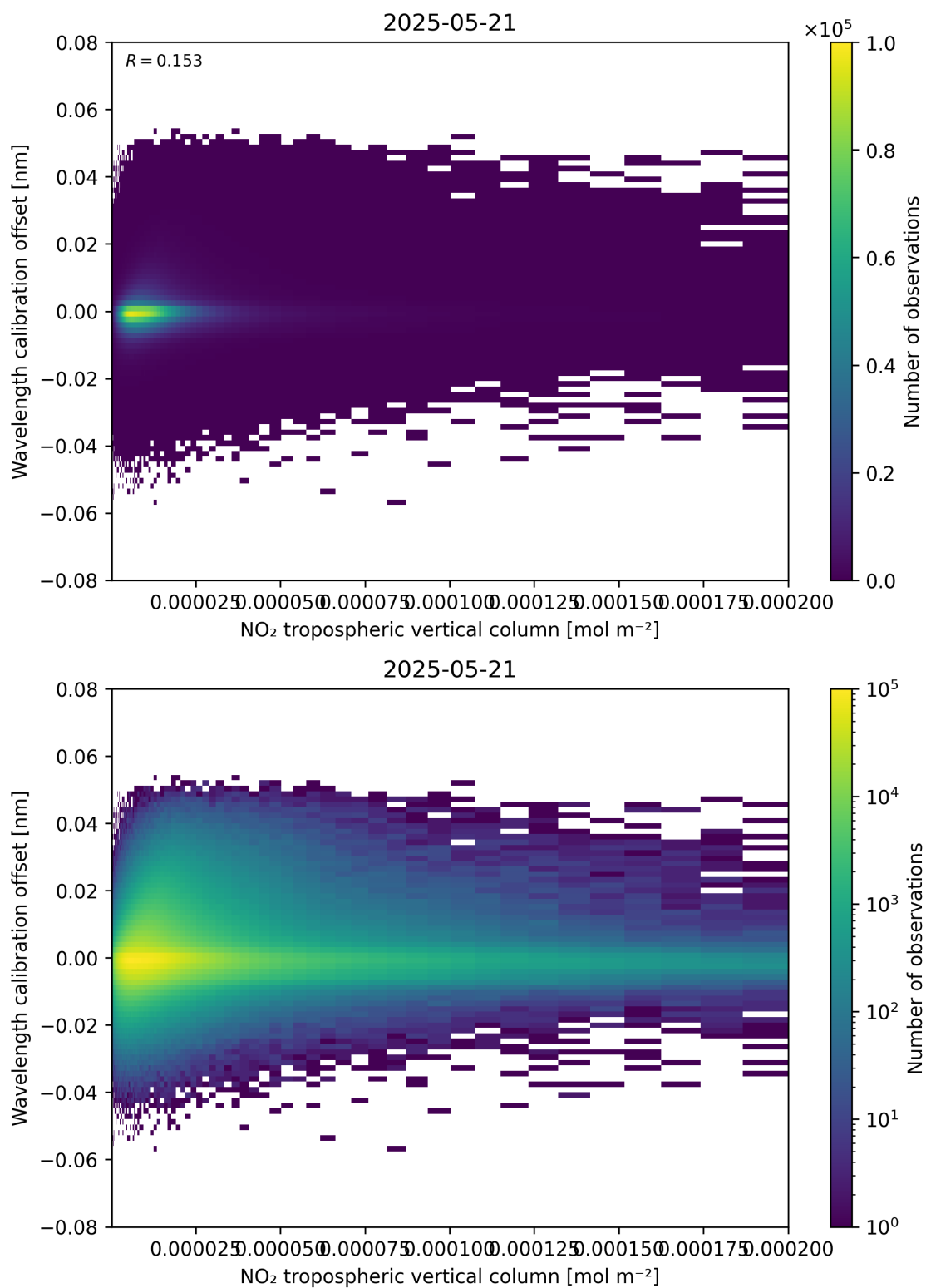
Figure 143: Scatter density plot of “NO 2 tropospheric vertical column” against “Wavelength calibration offset” for 2025-05-21 to 2025-05-22.
