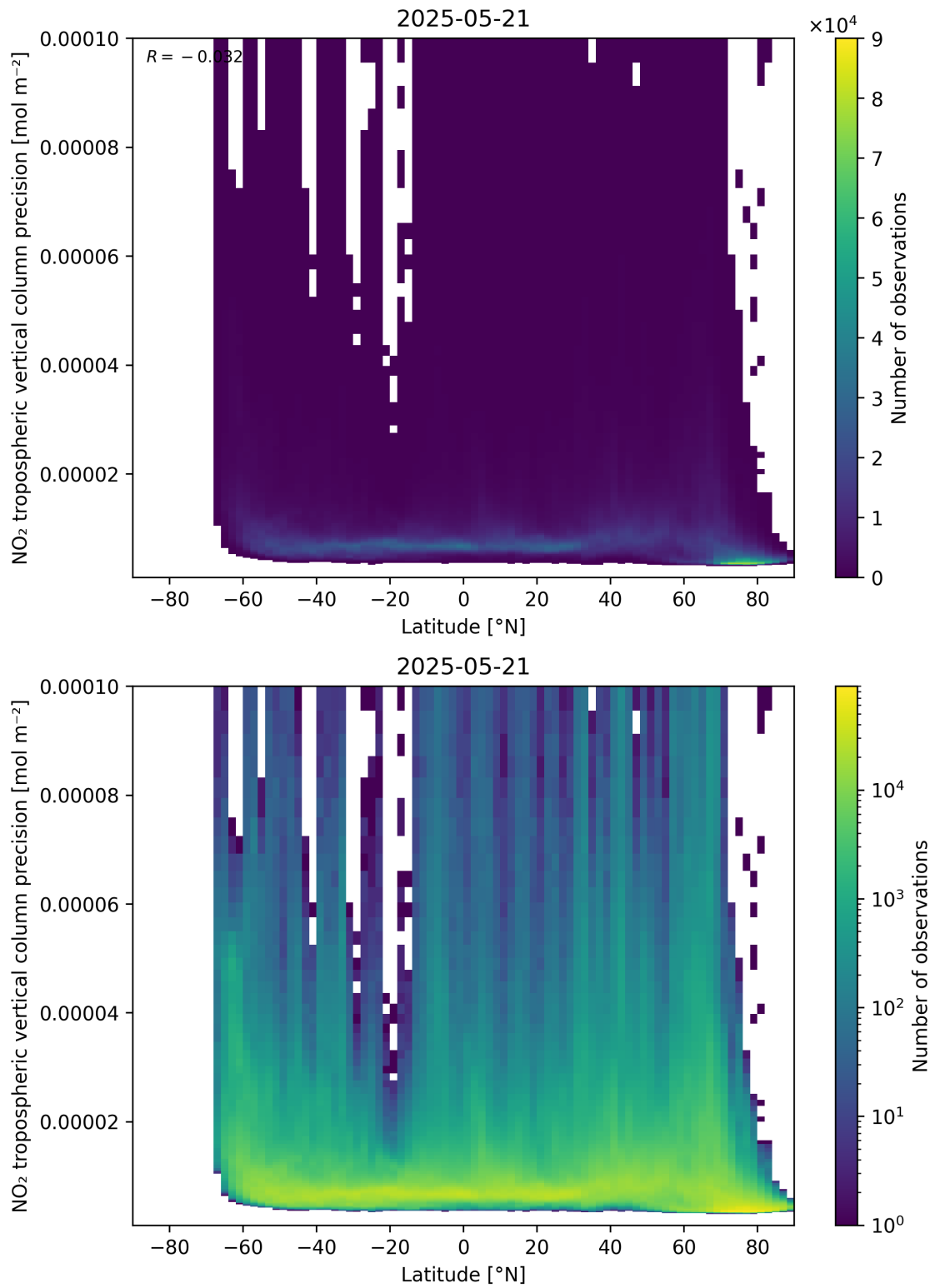
Figure 93: Scatter density plot of “Latitude” against “NO 2 tropospheric vertical column precision” for 2025-05-21 to 2025-05-22.
