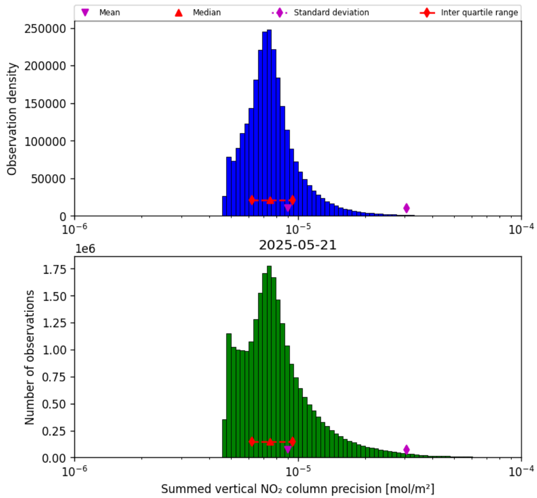
Figure 41: Histogram of “Summed vertical NO 2 column precision” for 2025-05-21 to 2025-05-22
