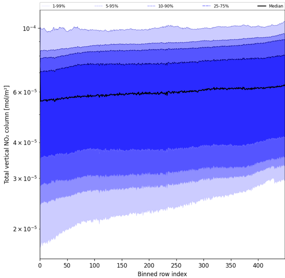
Figure 55: Along track statistics of “Total vertical NO 2 column” for 2025-05-21 to 2025-05-22
