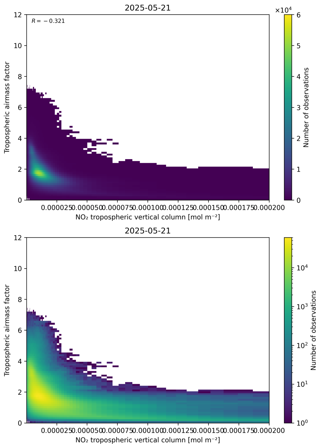
Figure 123: Scatter density plot of “NO 2 tropospheric vertical column” against “Tropospheric air mass factor” for 2025-05-21 to 2025-05-22.
