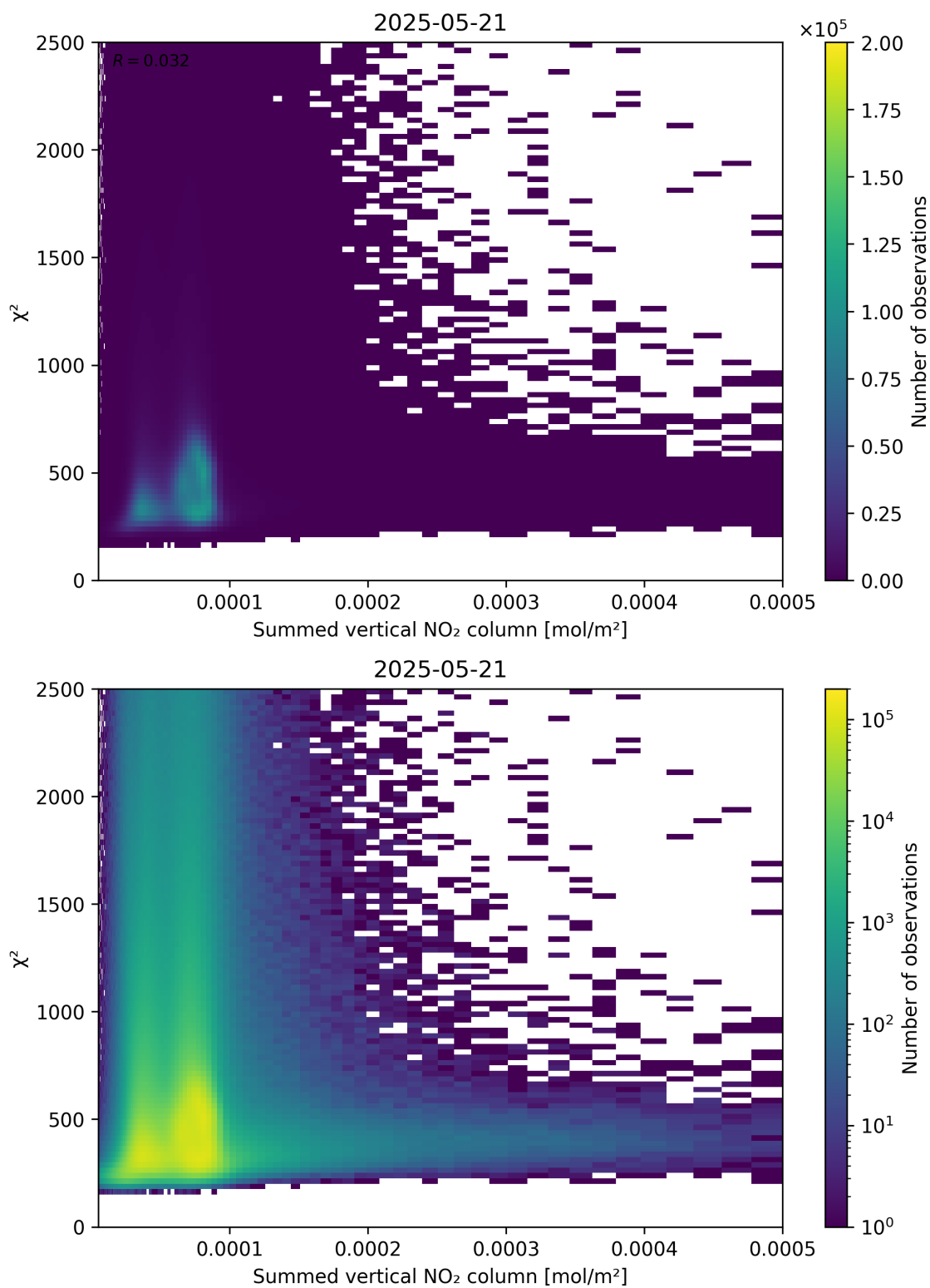
Figure 104: Scatter density plot of “Summed vertical NO 2 column” against “ \chi^2 ” for 2025-05-21 to 2025-05-22.
