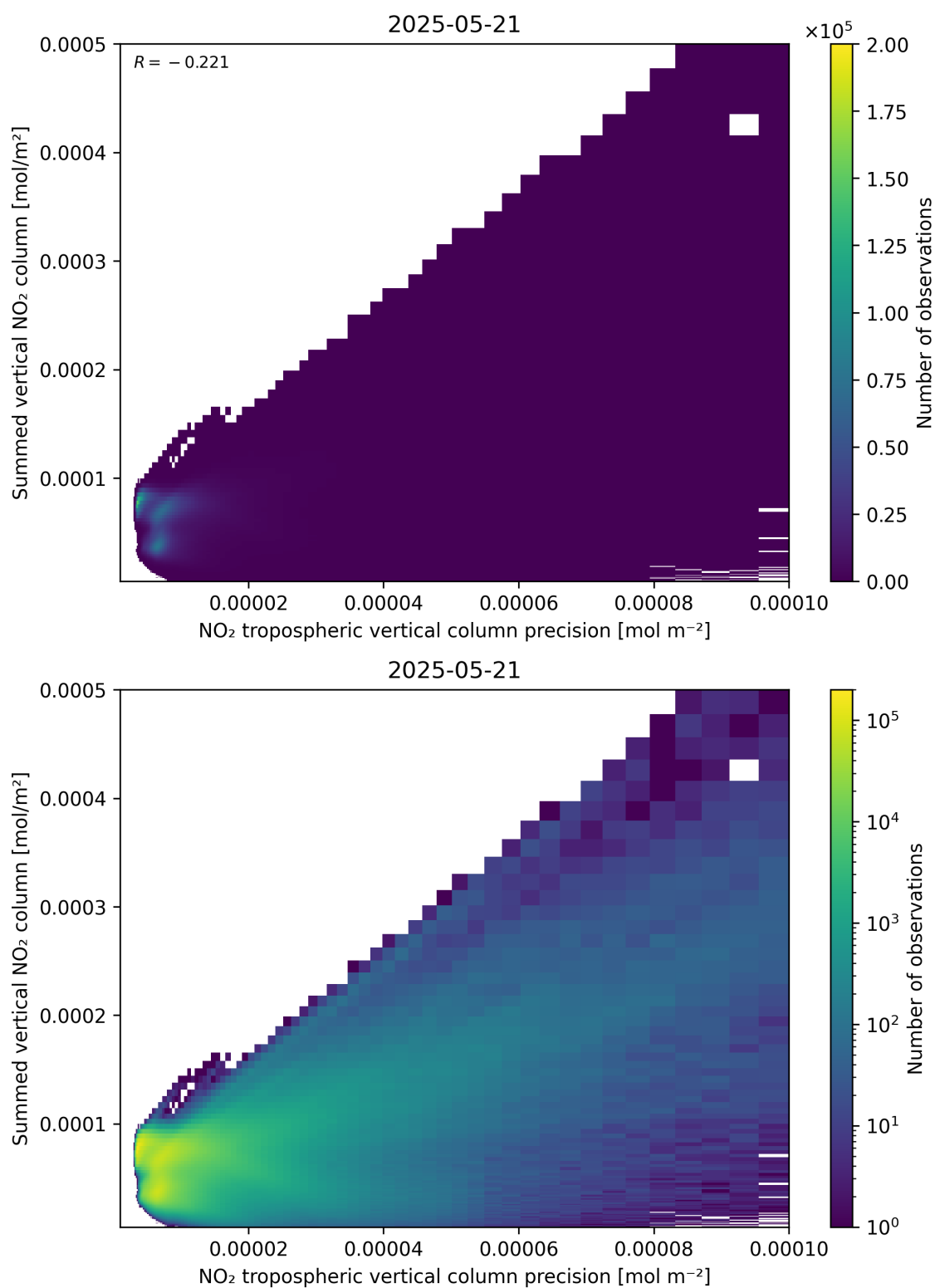
Figure 136: Scatter density plot of “NO 2 tropospheric vertical column precision” against “Summed vertical NO 2 column” for 2025-05-21 to 2025-05-22.
