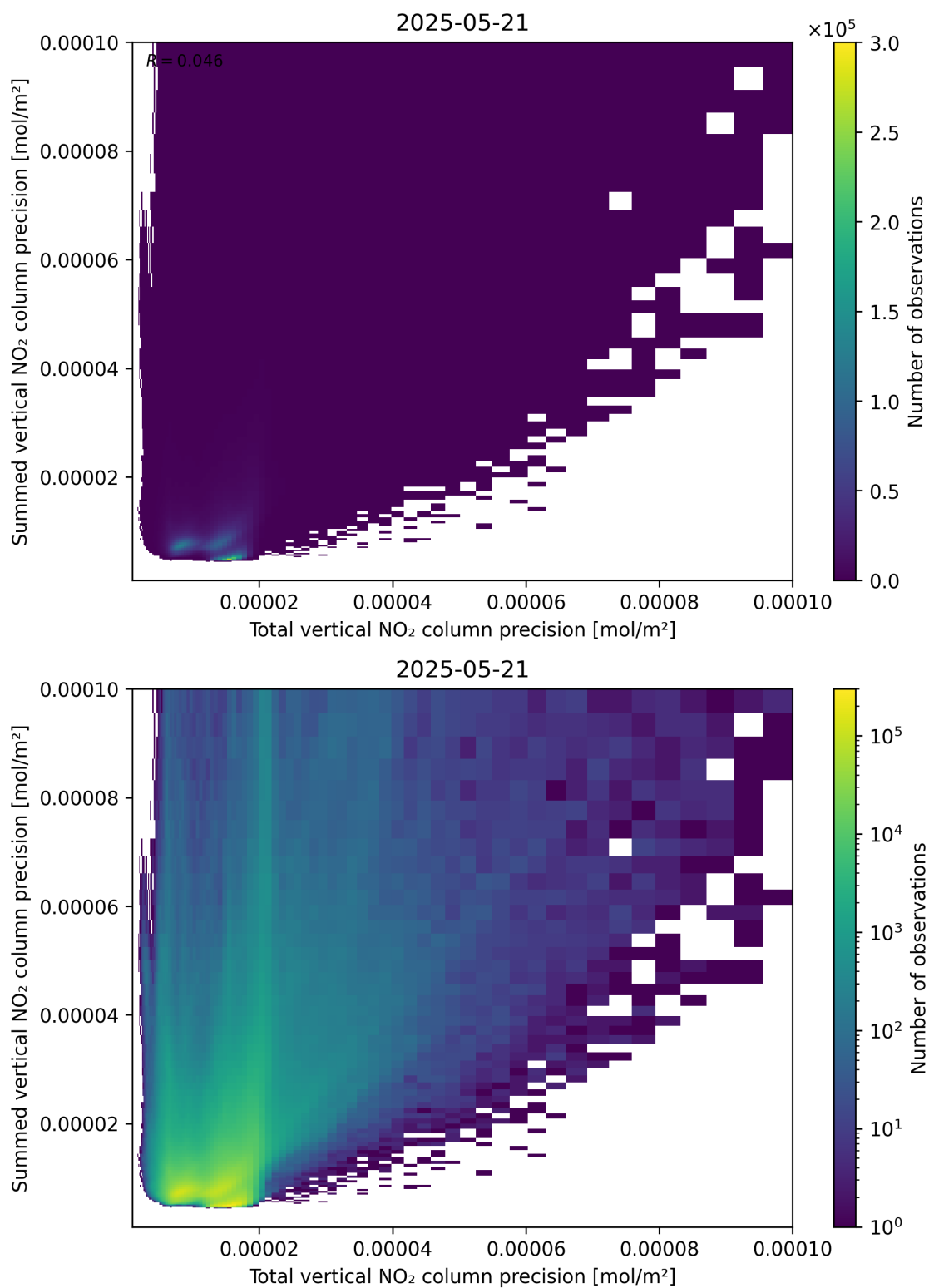
Figure 118: Scatter density plot of “Total vertical NO 2 column precision” against “Summed vertical NO 2 column precision” for 2025-05-21 to 2025-05-22.
