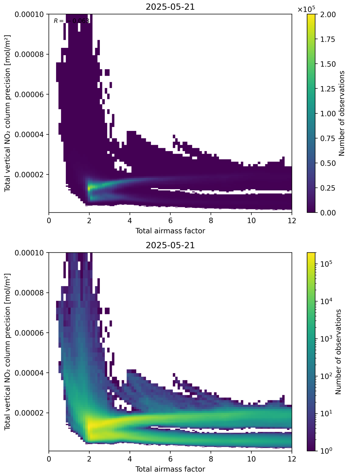
Figure 68: Scatter density plot of “Total airmass factor” against “Total vertical NO 2 column precision” for 2025-05-21 to 2025-05-22.
