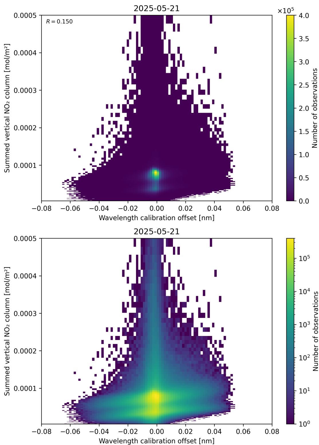
Figure 177: Scatter density plot of “Wavelength calibration offset” against “Summed vertical NO 2 column” for 2025-05-21 to 2025-05-22.
