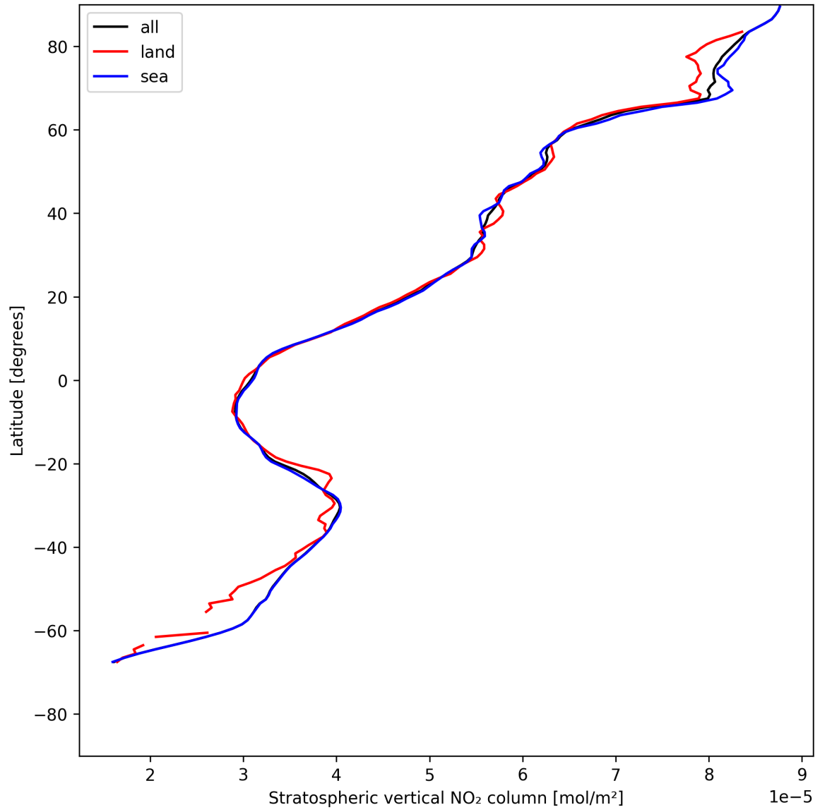
Figure 19: Zonal average of “Stratospheric vertical NO 2 column” for 2025-05-21 to 2025-05-22.
