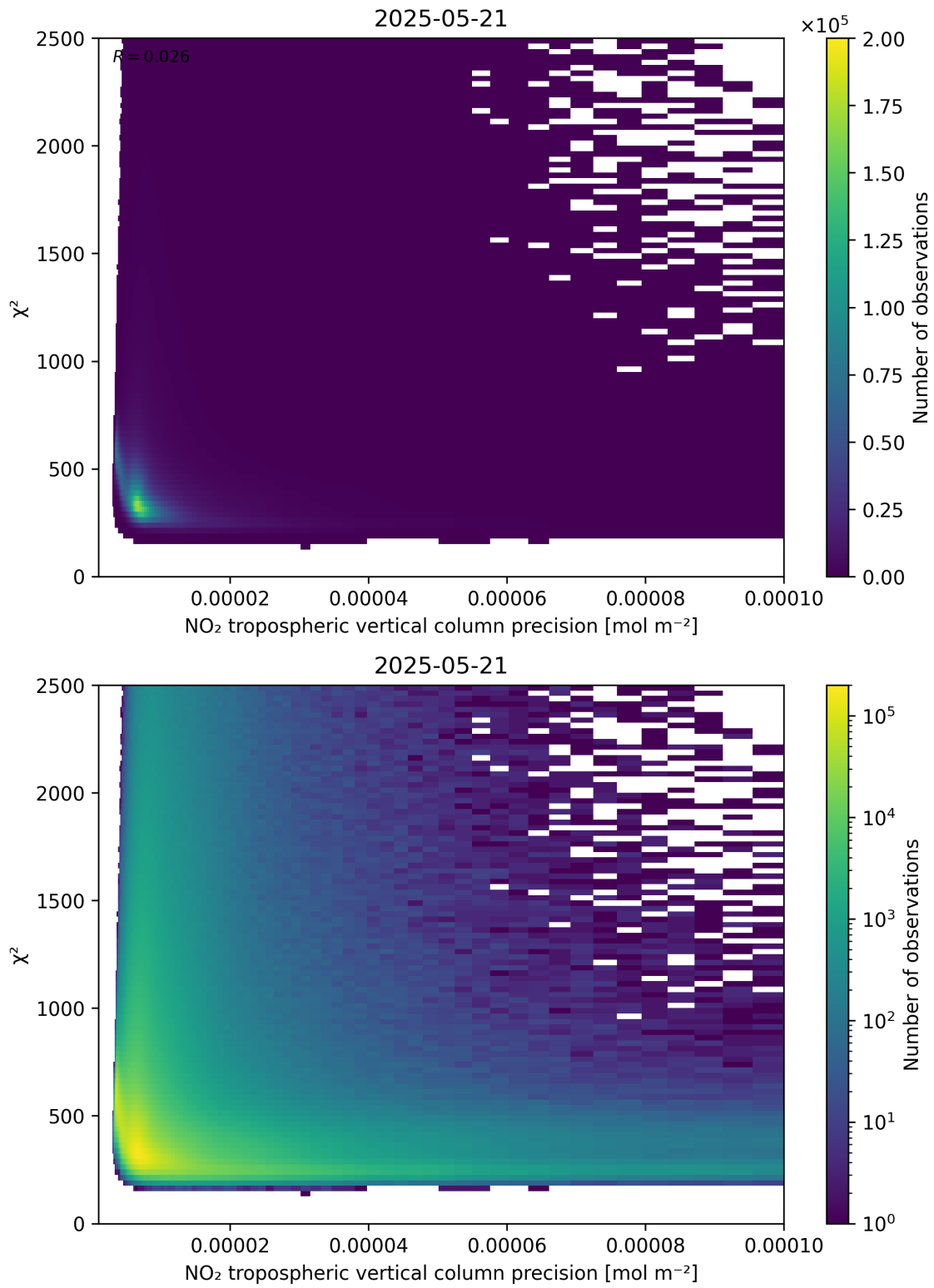
Figure 134: Scatter density plot of “NO 2 tropospheric vertical column precision” against “ \chi^2 ” for 2025-05-21 to 2025-05-22.
