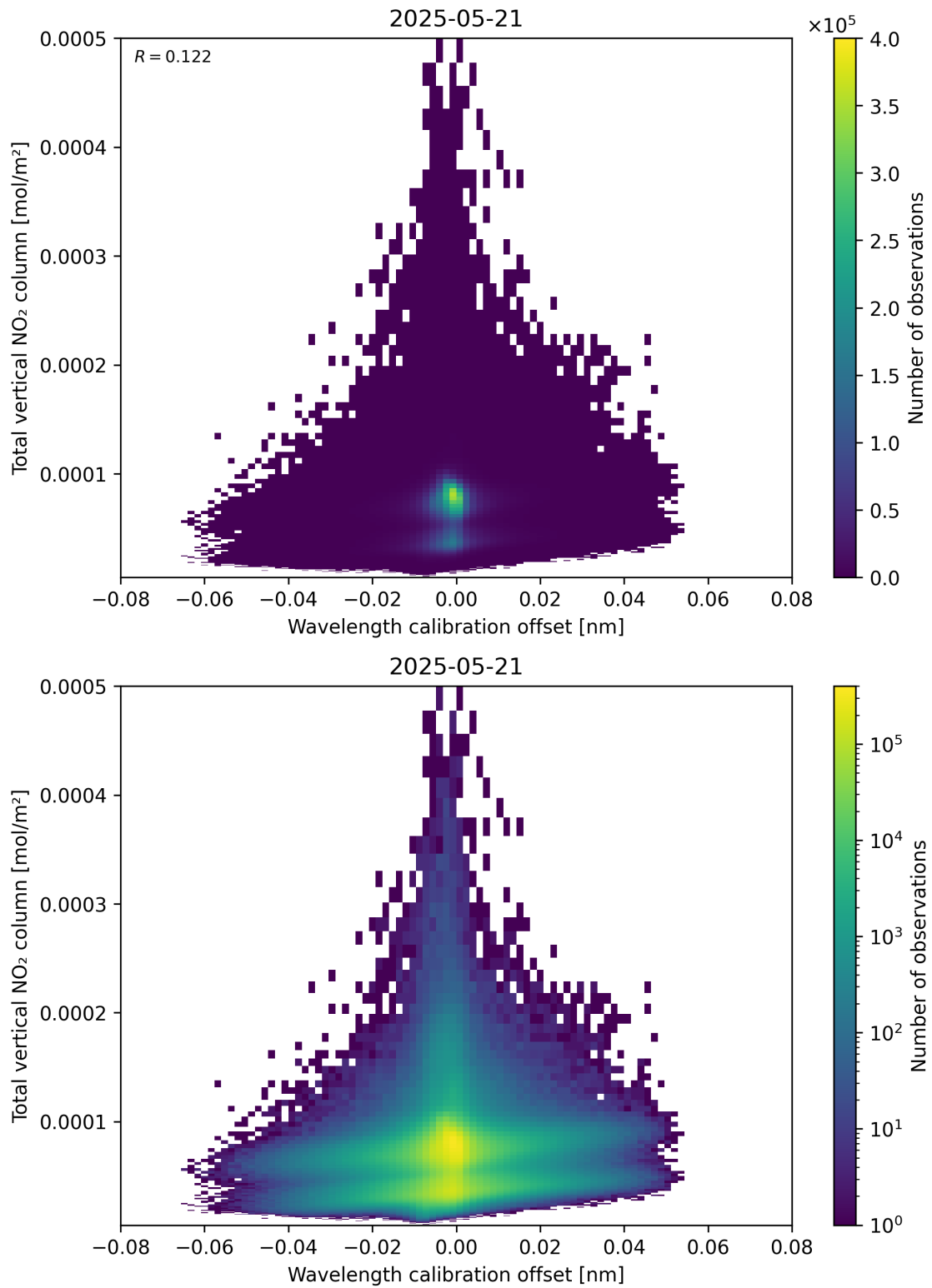
Figure 179: Scatter density plot of “Wavelength calibration offset” against “Total vertical NO 2 column” for 2025-05-21 to 2025-05-22.
