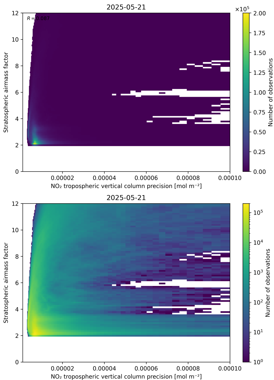
Figure 131: Scatter density plot of “NO 2 tropospheric vertical column precision” against “Stratospheric airmass factor” for 2025-05-21 to 2025-05-22.
