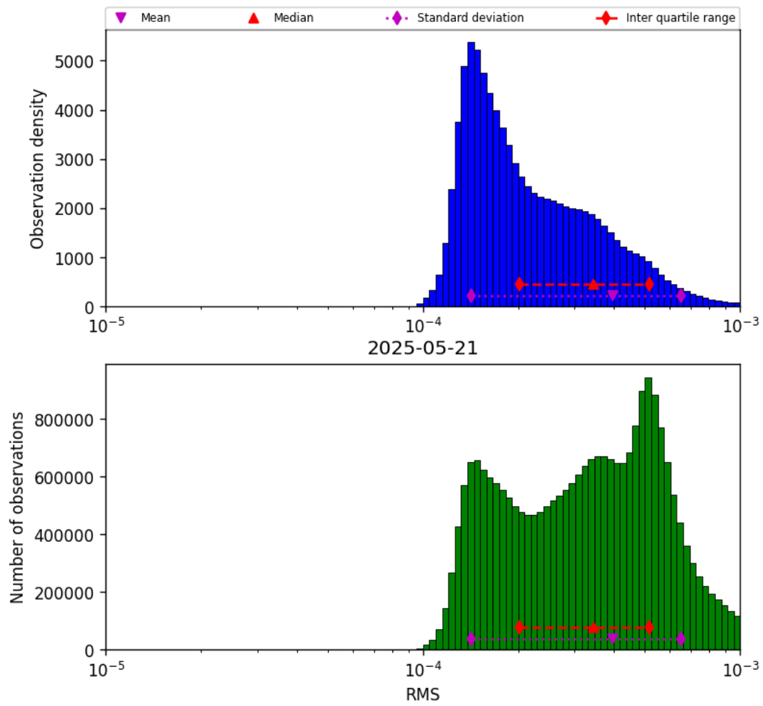
Figure 43: Histogram of “RMS” for 2025-05-21 to 2025-05-22
