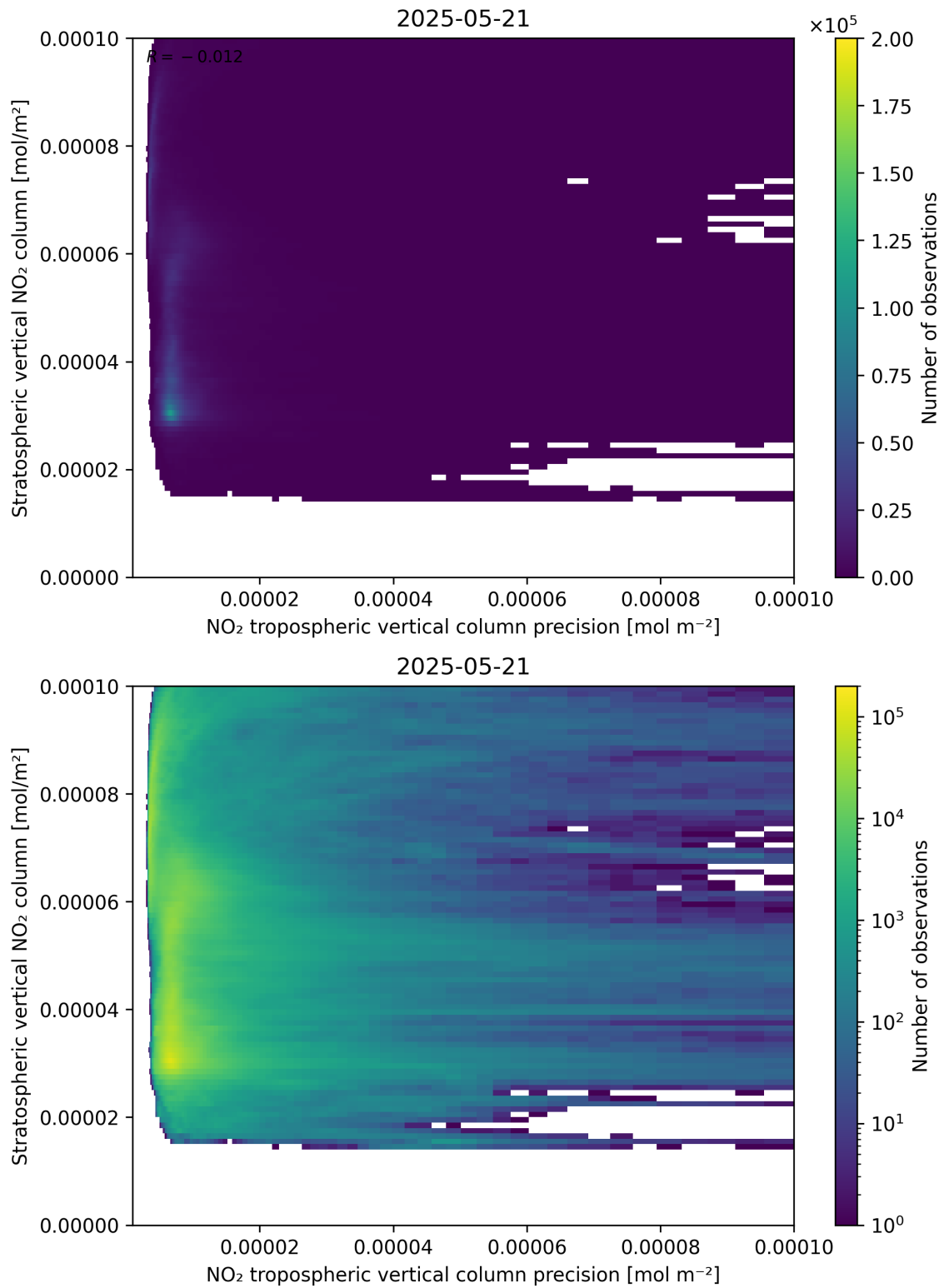
Figure 135: Scatter density plot of “NO 2 tropospheric vertical column precision” against “Stratospheric vertical NO 2 column” for 2025-05-21 to 2025-05-22.
