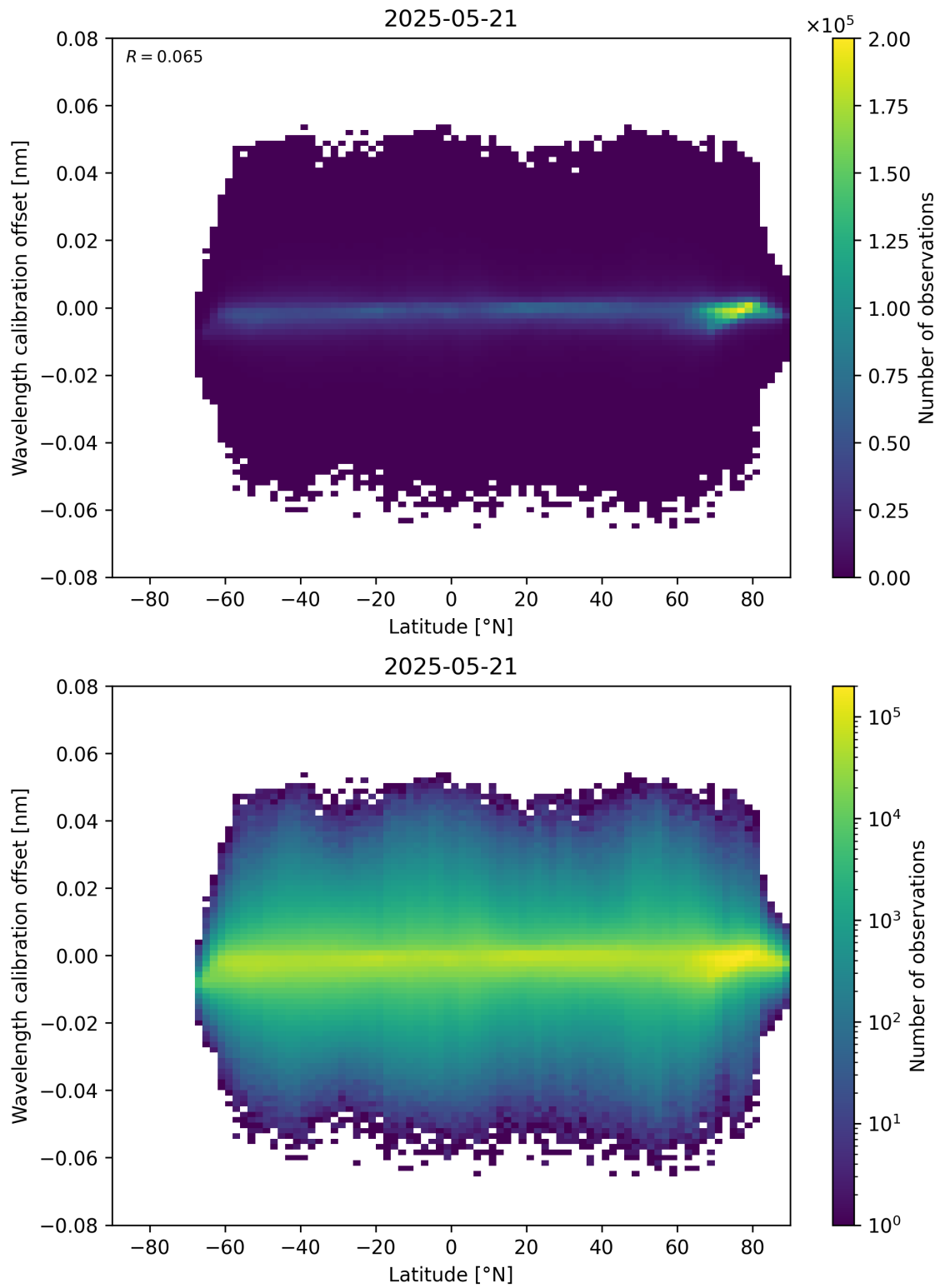
Figure 95: Scatter density plot of “Latitude” against “Wavelength calibration offset” for 2025-05-21 to 2025-05-22.
