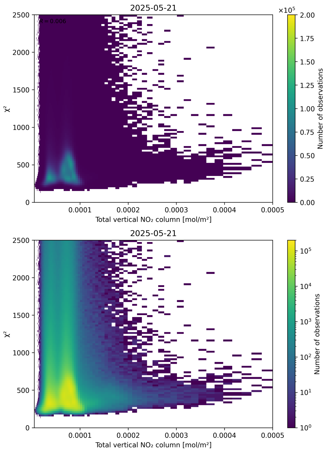
Figure 111: Scatter density plot of “Total vertical NO 2 column” against “ \chi^2 ” for 2025-05-21 to 2025-05-22.
