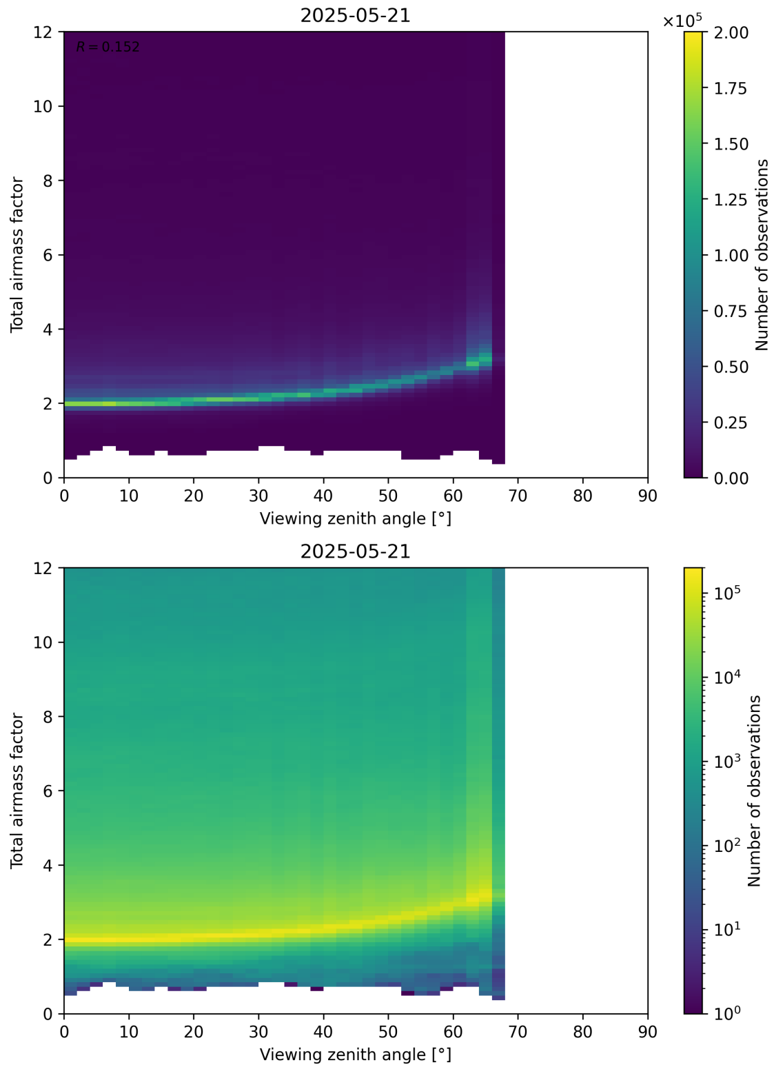
Figure 160: Scatter density plot of “Viewing zenith angle” against “Total airmass factor” for 2025-05-21 to 2025-05-22.
