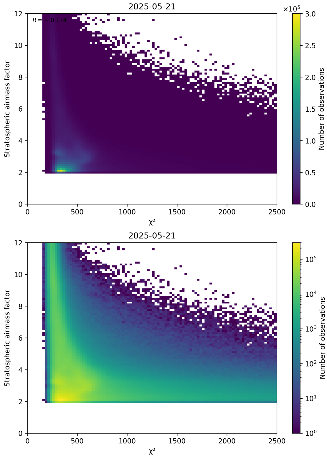
Figure 81: Scatter density plot of “ \chi^2 ” against “Stratospheric airmass factor” for 2025-05-21 to 2025-05-22.
