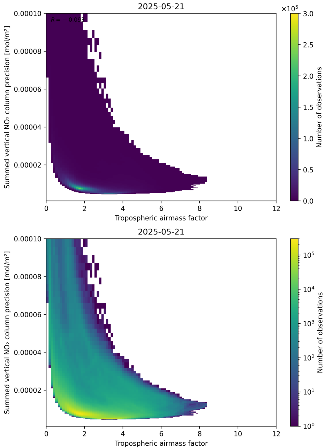
Figure 76: Scatter density plot of “Tropospheric air mass factor” against “Summed vertical NO 2 column precision” for 2025-05-21 to 2025-05-22.
