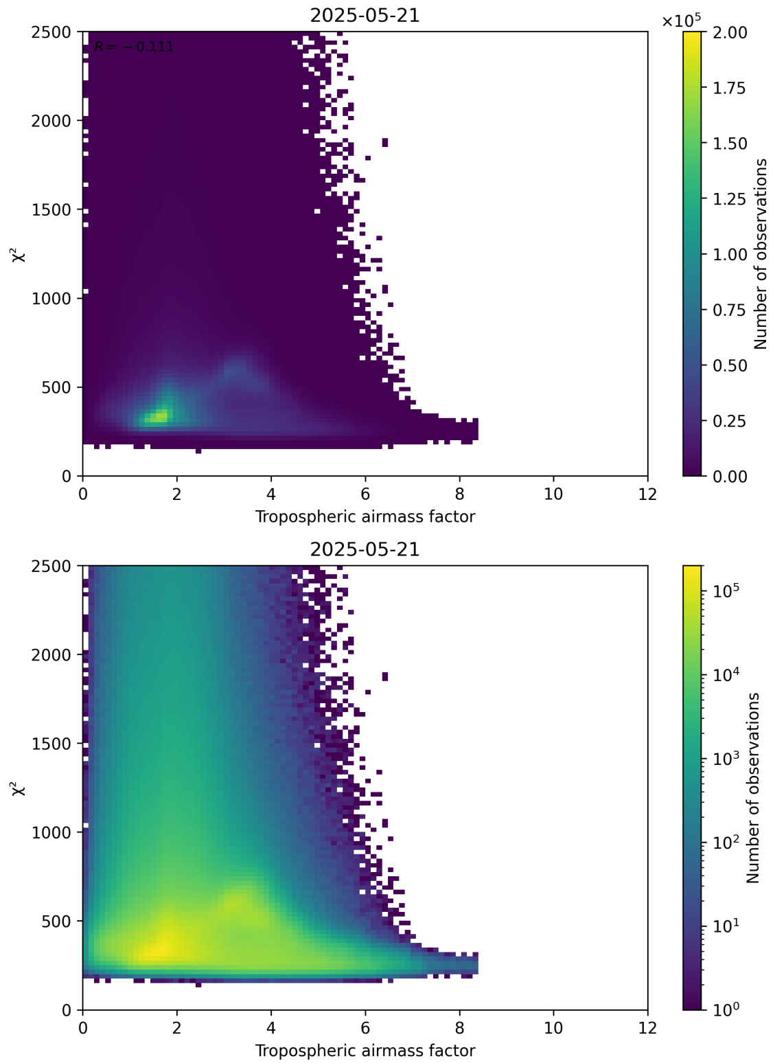
Figure 73: Scatter density plot of “Tropospheric airmass factor” against “ \chi^2 ” for 2025-05-21 to 2025-05-22.
