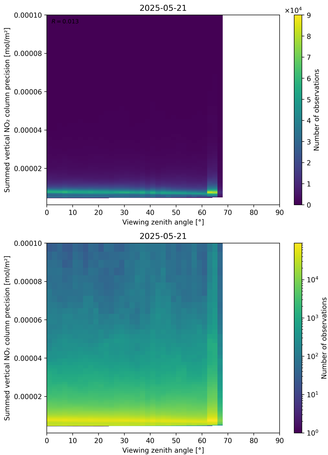
Figure 166: Scatter density plot of “Viewing zenith angle” against “Summed vertical NO 2 column precision” for 2025-05-21 to 2025-05-22.
