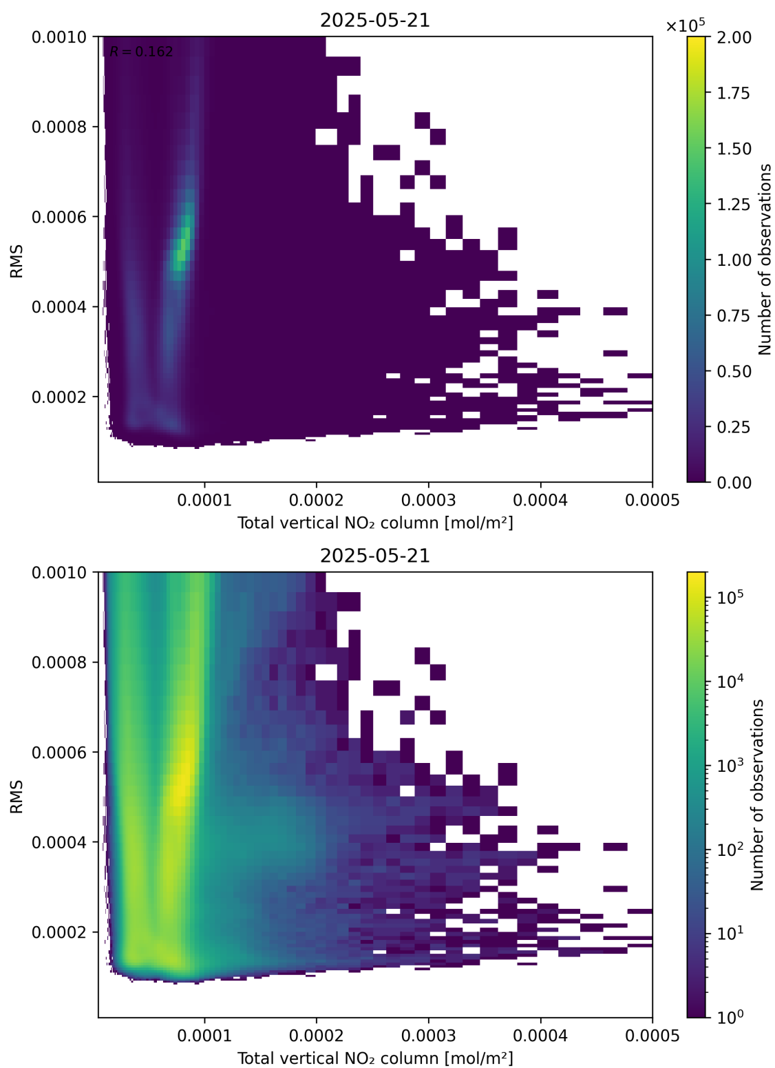
Figure 120: Scatter density plot of “Total vertical NO 2 column” against “RMS” for 2025-05-21 to 2025-05-22.
