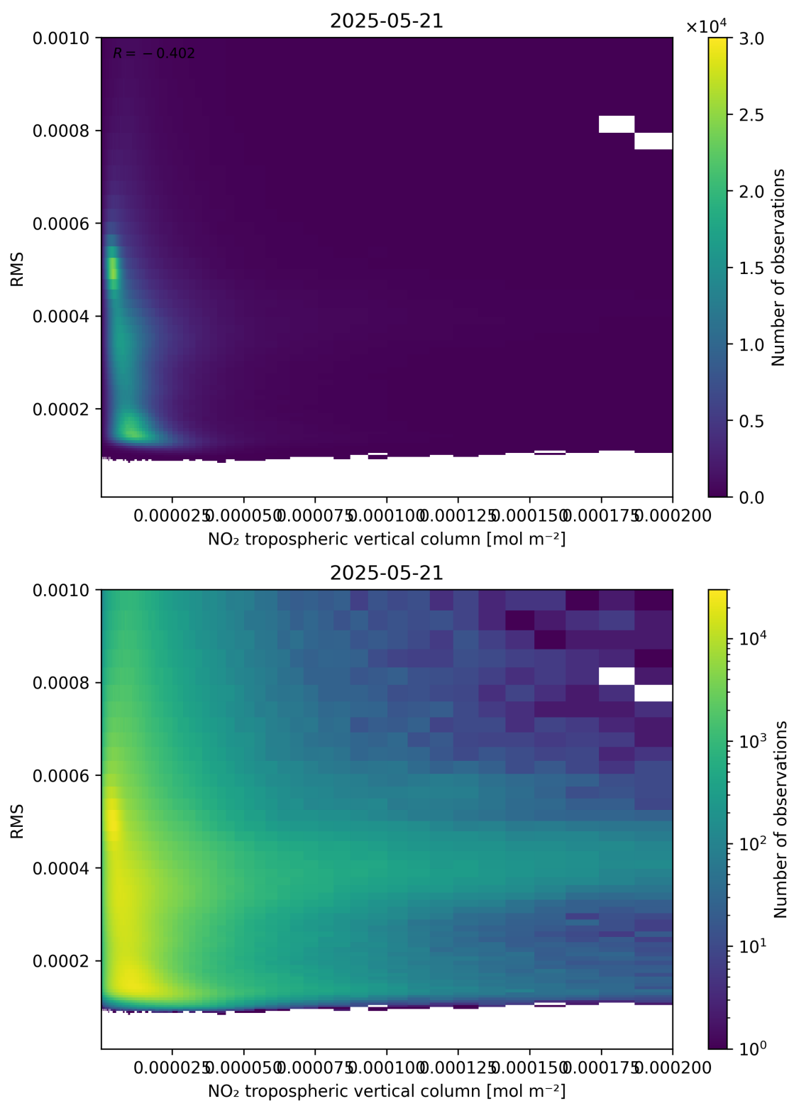
Figure 142: Scatter density plot of “NO 2 tropospheric vertical column” against “RMS” for 2025-05-21 to 2025-05-22.
