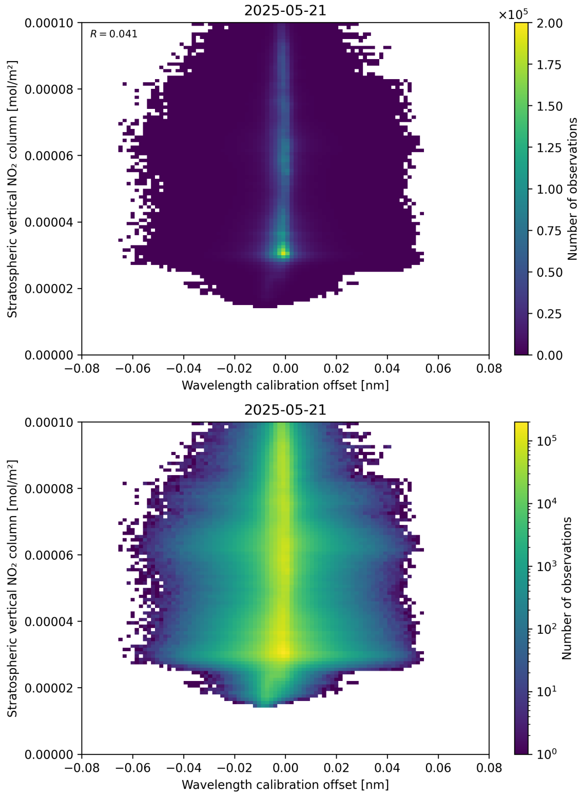
Figure 176: Scatter density plot of “Wavelength calibration offset” against “Stratospheric vertical NO 2 column” for 2025-05-21 to 2025-05-22.
