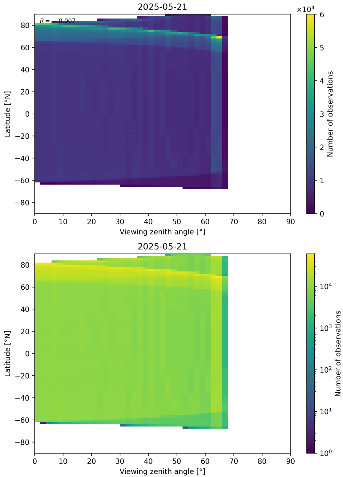
Figure 163: Scatter density plot of “Viewing zenith angle” against “Latitude” for 2025-05-21 to 2025-05-22.
