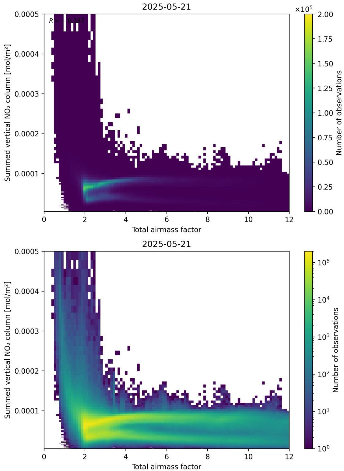
Figure 65: Scatter density plot of “Total airmass factor” against “Summed vertical NO 2 column” for 2025-05-21 to 2025-05-22.
