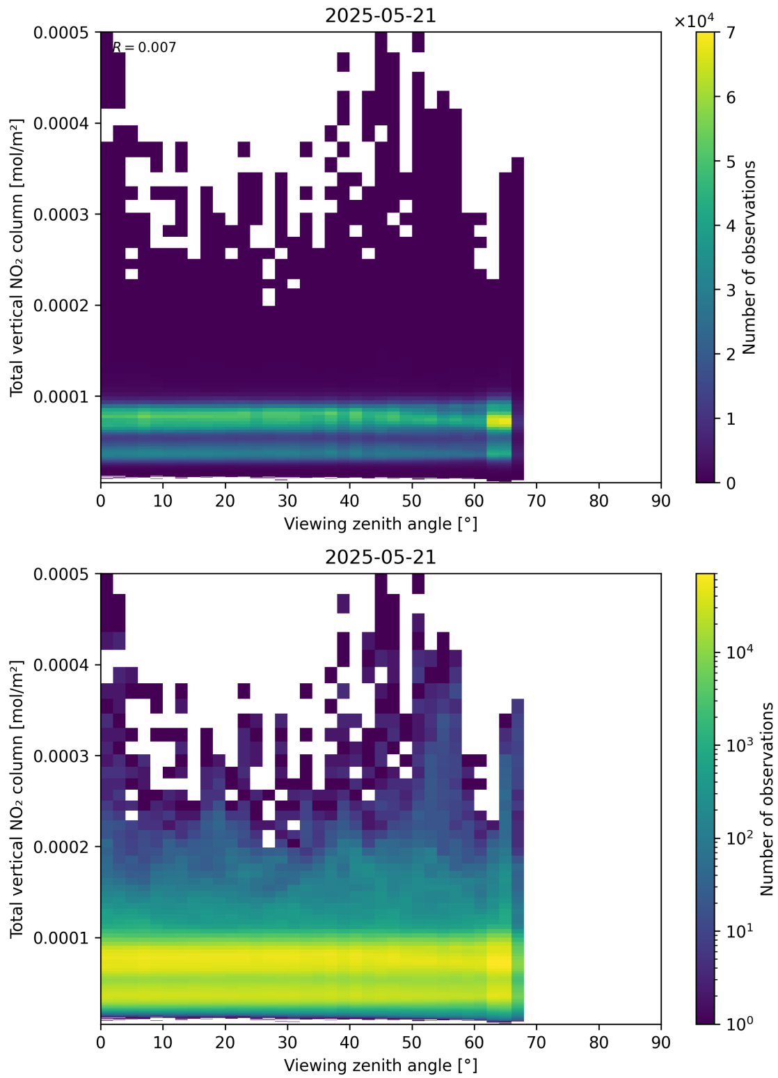
Figure 167: Scatter density plot of “Viewing zenith angle” against “Total vertical NO 2 column” for 2025-05-21 to 2025-05-22.
