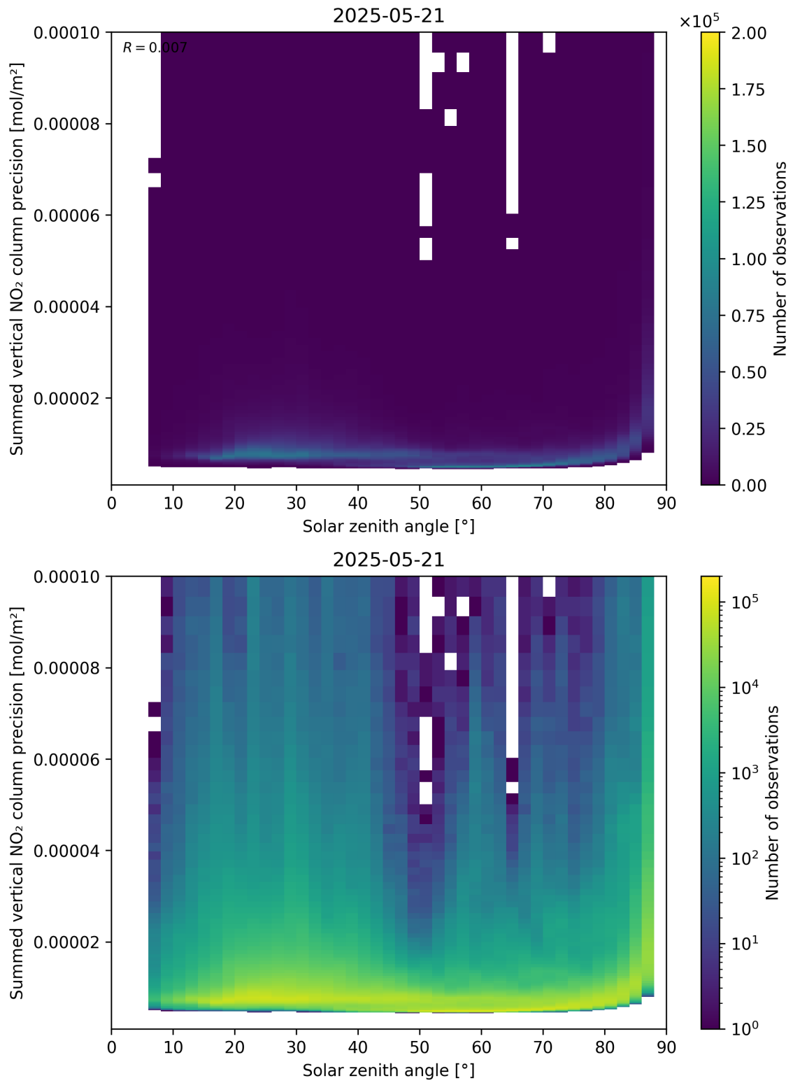
Figure 152: Scatter density plot of “Solar zenith angle” against “Summed vertical NO 2 column precision” for 2025-05-21 to 2025-05-22.
