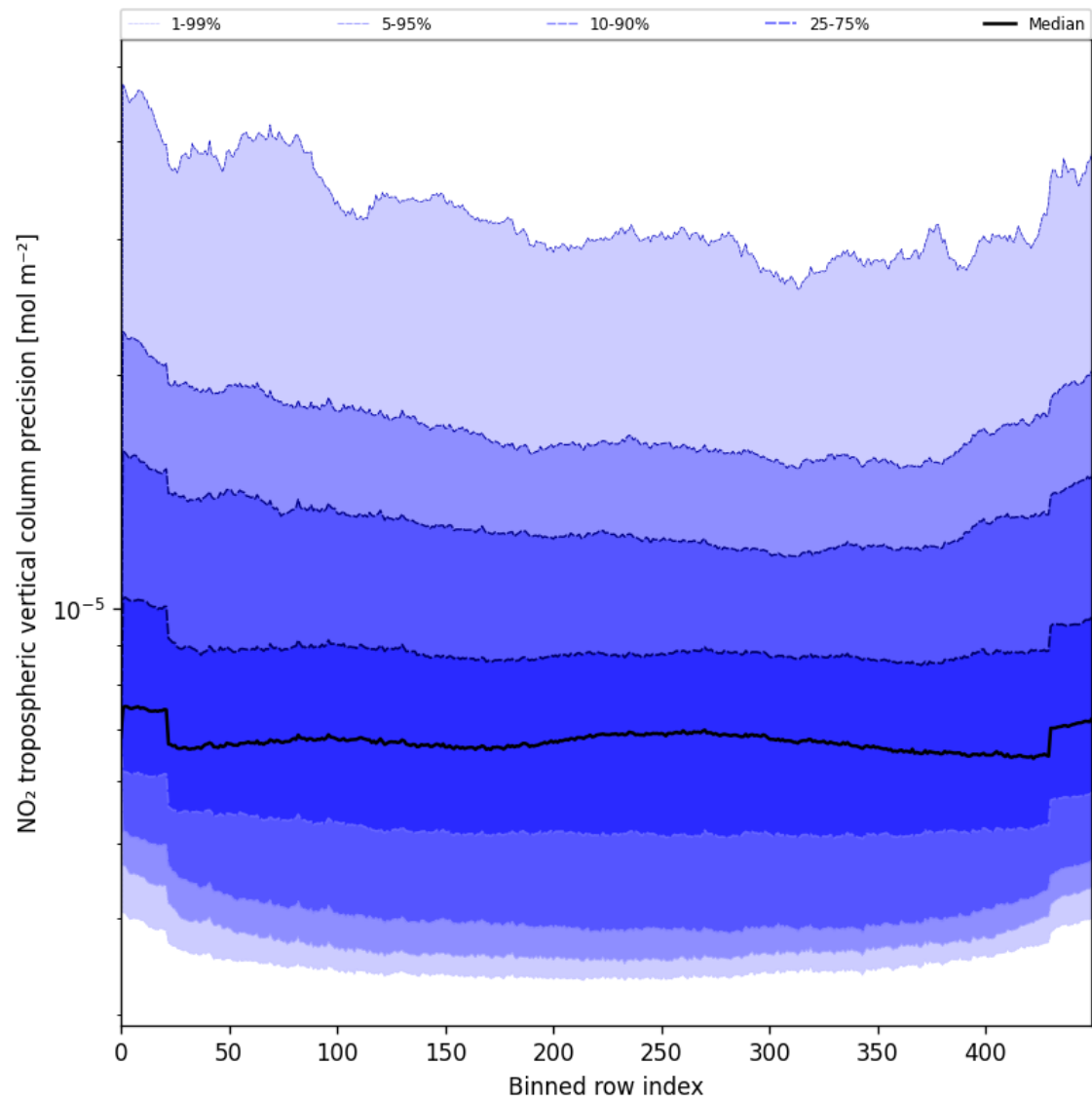
Figure 47: Along track statistics of “NO 2 tropospheric vertical column precision” for 2025-05-21 to 2025-05-22
