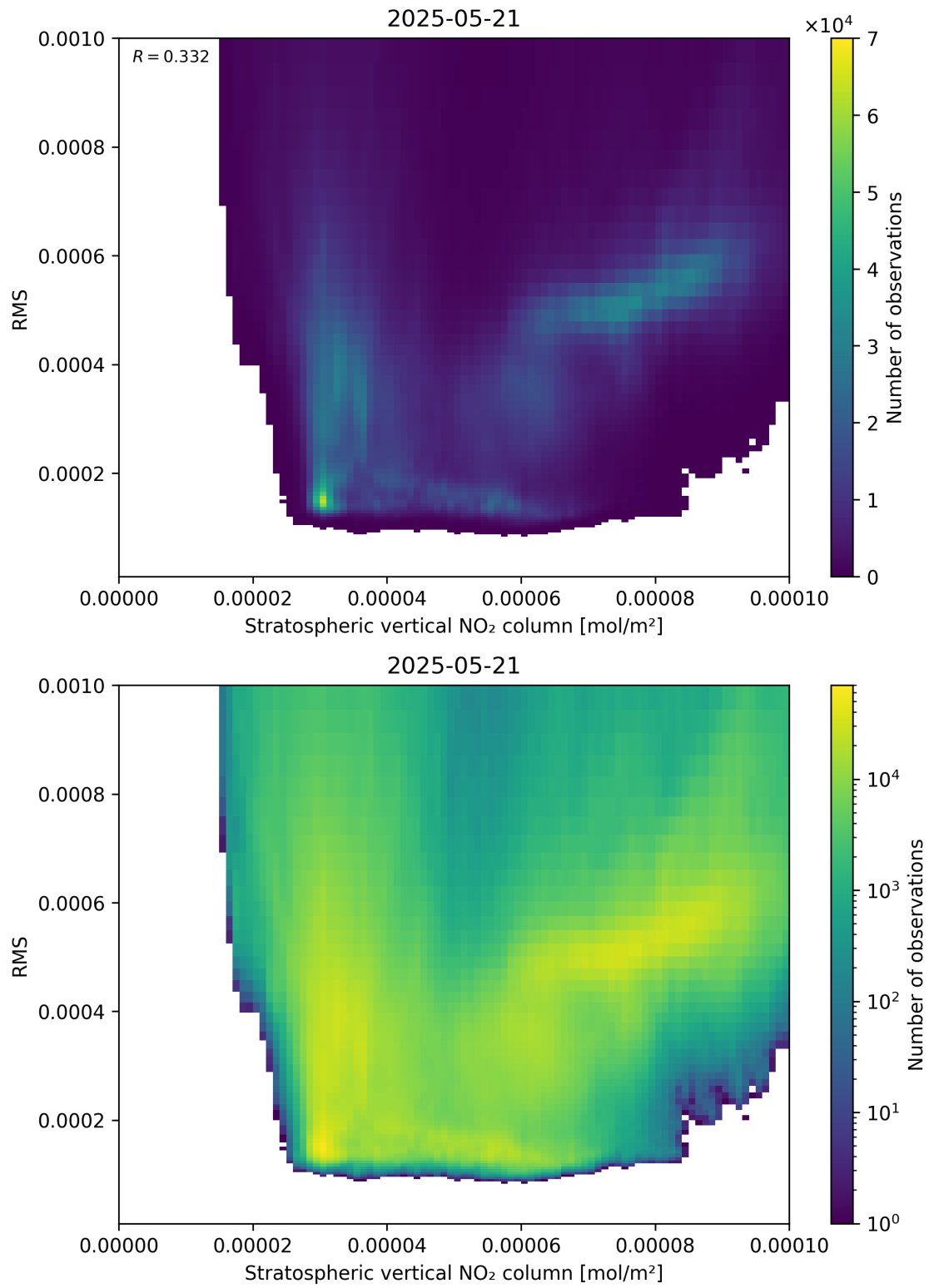
Figure 102: Scatter density plot of “Stratospheric vertical NO 2 column” against “RMS” for 2025-05-21 to 2025-05-22.
