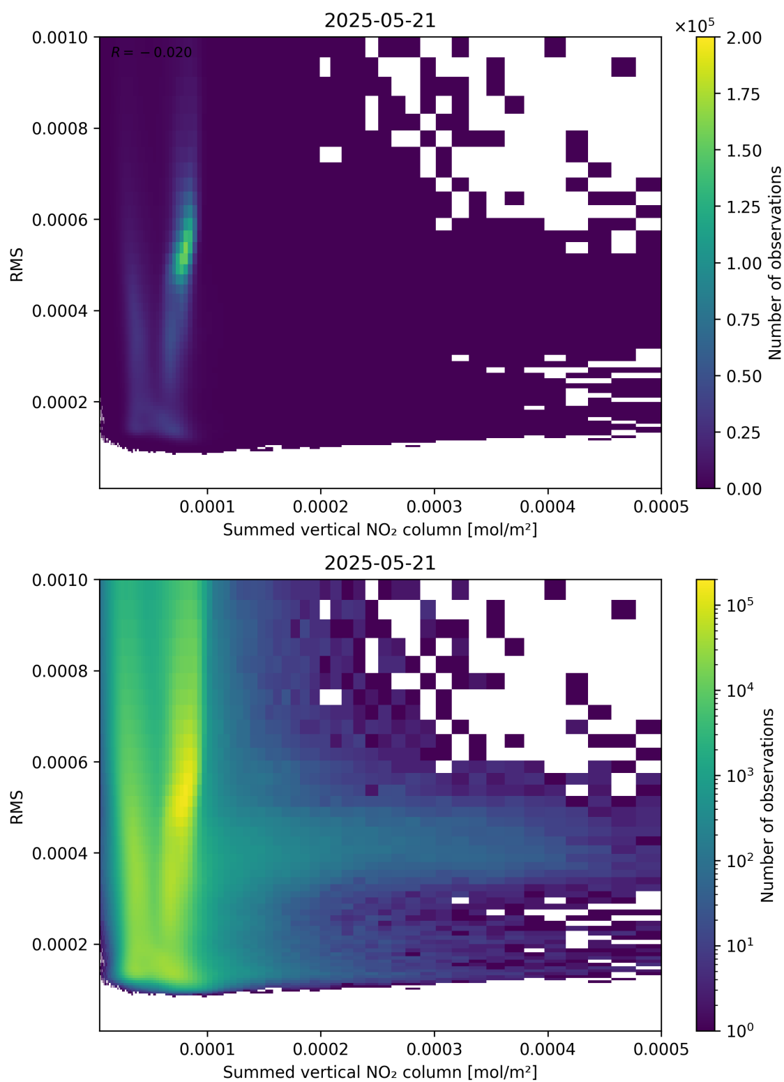
Figure 109: Scatter density plot of “Summed vertical NO 2 column” against “RMS” for 2025-05-21 to 2025-05-22.
