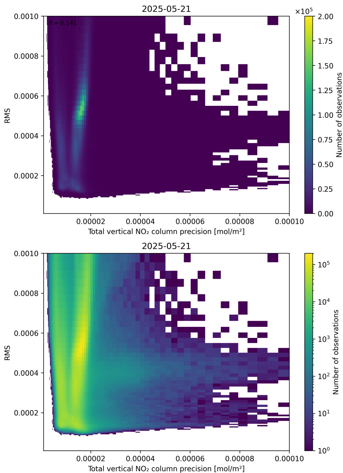
Figure 119: Scatter density plot of “Total vertical NO 2 column precision” against “RMS” for 2025-05-21 to 2025-05-22.
