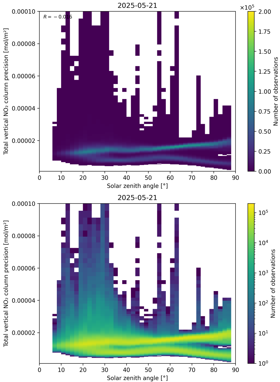
Figure 154: Scatter density plot of “Solar zenith angle” against “Total vertical NO 2 column precision” for 2025-05-21 to 2025-05-22.
