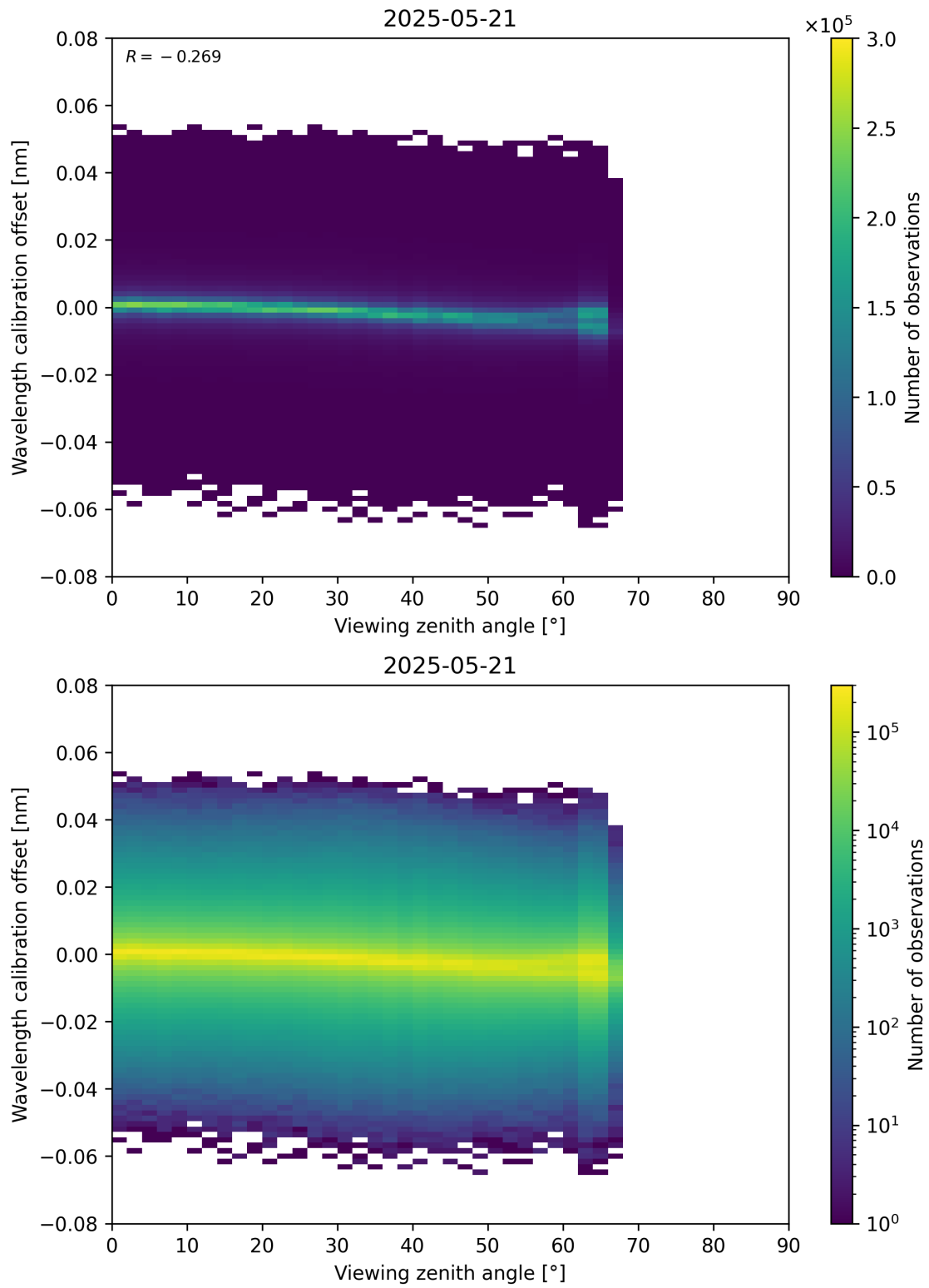
Figure 173: Scatter density plot of “Viewing zenith angle” against “Wavelength calibration offset” for 2025-05-21 to 2025-05-22.
