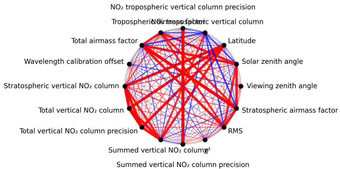
Figure 1: Map of correlation graph for 2025-05-21 to 2025-05-22.
