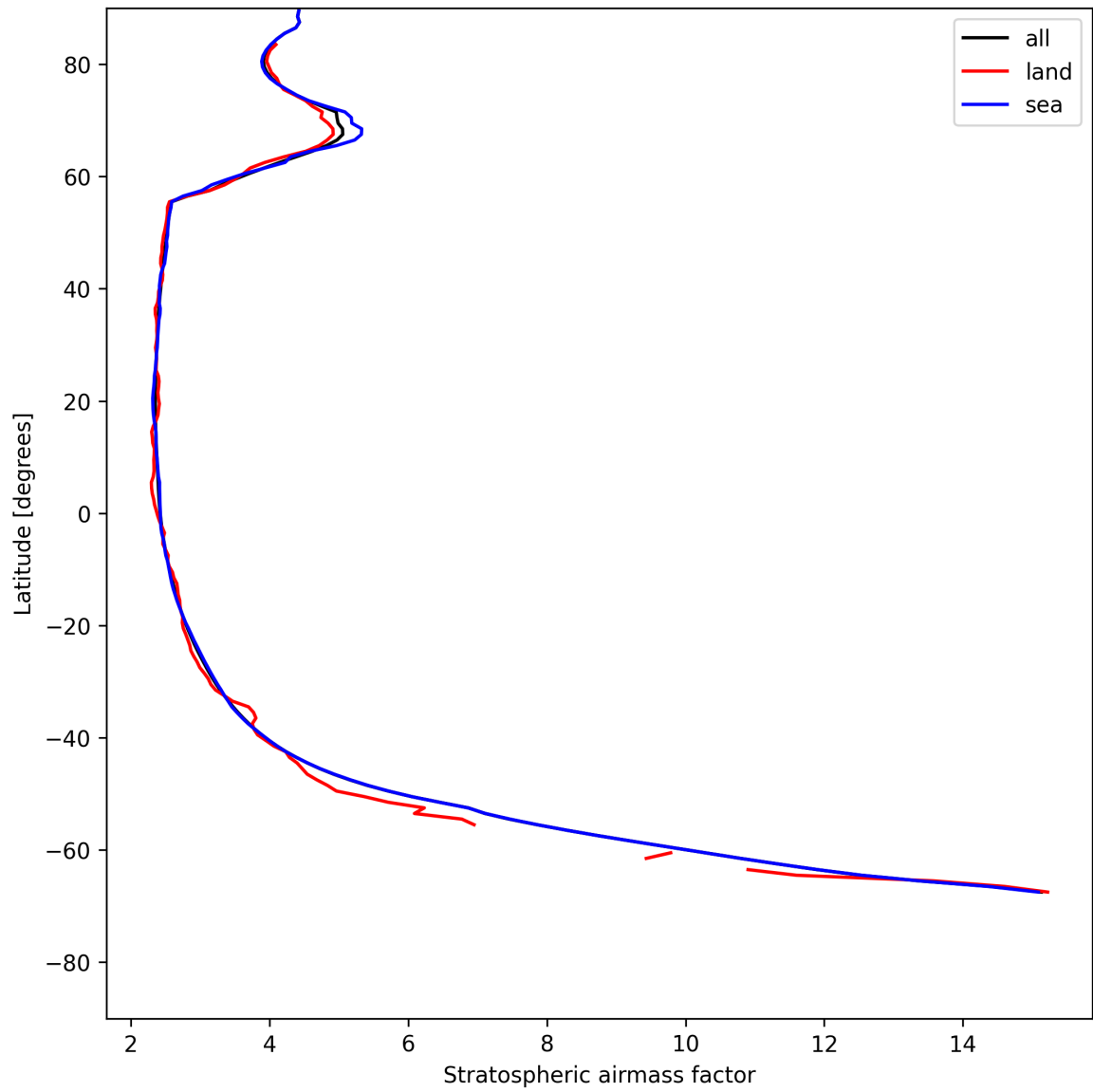
Figure 27: Zonal average of “Stratospheric air mass factor” for 2025-05-21 to 2025-05-22.
