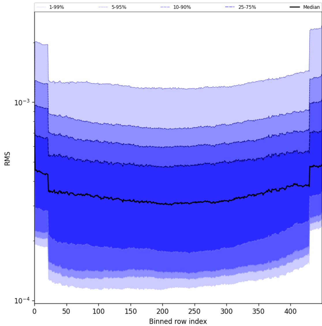
Figure 60: Along track statistics of “RMS” for 2025-05-21 to 2025-05-22
