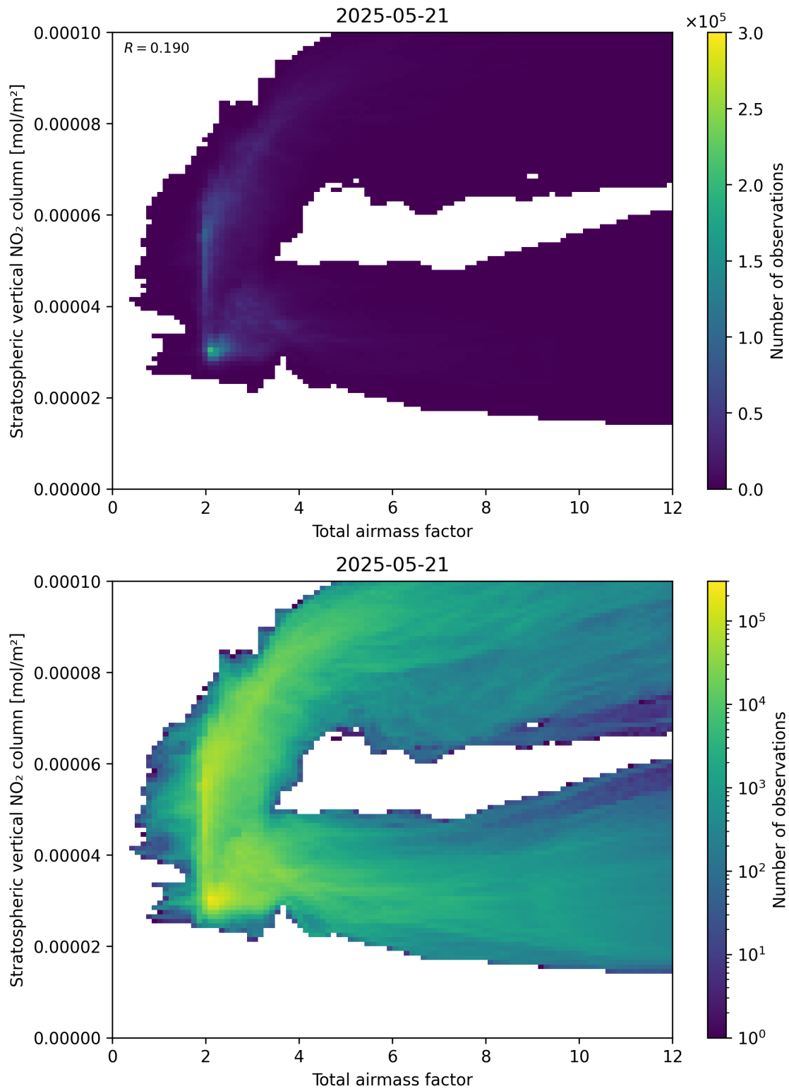
Figure 64: Scatter density plot of “Total airmass factor” against “Stratospheric vertical \text{NO}_2 column” for 2025-05-21 to 2025-05-22.
