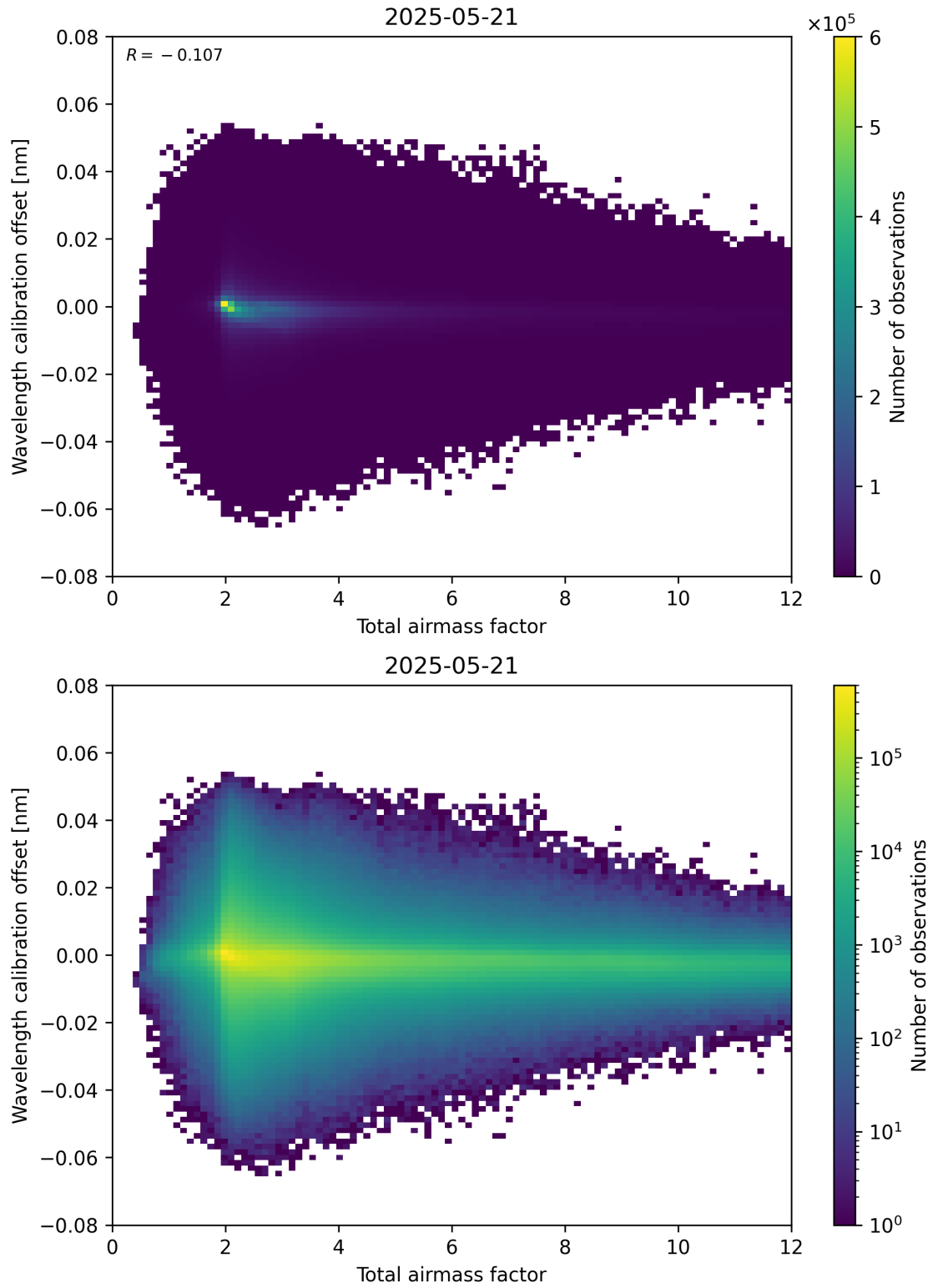
Figure 70: Scatter density plot of “Total airmass factor” against “Wavelength calibration offset” for 2025-05-21 to 2025-05-22.
