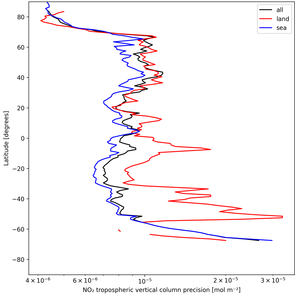
Figure 13: Zonal average of “NO 2 tropospheric vertical column precision” for 2025-05-21 to 2025-05-22.
