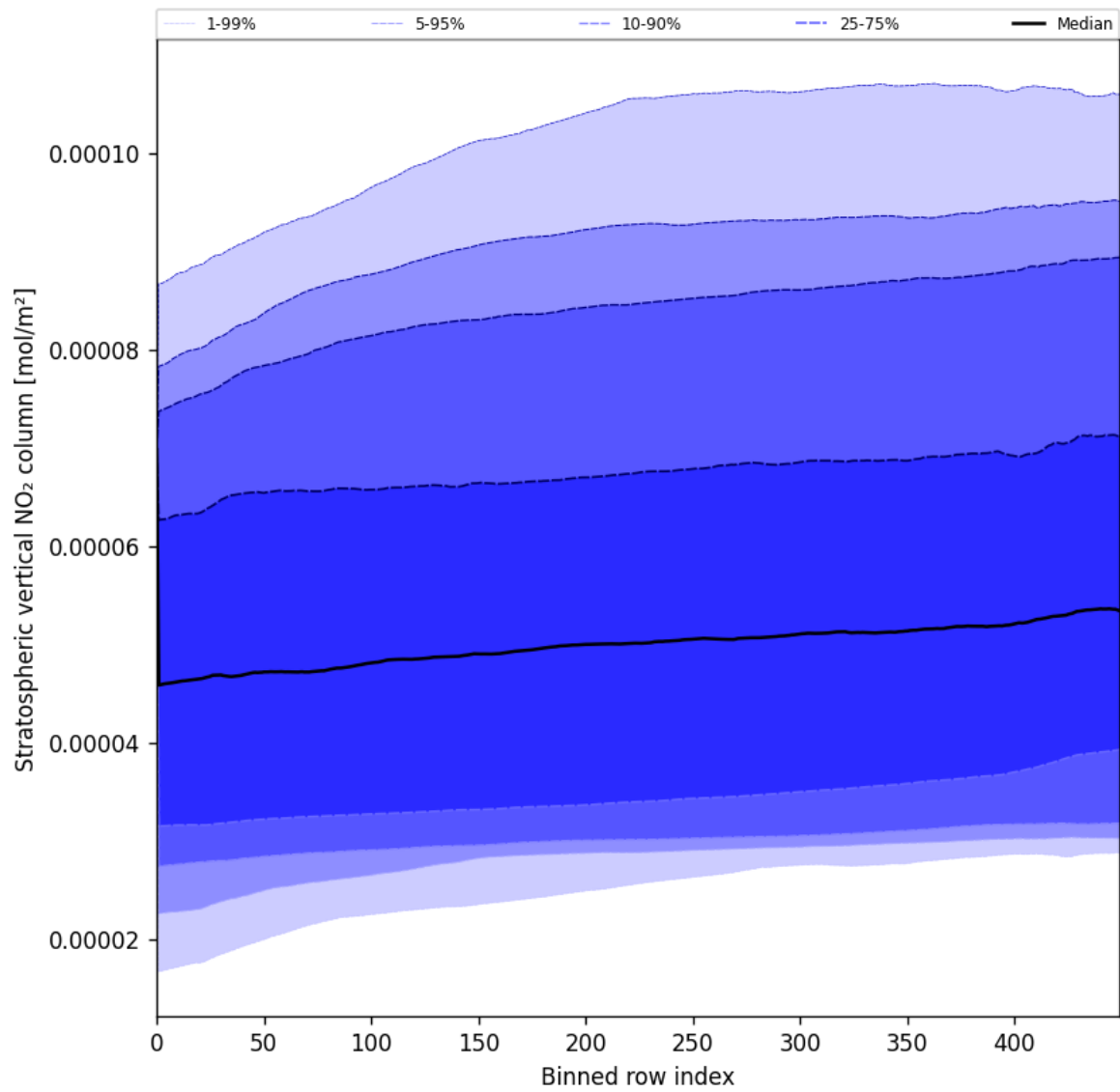
Figure 53: Along track statistics of “Stratospheric vertical NO 2 column” for 2025-05-21 to 2025-05-22
