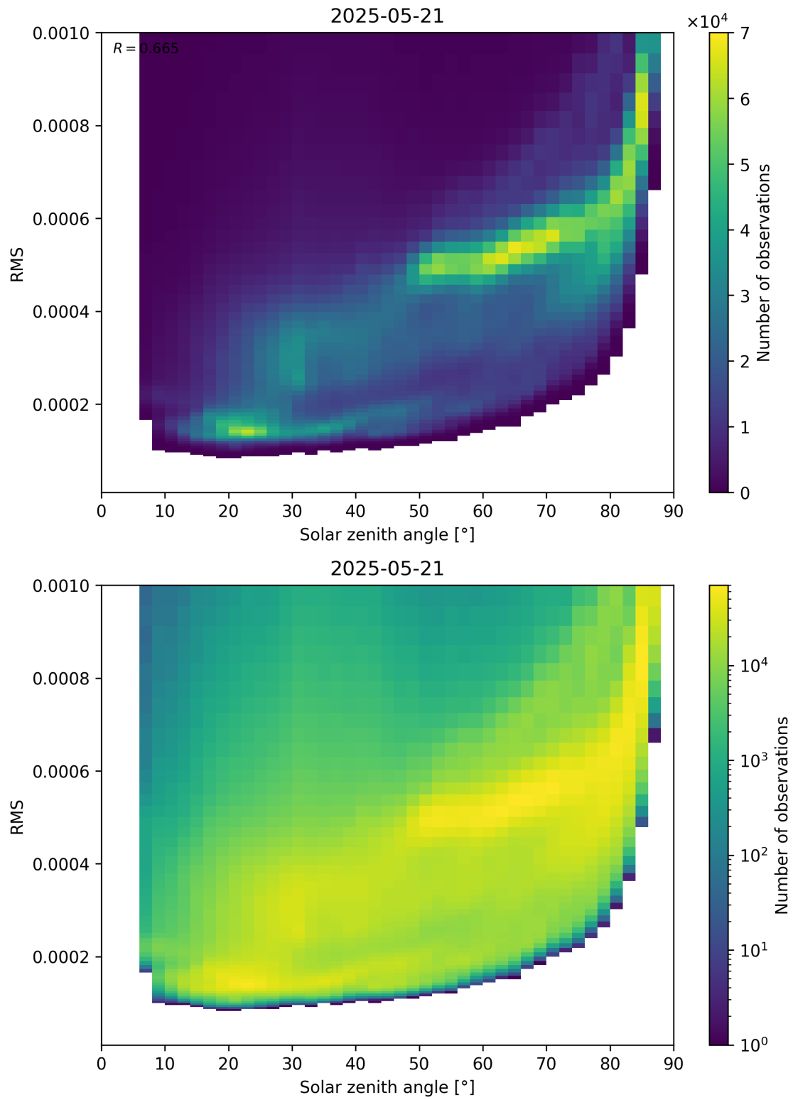
Figure 157: Scatter density plot of “Solar zenith angle” against “RMS” for 2025-05-21 to 2025-05-22.
