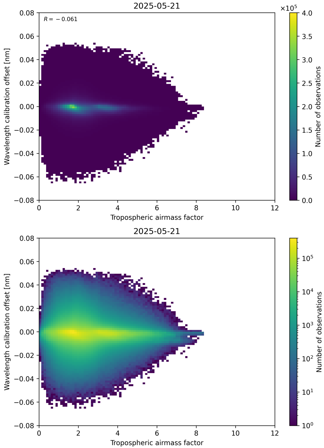
Figure 80: Scatter density plot of “Tropospheric airmass factor” against “Wavelength calibration offset” for 2025-05-21 to 2025-05-22.
