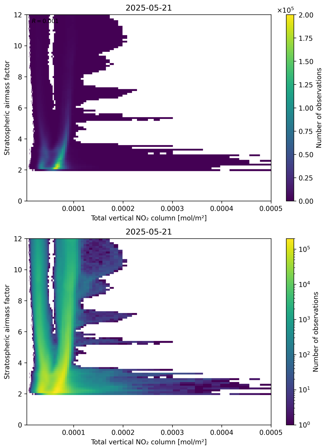
Figure 110: Scatter density plot of “Total vertical NO 2 column” against “Stratospheric airmass factor” for 2025-05-21 to 2025-05-22.
