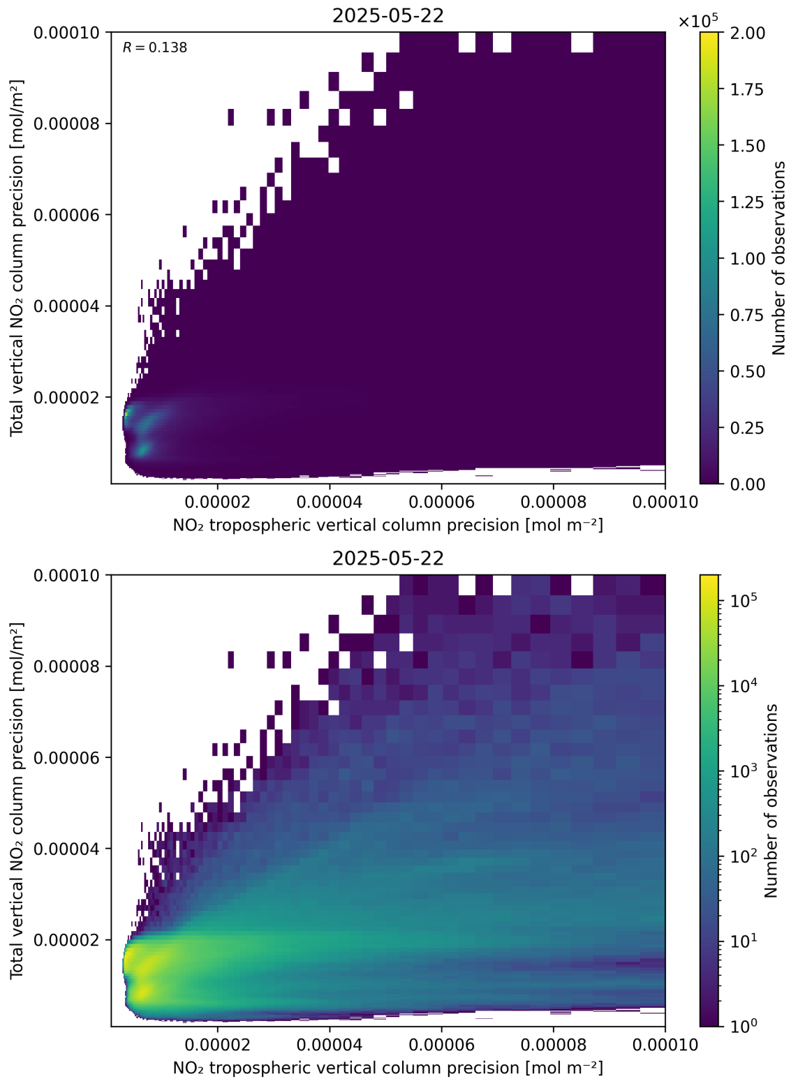
Figure 139: Scatter density plot of “NO 2 tropospheric vertical column precision” against “Total vertical NO 2 column precision” for 2025-05-21 to 2025-05-23.
