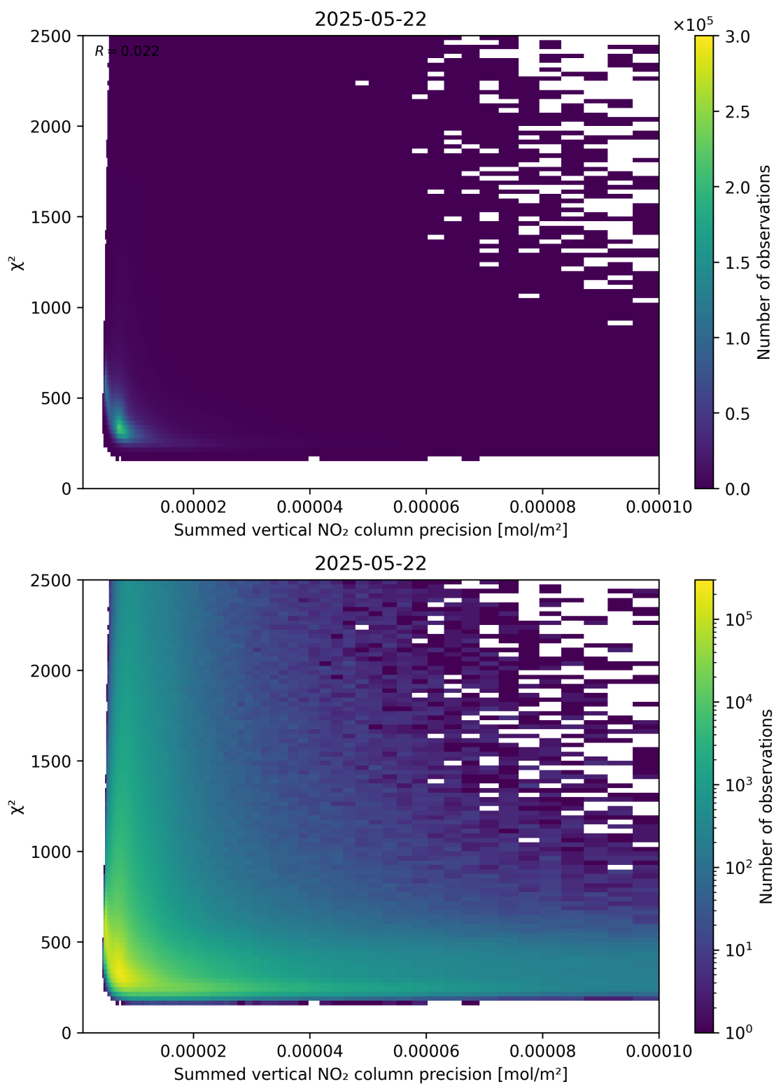
Figure 107: Scatter density plot of “Summed vertical NO 2 column precision” against “ \chi^2 ” for 2025-05-21 to 2025-05-23.
