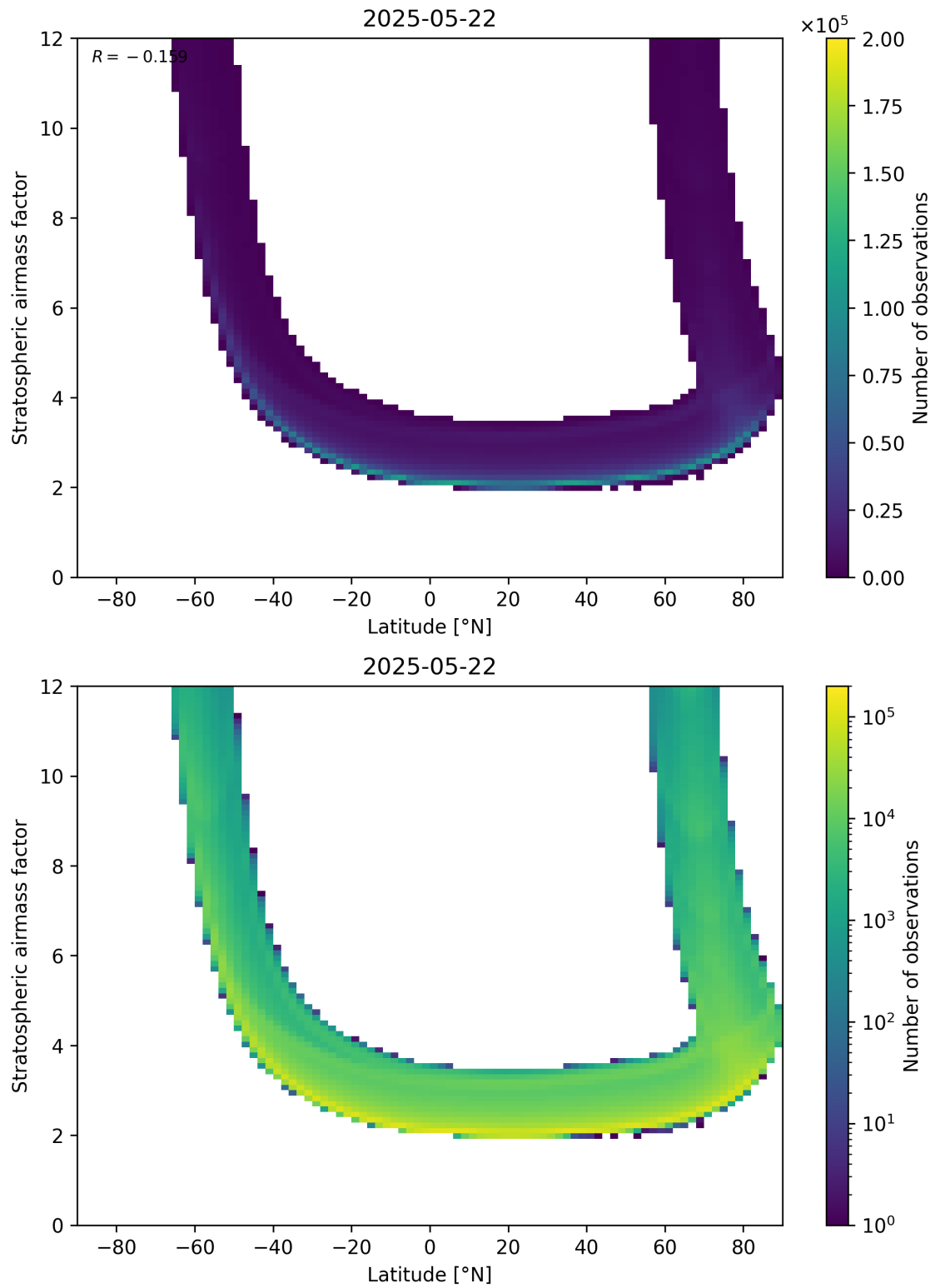
Figure 83: Scatter density plot of “Latitude” against “Stratospheric air mass factor” for 2025-05-21 to 2025-05-23.
