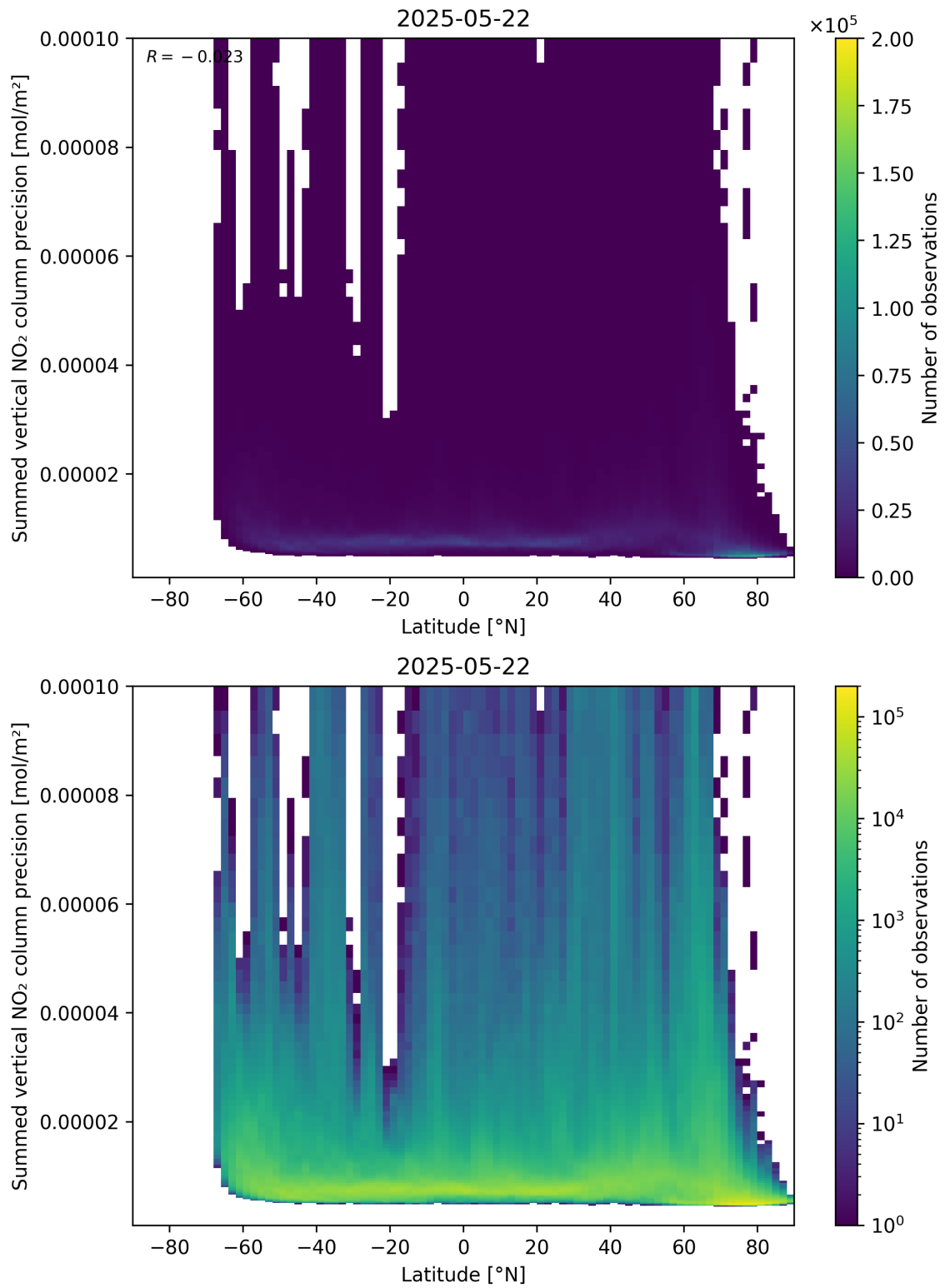
Figure 89: Scatter density plot of “Latitude” against “Summed vertical NO 2 column precision” for 2025-05-21 to 2025-05-23.
