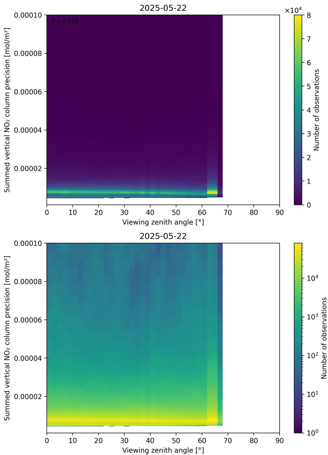
Figure 166: Scatter density plot of “Viewing zenith angle” against “Summed vertical NO 2 column precision” for 2025-05-21 to 2025-05-23.
