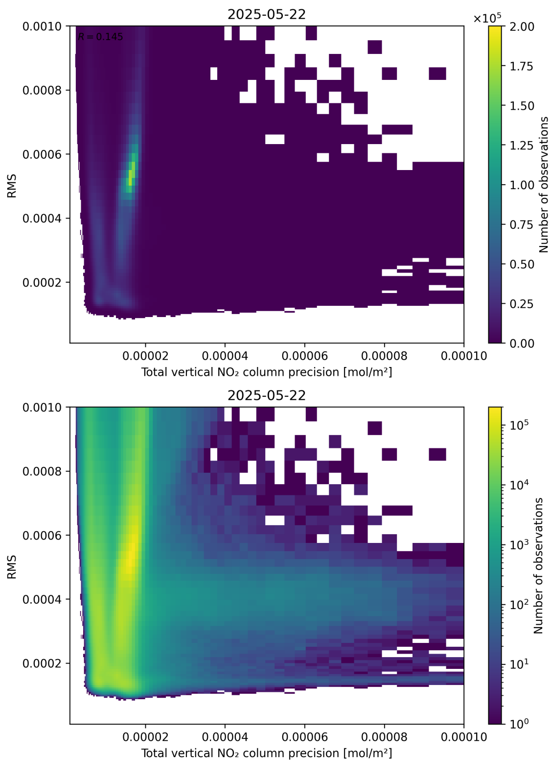
Figure 119: Scatter density plot of “Total vertical NO 2 column precision” against “RMS” for 2025-05-21 to 2025-05-23.
