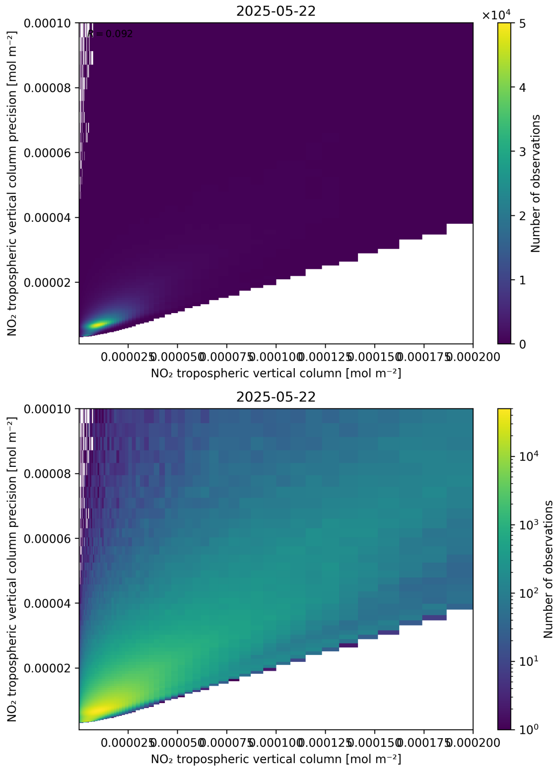
Figure 130: Scatter density plot of “NO 2 tropospheric vertical column” against “NO 2 tropospheric vertical column precision” for 2025-05-21 to 2025-05-23.
