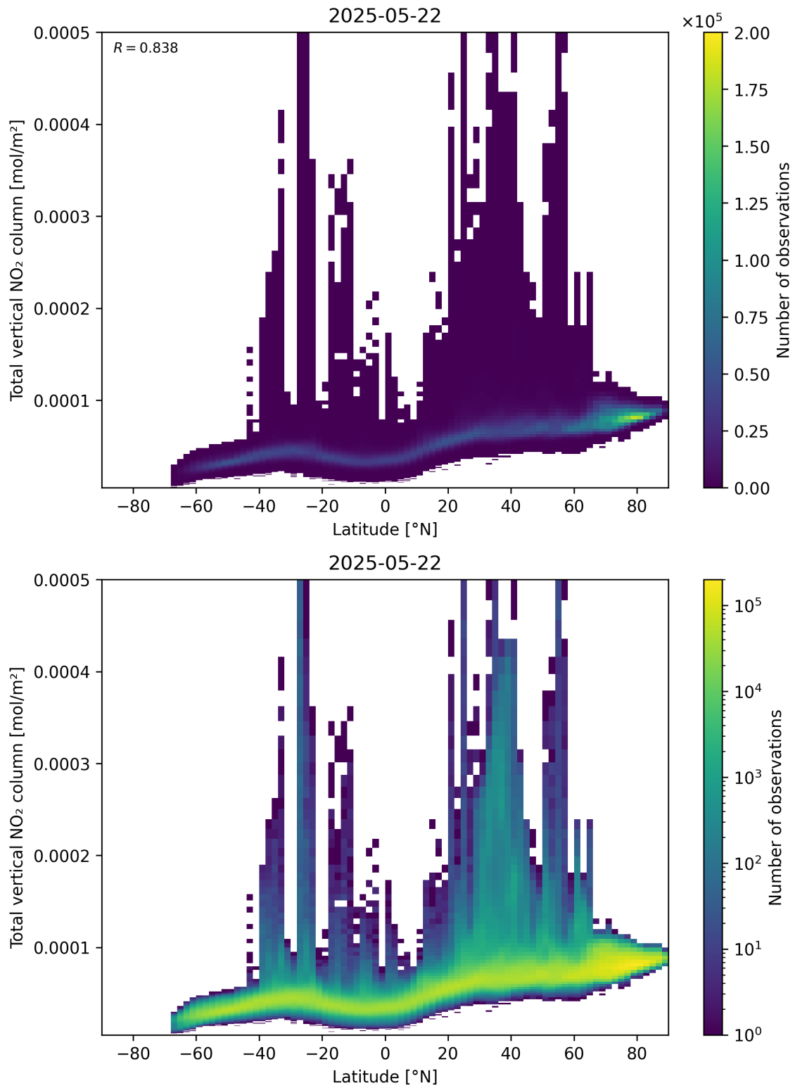
Figure 90: Scatter density plot of “Latitude” against “Total vertical NO 2 column” for 2025-05-21 to 2025-05-23.
