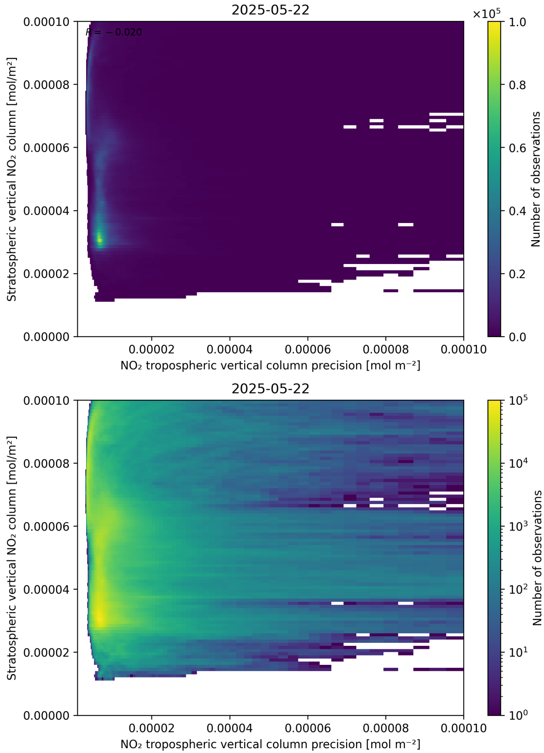
Figure 135: Scatter density plot of “NO 2 tropospheric vertical column precision” against “Stratospheric vertical NO 2 column” for 2025-05-21 to 2025-05-23.
