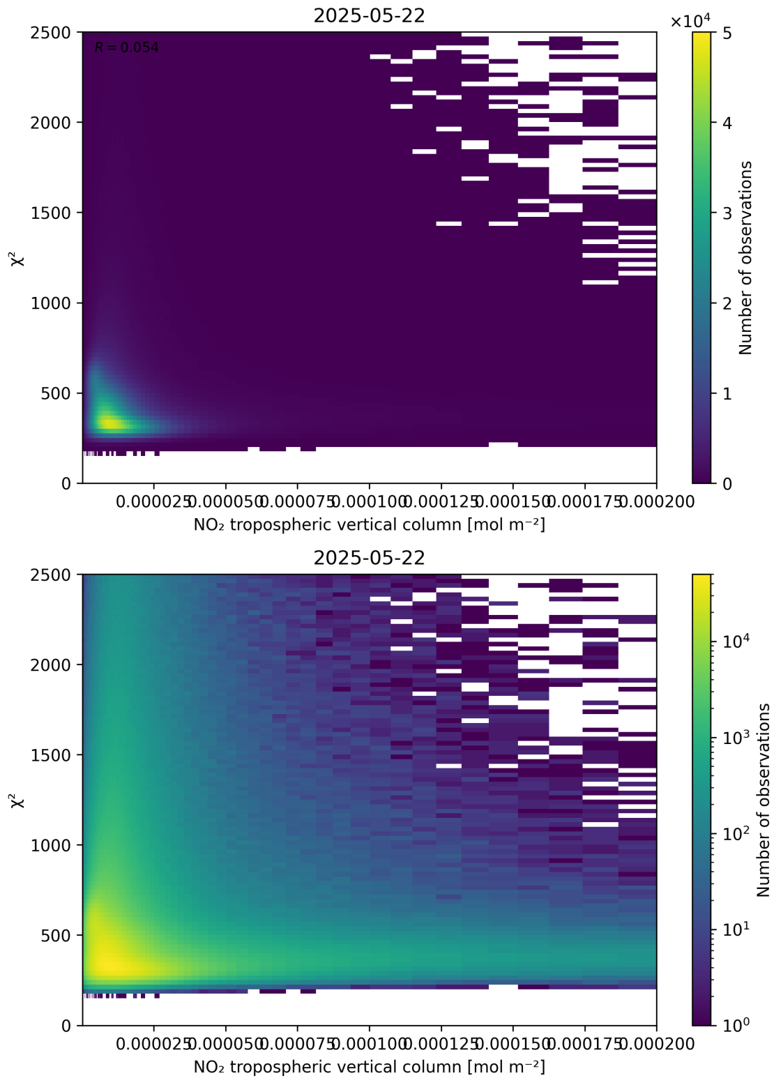
Figure 124: Scatter density plot of “NO 2 tropospheric vertical column” against “ \chi^2 ” for 2025-05-21 to 2025-05-23.
