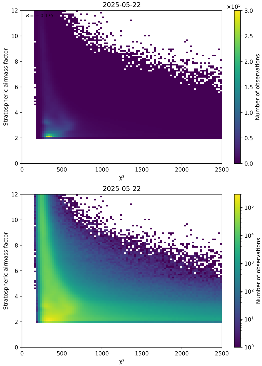
Figure 81: Scatter density plot of “ \chi^2 ” against “Stratospheric airmass factor” for 2025-05-21 to 2025-05-23.
