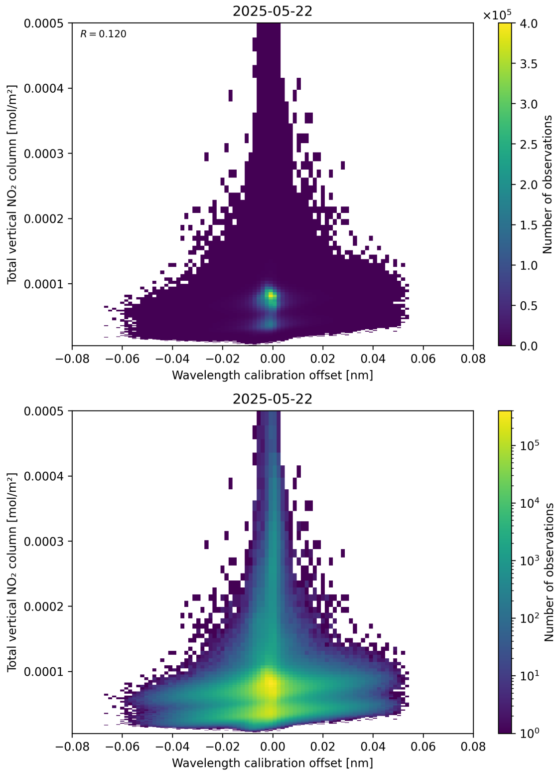
Figure 179: Scatter density plot of “Wavelength calibration offset” against “Total vertical NO 2 column” for 2025-05-21 to 2025-05-23.
