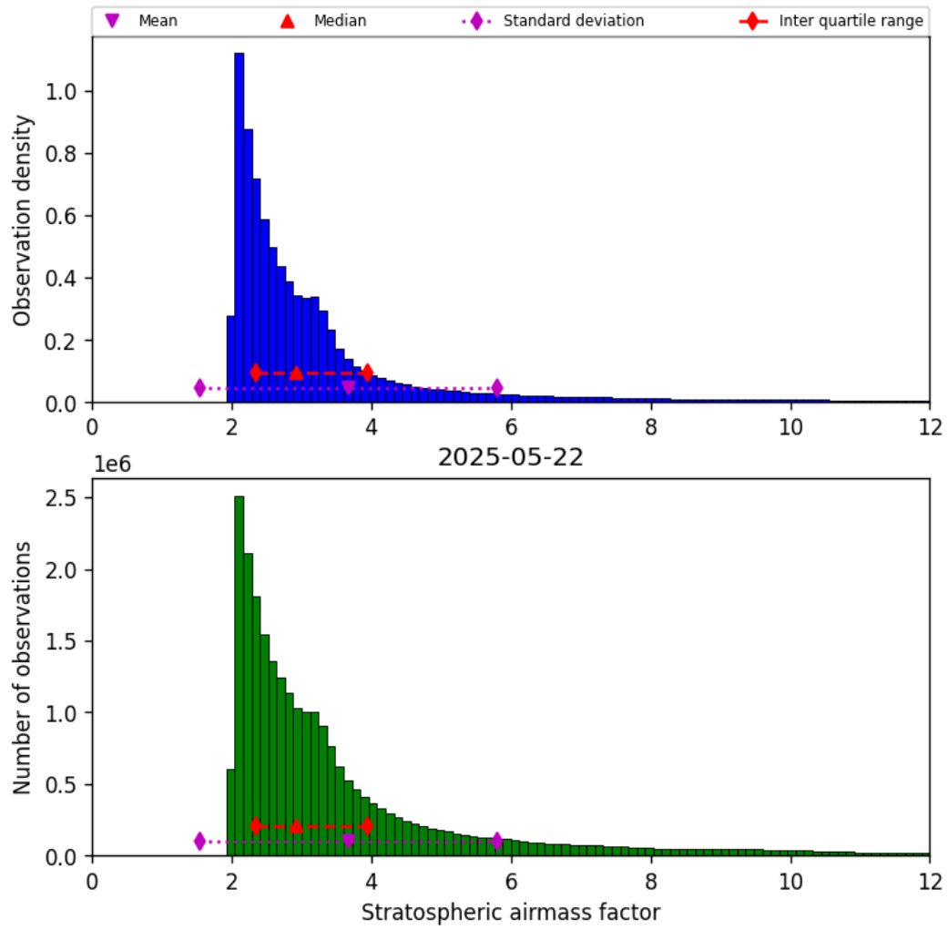
Figure 44: Histogram of “Stratospheric airmass factor” for 2025-05-21 to 2025-05-23
