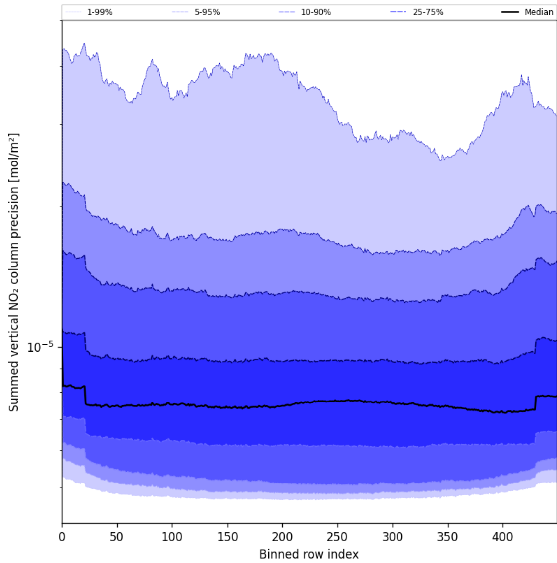
Figure 58: Along track statistics of “Summed vertical NO 2 column precision” for 2025-05-21 to 2025-05-23
