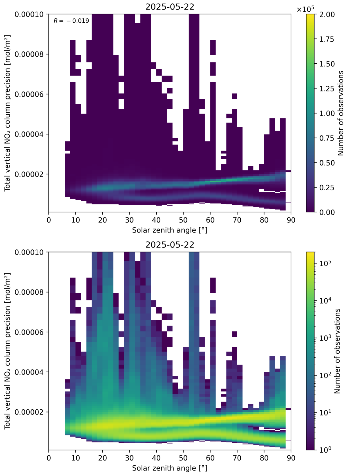
Figure 154: Scatter density plot of “Solar zenith angle” against “Total vertical NO 2 column precision” for 2025-05-21 to 2025-05-23.
