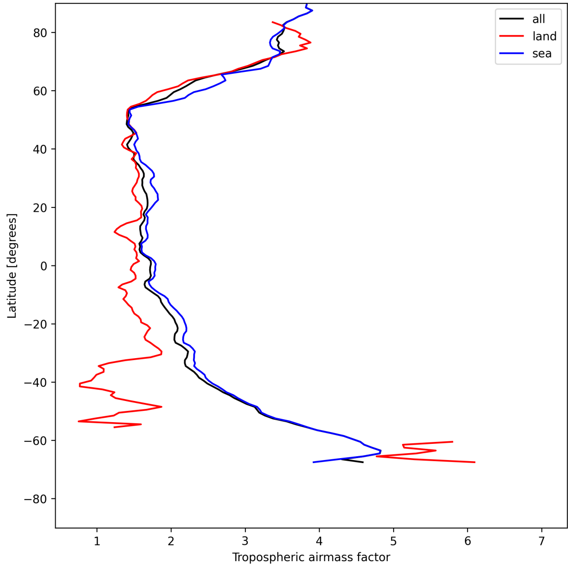
Figure 14: Zonal average of “Tropospheric air mass factor” for 2025-05-21 to 2025-05-23.
