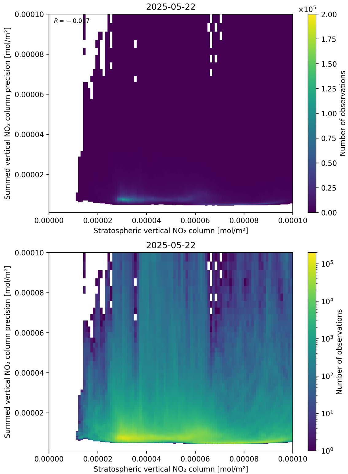
Figure 99: Scatter density plot of “Stratospheric vertical NO 2 column” against “Summed vertical NO 2 column precision” for 2025-05-21 to 2025-05-23.
