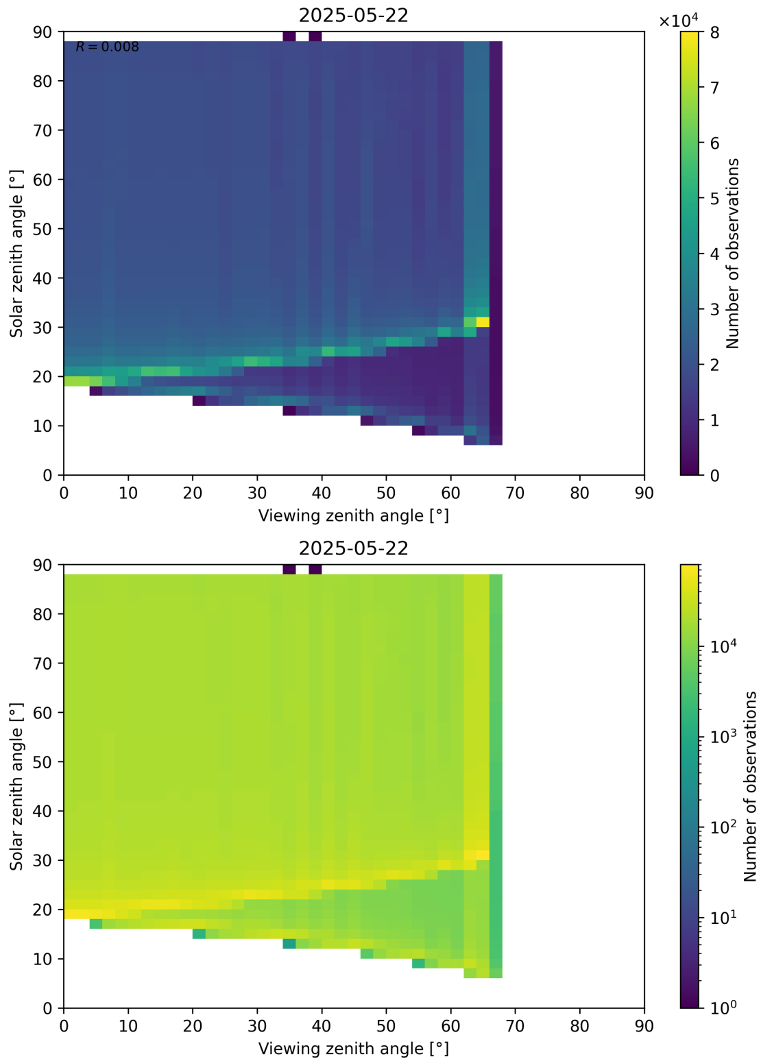
Figure 172: Scatter density plot of “Viewing zenith angle” against “Solar zenith angle” for 2025-05-21 to 2025-05-23.
