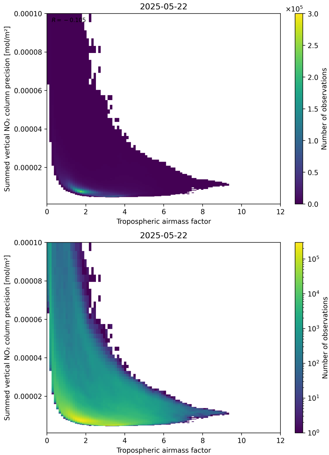
Figure 76: Scatter density plot of “Tropospheric air mass factor” against “Summed vertical NO 2 column precision” for 2025-05-21 to 2025-05-23.
