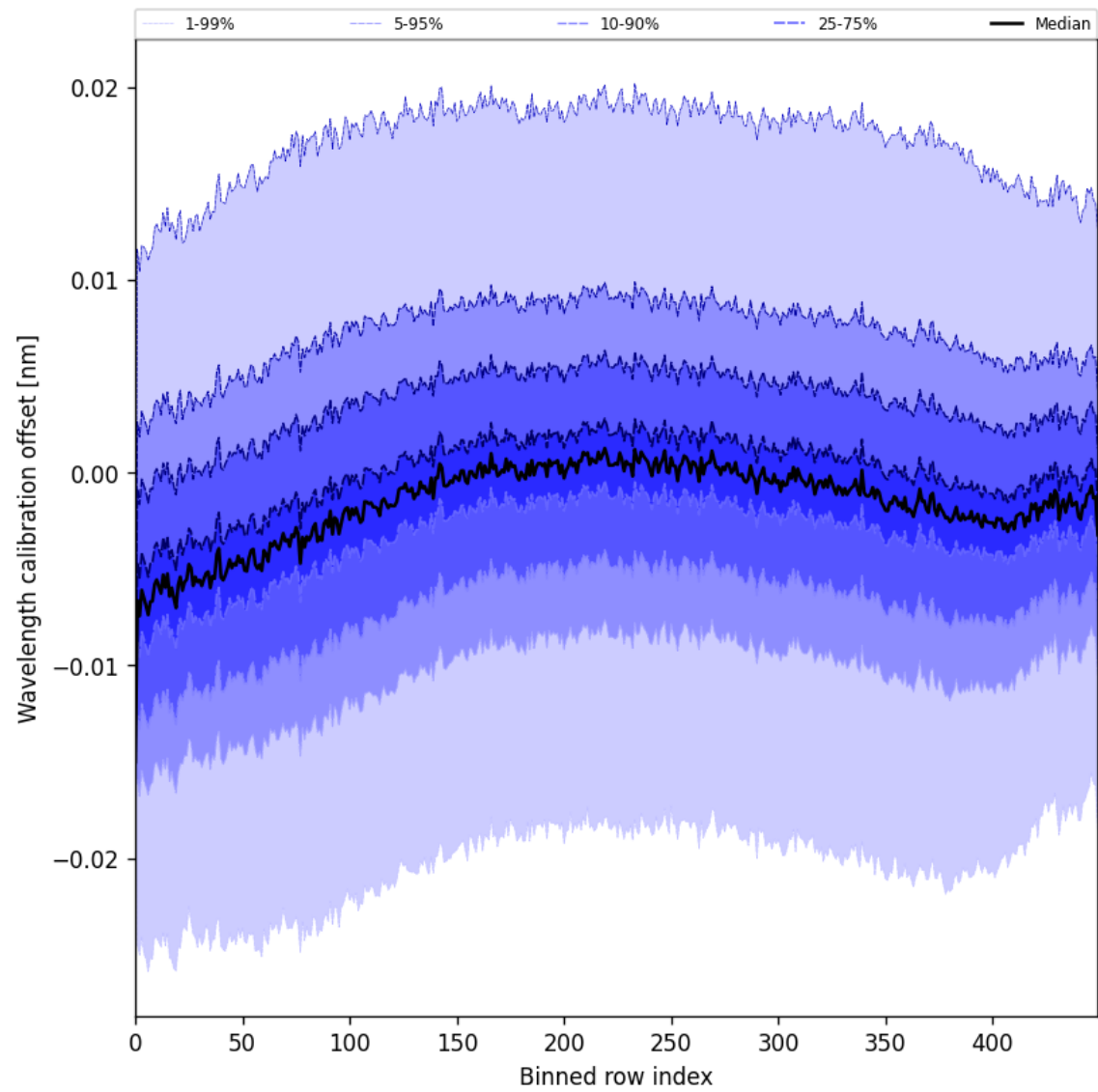
Figure 52: Along track statistics of “Wavelength calibration offset” for 2025-05-21 to 2025-05-23
