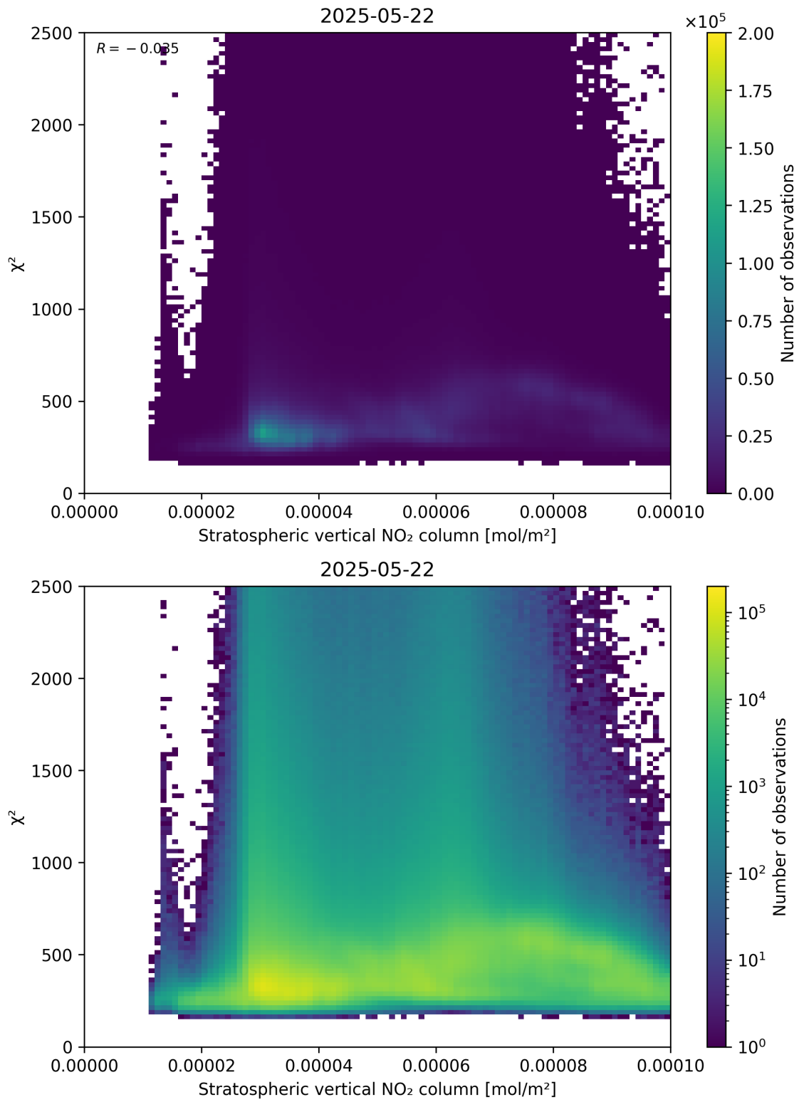
Figure 97: Scatter density plot of “Stratospheric vertical NO 2 column” against “ \chi^2 ” for 2025-05-21 to 2025-05-23.
