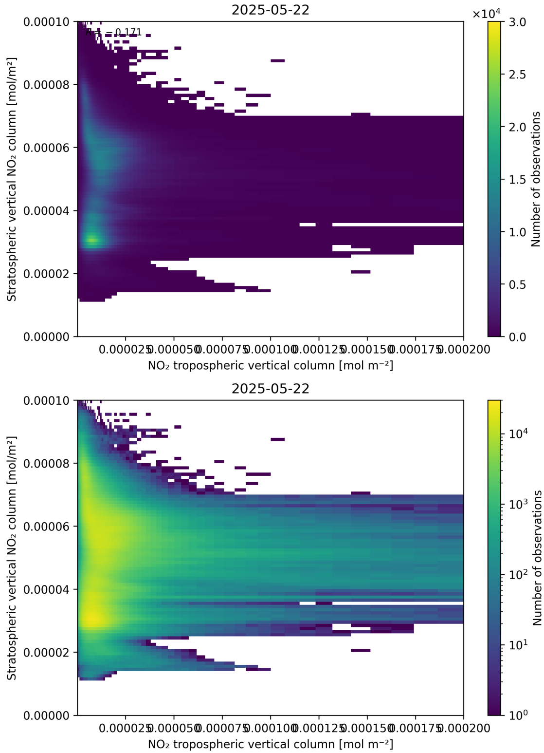
Figure 125: Scatter density plot of “NO 2 tropospheric vertical column” against “Stratospheric vertical NO 2 column” for 2025-05-21 to 2025-05-23.
