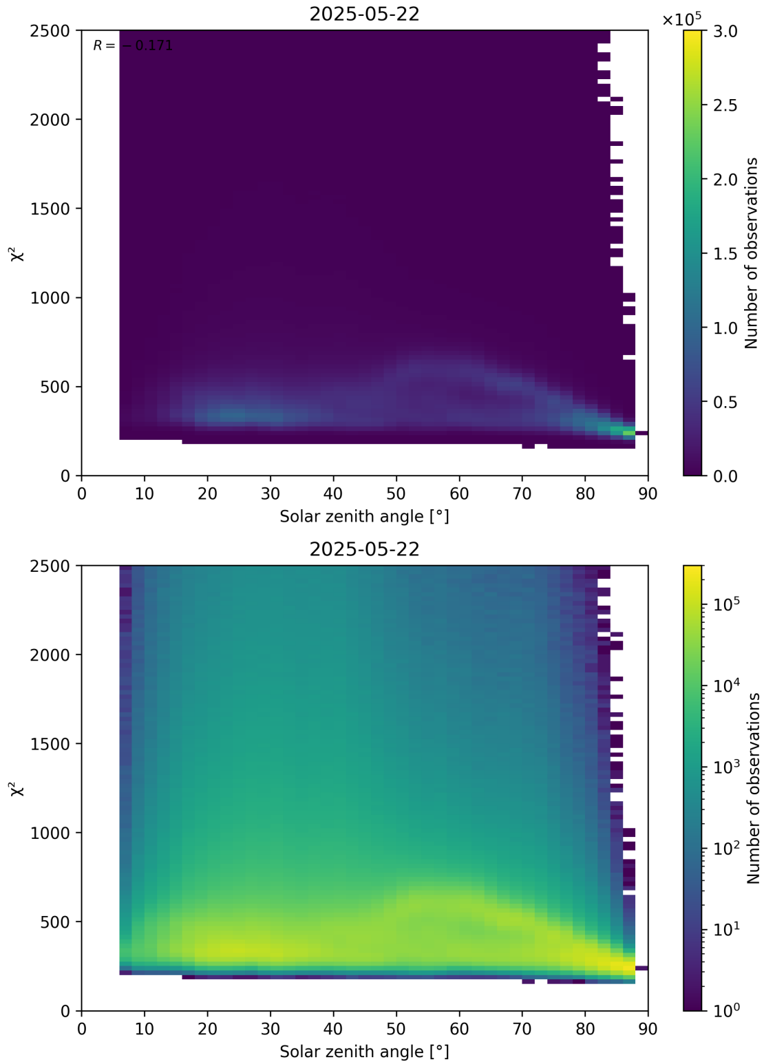
Figure 148: Scatter density plot of “Solar zenith angle” against “ \chi^2 ” for 2025-05-21 to 2025-05-23.
