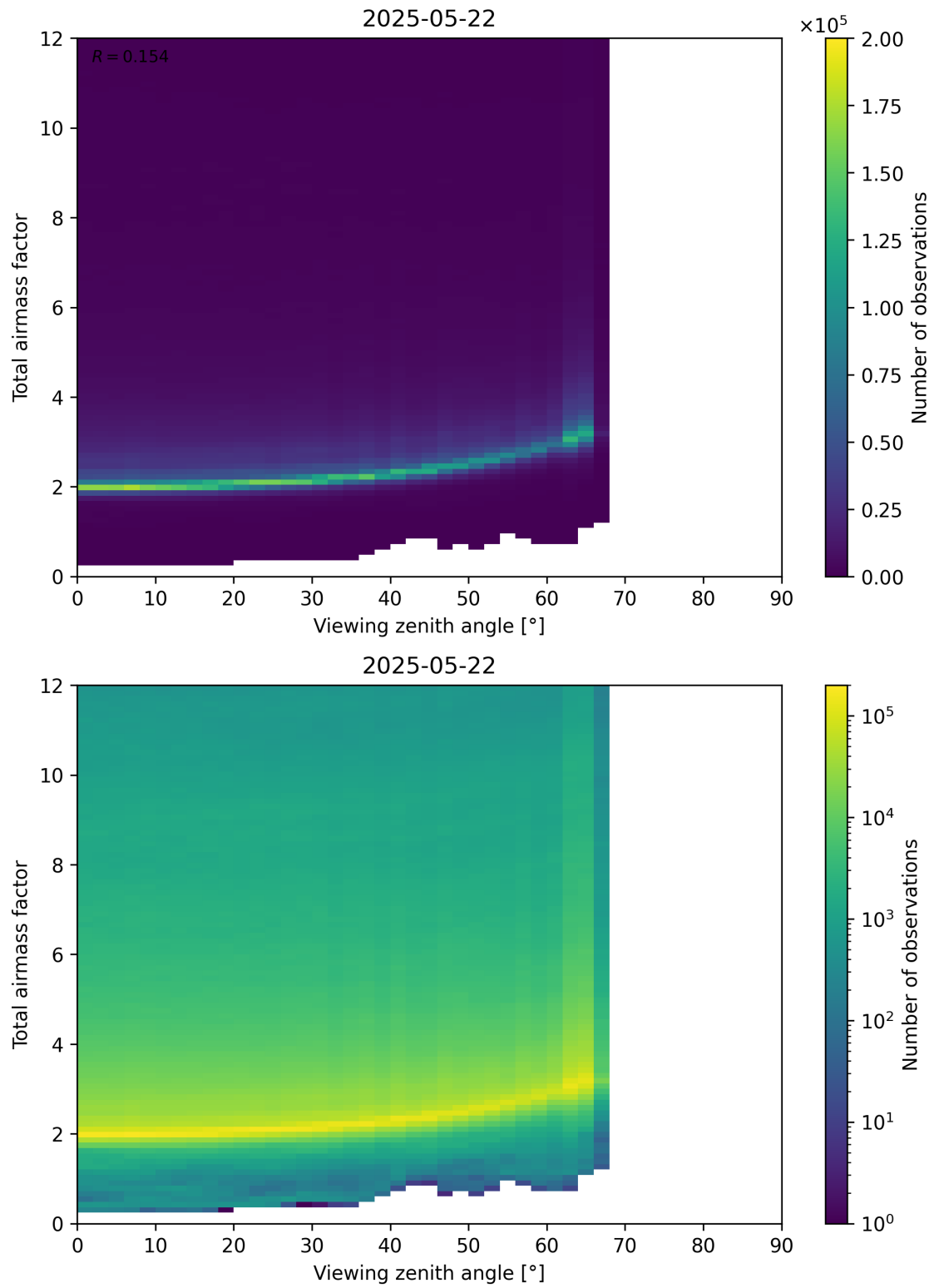
Figure 160: Scatter density plot of “Viewing zenith angle” against “Total airmass factor” for 2025-05-21 to 2025-05-23.
