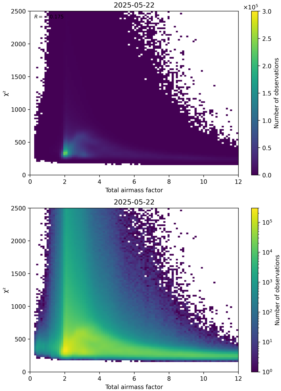
Figure 63: Scatter density plot of “Total airmass factor” against “ \chi^2 ” for 2025-05-21 to 2025-05-23.
