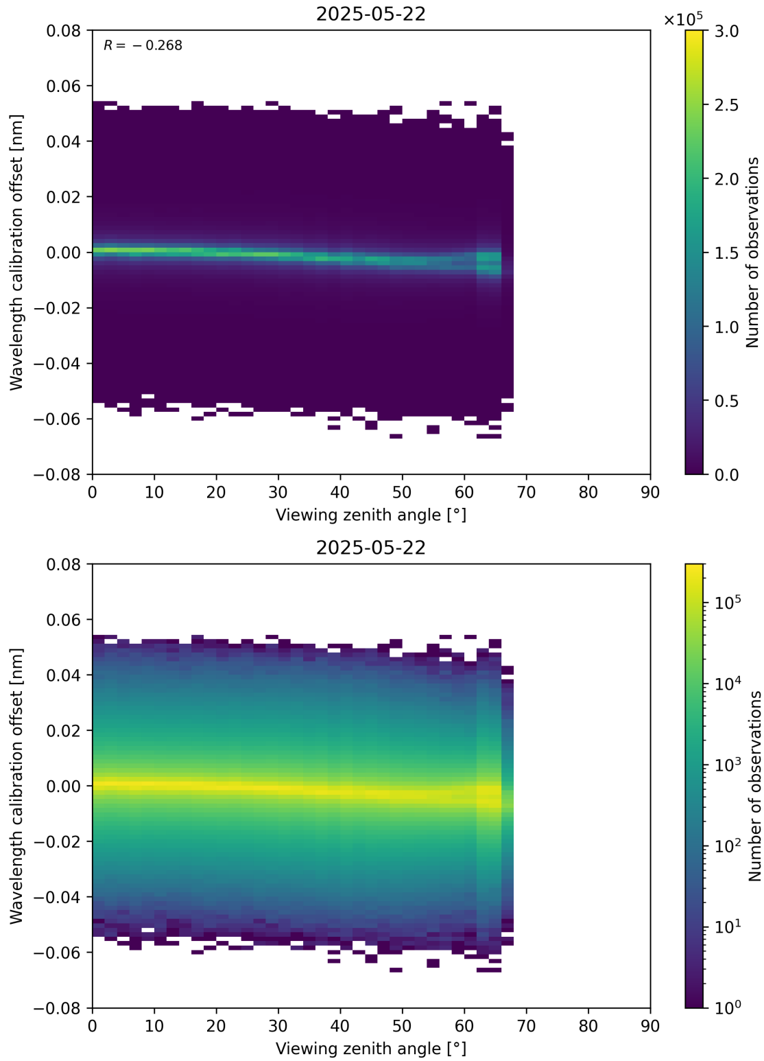
Figure 173: Scatter density plot of “Viewing zenith angle” against “Wavelength calibration offset” for 2025-05-21 to 2025-05-23.
