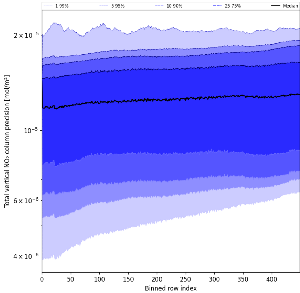
Figure 56: Along track statistics of “Total vertical NO 2 column precision” for 2025-05-21 to 2025-05-23
