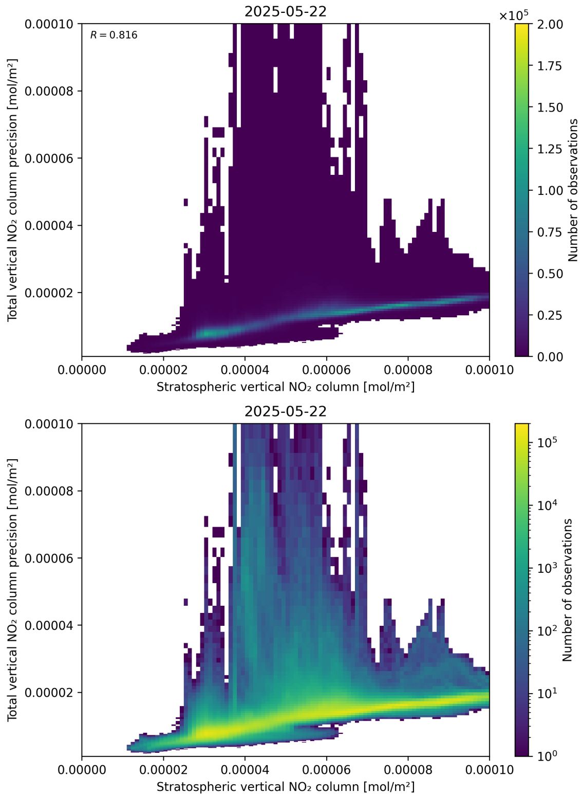
Figure 101: Scatter density plot of “Stratospheric vertical NO 2 column” against “Total vertical NO 2 column precision” for 2025-05-21 to 2025-05-23.
