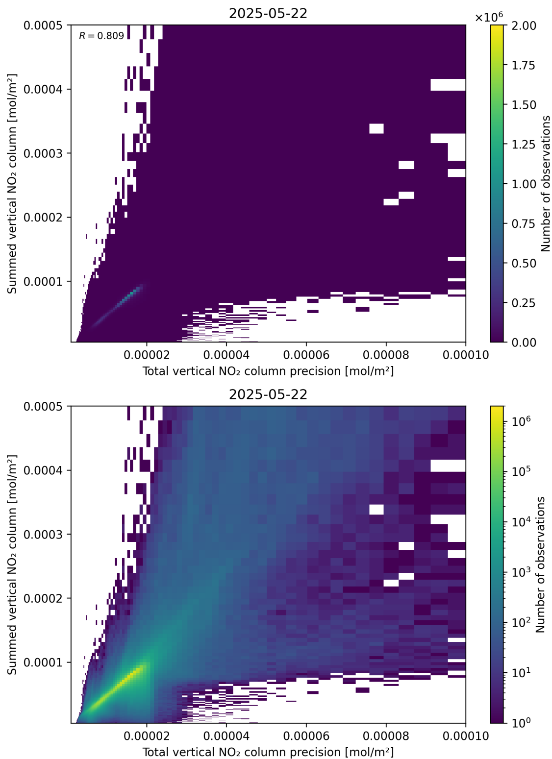
Figure 117: Scatter density plot of “Total vertical NO 2 column precision” against “Summed vertical NO 2 column” for 2025-05-21 to 2025-05-23.
