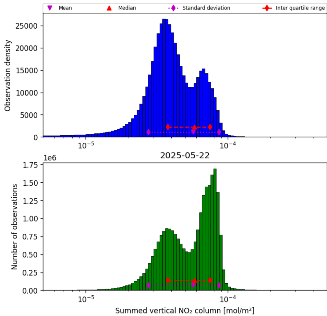
Figure 40: Histogram of “Summed vertical NO 2 column” for 2025-05-21 to 2025-05-23
