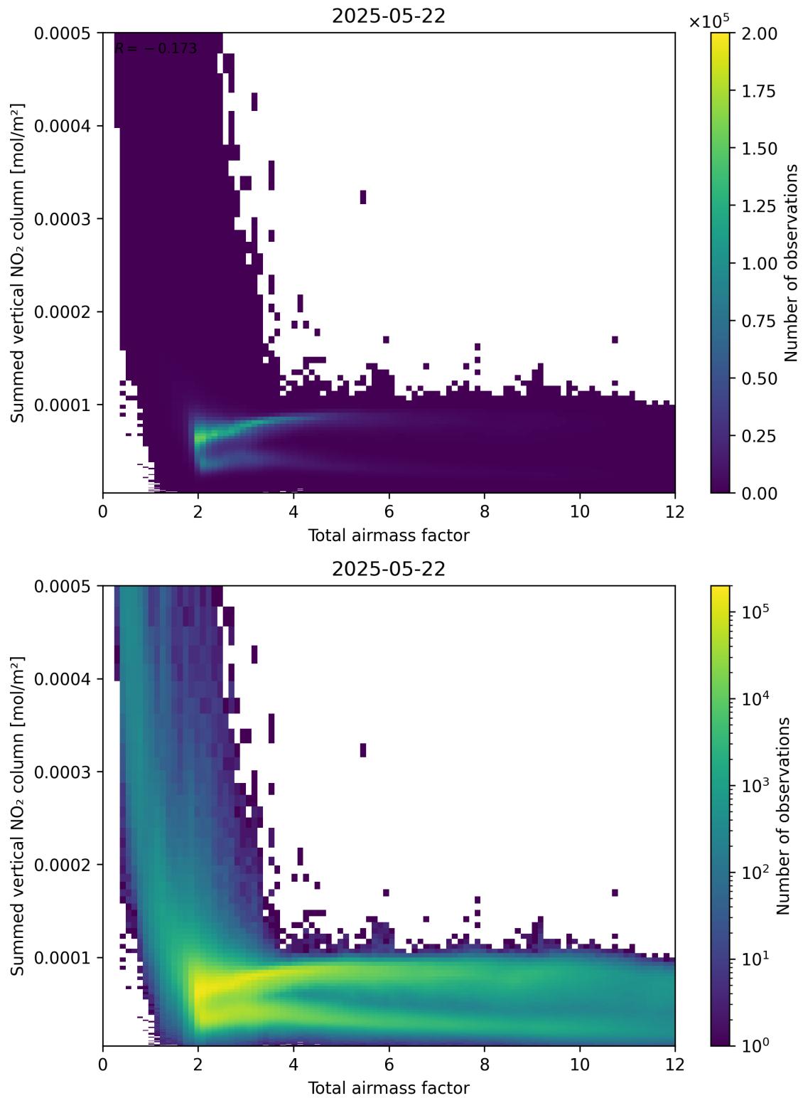
Figure 65: Scatter density plot of “Total airmass factor” against “Summed vertical NO 2 column” for 2025-05-21 to 2025-05-23.
