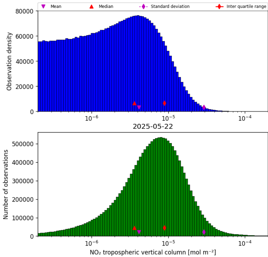
Figure 29: Histogram of “NO 2 tropospheric vertical column” for 2025-05-21 to 2025-05-23
