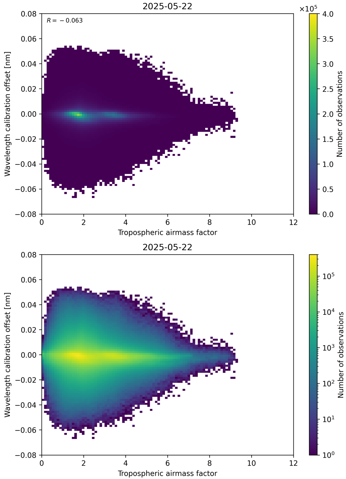
Figure 80: Scatter density plot of “Tropospheric airmass factor” against “Wavelength calibration offset” for 2025-05-21 to 2025-05-23.
