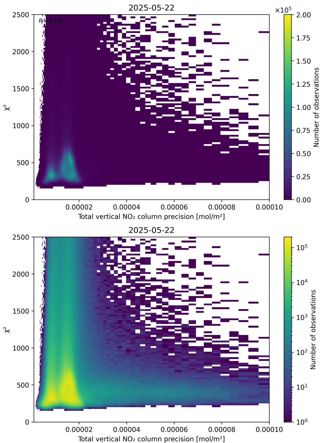
Figure 116: Scatter density plot of “Total vertical NO 2 column precision” against “ \chi^2 ” for 2025-05-21 to 2025-05-23.
