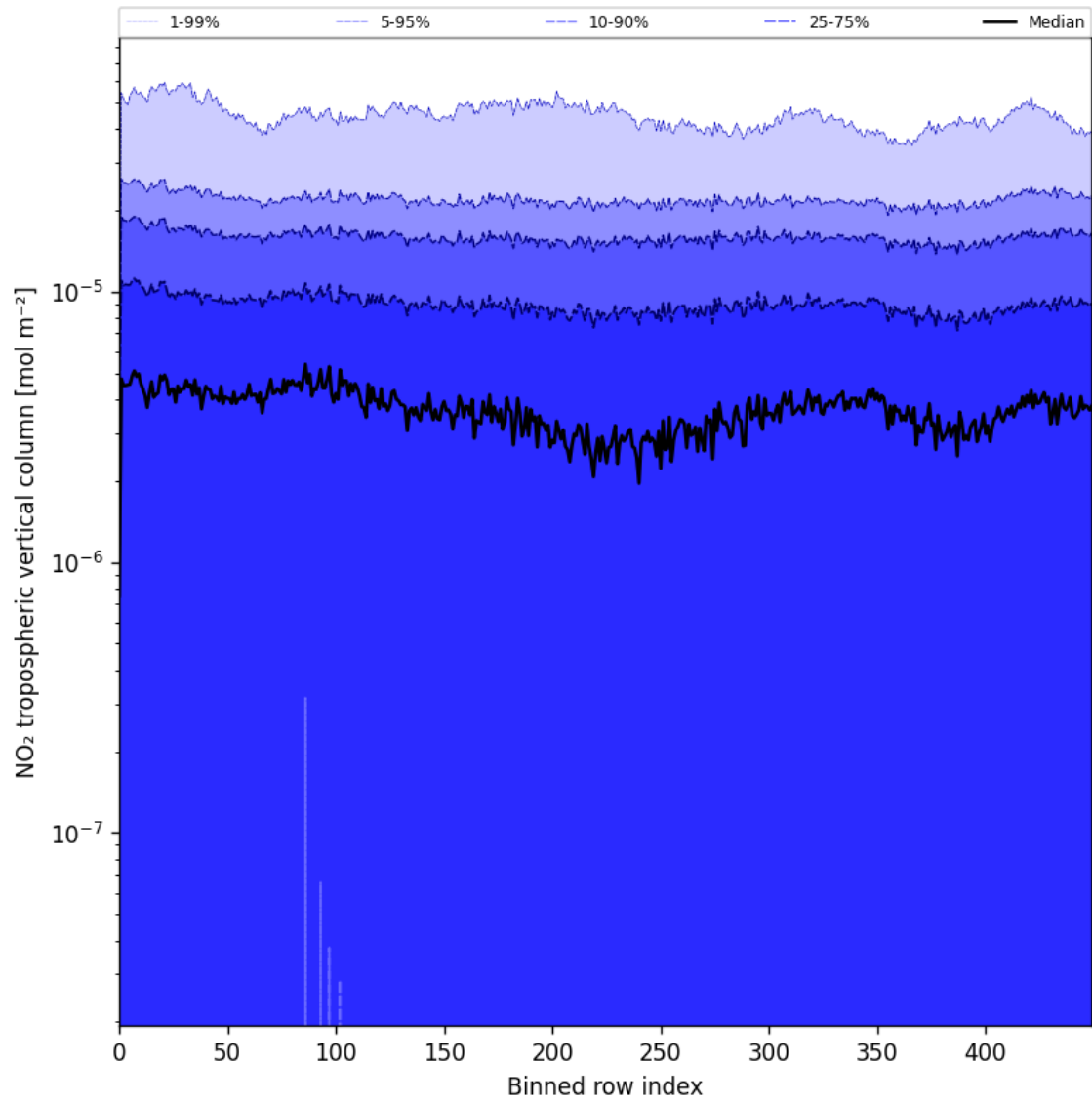
Figure 46: Along track statistics of “NO 2 tropospheric vertical column” for 2025-05-21 to 2025-05-23
