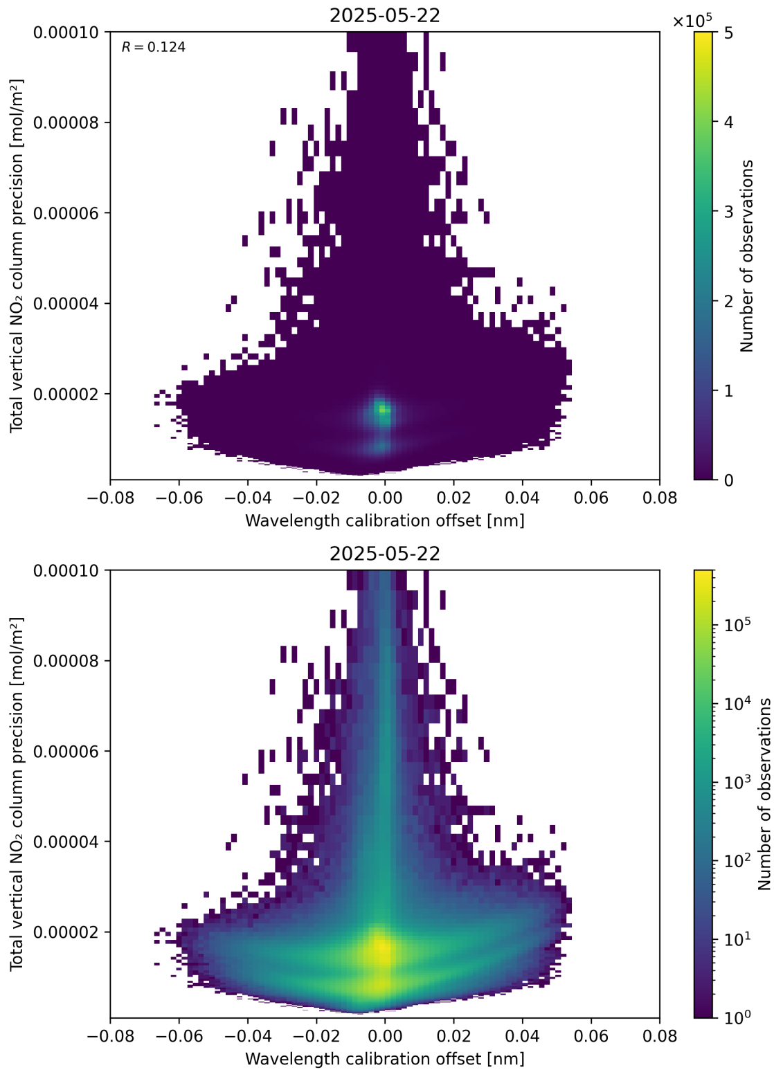
Figure 180: Scatter density plot of “Wavelength calibration offset” against “Total vertical NO 2 column precision” for 2025-05-21 to 2025-05-23.
