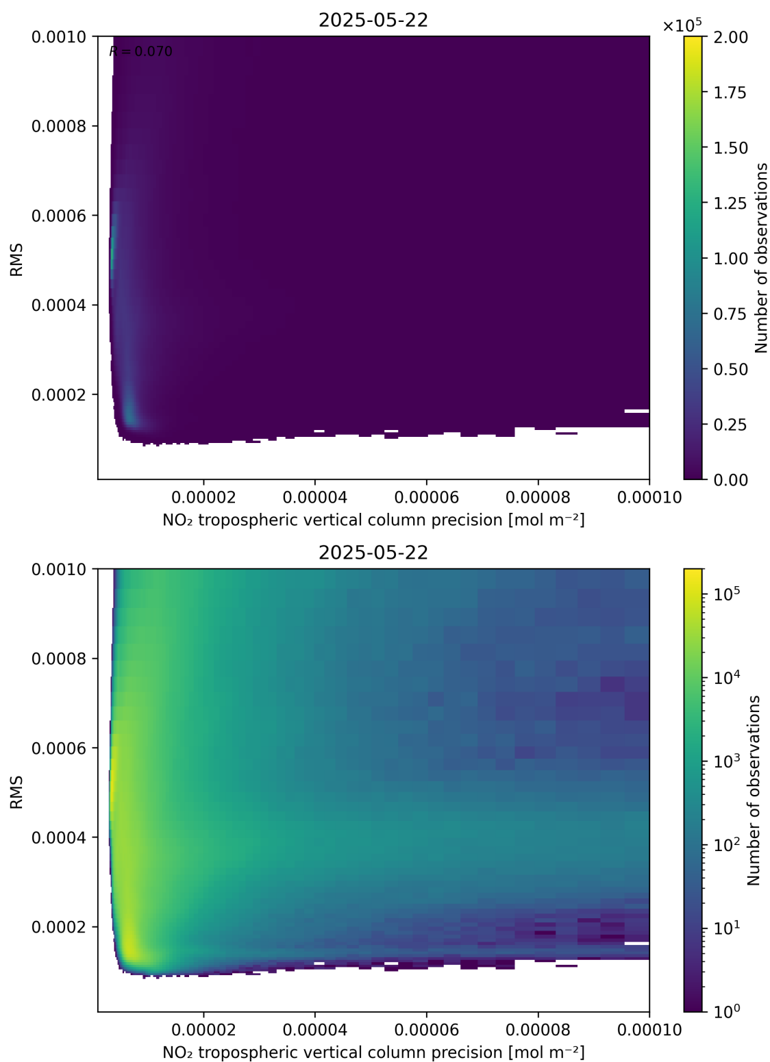
Figure 140: Scatter density plot of “NO 2 tropospheric vertical column precision” against “RMS” for 2025-05-21 to 2025-05-23.
