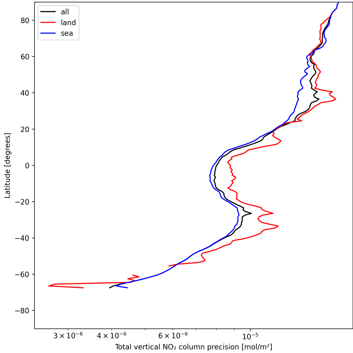
Figure 22: Zonal average of “Total vertical NO 2 column precision” for 2025-05-21 to 2025-05-23.
