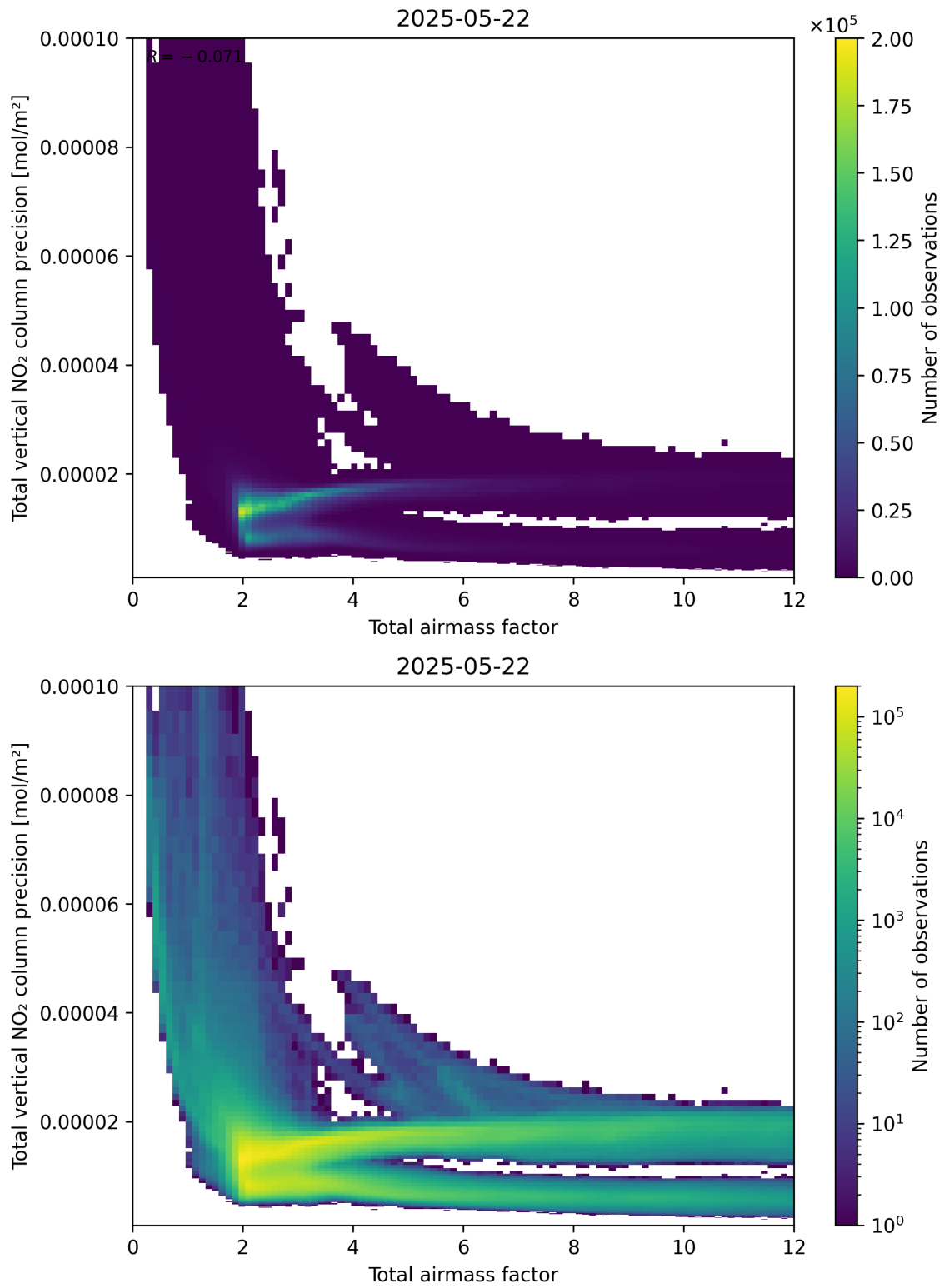
Figure 68: Scatter density plot of “Total airmass factor” against “Total vertical NO 2 column precision” for 2025-05-21 to 2025-05-23.
