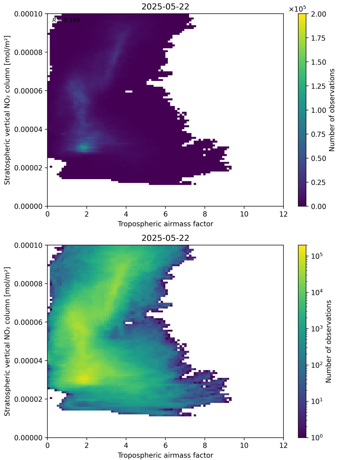
Figure 74: Scatter density plot of “Tropospheric air mass factor” against “Stratospheric vertical NO 2 column” for 2025-05-21 to 2025-05-23.
