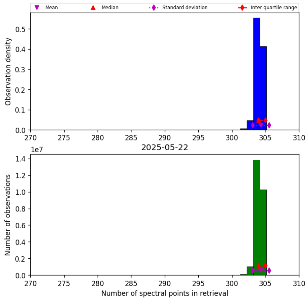
Figure 33: Histogram of “Number of spectral points in retrieval” for 2025-05-21 to 2025-05-23
