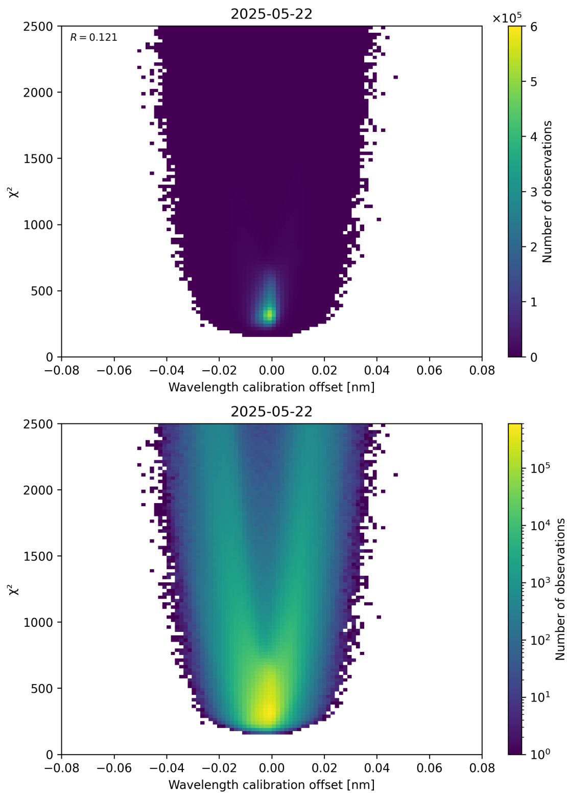
Figure 175: Scatter density plot of “Wavelength calibration offset” against “ \chi^2 ” for 2025-05-21 to 2025-05-23.
