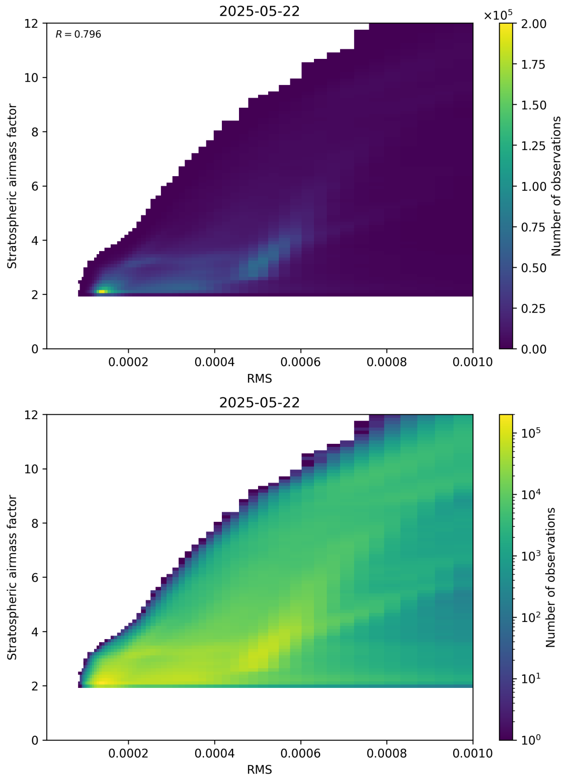
Figure 144: Scatter density plot of “RMS” against “Stratospheric airmass factor” for 2025-05-21 to 2025-05-23.
