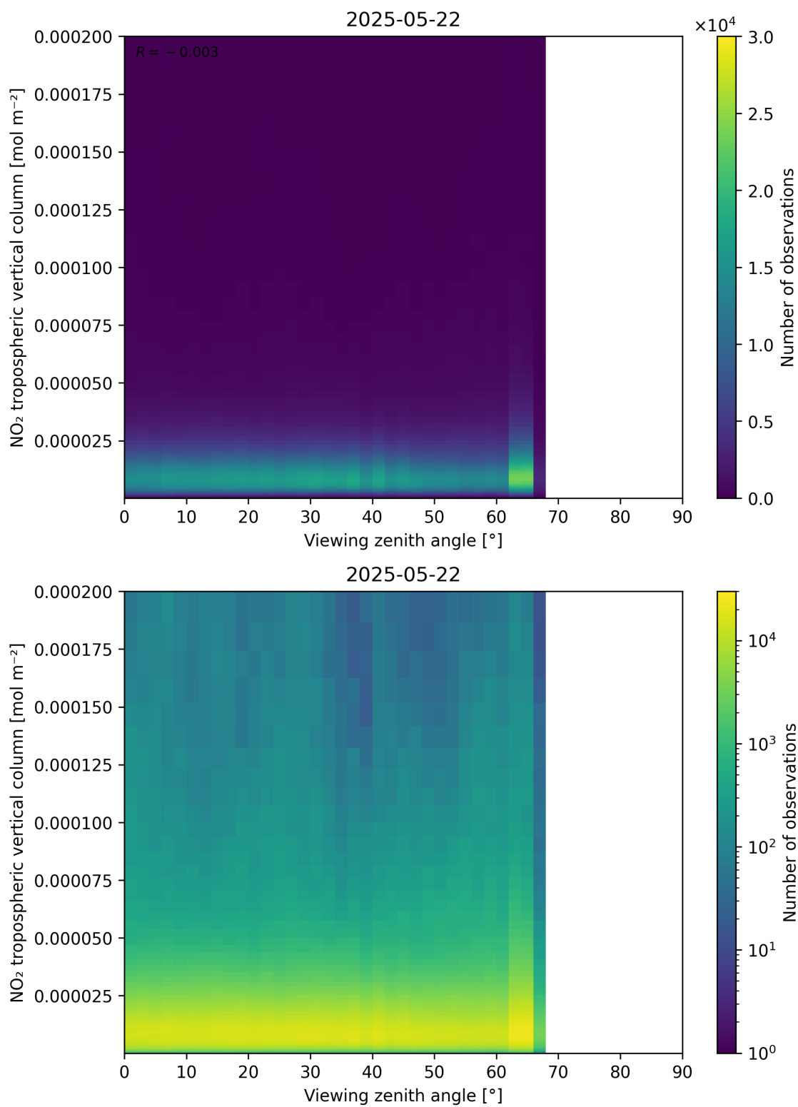
Figure 169: Scatter density plot of “Viewing zenith angle” against “NO 2 tropospheric vertical column” for 2025-05-21 to 2025-05-23.
