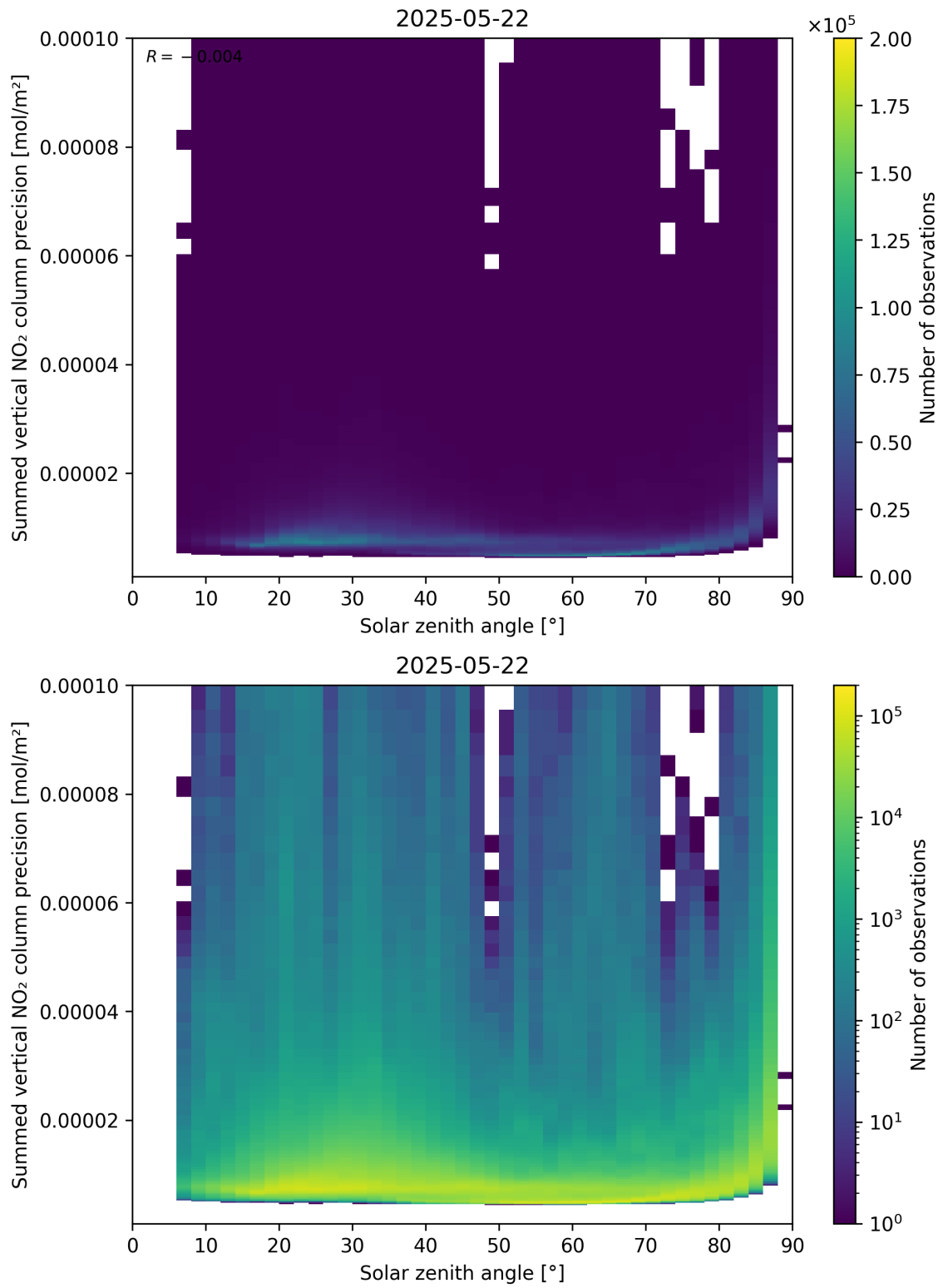
Figure 152: Scatter density plot of “Solar zenith angle” against “Summed vertical NO 2 column precision” for 2025-05-21 to 2025-05-23.
