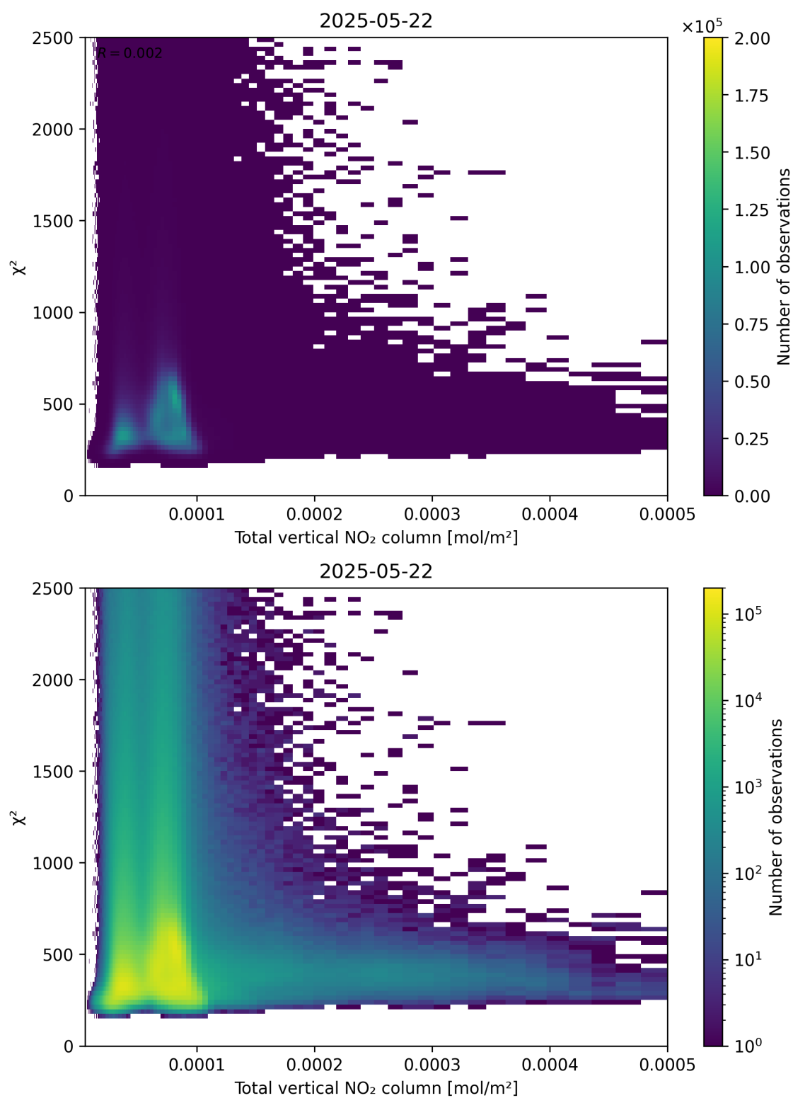
Figure 111: Scatter density plot of “Total vertical NO 2 column” against “ \chi^2 ” for 2025-05-21 to 2025-05-23.
