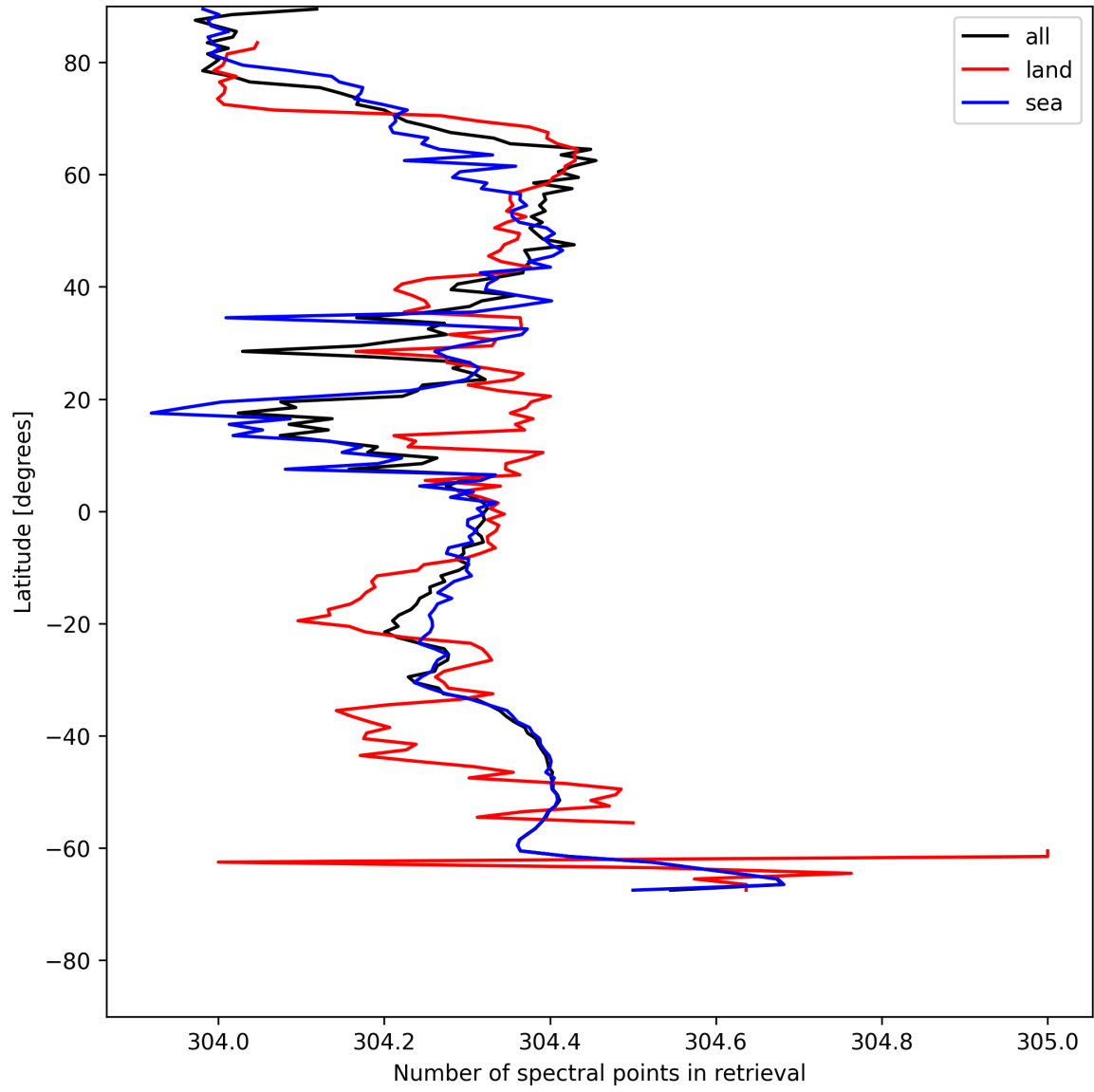
Figure 16: Zonal average of “Number of spectral points in retrieval” for 2025-05-21 to 2025-05-23.
