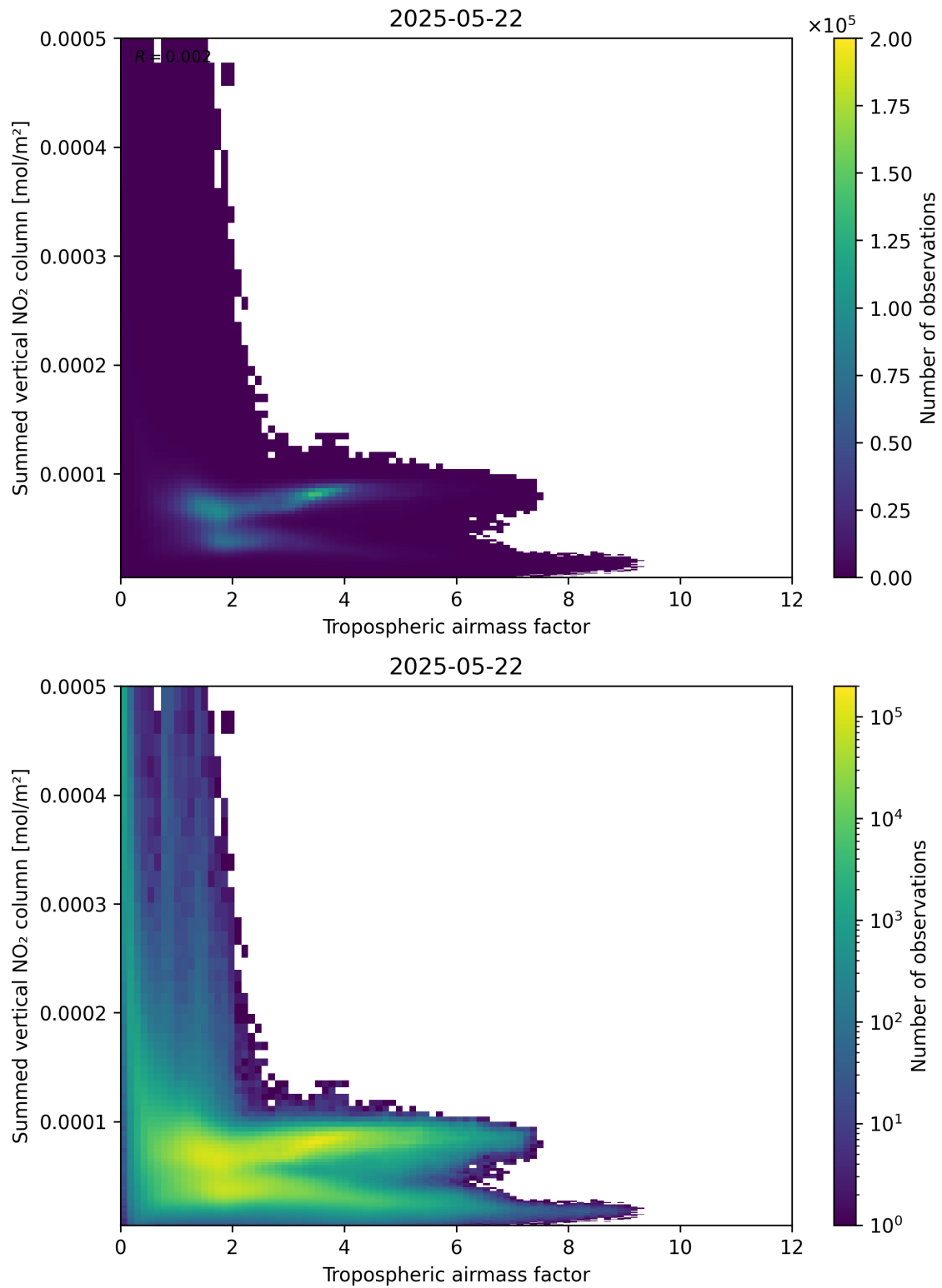
Figure 75: Scatter density plot of “Tropospheric air mass factor” against “Summed vertical NO 2 column” for 2025-05-21 to 2025-05-23.
