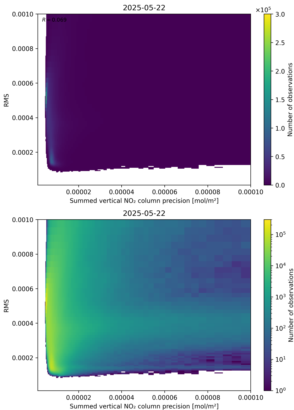
Figure 108: Scatter density plot of “Summed vertical NO 2 column precision” against “RMS” for 2025-05-21 to 2025-05-23.
