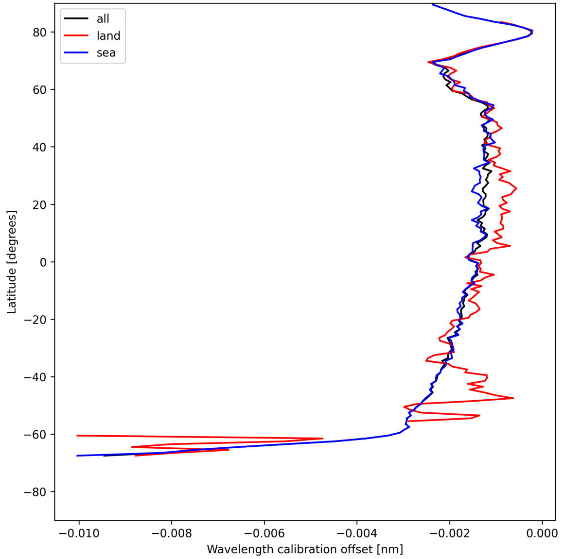
Figure 18: Zonal average of “Wavelength calibration offset” for 2025-05-21 to 2025-05-23.
