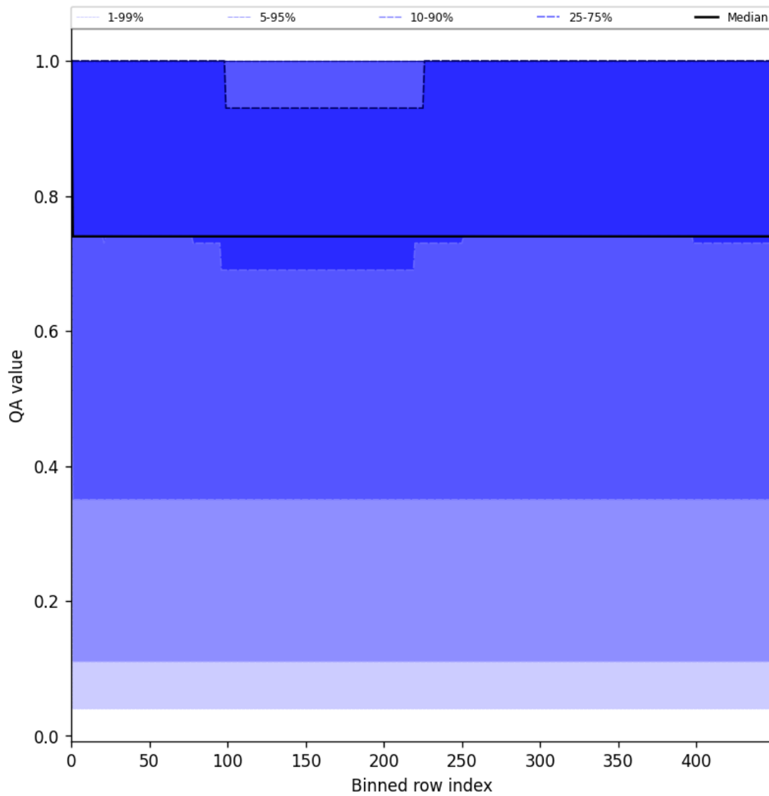
Figure 45: Along track statistics of “QA value” for 2025-05-21 to 2025-05-23
