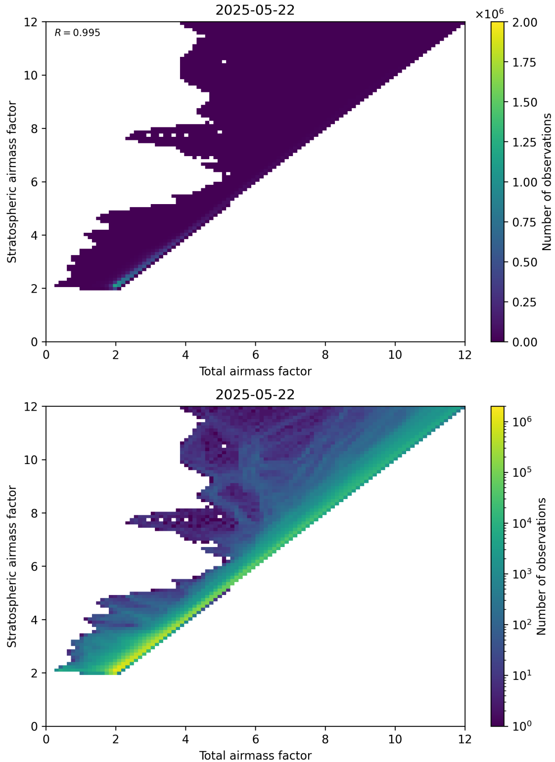
Figure 62: Scatter density plot of “Total airmass factor” against “Stratospheric airmass factor” for 2025-05-21 to 2025-05-23.
