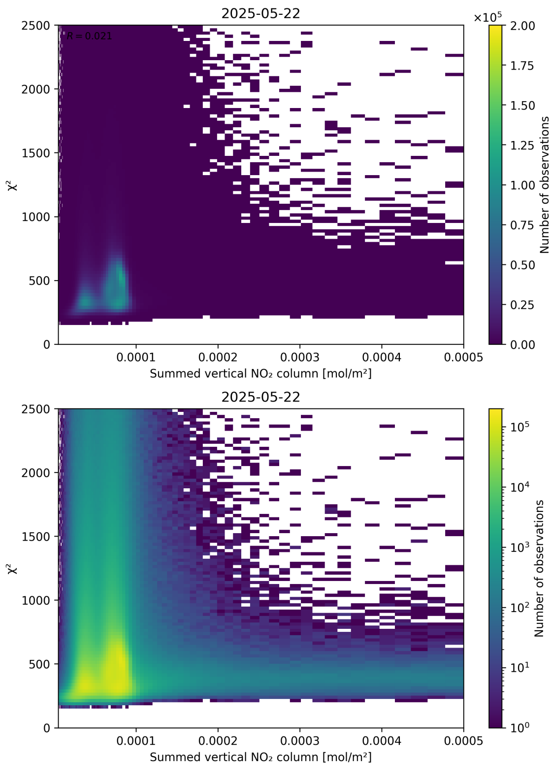
Figure 104: Scatter density plot of “Summed vertical NO 2 column” against “ \chi^2 ” for 2025-05-21 to 2025-05-23.
