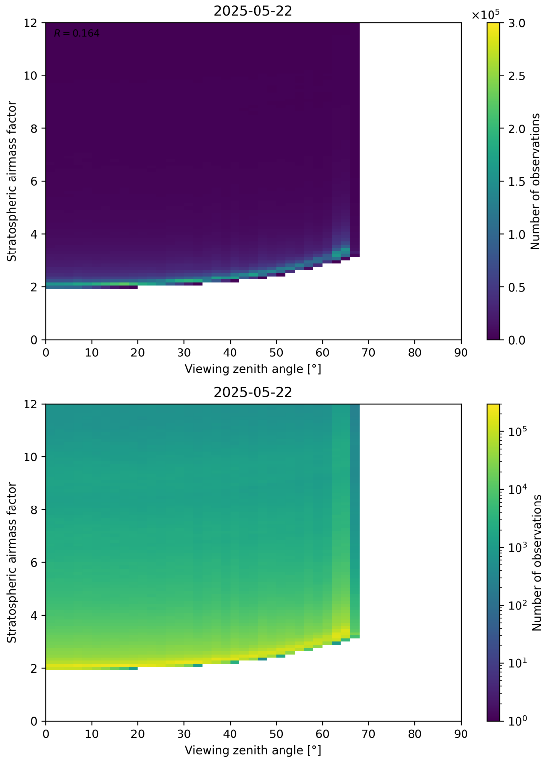
Figure 159: Scatter density plot of “Viewing zenith angle” against “Stratospheric airmass factor” for 2025-05-21 to 2025-05-23.
