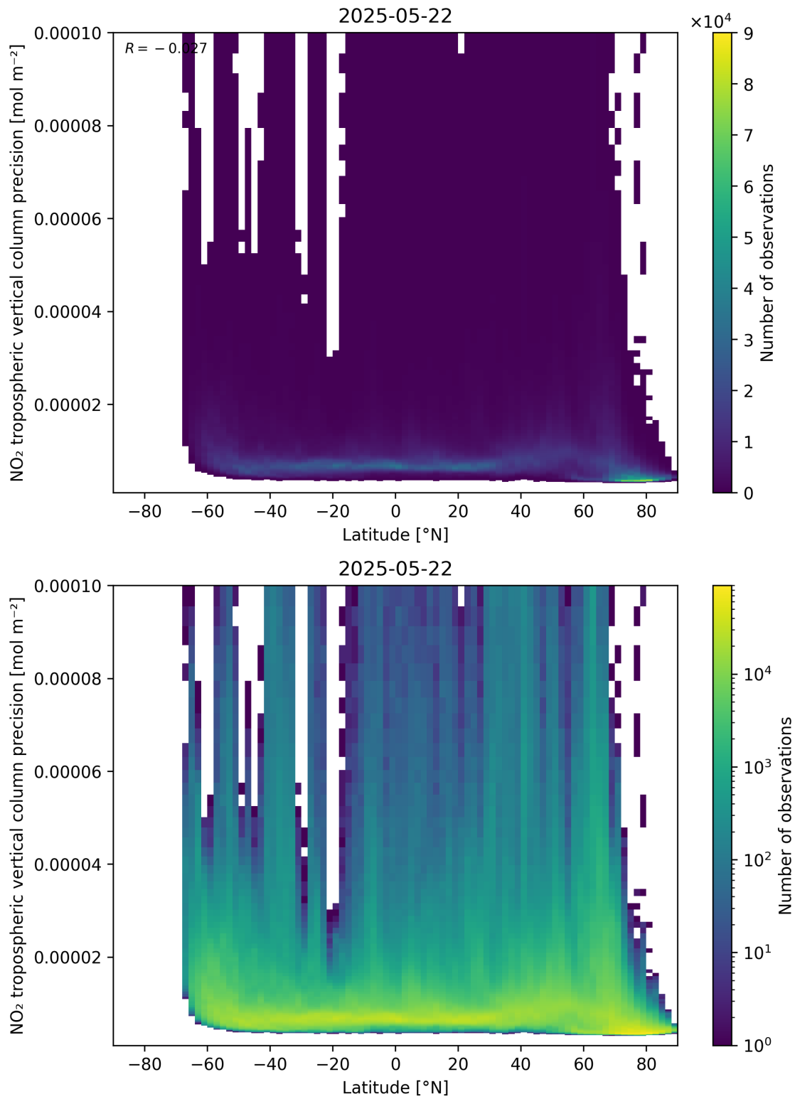
Figure 93: Scatter density plot of “Latitude” against “NO 2 tropospheric vertical column precision” for 2025-05-21 to 2025-05-23.
