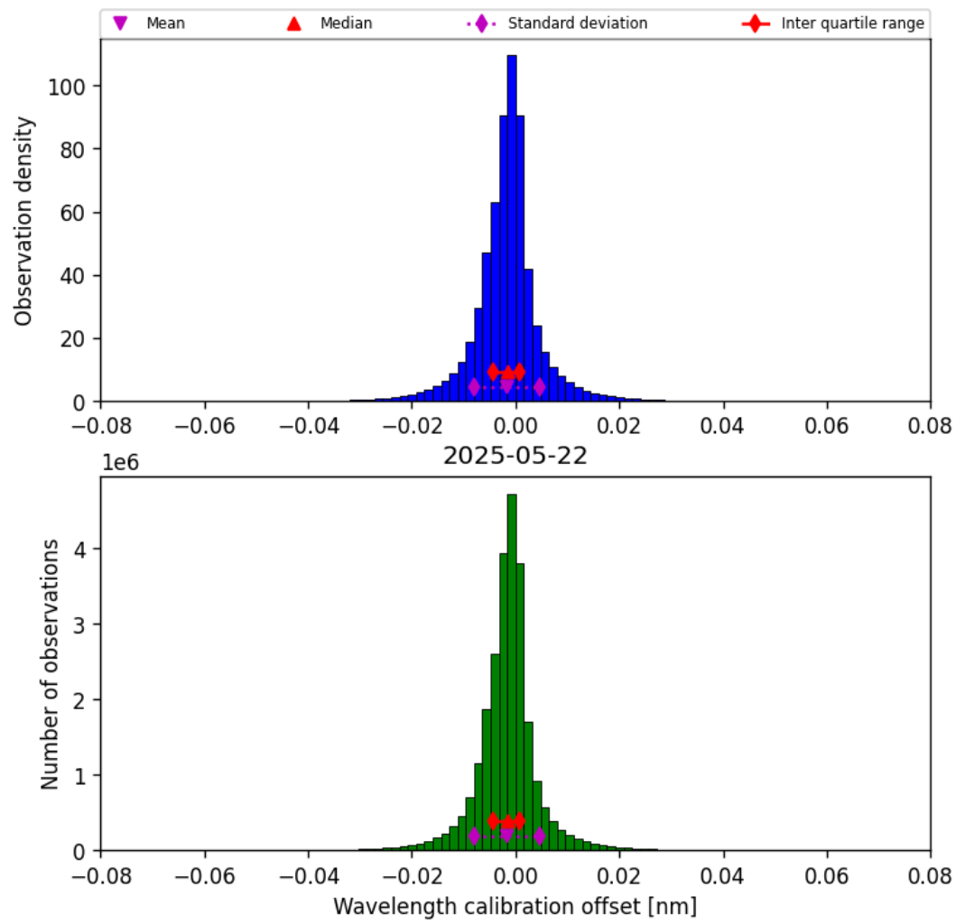
Figure 35: Histogram of “Wavelength calibration offset” for 2025-05-21 to 2025-05-23
