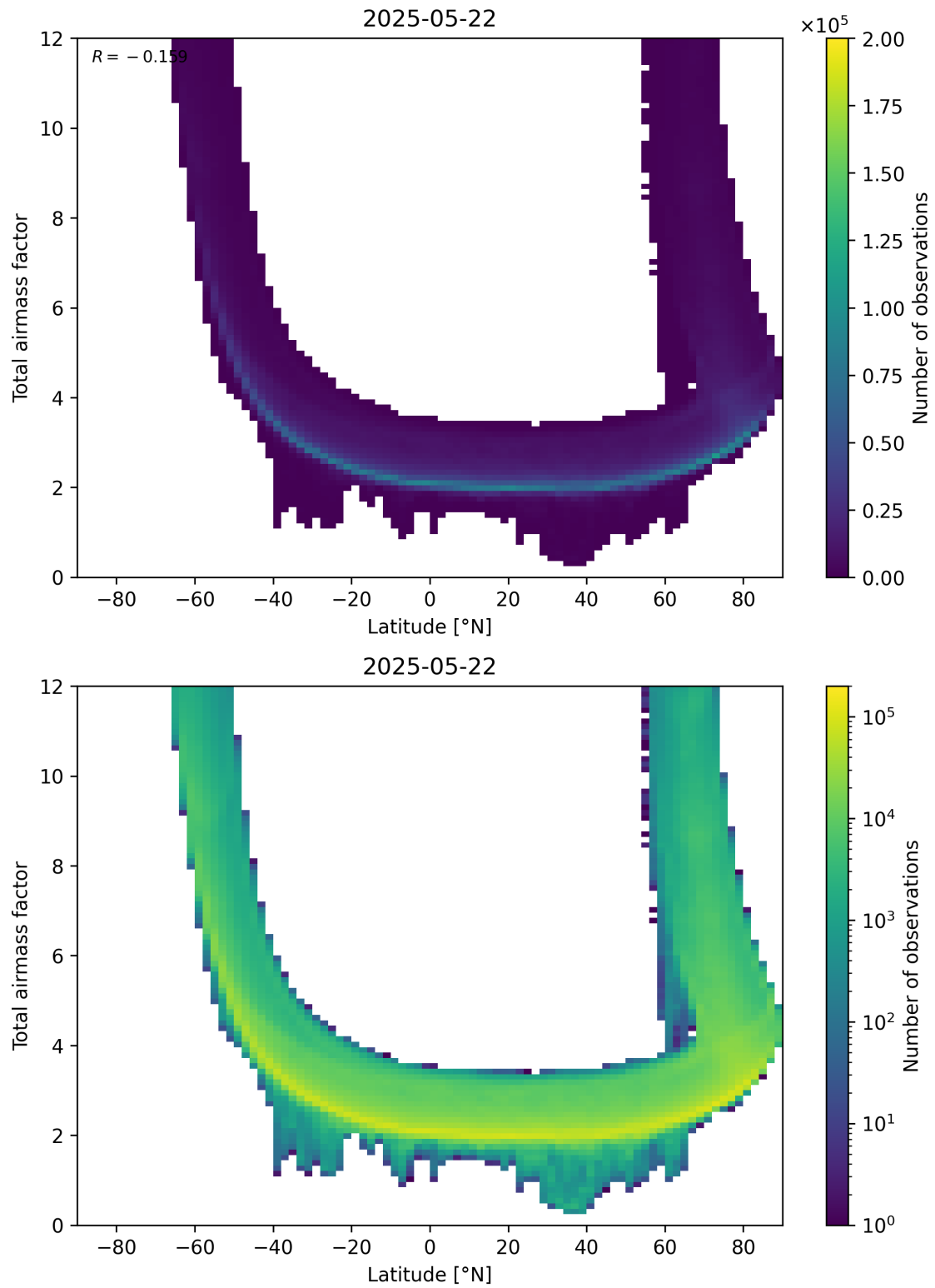
Figure 84: Scatter density plot of “Latitude” against “Total airmass factor” for 2025-05-21 to 2025-05-23.
