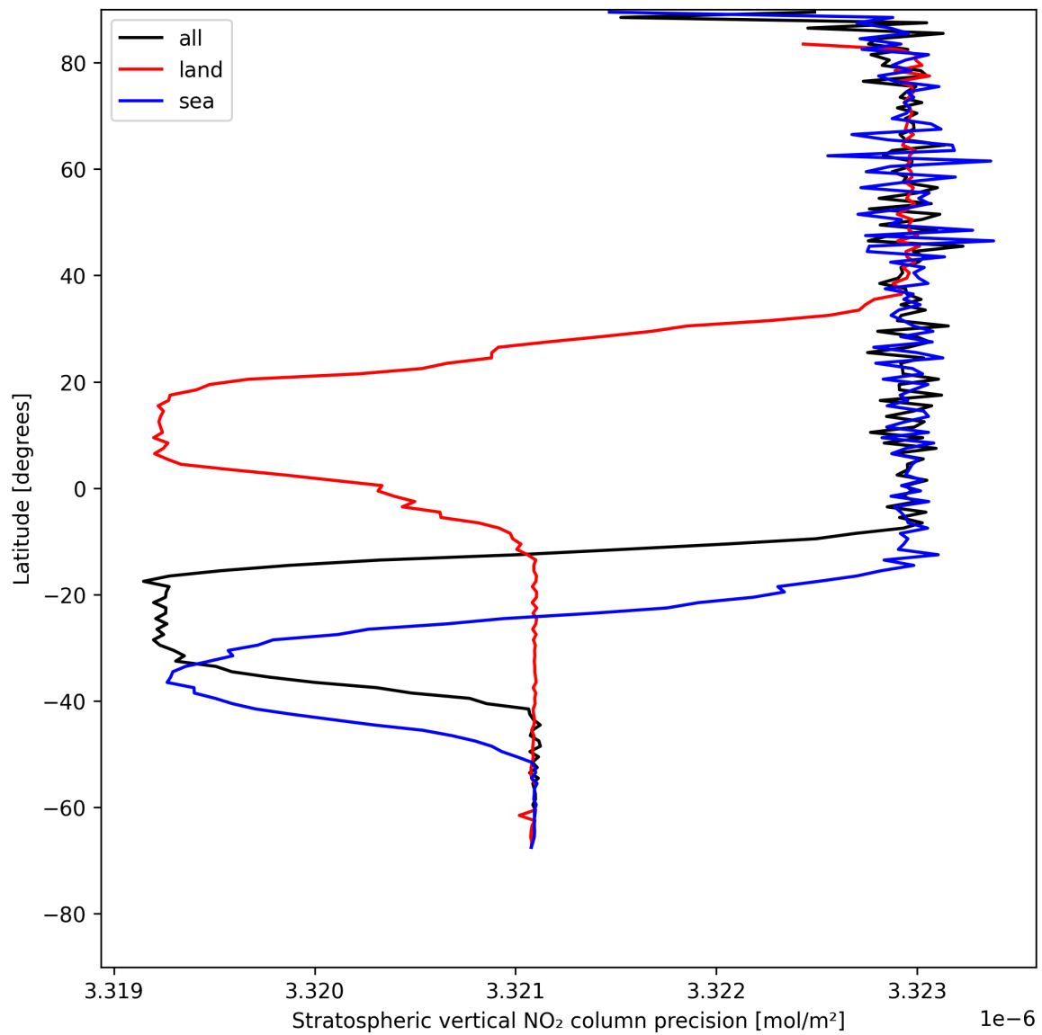
Figure 20: Zonal average of “Stratospheric vertical NO 2 column precision” for 2025-05-21 to 2025-05-23.
