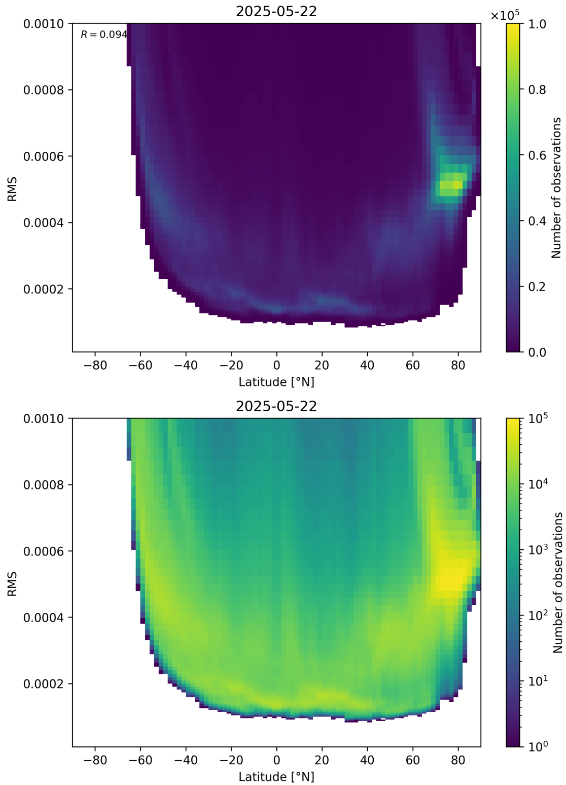
Figure 94: Scatter density plot of “Latitude” against “RMS” for 2025-05-21 to 2025-05-23.
