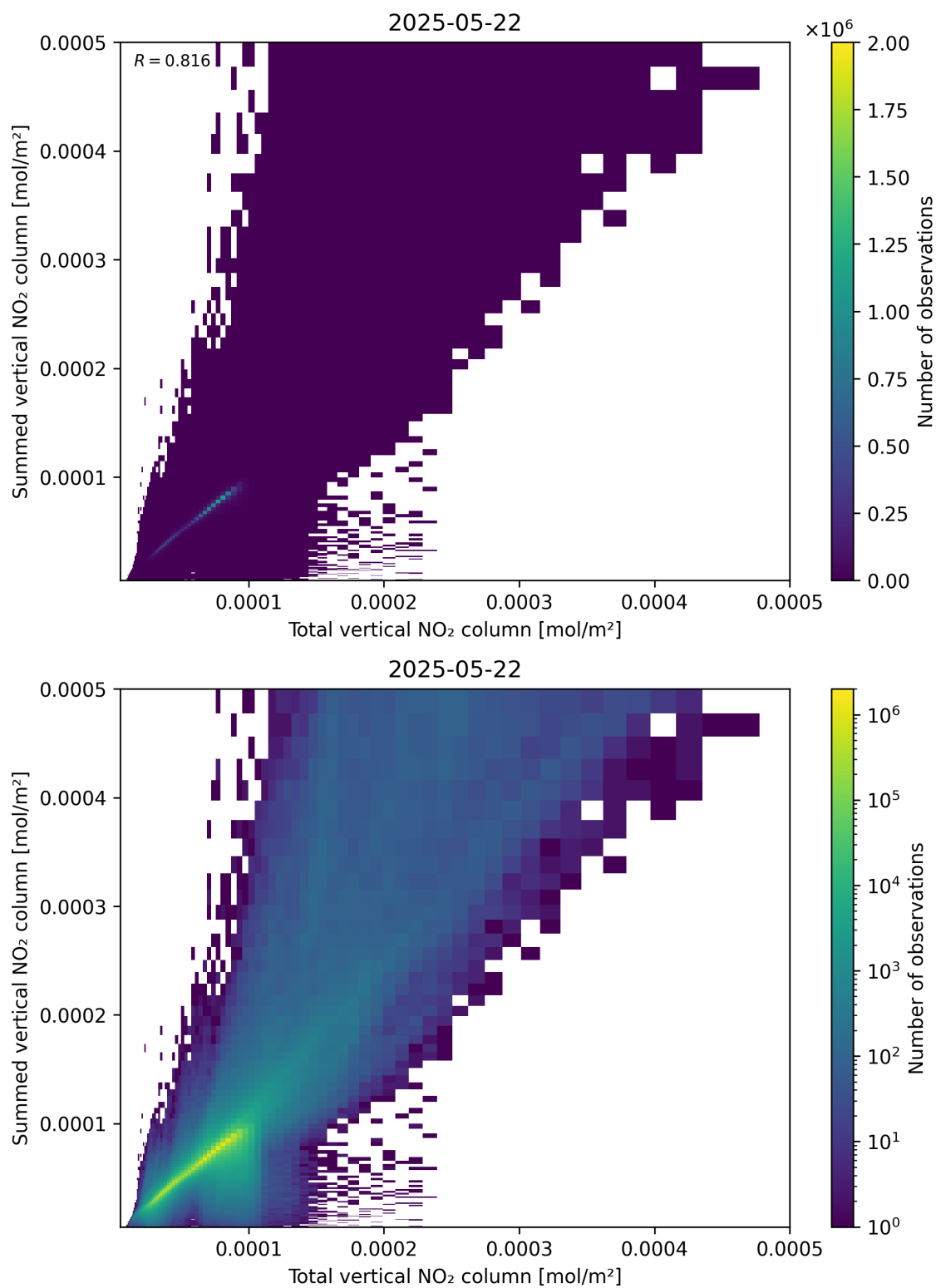
Figure 112: Scatter density plot of “Total vertical NO 2 column” against “Summed vertical NO 2 column” for 2025-05-21 to 2025-05-23.
