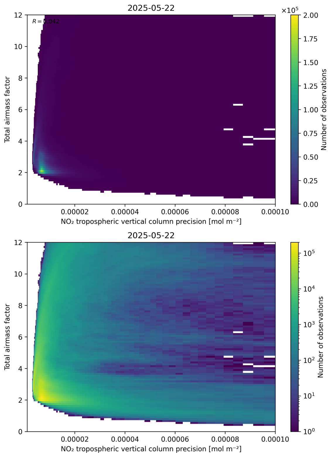
Figure 132: Scatter density plot of “NO 2 tropospheric vertical column precision” against “Total air mass factor” for 2025-05-21 to 2025-05-23.
