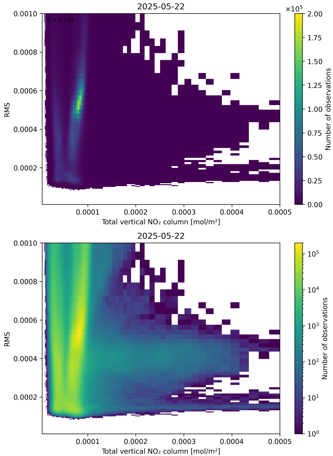
Figure 120: Scatter density plot of “Total vertical NO 2 column” against “RMS” for 2025-05-21 to 2025-05-23.
