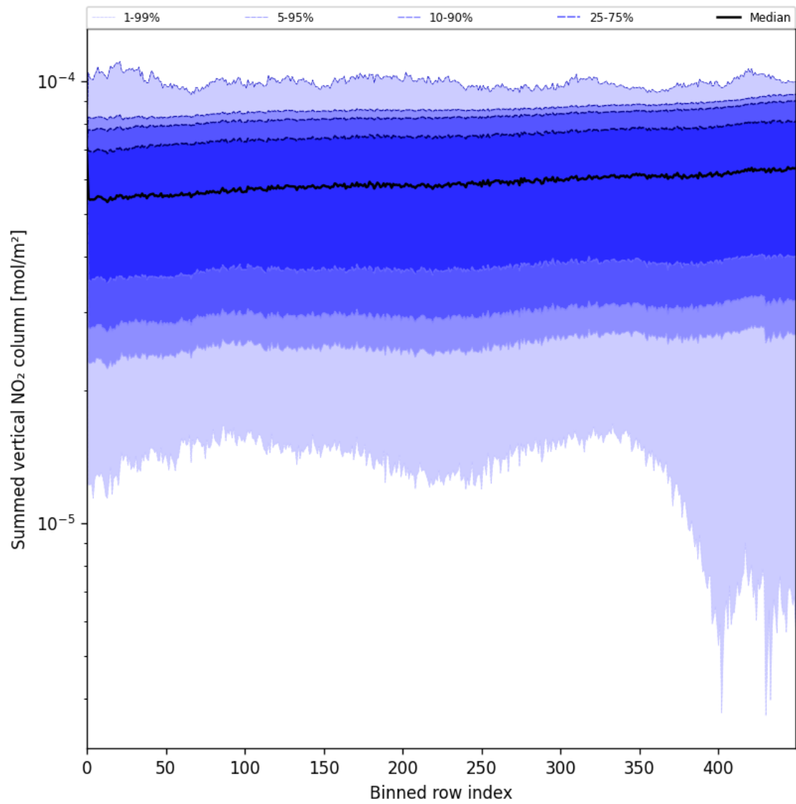
Figure 57: Along track statistics of “Summed vertical NO 2 column” for 2025-05-21 to 2025-05-23
