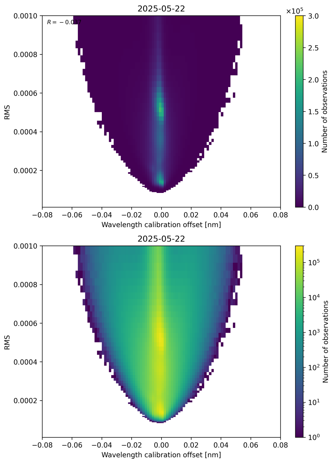
Figure 181: Scatter density plot of “Wavelength calibration offset” against “RMS” for 2025-05-21 to 2025-05-23.
