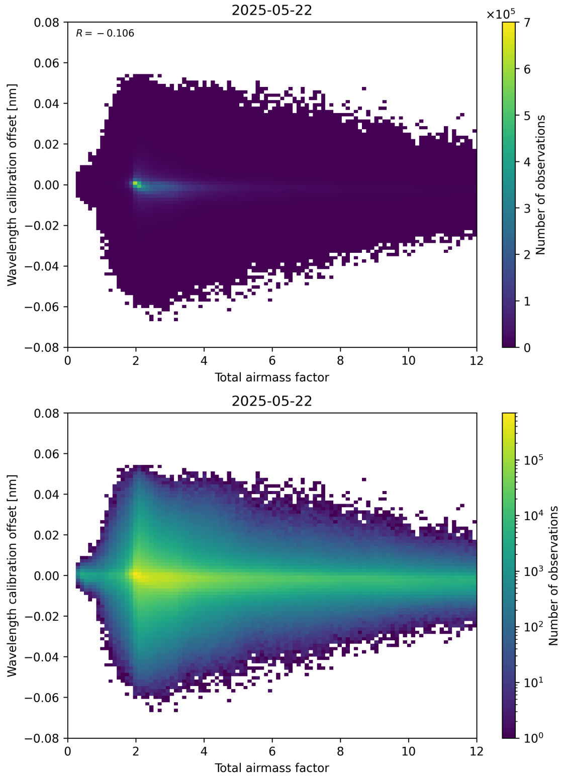
Figure 70: Scatter density plot of “Total airmass factor” against “Wavelength calibration offset” for 2025-05-21 to 2025-05-23.
