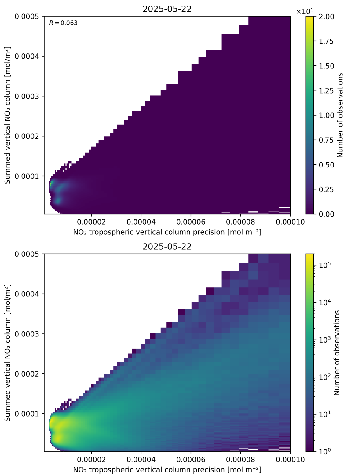
Figure 136: Scatter density plot of “NO 2 tropospheric vertical column precision” against “Summed vertical NO 2 column” for 2025-05-21 to 2025-05-23.
