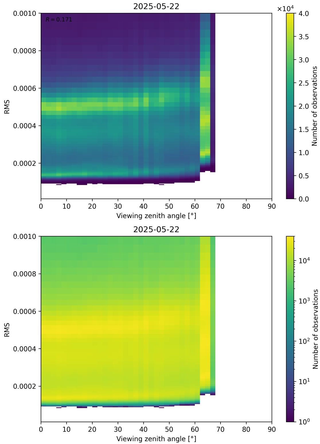
Figure 171: Scatter density plot of “Viewing zenith angle” against “RMS” for 2025-05-21 to 2025-05-23.
