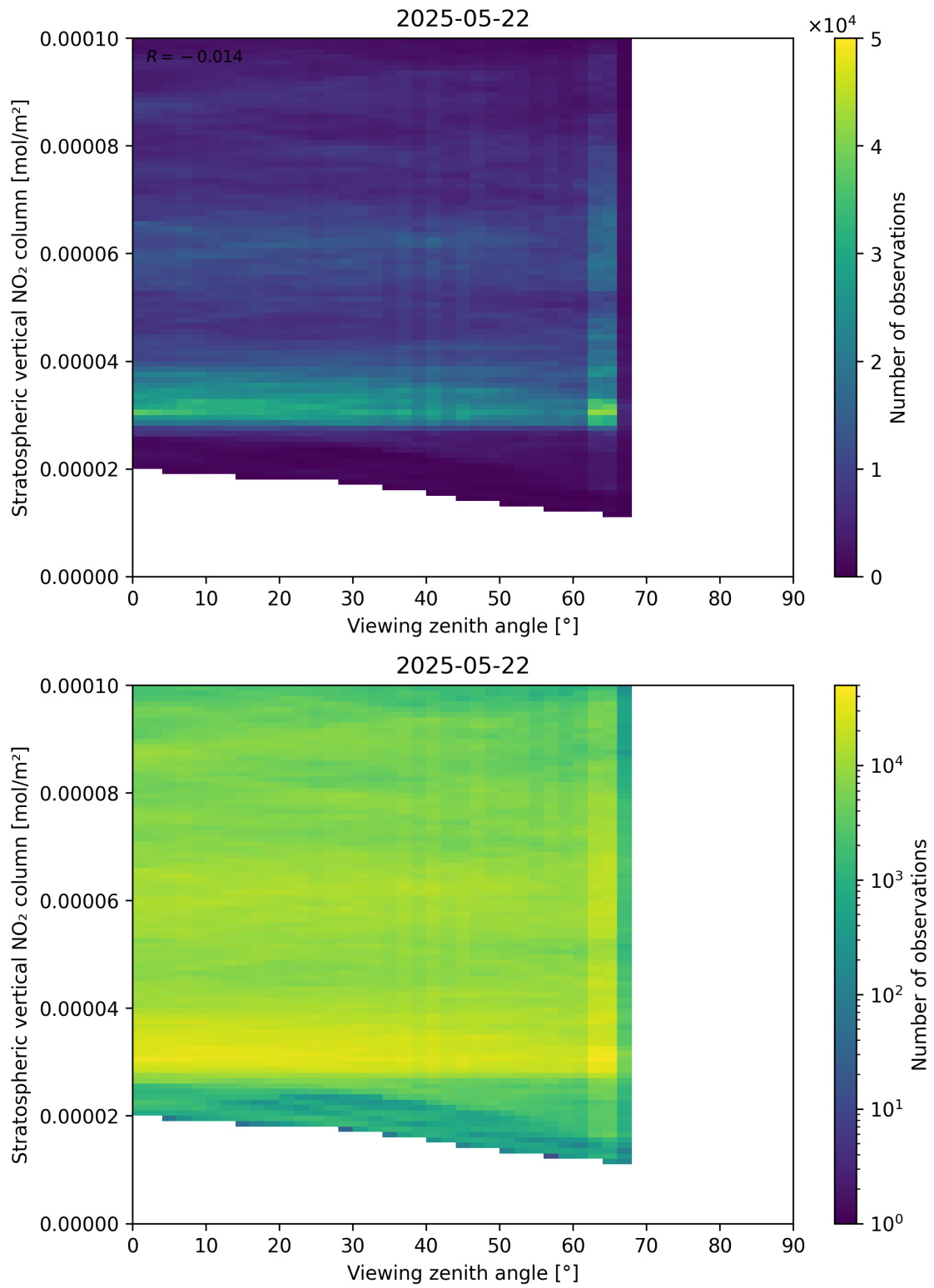
Figure 164: Scatter density plot of “Viewing zenith angle” against “Stratospheric vertical NO 2 column” for 2025-05-21 to 2025-05-23.
