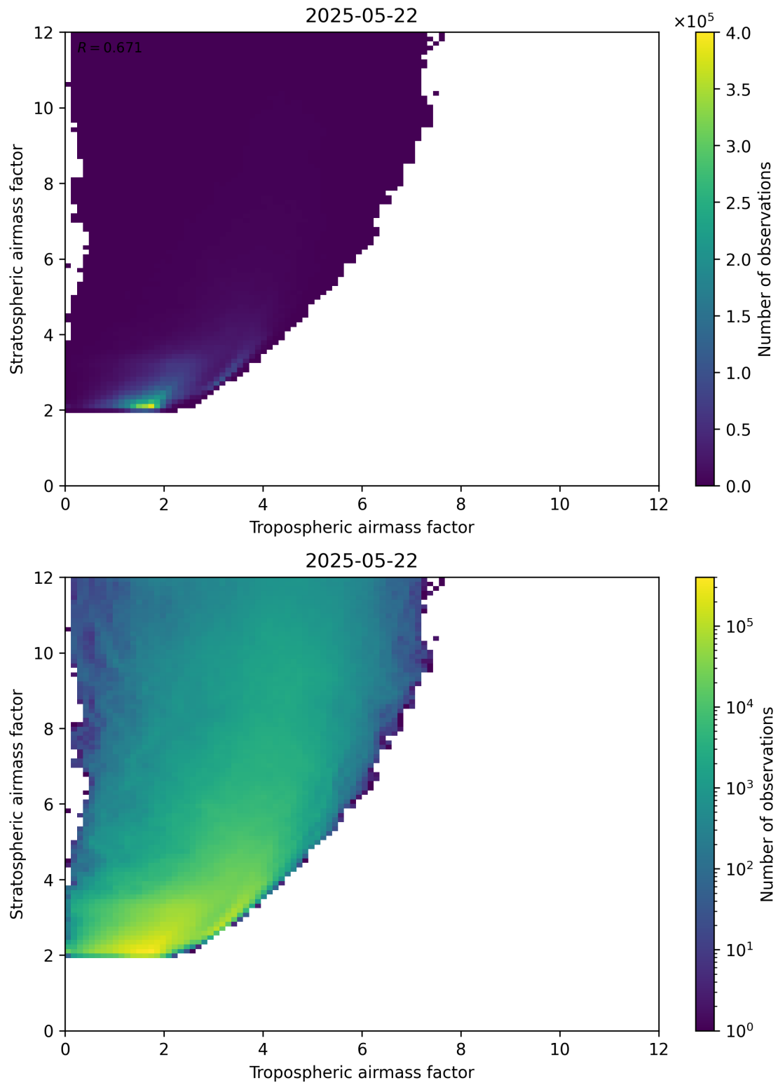
Figure 71: Scatter density plot of “Tropospheric airmass factor” against “Stratospheric airmass factor” for 2025-05-21 to 2025-05-23.
