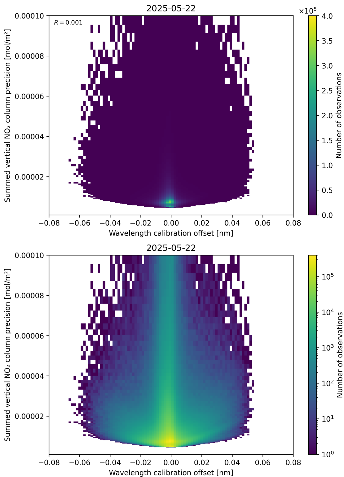
Figure 178: Scatter density plot of “Wavelength calibration offset” against “Summed vertical NO 2 column precision” for 2025-05-21 to 2025-05-23.
