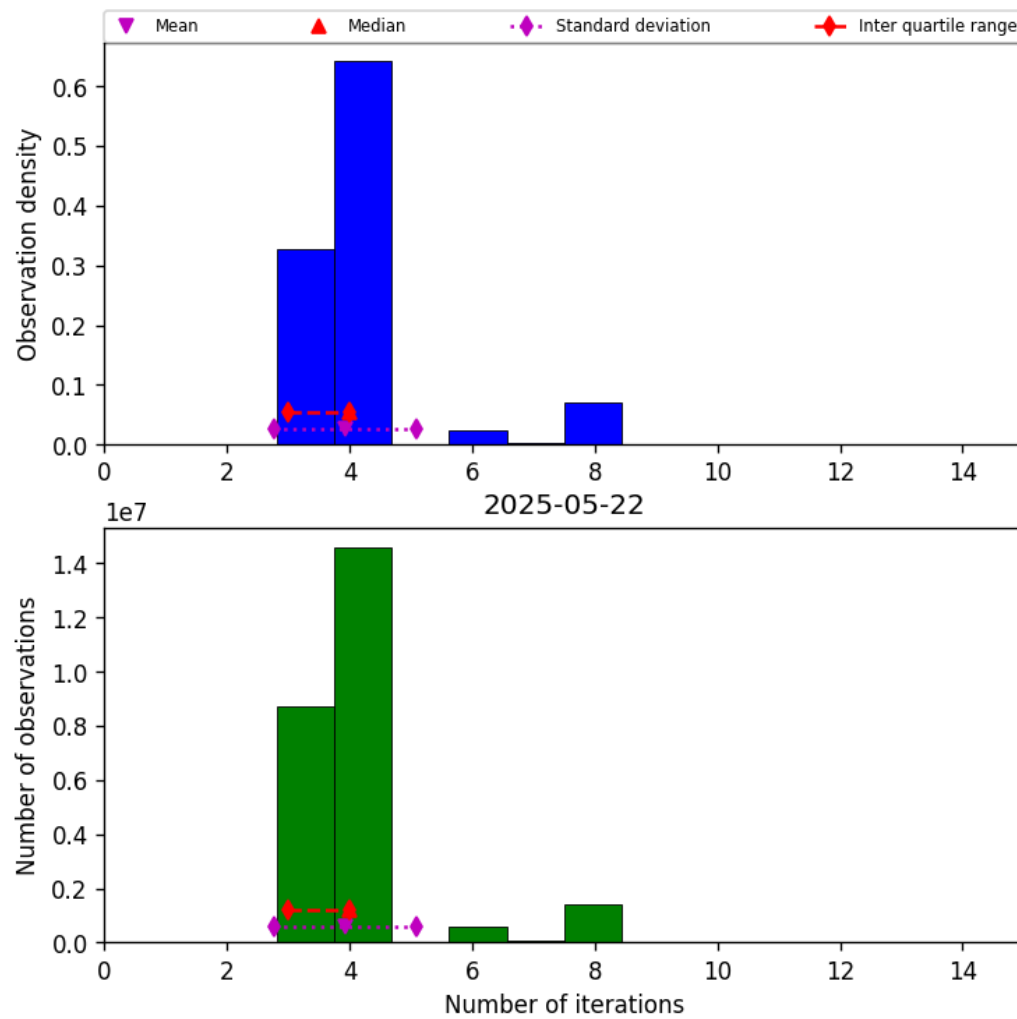
Figure 34: Histogram of “Number of iterations” for 2025-05-21 to 2025-05-23
