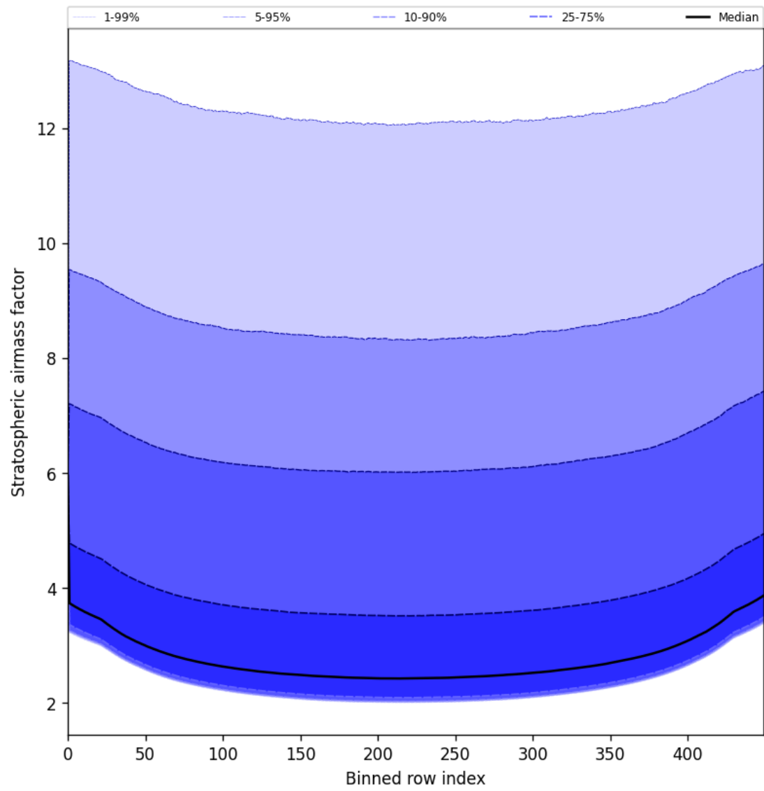
Figure 61: Along track statistics of “Stratospheric airmass factor” for 2025-05-21 to 2025-05-23
