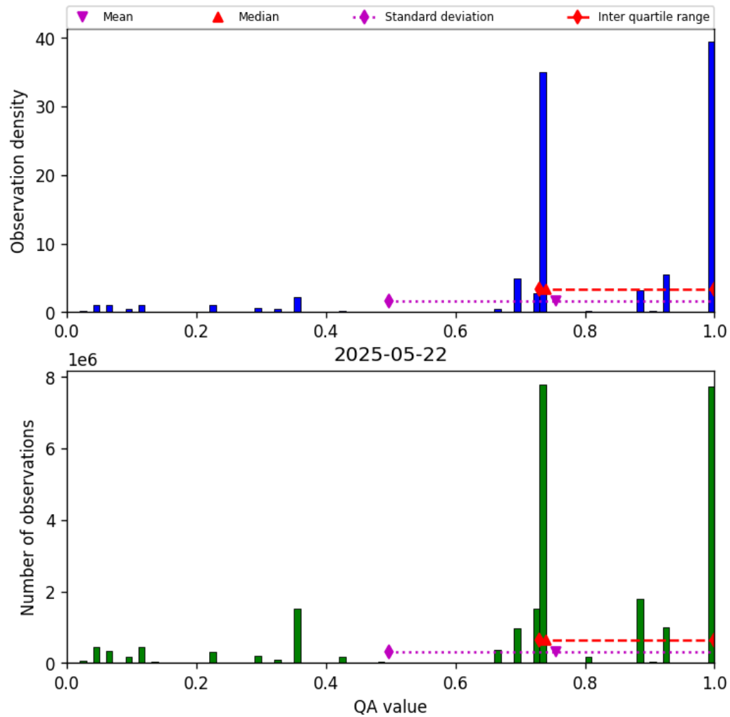
Figure 28: Histogram of “QA value” for 2025-05-21 to 2025-05-23
