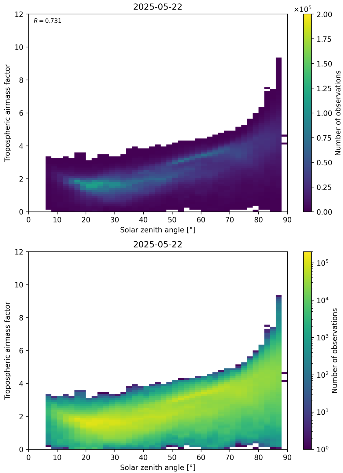
Figure 147: Scatter density plot of “Solar zenith angle” against “Tropospheric airmass factor” for 2025-05-21 to 2025-05-23.
