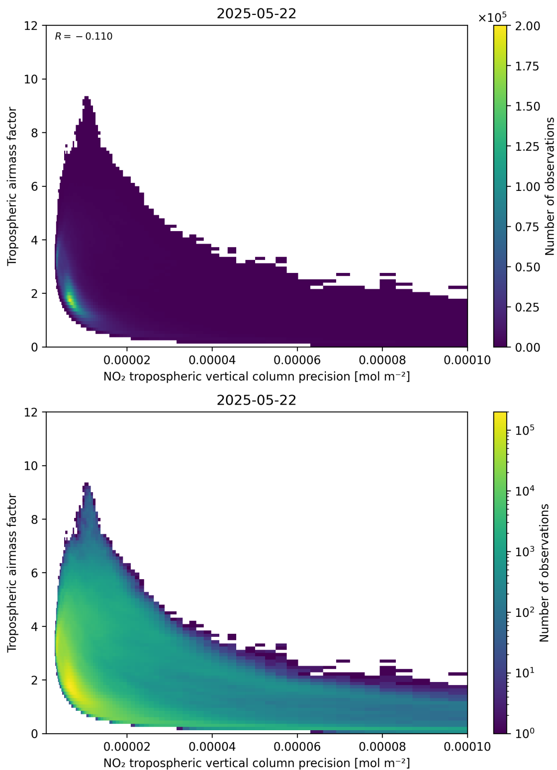
Figure 133: Scatter density plot of “NO 2 tropospheric vertical column precision” against “Tropospheric airmass factor” for 2025-05-21 to 2025-05-23.
