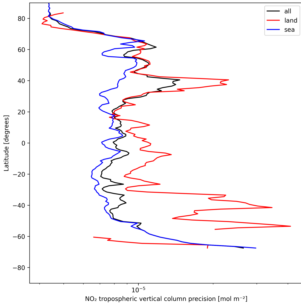
Figure 13: Zonal average of “NO 2 tropospheric vertical column precision” for 2025-05-21 to 2025-05-23.
