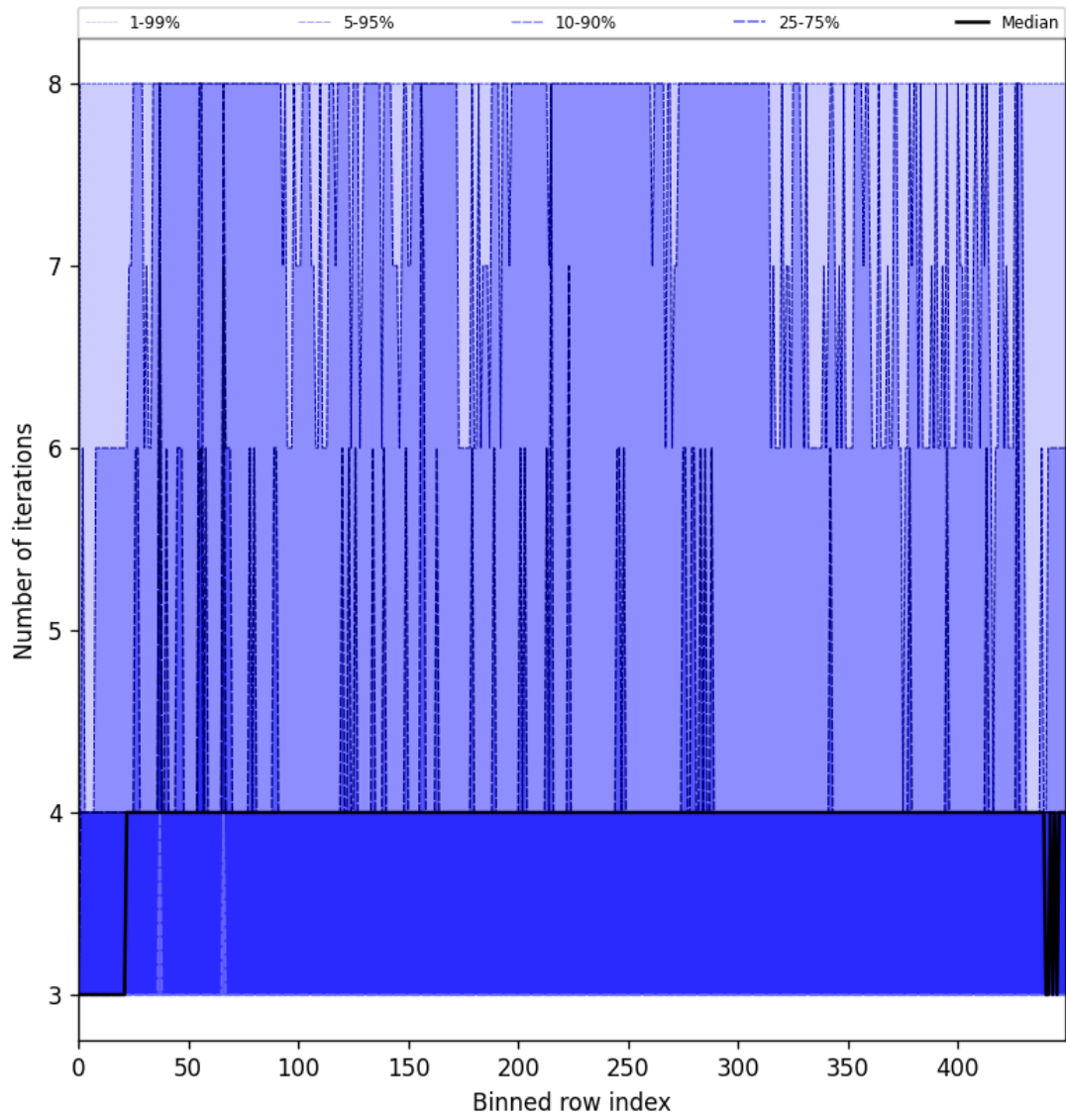
Figure 51: Along track statistics of “Number of iterations” for 2025-05-21 to 2025-05-23
