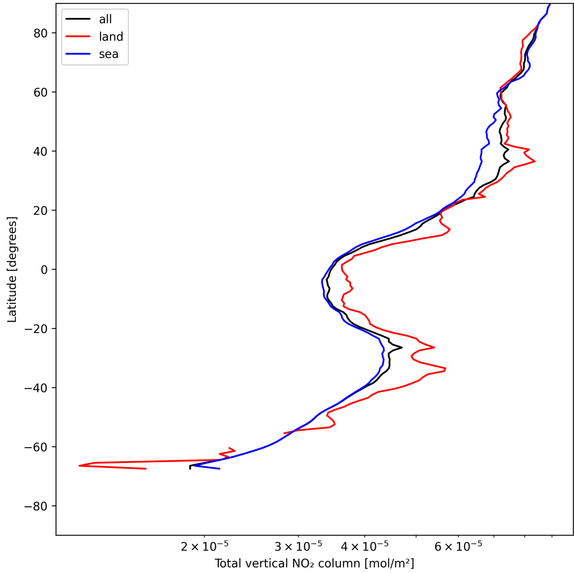
Figure 21: Zonal average of “Total vertical NO 2 column” for 2025-05-21 to 2025-05-23.
