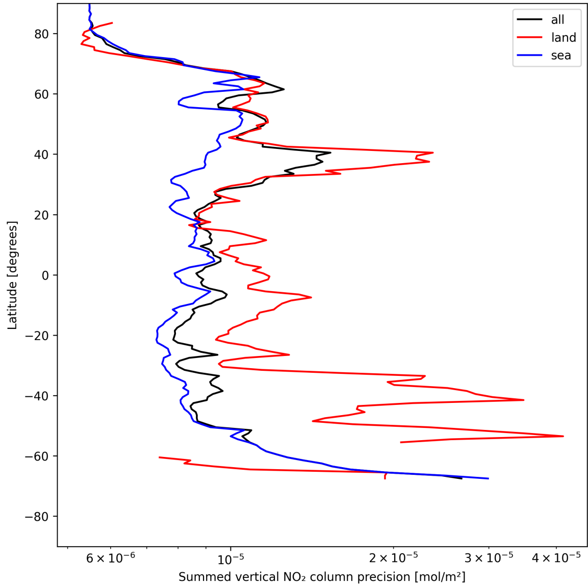
Figure 24: Zonal average of “Summed vertical NO 2 column precision” for 2025-05-21 to 2025-05-23.
