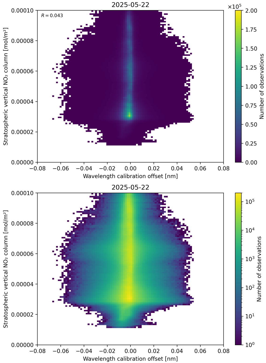
Figure 176: Scatter density plot of “Wavelength calibration offset” against “Stratospheric vertical NO 2 column” for 2025-05-21 to 2025-05-23.
