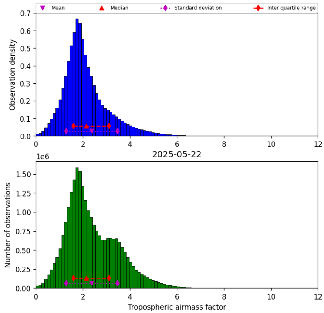
Figure 31: Histogram of “Tropospheric airmass factor” for 2025-05-21 to 2025-05-23
