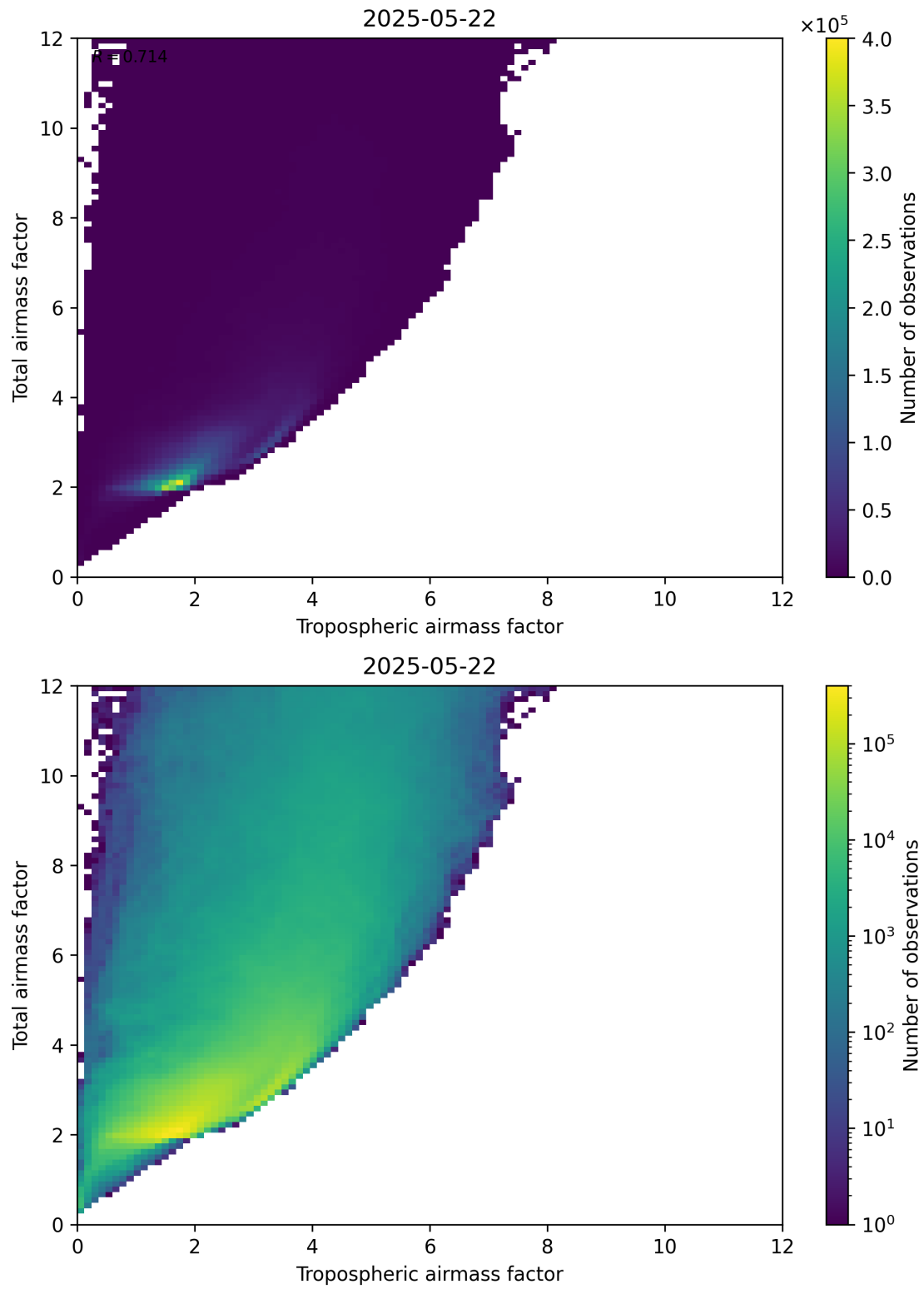
Figure 72: Scatter density plot of “Tropospheric airmass factor” against “Total airmass factor” for 2025-05-21 to 2025-05-23.
