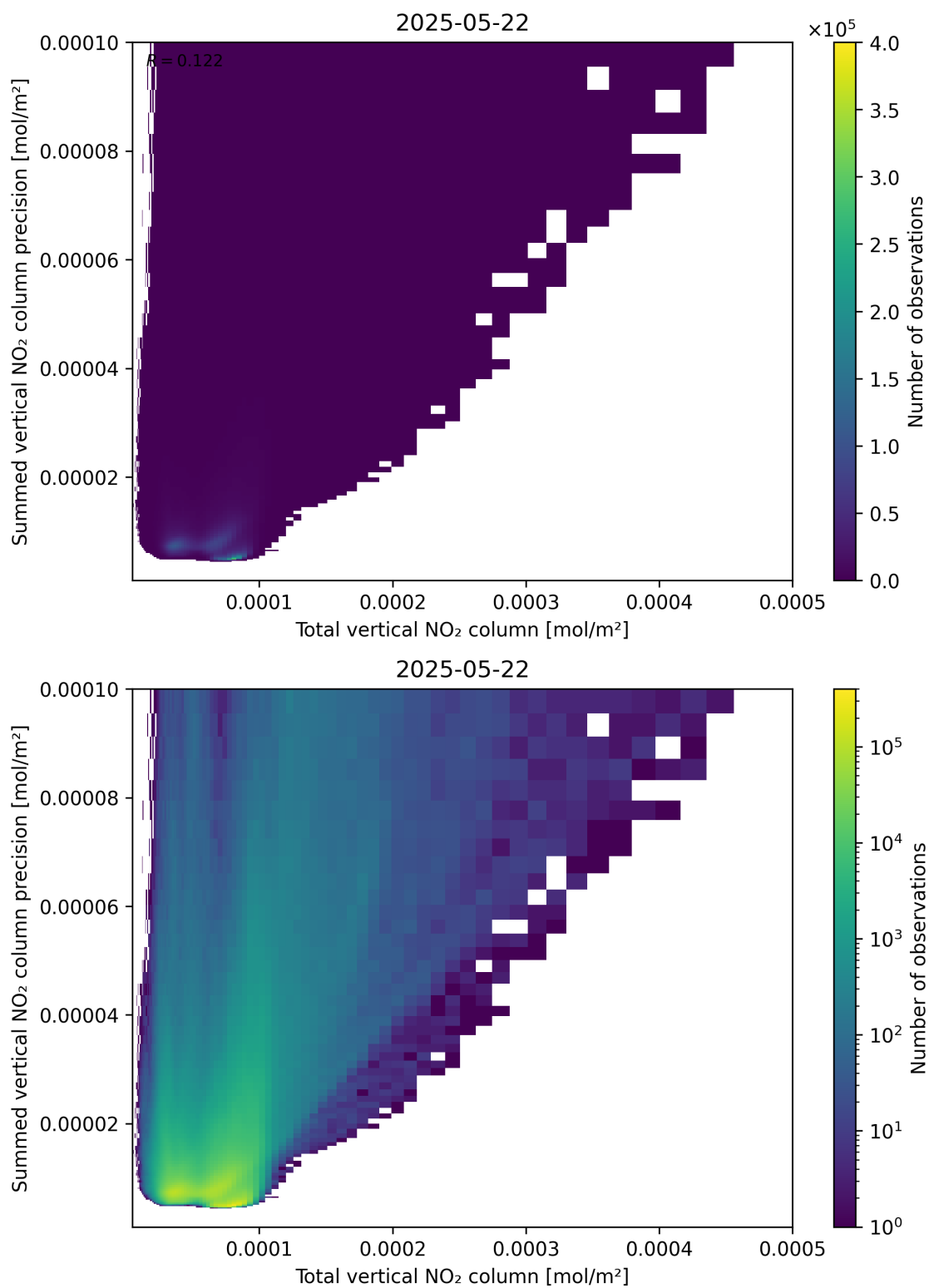
Figure 113: Scatter density plot of “Total vertical NO 2 column” against “Summed vertical NO 2 column precision” for 2025-05-21 to 2025-05-23.
