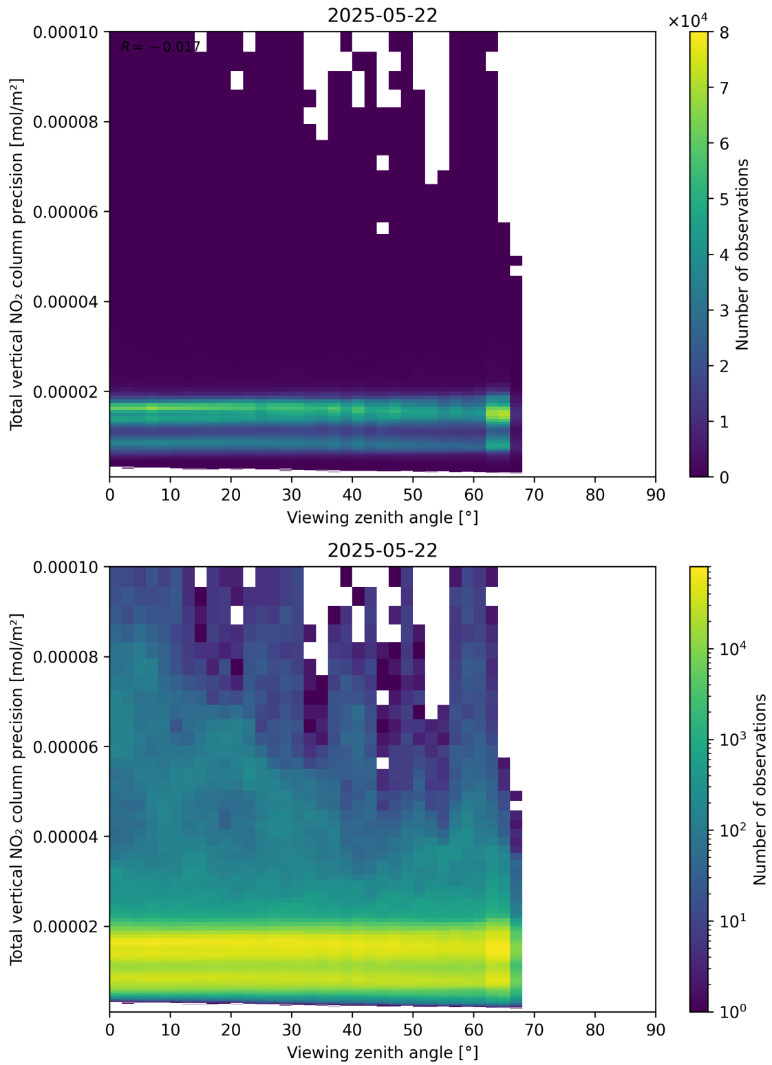
Figure 168: Scatter density plot of “Viewing zenith angle” against “Total vertical NO 2 column precision” for 2025-05-21 to 2025-05-23.
