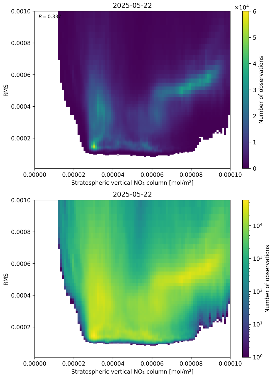
Figure 102: Scatter density plot of “Stratospheric vertical NO 2 column” against “RMS” for 2025-05-21 to 2025-05-23.
