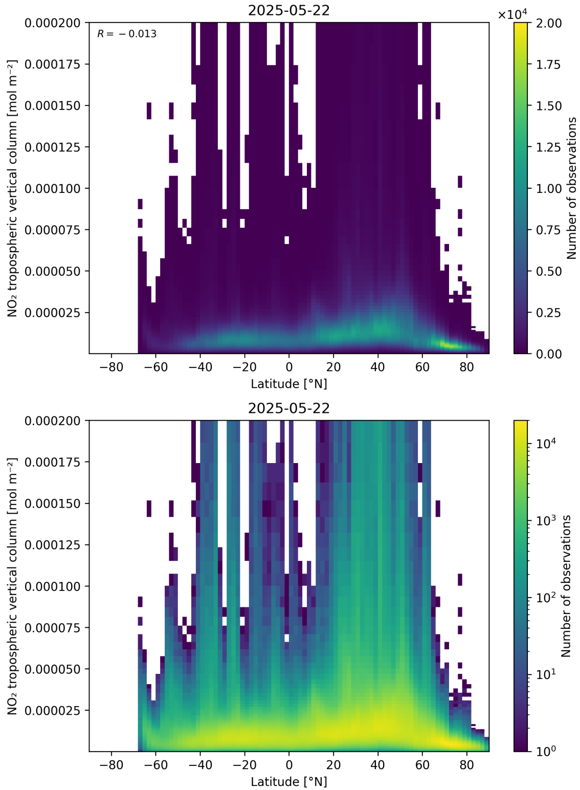
Figure 92: Scatter density plot of “Latitude” against “NO 2 tropospheric vertical column” for 2025-05-21 to 2025-05-23.
