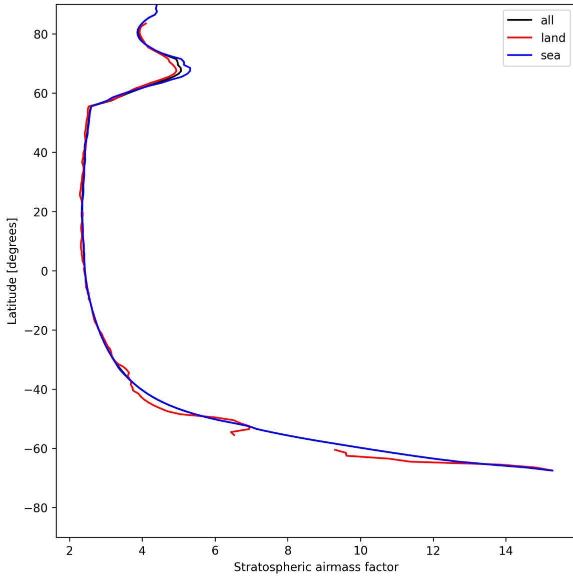
Figure 27: Zonal average of “Stratospheric airmass factor” for 2025-05-21 to 2025-05-23.
