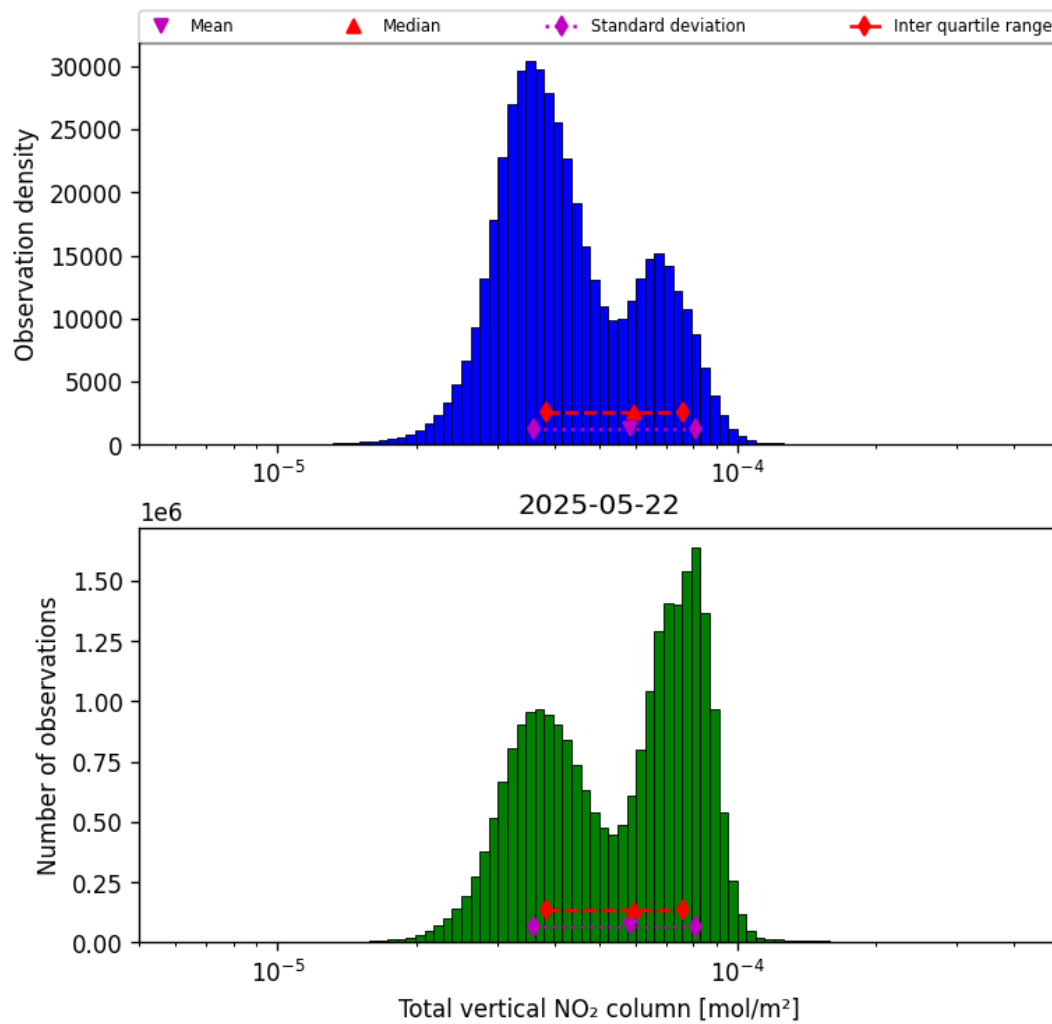
Figure 38: Histogram of "Total vertical NO 2 column" for 2025-05-21 to 2025-05-23
