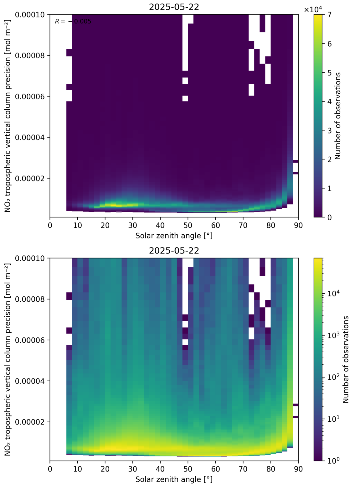
Figure 156: Scatter density plot of “Solar zenith angle” against “NO 2 tropospheric vertical column precision” for 2025-05-21 to 2025-05-23.
