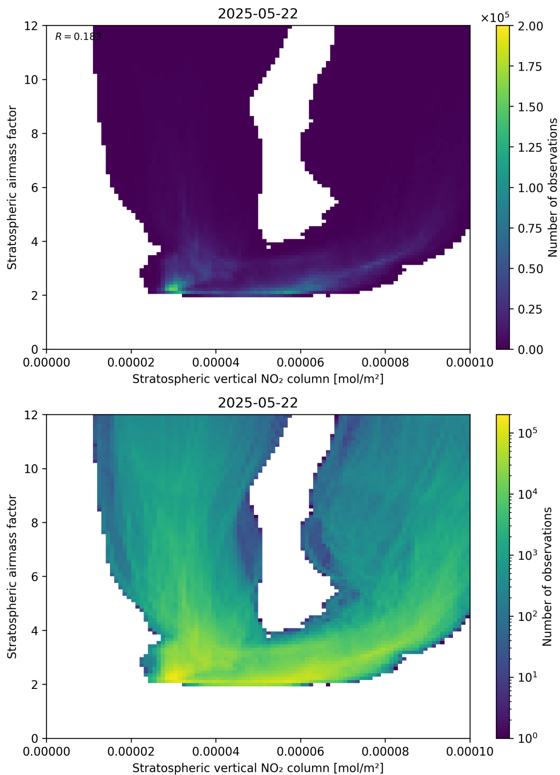
Figure 96: Scatter density plot of “Stratospheric vertical NO 2 column” against “Stratospheric airmass factor” for 2025-05-21 to 2025-05-23.
