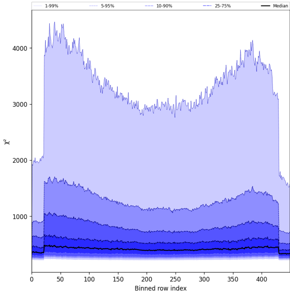
Figure 59: Along track statistics of “ \chi^2 ” for 2025-05-21 to 2025-05-23
