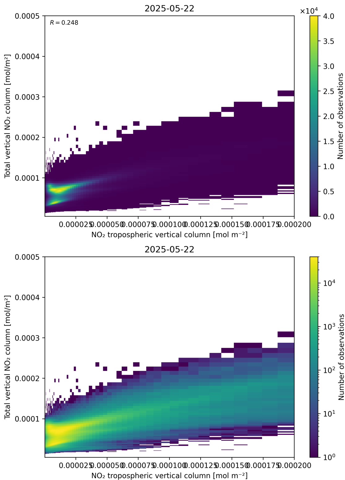
Figure 128: Scatter density plot of “NO 2 tropospheric vertical column” against “Total vertical NO 2 column” for 2025-05-21 to 2025-05-23.
