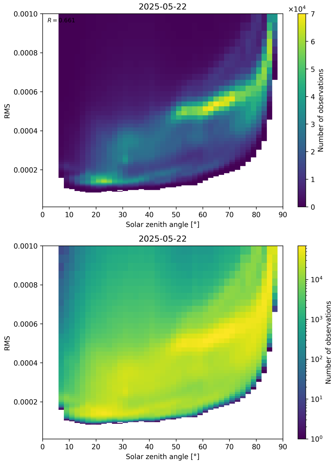
Figure 157: Scatter density plot of “Solar zenith angle” against “RMS” for 2025-05-21 to 2025-05-23.
