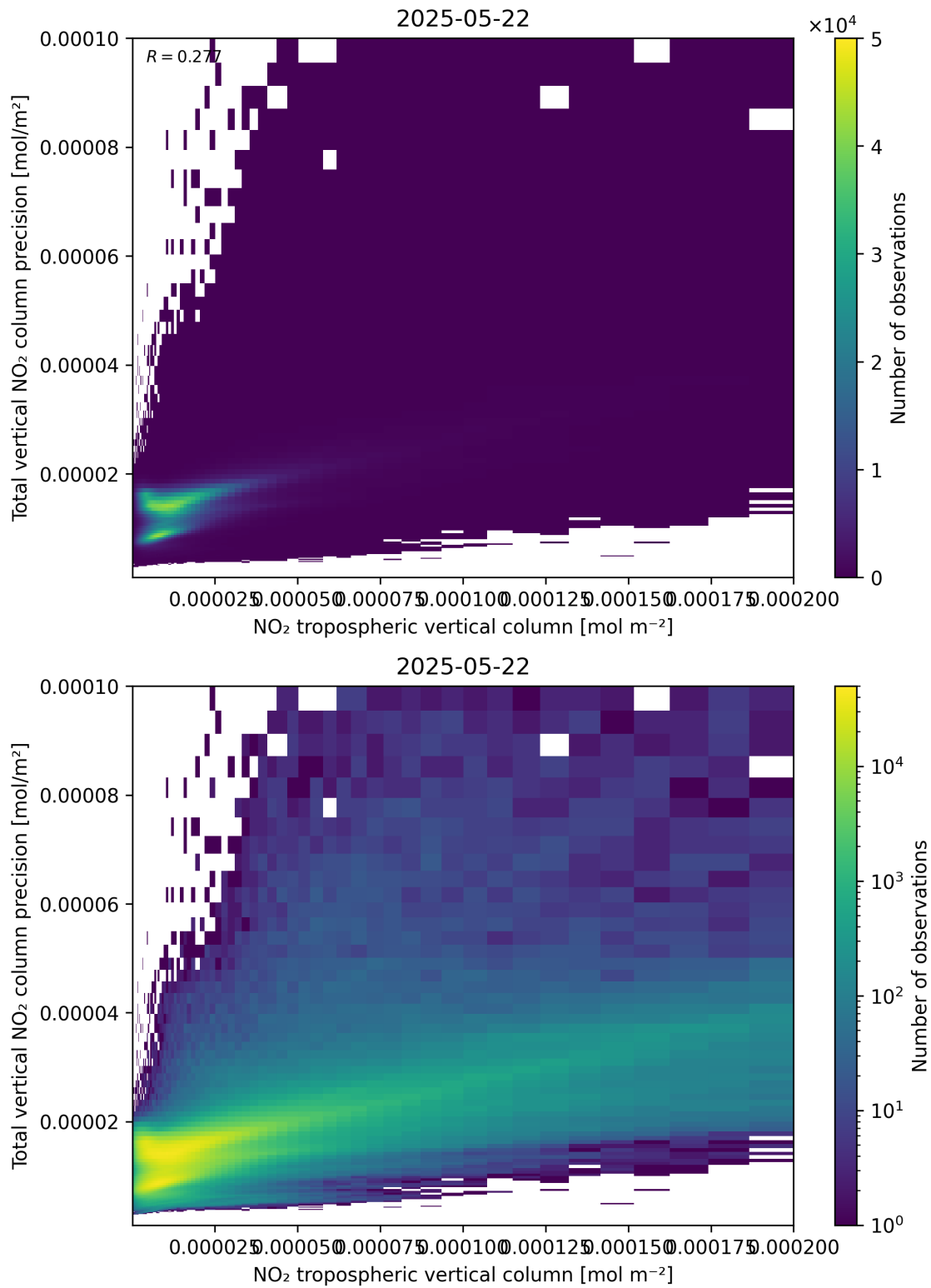
Figure 129: Scatter density plot of “NO 2 tropospheric vertical column” against “Total vertical NO 2 column precision” for 2025-05-21 to 2025-05-23.
