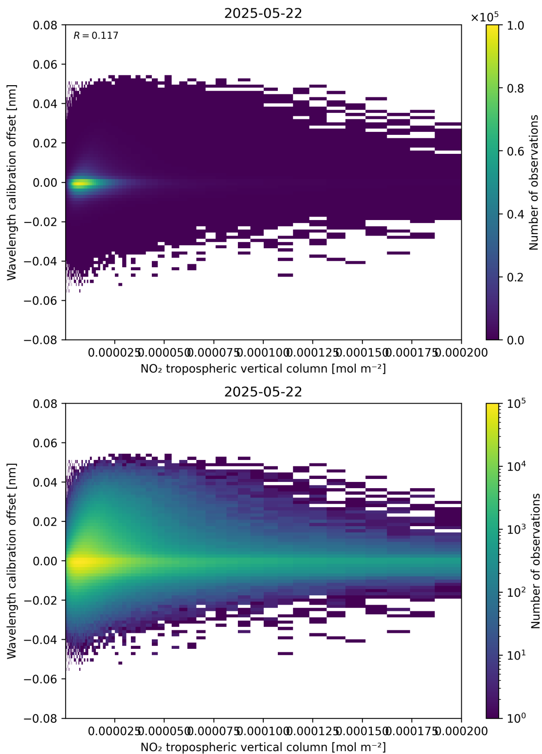
Figure 143: Scatter density plot of “NO 2 tropospheric vertical column” against “Wavelength calibration offset” for 2025-05-21 to 2025-05-23.
