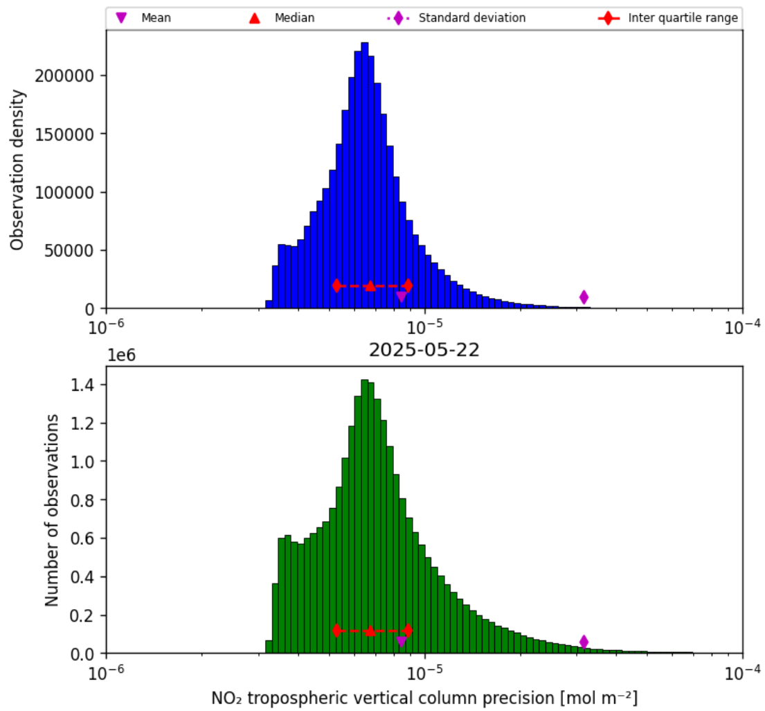
Figure 30: Histogram of “NO 2 tropospheric vertical column precision” for 2025-05-21 to 2025-05-23
