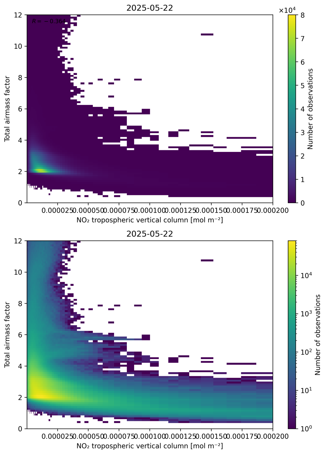
Figure 122: Scatter density plot of “NO 2 tropospheric vertical column” against “Total air mass factor” for 2025-05-21 to 2025-05-23.
