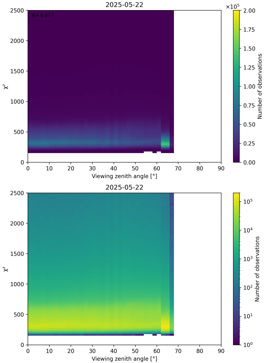
Figure 162: Scatter density plot of “Viewing zenith angle” against “ \chi^2 ” for 2025-05-21 to 2025-05-23.
