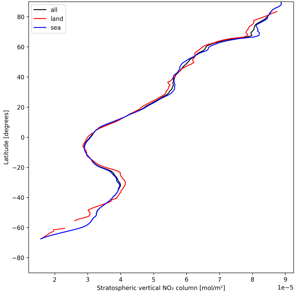
Figure 19: Zonal average of “Stratospheric vertical NO 2 column” for 2025-05-21 to 2025-05-23.
