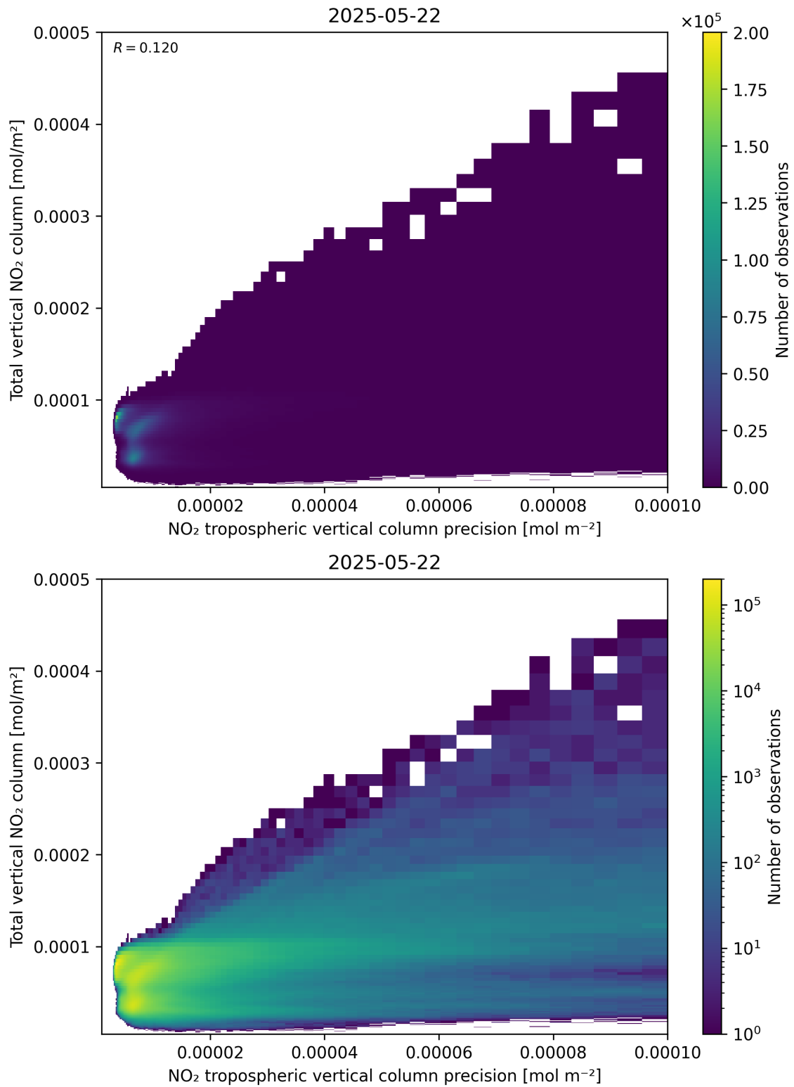
Figure 138: Scatter density plot of “NO 2 tropospheric vertical column precision” against “Total vertical NO 2 column” for 2025-05-21 to 2025-05-23.
