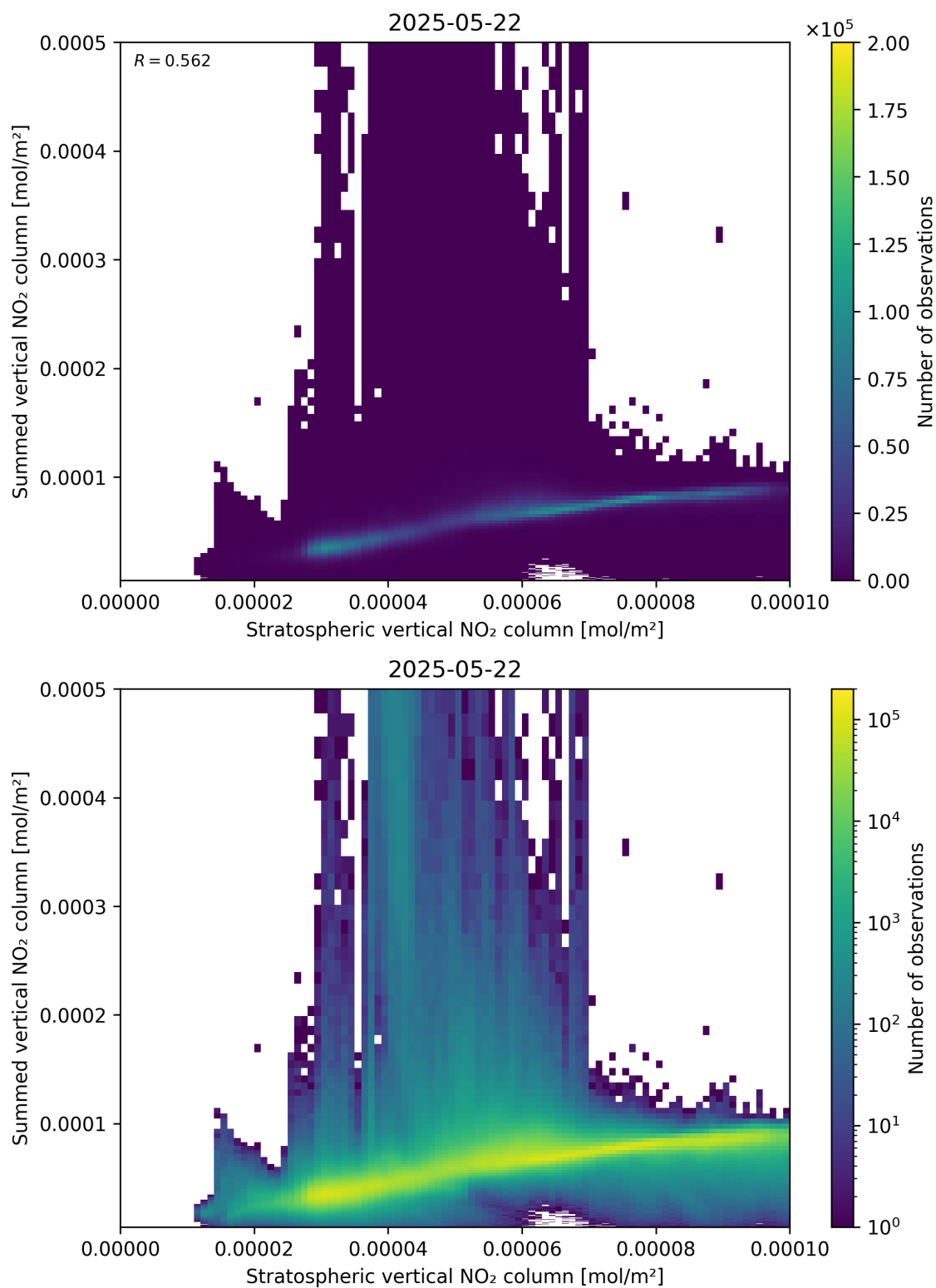
Figure 98: Scatter density plot of “Stratospheric vertical NO 2 column” against “Summed vertical NO 2 column” for 2025-05-21 to 2025-05-23.
