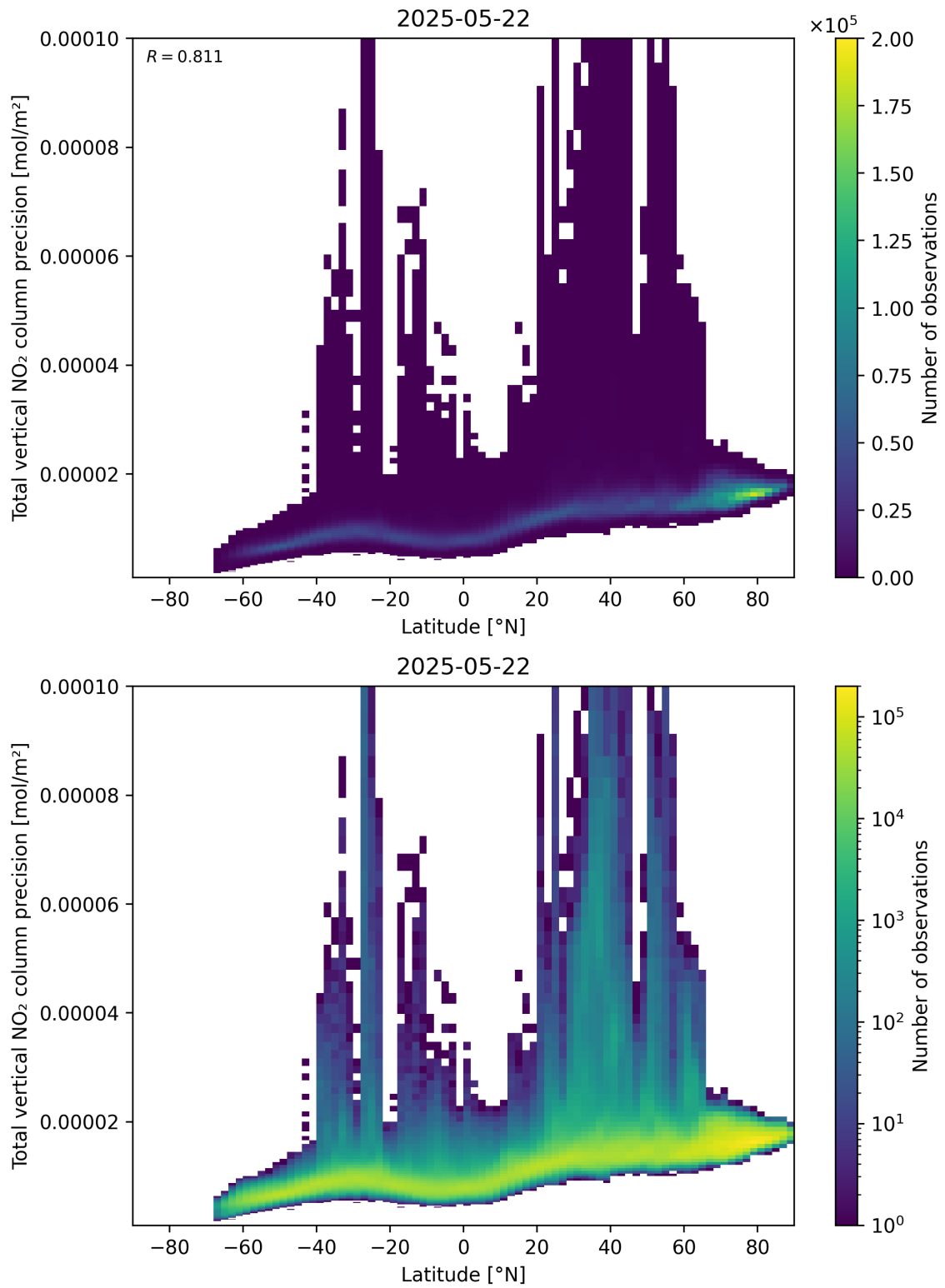
Figure 91: Scatter density plot of “Latitude” against “Total vertical NO 2 column precision” for 2025-05-21 to 2025-05-23.
