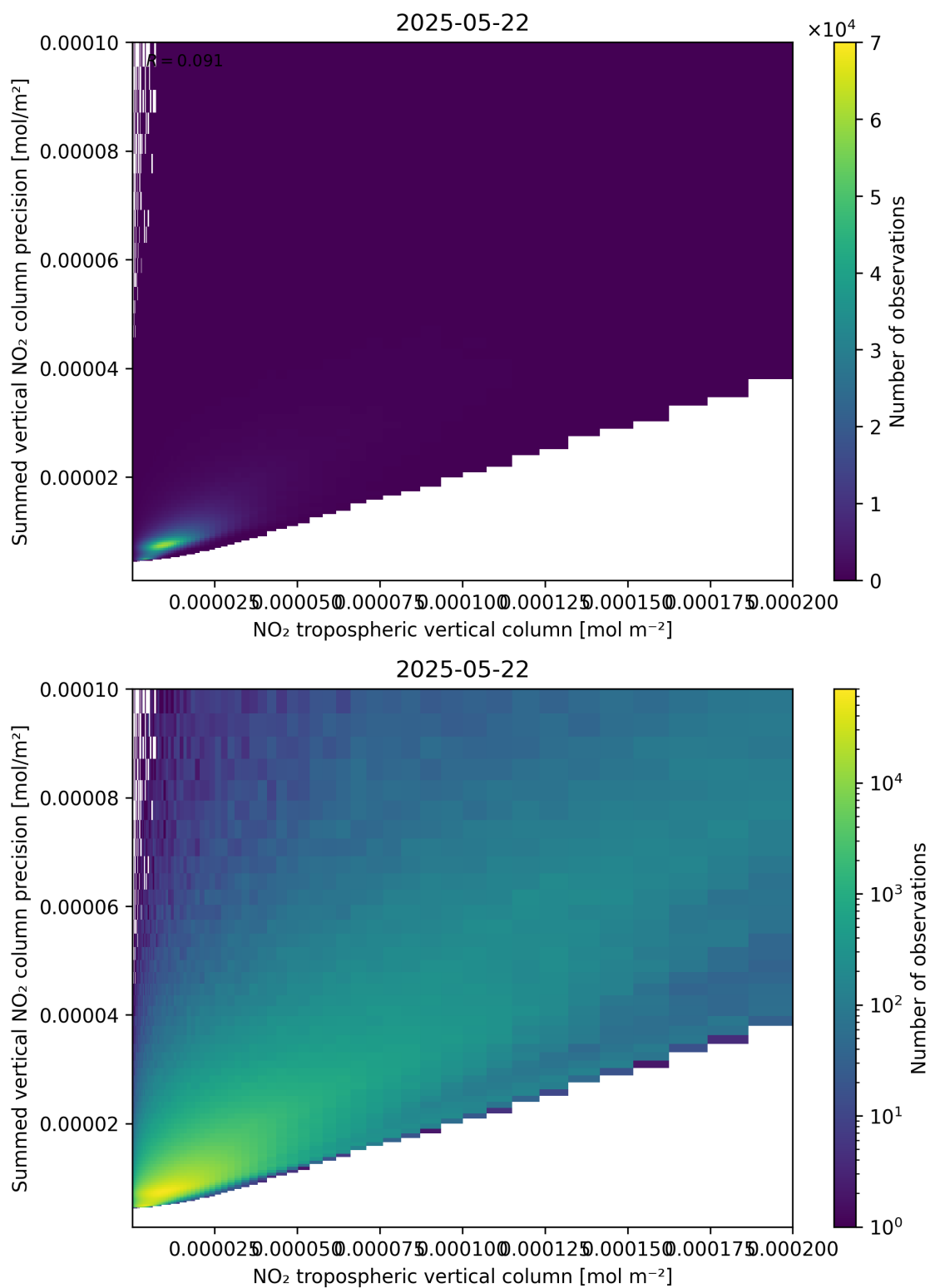
Figure 127: Scatter density plot of “NO 2 tropospheric vertical column” against “Summed vertical NO 2 column precision” for 2025-05-21 to 2025-05-23.
