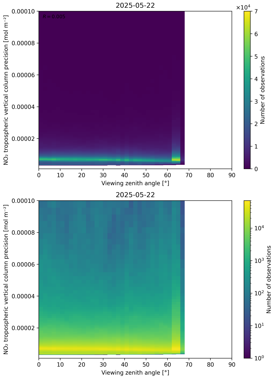
Figure 170: Scatter density plot of “Viewing zenith angle” against “NO 2 tropospheric vertical column precision” for 2025-05-21 to 2025-05-23.
