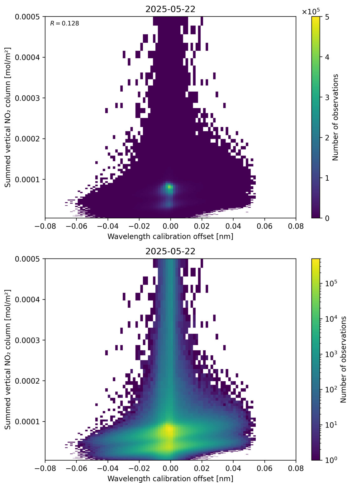
Figure 177: Scatter density plot of “Wavelength calibration offset” against “Summed vertical NO 2 column” for 2025-05-21 to 2025-05-23.
