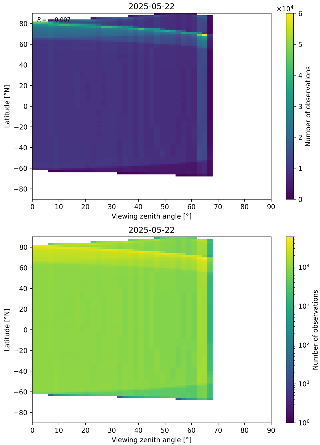
Figure 163: Scatter density plot of “Viewing zenith angle” against “Latitude” for 2025-05-21 to 2025-05-23.
