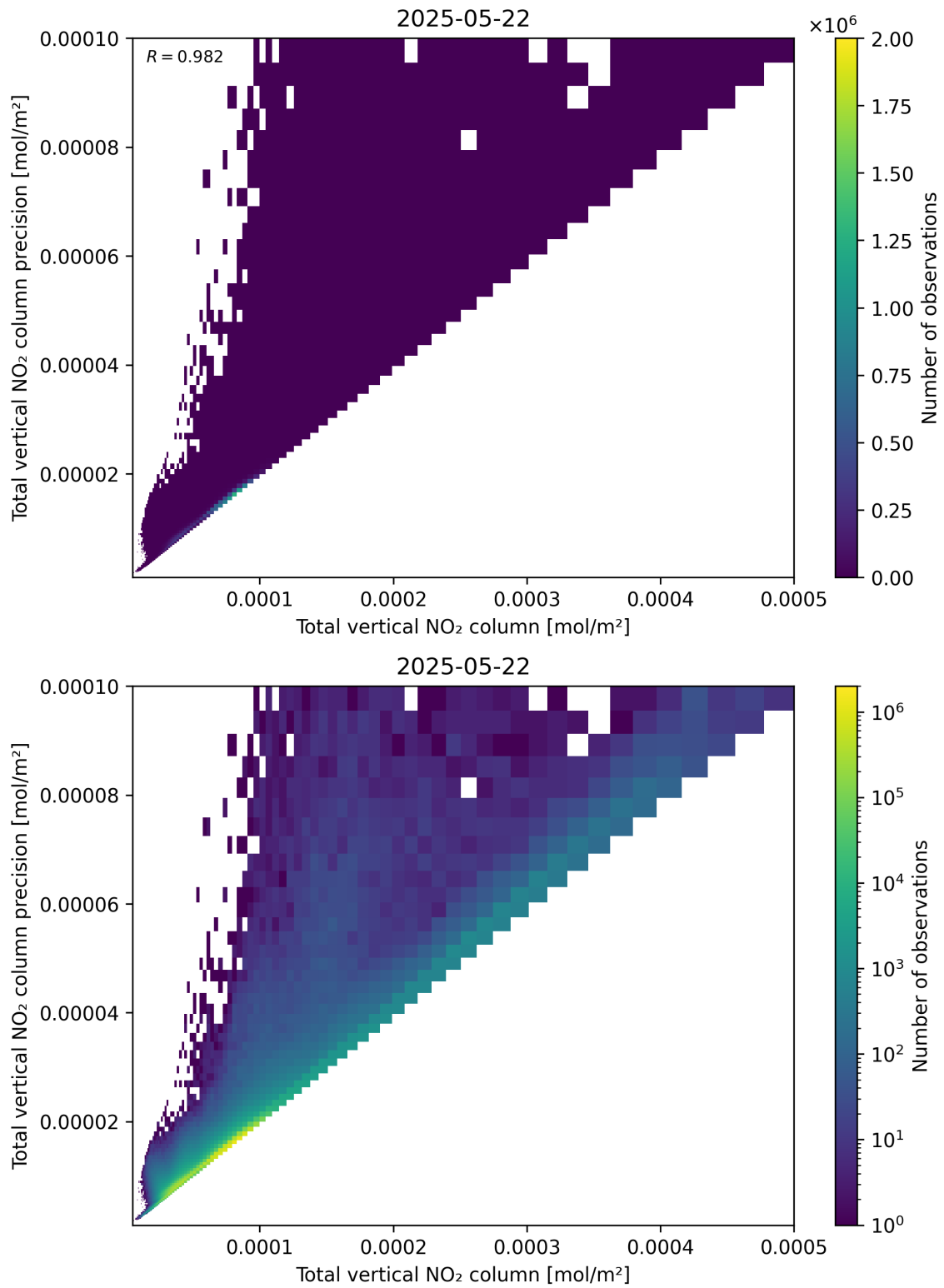
Figure 114: Scatter density plot of “Total vertical NO 2 column” against “Total vertical NO 2 column precision” for 2025-05-21 to 2025-05-23.
