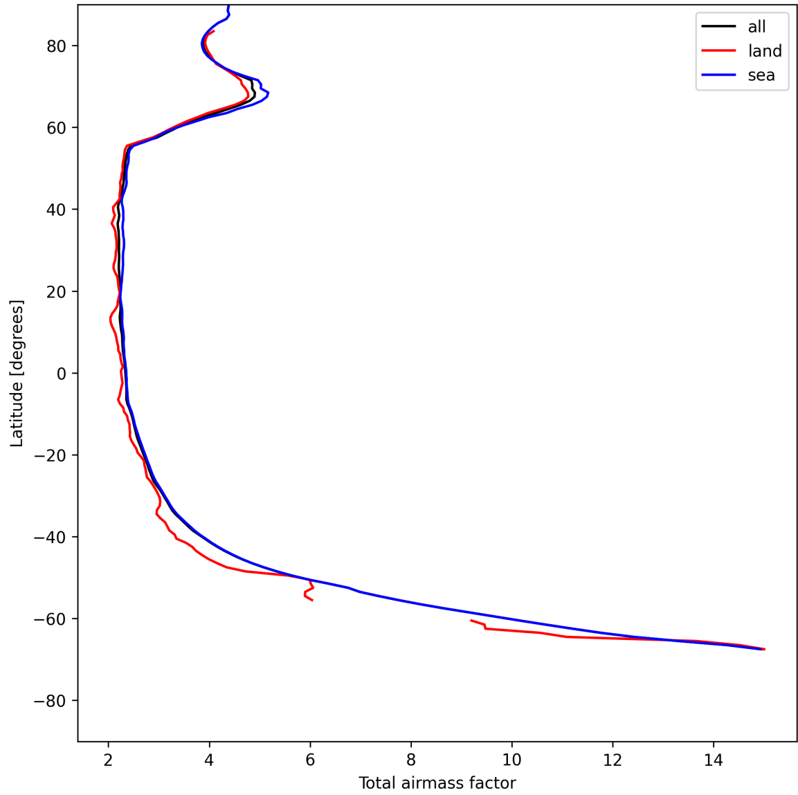
Figure 15: Zonal average of “Total airmass factor” for 2025-05-21 to 2025-05-23.
