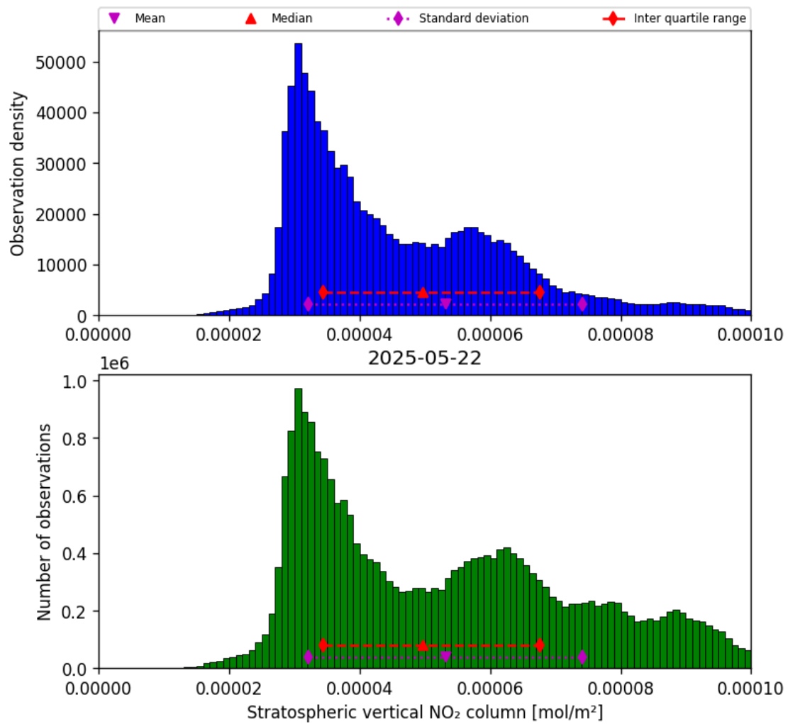
Figure 36: Histogram of “Stratospheric vertical NO 2 column” for 2025-05-21 to 2025-05-23
