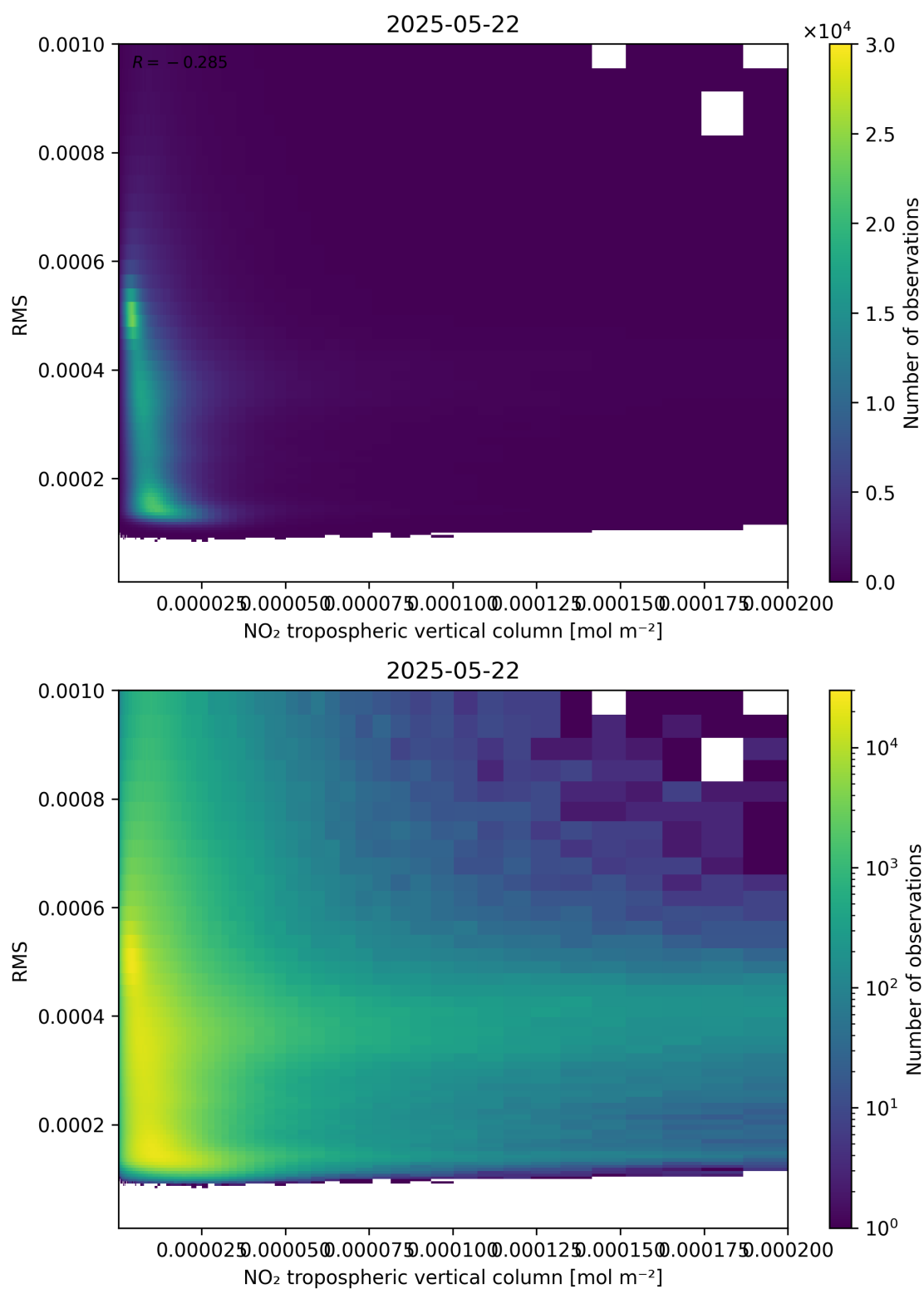
Figure 142: Scatter density plot of “NO 2 tropospheric vertical column” against “RMS” for 2025-05-21 to 2025-05-23.
