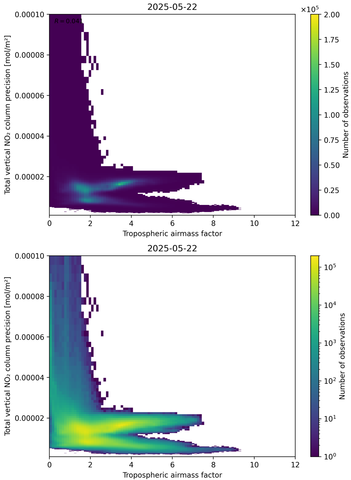
Figure 78: Scatter density plot of “Tropospheric air mass factor” against “Total vertical NO 2 column precision” for 2025-05-21 to 2025-05-23.
