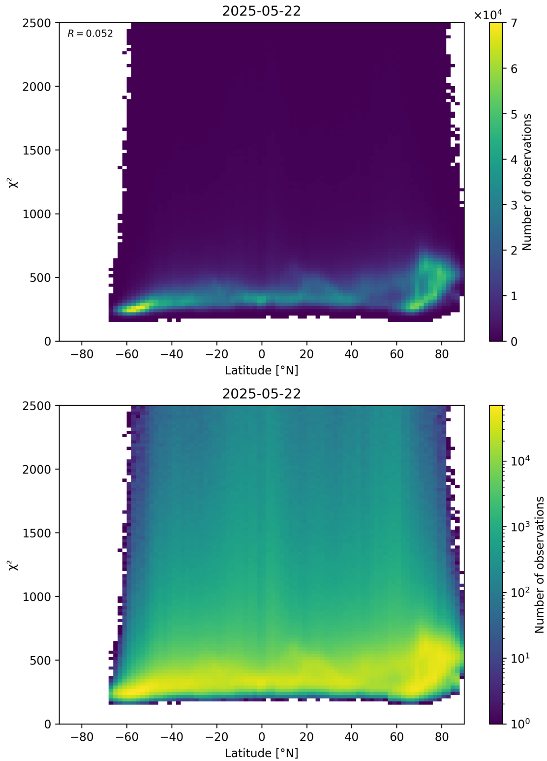
Figure 86: Scatter density plot of “Latitude” against “ \chi^2 ” for 2025-05-21 to 2025-05-23.
