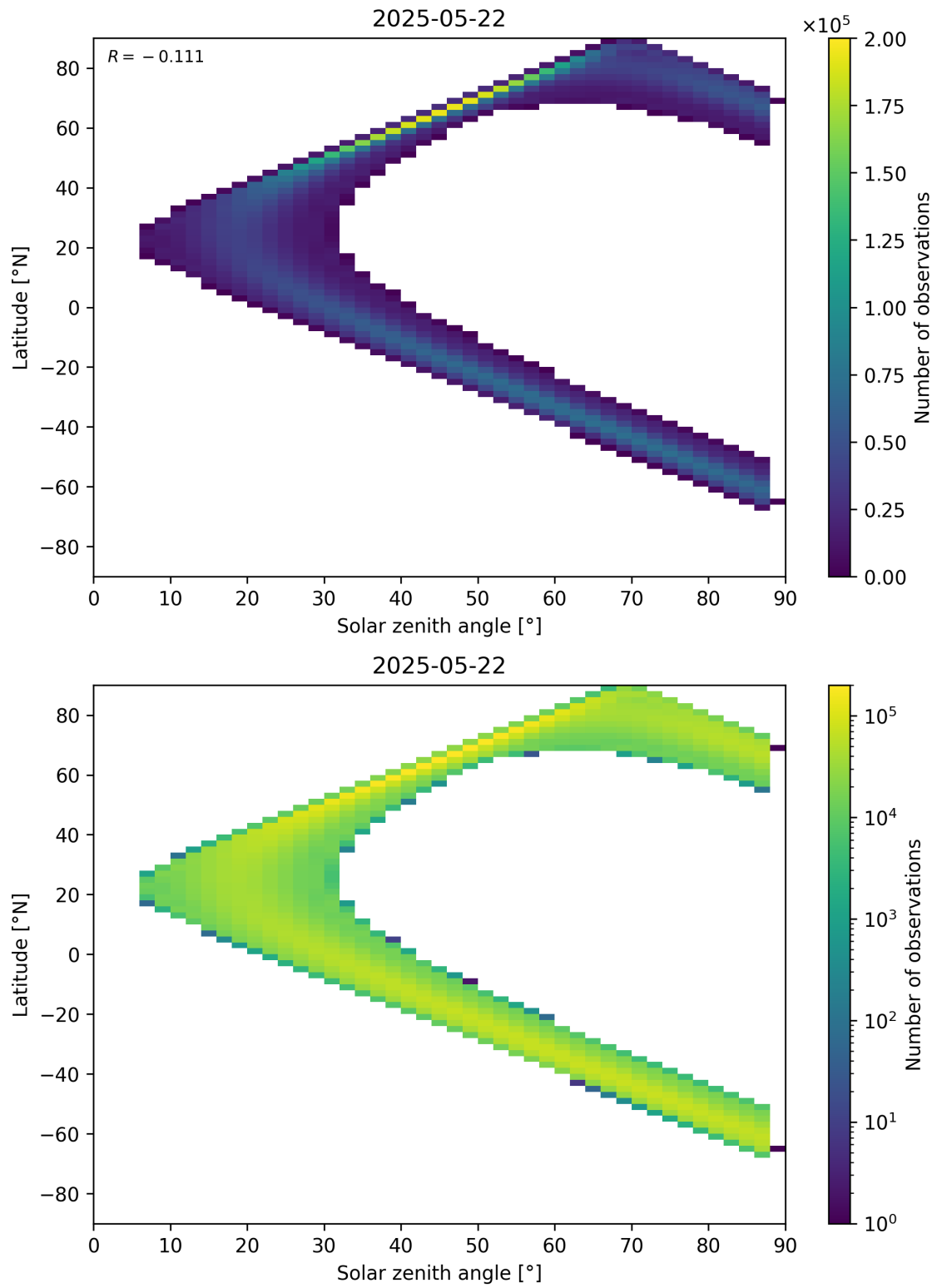
Figure 149: Scatter density plot of “Solar zenith angle” against “Latitude” for 2025-05-21 to 2025-05-23.
