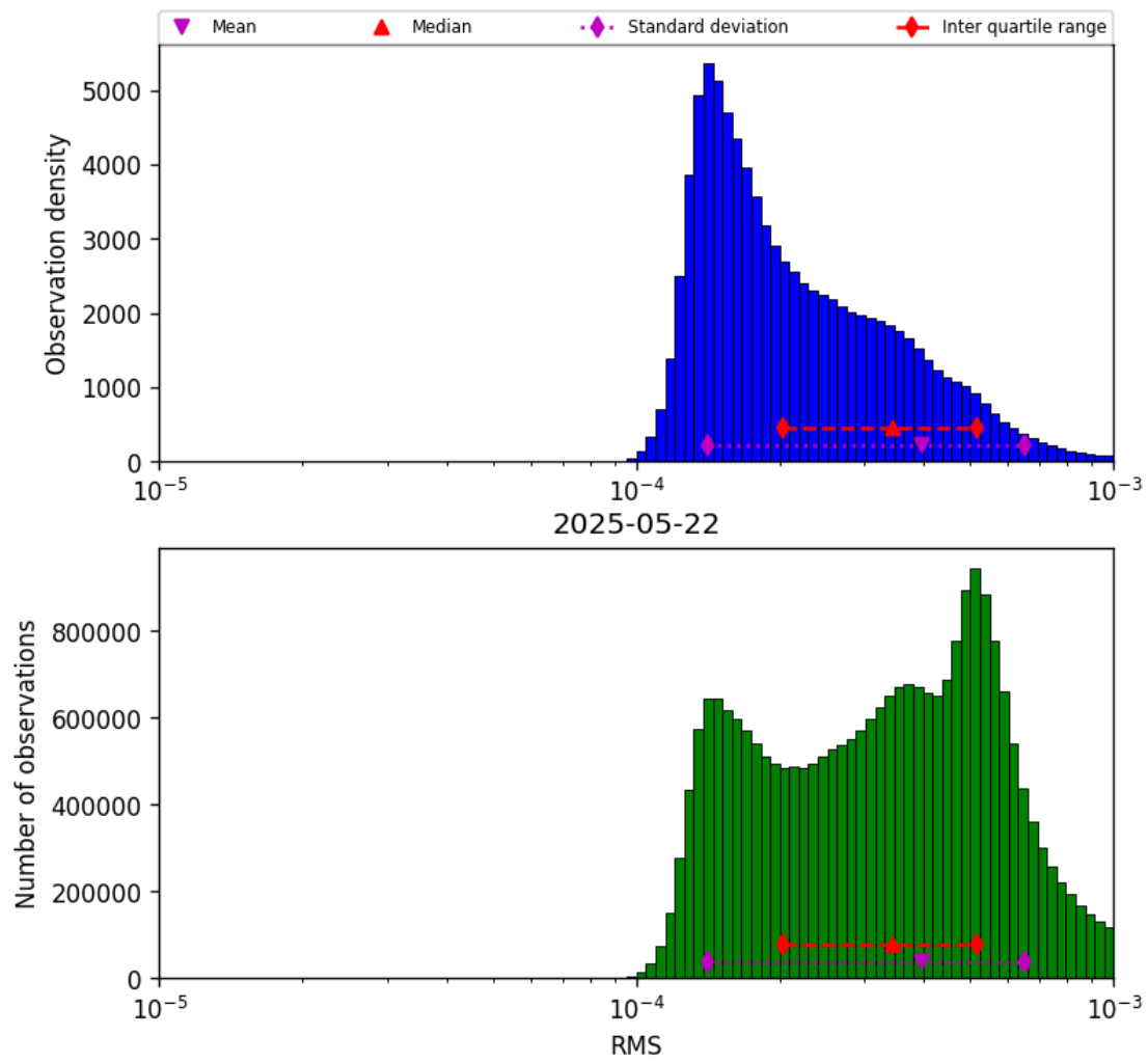
Figure 43: Histogram of “RMS” for 2025-05-21 to 2025-05-23
