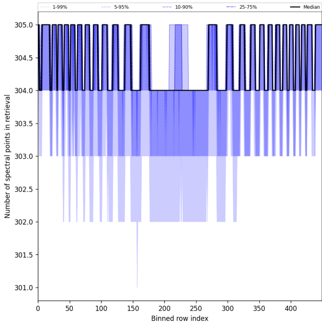
Figure 50: Along track statistics of “Number of spectral points in retrieval” for 2025-05-21 to 2025-05-23
