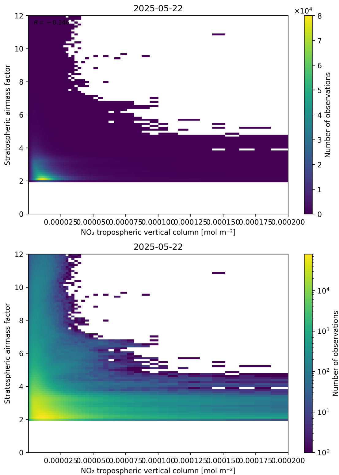
Figure 121: Scatter density plot of “NO 2 tropospheric vertical column” against “Stratospheric air mass factor” for 2025-05-21 to 2025-05-23.
