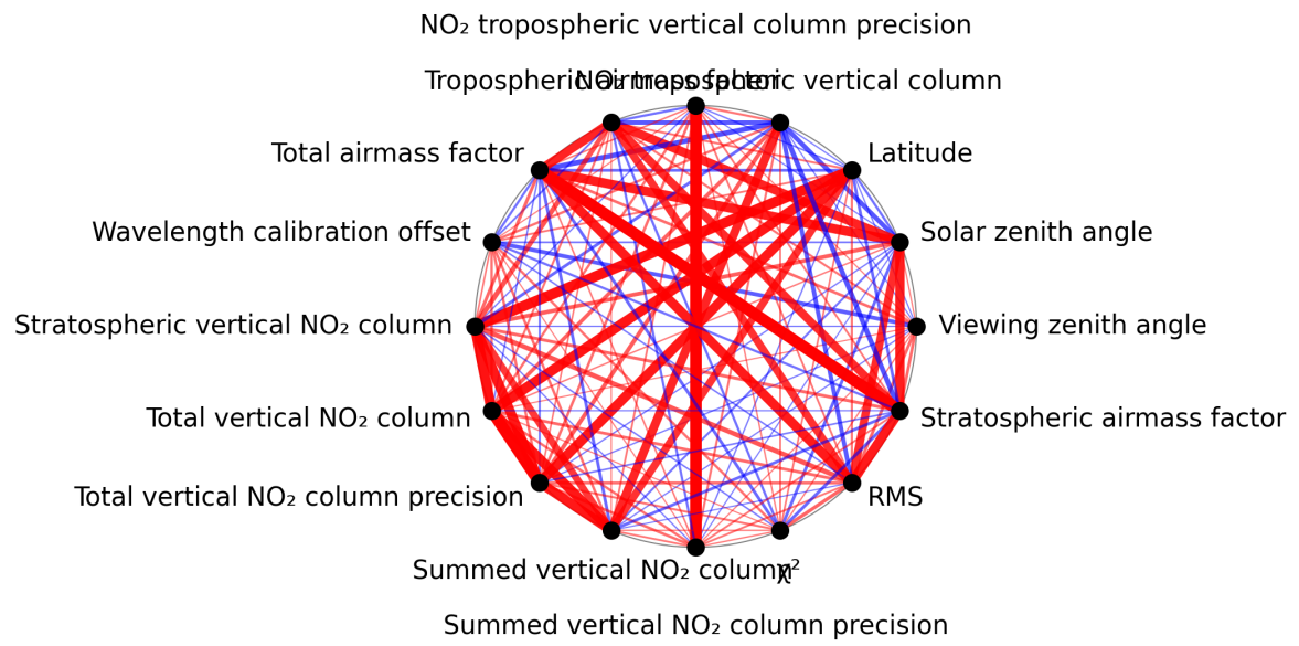
Figure 1: Map of correlation graph for 2025-05-21 to 2025-05-23.
