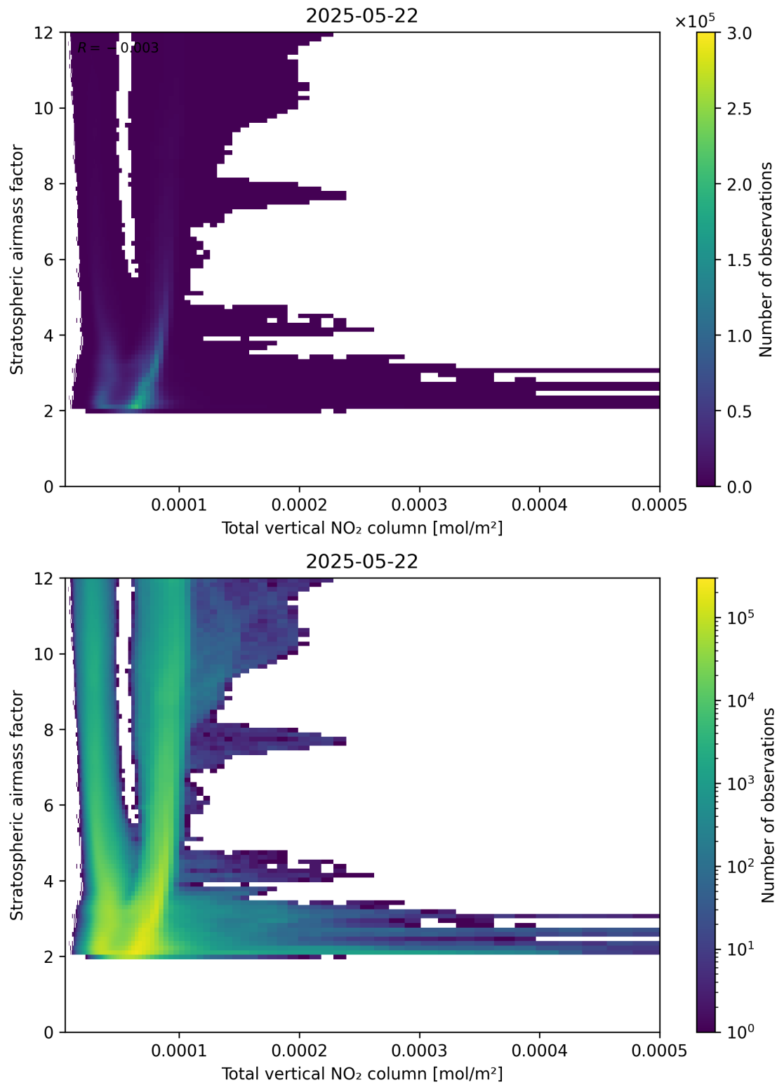
Figure 110: Scatter density plot of “Total vertical NO 2 column” against “Stratospheric airmass factor” for 2025-05-21 to 2025-05-23.
