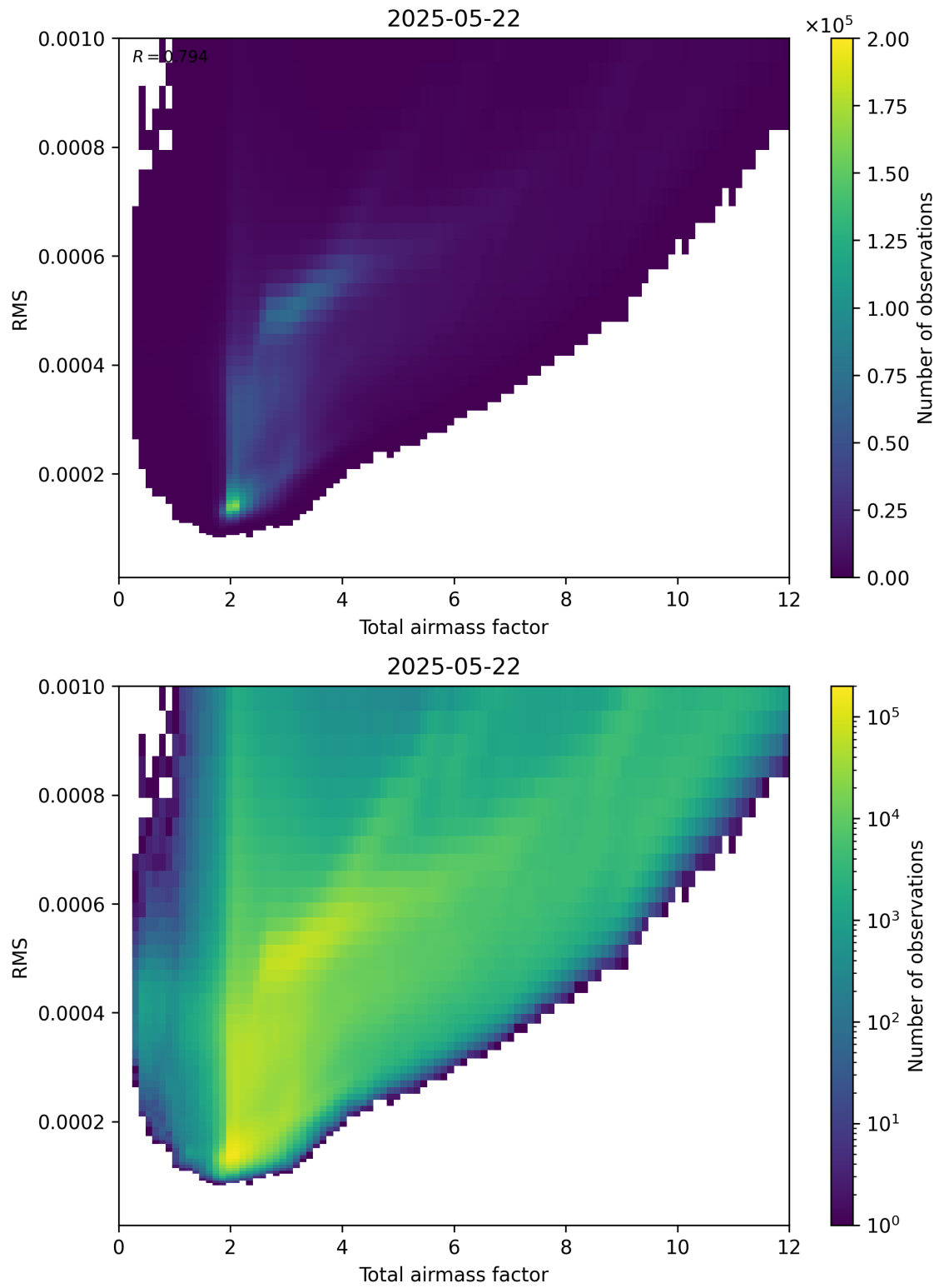
Figure 69: Scatter density plot of “Total airmass factor” against “RMS” for 2025-05-21 to 2025-05-23.
