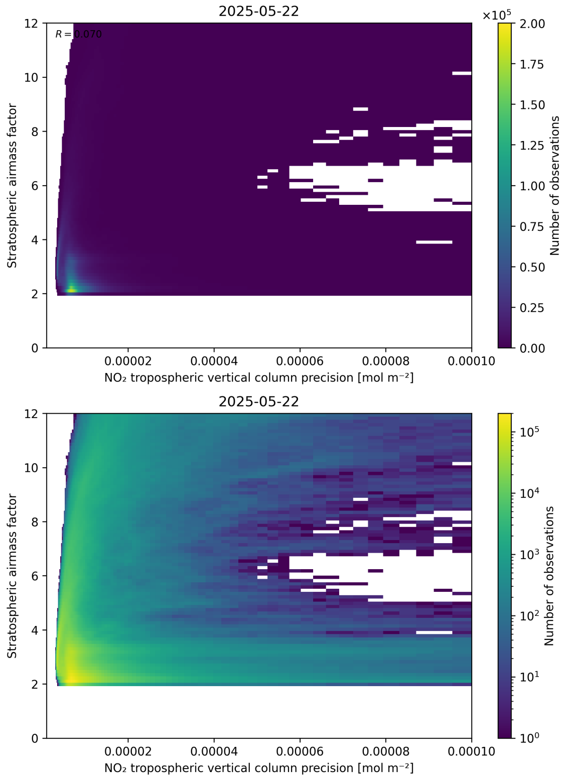
Figure 131: Scatter density plot of “NO 2 tropospheric vertical column precision” against “Stratospheric airmass factor” for 2025-05-21 to 2025-05-23.
