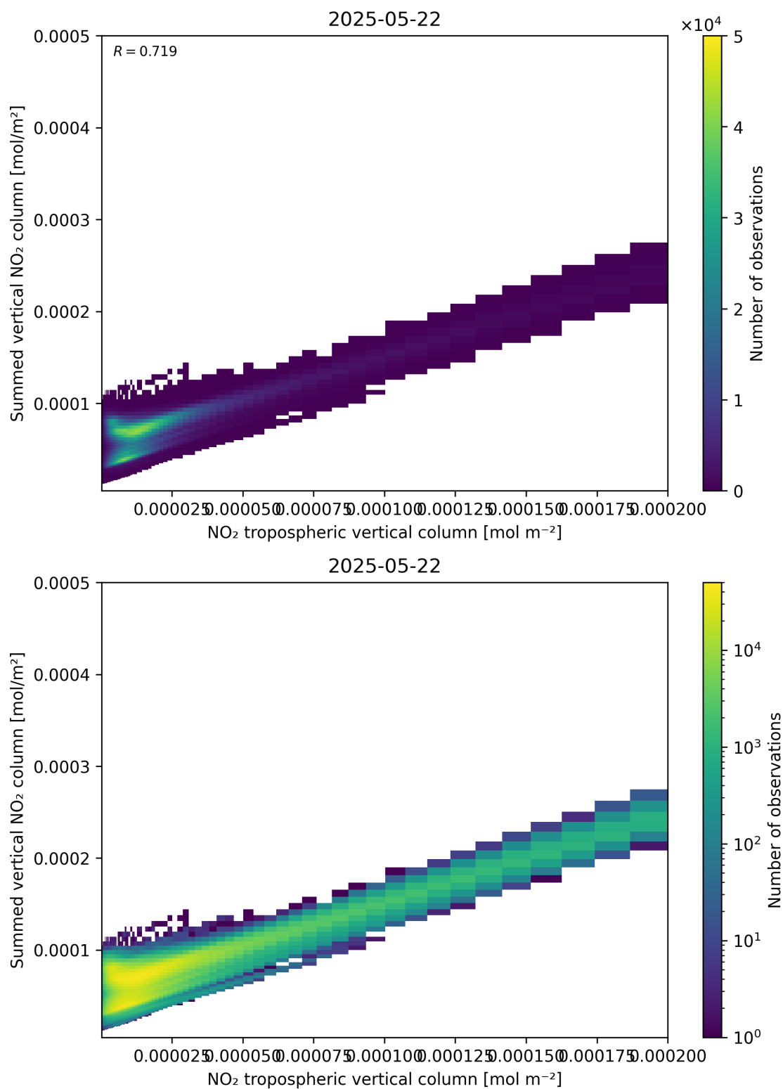
Figure 126: Scatter density plot of “NO 2 tropospheric vertical column” against “Summed vertical NO 2 column” for 2025-05-21 to 2025-05-23.
