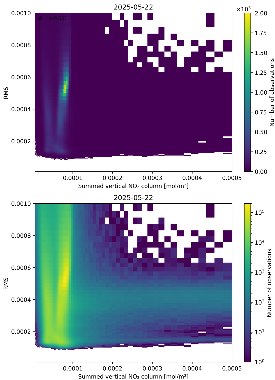
Figure 109: Scatter density plot of “Summed vertical NO 2 column” against “RMS” for 2025-05-21 to 2025-05-23.
