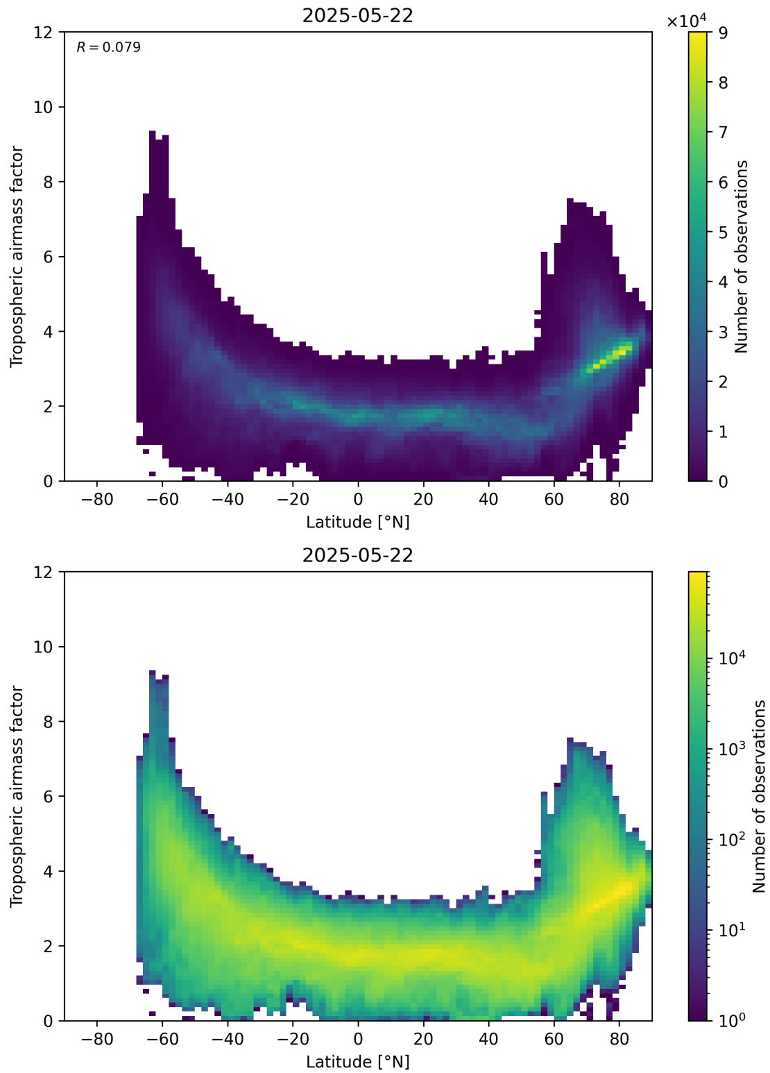
Figure 85: Scatter density plot of “Latitude” against “Tropospheric air mass factor” for 2025-05-21 to 2025-05-23.
