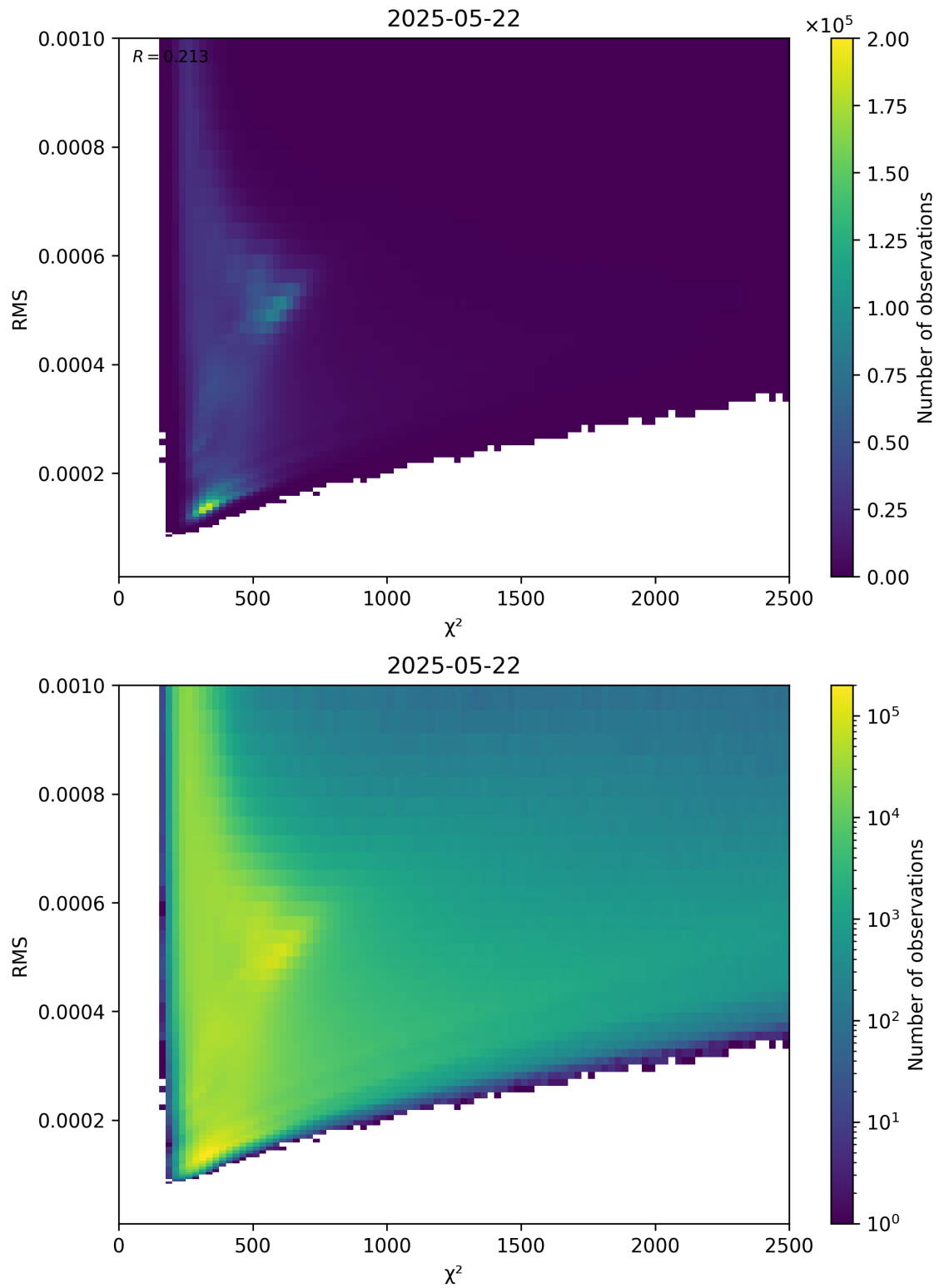
Figure 82: Scatter density plot of “ \chi^2 ” against “RMS” for 2025-05-21 to 2025-05-23.
