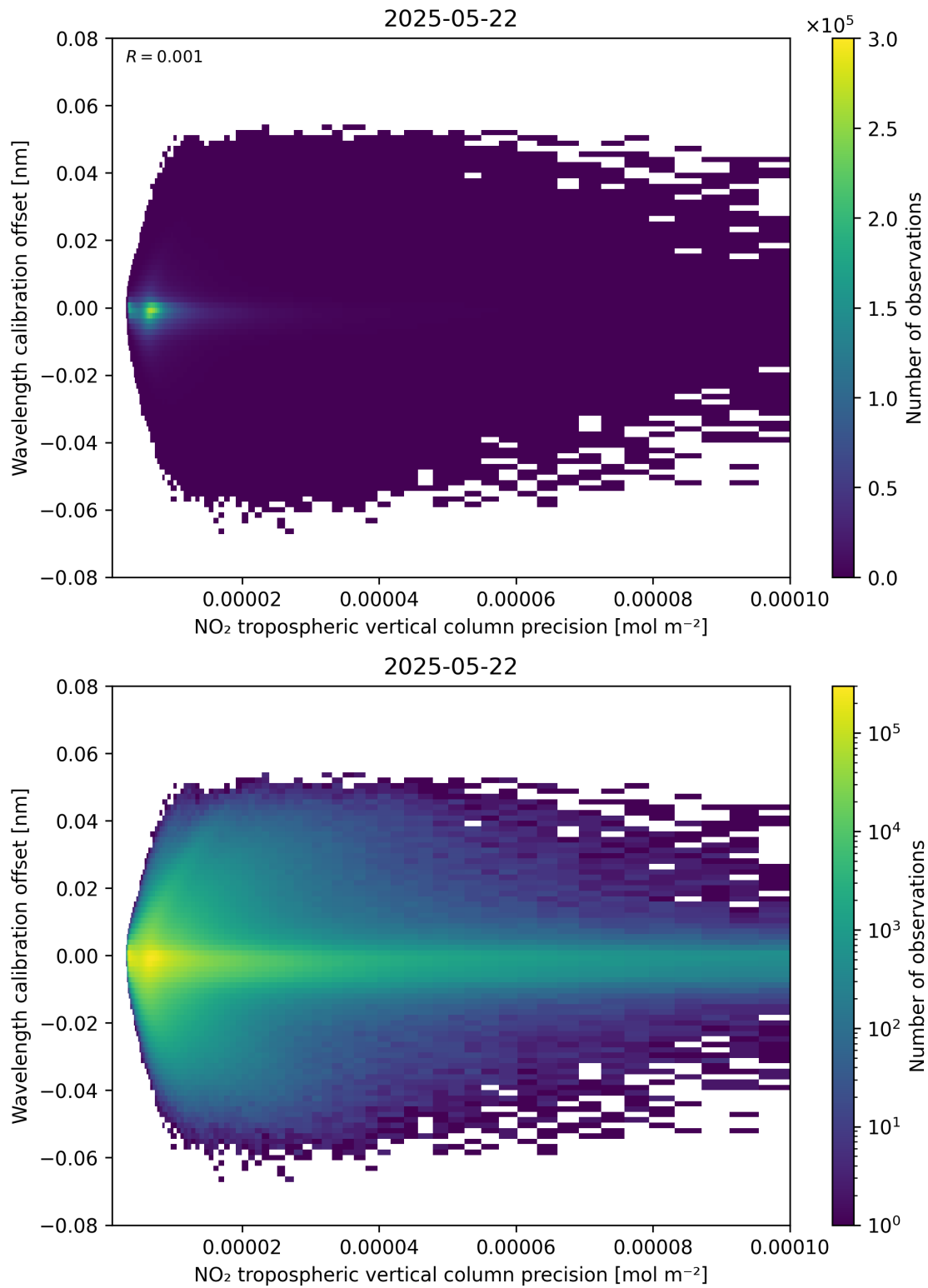
Figure 141: Scatter density plot of “NO 2 tropospheric vertical column precision” against “Wavelength calibration offset” for 2025-05-21 to 2025-05-23.
