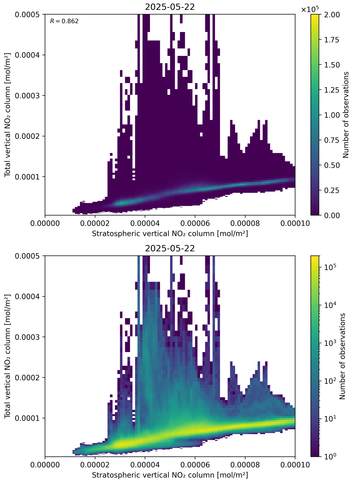
Figure 100: Scatter density plot of “Stratospheric vertical NO 2 column” against “Total vertical NO 2 column” for 2025-05-21 to 2025-05-23.
