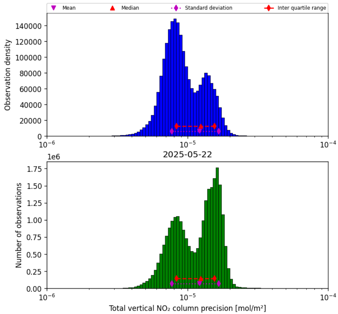
Figure 39: Histogram of “Total vertical NO 2 column precision” for 2025-05-21 to 2025-05-23
