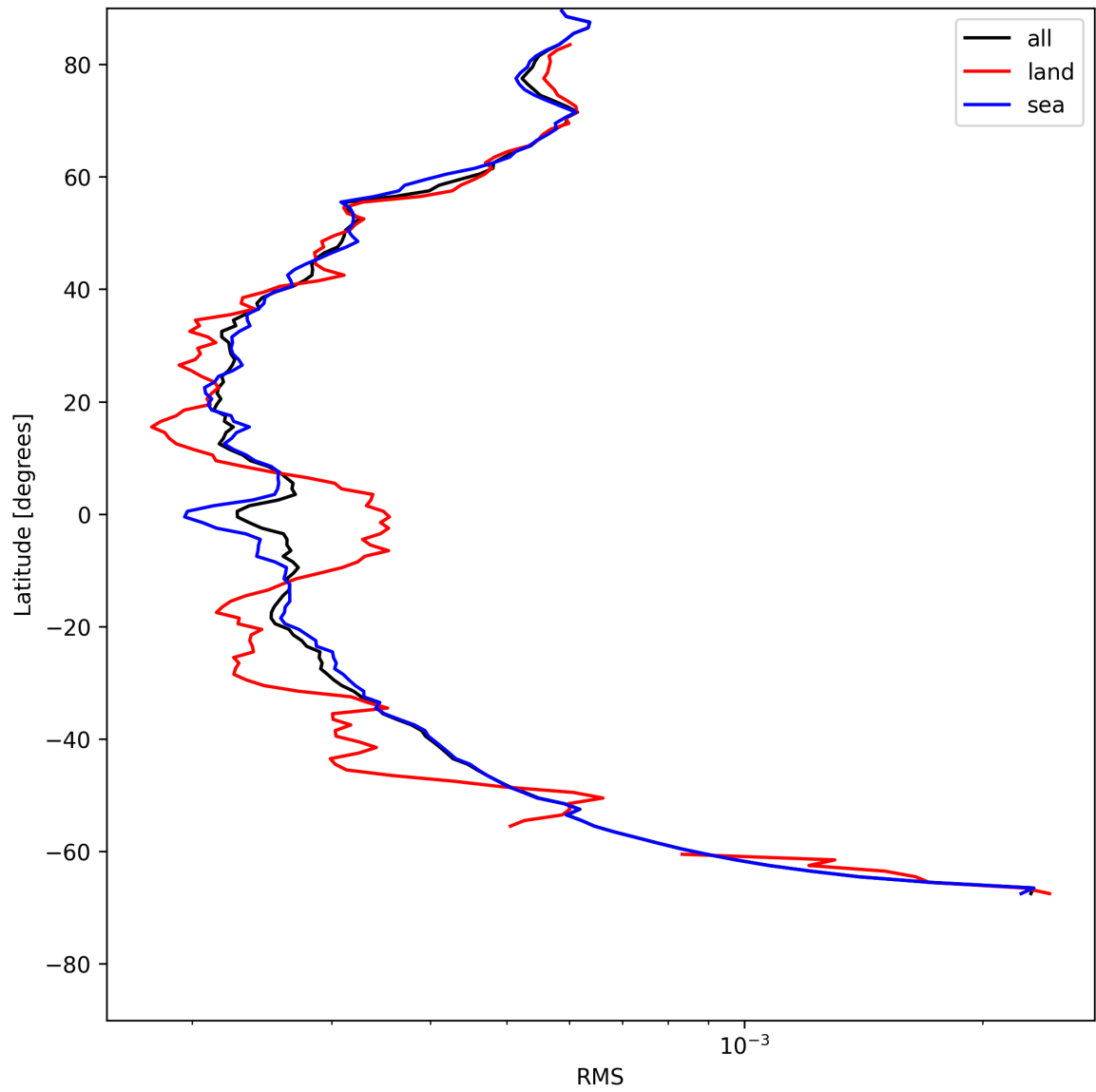
Figure 26: Zonal average of “RMS” for 2025-05-21 to 2025-05-23.
