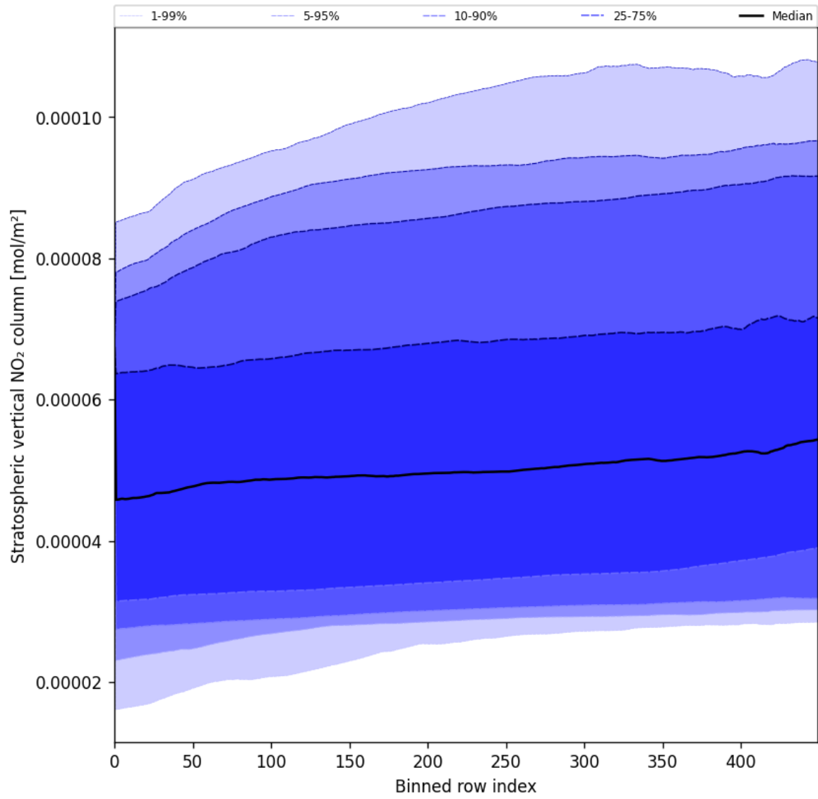
Figure 53: Along track statistics of “Stratospheric vertical NO 2 column” for 2025-05-21 to 2025-05-23
