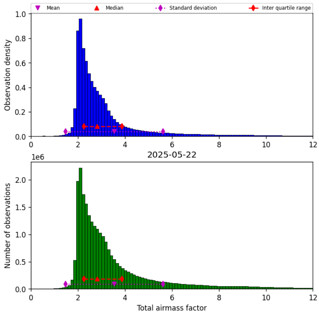
Figure 32: Histogram of “Total airmass factor” for 2025-05-21 to 2025-05-23
