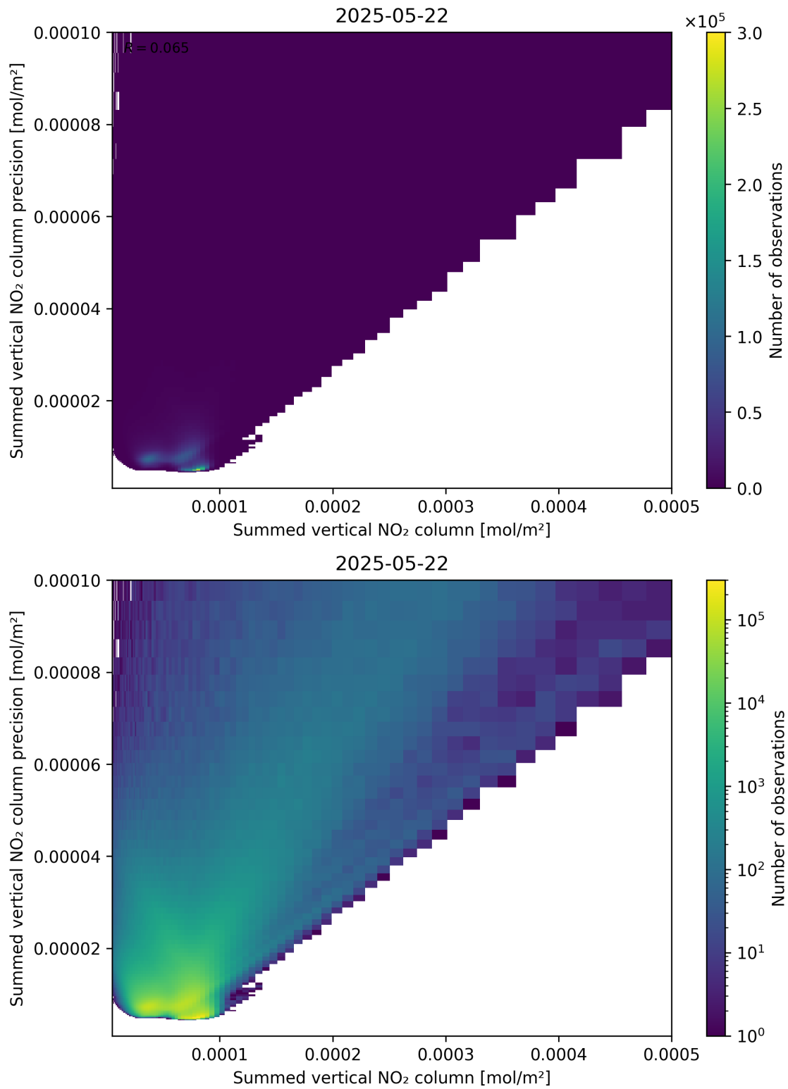
Figure 105: Scatter density plot of “Summed vertical NO 2 column” against “Summed vertical NO 2 column precision” for 2025-05-21 to 2025-05-23.
