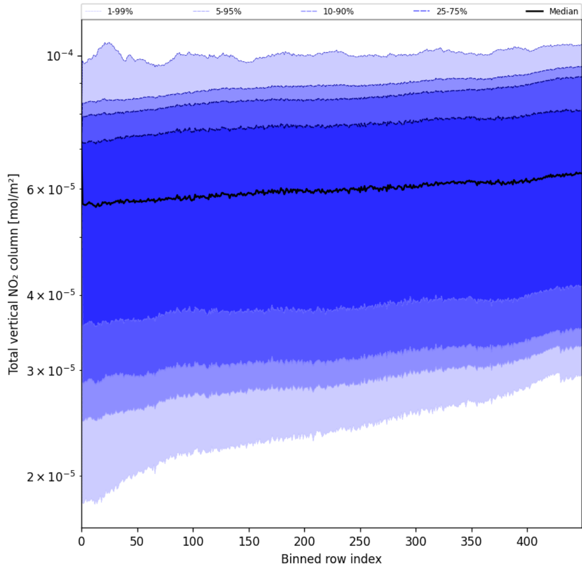
Figure 55: Along track statistics of “Total vertical NO 2 column” for 2025-05-21 to 2025-05-23
