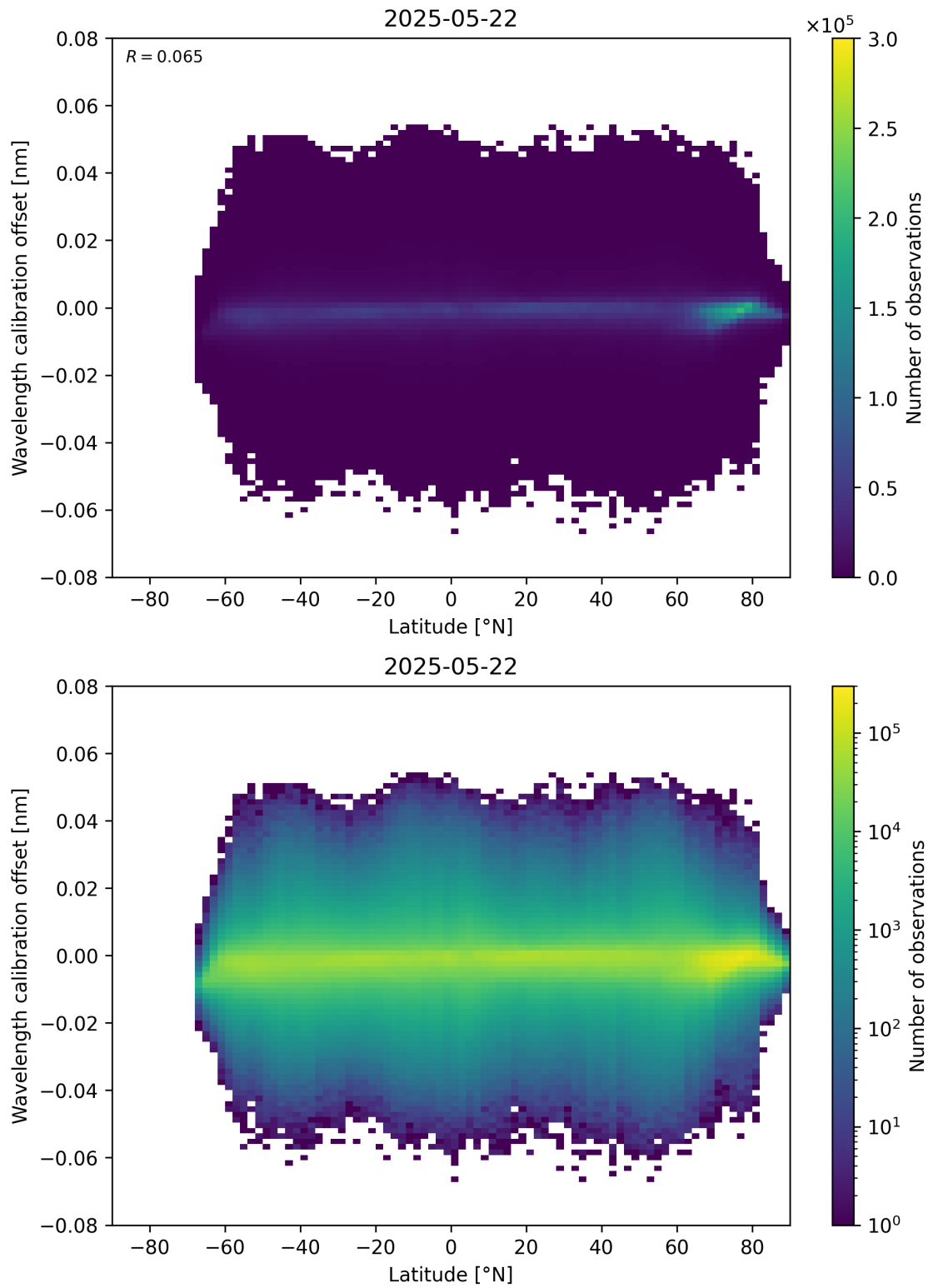
Figure 95: Scatter density plot of “Latitude” against “Wavelength calibration offset” for 2025-05-21 to 2025-05-23.
