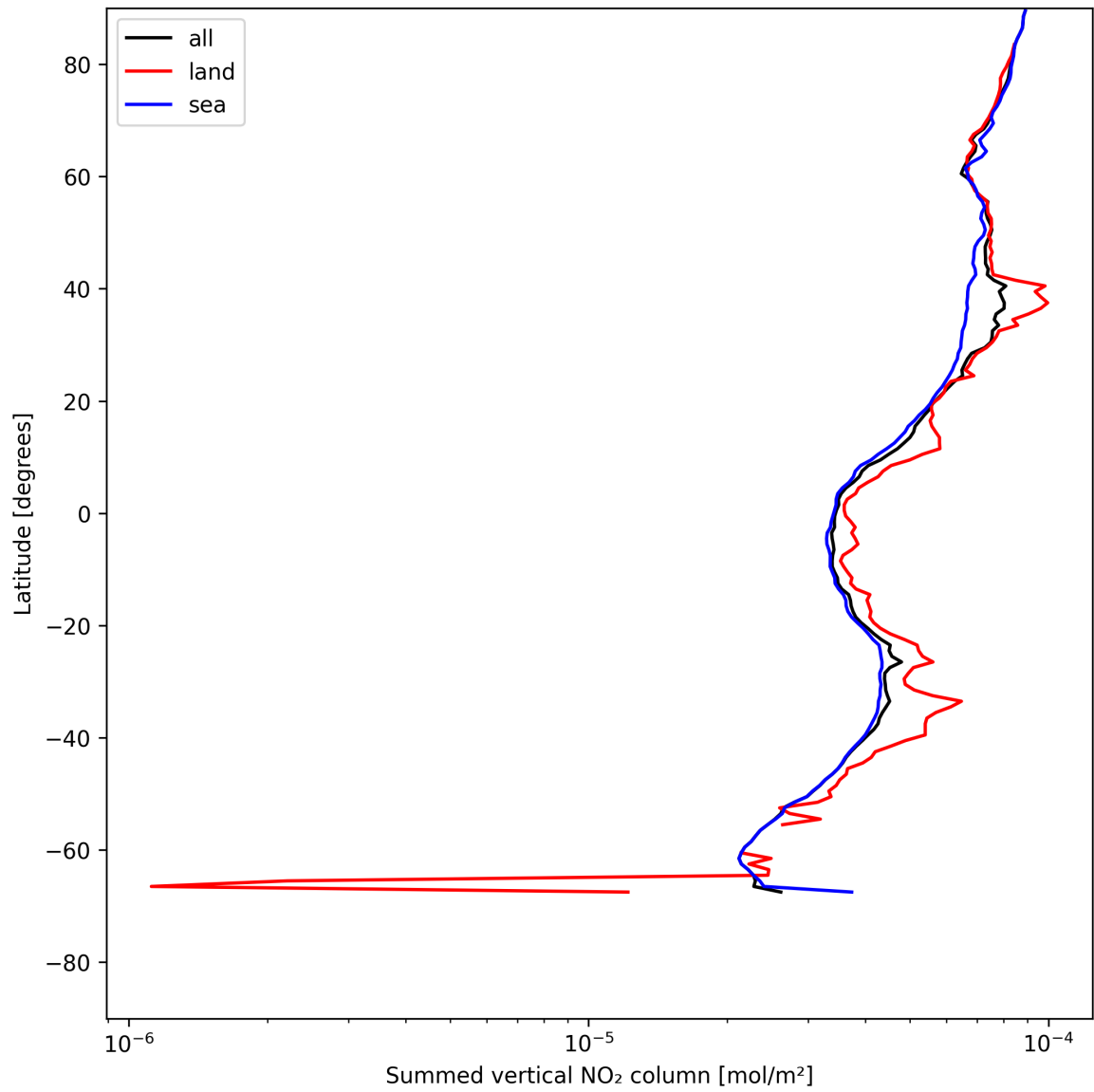
Figure 23: Zonal average of “Summed vertical NO 2 column” for 2025-05-21 to 2025-05-23.
