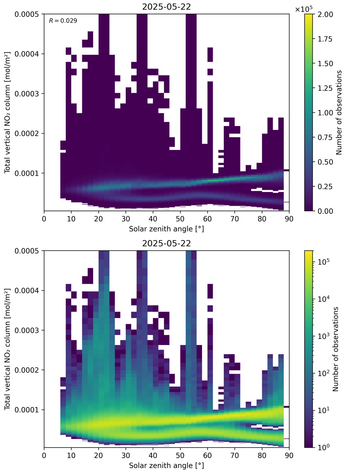
Figure 153: Scatter density plot of “Solar zenith angle” against “Total vertical NO 2 column” for 2025-05-21 to 2025-05-23.
