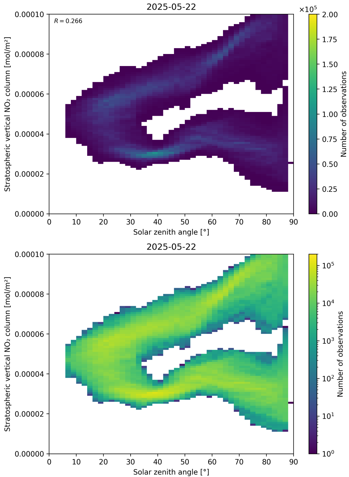
Figure 150: Scatter density plot of “Solar zenith angle” against “Stratospheric vertical NO 2 column” for 2025-05-21 to 2025-05-23.
