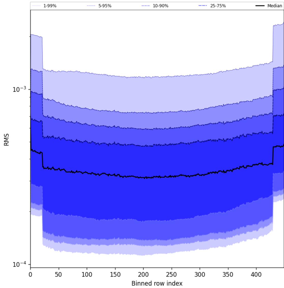
Figure 60: Along track statistics of “RMS” for 2025-05-21 to 2025-05-23
