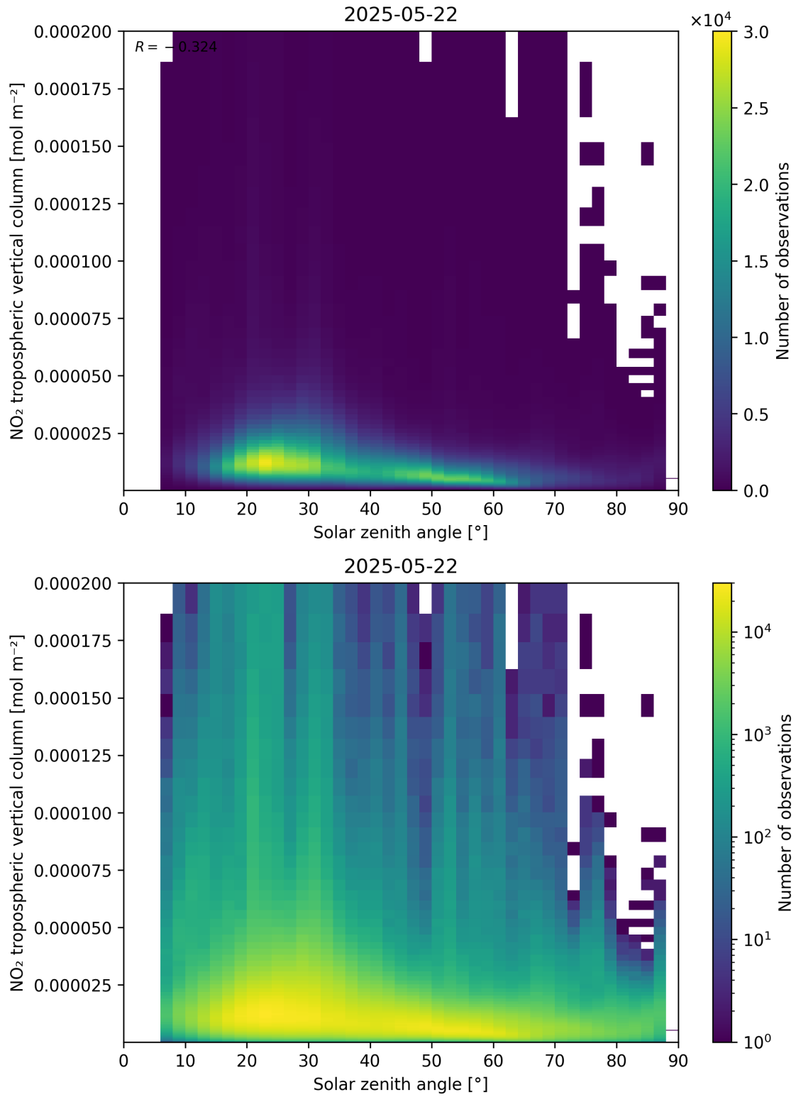
Figure 155: Scatter density plot of “Solar zenith angle” against “NO 2 tropospheric vertical column” for 2025-05-21 to 2025-05-23.
