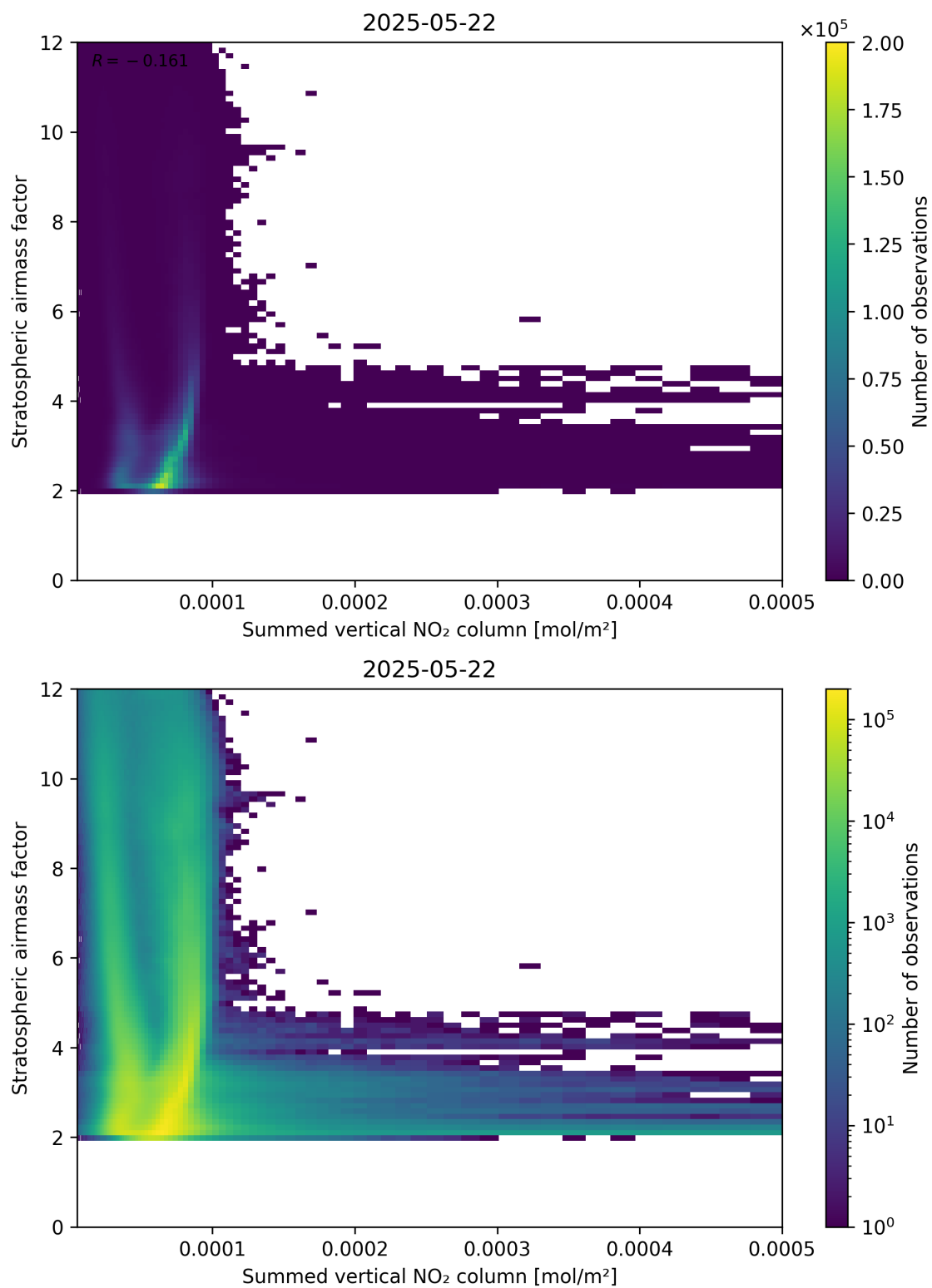
Figure 103: Scatter density plot of “Summed vertical NO 2 column” against “Stratospheric airmass factor” for 2025-05-21 to 2025-05-23.
