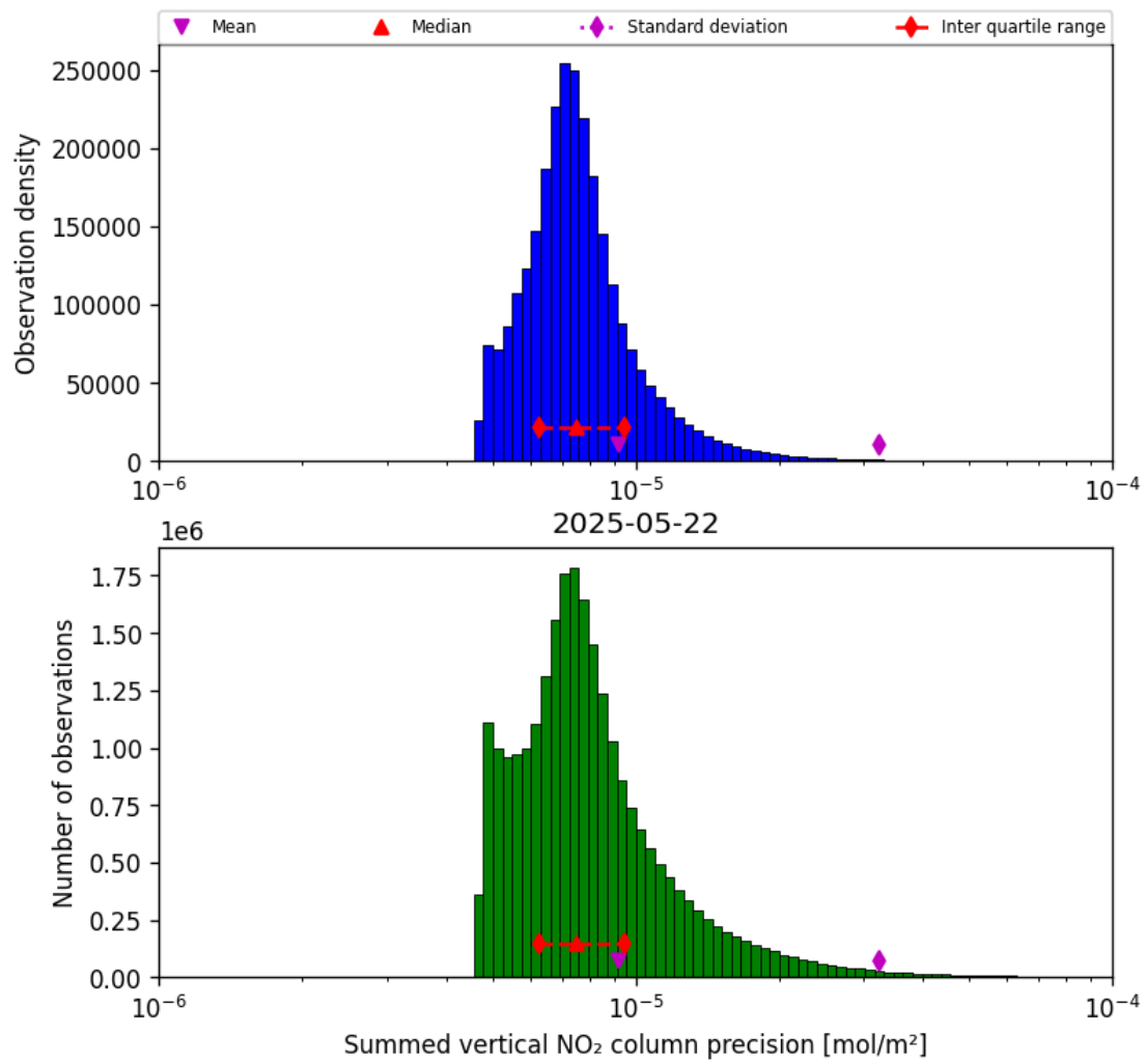
Figure 41: Histogram of "Summed vertical NO 2 column precision" for 2025-05-21 to 2025-05-23
