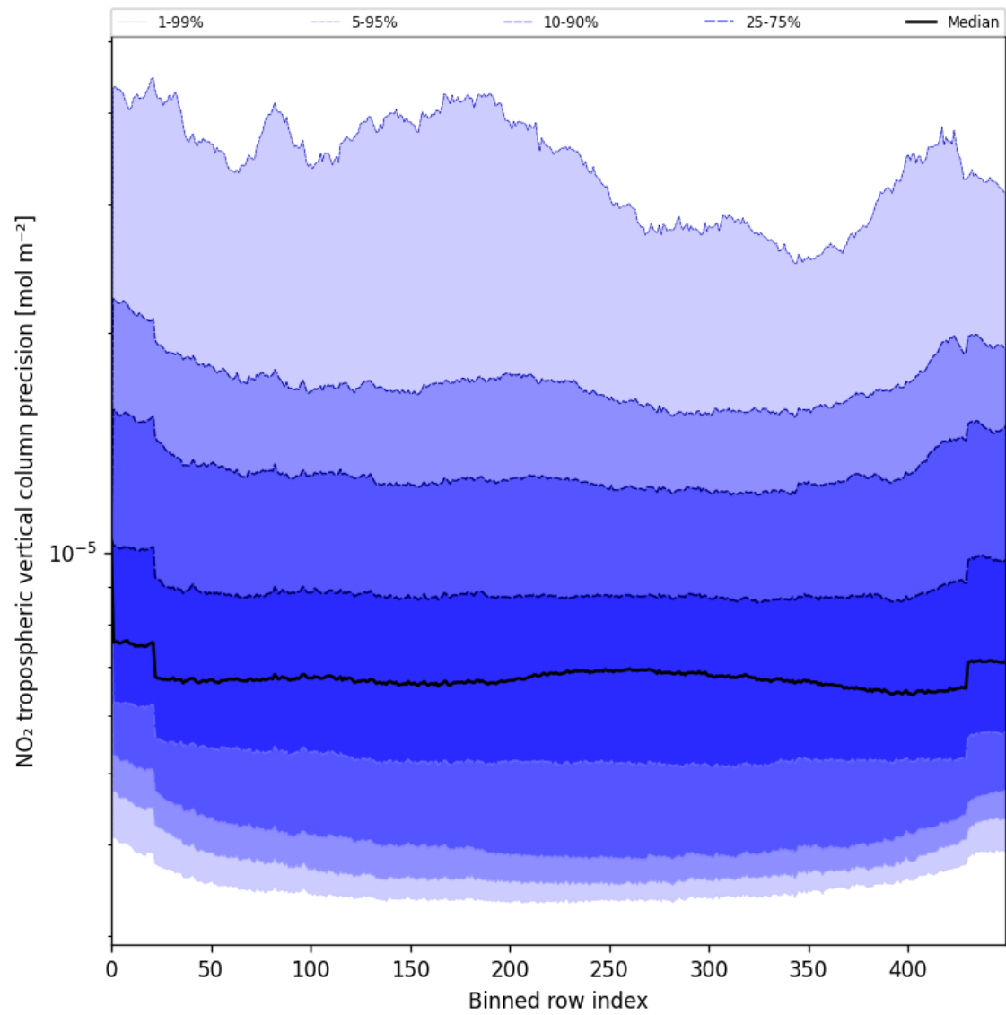
Figure 47: Along track statistics of “NO 2 tropospheric vertical column precision” for 2025-05-21 to 2025-05-23
