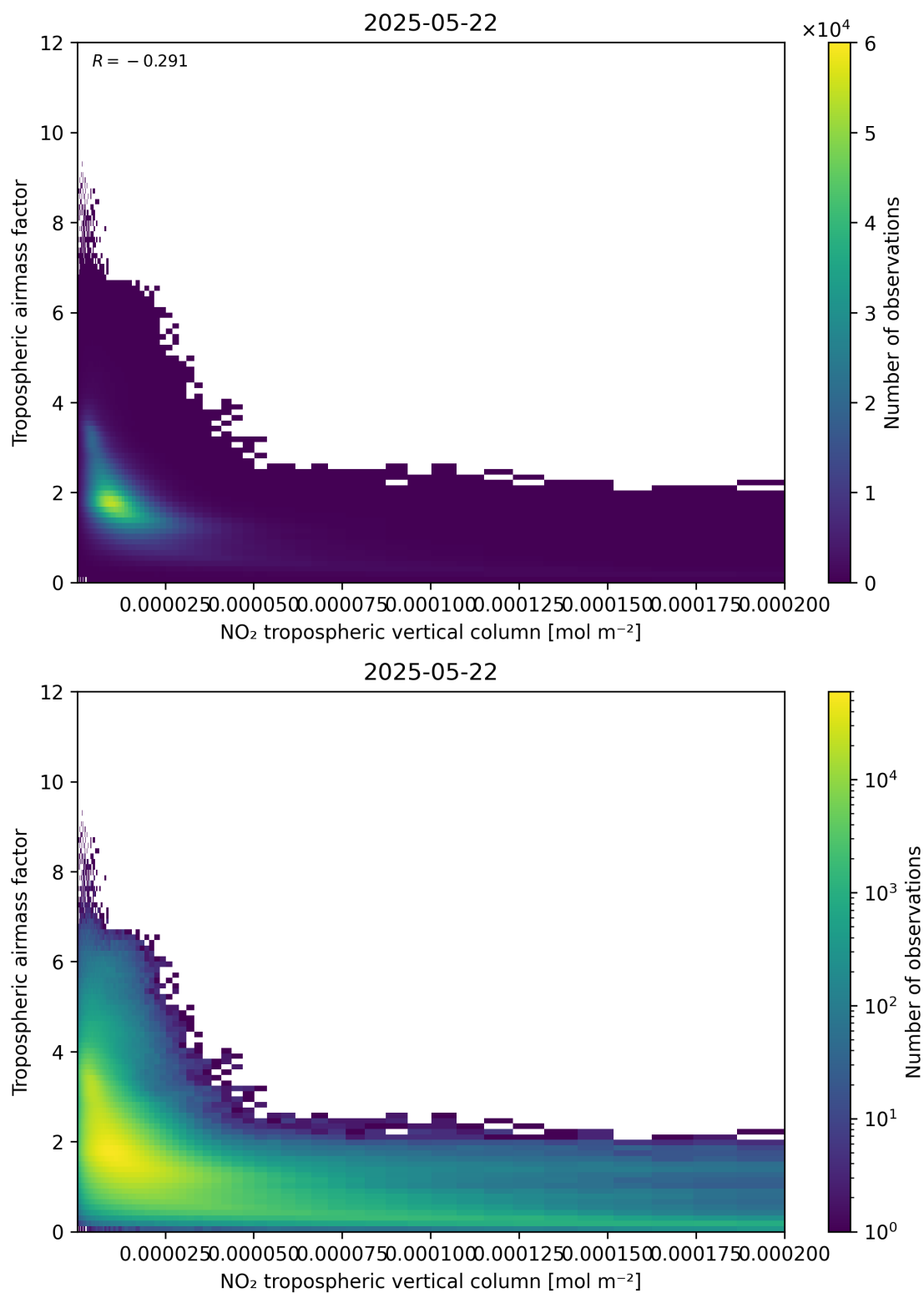
Figure 123: Scatter density plot of “NO 2 tropospheric vertical column” against “Tropospheric airmass factor” for 2025-05-21 to 2025-05-23.
