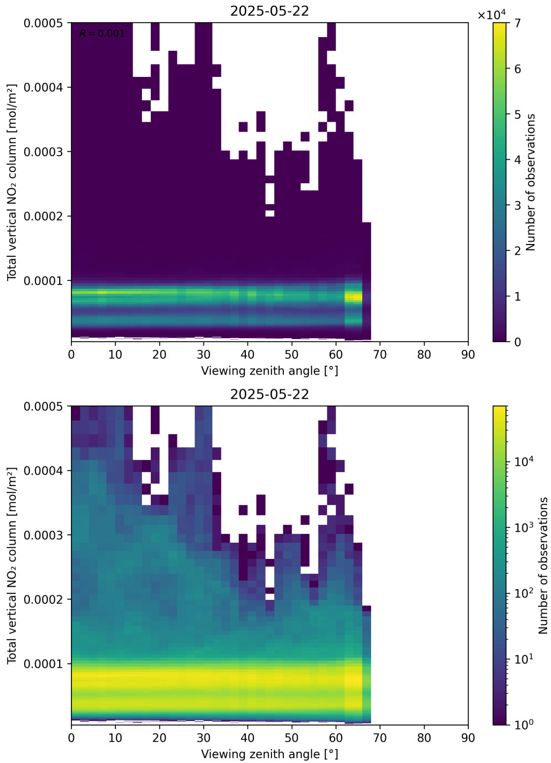
Figure 167: Scatter density plot of “Viewing zenith angle” against “Total vertical NO 2 column” for 2025-05-21 to 2025-05-23.
