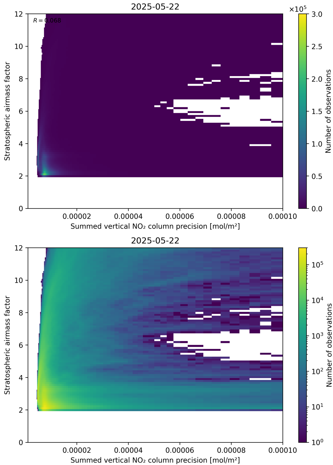
Figure 106: Scatter density plot of “Summed vertical NO 2 column precision” against “Stratospheric airmass factor” for 2025-05-21 to 2025-05-23.
