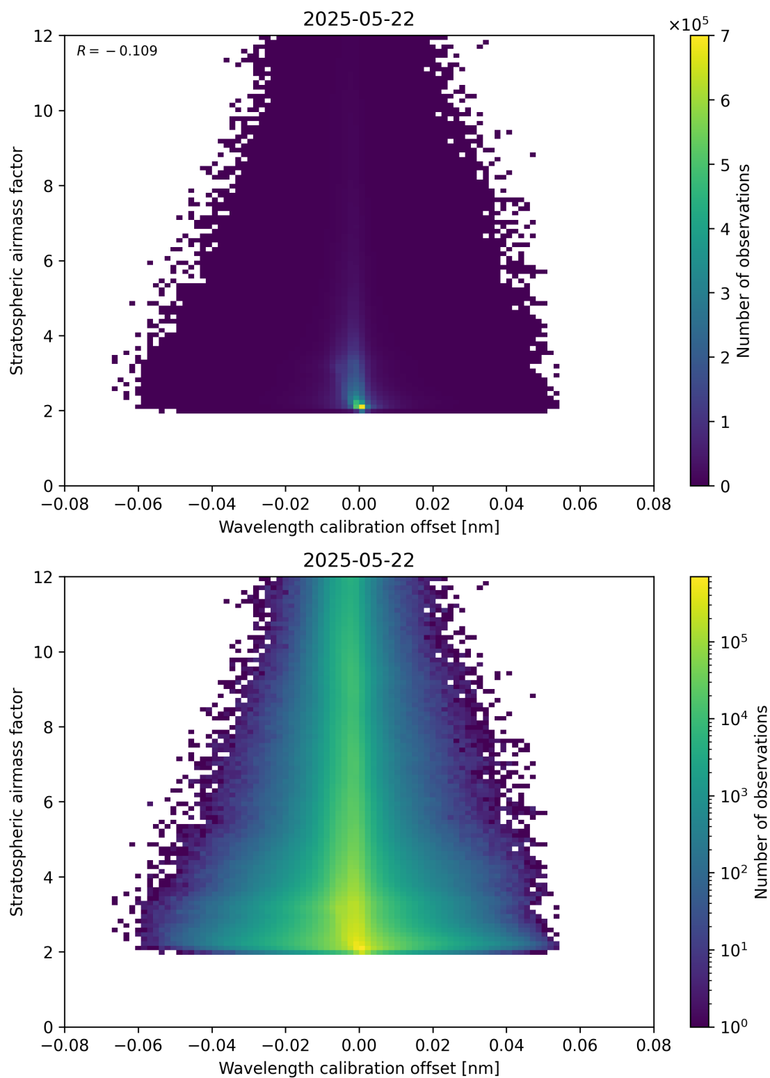
Figure 174: Scatter density plot of “Wavelength calibration offset” against “Stratospheric airmass factor” for 2025-05-21 to 2025-05-23.
