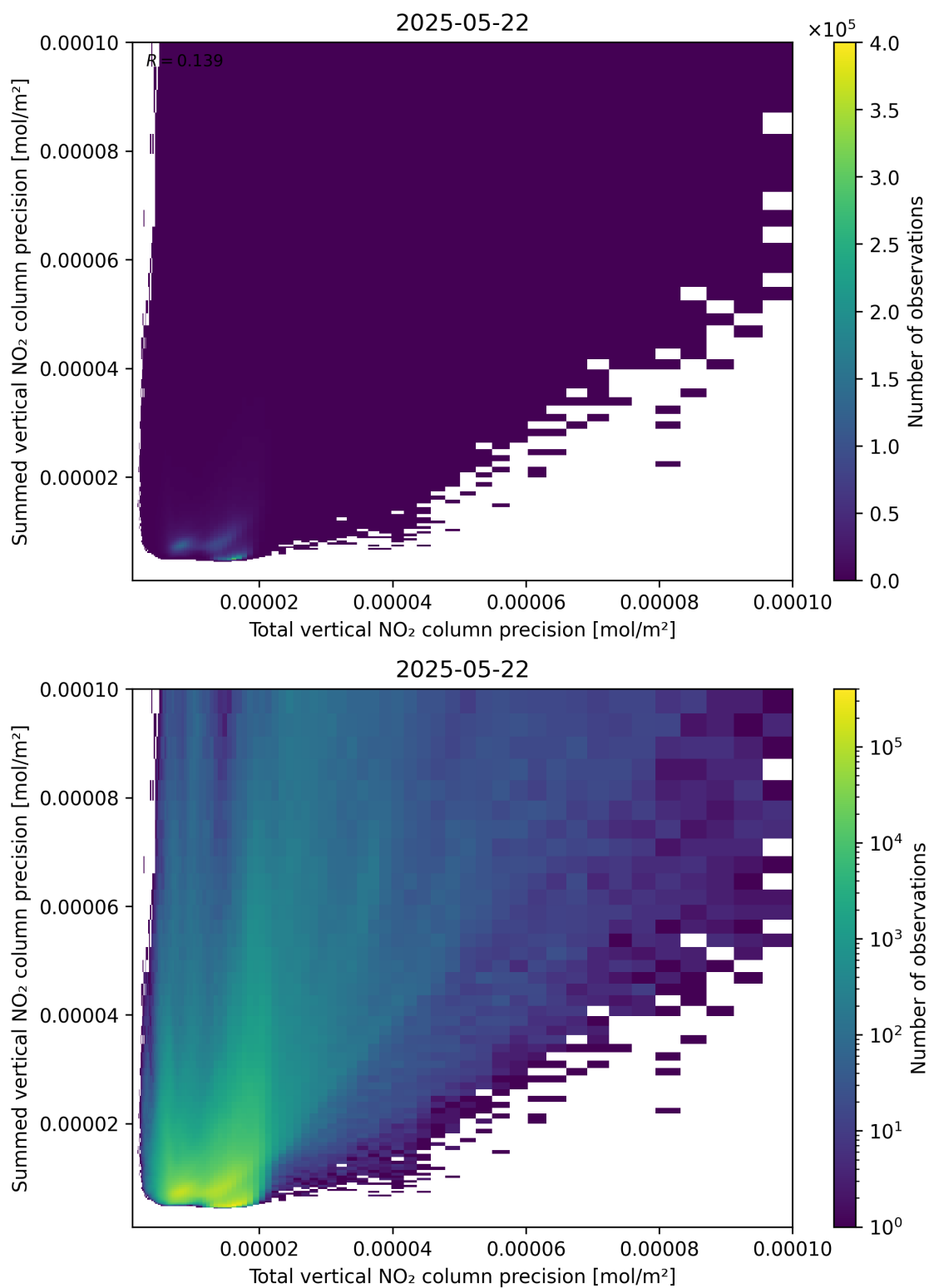
Figure 118: Scatter density plot of “Total vertical NO 2 column precision” against “Summed vertical NO 2 column precision” for 2025-05-21 to 2025-05-23.
