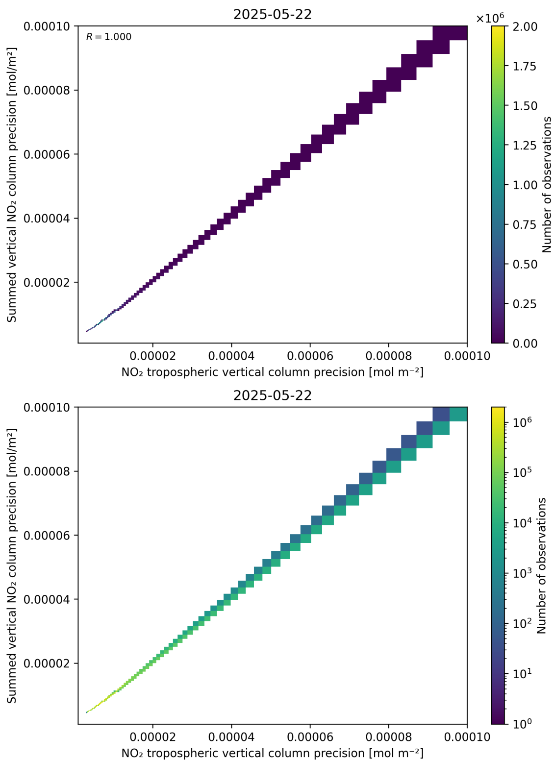
Figure 137: Scatter density plot of “NO 2 tropospheric vertical column precision” against “Summed vertical NO 2 column precision” for 2025-05-21 to 2025-05-23.
