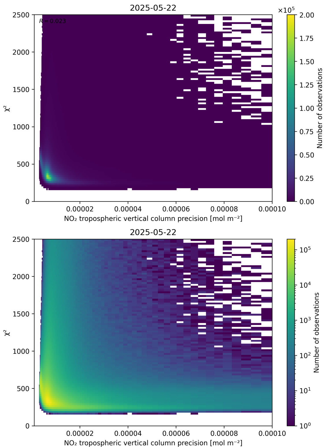
Figure 134: Scatter density plot of “NO 2 tropospheric vertical column precision” against “ \chi^2 ” for 2025-05-21 to 2025-05-23.
