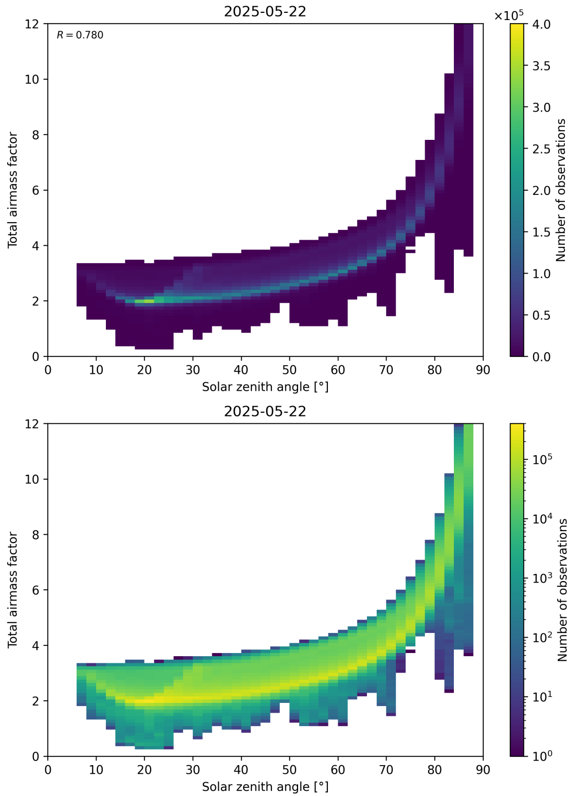
Figure 146: Scatter density plot of “Solar zenith angle” against “Total air mass factor” for 2025-05-21 to 2025-05-23.
