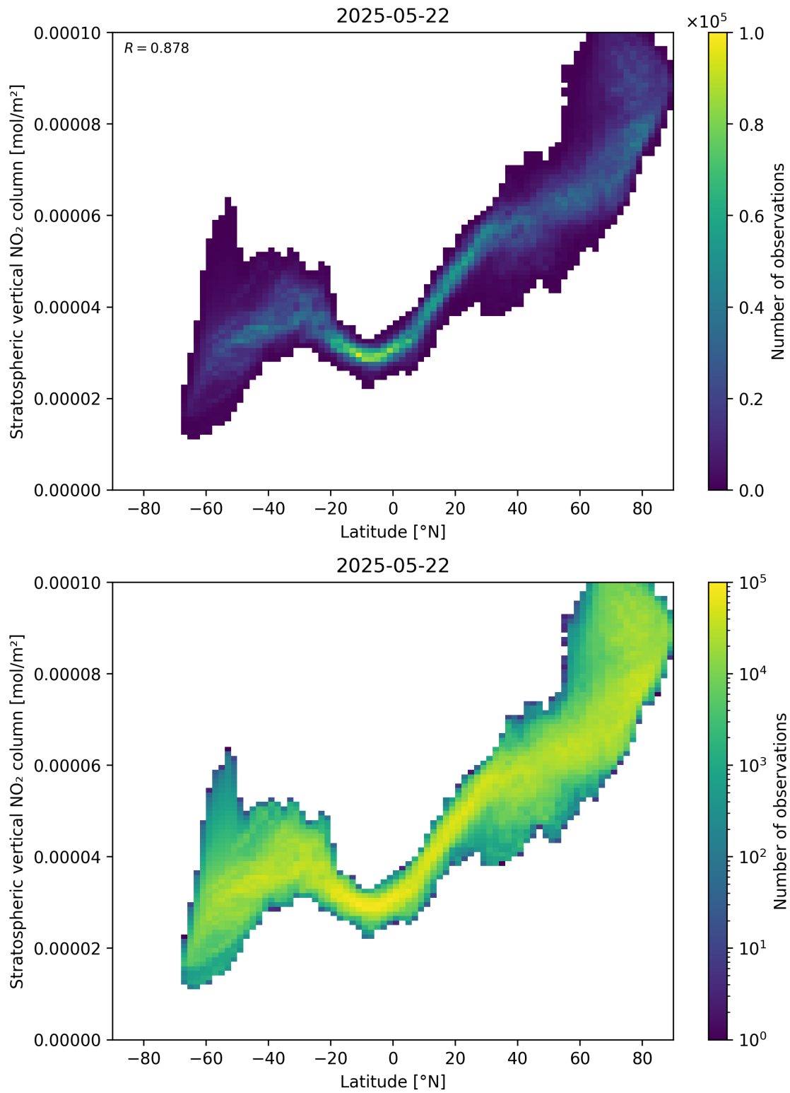
Figure 87: Scatter density plot of “Latitude” against “Stratospheric vertical \text{NO}_2 column” for 2025-05-21 to 2025-05-23.
