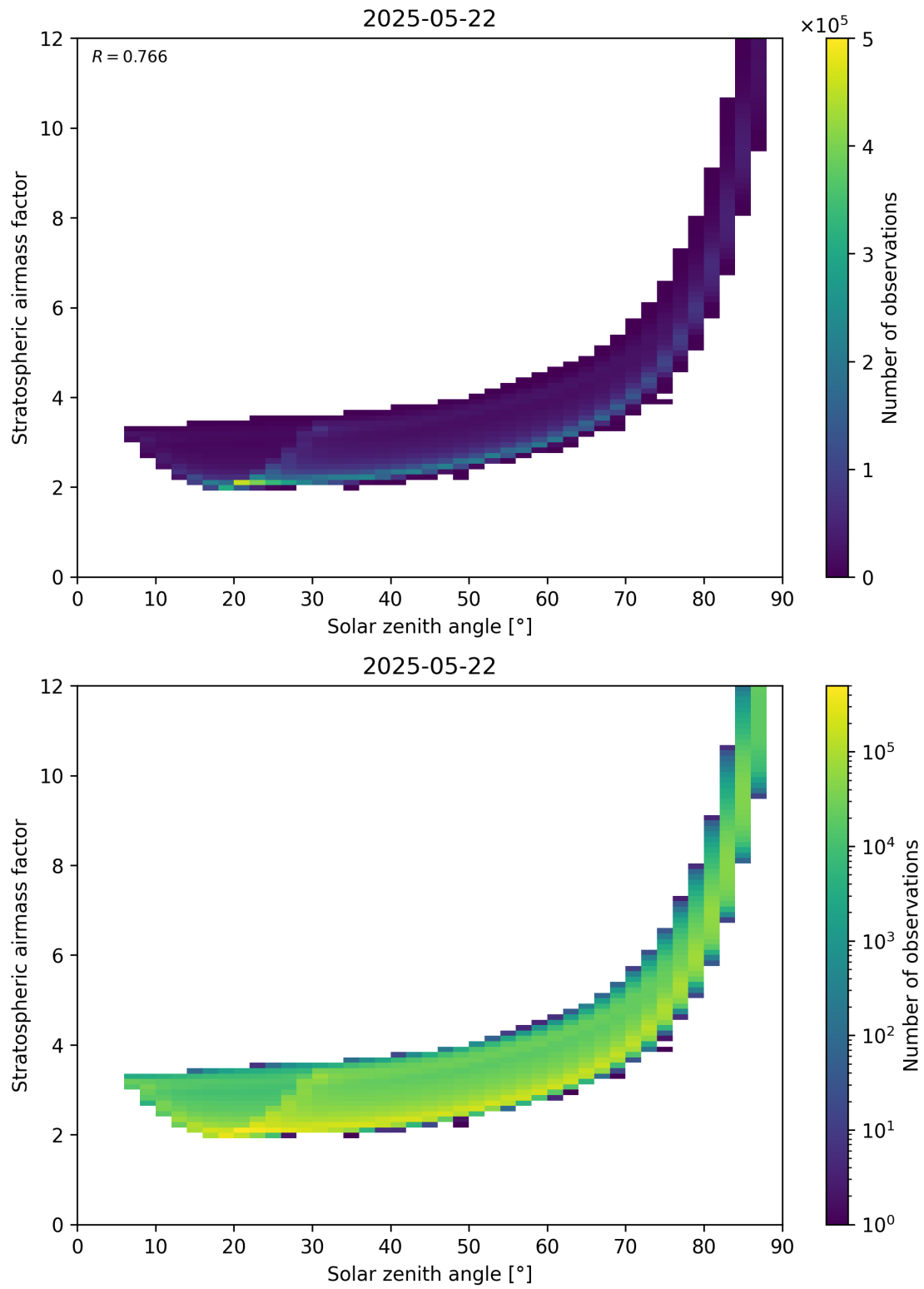
Figure 145: Scatter density plot of “Solar zenith angle” against “Stratospheric airmass factor” for 2025-05-21 to 2025-05-23.
