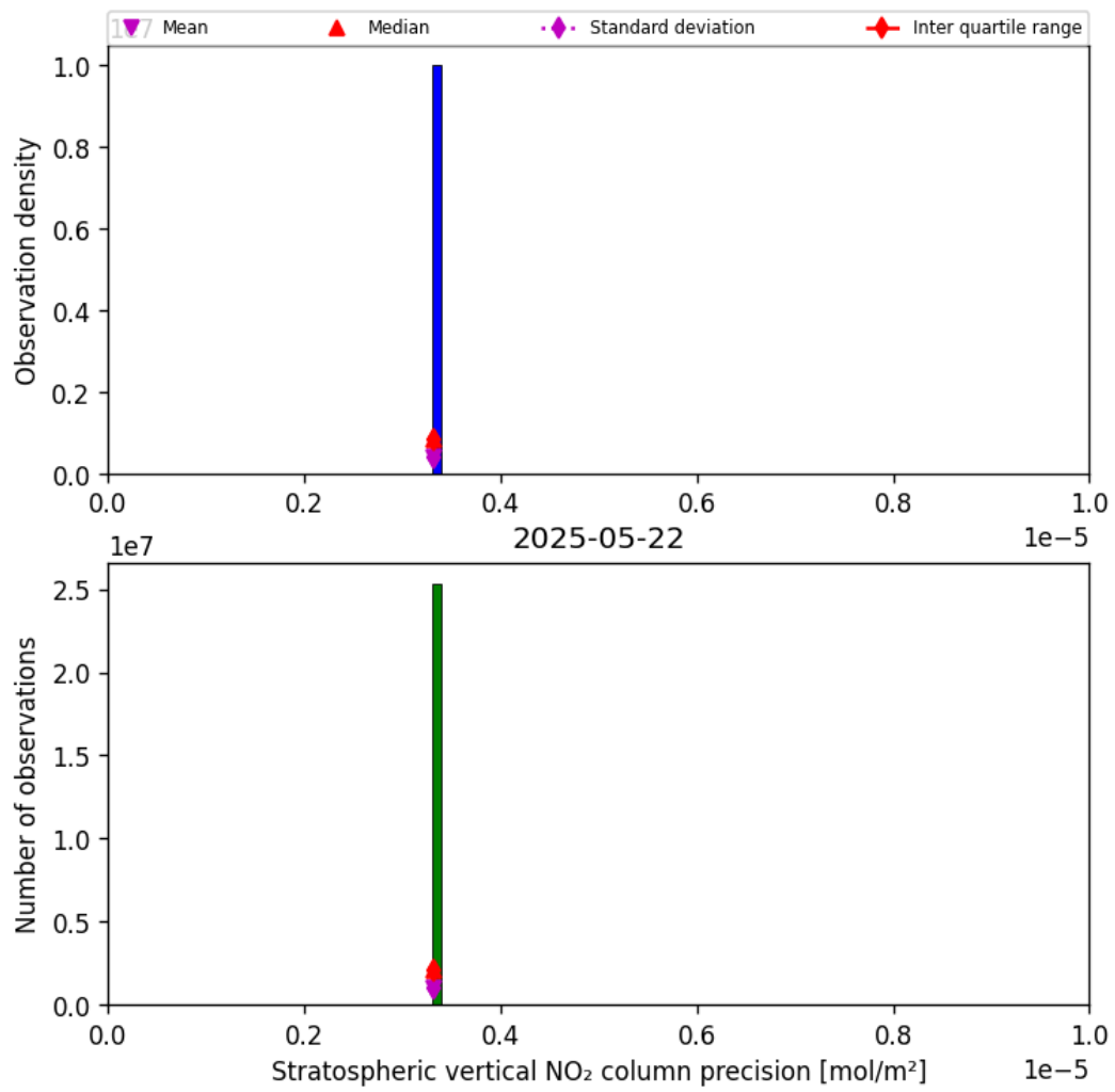
Figure 37: Histogram of “Stratospheric vertical NO 2 column precision” for 2025-05-21 to 2025-05-23
