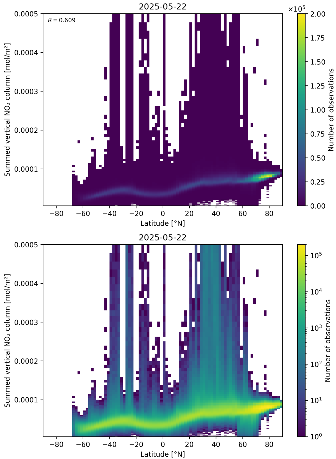
Figure 88: Scatter density plot of “Latitude” against “Summed vertical NO 2 column” for 2025-05-21 to 2025-05-23.
