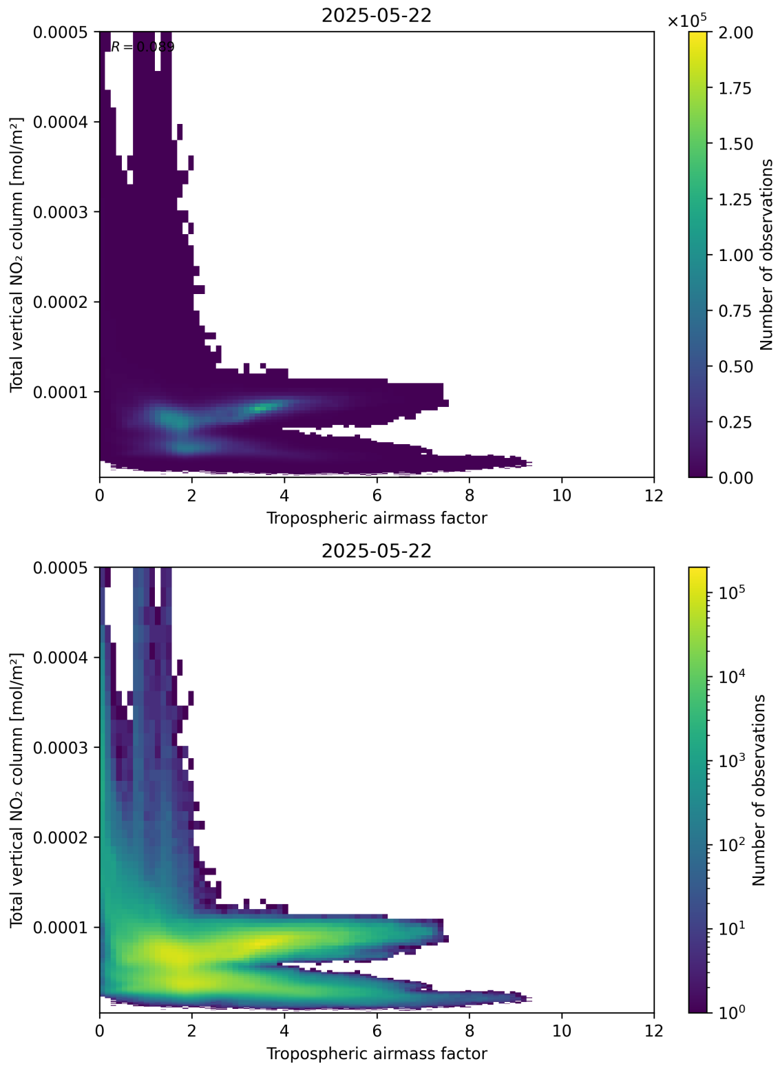
Figure 77: Scatter density plot of “Tropospheric airmass factor” against “Total vertical NO 2 column” for 2025-05-21 to 2025-05-23.
