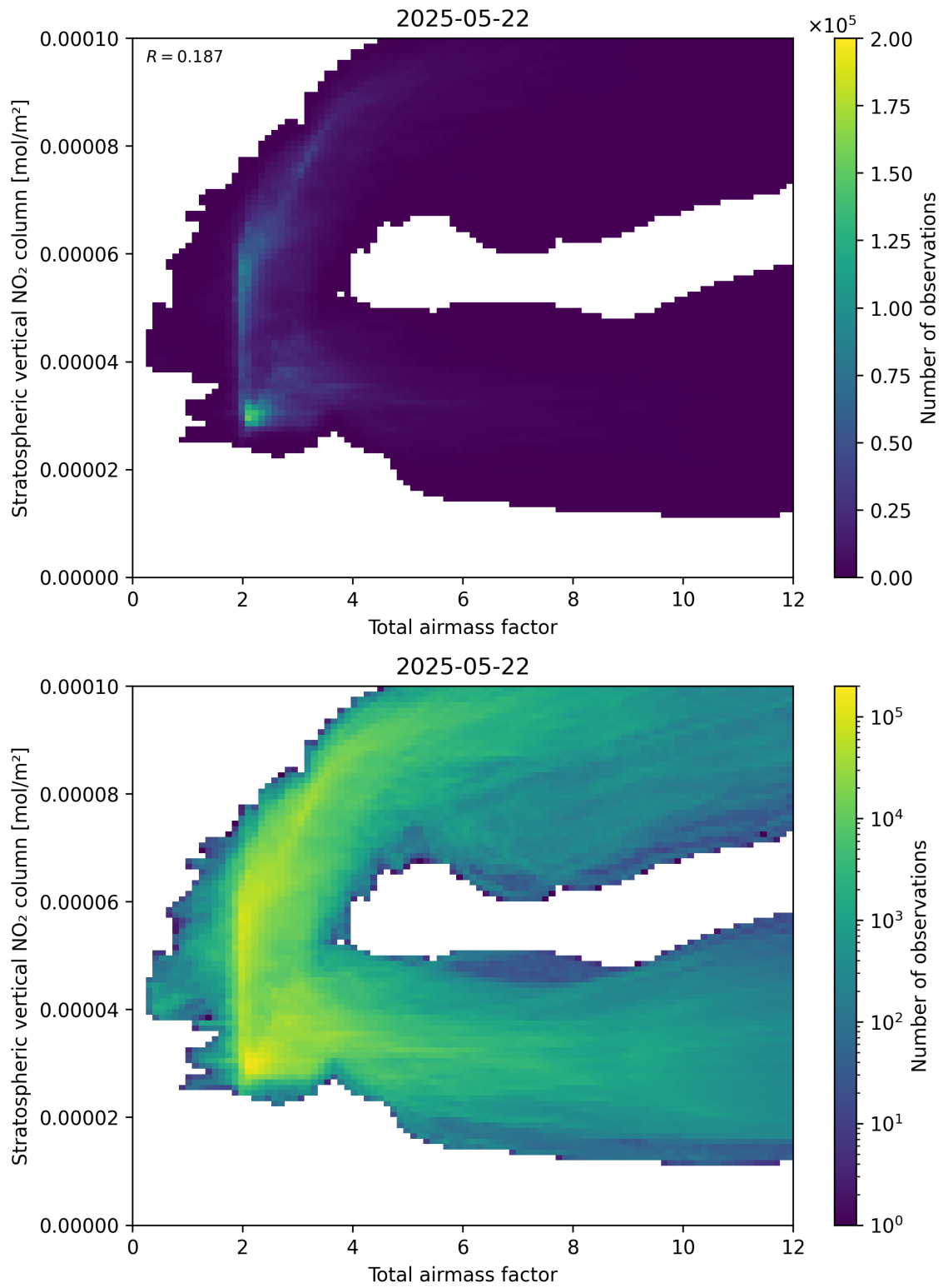
Figure 64: Scatter density plot of “Total airmass factor” against “Stratospheric vertical \text{NO}_2 column” for 2025-05-21 to 2025-05-23.
