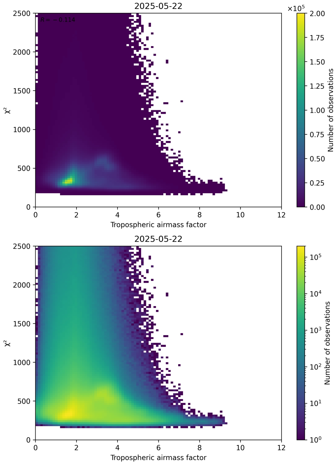
Figure 73: Scatter density plot of “Tropospheric airmass factor” against “ \chi^2 ” for 2025-05-21 to 2025-05-23.
