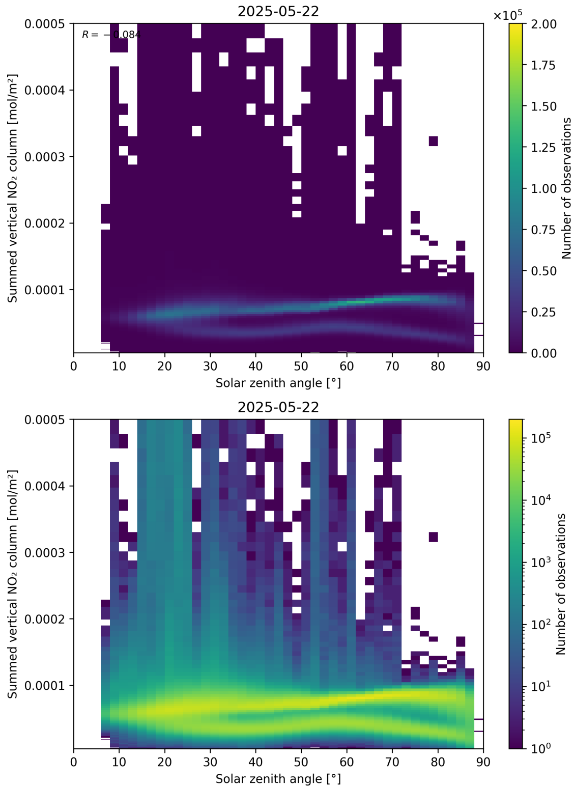
Figure 151: Scatter density plot of “Solar zenith angle” against “Summed vertical NO 2 column” for 2025-05-21 to 2025-05-23.
