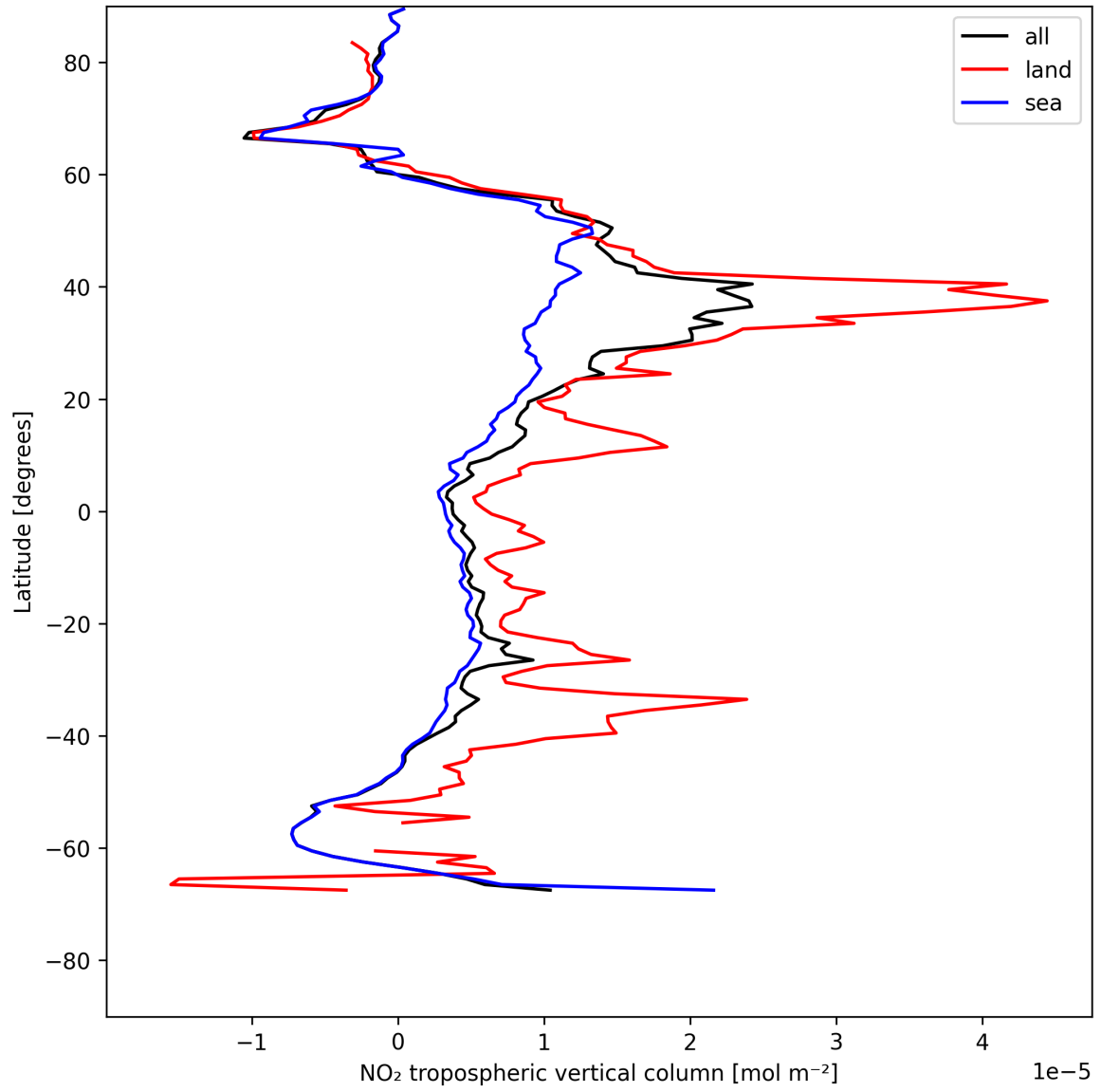
Figure 12: Zonal average of “NO 2 tropospheric vertical column” for 2025-05-21 to 2025-05-23.
