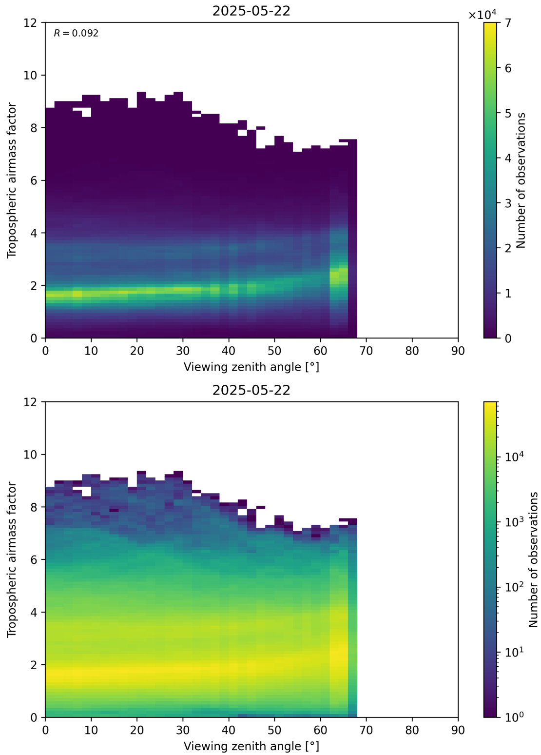
Figure 161: Scatter density plot of “Viewing zenith angle” against “Tropospheric airmass factor” for 2025-05-21 to 2025-05-23.
