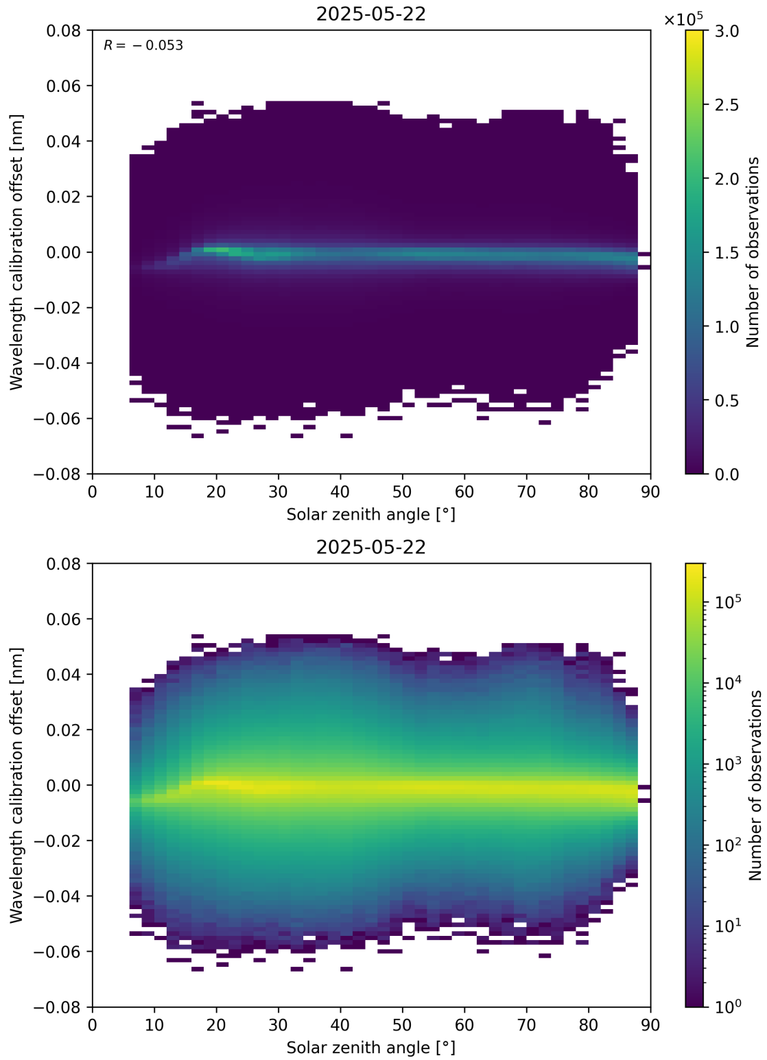
Figure 158: Scatter density plot of “Solar zenith angle” against “Wavelength calibration offset” for 2025-05-21 to 2025-05-23.
