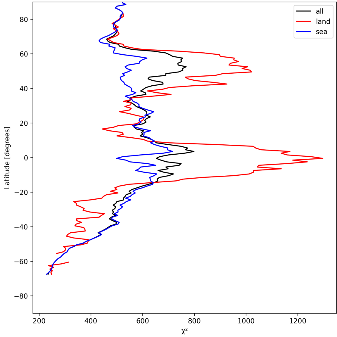
Figure 25: Zonal average of “ \chi^2 ” for 2025-05-21 to 2025-05-23.
