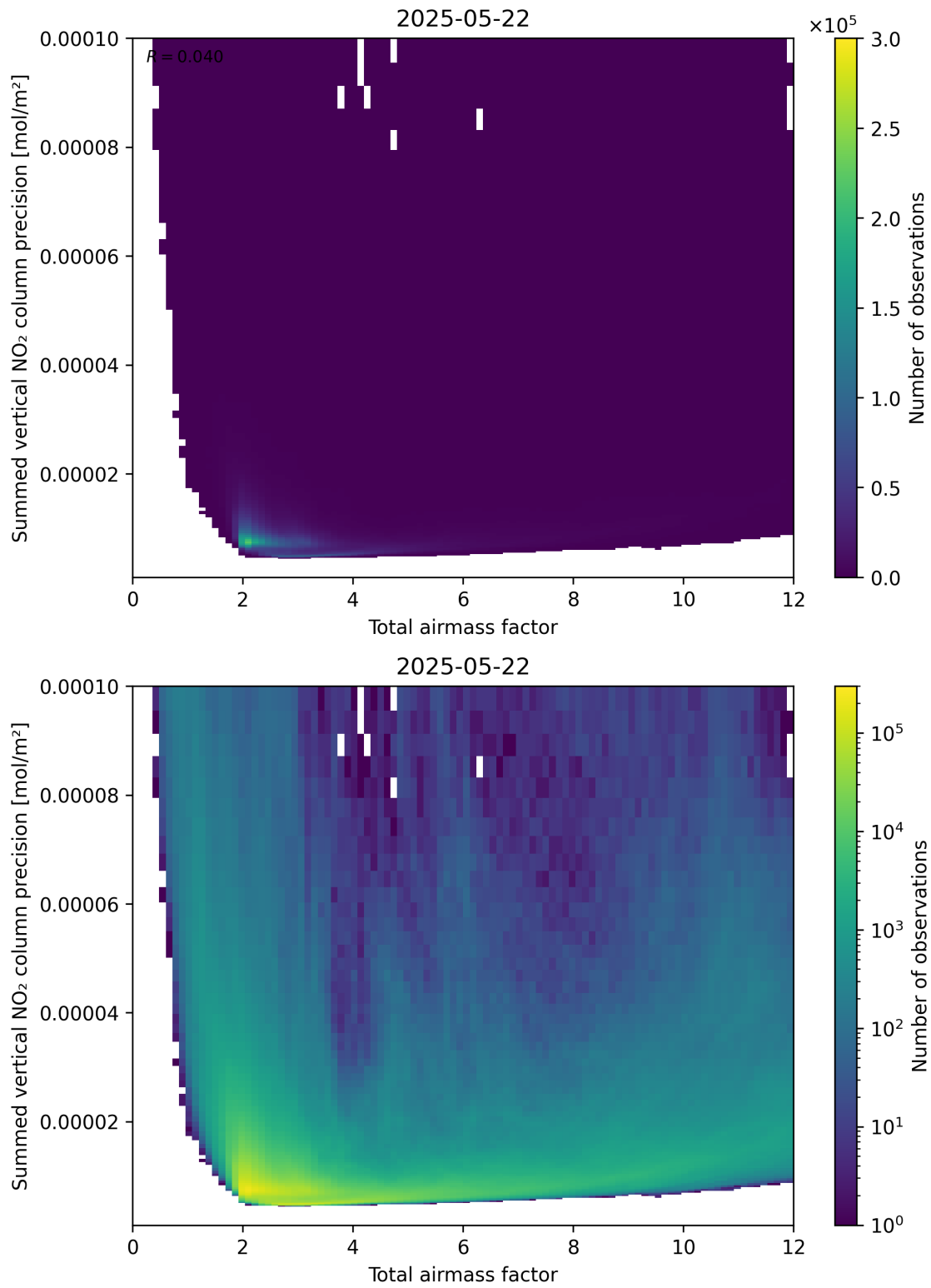
Figure 66: Scatter density plot of “Total airmass factor” against “Summed vertical NO 2 column precision” for 2025-05-21 to 2025-05-23.
