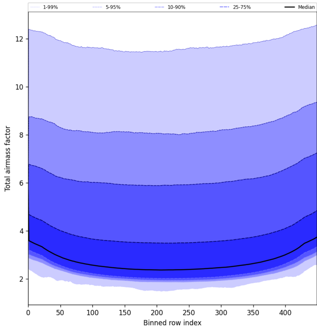
Figure 49: Along track statistics of “Total airmass factor” for 2025-05-21 to 2025-05-23
