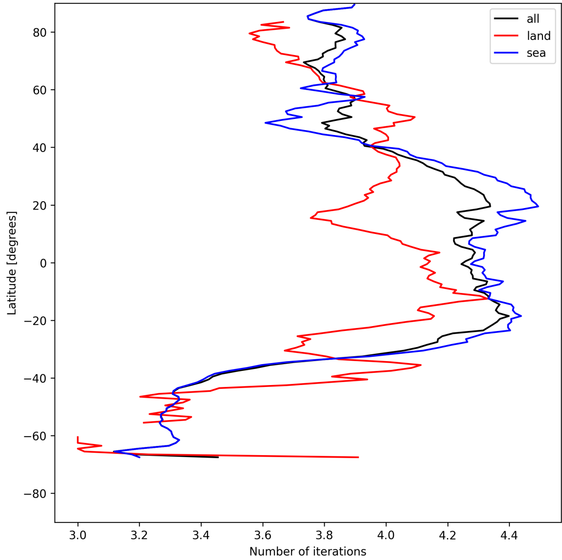
Figure 17: Zonal average of “Number of iterations” for 2025-05-21 to 2025-05-23.
