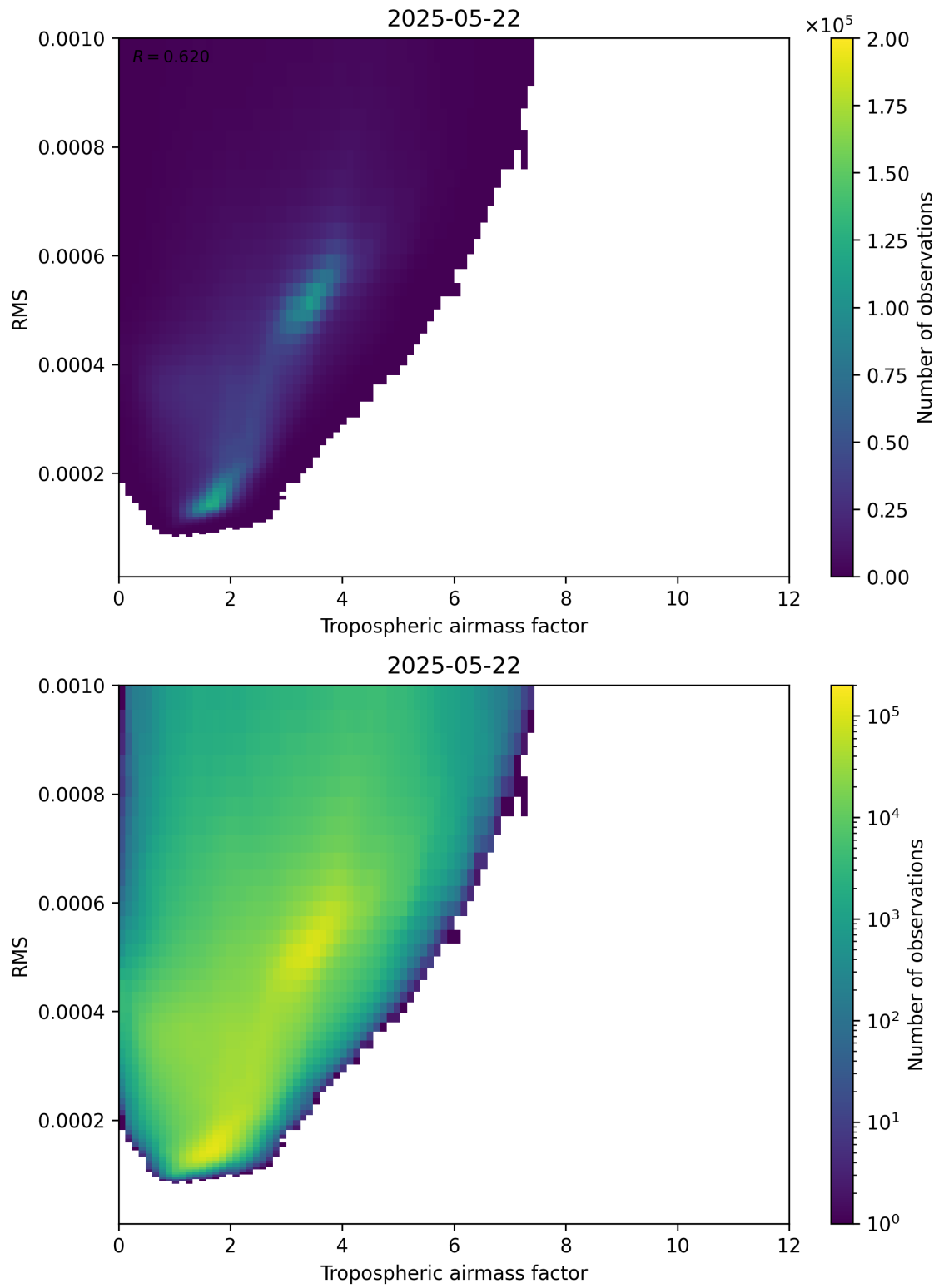
Figure 79: Scatter density plot of “Tropospheric airmass factor” against “RMS” for 2025-05-21 to 2025-05-23.
