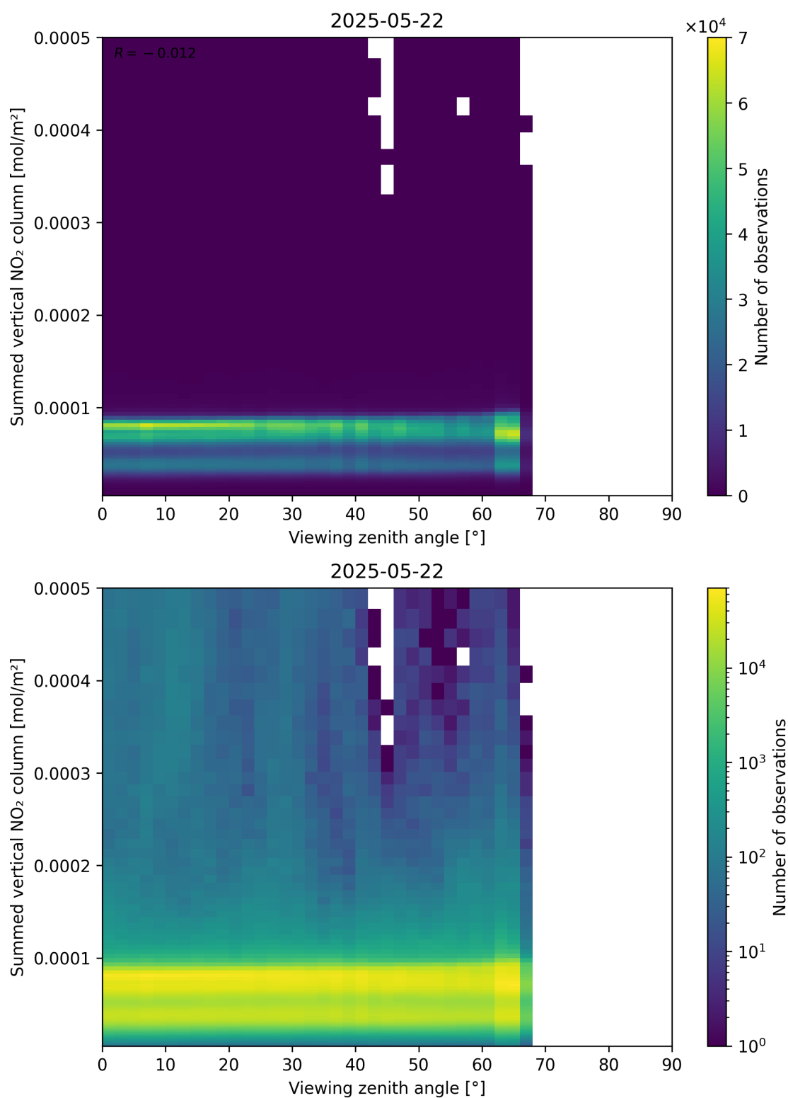
Figure 165: Scatter density plot of “Viewing zenith angle” against “Summed vertical NO 2 column” for 2025-05-21 to 2025-05-23.
