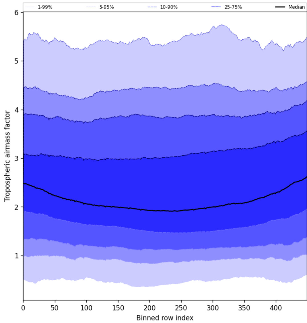
Figure 48: Along track statistics of “Tropospheric air mass factor” for 2025-05-21 to 2025-05-23
