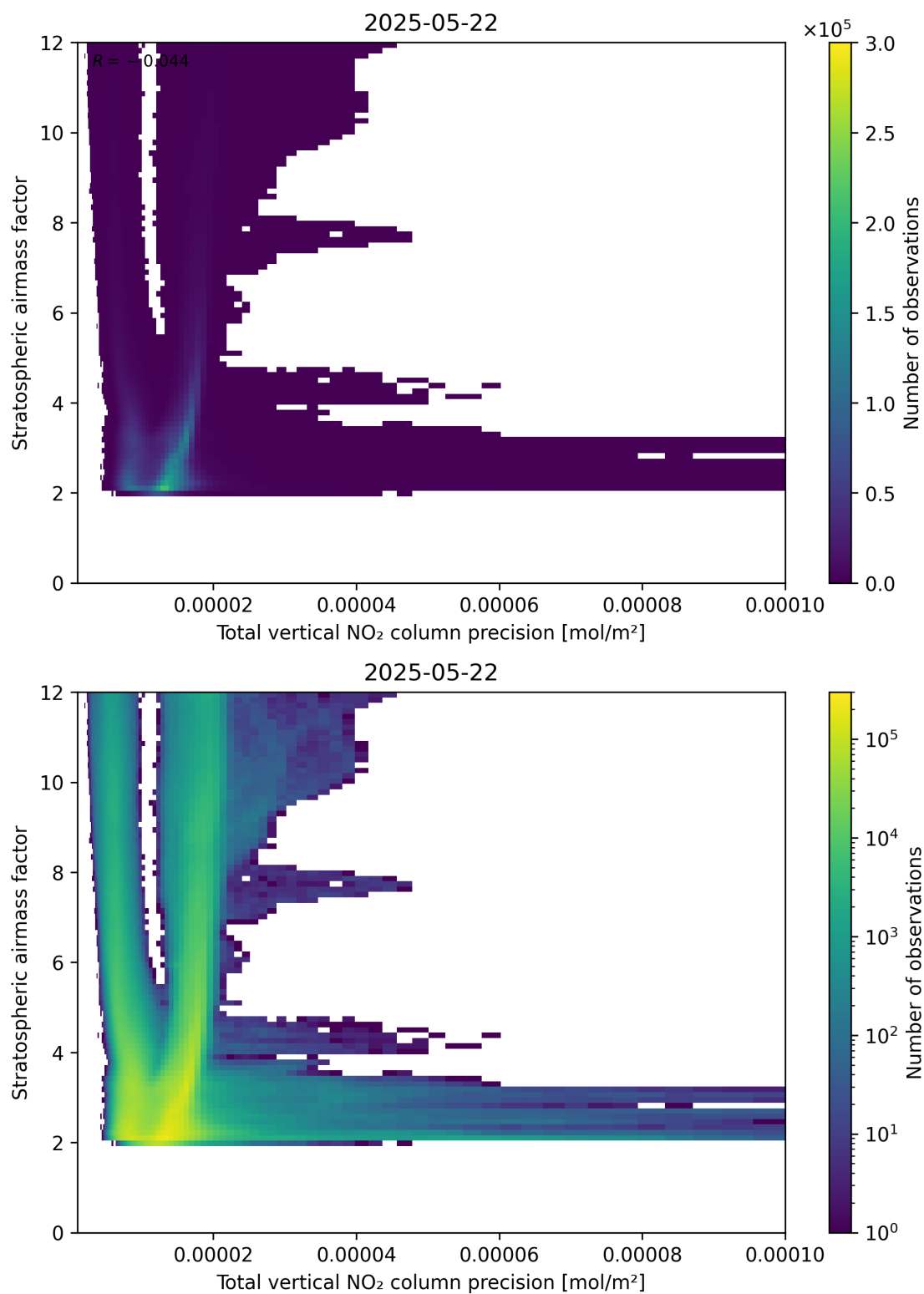
Figure 115: Scatter density plot of “Total vertical NO 2 column precision” against “Stratospheric air mass factor” for 2025-05-21 to 2025-05-23.
