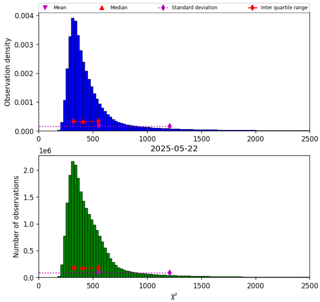
Figure 42: Histogram of " \chi^2 " for 2025-05-21 to 2025-05-23
