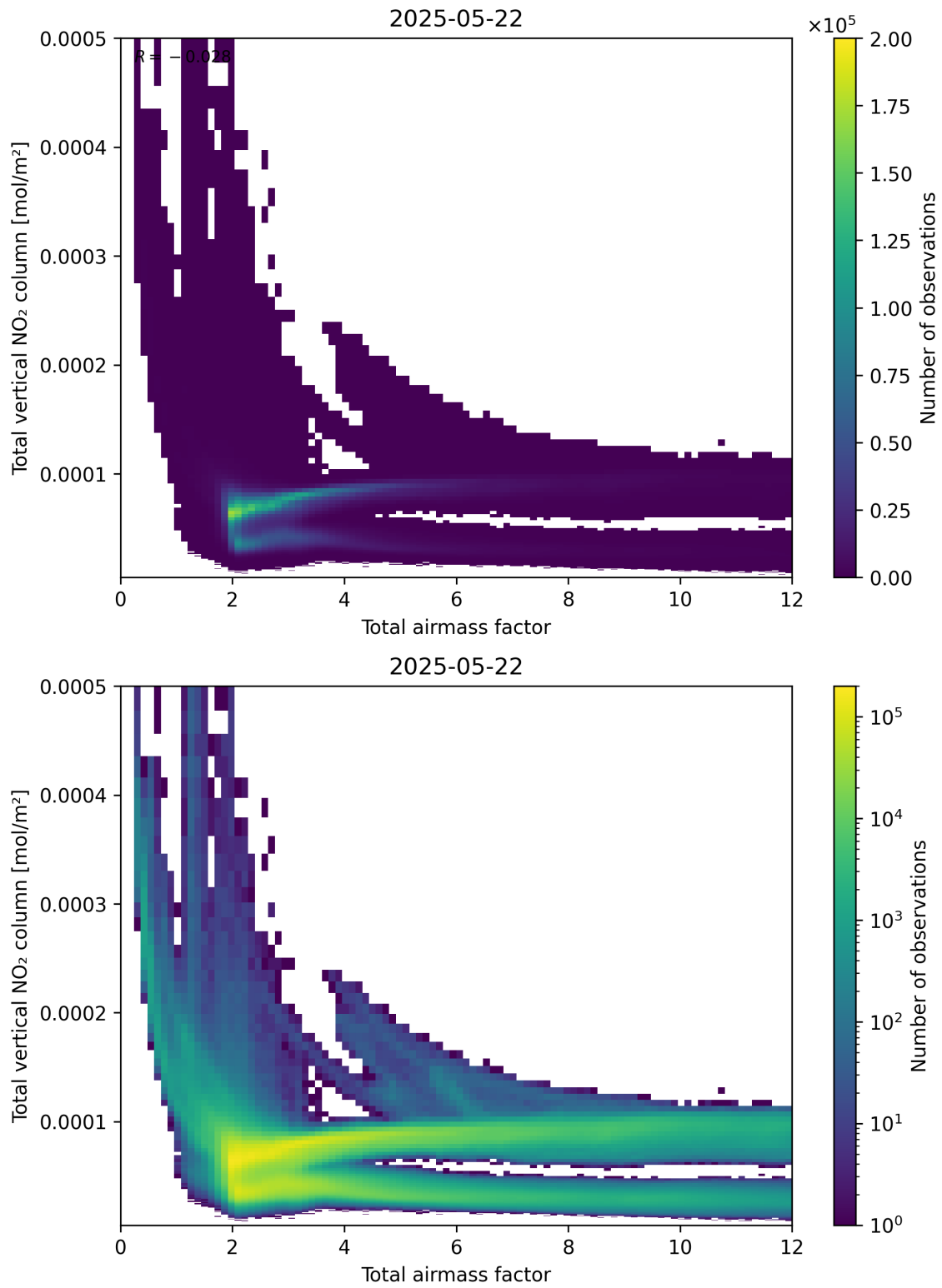
Figure 67: Scatter density plot of “Total airmass factor” against “Total vertical NO 2 column” for 2025-05-21 to 2025-05-23.
