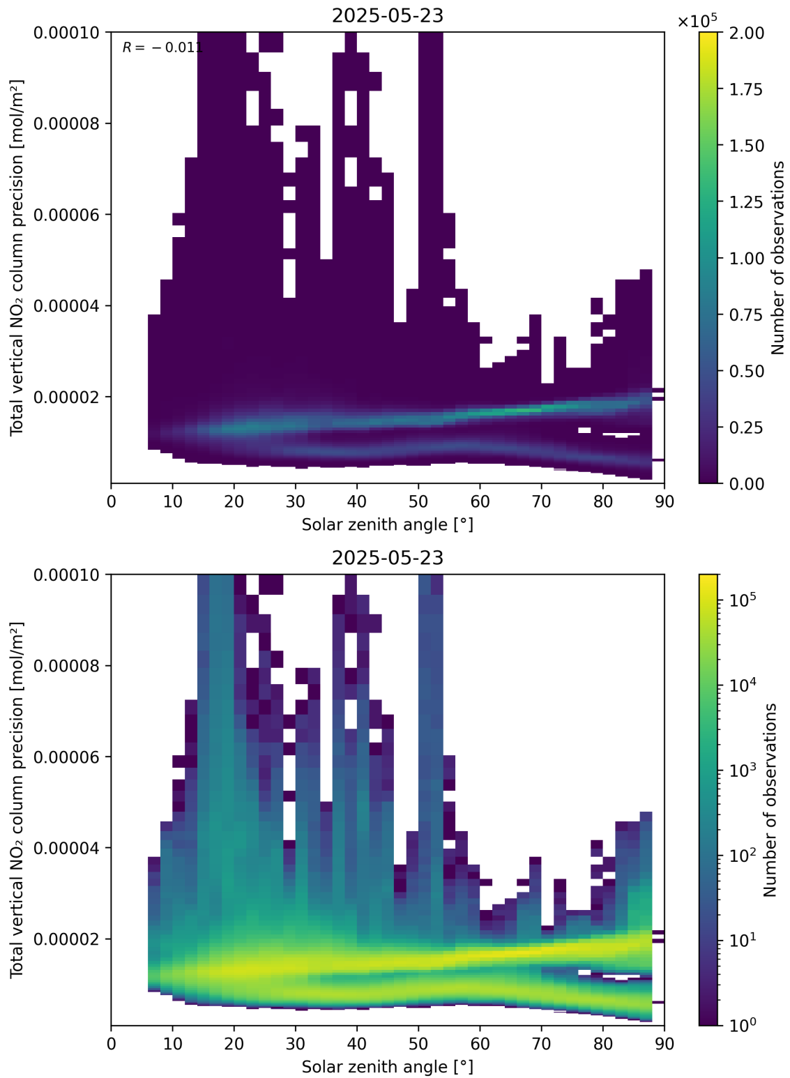
Figure 154: Scatter density plot of “Solar zenith angle” against “Total vertical NO 2 column precision” for 2025-05-22 to 2025-05-24.
