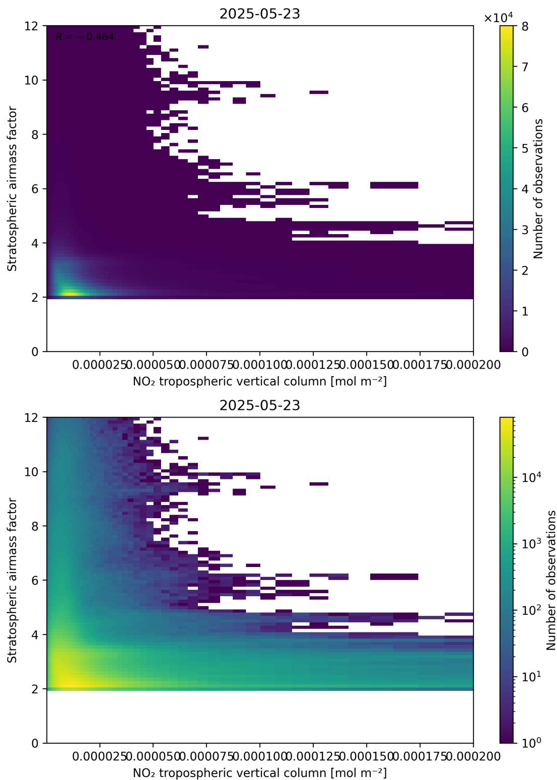
Figure 121: Scatter density plot of “NO 2 tropospheric vertical column” against “Stratospheric air mass factor” for 2025-05-22 to 2025-05-24.
