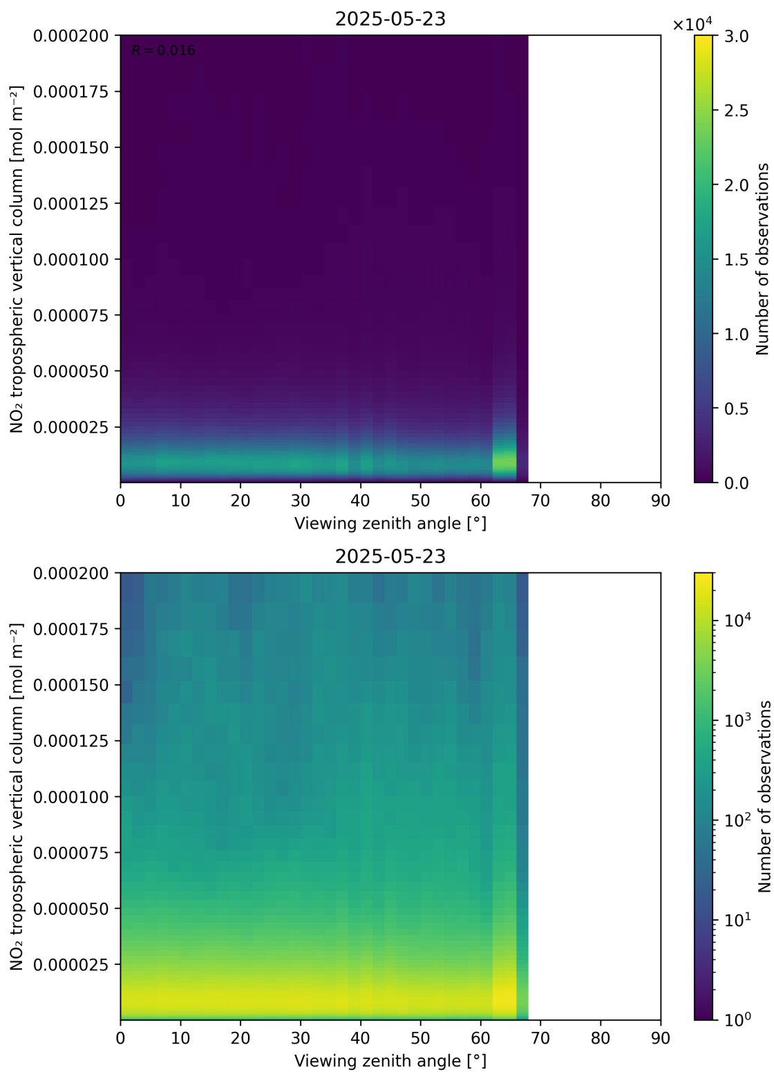
Figure 169: Scatter density plot of “Viewing zenith angle” against “NO 2 tropospheric vertical column” for 2025-05-22 to 2025-05-24.
