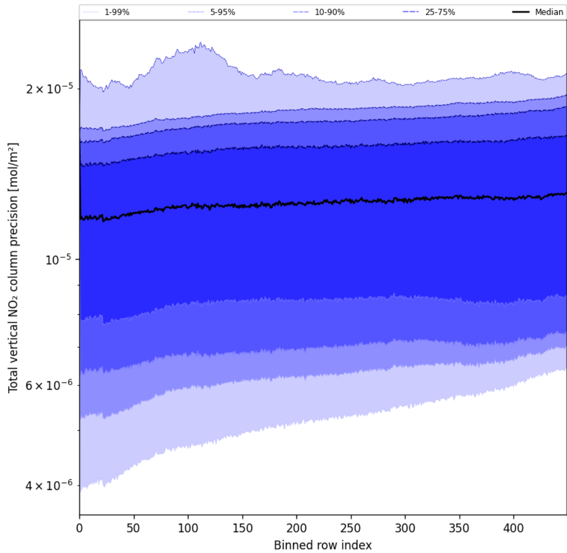
Figure 56: Along track statistics of "Total vertical NO 2 column precision" for 2025-05-22 to 2025-05-24
