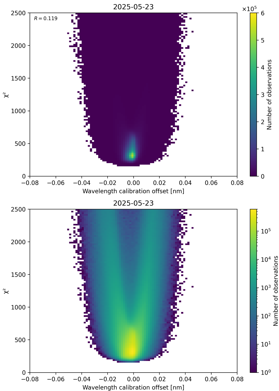
Figure 175: Scatter density plot of “Wavelength calibration offset” against “ \chi^2 ” for 2025-05-22 to 2025-05-24.
