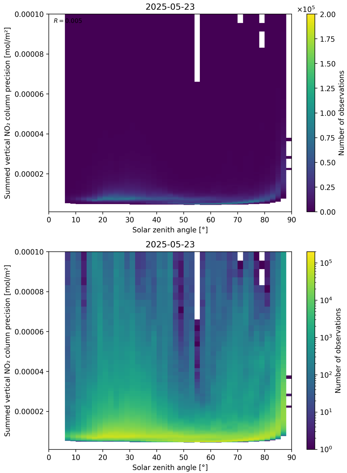
Figure 152: Scatter density plot of “Solar zenith angle” against “Summed vertical NO 2 column precision” for 2025-05-22 to 2025-05-24.
