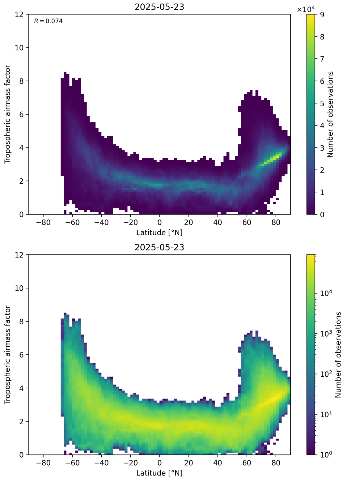
Figure 85: Scatter density plot of “Latitude” against “Tropospheric air mass factor” for 2025-05-22 to 2025-05-24.
