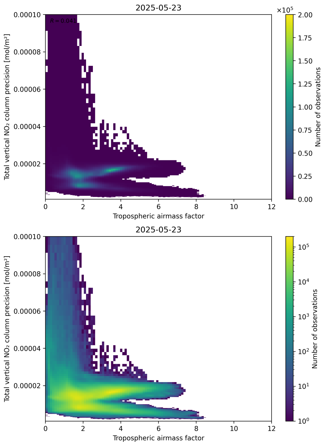
Figure 78: Scatter density plot of “Tropospheric air mass factor” against “Total vertical NO 2 column precision” for 2025-05-22 to 2025-05-24.
