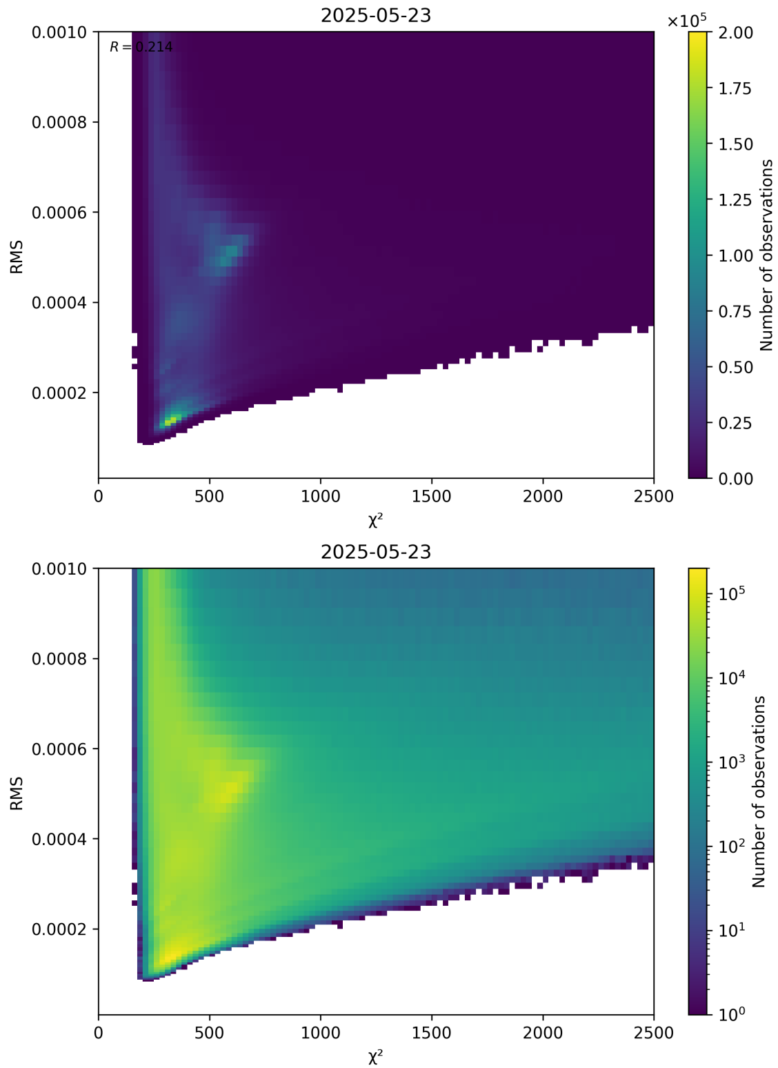
Figure 82: Scatter density plot of “ \chi^2 ” against “RMS” for 2025-05-22 to 2025-05-24.
