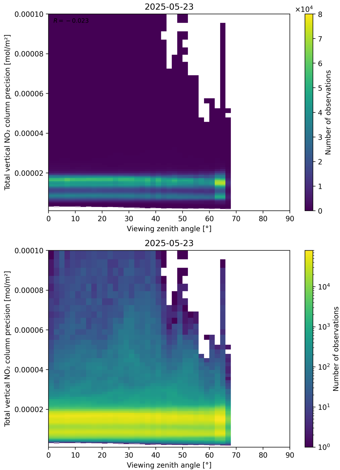
Figure 168: Scatter density plot of “Viewing zenith angle” against “Total vertical NO 2 column precision” for 2025-05-22 to 2025-05-24.
