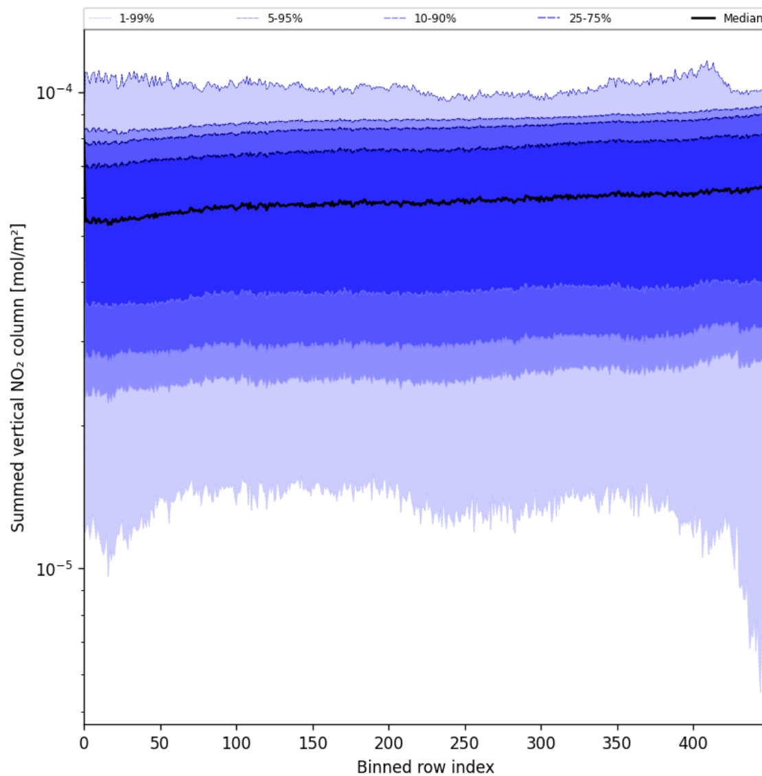
Figure 57: Along track statistics of “Summed vertical NO 2 column” for 2025-05-22 to 2025-05-24
