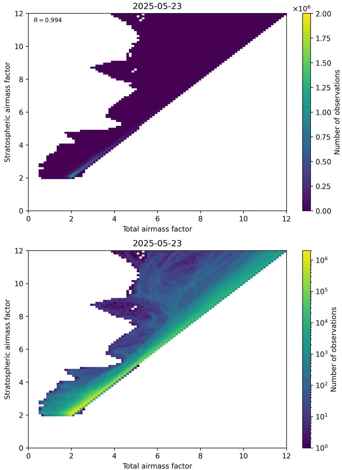
Figure 62: Scatter density plot of “Total airmass factor” against “Stratospheric airmass factor” for 2025-05-22 to 2025-05-24.
