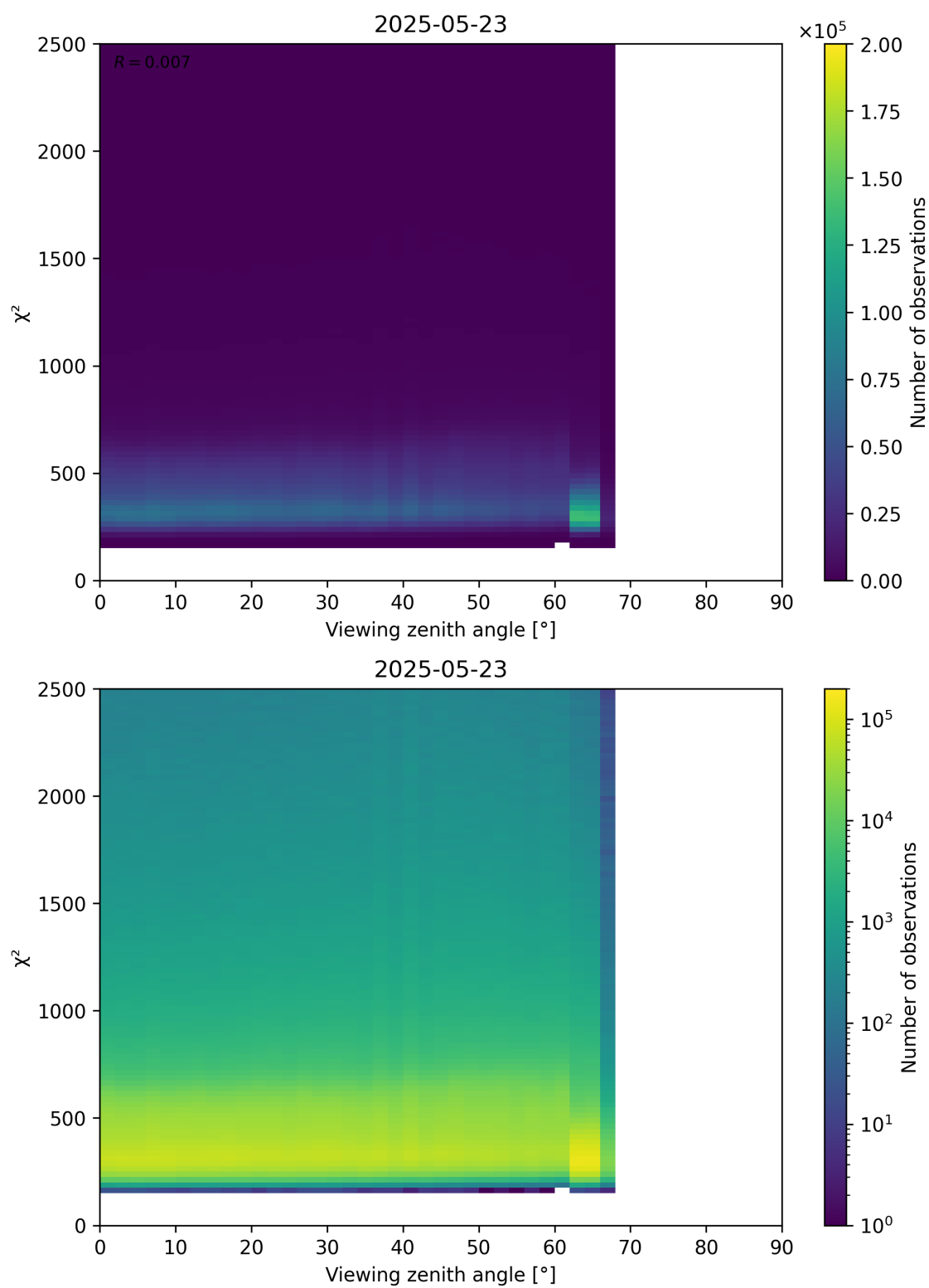
Figure 162: Scatter density plot of “Viewing zenith angle” against “ \chi^2 ” for 2025-05-22 to 2025-05-24.
