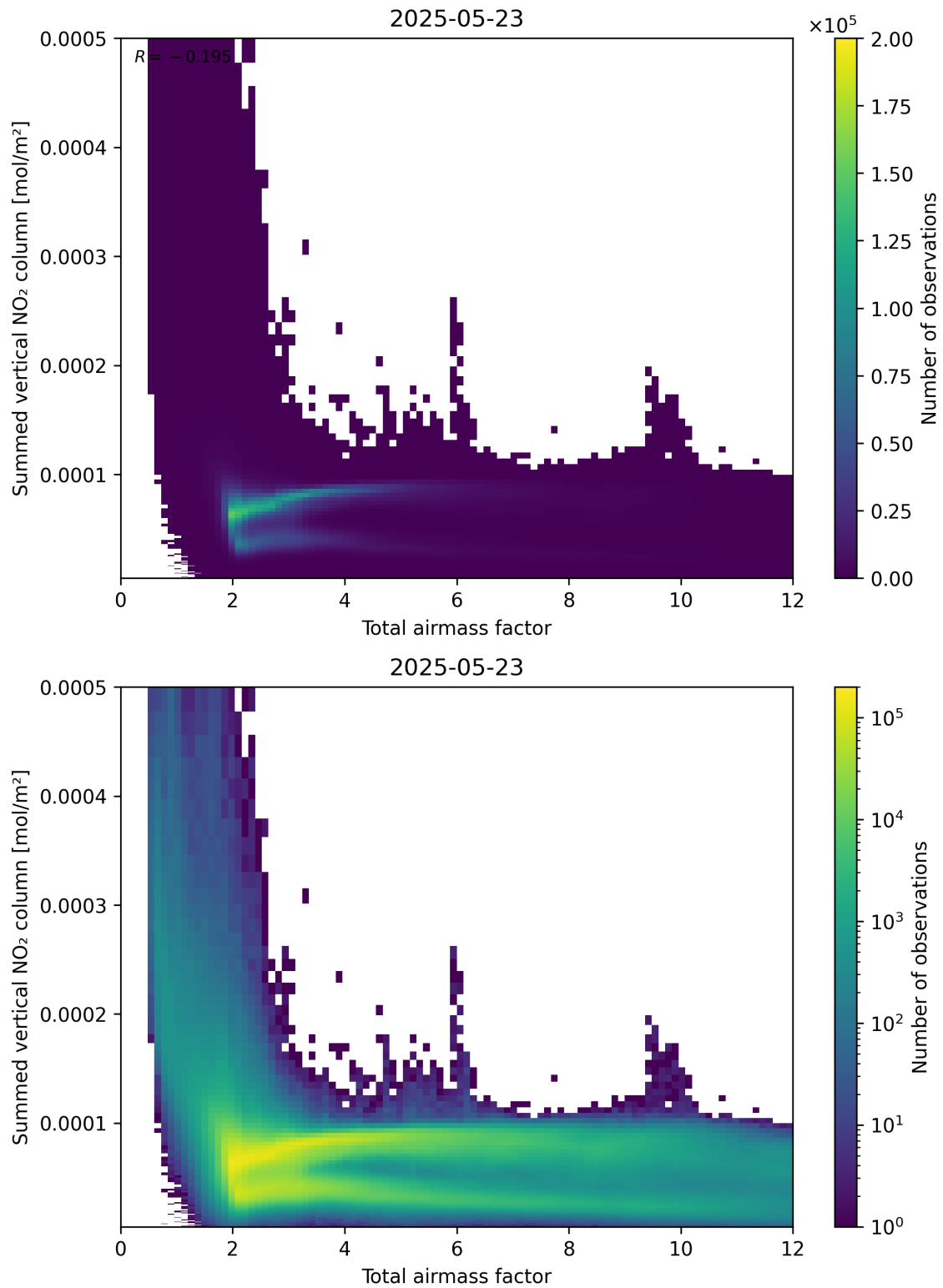
Figure 65: Scatter density plot of “Total airmass factor” against “Summed vertical NO 2 column” for 2025-05-22 to 2025-05-24.
