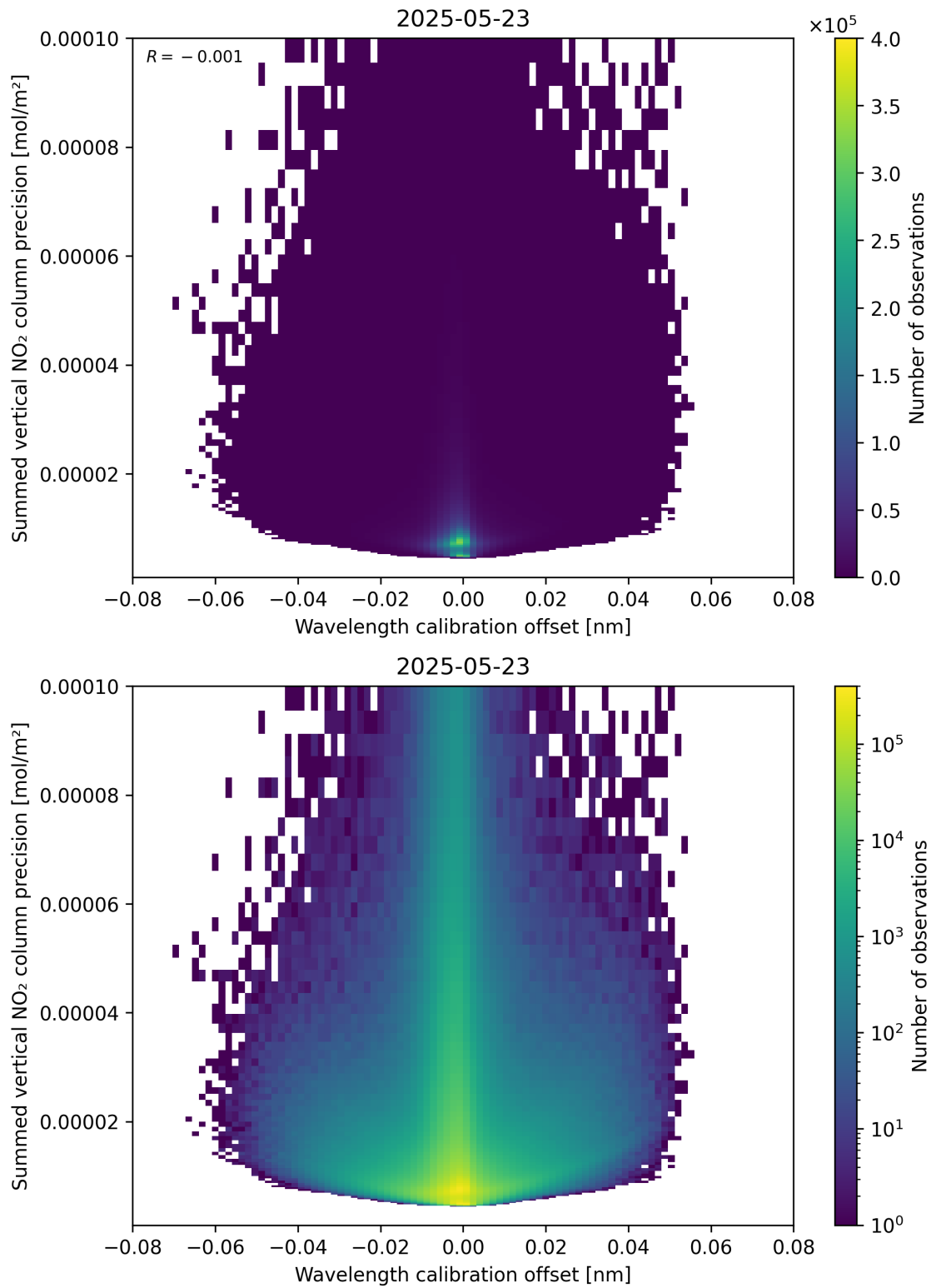
Figure 178: Scatter density plot of “Wavelength calibration offset” against “Summed vertical NO 2 column precision” for 2025-05-22 to 2025-05-24.
