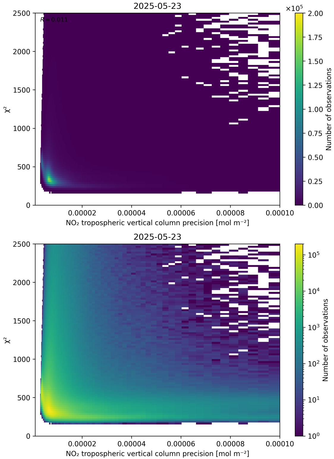
Figure 134: Scatter density plot of “NO 2 tropospheric vertical column precision” against “ \chi^2 ” for 2025-05-22 to 2025-05-24.
