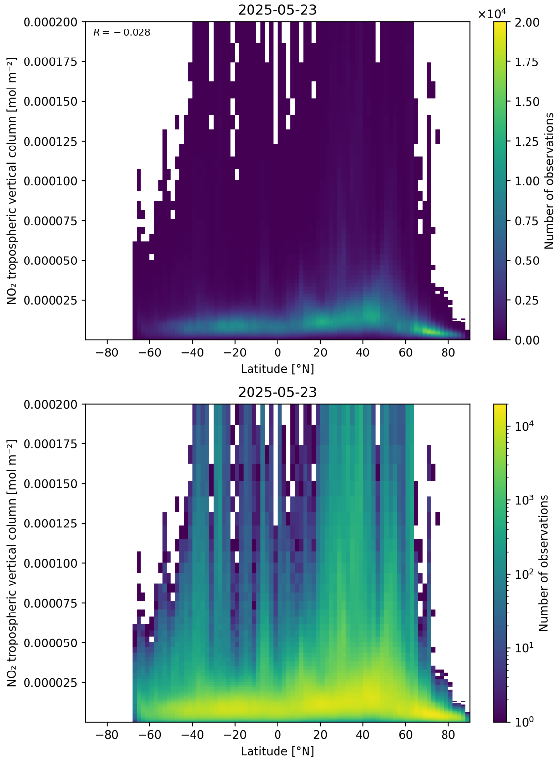
Figure 92: Scatter density plot of “Latitude” against “NO 2 tropospheric vertical column” for 2025-05-22 to 2025-05-24.
