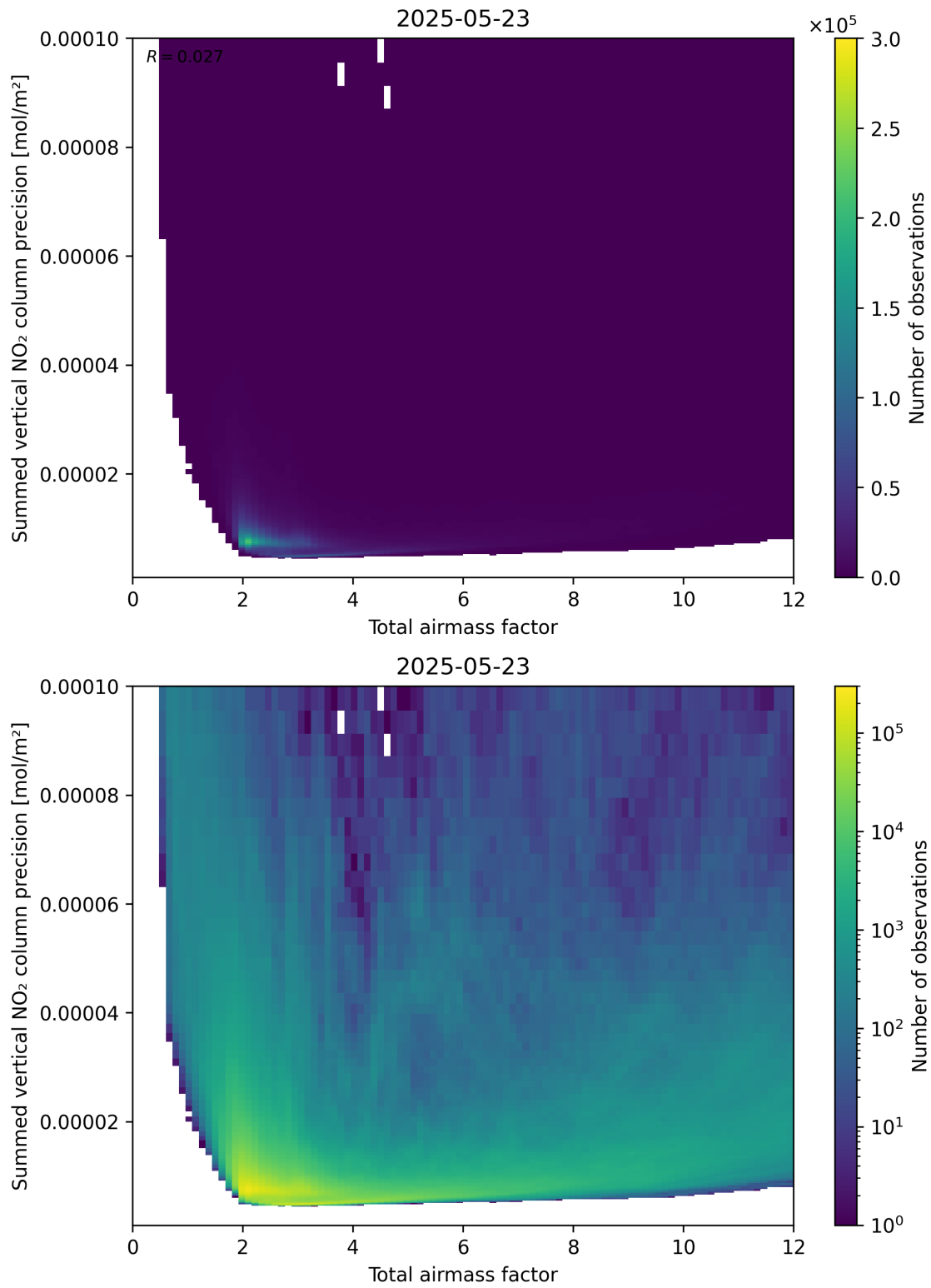
Figure 66: Scatter density plot of “Total airmass factor” against “Summed vertical NO 2 column precision” for 2025-05-22 to 2025-05-24.
