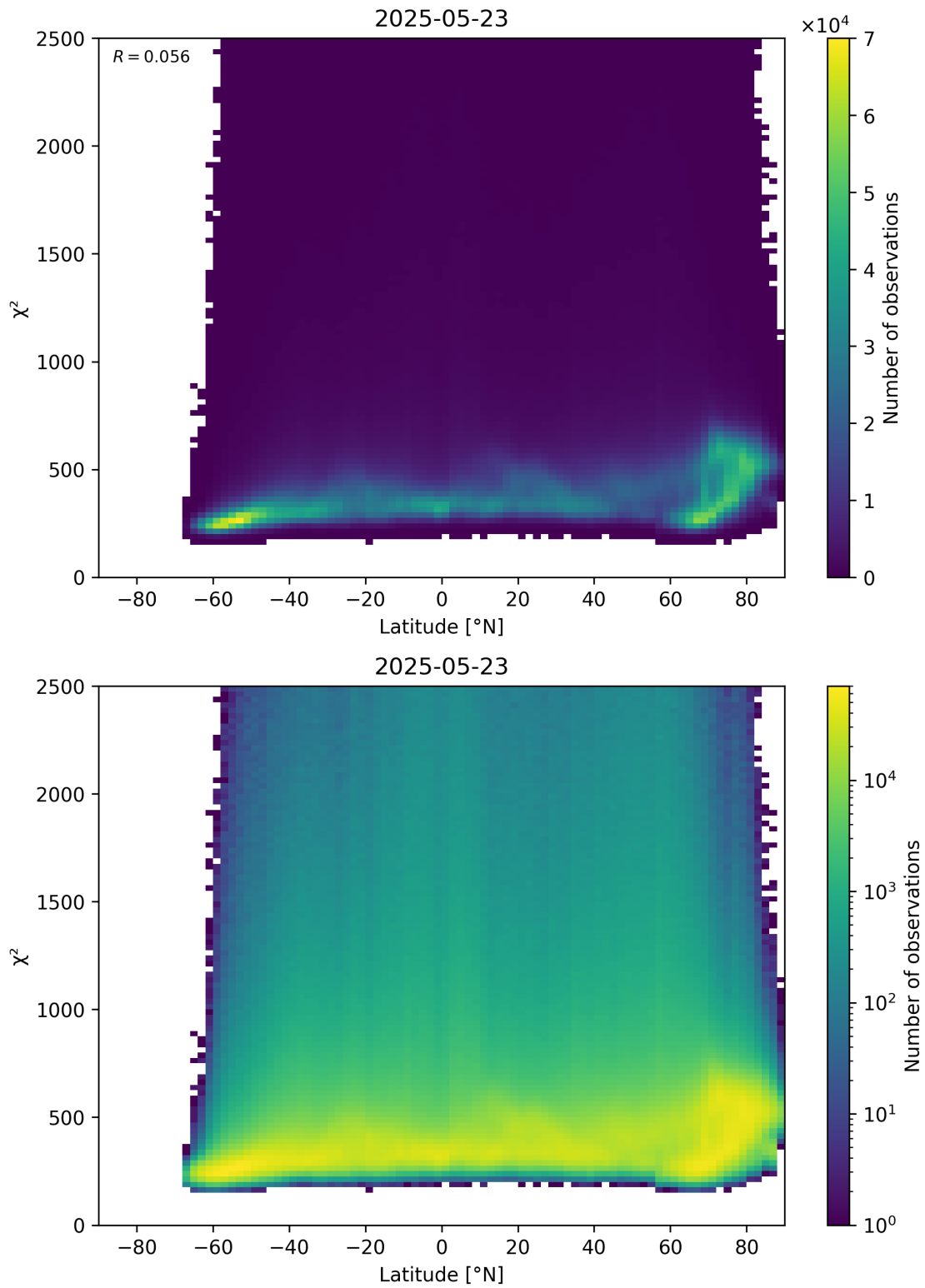
Figure 86: Scatter density plot of “Latitude” against “ \chi^2 ” for 2025-05-22 to 2025-05-24.
