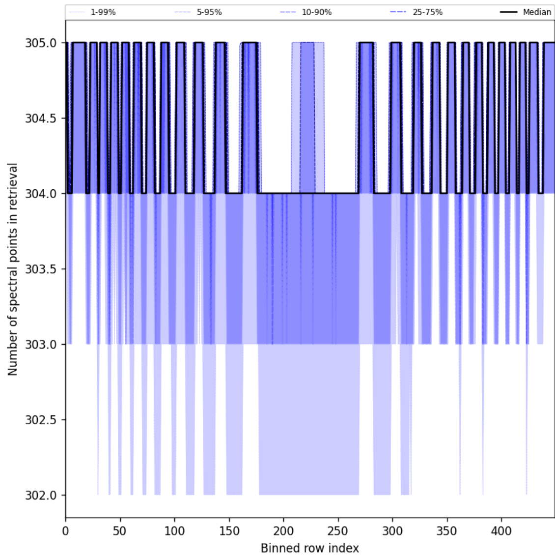
Figure 50: Along track statistics of “Number of spectral points in retrieval” for 2025-05-22 to 2025-05-24
