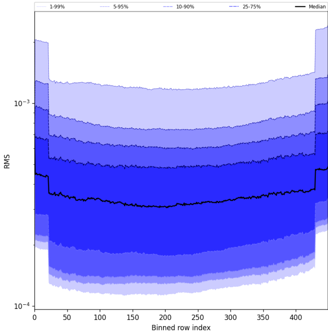
Figure 60: Along track statistics of “RMS” for 2025-05-22 to 2025-05-24
