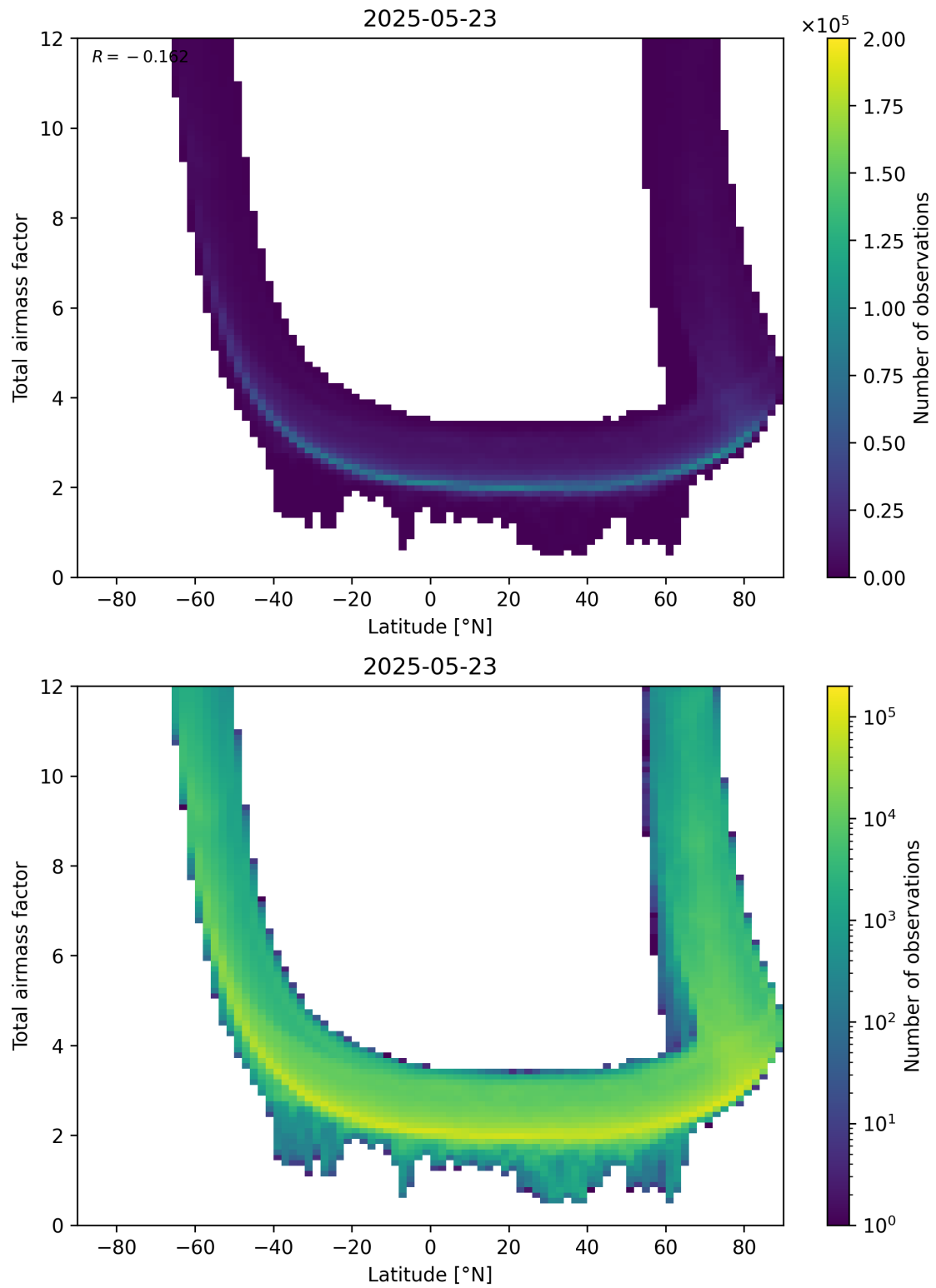
Figure 84: Scatter density plot of “Latitude” against “Total airmass factor” for 2025-05-22 to 2025-05-24.
