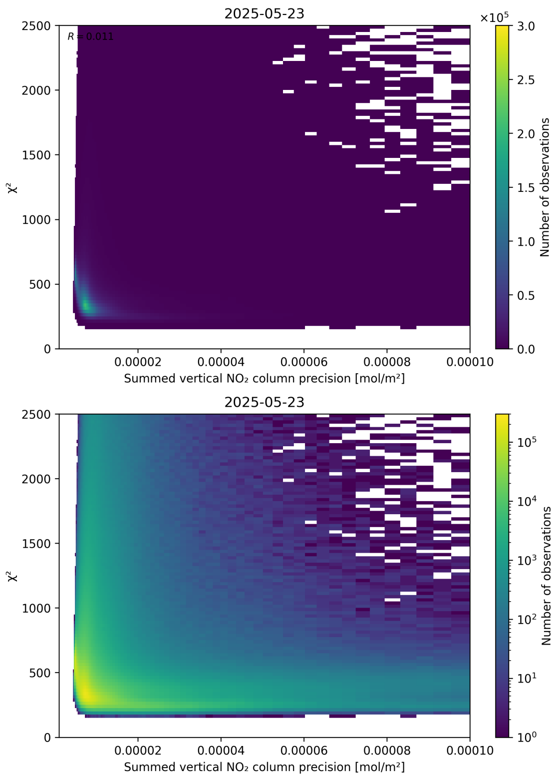
Figure 107: Scatter density plot of “Summed vertical NO 2 column precision” against “ \chi^2 ” for 2025-05-22 to 2025-05-24.
