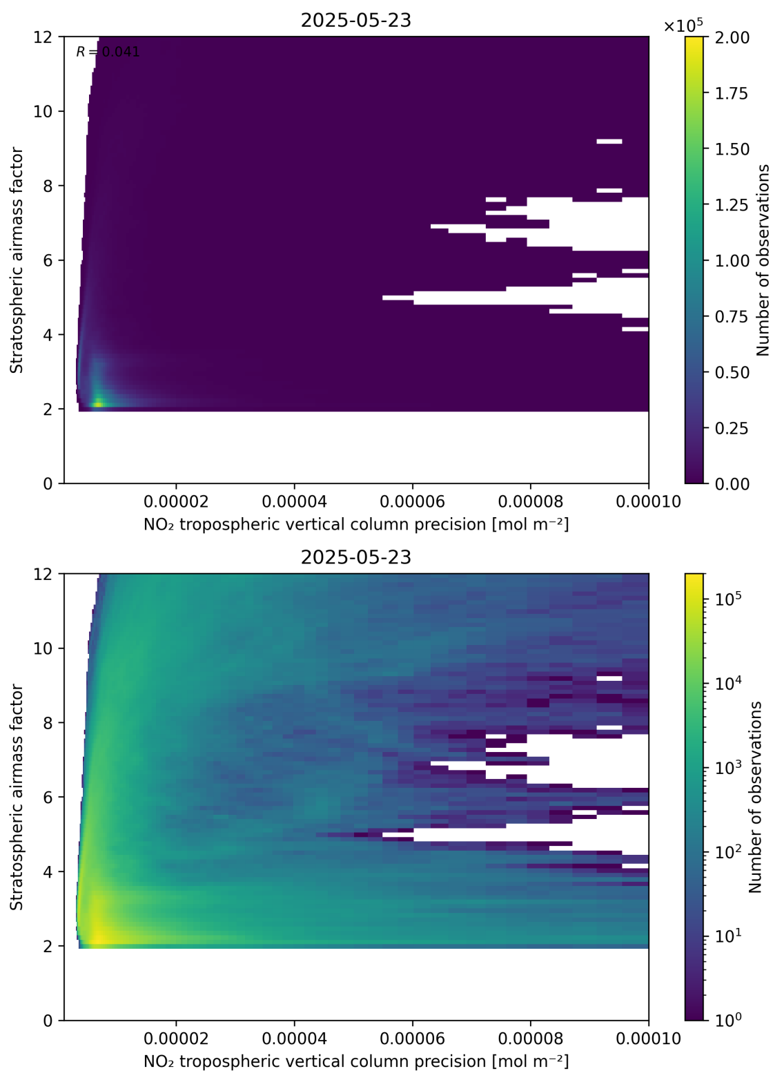
Figure 131: Scatter density plot of “NO 2 tropospheric vertical column precision” against “Stratospheric airmass factor” for 2025-05-22 to 2025-05-24.
