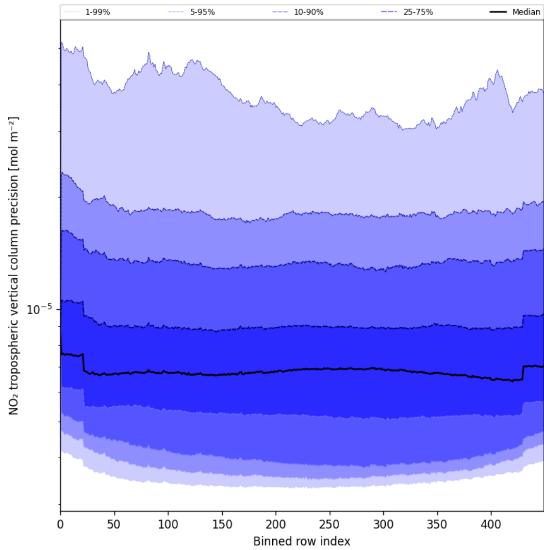
Figure 47: Along track statistics of “NO 2 tropospheric vertical column precision” for 2025-05-22 to 2025-05-24
