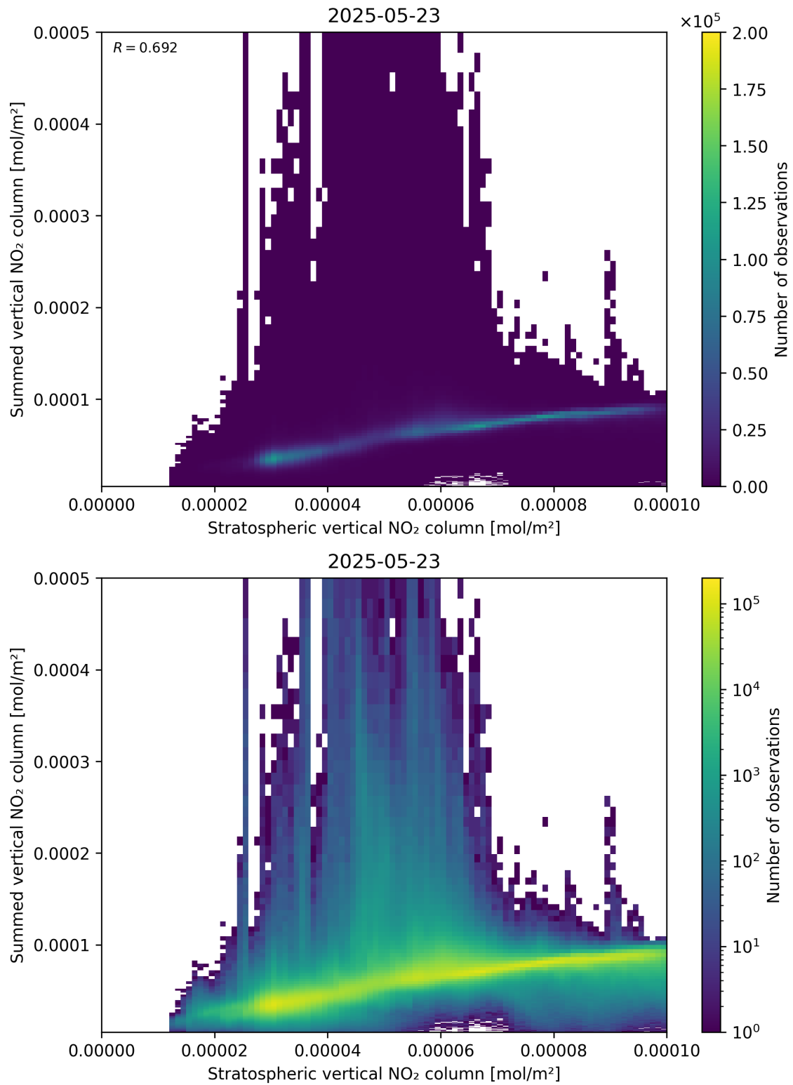
Figure 98: Scatter density plot of “Stratospheric vertical NO 2 column” against “Summed vertical NO 2 column” for 2025-05-22 to 2025-05-24.
