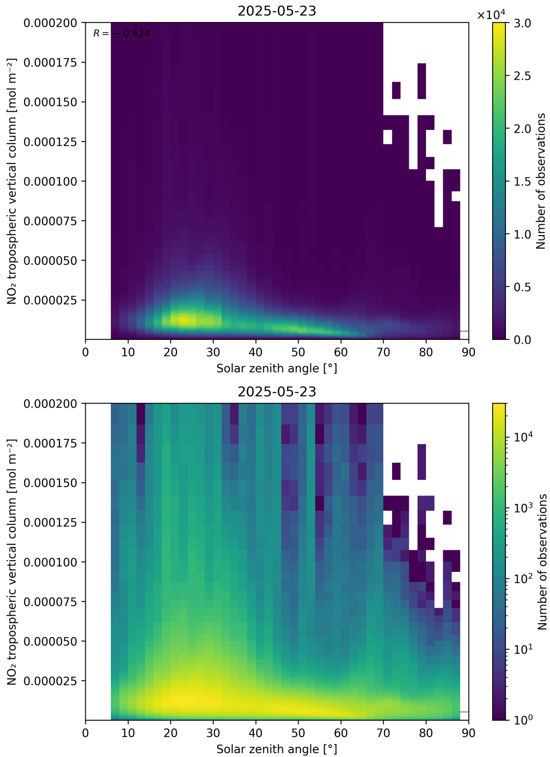
Figure 155: Scatter density plot of “Solar zenith angle” against “NO 2 tropospheric vertical column” for 2025-05-22 to 2025-05-24.
