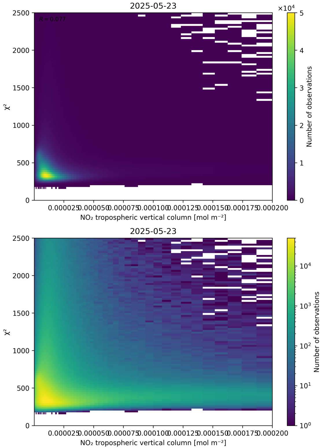
Figure 124: Scatter density plot of “NO 2 tropospheric vertical column” against “ \chi^2 ” for 2025-05-22 to 2025-05-24.
