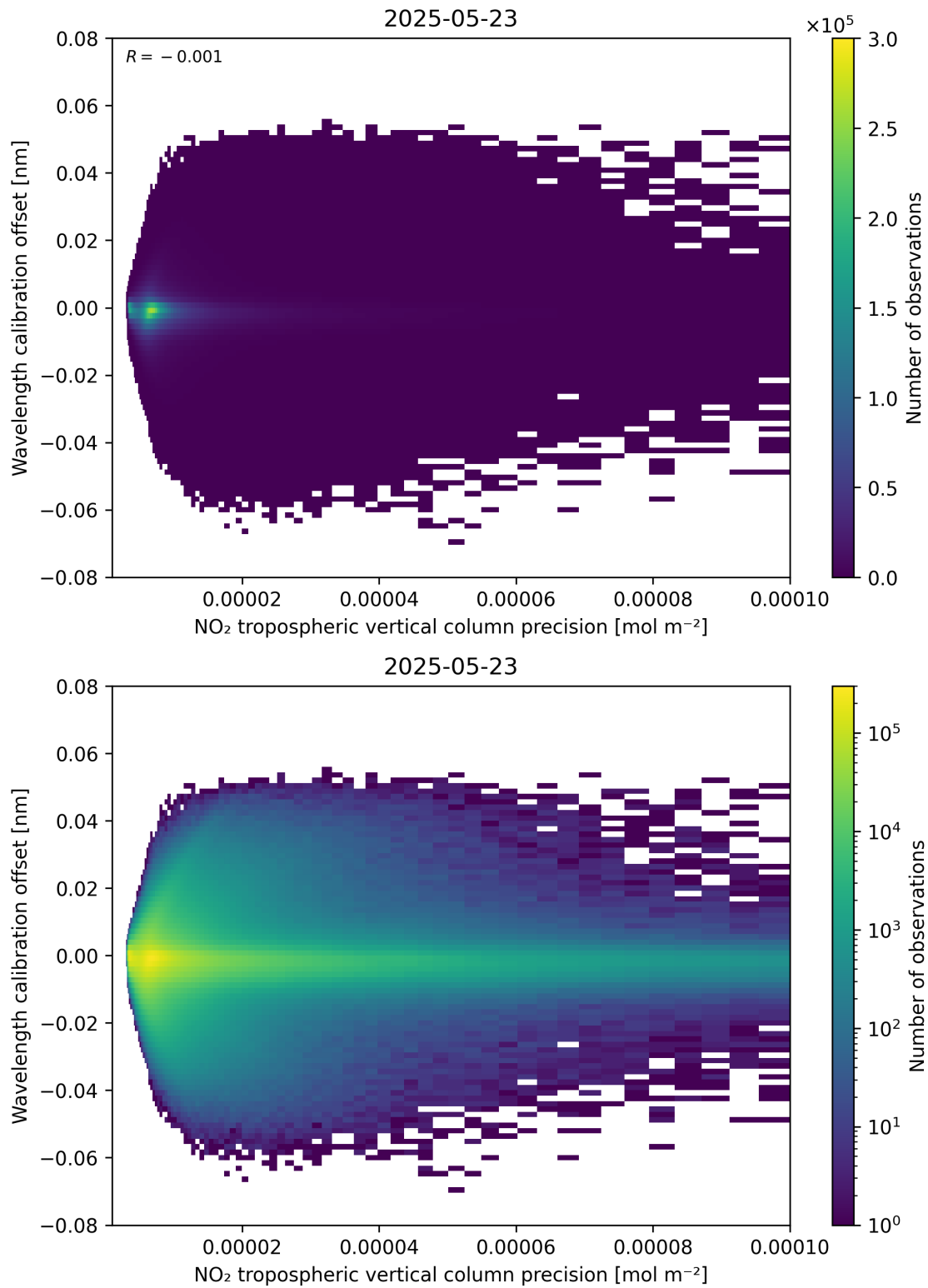
Figure 141: Scatter density plot of “NO 2 tropospheric vertical column precision” against “Wavelength calibration offset” for 2025-05-22 to 2025-05-24.
