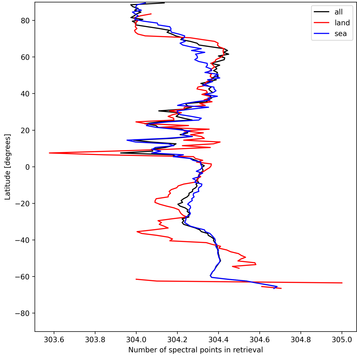
Figure 16: Zonal average of “Number of spectral points in retrieval” for 2025-05-22 to 2025-05-24.
