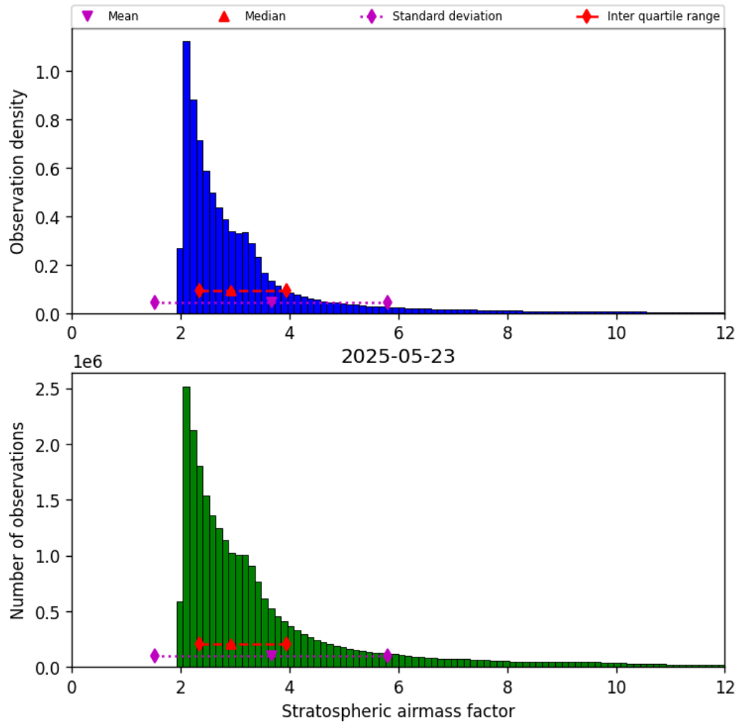
Figure 44: Histogram of “Stratospheric airmass factor” for 2025-05-22 to 2025-05-24
