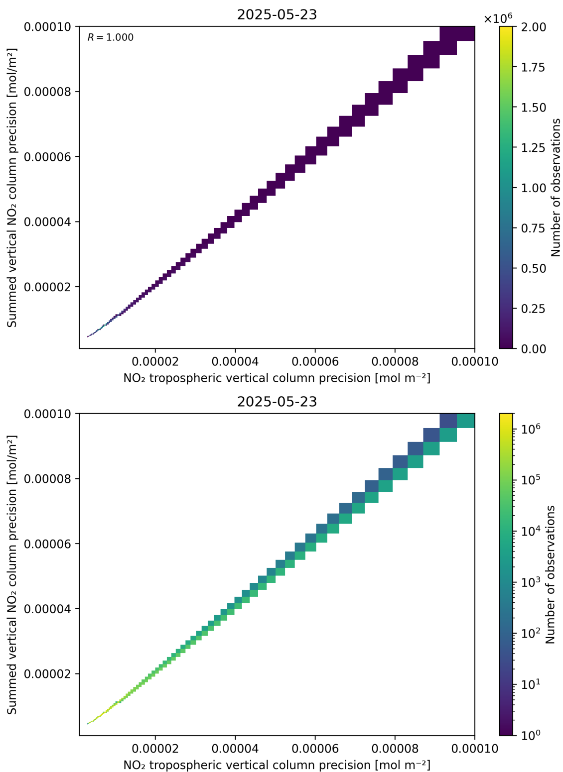
Figure 137: Scatter density plot of “NO 2 tropospheric vertical column precision” against “Summed vertical NO 2 column precision” for 2025-05-22 to 2025-05-24.
