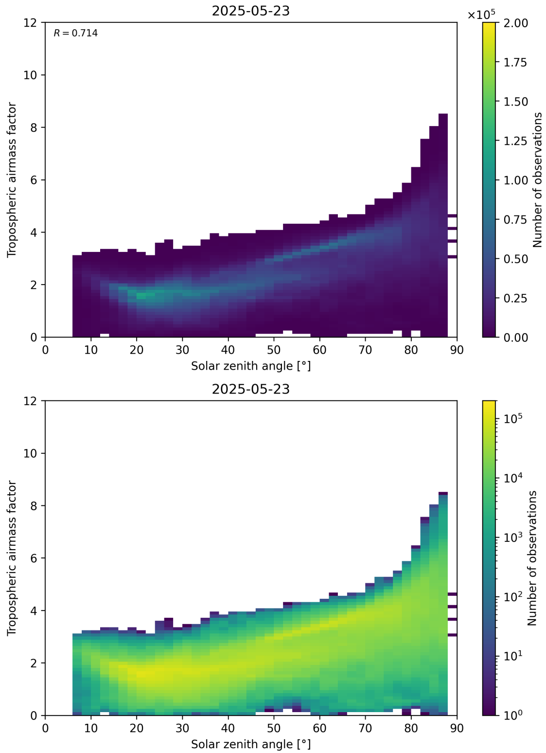
Figure 147: Scatter density plot of “Solar zenith angle” against “Tropospheric airmass factor” for 2025-05-22 to 2025-05-24.
