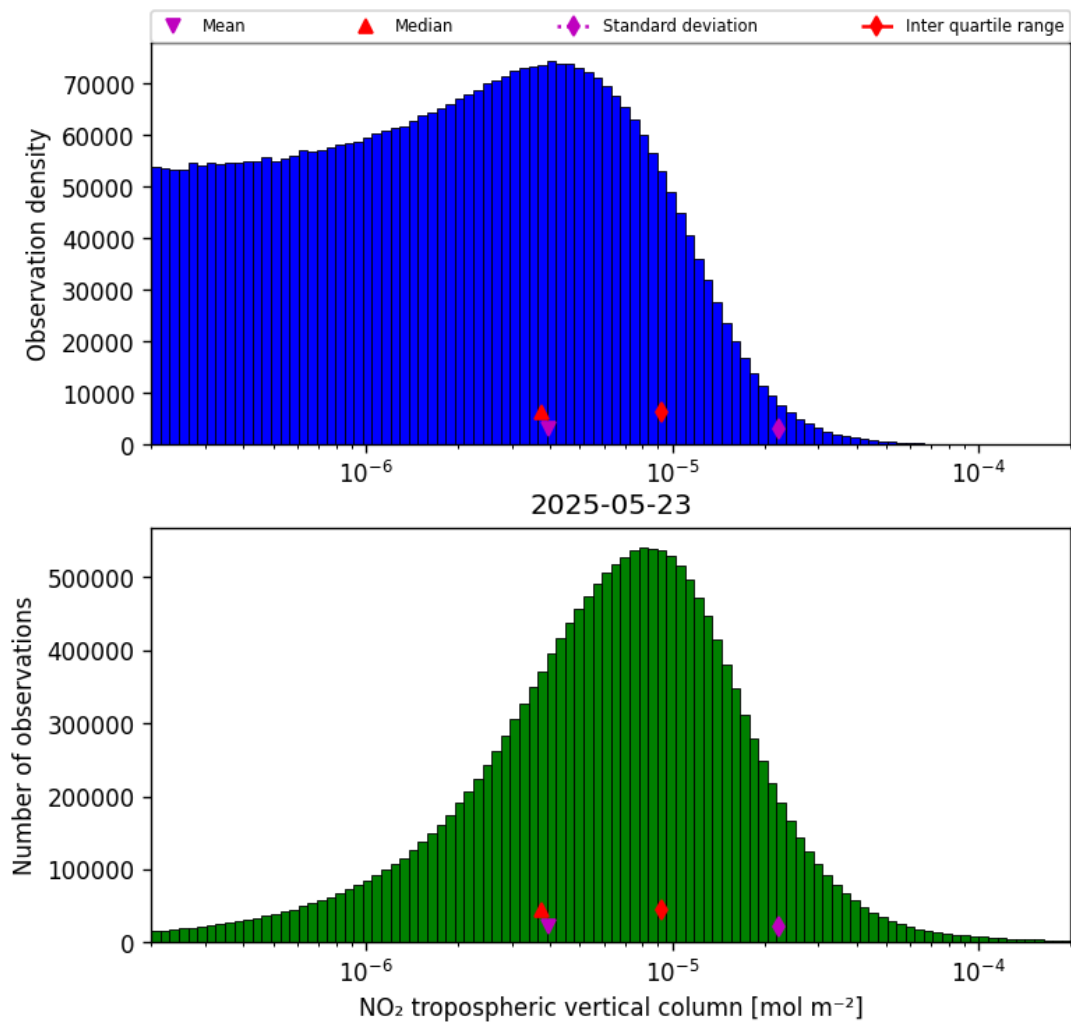
Figure 29: Histogram of “NO 2 tropospheric vertical column” for 2025-05-22 to 2025-05-24
