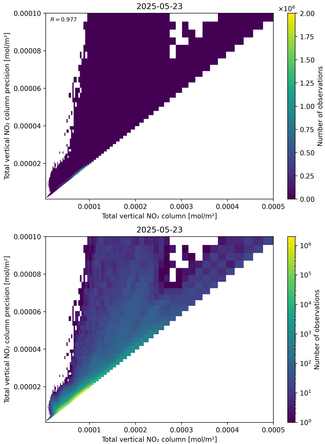
Figure 114: Scatter density plot of “Total vertical NO 2 column” against “Total vertical NO 2 column precision” for 2025-05-22 to 2025-05-24.
