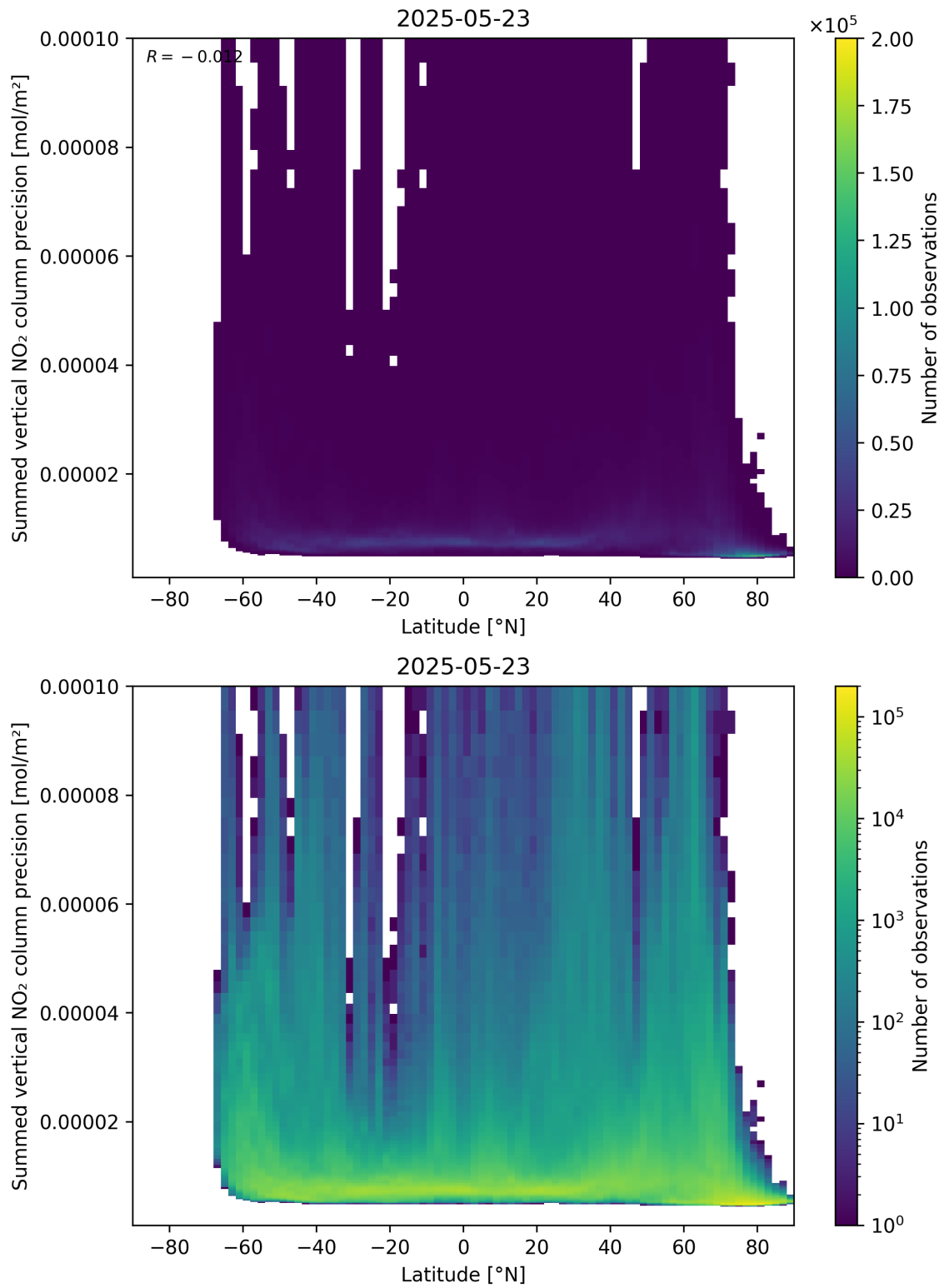
Figure 89: Scatter density plot of “Latitude” against “Summed vertical NO 2 column precision” for 2025-05-22 to 2025-05-24.
