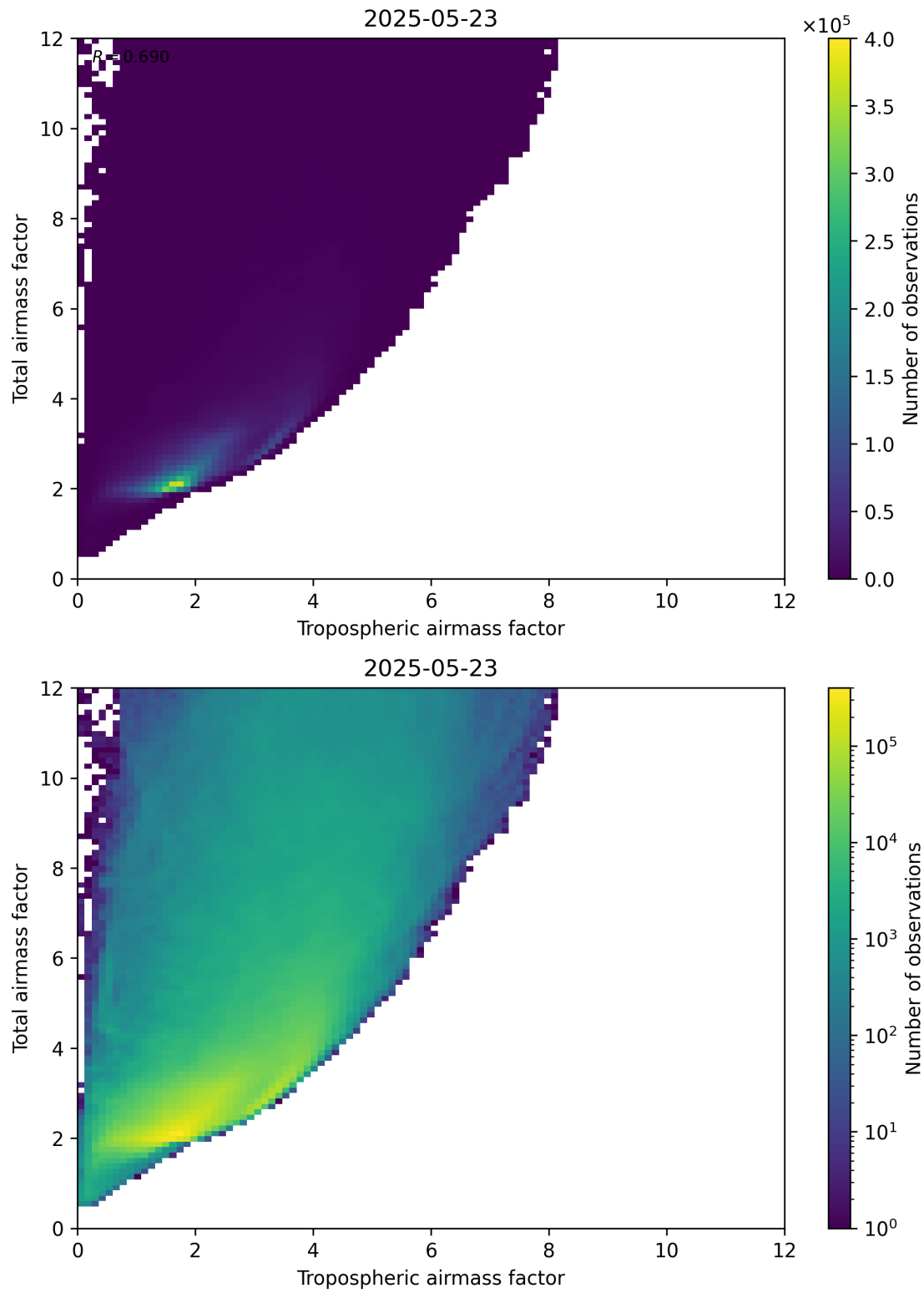
Figure 72: Scatter density plot of “Tropospheric airmass factor” against “Total airmass factor” for 2025-05-22 to 2025-05-24.
