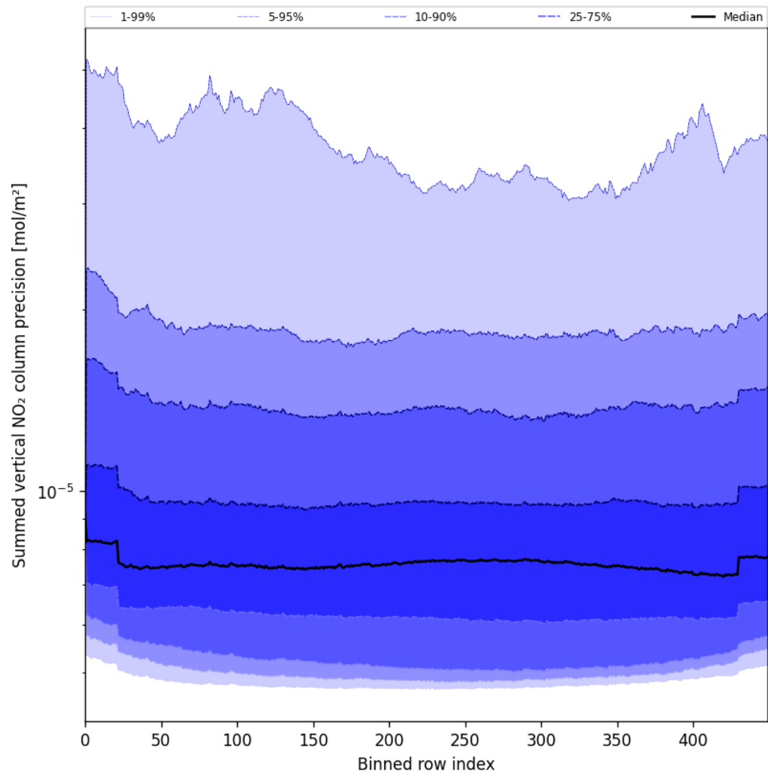
Figure 58: Along track statistics of “Summed vertical NO 2 column precision” for 2025-05-22 to 2025-05-24
