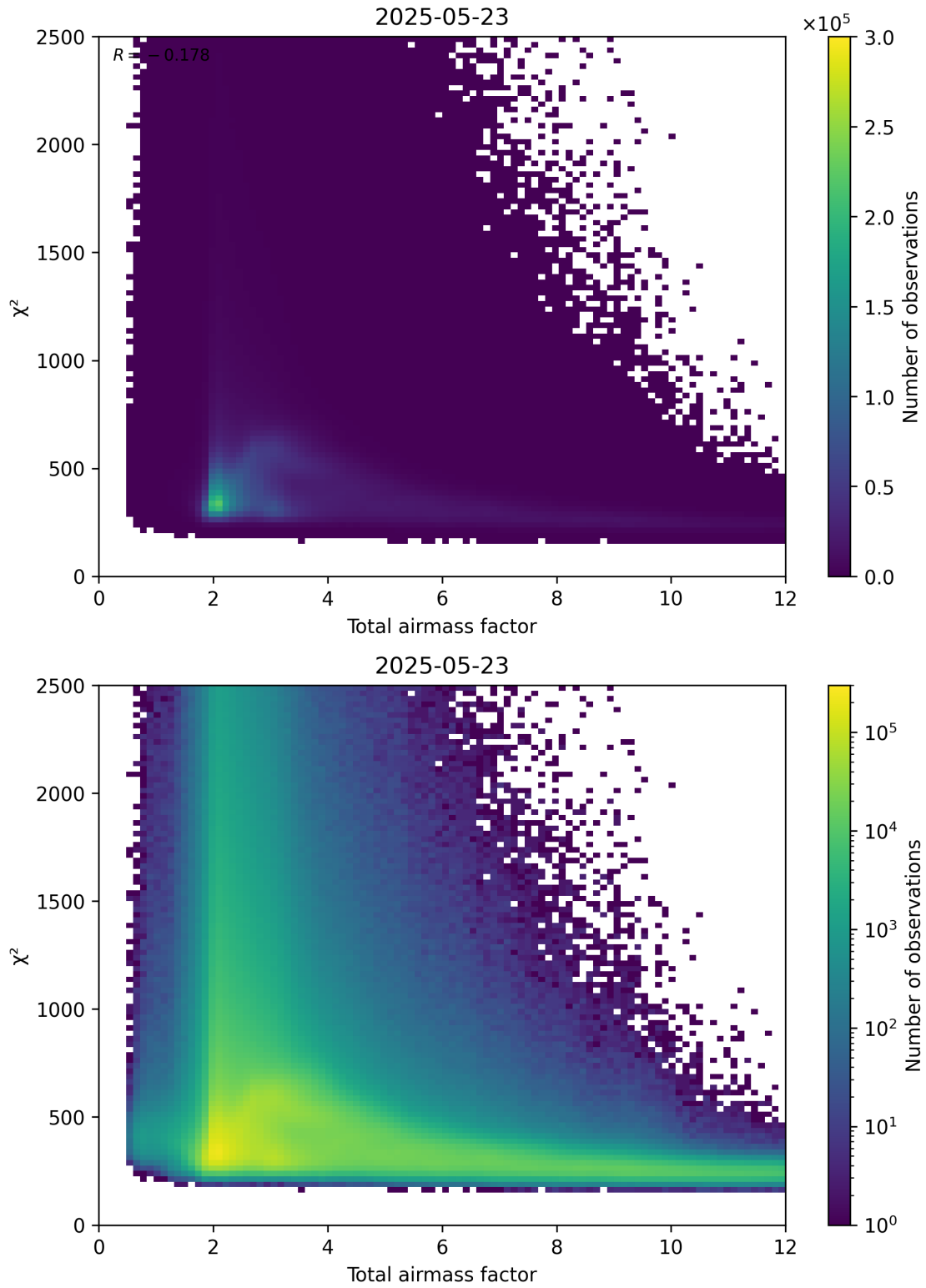
Figure 63: Scatter density plot of “Total airmass factor” against “ \chi^2 ” for 2025-05-22 to 2025-05-24.
