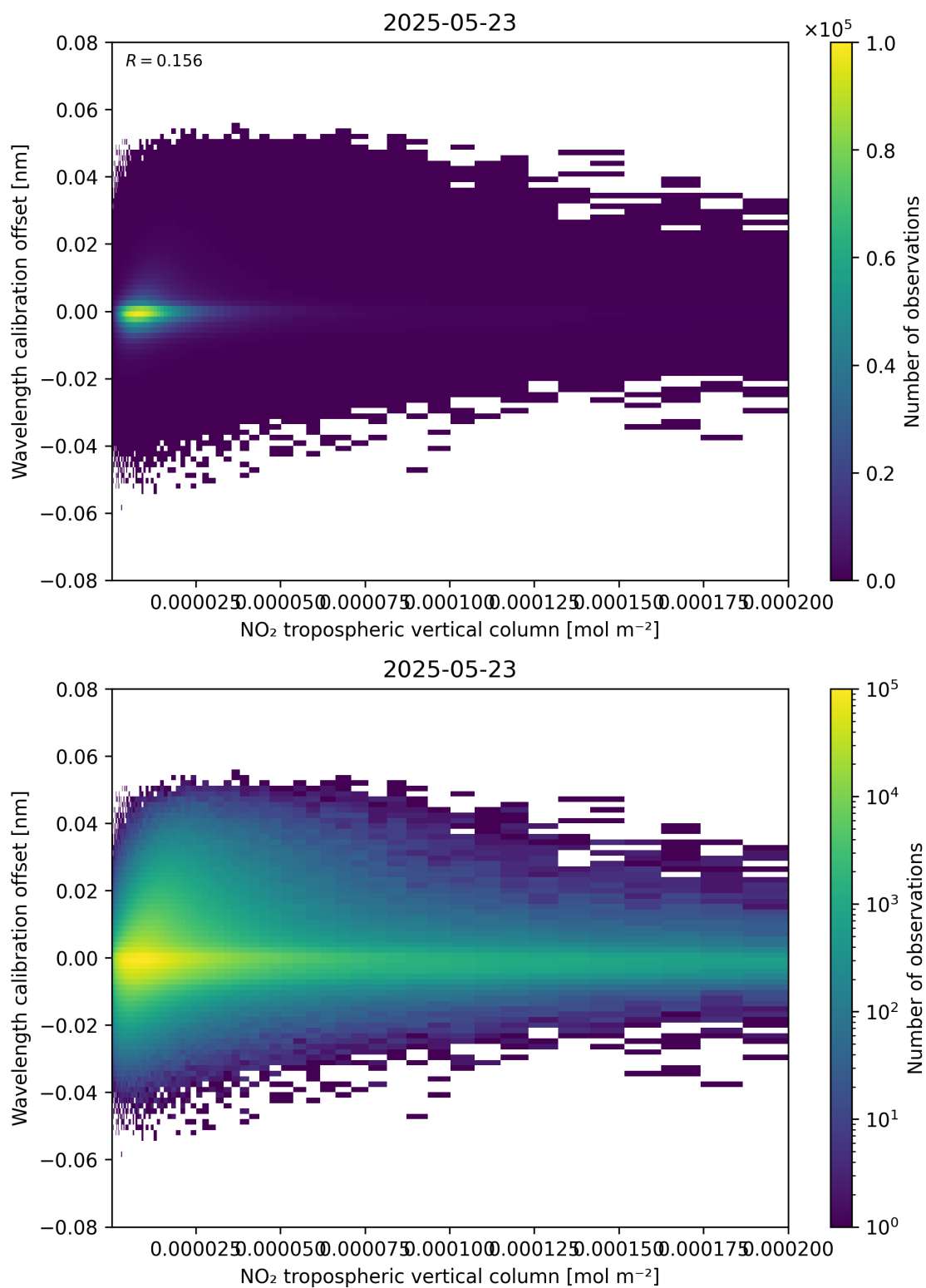
Figure 143: Scatter density plot of “NO 2 tropospheric vertical column” against “Wavelength calibration offset” for 2025-05-22 to 2025-05-24.
