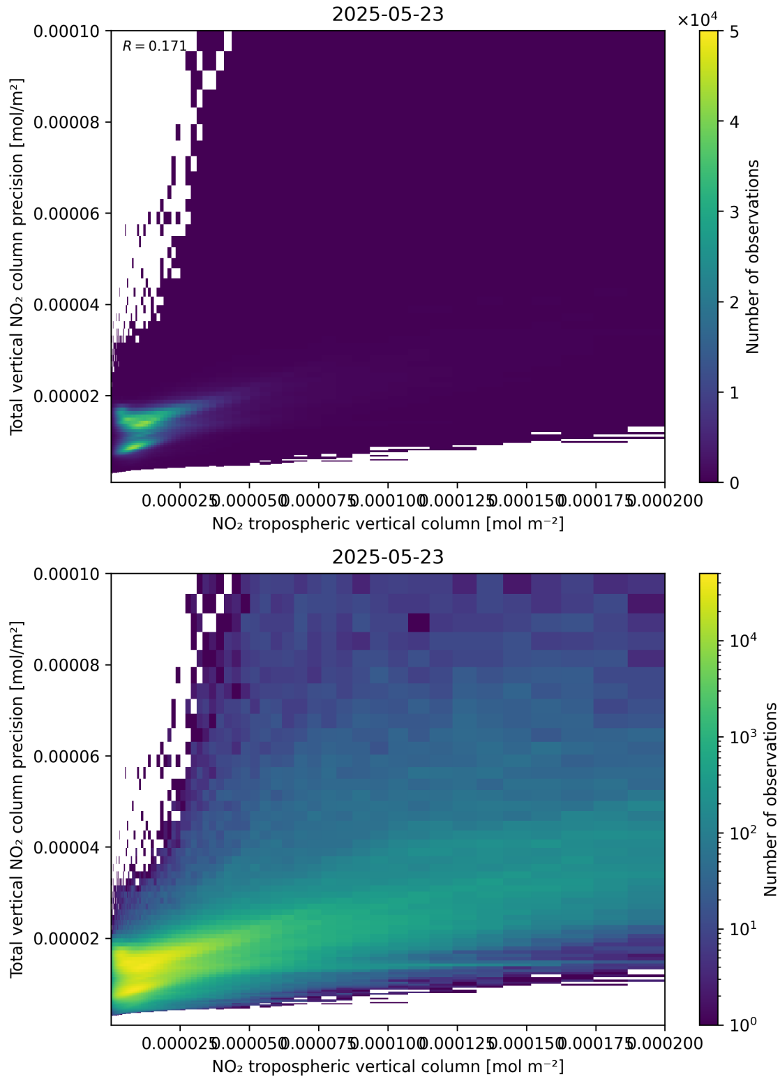
Figure 129: Scatter density plot of “NO 2 tropospheric vertical column” against “Total vertical NO 2 column precision” for 2025-05-22 to 2025-05-24.
