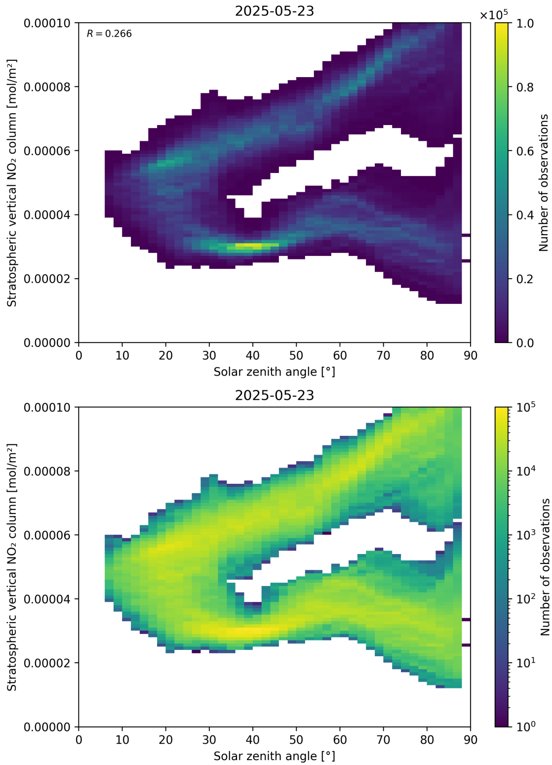
Figure 150: Scatter density plot of “Solar zenith angle” against “Stratospheric vertical NO 2 column” for 2025-05-22 to 2025-05-24.
