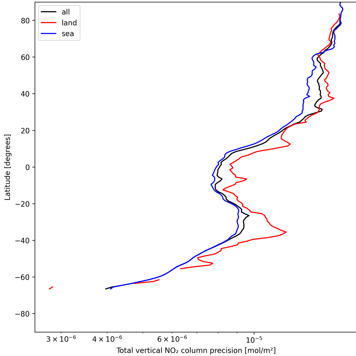
Figure 22: Zonal average of “Total vertical NO 2 column precision” for 2025-05-22 to 2025-05-24.
