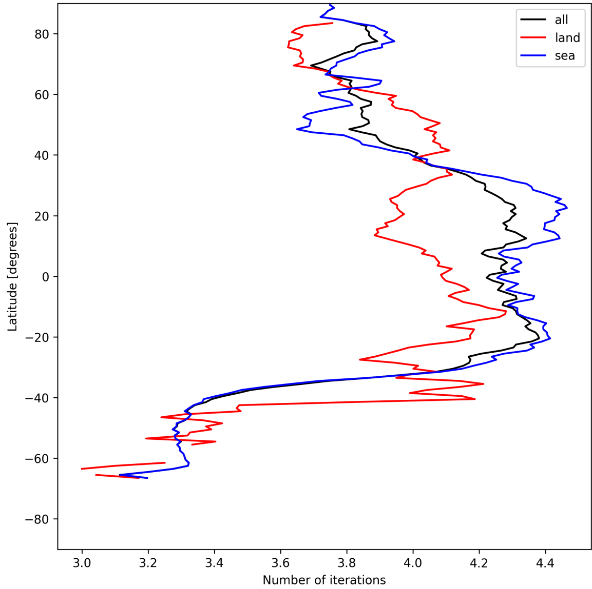
Figure 17: Zonal average of “Number of iterations” for 2025-05-22 to 2025-05-24.
