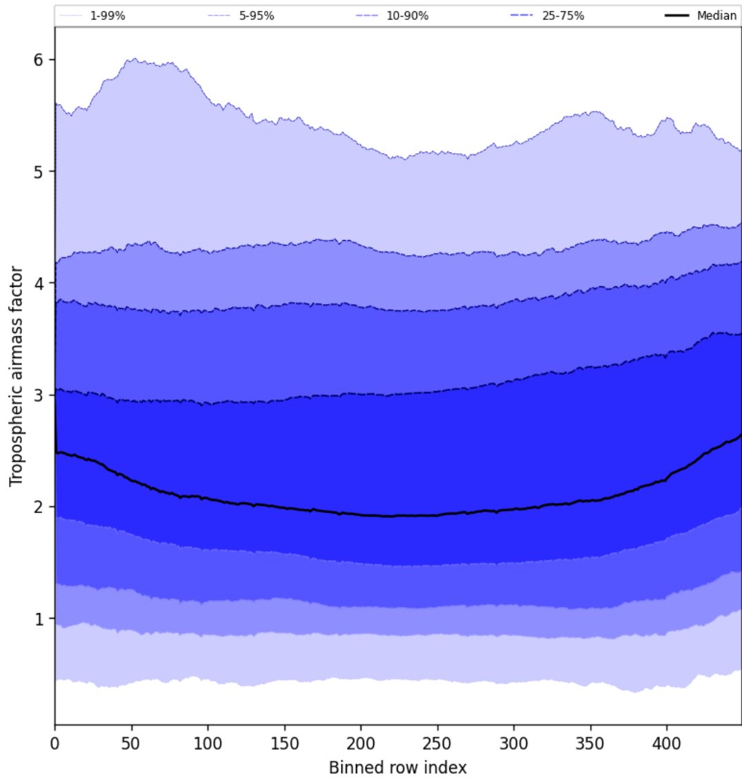
Figure 48: Along track statistics of “Tropospheric airmass factor” for 2025-05-22 to 2025-05-24
