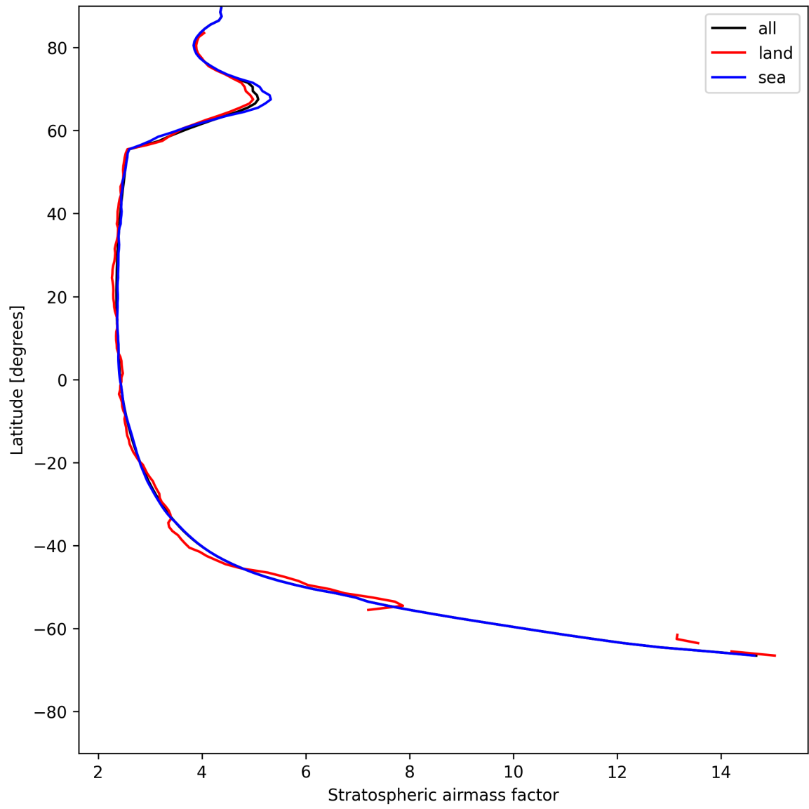
Figure 27: Zonal average of “Stratospheric airmass factor” for 2025-05-22 to 2025-05-24.
