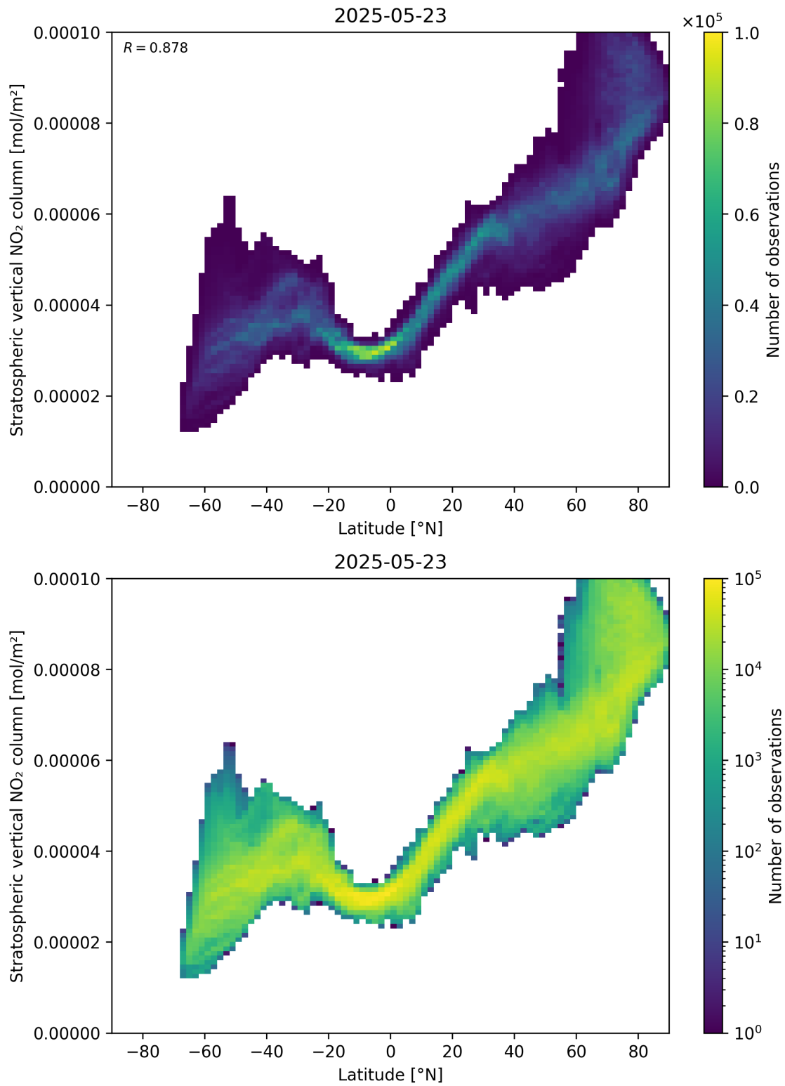
Figure 87: Scatter density plot of “Latitude” against “Stratospheric vertical \text{NO}_2 column” for 2025-05-22 to 2025-05-24.
