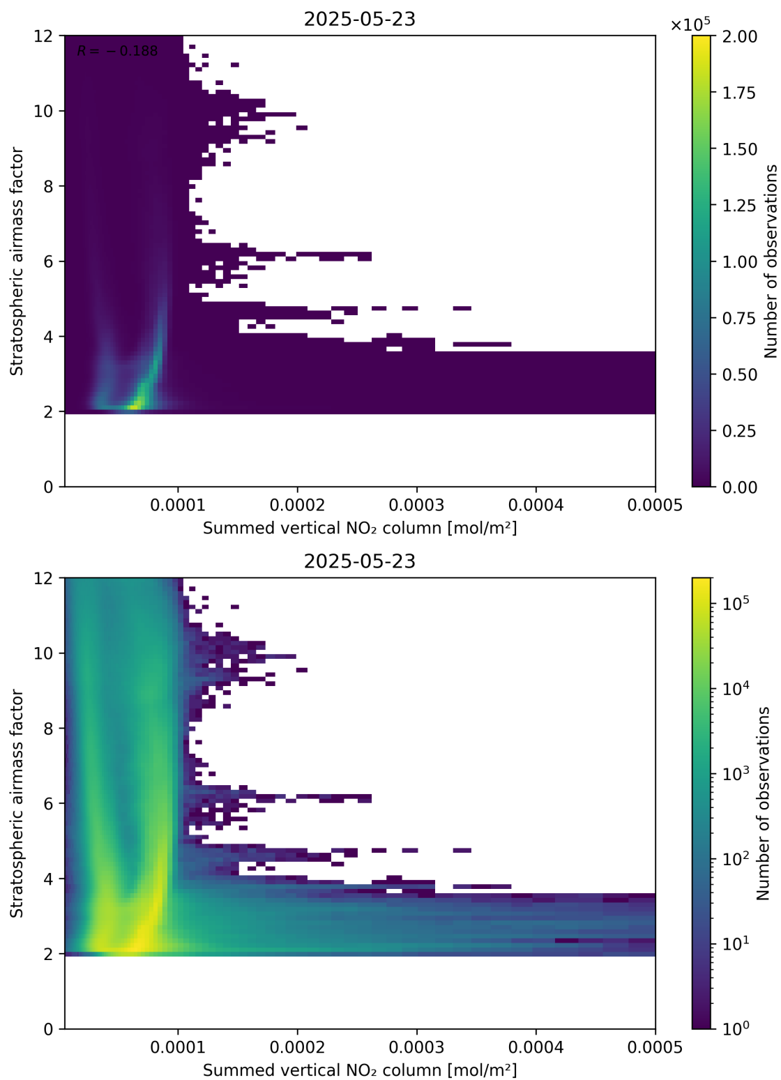
Figure 103: Scatter density plot of “Summed vertical NO 2 column” against “Stratospheric air mass factor” for 2025-05-22 to 2025-05-24.
