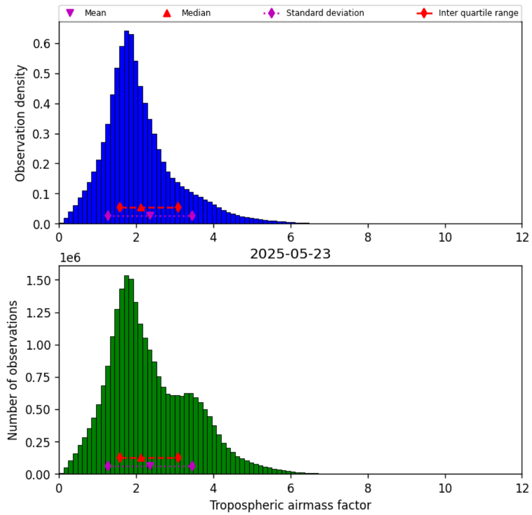
Figure 31: Histogram of “Tropospheric airmass factor” for 2025-05-22 to 2025-05-24
