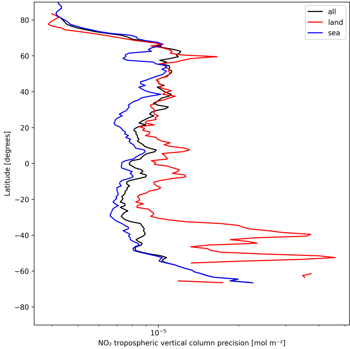
Figure 13: Zonal average of “NO 2 tropospheric vertical column precision” for 2025-05-22 to 2025-05-24.
