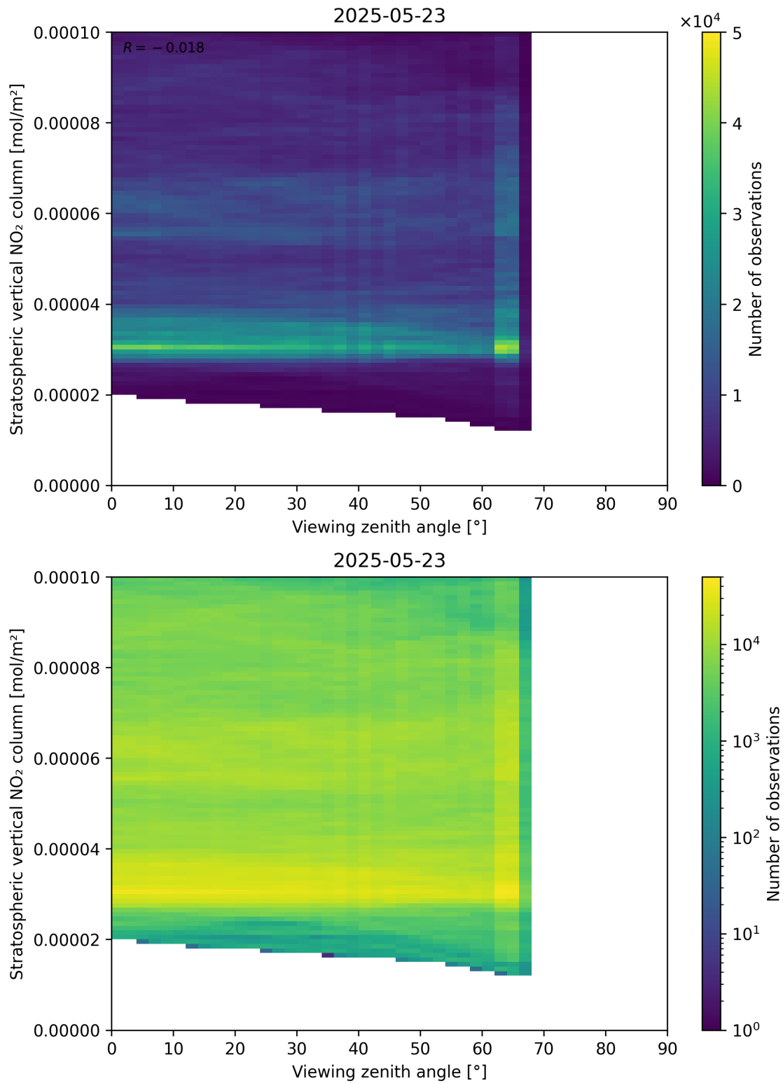
Figure 164: Scatter density plot of “Viewing zenith angle” against “Stratospheric vertical NO 2 column” for 2025-05-22 to 2025-05-24.
