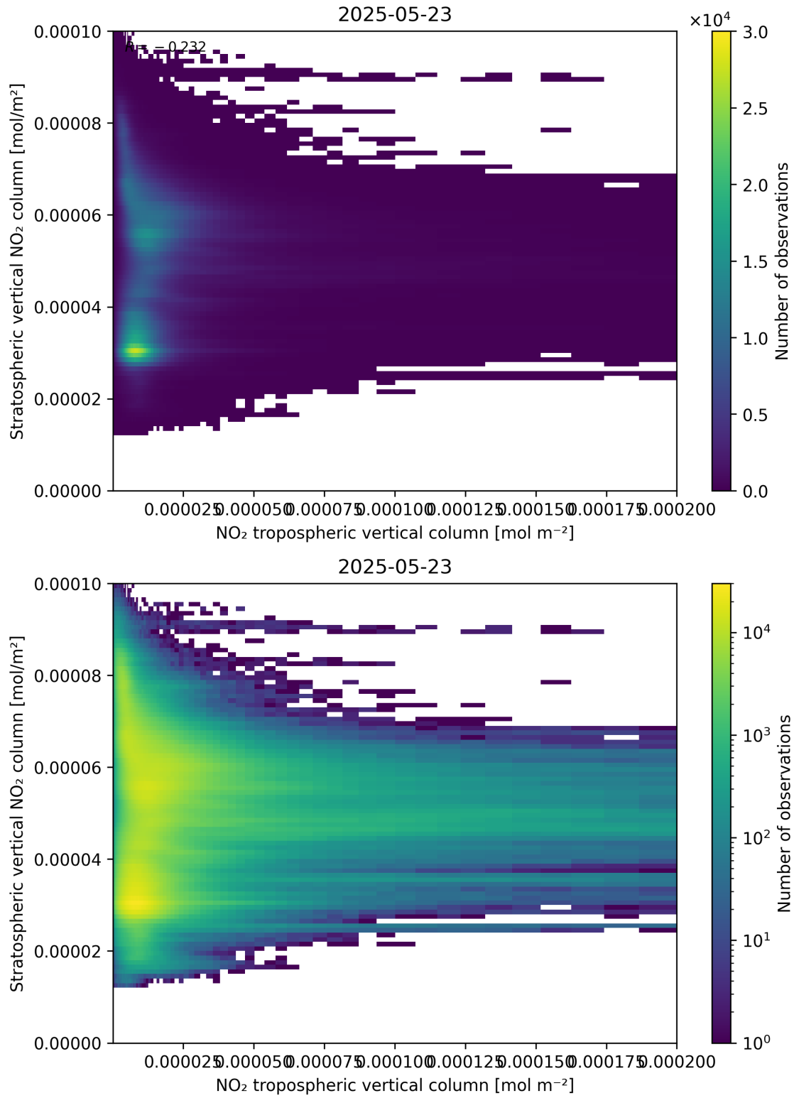
Figure 125: Scatter density plot of “NO 2 tropospheric vertical column” against “Stratospheric vertical NO 2 column” for 2025-05-22 to 2025-05-24.
