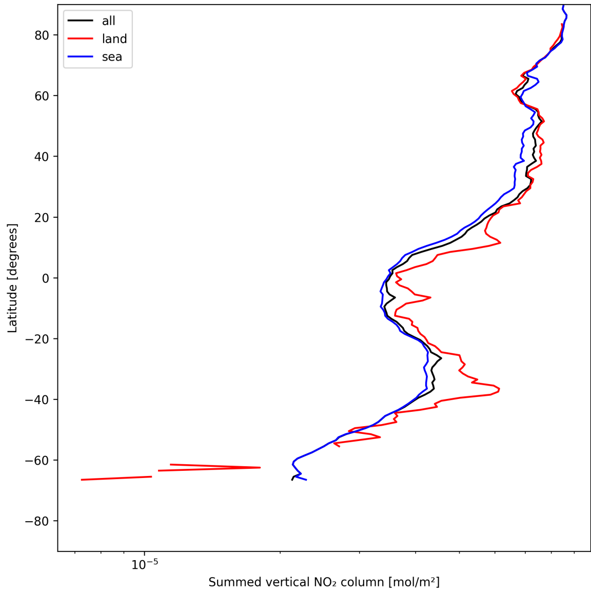
Figure 23: Zonal average of “Summed vertical NO 2 column” for 2025-05-22 to 2025-05-24.
