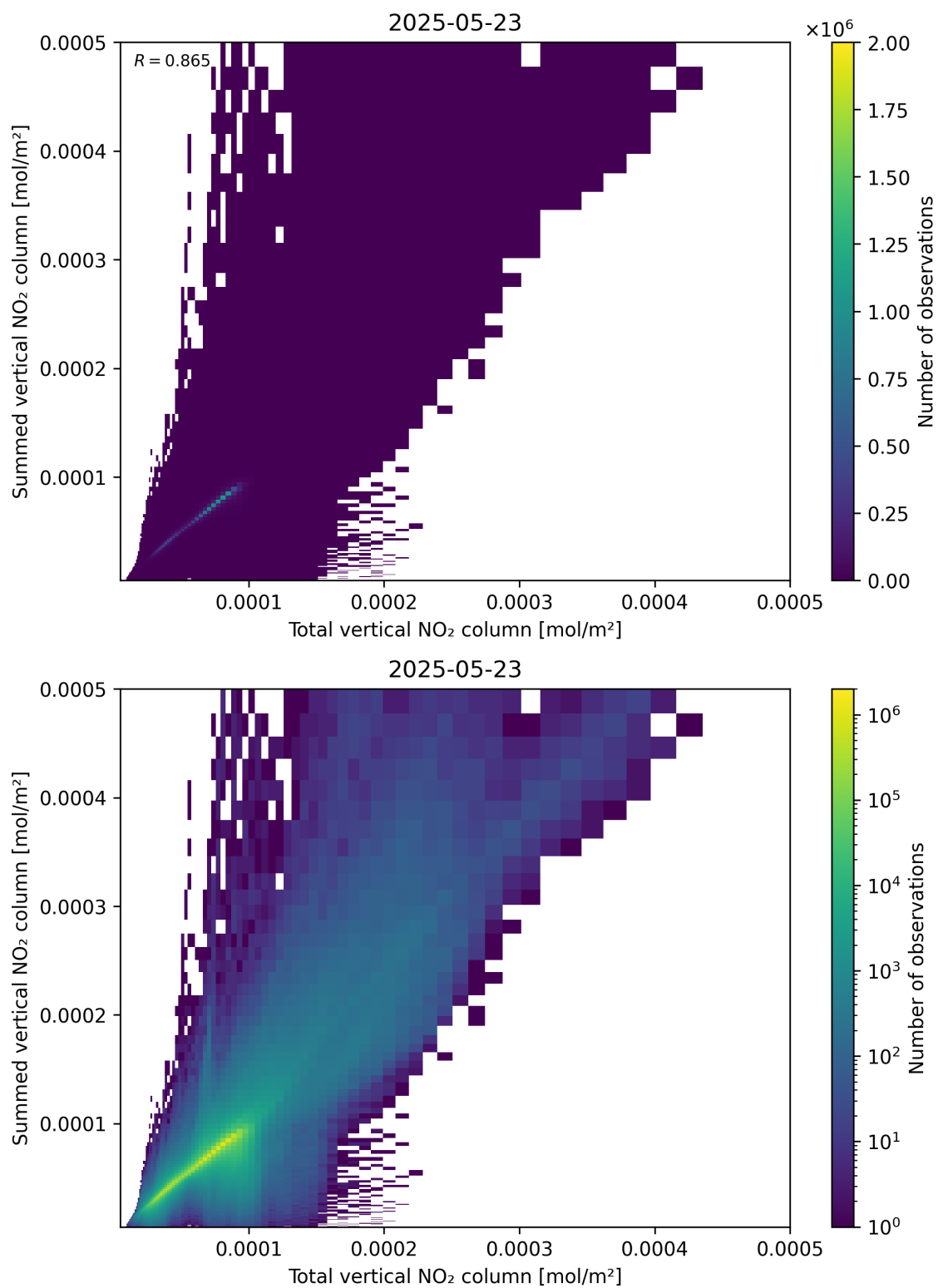
Figure 112: Scatter density plot of “Total vertical NO 2 column” against “Summed vertical NO 2 column” for 2025-05-22 to 2025-05-24.
