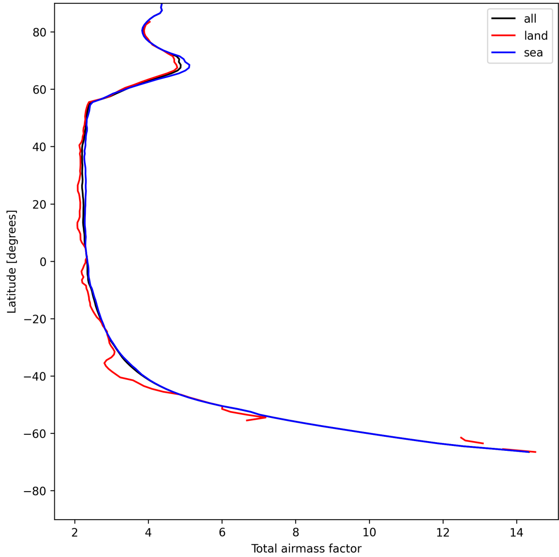
Figure 15: Zonal average of “Total airmass factor” for 2025-05-22 to 2025-05-24.
