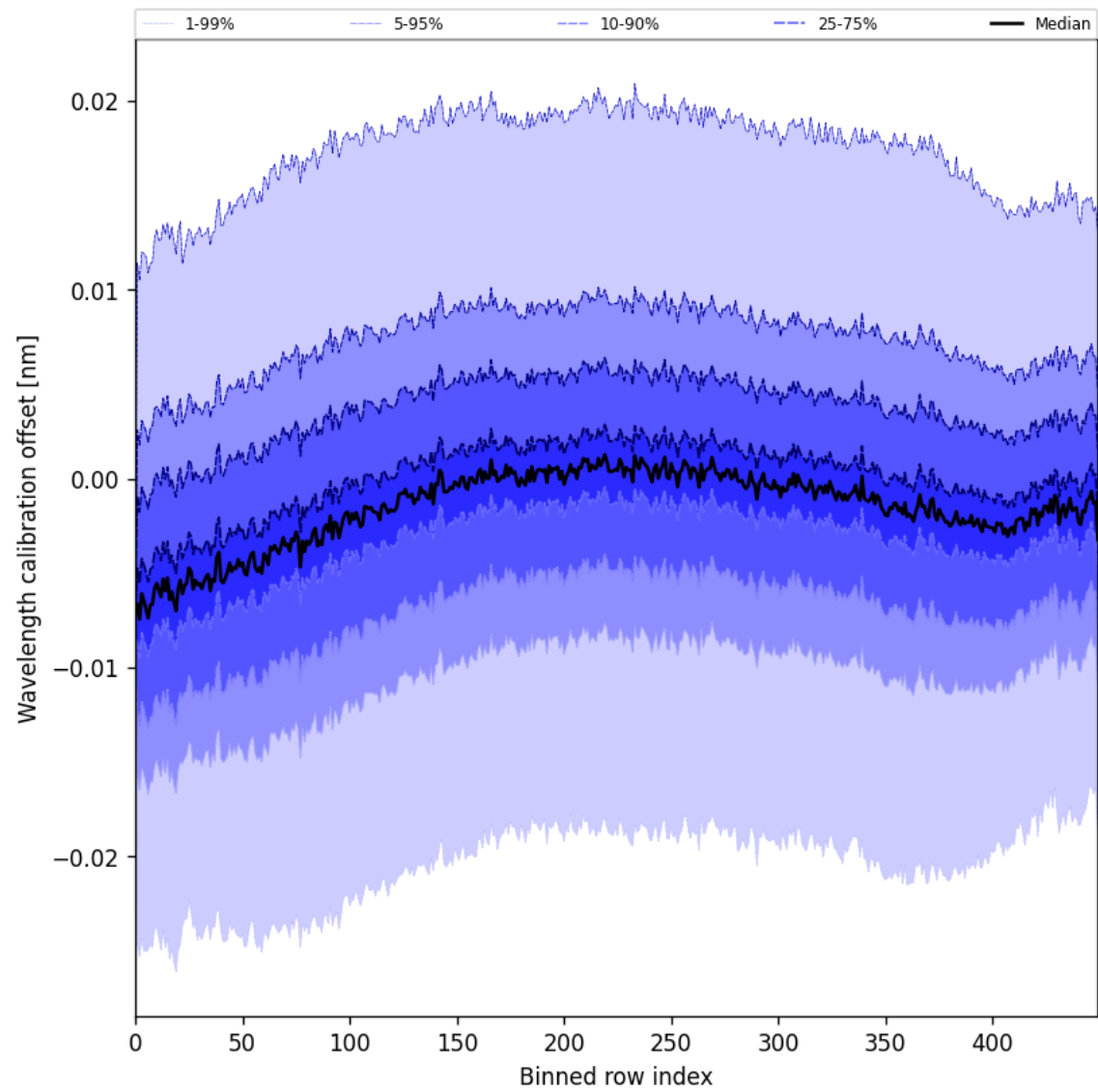
Figure 52: Along track statistics of “Wavelength calibration offset” for 2025-05-22 to 2025-05-24
