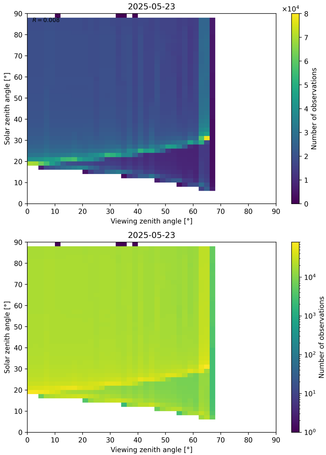
Figure 172: Scatter density plot of “Viewing zenith angle” against “Solar zenith angle” for 2025-05-22 to 2025-05-24.
