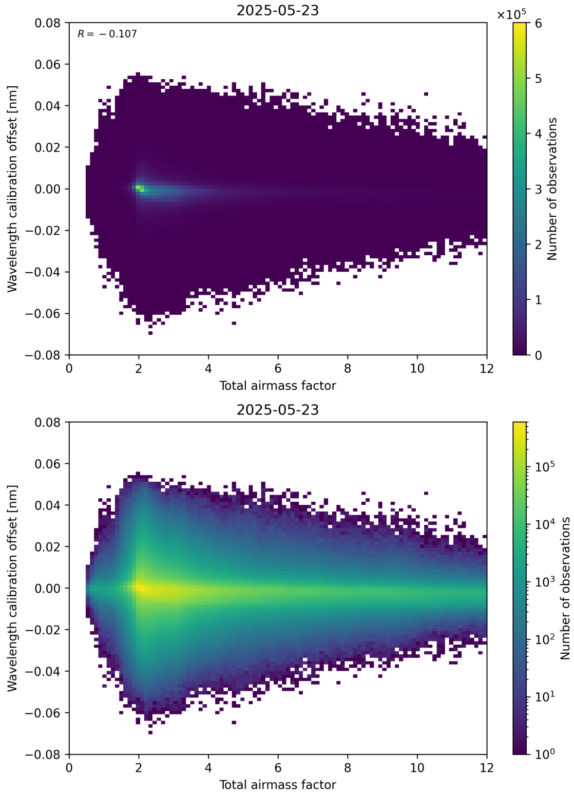
Figure 70: Scatter density plot of “Total airmass factor” against “Wavelength calibration offset” for 2025-05-22 to 2025-05-24.
