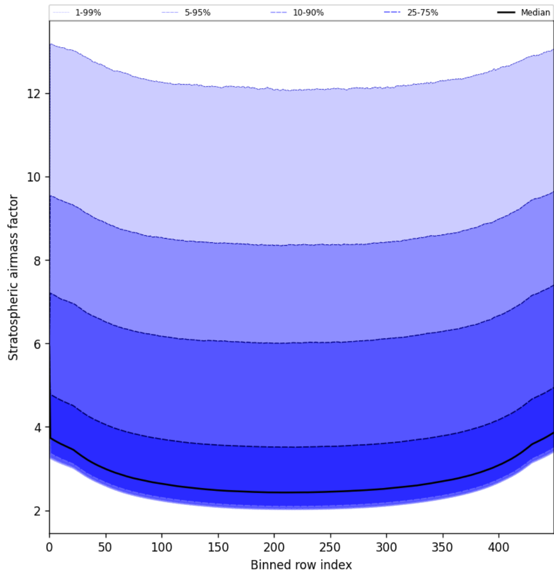
Figure 61: Along track statistics of “Stratospheric airmass factor” for 2025-05-22 to 2025-05-24
