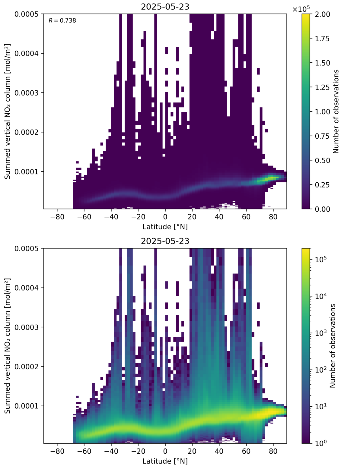
Figure 88: Scatter density plot of “Latitude” against “Summed vertical NO 2 column” for 2025-05-22 to 2025-05-24.
