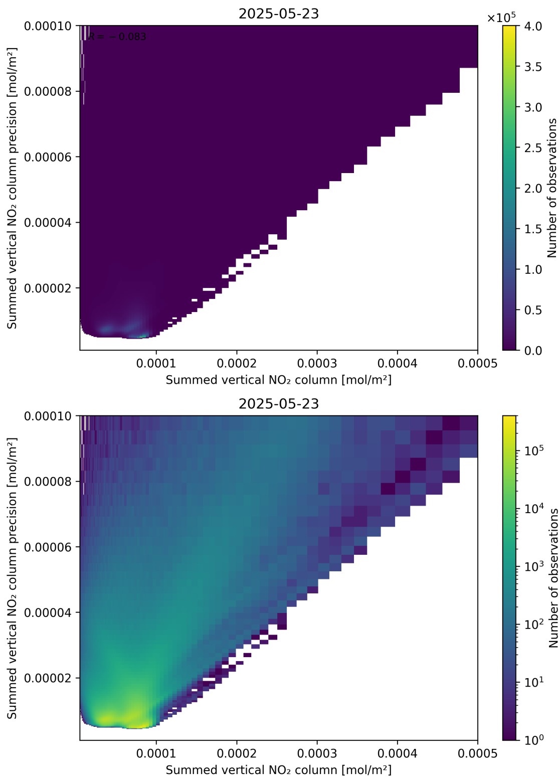
Figure 105: Scatter density plot of “Summed vertical NO 2 column” against “Summed vertical NO 2 column precision” for 2025-05-22 to 2025-05-24.
