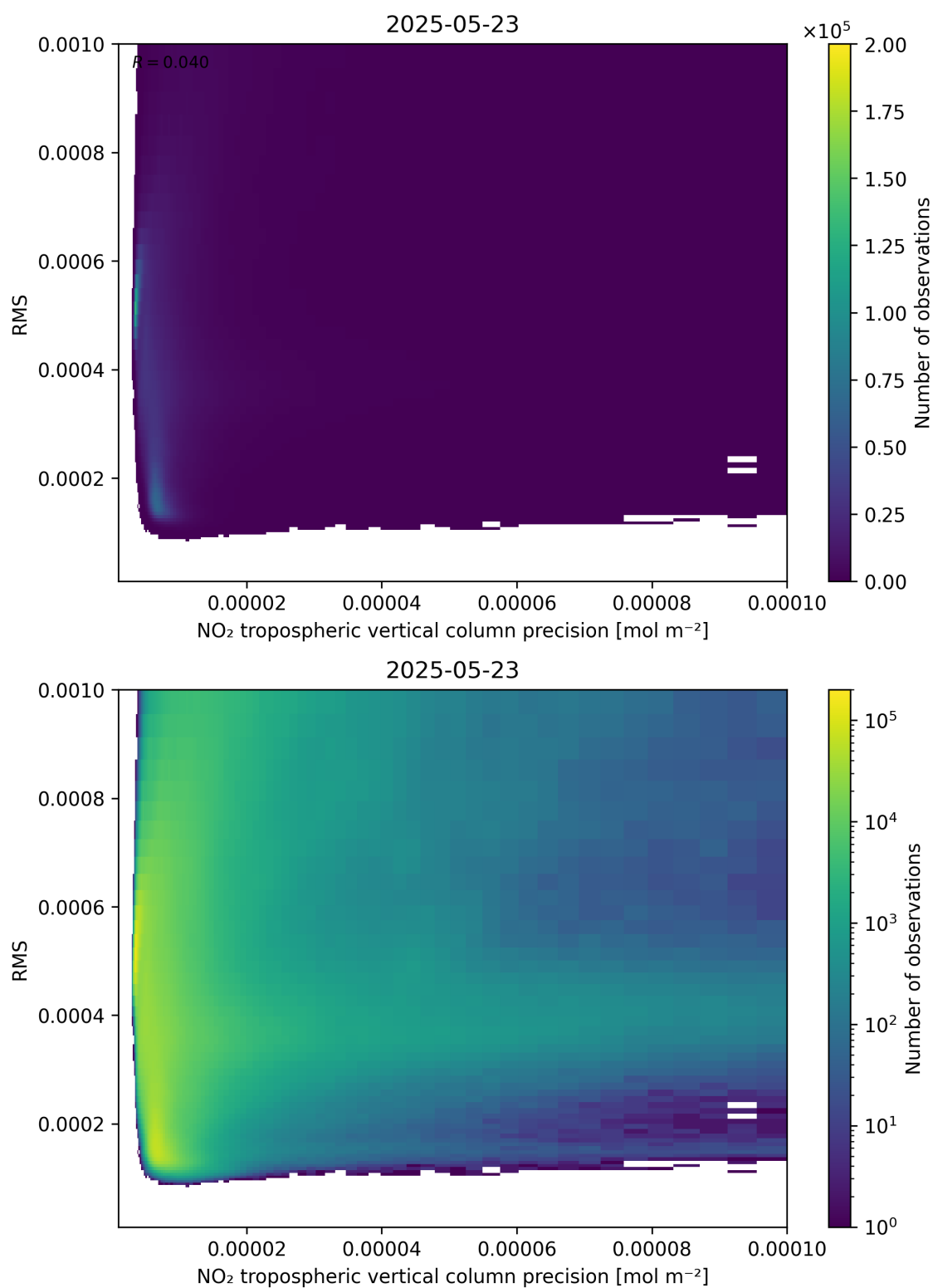
Figure 140: Scatter density plot of “NO 2 tropospheric vertical column precision” against “RMS” for 2025-05-22 to 2025-05-24.
