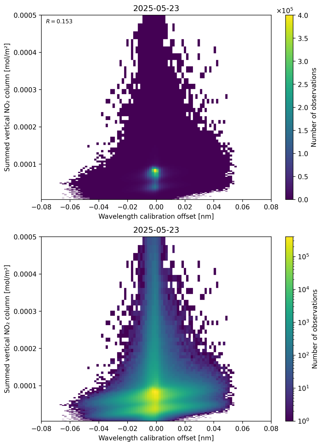
Figure 177: Scatter density plot of “Wavelength calibration offset” against “Summed vertical NO 2 column” for 2025-05-22 to 2025-05-24.
