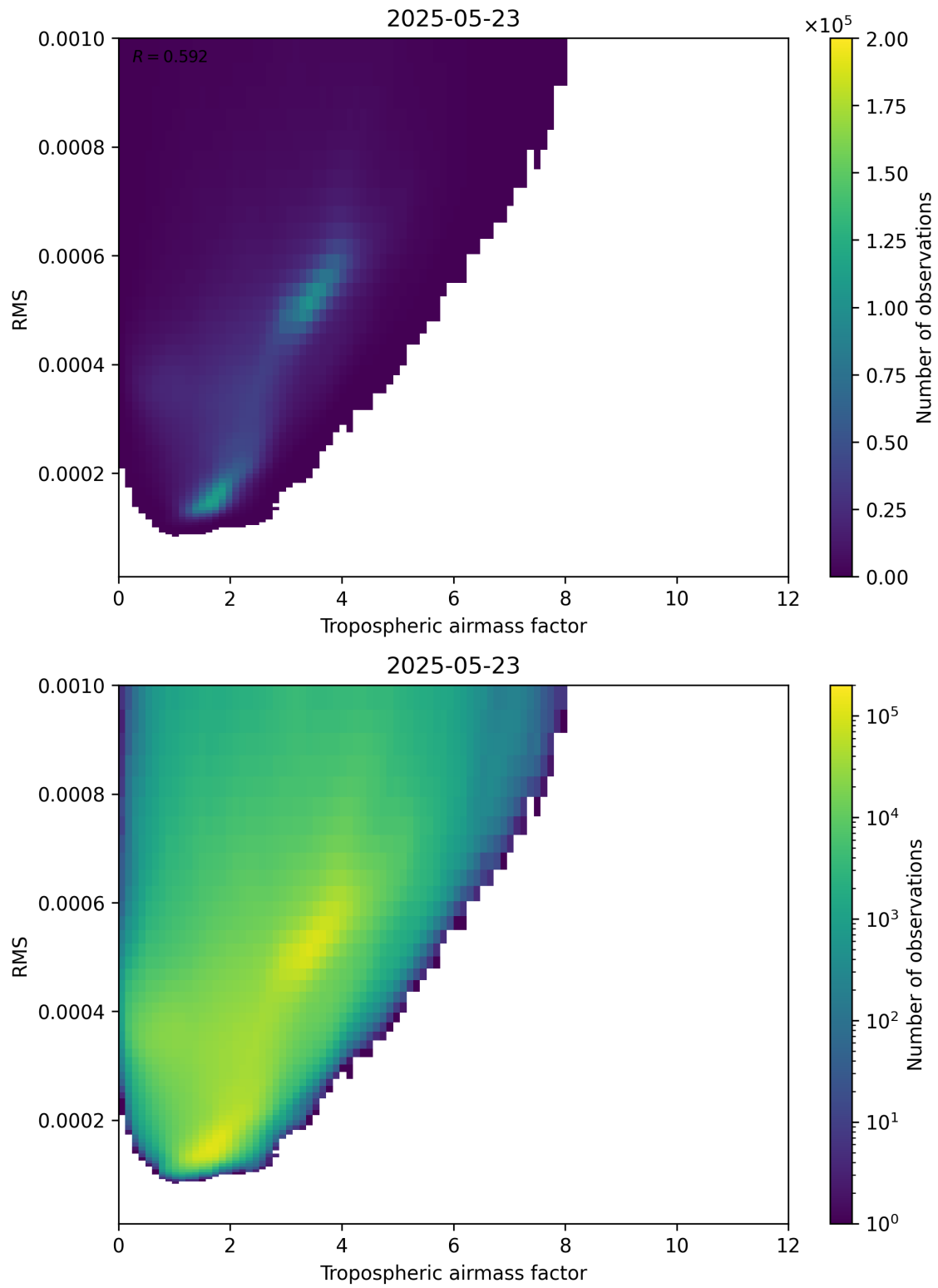
Figure 79: Scatter density plot of “Tropospheric airmass factor” against “RMS” for 2025-05-22 to 2025-05-24.
