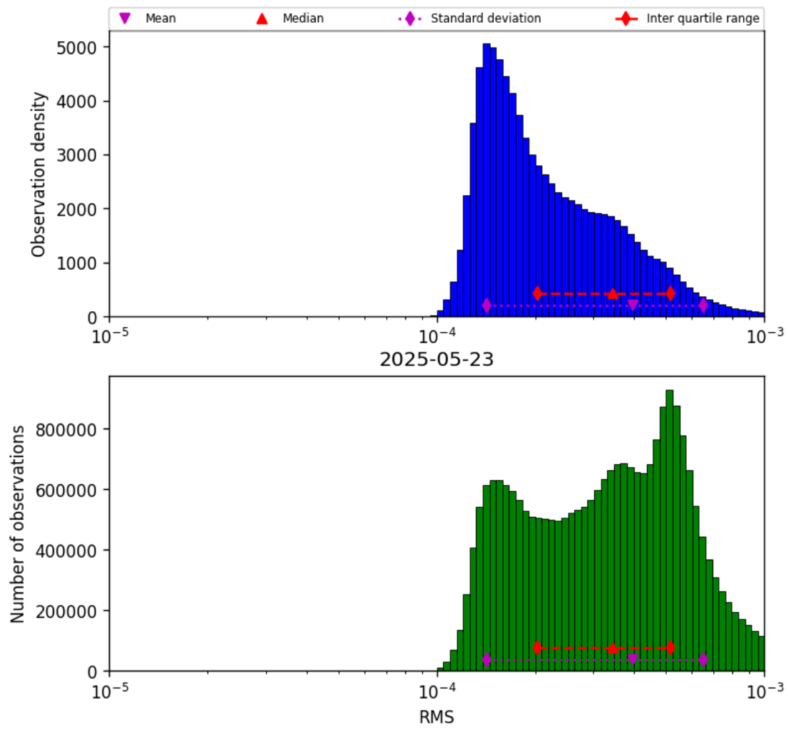
Figure 43: Histogram of “RMS” for 2025-05-22 to 2025-05-24
