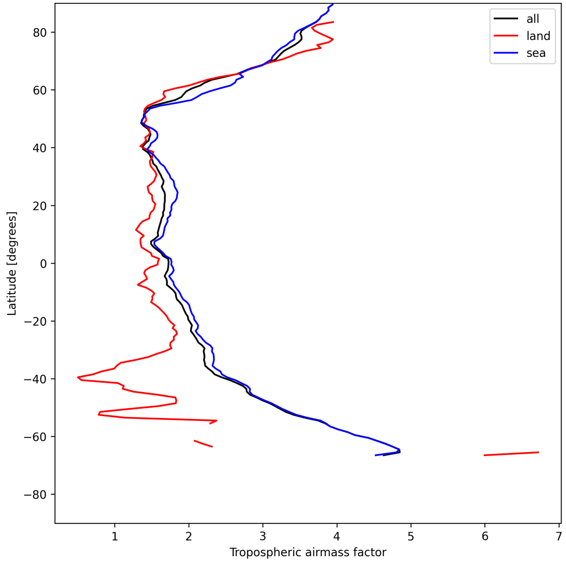
Figure 14: Zonal average of “Tropospheric air mass factor” for 2025-05-22 to 2025-05-24.
