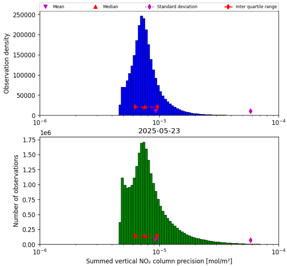
Figure 41: Histogram of "Summed vertical NO 2 column precision" for 2025-05-22 to 2025-05-24
