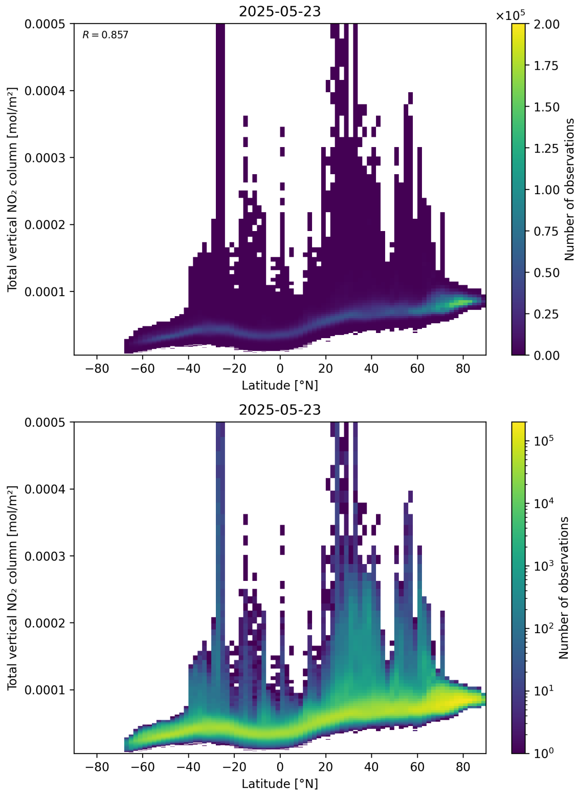
Figure 90: Scatter density plot of “Latitude” against “Total vertical NO 2 column” for 2025-05-22 to 2025-05-24.
