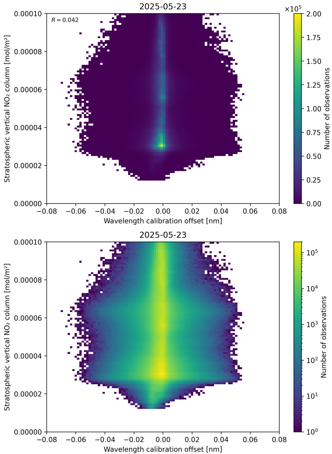
Figure 176: Scatter density plot of “Wavelength calibration offset” against “Stratospheric vertical NO 2 column” for 2025-05-22 to 2025-05-24.
