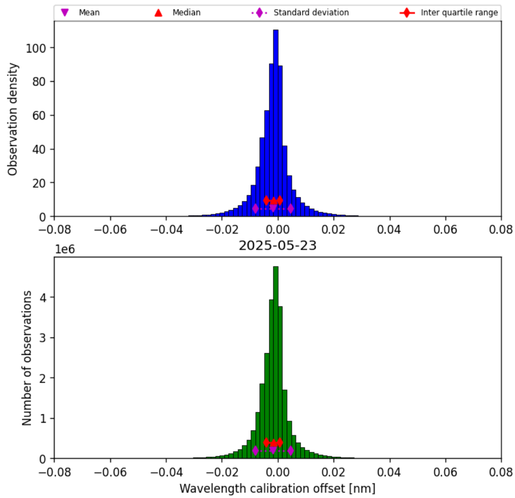
Figure 35: Histogram of “Wavelength calibration offset” for 2025-05-22 to 2025-05-24
