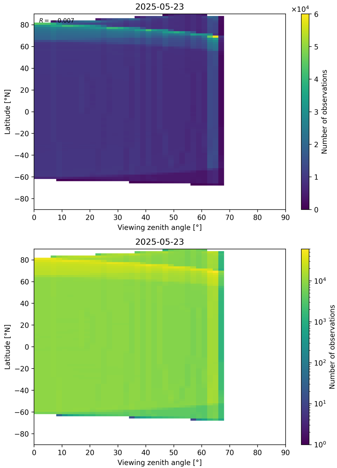
Figure 163: Scatter density plot of “Viewing zenith angle” against “Latitude” for 2025-05-22 to 2025-05-24.
