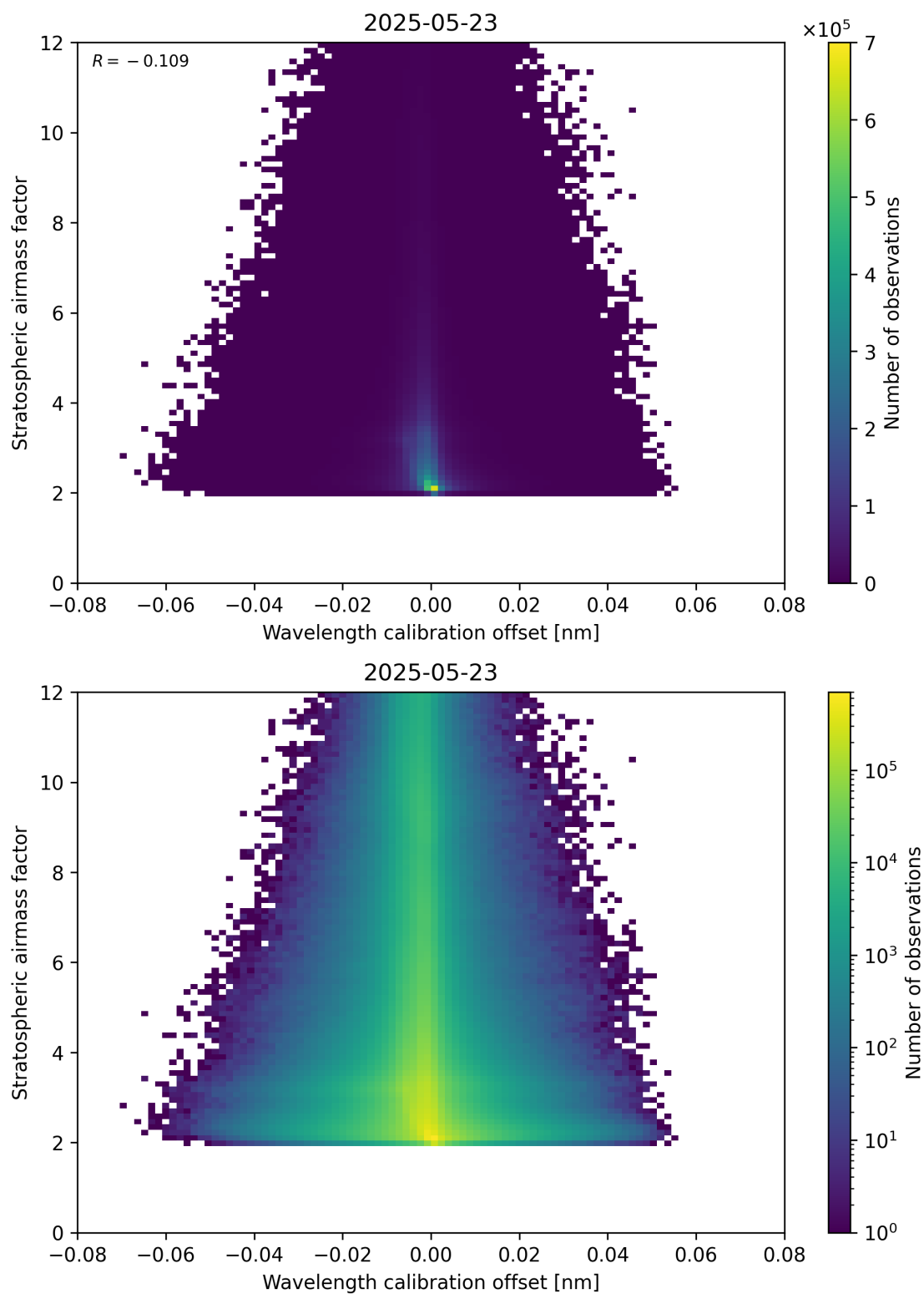
Figure 174: Scatter density plot of “Wavelength calibration offset” against “Stratospheric airmass factor” for 2025-05-22 to 2025-05-24.
