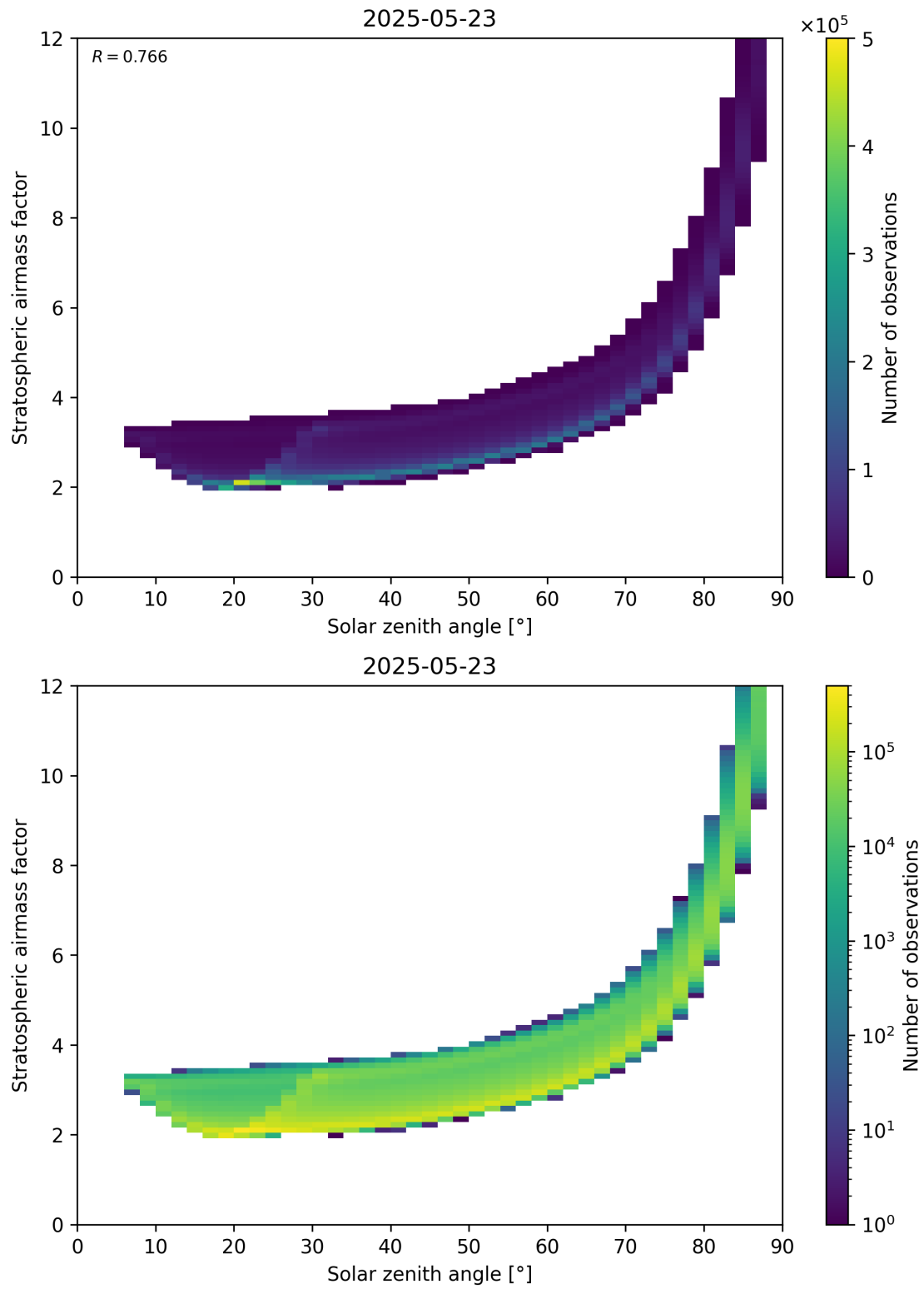
Figure 145: Scatter density plot of “Solar zenith angle” against “Stratospheric airmass factor” for 2025-05-22 to 2025-05-24.
