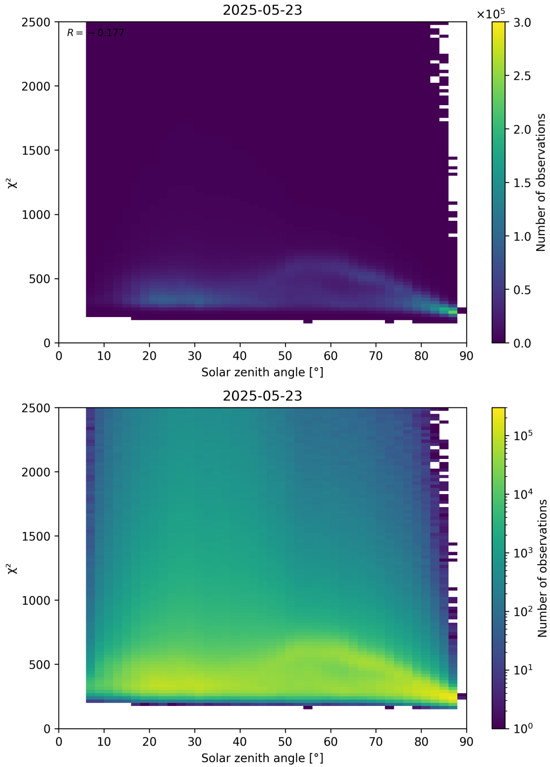
Figure 148: Scatter density plot of “Solar zenith angle” against “ \chi^2 ” for 2025-05-22 to 2025-05-24.
