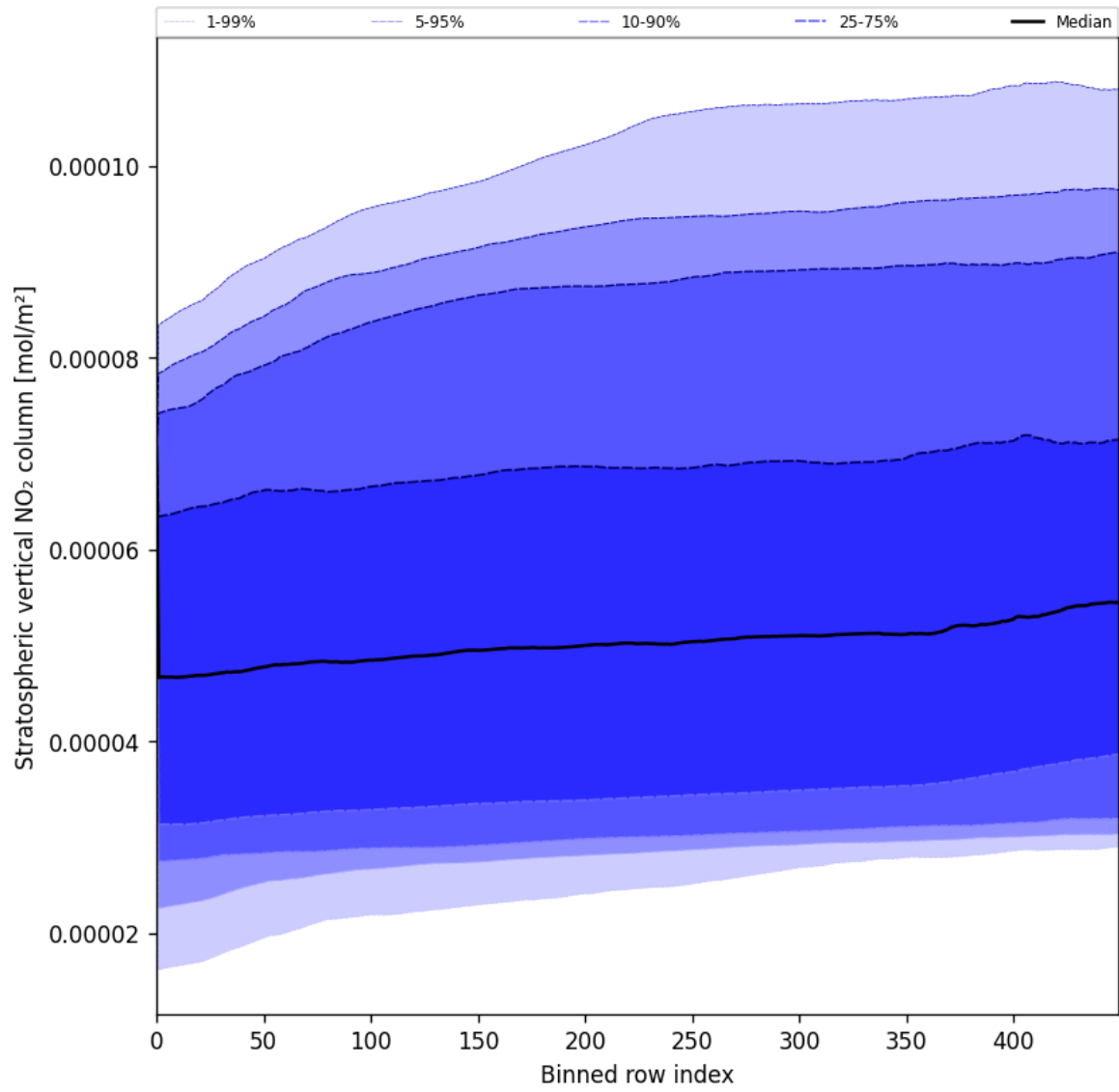
Figure 53: Along track statistics of “Stratospheric vertical NO 2 column” for 2025-05-22 to 2025-05-24
