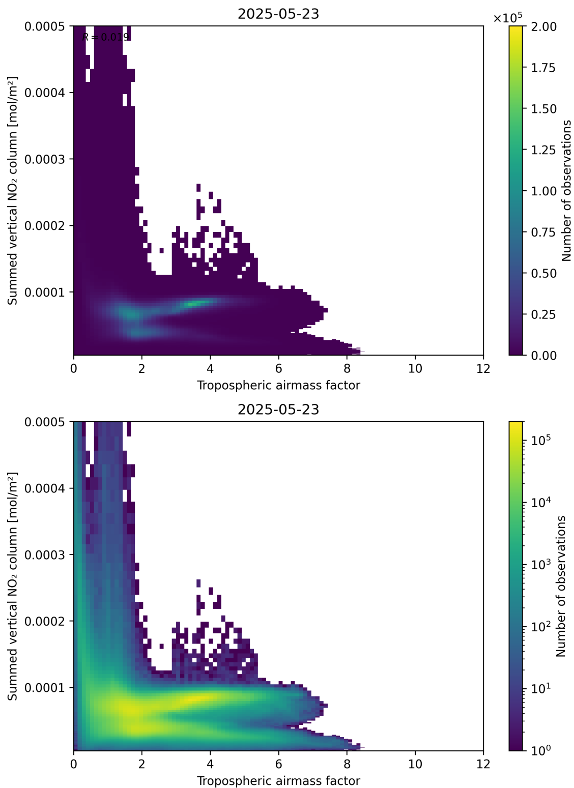
Figure 75: Scatter density plot of “Tropospheric air mass factor” against “Summed vertical NO 2 column” for 2025-05-22 to 2025-05-24.
