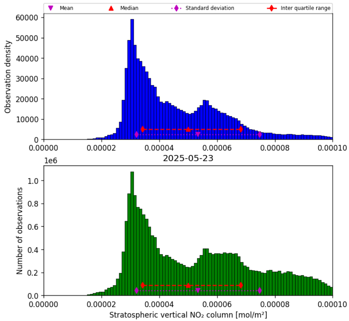
Figure 36: Histogram of “Stratospheric vertical NO 2 column” for 2025-05-22 to 2025-05-24
