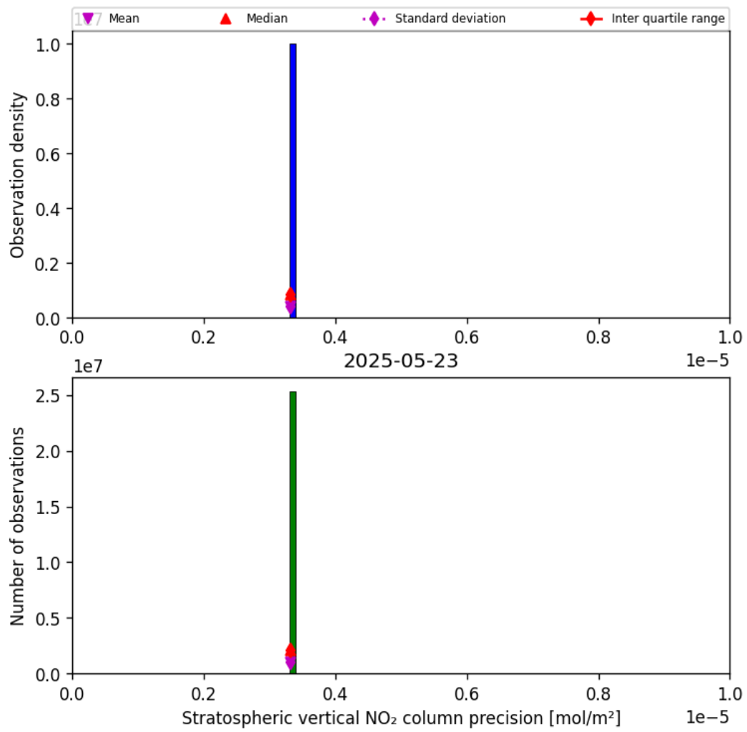
Figure 37: Histogram of “Stratospheric vertical NO 2 column precision” for 2025-05-22 to 2025-05-24
