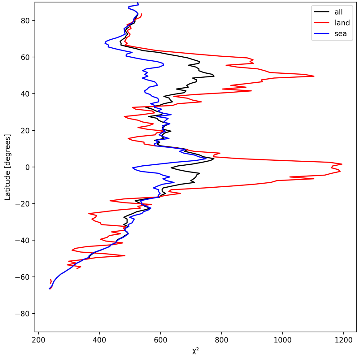
Figure 25: Zonal average of “ \chi^2 ” for 2025-05-22 to 2025-05-24.
