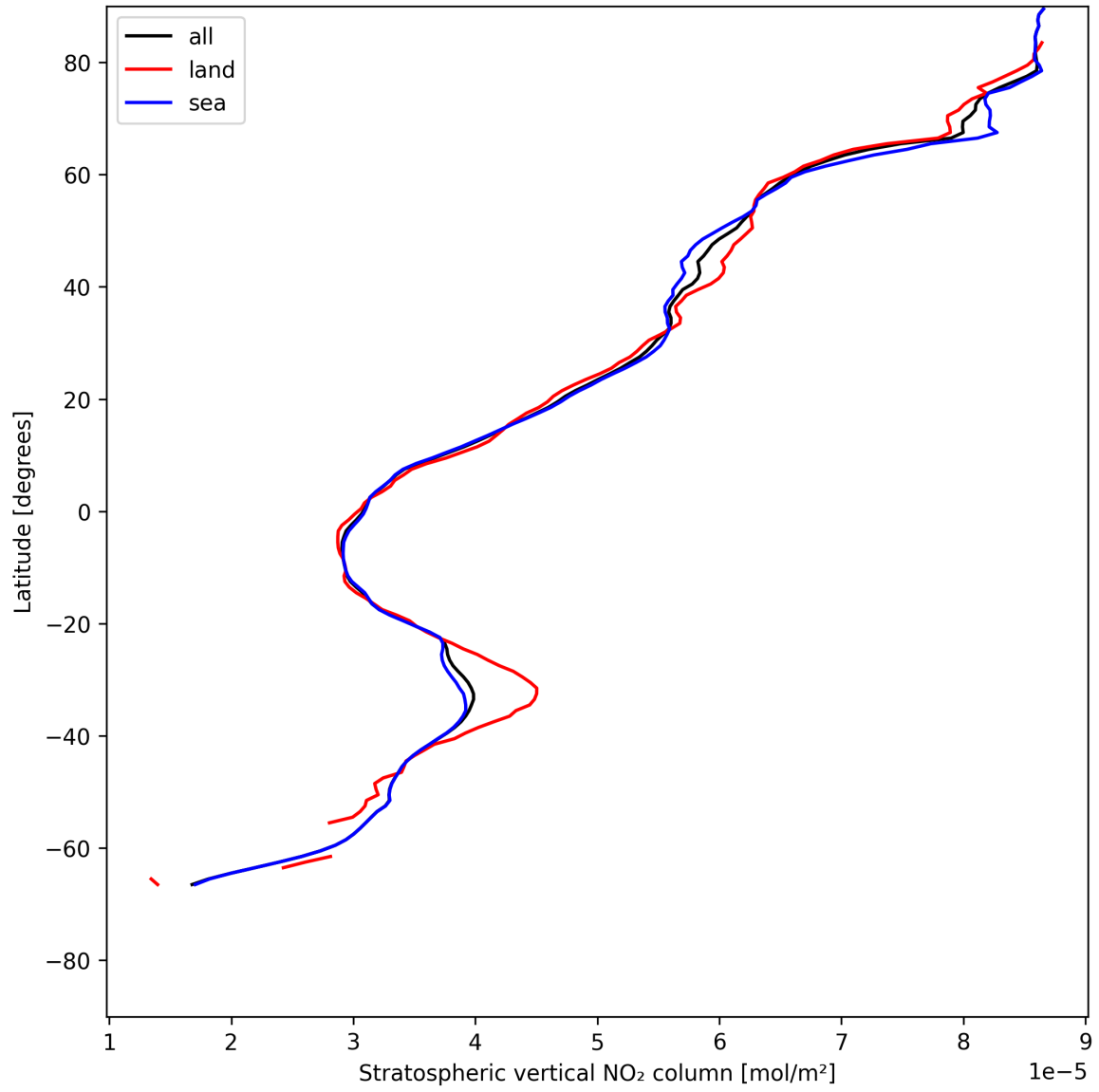
Figure 19: Zonal average of “Stratospheric vertical NO 2 column” for 2025-05-22 to 2025-05-24.
