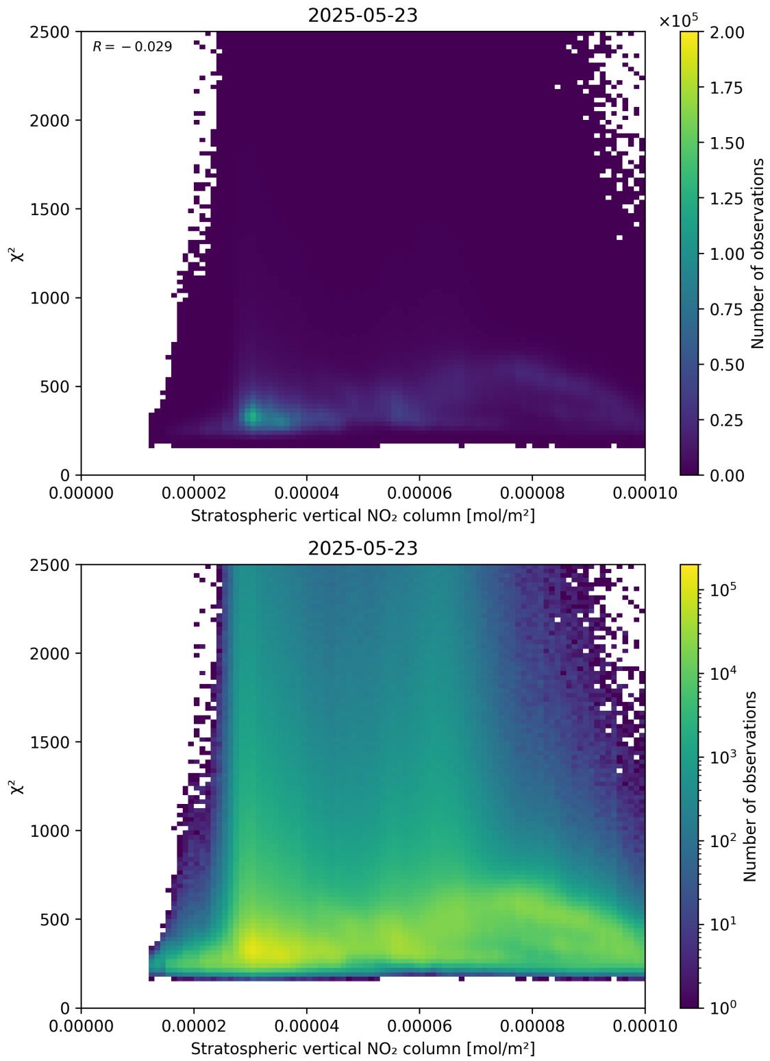
Figure 97: Scatter density plot of “Stratospheric vertical NO 2 column” against “ \chi^2 ” for 2025-05-22 to 2025-05-24.
