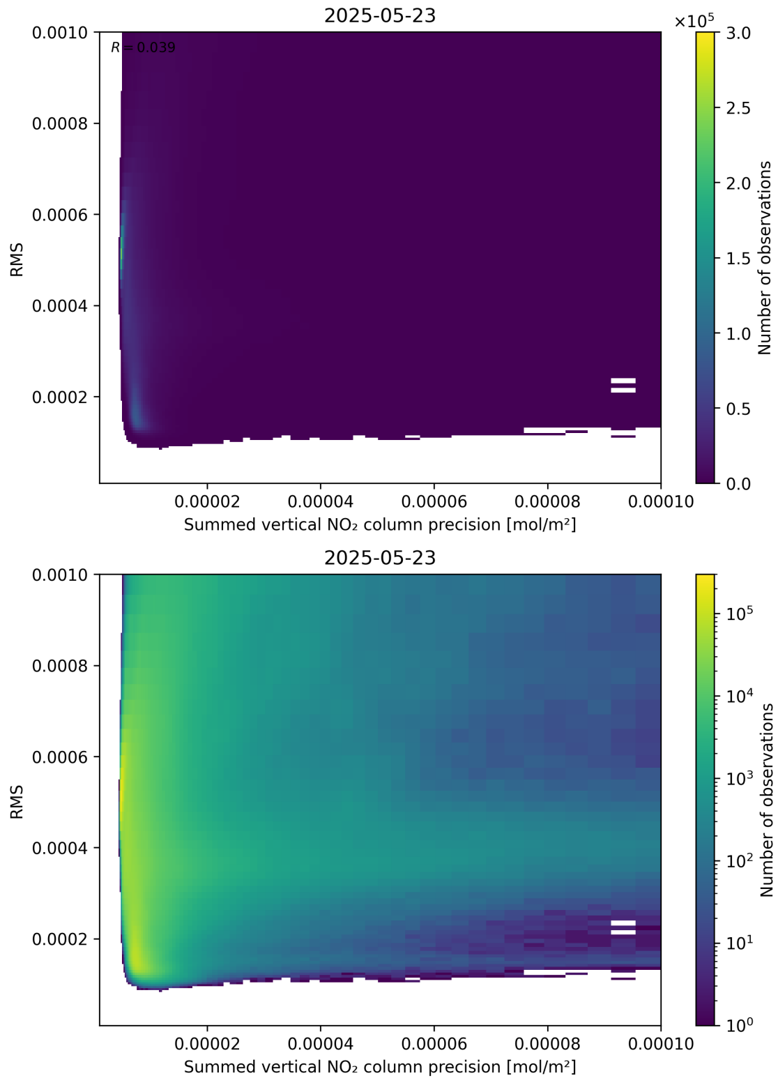
Figure 108: Scatter density plot of “Summed vertical NO 2 column precision” against “RMS” for 2025-05-22 to 2025-05-24.
