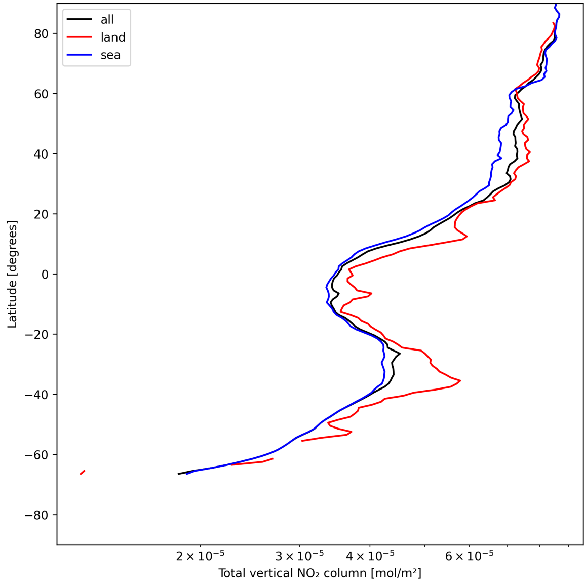
Figure 21: Zonal average of “Total vertical NO 2 column” for 2025-05-22 to 2025-05-24.
