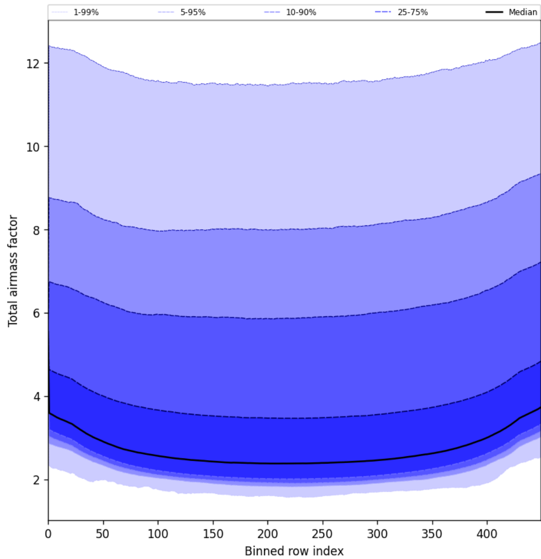
Figure 49: Along track statistics of “Total airmass factor” for 2025-05-22 to 2025-05-24
