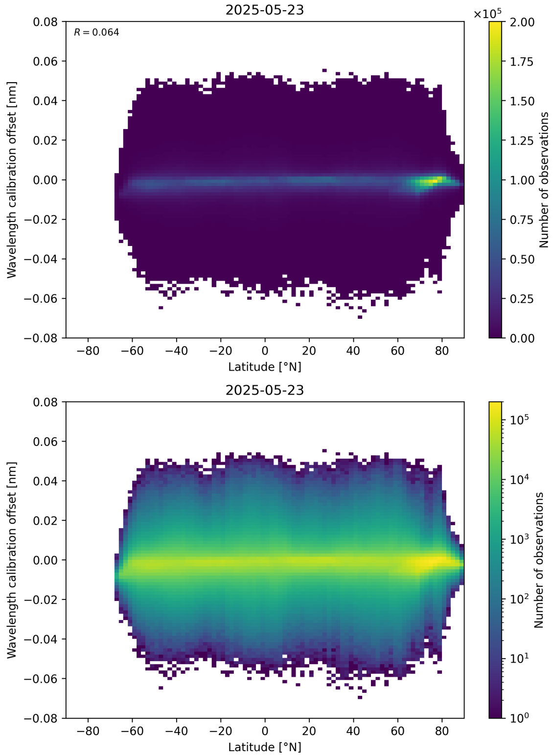
Figure 95: Scatter density plot of “Latitude” against “Wavelength calibration offset” for 2025-05-22 to 2025-05-24.
