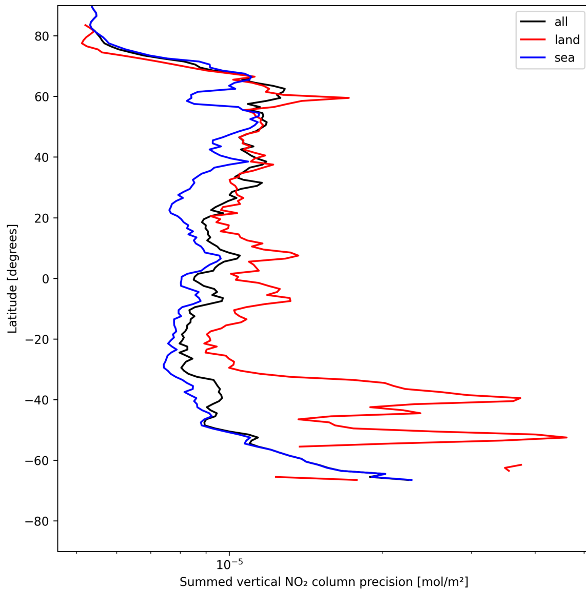
Figure 24: Zonal average of “Summed vertical NO 2 column precision” for 2025-05-22 to 2025-05-24.
