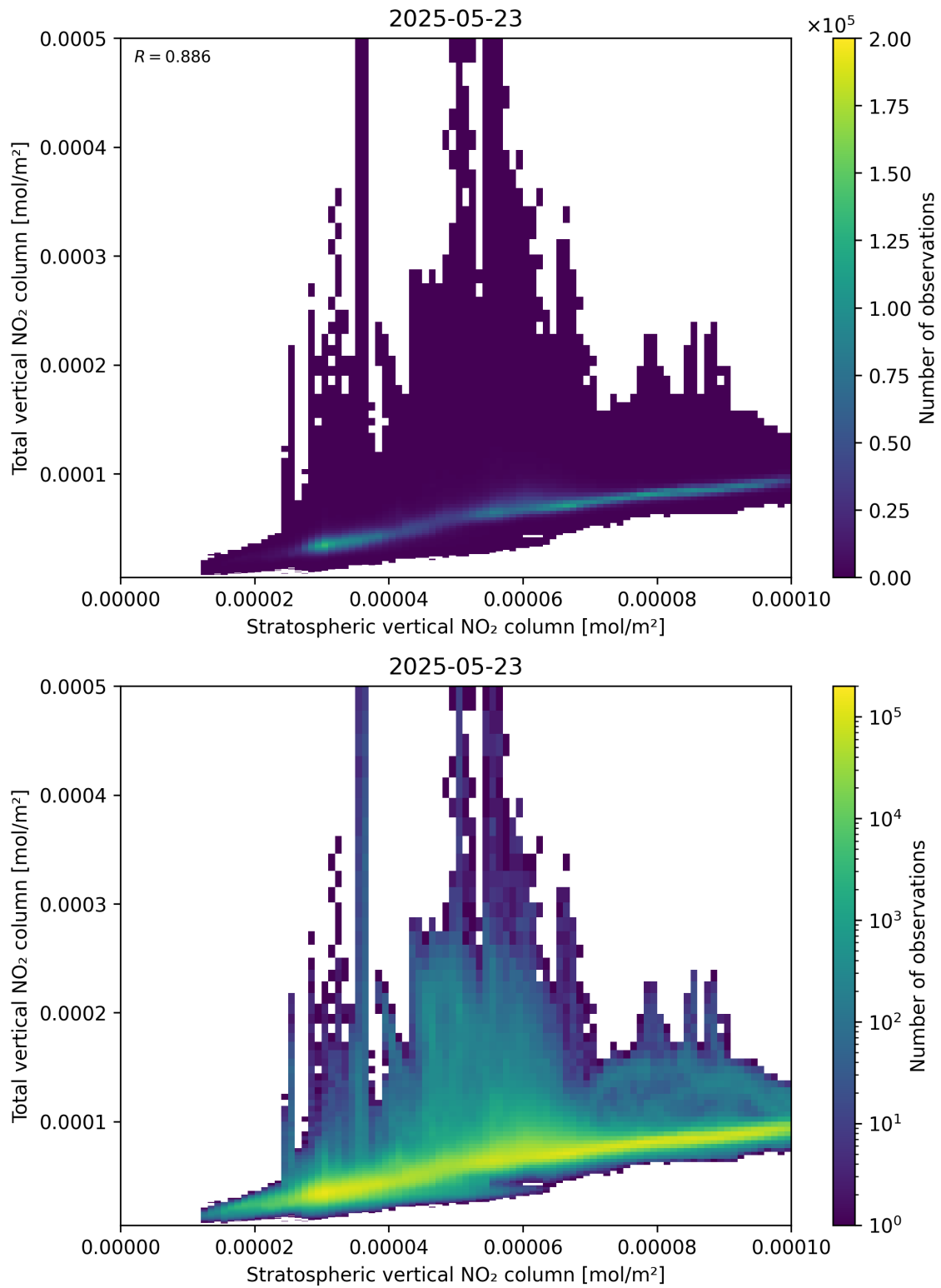
Figure 100: Scatter density plot of “Stratospheric vertical NO 2 column” against “Total vertical NO 2 column” for 2025-05-22 to 2025-05-24.
