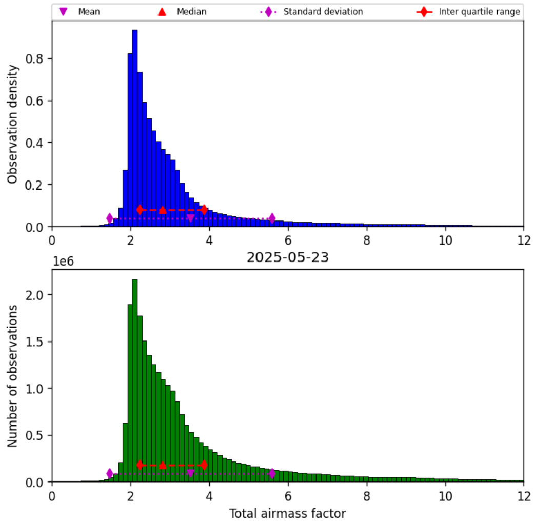
Figure 32: Histogram of “Total airmass factor” for 2025-05-22 to 2025-05-24
