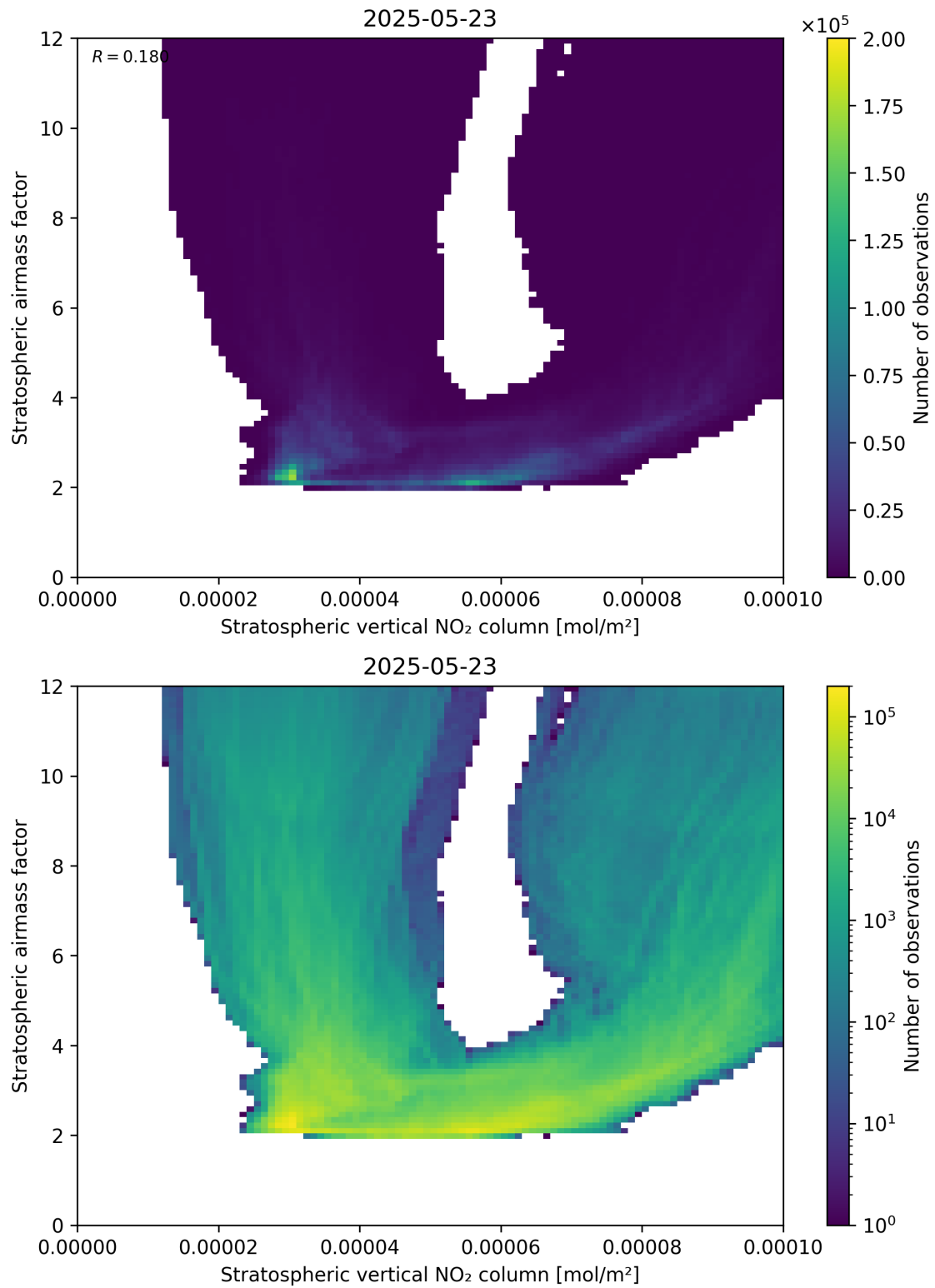
Figure 96: Scatter density plot of “Stratospheric vertical NO 2 column” against “Stratospheric airmass factor” for 2025-05-22 to 2025-05-24.
