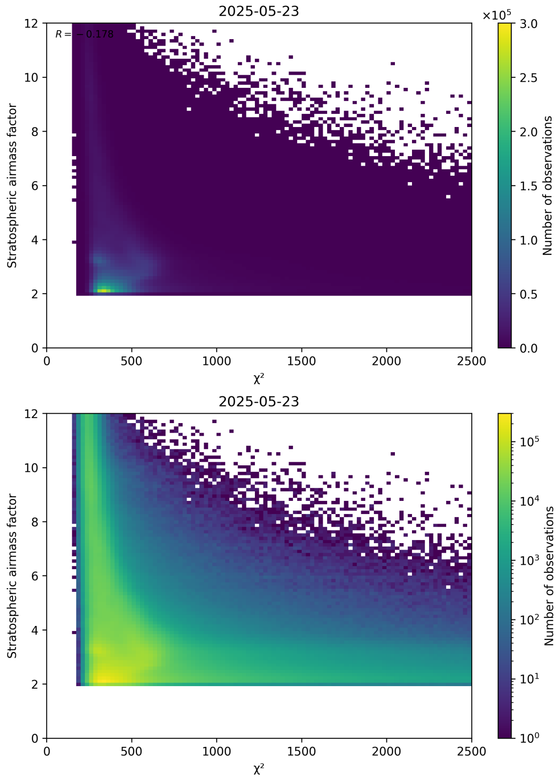
Figure 81: Scatter density plot of “ \chi^2 ” against “Stratospheric airmass factor” for 2025-05-22 to 2025-05-24.
