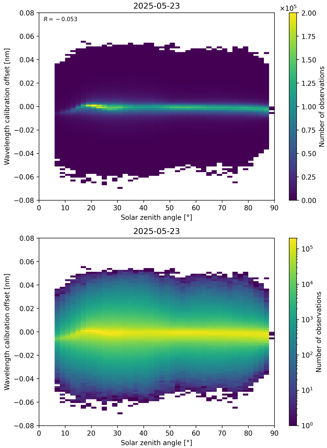
Figure 158: Scatter density plot of “Solar zenith angle” against “Wavelength calibration offset” for 2025-05-22 to 2025-05-24.
