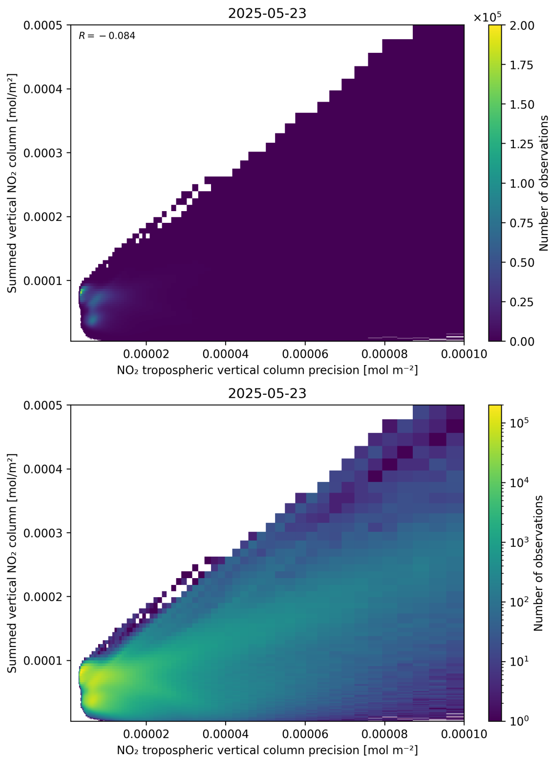
Figure 136: Scatter density plot of “NO 2 tropospheric vertical column precision” against “Summed vertical NO 2 column” for 2025-05-22 to 2025-05-24.
