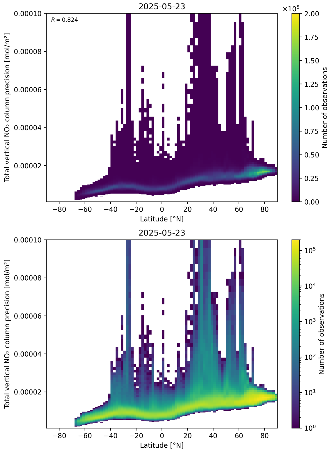
Figure 91: Scatter density plot of “Latitude” against “Total vertical NO 2 column precision” for 2025-05-22 to 2025-05-24.
