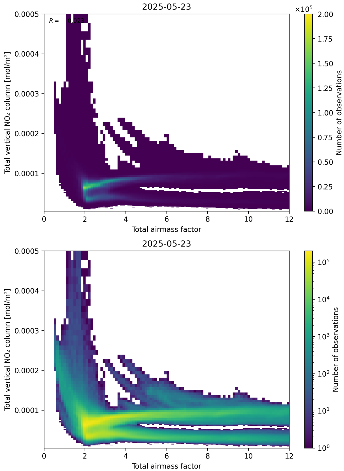
Figure 67: Scatter density plot of “Total airmass factor” against “Total vertical NO 2 column” for 2025-05-22 to 2025-05-24.
