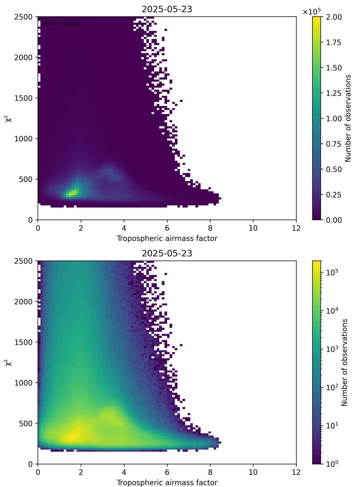
Figure 73: Scatter density plot of “Tropospheric airmass factor” against “ \chi^2 ” for 2025-05-22 to 2025-05-24.
