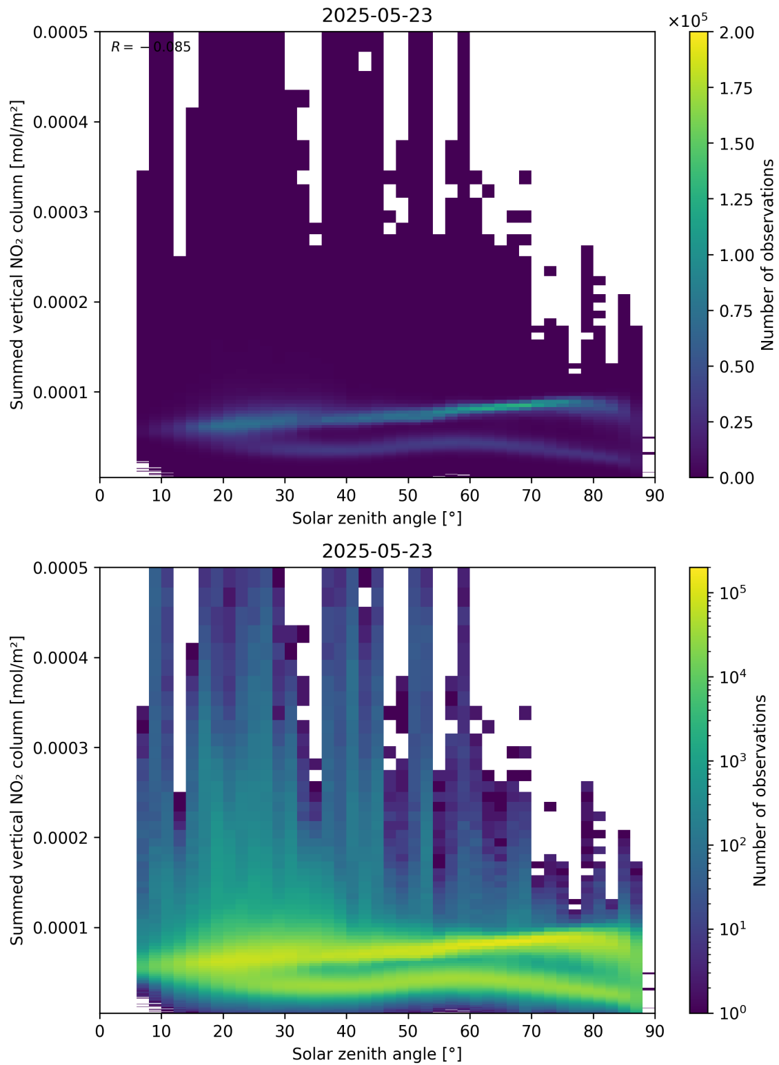
Figure 151: Scatter density plot of “Solar zenith angle” against “Summed vertical NO 2 column” for 2025-05-22 to 2025-05-24.
