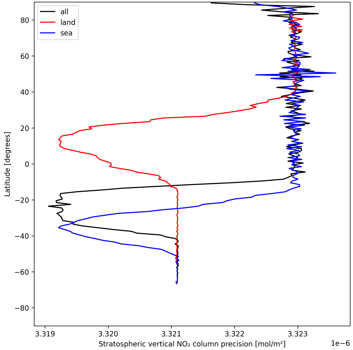
Figure 20: Zonal average of “Stratospheric vertical NO 2 column precision” for 2025-05-22 to 2025-05-24.
