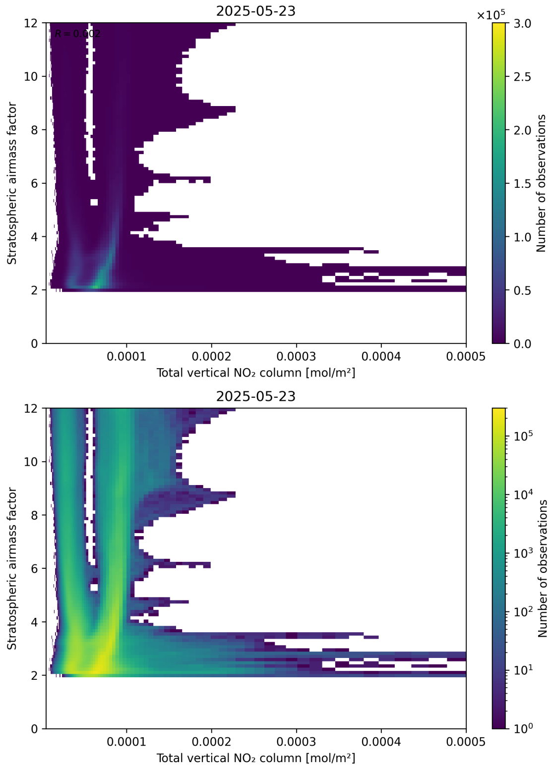
Figure 110: Scatter density plot of “Total vertical NO 2 column” against “Stratospheric airmass factor” for 2025-05-22 to 2025-05-24.
