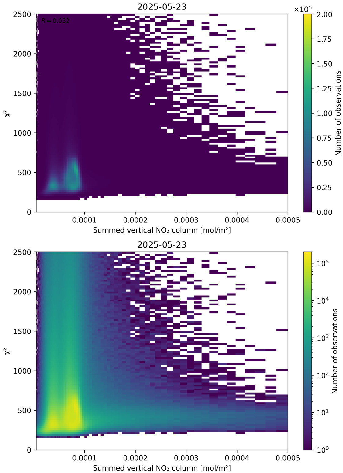
Figure 104: Scatter density plot of “Summed vertical NO 2 column” against “ \chi^2 ” for 2025-05-22 to 2025-05-24.
