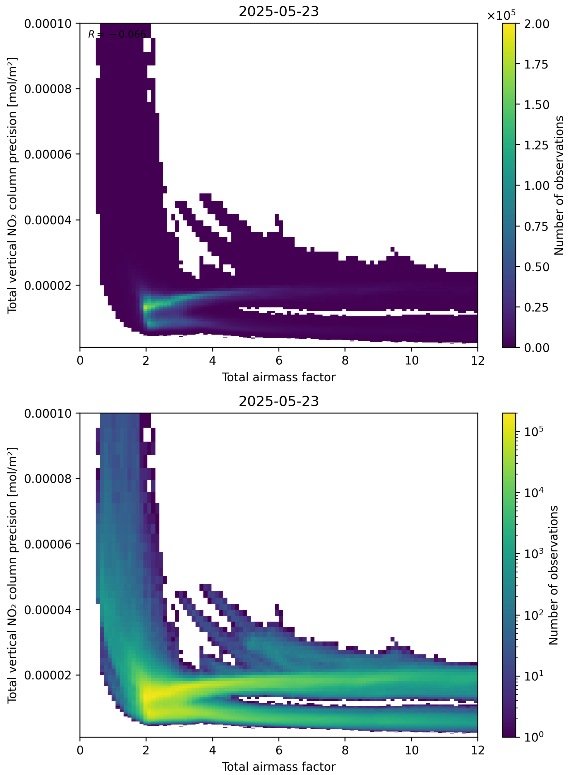
Figure 68: Scatter density plot of “Total airmass factor” against “Total vertical NO 2 column precision” for 2025-05-22 to 2025-05-24.
