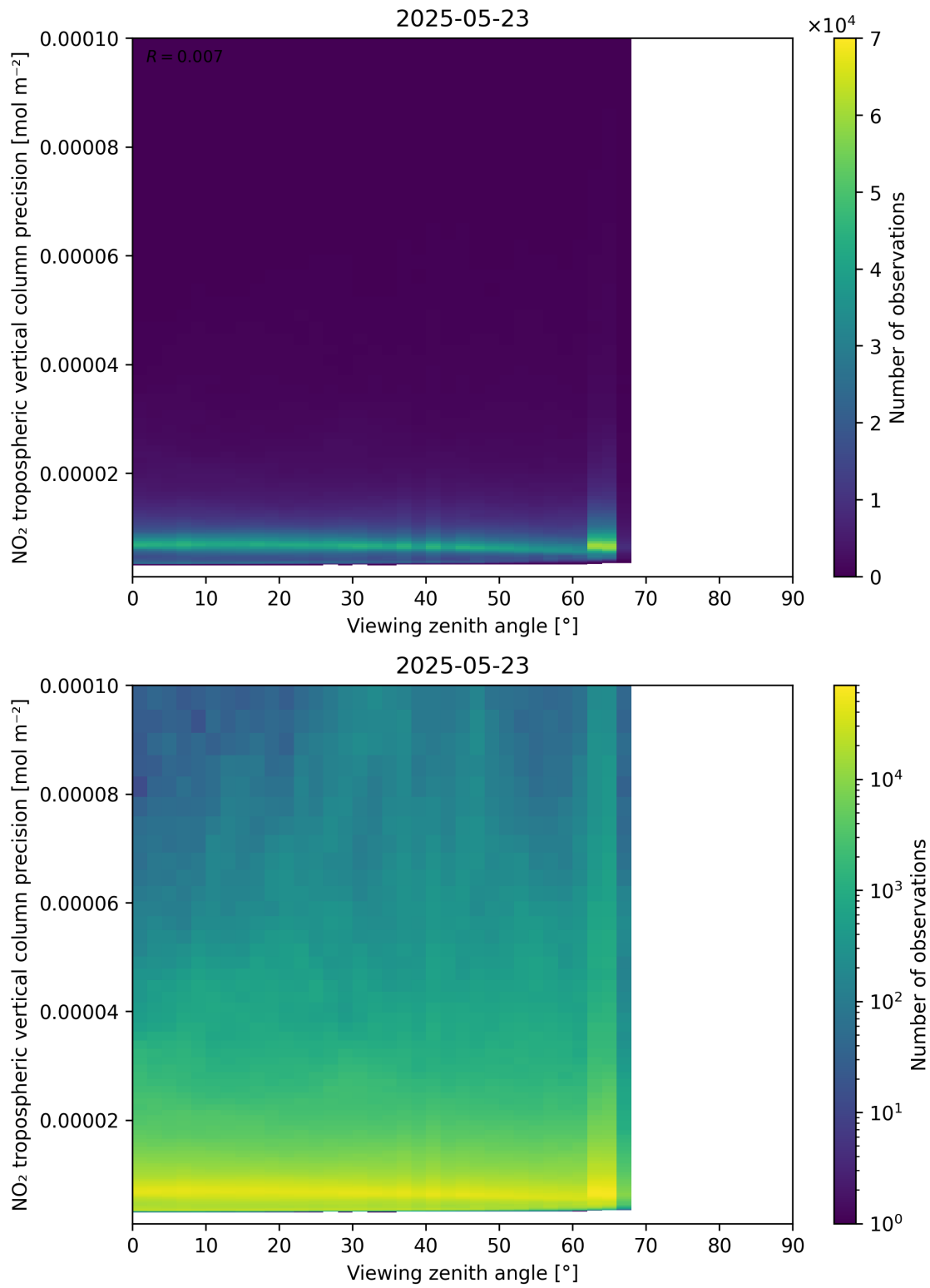
Figure 170: Scatter density plot of “Viewing zenith angle” against “NO 2 tropospheric vertical column precision” for 2025-05-22 to 2025-05-24.
