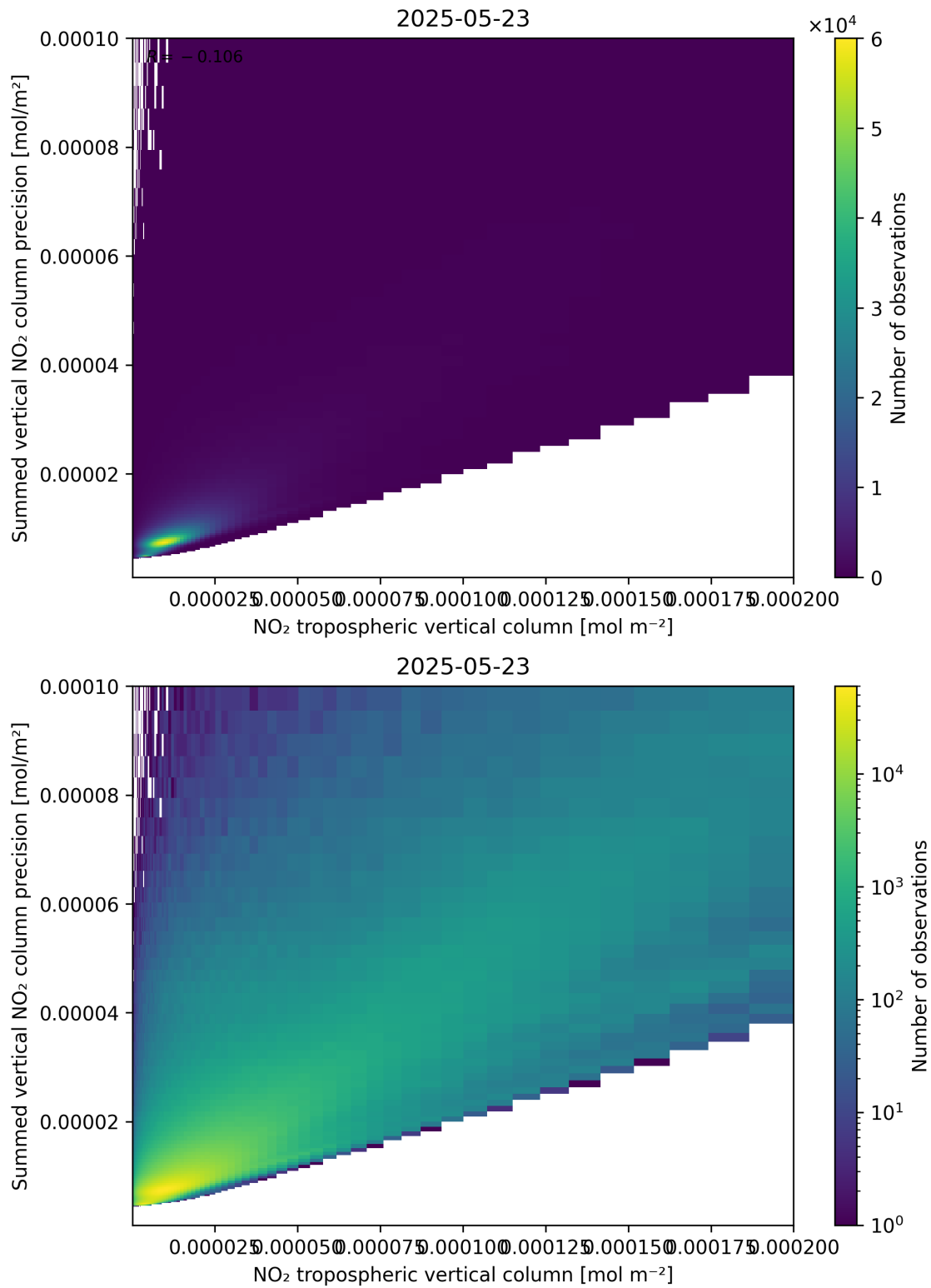
Figure 127: Scatter density plot of “NO 2 tropospheric vertical column” against “Summed vertical NO 2 column precision” for 2025-05-22 to 2025-05-24.
