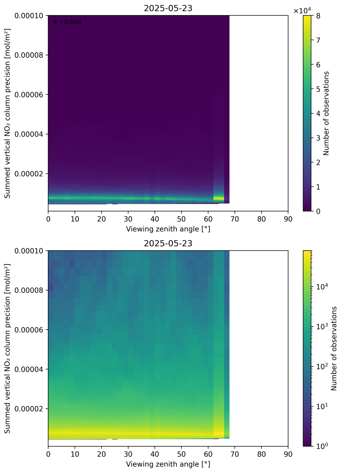
Figure 166: Scatter density plot of “Viewing zenith angle” against “Summed vertical NO 2 column precision” for 2025-05-22 to 2025-05-24.
