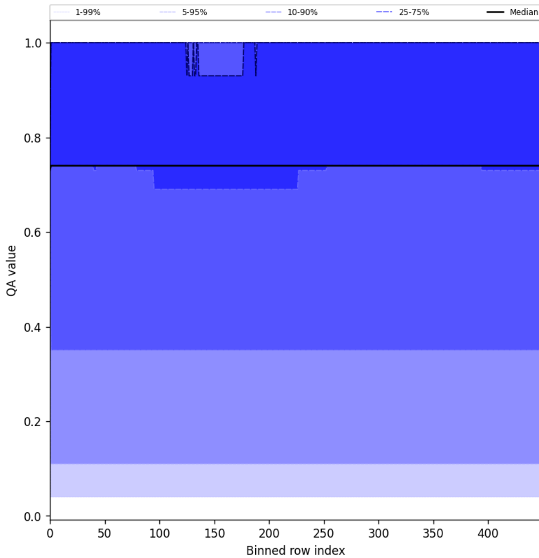
Figure 45: Along track statistics of “QA value” for 2025-05-22 to 2025-05-24
