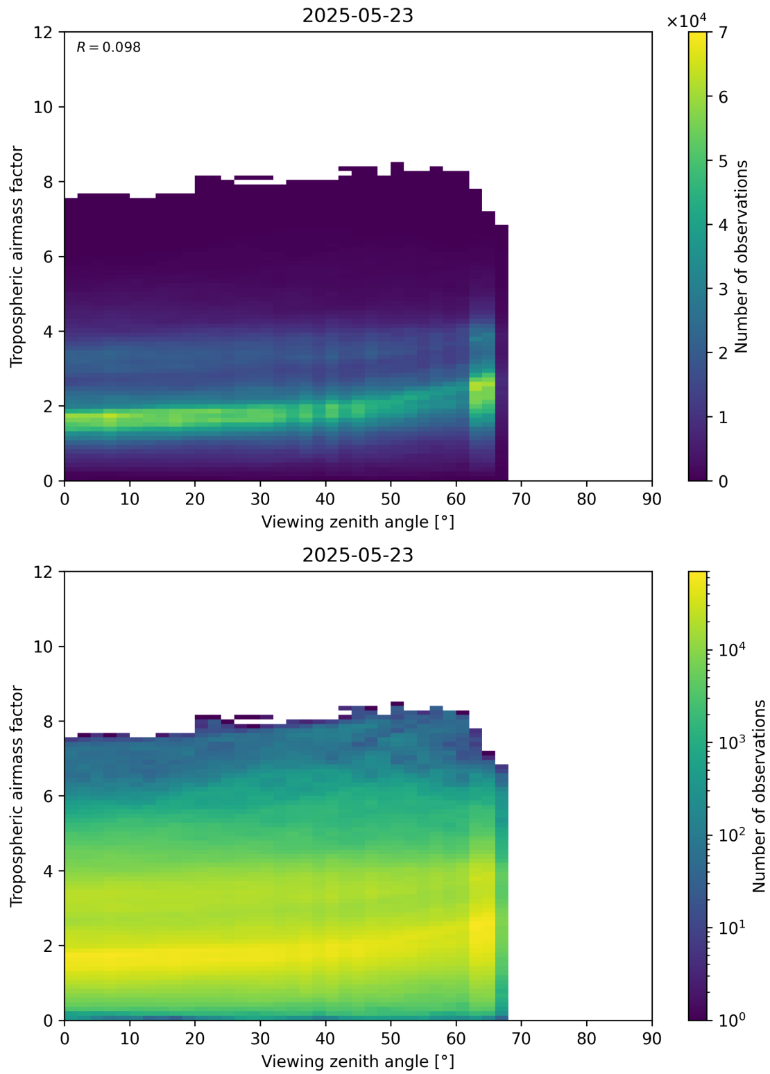
Figure 161: Scatter density plot of “Viewing zenith angle” against “Tropospheric airmass factor” for 2025-05-22 to 2025-05-24.
