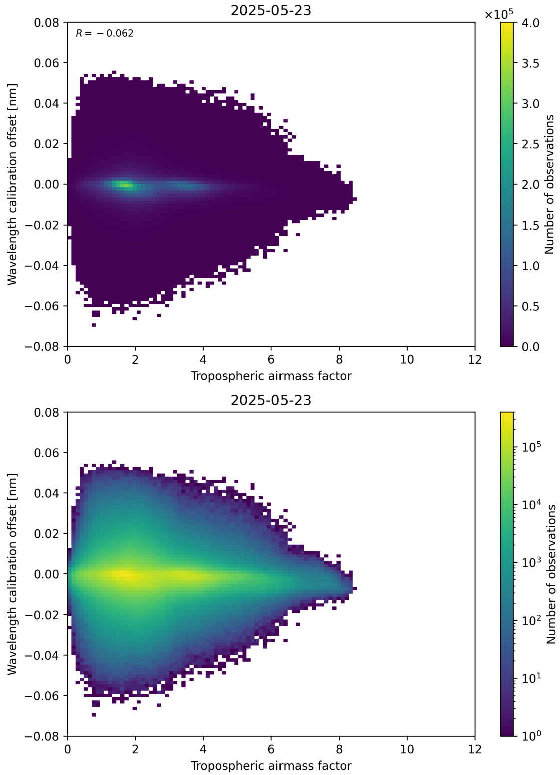
Figure 80: Scatter density plot of “Tropospheric airmass factor” against “Wavelength calibration offset” for 2025-05-22 to 2025-05-24.
