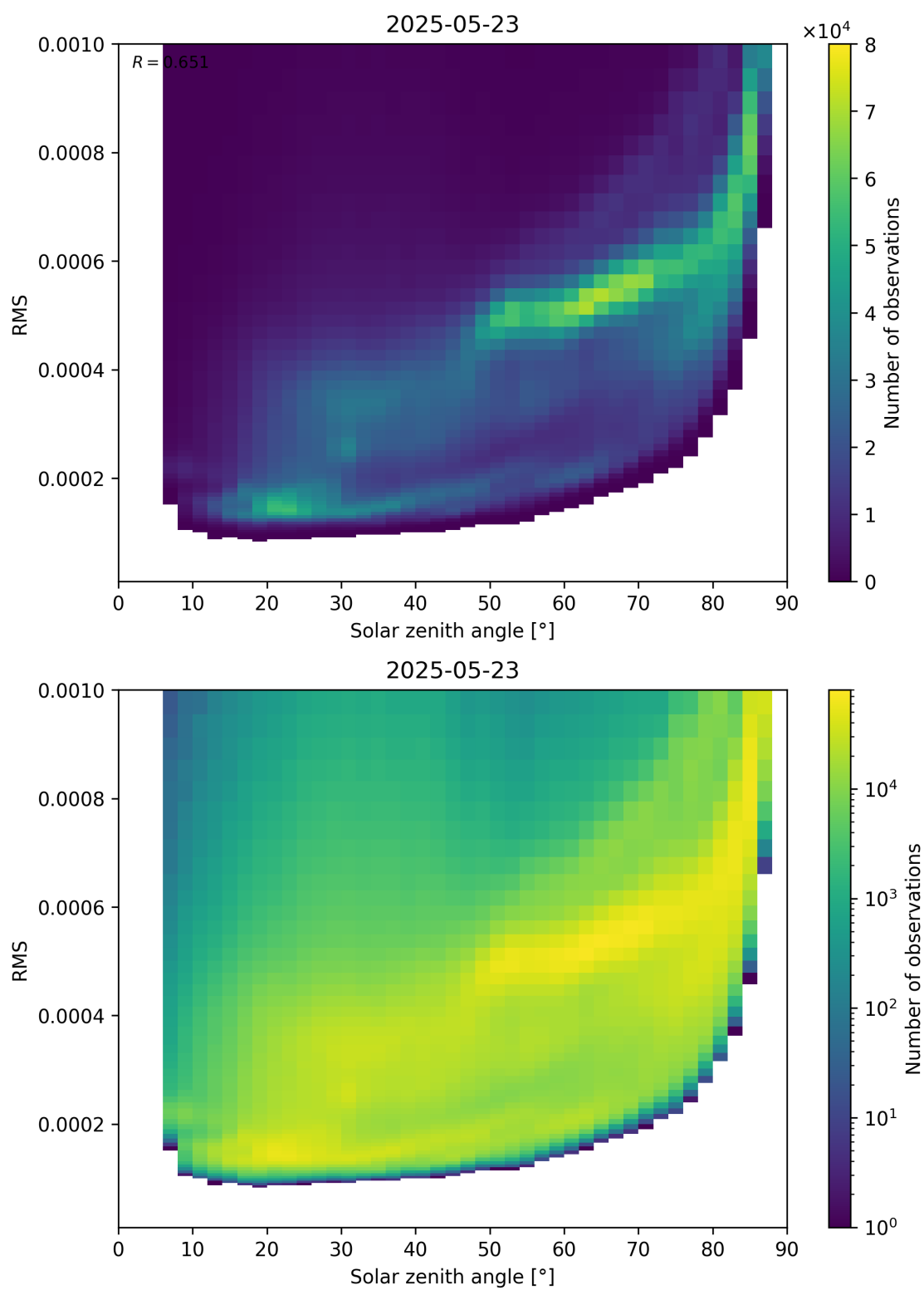
Figure 157: Scatter density plot of “Solar zenith angle” against “RMS” for 2025-05-22 to 2025-05-24.
