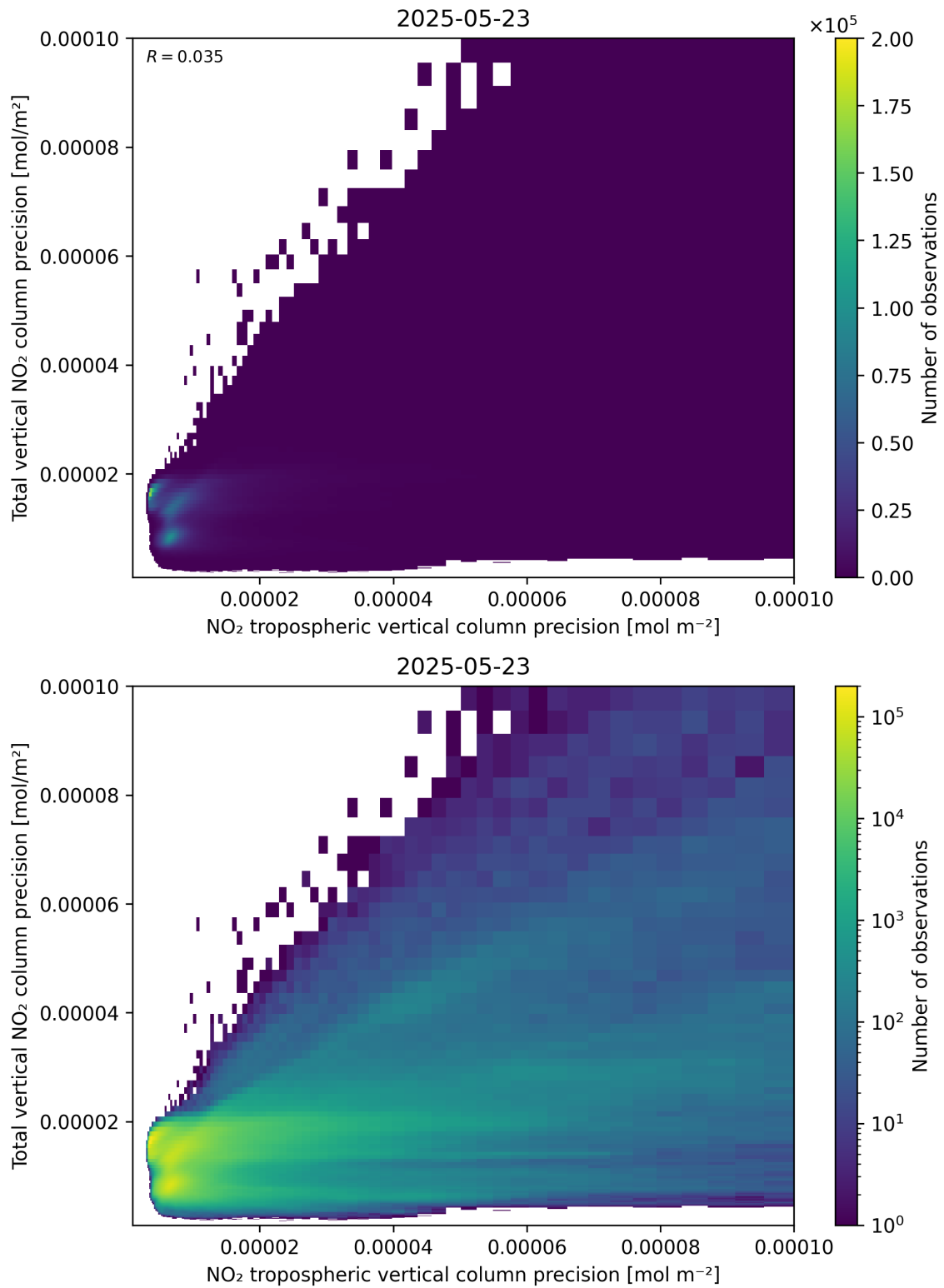
Figure 139: Scatter density plot of “NO 2 tropospheric vertical column precision” against “Total vertical NO 2 column precision” for 2025-05-22 to 2025-05-24.
