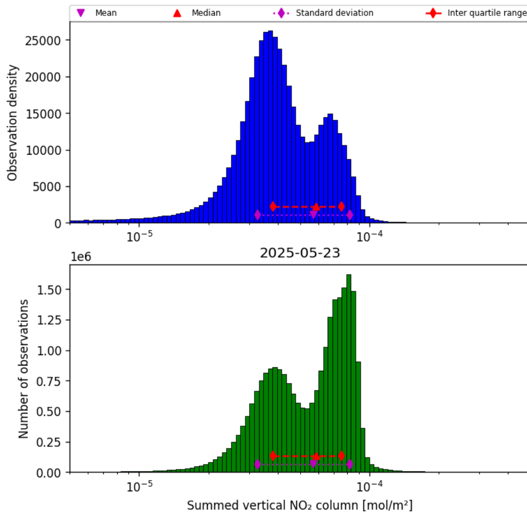
Figure 40: Histogram of “Summed vertical NO 2 column” for 2025-05-22 to 2025-05-24
