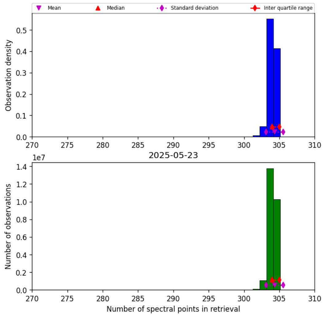
Figure 33: Histogram of “Number of spectral points in retrieval” for 2025-05-22 to 2025-05-24
