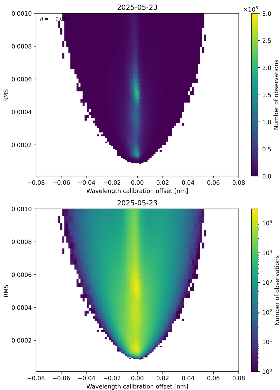
Figure 181: Scatter density plot of “Wavelength calibration offset” against “RMS” for 2025-05-22 to 2025-05-24.
