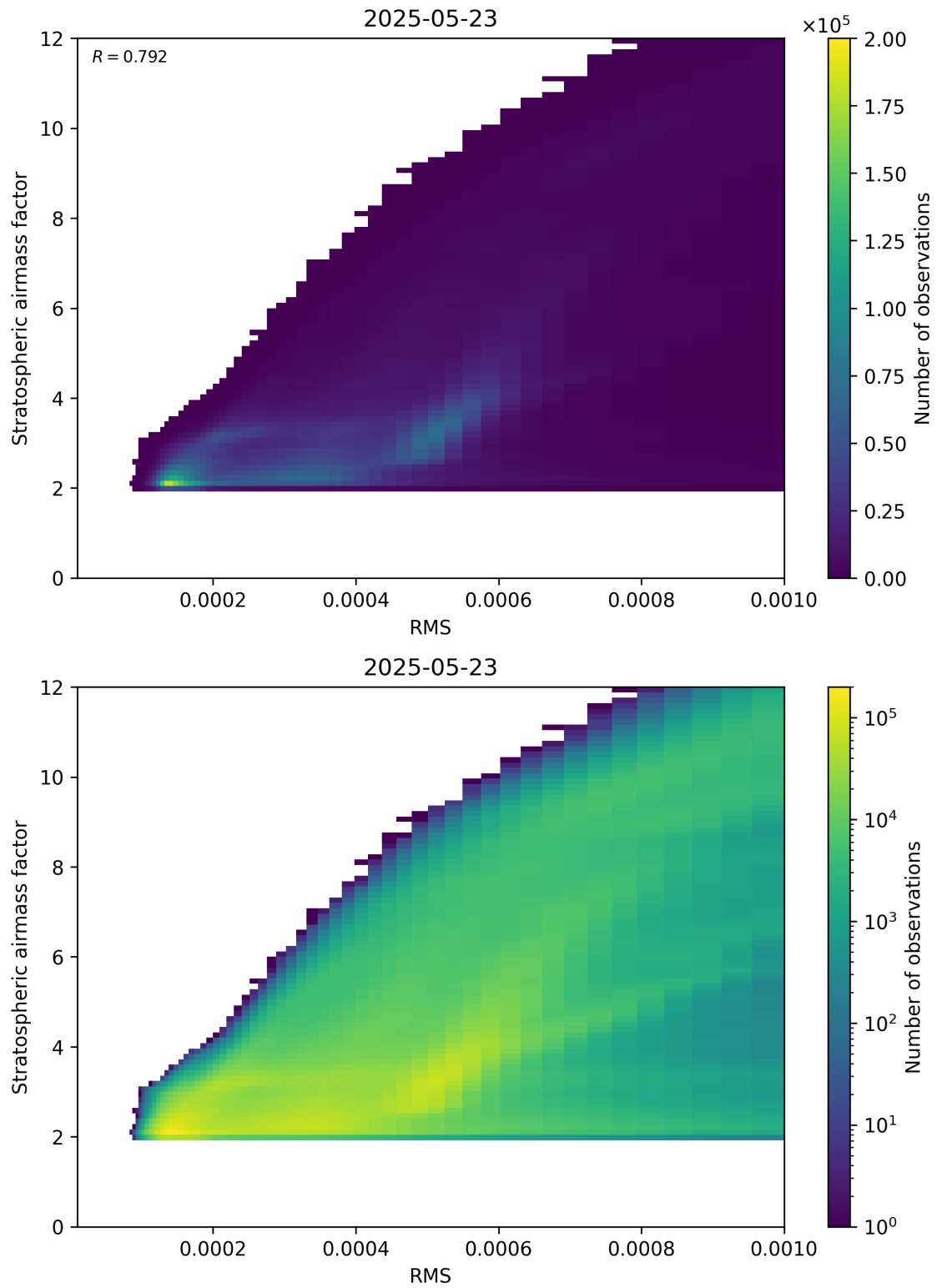
Figure 144: Scatter density plot of “RMS” against “Stratospheric airmass factor” for 2025-05-22 to 2025-05-24.
