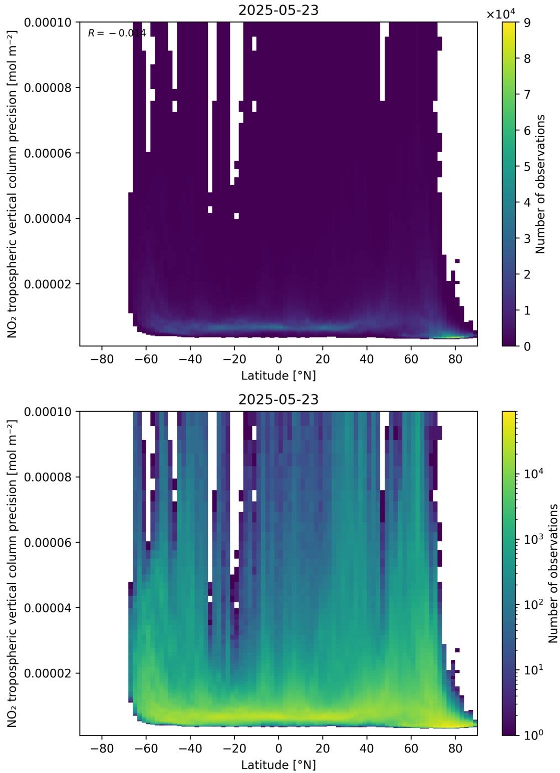
Figure 93: Scatter density plot of “Latitude” against “NO 2 tropospheric vertical column precision” for 2025-05-22 to 2025-05-24.
