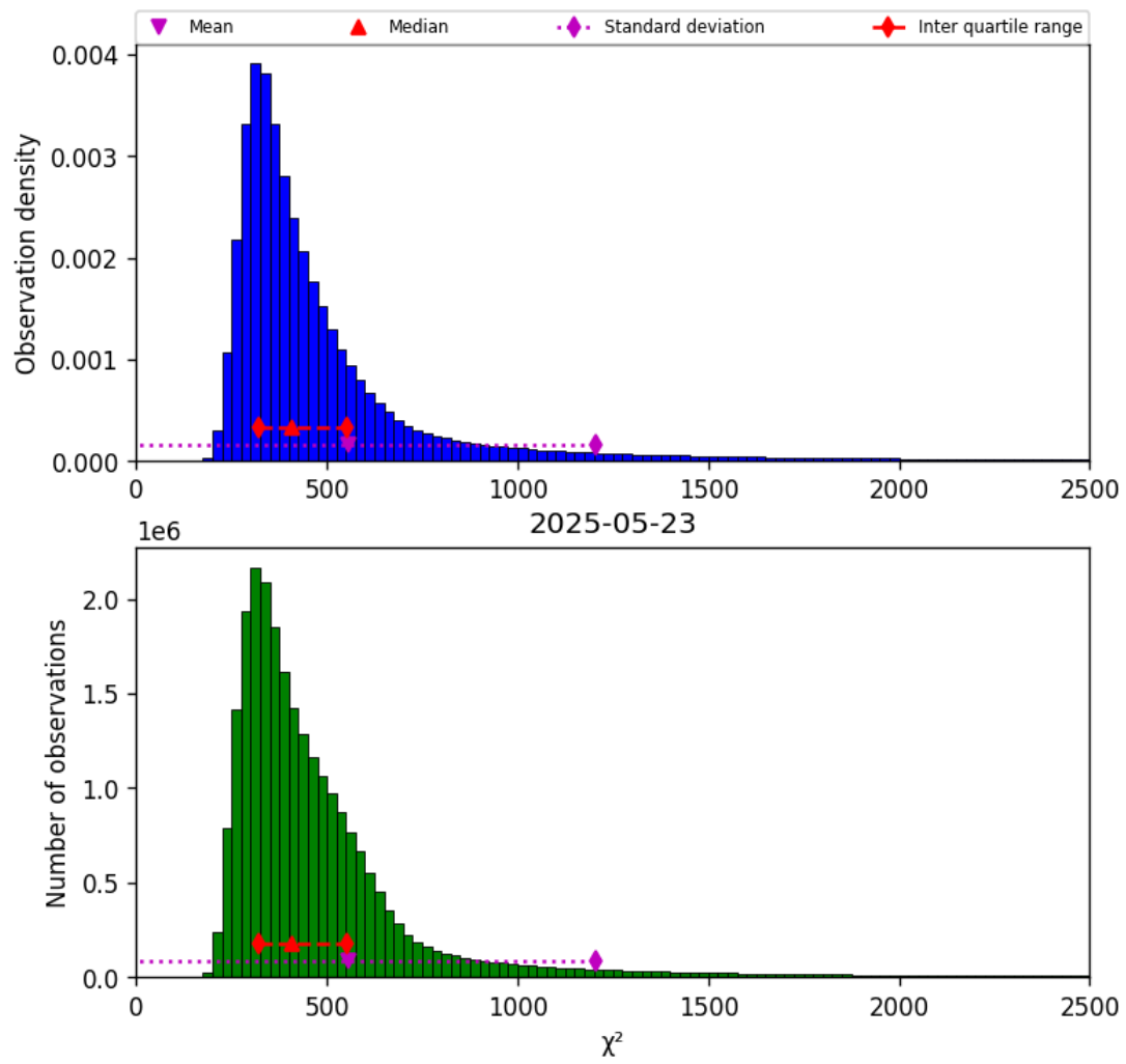
Figure 42: Histogram of " \chi^2 " for 2025-05-22 to 2025-05-24
