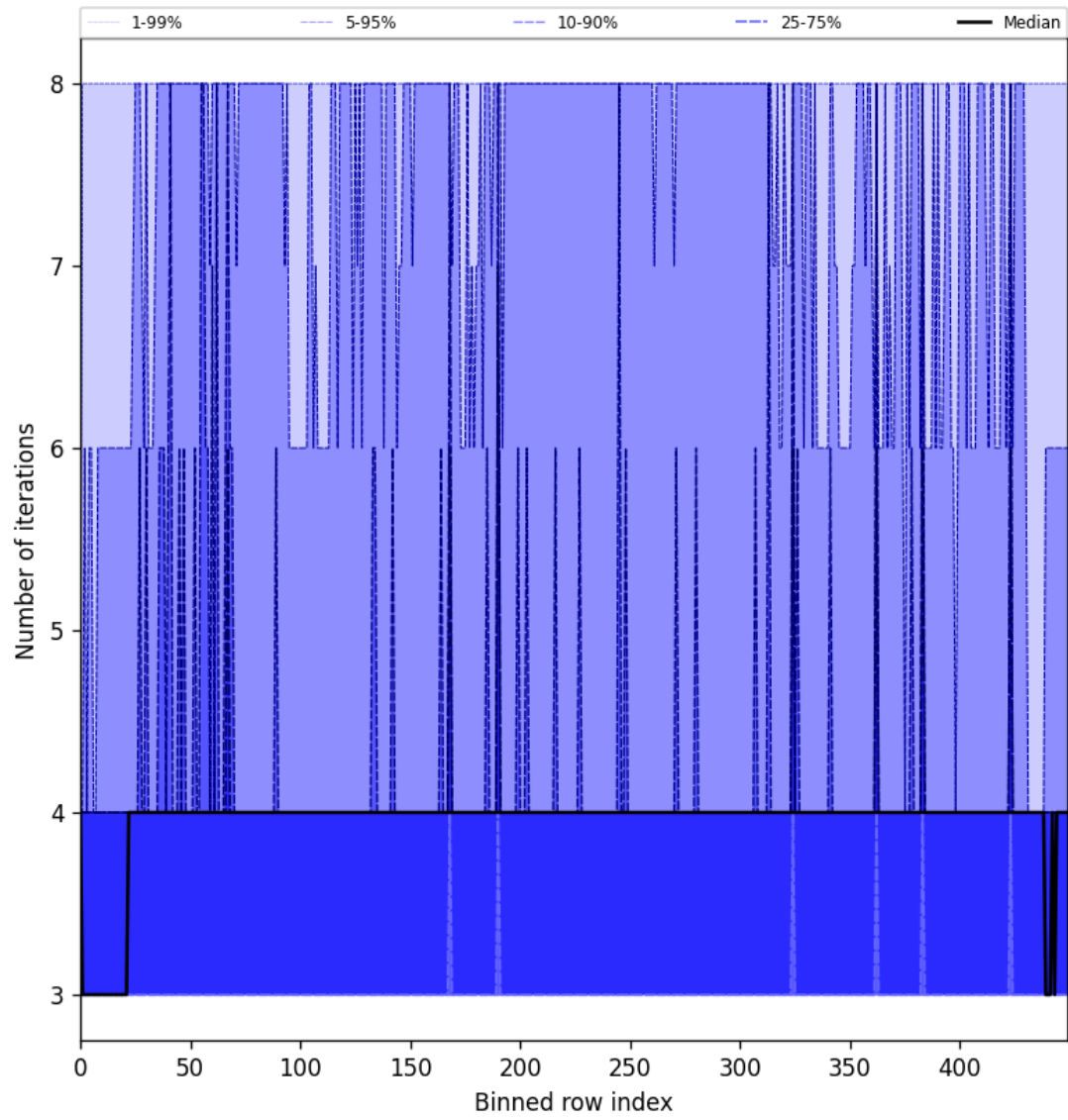
Figure 51: Along track statistics of “Number of iterations” for 2025-05-22 to 2025-05-24
