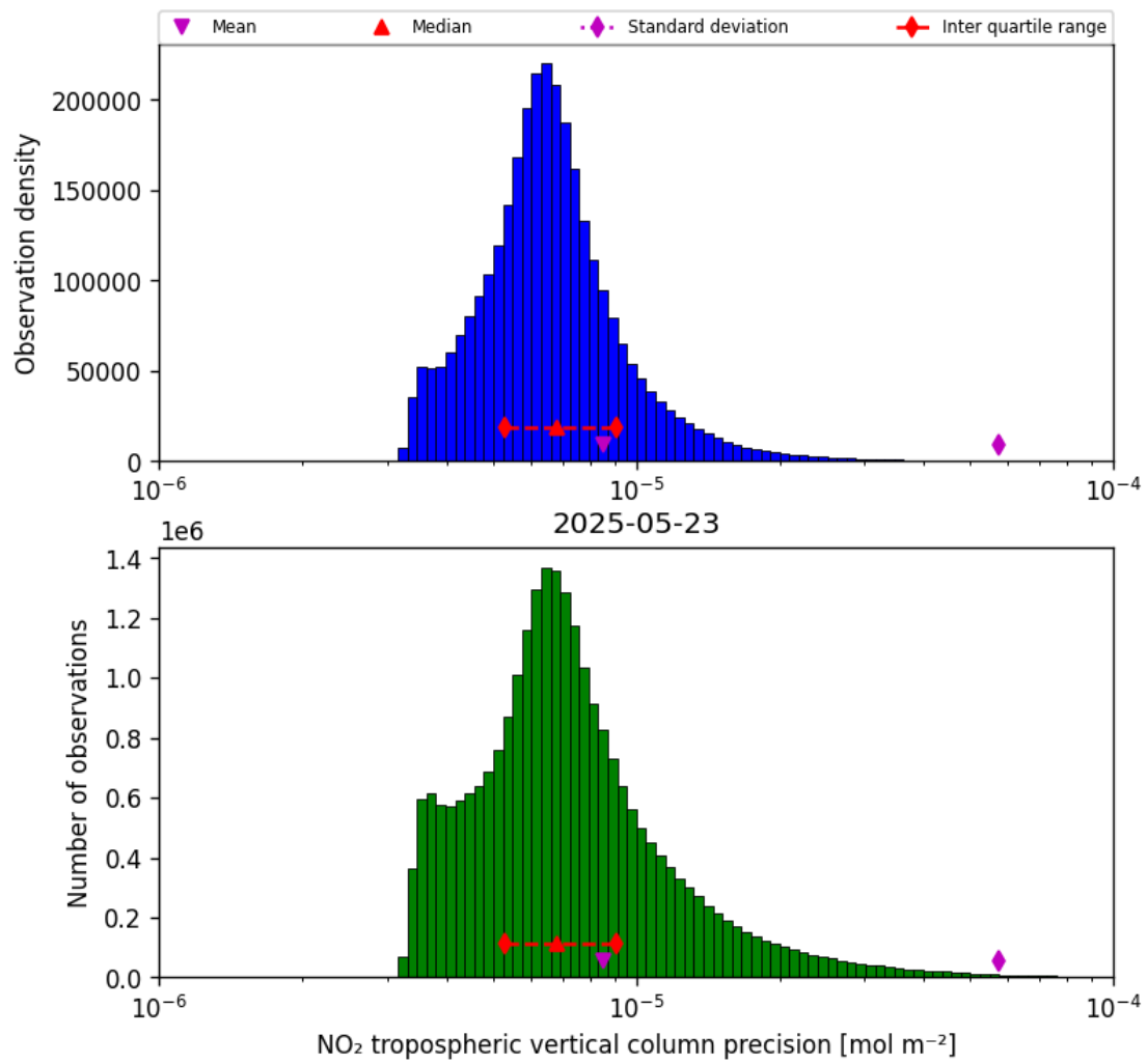
Figure 30: Histogram of “NO 2 tropospheric vertical column precision” for 2025-05-22 to 2025-05-24
