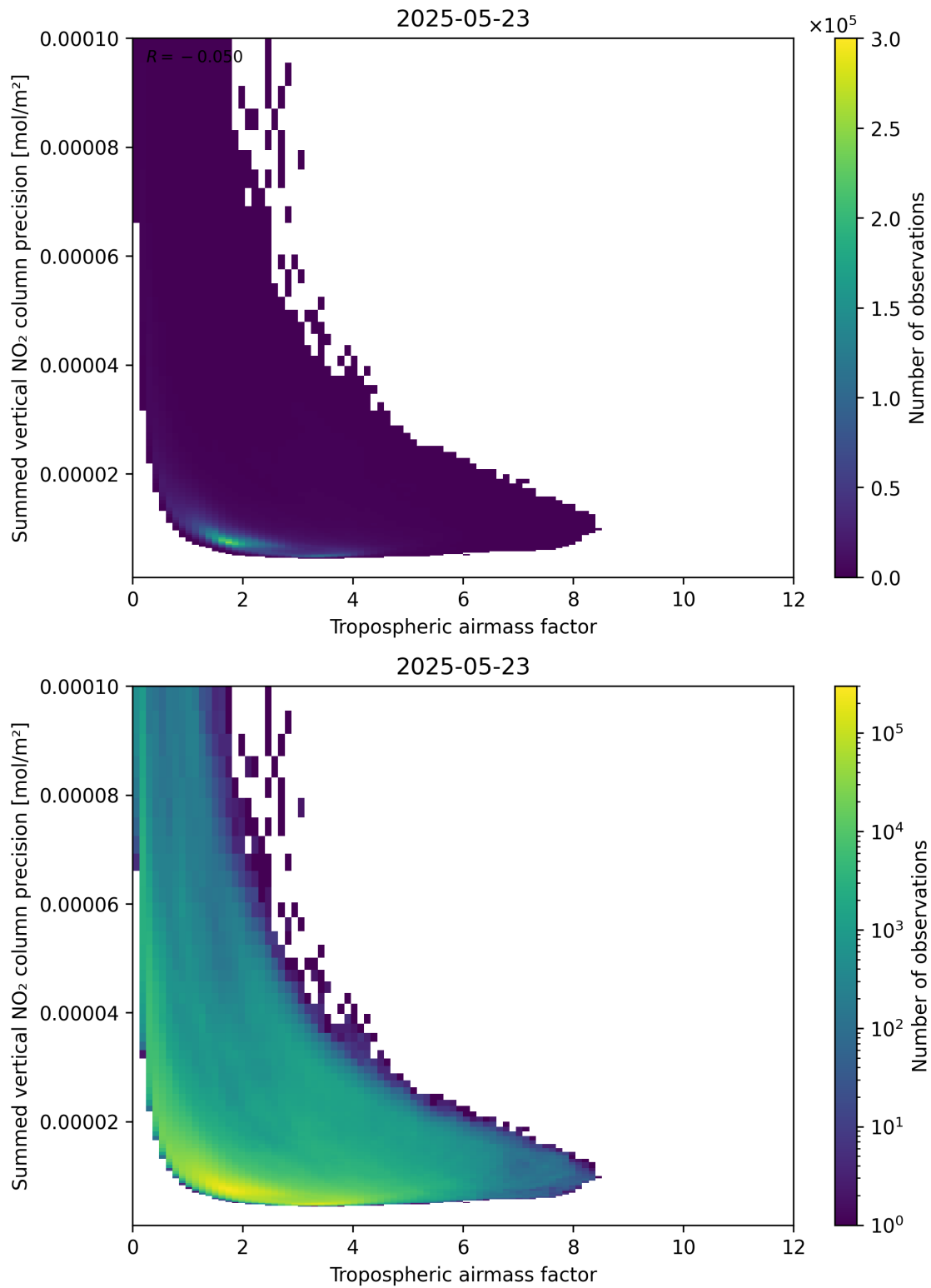
Figure 76: Scatter density plot of “Tropospheric air mass factor” against “Summed vertical NO 2 column precision” for 2025-05-22 to 2025-05-24.
