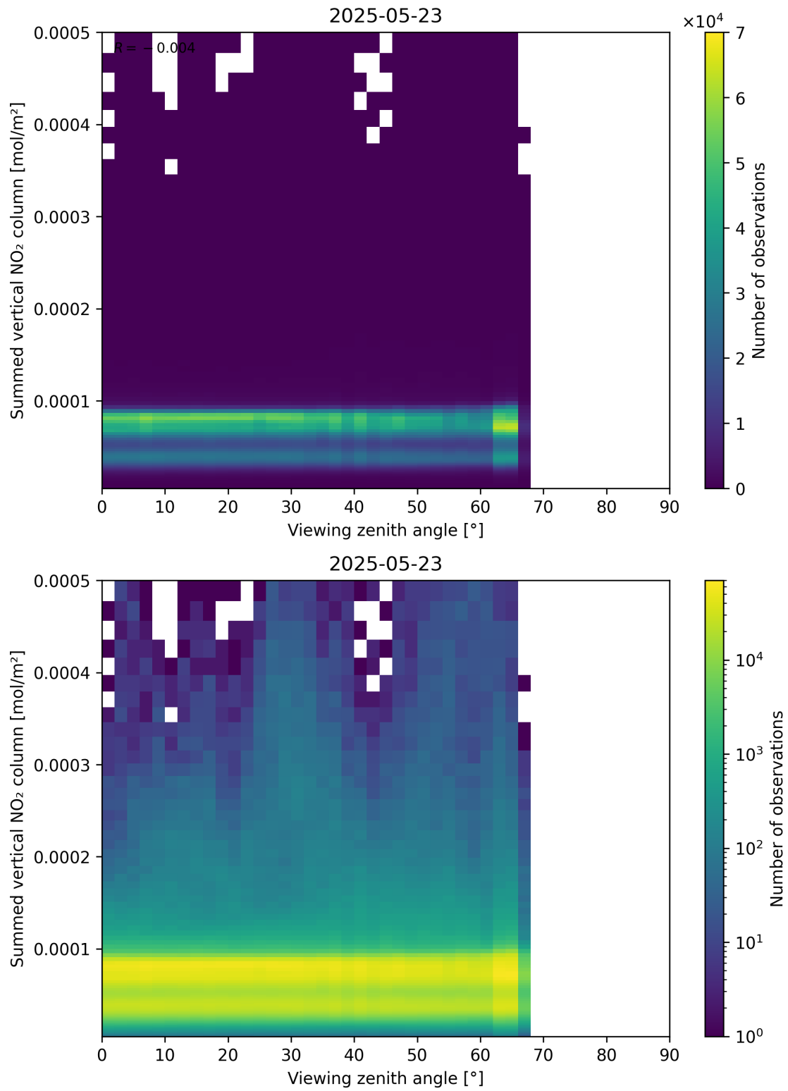
Figure 165: Scatter density plot of “Viewing zenith angle” against “Summed vertical NO 2 column” for 2025-05-22 to 2025-05-24.
