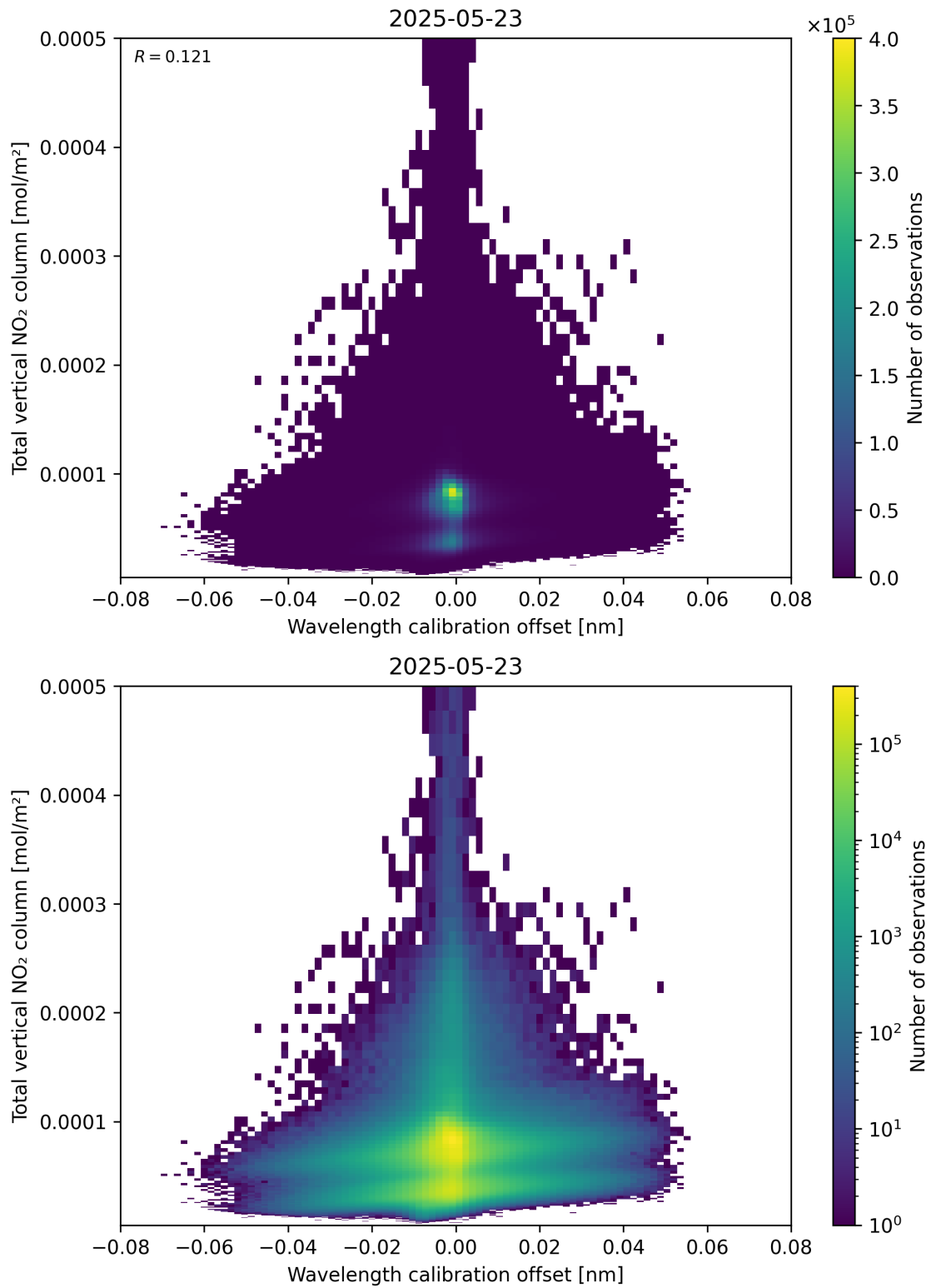
Figure 179: Scatter density plot of “Wavelength calibration offset” against “Total vertical NO 2 column” for 2025-05-22 to 2025-05-24.
