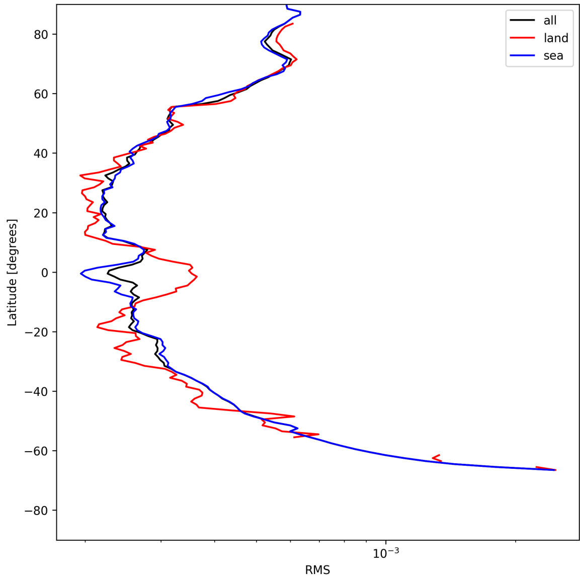
Figure 26: Zonal average of “RMS” for 2025-05-22 to 2025-05-24.
