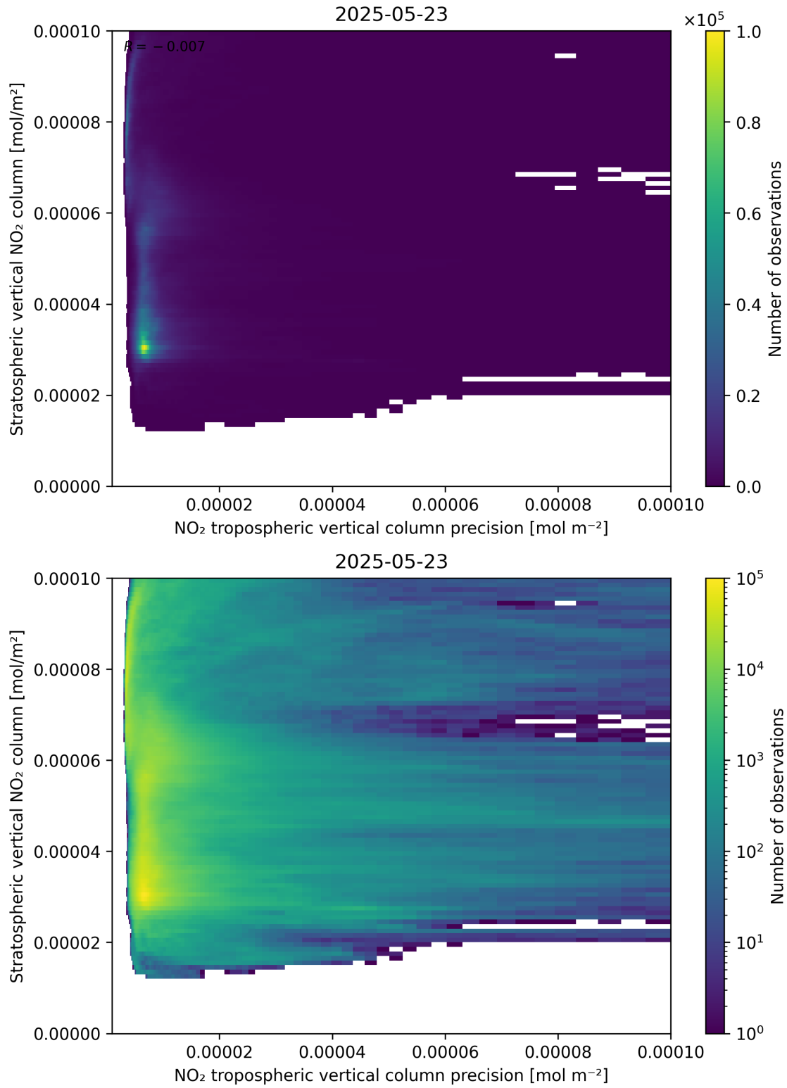
Figure 135: Scatter density plot of “NO 2 tropospheric vertical column precision” against “Stratospheric vertical NO 2 column” for 2025-05-22 to 2025-05-24.
