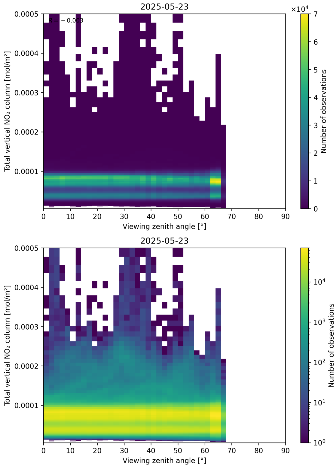
Figure 167: Scatter density plot of “Viewing zenith angle” against “Total vertical NO 2 column” for 2025-05-22 to 2025-05-24.
