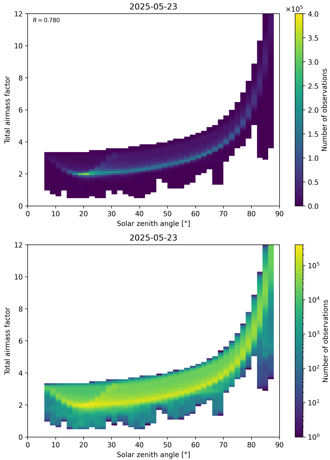
Figure 146: Scatter density plot of “Solar zenith angle” against “Total air mass factor” for 2025-05-22 to 2025-05-24.
