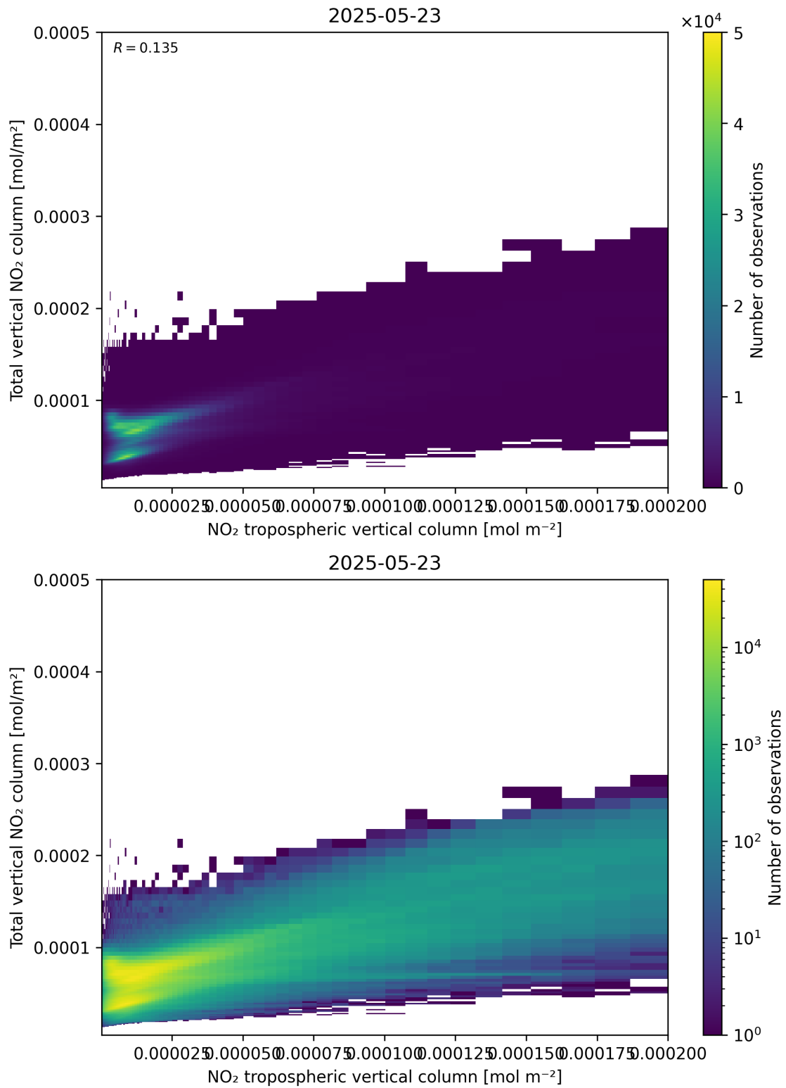
Figure 128: Scatter density plot of “NO 2 tropospheric vertical column” against “Total vertical NO 2 column” for 2025-05-22 to 2025-05-24.
