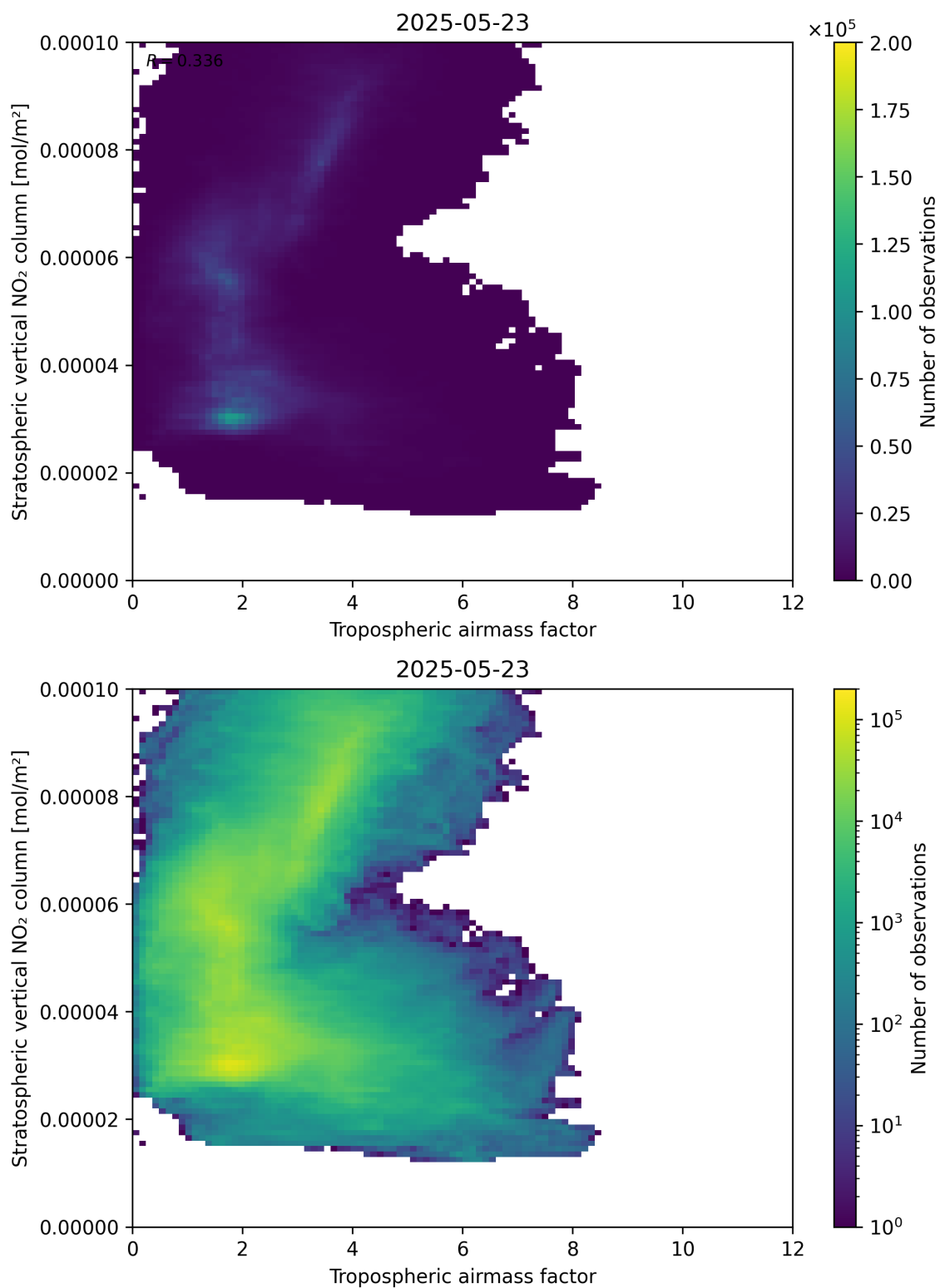
Figure 74: Scatter density plot of “Tropospheric air mass factor” against “Stratospheric vertical NO 2 column” for 2025-05-22 to 2025-05-24.
