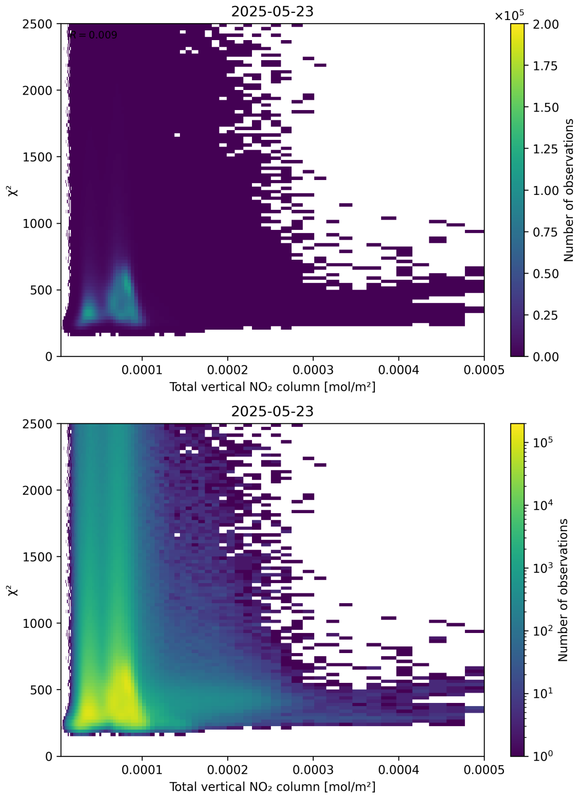
Figure 111: Scatter density plot of “Total vertical NO 2 column” against “ \chi^2 ” for 2025-05-22 to 2025-05-24.
