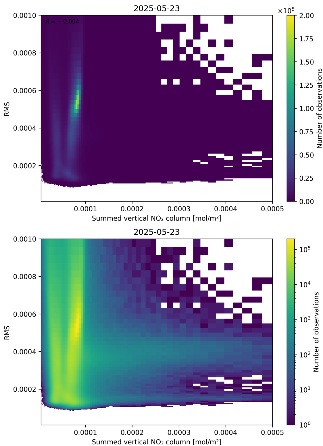
Figure 109: Scatter density plot of “Summed vertical NO 2 column” against “RMS” for 2025-05-22 to 2025-05-24.
