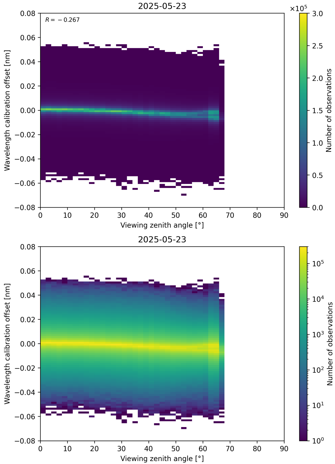
Figure 173: Scatter density plot of “Viewing zenith angle” against “Wavelength calibration offset” for 2025-05-22 to 2025-05-24.
