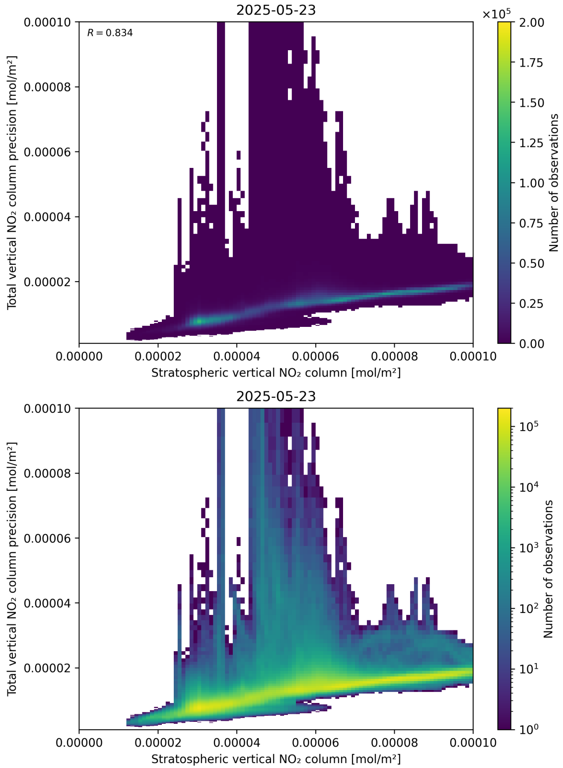
Figure 101: Scatter density plot of “Stratospheric vertical NO 2 column” against “Total vertical NO 2 column precision” for 2025-05-22 to 2025-05-24.
