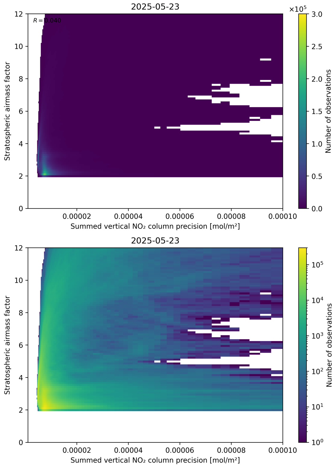
Figure 106: Scatter density plot of “Summed vertical NO 2 column precision” against “Stratospheric airmass factor” for 2025-05-22 to 2025-05-24.
