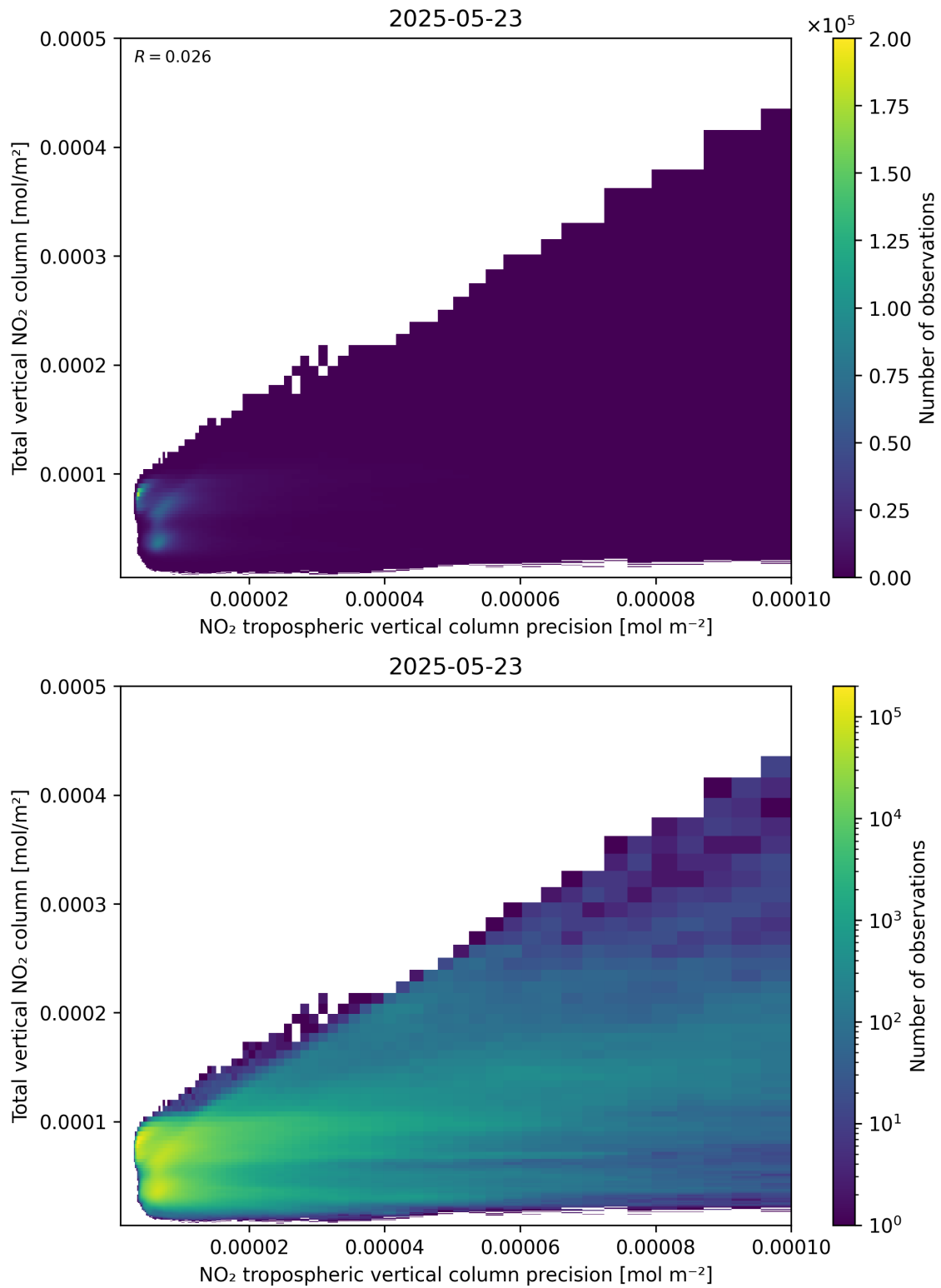
Figure 138: Scatter density plot of “NO 2 tropospheric vertical column precision” against “Total vertical NO 2 column” for 2025-05-22 to 2025-05-24.
