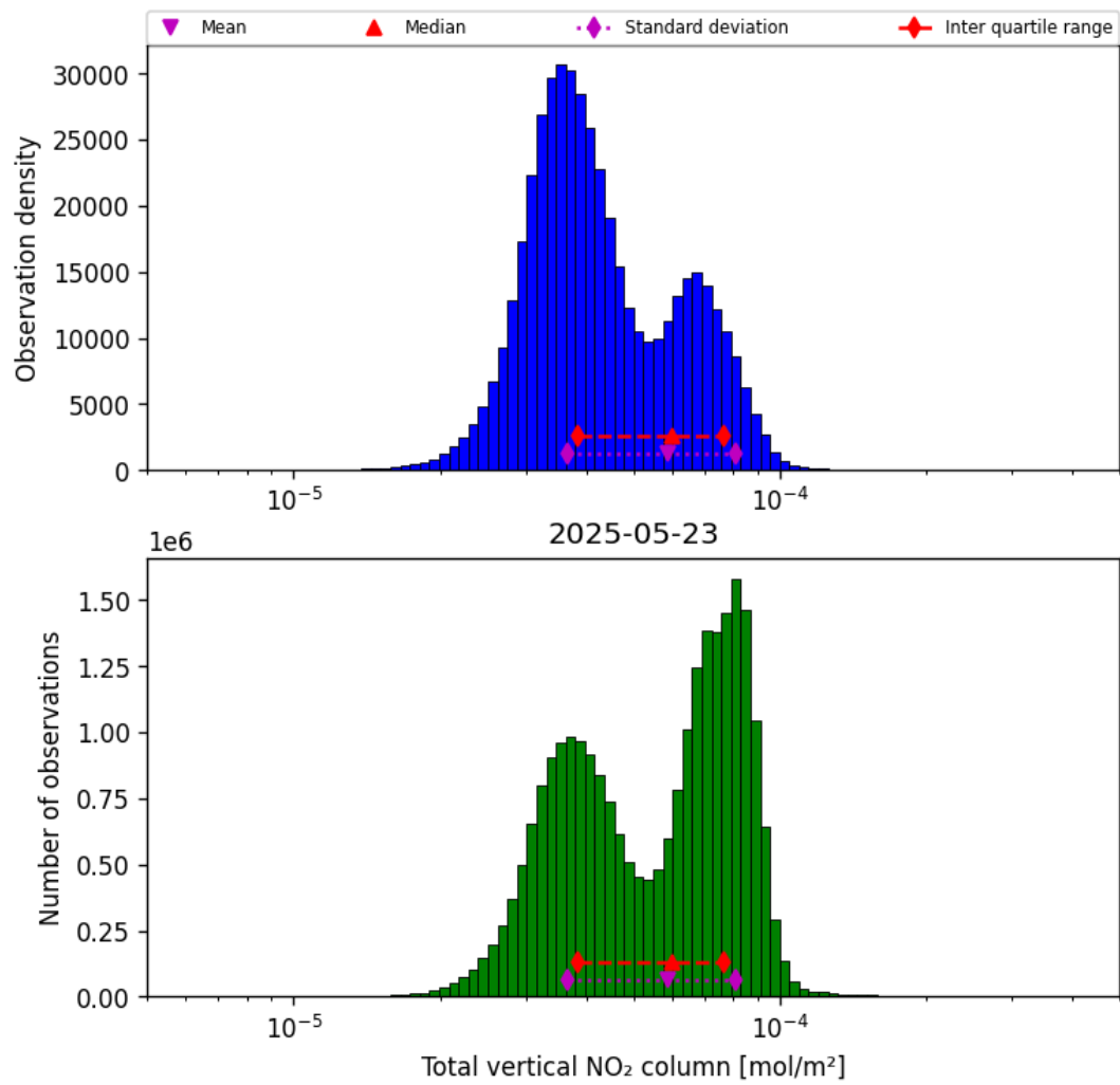
Figure 38: Histogram of “Total vertical NO 2 column” for 2025-05-22 to 2025-05-24
