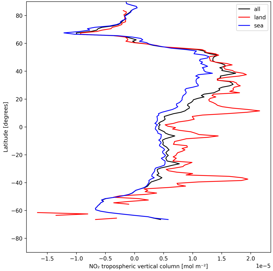
Figure 12: Zonal average of “NO 2 tropospheric vertical column” for 2025-05-22 to 2025-05-24.
