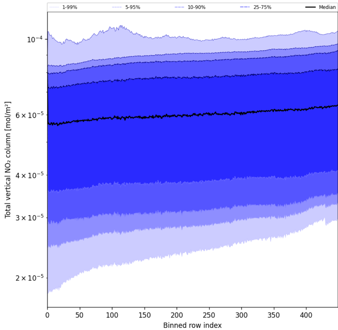
Figure 55: Along track statistics of “Total vertical NO 2 column” for 2025-05-22 to 2025-05-24
