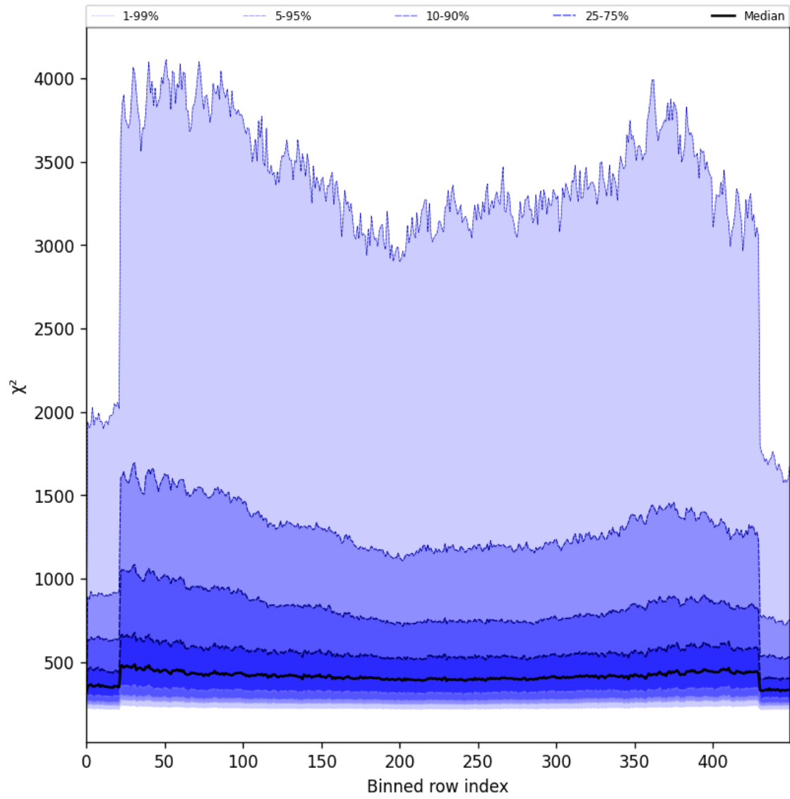
Figure 59: Along track statistics of “ \chi^2 ” for 2025-05-22 to 2025-05-24
