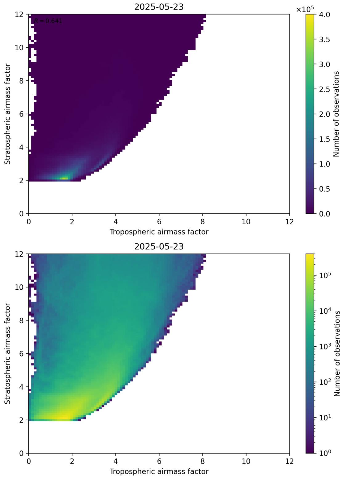
Figure 71: Scatter density plot of “Tropospheric airmass factor” against “Stratospheric airmass factor” for 2025-05-22 to 2025-05-24.
