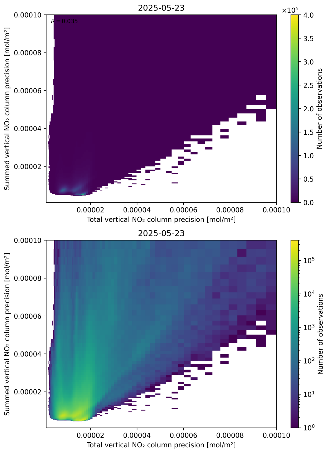
Figure 118: Scatter density plot of “Total vertical NO 2 column precision” against “Summed vertical NO 2 column precision” for 2025-05-22 to 2025-05-24.
