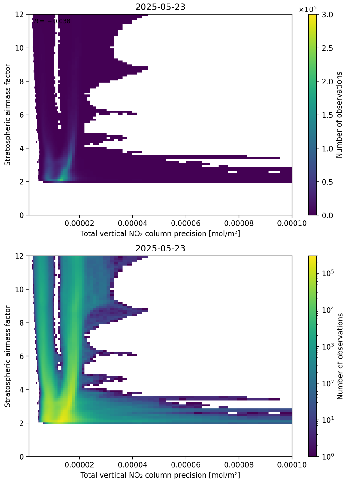
Figure 115: Scatter density plot of “Total vertical NO 2 column precision” against “Stratospheric air mass factor” for 2025-05-22 to 2025-05-24.
