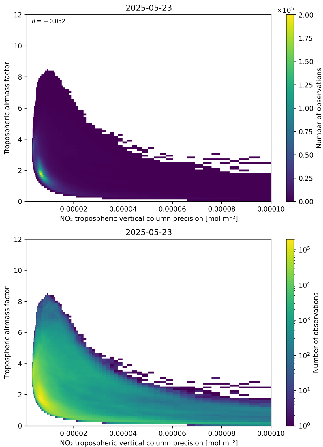
Figure 133: Scatter density plot of “NO 2 tropospheric vertical column precision” against “Tropospheric airmass factor” for 2025-05-22 to 2025-05-24.
