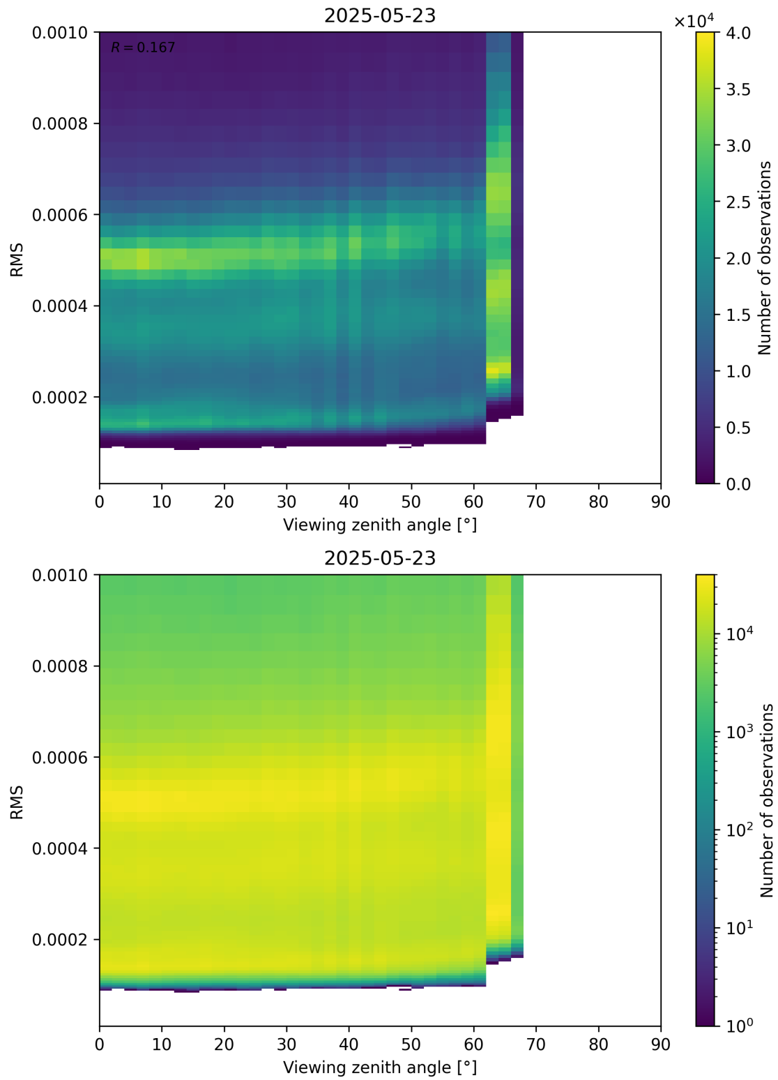
Figure 171: Scatter density plot of “Viewing zenith angle” against “RMS” for 2025-05-22 to 2025-05-24.
