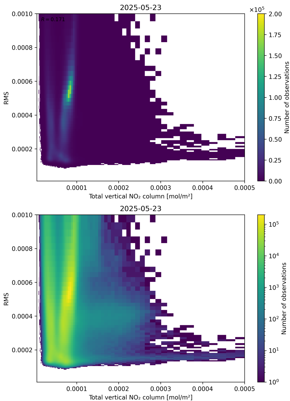
Figure 120: Scatter density plot of “Total vertical NO 2 column” against “RMS” for 2025-05-22 to 2025-05-24.
