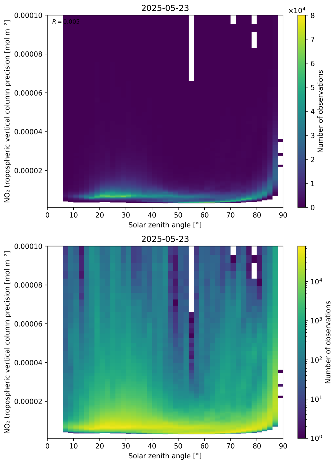
Figure 156: Scatter density plot of “Solar zenith angle” against “NO 2 tropospheric vertical column precision” for 2025-05-22 to 2025-05-24.
