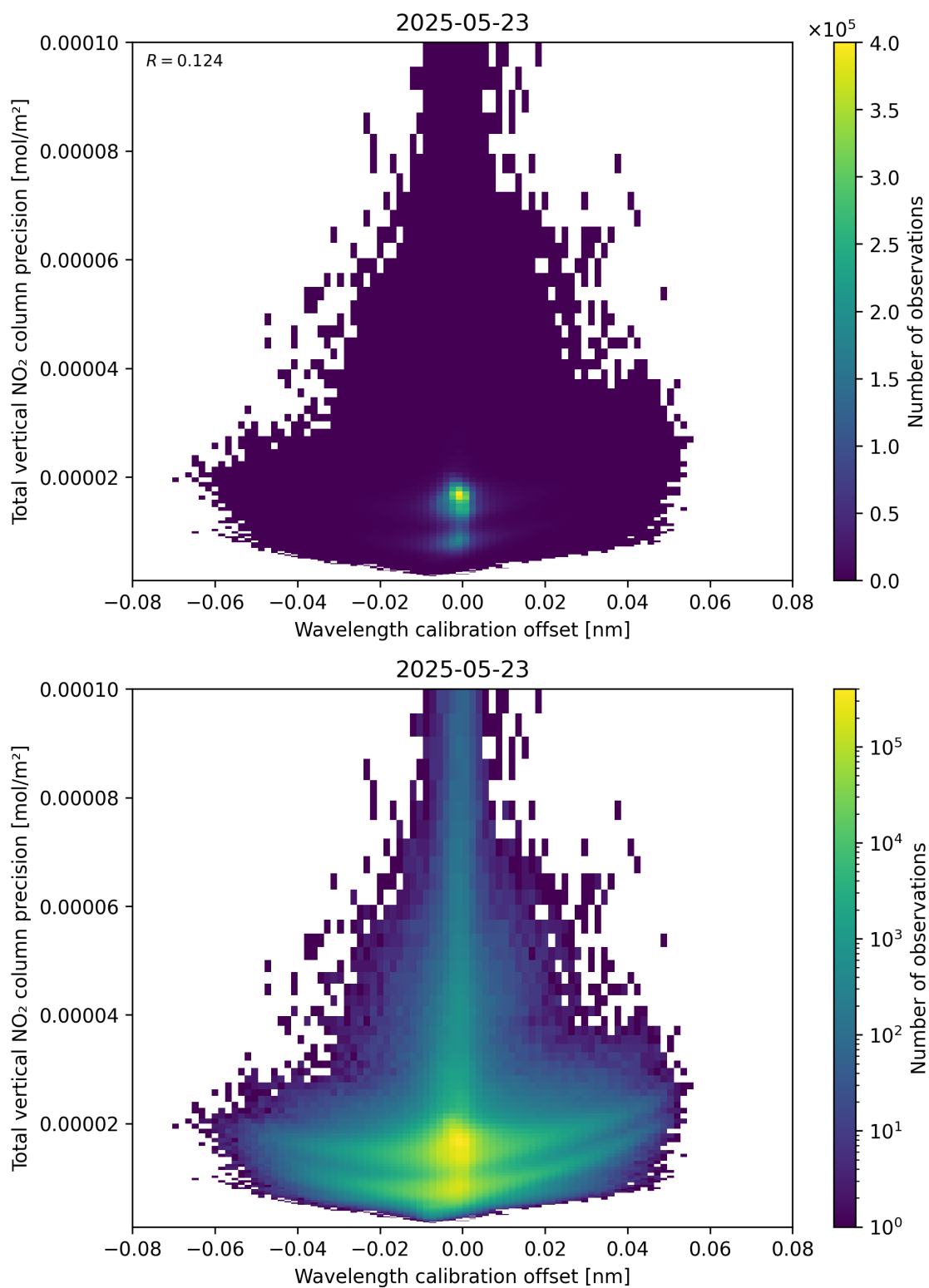
Figure 180: Scatter density plot of “Wavelength calibration offset” against “Total vertical NO 2 column precision” for 2025-05-22 to 2025-05-24.
