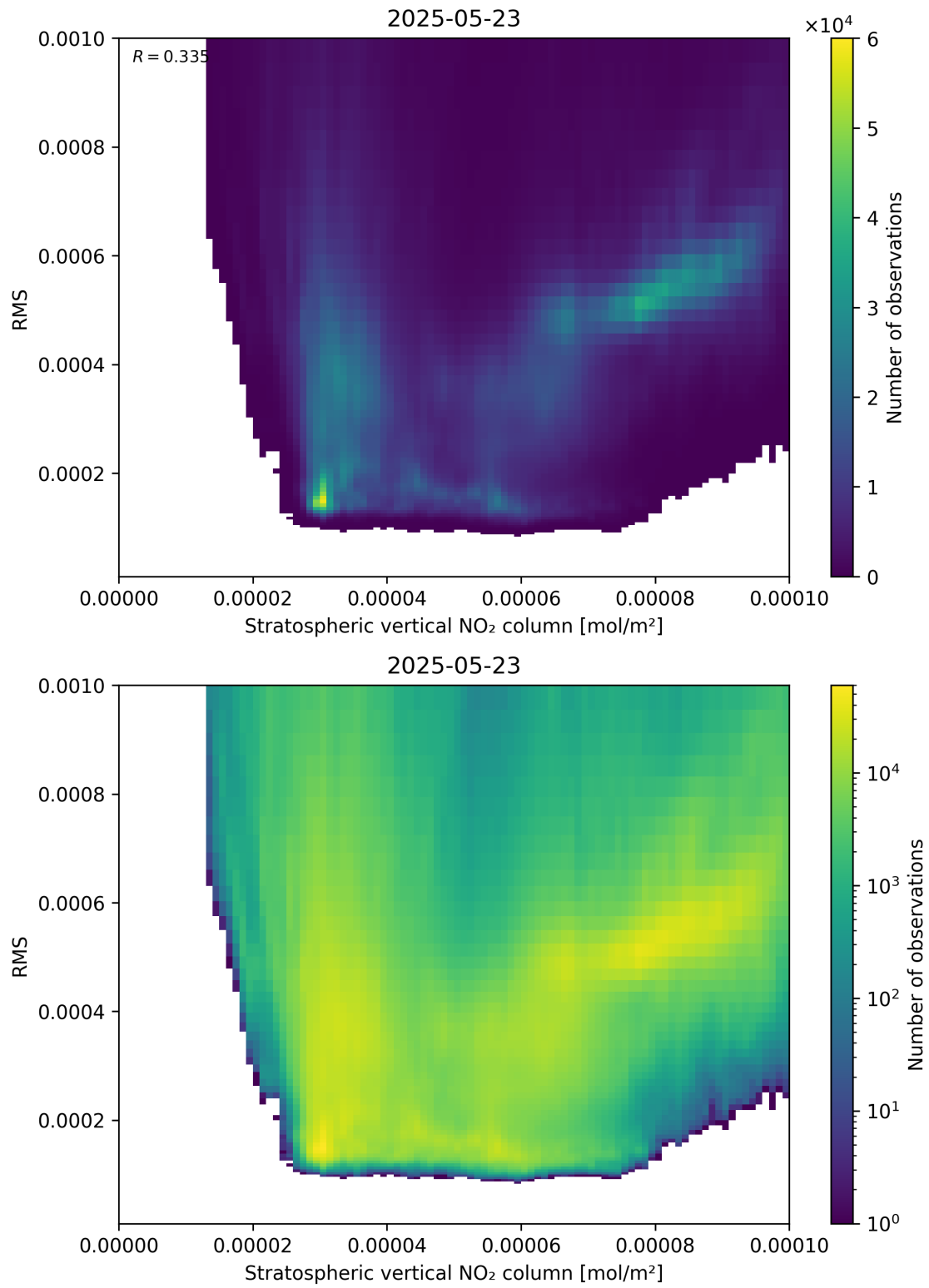
Figure 102: Scatter density plot of “Stratospheric vertical NO 2 column” against “RMS” for 2025-05-22 to 2025-05-24.
