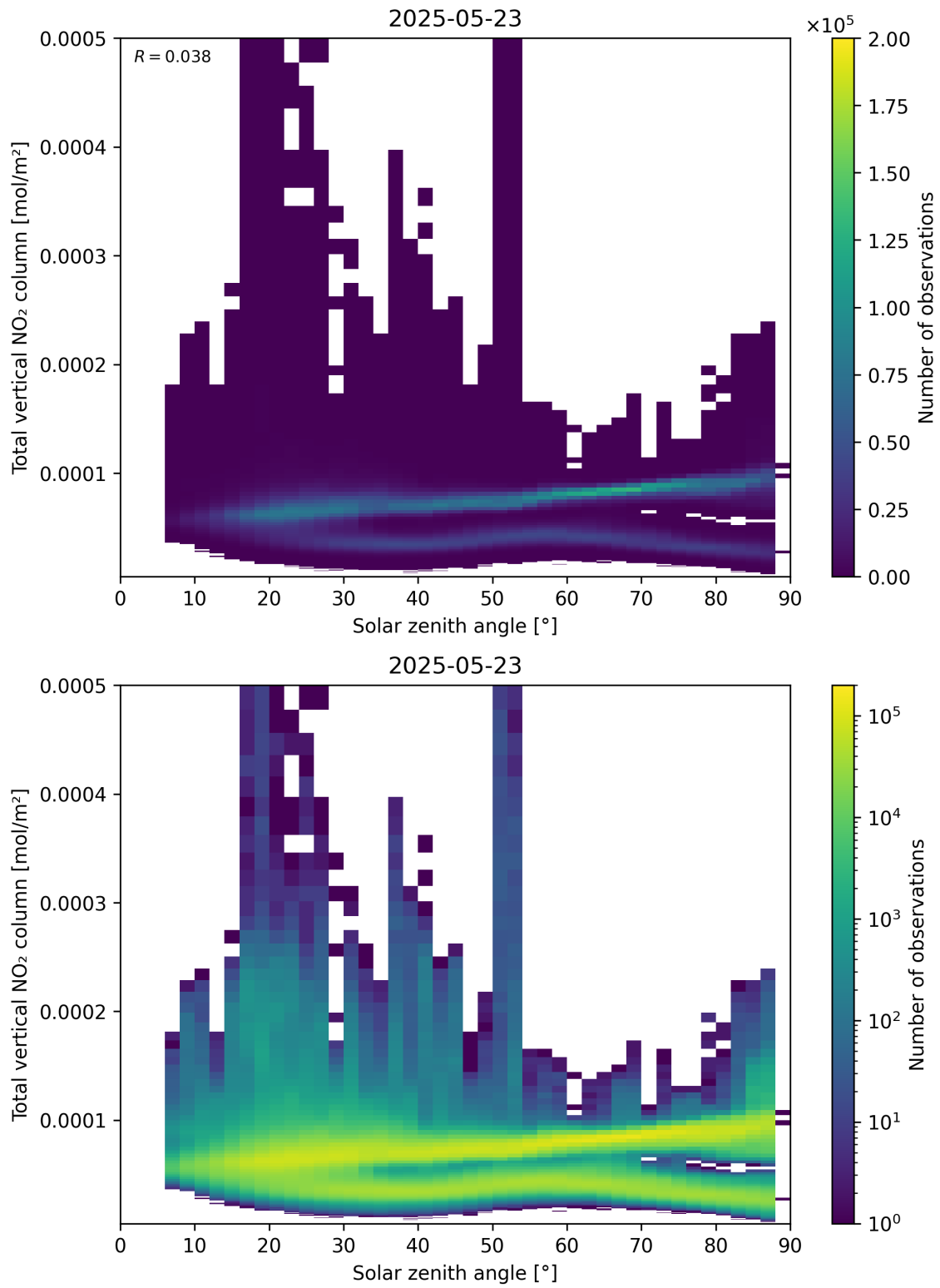
Figure 153: Scatter density plot of “Solar zenith angle” against “Total vertical NO 2 column” for 2025-05-22 to 2025-05-24.
