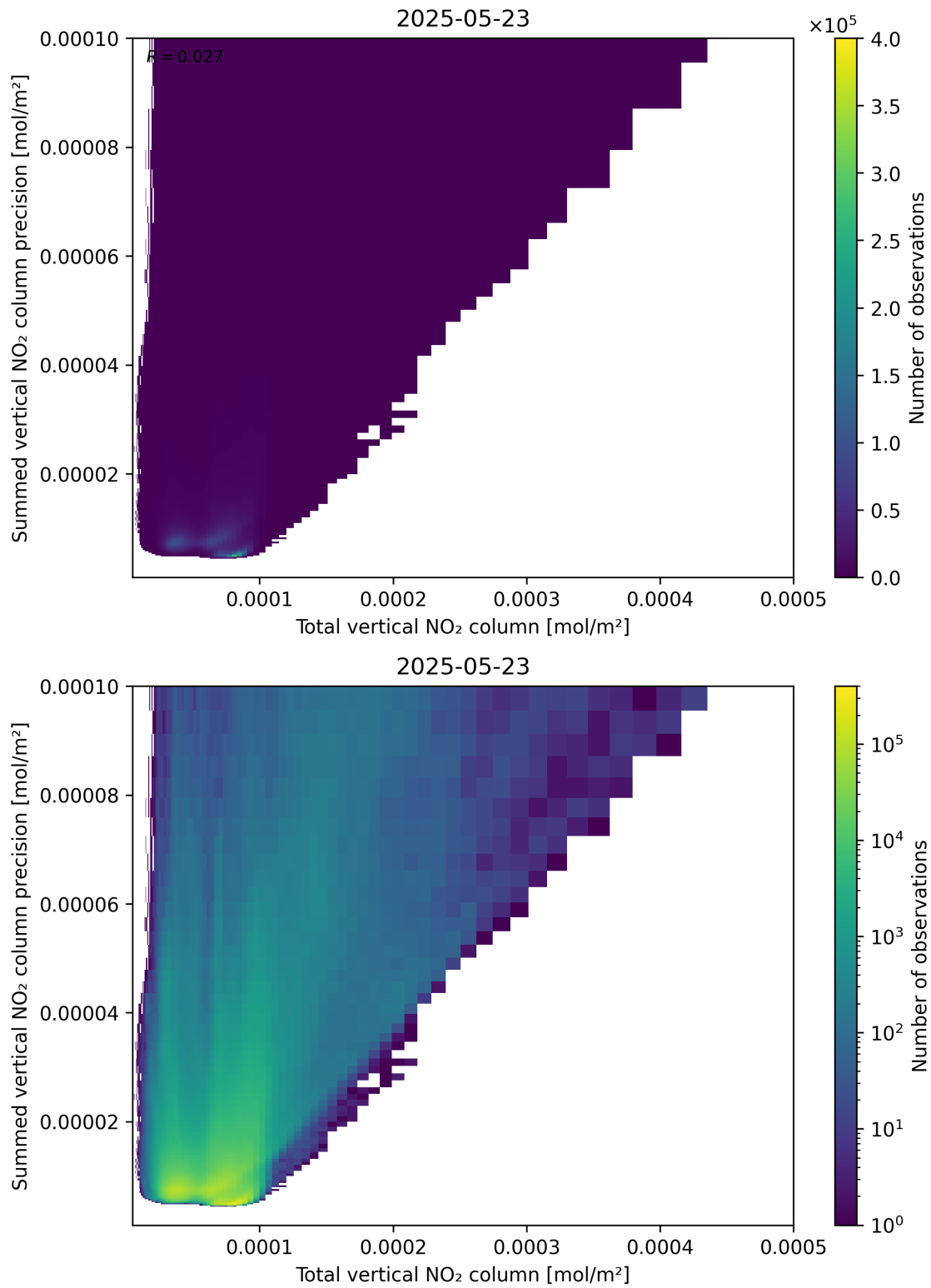
Figure 113: Scatter density plot of “Total vertical NO 2 column” against “Summed vertical NO 2 column precision” for 2025-05-22 to 2025-05-24.
