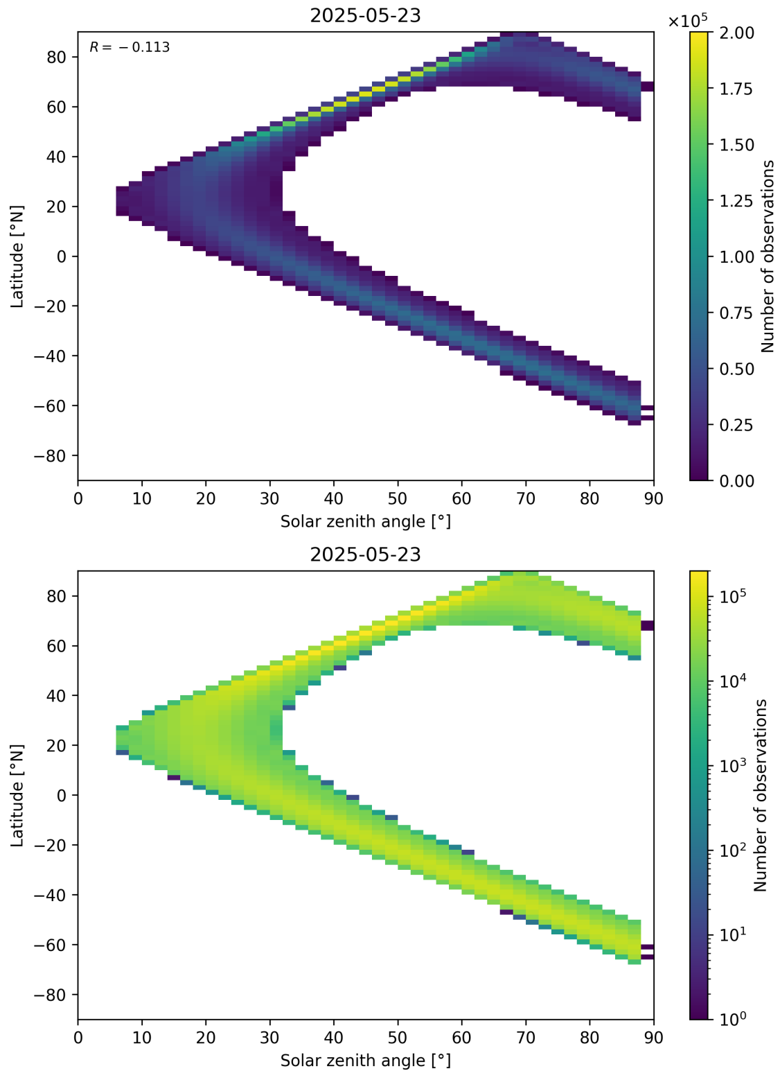
Figure 149: Scatter density plot of “Solar zenith angle” against “Latitude” for 2025-05-22 to 2025-05-24.
