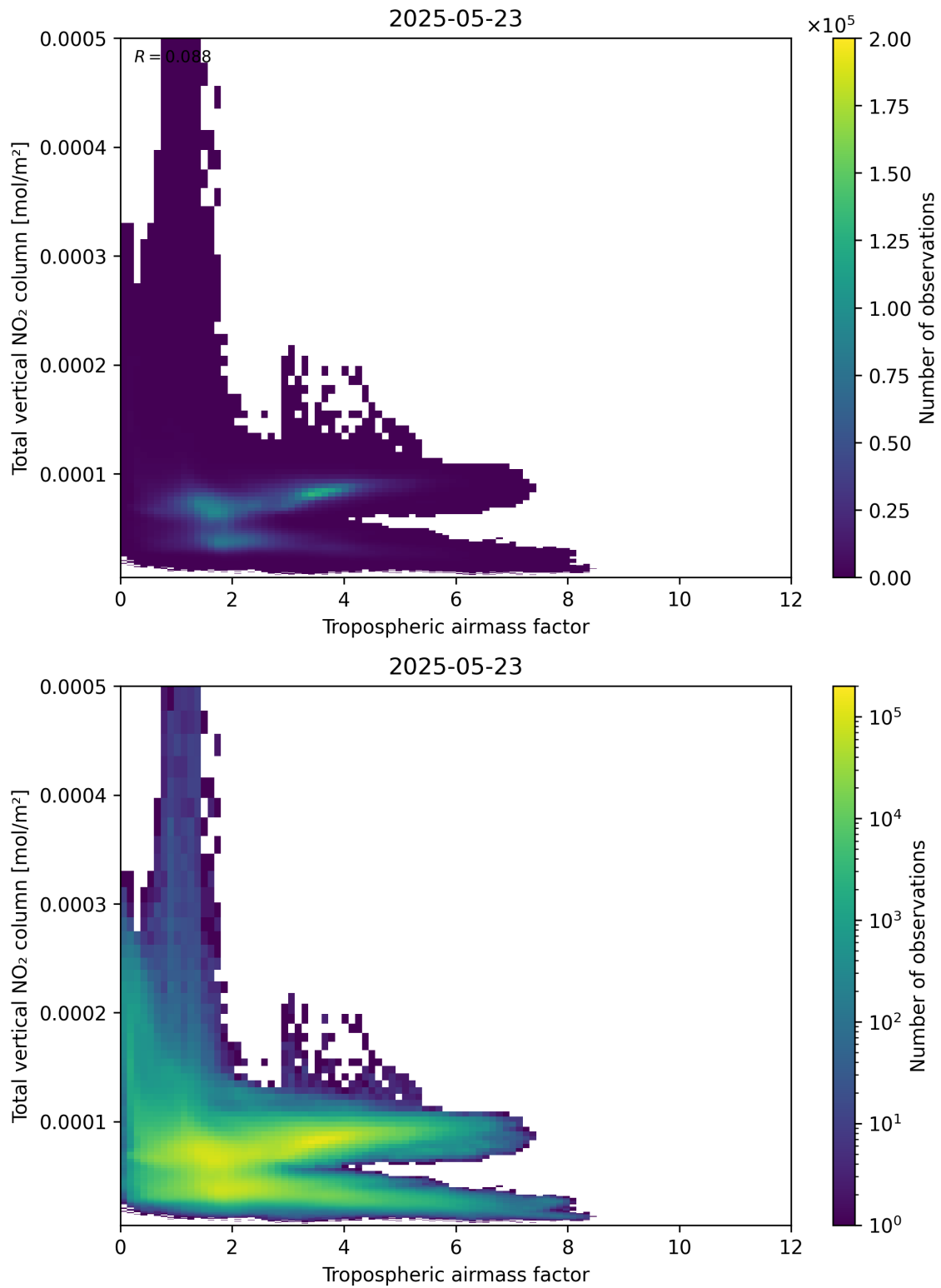
Figure 77: Scatter density plot of “Tropospheric airmass factor” against “Total vertical NO 2 column” for 2025-05-22 to 2025-05-24.
