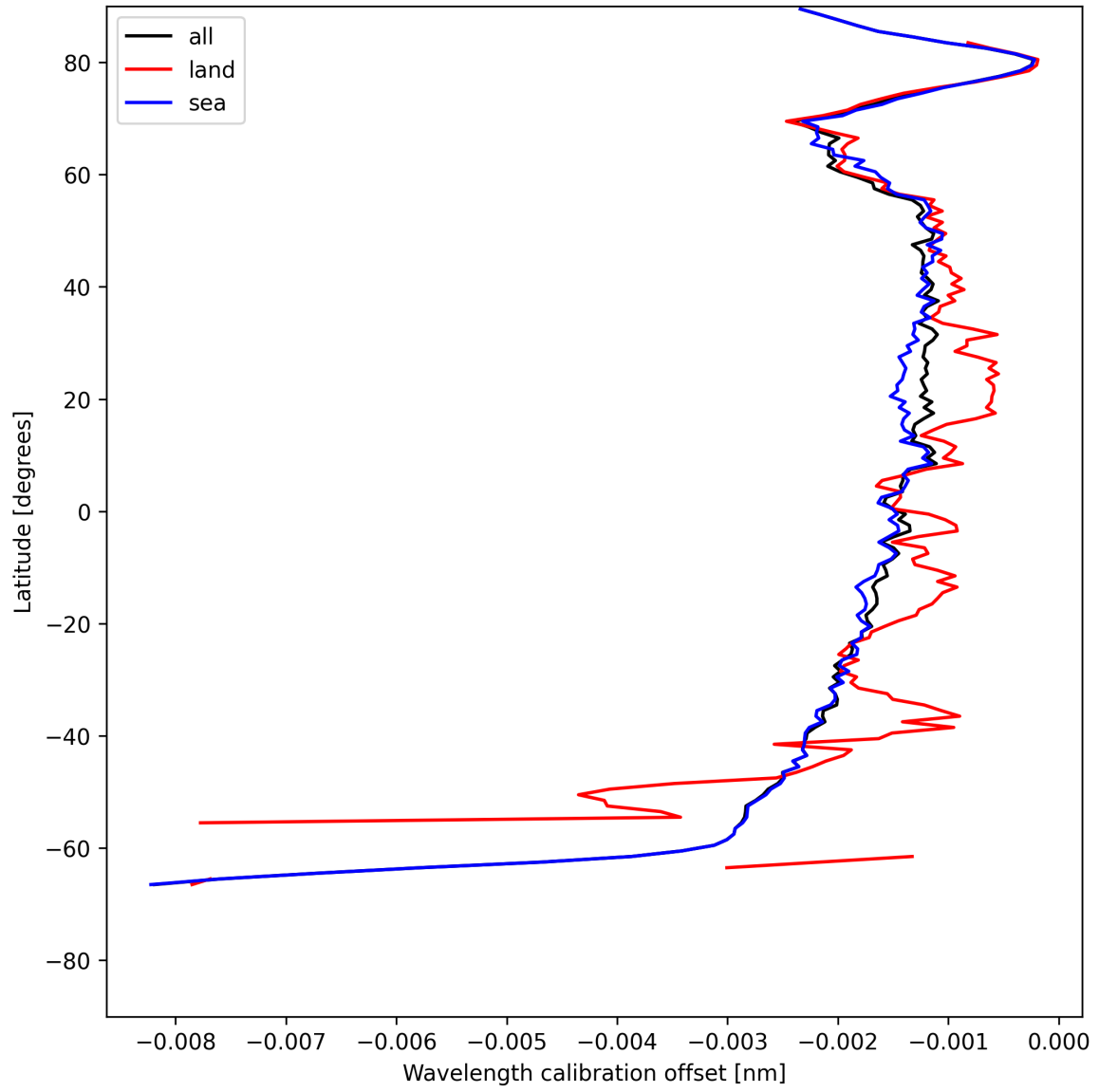
Figure 18: Zonal average of “Wavelength calibration offset” for 2025-05-22 to 2025-05-24.
