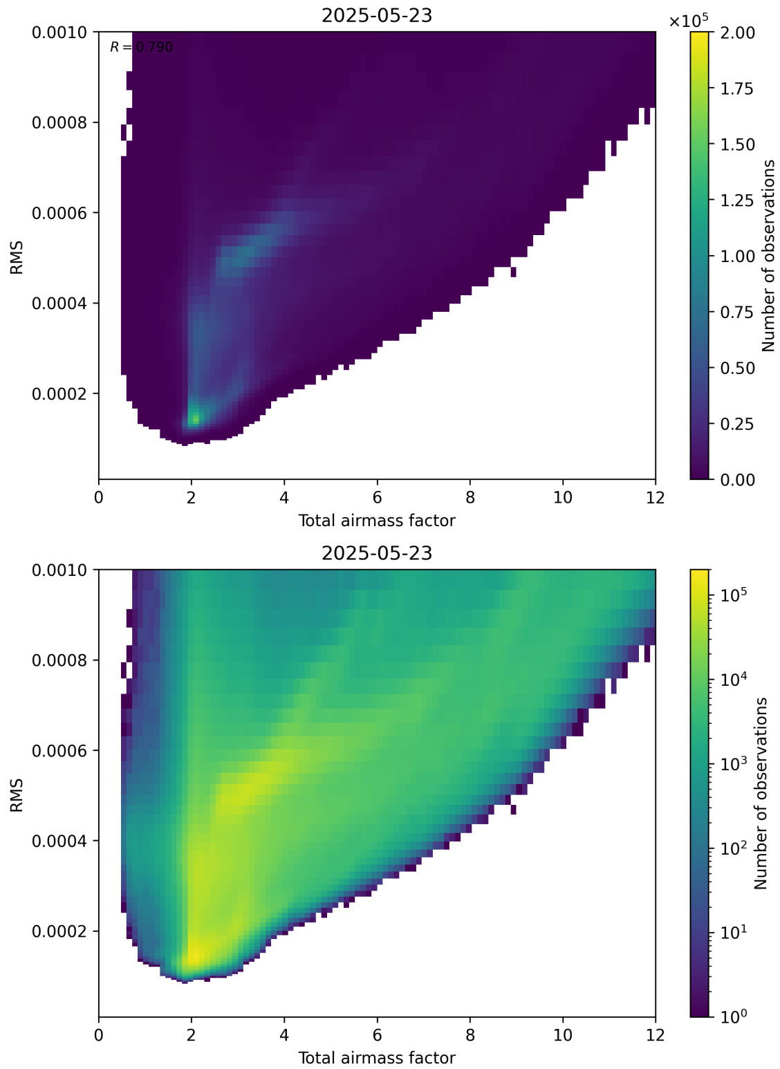
Figure 69: Scatter density plot of “Total airmass factor” against “RMS” for 2025-05-22 to 2025-05-24.
