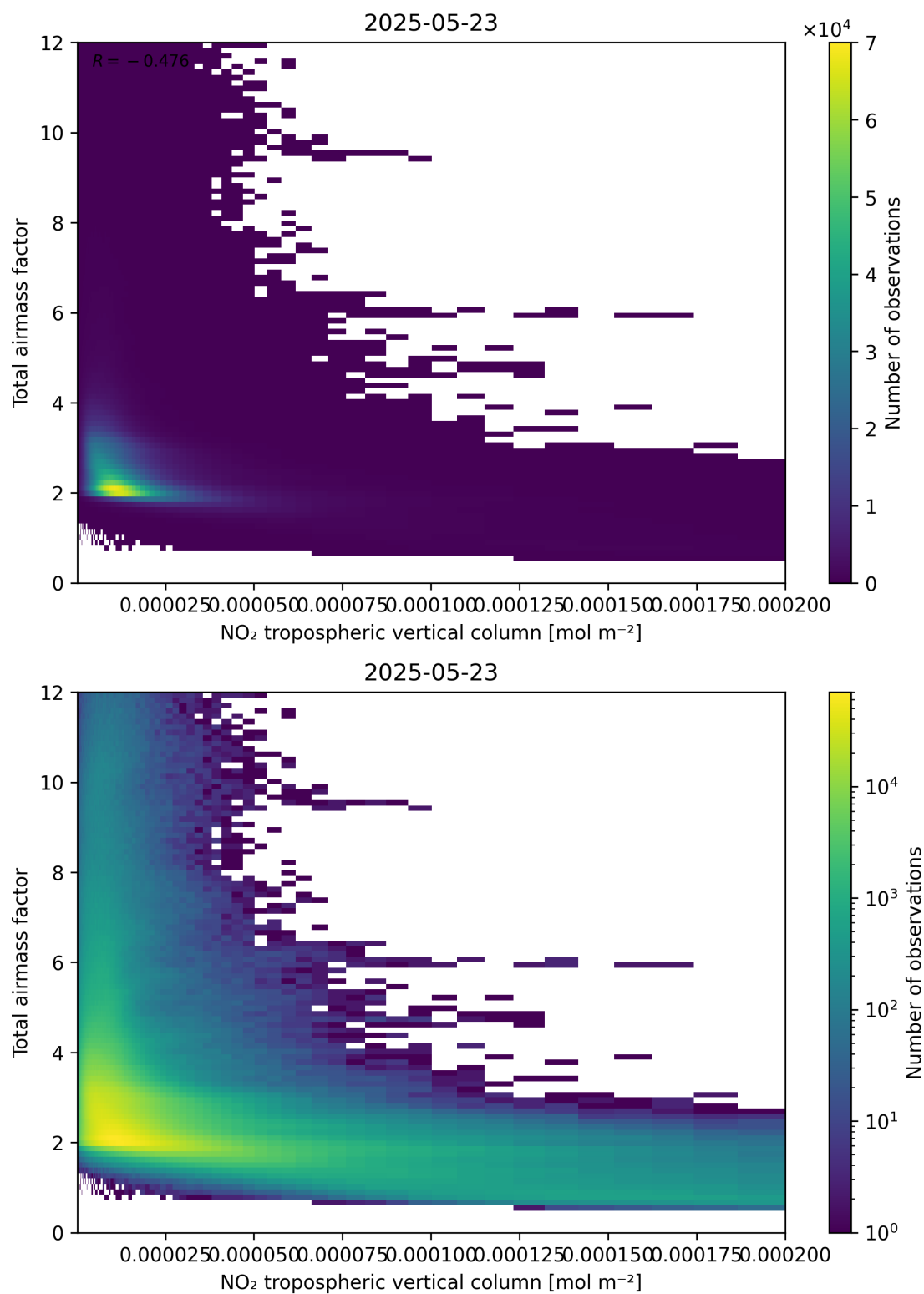
Figure 122: Scatter density plot of “NO 2 tropospheric vertical column” against “Total air mass factor” for 2025-05-22 to 2025-05-24.
