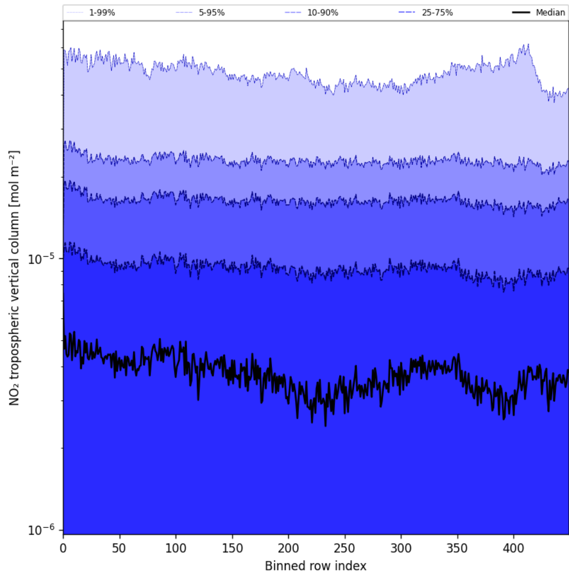
Figure 46: Along track statistics of “NO 2 tropospheric vertical column” for 2025-05-22 to 2025-05-24
