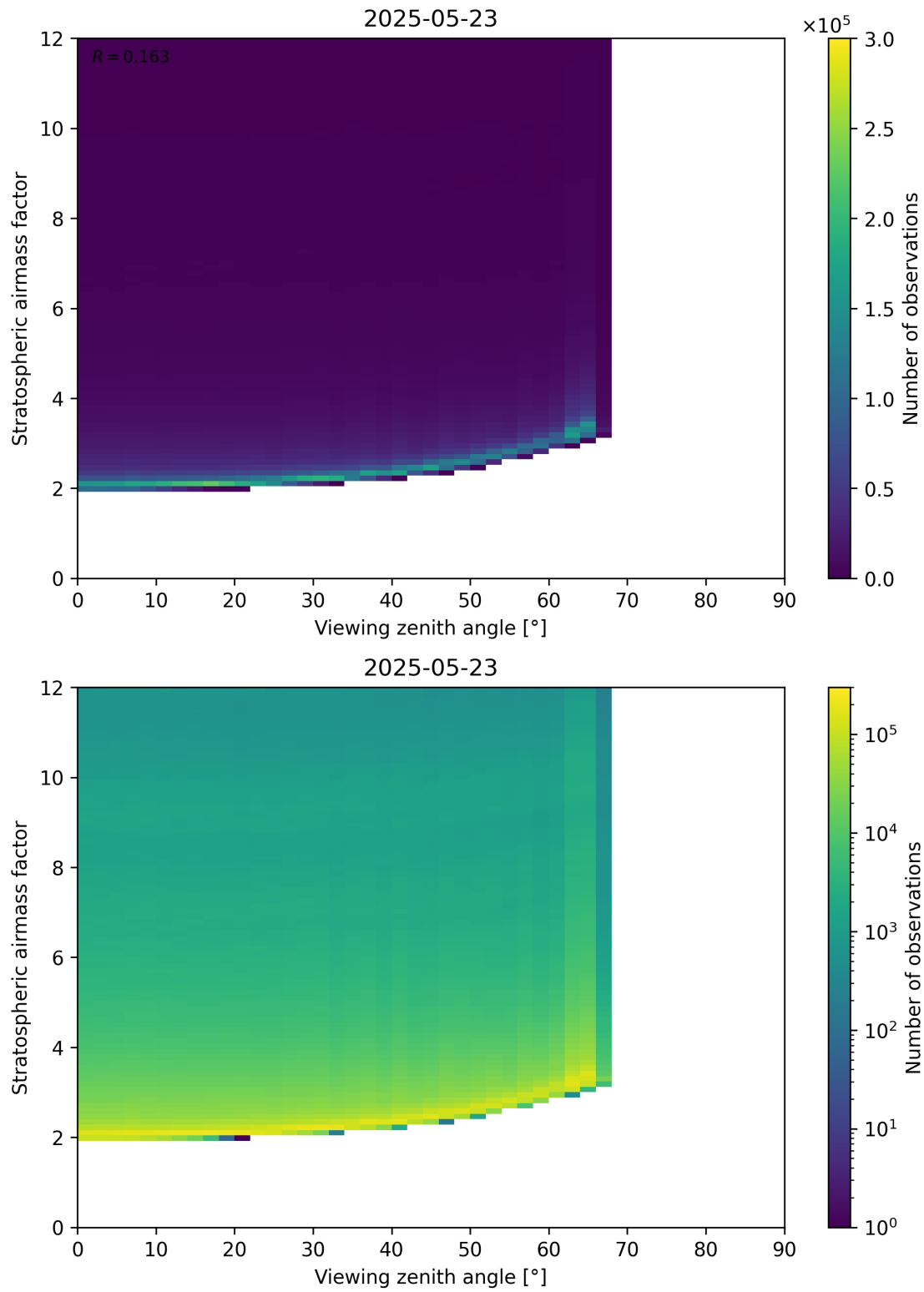
Figure 159: Scatter density plot of “Viewing zenith angle” against “Stratospheric airmass factor” for 2025-05-22 to 2025-05-24.
