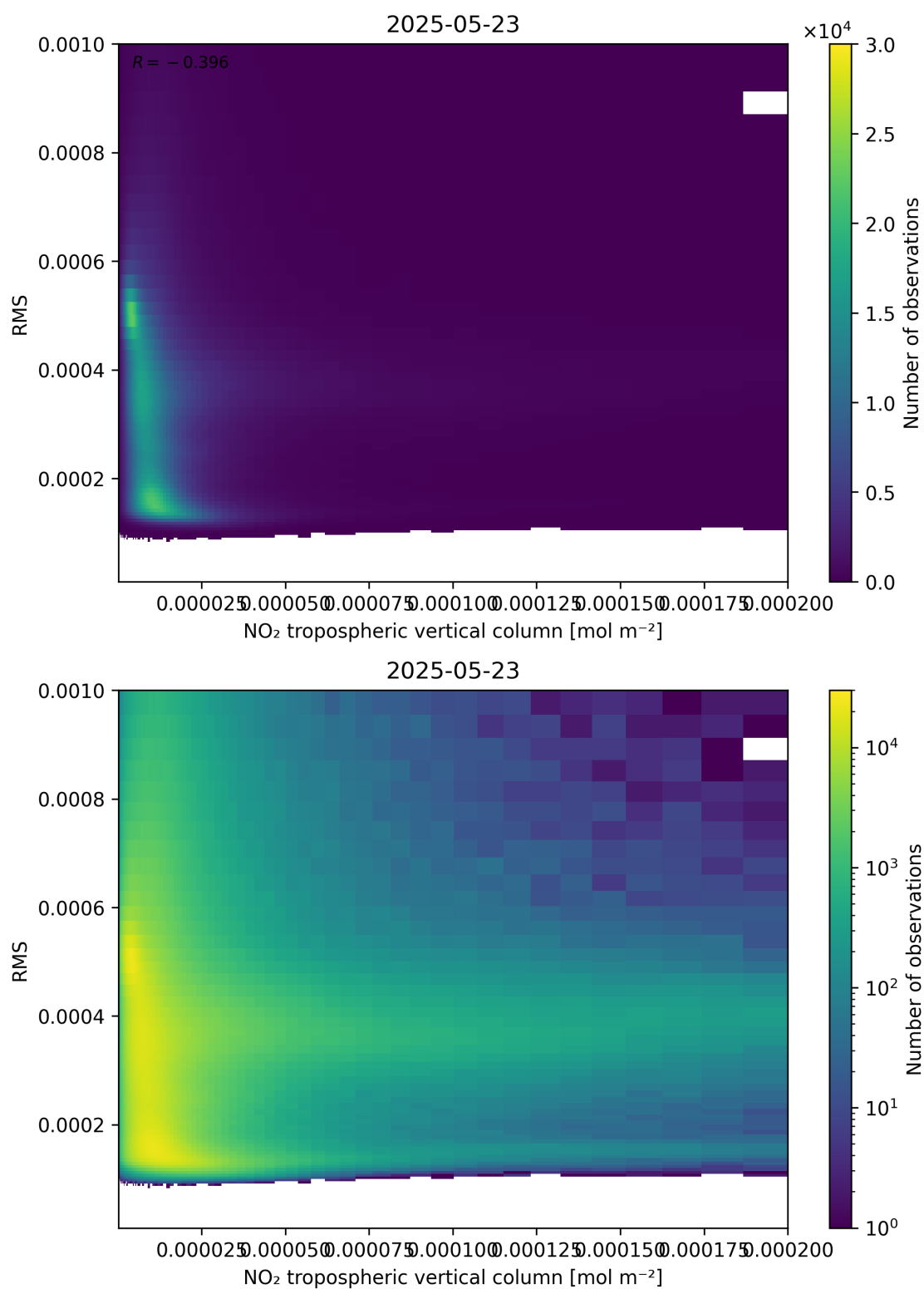
Figure 142: Scatter density plot of “NO 2 tropospheric vertical column” against “RMS” for 2025-05-22 to 2025-05-24.
