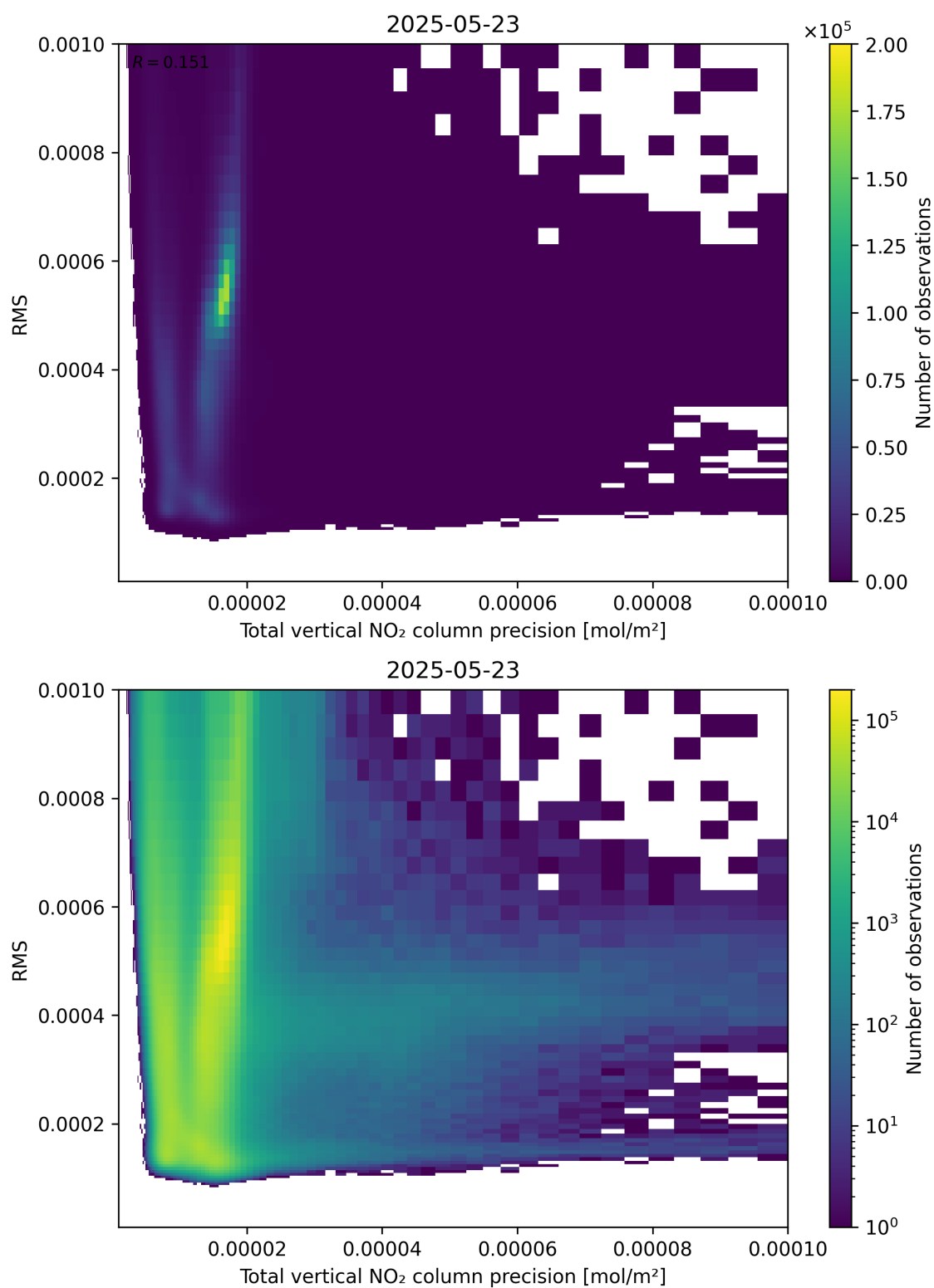
Figure 119: Scatter density plot of “Total vertical NO 2 column precision” against “RMS” for 2025-05-22 to 2025-05-24.
