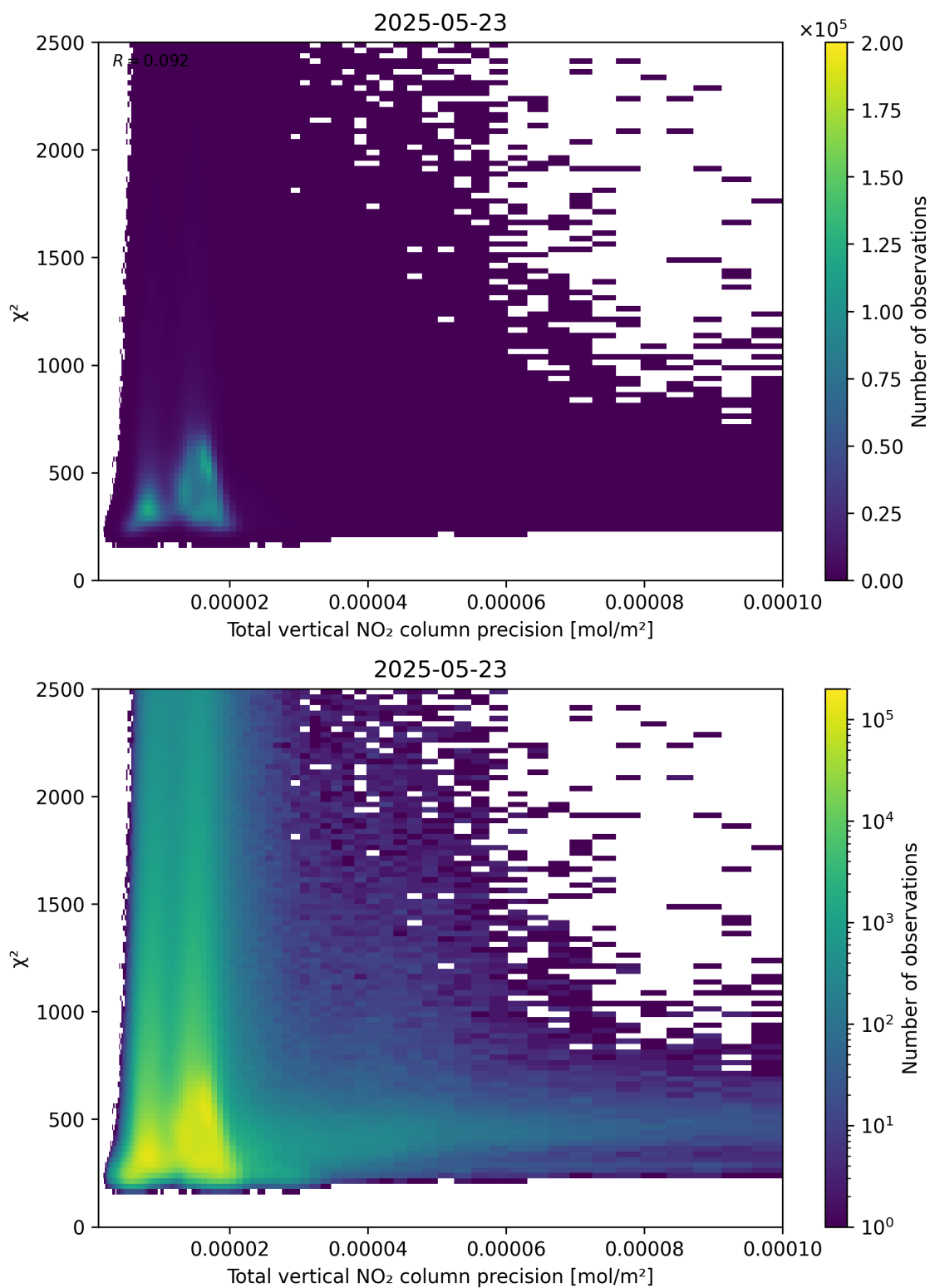
Figure 116: Scatter density plot of “Total vertical NO 2 column precision” against “ \chi^2 ” for 2025-05-22 to 2025-05-24.
