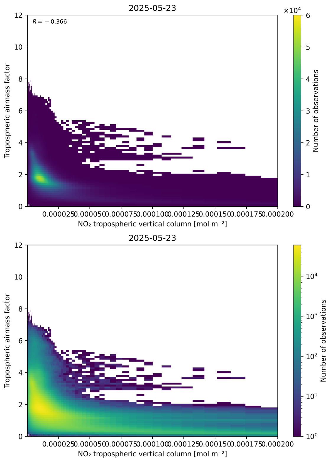
Figure 123: Scatter density plot of “NO 2 tropospheric vertical column” against “Tropospheric air mass factor” for 2025-05-22 to 2025-05-24.
