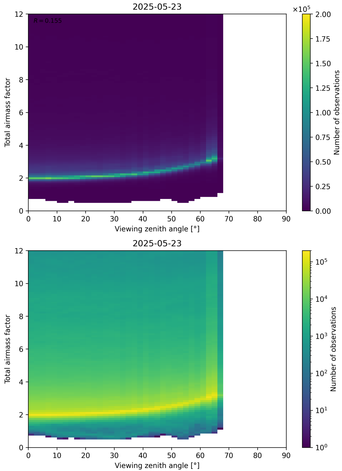
Figure 160: Scatter density plot of “Viewing zenith angle” against “Total airmass factor” for 2025-05-22 to 2025-05-24.
