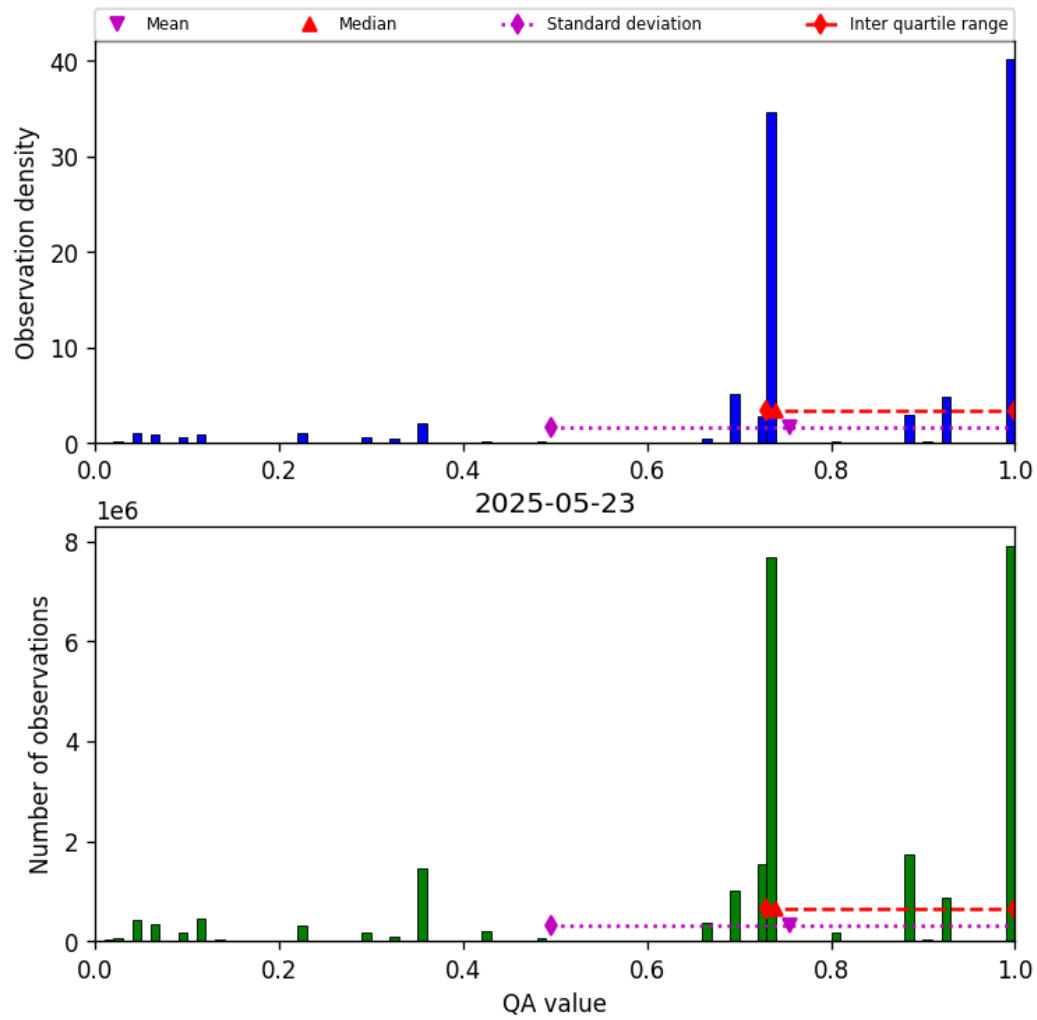
Figure 28: Histogram of “QA value” for 2025-05-22 to 2025-05-24
