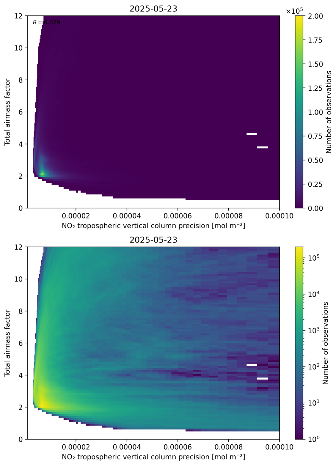
Figure 132: Scatter density plot of “NO 2 tropospheric vertical column precision” against “Total air mass factor” for 2025-05-22 to 2025-05-24.
