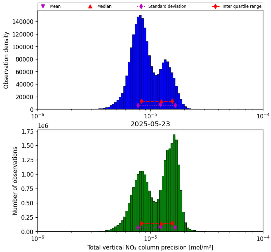
Figure 39: Histogram of “Total vertical NO 2 column precision” for 2025-05-22 to 2025-05-24
