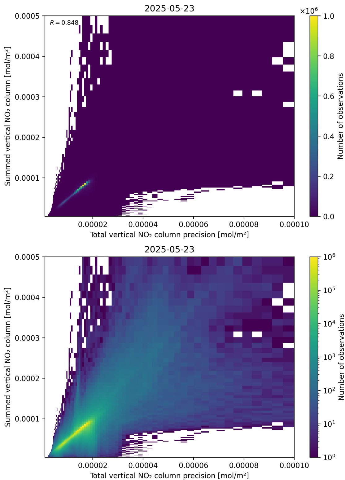
Figure 117: Scatter density plot of “Total vertical NO 2 column precision” against “Summed vertical NO 2 column” for 2025-05-22 to 2025-05-24.
