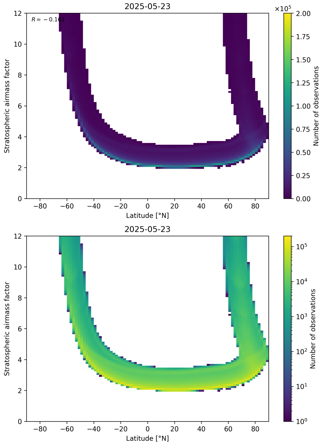
Figure 83: Scatter density plot of “Latitude” against “Stratospheric air mass factor” for 2025-05-22 to 2025-05-24.
