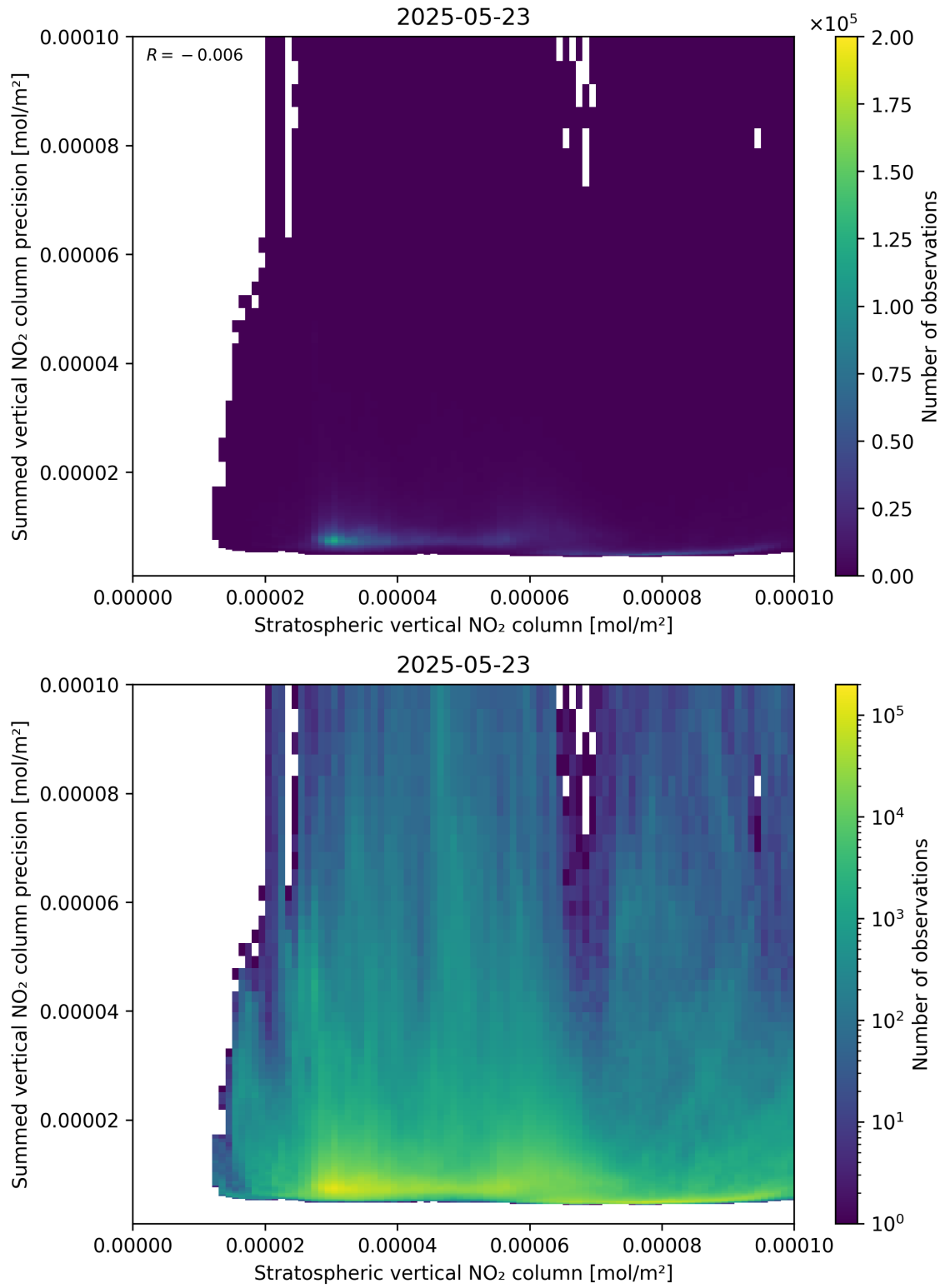
Figure 99: Scatter density plot of “Stratospheric vertical NO 2 column” against “Summed vertical NO 2 column precision” for 2025-05-22 to 2025-05-24.
