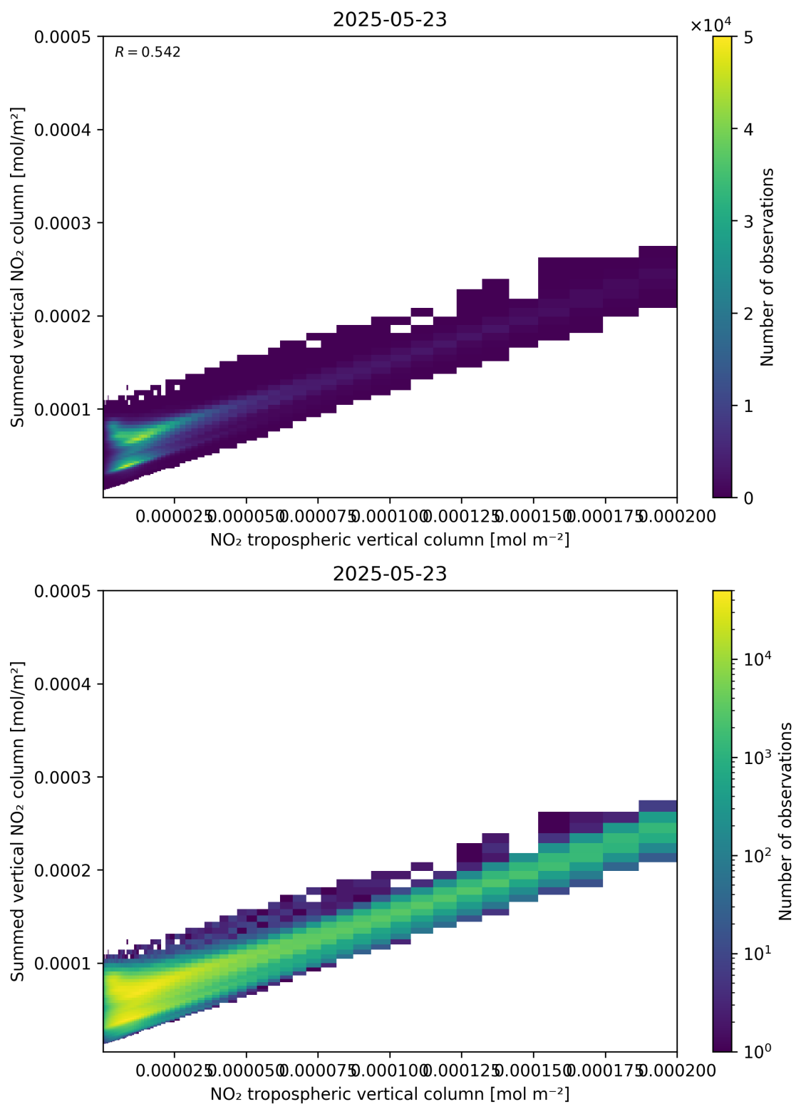
Figure 126: Scatter density plot of “NO 2 tropospheric vertical column” against “Summed vertical NO 2 column” for 2025-05-22 to 2025-05-24.
