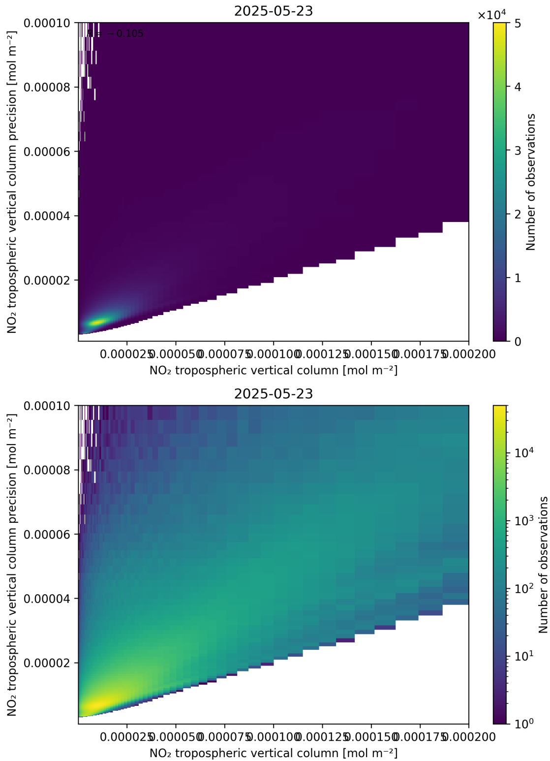
Figure 130: Scatter density plot of “NO 2 tropospheric vertical column” against “NO 2 tropospheric vertical column precision” for 2025-05-22 to 2025-05-24.
