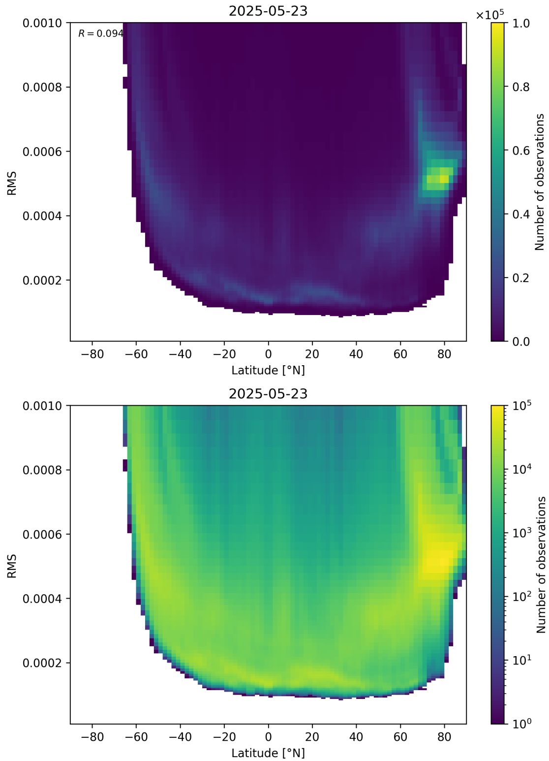
Figure 94: Scatter density plot of “Latitude” against “RMS” for 2025-05-22 to 2025-05-24.
