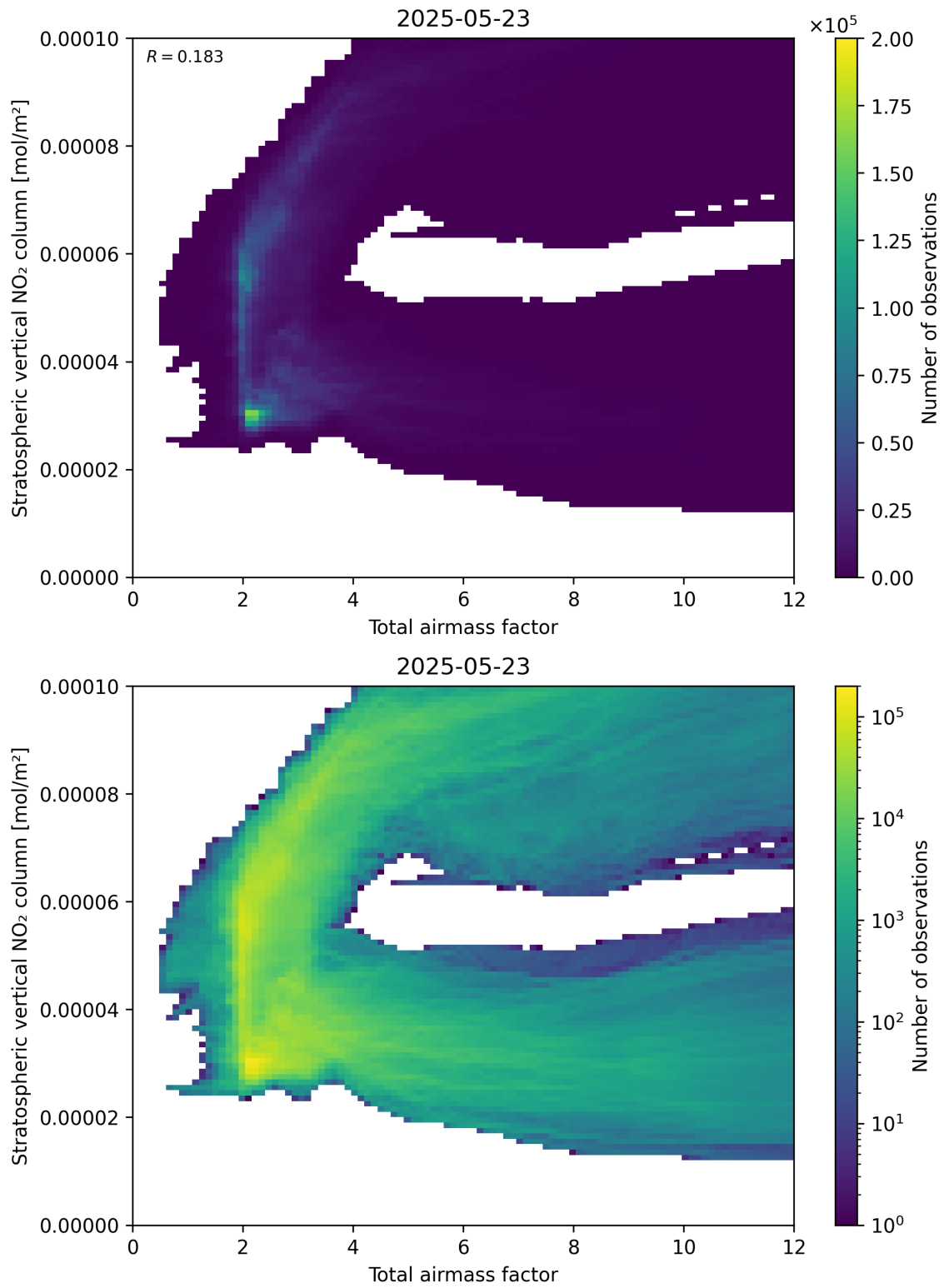
Figure 64: Scatter density plot of “Total airmass factor” against “Stratospheric vertical NO 2 column” for 2025-05-22 to 2025-05-24.
