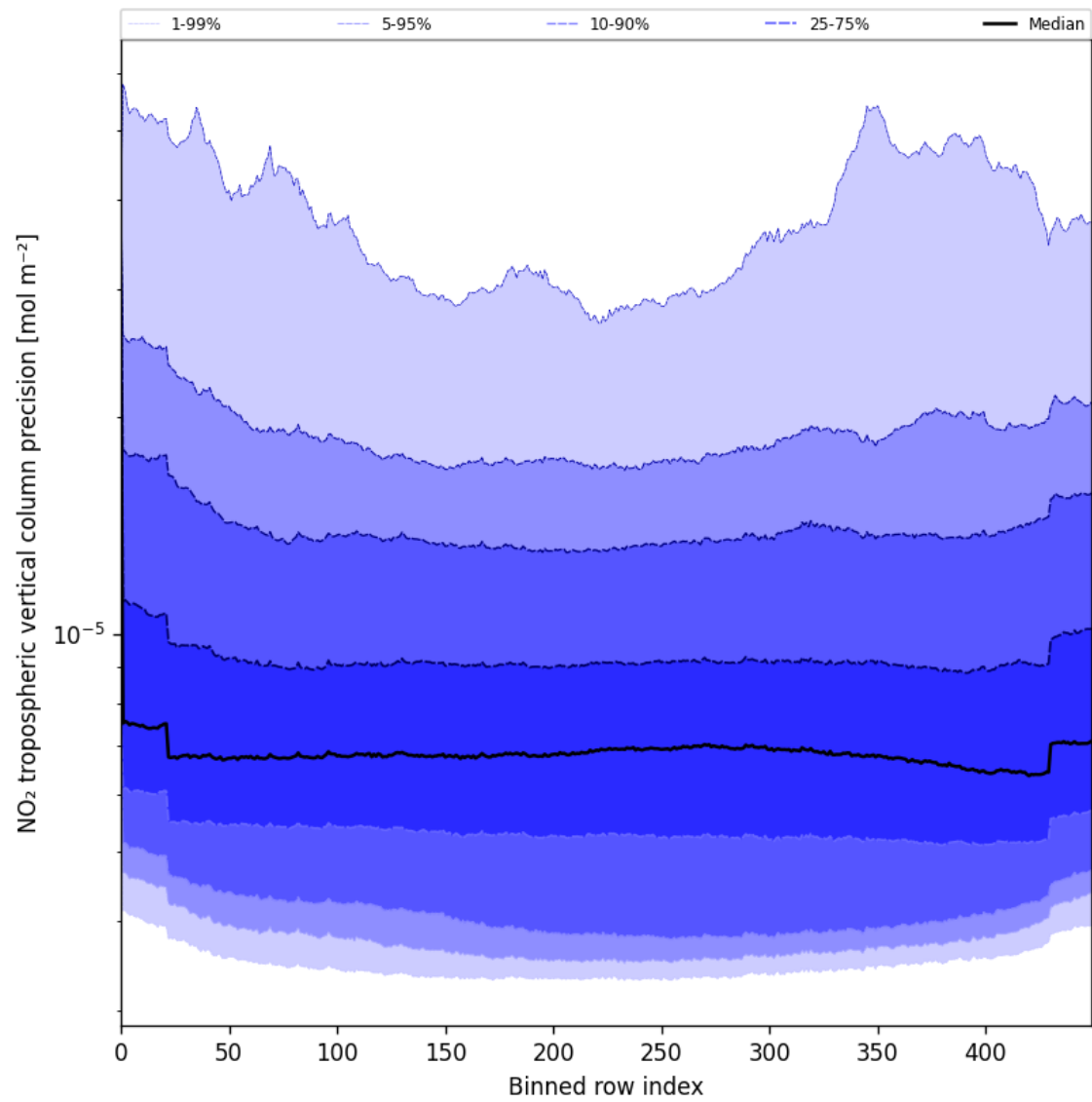
Figure 47: Along track statistics of “NO 2 tropospheric vertical column precision” for 2025-05-23 to 2025-05-25
