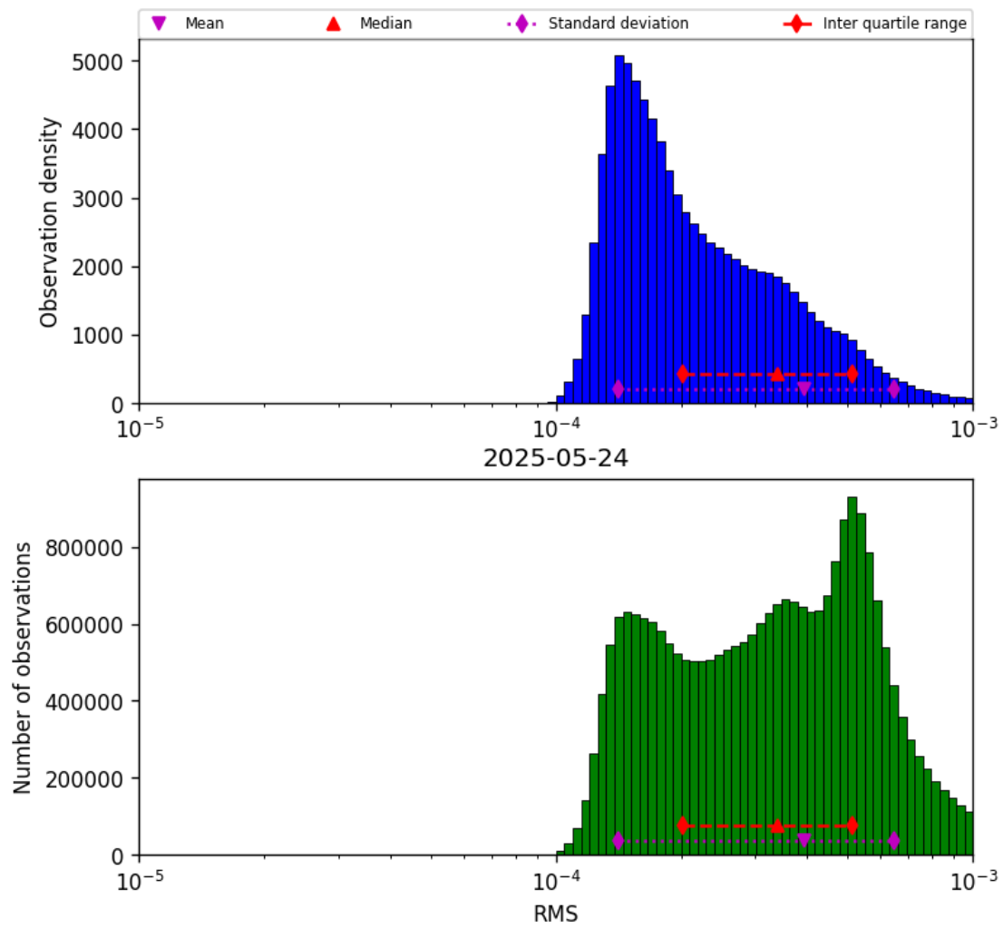
Figure 43: Histogram of “RMS” for 2025-05-23 to 2025-05-25
