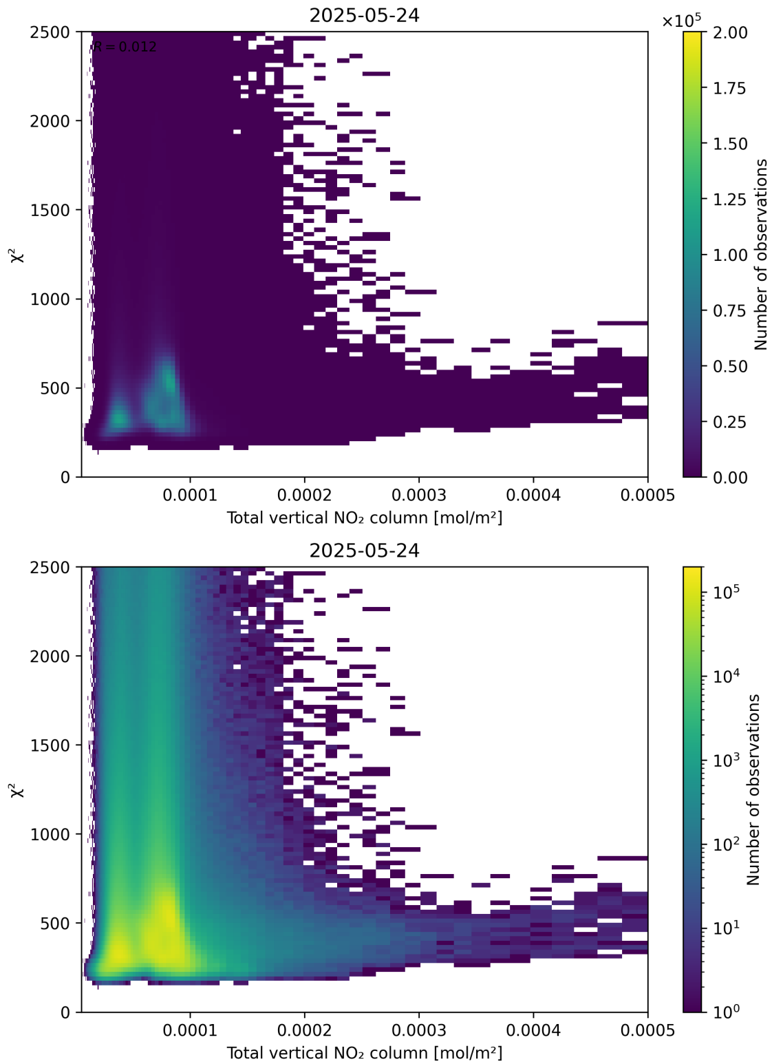
Figure 111: Scatter density plot of “Total vertical NO 2 column” against “ \chi^2 ” for 2025-05-23 to 2025-05-25.
