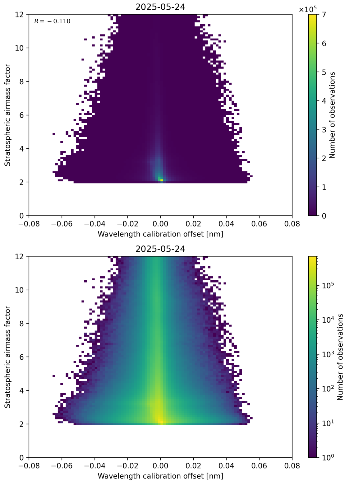
Figure 174: Scatter density plot of “Wavelength calibration offset” against “Stratospheric airmass factor” for 2025-05-23 to 2025-05-25.
