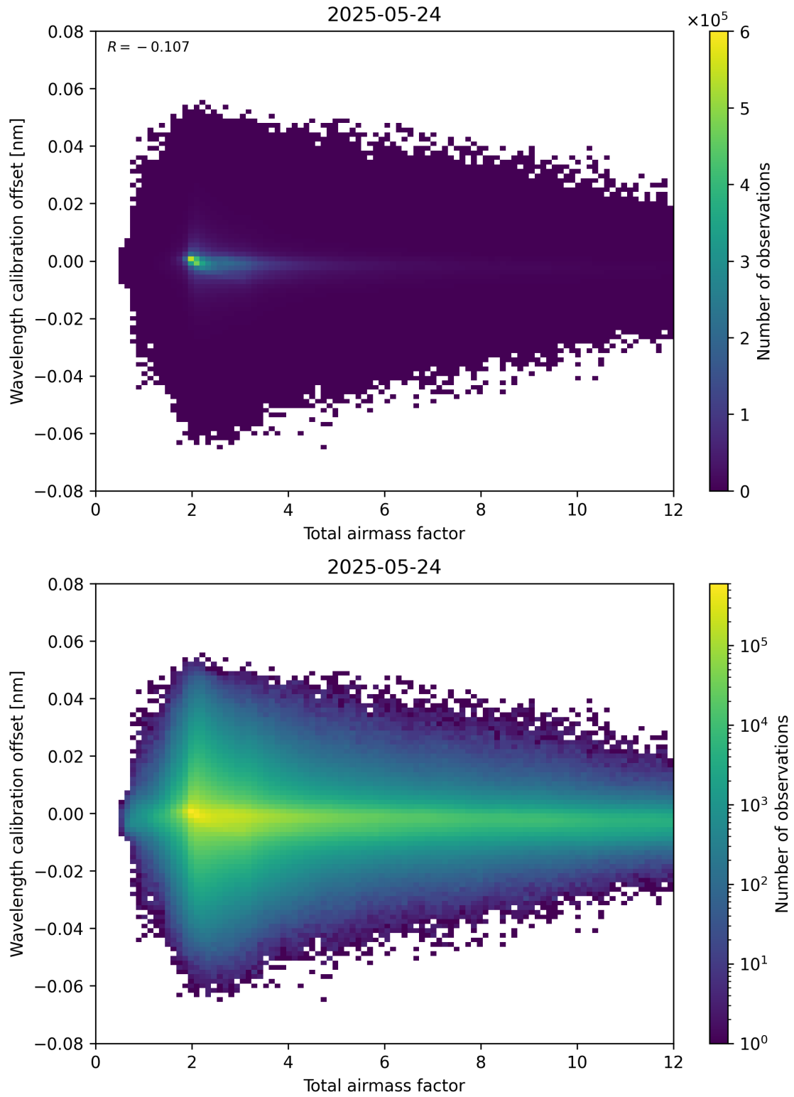
Figure 70: Scatter density plot of “Total airmass factor” against “Wavelength calibration offset” for 2025-05-23 to 2025-05-25.
