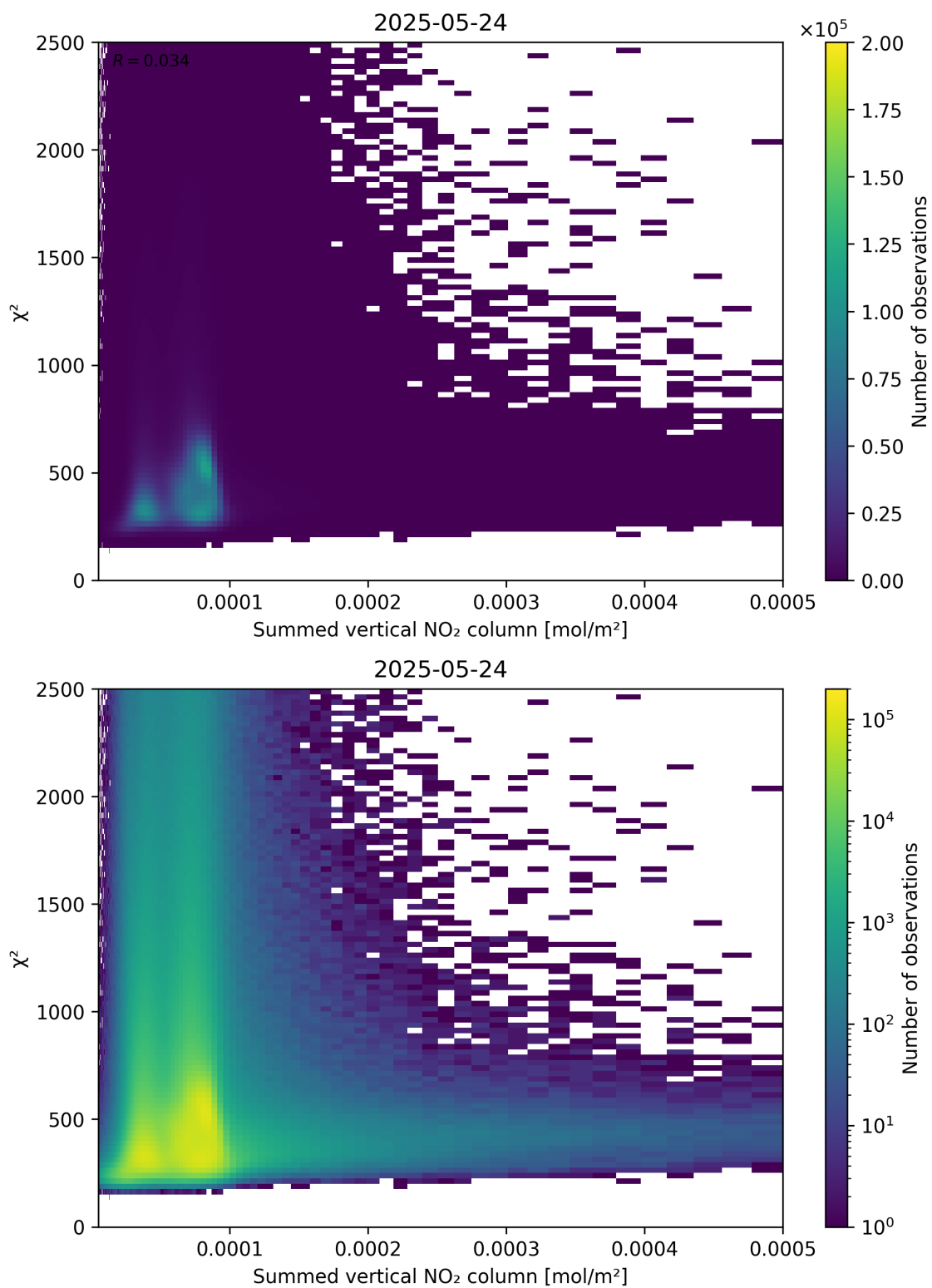
Figure 104: Scatter density plot of “Summed vertical NO 2 column” against “ \chi^2 ” for 2025-05-23 to 2025-05-25.
