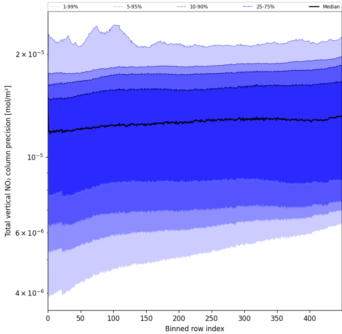
Figure 56: Along track statistics of “Total vertical NO 2 column precision” for 2025-05-23 to 2025-05-25
