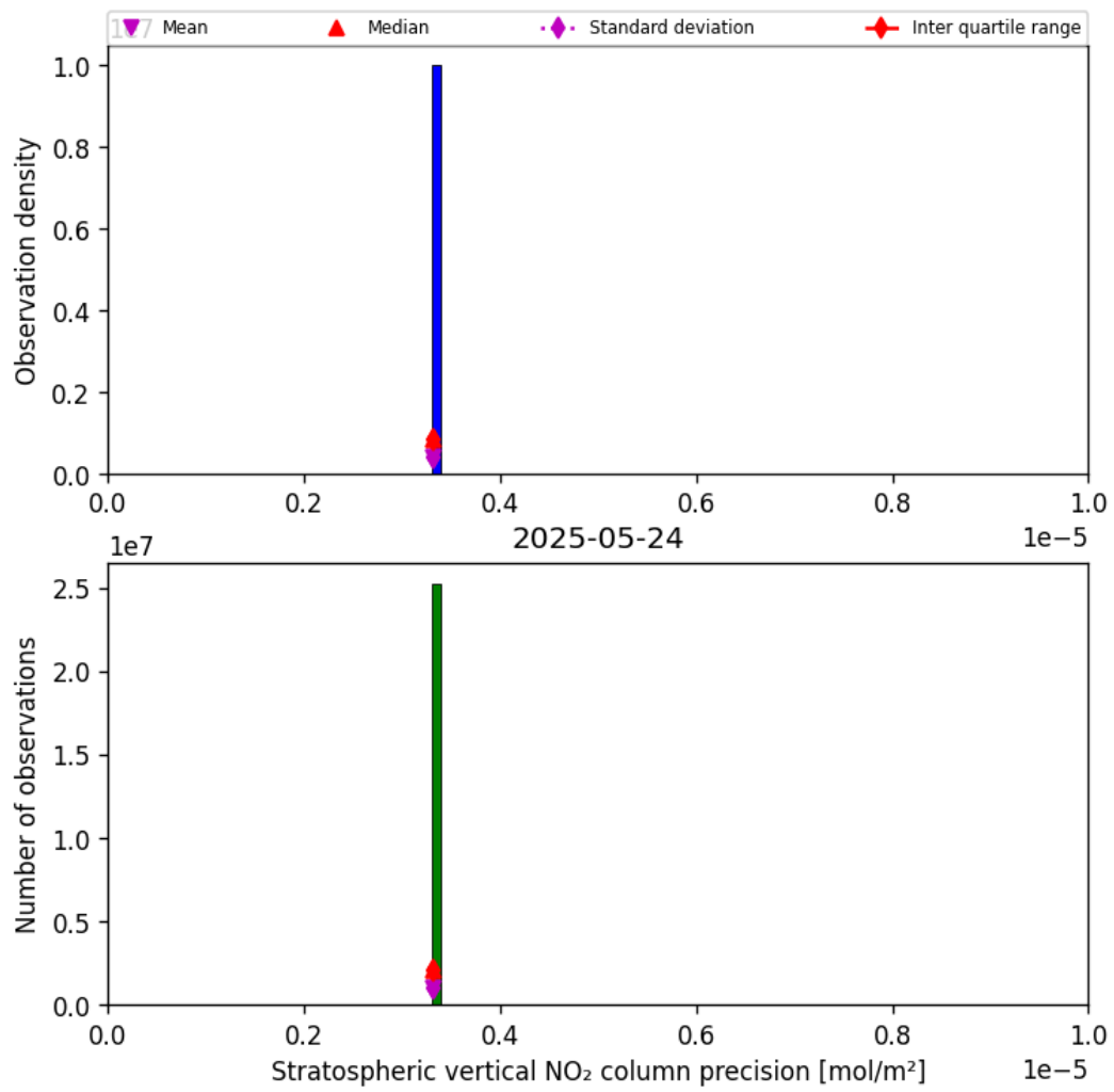
Figure 37: Histogram of “Stratospheric vertical NO 2 column precision” for 2025-05-23 to 2025-05-25
