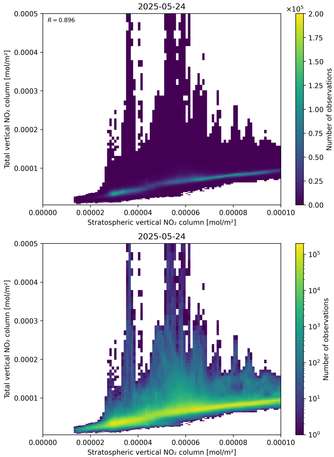
Figure 100: Scatter density plot of “Stratospheric vertical NO 2 column” against “Total vertical NO 2 column” for 2025-05-23 to 2025-05-25.
