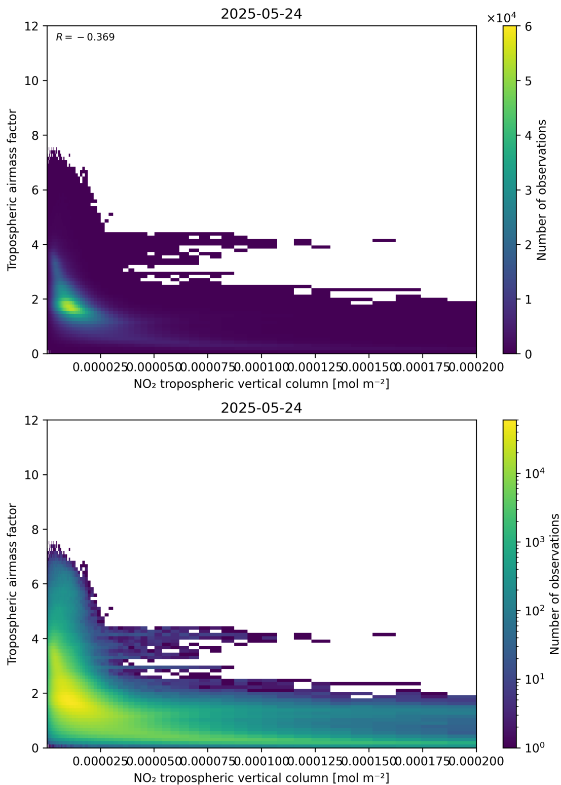
Figure 123: Scatter density plot of “NO 2 tropospheric vertical column” against “Tropospheric airmass factor” for 2025-05-23 to 2025-05-25.
