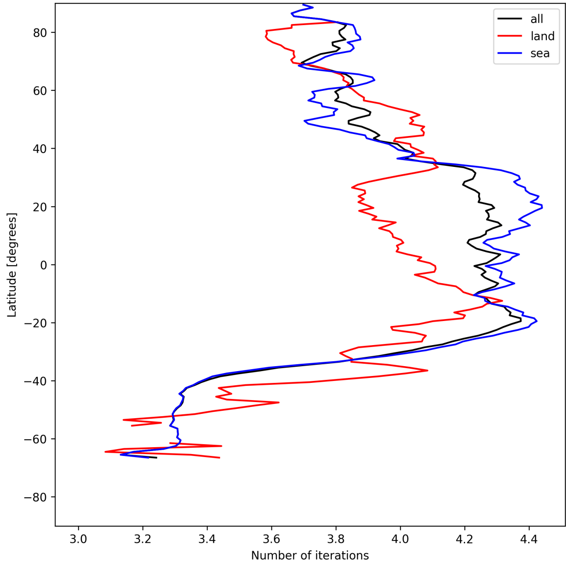
Figure 17: Zonal average of “Number of iterations” for 2025-05-23 to 2025-05-25.
