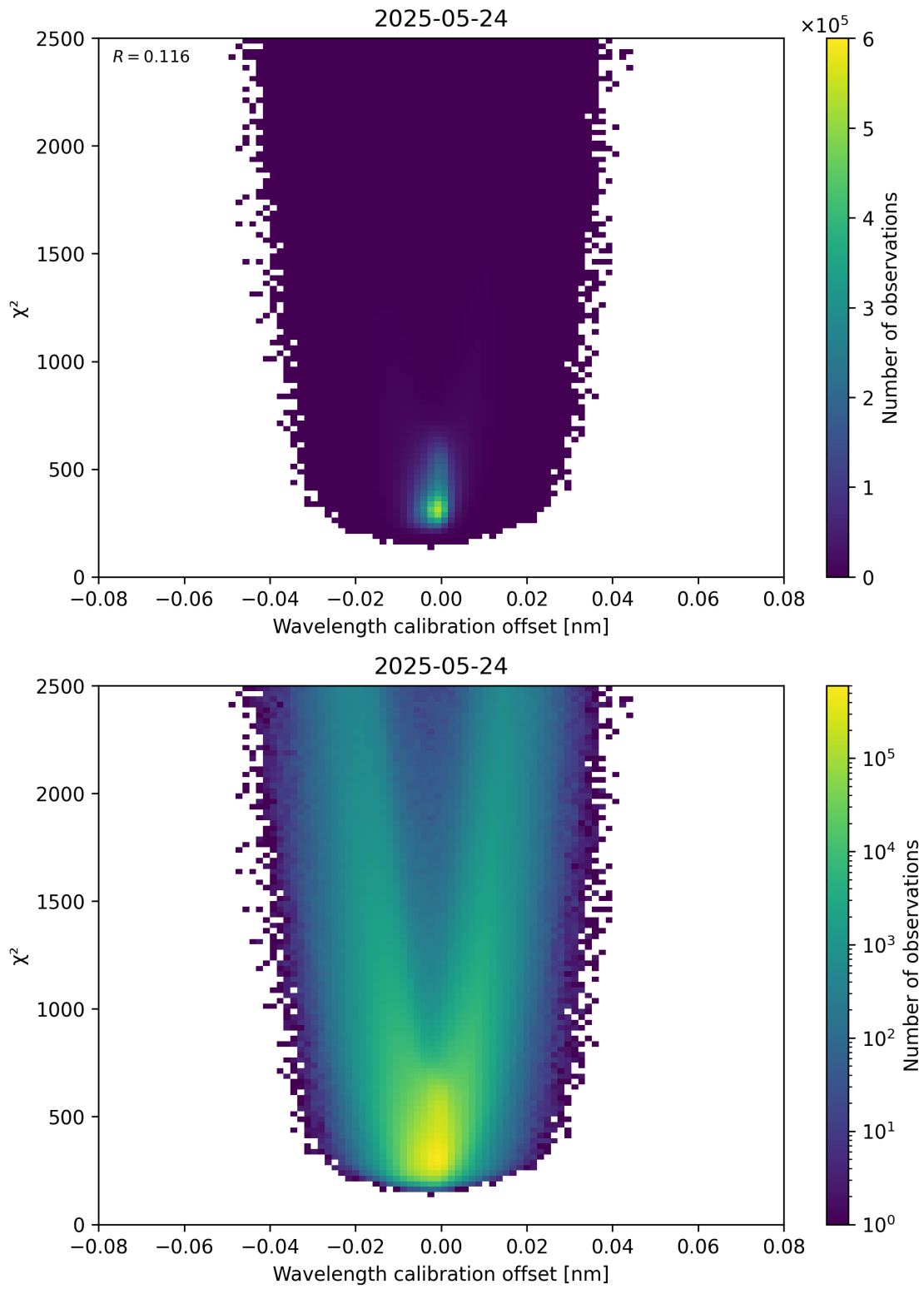
Figure 175: Scatter density plot of “Wavelength calibration offset” against “ \chi^2 ” for 2025-05-23 to 2025-05-25.
