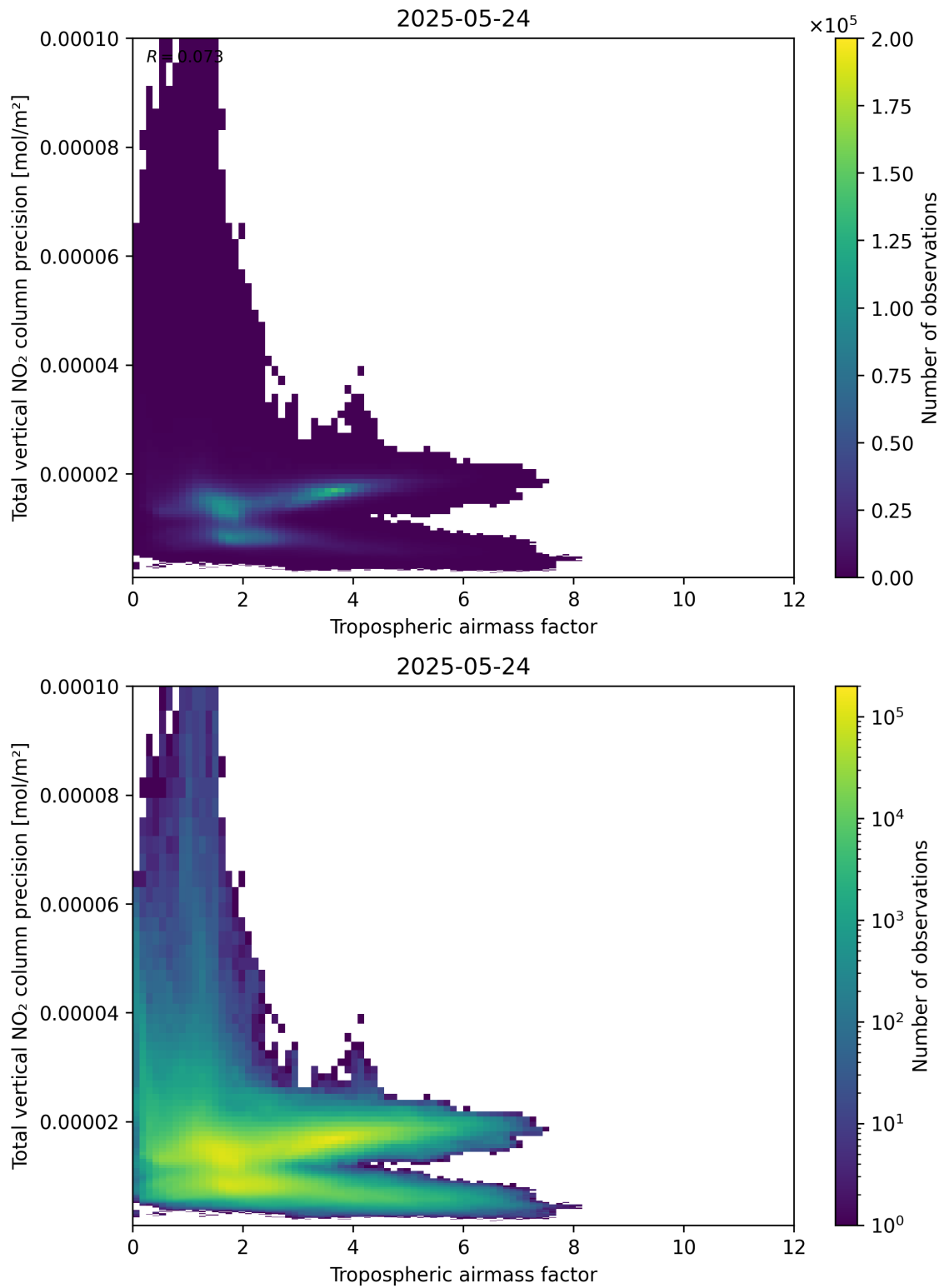
Figure 78: Scatter density plot of “Tropospheric air mass factor” against “Total vertical NO 2 column precision” for 2025-05-23 to 2025-05-25.
