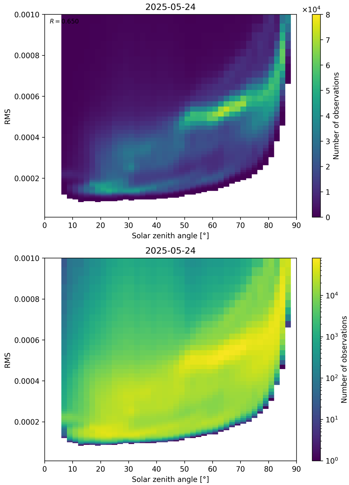
Figure 157: Scatter density plot of “Solar zenith angle” against “RMS” for 2025-05-23 to 2025-05-25.
