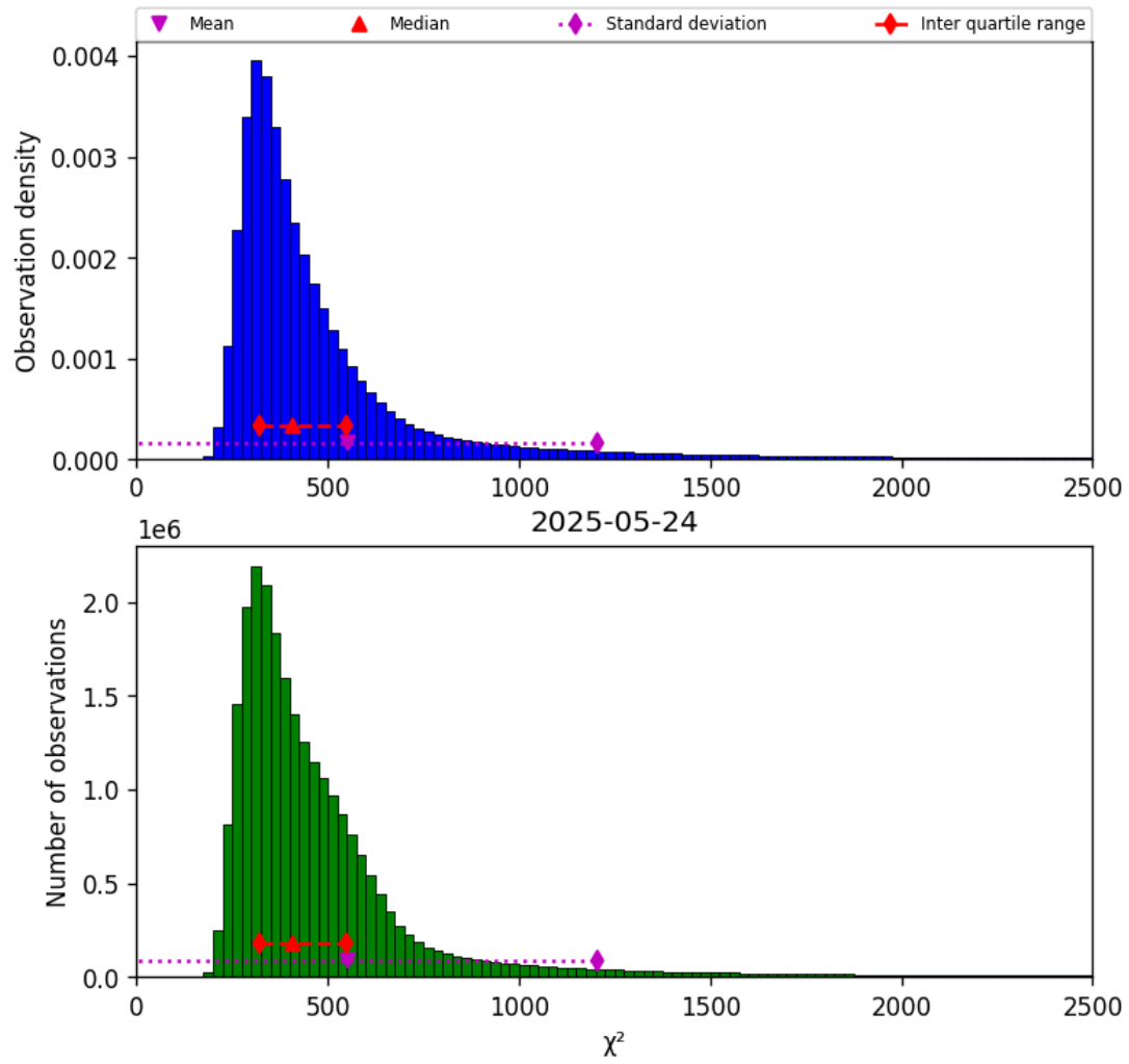
Figure 42: Histogram of “ \chi^2 ” for 2025-05-23 to 2025-05-25
