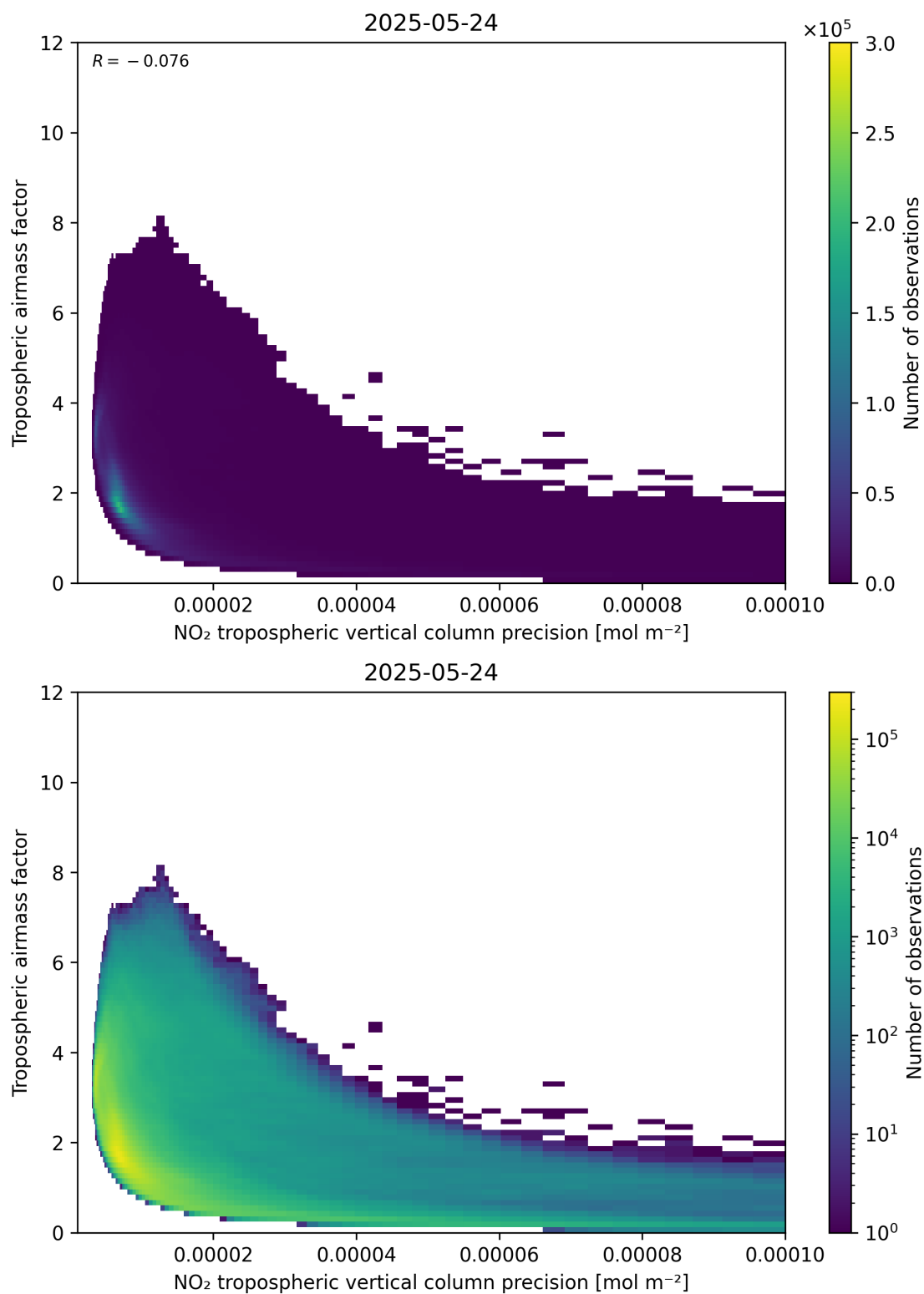
Figure 133: Scatter density plot of “NO 2 tropospheric vertical column precision” against “Tropospheric air mass factor” for 2025-05-23 to 2025-05-25.
