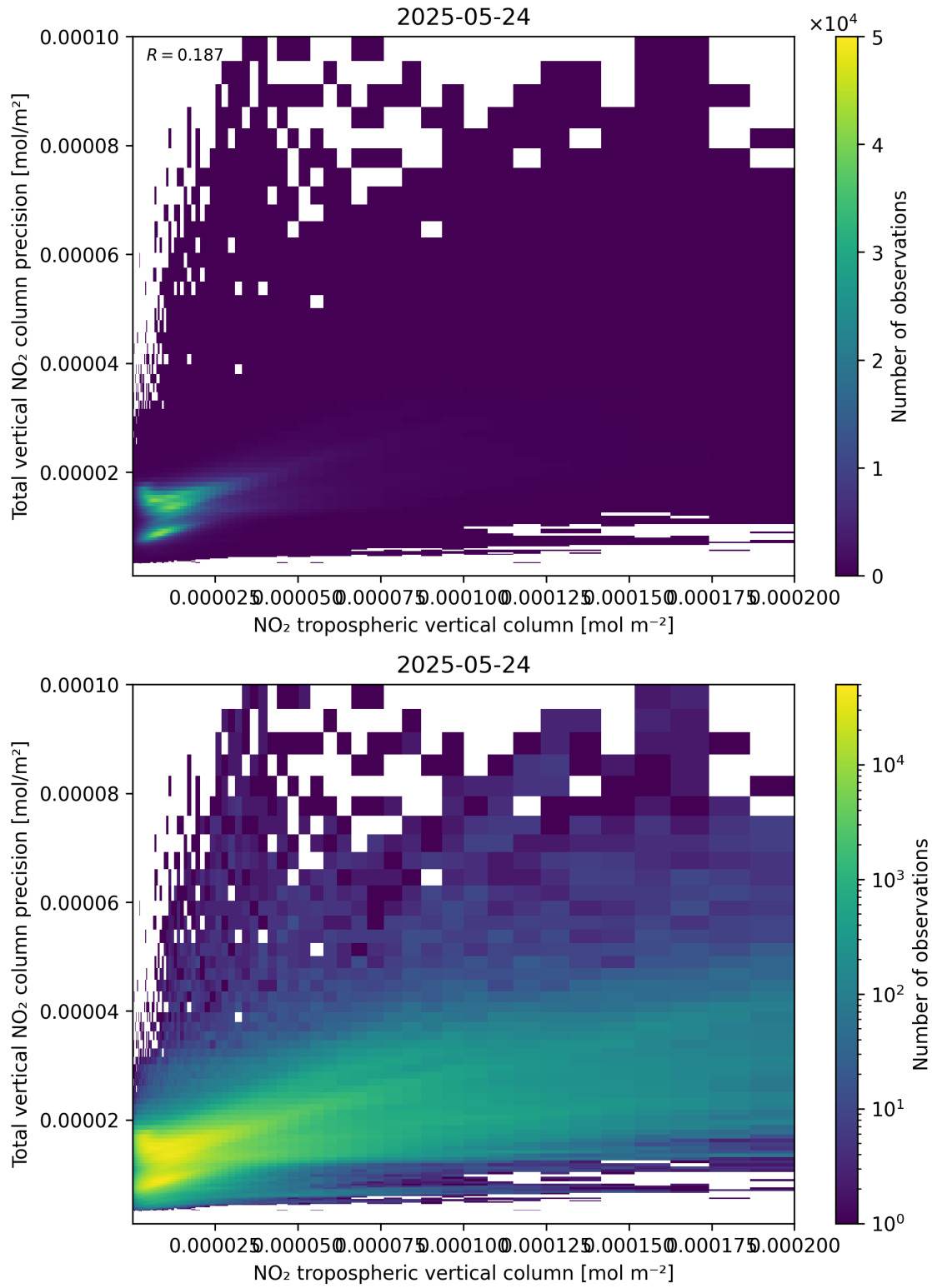
Figure 129: Scatter density plot of “NO 2 tropospheric vertical column” against “Total vertical NO 2 column precision” for 2025-05-23 to 2025-05-25.
