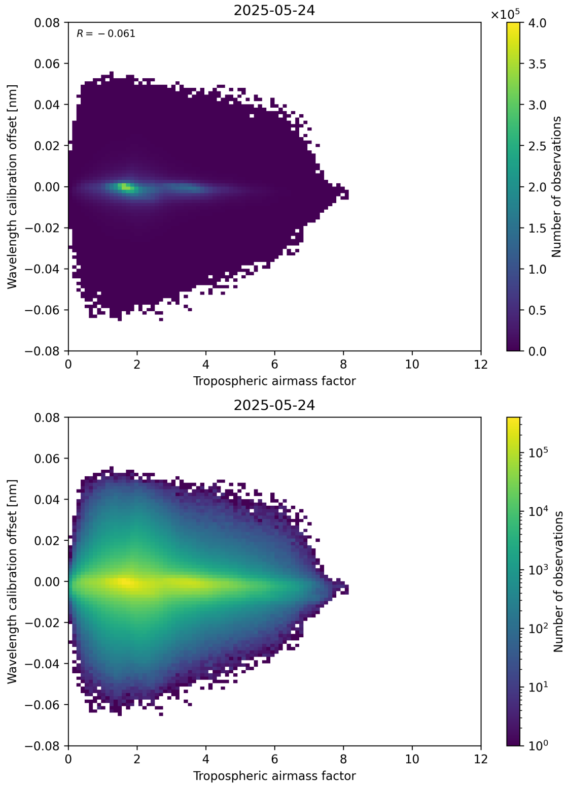
Figure 80: Scatter density plot of “Tropospheric air mass factor” against “Wavelength calibration offset” for 2025-05-23 to 2025-05-25.
