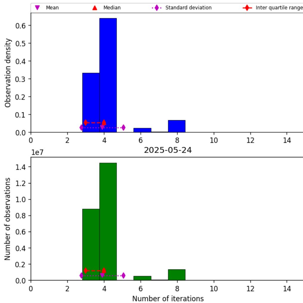
Figure 34: Histogram of “Number of iterations” for 2025-05-23 to 2025-05-25
