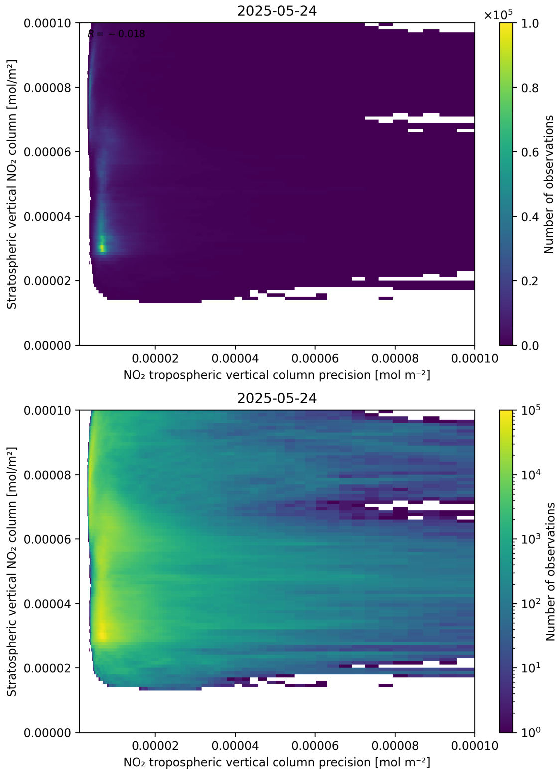
Figure 135: Scatter density plot of “NO 2 tropospheric vertical column precision” against “Stratospheric vertical NO 2 column” for 2025-05-23 to 2025-05-25.
