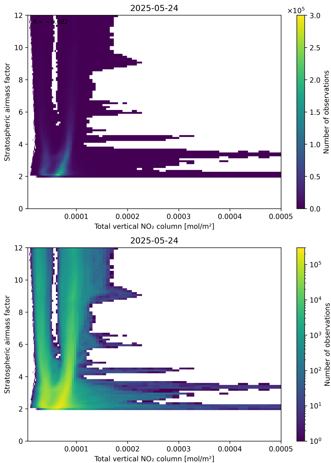
Figure 110: Scatter density plot of “Total vertical NO 2 column” against “Stratospheric air mass factor” for 2025-05-23 to 2025-05-25.
