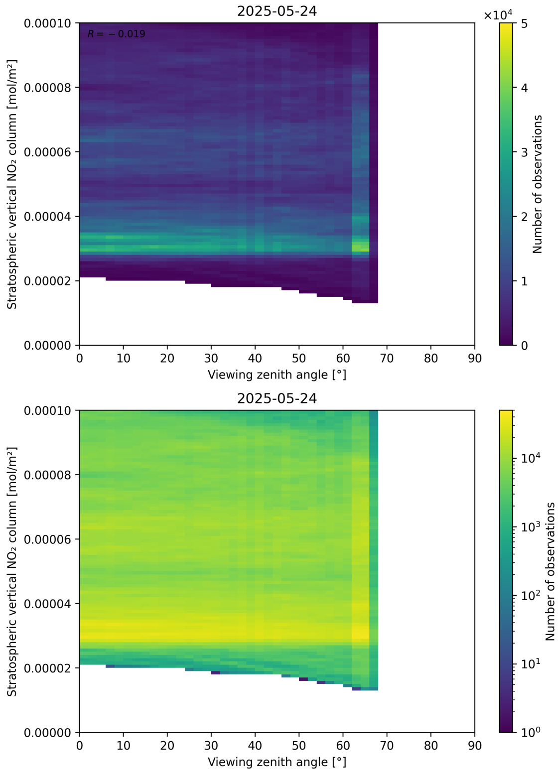
Figure 164: Scatter density plot of “Viewing zenith angle” against “Stratospheric vertical NO 2 column” for 2025-05-23 to 2025-05-25.
