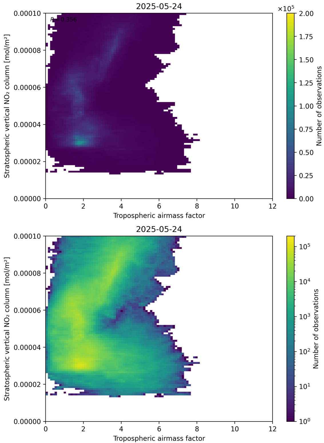
Figure 74: Scatter density plot of “Tropospheric air mass factor” against “Stratospheric vertical NO 2 column” for 2025-05-23 to 2025-05-25.
