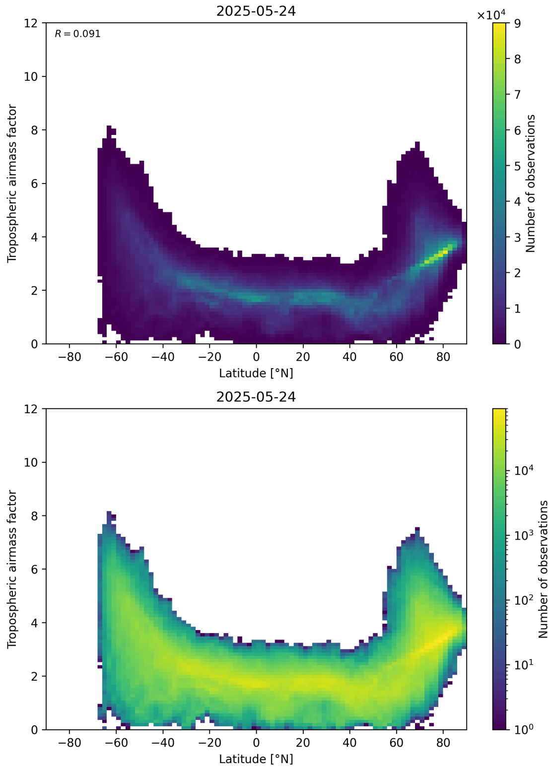
Figure 85: Scatter density plot of “Latitude” against “Tropospheric airmass factor” for 2025-05-23 to 2025-05-25.
