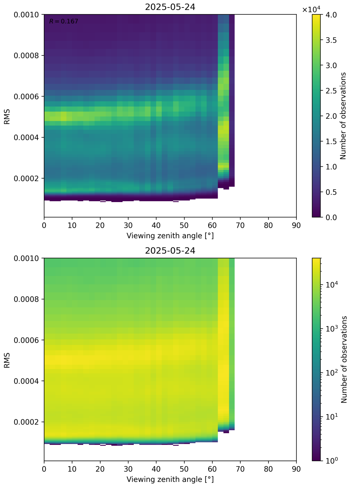
Figure 171: Scatter density plot of “Viewing zenith angle” against “RMS” for 2025-05-23 to 2025-05-25.
