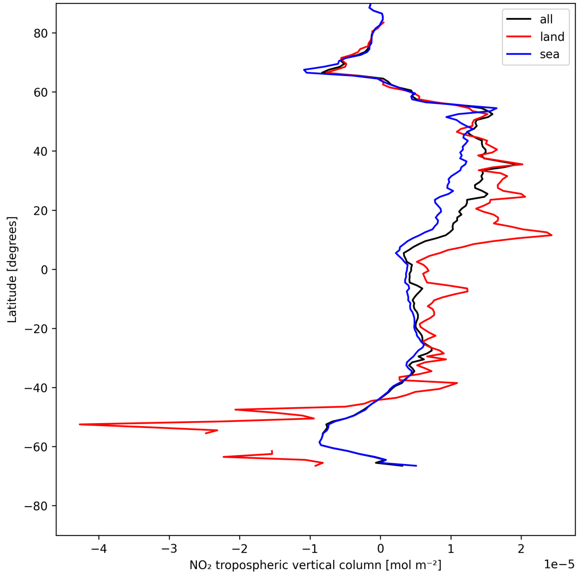
Figure 12: Zonal average of “NO 2 tropospheric vertical column” for 2025-05-23 to 2025-05-25.
