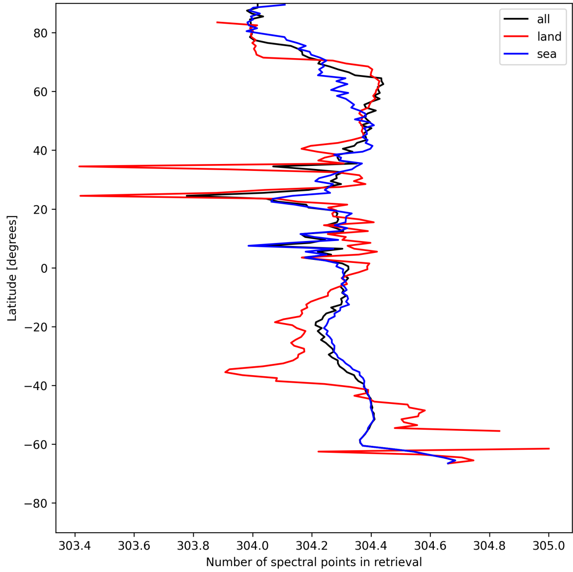
Figure 16: Zonal average of “Number of spectral points in retrieval” for 2025-05-23 to 2025-05-25.
