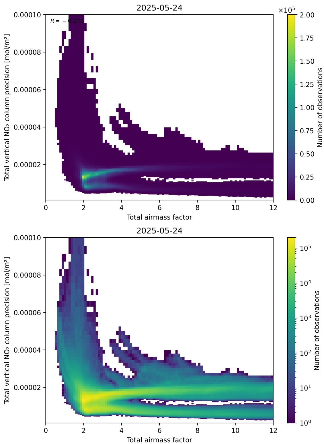
Figure 68: Scatter density plot of “Total airmass factor” against “Total vertical NO 2 column precision” for 2025-05-23 to 2025-05-25.
