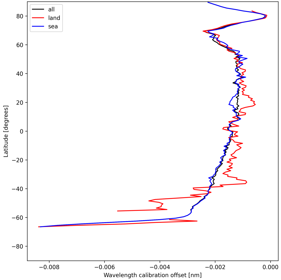
Figure 18: Zonal average of “Wavelength calibration offset” for 2025-05-23 to 2025-05-25.
