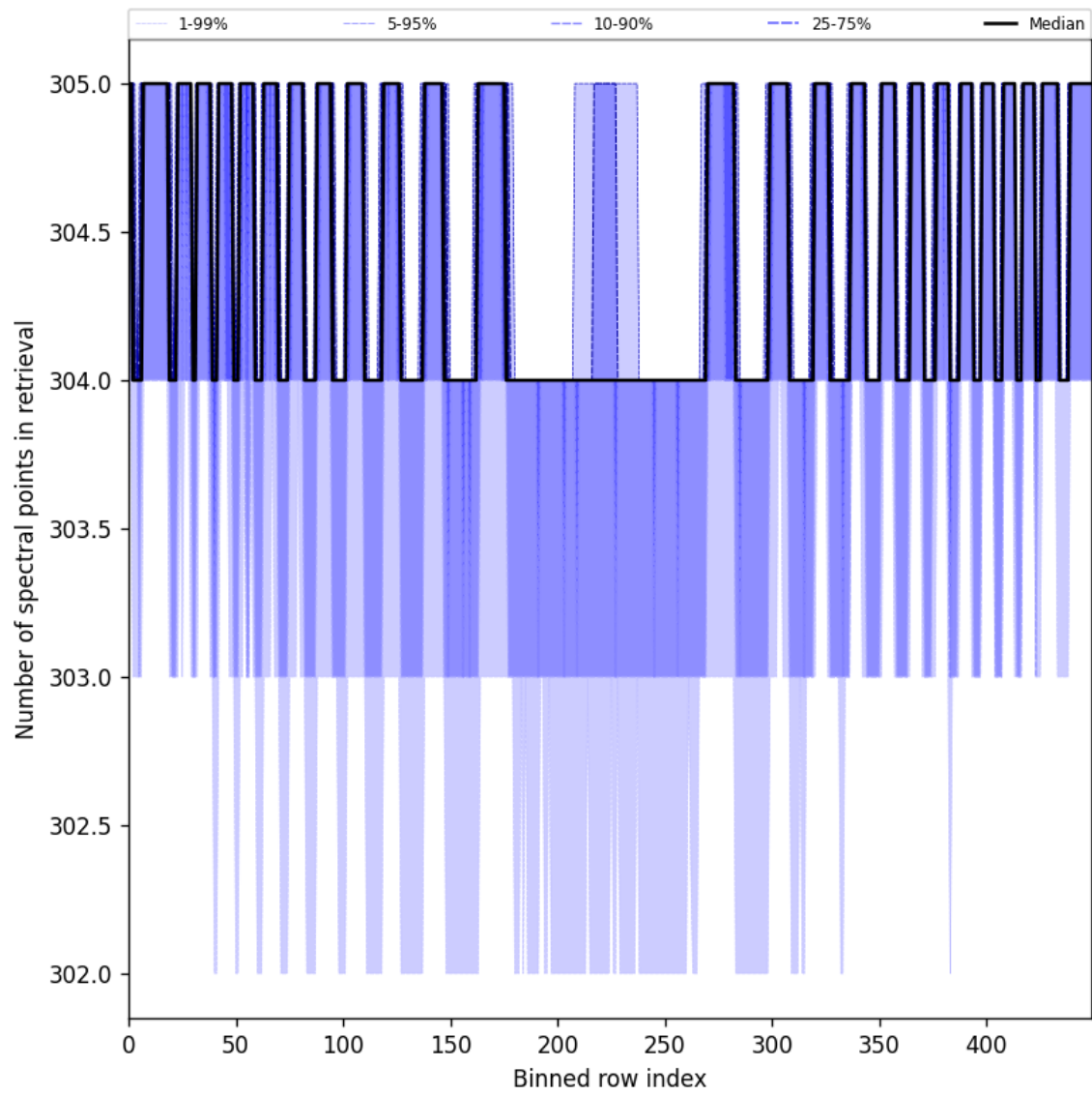
Figure 50: Along track statistics of “Number of spectral points in retrieval” for 2025-05-23 to 2025-05-25
