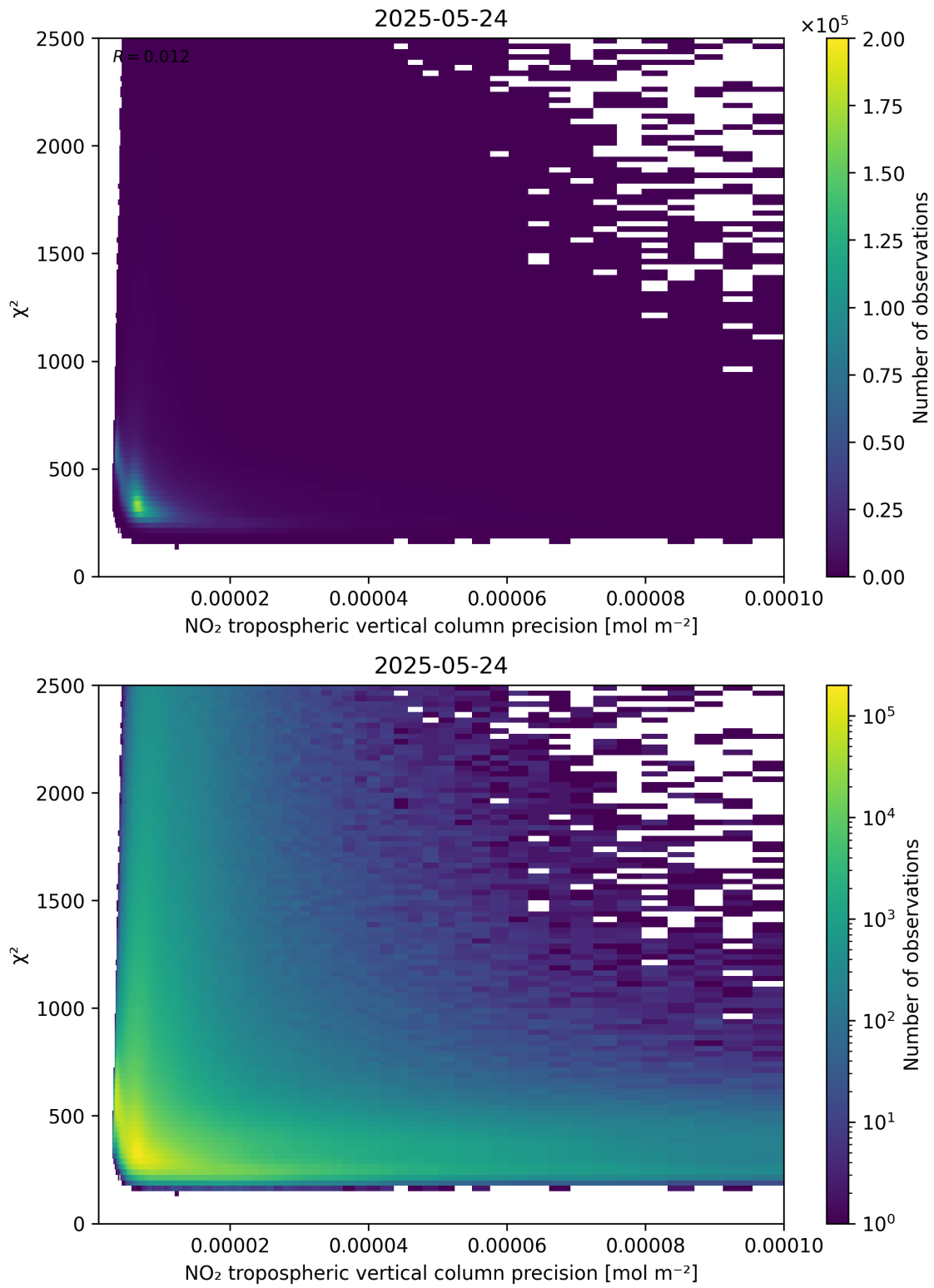
Figure 134: Scatter density plot of “NO 2 tropospheric vertical column precision” against “ \chi^2 ” for 2025-05-23 to 2025-05-25.
