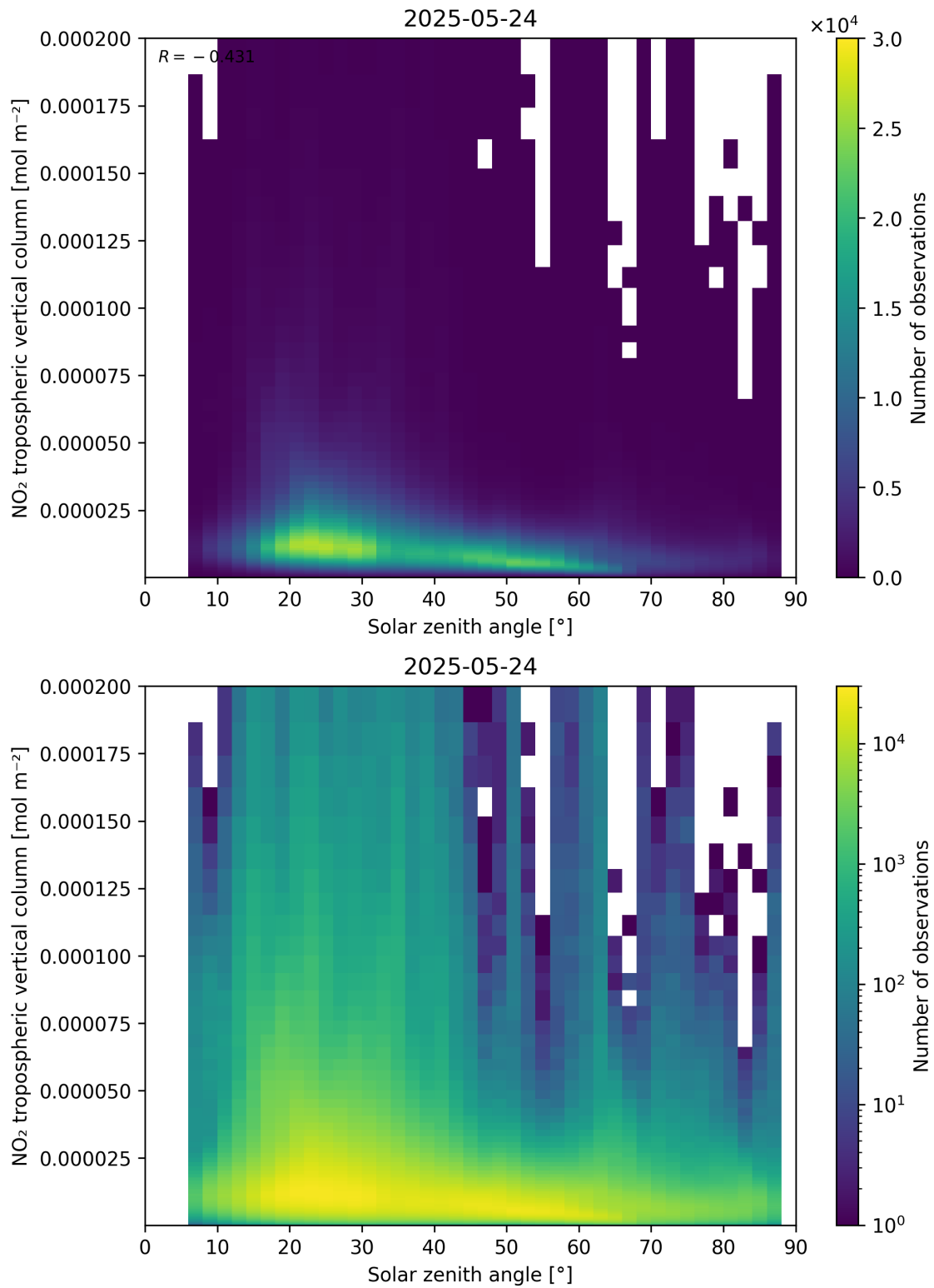
Figure 155: Scatter density plot of “Solar zenith angle” against “NO 2 tropospheric vertical column” for 2025-05-23 to 2025-05-25.
