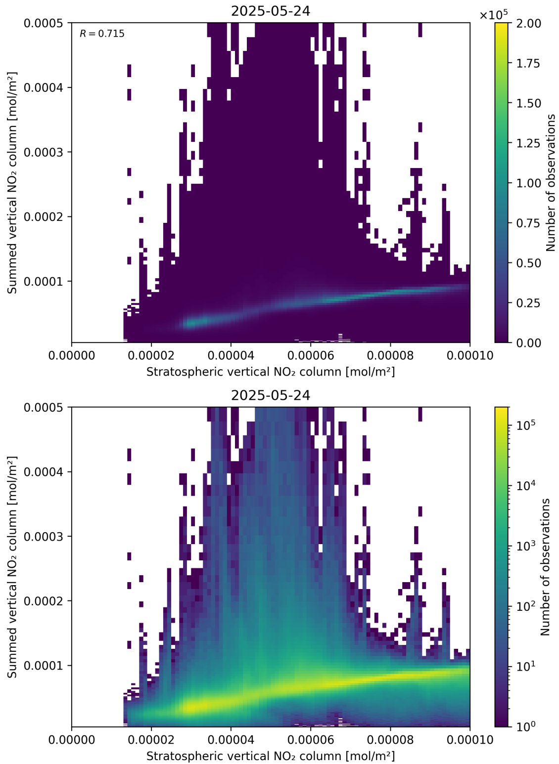
Figure 98: Scatter density plot of “Stratospheric vertical NO 2 column” against “Summed vertical NO 2 column” for 2025-05-23 to 2025-05-25.
