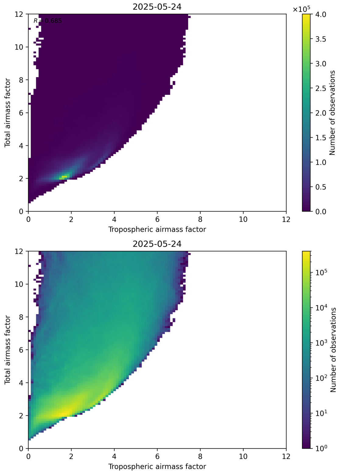
Figure 72: Scatter density plot of “Tropospheric airmass factor” against “Total airmass factor” for 2025-05-23 to 2025-05-25.
