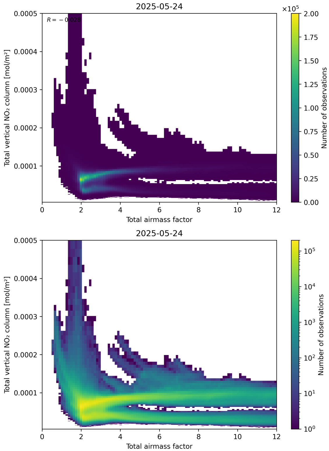
Figure 67: Scatter density plot of “Total airmass factor” against “Total vertical NO 2 column” for 2025-05-23 to 2025-05-25.
