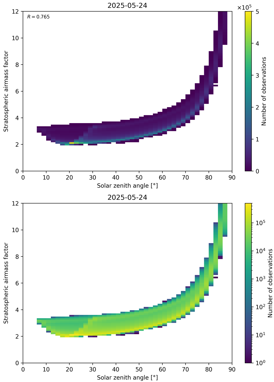
Figure 145: Scatter density plot of “Solar zenith angle” against “Stratospheric airmass factor” for 2025-05-23 to 2025-05-25.
