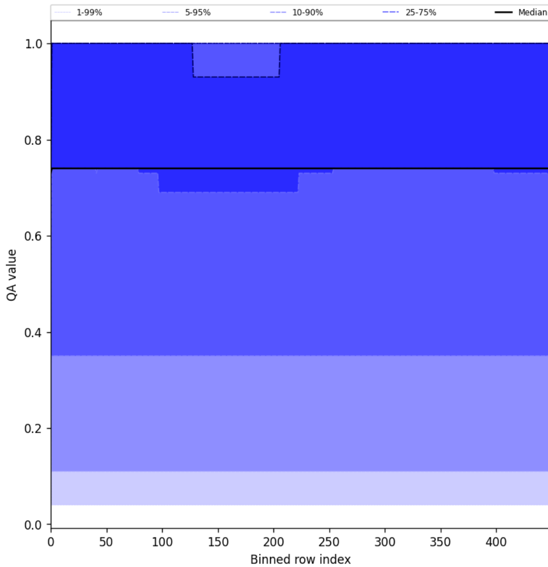
Figure 45: Along track statistics of “QA value” for 2025-05-23 to 2025-05-25
