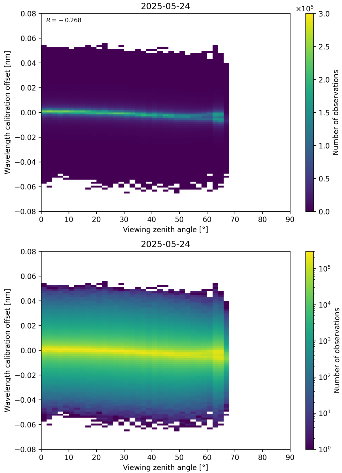
Figure 173: Scatter density plot of “Viewing zenith angle” against “Wavelength calibration offset” for 2025-05-23 to 2025-05-25.
