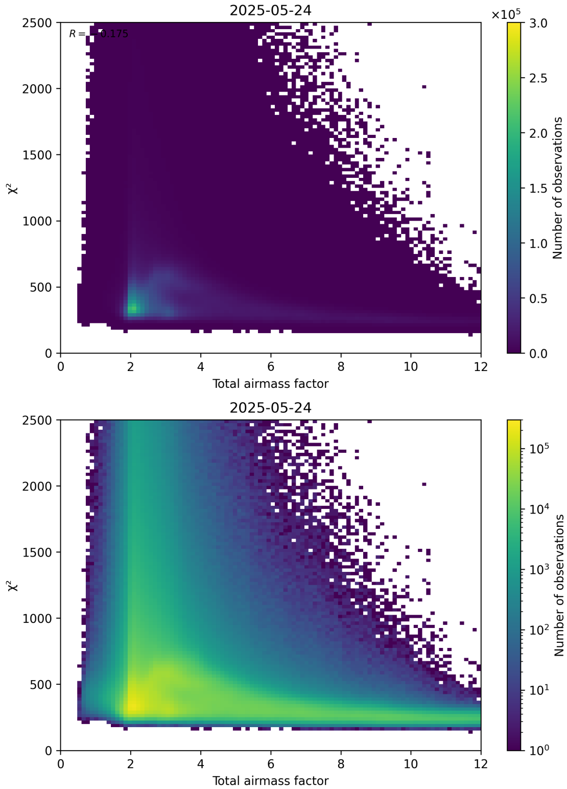
Figure 63: Scatter density plot of “Total airmass factor” against “ \chi^2 ” for 2025-05-23 to 2025-05-25.
