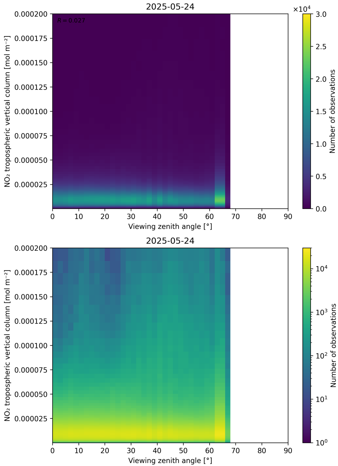
Figure 169: Scatter density plot of “Viewing zenith angle” against “NO 2 tropospheric vertical column” for 2025-05-23 to 2025-05-25.
