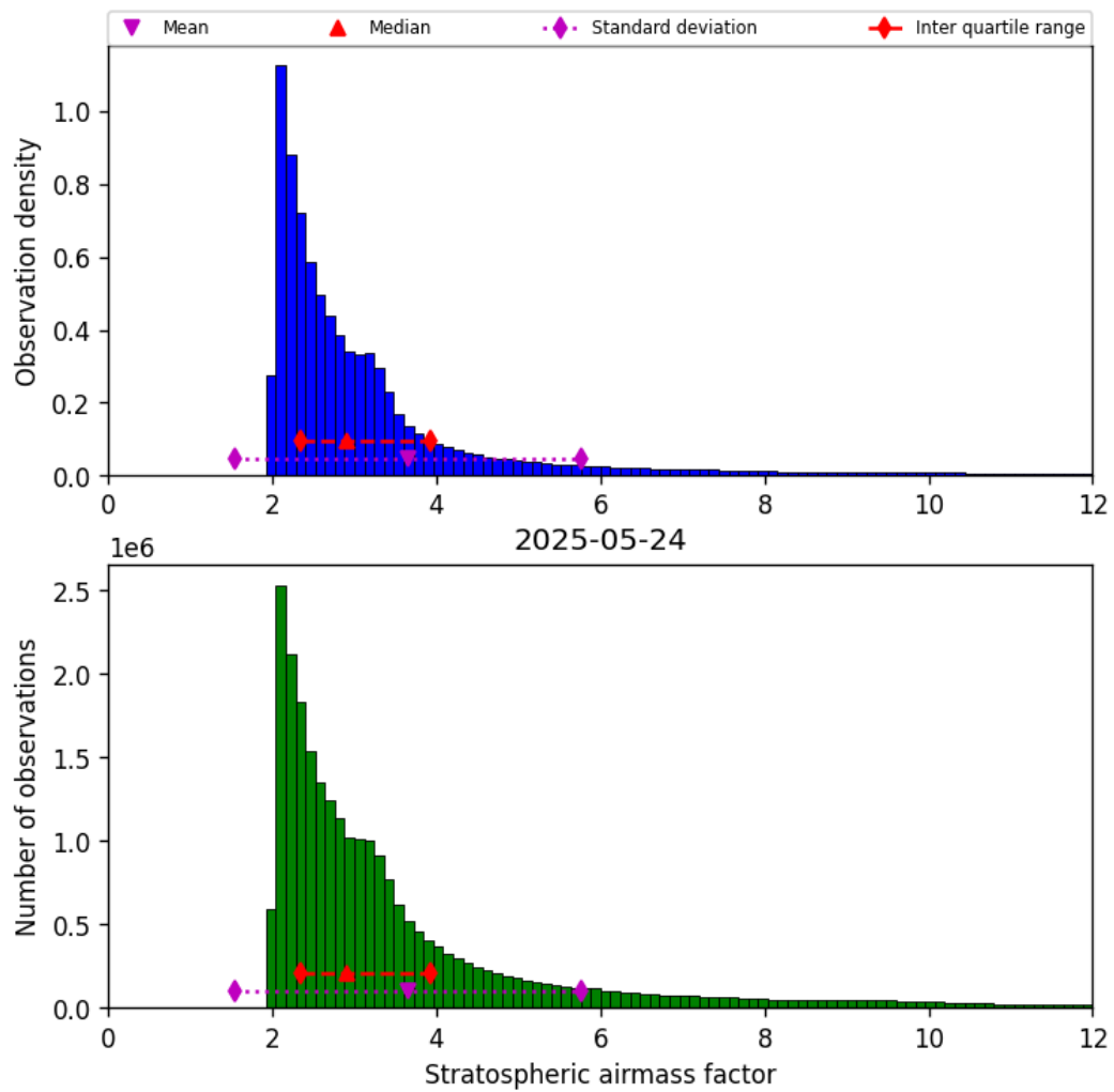
Figure 44: Histogram of “Stratospheric airmass factor” for 2025-05-23 to 2025-05-25
