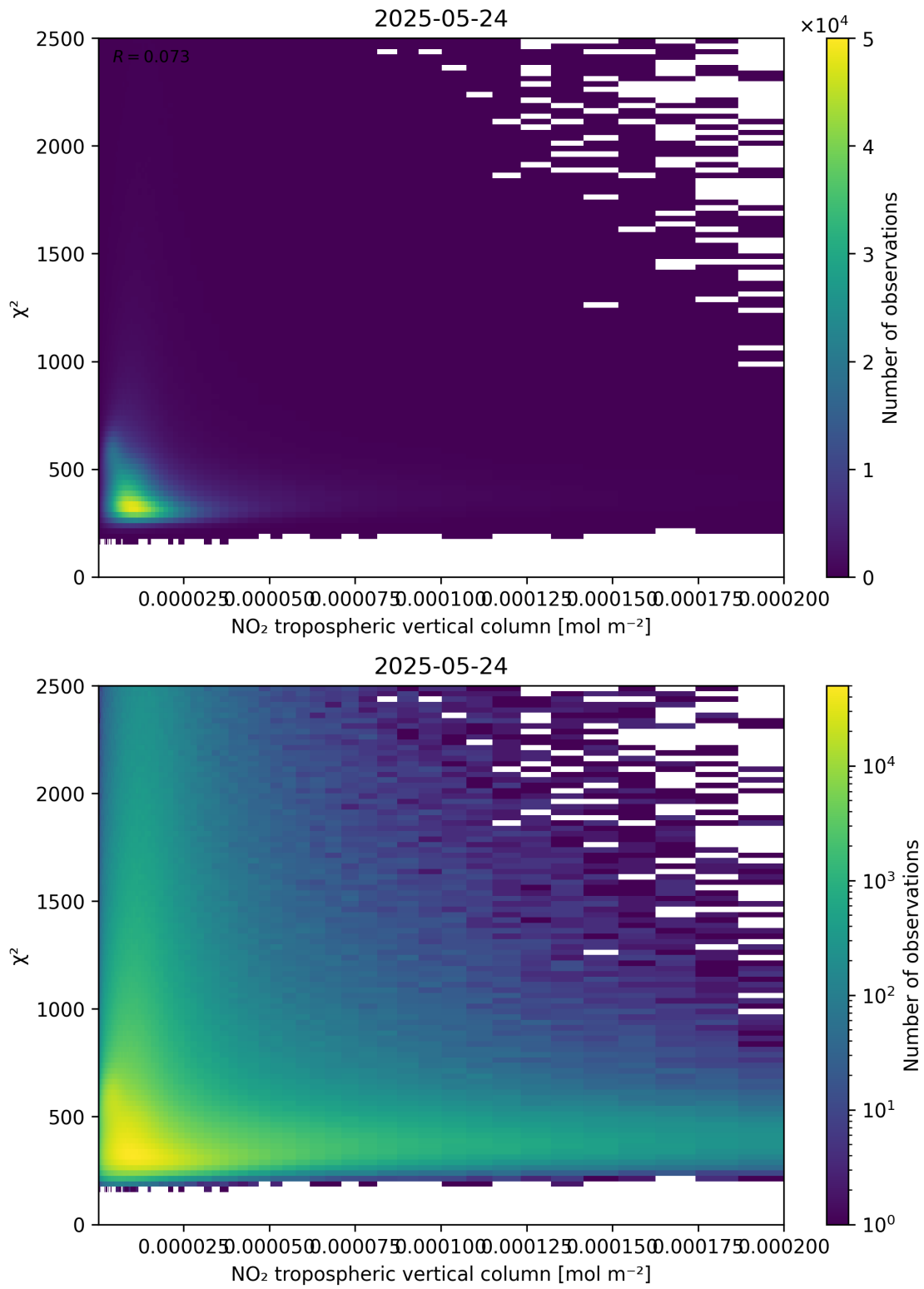
Figure 124: Scatter density plot of “NO 2 tropospheric vertical column” against “ \chi^2 ” for 2025-05-23 to 2025-05-25.
