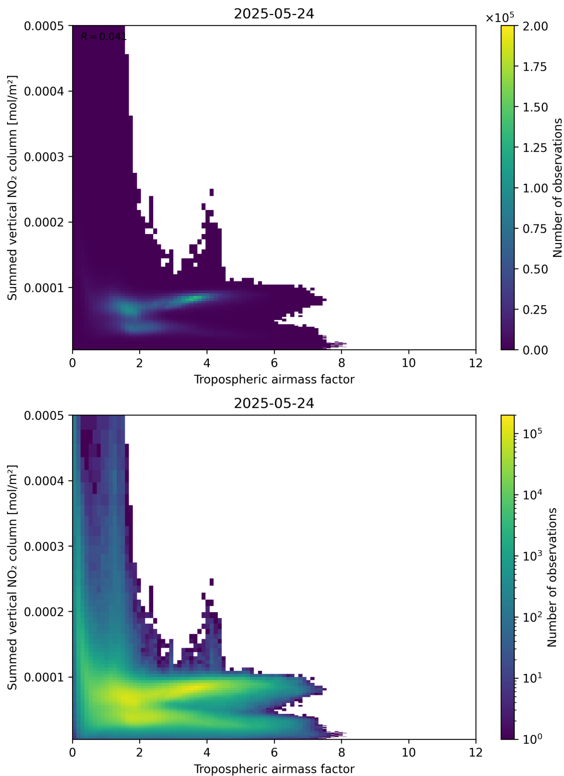
Figure 75: Scatter density plot of “Tropospheric air mass factor” against “Summed vertical NO 2 column” for 2025-05-23 to 2025-05-25.
