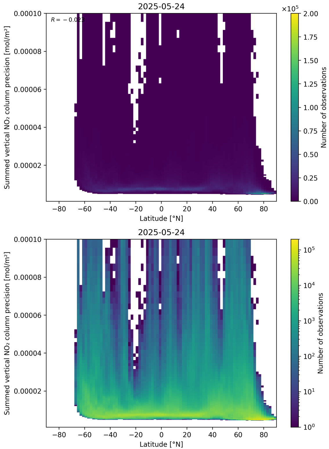
Figure 89: Scatter density plot of “Latitude” against “Summed vertical NO 2 column precision” for 2025-05-23 to 2025-05-25.
