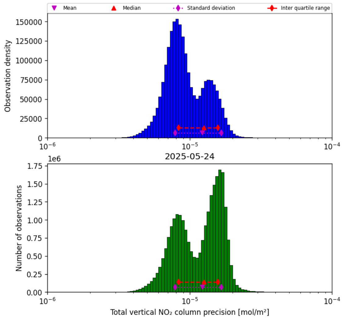
Figure 39: Histogram of "Total vertical NO 2 column precision" for 2025-05-23 to 2025-05-25
