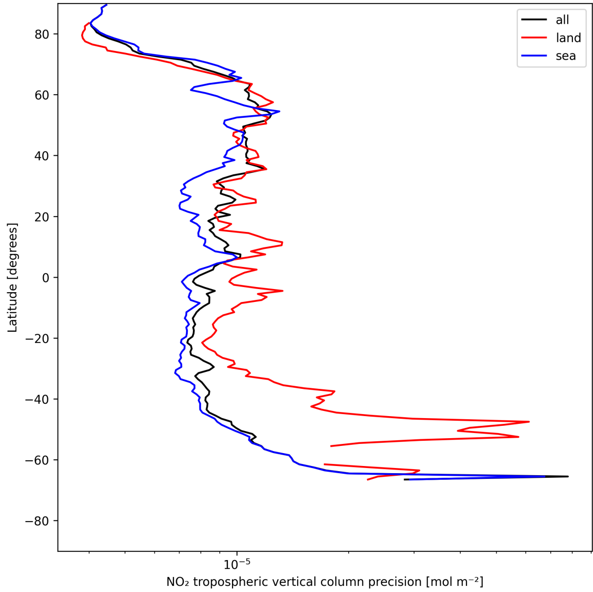
Figure 13: Zonal average of “NO 2 tropospheric vertical column precision” for 2025-05-23 to 2025-05-25.
