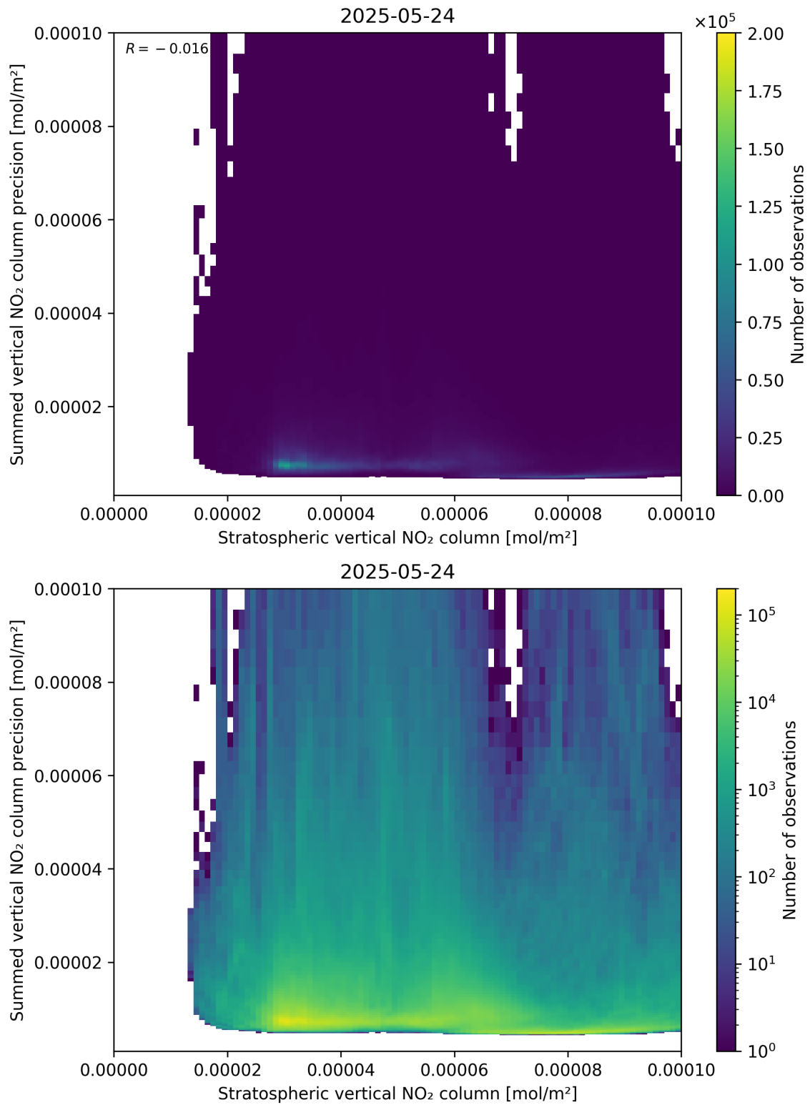
Figure 99: Scatter density plot of “Stratospheric vertical NO 2 column” against “Summed vertical NO 2 column precision” for 2025-05-23 to 2025-05-25.
