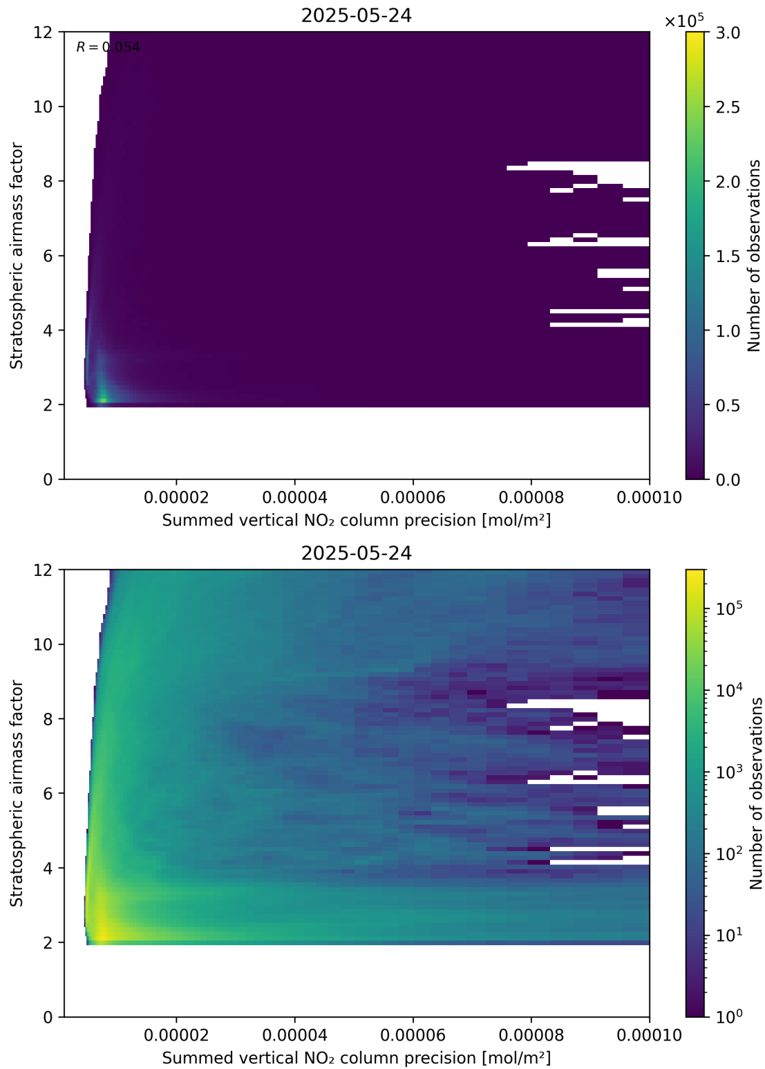
Figure 106: Scatter density plot of “Summed vertical NO 2 column precision” against “Stratospheric airmass factor” for 2025-05-23 to 2025-05-25.
