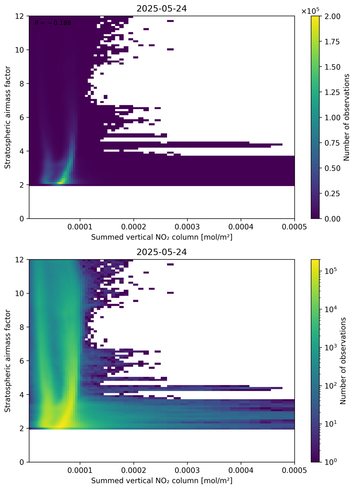
Figure 103: Scatter density plot of “Summed vertical NO 2 column” against “Stratospheric air mass factor” for 2025-05-23 to 2025-05-25.
