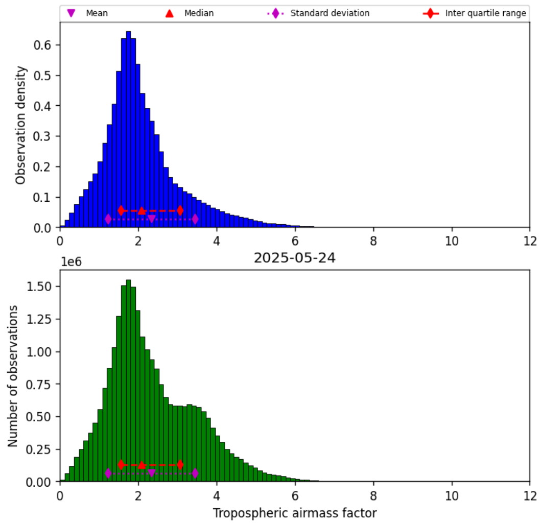
Figure 31: Histogram of “Tropospheric airmass factor” for 2025-05-23 to 2025-05-25
