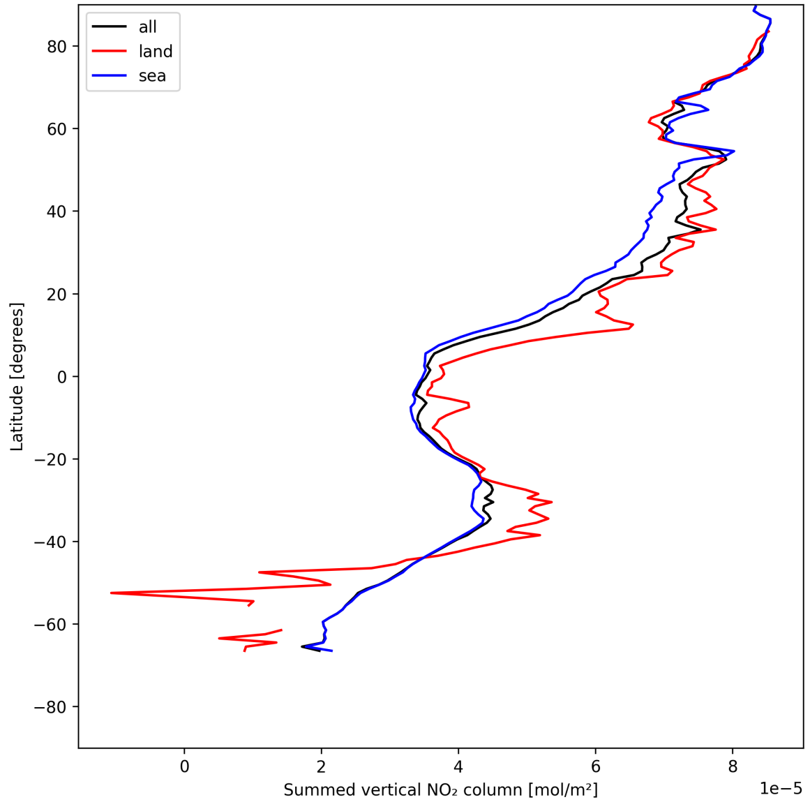
Figure 23: Zonal average of “Summed vertical NO 2 column” for 2025-05-23 to 2025-05-25.
