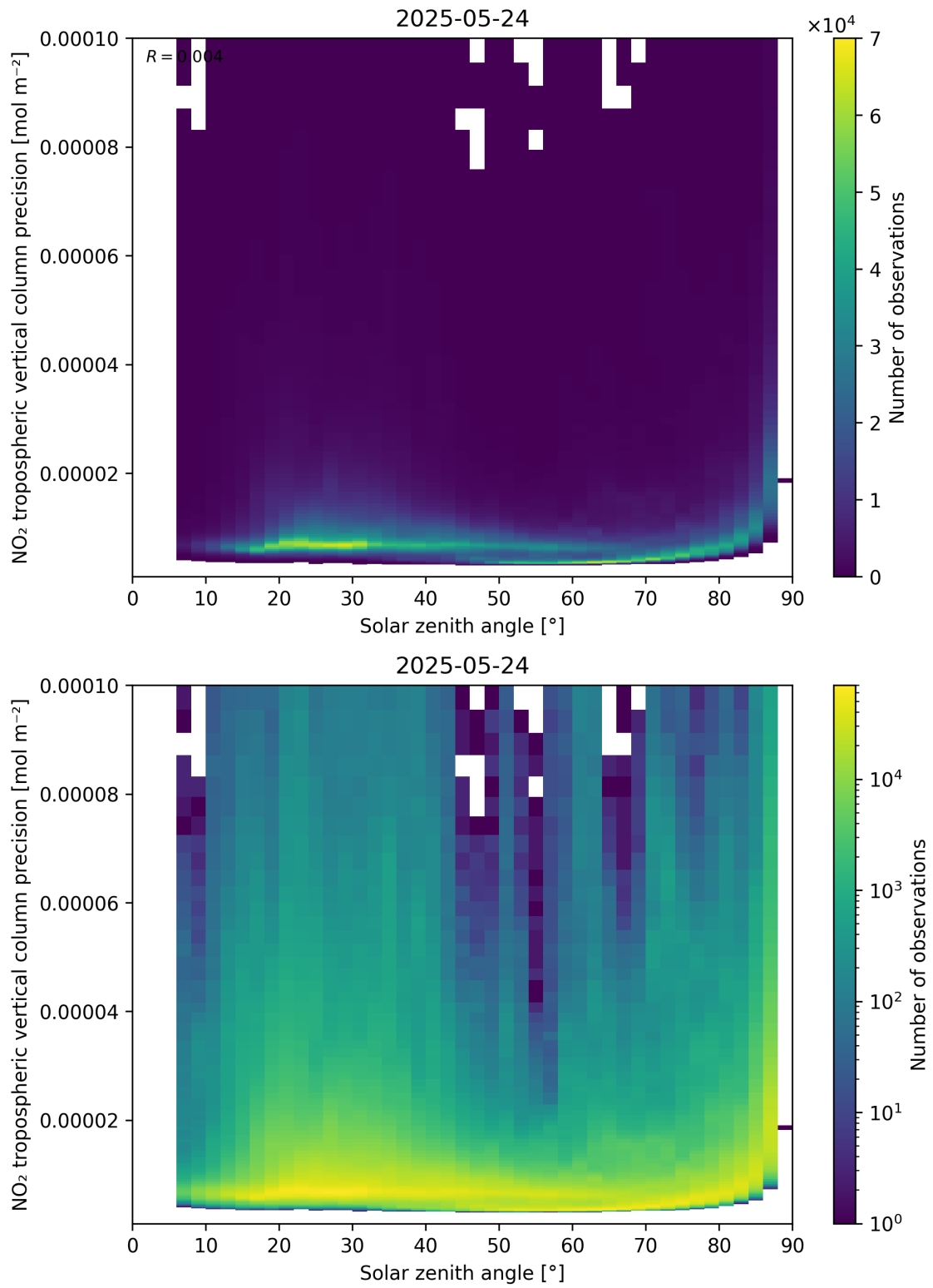
Figure 156: Scatter density plot of “Solar zenith angle” against “NO 2 tropospheric vertical column precision” for 2025-05-23 to 2025-05-25.
