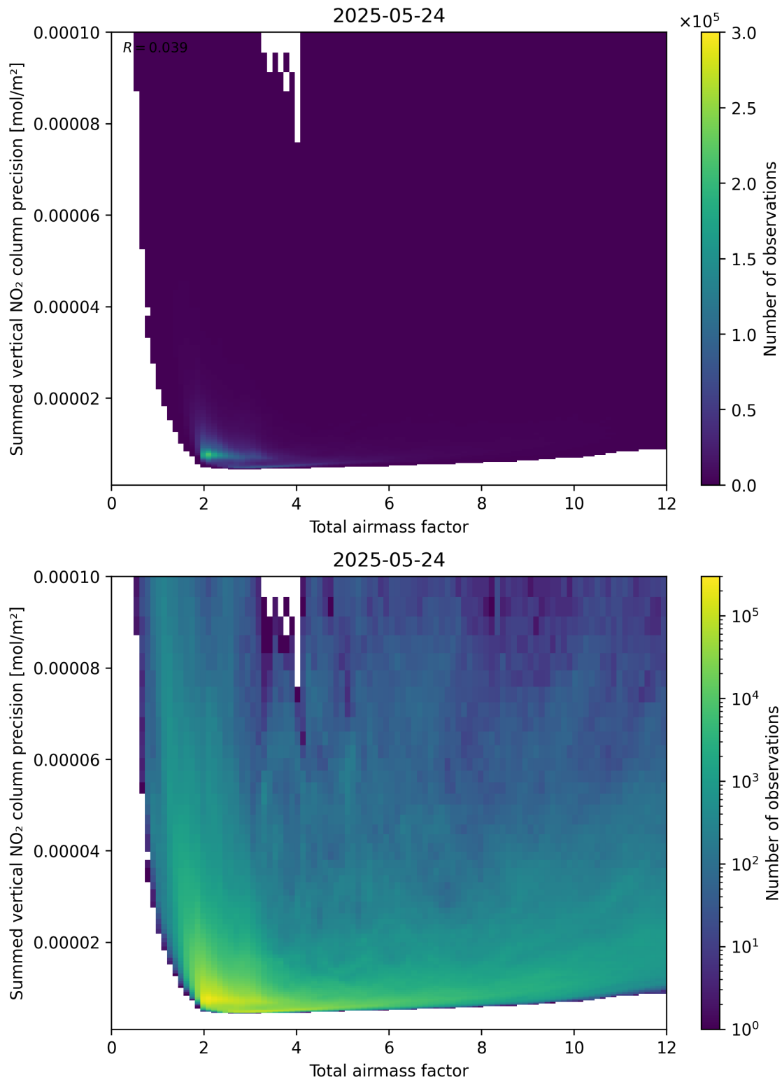
Figure 66: Scatter density plot of “Total airmass factor” against “Summed vertical NO 2 column precision” for 2025-05-23 to 2025-05-25.
