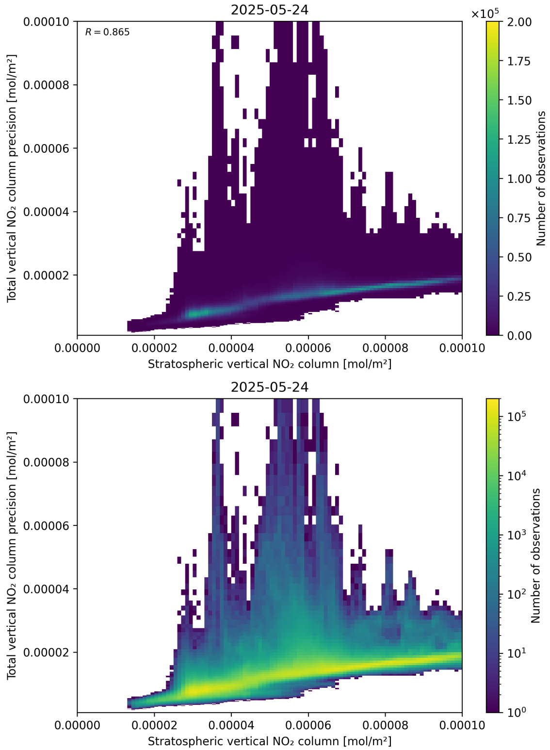
Figure 101: Scatter density plot of “Stratospheric vertical NO 2 column” against “Total vertical NO 2 column precision” for 2025-05-23 to 2025-05-25.
