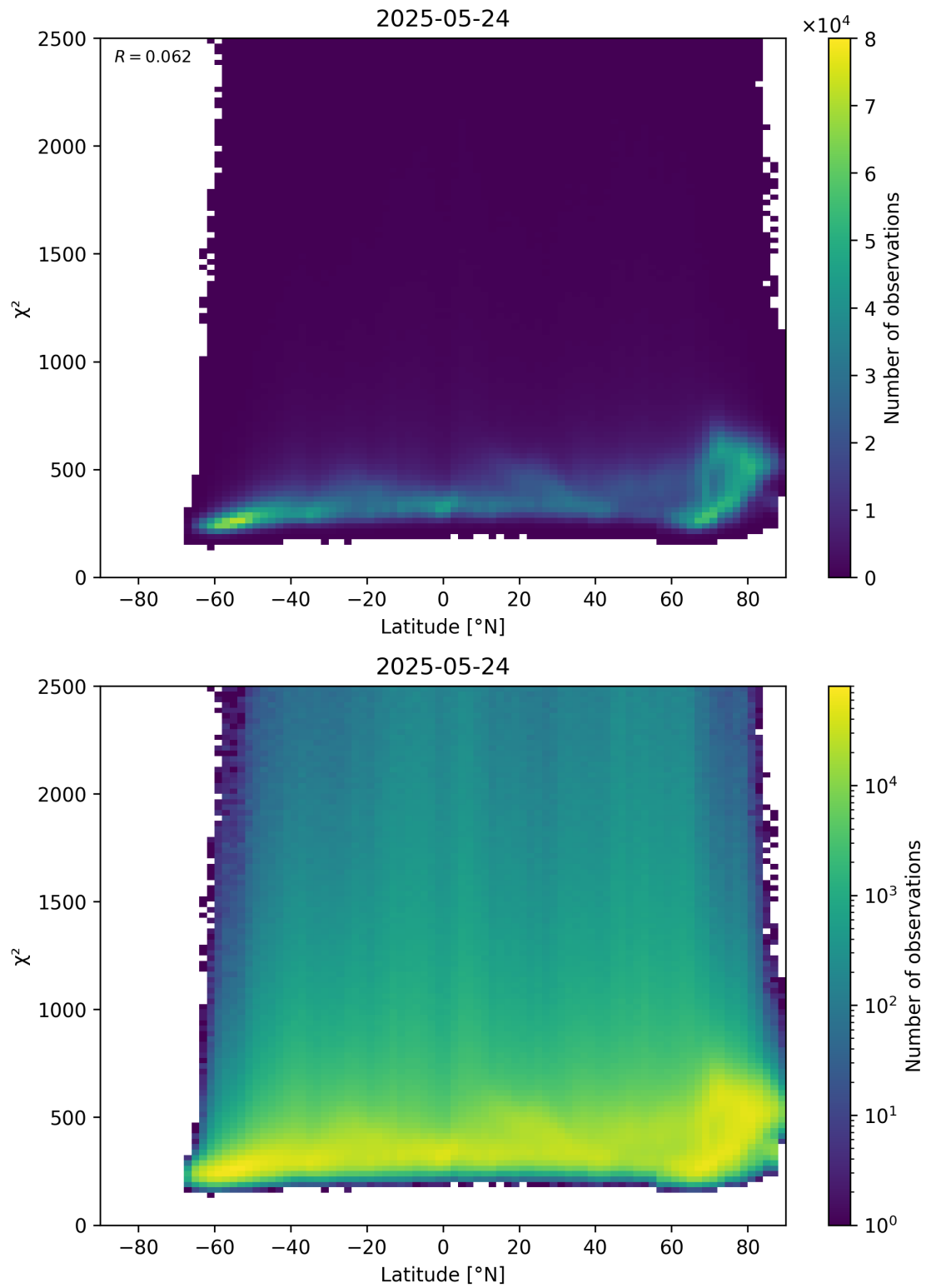
Figure 86: Scatter density plot of “Latitude” against “ \chi^2 ” for 2025-05-23 to 2025-05-25.
