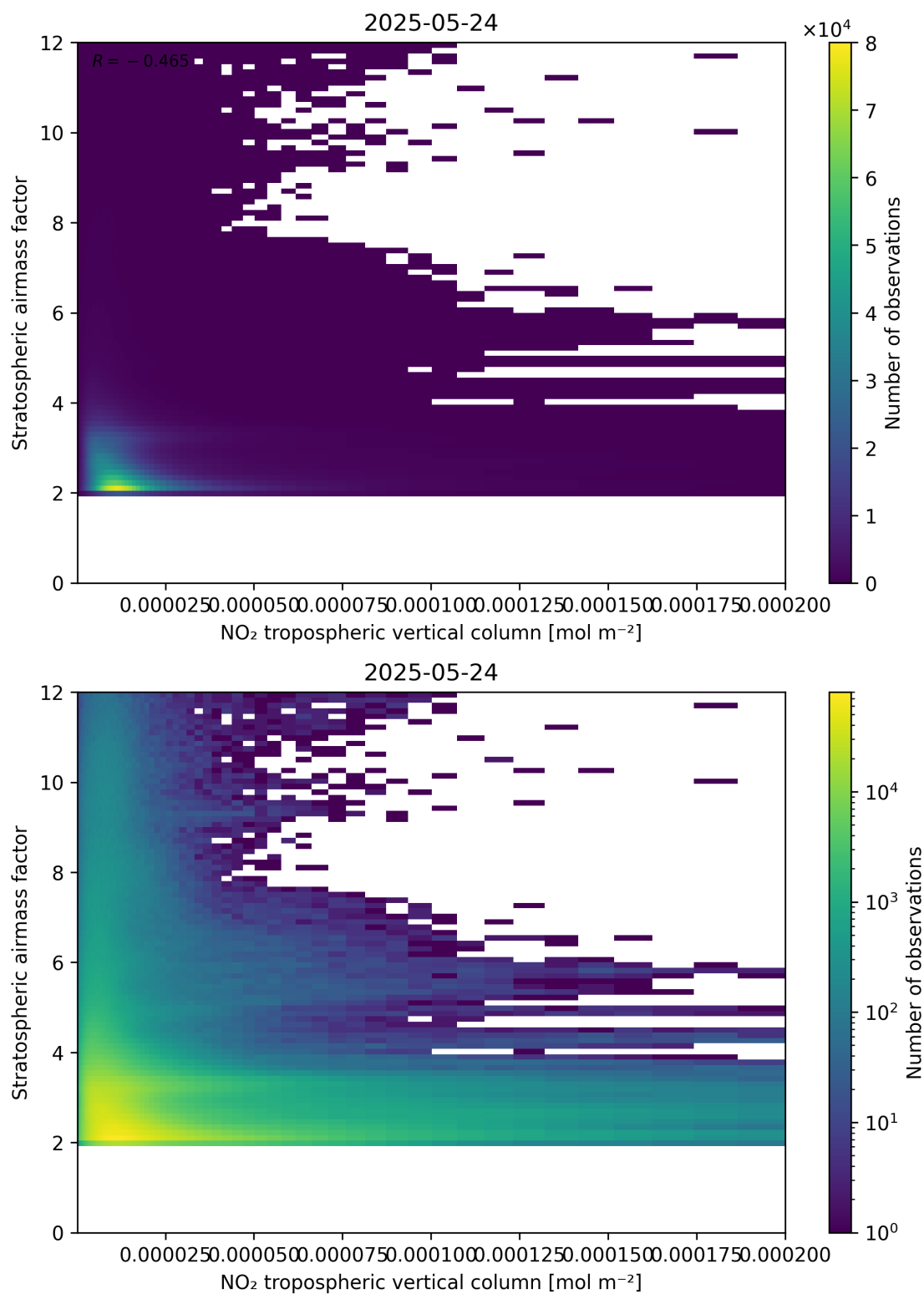
Figure 121: Scatter density plot of “NO 2 tropospheric vertical column” against “Stratospheric air mass factor” for 2025-05-23 to 2025-05-25.
