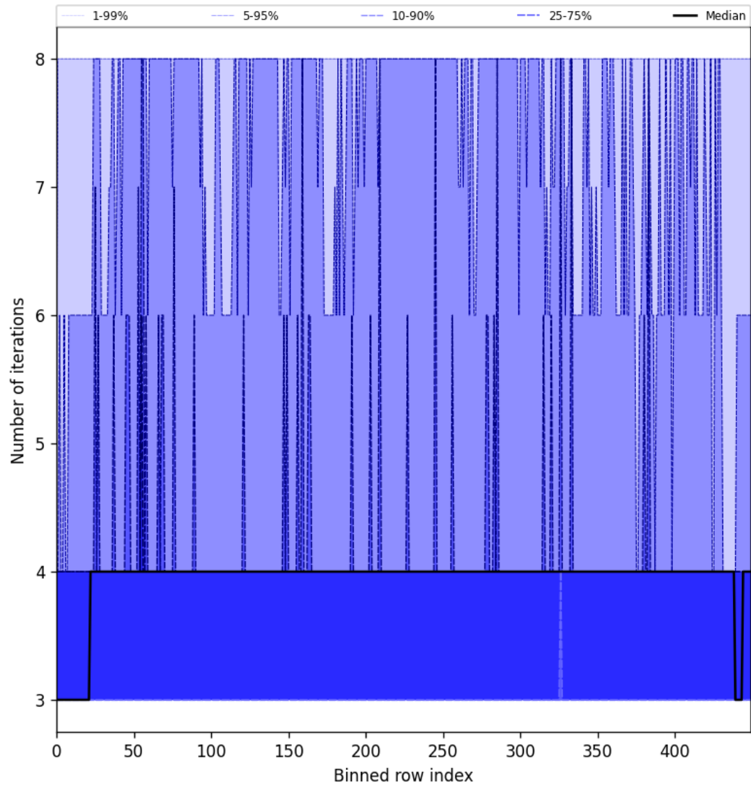
Figure 51: Along track statistics of “Number of iterations” for 2025-05-23 to 2025-05-25
