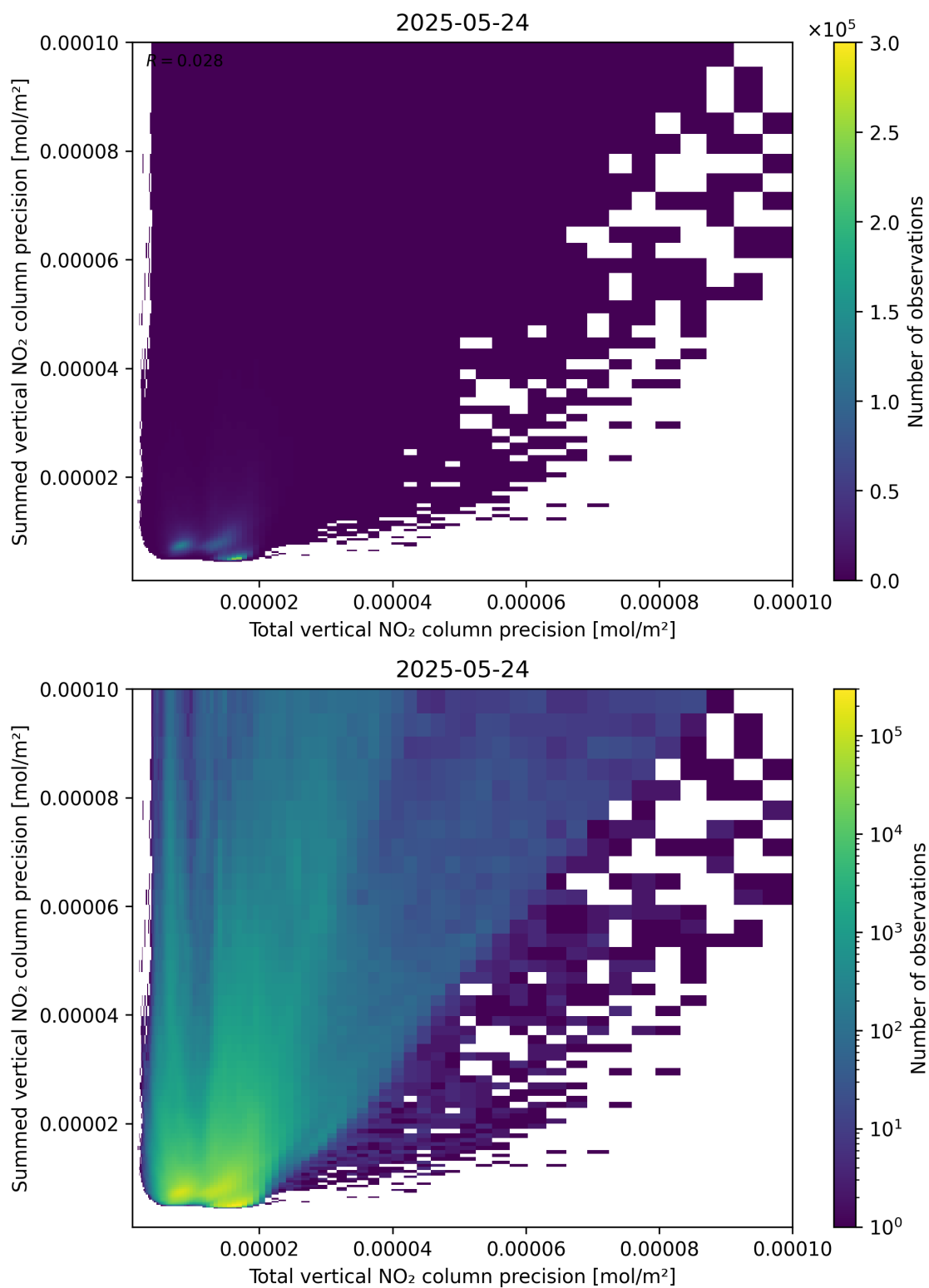
Figure 118: Scatter density plot of “Total vertical NO 2 column precision” against “Summed vertical NO 2 column precision” for 2025-05-23 to 2025-05-25.
