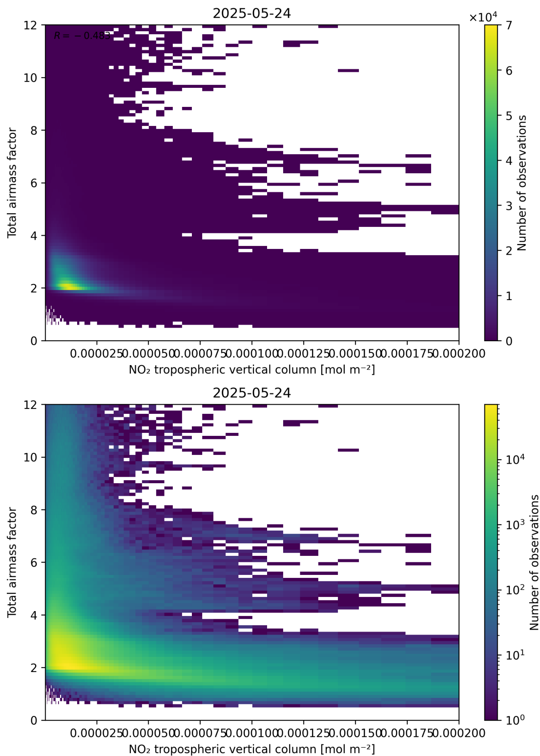
Figure 122: Scatter density plot of “NO 2 tropospheric vertical column” against “Total air mass factor” for 2025-05-23 to 2025-05-25.
