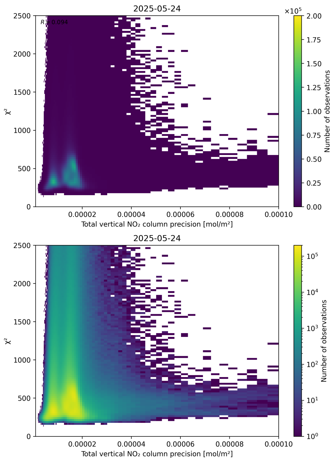
Figure 116: Scatter density plot of “Total vertical NO 2 column precision” against “ \chi^2 ” for 2025-05-23 to 2025-05-25.
