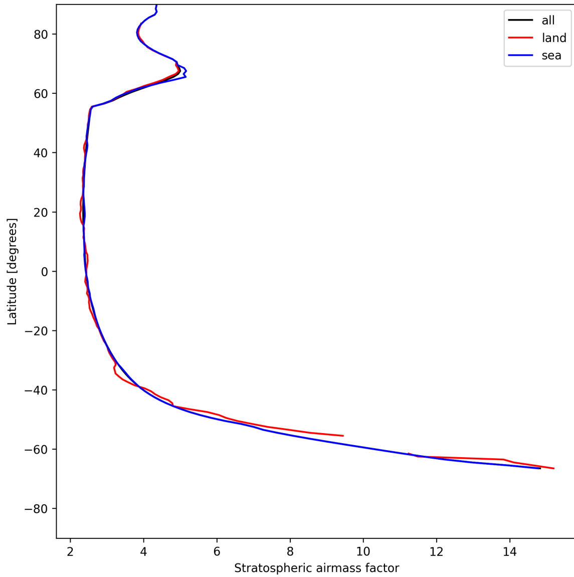
Figure 27: Zonal average of “Stratospheric airmass factor” for 2025-05-23 to 2025-05-25.
