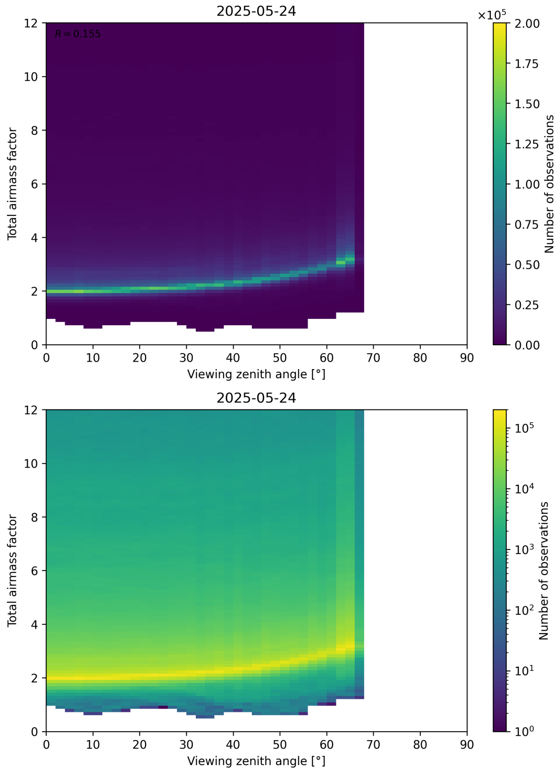
Figure 160: Scatter density plot of “Viewing zenith angle” against “Total airmass factor” for 2025-05-23 to 2025-05-25.
