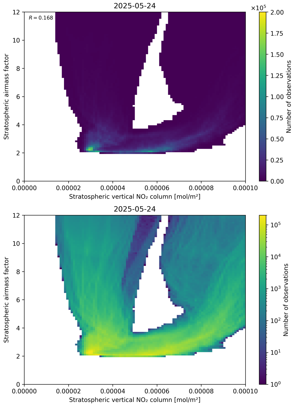
Figure 96: Scatter density plot of “Stratospheric vertical NO 2 column” against “Stratospheric airmass factor” for 2025-05-23 to 2025-05-25.
