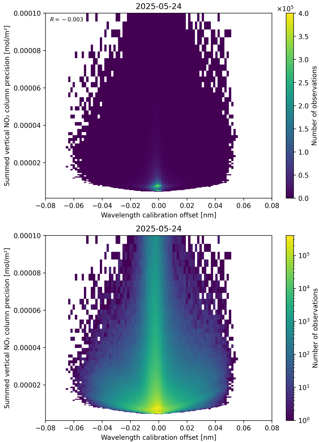
Figure 178: Scatter density plot of “Wavelength calibration offset” against “Summed vertical NO 2 column precision” for 2025-05-23 to 2025-05-25.
