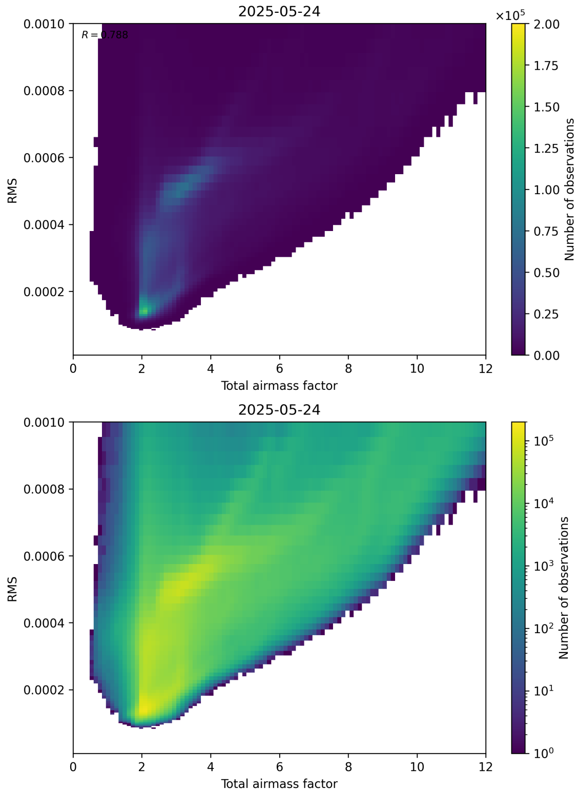
Figure 69: Scatter density plot of “Total airmass factor” against “RMS” for 2025-05-23 to 2025-05-25.
