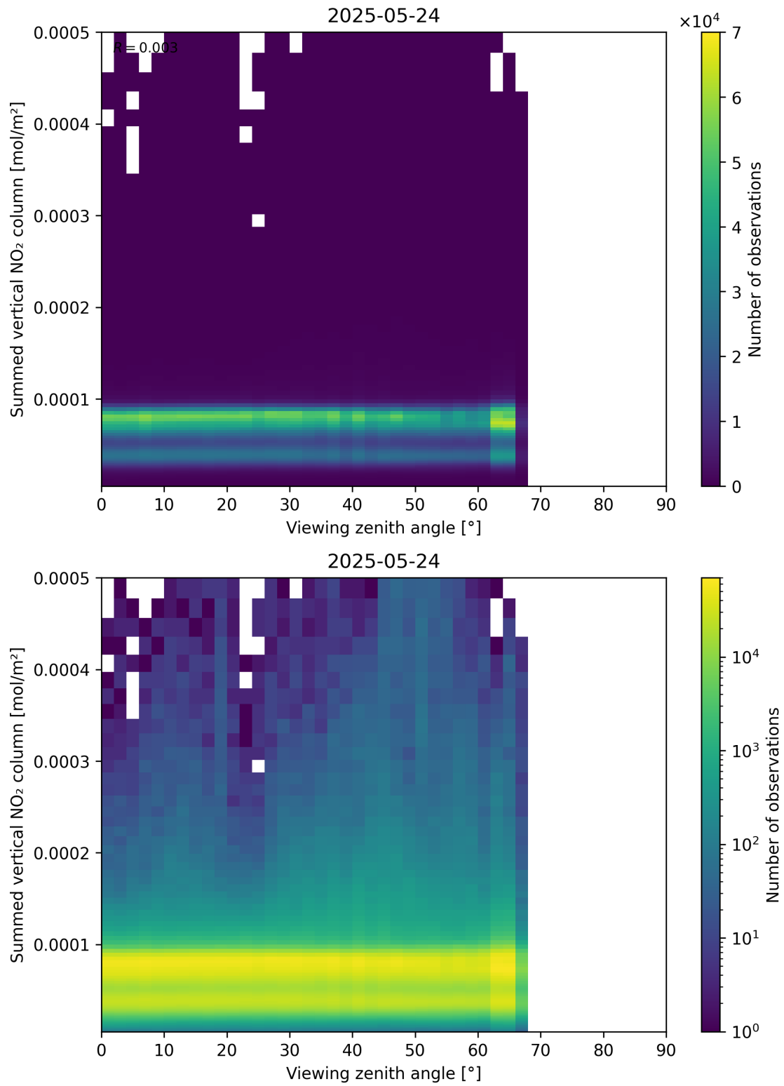
Figure 165: Scatter density plot of “Viewing zenith angle” against “Summed vertical NO 2 column” for 2025-05-23 to 2025-05-25.
