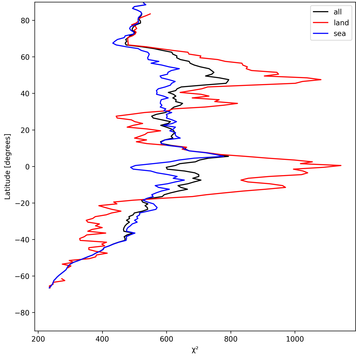
Figure 25: Zonal average of “ \chi^2 ” for 2025-05-23 to 2025-05-25.
