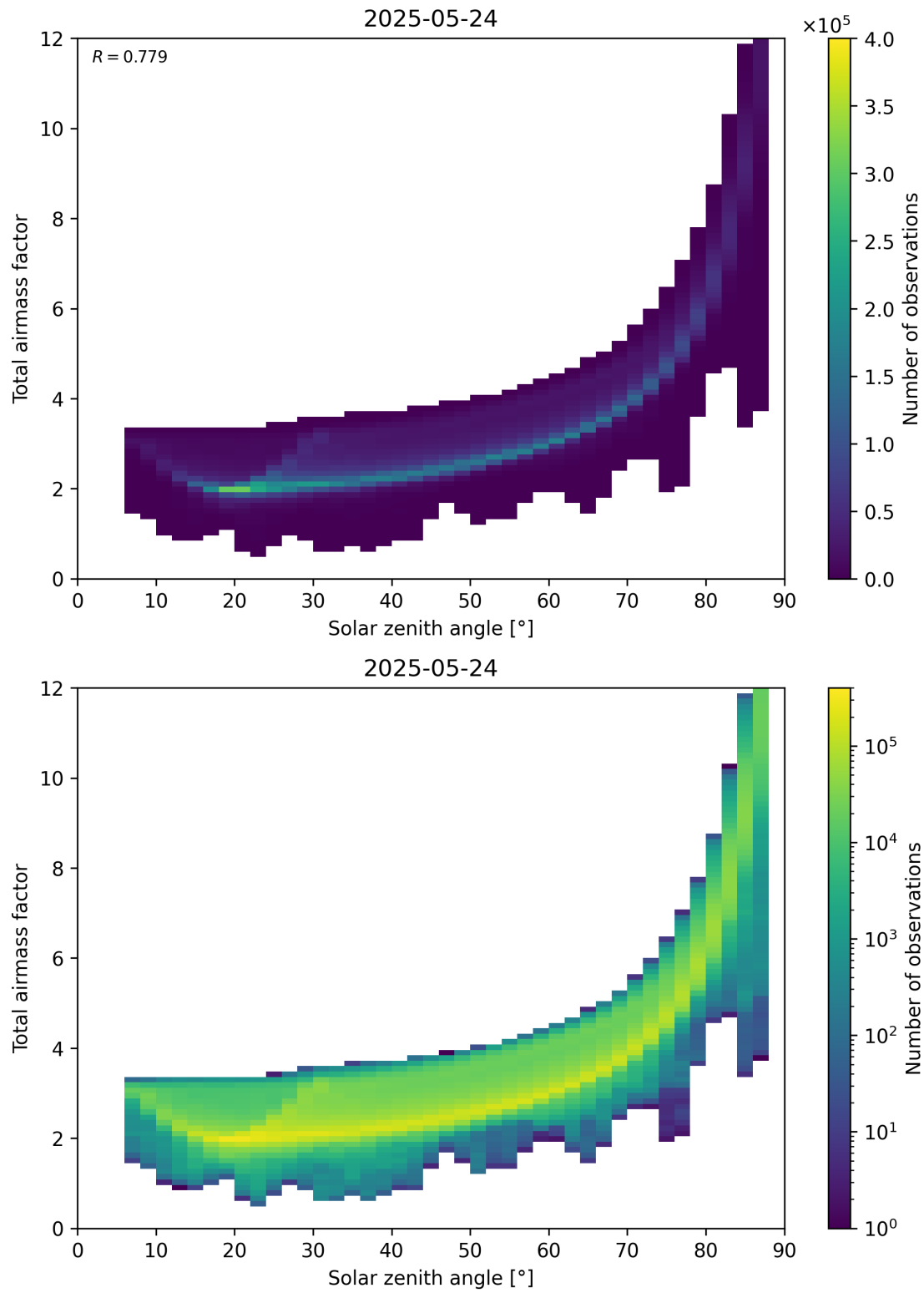
Figure 146: Scatter density plot of “Solar zenith angle” against “Total air mass factor” for 2025-05-23 to 2025-05-25.
