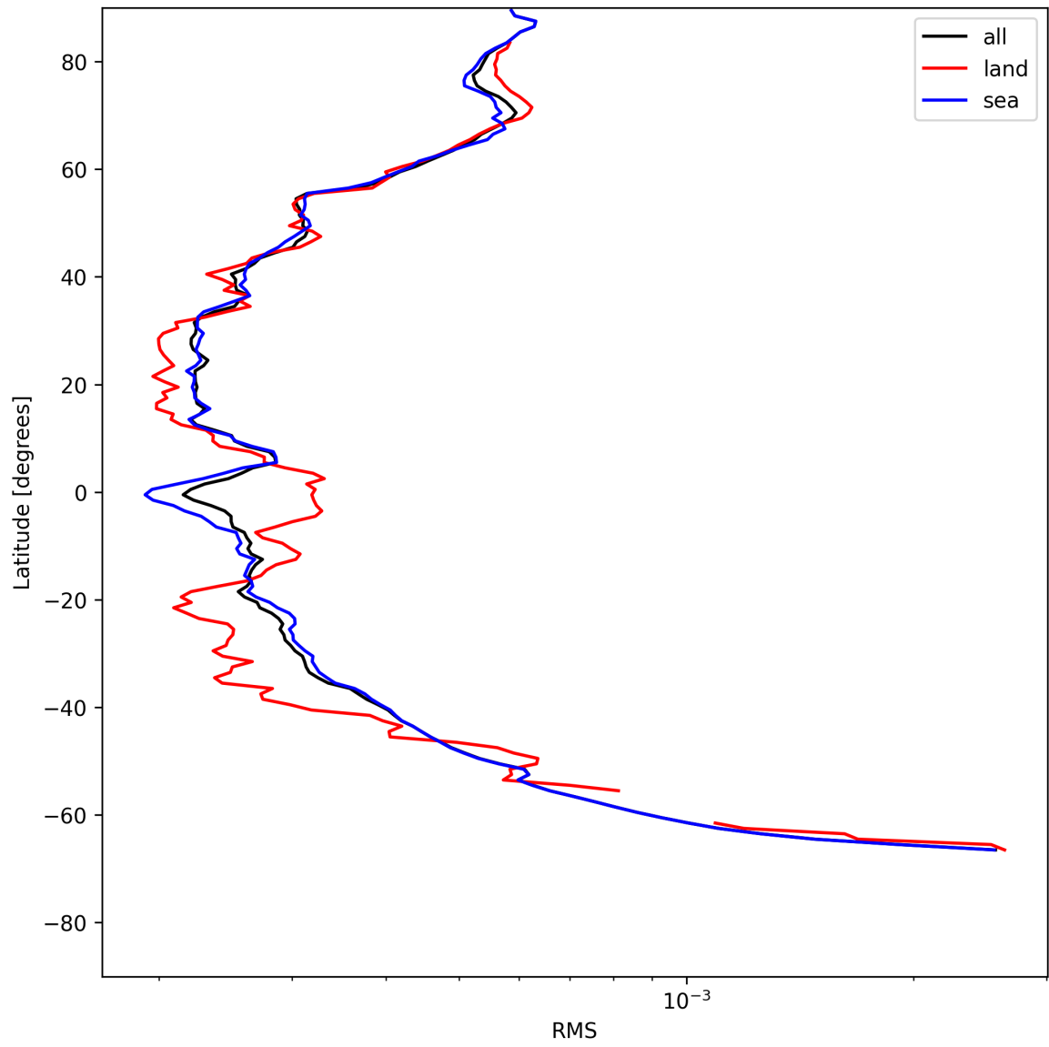
Figure 26: Zonal average of “RMS” for 2025-05-23 to 2025-05-25.
