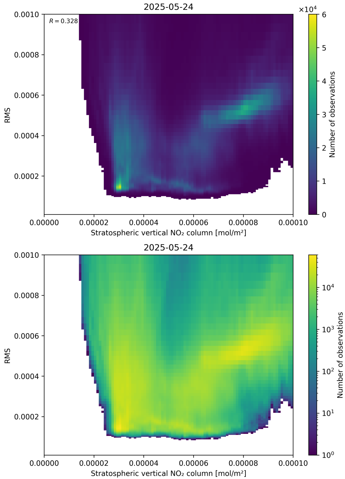
Figure 102: Scatter density plot of “Stratospheric vertical NO 2 column” against “RMS” for 2025-05-23 to 2025-05-25.
