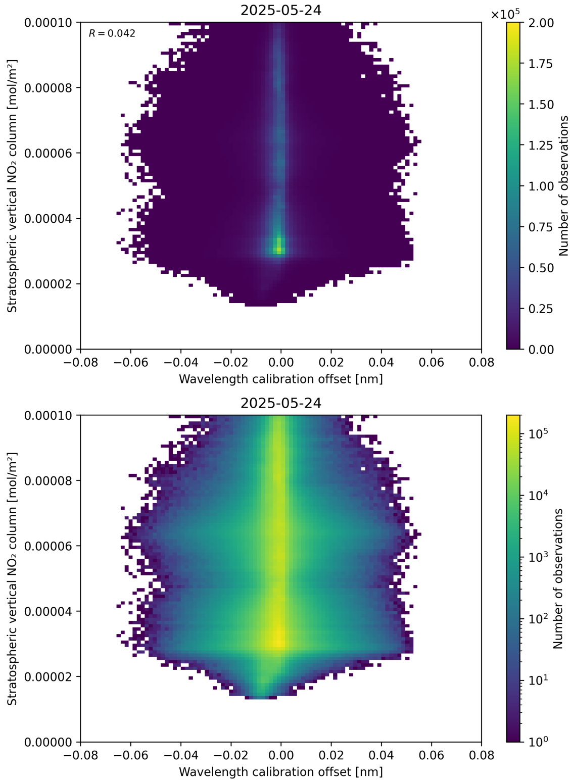
Figure 176: Scatter density plot of “Wavelength calibration offset” against “Stratospheric vertical NO 2 column” for 2025-05-23 to 2025-05-25.
