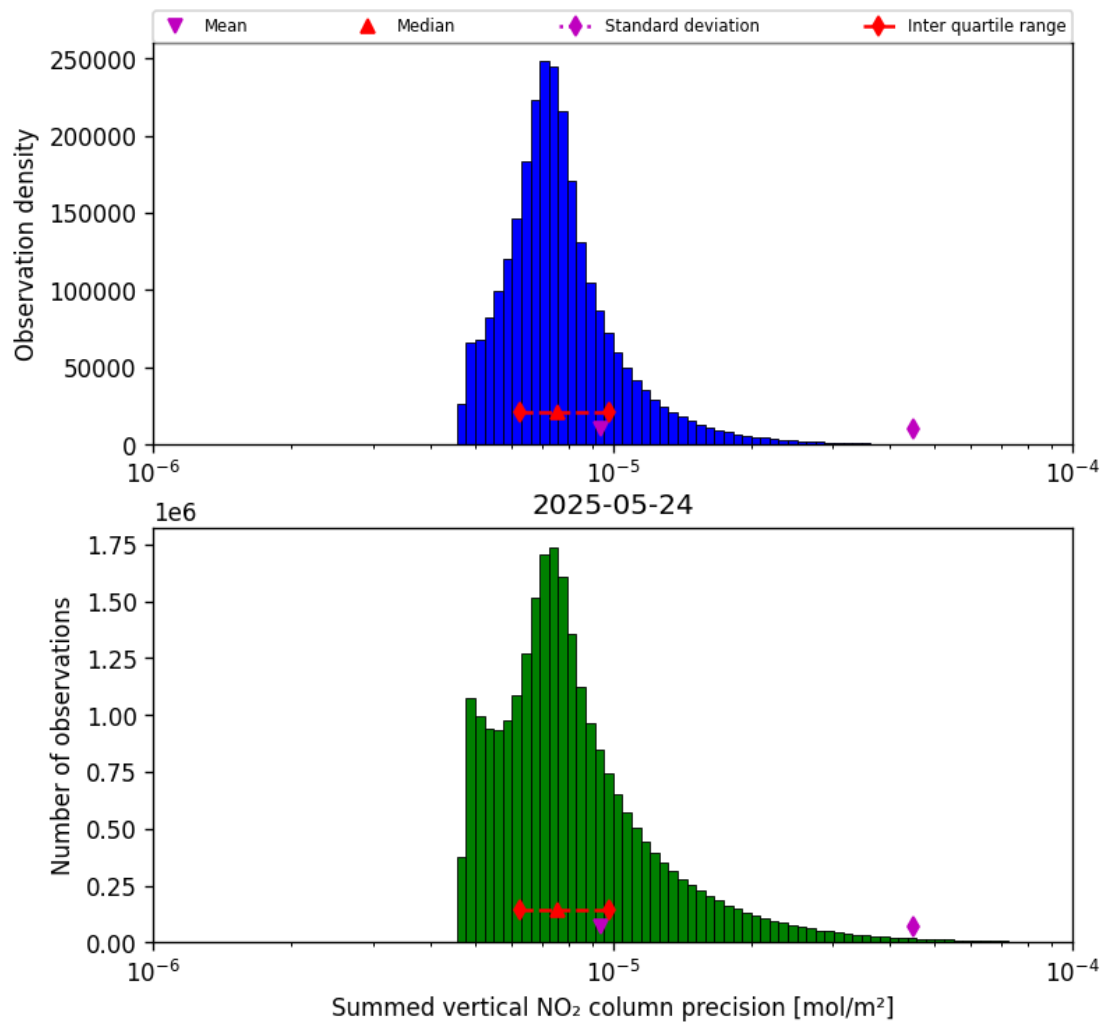
Figure 41: Histogram of “Summed vertical NO 2 column precision” for 2025-05-23 to 2025-05-25
