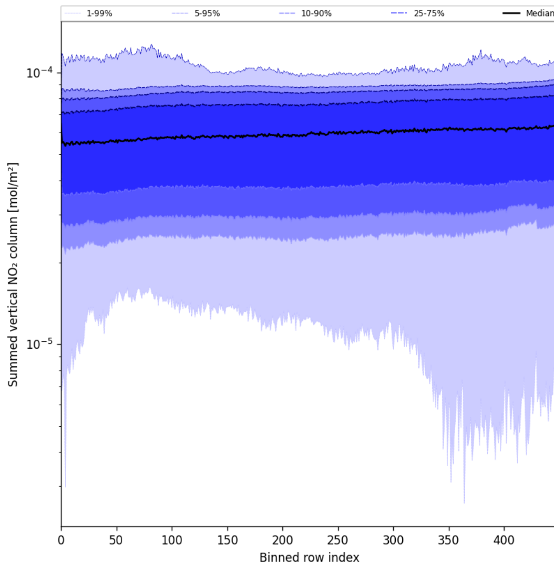
Figure 57: Along track statistics of “Summed vertical NO 2 column” for 2025-05-23 to 2025-05-25
