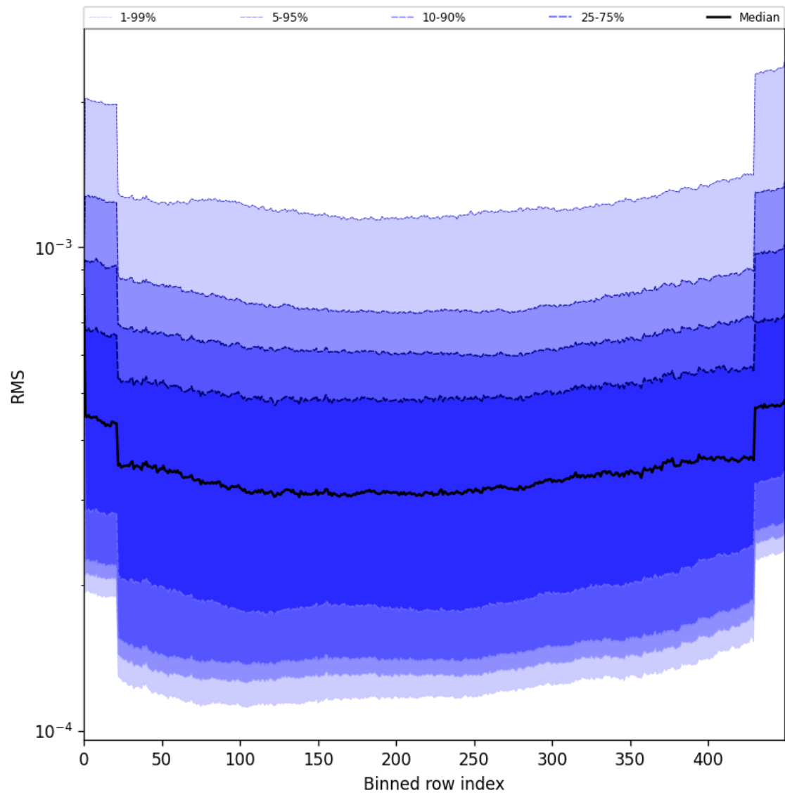
Figure 60: Along track statistics of “RMS” for 2025-05-23 to 2025-05-25
