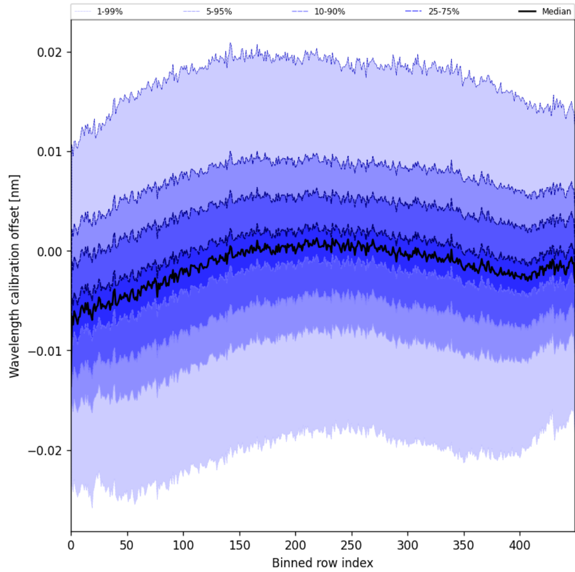
Figure 52: Along track statistics of “Wavelength calibration offset” for 2025-05-23 to 2025-05-25
