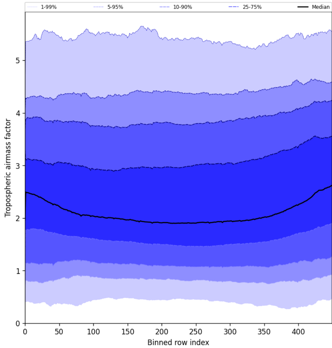
Figure 48: Along track statistics of “Tropospheric air mass factor” for 2025-05-23 to 2025-05-25
