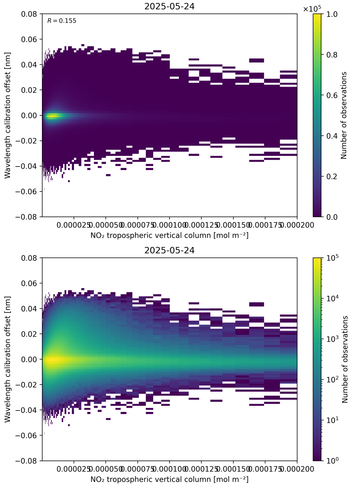
Figure 143: Scatter density plot of “NO 2 tropospheric vertical column” against “Wavelength calibration offset” for 2025-05-23 to 2025-05-25.
