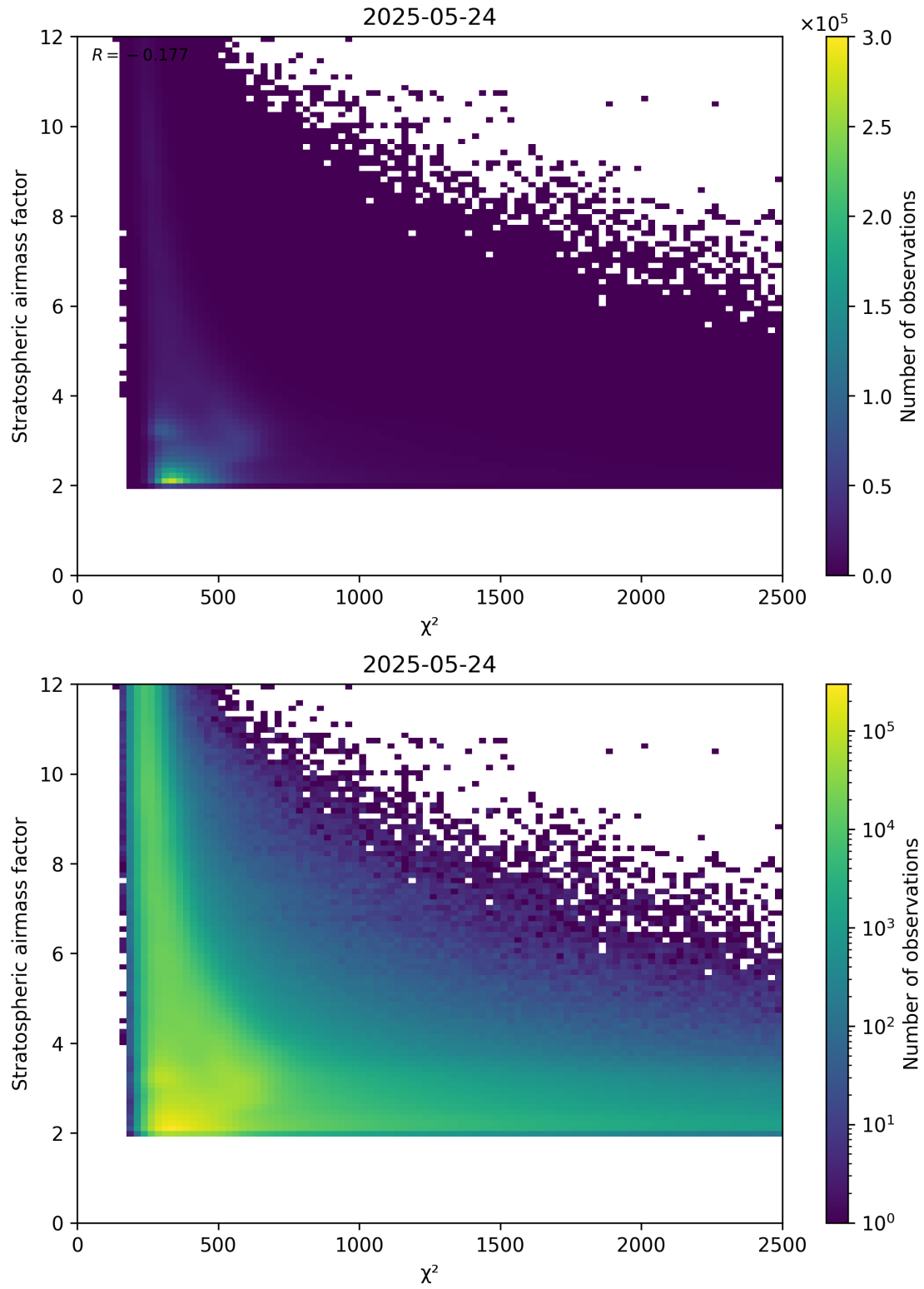
Figure 81: Scatter density plot of “ \chi^2 ” against “Stratospheric airmass factor” for 2025-05-23 to 2025-05-25.
