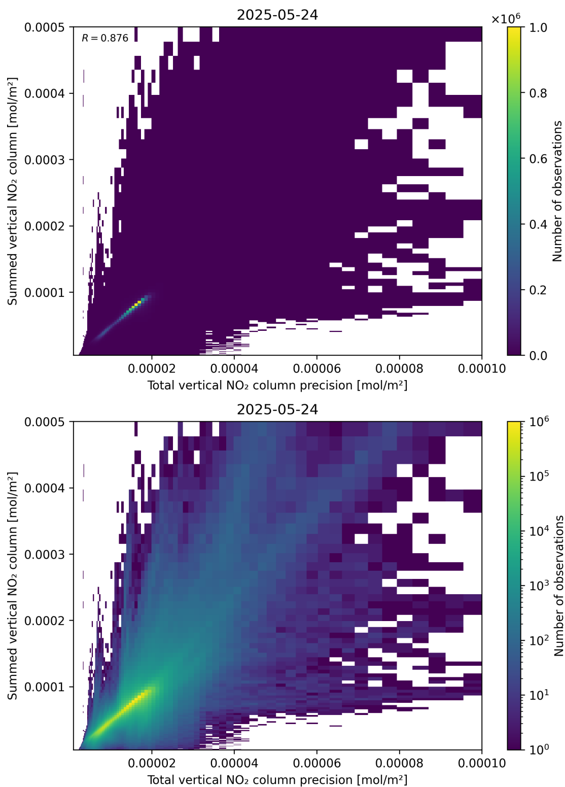
Figure 117: Scatter density plot of “Total vertical NO 2 column precision” against “Summed vertical NO 2 column” for 2025-05-23 to 2025-05-25.
