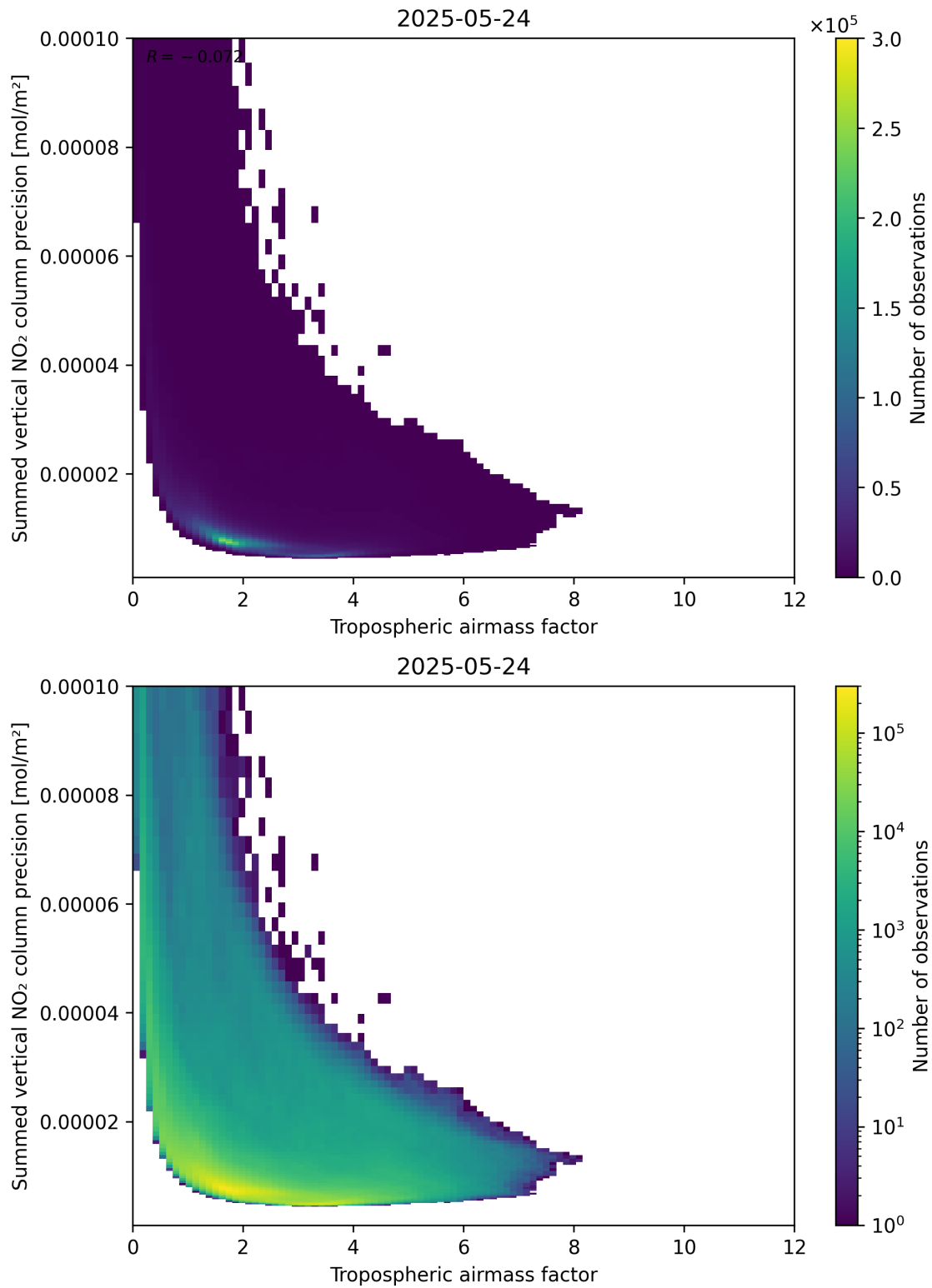
Figure 76: Scatter density plot of “Tropospheric air mass factor” against “Summed vertical NO 2 column precision” for 2025-05-23 to 2025-05-25.
