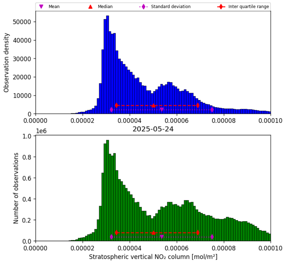
Figure 36: Histogram of “Stratospheric vertical NO 2 column” for 2025-05-23 to 2025-05-25
