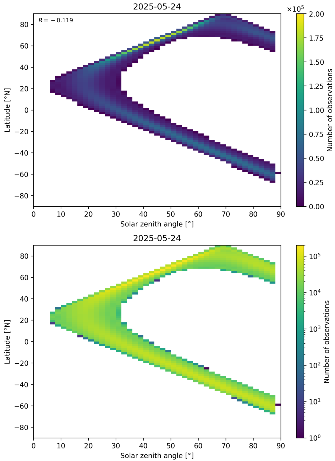
Figure 149: Scatter density plot of “Solar zenith angle” against “Latitude” for 2025-05-23 to 2025-05-25.
