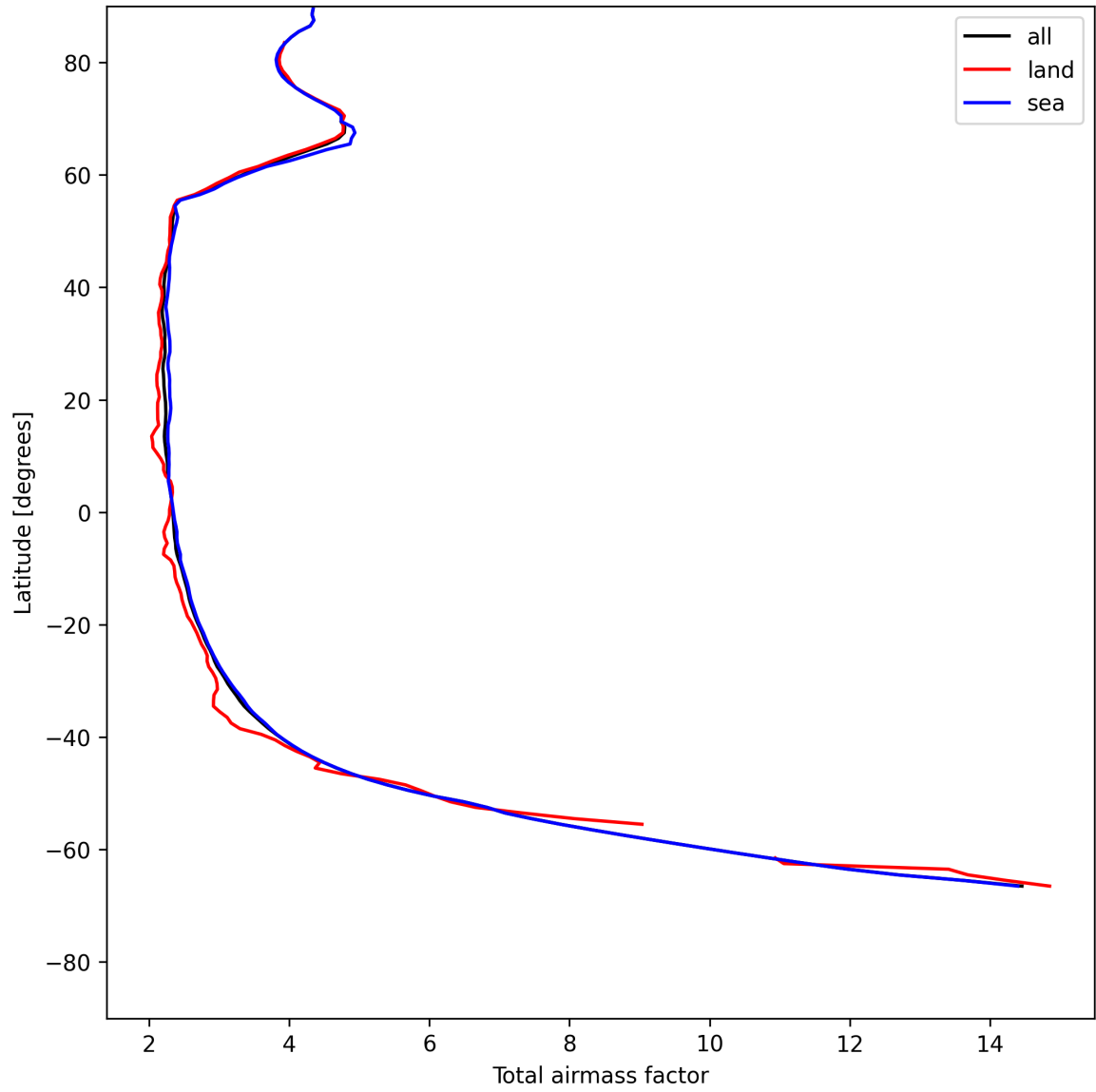
Figure 15: Zonal average of “Total airmass factor” for 2025-05-23 to 2025-05-25.
