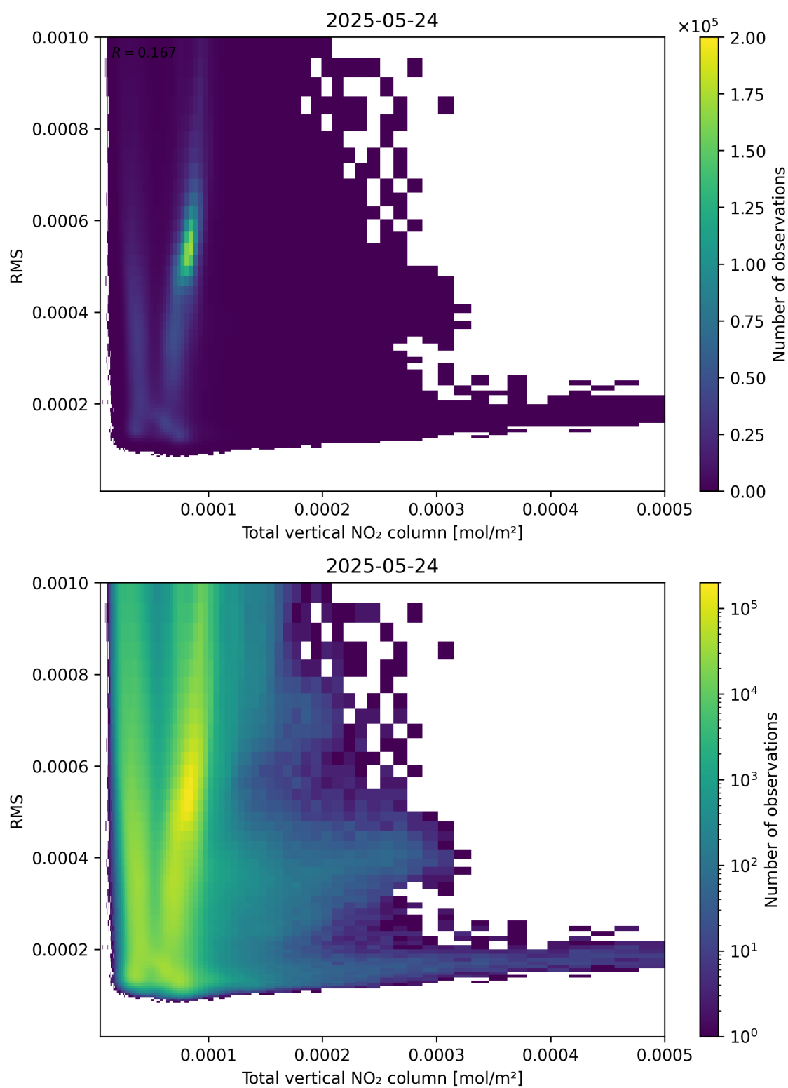
Figure 120: Scatter density plot of “Total vertical NO 2 column” against “RMS” for 2025-05-23 to 2025-05-25.
