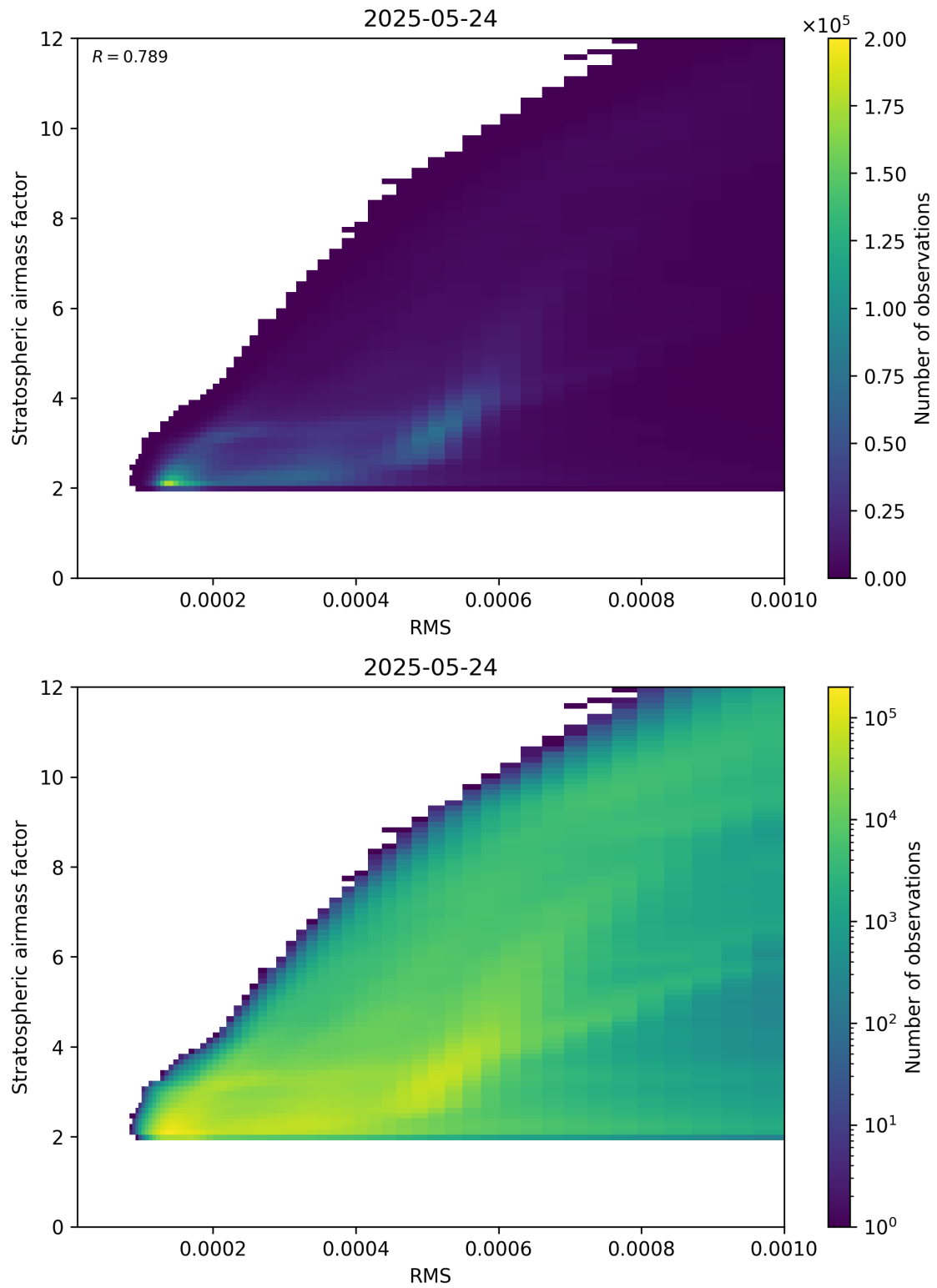
Figure 144: Scatter density plot of “RMS” against “Stratospheric airmass factor” for 2025-05-23 to 2025-05-25.
