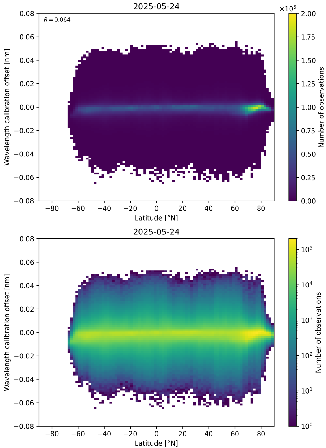
Figure 95: Scatter density plot of “Latitude” against “Wavelength calibration offset” for 2025-05-23 to 2025-05-25.
