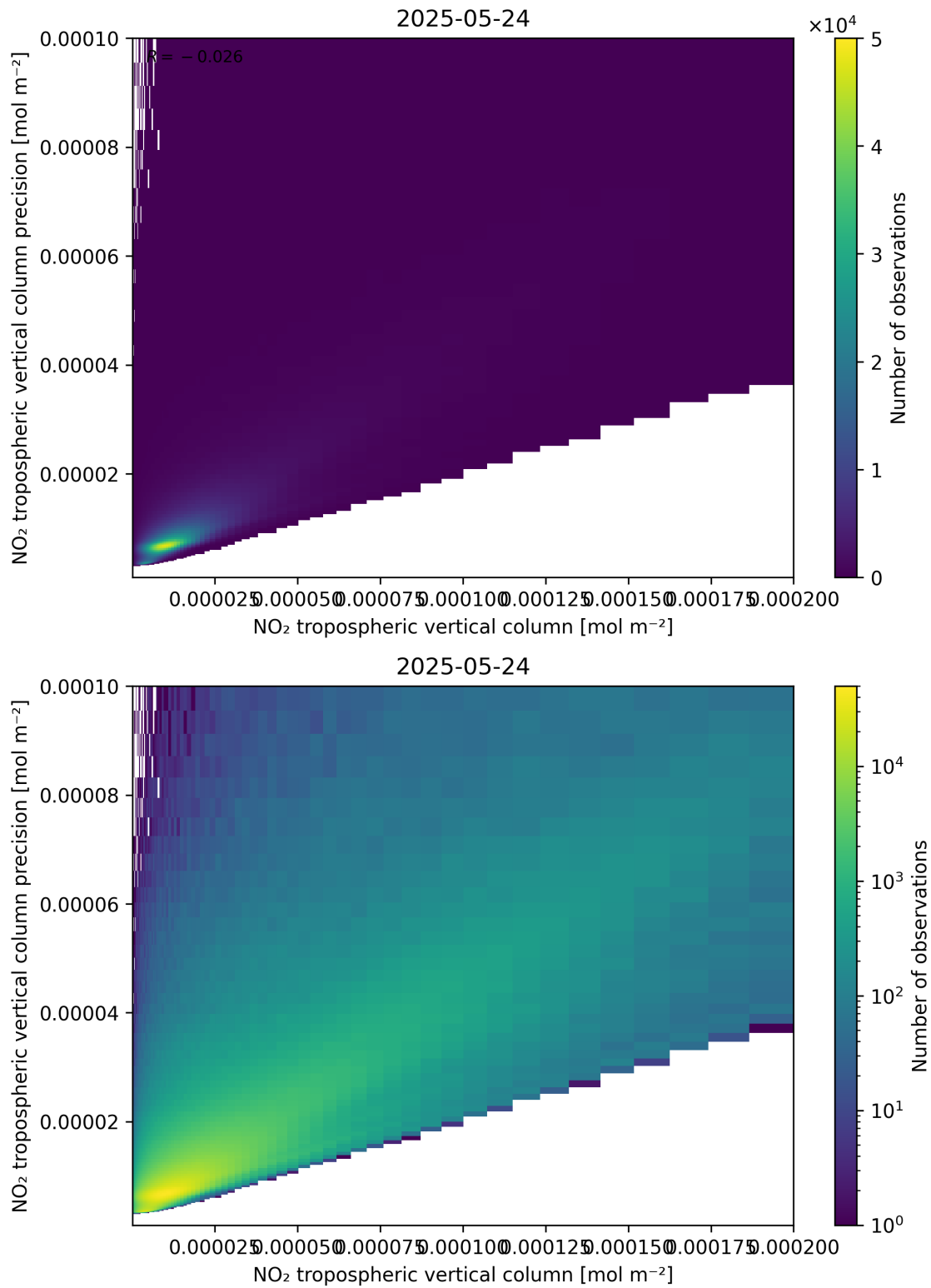
Figure 130: Scatter density plot of “NO 2 tropospheric vertical column” against “NO 2 tropospheric vertical column precision” for 2025-05-23 to 2025-05-25.
