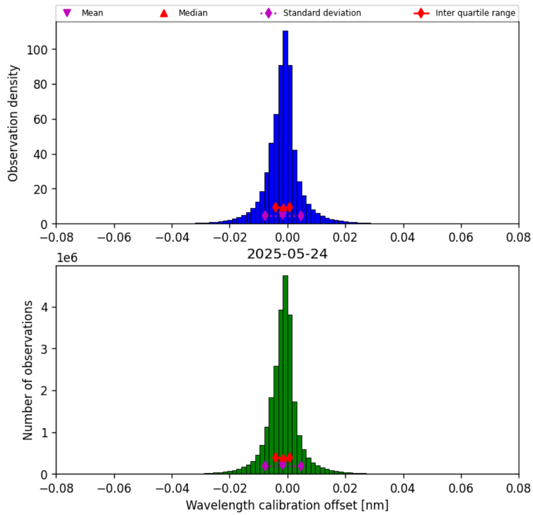
Figure 35: Histogram of “Wavelength calibration offset” for 2025-05-23 to 2025-05-25
