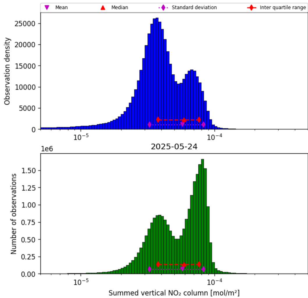
Figure 40: Histogram of “Summed vertical NO 2 column” for 2025-05-23 to 2025-05-25
