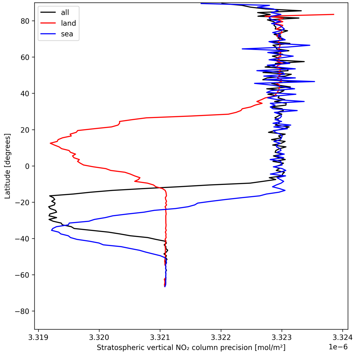
Figure 20: Zonal average of “Stratospheric vertical NO 2 column precision” for 2025-05-23 to 2025-05-25.
