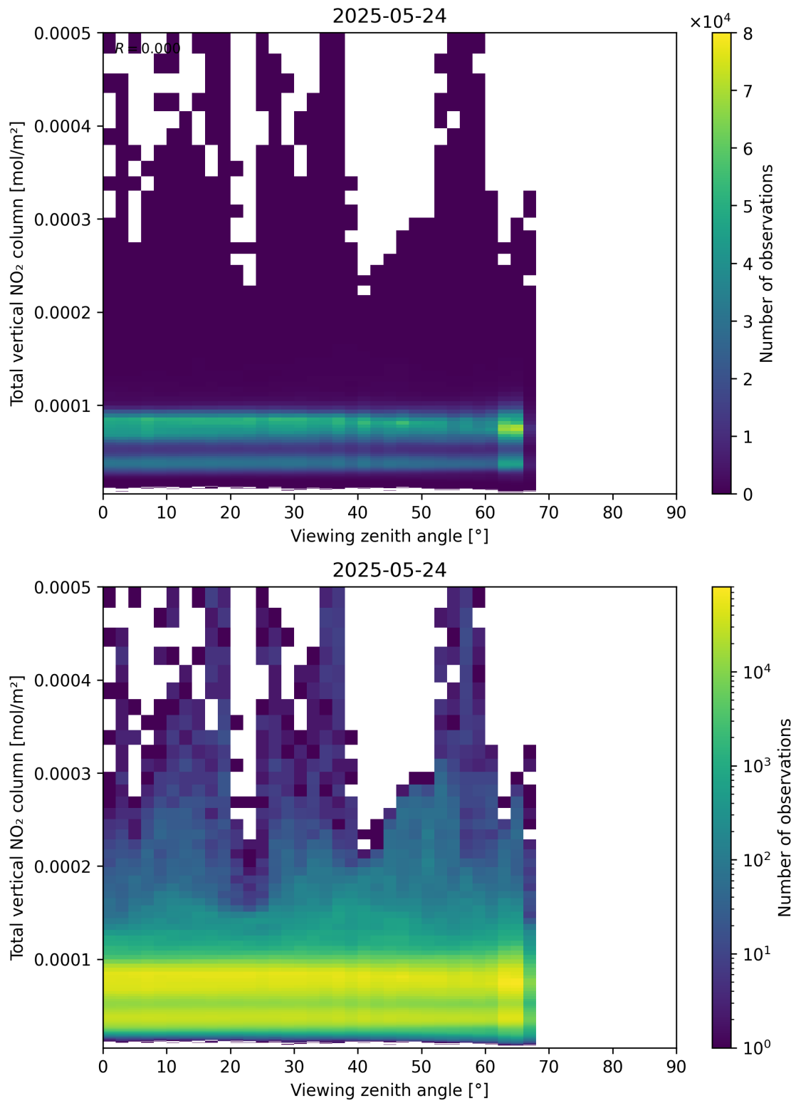
Figure 167: Scatter density plot of “Viewing zenith angle” against “Total vertical NO 2 column” for 2025-05-23 to 2025-05-25.
