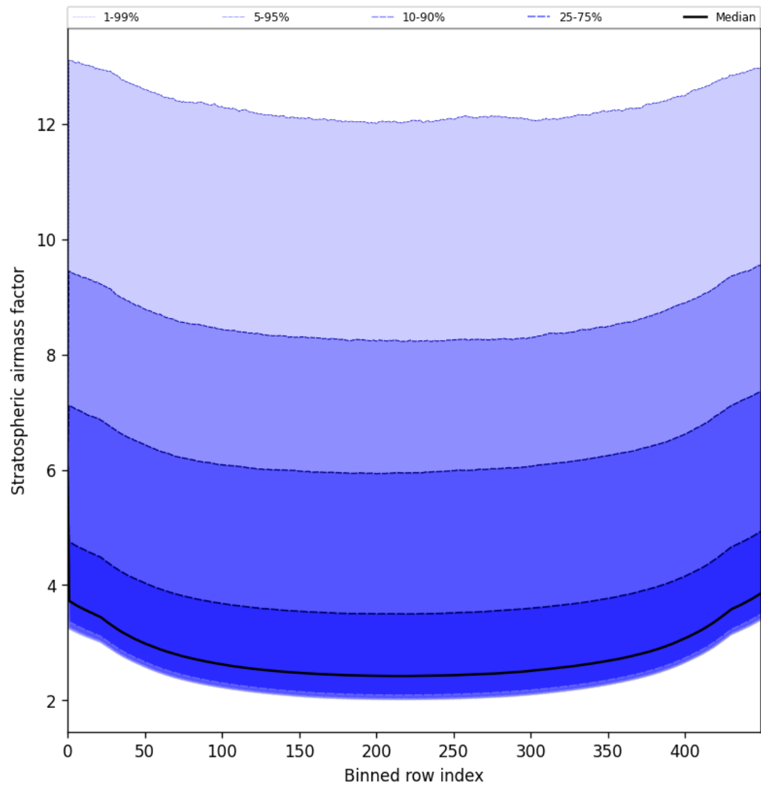
Figure 61: Along track statistics of “Stratospheric airmass factor” for 2025-05-23 to 2025-05-25
