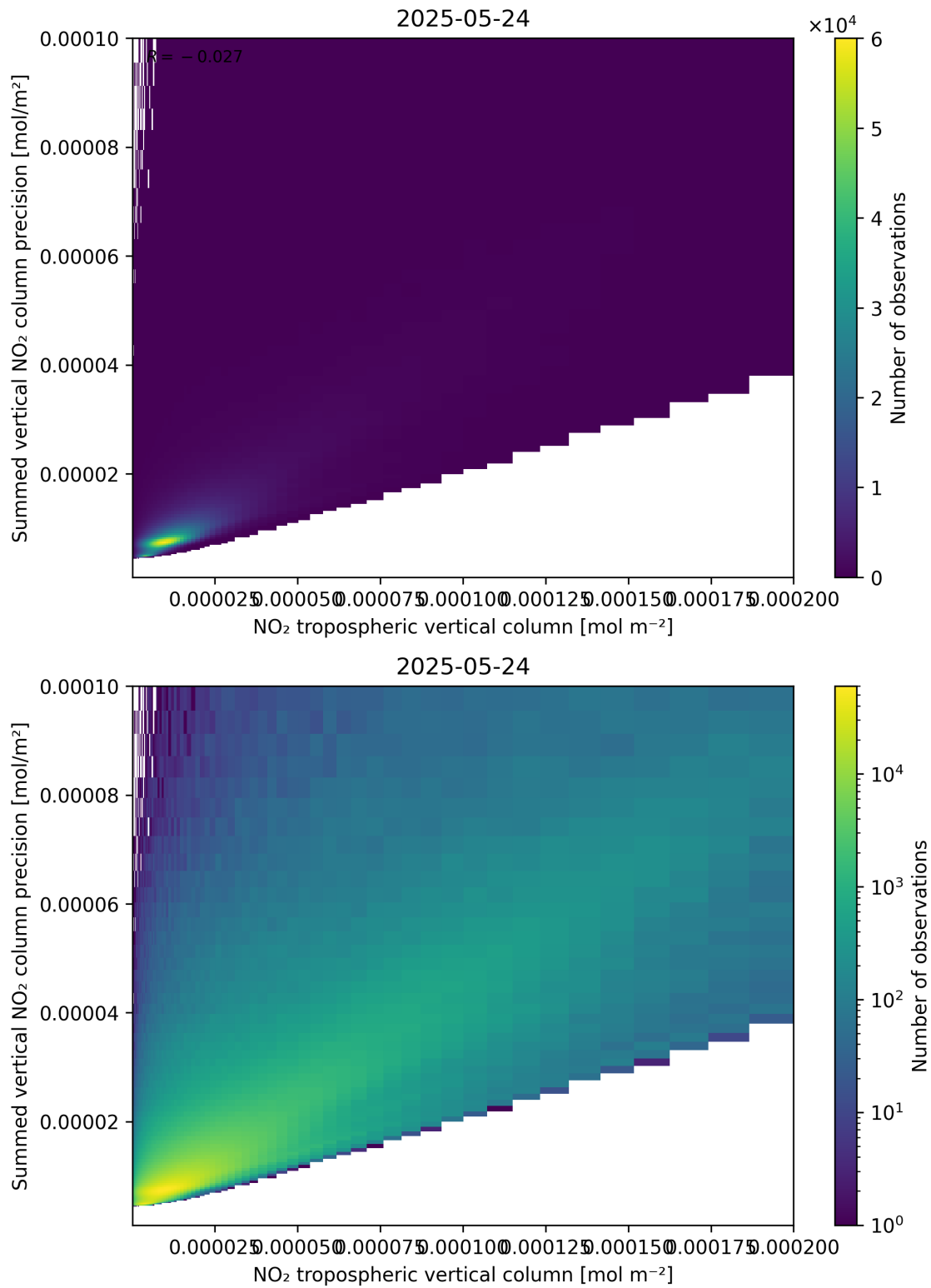
Figure 127: Scatter density plot of “NO 2 tropospheric vertical column” against “Summed vertical NO 2 column precision” for 2025-05-23 to 2025-05-25.
