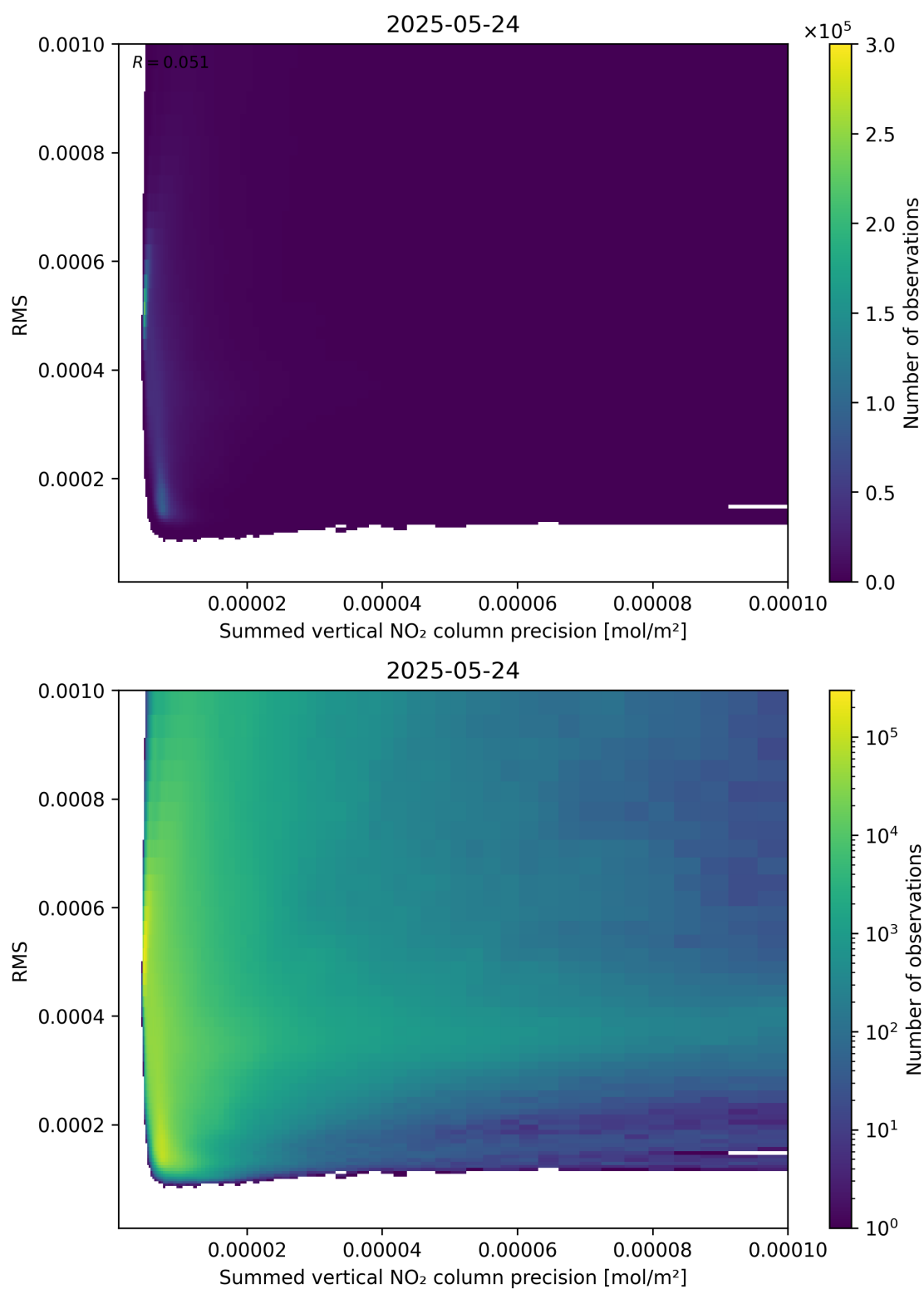
Figure 108: Scatter density plot of “Summed vertical NO 2 column precision” against “RMS” for 2025-05-23 to 2025-05-25.
