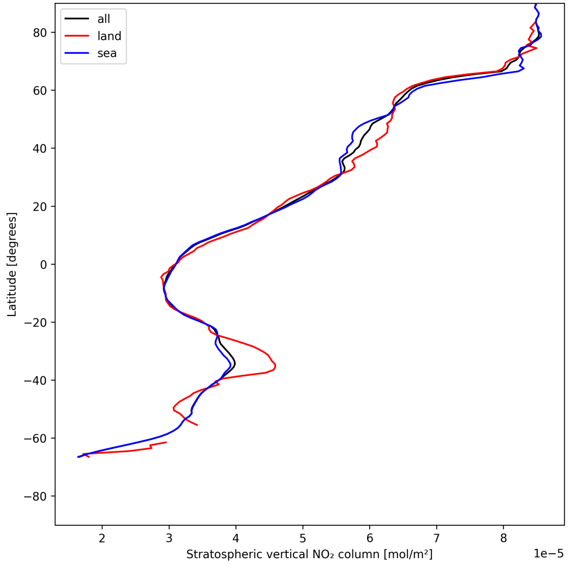
Figure 19: Zonal average of “Stratospheric vertical NO 2 column” for 2025-05-23 to 2025-05-25.
