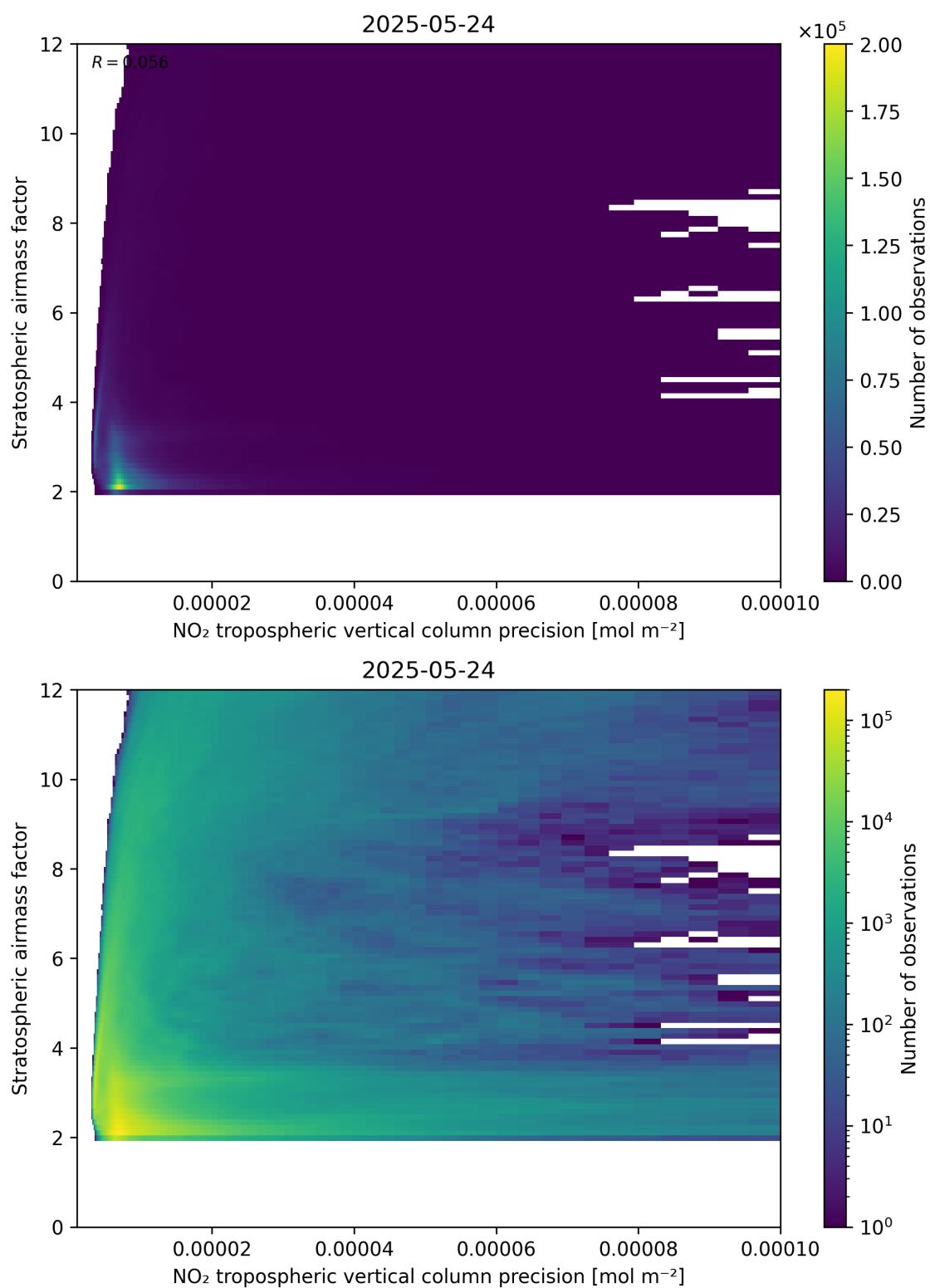
Figure 131: Scatter density plot of “NO 2 tropospheric vertical column precision” against “Stratospheric airmass factor” for 2025-05-23 to 2025-05-25.
