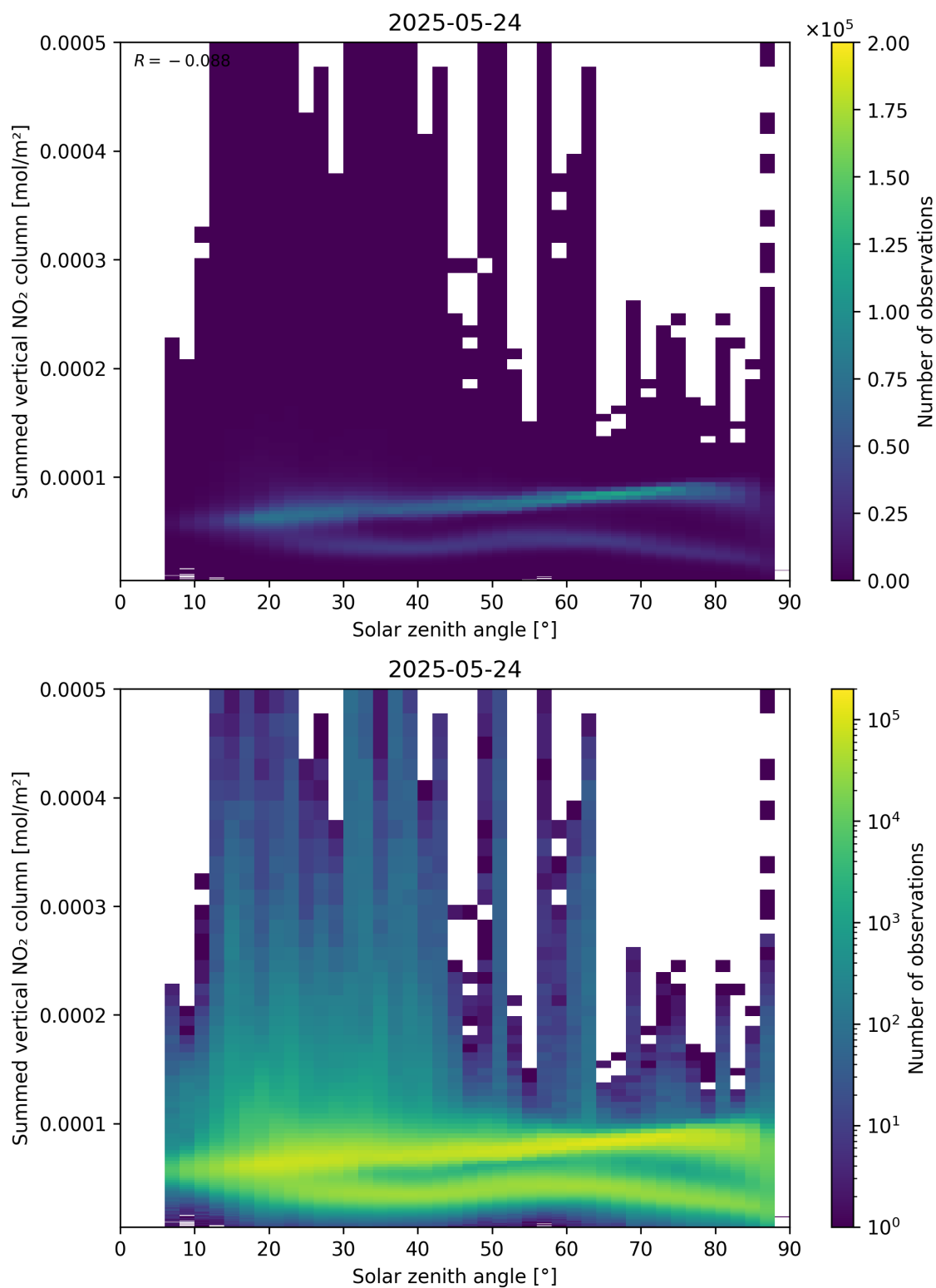
Figure 151: Scatter density plot of “Solar zenith angle” against “Summed vertical NO 2 column” for 2025-05-23 to 2025-05-25.
