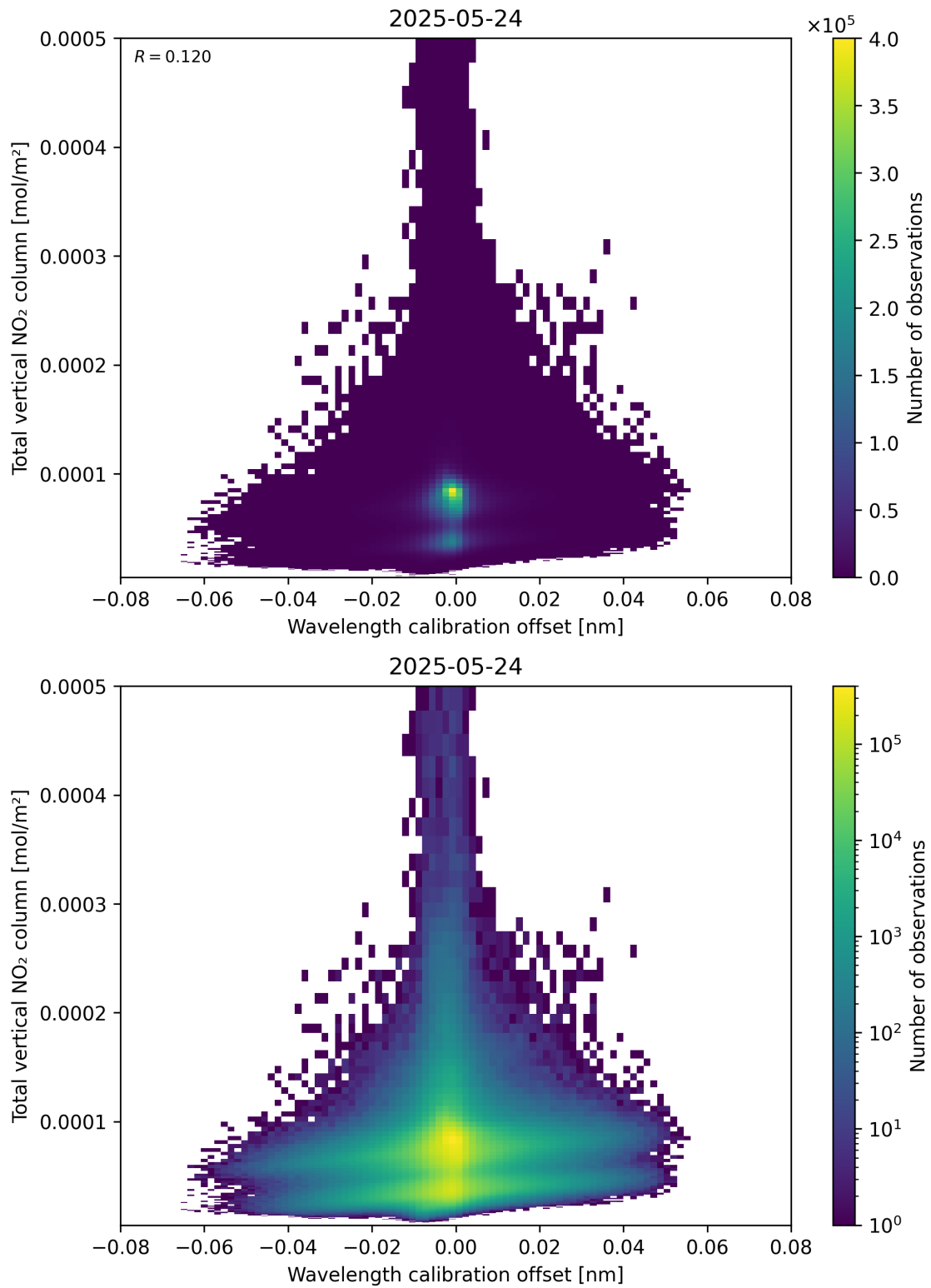
Figure 179: Scatter density plot of “Wavelength calibration offset” against “Total vertical NO 2 column” for 2025-05-23 to 2025-05-25.
