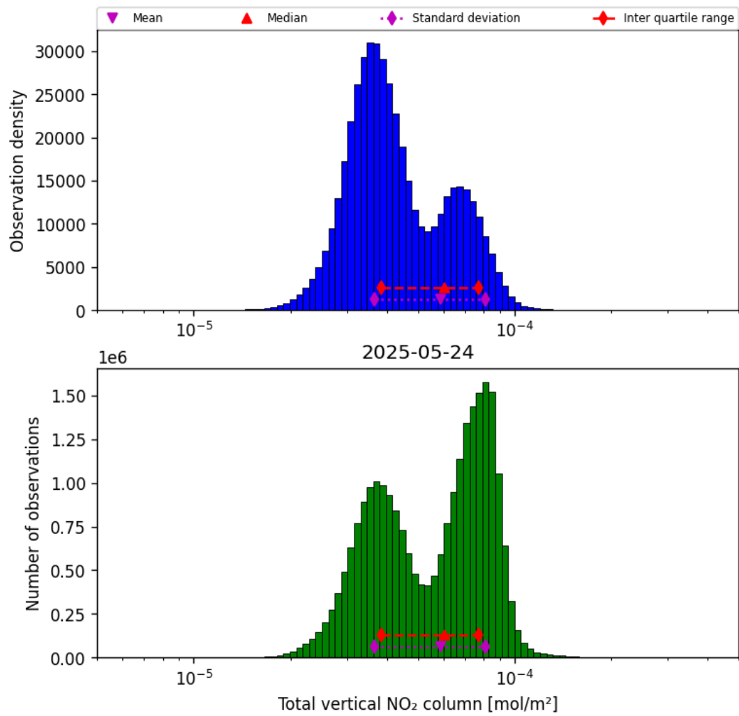
Figure 38: Histogram of “Total vertical NO 2 column” for 2025-05-23 to 2025-05-25
