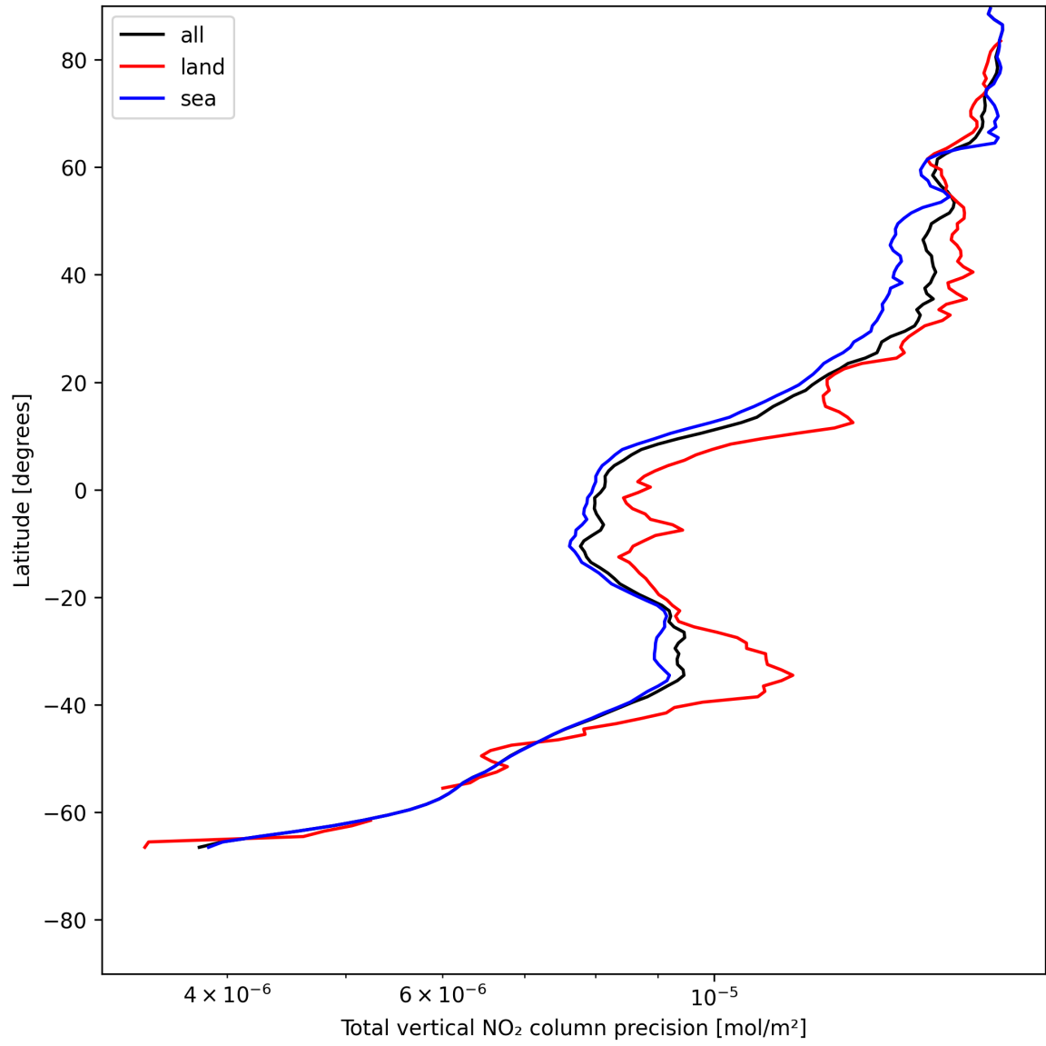
Figure 22: Zonal average of “Total vertical NO 2 column precision” for 2025-05-23 to 2025-05-25.
