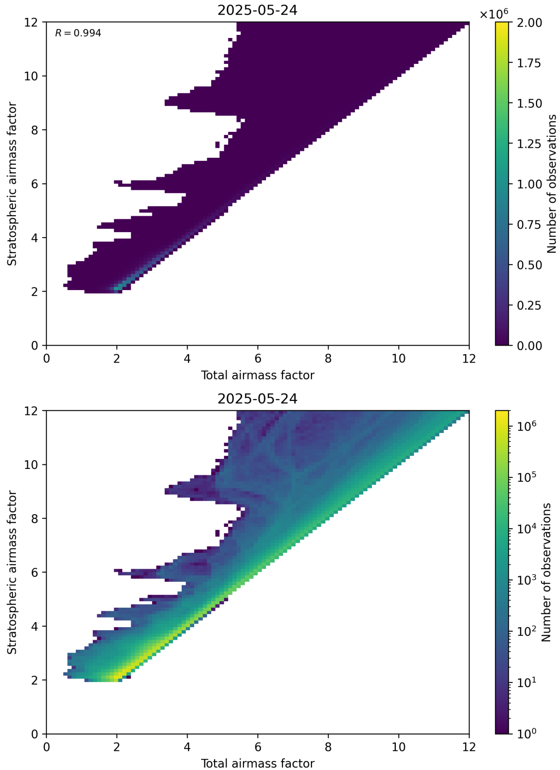
Figure 62: Scatter density plot of “Total airmass factor” against “Stratospheric airmass factor” for 2025-05-23 to 2025-05-25.
