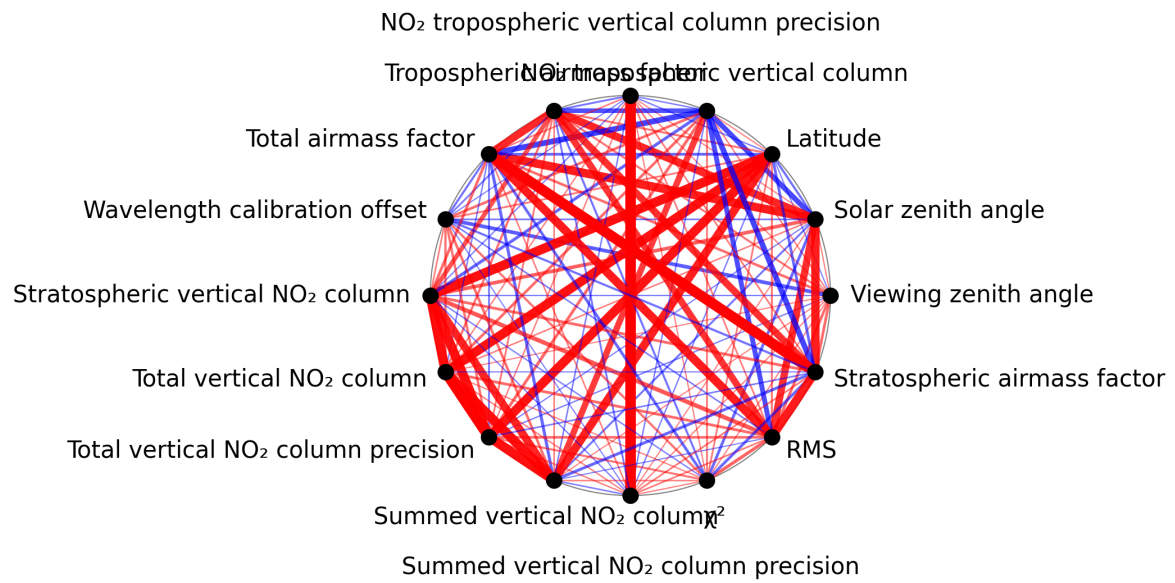
Figure 1: Map of correlation graph for 2025-05-23 to 2025-05-25.
