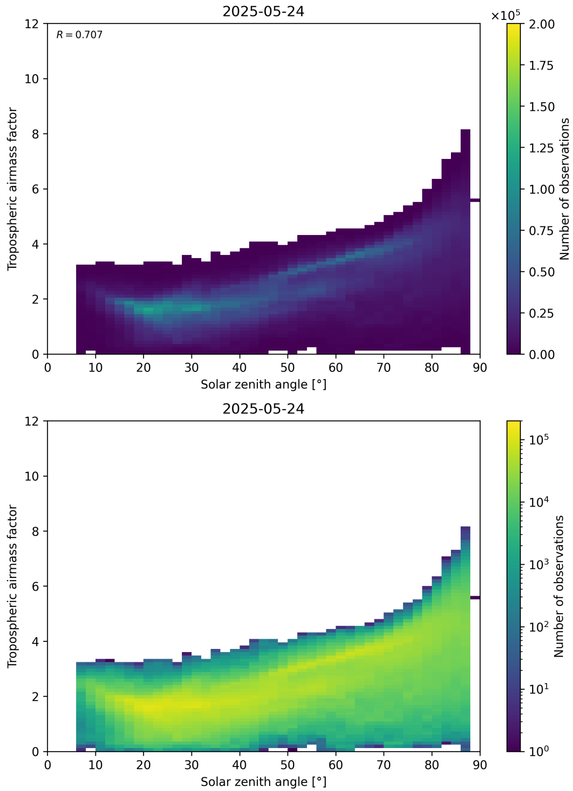
Figure 147: Scatter density plot of “Solar zenith angle” against “Tropospheric airmass factor” for 2025-05-23 to 2025-05-25.
