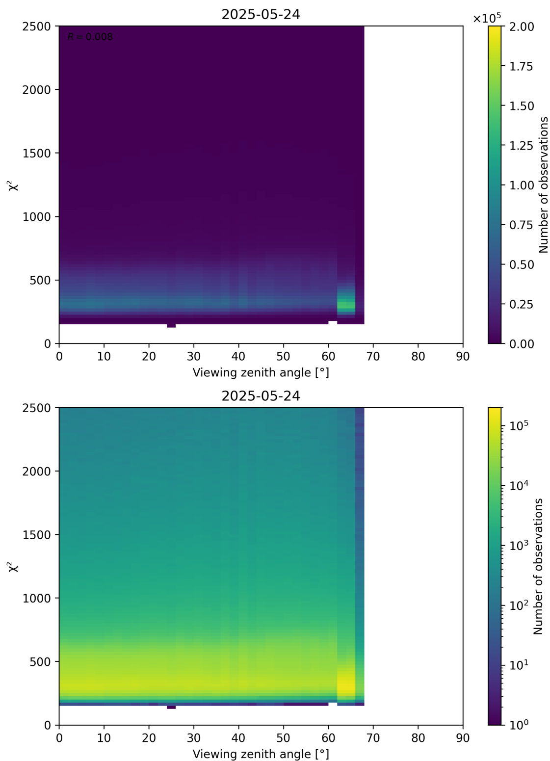
Figure 162: Scatter density plot of “Viewing zenith angle” against “ \chi^2 ” for 2025-05-23 to 2025-05-25.
