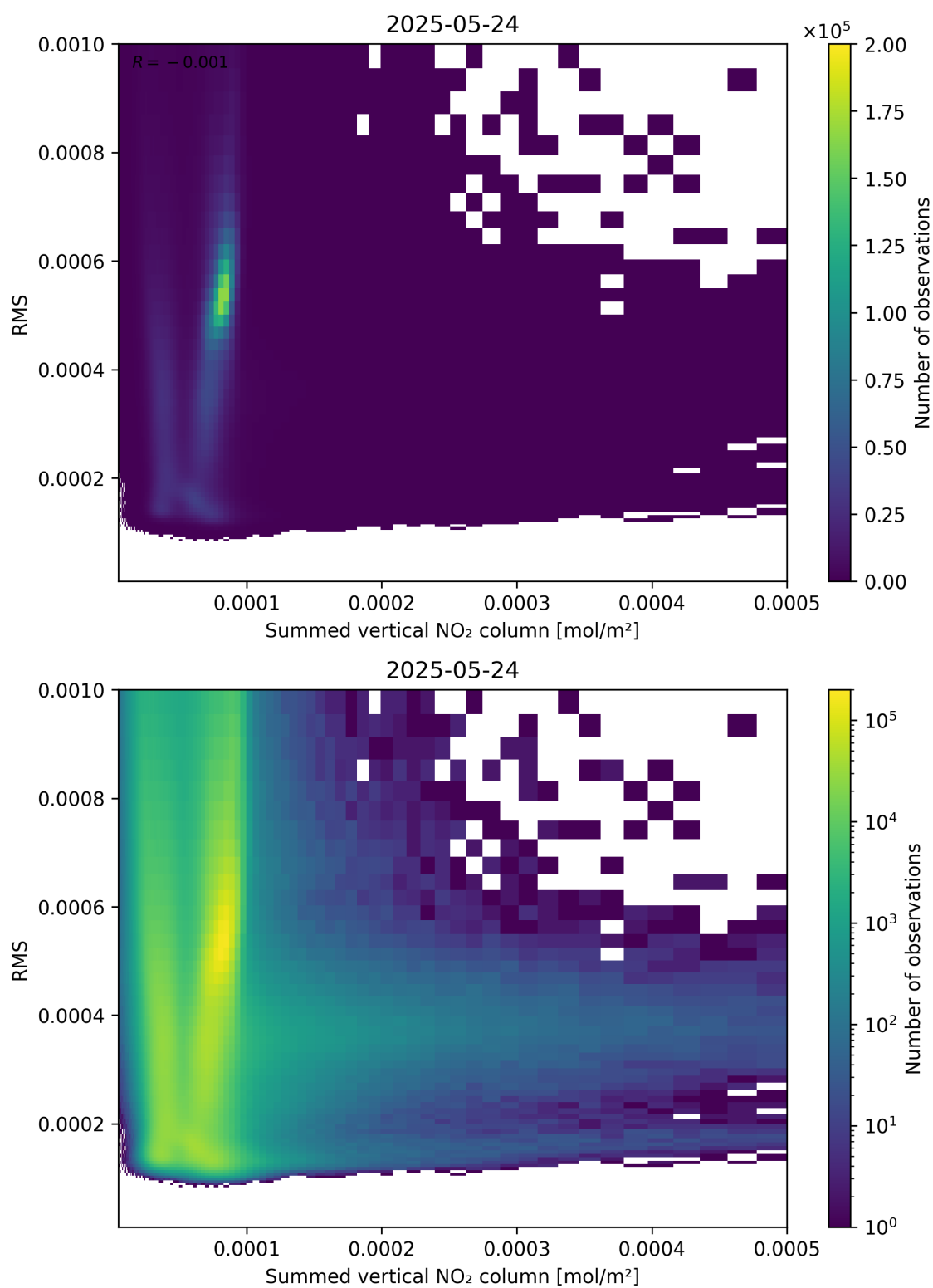
Figure 109: Scatter density plot of “Summed vertical NO 2 column” against “RMS” for 2025-05-23 to 2025-05-25.
