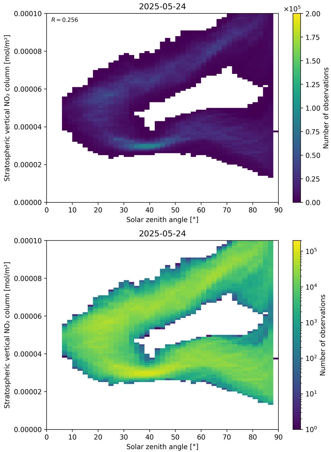
Figure 150: Scatter density plot of “Solar zenith angle” against “Stratospheric vertical NO 2 column” for 2025-05-23 to 2025-05-25.
