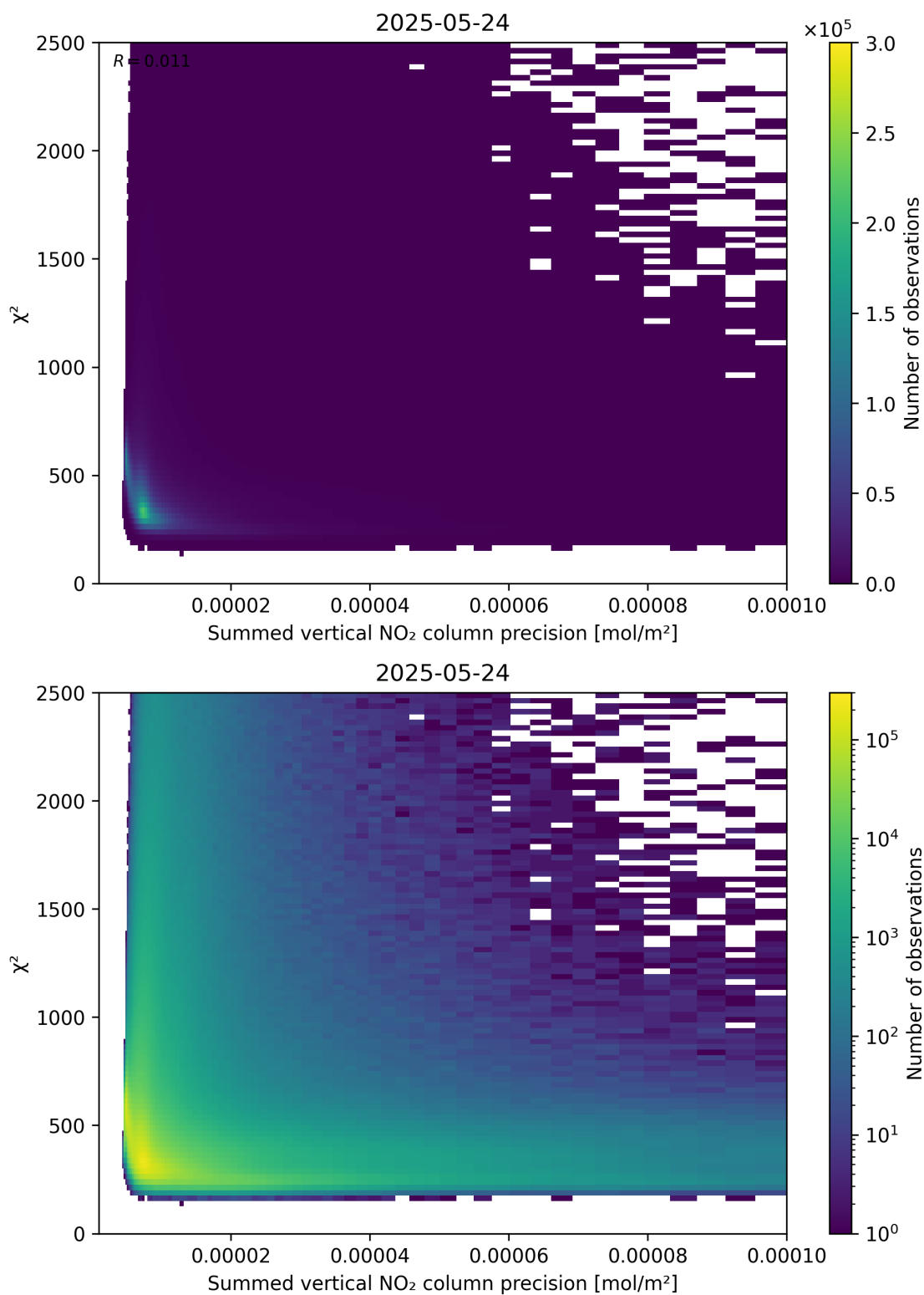
Figure 107: Scatter density plot of “Summed vertical NO 2 column precision” against “ \chi^2 ” for 2025-05-23 to 2025-05-25.
