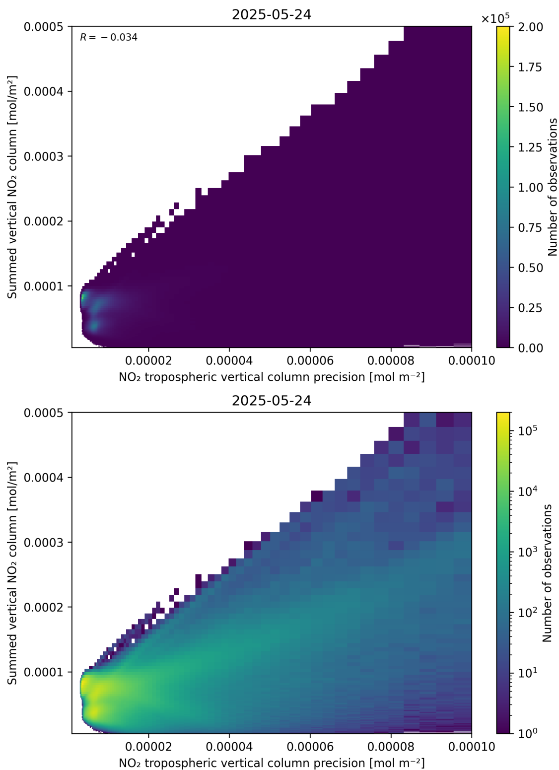
Figure 136: Scatter density plot of “NO 2 tropospheric vertical column precision” against “Summed vertical NO 2 column” for 2025-05-23 to 2025-05-25.
