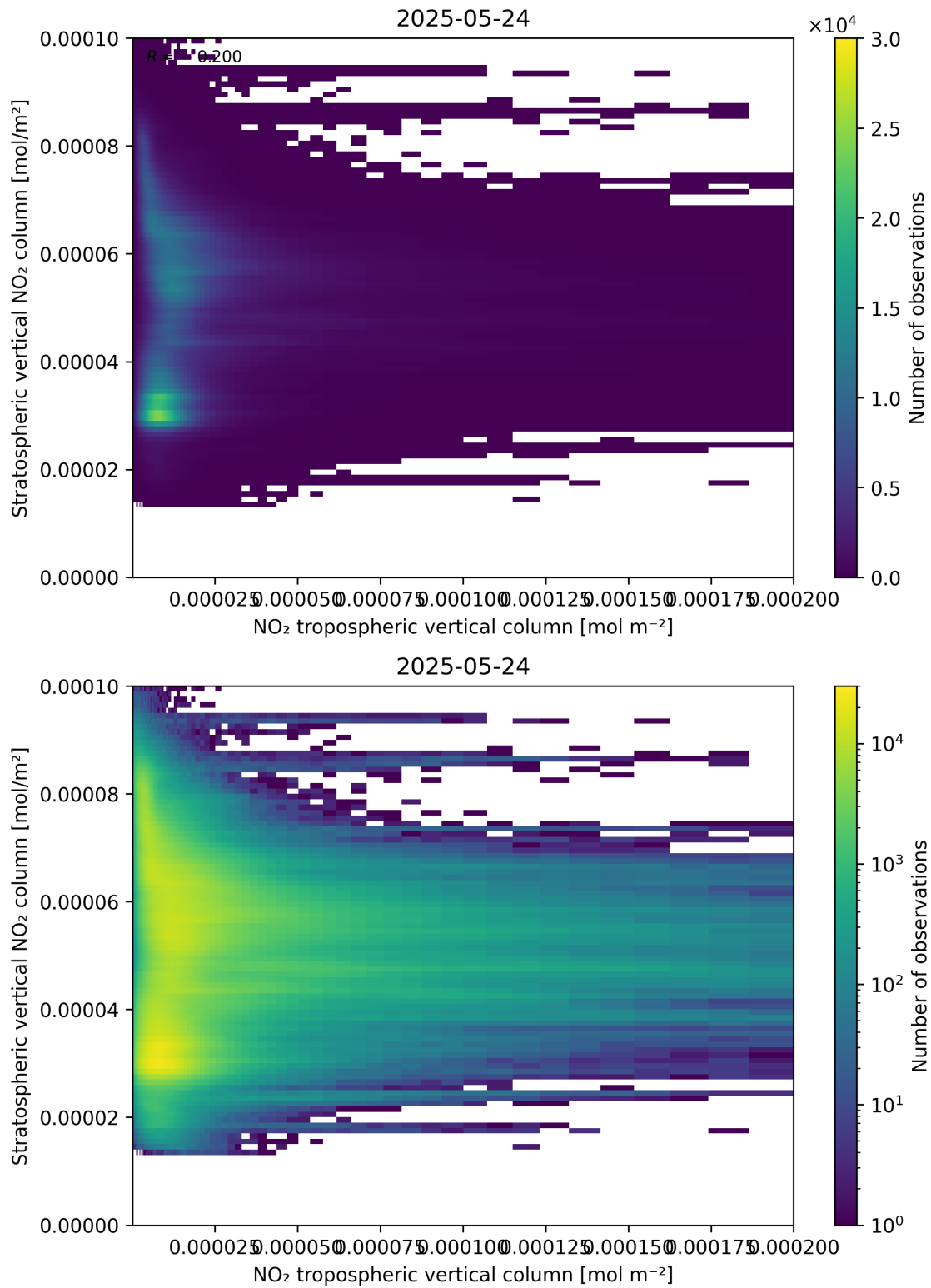
Figure 125: Scatter density plot of “NO 2 tropospheric vertical column” against “Stratospheric vertical NO 2 column” for 2025-05-23 to 2025-05-25.
