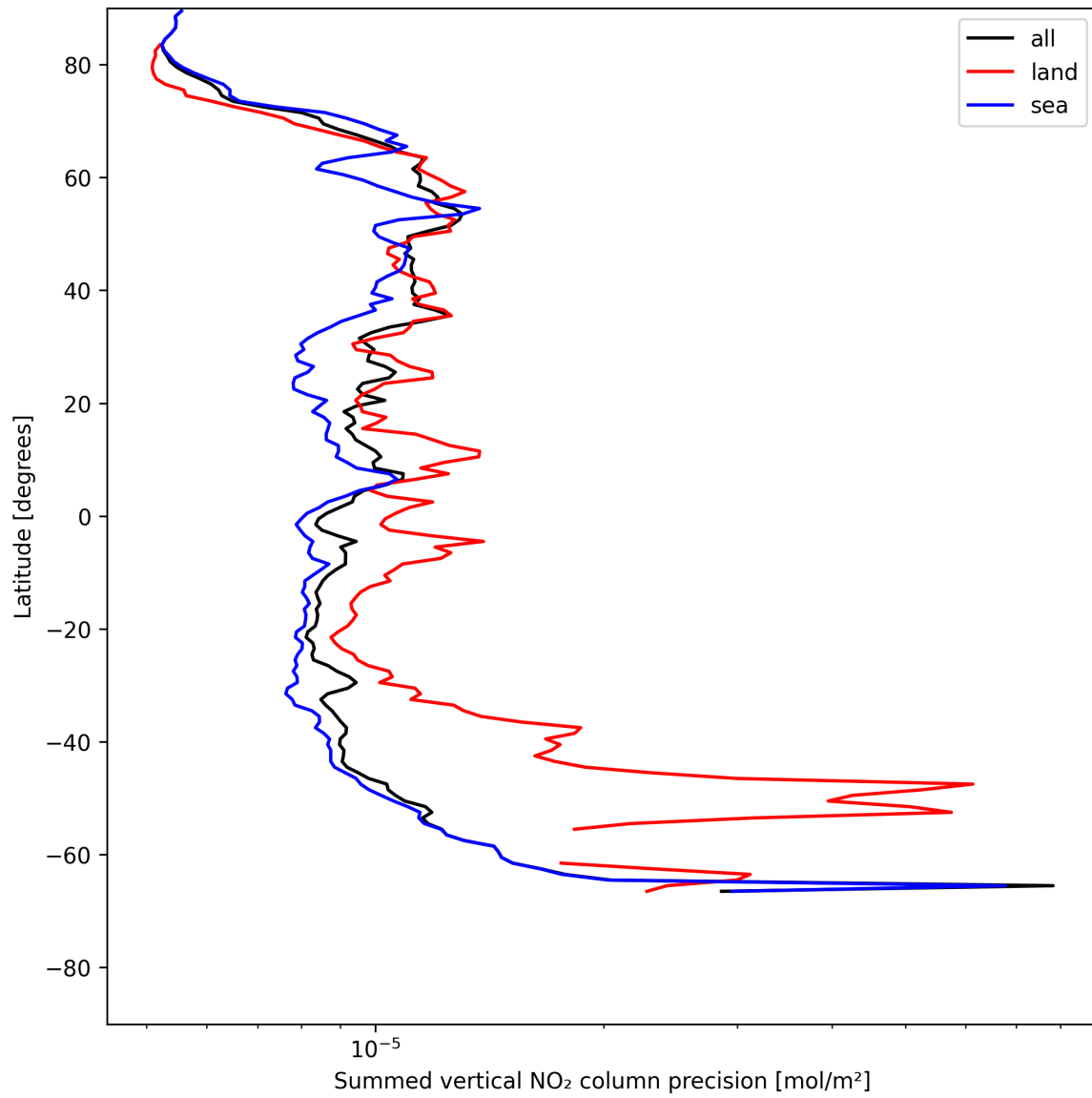
Figure 24: Zonal average of “Summed vertical NO 2 column precision” for 2025-05-23 to 2025-05-25.
