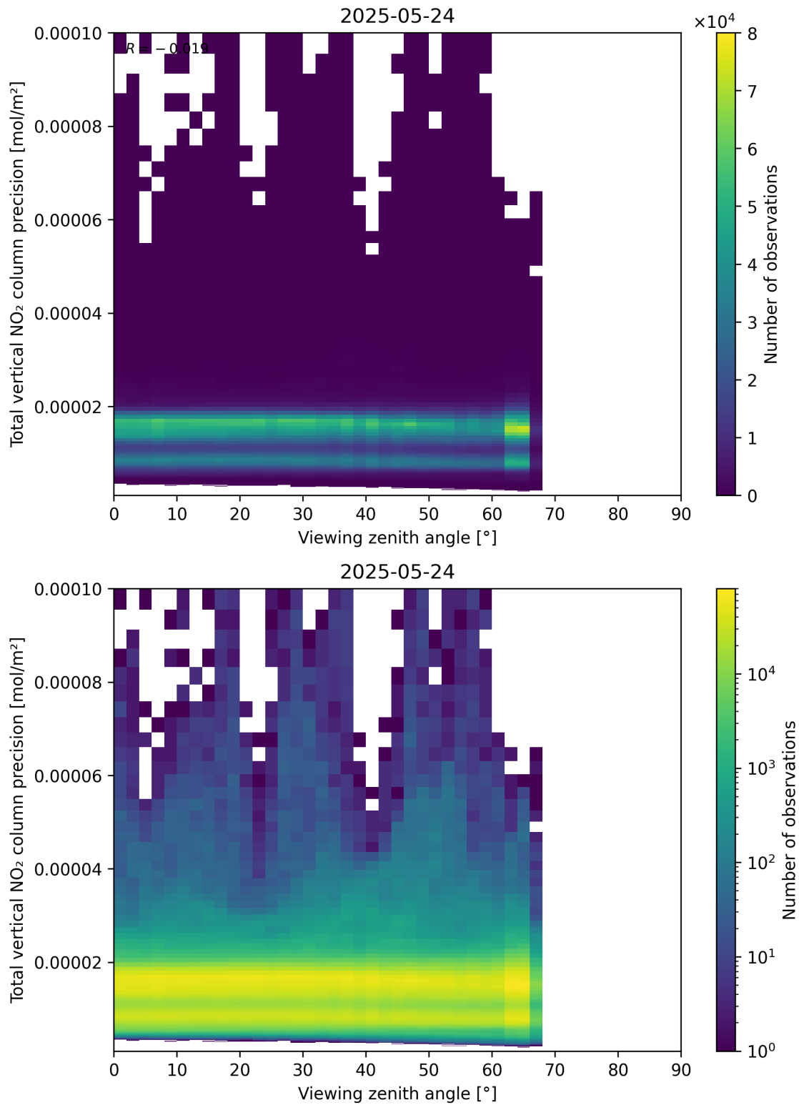
Figure 168: Scatter density plot of “Viewing zenith angle” against “Total vertical NO 2 column precision” for 2025-05-23 to 2025-05-25.
