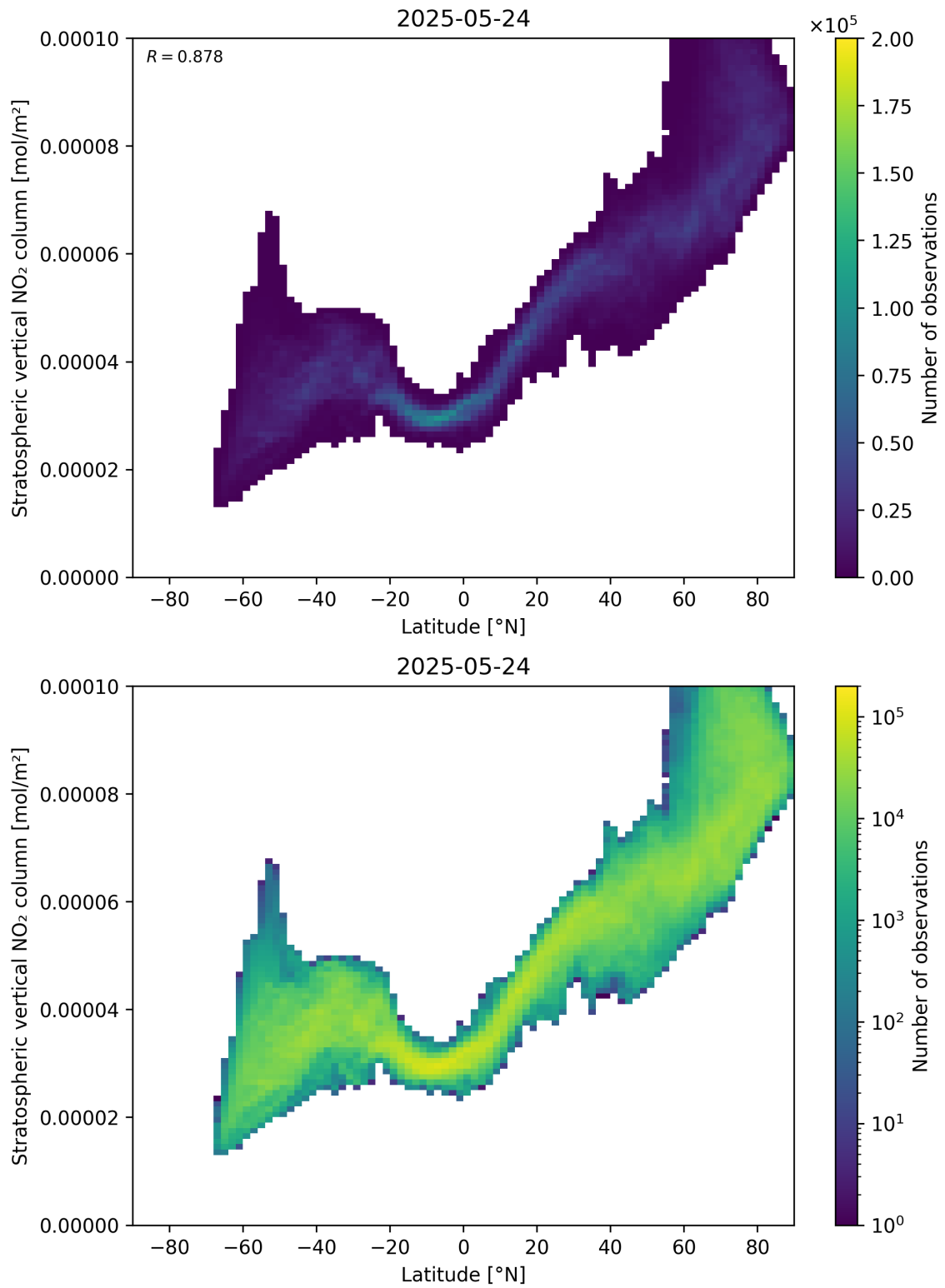
Figure 87: Scatter density plot of “Latitude” against “Stratospheric vertical NO 2 column” for 2025-05-23 to 2025-05-25.
