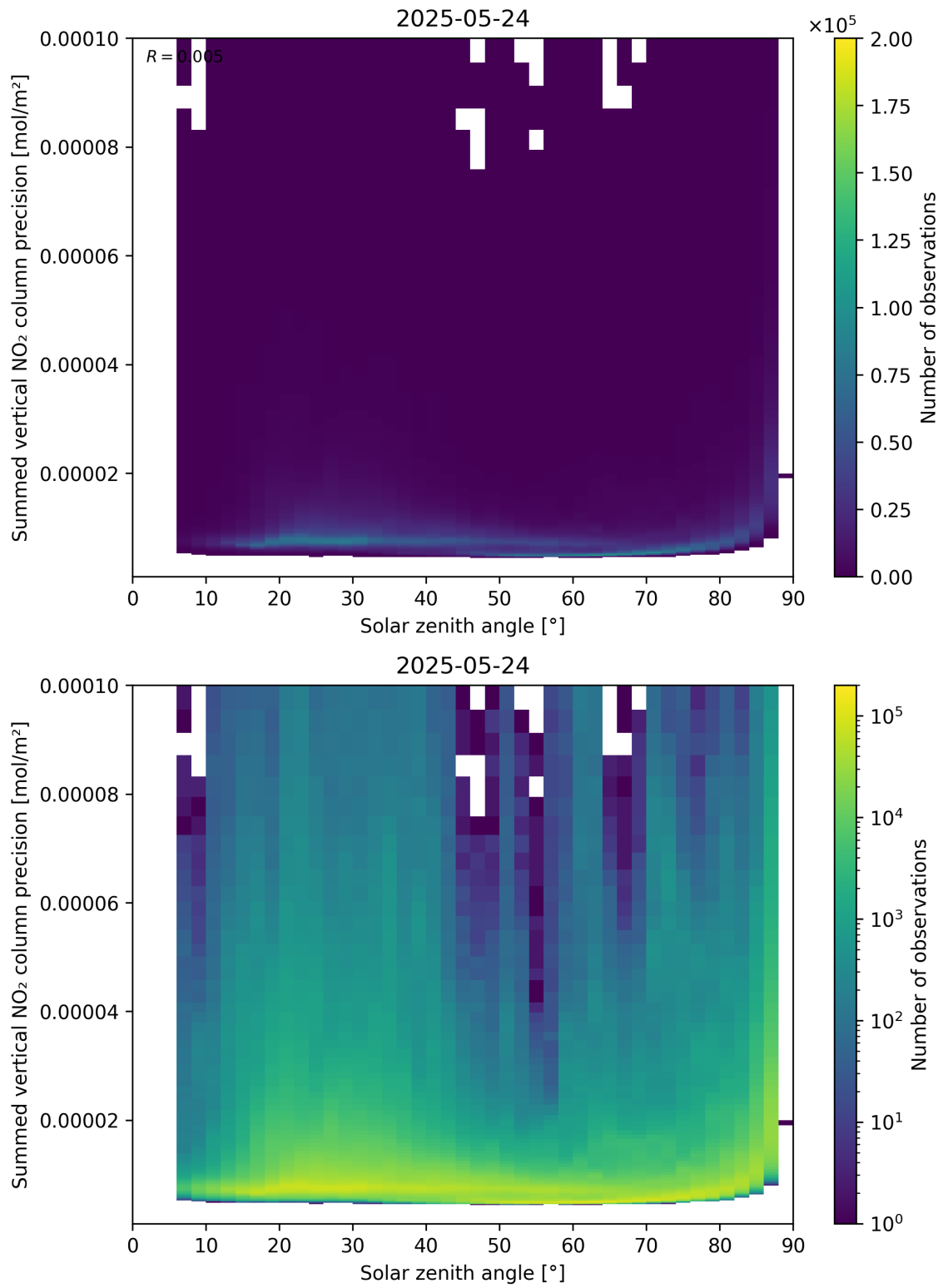
Figure 152: Scatter density plot of “Solar zenith angle” against “Summed vertical NO 2 column precision” for 2025-05-23 to 2025-05-25.
