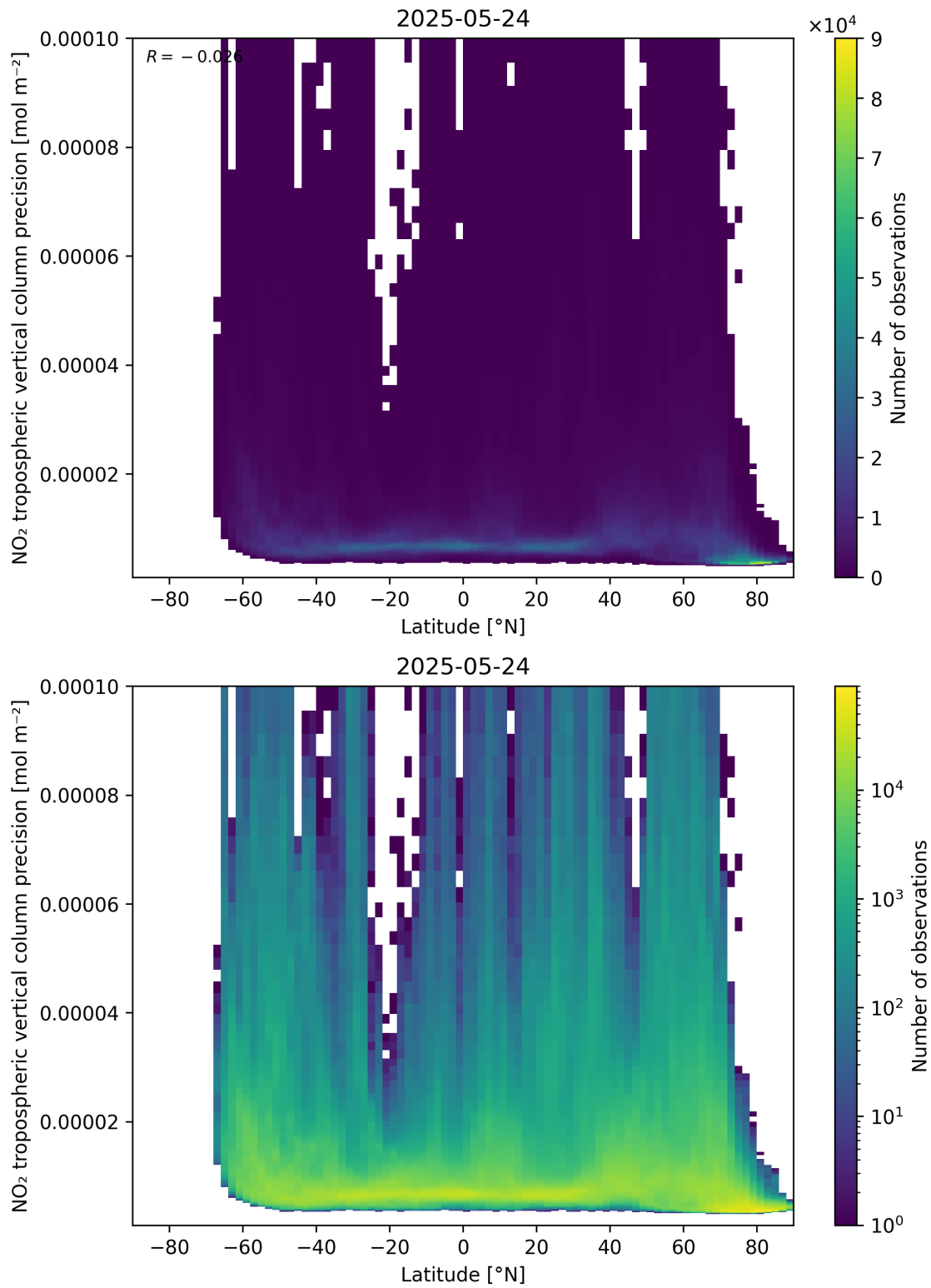
Figure 93: Scatter density plot of “Latitude” against “NO 2 tropospheric vertical column precision” for 2025-05-23 to 2025-05-25.
