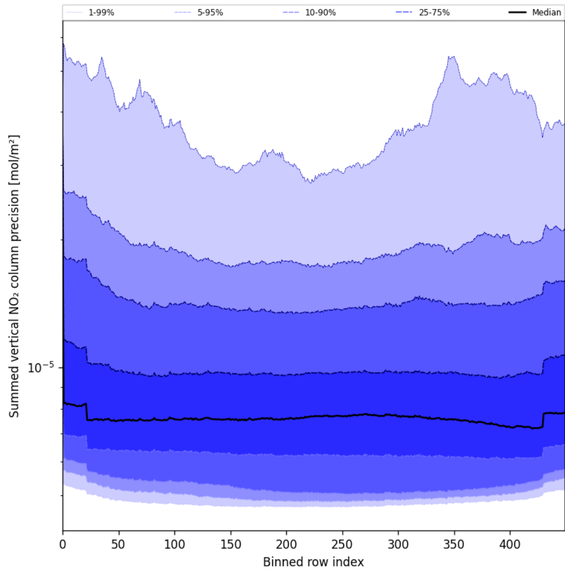
Figure 58: Along track statistics of “Summed vertical NO 2 column precision” for 2025-05-23 to 2025-05-25
