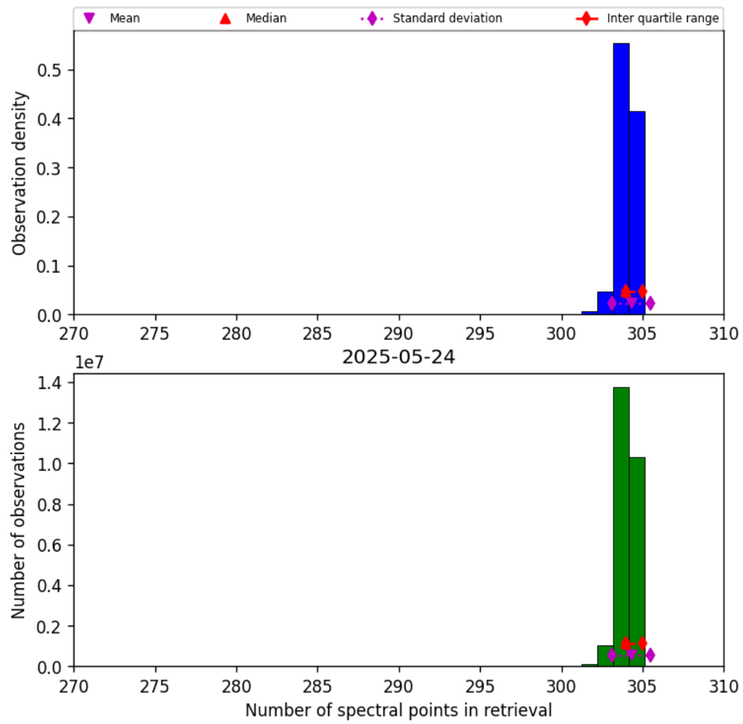
Figure 33: Histogram of “Number of spectral points in retrieval” for 2025-05-23 to 2025-05-25
