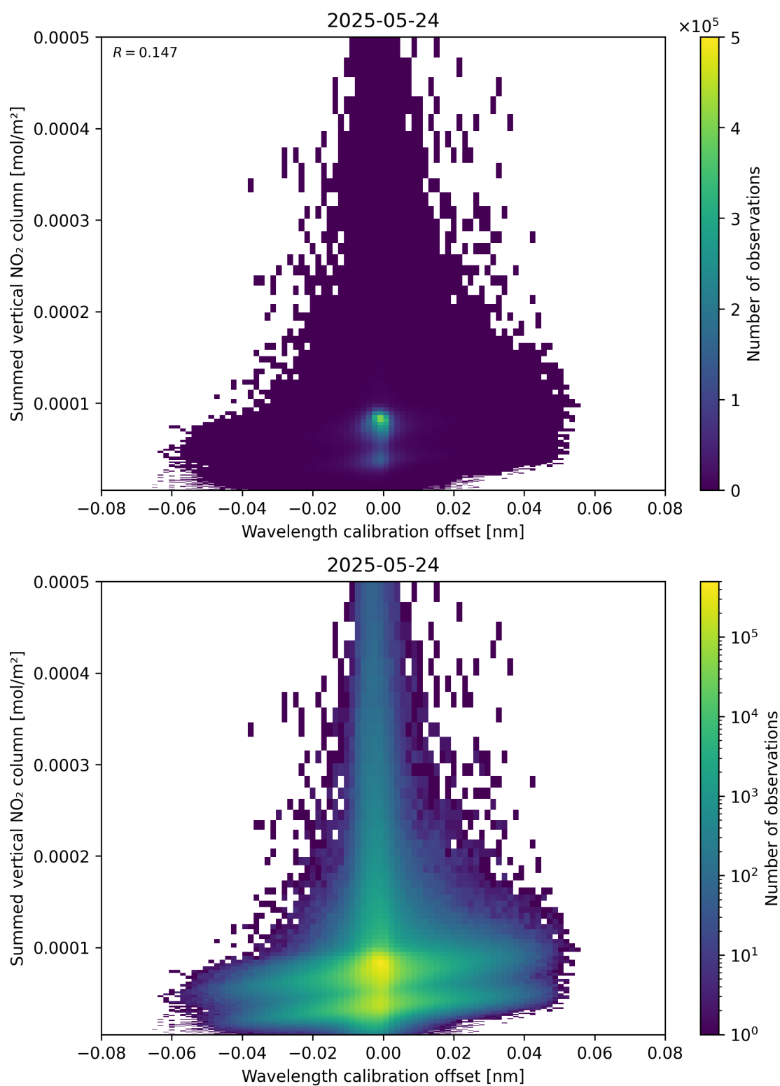
Figure 177: Scatter density plot of “Wavelength calibration offset” against “Summed vertical NO 2 column” for 2025-05-23 to 2025-05-25.
