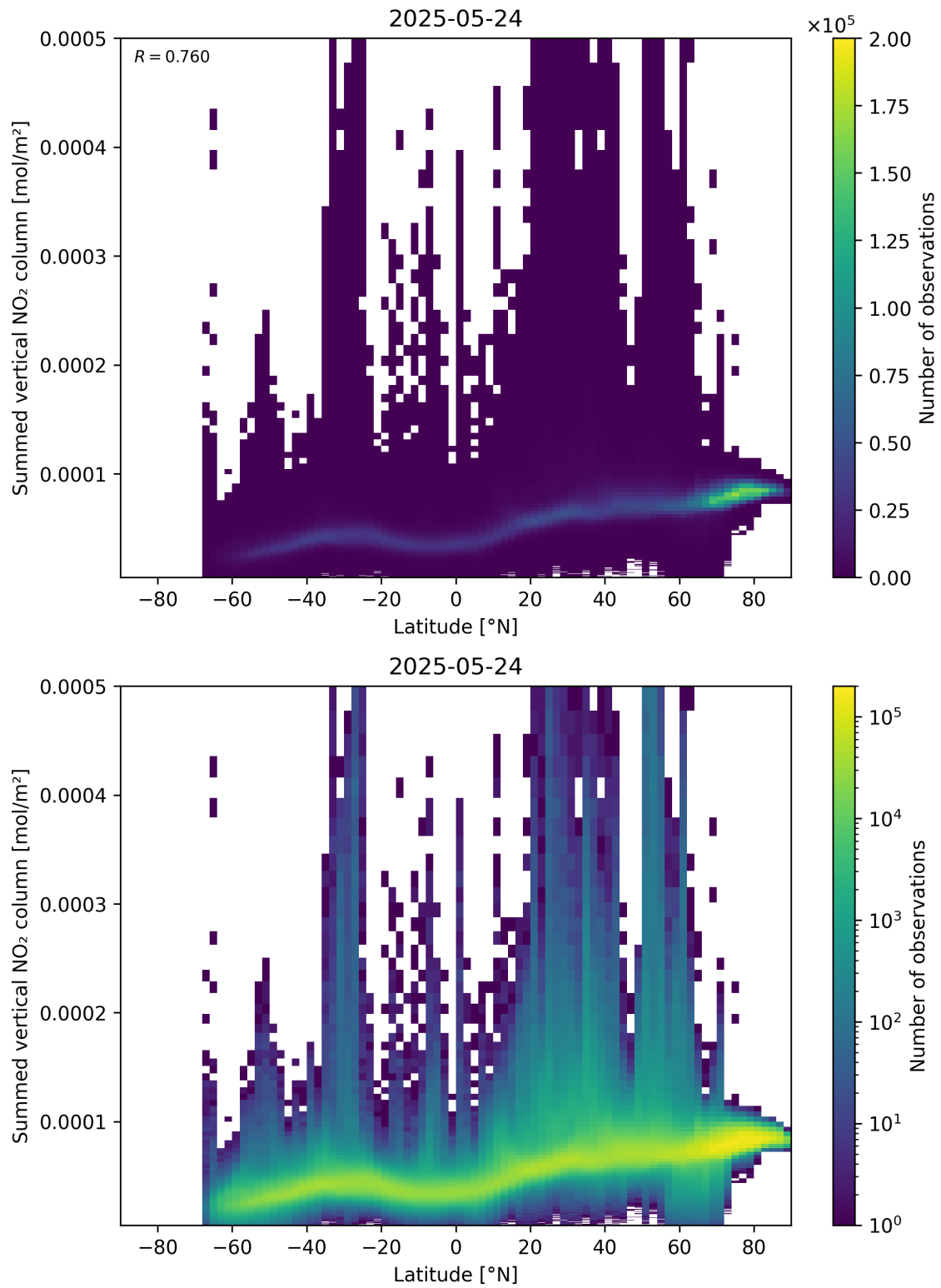
Figure 88: Scatter density plot of “Latitude” against “Summed vertical NO 2 column” for 2025-05-23 to 2025-05-25.
