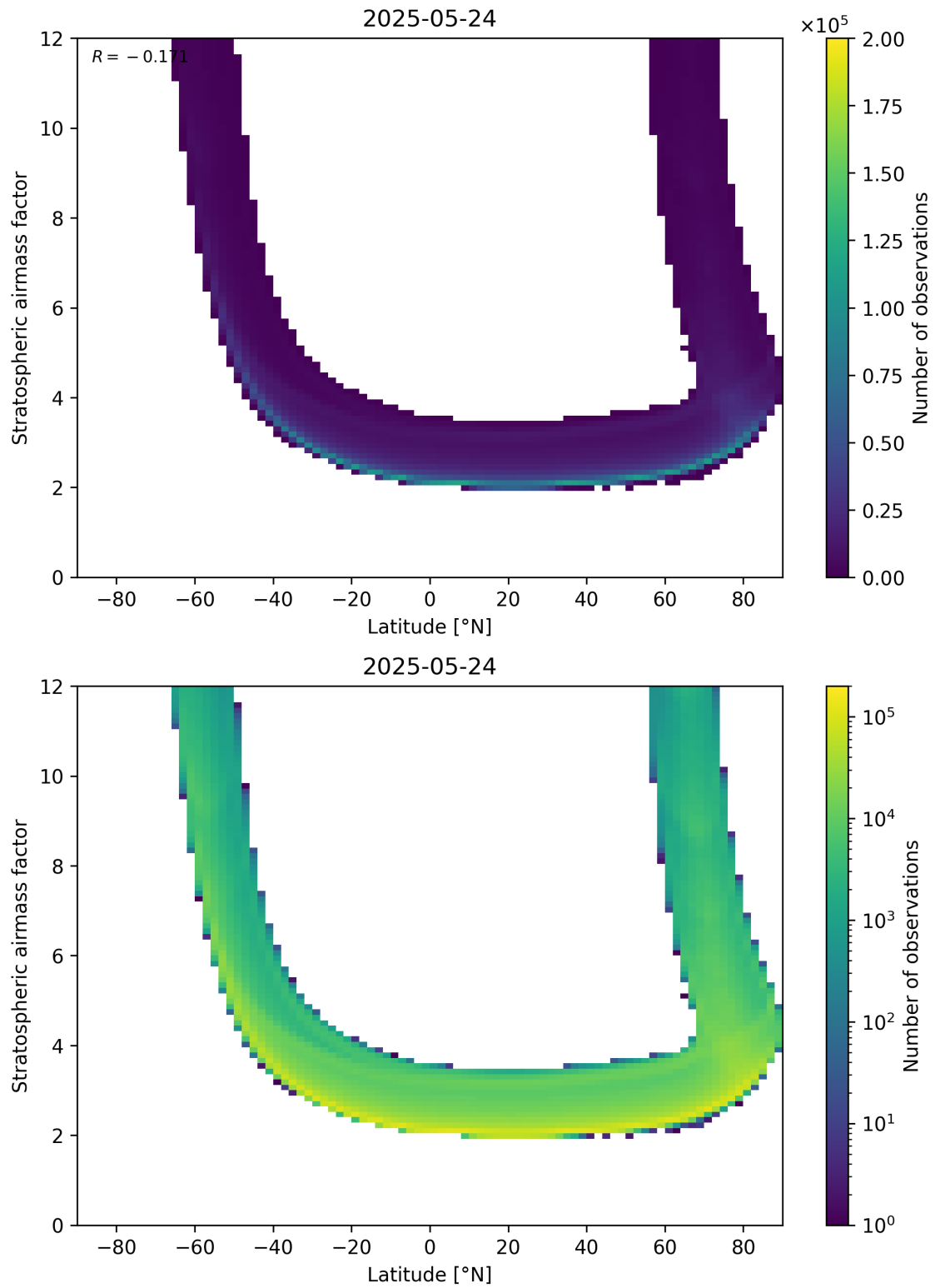
Figure 83: Scatter density plot of “Latitude” against “Stratospheric air mass factor” for 2025-05-23 to 2025-05-25.
