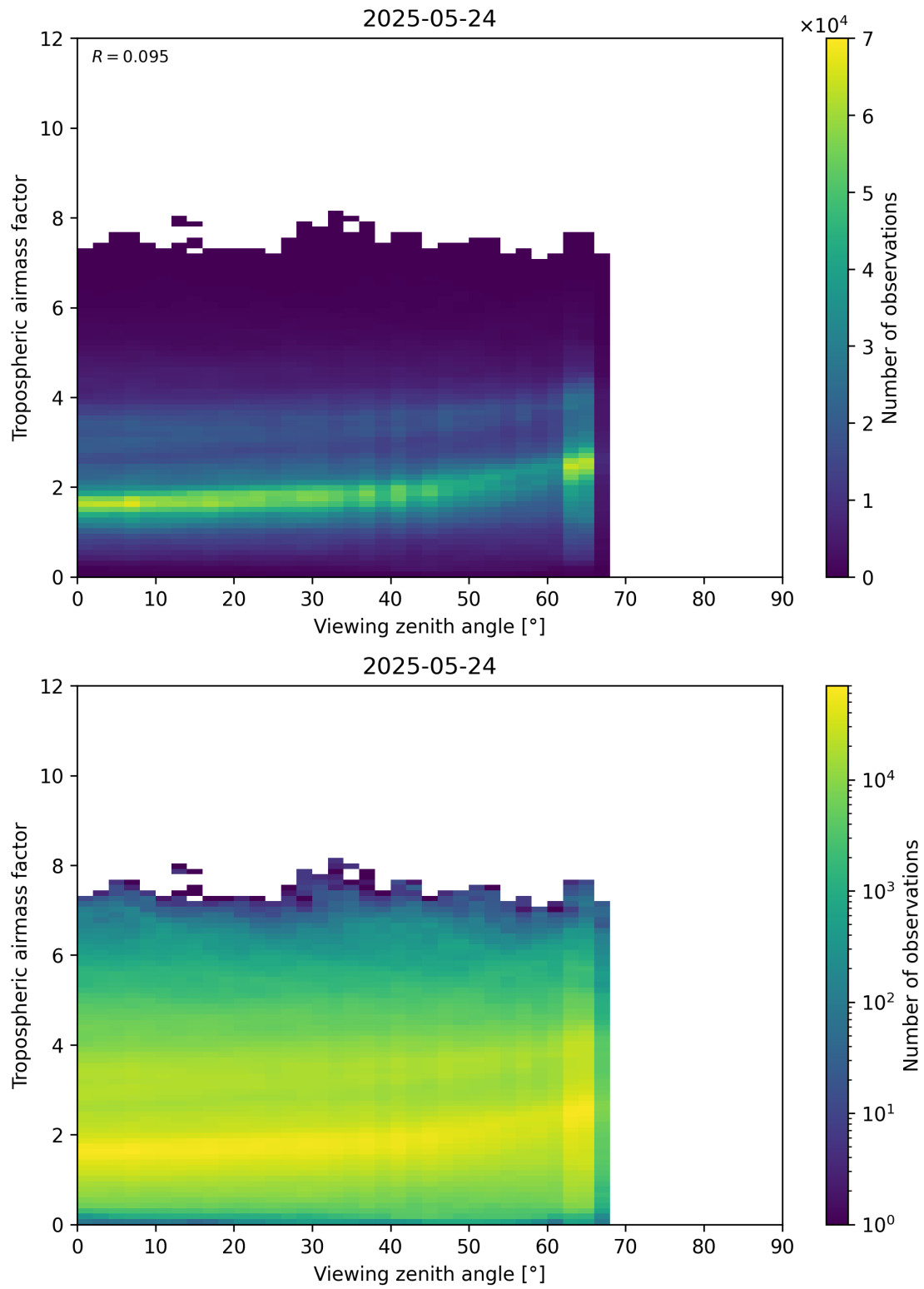
Figure 161: Scatter density plot of “Viewing zenith angle” against “Tropospheric airmass factor” for 2025-05-23 to 2025-05-25.
