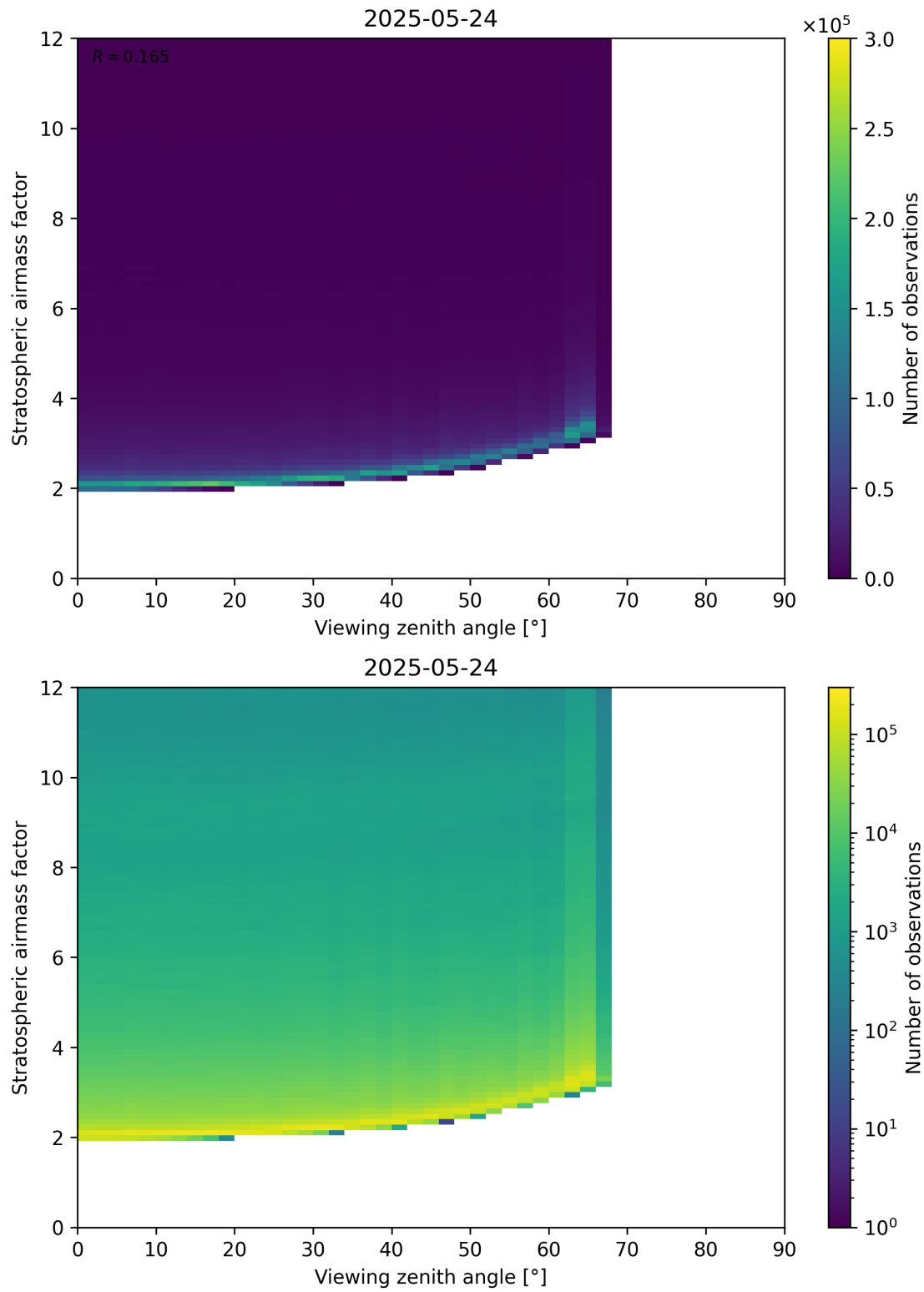
Figure 159: Scatter density plot of “Viewing zenith angle” against “Stratospheric airmass factor” for 2025-05-23 to 2025-05-25.
