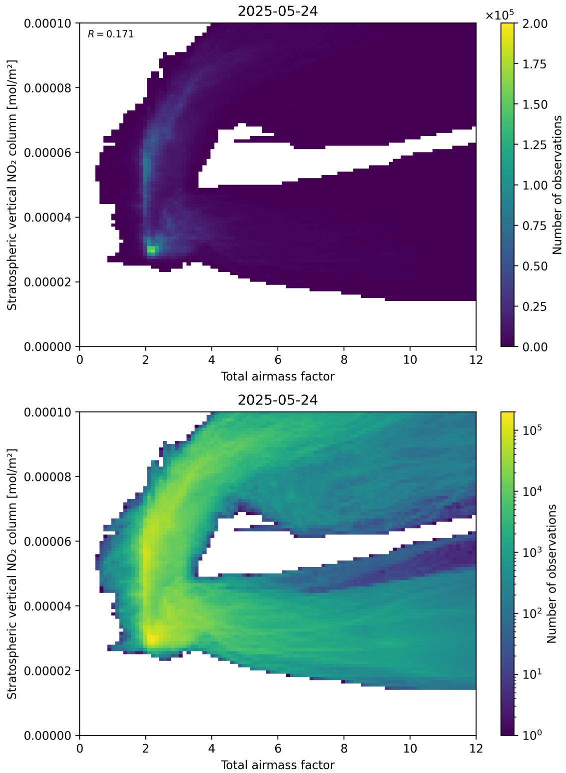
Figure 64: Scatter density plot of “Total airmass factor” against “Stratospheric vertical \text{NO}_2 column” for 2025-05-23 to 2025-05-25.
