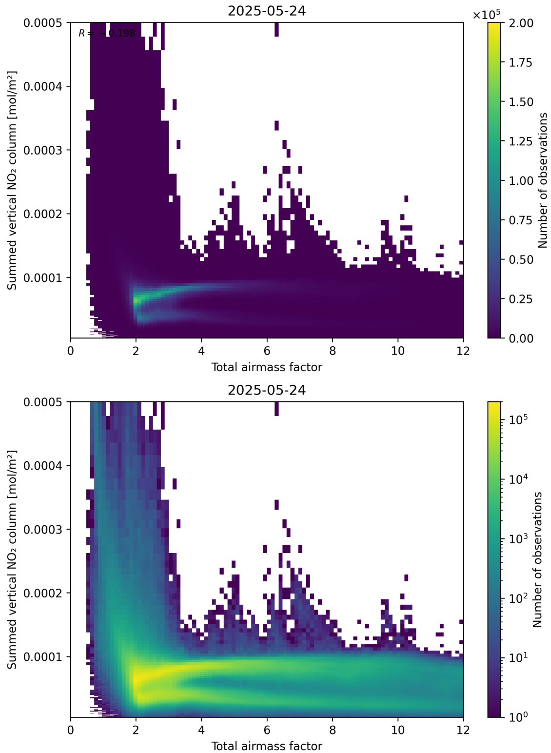
Figure 65: Scatter density plot of “Total airmass factor” against “Summed vertical NO 2 column” for 2025-05-23 to 2025-05-25.
