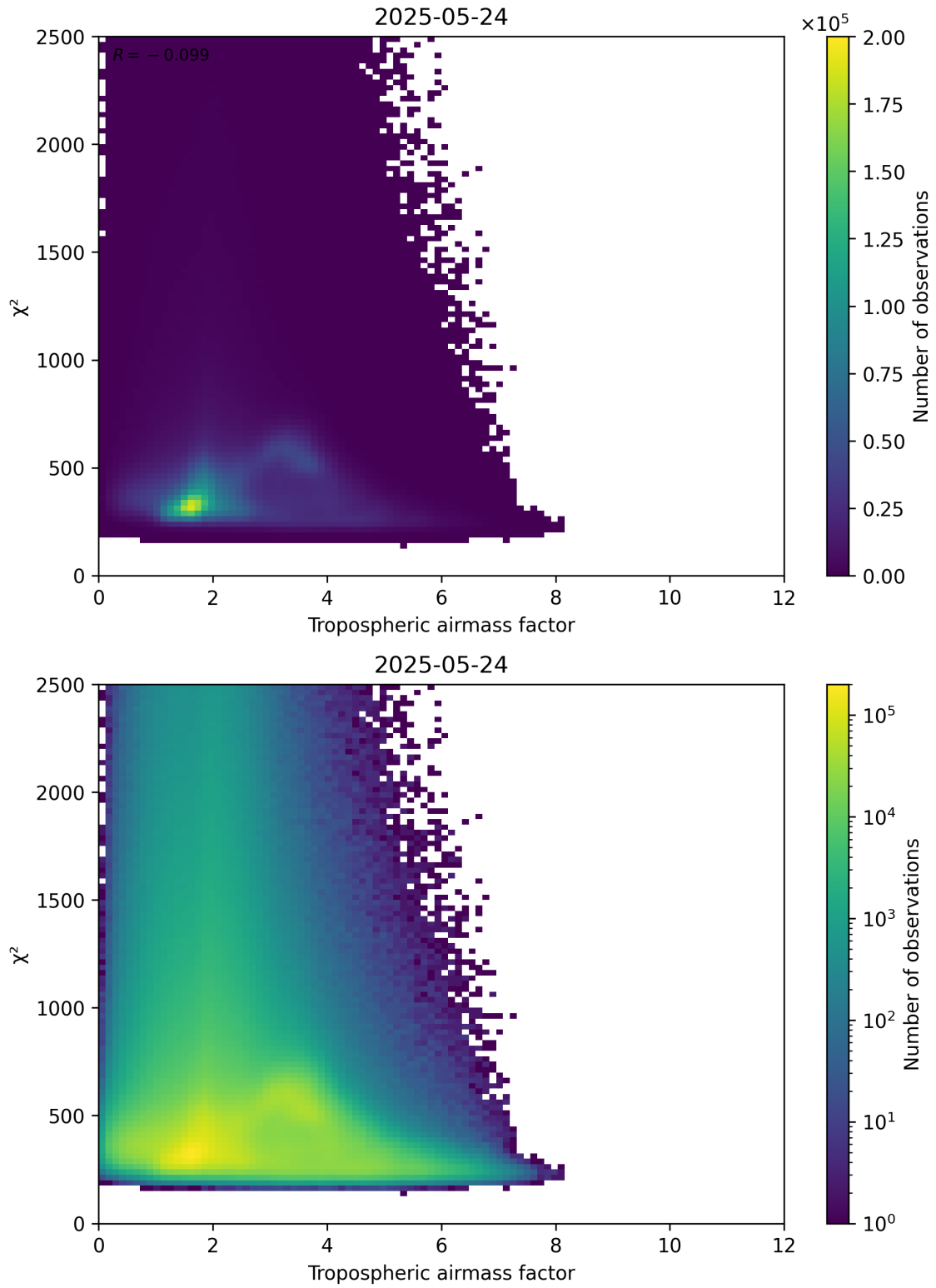
Figure 73: Scatter density plot of “Tropospheric airmass factor” against “ \chi^2 ” for 2025-05-23 to 2025-05-25.
