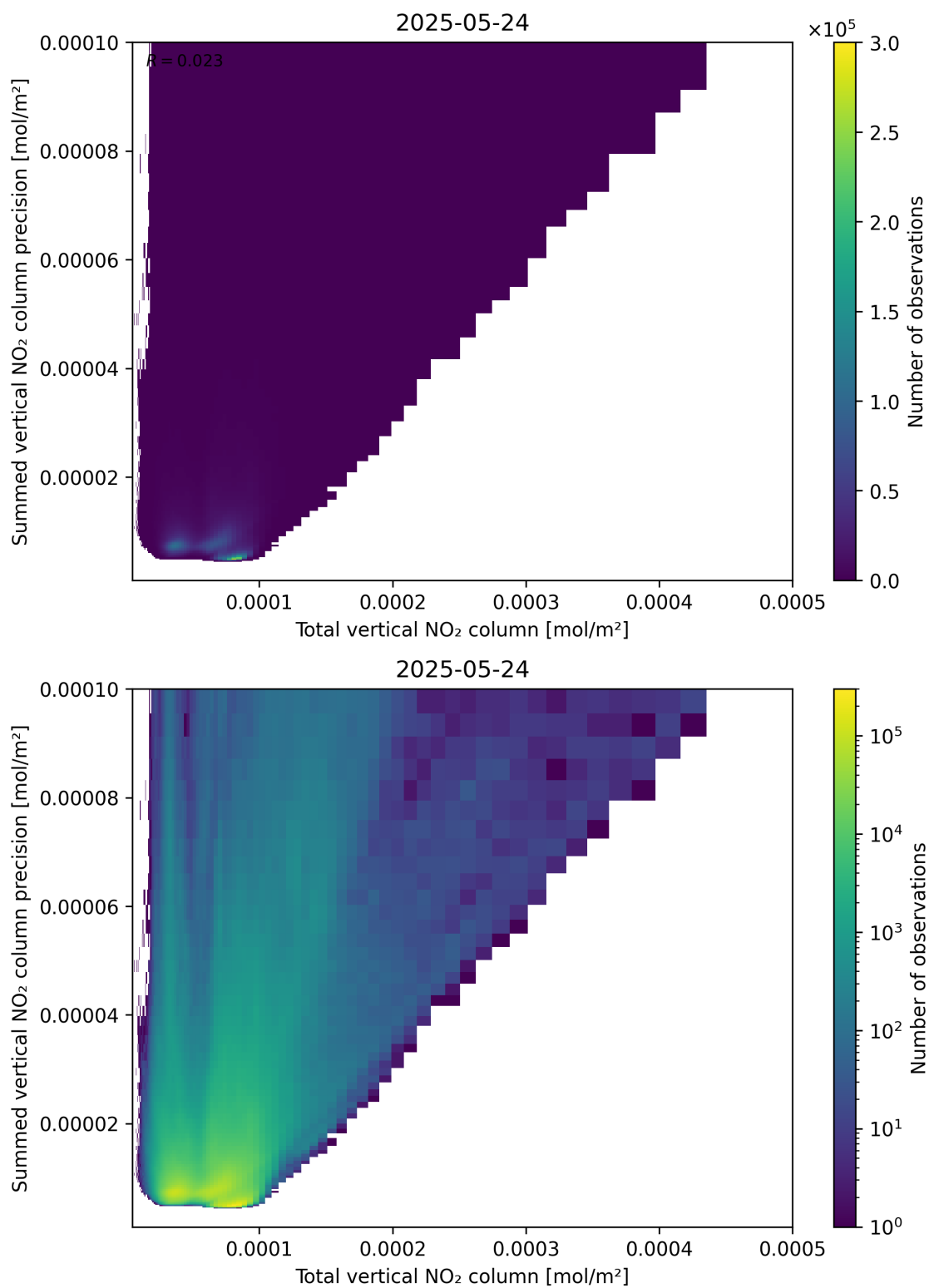
Figure 113: Scatter density plot of “Total vertical NO 2 column” against “Summed vertical NO 2 column precision” for 2025-05-23 to 2025-05-25.
