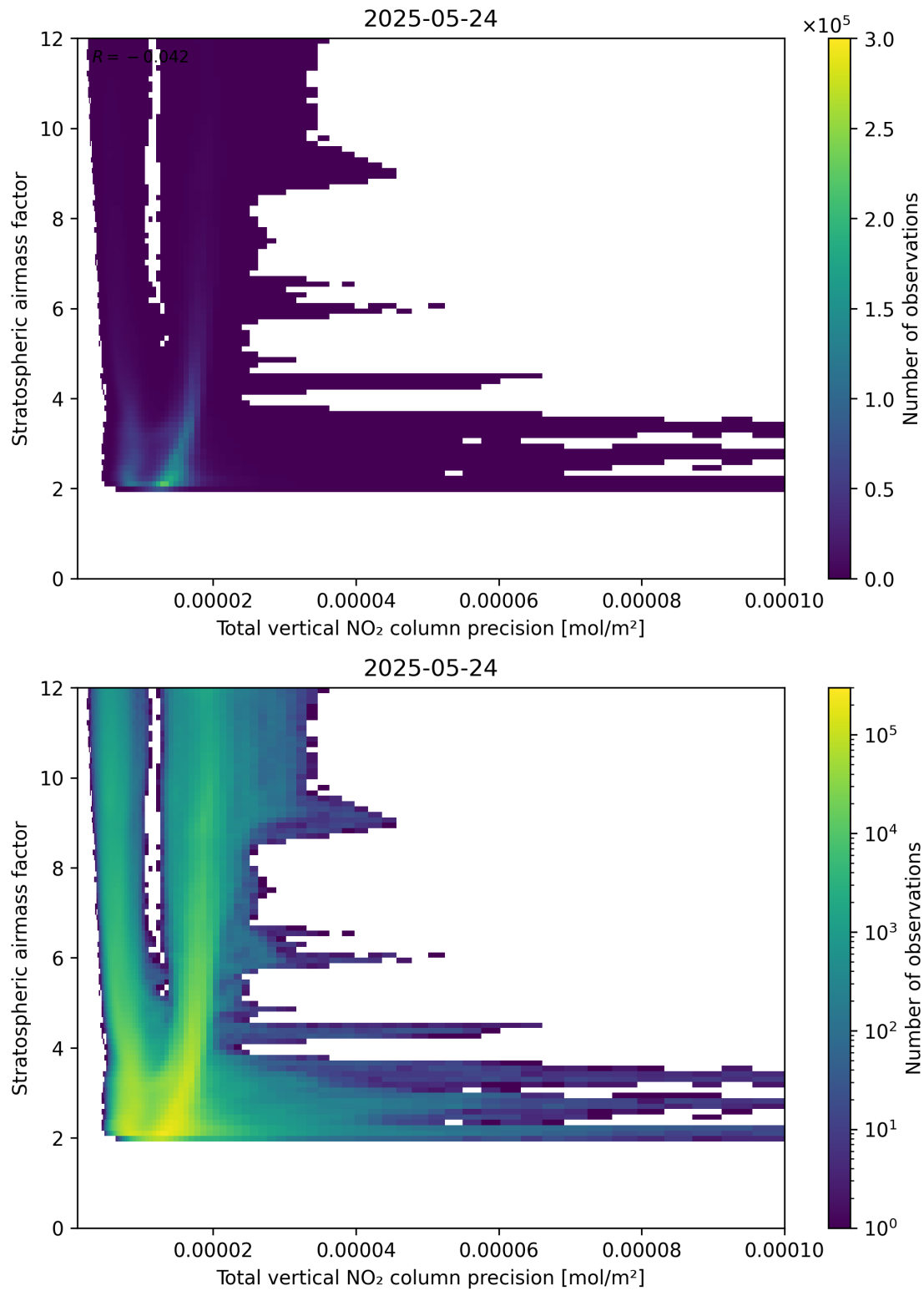
Figure 115: Scatter density plot of “Total vertical NO 2 column precision” against “Stratospheric air mass factor” for 2025-05-23 to 2025-05-25.
