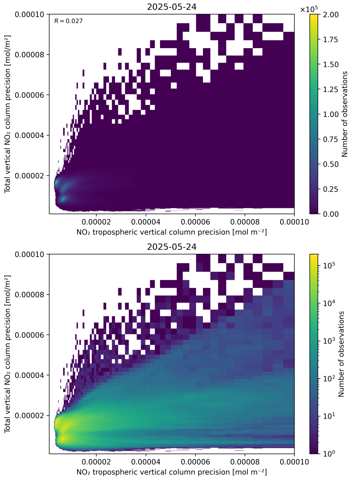
Figure 139: Scatter density plot of “NO 2 tropospheric vertical column precision” against “Total vertical NO 2 column precision” for 2025-05-23 to 2025-05-25.
