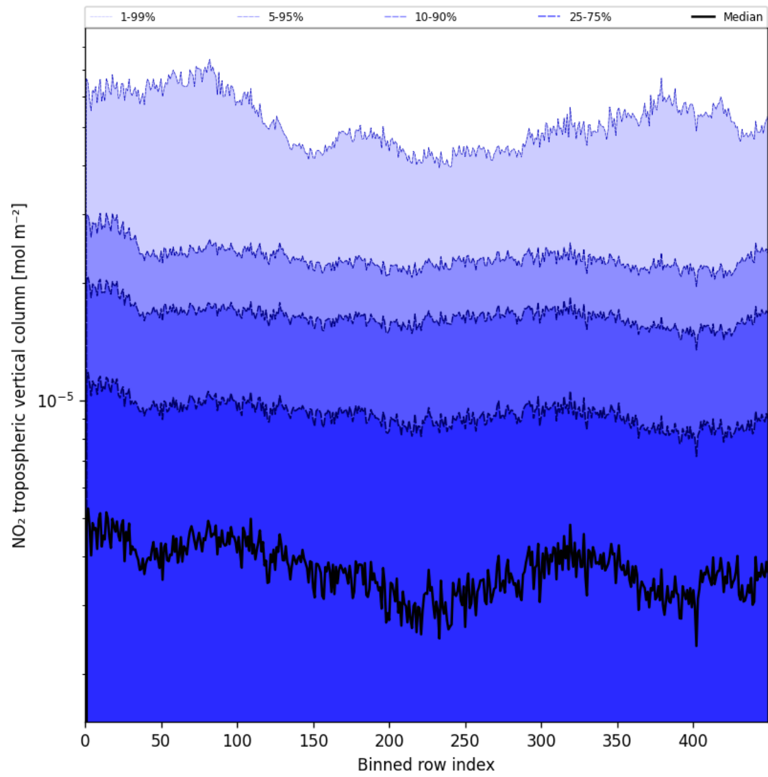
Figure 46: Along track statistics of “NO 2 tropospheric vertical column” for 2025-05-23 to 2025-05-25
