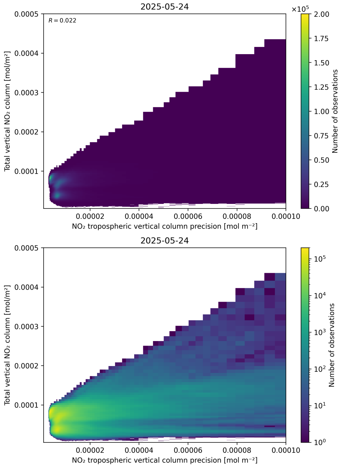
Figure 138: Scatter density plot of “NO 2 tropospheric vertical column precision” against “Total vertical NO 2 column” for 2025-05-23 to 2025-05-25.
