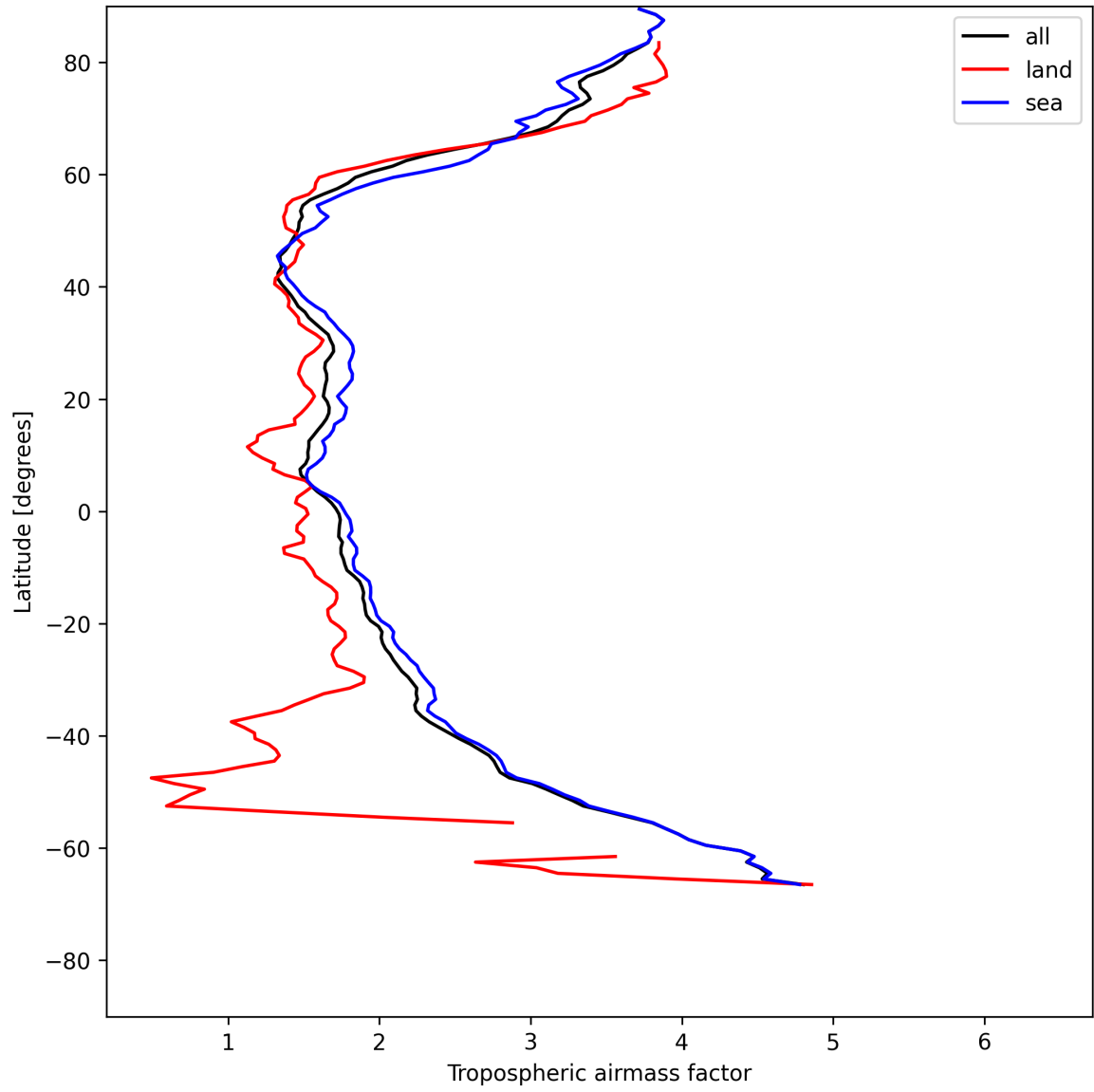
Figure 14: Zonal average of “Tropospheric airmass factor” for 2025-05-23 to 2025-05-25.
