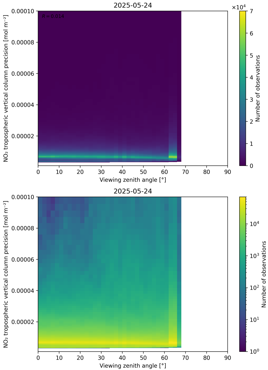
Figure 170: Scatter density plot of “Viewing zenith angle” against “NO 2 tropospheric vertical column precision” for 2025-05-23 to 2025-05-25.
