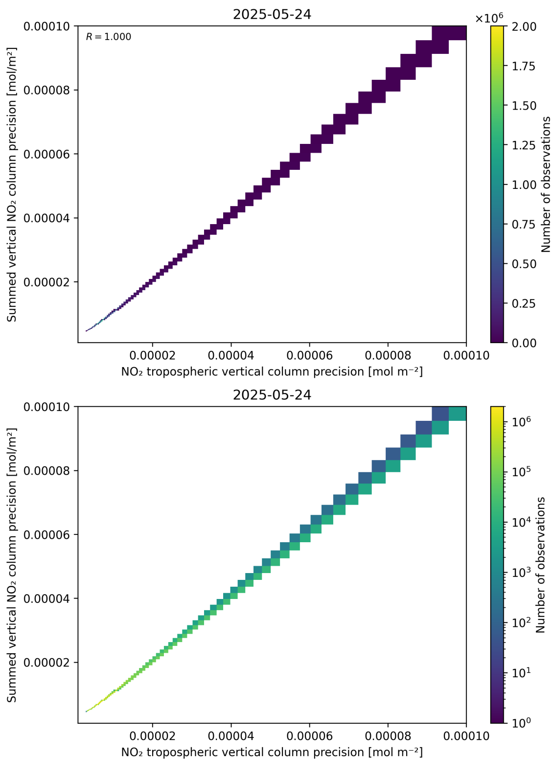
Figure 137: Scatter density plot of “NO 2 tropospheric vertical column precision” against “Summed vertical NO 2 column precision” for 2025-05-23 to 2025-05-25.
