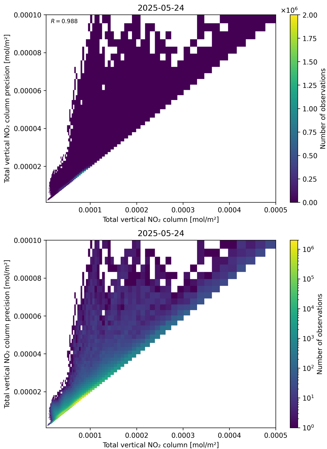
Figure 114: Scatter density plot of “Total vertical NO 2 column” against “Total vertical NO 2 column precision” for 2025-05-23 to 2025-05-25.
