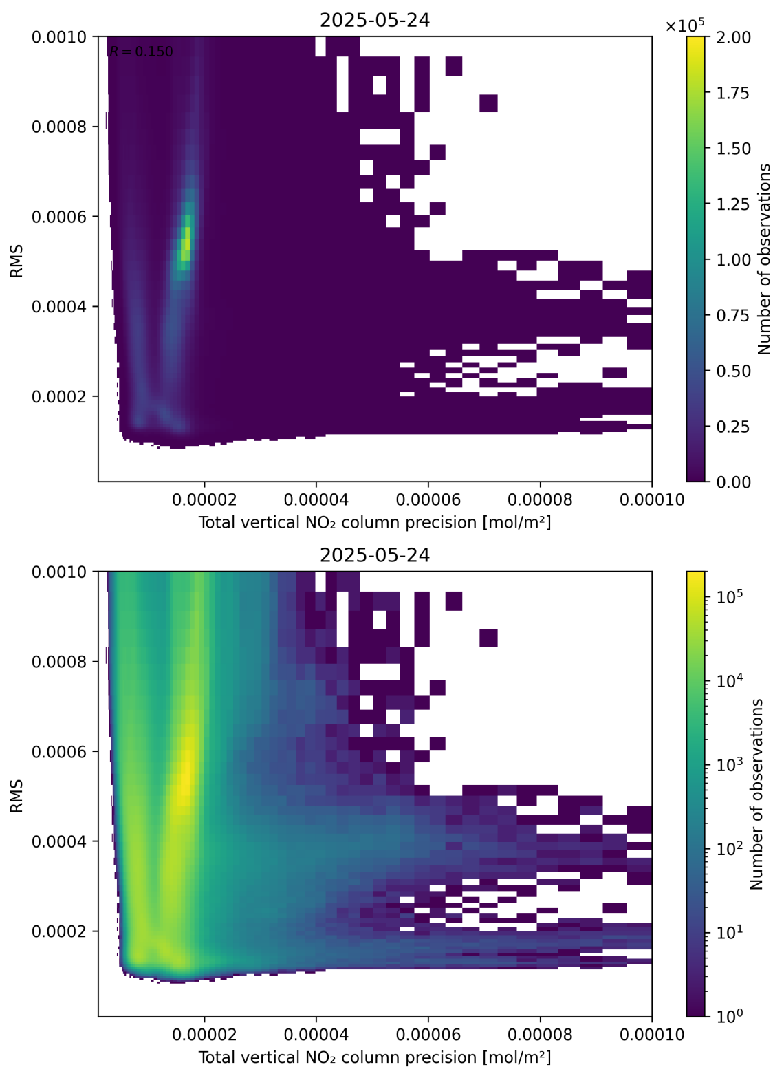
Figure 119: Scatter density plot of “Total vertical NO 2 column precision” against “RMS” for 2025-05-23 to 2025-05-25.
