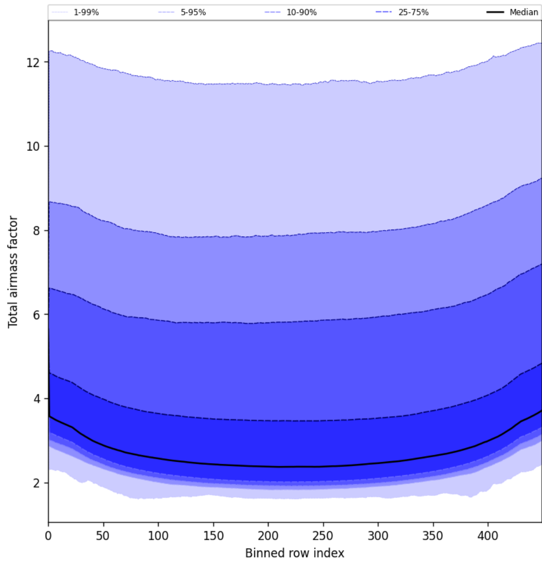
Figure 49: Along track statistics of “Total airmass factor” for 2025-05-23 to 2025-05-25
