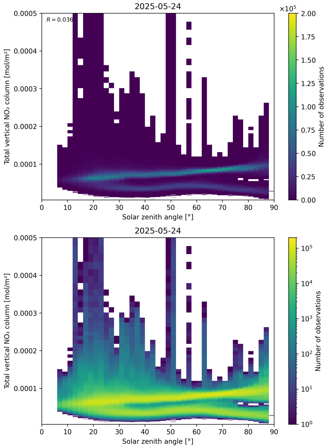
Figure 153: Scatter density plot of “Solar zenith angle” against “Total vertical NO 2 column” for 2025-05-23 to 2025-05-25.
