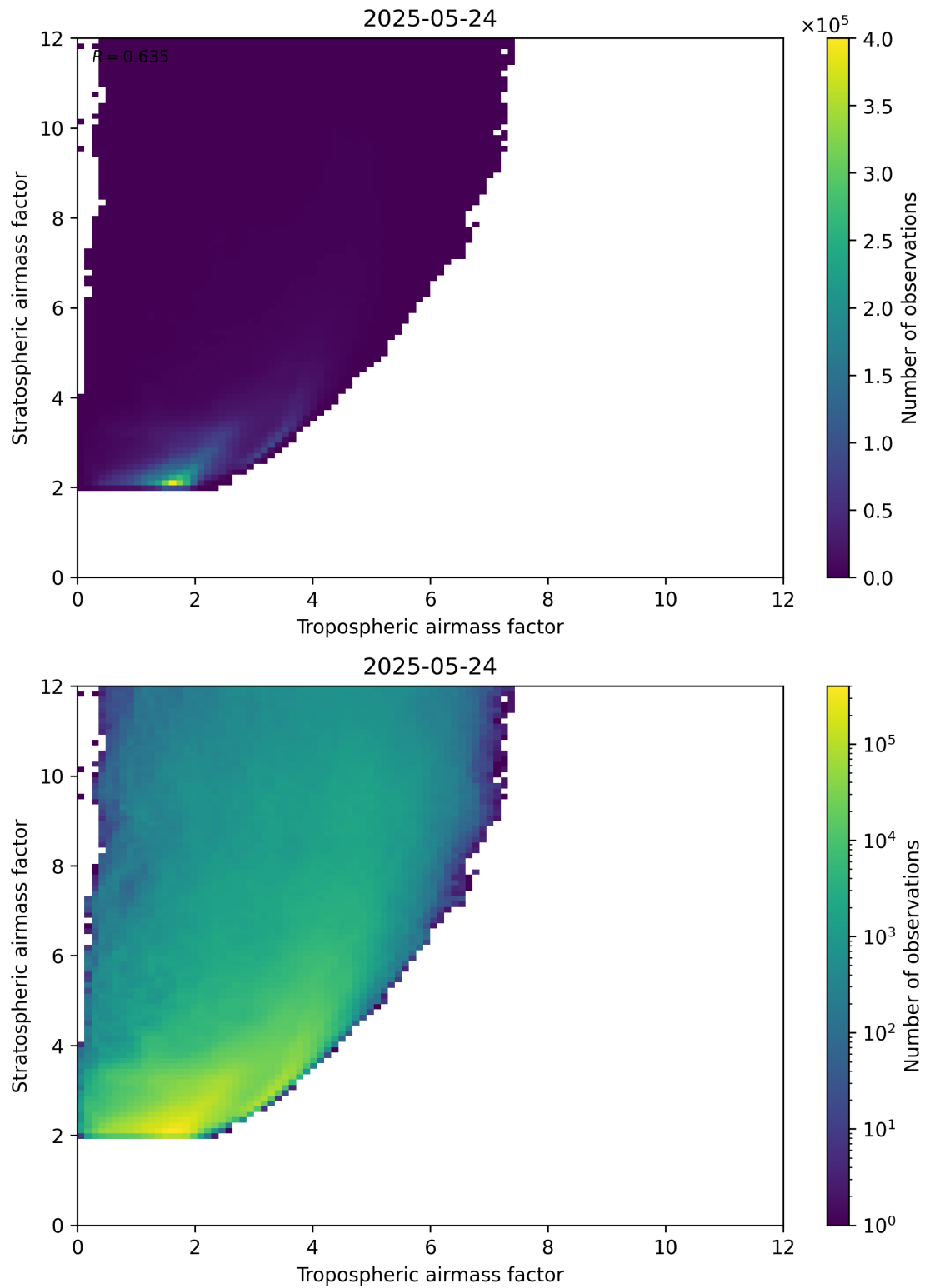
Figure 71: Scatter density plot of “Tropospheric airmass factor” against “Stratospheric airmass factor” for 2025-05-23 to 2025-05-25.
