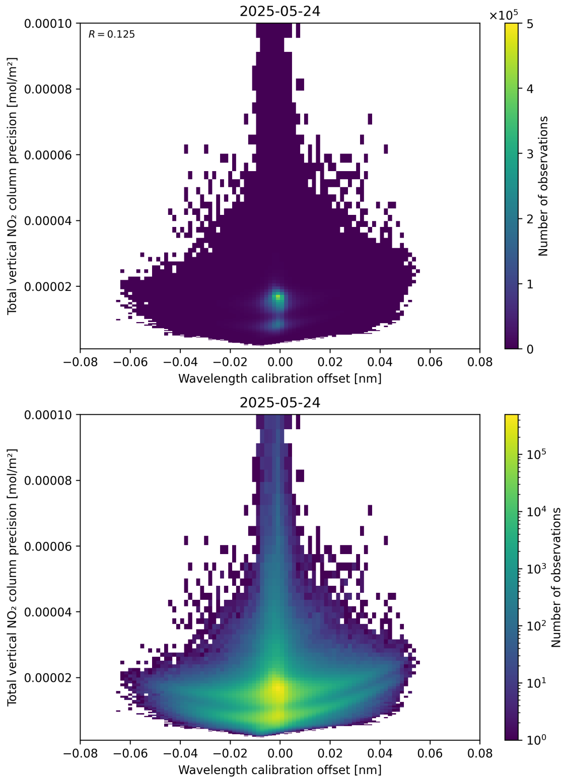
Figure 180: Scatter density plot of “Wavelength calibration offset” against “Total vertical NO 2 column precision” for 2025-05-23 to 2025-05-25.
