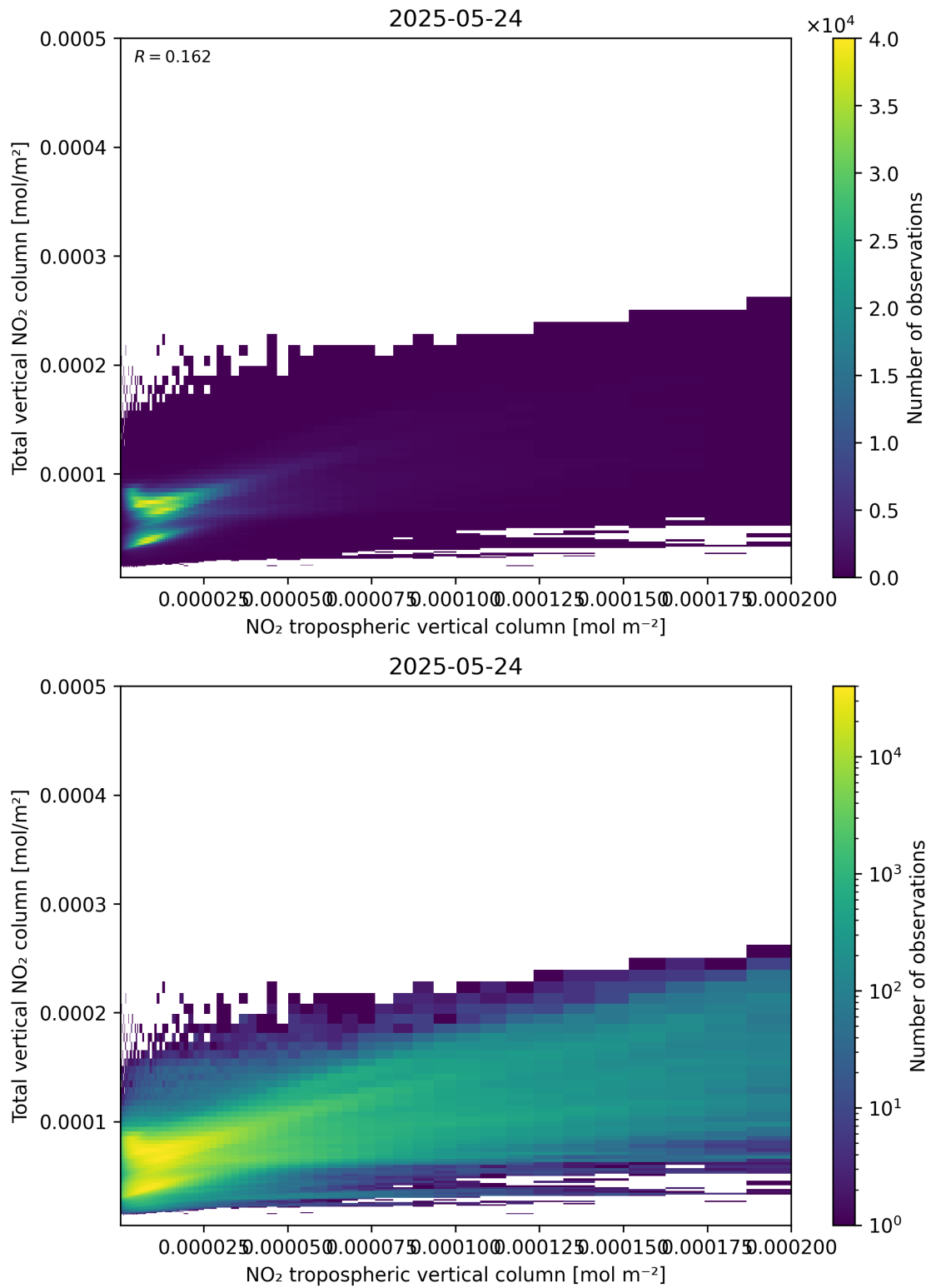
Figure 128: Scatter density plot of “NO 2 tropospheric vertical column” against “Total vertical NO 2 column” for 2025-05-23 to 2025-05-25.
