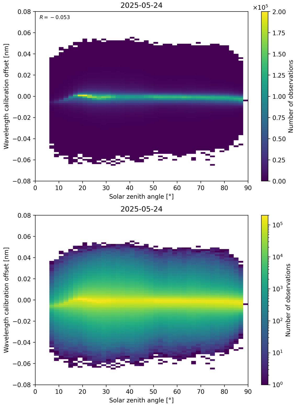
Figure 158: Scatter density plot of “Solar zenith angle” against “Wavelength calibration offset” for 2025-05-23 to 2025-05-25.
