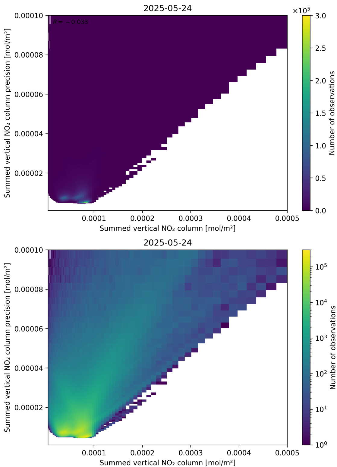
Figure 105: Scatter density plot of “Summed vertical NO 2 column” against “Summed vertical NO 2 column precision” for 2025-05-23 to 2025-05-25.
