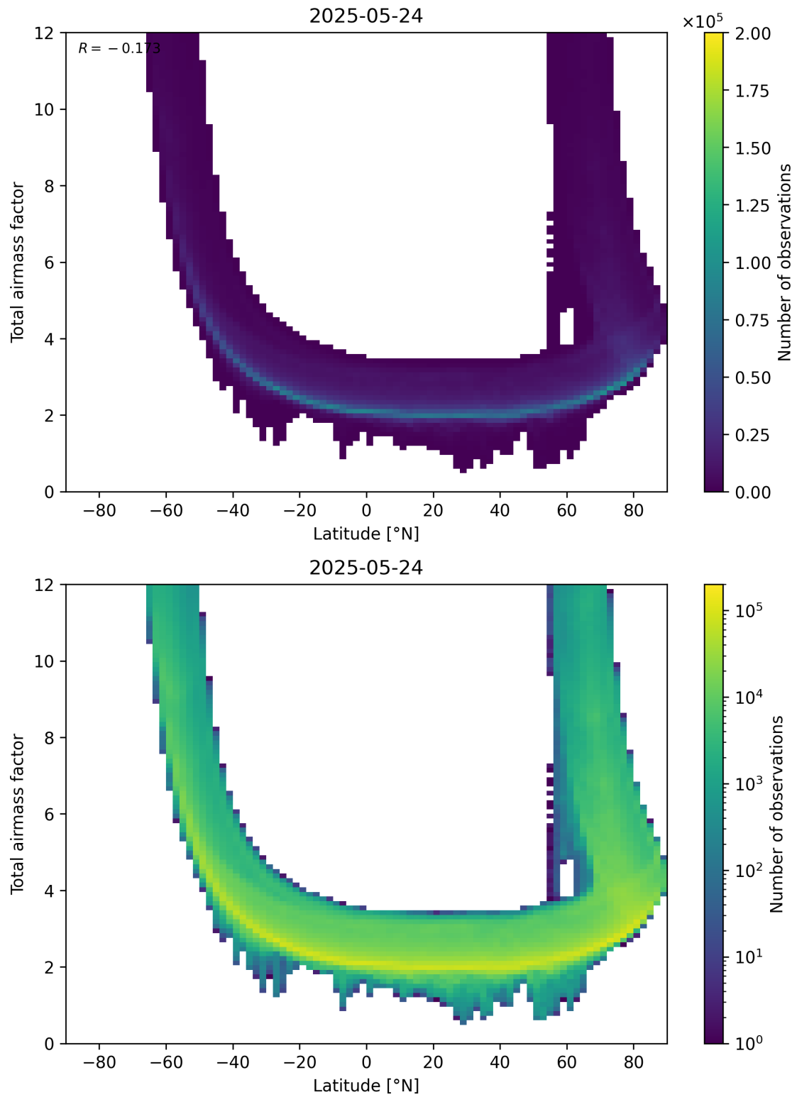
Figure 84: Scatter density plot of “Latitude” against “Total airmass factor” for 2025-05-23 to 2025-05-25.
