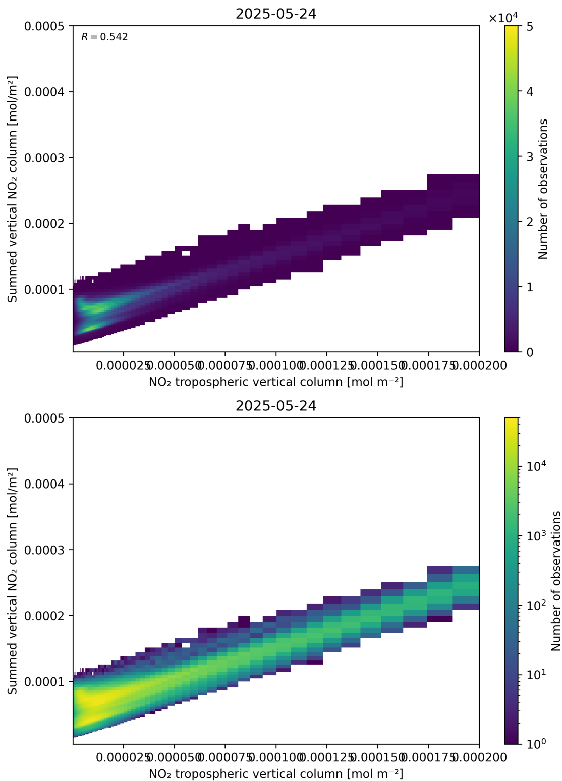
Figure 126: Scatter density plot of “NO 2 tropospheric vertical column” against “Summed vertical NO 2 column” for 2025-05-23 to 2025-05-25.
