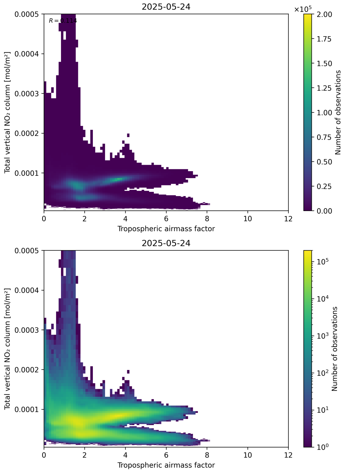
Figure 77: Scatter density plot of “Tropospheric airmass factor” against “Total vertical NO 2 column” for 2025-05-23 to 2025-05-25.
