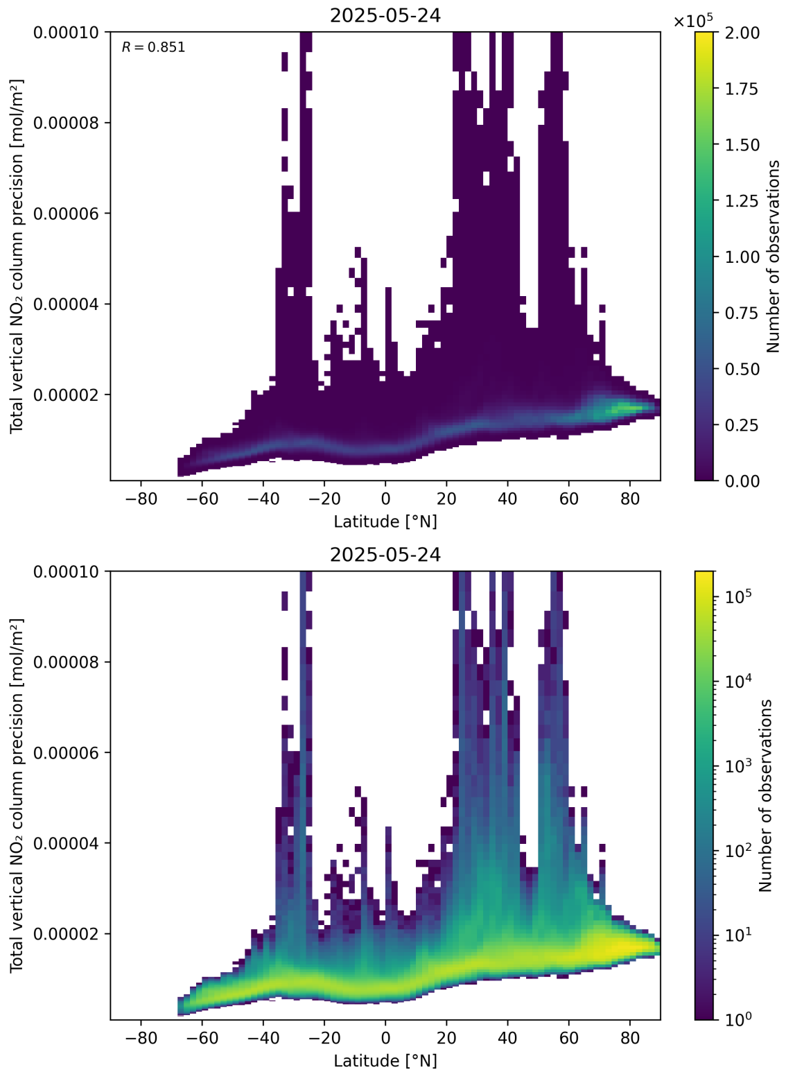
Figure 91: Scatter density plot of “Latitude” against “Total vertical NO 2 column precision” for 2025-05-23 to 2025-05-25.
