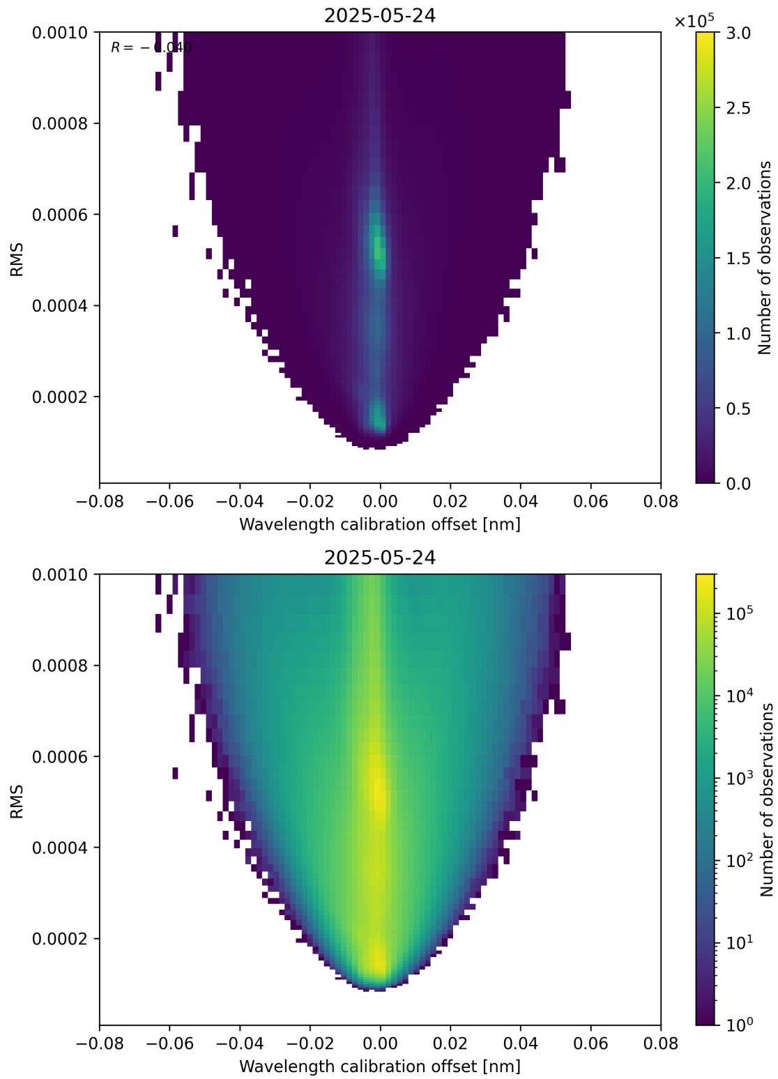
Figure 181: Scatter density plot of “Wavelength calibration offset” against “RMS” for 2025-05-23 to 2025-05-25.
