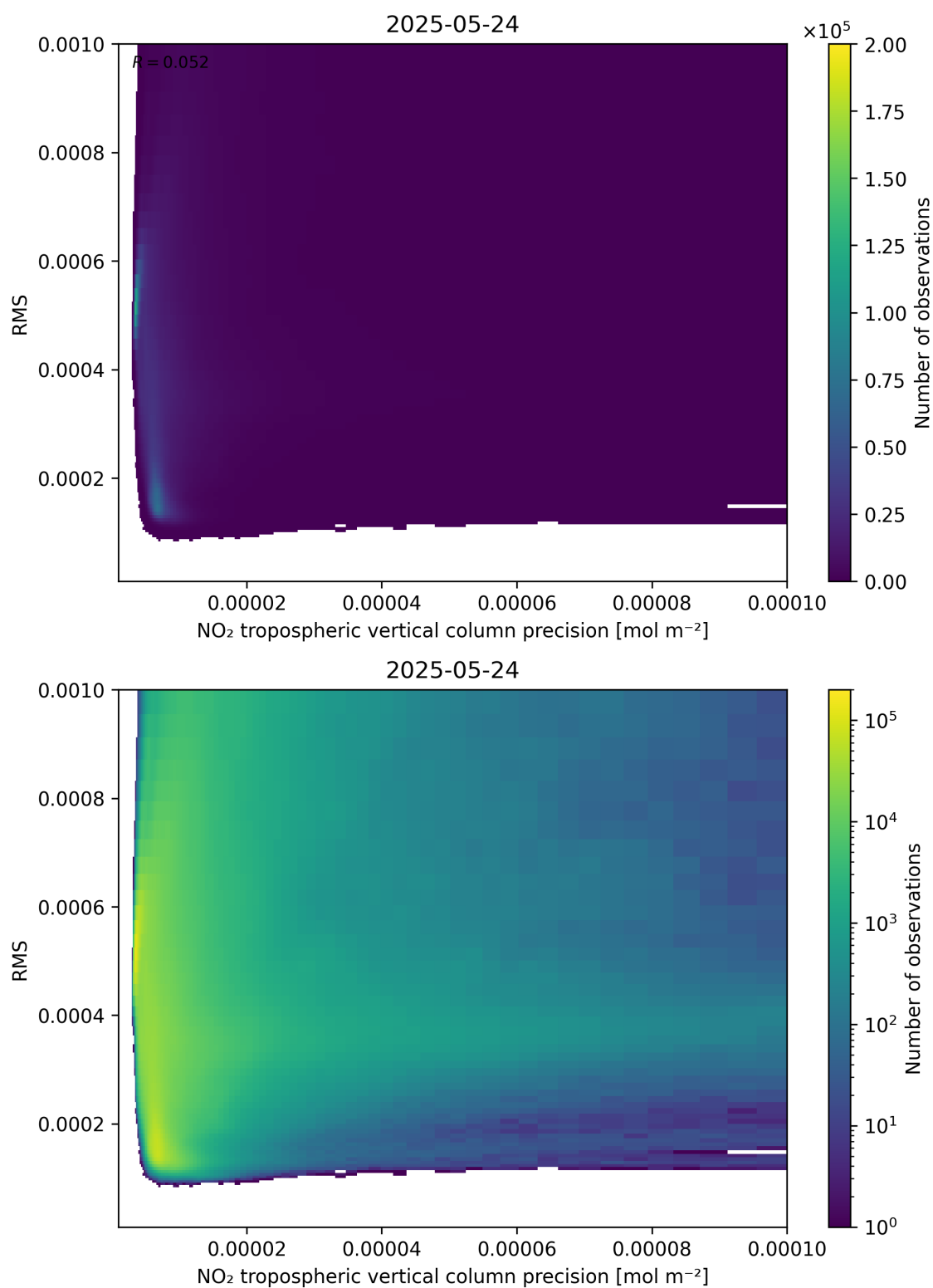
Figure 140: Scatter density plot of “NO 2 tropospheric vertical column precision” against “RMS” for 2025-05-23 to 2025-05-25.
