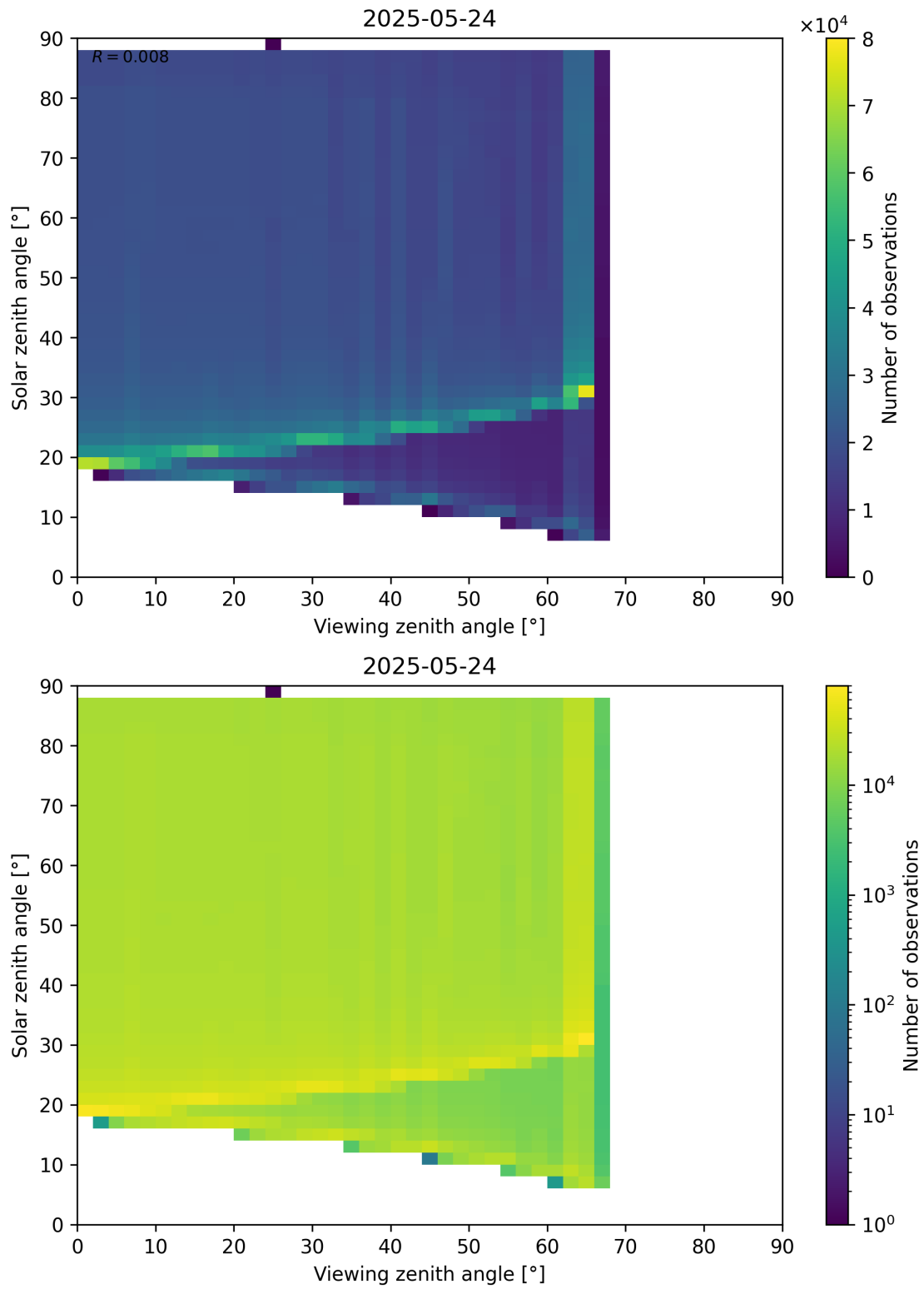
Figure 172: Scatter density plot of “Viewing zenith angle” against “Solar zenith angle” for 2025-05-23 to 2025-05-25.
