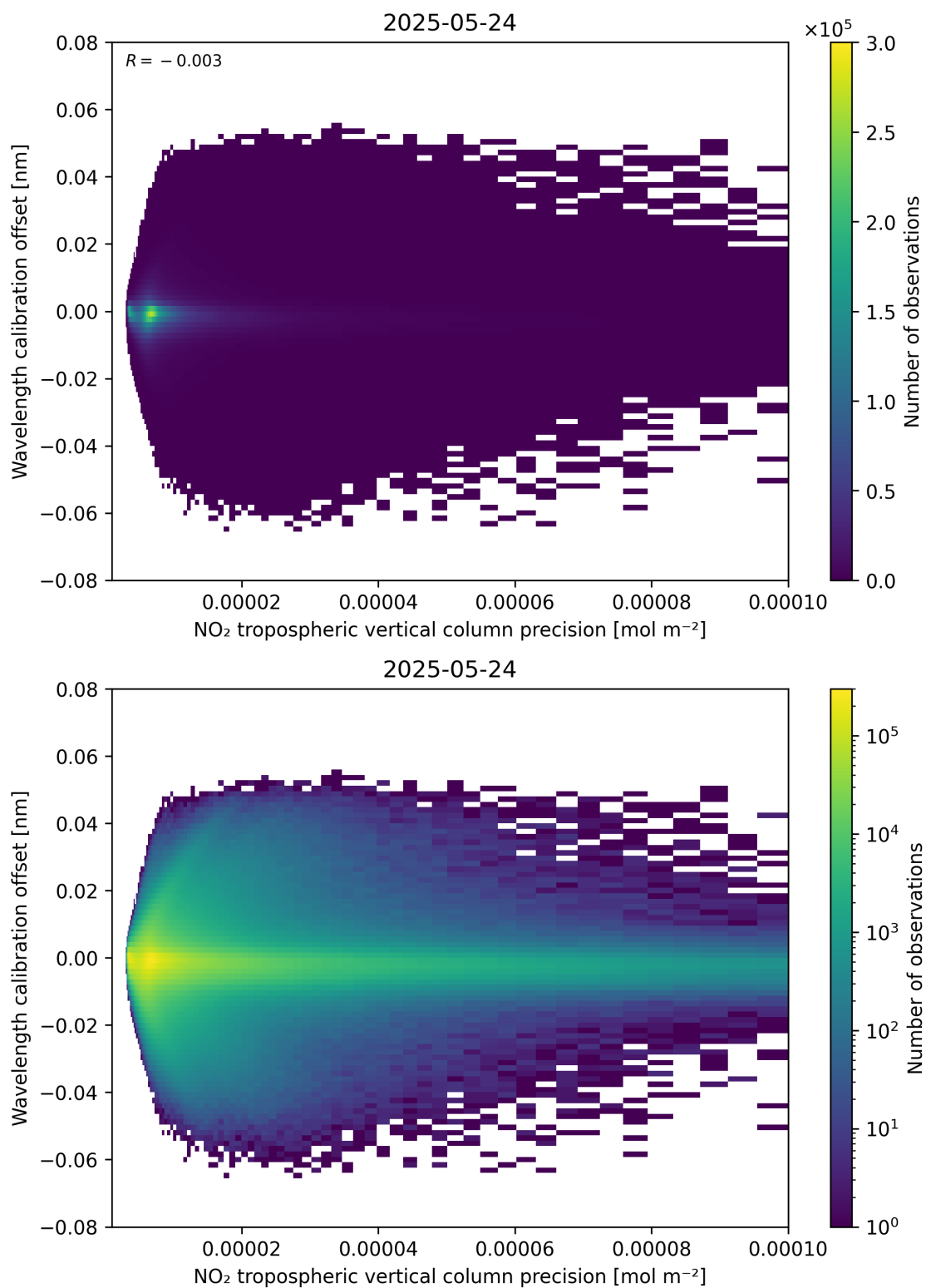
Figure 141: Scatter density plot of “NO 2 tropospheric vertical column precision” against “Wavelength calibration offset” for 2025-05-23 to 2025-05-25.
