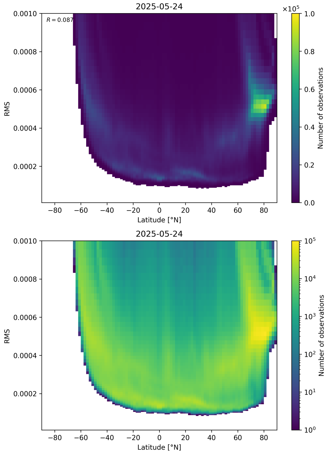
Figure 94: Scatter density plot of “Latitude” against “RMS” for 2025-05-23 to 2025-05-25.
