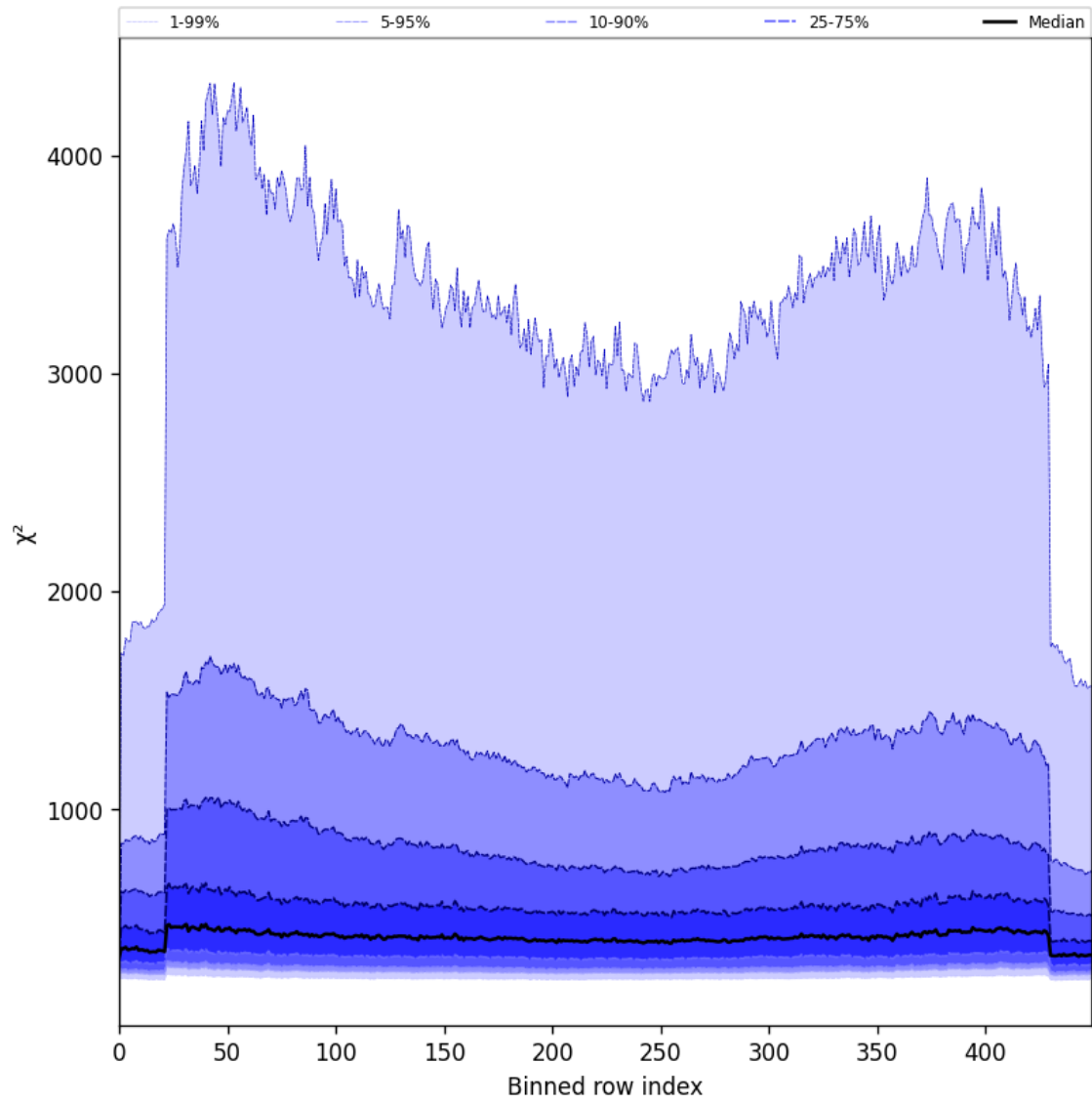
Figure 59: Along track statistics of “ \chi^2 ” for 2025-05-23 to 2025-05-25
