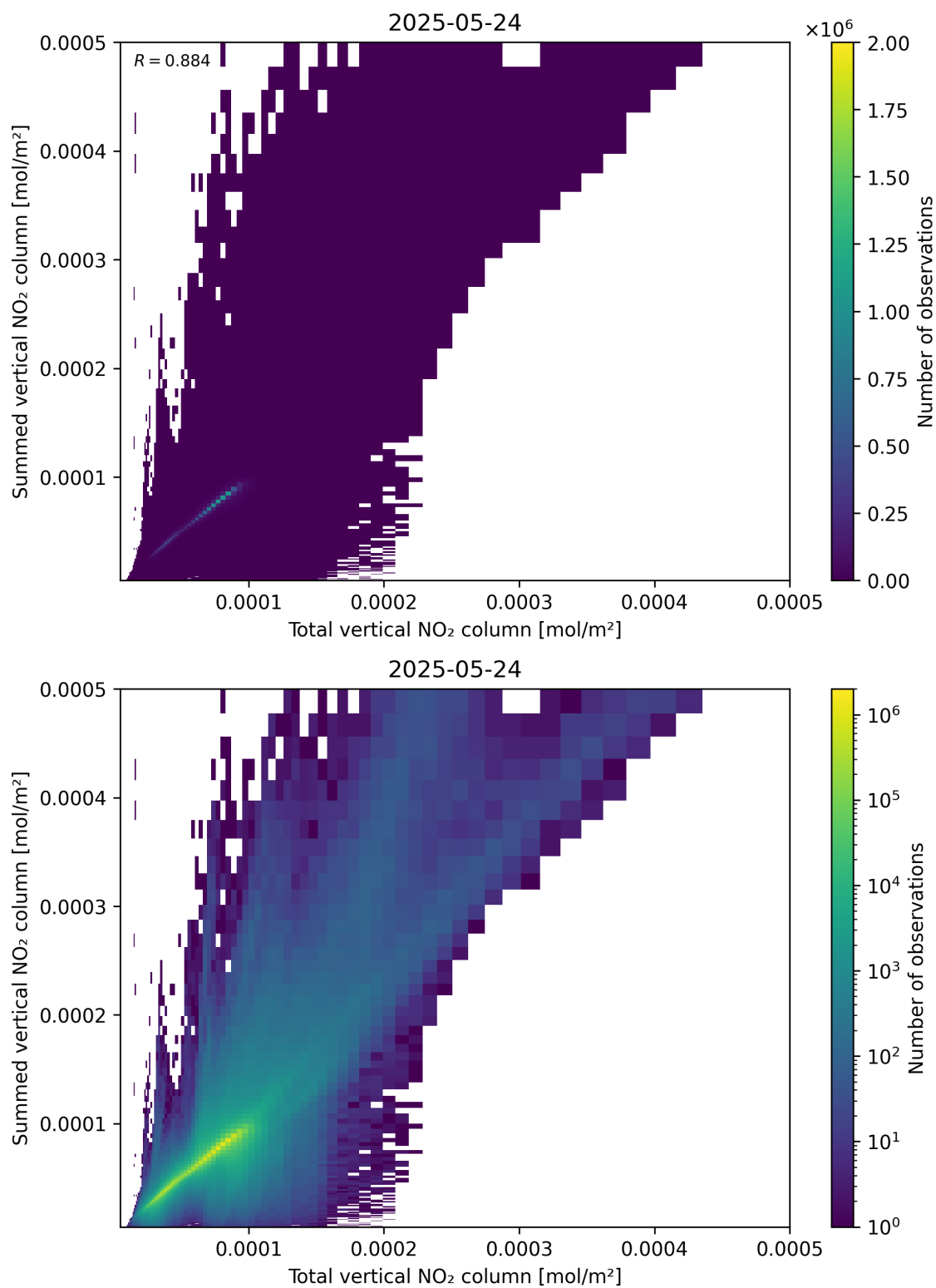
Figure 112: Scatter density plot of “Total vertical NO 2 column” against “Summed vertical NO 2 column” for 2025-05-23 to 2025-05-25.
