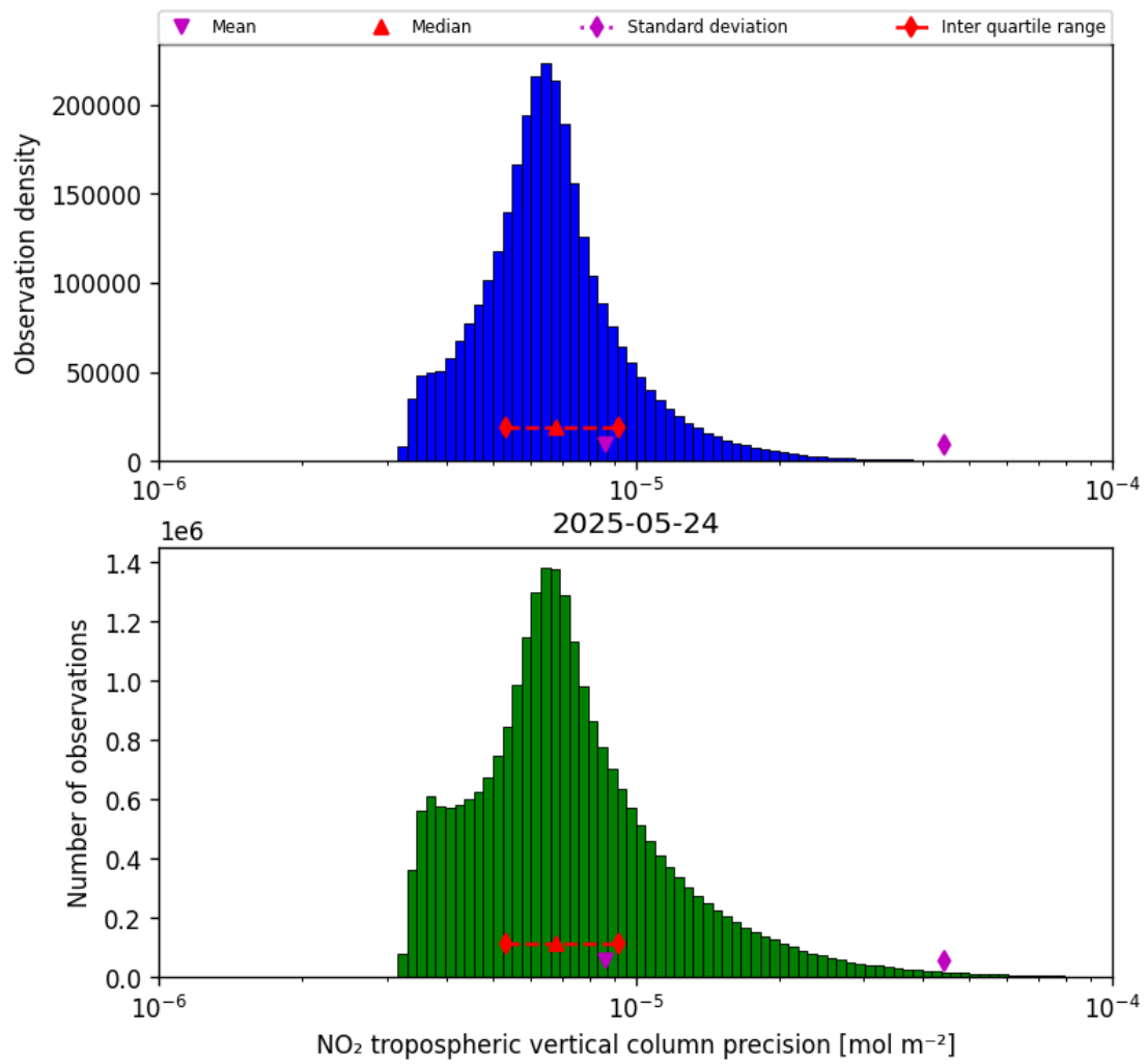
Figure 30: Histogram of “NO 2 tropospheric vertical column precision” for 2025-05-23 to 2025-05-25
