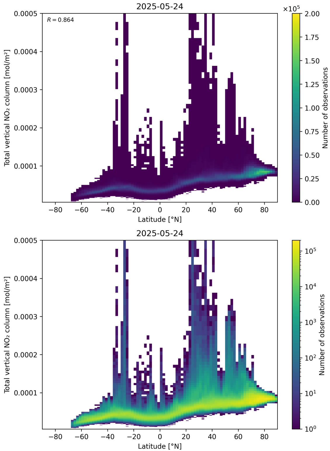
Figure 90: Scatter density plot of “Latitude” against “Total vertical NO 2 column” for 2025-05-23 to 2025-05-25.
