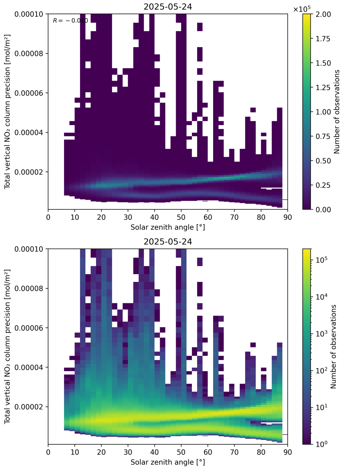
Figure 154: Scatter density plot of “Solar zenith angle” against “Total vertical NO 2 column precision” for 2025-05-23 to 2025-05-25.
