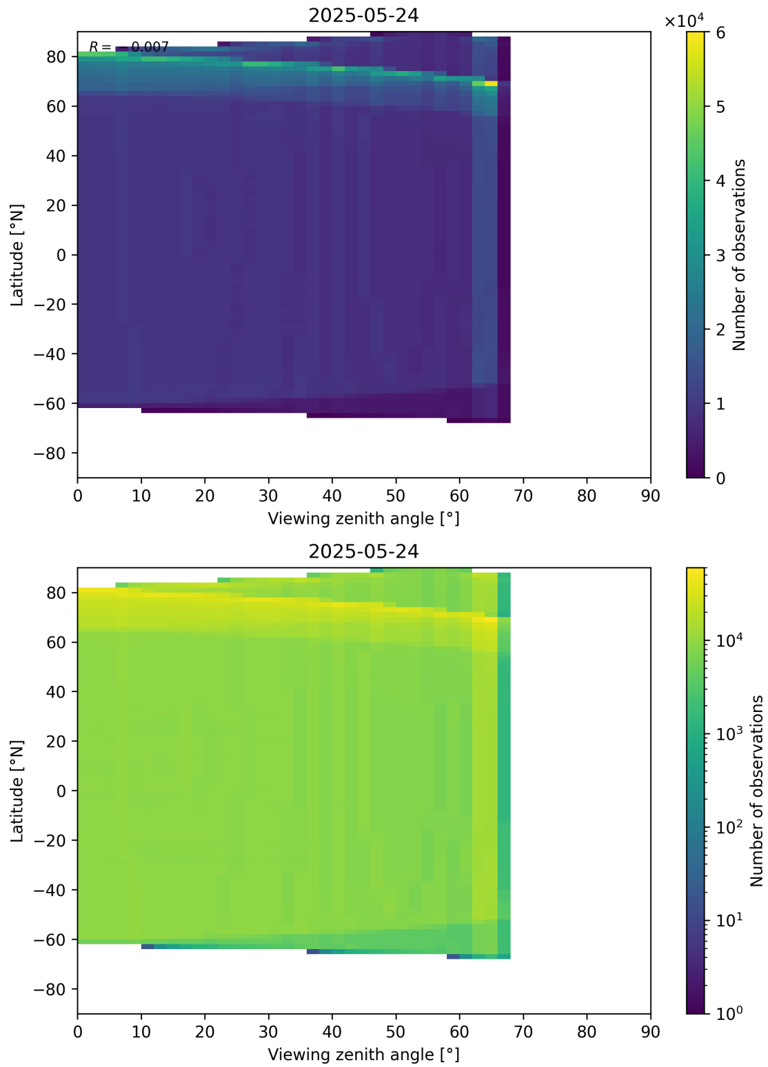
Figure 163: Scatter density plot of “Viewing zenith angle” against “Latitude” for 2025-05-23 to 2025-05-25.
