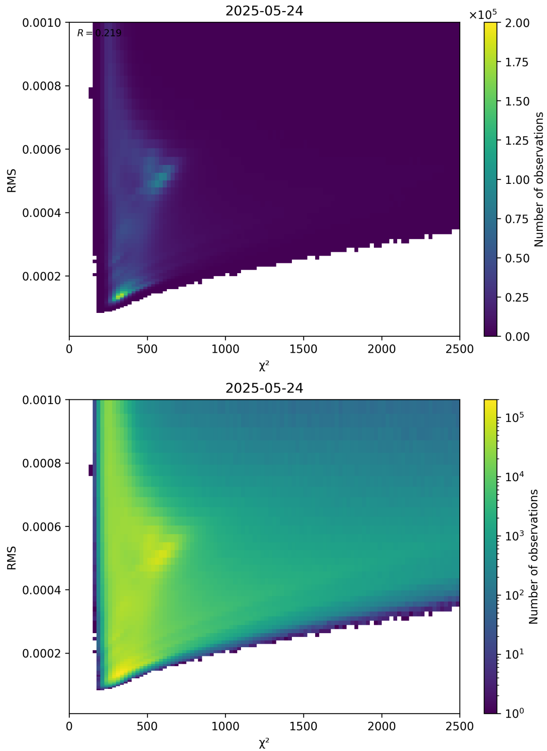
Figure 82: Scatter density plot of “ \chi^2 ” against “RMS” for 2025-05-23 to 2025-05-25.
