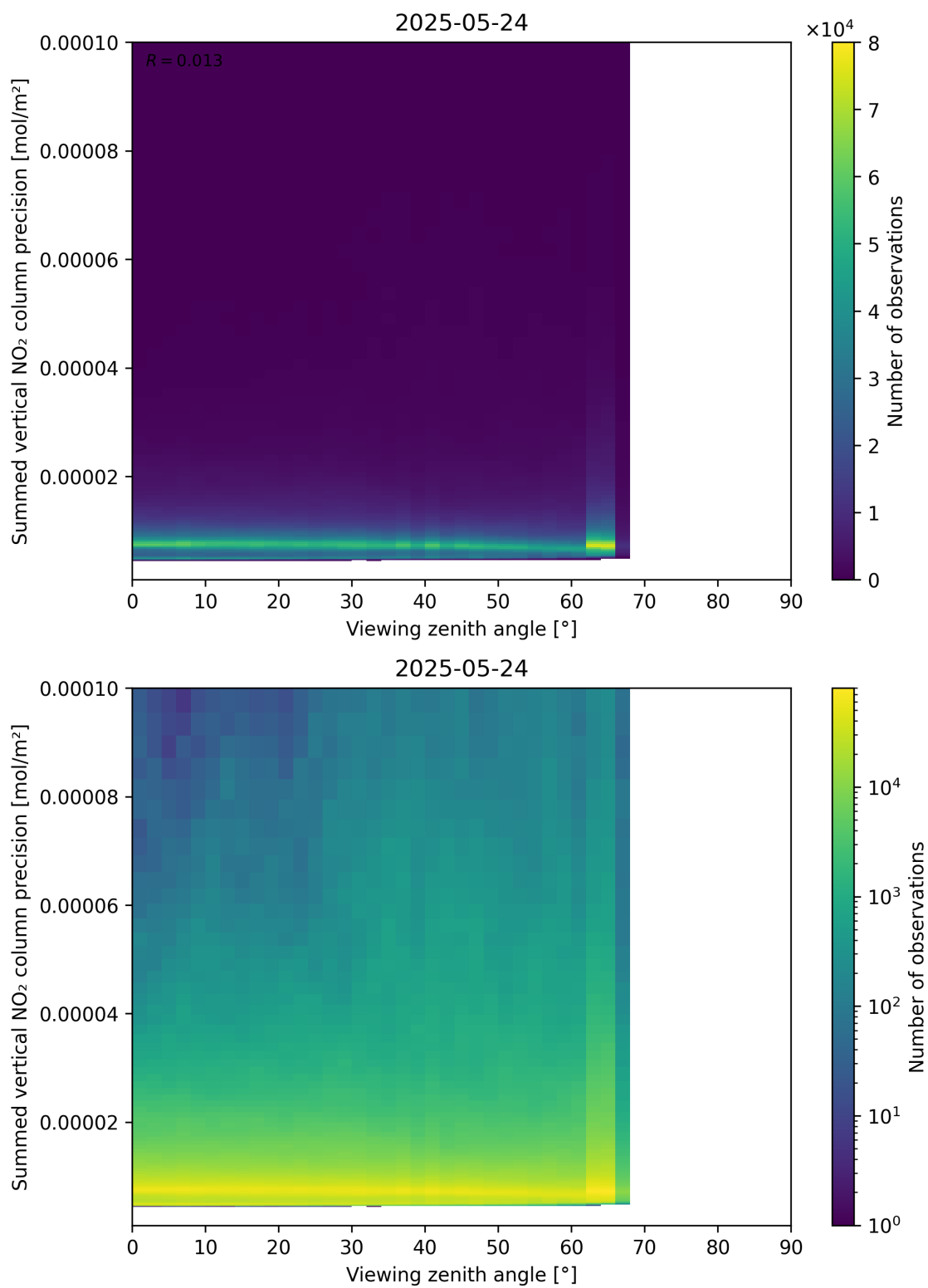
Figure 166: Scatter density plot of “Viewing zenith angle” against “Summed vertical NO 2 column precision” for 2025-05-23 to 2025-05-25.
