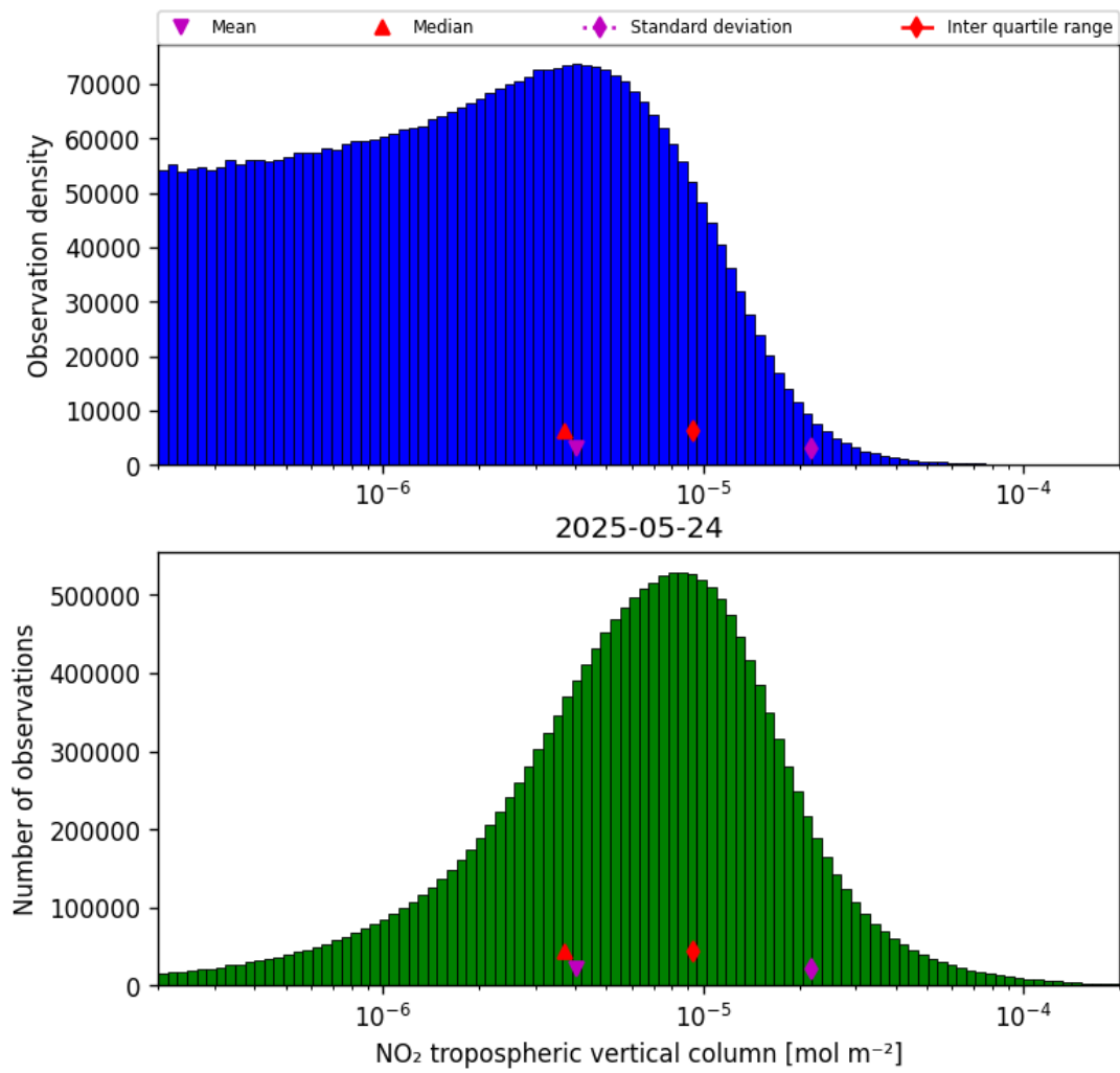
Figure 29: Histogram of “NO 2 tropospheric vertical column” for 2025-05-23 to 2025-05-25
