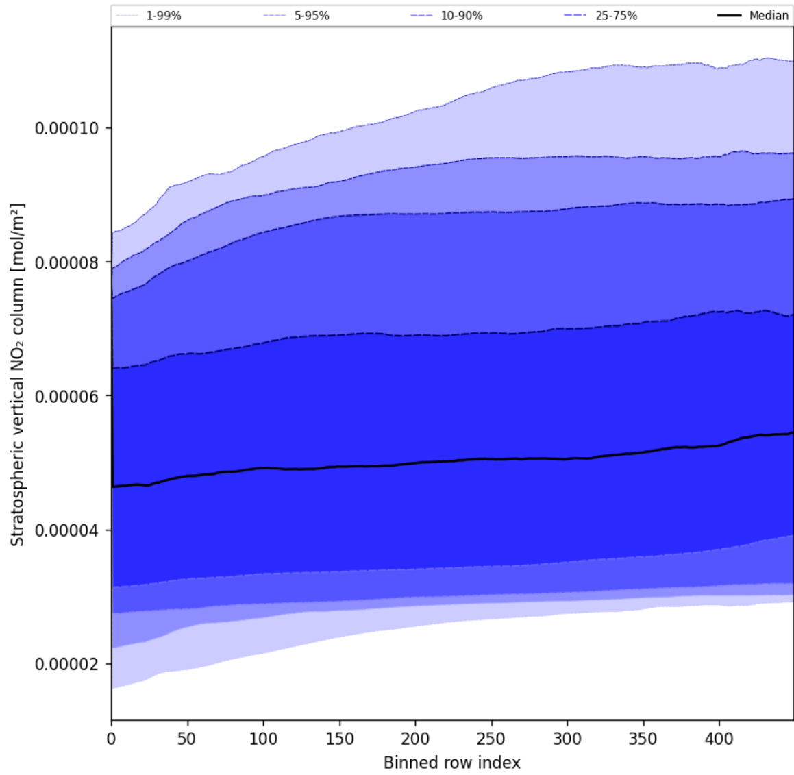
Figure 53: Along track statistics of “Stratospheric vertical NO 2 column” for 2025-05-23 to 2025-05-25
