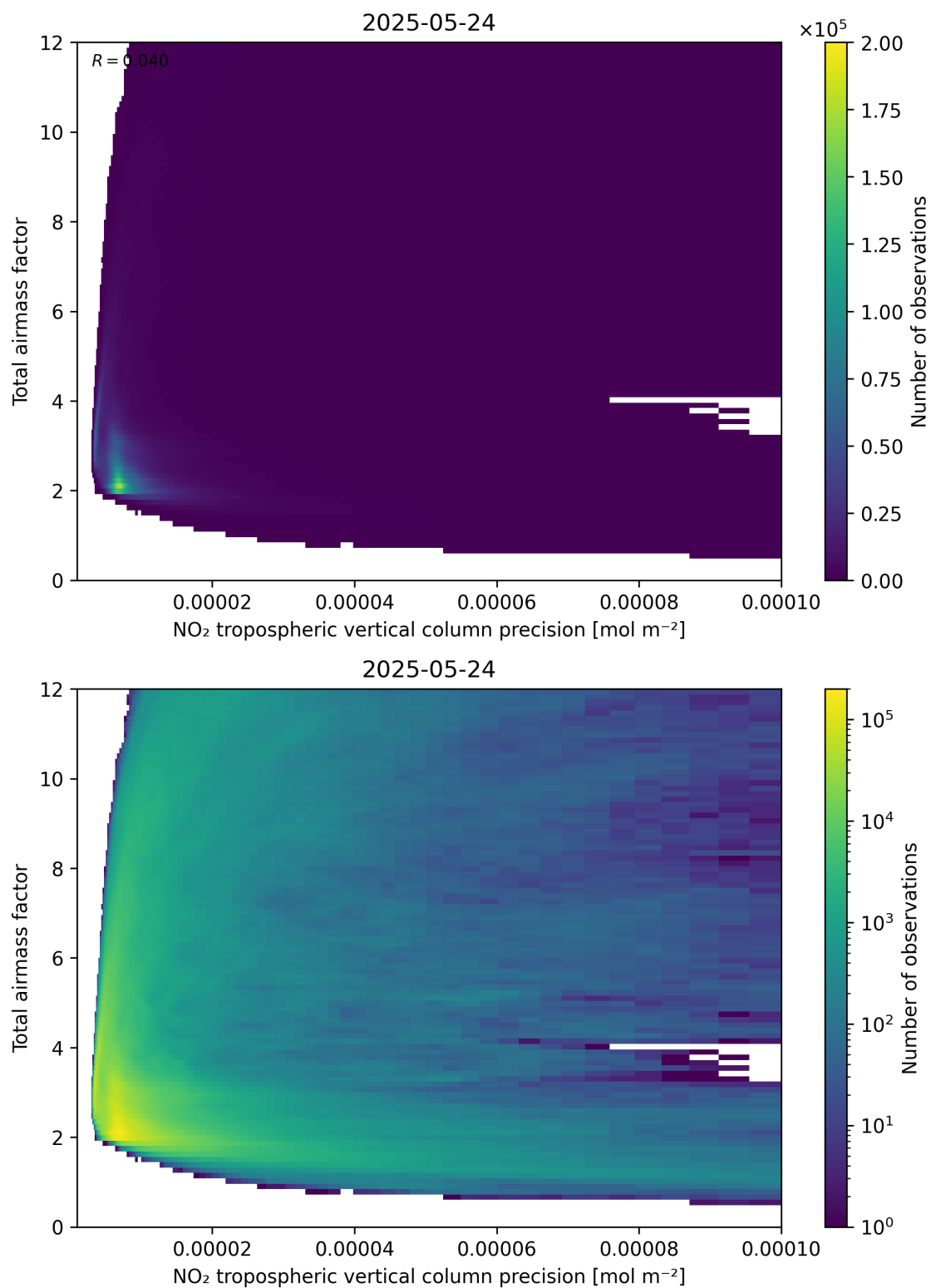
Figure 132: Scatter density plot of “NO 2 tropospheric vertical column precision” against “Total air mass factor” for 2025-05-23 to 2025-05-25.
