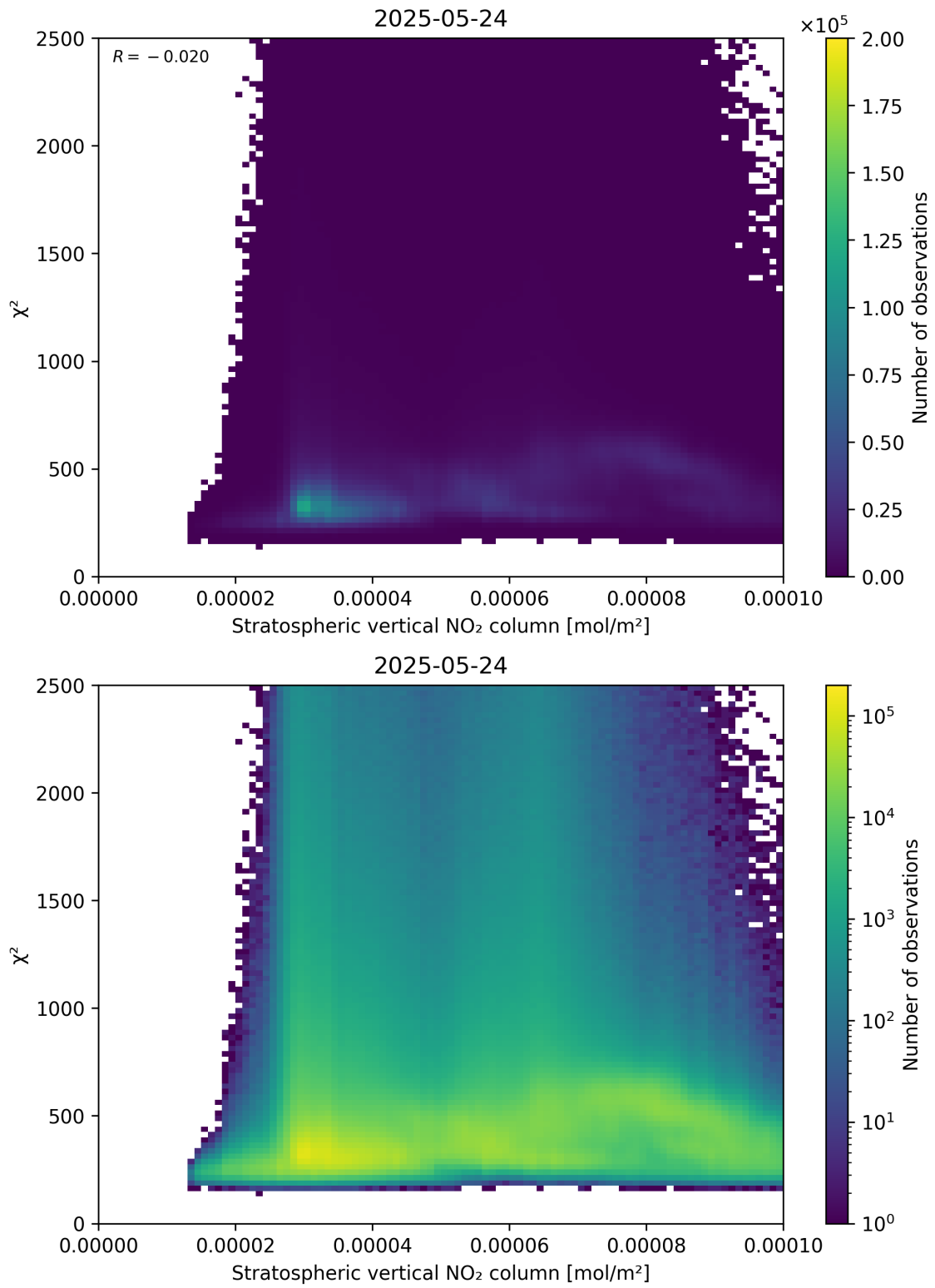
Figure 97: Scatter density plot of “Stratospheric vertical NO 2 column” against “ \chi^2 ” for 2025-05-23 to 2025-05-25.
