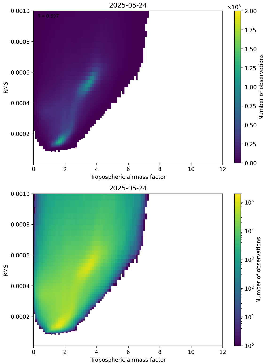
Figure 79: Scatter density plot of “Tropospheric airmass factor” against “RMS” for 2025-05-23 to 2025-05-25.
