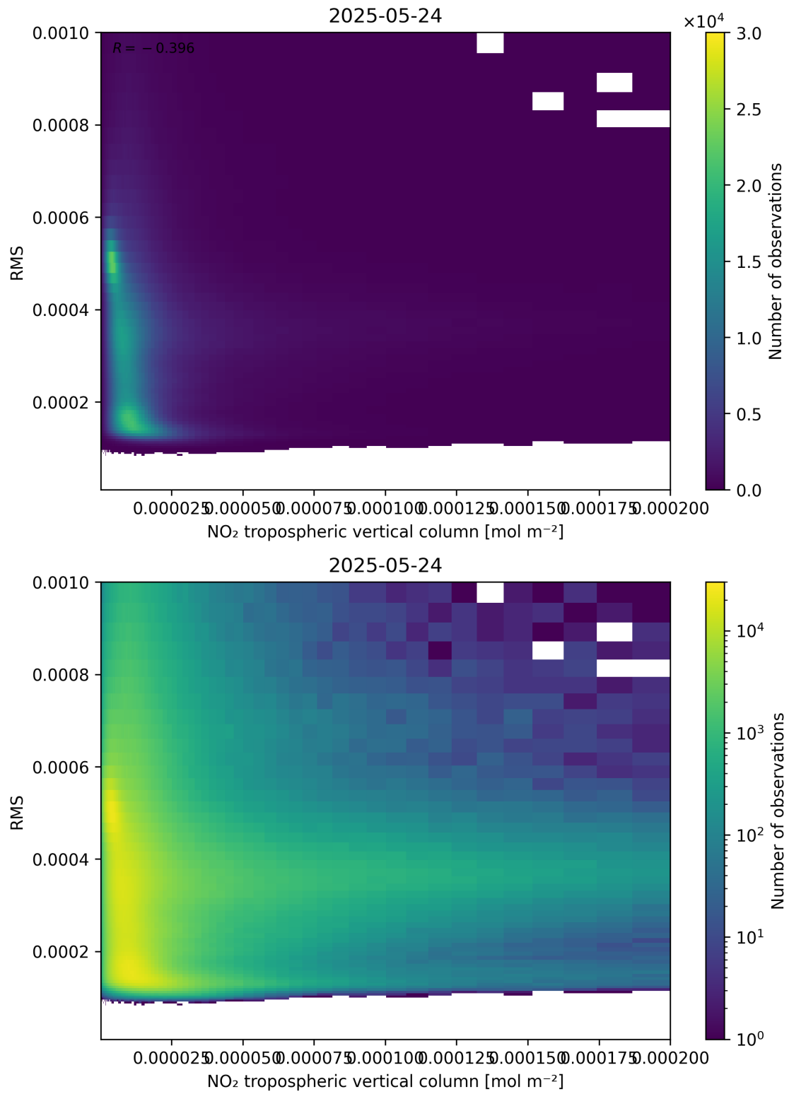
Figure 142: Scatter density plot of “NO 2 tropospheric vertical column” against “RMS” for 2025-05-23 to 2025-05-25.
