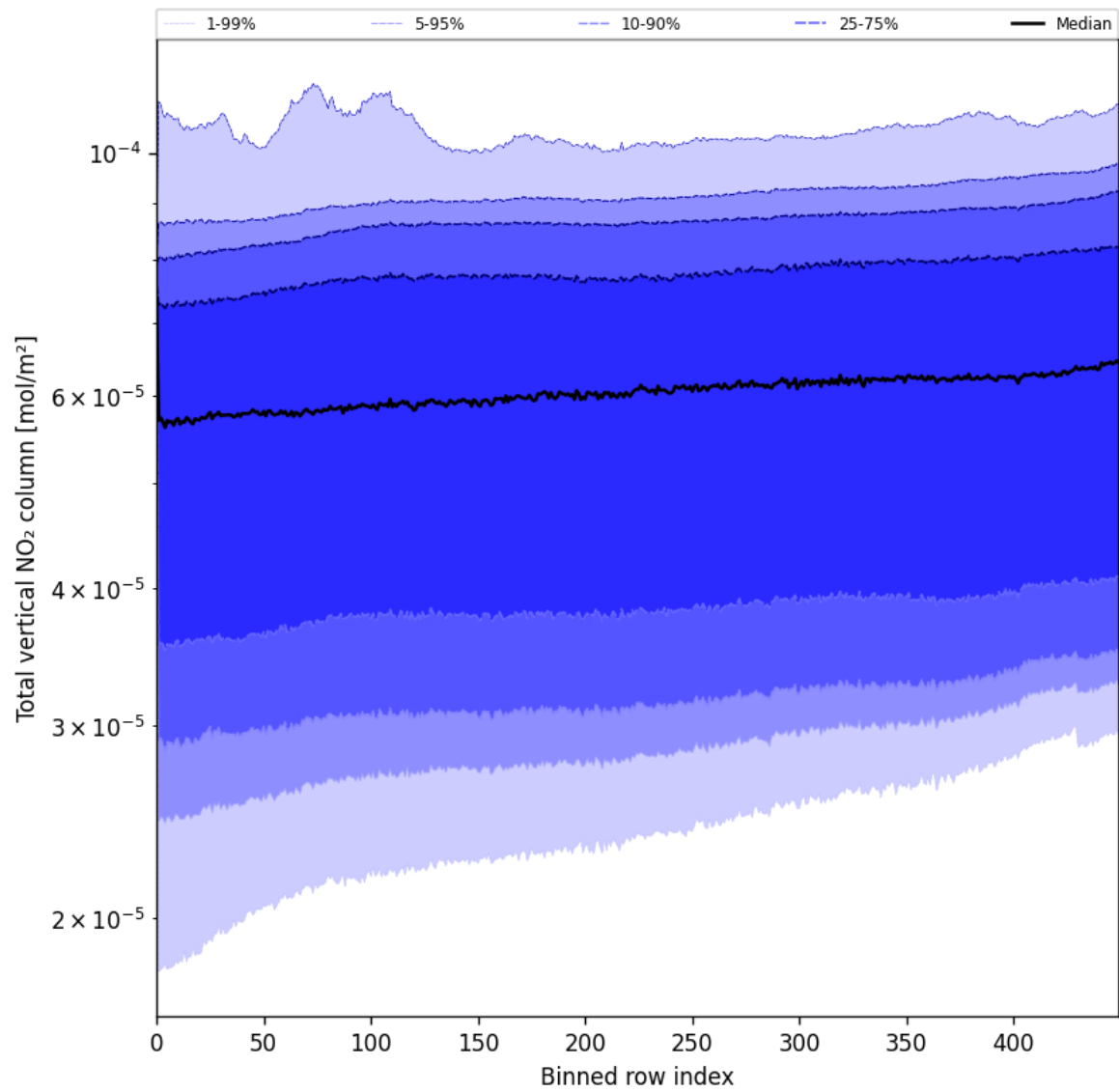
Figure 55: Along track statistics of “Total vertical NO 2 column” for 2025-05-23 to 2025-05-25
