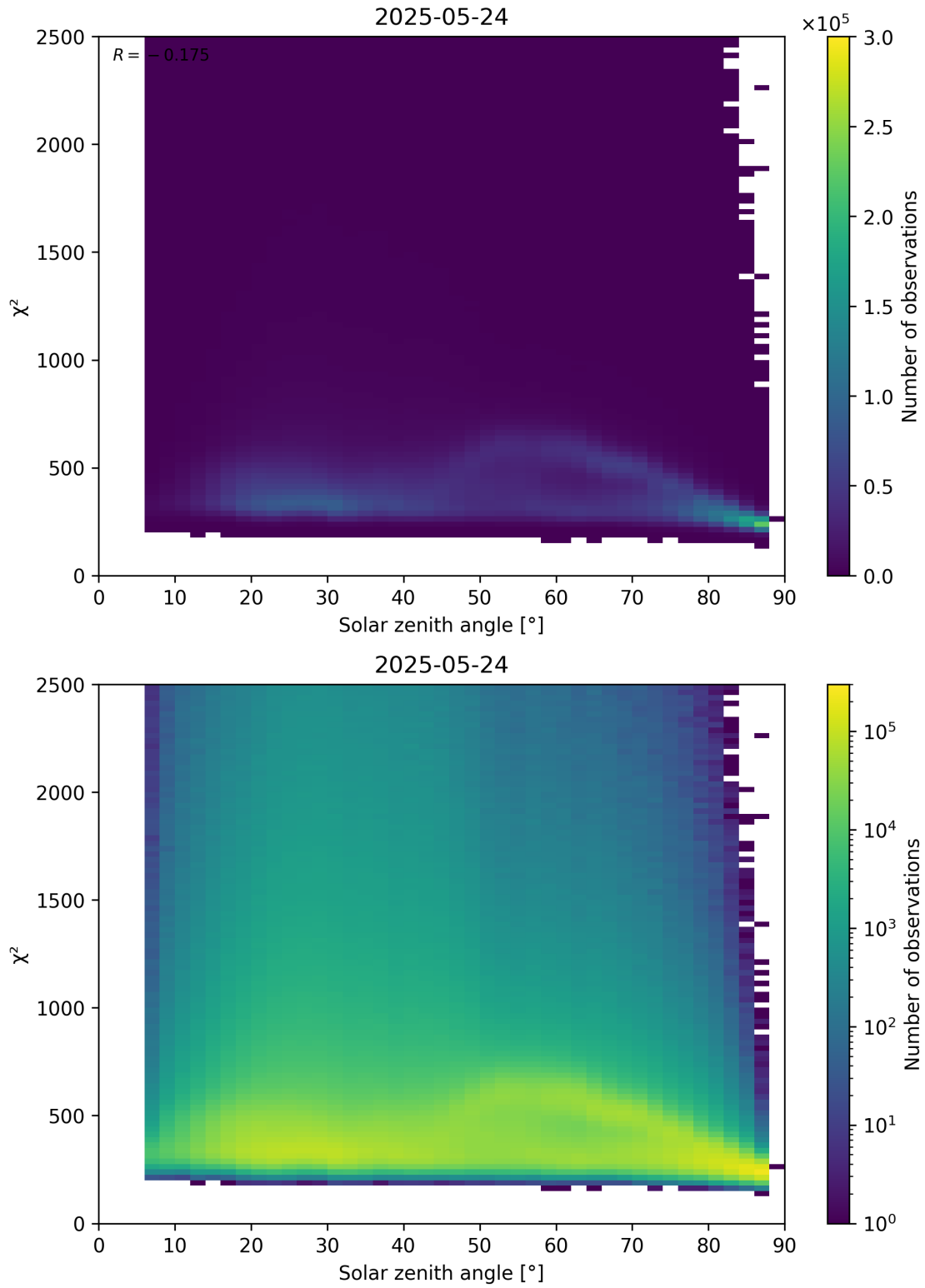
Figure 148: Scatter density plot of “Solar zenith angle” against “ \chi^2 ” for 2025-05-23 to 2025-05-25.
