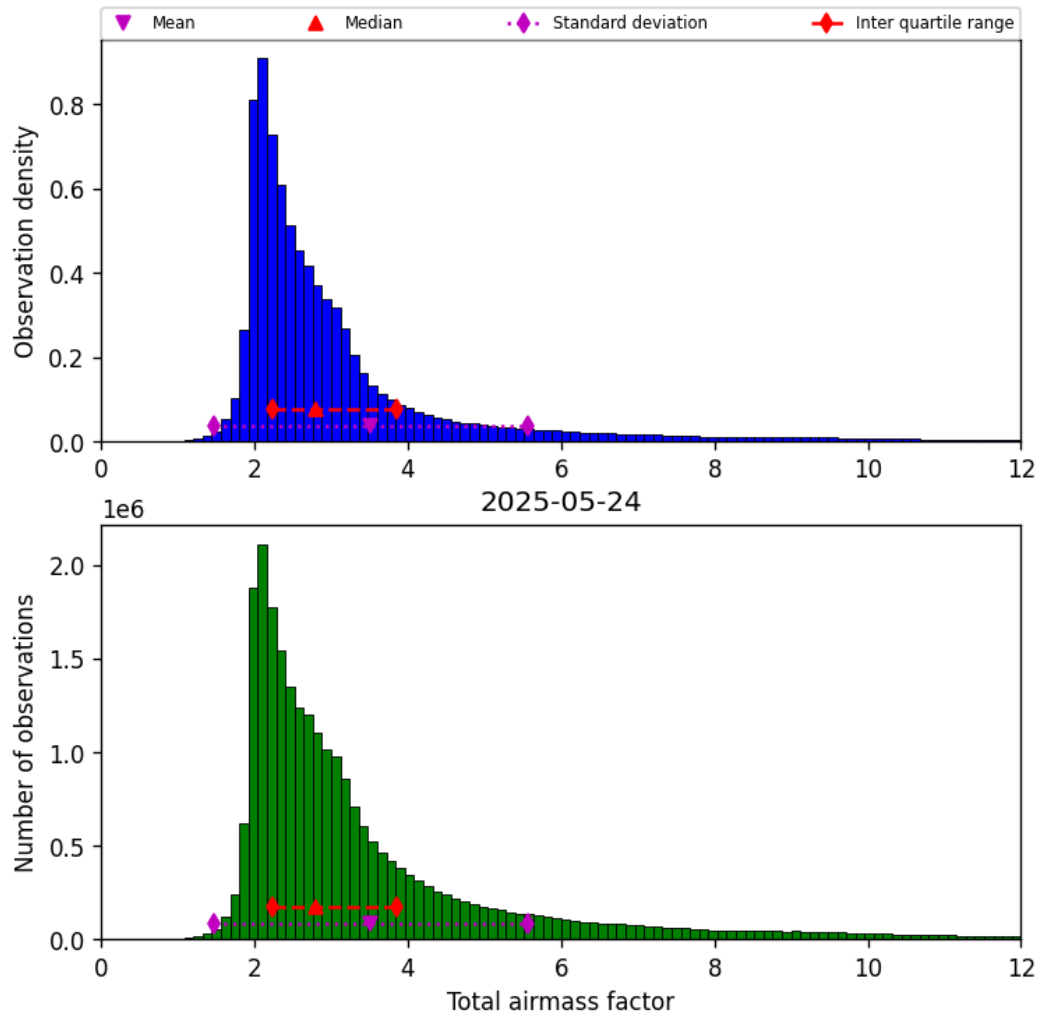
Figure 32: Histogram of “Total airmass factor” for 2025-05-23 to 2025-05-25
