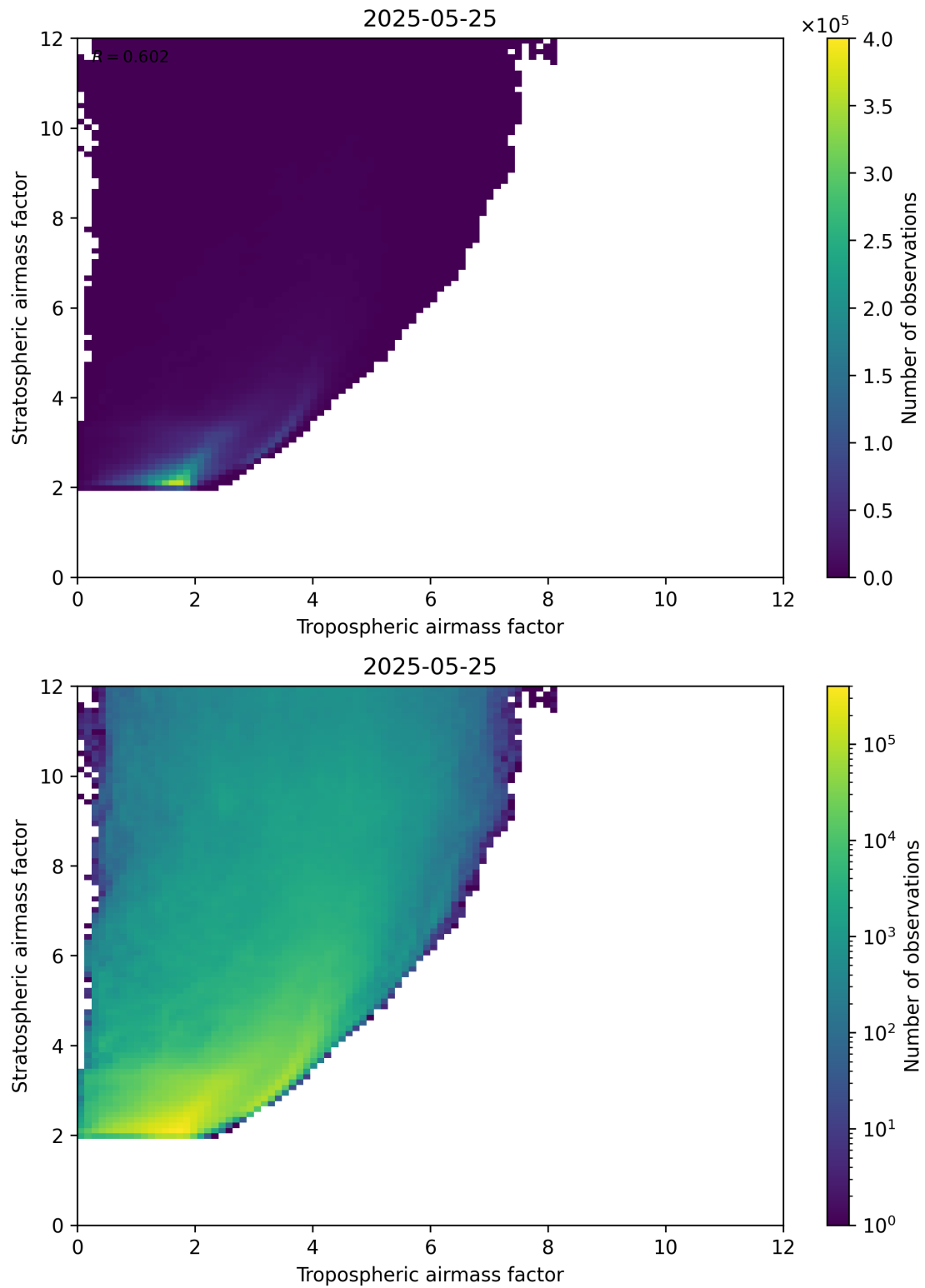
Figure 71: Scatter density plot of “Tropospheric airmass factor” against “Stratospheric airmass factor” for 2025-05-24 to 2025-05-26.
