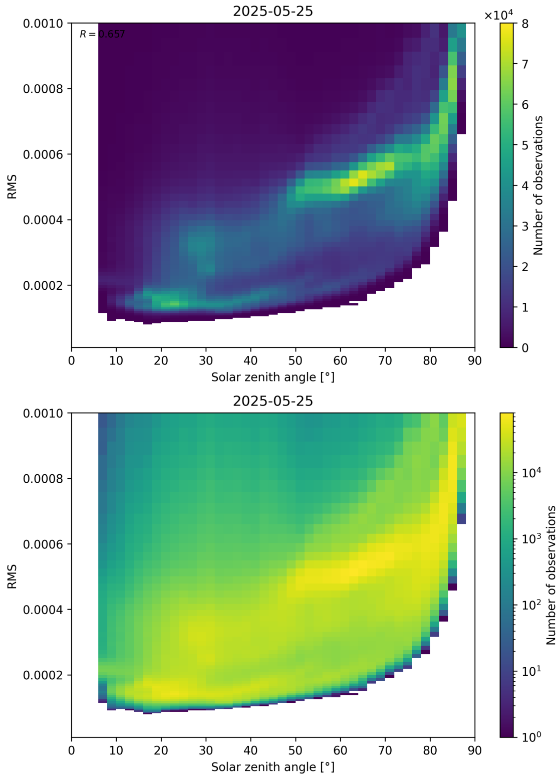
Figure 157: Scatter density plot of “Solar zenith angle” against “RMS” for 2025-05-24 to 2025-05-26.
