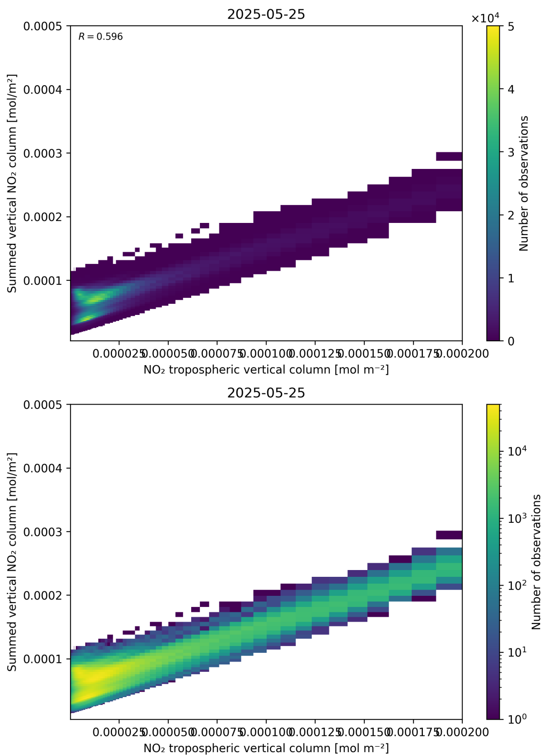
Figure 126: Scatter density plot of “NO 2 tropospheric vertical column” against “Summed vertical NO 2 column” for 2025-05-24 to 2025-05-26.
