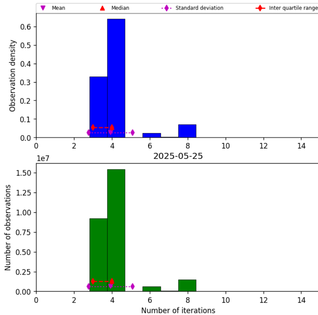
Figure 34: Histogram of “Number of iterations” for 2025-05-24 to 2025-05-26
