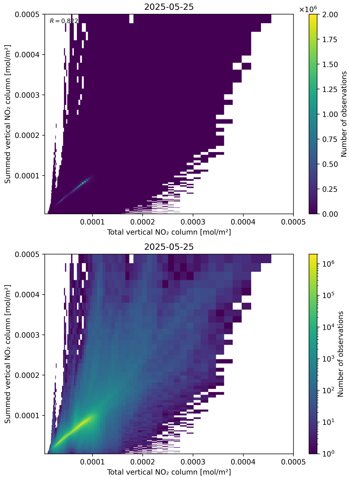
Figure 112: Scatter density plot of “Total vertical NO 2 column” against “Summed vertical NO 2 column” for 2025-05-24 to 2025-05-26.
