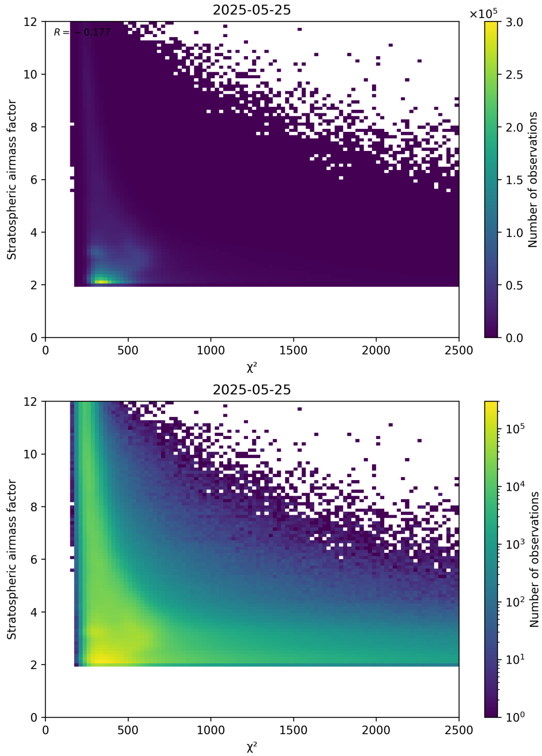
Figure 81: Scatter density plot of “ \chi^2 ” against “Stratospheric airmass factor” for 2025-05-24 to 2025-05-26.
