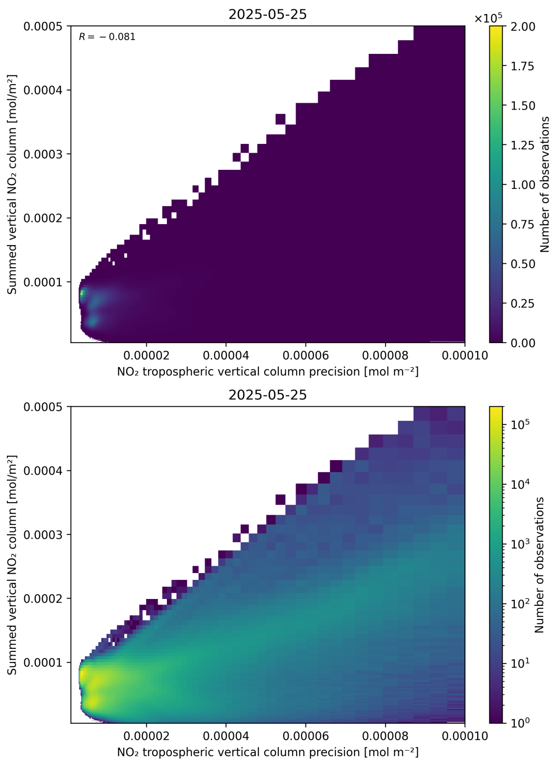
Figure 136: Scatter density plot of “NO 2 tropospheric vertical column precision” against “Summed vertical NO 2 column” for 2025-05-24 to 2025-05-26.
