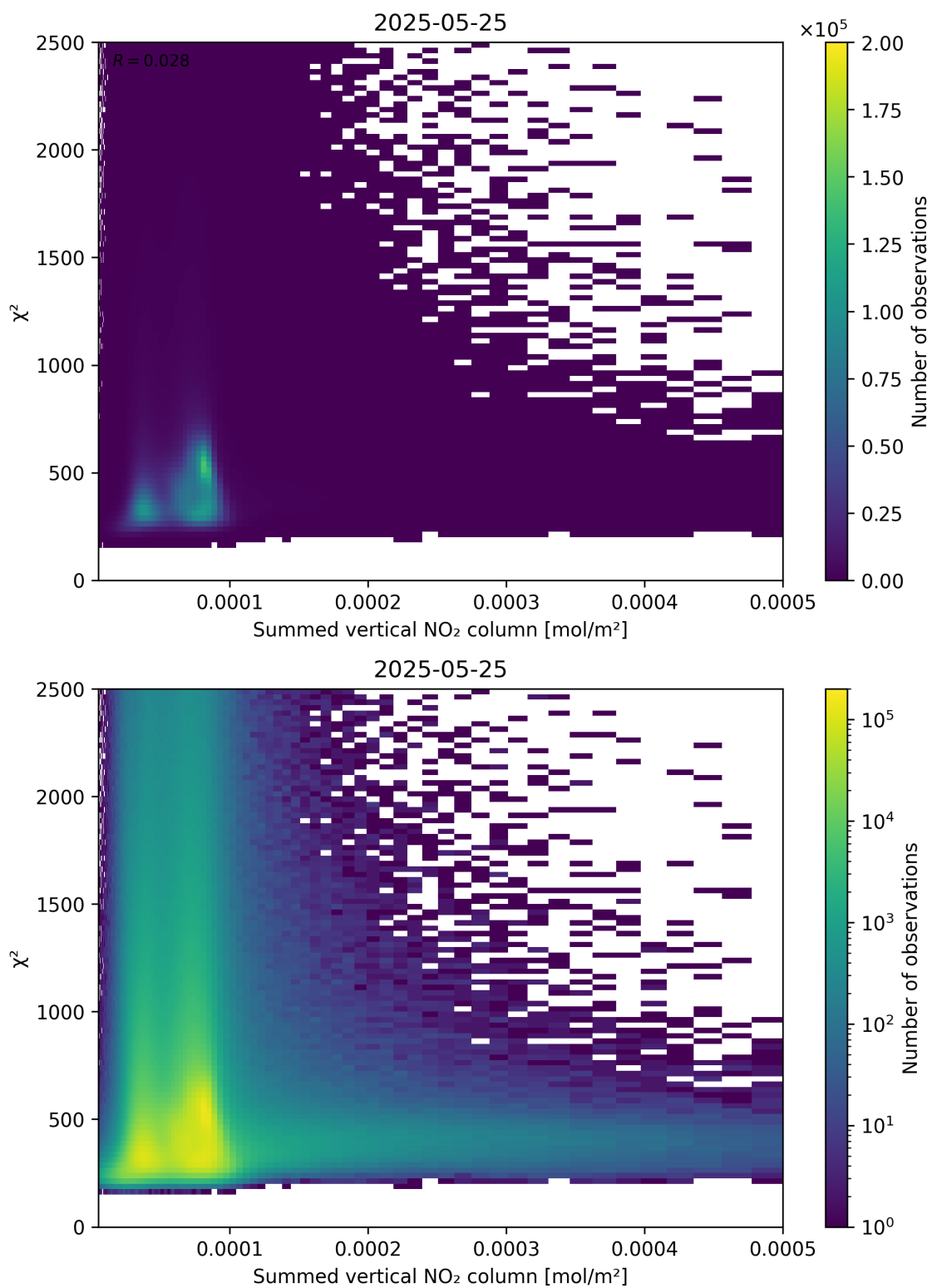
Figure 104: Scatter density plot of “Summed vertical NO 2 column” against “ \chi^2 ” for 2025-05-24 to 2025-05-26.
