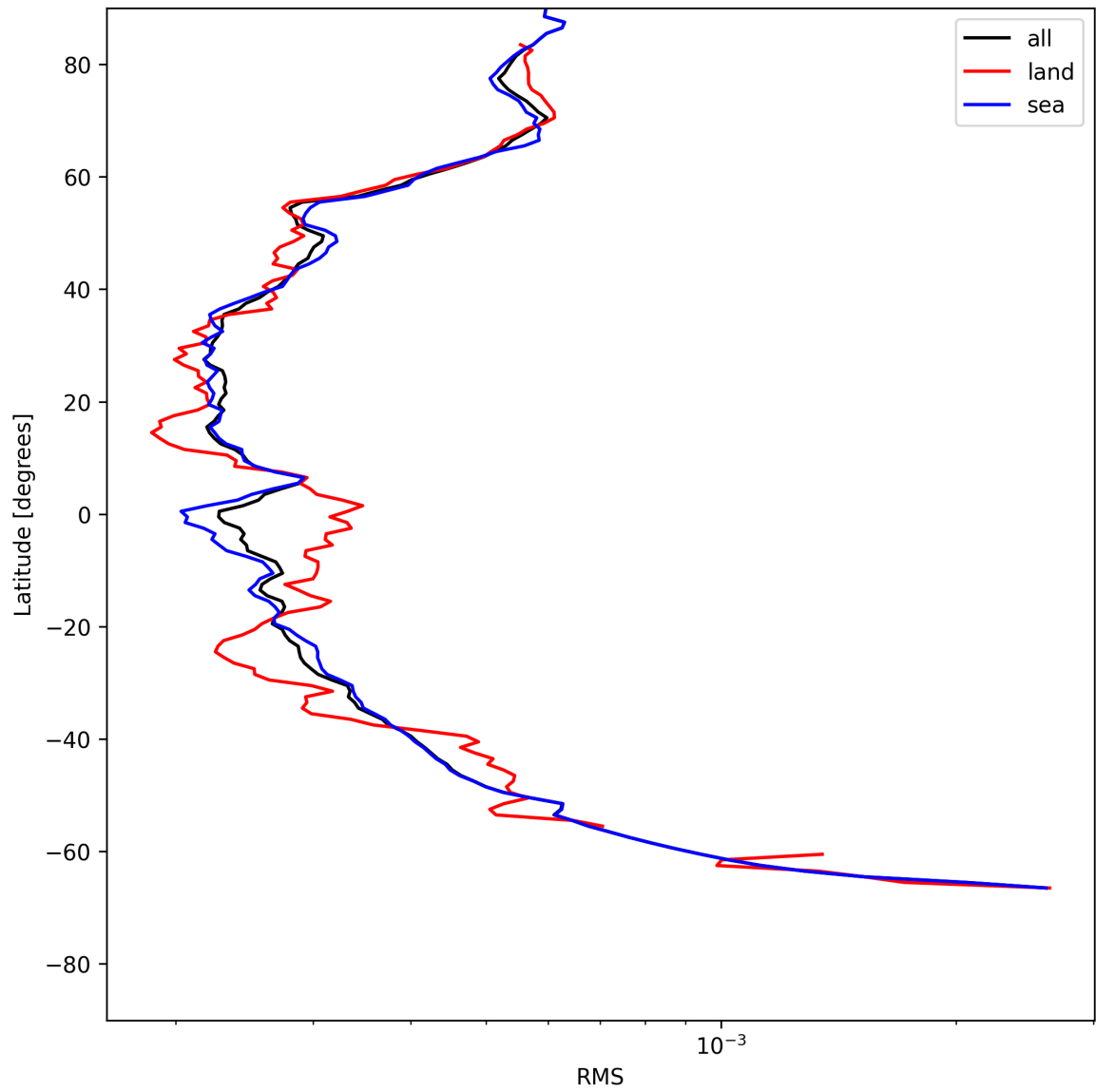
Figure 26: Zonal average of “RMS” for 2025-05-24 to 2025-05-26.
