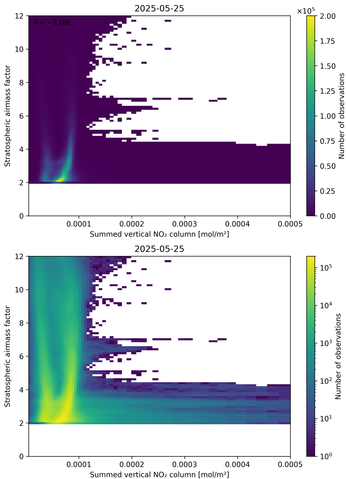
Figure 103: Scatter density plot of “Summed vertical NO 2 column” against “Stratospheric air mass factor” for 2025-05-24 to 2025-05-26.
