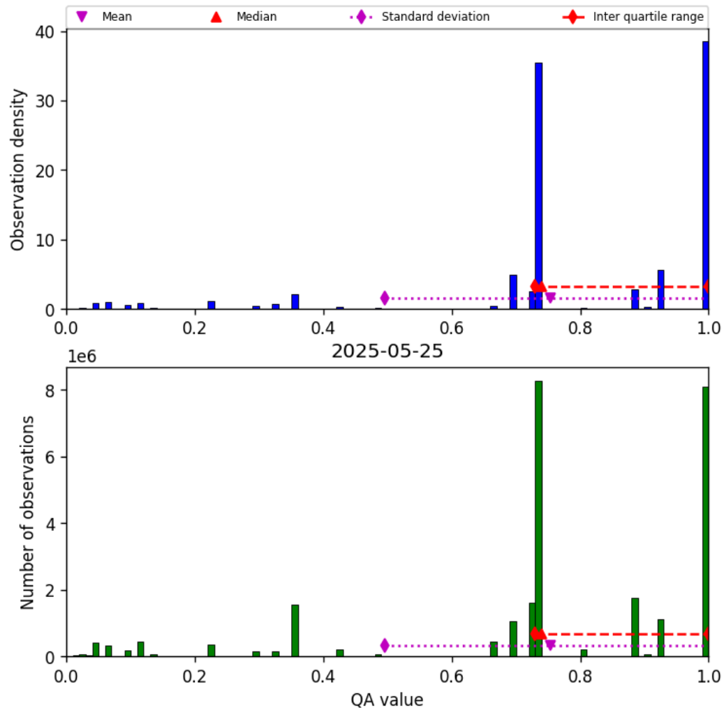
Figure 28: Histogram of “QA value” for 2025-05-24 to 2025-05-26
