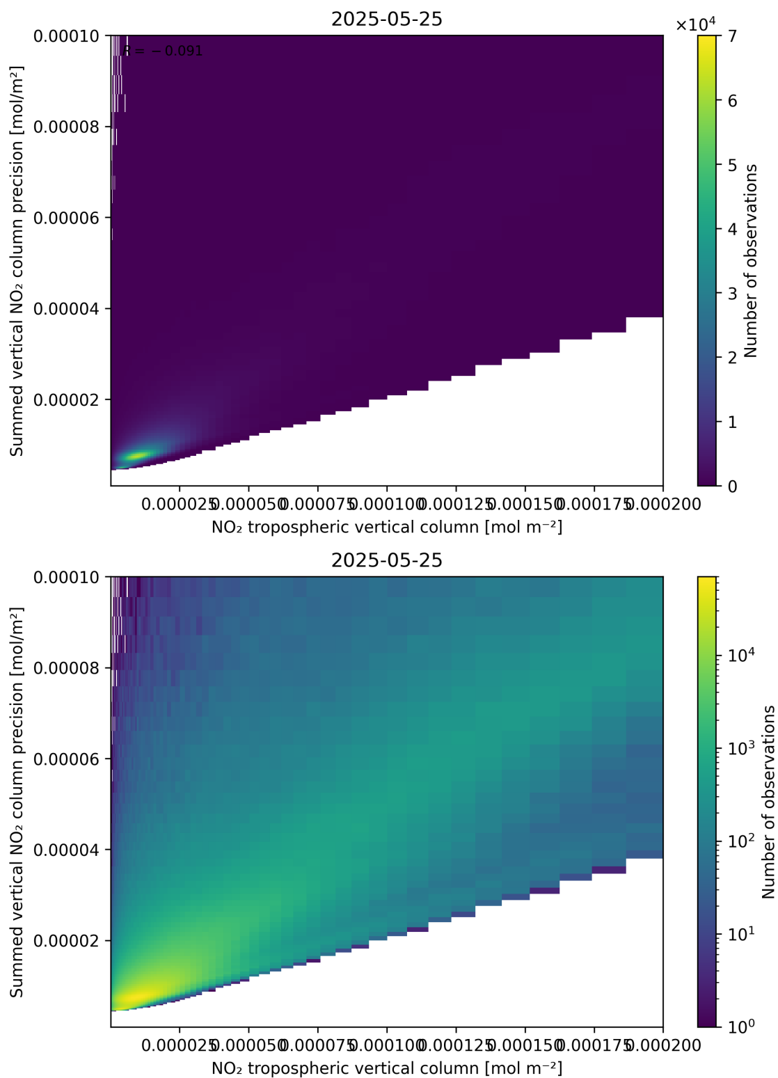
Figure 127: Scatter density plot of “NO 2 tropospheric vertical column” against “Summed vertical NO 2 column precision” for 2025-05-24 to 2025-05-26.
