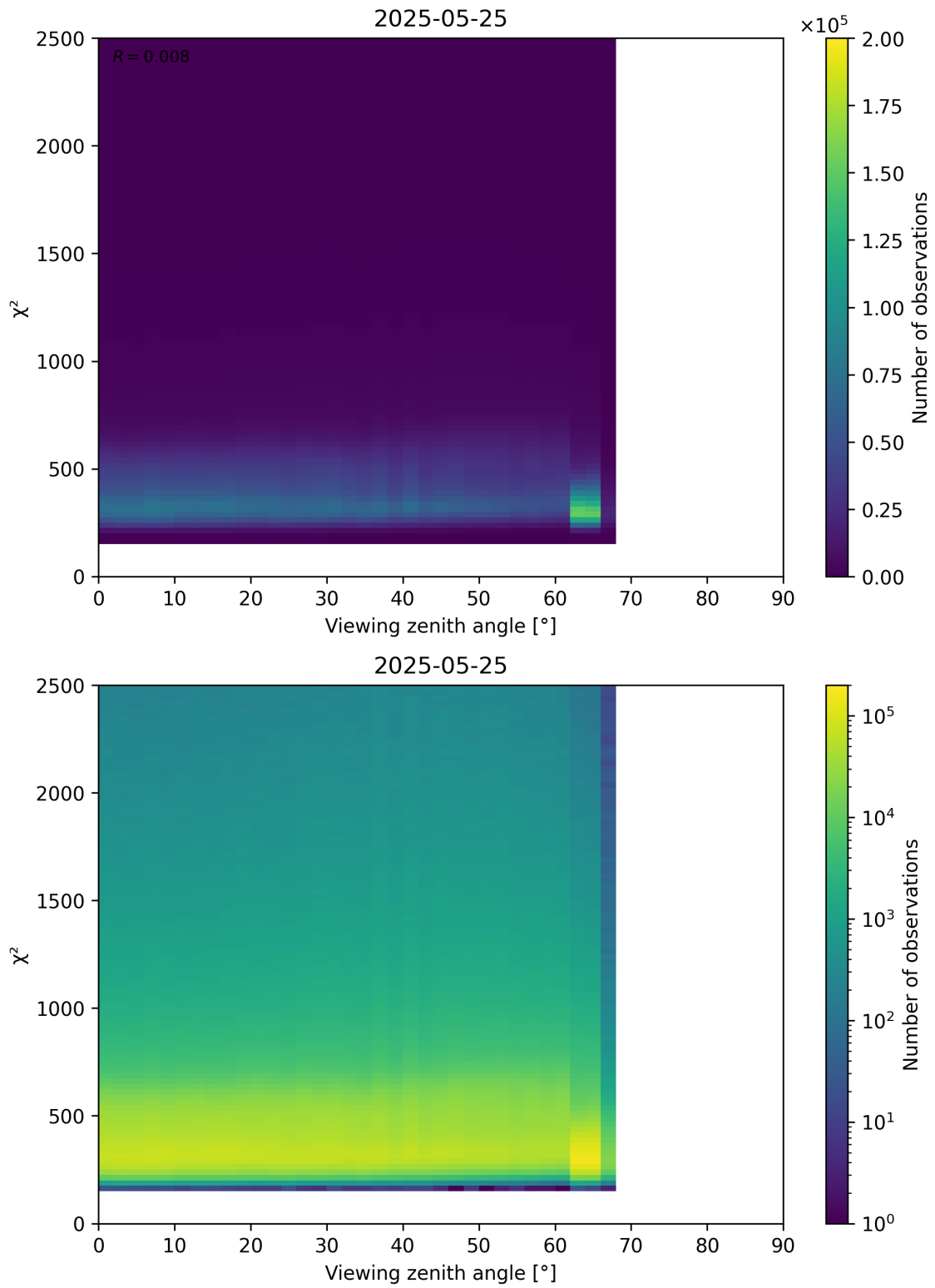
Figure 162: Scatter density plot of “Viewing zenith angle” against “ \chi^2 ” for 2025-05-24 to 2025-05-26.
