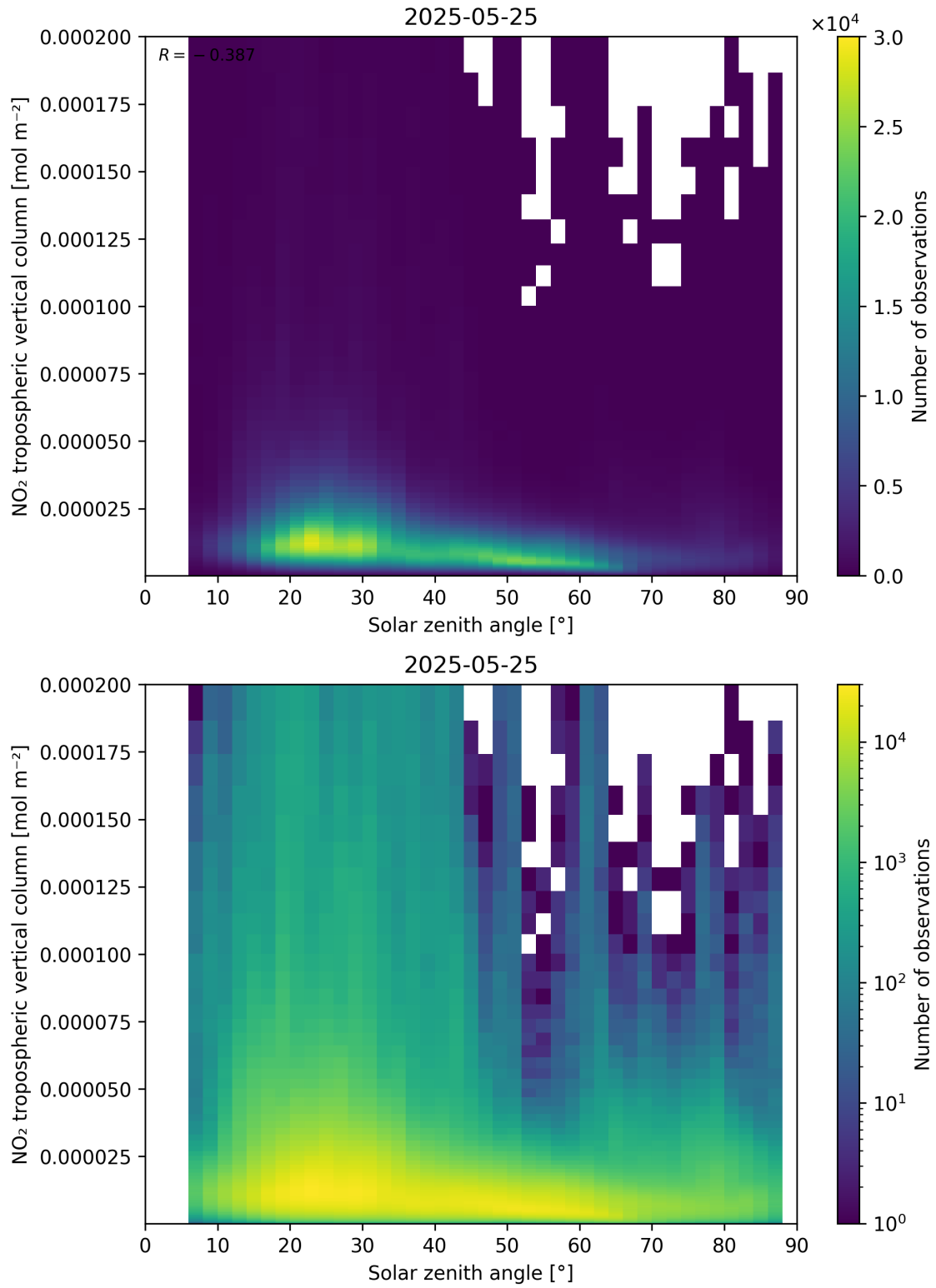
Figure 155: Scatter density plot of “Solar zenith angle” against “NO 2 tropospheric vertical column” for 2025-05-24 to 2025-05-26.
