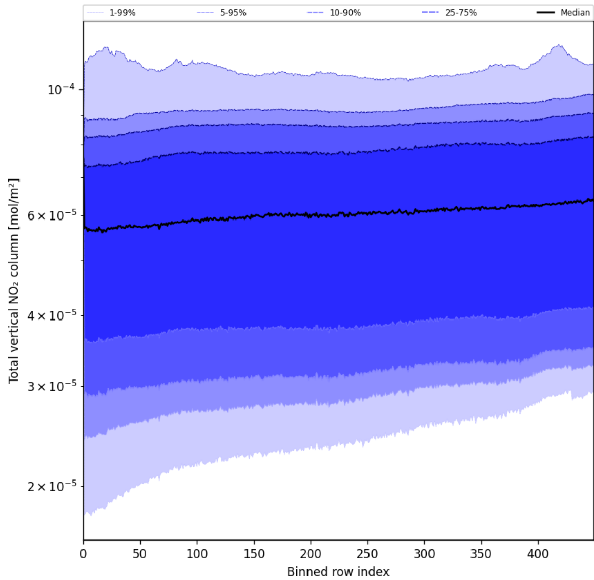
Figure 55: Along track statistics of “Total vertical NO 2 column” for 2025-05-24 to 2025-05-26
