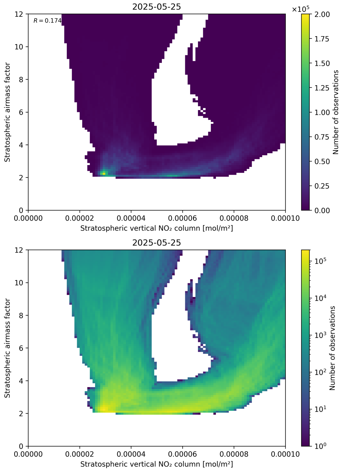
Figure 96: Scatter density plot of “Stratospheric vertical NO 2 column” against “Stratospheric airmass factor” for 2025-05-24 to 2025-05-26.
