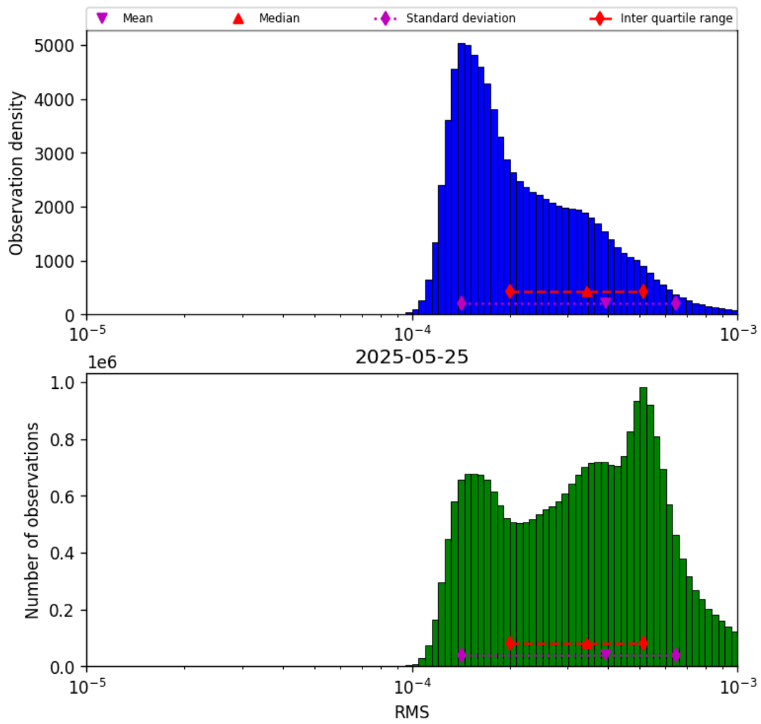
Figure 43: Histogram of “RMS” for 2025-05-24 to 2025-05-26
