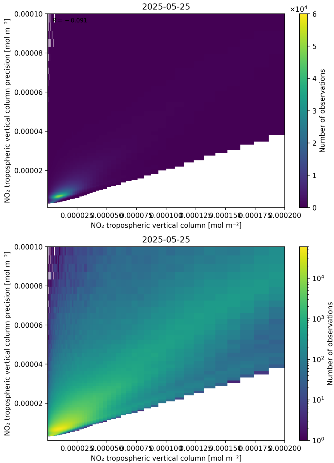
Figure 130: Scatter density plot of “NO 2 tropospheric vertical column” against “NO 2 tropospheric vertical column precision” for 2025-05-24 to 2025-05-26.
