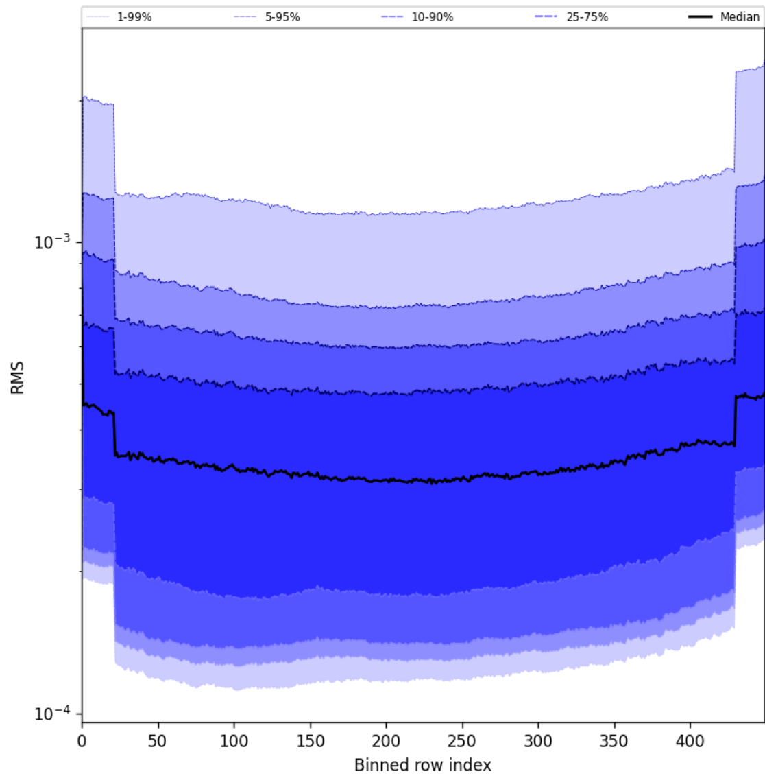
Figure 60: Along track statistics of “RMS” for 2025-05-24 to 2025-05-26
