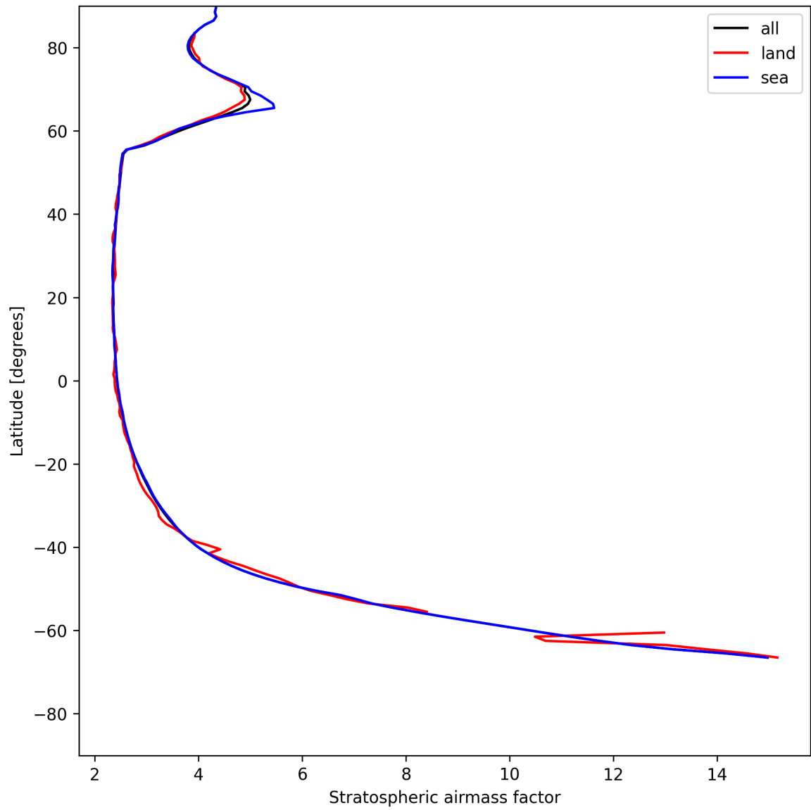
Figure 27: Zonal average of “Stratospheric airmass factor” for 2025-05-24 to 2025-05-26.
