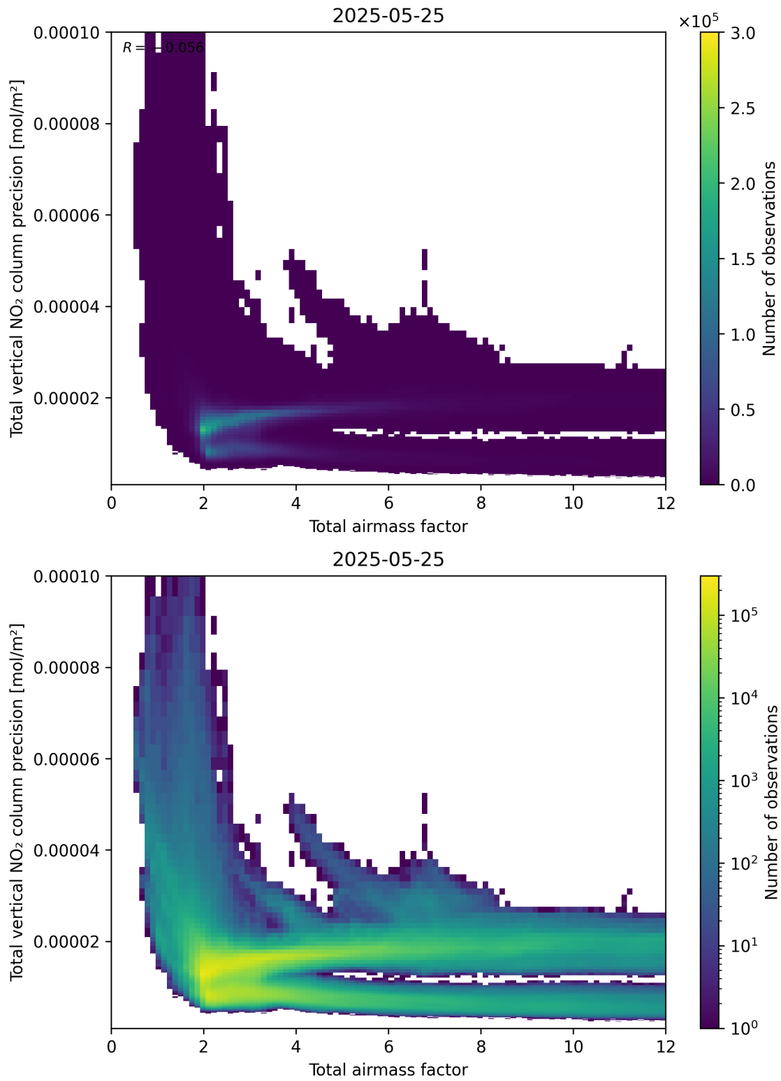
Figure 68: Scatter density plot of “Total airmass factor” against “Total vertical NO 2 column precision” for 2025-05-24 to 2025-05-26.
