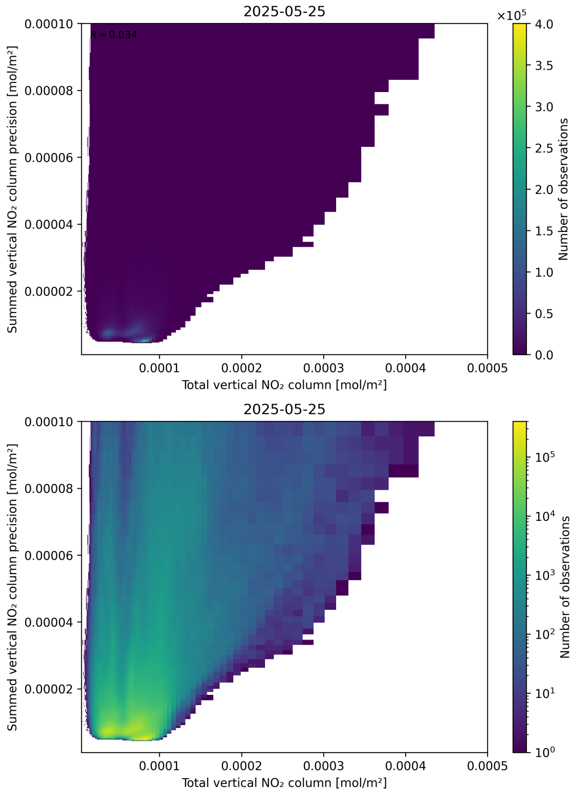
Figure 113: Scatter density plot of “Total vertical NO 2 column” against “Summed vertical NO 2 column precision” for 2025-05-24 to 2025-05-26.
