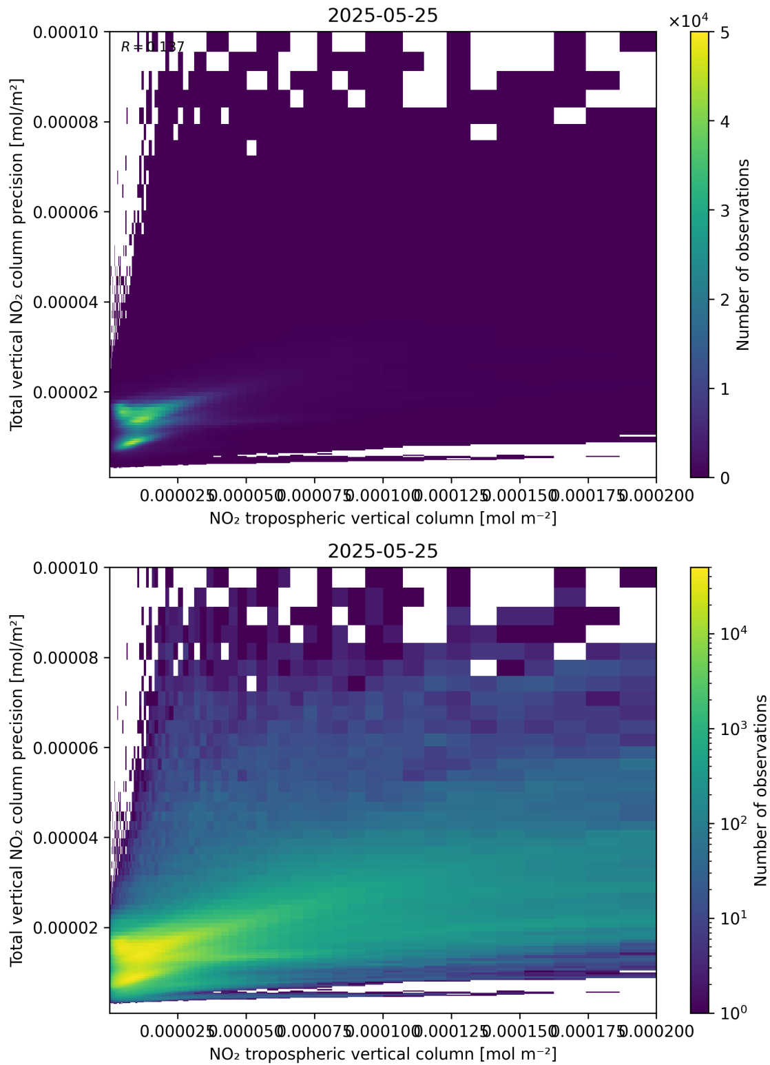
Figure 129: Scatter density plot of “NO 2 tropospheric vertical column” against “Total vertical NO 2 column precision” for 2025-05-24 to 2025-05-26.
