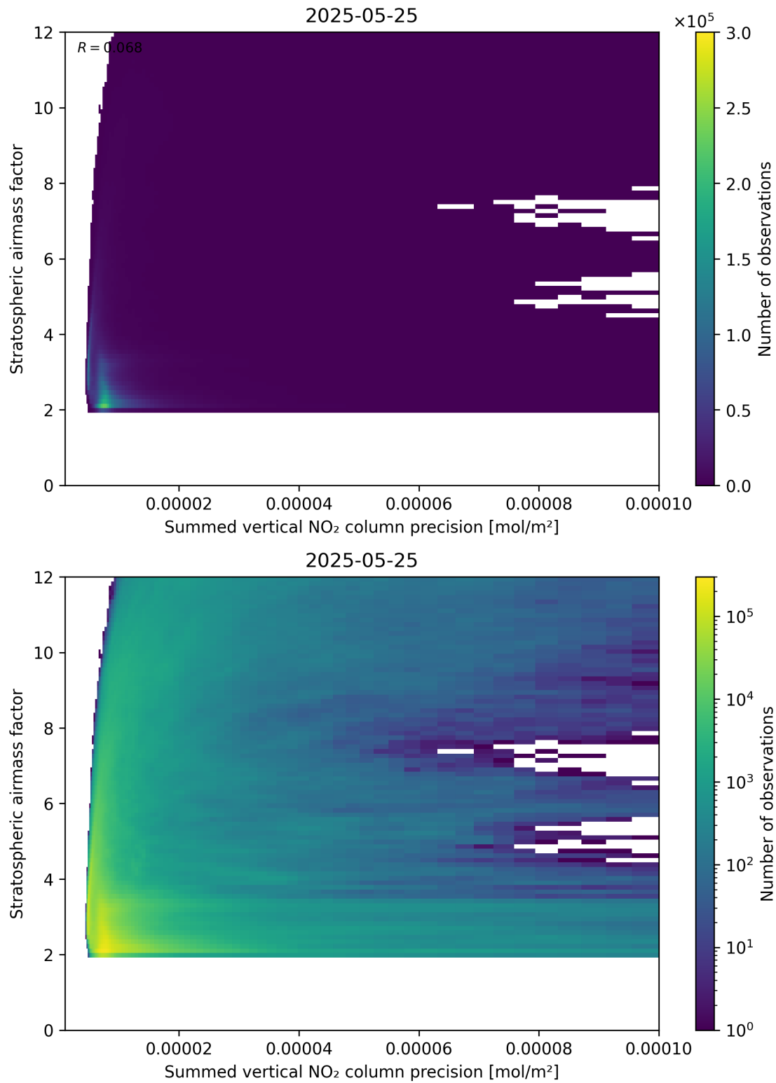
Figure 106: Scatter density plot of “Summed vertical NO 2 column precision” against “Stratospheric airmass factor” for 2025-05-24 to 2025-05-26.
