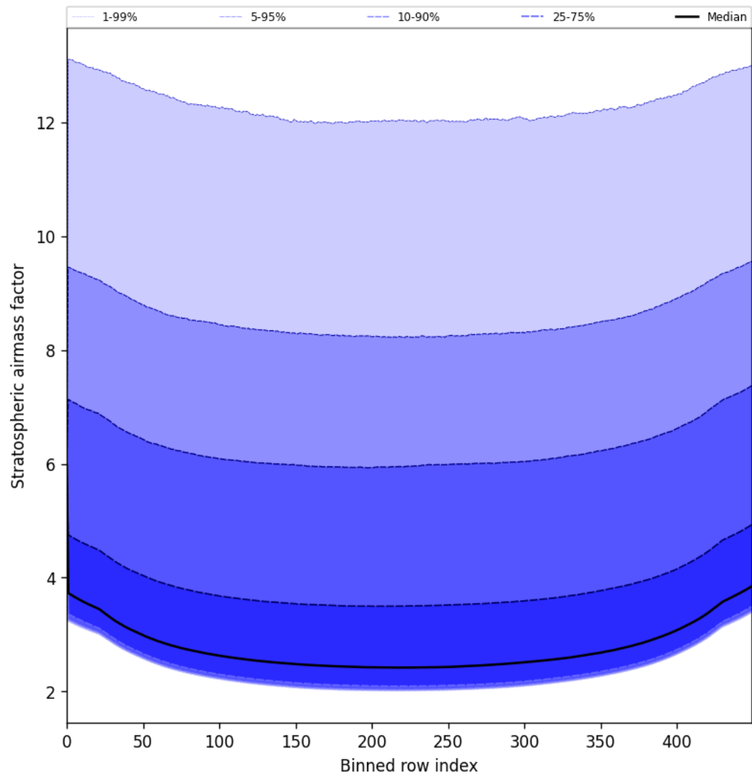
Figure 61: Along track statistics of “Stratospheric airmass factor” for 2025-05-24 to 2025-05-26
