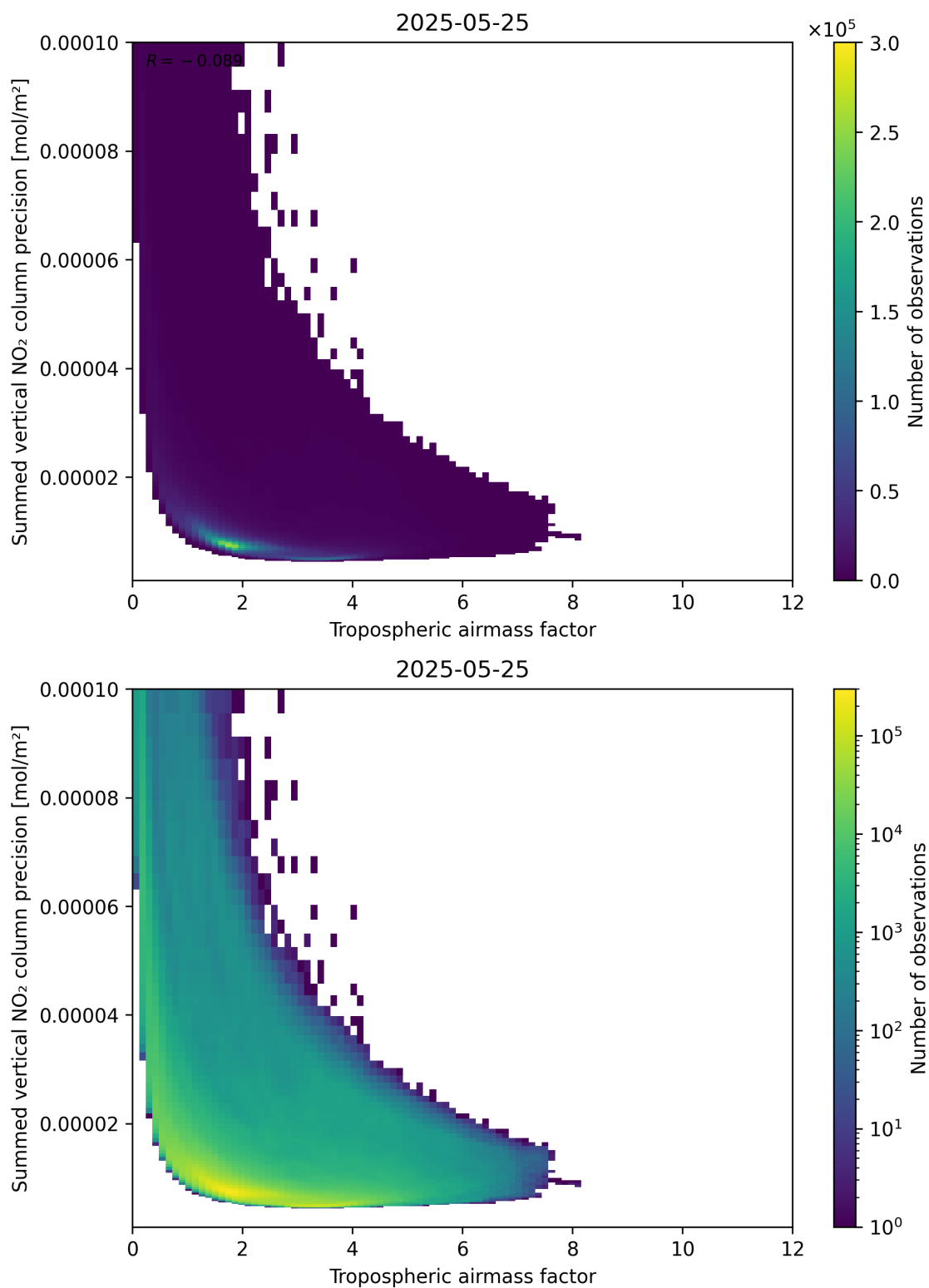
Figure 76: Scatter density plot of “Tropospheric air mass factor” against “Summed vertical NO 2 column precision” for 2025-05-24 to 2025-05-26.
