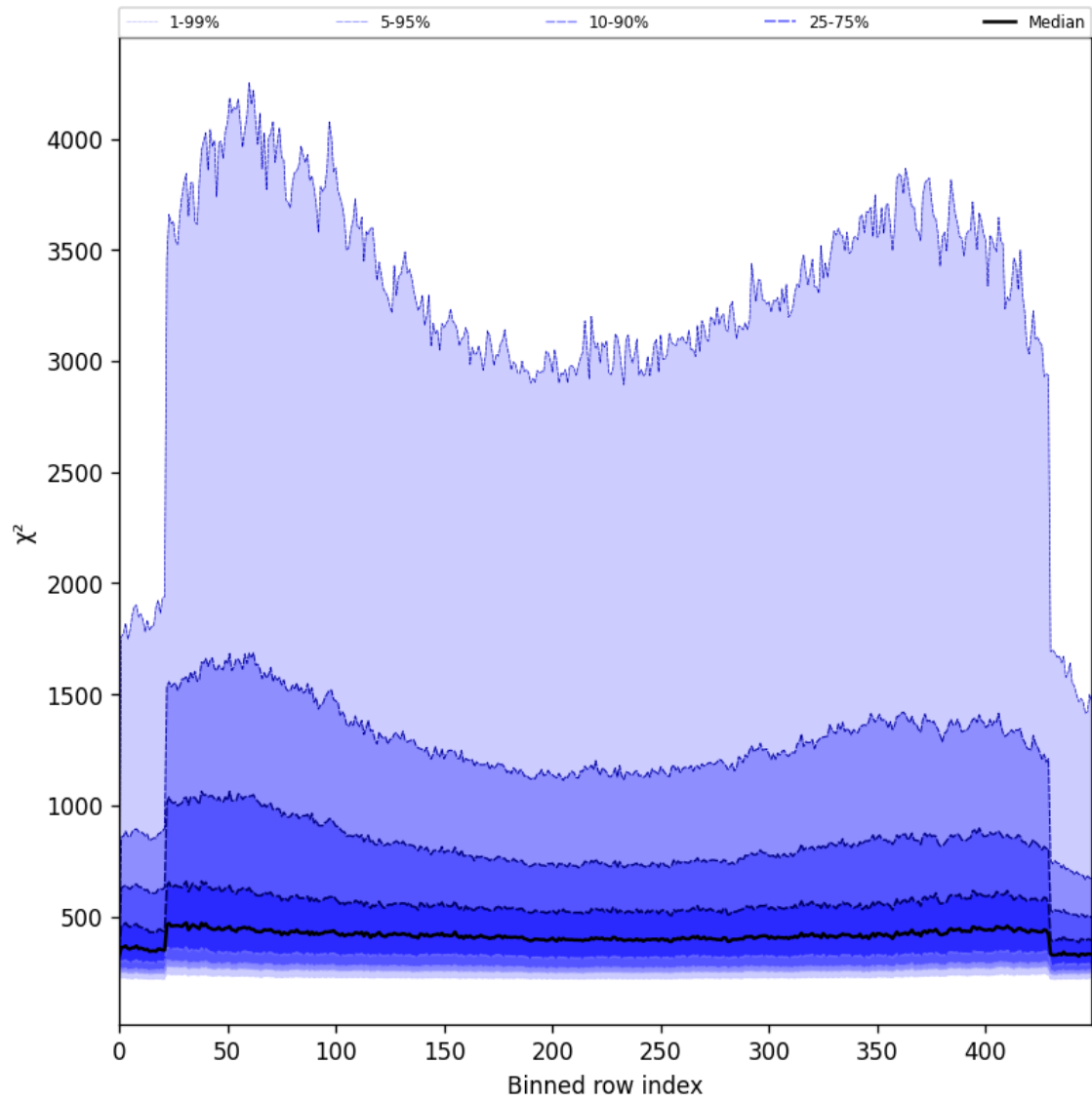
Figure 59: Along track statistics of “ \chi^2 ” for 2025-05-24 to 2025-05-26
