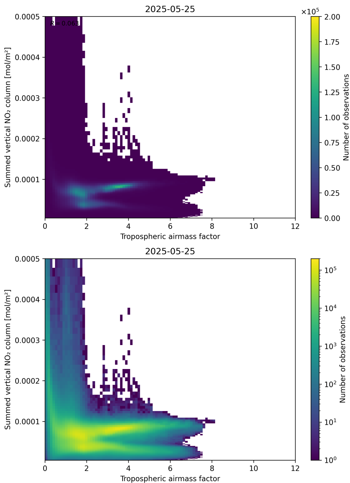
Figure 75: Scatter density plot of “Tropospheric airmass factor” against “Summed vertical NO 2 column” for 2025-05-24 to 2025-05-26.
