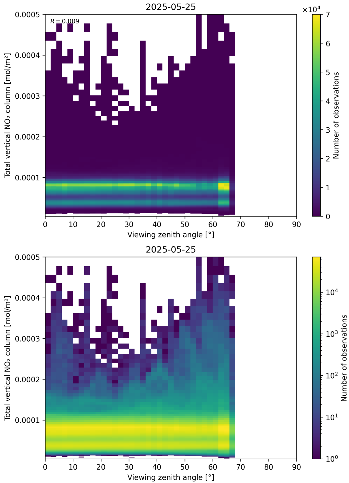
Figure 167: Scatter density plot of “Viewing zenith angle” against “Total vertical NO 2 column” for 2025-05-24 to 2025-05-26.
