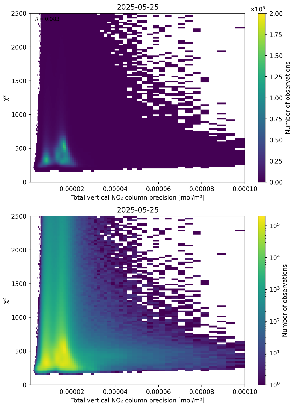
Figure 116: Scatter density plot of “Total vertical NO 2 column precision” against “ \chi^2 ” for 2025-05-24 to 2025-05-26.
