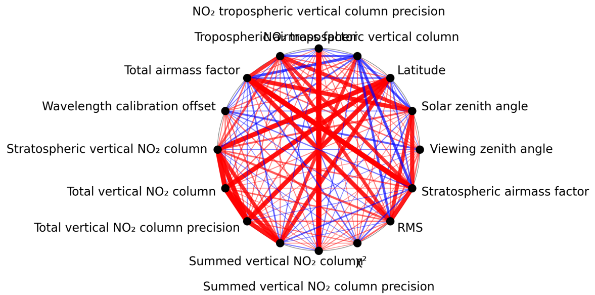
Figure 1: Map of correlation graph for 2025-05-24 to 2025-05-26.
