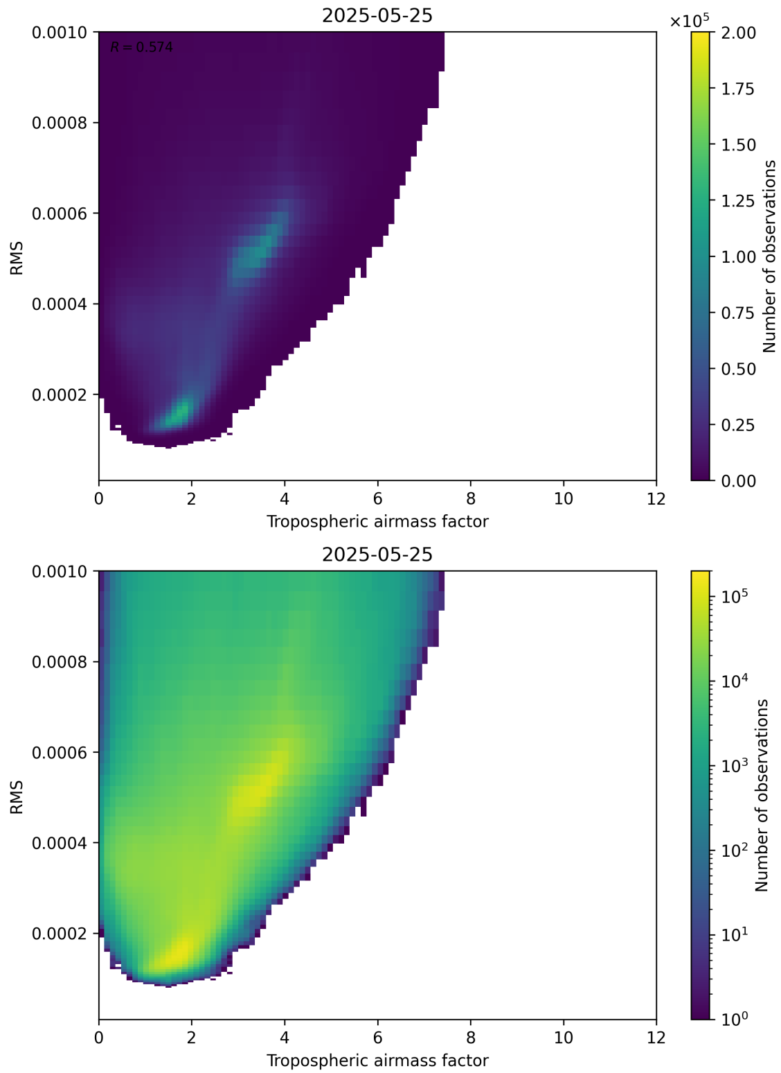
Figure 79: Scatter density plot of “Tropospheric airmass factor” against “RMS” for 2025-05-24 to 2025-05-26.
