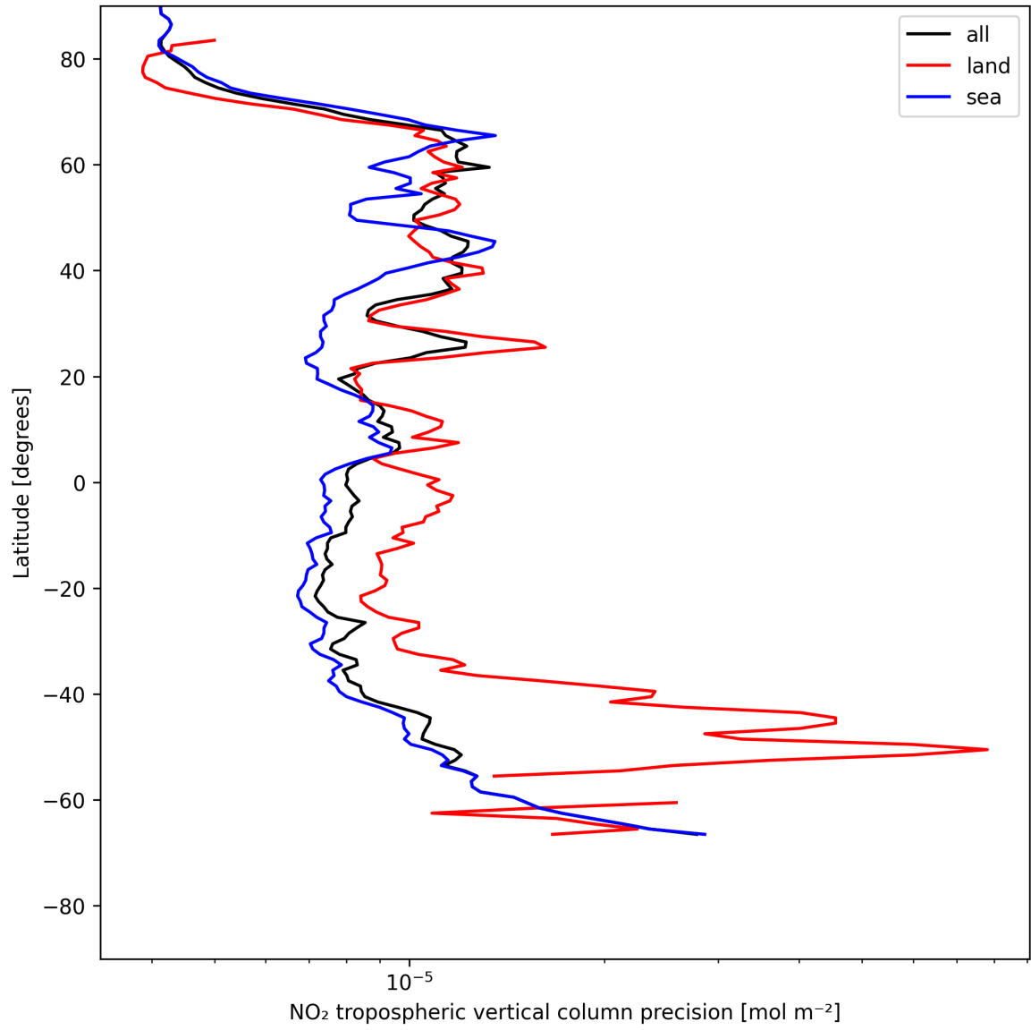
Figure 13: Zonal average of “NO 2 tropospheric vertical column precision” for 2025-05-24 to 2025-05-26.
