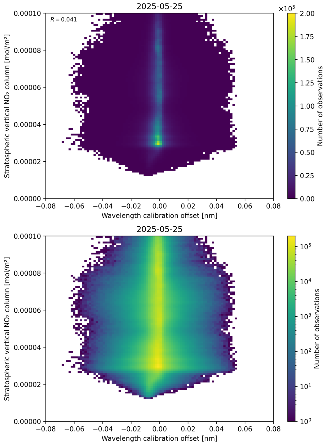
Figure 176: Scatter density plot of “Wavelength calibration offset” against “Stratospheric vertical NO 2 column” for 2025-05-24 to 2025-05-26.
