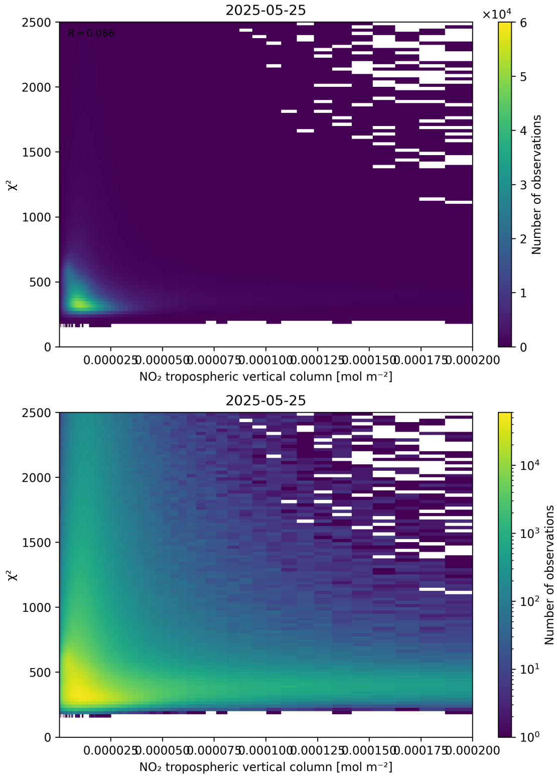
Figure 124: Scatter density plot of “NO 2 tropospheric vertical column” against “ \chi^2 ” for 2025-05-24 to 2025-05-26.
