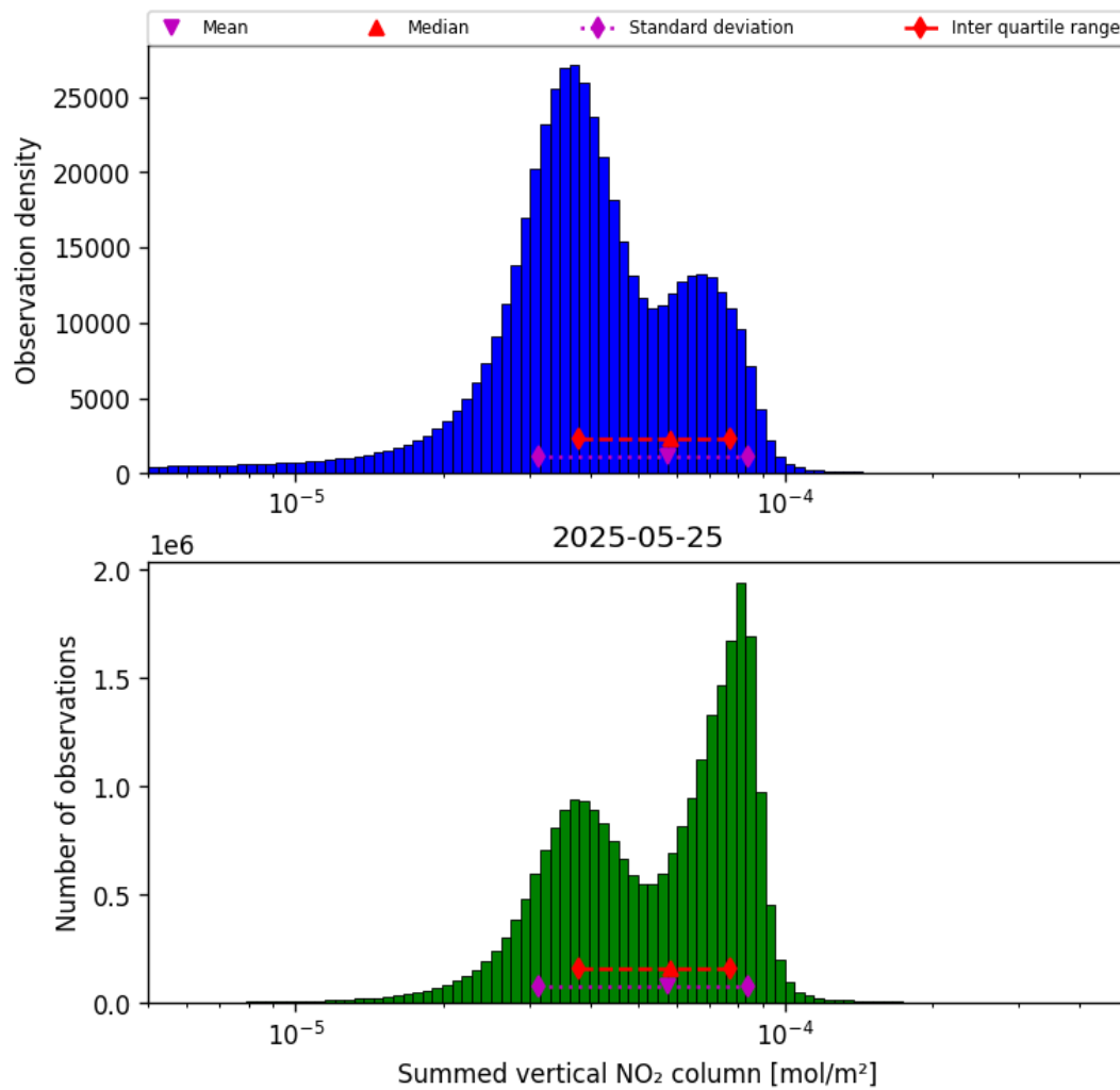
Figure 40: Histogram of “Summed vertical NO 2 column” for 2025-05-24 to 2025-05-26
