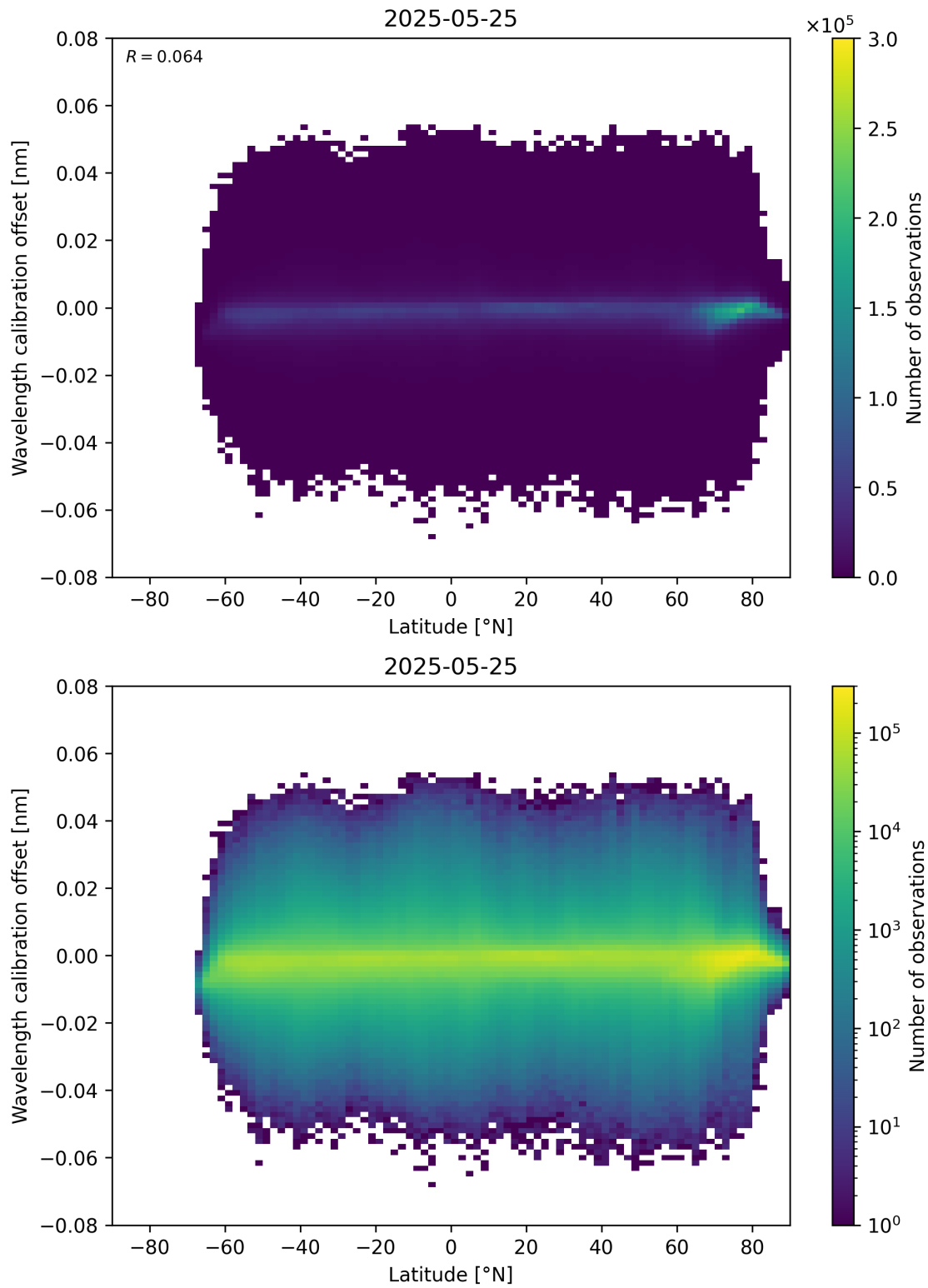
Figure 95: Scatter density plot of “Latitude” against “Wavelength calibration offset” for 2025-05-24 to 2025-05-26.
