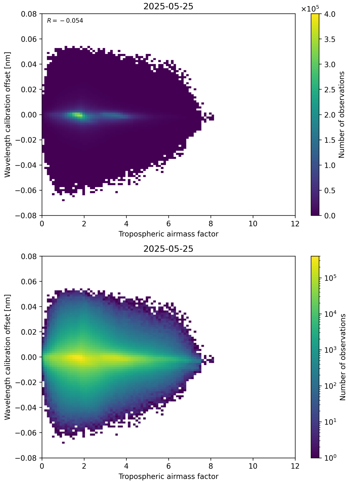
Figure 80: Scatter density plot of “Tropospheric airmass factor” against “Wavelength calibration offset” for 2025-05-24 to 2025-05-26.
