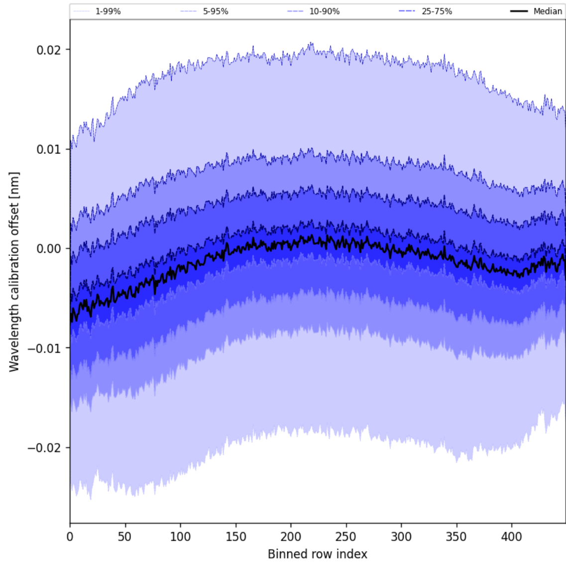
Figure 52: Along track statistics of “Wavelength calibration offset” for 2025-05-24 to 2025-05-26
