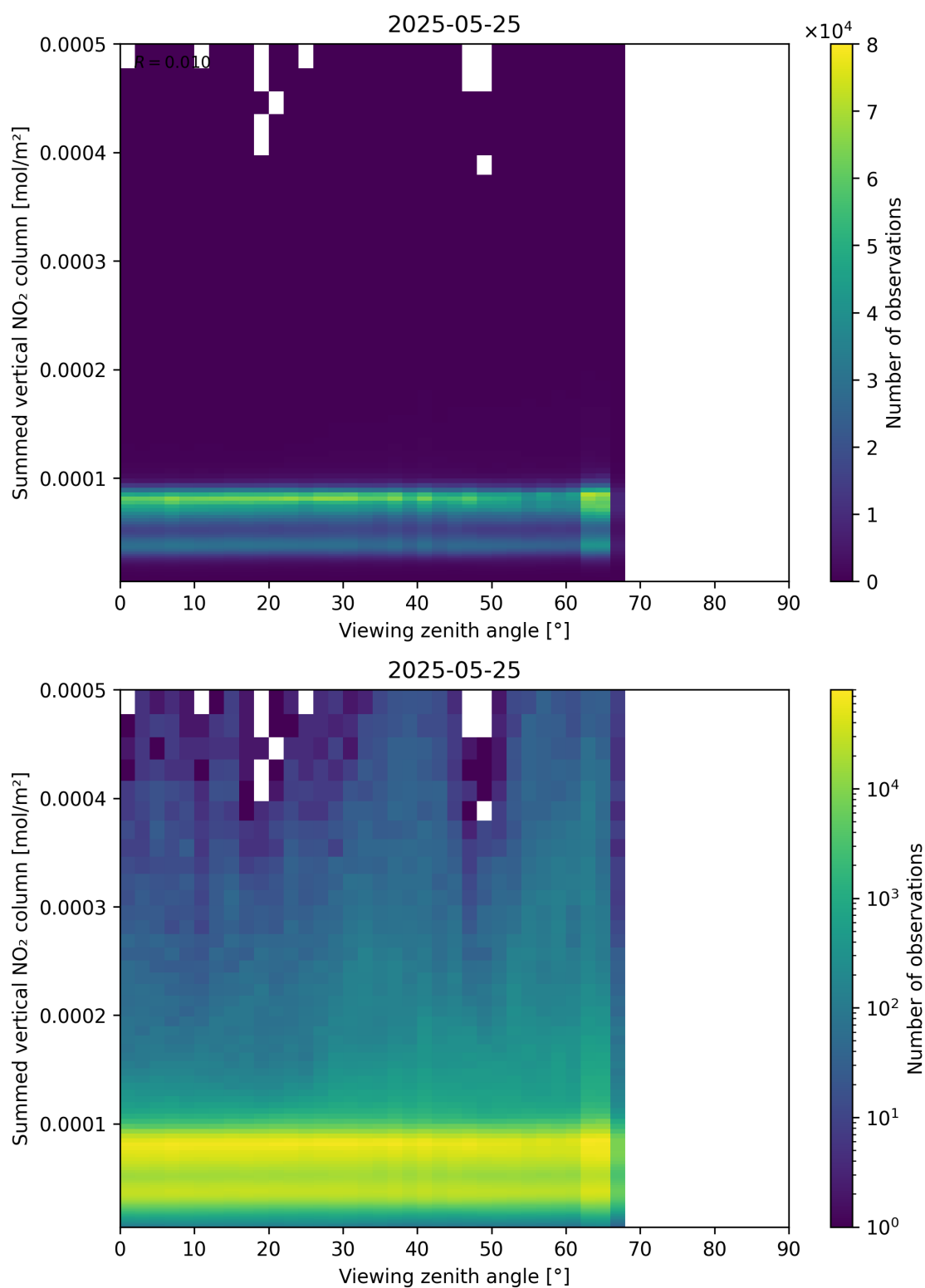
Figure 165: Scatter density plot of “Viewing zenith angle” against “Summed vertical NO 2 column” for 2025-05-24 to 2025-05-26.
