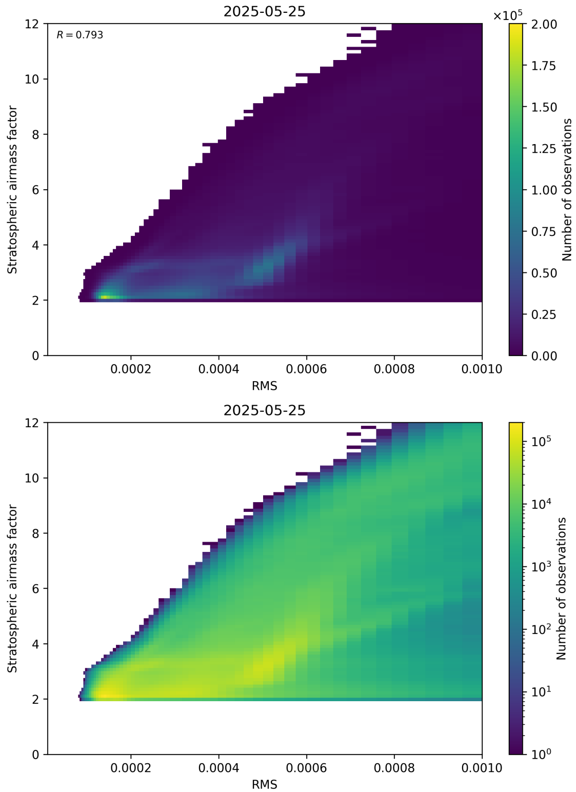
Figure 144: Scatter density plot of “RMS” against “Stratospheric airmass factor” for 2025-05-24 to 2025-05-26.
