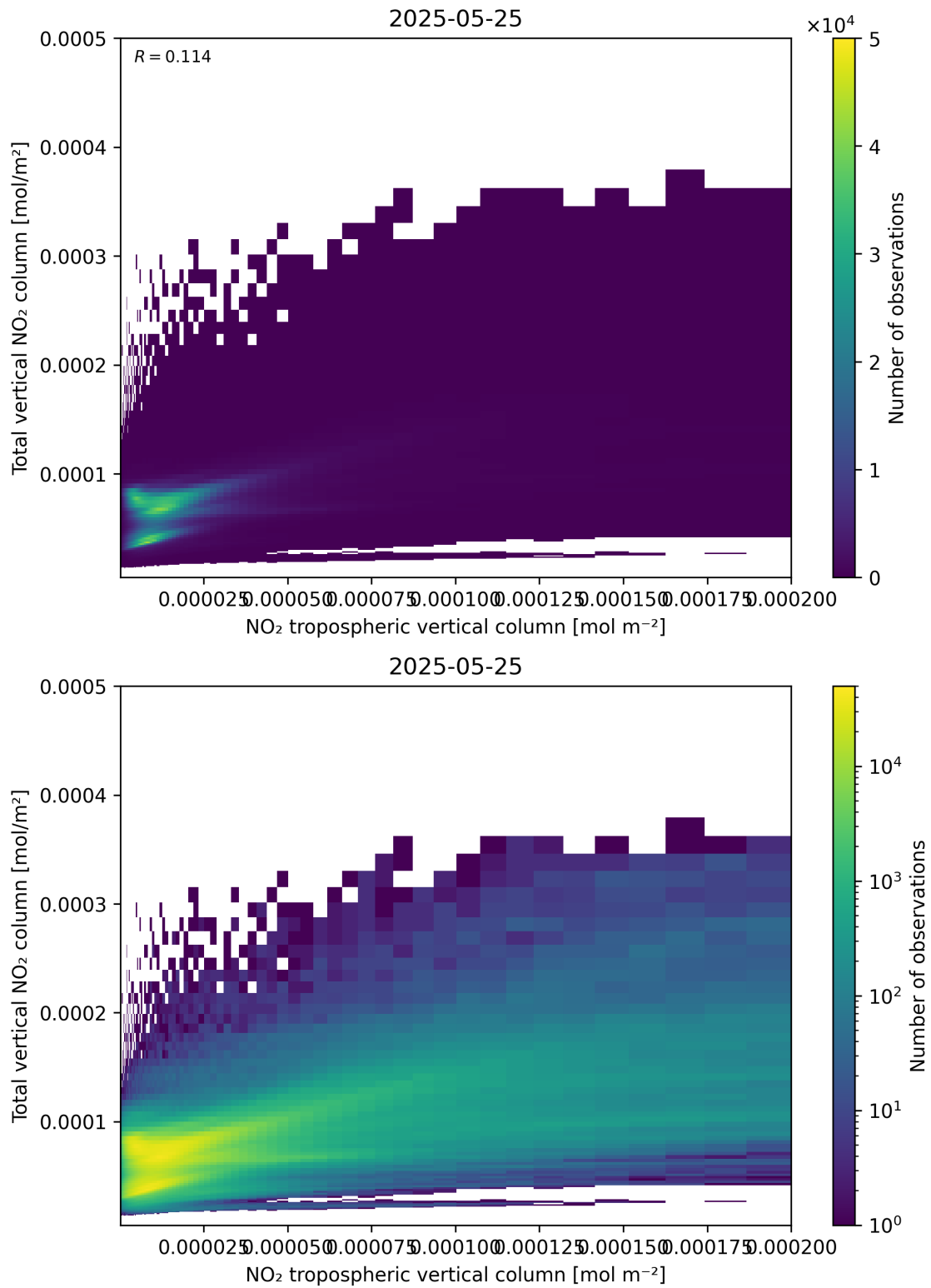
Figure 128: Scatter density plot of “NO 2 tropospheric vertical column” against “Total vertical NO 2 column” for 2025-05-24 to 2025-05-26.
