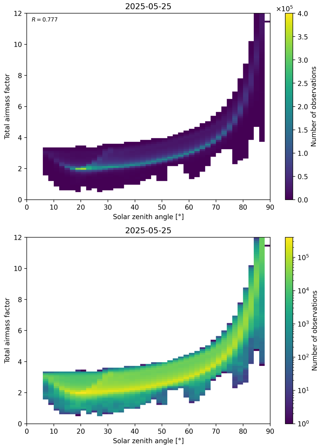
Figure 146: Scatter density plot of “Solar zenith angle” against “Total air mass factor” for 2025-05-24 to 2025-05-26.
