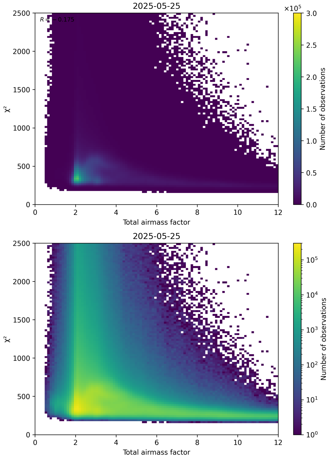
Figure 63: Scatter density plot of “Total airmass factor” against “ \chi^2 ” for 2025-05-24 to 2025-05-26.
