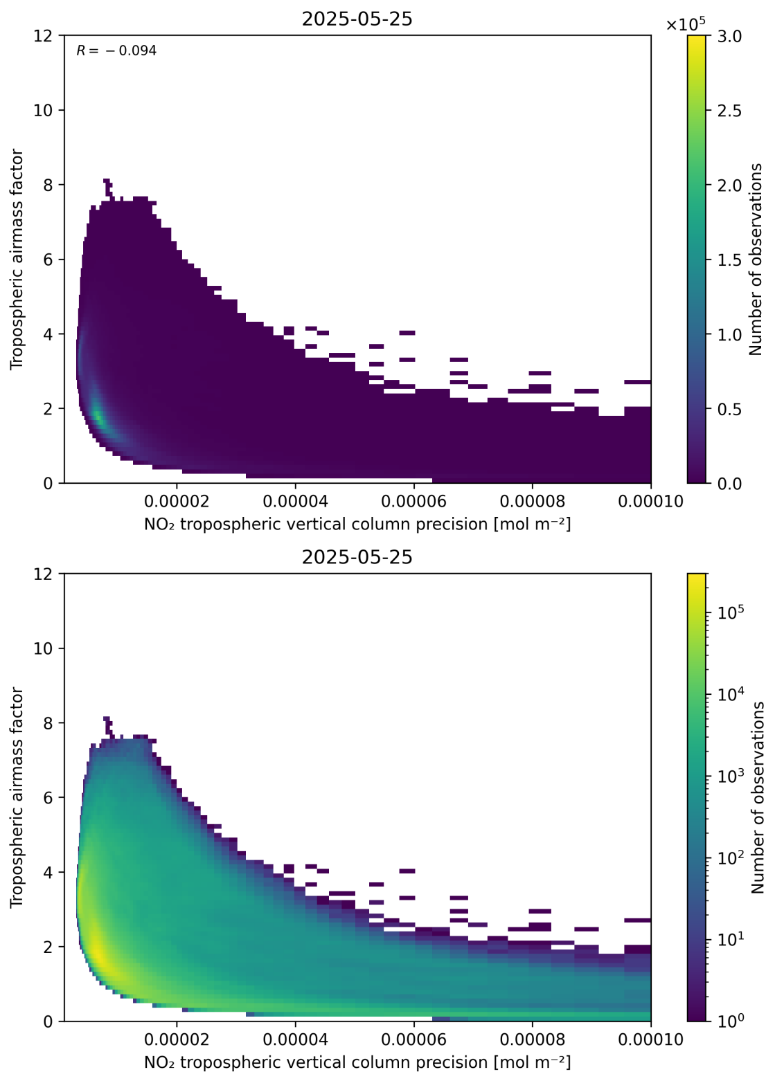
Figure 133: Scatter density plot of “NO 2 tropospheric vertical column precision” against “Tropospheric airmass factor” for 2025-05-24 to 2025-05-26.
