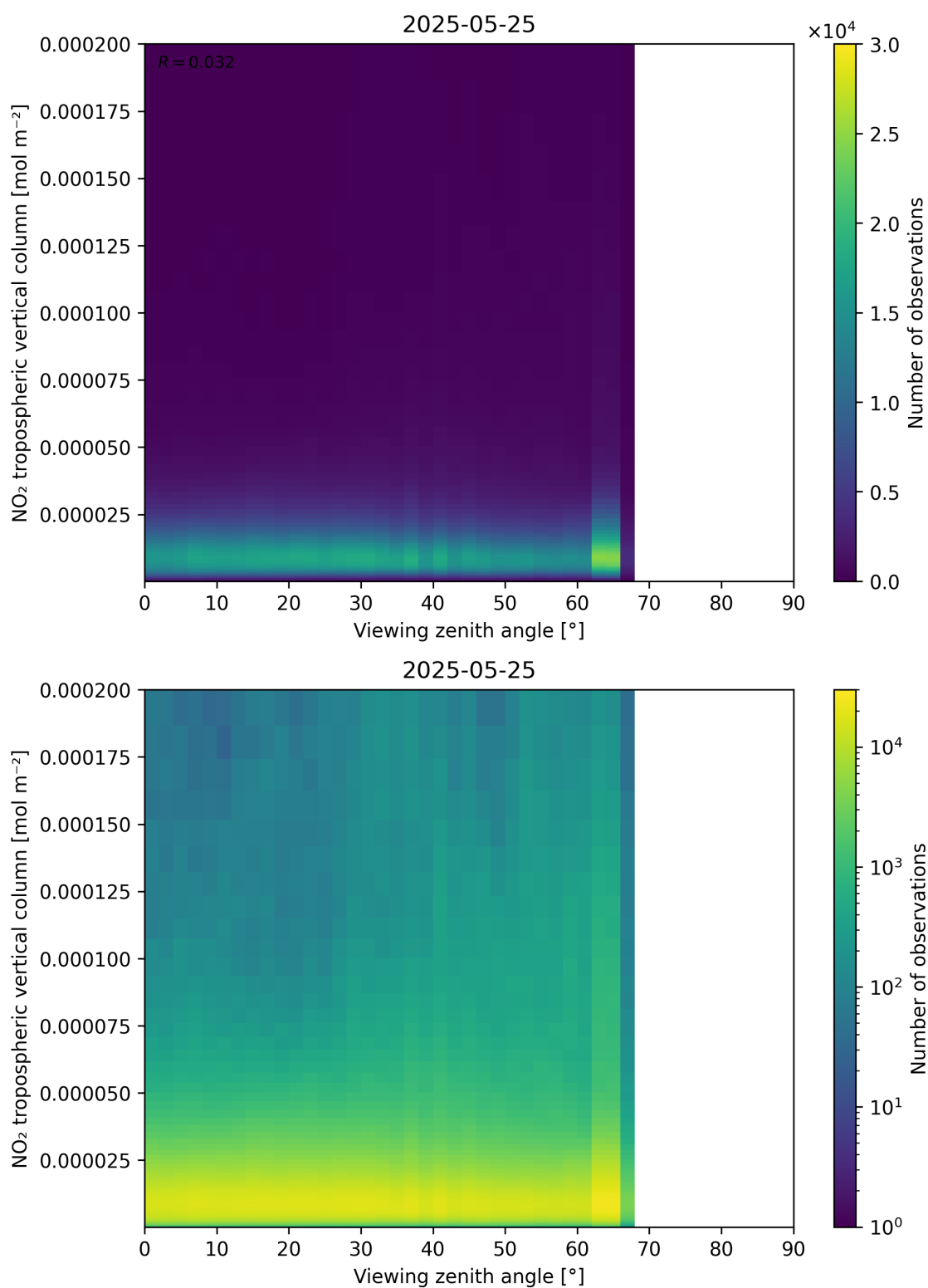
Figure 169: Scatter density plot of “Viewing zenith angle” against “NO 2 tropospheric vertical column” for 2025-05-24 to 2025-05-26.
