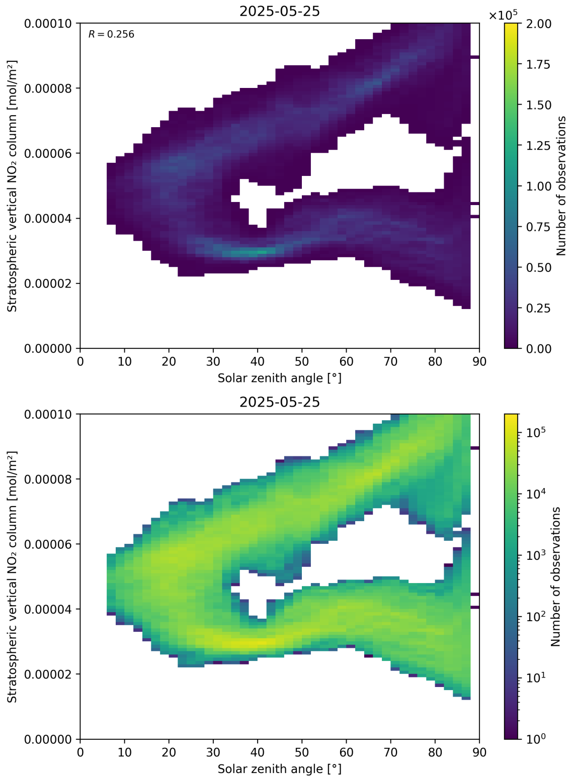
Figure 150: Scatter density plot of “Solar zenith angle” against “Stratospheric vertical NO 2 column” for 2025-05-24 to 2025-05-26.
