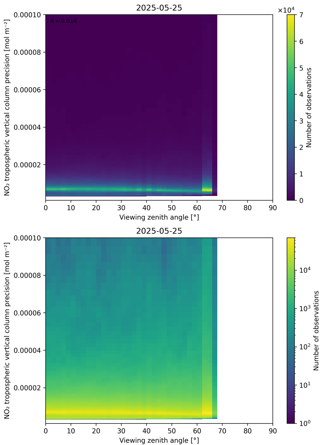
Figure 170: Scatter density plot of “Viewing zenith angle” against “NO 2 tropospheric vertical column precision” for 2025-05-24 to 2025-05-26.
