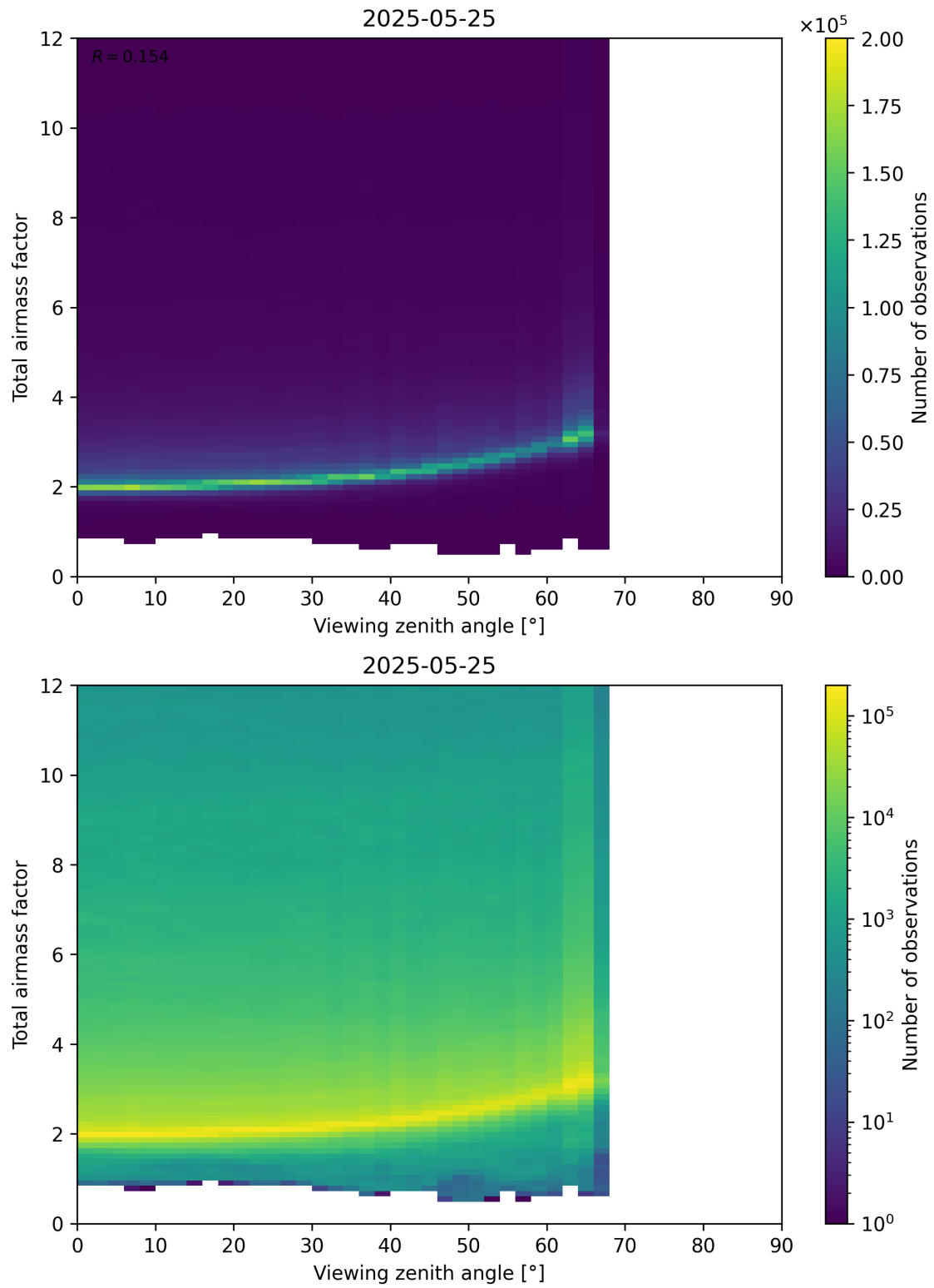
Figure 160: Scatter density plot of “Viewing zenith angle” against “Total airmass factor” for 2025-05-24 to 2025-05-26.
