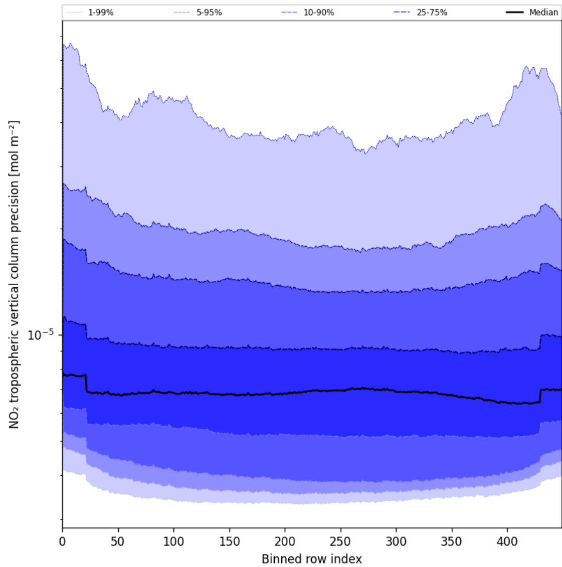
Figure 47: Along track statistics of “NO 2 tropospheric vertical column precision” for 2025-05-24 to 2025-05-26
