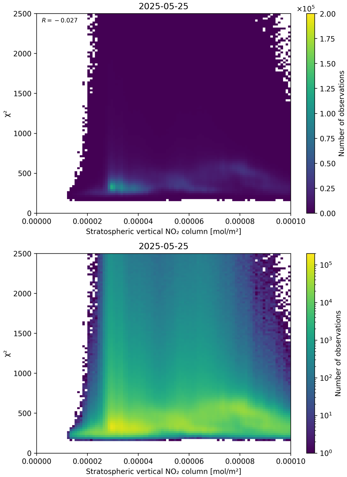
Figure 97: Scatter density plot of “Stratospheric vertical NO 2 column” against “ \chi^2 ” for 2025-05-24 to 2025-05-26.
