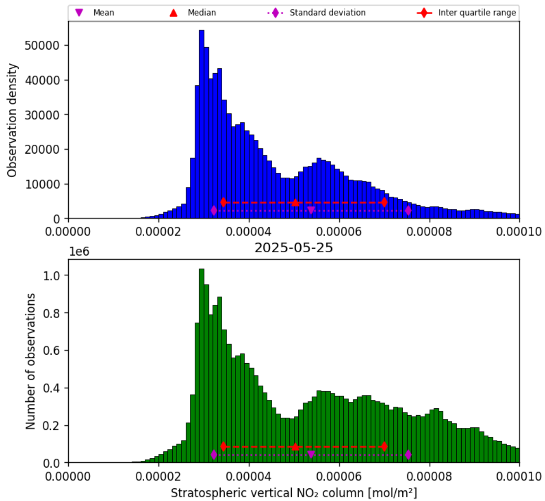
Figure 36: Histogram of “Stratospheric vertical NO 2 column” for 2025-05-24 to 2025-05-26
