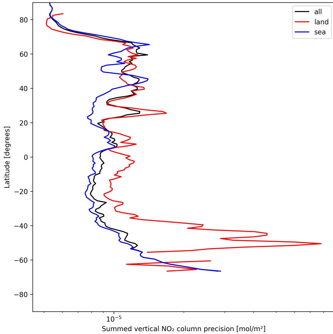
Figure 24: Zonal average of “Summed vertical NO 2 column precision” for 2025-05-24 to 2025-05-26.
