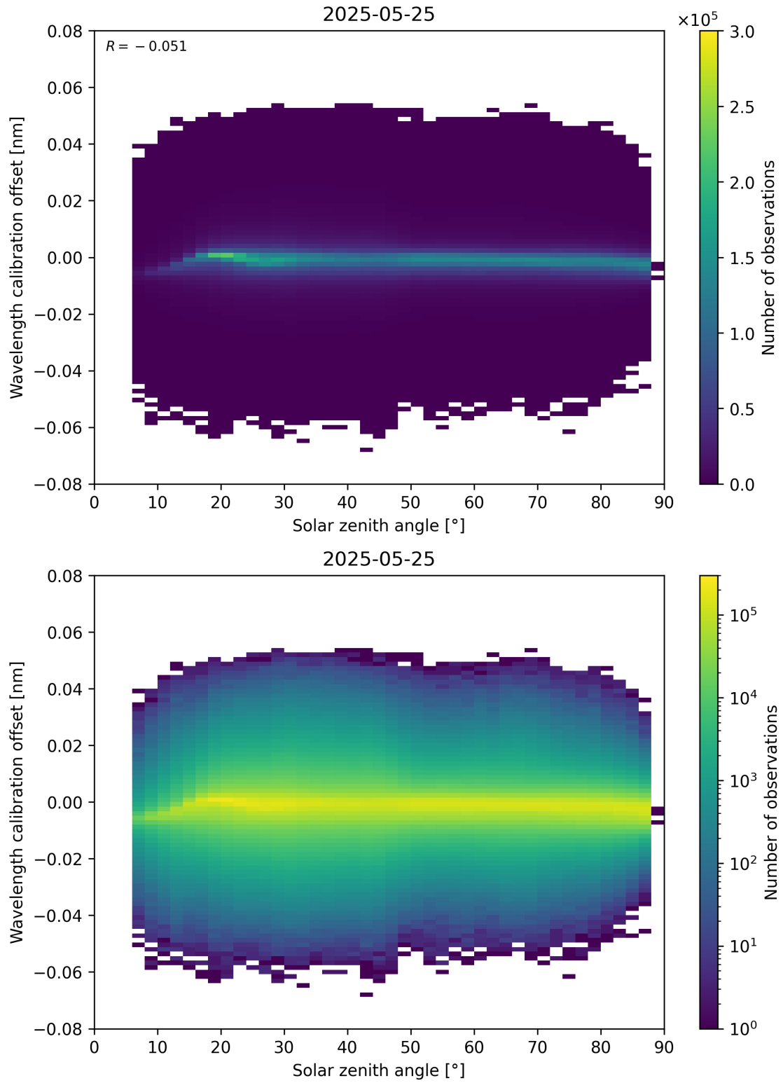
Figure 158: Scatter density plot of “Solar zenith angle” against “Wavelength calibration offset” for 2025-05-24 to 2025-05-26.
