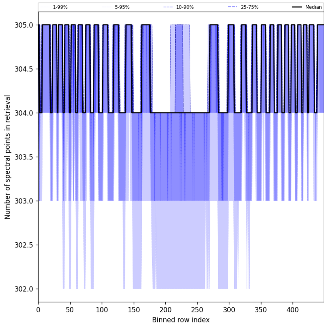
Figure 50: Along track statistics of “Number of spectral points in retrieval” for 2025-05-24 to 2025-05-26
