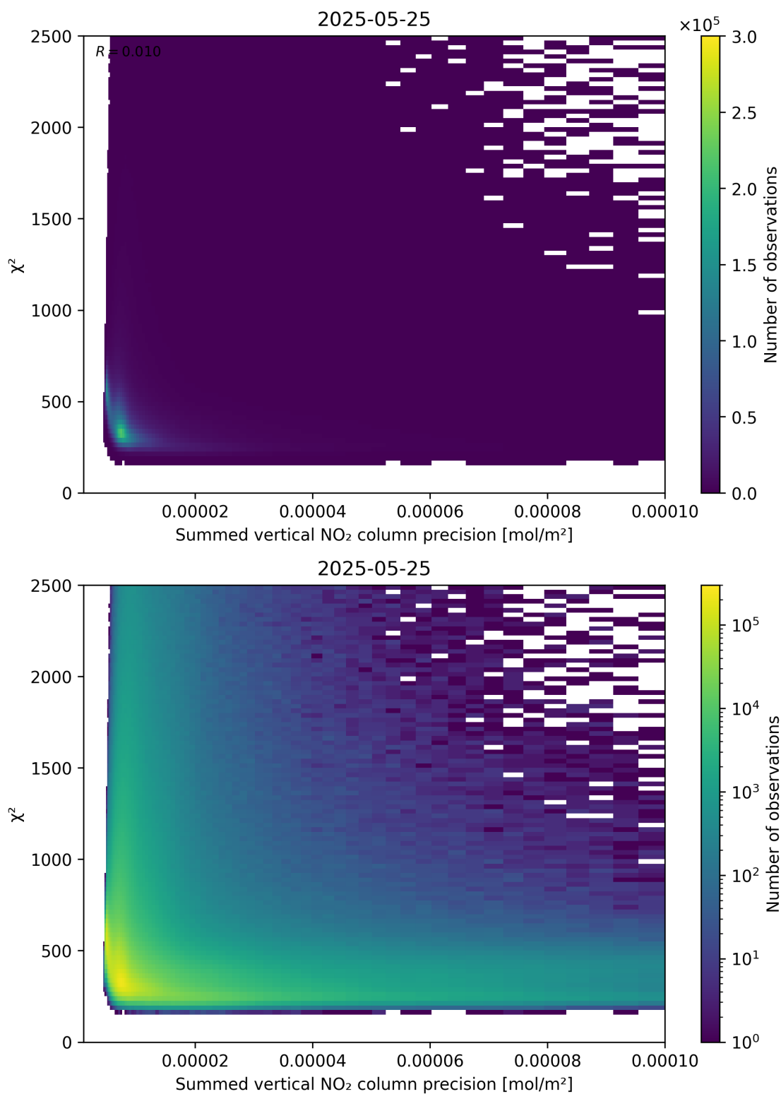
Figure 107: Scatter density plot of “Summed vertical NO 2 column precision” against “ \chi^2 ” for 2025-05-24 to 2025-05-26.
