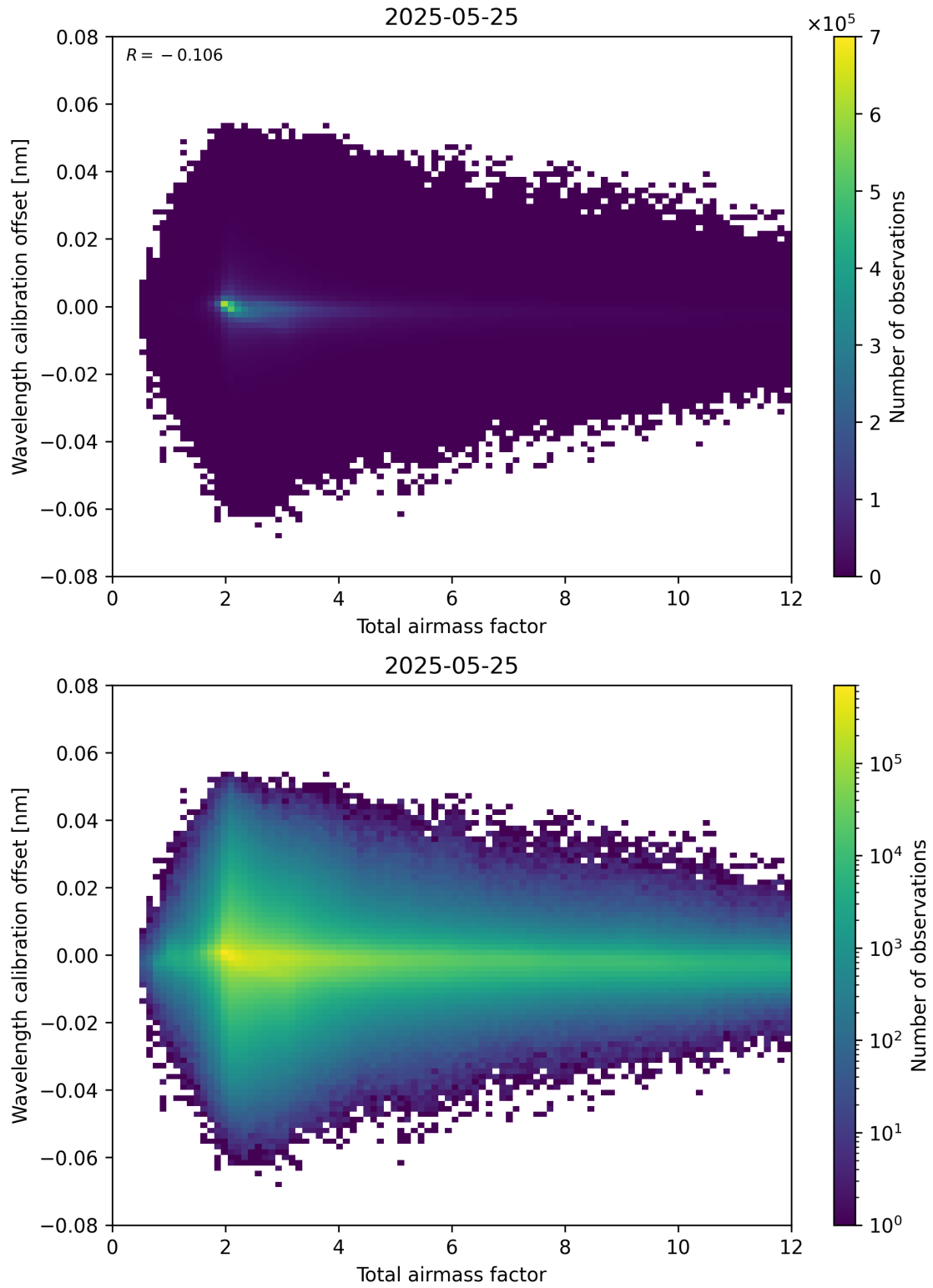
Figure 70: Scatter density plot of “Total airmass factor” against “Wavelength calibration offset” for 2025-05-24 to 2025-05-26.
