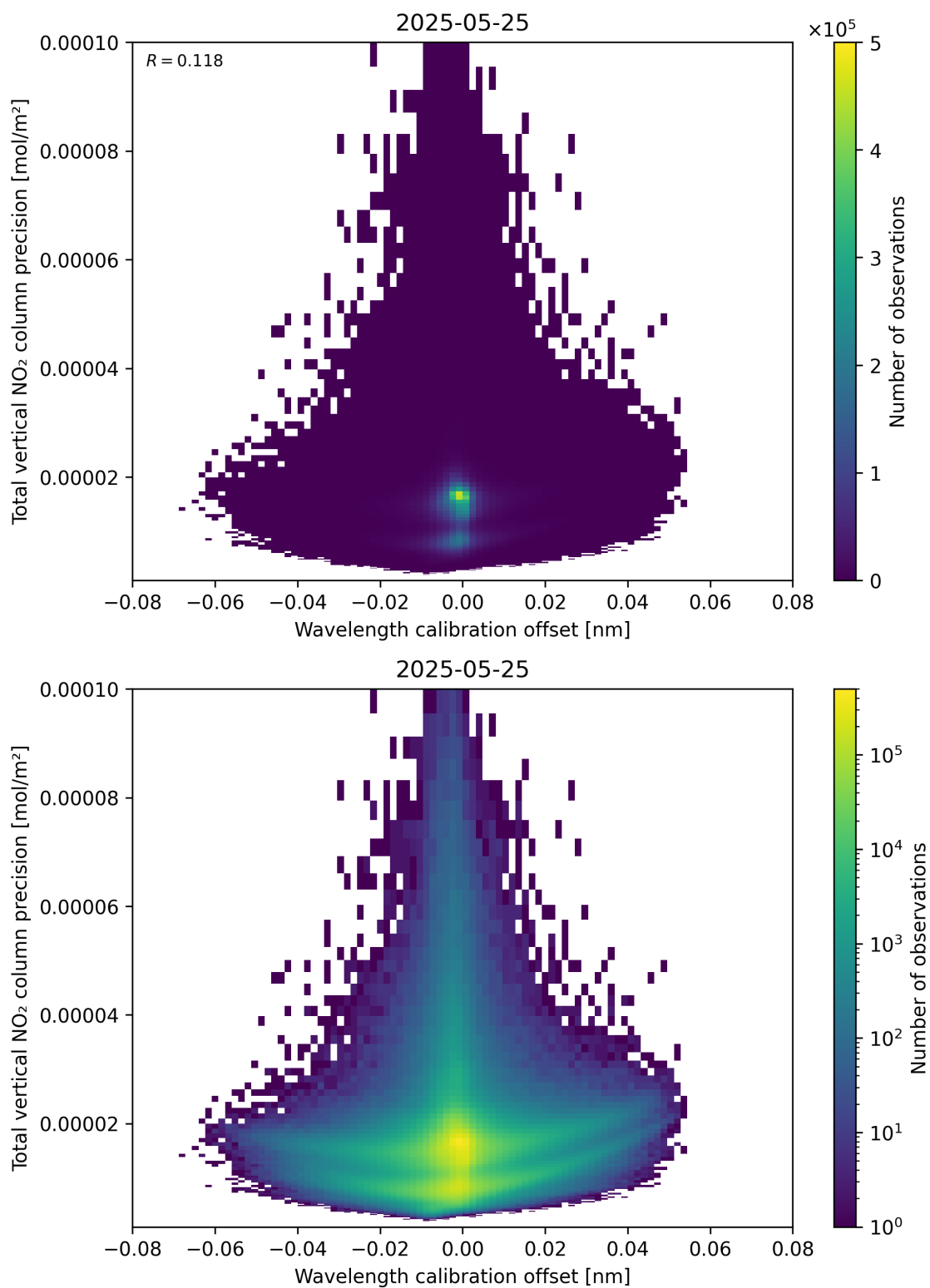
Figure 180: Scatter density plot of “Wavelength calibration offset” against “Total vertical NO 2 column precision” for 2025-05-24 to 2025-05-26.
