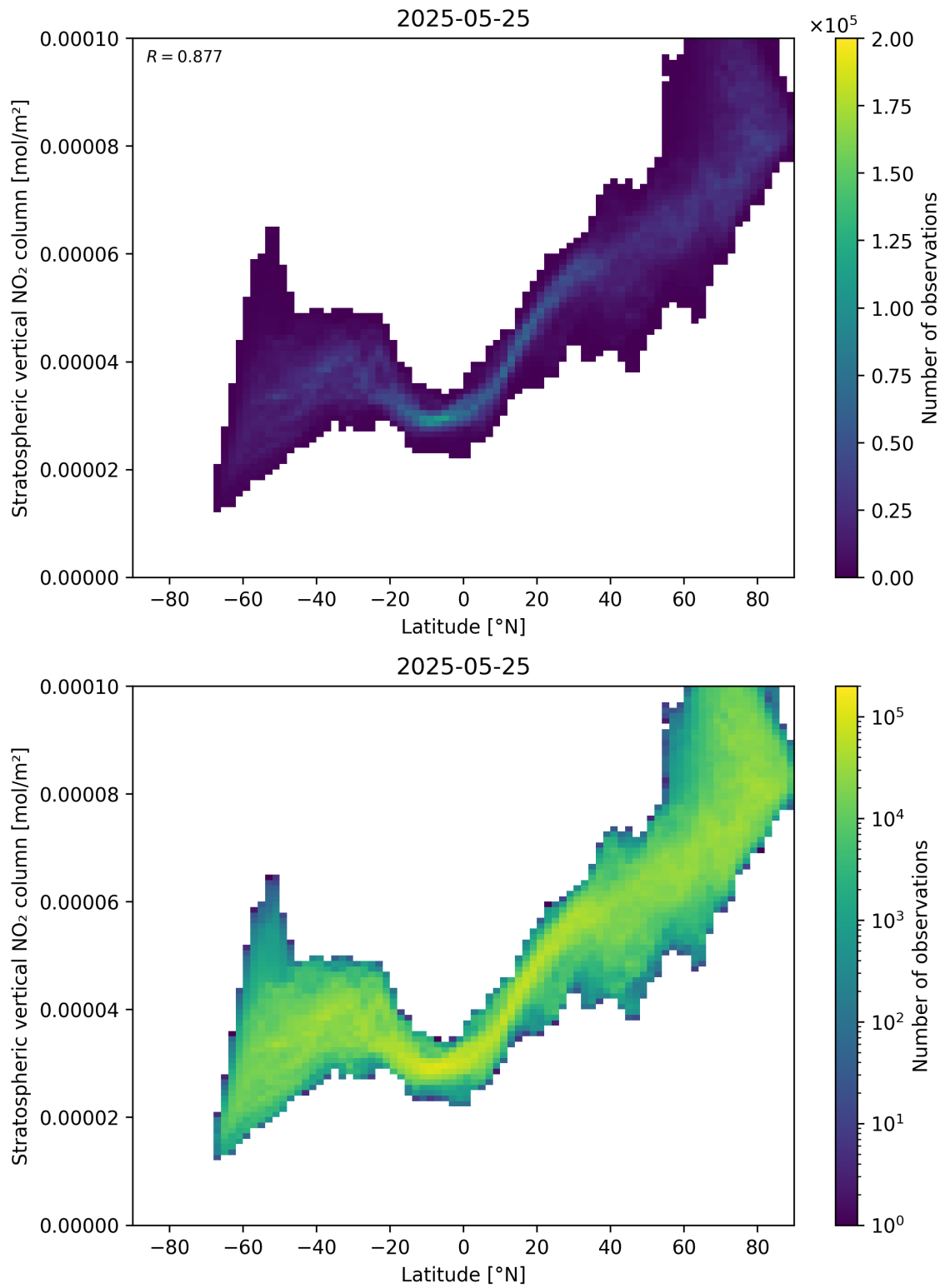
Figure 87: Scatter density plot of “Latitude” against “Stratospheric vertical NO 2 column” for 2025-05-24 to 2025-05-26.
