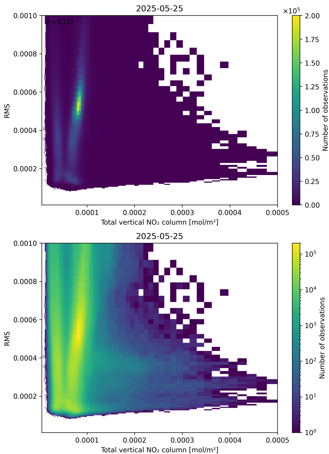
Figure 120: Scatter density plot of “Total vertical NO 2 column” against “RMS” for 2025-05-24 to 2025-05-26.
