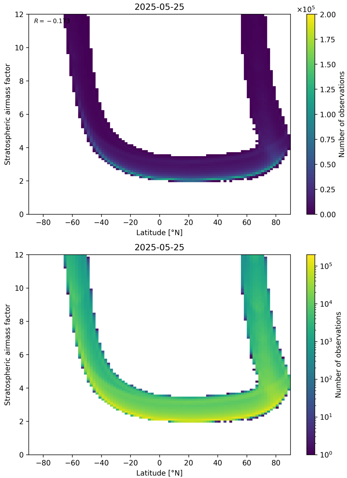
Figure 83: Scatter density plot of “Latitude” against “Stratospheric air mass factor” for 2025-05-24 to 2025-05-26.
