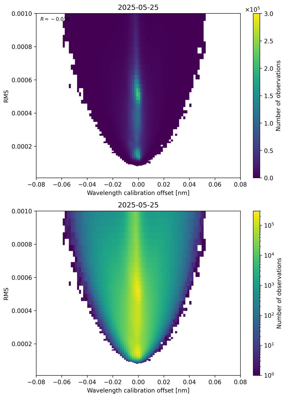
Figure 181: Scatter density plot of “Wavelength calibration offset” against “RMS” for 2025-05-24 to 2025-05-26.
