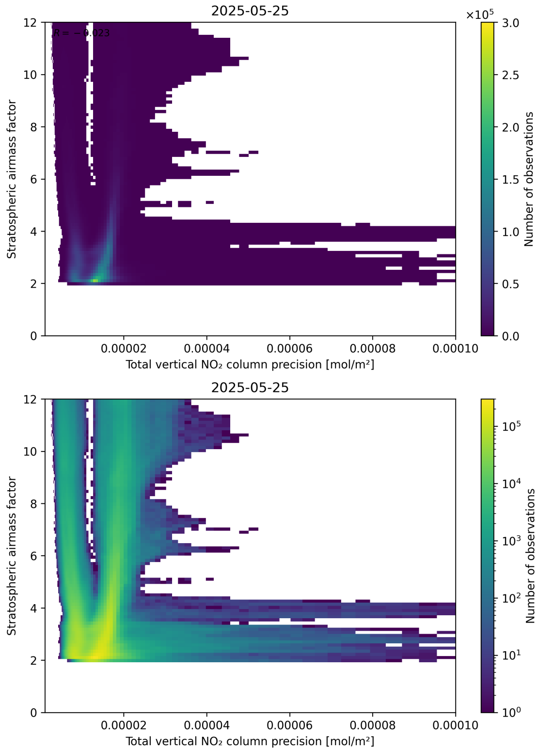
Figure 115: Scatter density plot of “Total vertical NO 2 column precision” against “Stratospheric air mass factor” for 2025-05-24 to 2025-05-26.
