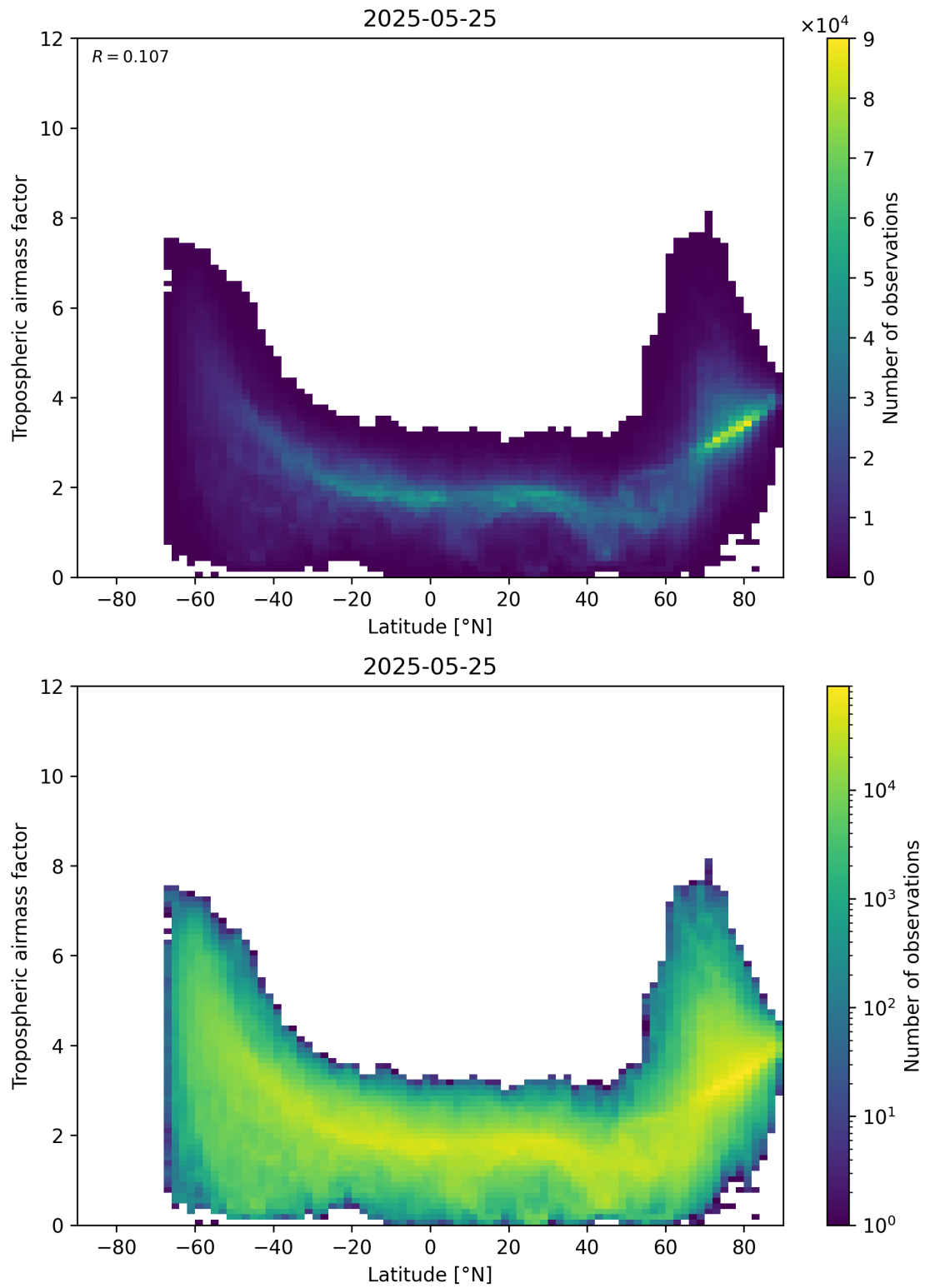
Figure 85: Scatter density plot of “Latitude” against “Tropospheric air mass factor” for 2025-05-24 to 2025-05-26.
