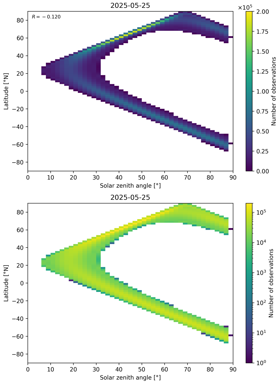
Figure 149: Scatter density plot of “Solar zenith angle” against “Latitude” for 2025-05-24 to 2025-05-26.
