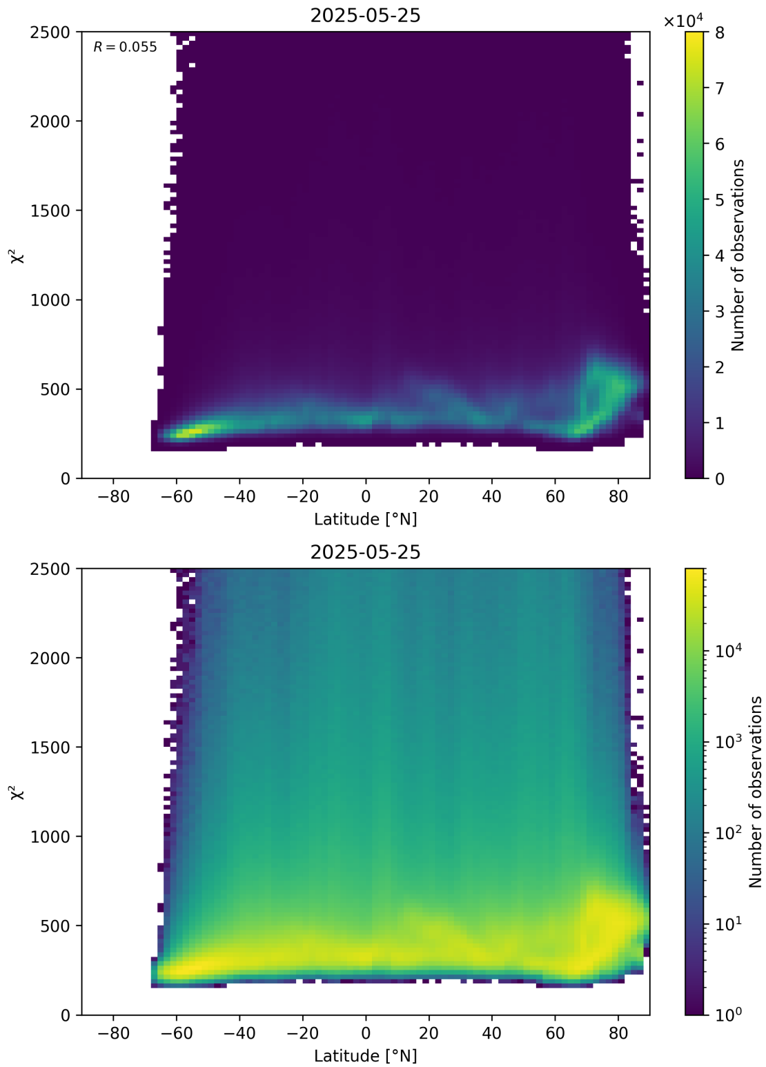
Figure 86: Scatter density plot of “Latitude” against “ \chi^2 ” for 2025-05-24 to 2025-05-26.
