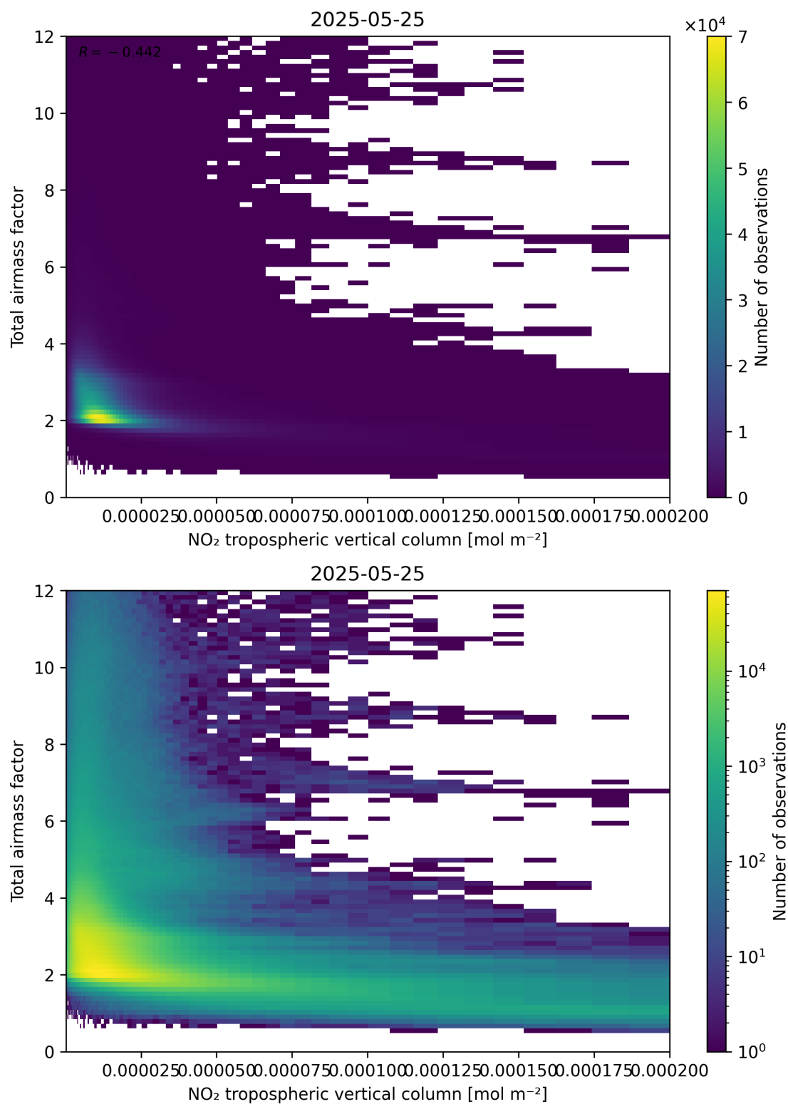
Figure 122: Scatter density plot of “NO 2 tropospheric vertical column” against “Total air mass factor” for 2025-05-24 to 2025-05-26.
