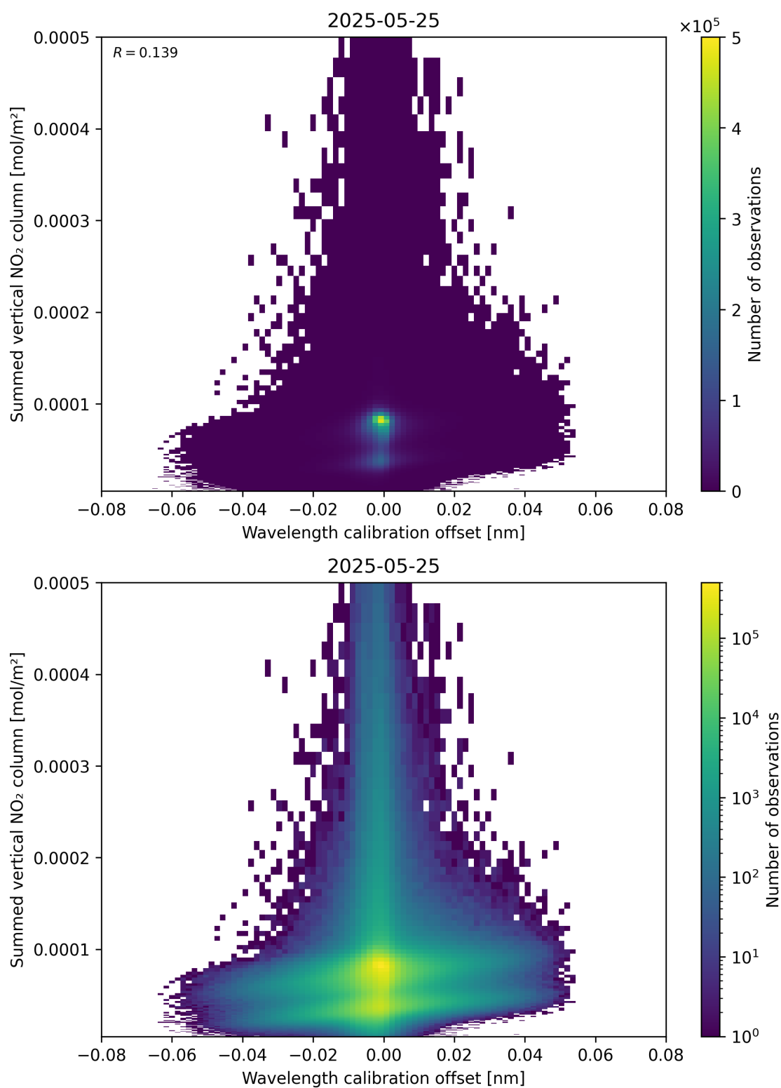
Figure 177: Scatter density plot of “Wavelength calibration offset” against “Summed vertical NO 2 column” for 2025-05-24 to 2025-05-26.
