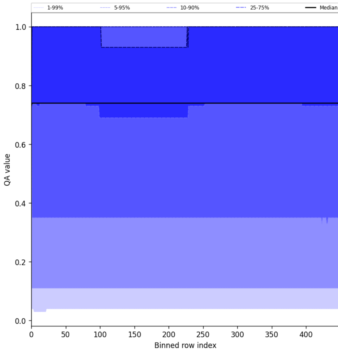
Figure 45: Along track statistics of “QA value” for 2025-05-24 to 2025-05-26
