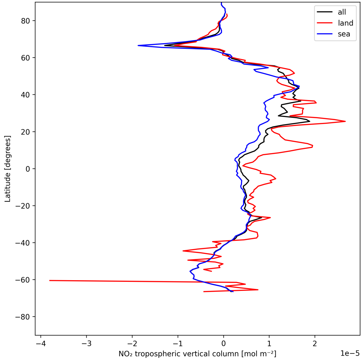
Figure 12: Zonal average of “NO 2 tropospheric vertical column” for 2025-05-24 to 2025-05-26.
