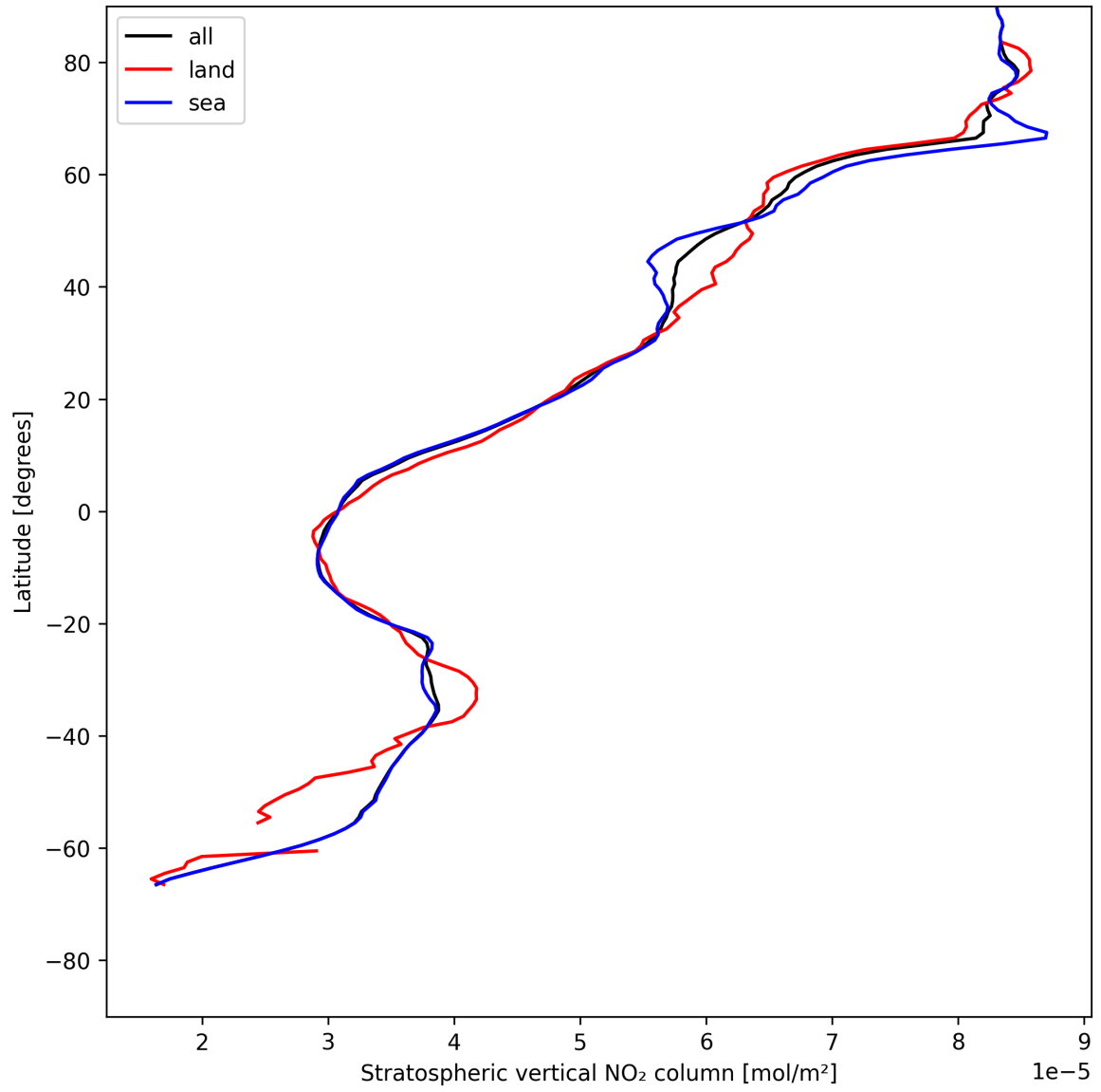
Figure 19: Zonal average of “Stratospheric vertical NO 2 column” for 2025-05-24 to 2025-05-26.
