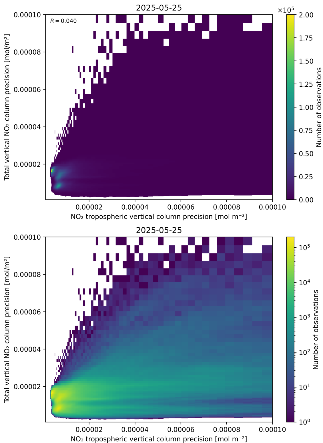
Figure 139: Scatter density plot of “NO 2 tropospheric vertical column precision” against “Total vertical NO 2 column precision” for 2025-05-24 to 2025-05-26.
