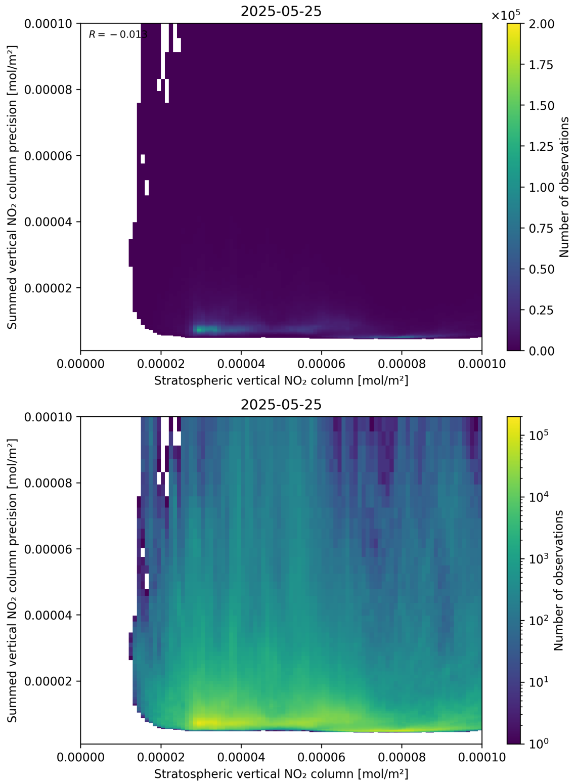
Figure 99: Scatter density plot of “Stratospheric vertical NO 2 column” against “Summed vertical NO 2 column precision” for 2025-05-24 to 2025-05-26.
