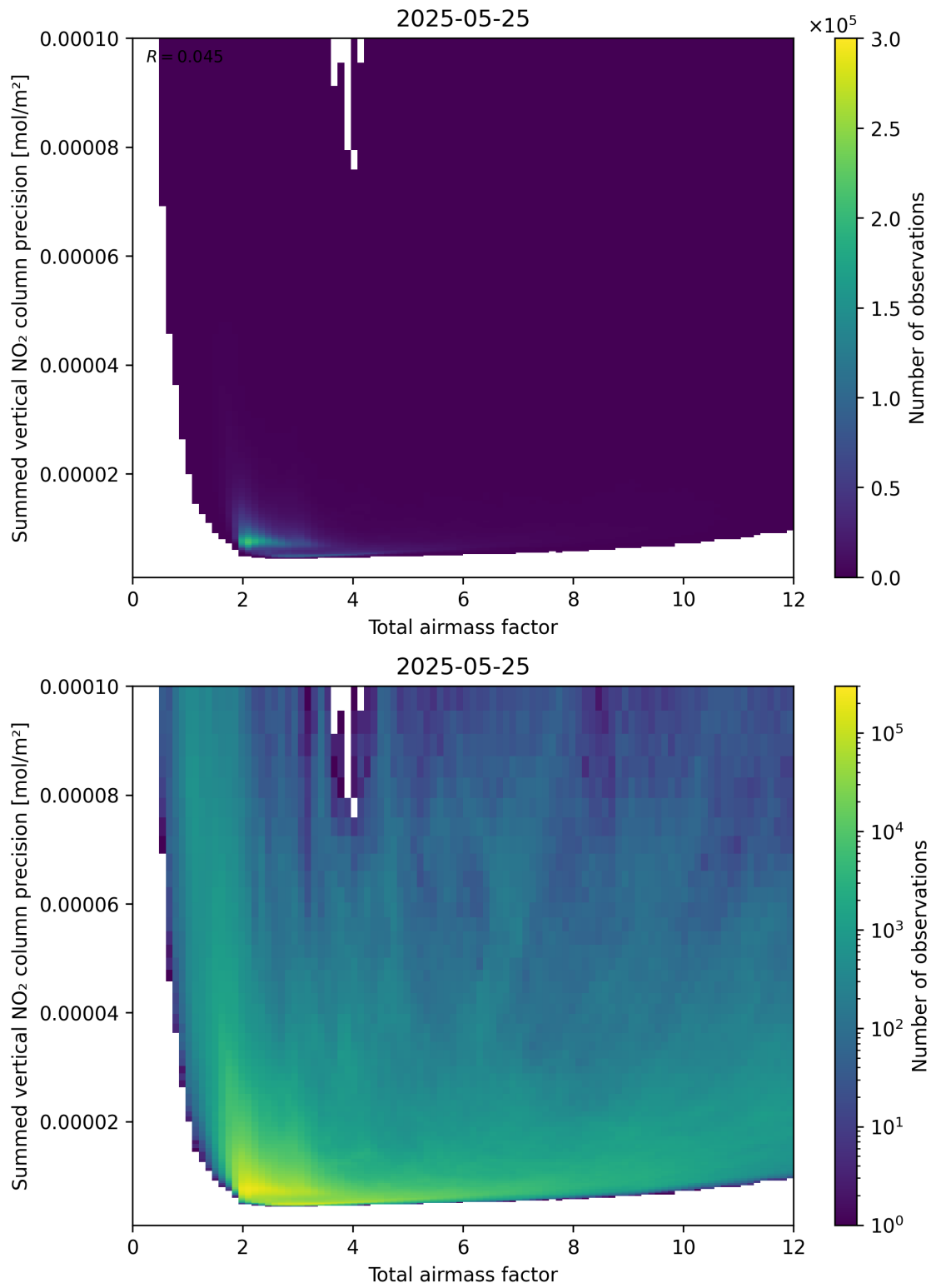
Figure 66: Scatter density plot of “Total airmass factor” against “Summed vertical NO 2 column precision” for 2025-05-24 to 2025-05-26.
