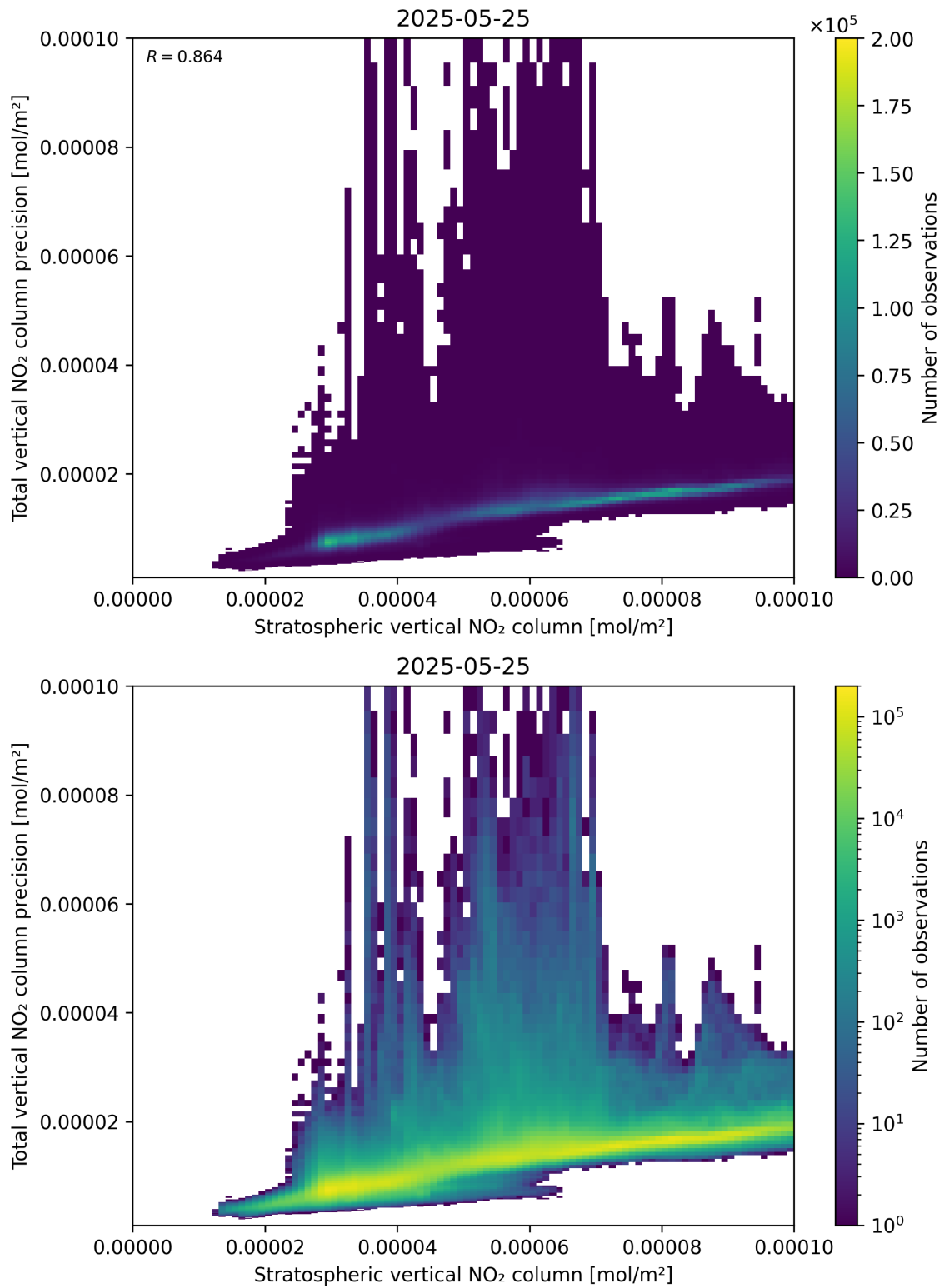
Figure 101: Scatter density plot of “Stratospheric vertical NO 2 column” against “Total vertical NO 2 column precision” for 2025-05-24 to 2025-05-26.
