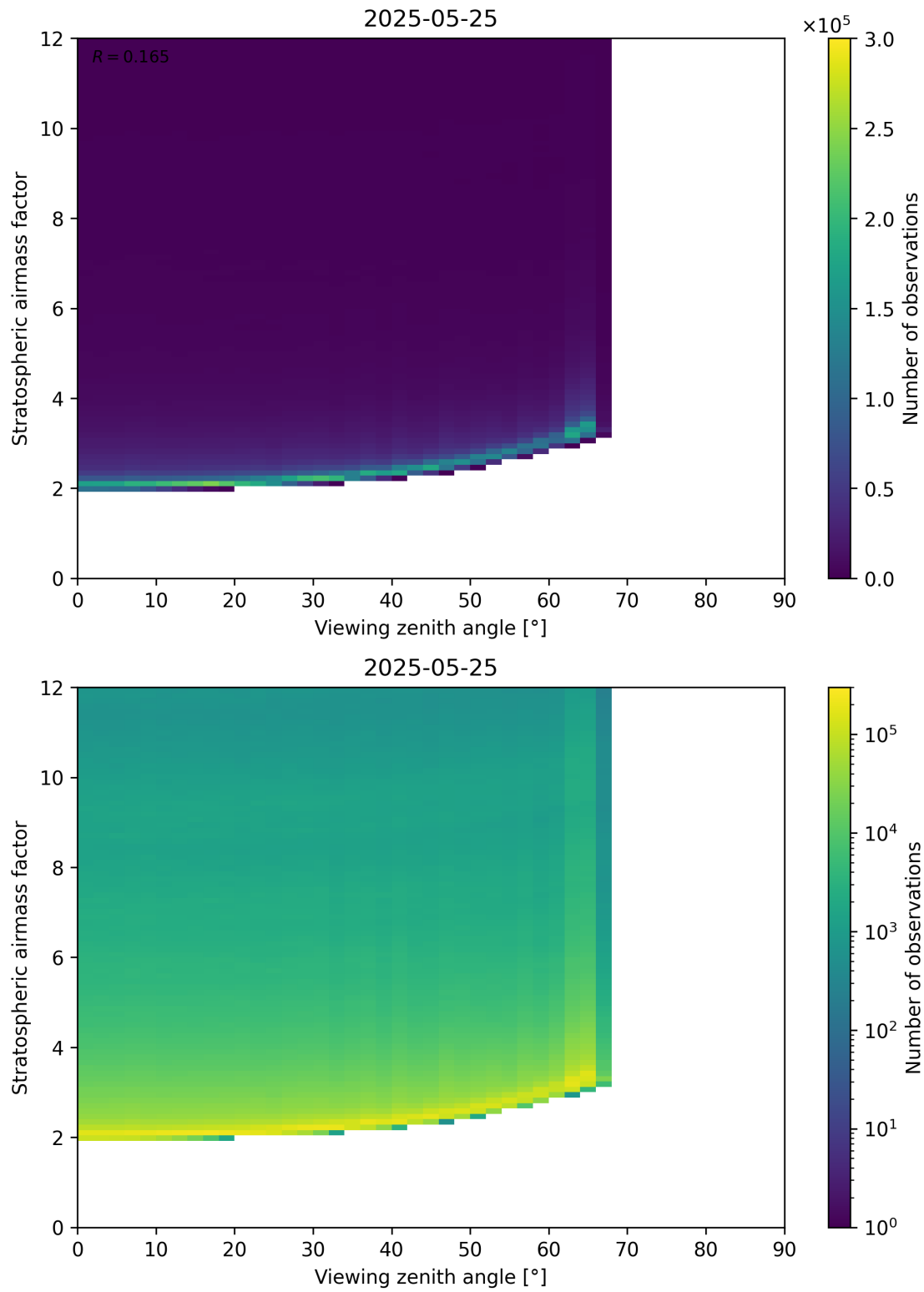
Figure 159: Scatter density plot of “Viewing zenith angle” against “Stratospheric airmass factor” for 2025-05-24 to 2025-05-26.
