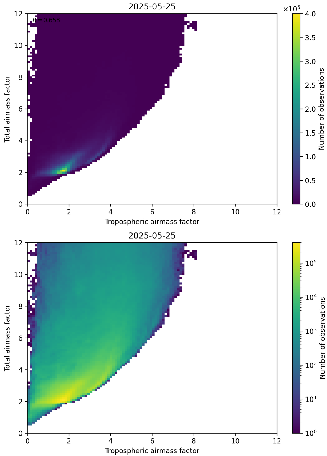
Figure 72: Scatter density plot of “Tropospheric airmass factor” against “Total airmass factor” for 2025-05-24 to 2025-05-26.
