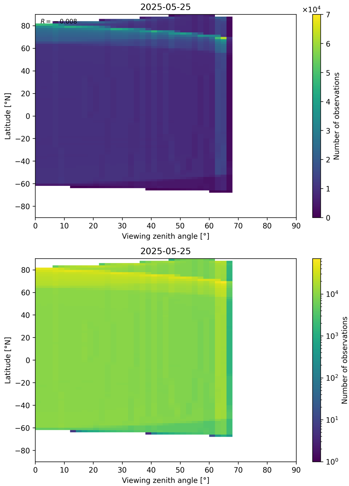
Figure 163: Scatter density plot of “Viewing zenith angle” against “Latitude” for 2025-05-24 to 2025-05-26.
