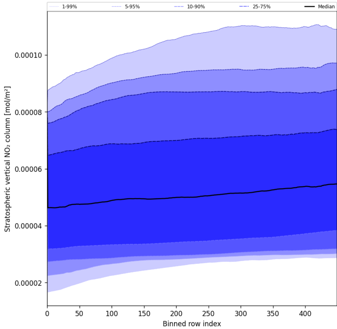
Figure 53: Along track statistics of “Stratospheric vertical NO 2 column” for 2025-05-24 to 2025-05-26
