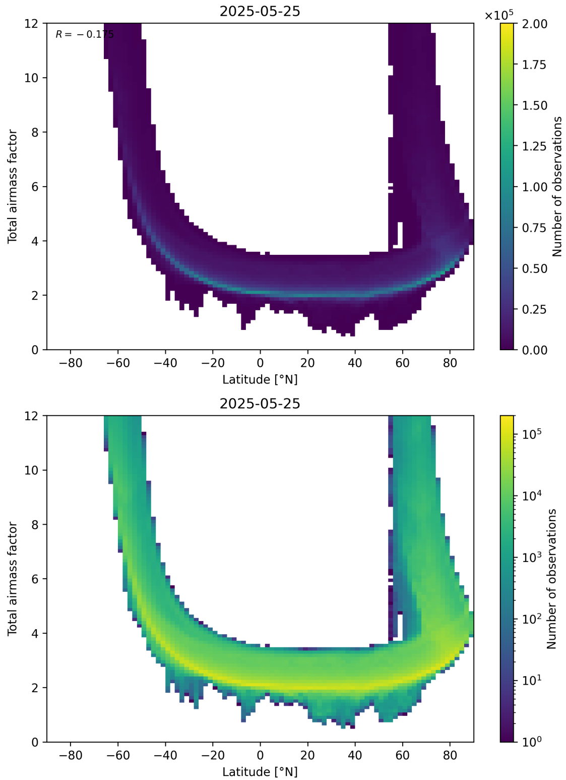
Figure 84: Scatter density plot of “Latitude” against “Total airmass factor” for 2025-05-24 to 2025-05-26.
