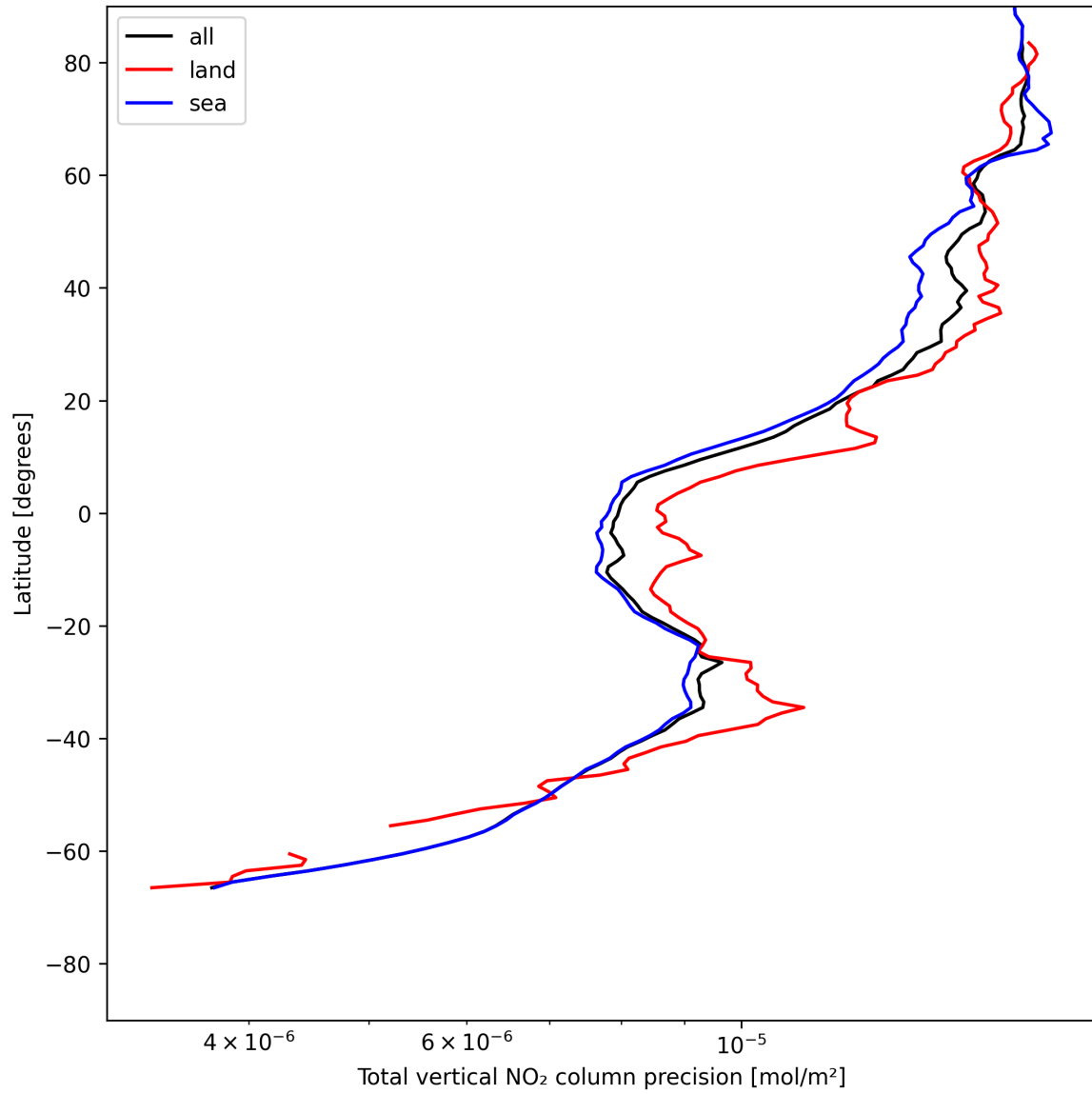
Figure 22: Zonal average of “Total vertical NO 2 column precision” for 2025-05-24 to 2025-05-26.
