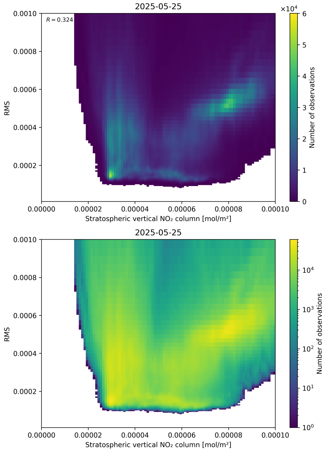
Figure 102: Scatter density plot of “Stratospheric vertical NO 2 column” against “RMS” for 2025-05-24 to 2025-05-26.
