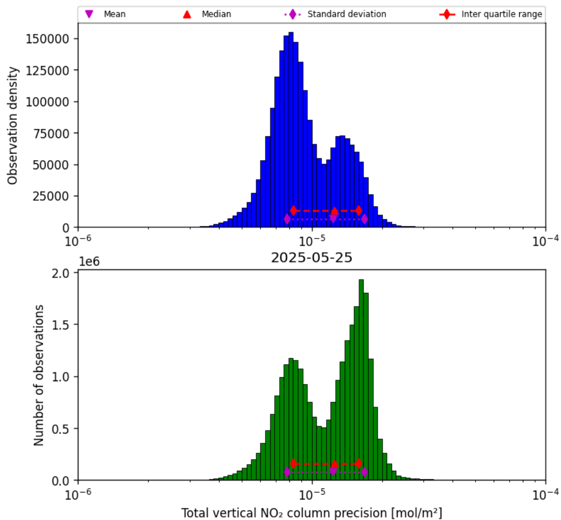
Figure 39: Histogram of "Total vertical NO 2 column precision" for 2025-05-24 to 2025-05-26
