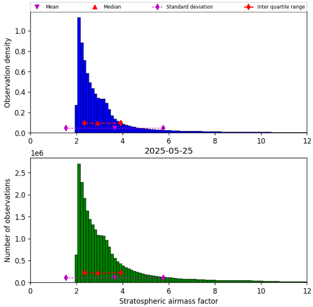
Figure 44: Histogram of “Stratospheric airmass factor” for 2025-05-24 to 2025-05-26
