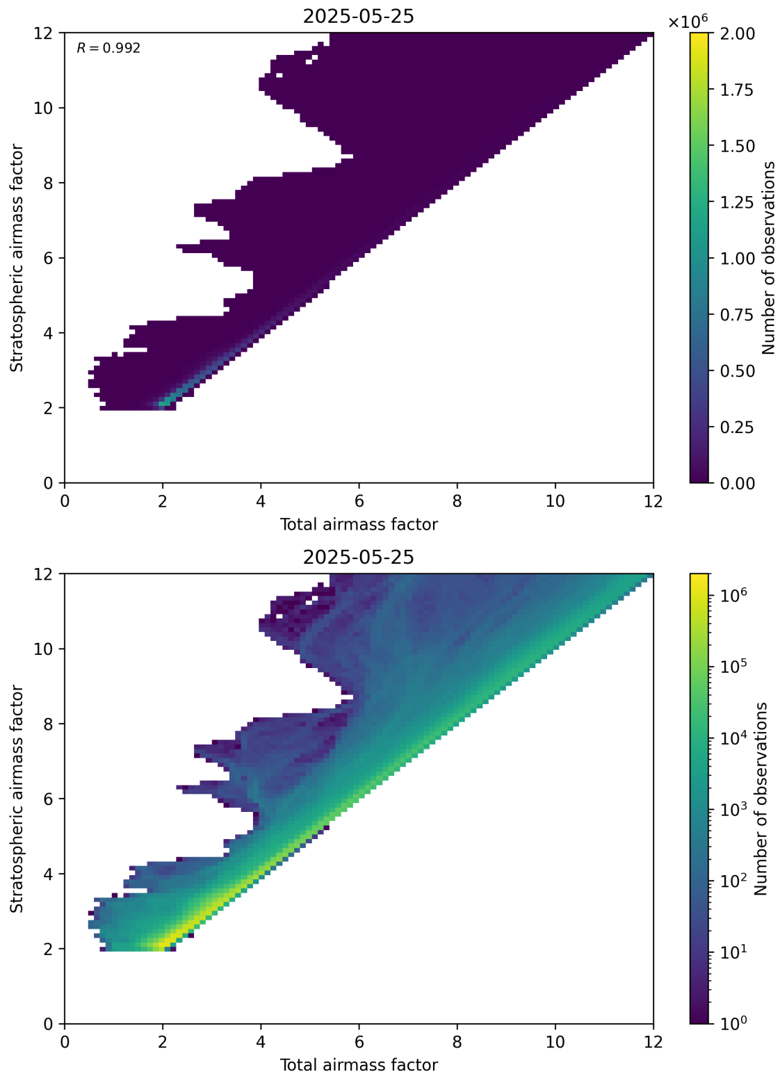
Figure 62: Scatter density plot of “Total airmass factor” against “Stratospheric airmass factor” for 2025-05-24 to 2025-05-26.
