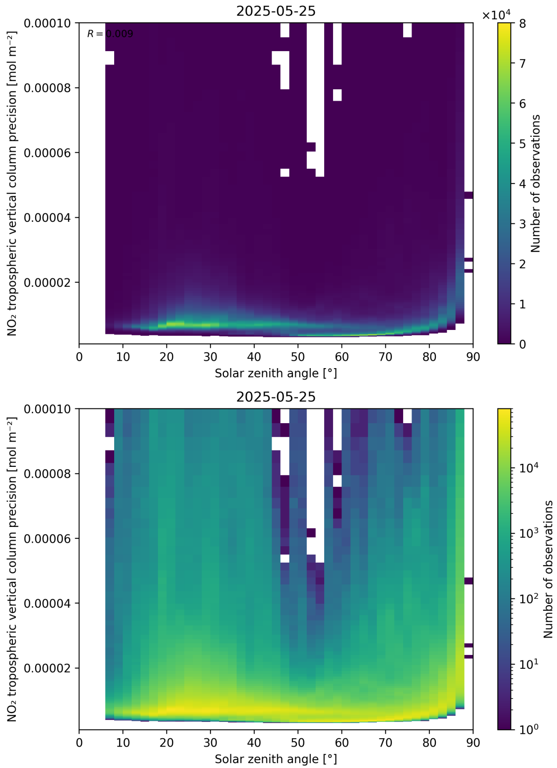
Figure 156: Scatter density plot of “Solar zenith angle” against “NO 2 tropospheric vertical column precision” for 2025-05-24 to 2025-05-26.
