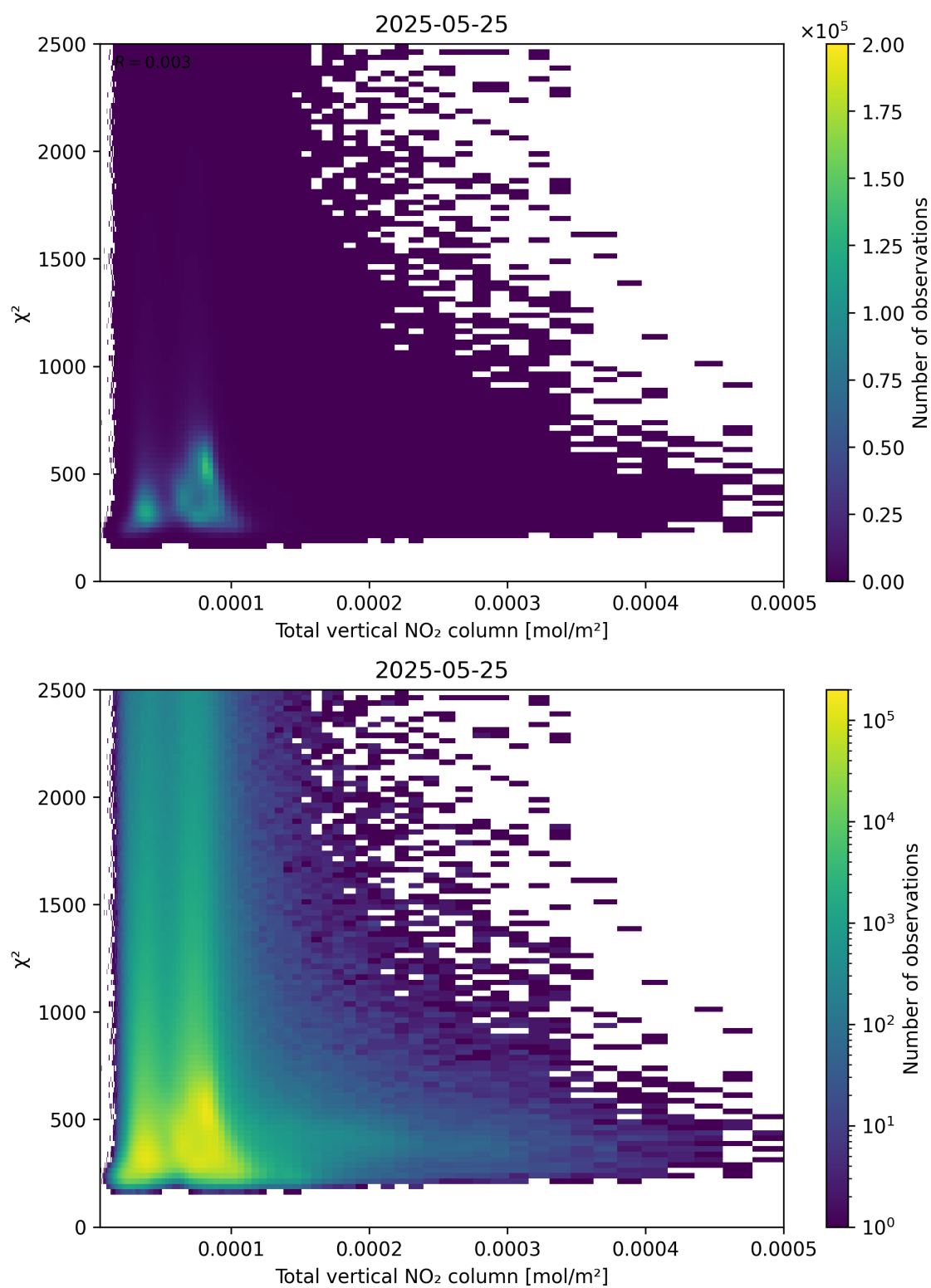
Figure 111: Scatter density plot of “Total vertical NO 2 column” against “ \chi^2 ” for 2025-05-24 to 2025-05-26.
