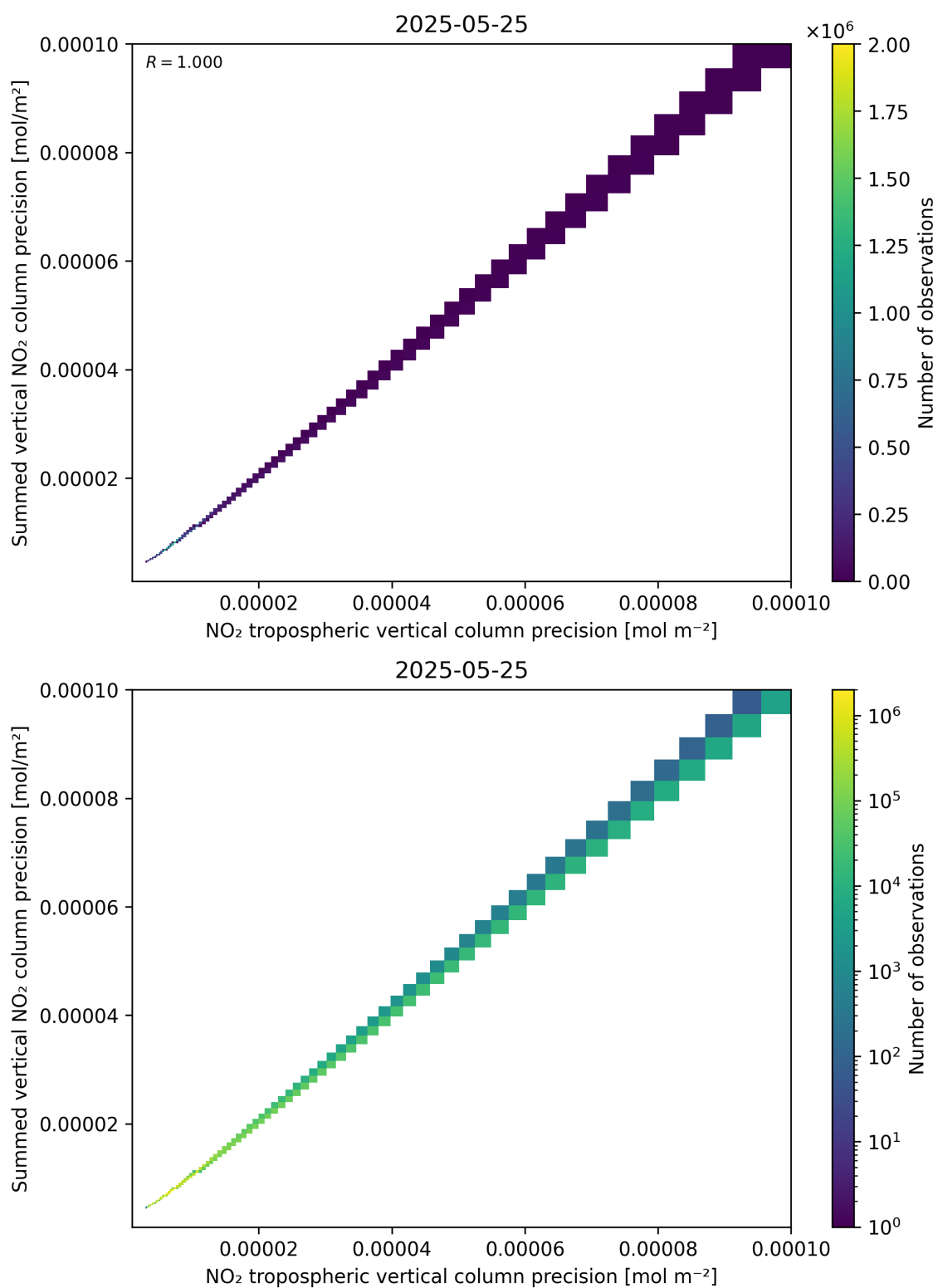
Figure 137: Scatter density plot of “NO 2 tropospheric vertical column precision” against “Summed vertical NO 2 column precision” for 2025-05-24 to 2025-05-26.
