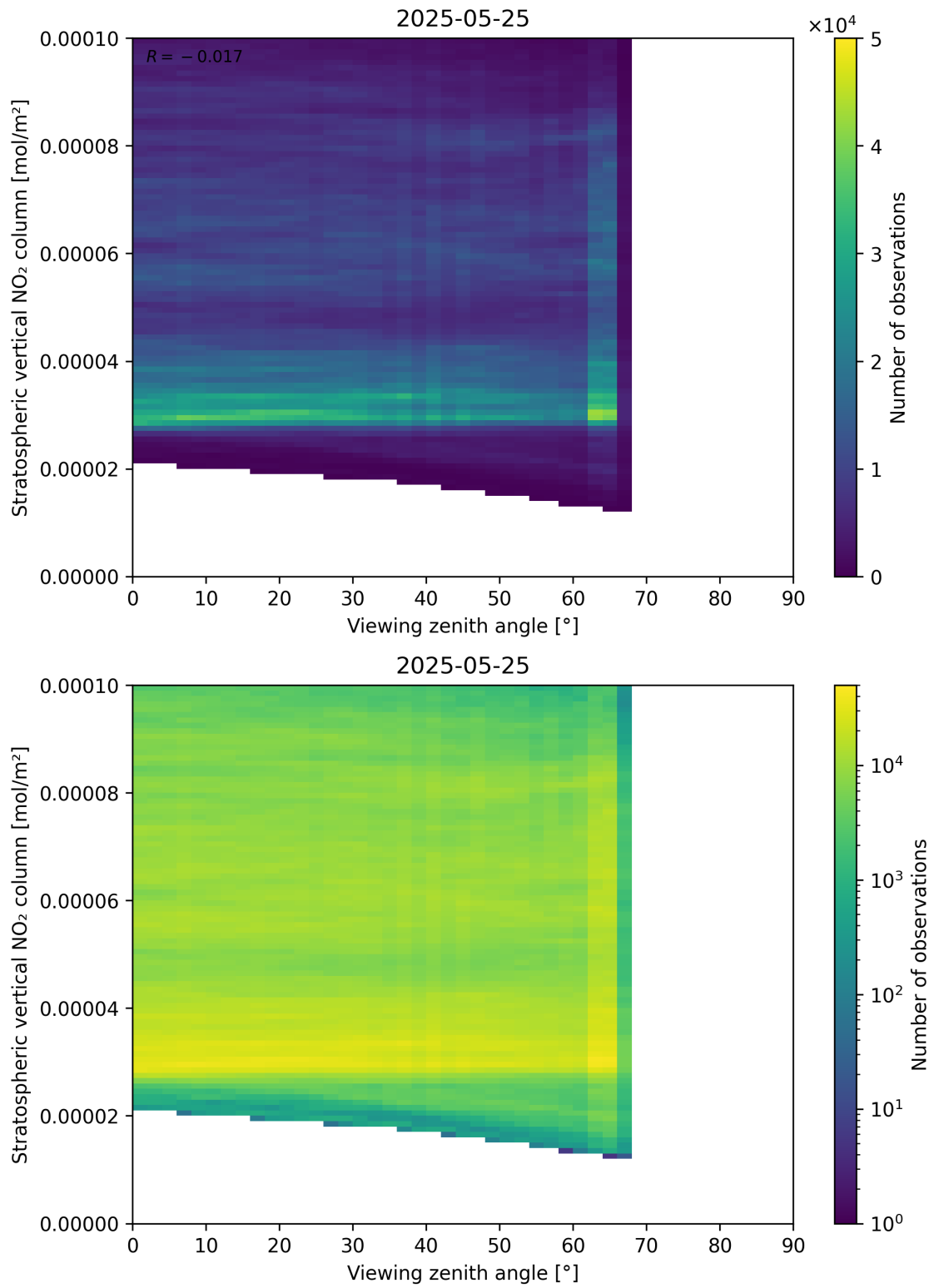
Figure 164: Scatter density plot of “Viewing zenith angle” against “Stratospheric vertical NO 2 column” for 2025-05-24 to 2025-05-26.
