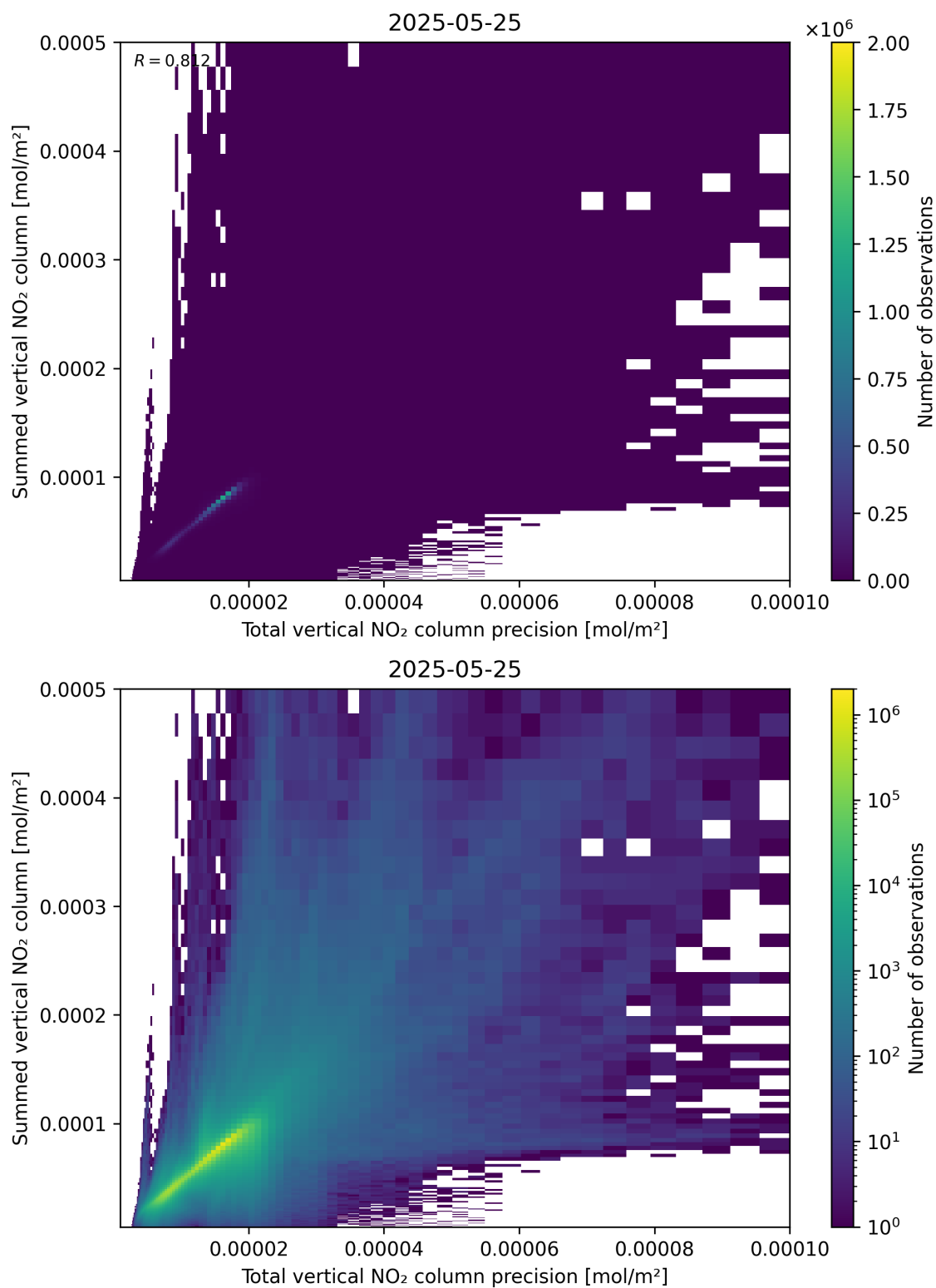
Figure 117: Scatter density plot of “Total vertical NO 2 column precision” against “Summed vertical NO 2 column” for 2025-05-24 to 2025-05-26.
