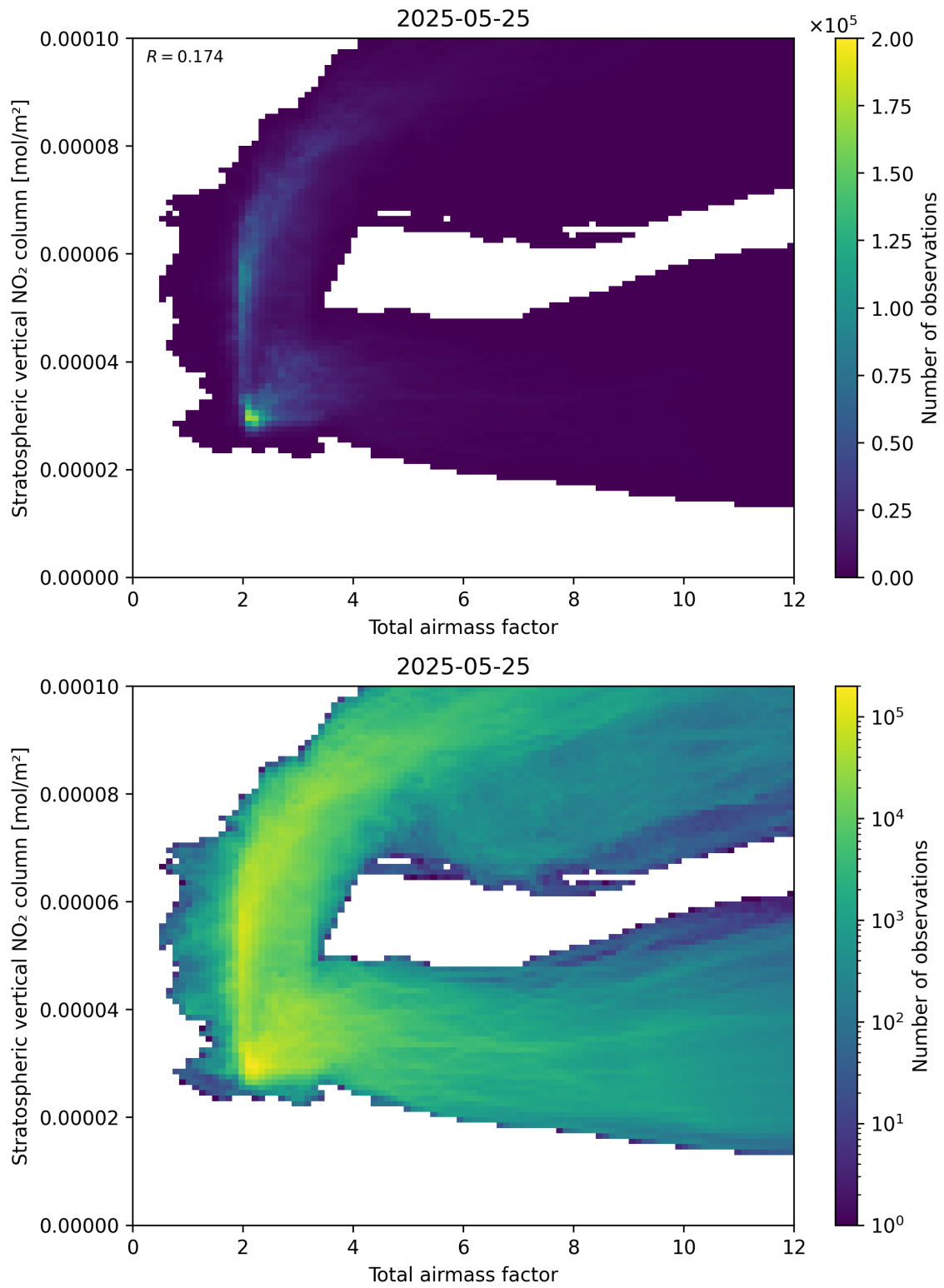
Figure 64: Scatter density plot of “Total airmass factor” against “Stratospheric vertical \text{NO}_2 column” for 2025-05-24 to 2025-05-26.
