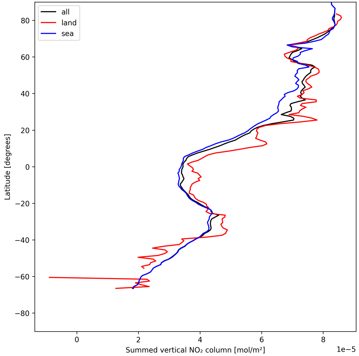
Figure 23: Zonal average of “Summed vertical NO 2 column” for 2025-05-24 to 2025-05-26.
