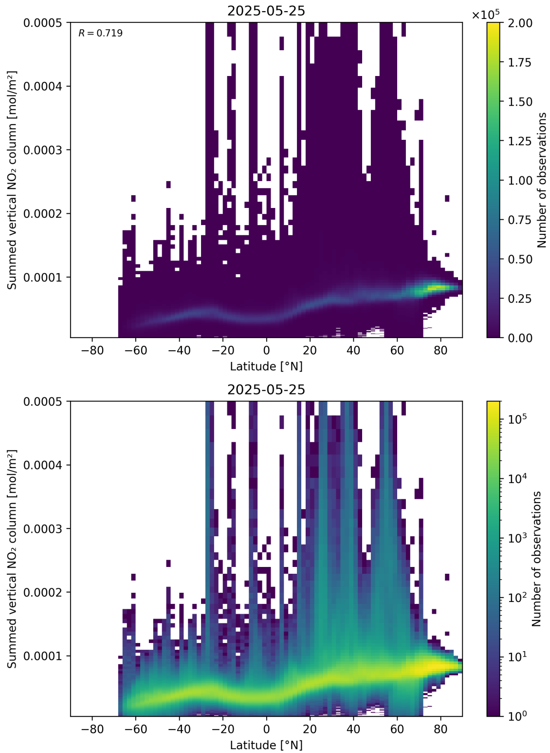
Figure 88: Scatter density plot of “Latitude” against “Summed vertical NO 2 column” for 2025-05-24 to 2025-05-26.
