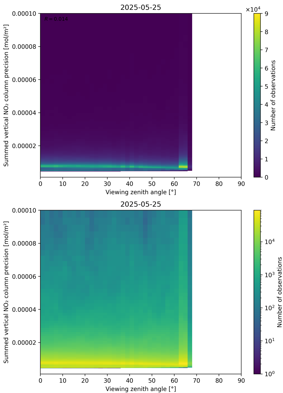
Figure 166: Scatter density plot of “Viewing zenith angle” against “Summed vertical NO 2 column precision” for 2025-05-24 to 2025-05-26.
