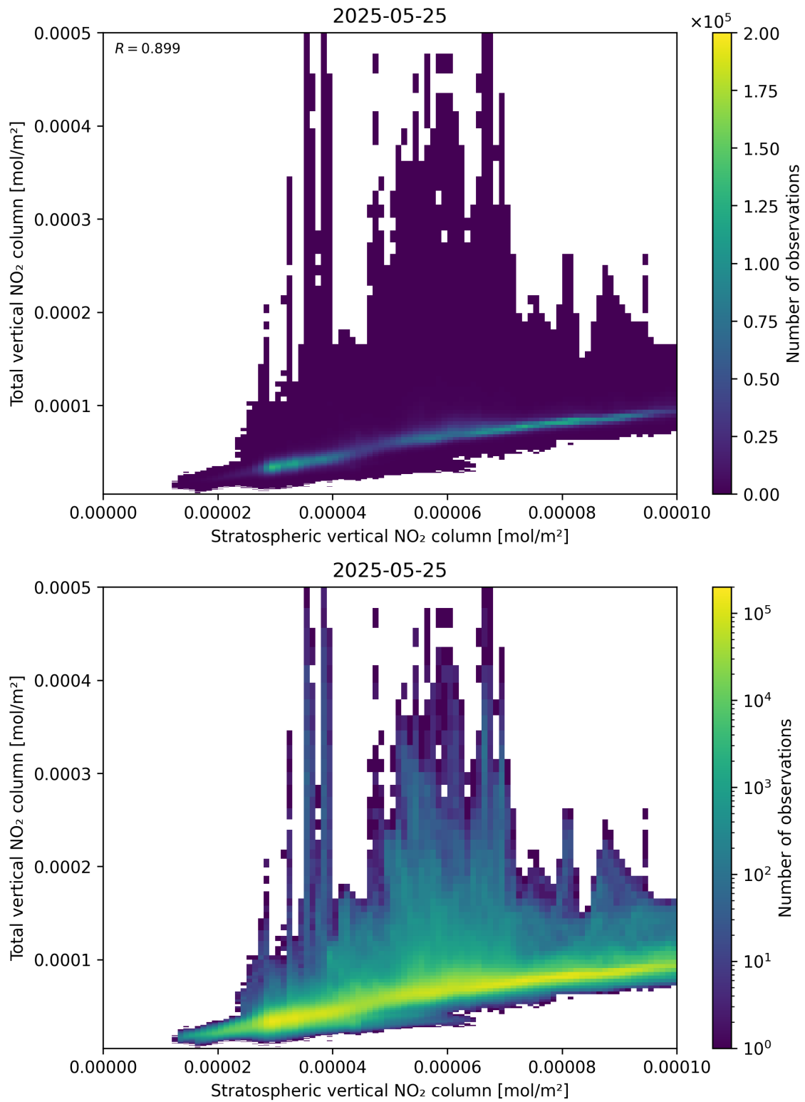
Figure 100: Scatter density plot of “Stratospheric vertical NO 2 column” against “Total vertical NO 2 column” for 2025-05-24 to 2025-05-26.
