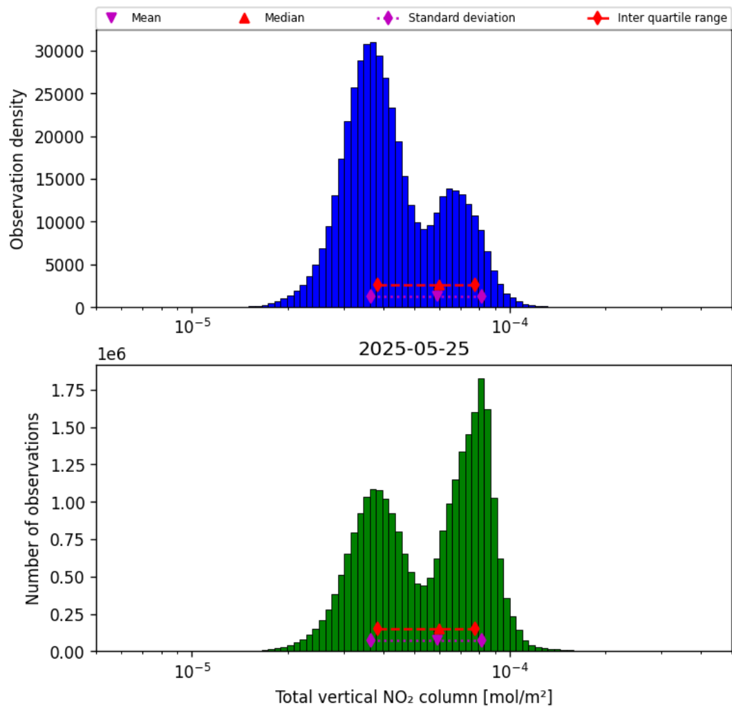
Figure 38: Histogram of “Total vertical NO 2 column” for 2025-05-24 to 2025-05-26
