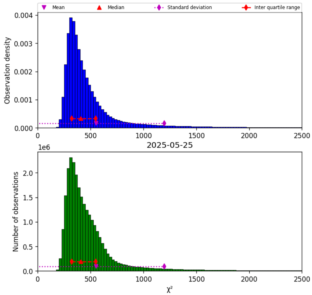
Figure 42: Histogram of “ \chi^2 ” for 2025-05-24 to 2025-05-26
