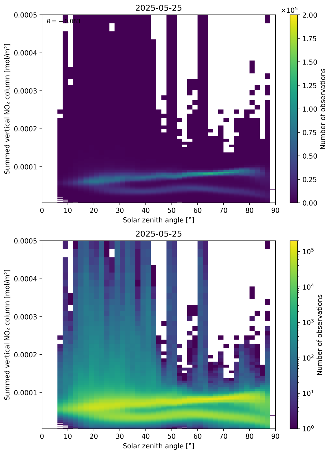
Figure 151: Scatter density plot of “Solar zenith angle” against “Summed vertical NO 2 column” for 2025-05-24 to 2025-05-26.
