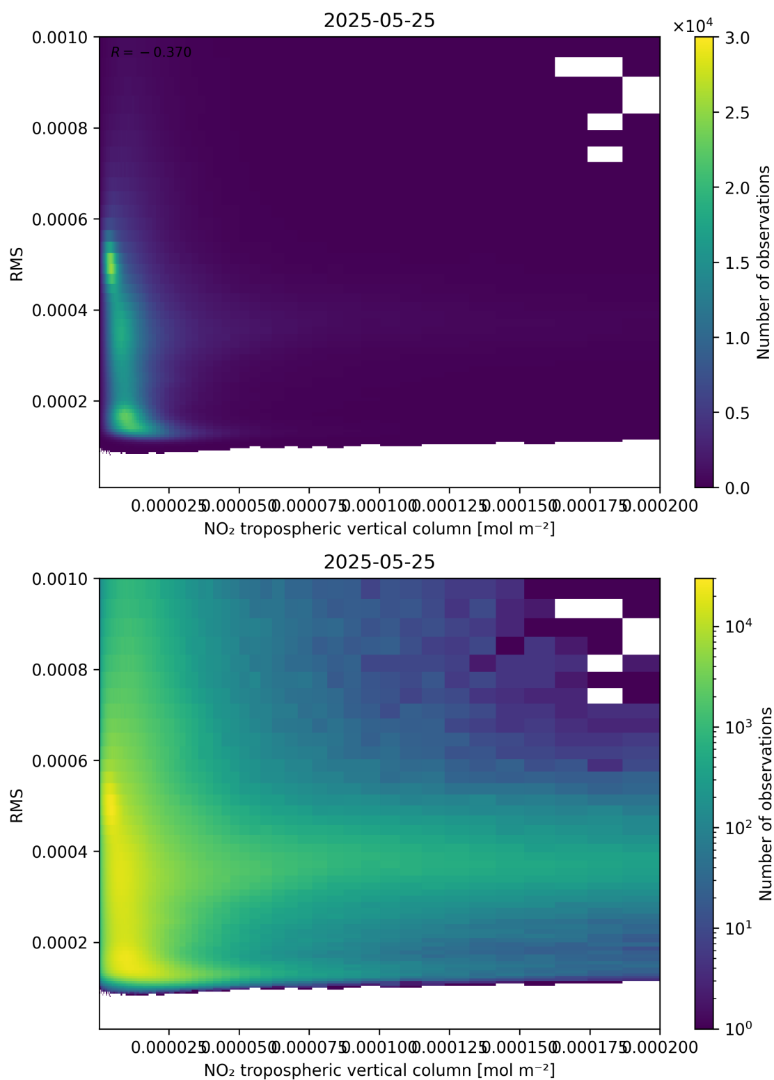
Figure 142: Scatter density plot of “NO 2 tropospheric vertical column” against “RMS” for 2025-05-24 to 2025-05-26.
