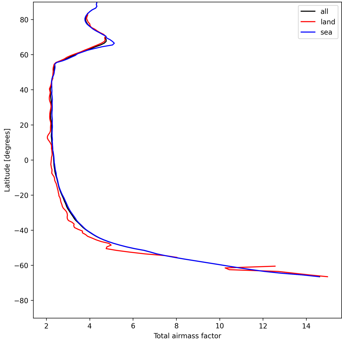
Figure 15: Zonal average of “Total airmass factor” for 2025-05-24 to 2025-05-26.
