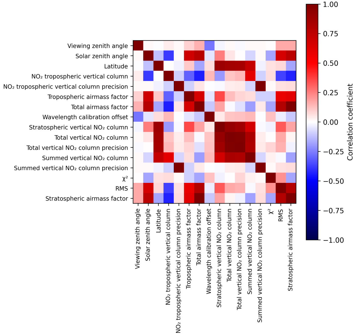
Figure 2: Map of correlation matrix for 2025-05-24 to 2025-05-26.
