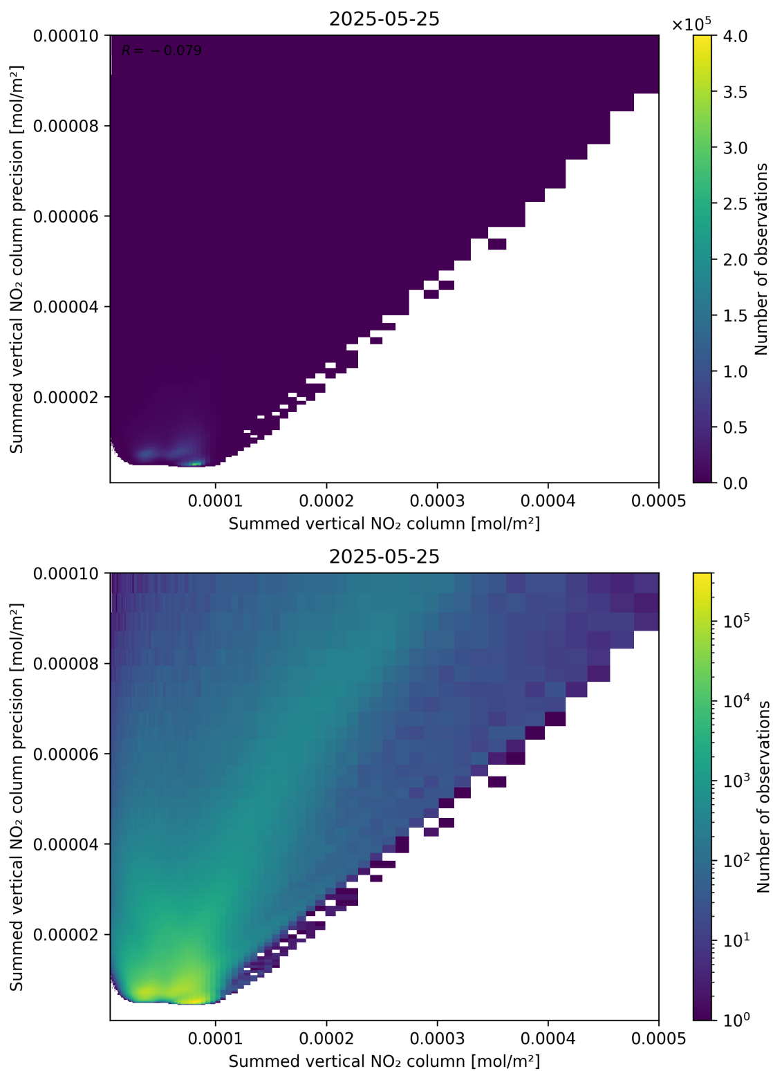
Figure 105: Scatter density plot of “Summed vertical NO 2 column” against “Summed vertical NO 2 column precision” for 2025-05-24 to 2025-05-26.
