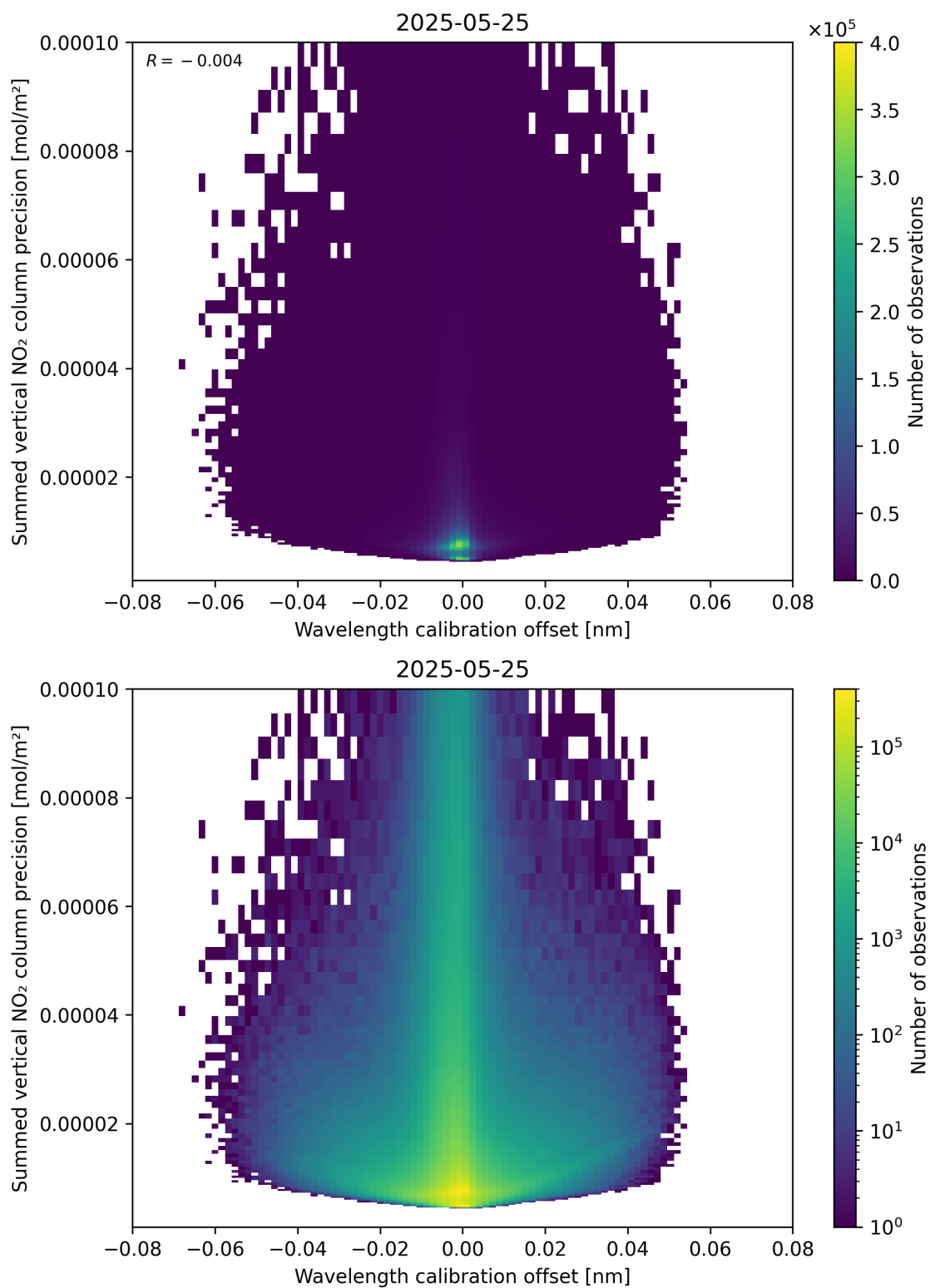
Figure 178: Scatter density plot of “Wavelength calibration offset” against “Summed vertical NO 2 column precision” for 2025-05-24 to 2025-05-26.
