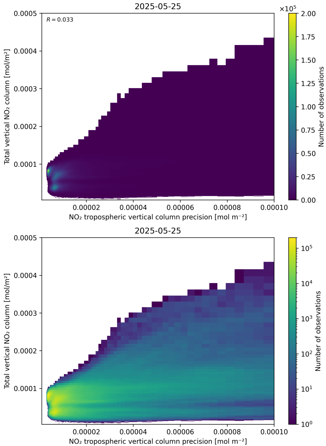
Figure 138: Scatter density plot of “NO 2 tropospheric vertical column precision” against “Total vertical NO 2 column” for 2025-05-24 to 2025-05-26.
