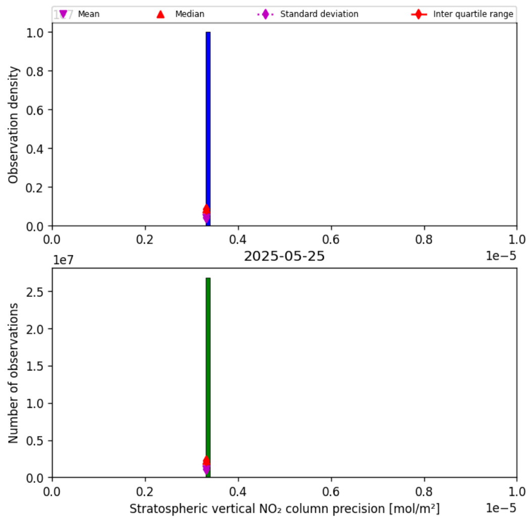
Figure 37: Histogram of “Stratospheric vertical NO 2 column precision” for 2025-05-24 to 2025-05-26
