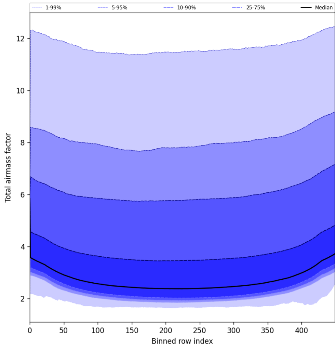
Figure 49: Along track statistics of “Total airmass factor” for 2025-05-24 to 2025-05-26
