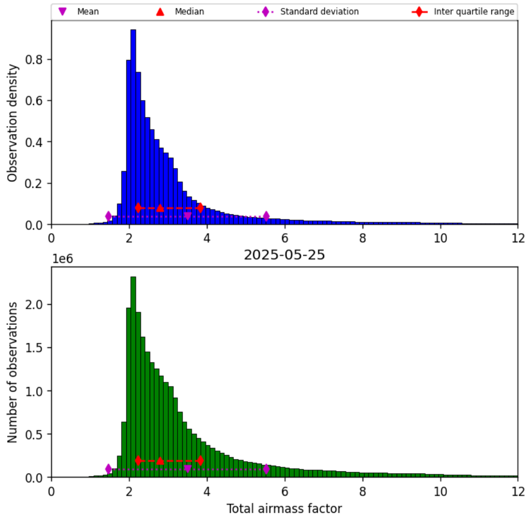
Figure 32: Histogram of “Total airmass factor” for 2025-05-24 to 2025-05-26
