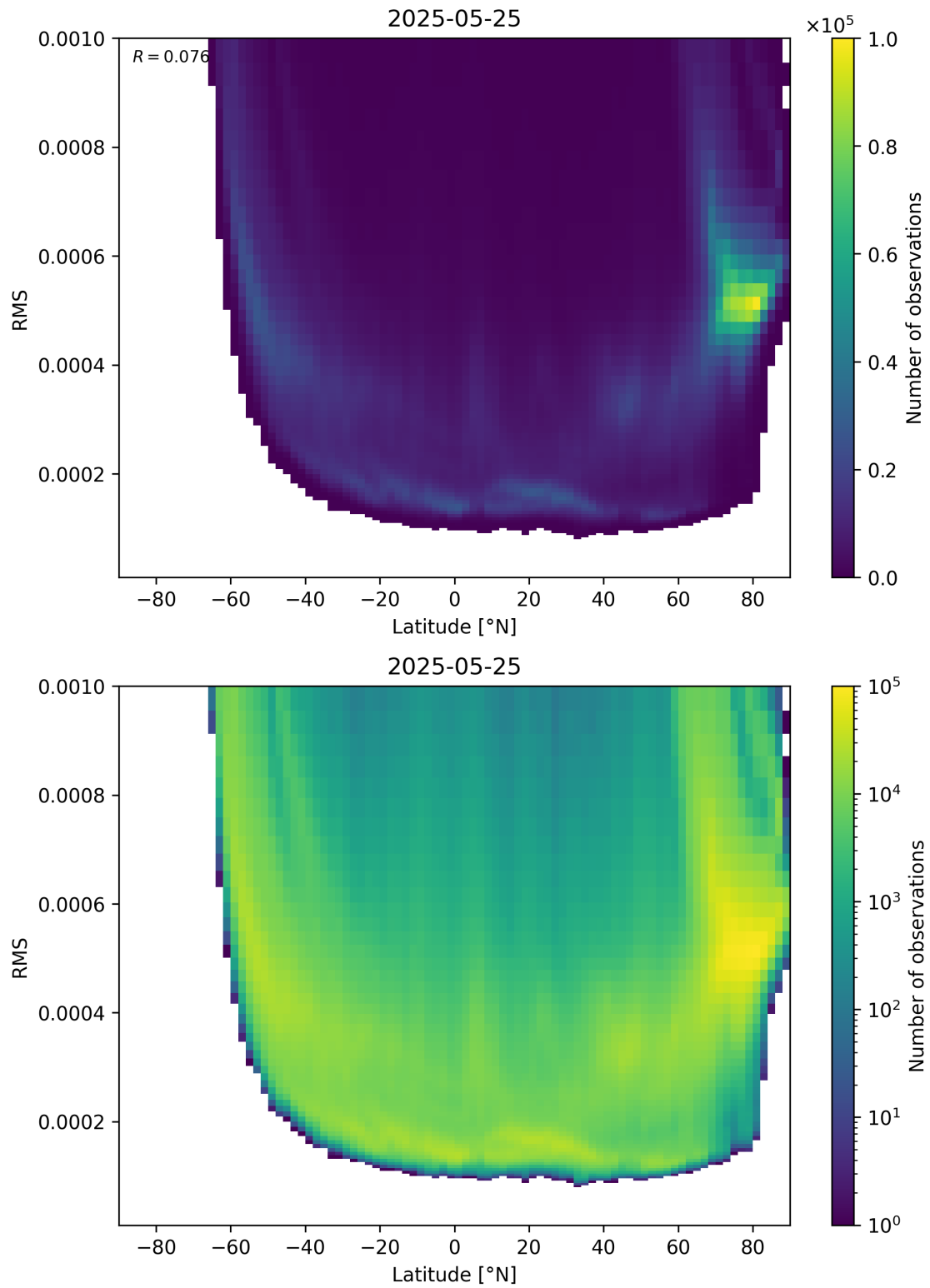
Figure 94: Scatter density plot of “Latitude” against “RMS” for 2025-05-24 to 2025-05-26.
