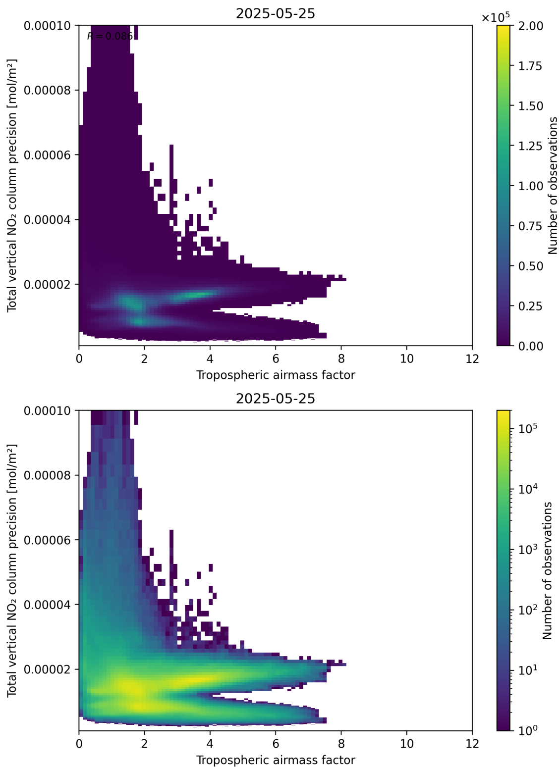
Figure 78: Scatter density plot of “Tropospheric air mass factor” against “Total vertical NO 2 column precision” for 2025-05-24 to 2025-05-26.
