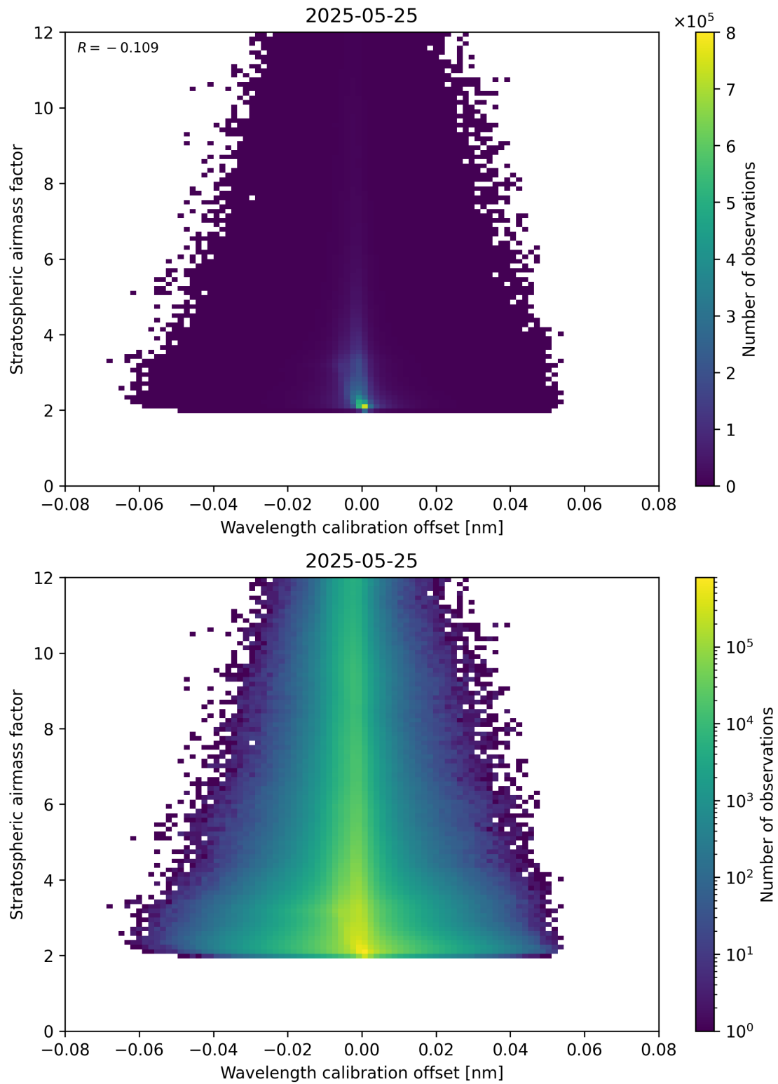
Figure 174: Scatter density plot of “Wavelength calibration offset” against “Stratospheric airmass factor” for 2025-05-24 to 2025-05-26.
