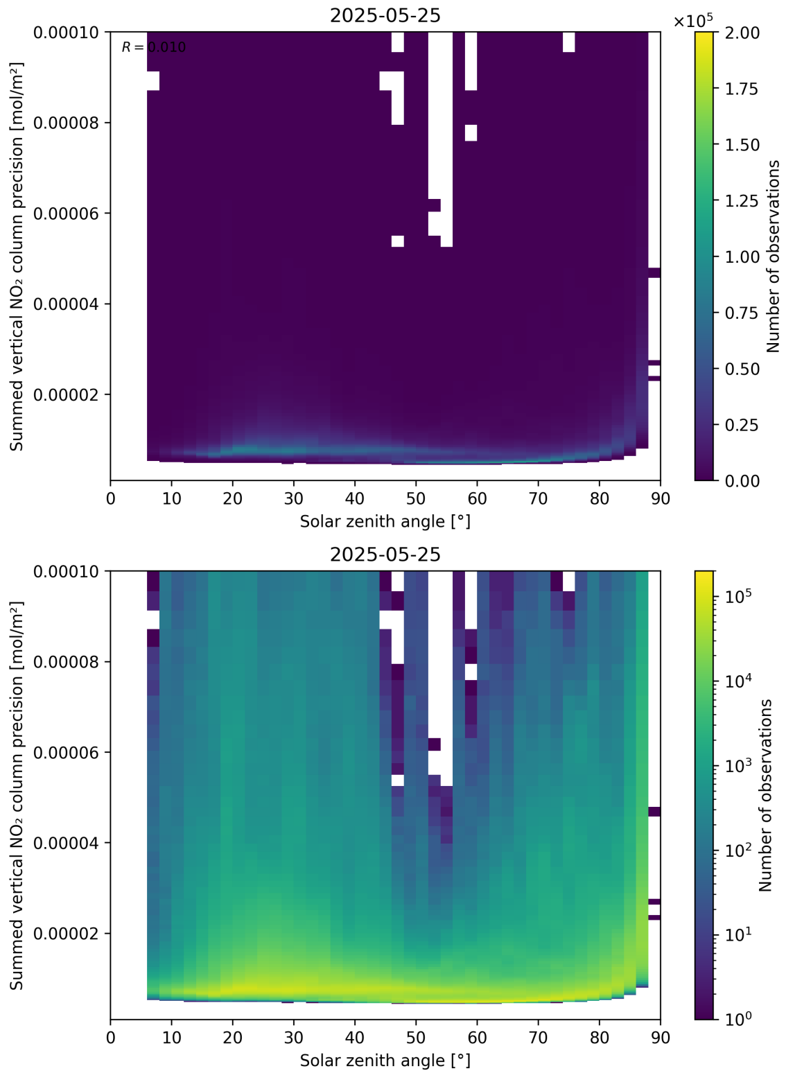
Figure 152: Scatter density plot of “Solar zenith angle” against “Summed vertical NO 2 column precision” for 2025-05-24 to 2025-05-26.
