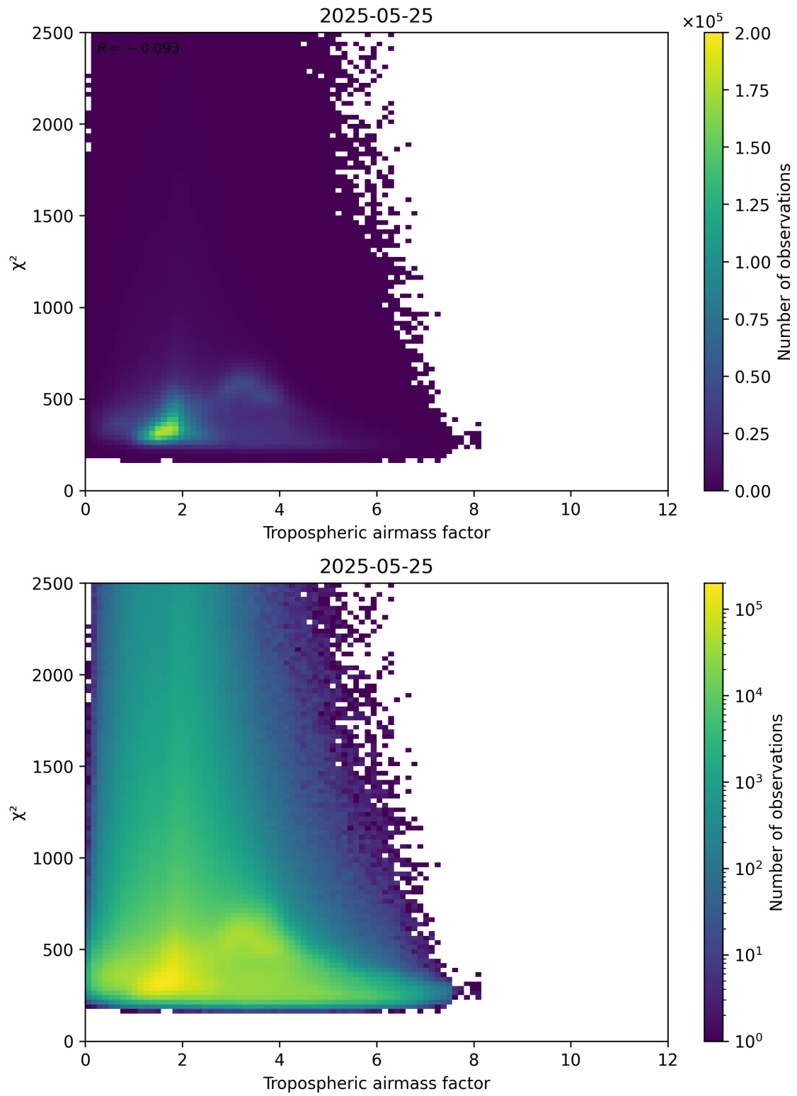
Figure 73: Scatter density plot of “Tropospheric airmass factor” against “ \chi^2 ” for 2025-05-24 to 2025-05-26.
