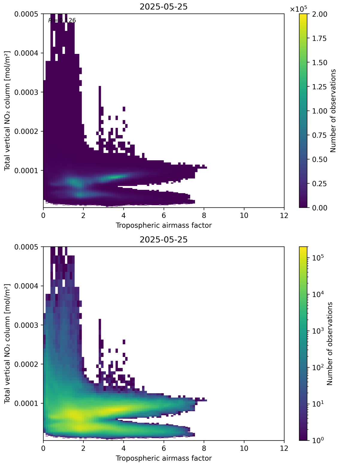
Figure 77: Scatter density plot of “Tropospheric airmass factor” against “Total vertical NO 2 column” for 2025-05-24 to 2025-05-26.
