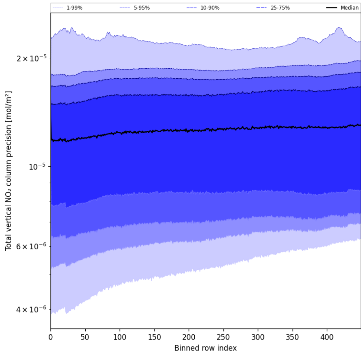
Figure 56: Along track statistics of "Total vertical NO 2 column precision" for 2025-05-24 to 2025-05-26
