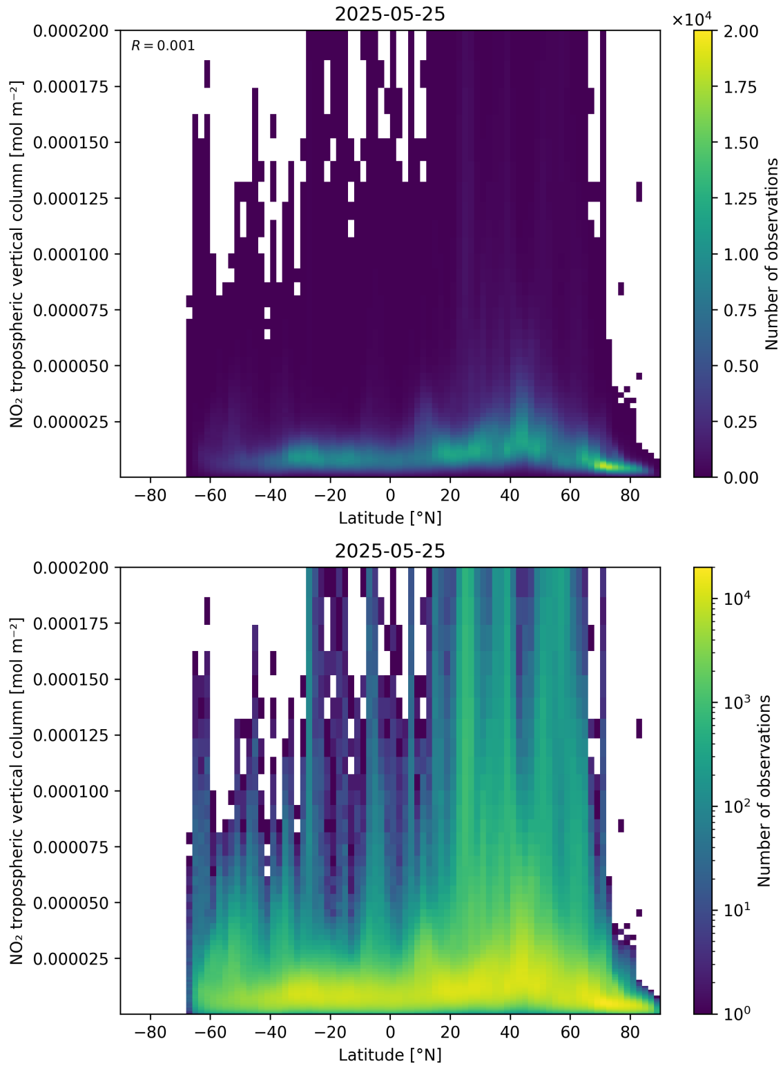
Figure 92: Scatter density plot of “Latitude” against “NO 2 tropospheric vertical column” for 2025-05-24 to 2025-05-26.
