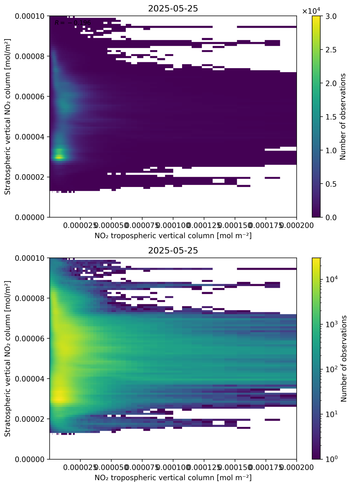
Figure 125: Scatter density plot of “NO 2 tropospheric vertical column” against “Stratospheric vertical NO 2 column” for 2025-05-24 to 2025-05-26.
