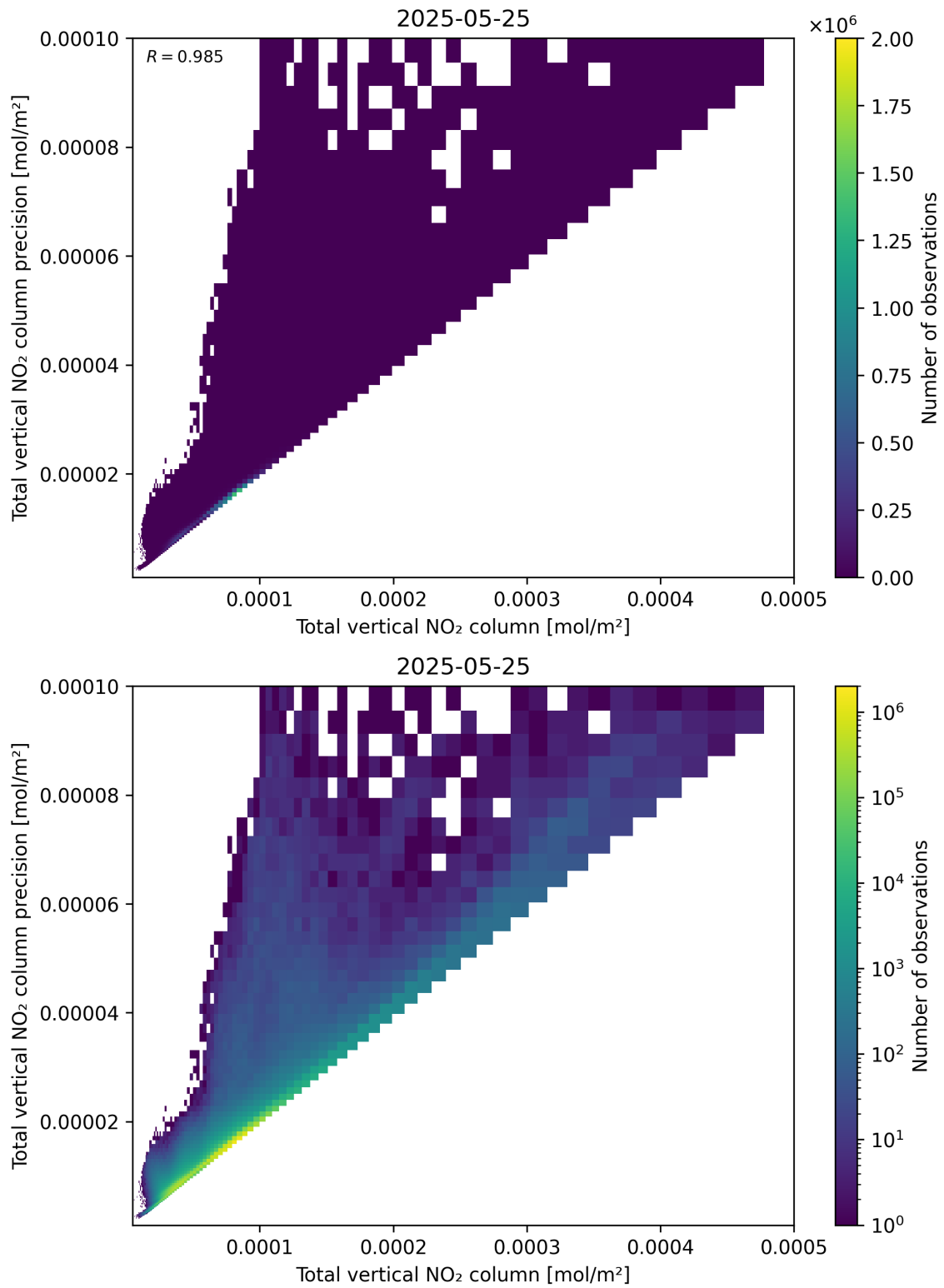
Figure 114: Scatter density plot of “Total vertical NO 2 column” against “Total vertical NO 2 column precision” for 2025-05-24 to 2025-05-26.
