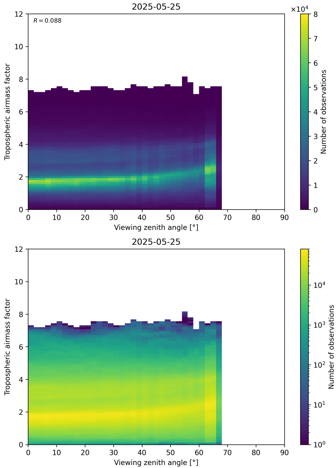
Figure 161: Scatter density plot of “Viewing zenith angle” against “Tropospheric airmass factor” for 2025-05-24 to 2025-05-26.
