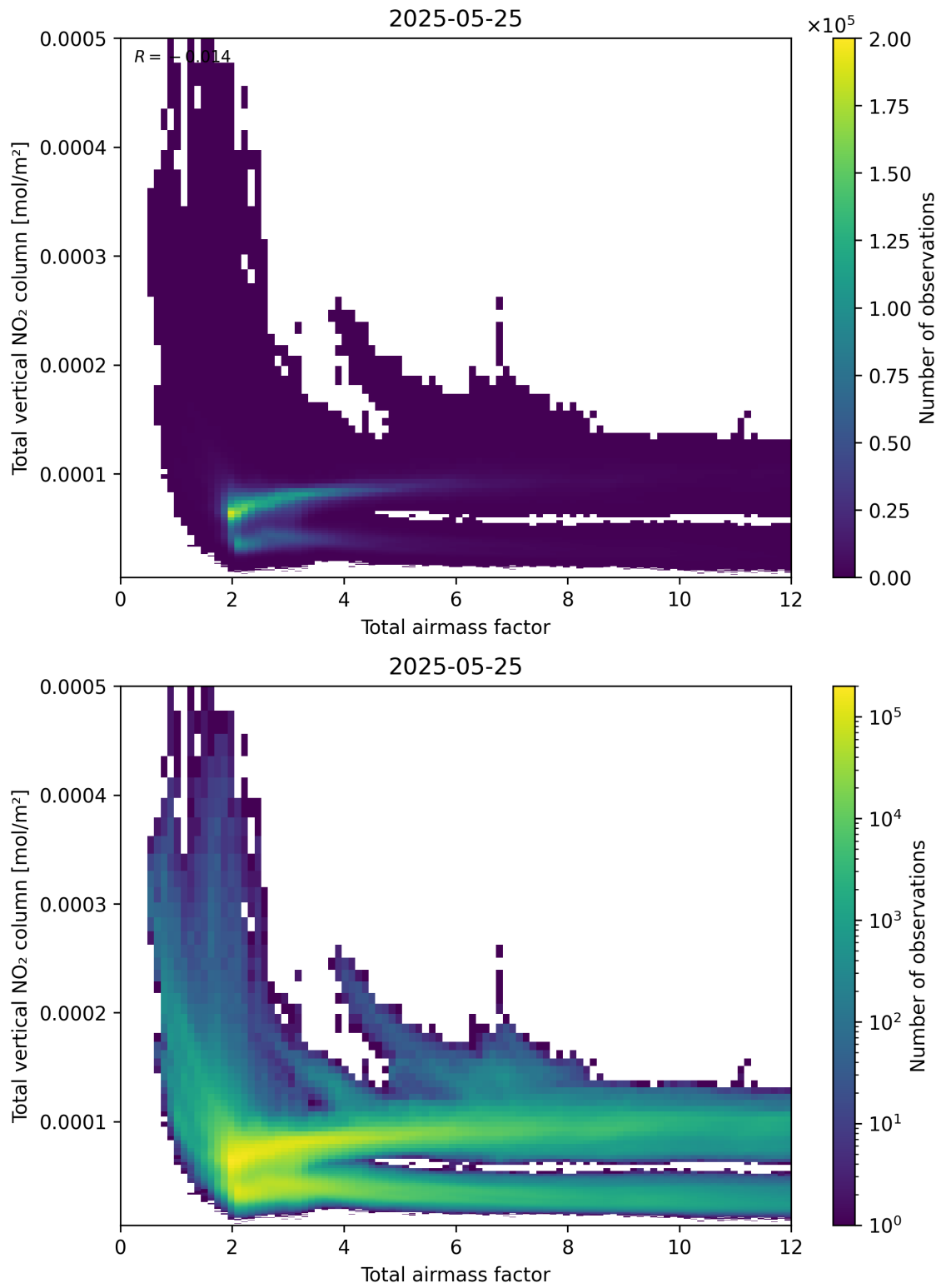
Figure 67: Scatter density plot of “Total airmass factor” against “Total vertical NO 2 column” for 2025-05-24 to 2025-05-26.
