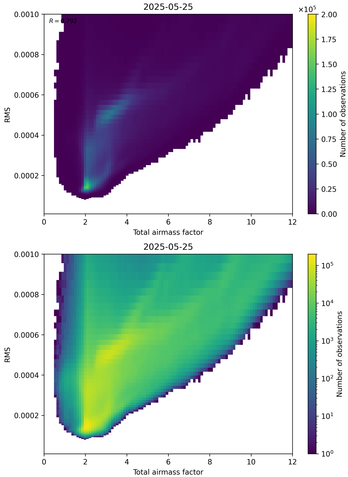
Figure 69: Scatter density plot of “Total airmass factor” against “RMS” for 2025-05-24 to 2025-05-26.
