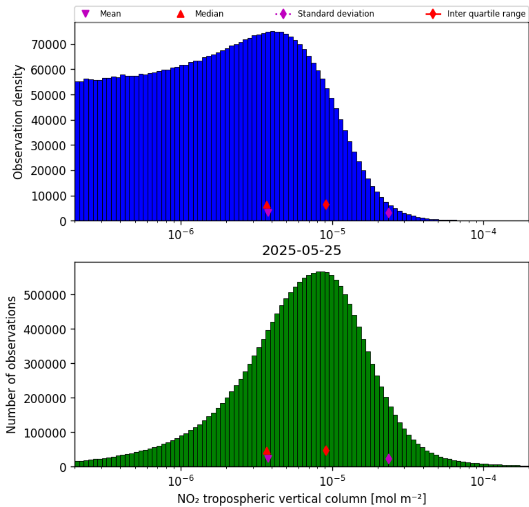
Figure 29: Histogram of “NO 2 tropospheric vertical column” for 2025-05-24 to 2025-05-26
