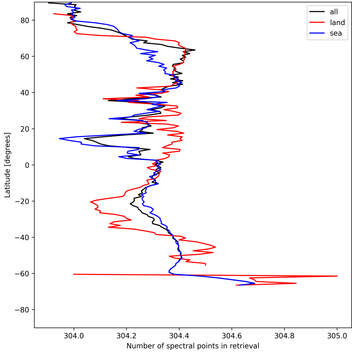
Figure 16: Zonal average of “Number of spectral points in retrieval” for 2025-05-24 to 2025-05-26.
