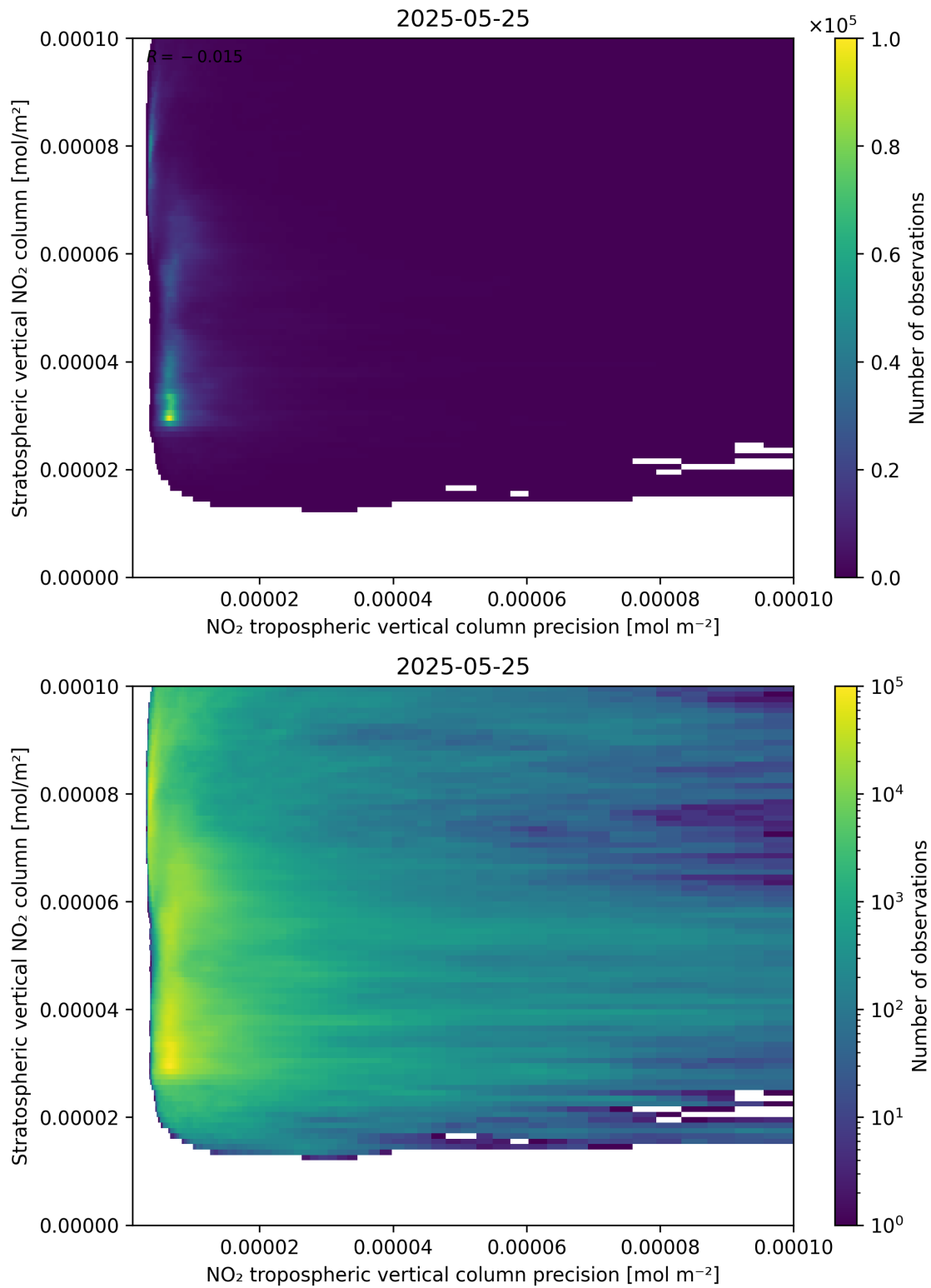
Figure 135: Scatter density plot of “NO 2 tropospheric vertical column precision” against “Stratospheric vertical NO 2 column” for 2025-05-24 to 2025-05-26.
