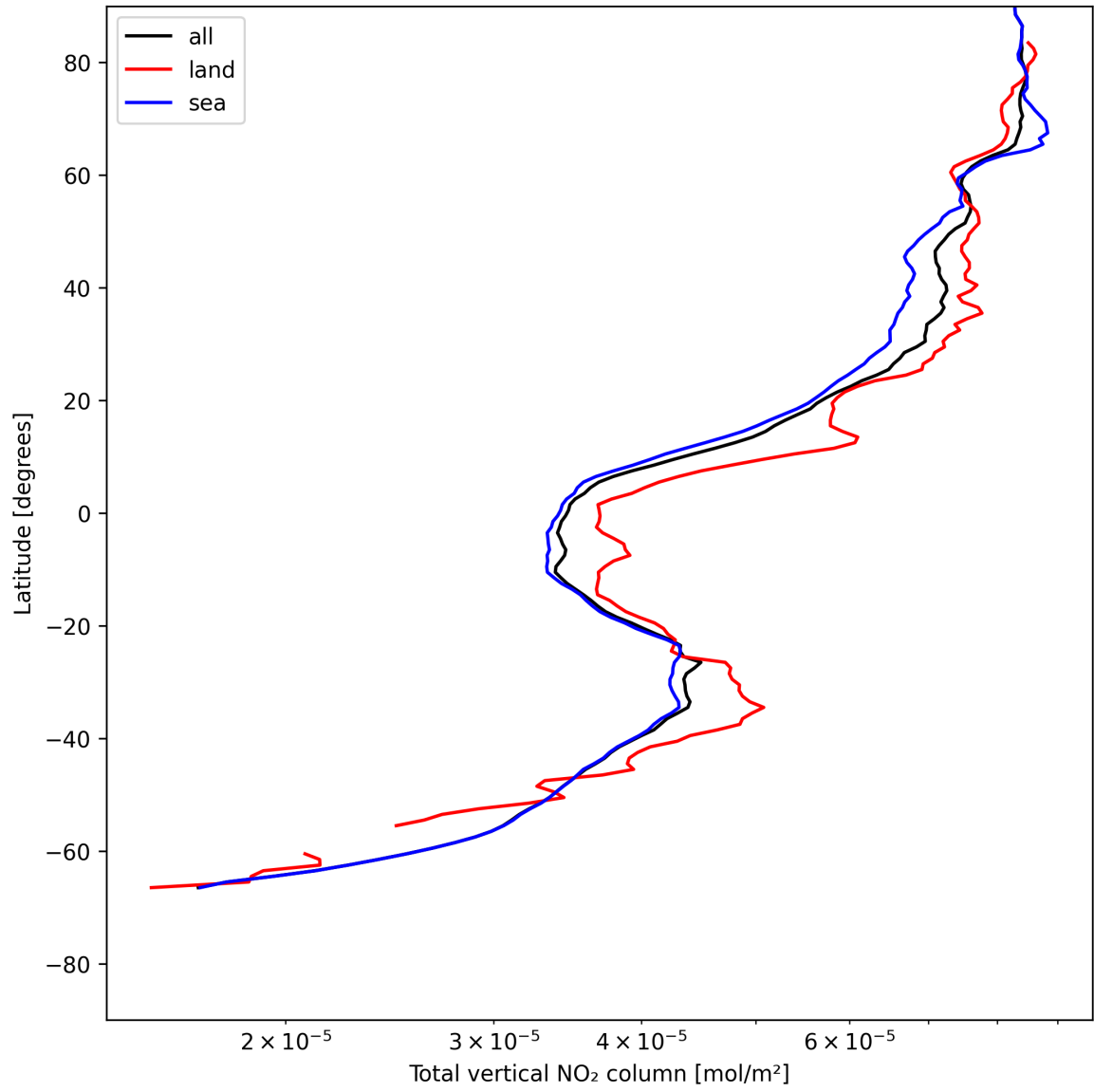
Figure 21: Zonal average of “Total vertical NO 2 column” for 2025-05-24 to 2025-05-26.
