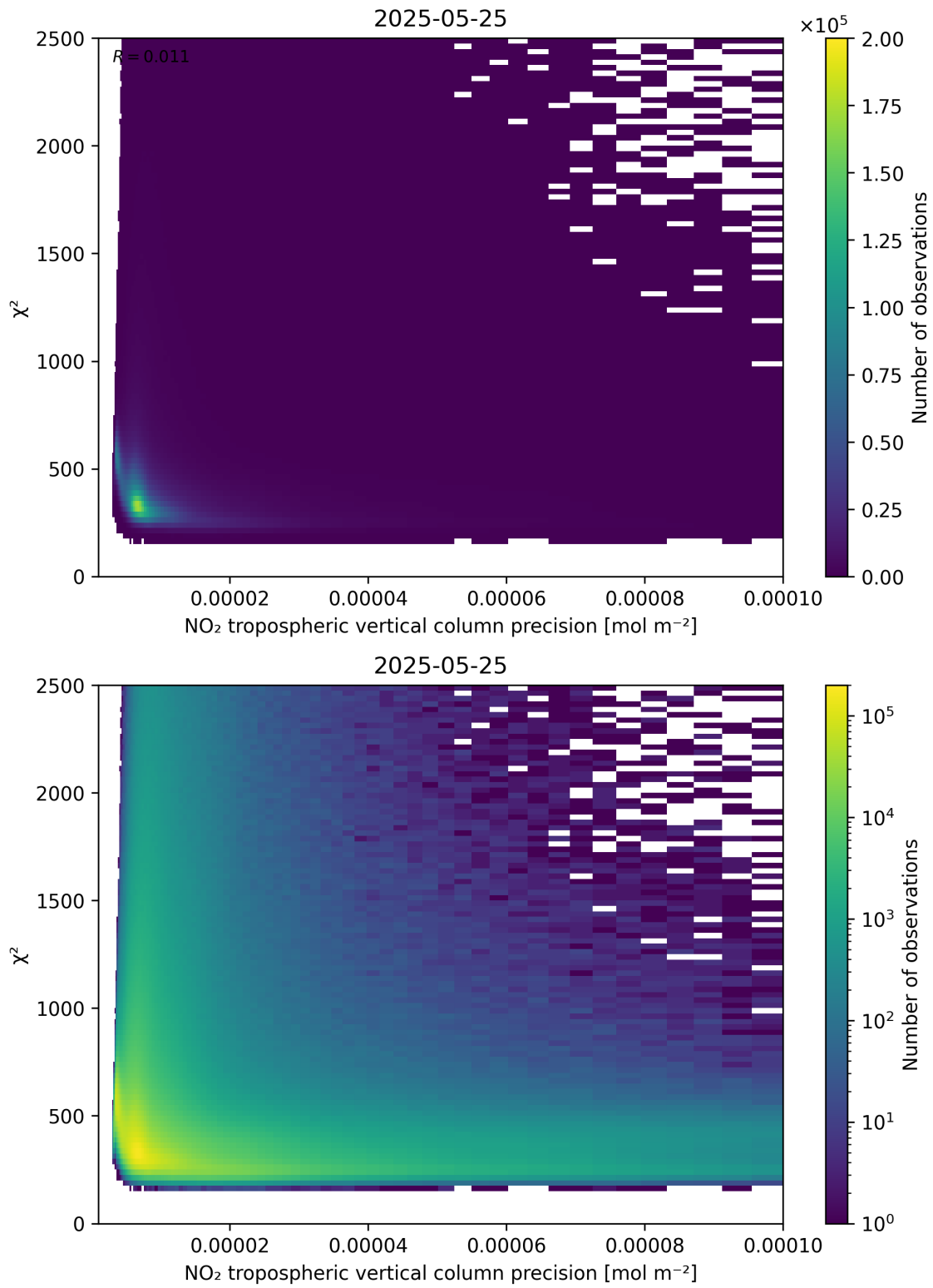
Figure 134: Scatter density plot of “NO 2 tropospheric vertical column precision” against “ \chi^2 ” for 2025-05-24 to 2025-05-26.
