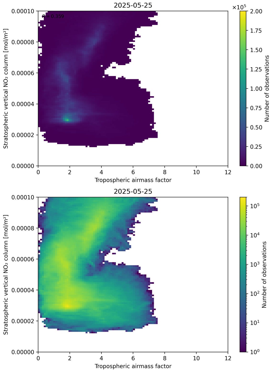
Figure 74: Scatter density plot of “Tropospheric air mass factor” against “Stratospheric vertical NO 2 column” for 2025-05-24 to 2025-05-26.
