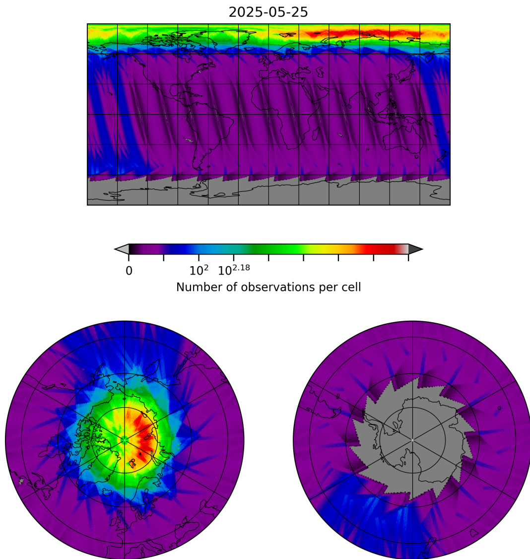
Figure 10: Map of the number of observations for 2025-05-24 to 2025-05-26
