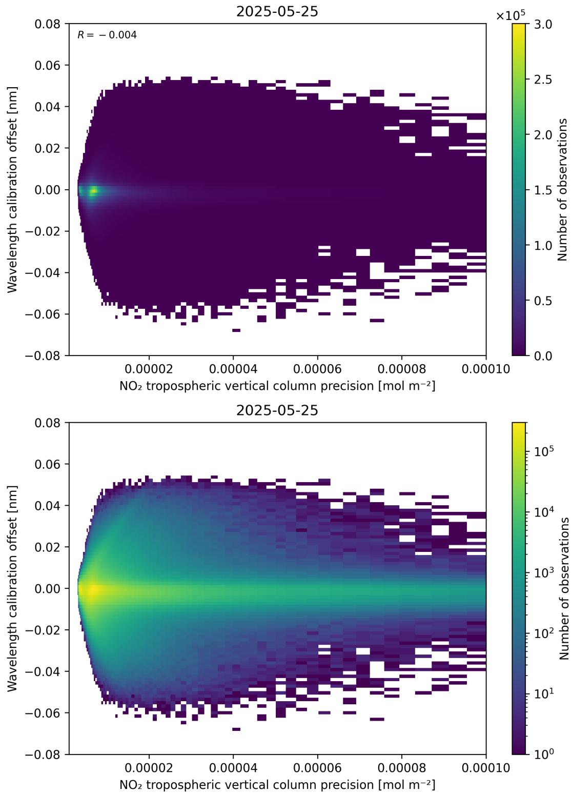
Figure 141: Scatter density plot of “NO 2 tropospheric vertical column precision” against “Wavelength calibration offset” for 2025-05-24 to 2025-05-26.
