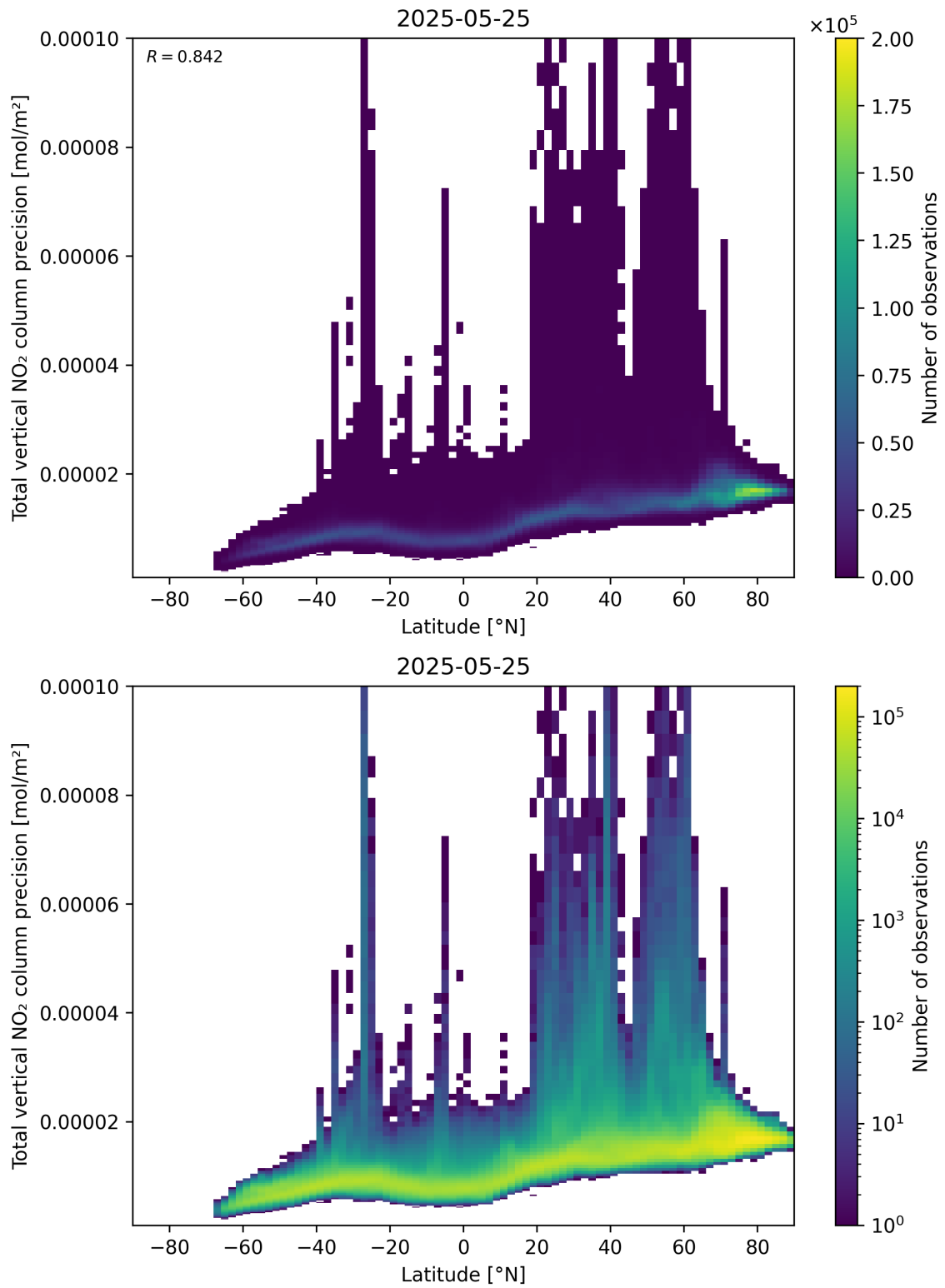
Figure 91: Scatter density plot of “Latitude” against “Total vertical NO 2 column precision” for 2025-05-24 to 2025-05-26.
