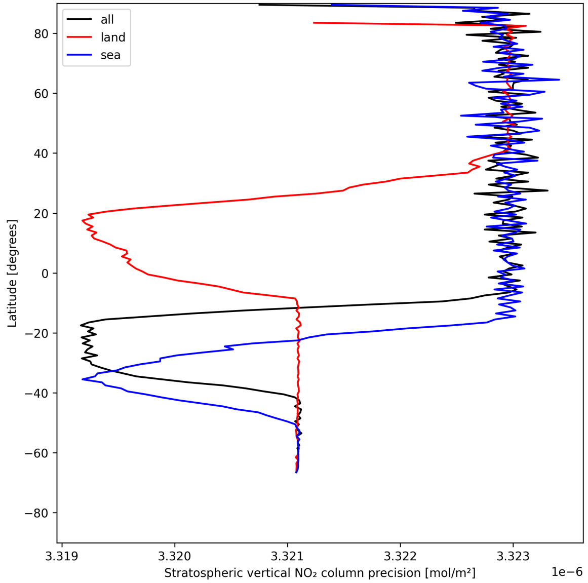
Figure 20: Zonal average of “Stratospheric vertical NO 2 column precision” for 2025-05-24 to 2025-05-26.
