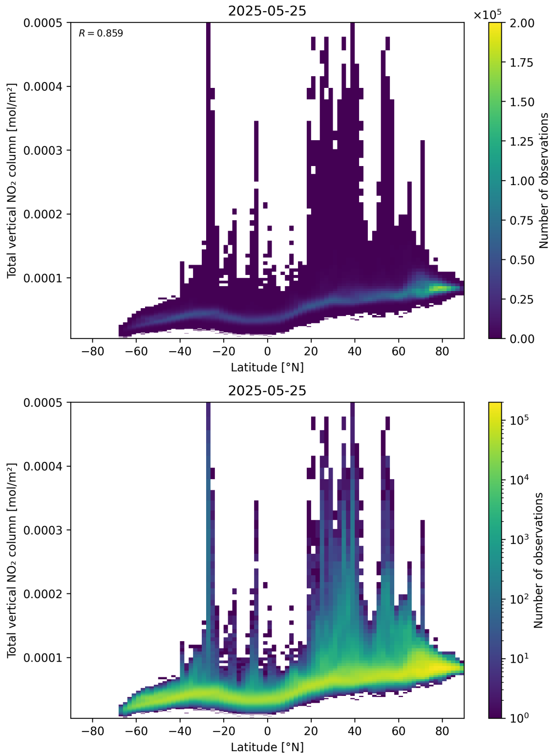
Figure 90: Scatter density plot of “Latitude” against “Total vertical NO 2 column” for 2025-05-24 to 2025-05-26.
