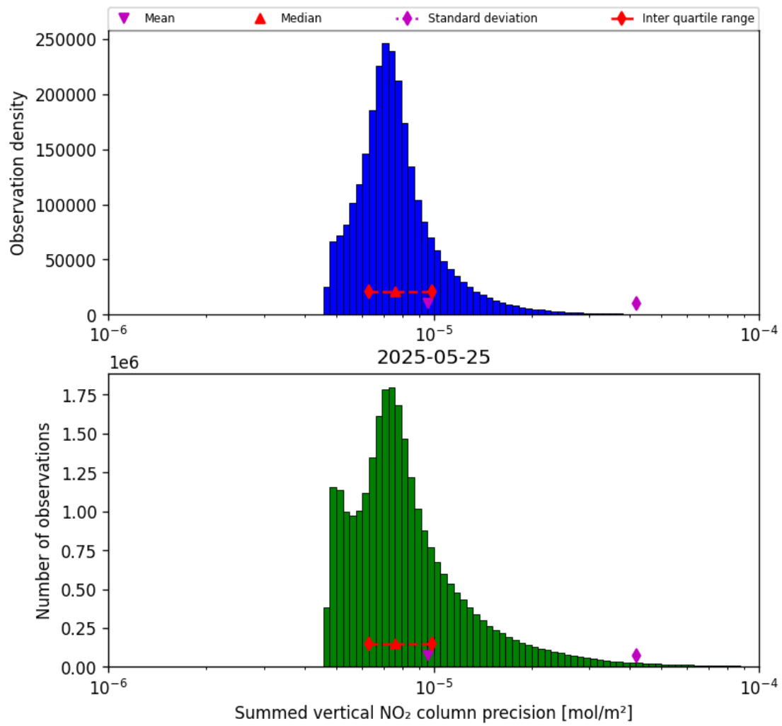
Figure 41: Histogram of "Summed vertical NO 2 column precision" for 2025-05-24 to 2025-05-26
