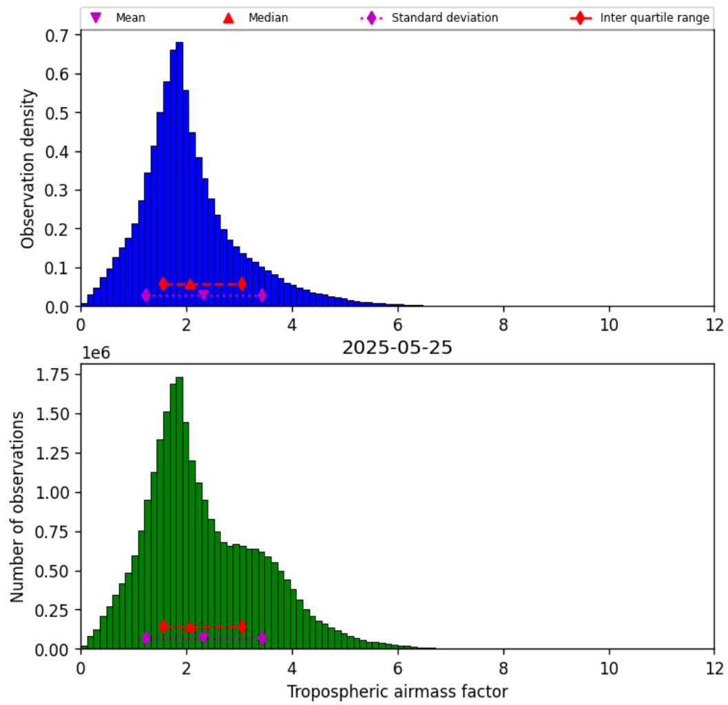
Figure 31: Histogram of “Tropospheric airmass factor” for 2025-05-24 to 2025-05-26
