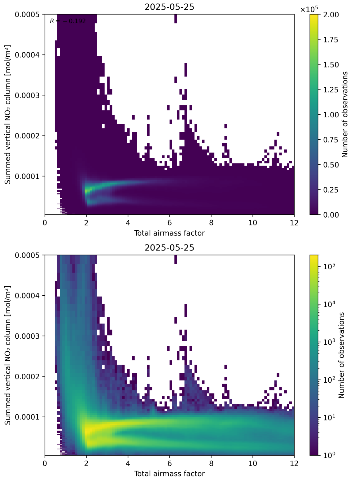
Figure 65: Scatter density plot of “Total airmass factor” against “Summed vertical NO 2 column” for 2025-05-24 to 2025-05-26.
