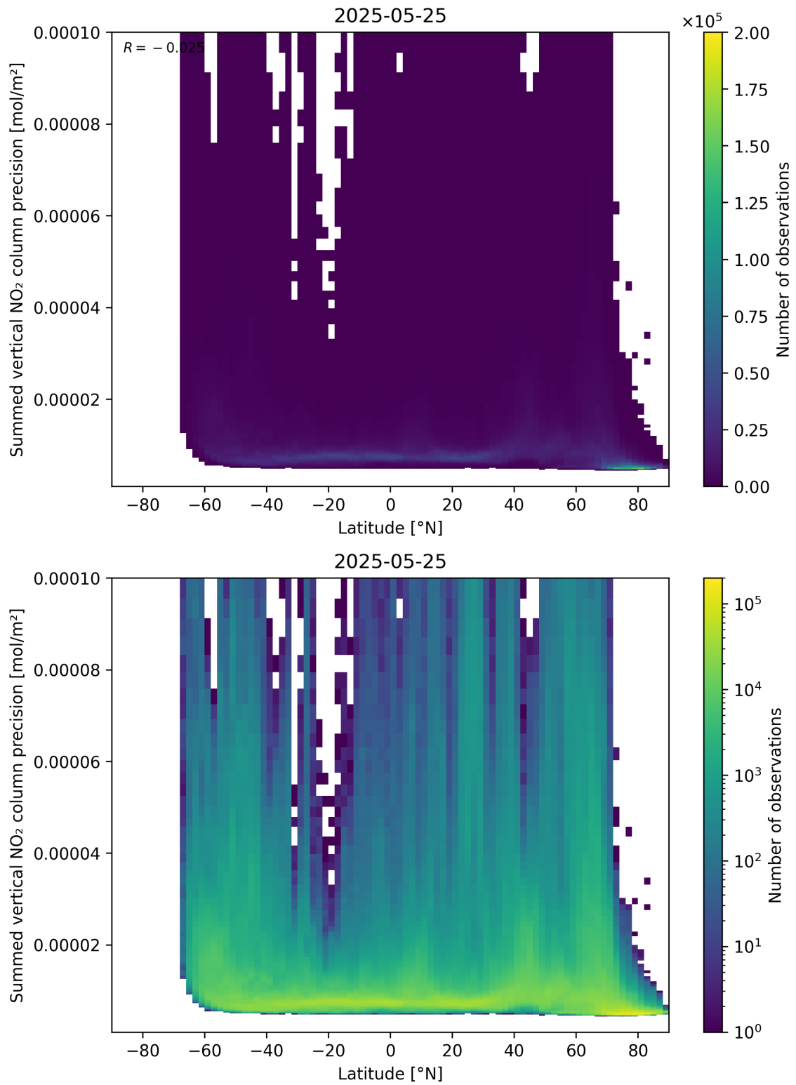
Figure 89: Scatter density plot of “Latitude” against “Summed vertical NO 2 column precision” for 2025-05-24 to 2025-05-26.
