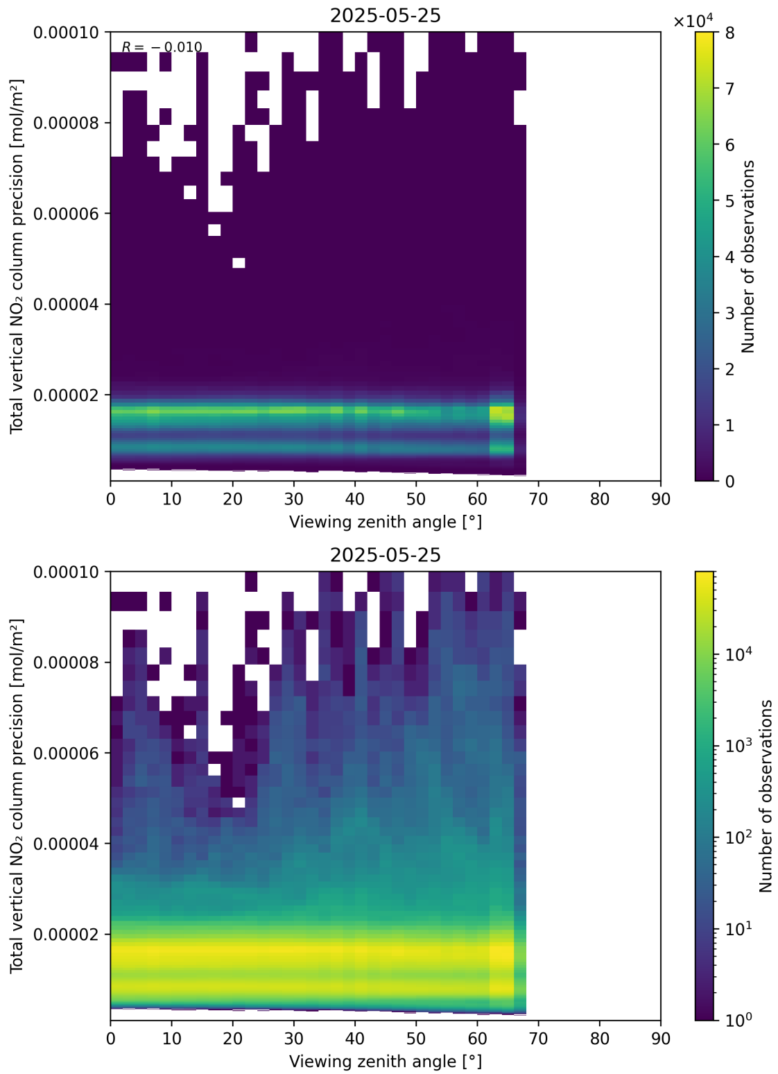
Figure 168: Scatter density plot of “Viewing zenith angle” against “Total vertical NO 2 column precision” for 2025-05-24 to 2025-05-26.
