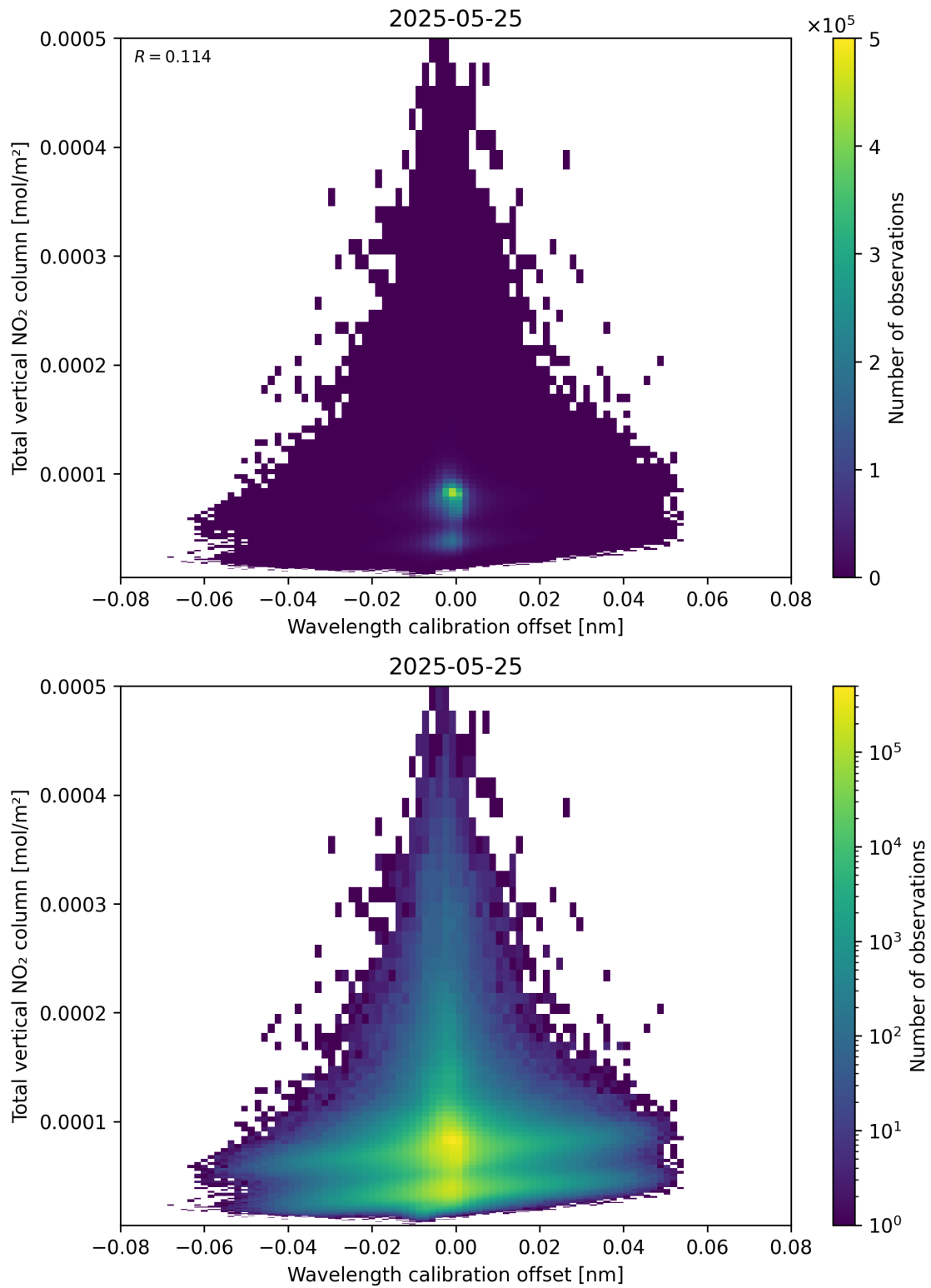
Figure 179: Scatter density plot of “Wavelength calibration offset” against “Total vertical NO 2 column” for 2025-05-24 to 2025-05-26.
