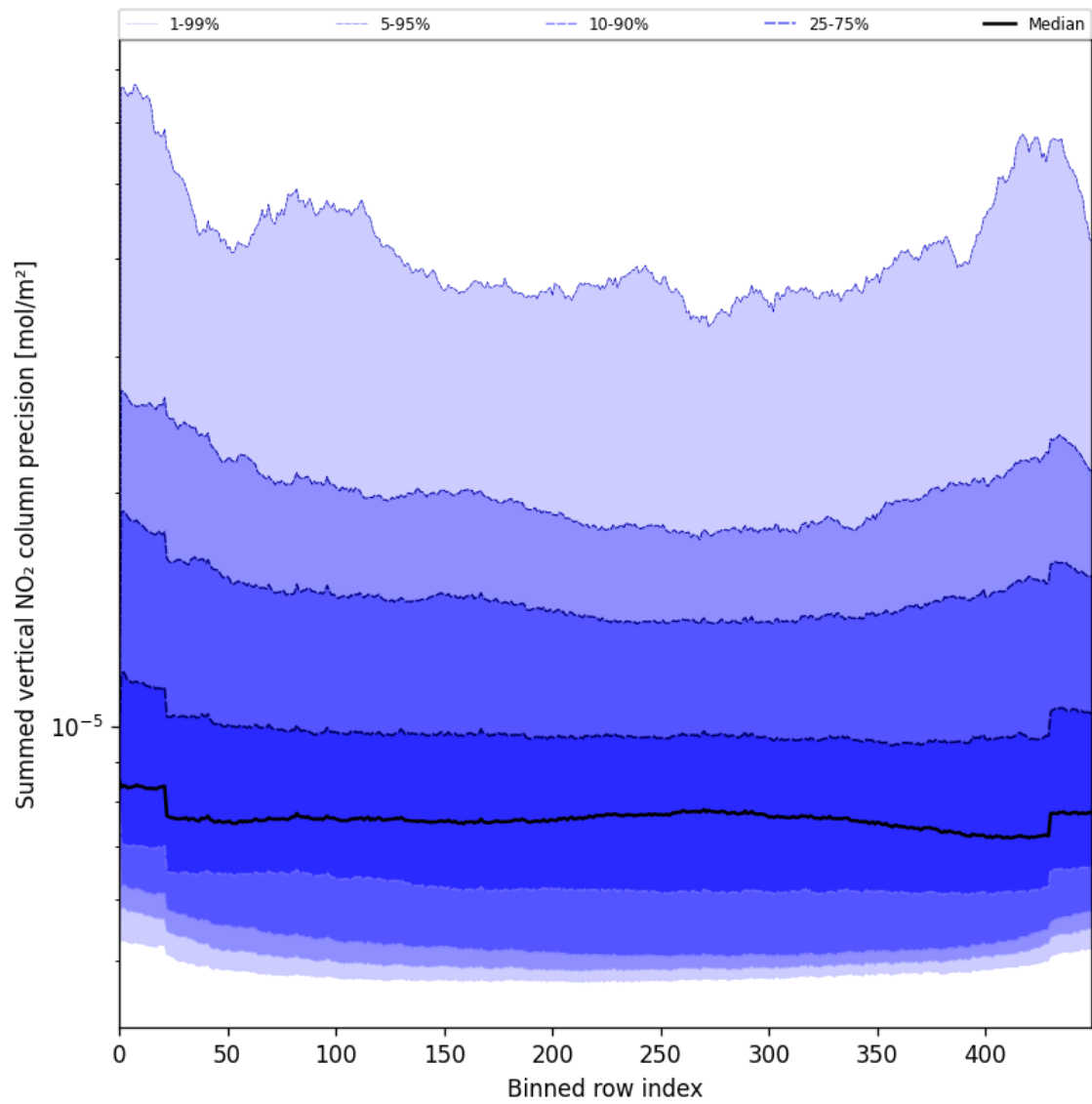
Figure 58: Along track statistics of “Summed vertical NO 2 column precision” for 2025-05-24 to 2025-05-26
