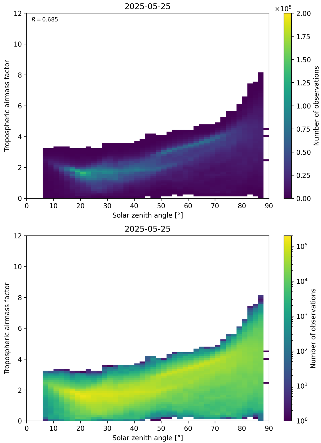
Figure 147: Scatter density plot of “Solar zenith angle” against “Tropospheric airmass factor” for 2025-05-24 to 2025-05-26.
