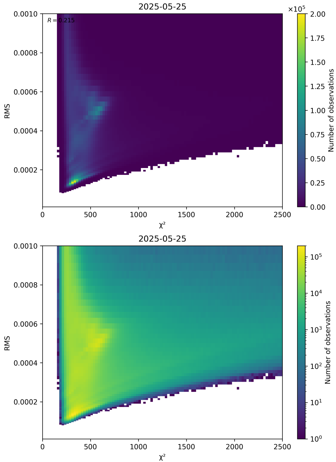
Figure 82: Scatter density plot of “ \chi^2 ” against “RMS” for 2025-05-24 to 2025-05-26.
