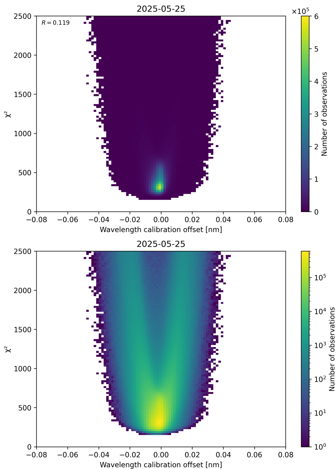
Figure 175: Scatter density plot of “Wavelength calibration offset” against “ \chi^2 ” for 2025-05-24 to 2025-05-26.
