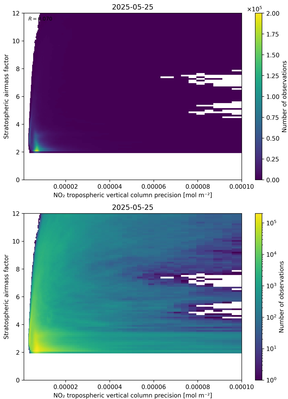
Figure 131: Scatter density plot of “NO 2 tropospheric vertical column precision” against “Stratospheric airmass factor” for 2025-05-24 to 2025-05-26.
