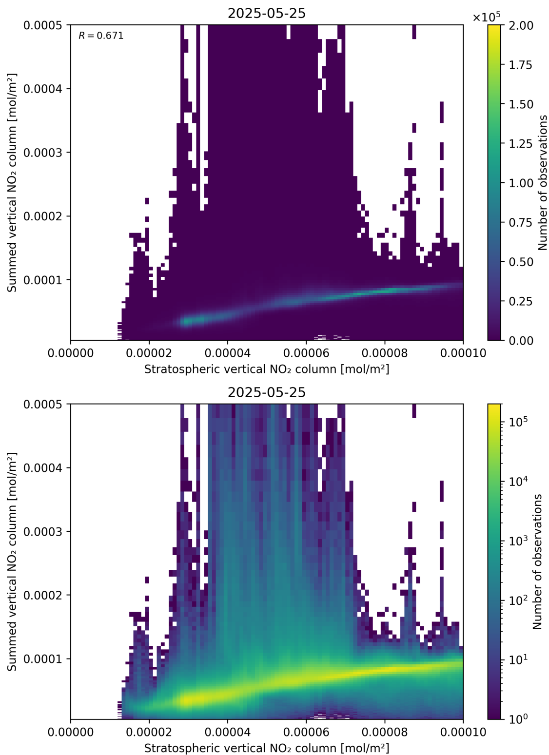
Figure 98: Scatter density plot of “Stratospheric vertical NO 2 column” against “Summed vertical NO 2 column” for 2025-05-24 to 2025-05-26.
