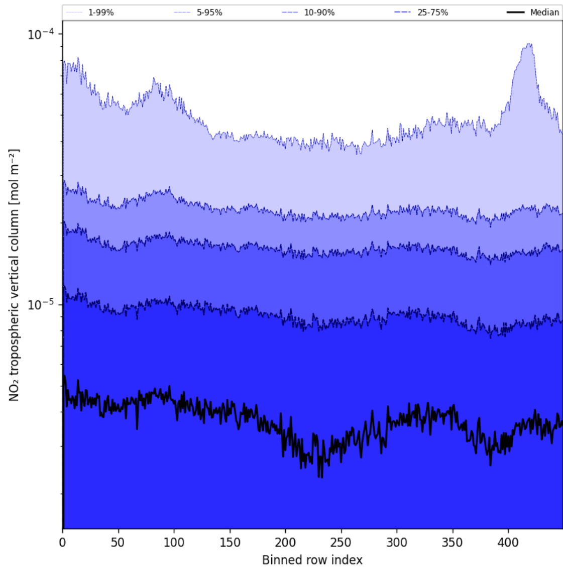
Figure 46: Along track statistics of “NO 2 tropospheric vertical column” for 2025-05-24 to 2025-05-26
