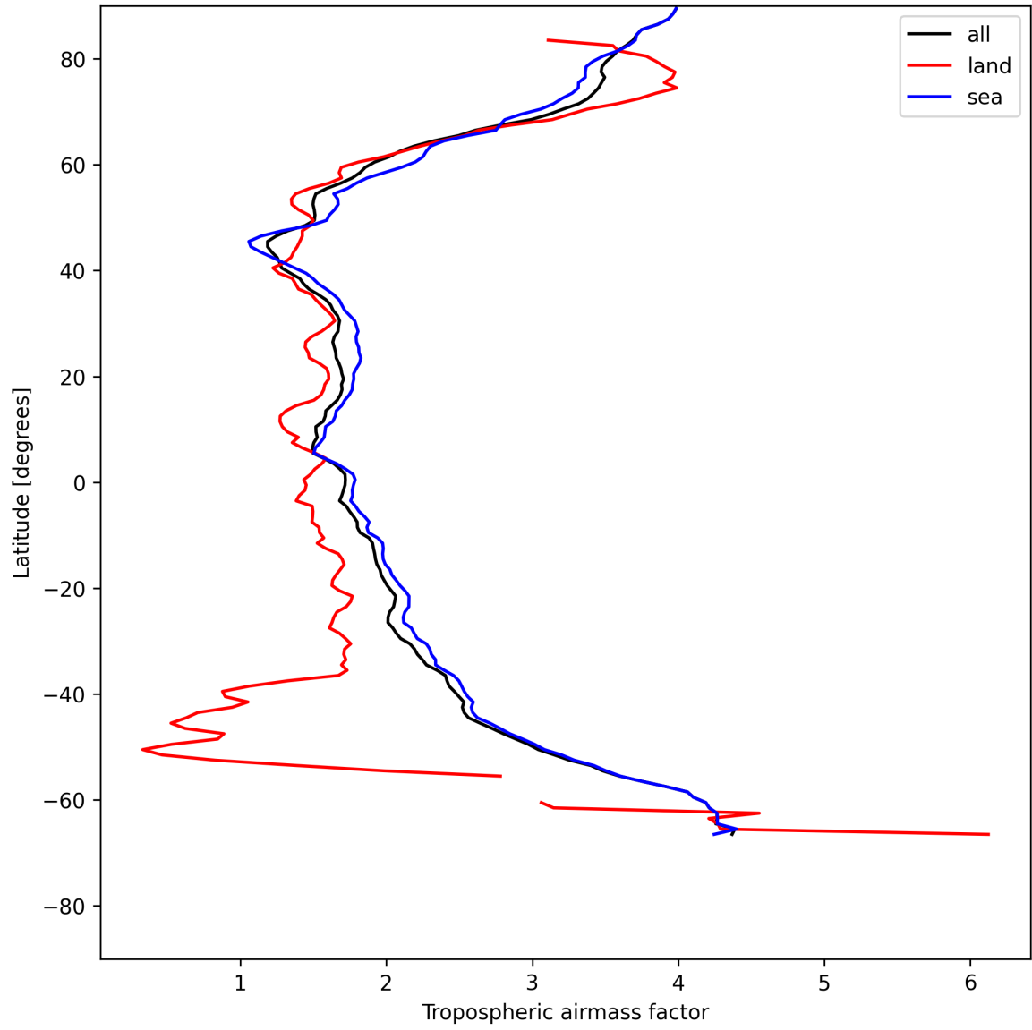
Figure 14: Zonal average of “Tropospheric airmass factor” for 2025-05-24 to 2025-05-26.
