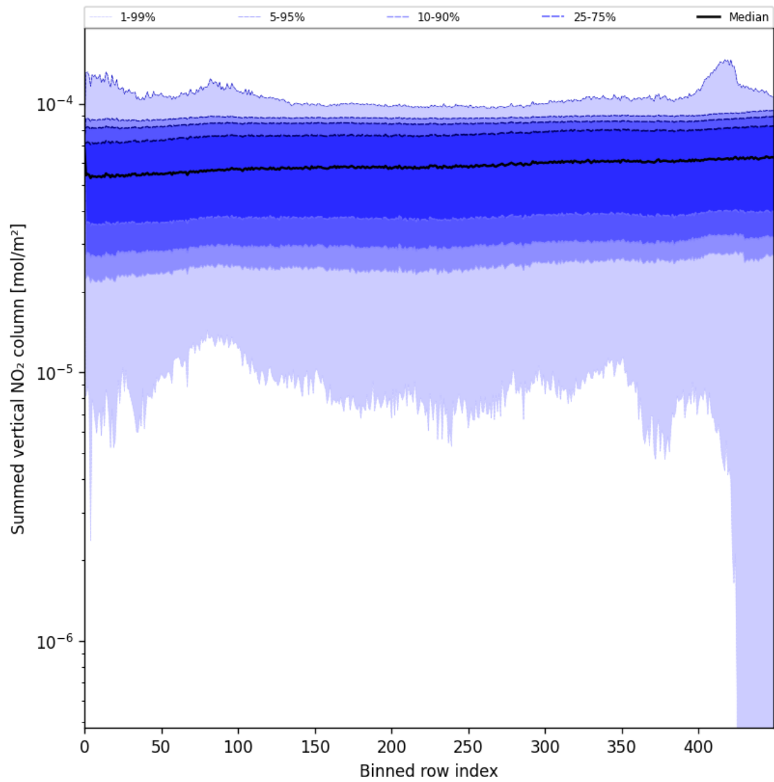
Figure 57: Along track statistics of “Summed vertical NO 2 column” for 2025-05-24 to 2025-05-26
