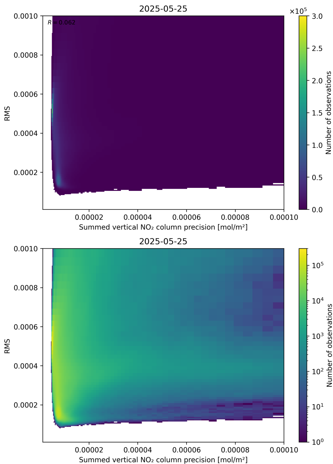
Figure 108: Scatter density plot of “Summed vertical NO 2 column precision” against “RMS” for 2025-05-24 to 2025-05-26.
