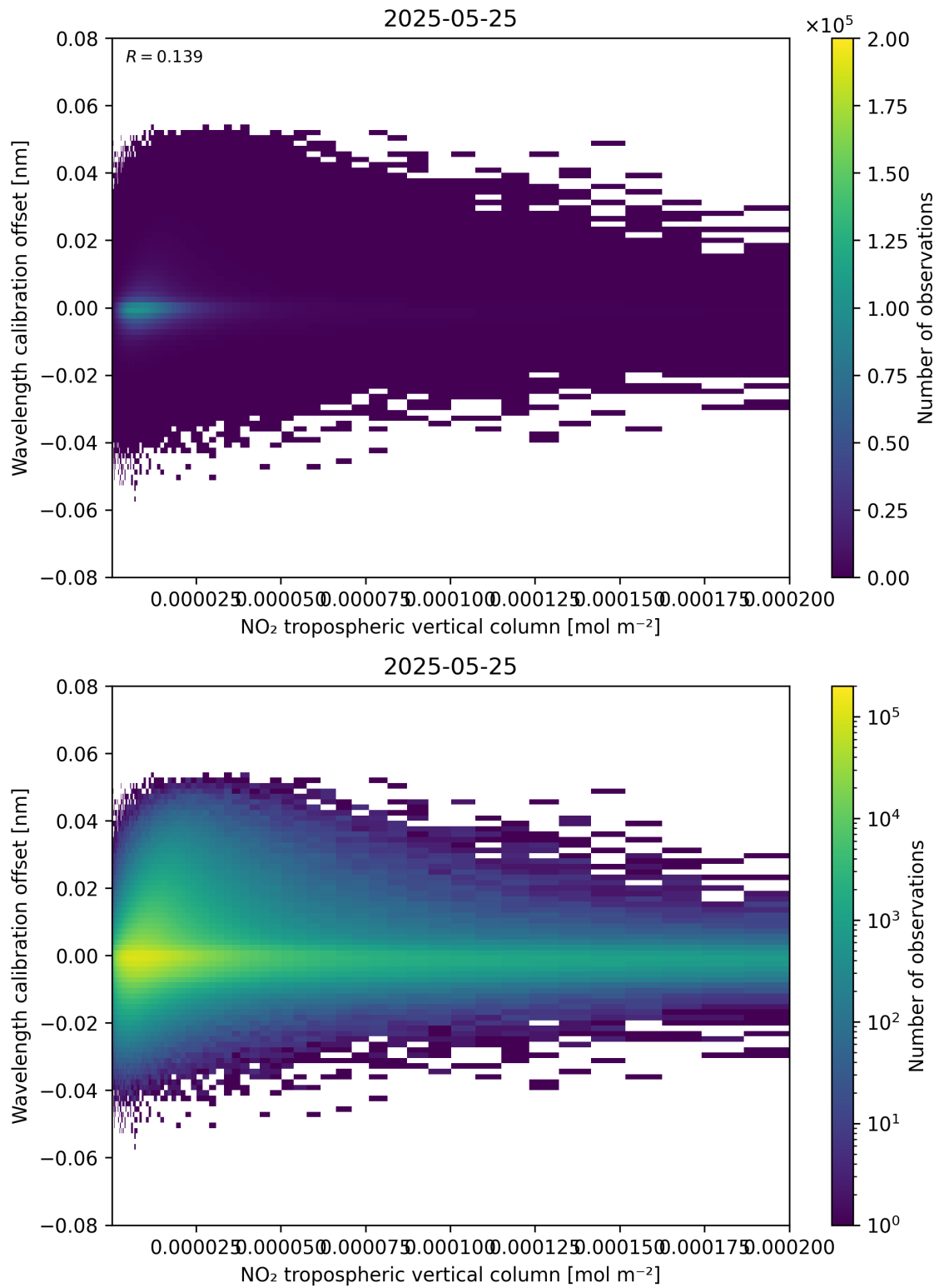
Figure 143: Scatter density plot of “NO 2 tropospheric vertical column” against “Wavelength calibration offset” for 2025-05-24 to 2025-05-26.
