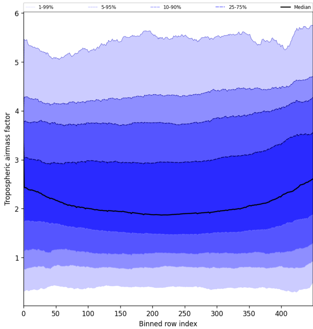
Figure 48: Along track statistics of “Tropospheric airmass factor” for 2025-05-24 to 2025-05-26
