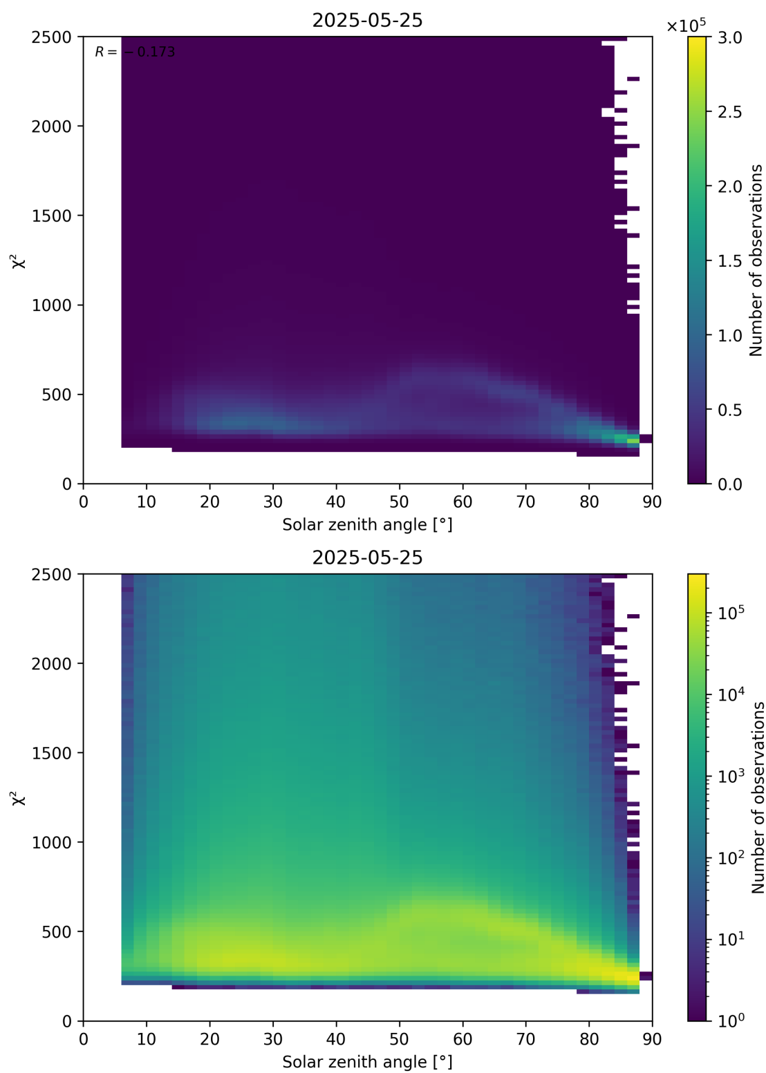
Figure 148: Scatter density plot of “Solar zenith angle” against “ \chi^2 ” for 2025-05-24 to 2025-05-26.
