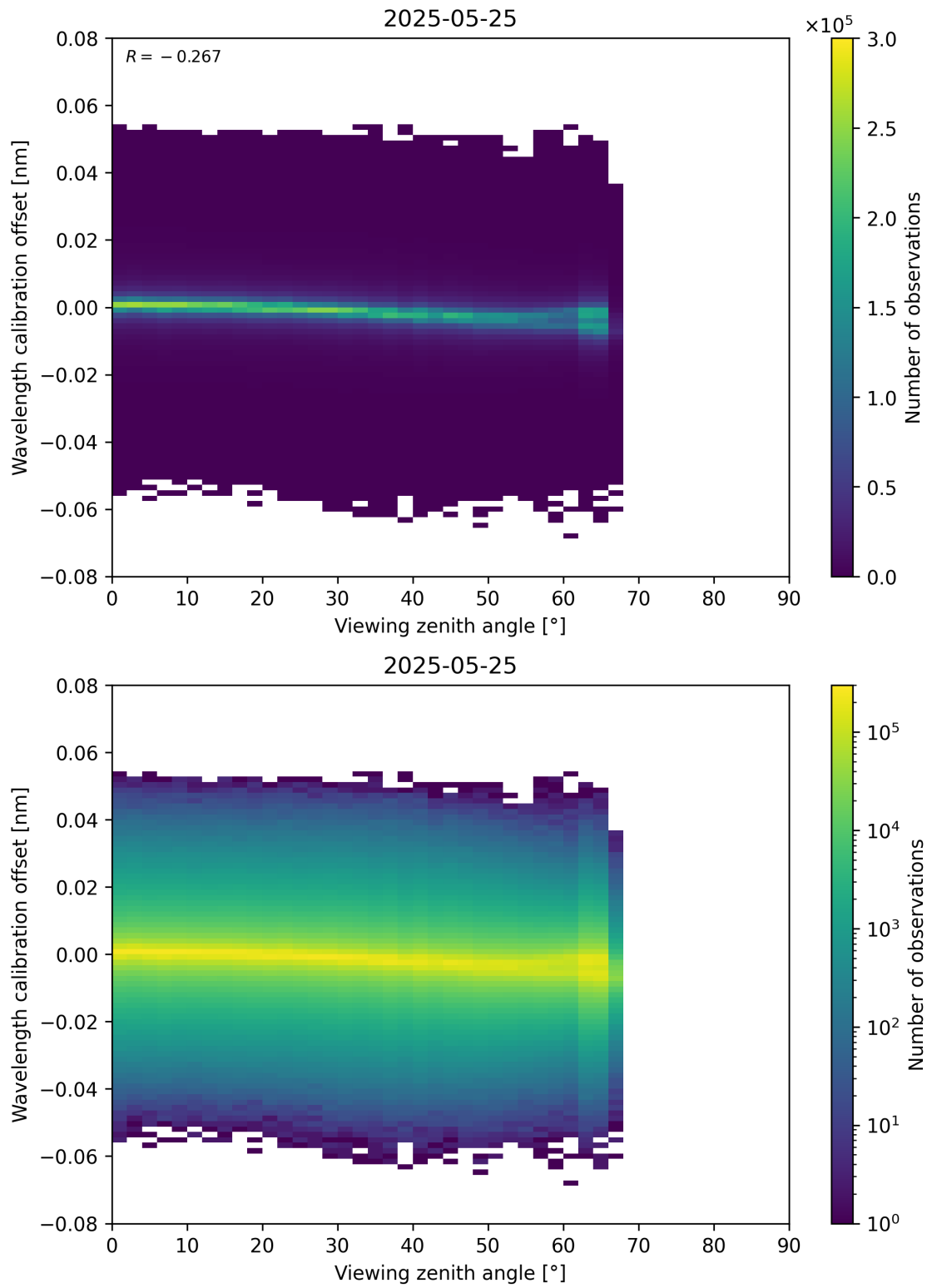
Figure 173: Scatter density plot of “Viewing zenith angle” against “Wavelength calibration offset” for 2025-05-24 to 2025-05-26.
