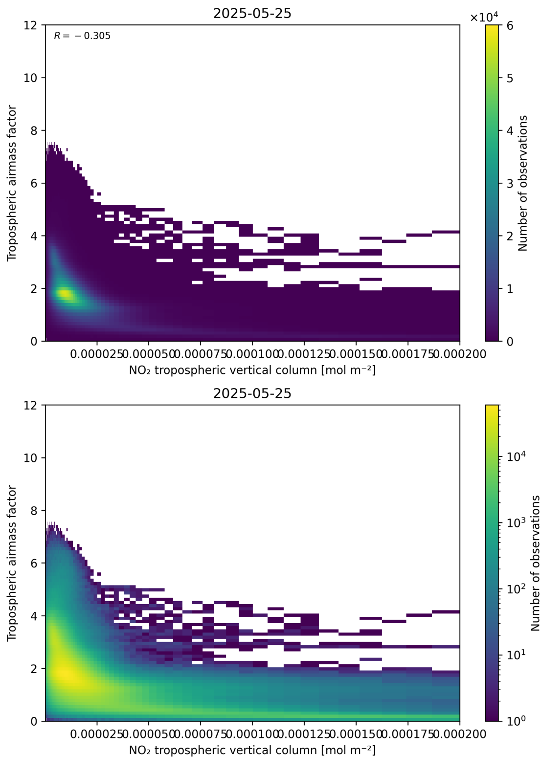
Figure 123: Scatter density plot of “NO 2 tropospheric vertical column” against “Tropospheric air mass factor” for 2025-05-24 to 2025-05-26.
