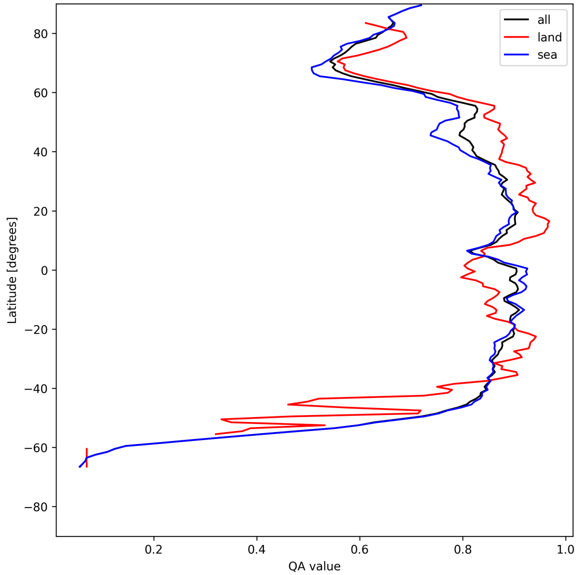
Figure 11: Zonal average of “QA value” for 2025-05-24 to 2025-05-26.
