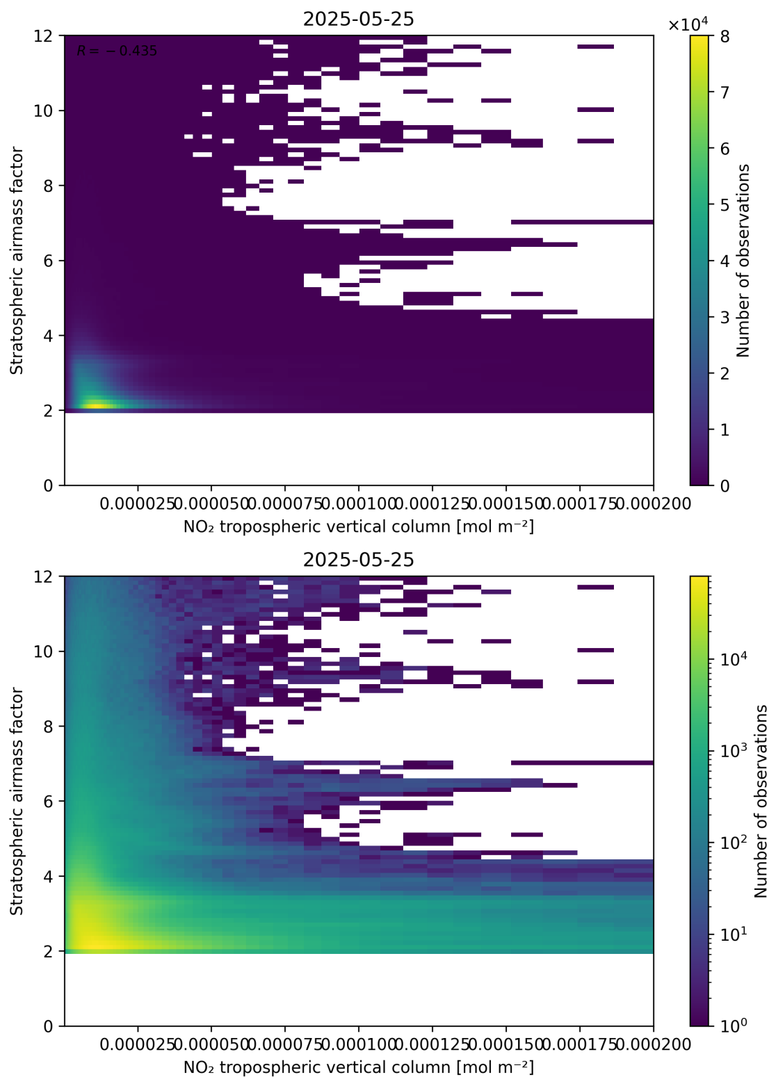
Figure 121: Scatter density plot of “NO 2 tropospheric vertical column” against “Stratospheric air mass factor” for 2025-05-24 to 2025-05-26.
