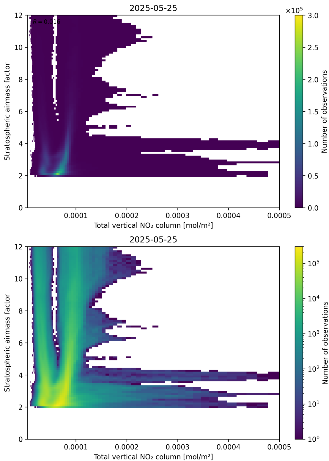
Figure 110: Scatter density plot of “Total vertical NO 2 column” against “Stratospheric airmass factor” for 2025-05-24 to 2025-05-26.
