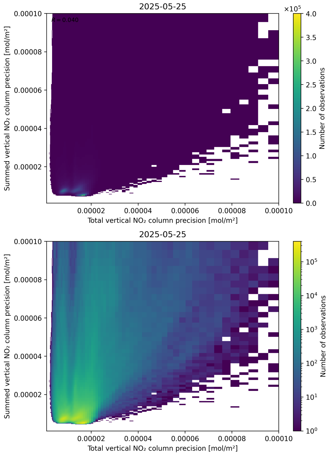
Figure 118: Scatter density plot of “Total vertical NO 2 column precision” against “Summed vertical NO 2 column precision” for 2025-05-24 to 2025-05-26.
