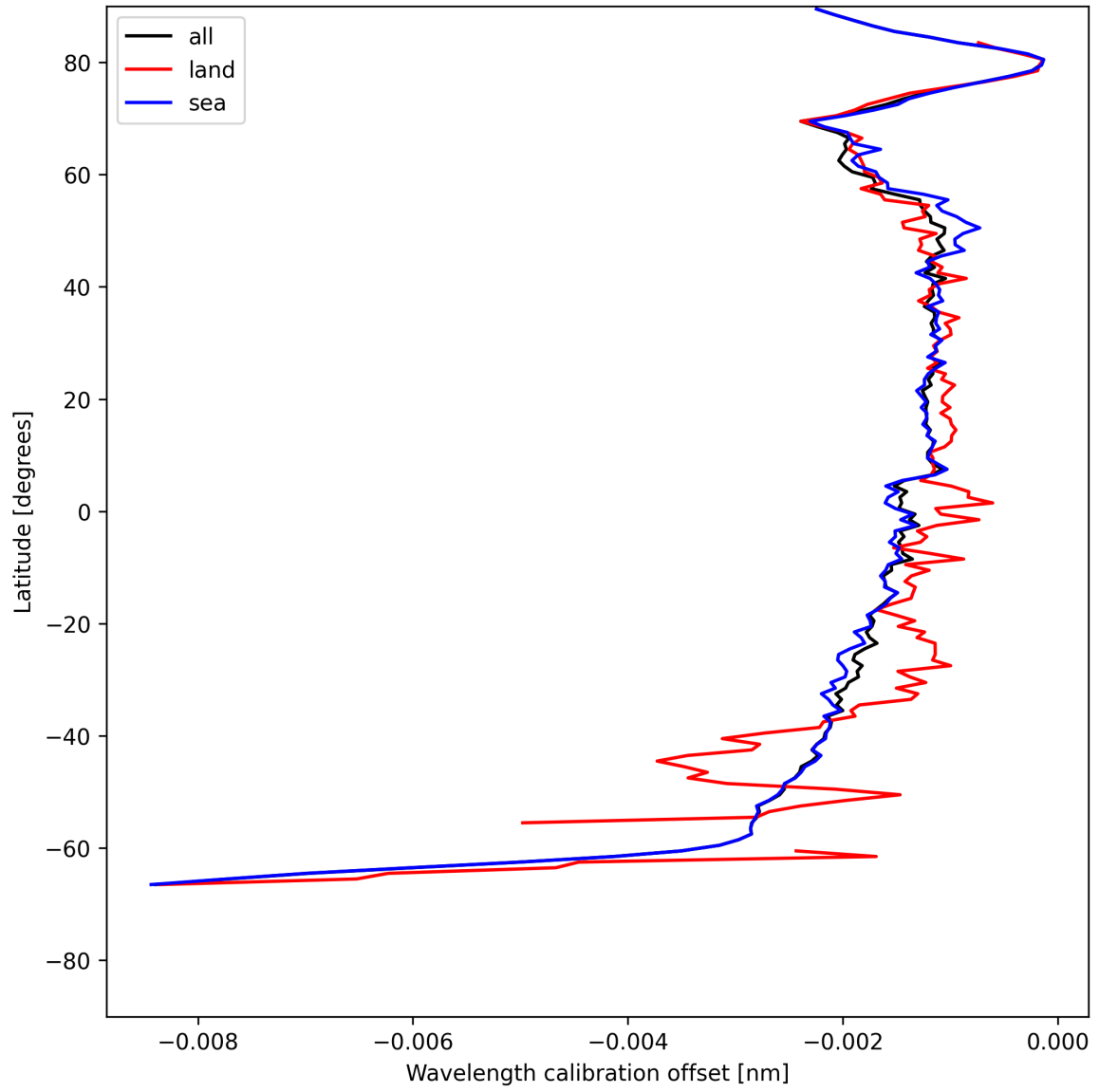
Figure 18: Zonal average of “Wavelength calibration offset” for 2025-05-24 to 2025-05-26.
