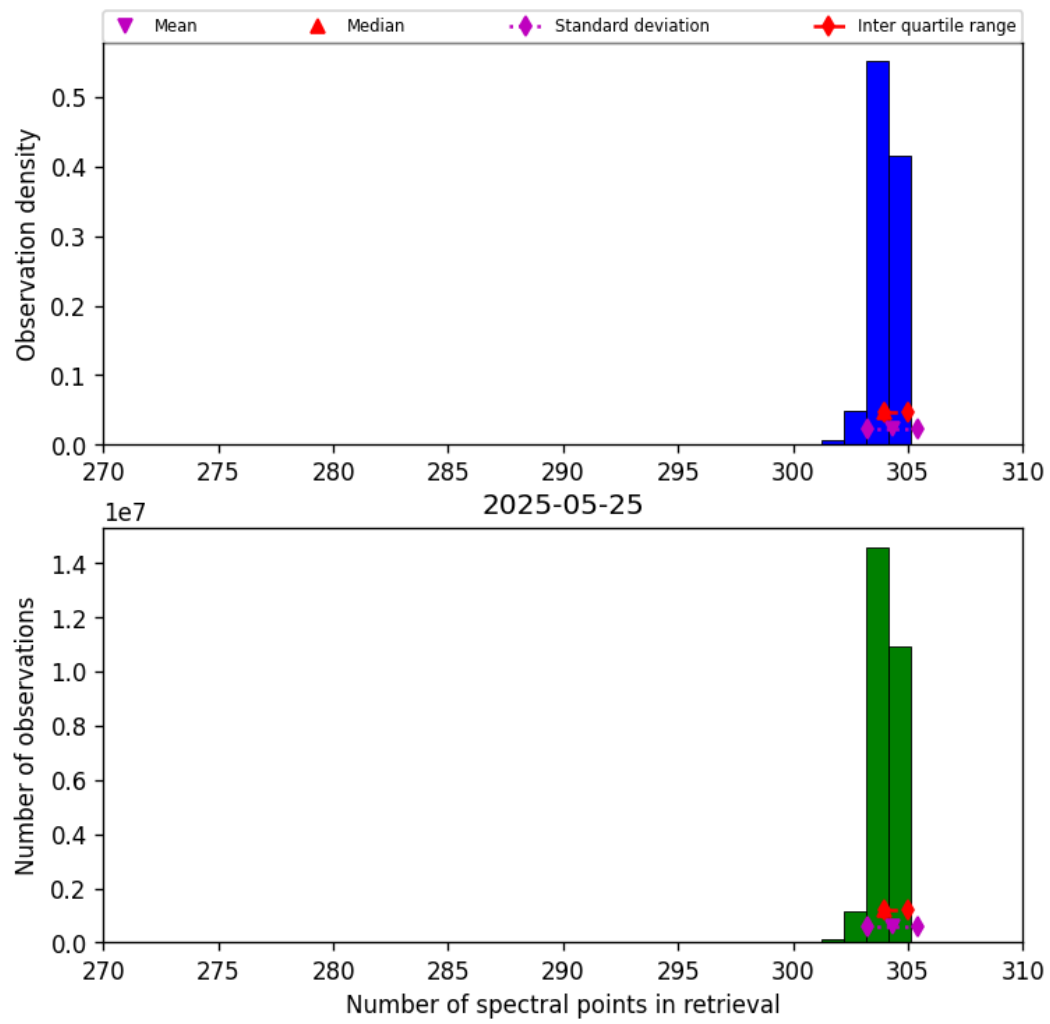
Figure 33: Histogram of “Number of spectral points in retrieval” for 2025-05-24 to 2025-05-26
