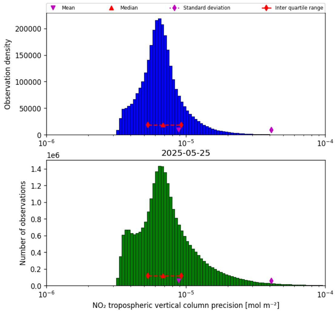
Figure 30: Histogram of “NO 2 tropospheric vertical column precision” for 2025-05-24 to 2025-05-26
