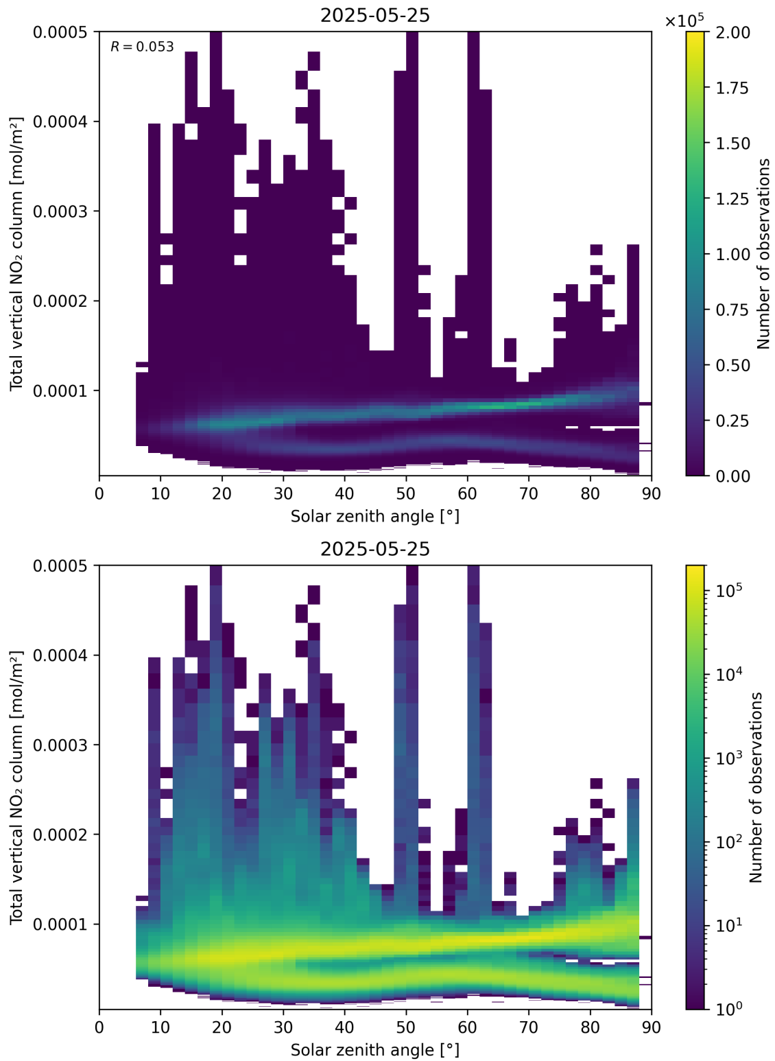
Figure 153: Scatter density plot of “Solar zenith angle” against “Total vertical NO 2 column” for 2025-05-24 to 2025-05-26.
