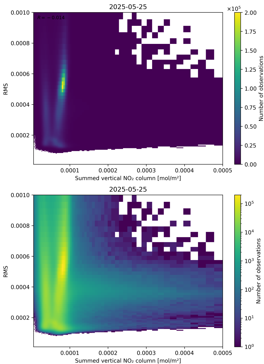
Figure 109: Scatter density plot of “Summed vertical NO 2 column” against “RMS” for 2025-05-24 to 2025-05-26.
