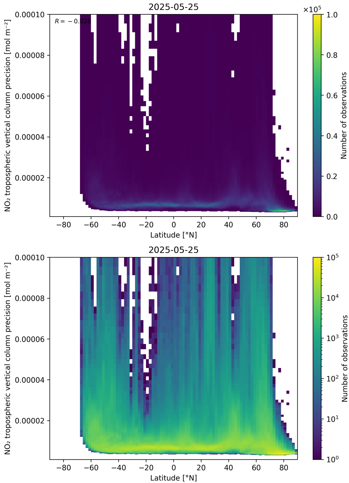
Figure 93: Scatter density plot of “Latitude” against “NO 2 tropospheric vertical column precision” for 2025-05-24 to 2025-05-26.
