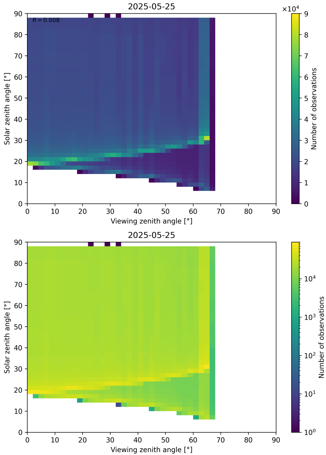
Figure 172: Scatter density plot of “Viewing zenith angle” against “Solar zenith angle” for 2025-05-24 to 2025-05-26.
