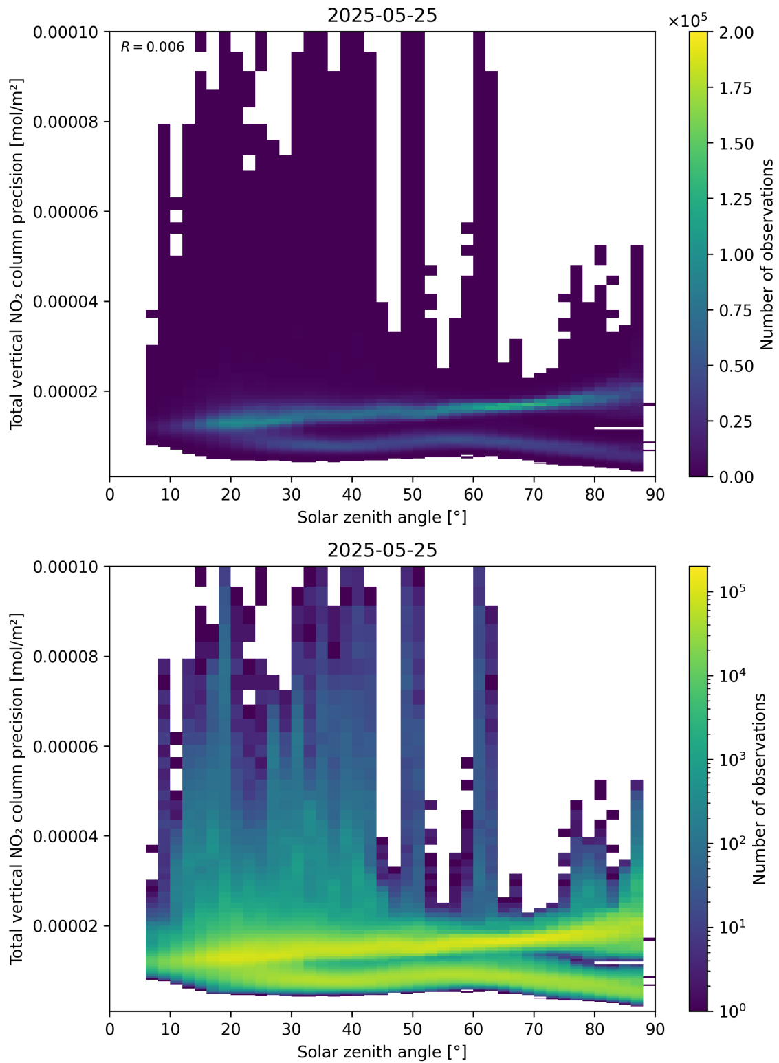
Figure 154: Scatter density plot of “Solar zenith angle” against “Total vertical NO 2 column precision” for 2025-05-24 to 2025-05-26.
