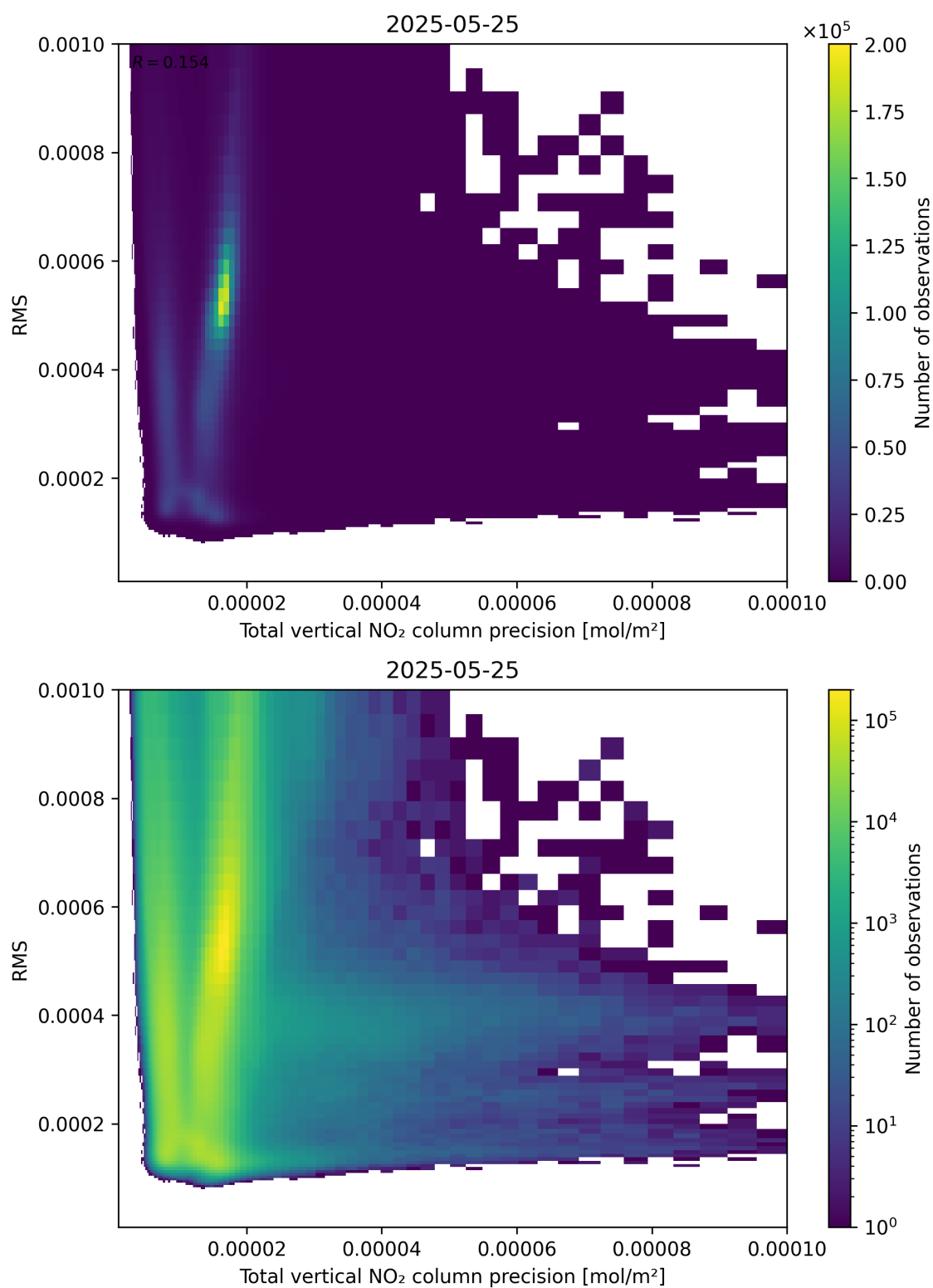
Figure 119: Scatter density plot of “Total vertical NO 2 column precision” against “RMS” for 2025-05-24 to 2025-05-26.
