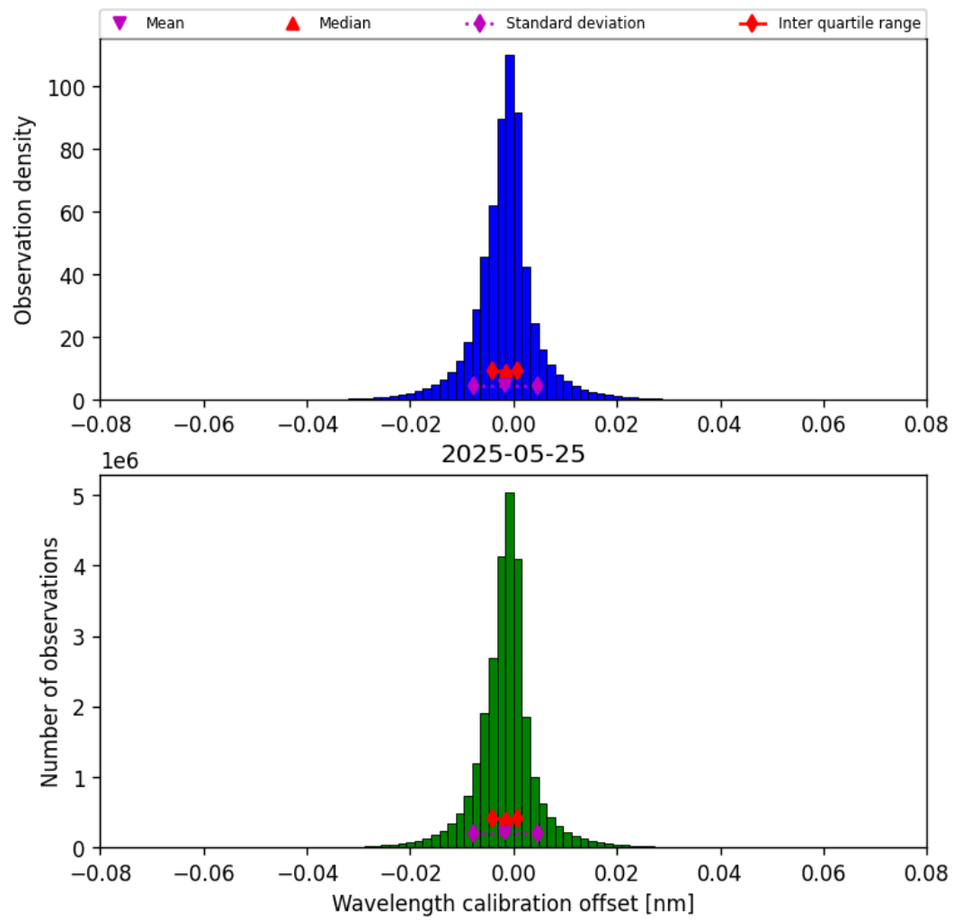
Figure 35: Histogram of “Wavelength calibration offset” for 2025-05-24 to 2025-05-26
