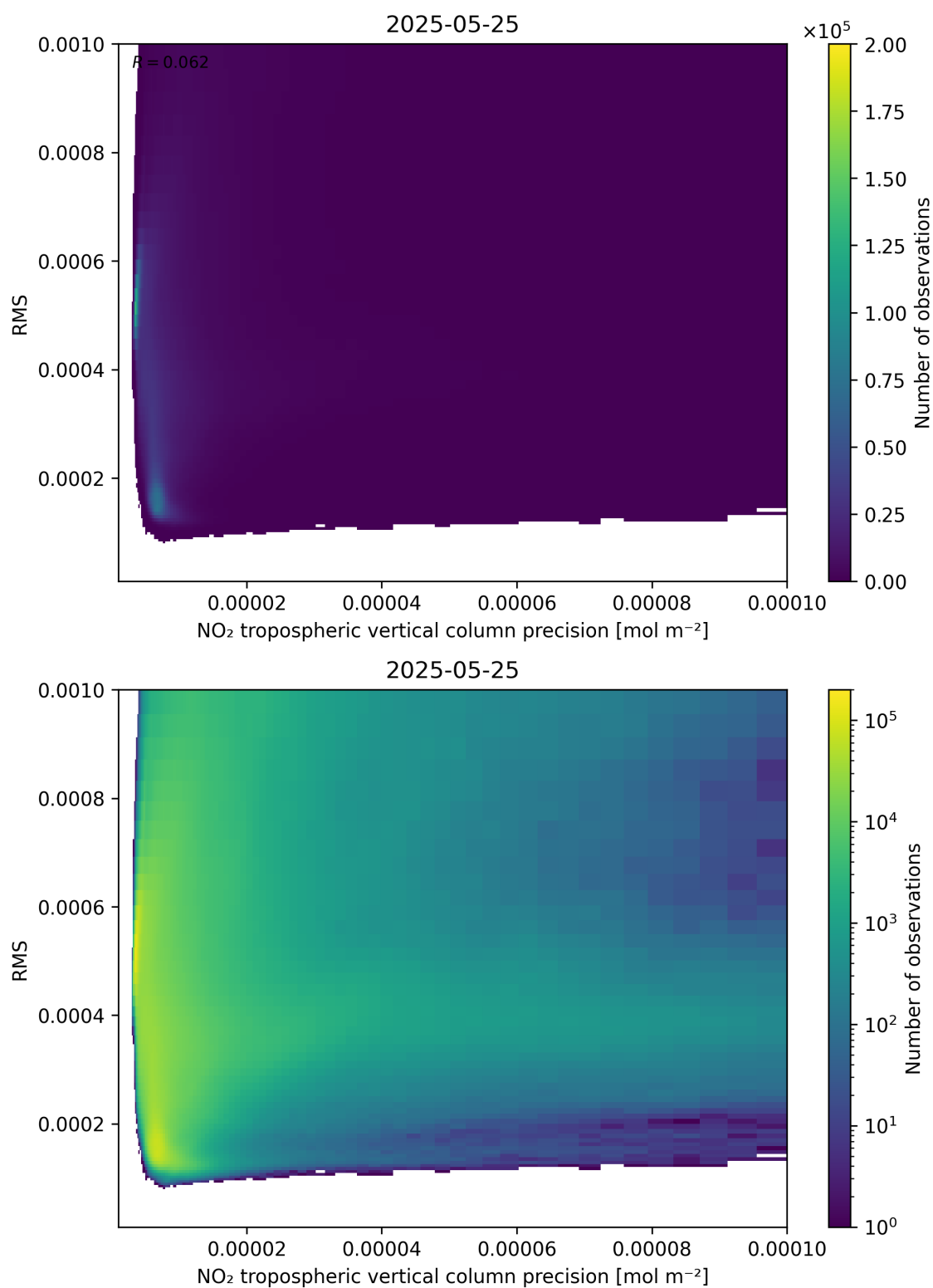
Figure 140: Scatter density plot of “NO 2 tropospheric vertical column precision” against “RMS” for 2025-05-24 to 2025-05-26.
