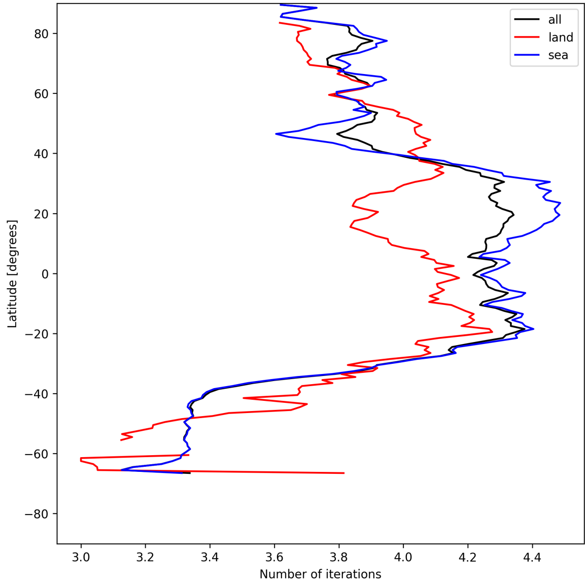
Figure 17: Zonal average of “Number of iterations” for 2025-05-24 to 2025-05-26.
