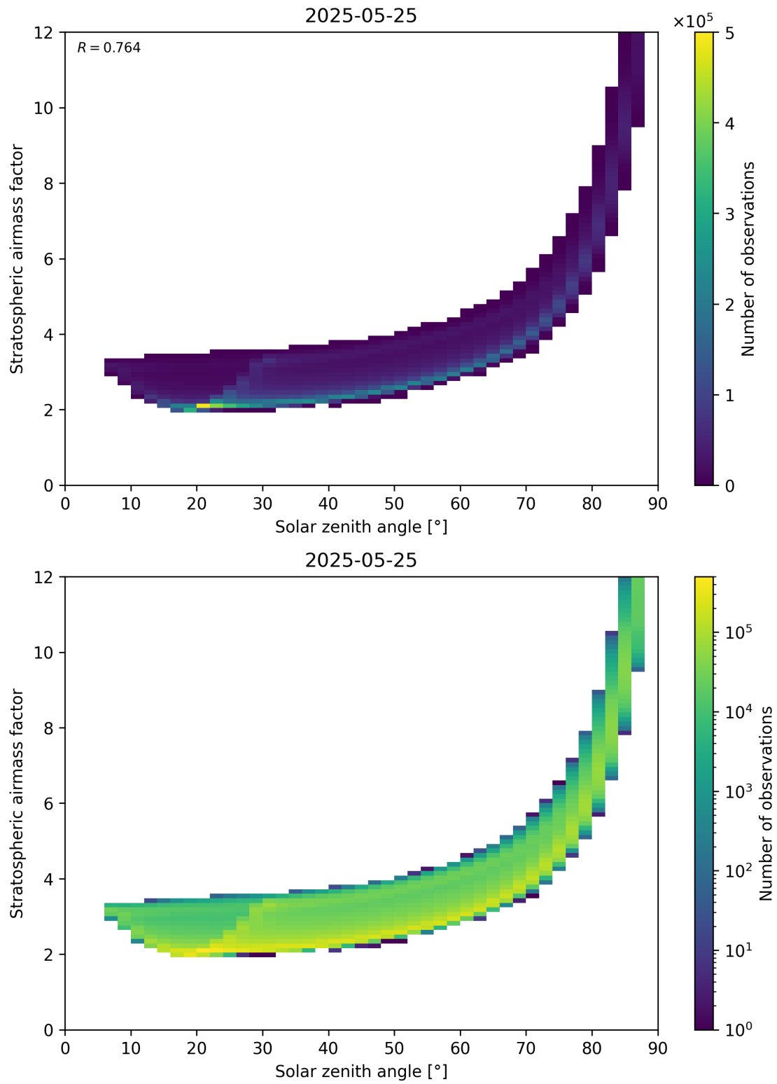
Figure 145: Scatter density plot of “Solar zenith angle” against “Stratospheric airmass factor” for 2025-05-24 to 2025-05-26.
