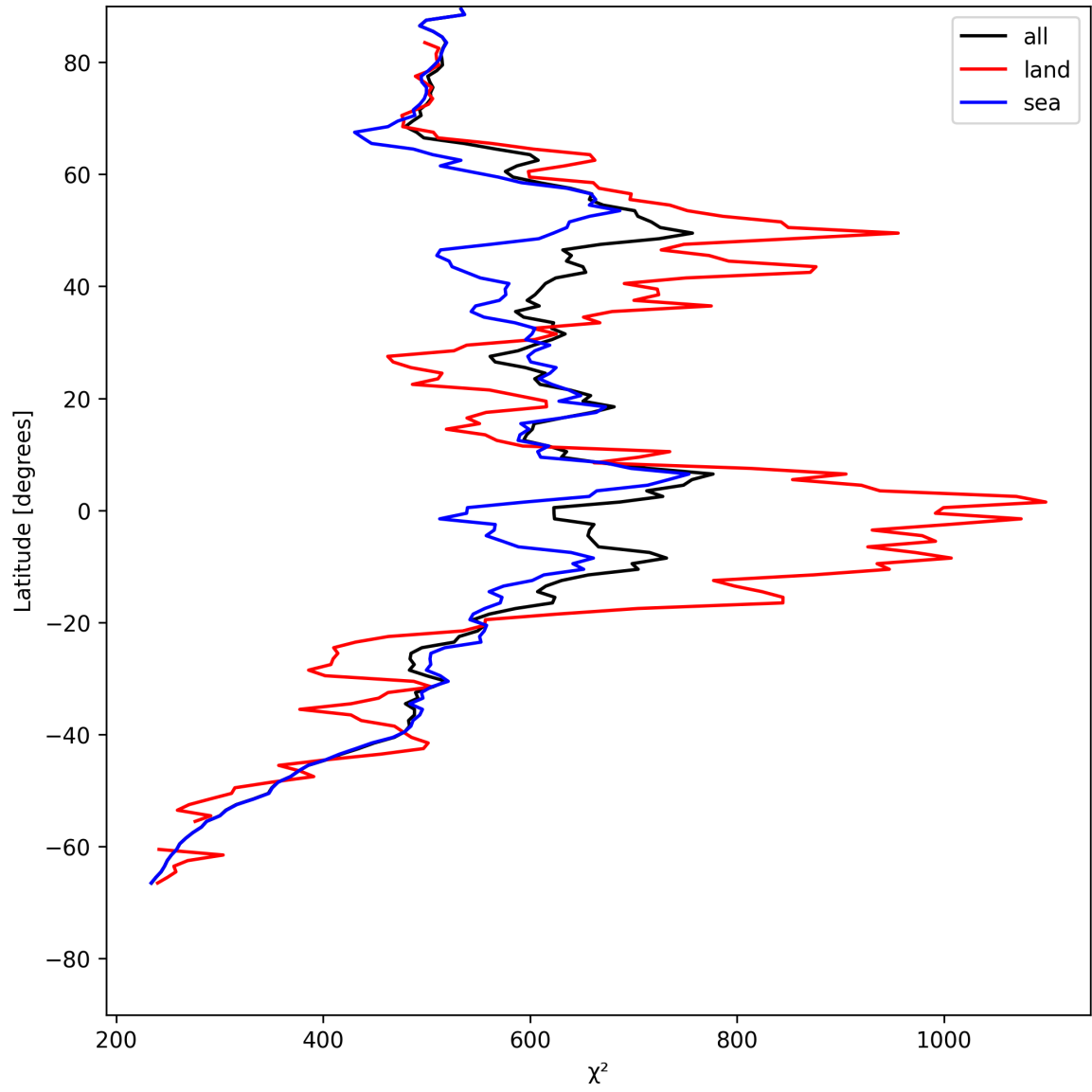
Figure 25: Zonal average of “ \chi^2 ” for 2025-05-24 to 2025-05-26.
