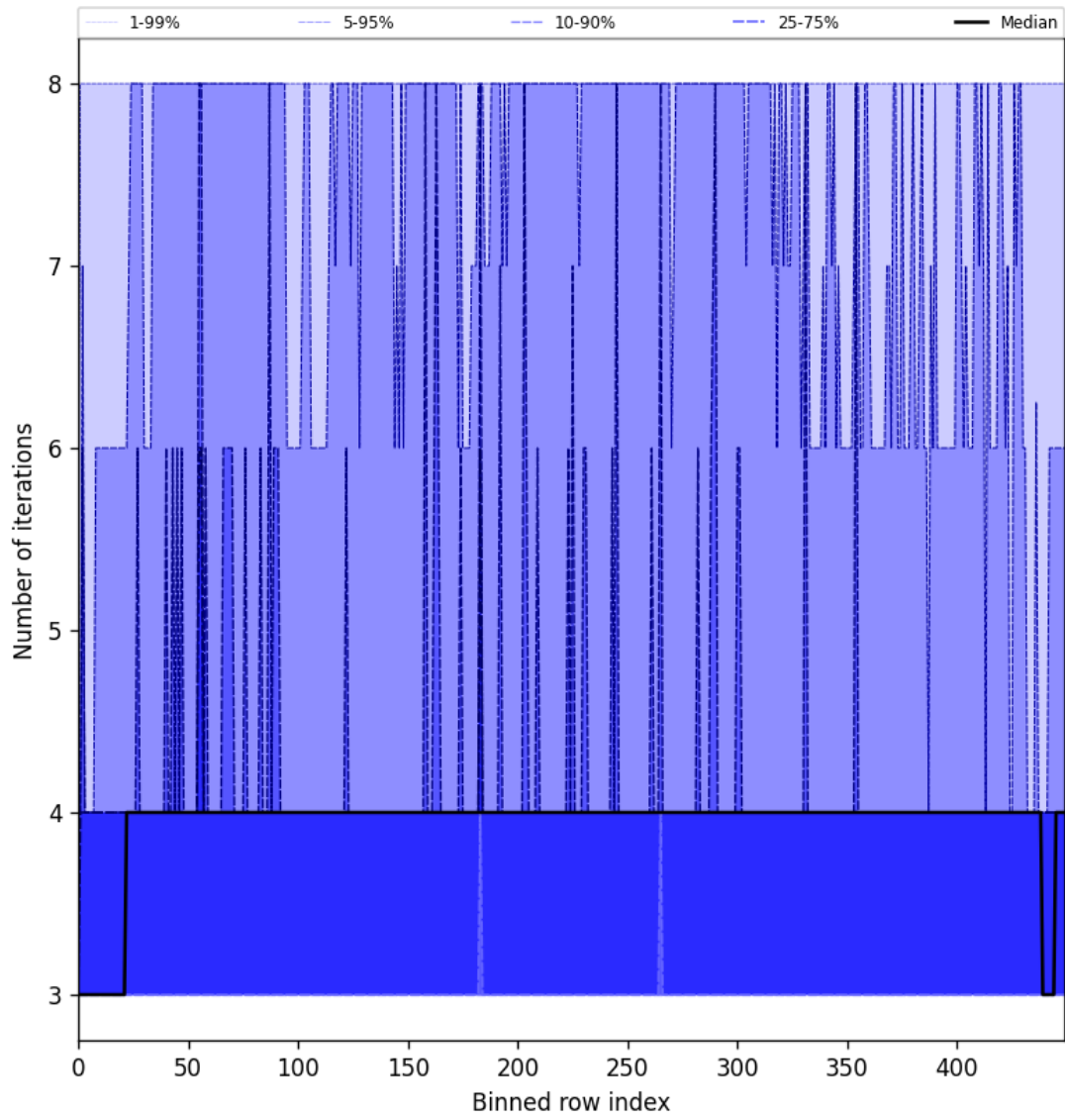
Figure 51: Along track statistics of “Number of iterations” for 2025-05-24 to 2025-05-26
