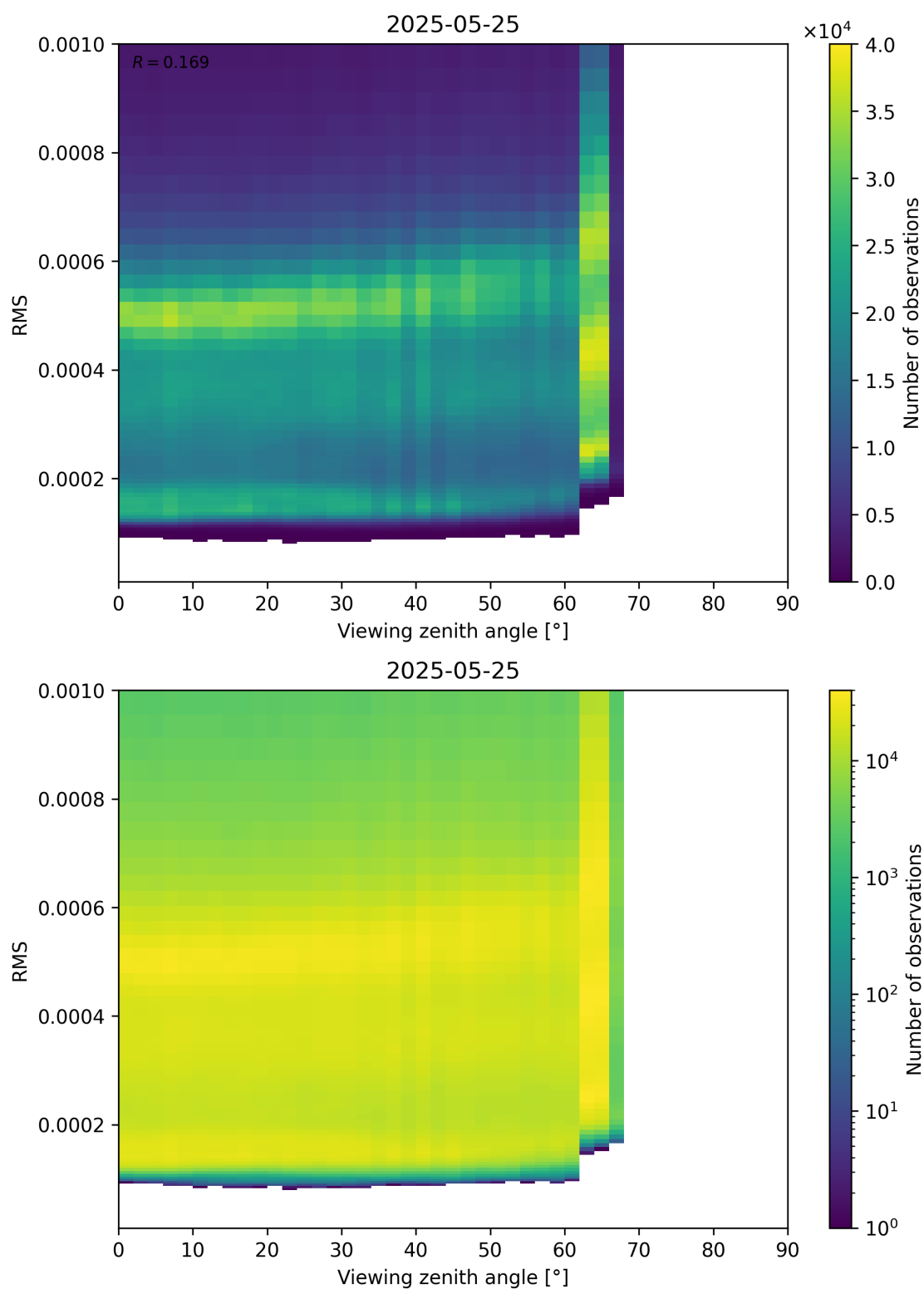
Figure 171: Scatter density plot of “Viewing zenith angle” against “RMS” for 2025-05-24 to 2025-05-26.
