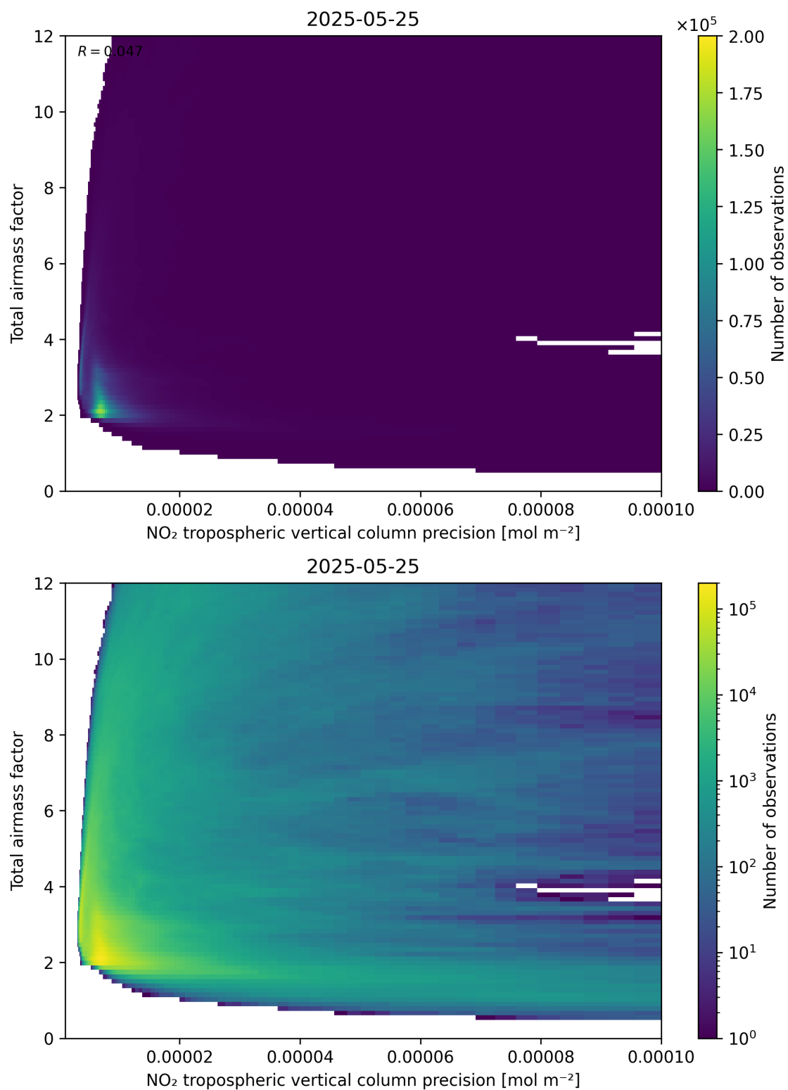
Figure 132: Scatter density plot of “NO 2 tropospheric vertical column precision” against “Total air mass factor” for 2025-05-24 to 2025-05-26.
