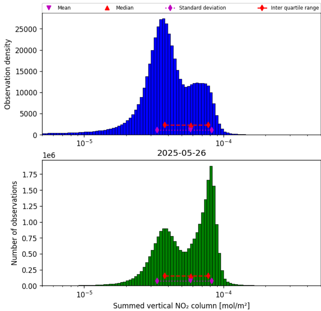
Figure 40: Histogram of “Summed vertical NO 2 column” for 2025-05-26 to 2025-05-27
