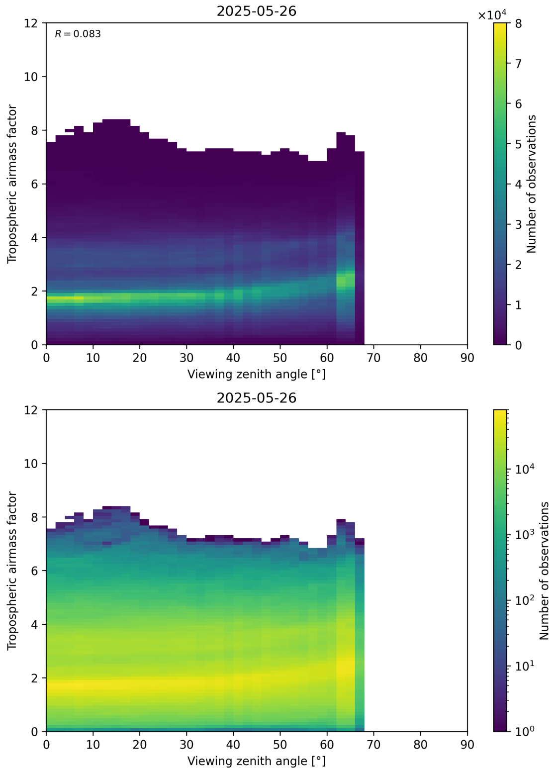
Figure 161: Scatter density plot of “Viewing zenith angle” against “Tropospheric airmass factor” for 2025-05-26 to 2025-05-27.
