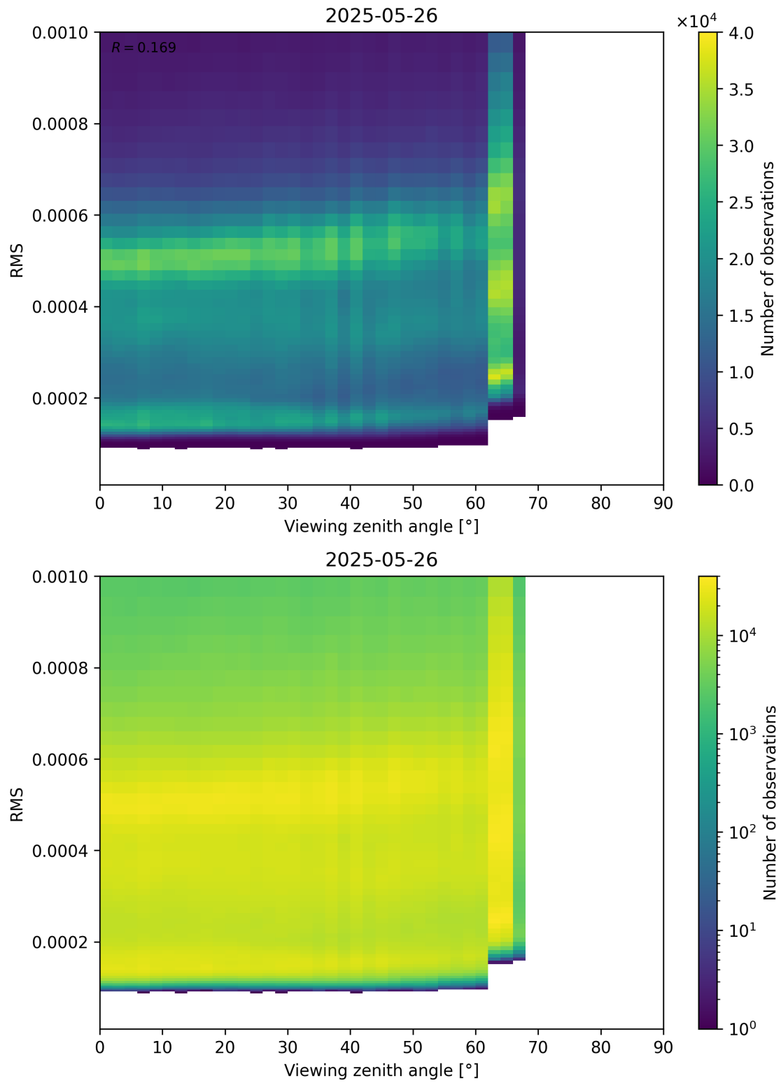
Figure 171: Scatter density plot of “Viewing zenith angle” against “RMS” for 2025-05-26 to 2025-05-27.
