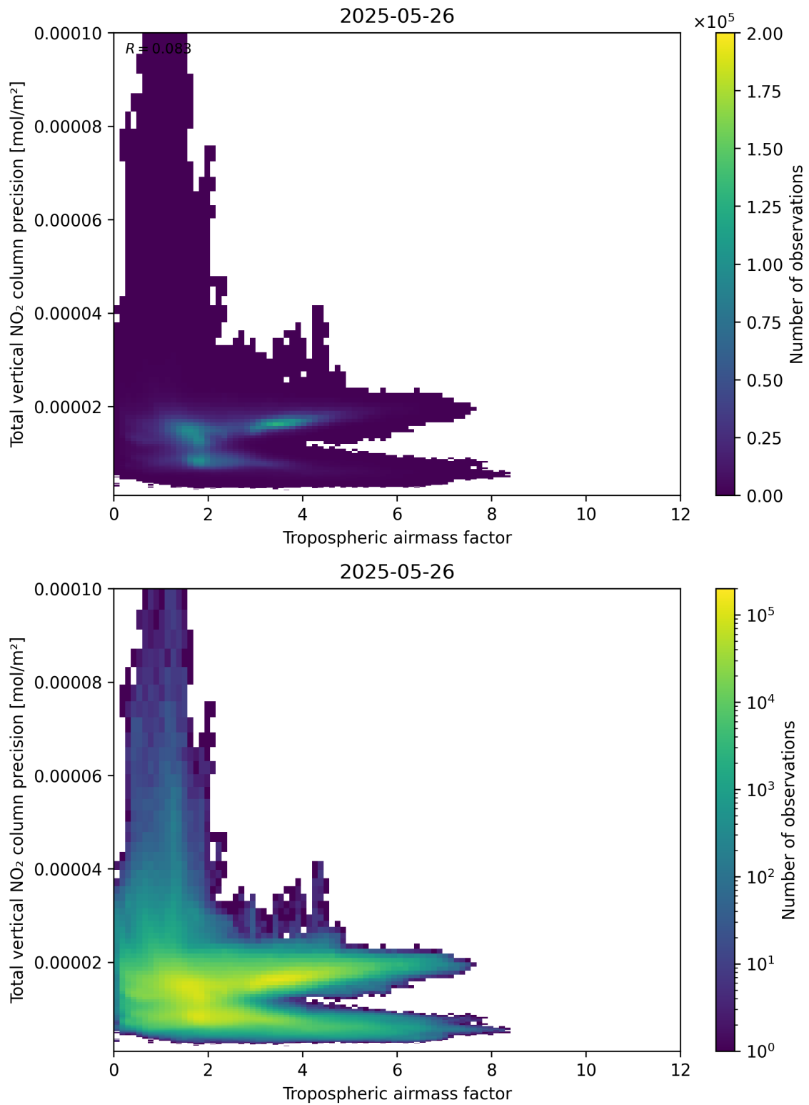
Figure 78: Scatter density plot of “Tropospheric airmass factor” against “Total vertical NO 2 column precision” for 2025-05-26 to 2025-05-27.
