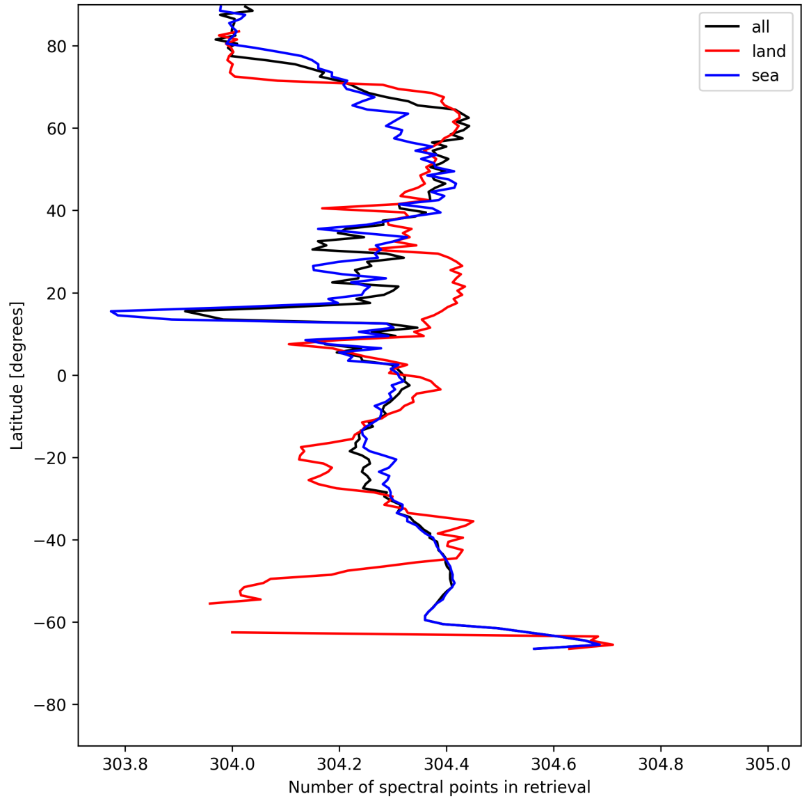
Figure 16: Zonal average of “Number of spectral points in retrieval” for 2025-05-26 to 2025-05-27.
