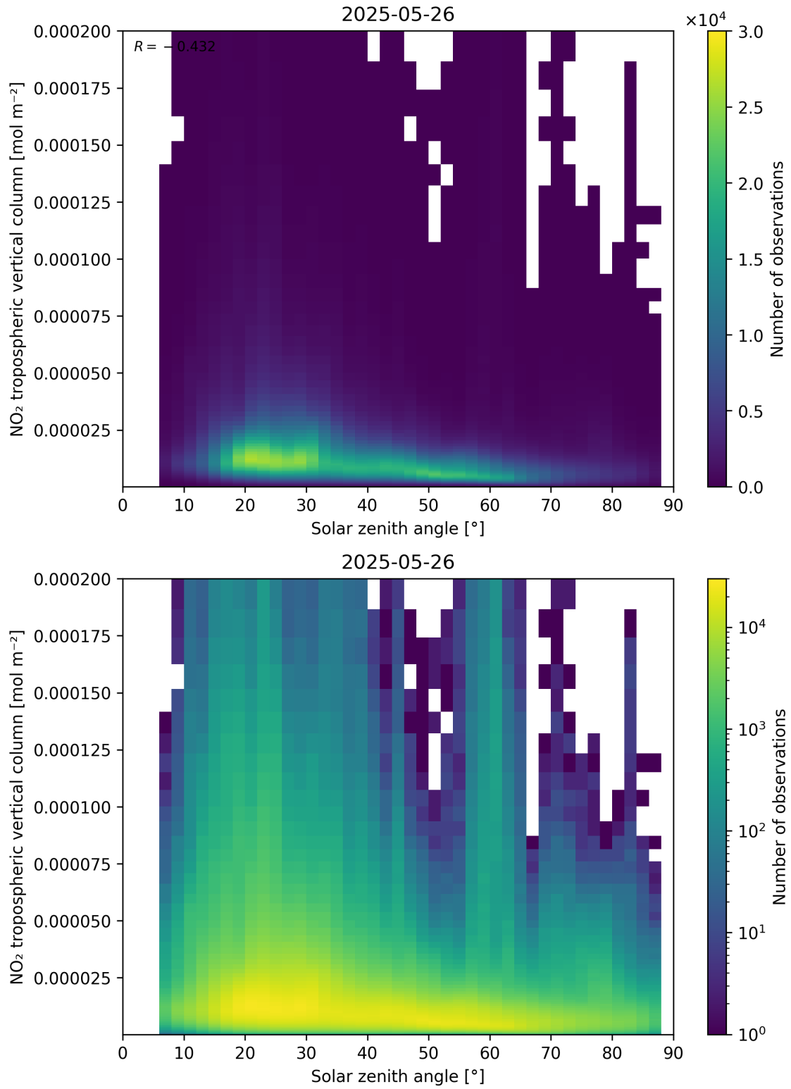
Figure 155: Scatter density plot of “Solar zenith angle” against “NO 2 tropospheric vertical column” for 2025-05-26 to 2025-05-27.
