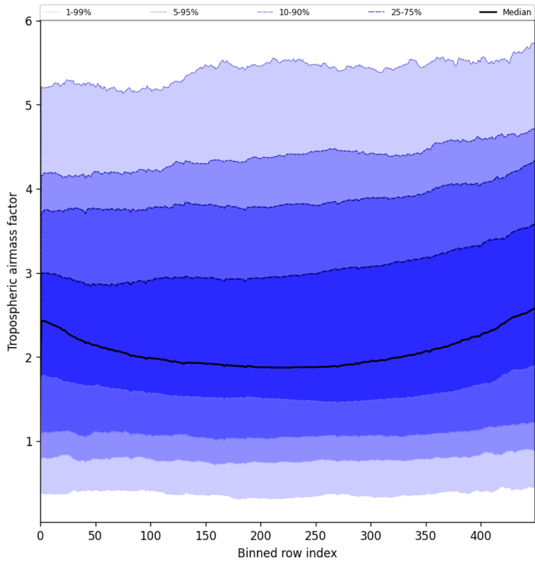
Figure 48: Along track statistics of “Tropospheric airmass factor” for 2025-05-26 to 2025-05-27
