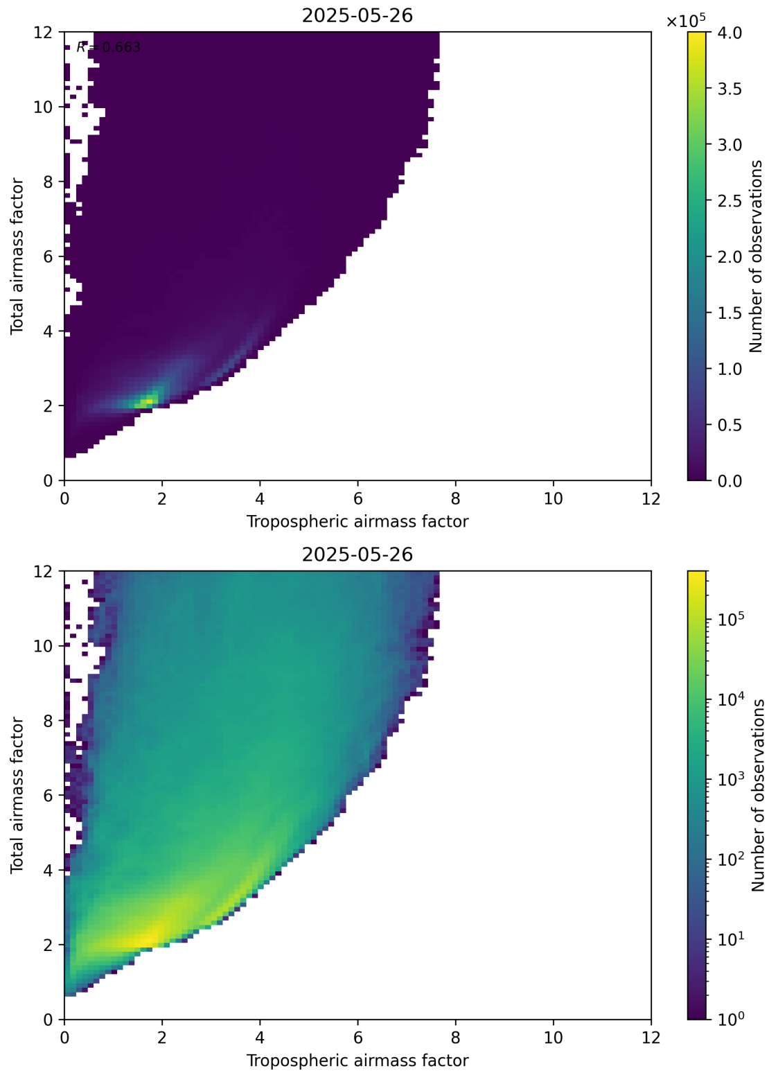
Figure 72: Scatter density plot of “Tropospheric airmass factor” against “Total airmass factor” for 2025-05-26 to 2025-05-27.
