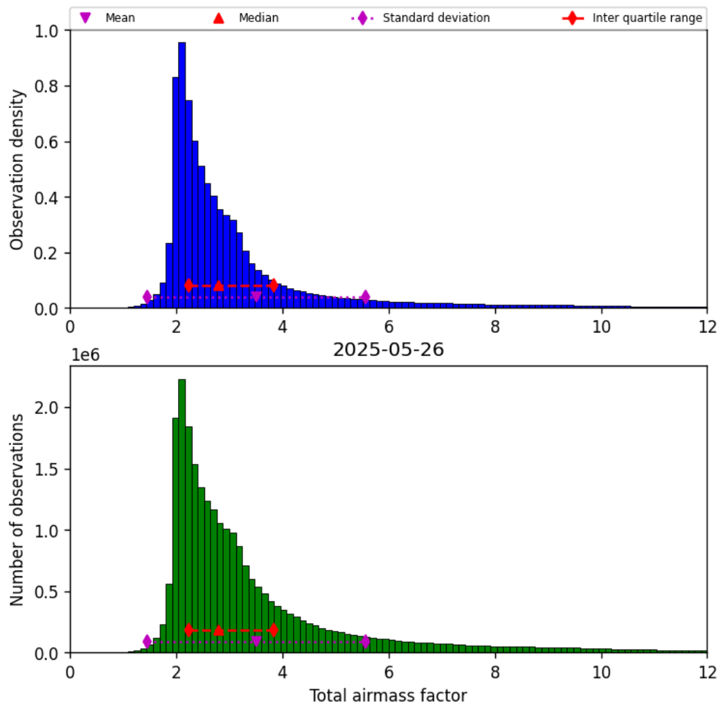
Figure 32: Histogram of “Total airmass factor” for 2025-05-26 to 2025-05-27
