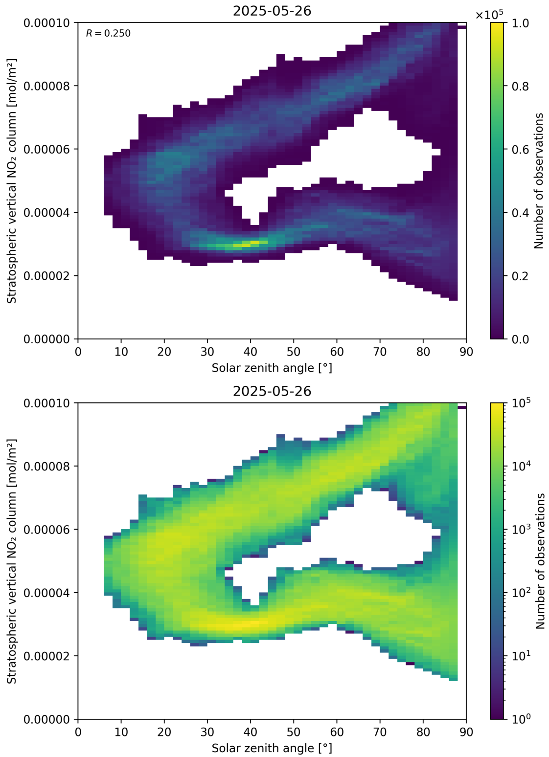
Figure 150: Scatter density plot of “Solar zenith angle” against “Stratospheric vertical NO 2 column” for 2025-05-26 to 2025-05-27.
