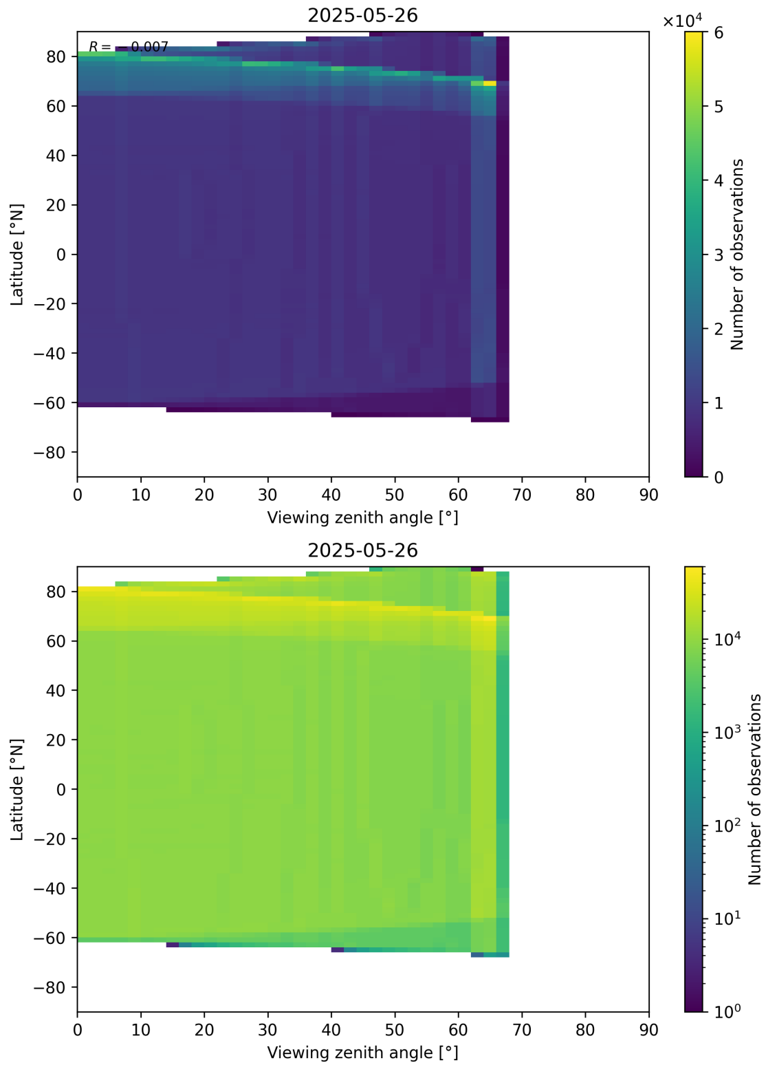
Figure 163: Scatter density plot of “Viewing zenith angle” against “Latitude” for 2025-05-26 to 2025-05-27.
