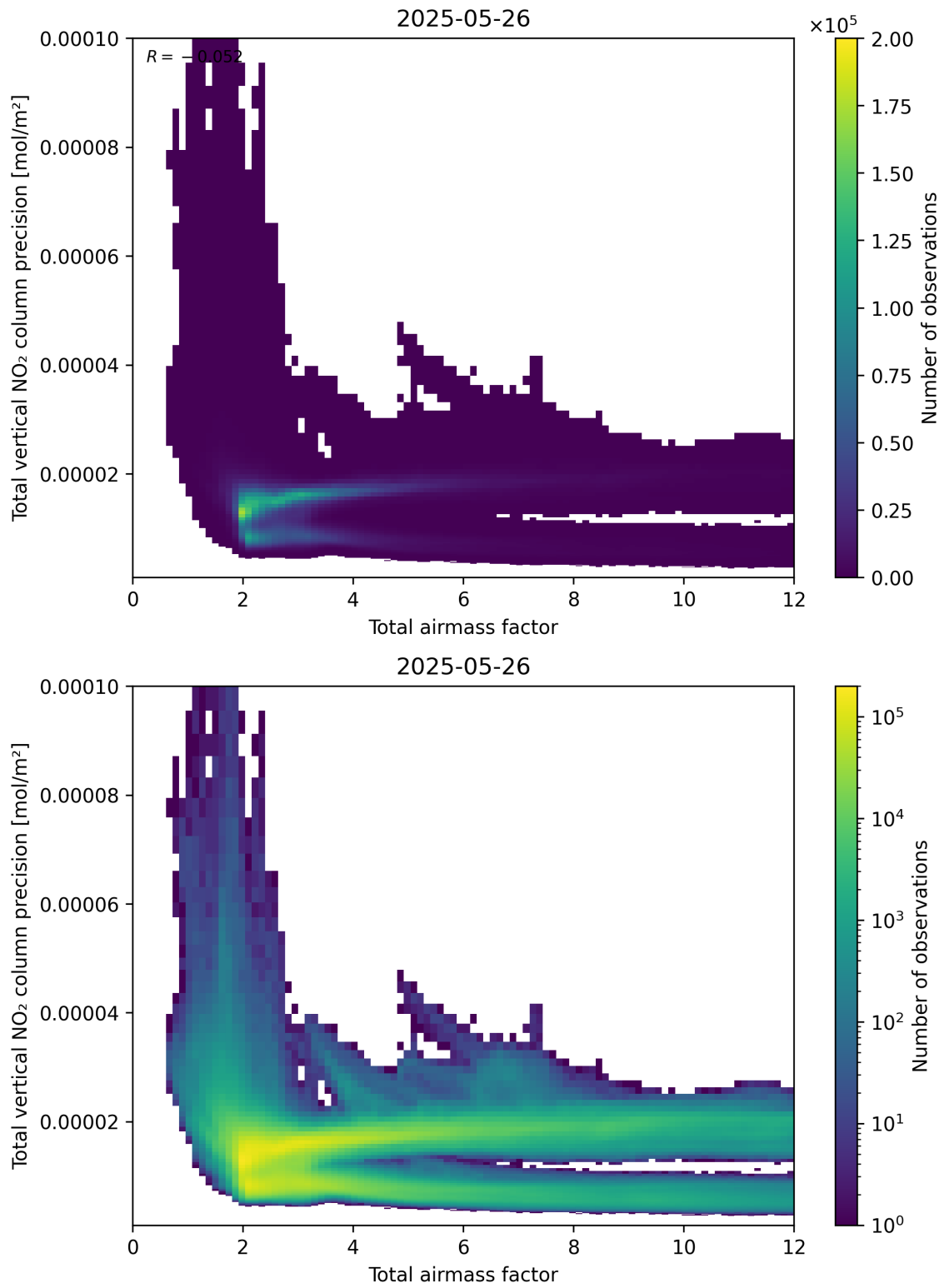
Figure 68: Scatter density plot of “Total airmass factor” against “Total vertical NO 2 column precision” for 2025-05-26 to 2025-05-27.
