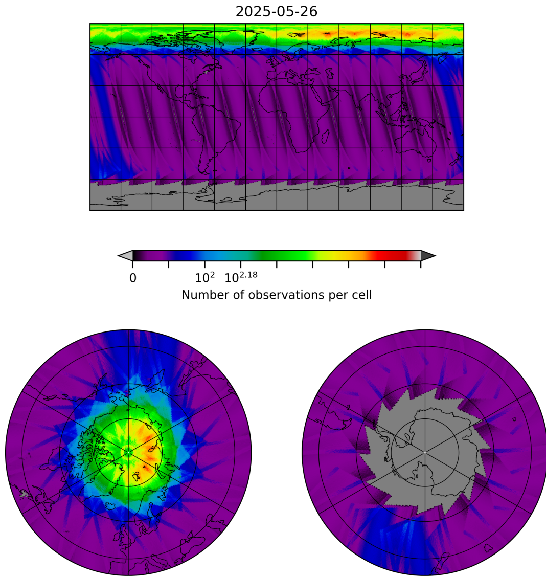
Figure 10: Map of the number of observations for 2025-05-26 to 2025-05-27
