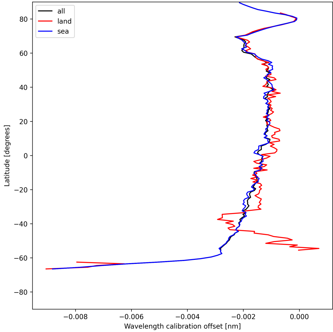
Figure 18: Zonal average of “Wavelength calibration offset” for 2025-05-26 to 2025-05-27.
