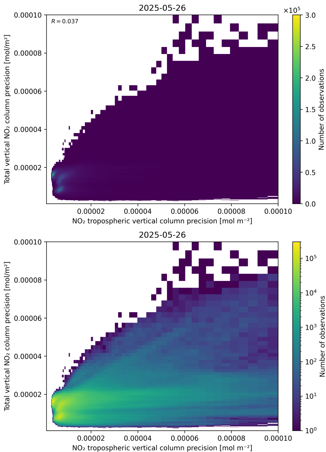
Figure 139: Scatter density plot of “NO 2 tropospheric vertical column precision” against “Total vertical NO 2 column precision” for 2025-05-26 to 2025-05-27.
