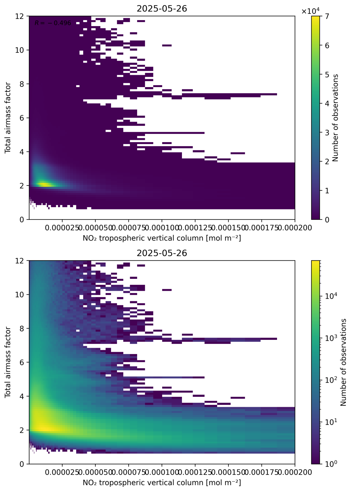
Figure 122: Scatter density plot of “NO 2 tropospheric vertical column” against “Total airmass factor” for 2025-05-26 to 2025-05-27.
