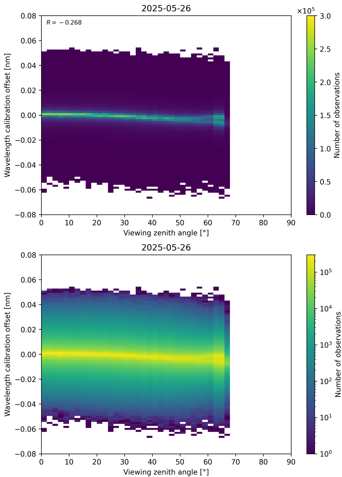
Figure 173: Scatter density plot of “Viewing zenith angle” against “Wavelength calibration offset” for 2025-05-26 to 2025-05-27.
