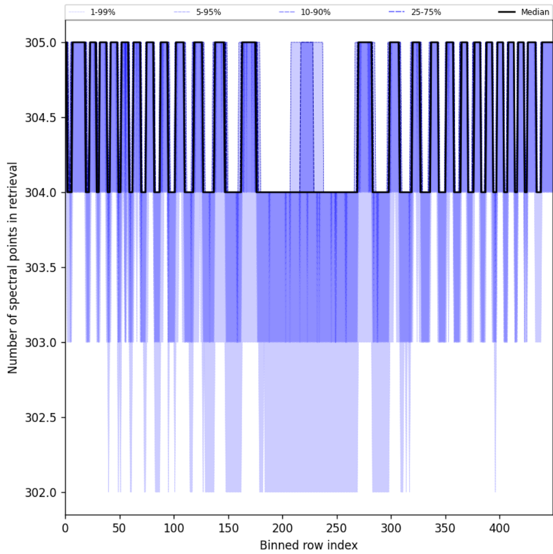
Figure 50: Along track statistics of “Number of spectral points in retrieval” for 2025-05-26 to 2025-05-27
