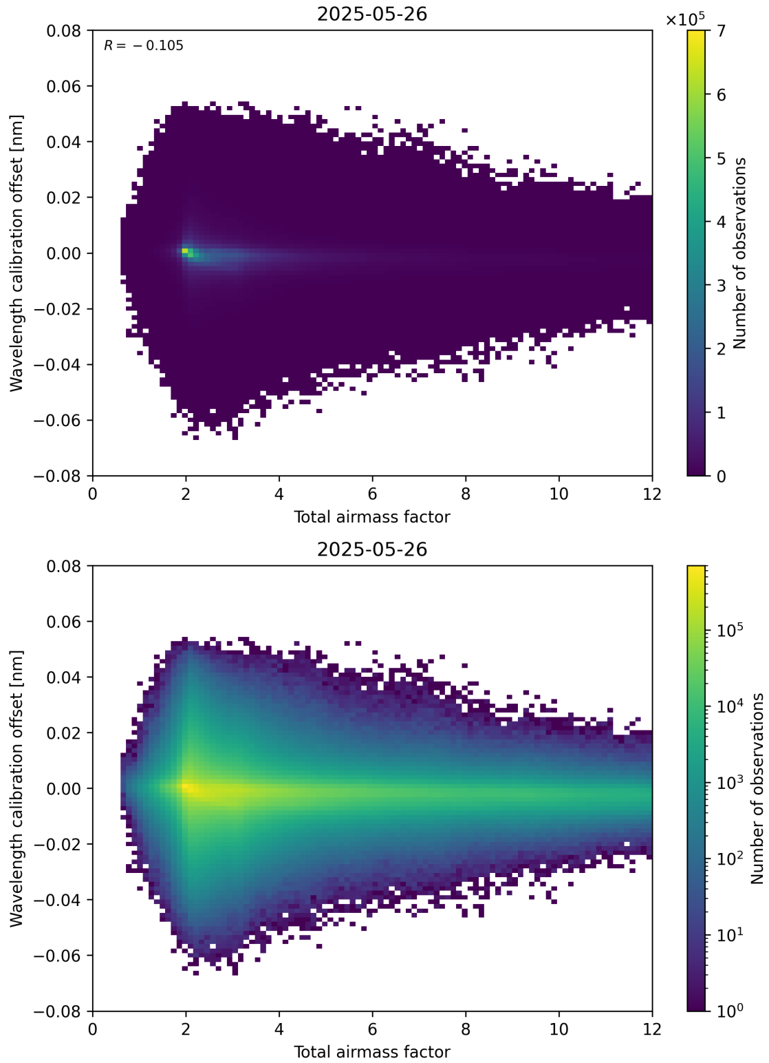
Figure 70: Scatter density plot of “Total airmass factor” against “Wavelength calibration offset” for 2025-05-26 to 2025-05-27.
