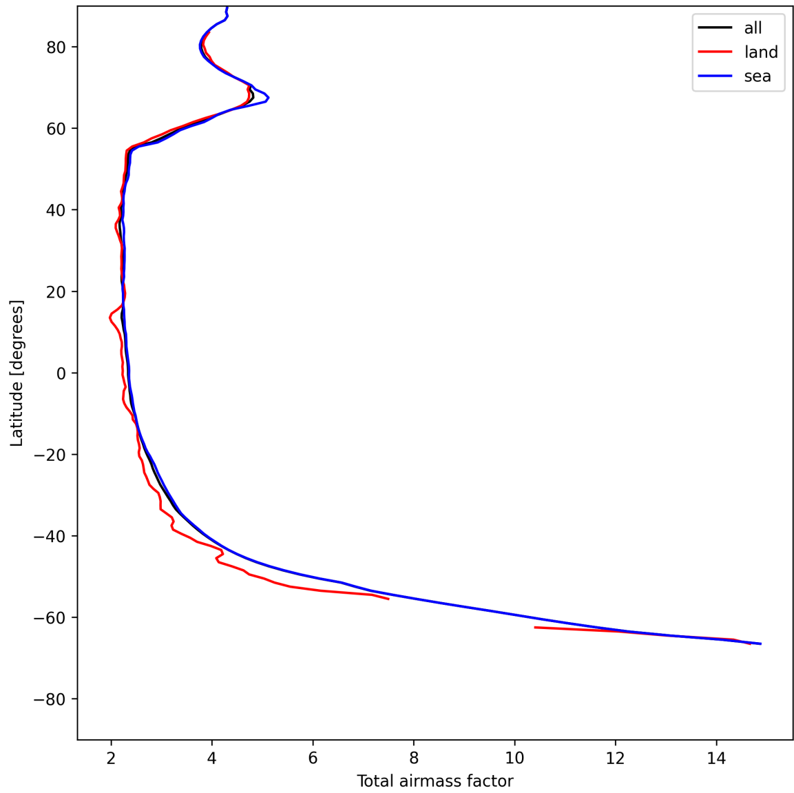
Figure 15: Zonal average of “Total airmass factor” for 2025-05-26 to 2025-05-27.
