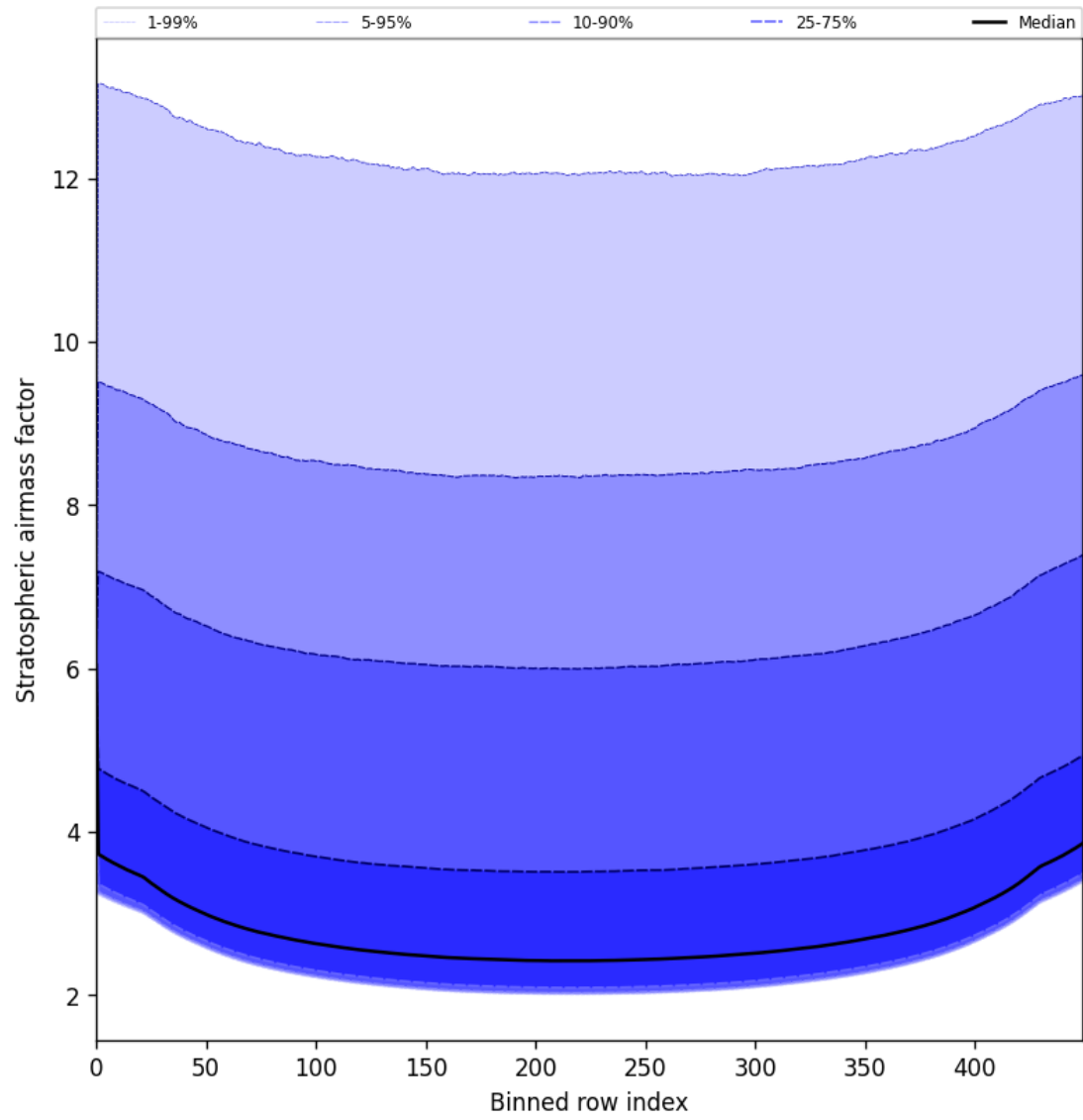
Figure 61: Along track statistics of “Stratospheric airmass factor” for 2025-05-26 to 2025-05-27
