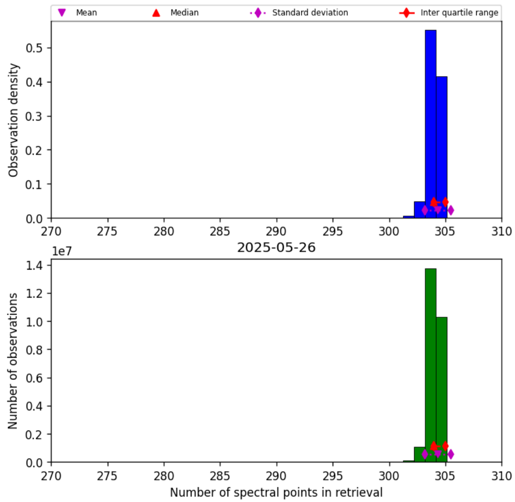
Figure 33: Histogram of “Number of spectral points in retrieval” for 2025-05-26 to 2025-05-27
