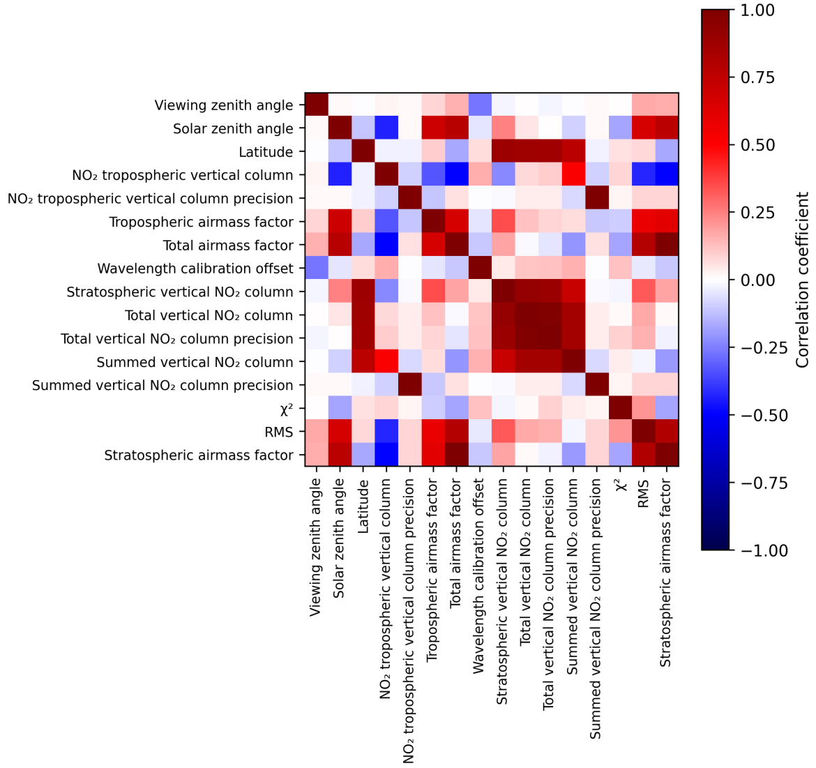
Figure 2: Map of correlation matrix for 2025-05-26 to 2025-05-27.
