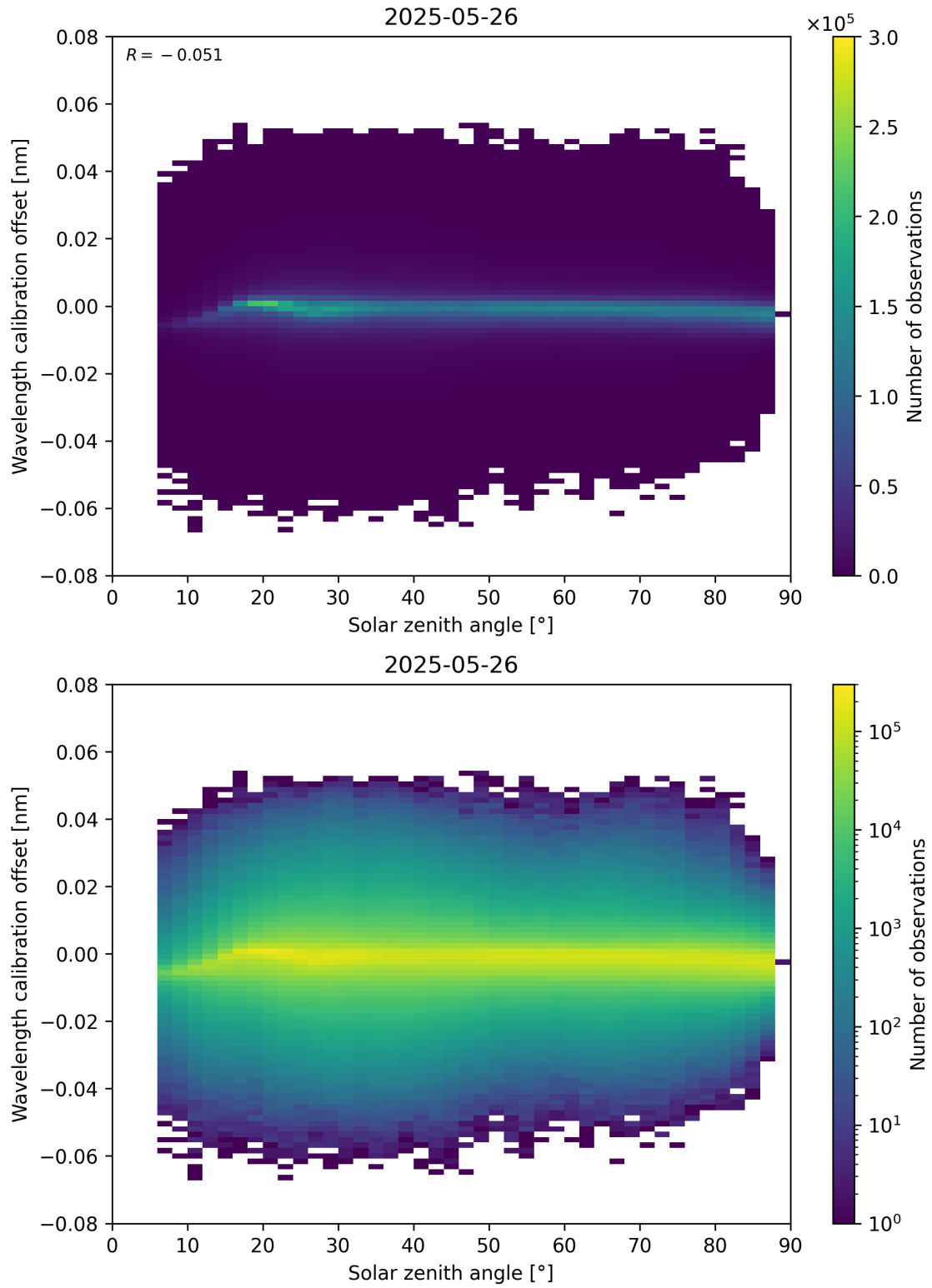
Figure 158: Scatter density plot of “Solar zenith angle” against “Wavelength calibration offset” for 2025-05-26 to 2025-05-27.
