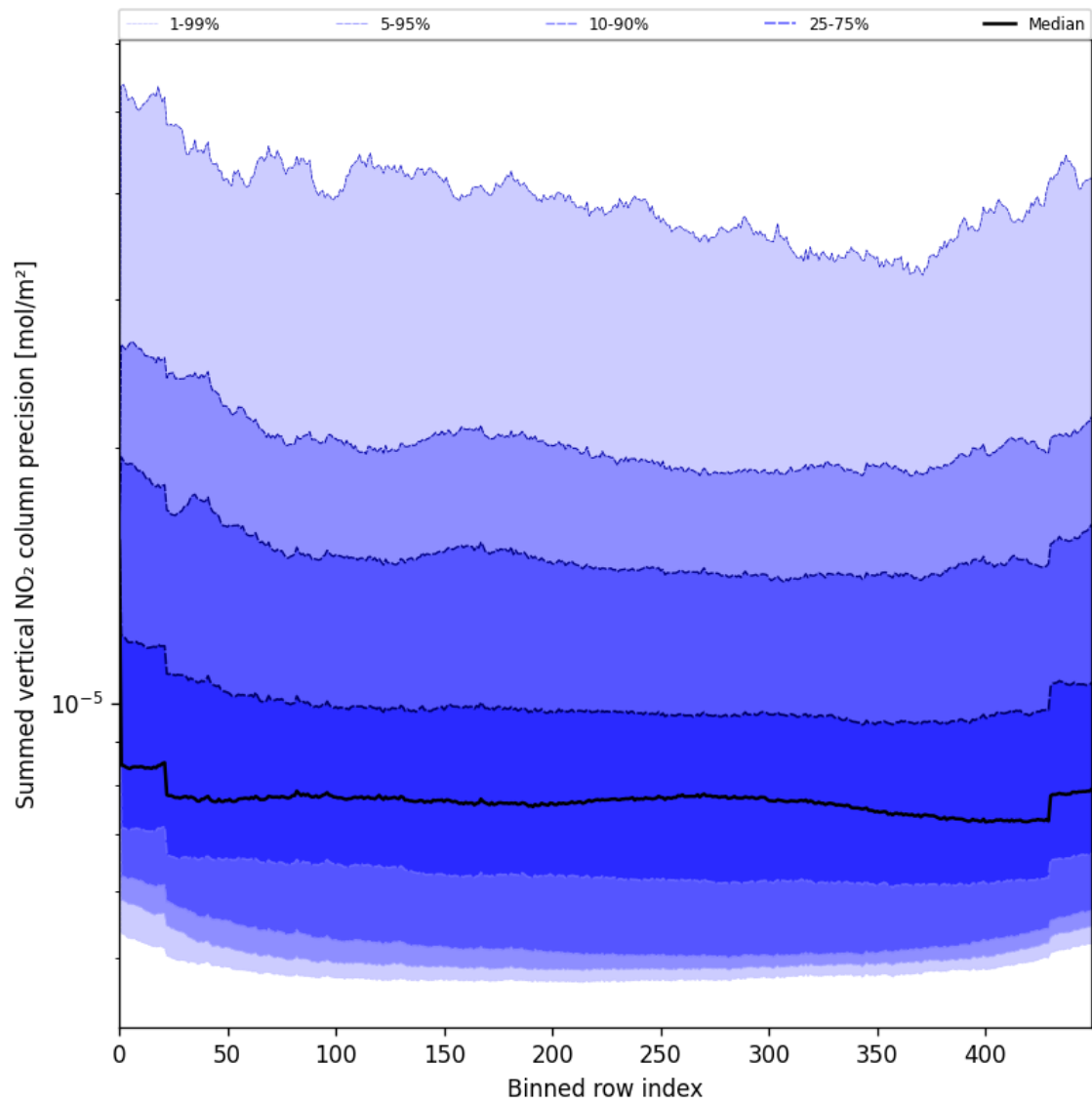
Figure 58: Along track statistics of “Summed vertical NO 2 column precision” for 2025-05-26 to 2025-05-27
