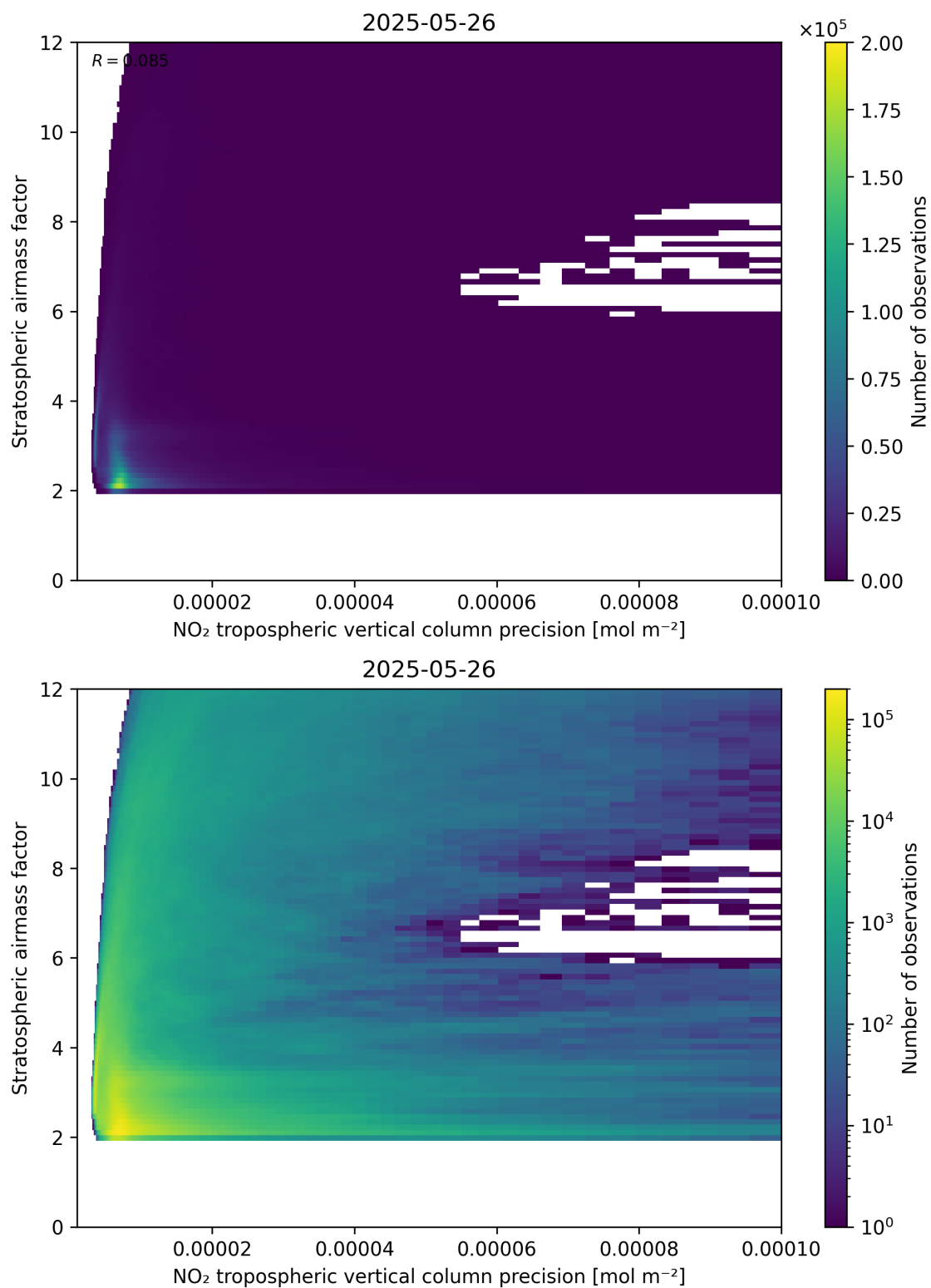
Figure 131: Scatter density plot of “NO 2 tropospheric vertical column precision” against “Stratospheric airmass factor” for 2025-05-26 to 2025-05-27.
