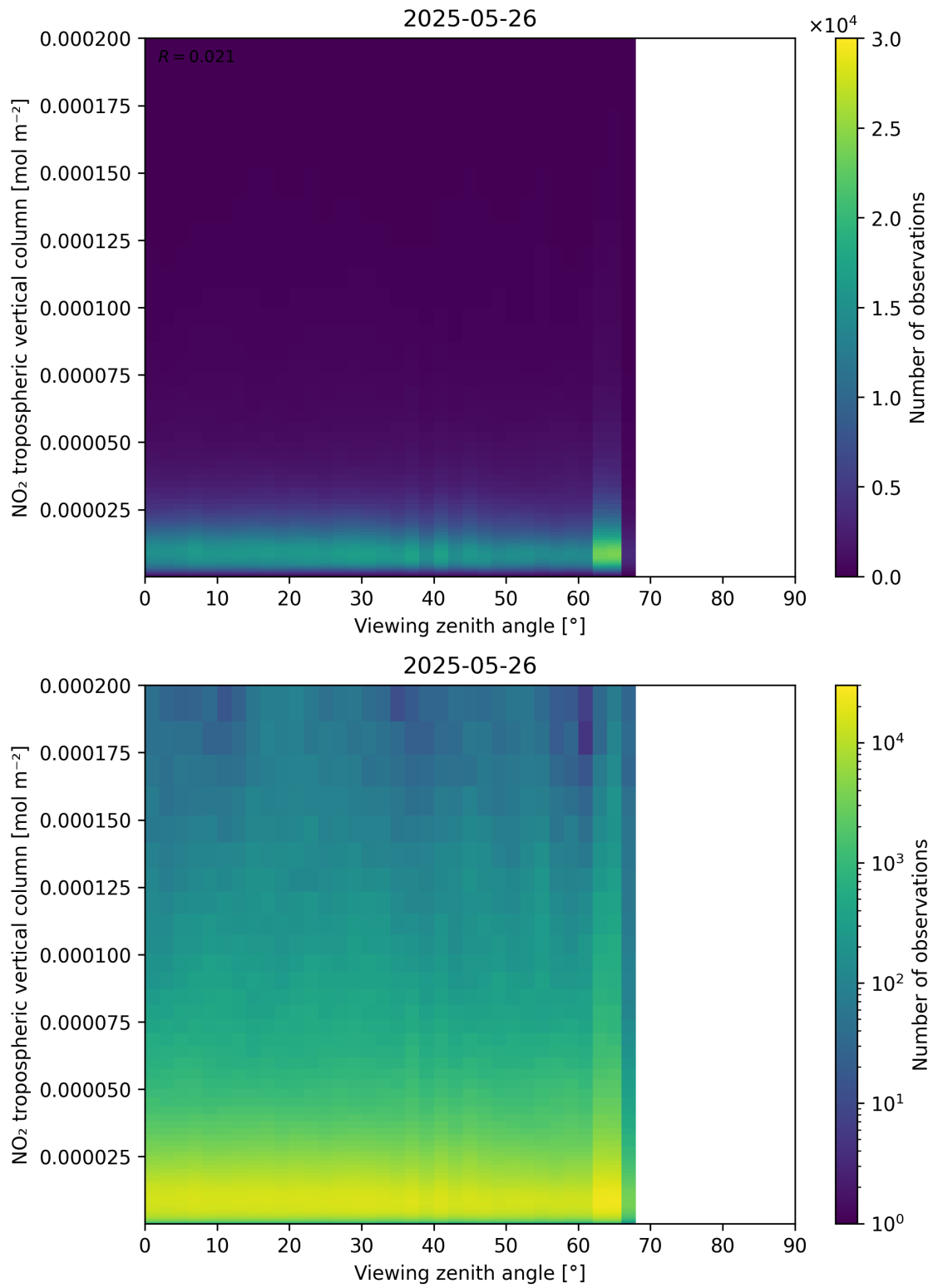
Figure 169: Scatter density plot of “Viewing zenith angle” against “NO 2 tropospheric vertical column” for 2025-05-26 to 2025-05-27.
