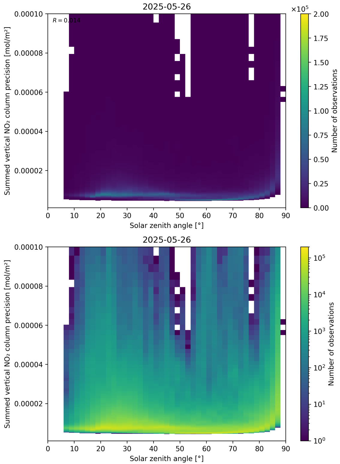
Figure 152: Scatter density plot of “Solar zenith angle” against “Summed vertical NO 2 column precision” for 2025-05-26 to 2025-05-27.
