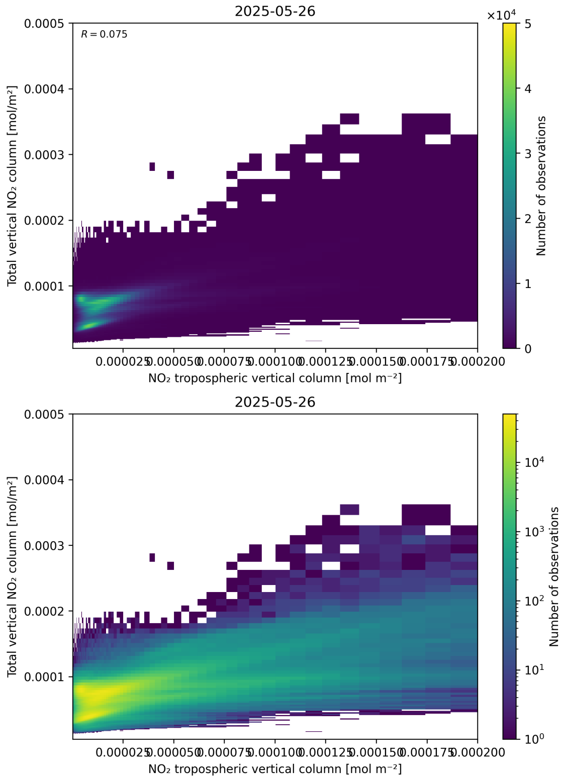
Figure 128: Scatter density plot of “NO 2 tropospheric vertical column” against “Total vertical NO 2 column” for 2025-05-26 to 2025-05-27.
