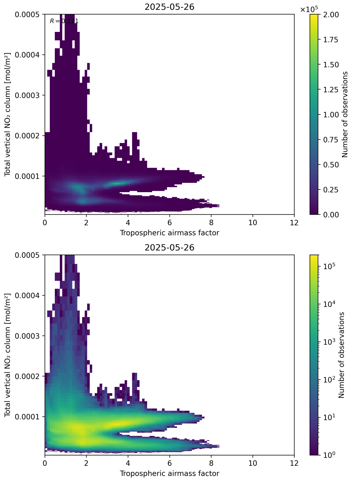
Figure 77: Scatter density plot of “Tropospheric airmass factor” against “Total vertical NO 2 column” for 2025-05-26 to 2025-05-27.
