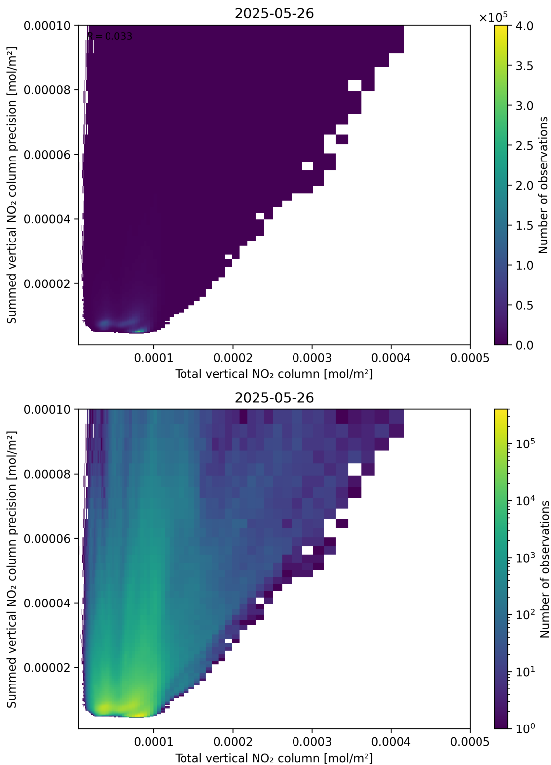
Figure 113: Scatter density plot of “Total vertical NO 2 column” against “Summed vertical NO 2 column precision” for 2025-05-26 to 2025-05-27.
