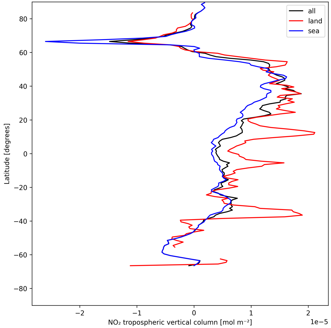
Figure 12: Zonal average of “NO 2 tropospheric vertical column” for 2025-05-26 to 2025-05-27.
