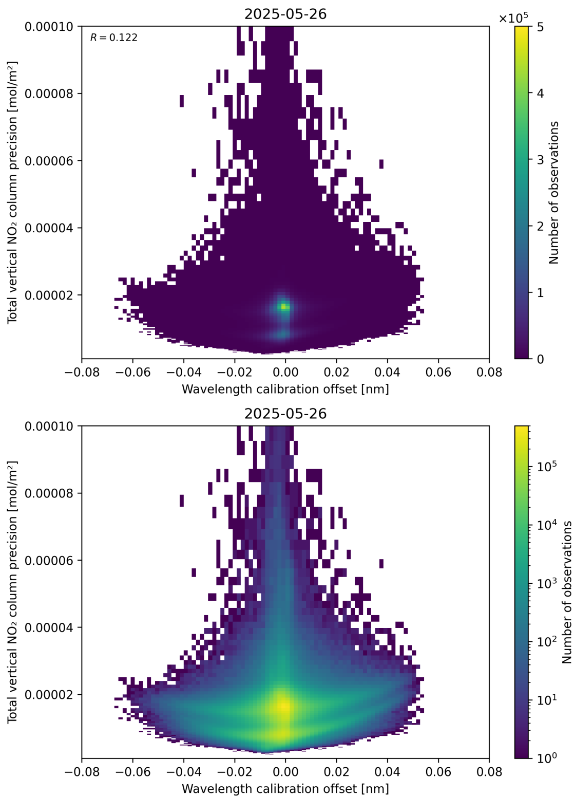
Figure 180: Scatter density plot of “Wavelength calibration offset” against “Total vertical NO 2 column precision” for 2025-05-26 to 2025-05-27.
