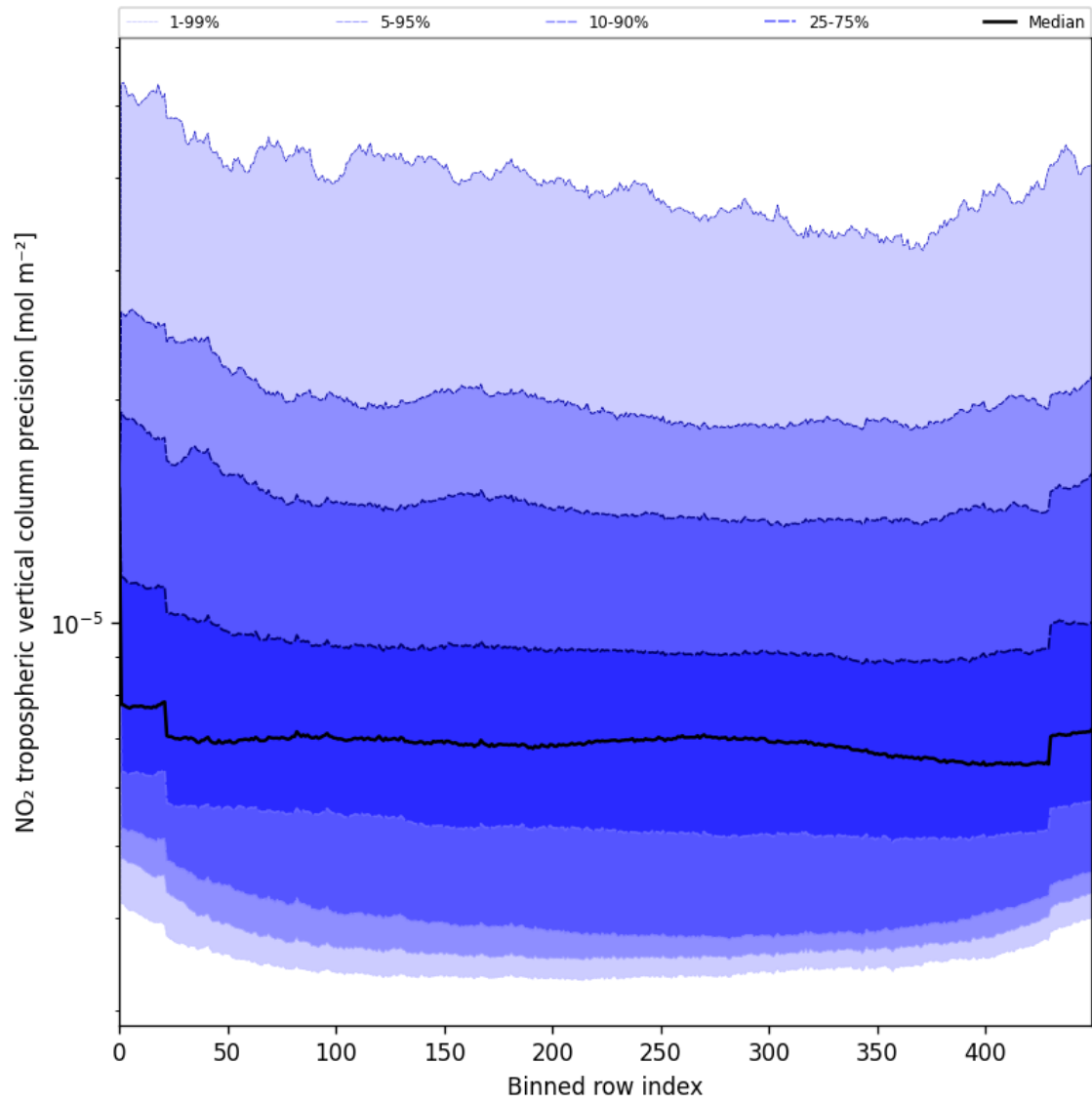
Figure 47: Along track statistics of “NO 2 tropospheric vertical column precision” for 2025-05-26 to 2025-05-27
