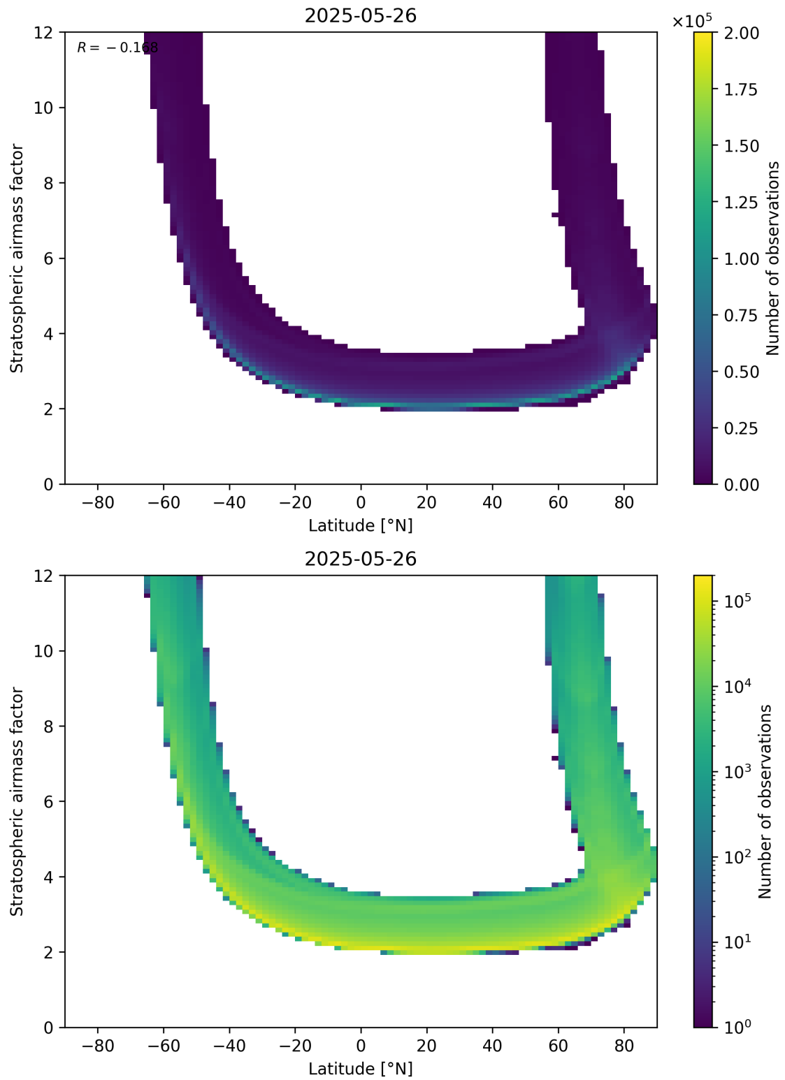
Figure 83: Scatter density plot of “Latitude” against “Stratospheric air mass factor” for 2025-05-26 to 2025-05-27.
