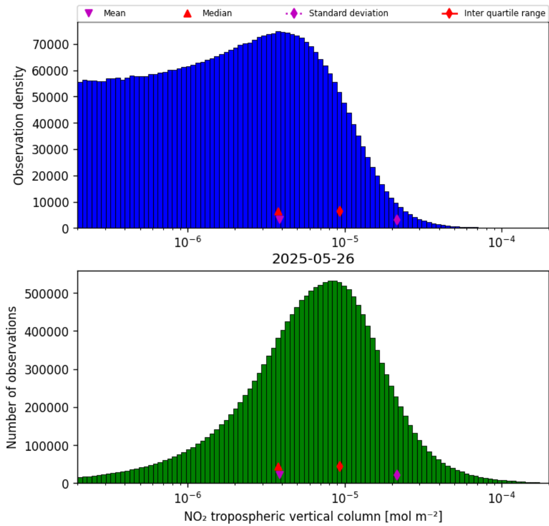
Figure 29: Histogram of “NO 2 tropospheric vertical column” for 2025-05-26 to 2025-05-27
