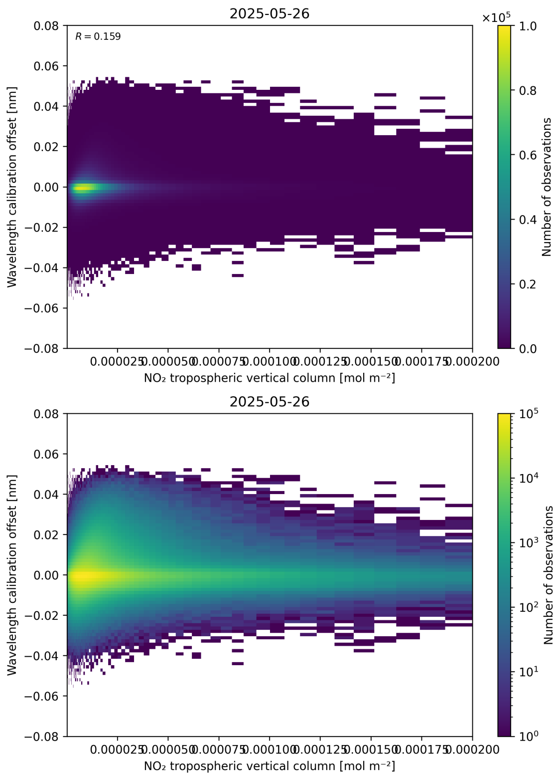
Figure 143: Scatter density plot of “NO 2 tropospheric vertical column” against “Wavelength calibration offset” for 2025-05-26 to 2025-05-27.
