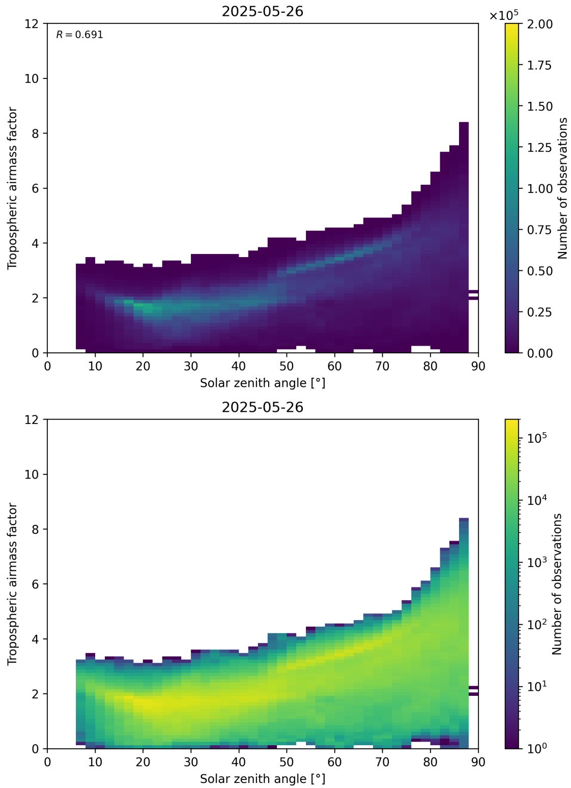
Figure 147: Scatter density plot of “Solar zenith angle” against “Tropospheric airmass factor” for 2025-05-26 to 2025-05-27.
