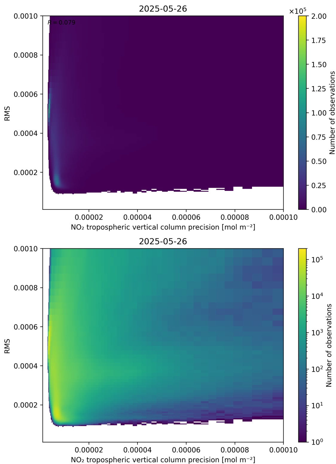
Figure 140: Scatter density plot of “NO 2 tropospheric vertical column precision” against “RMS” for 2025-05-26 to 2025-05-27.
