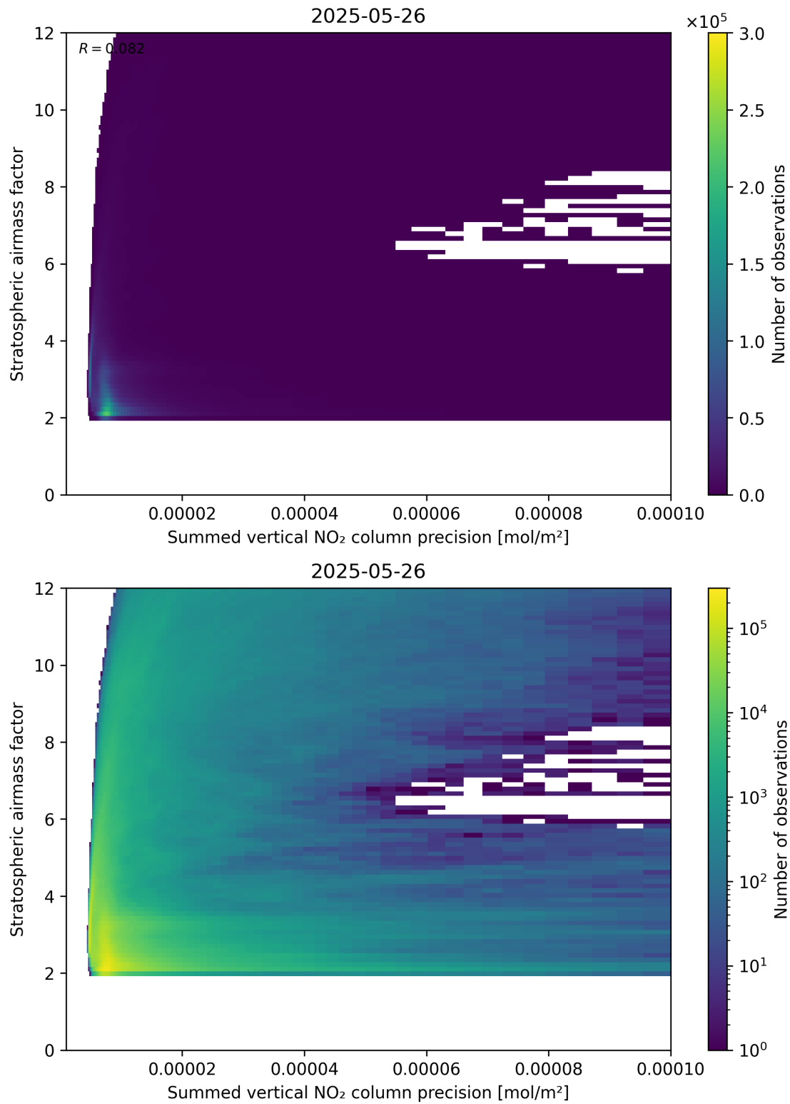
Figure 106: Scatter density plot of “Summed vertical NO 2 column precision” against “Stratospheric airmass factor” for 2025-05-26 to 2025-05-27.
