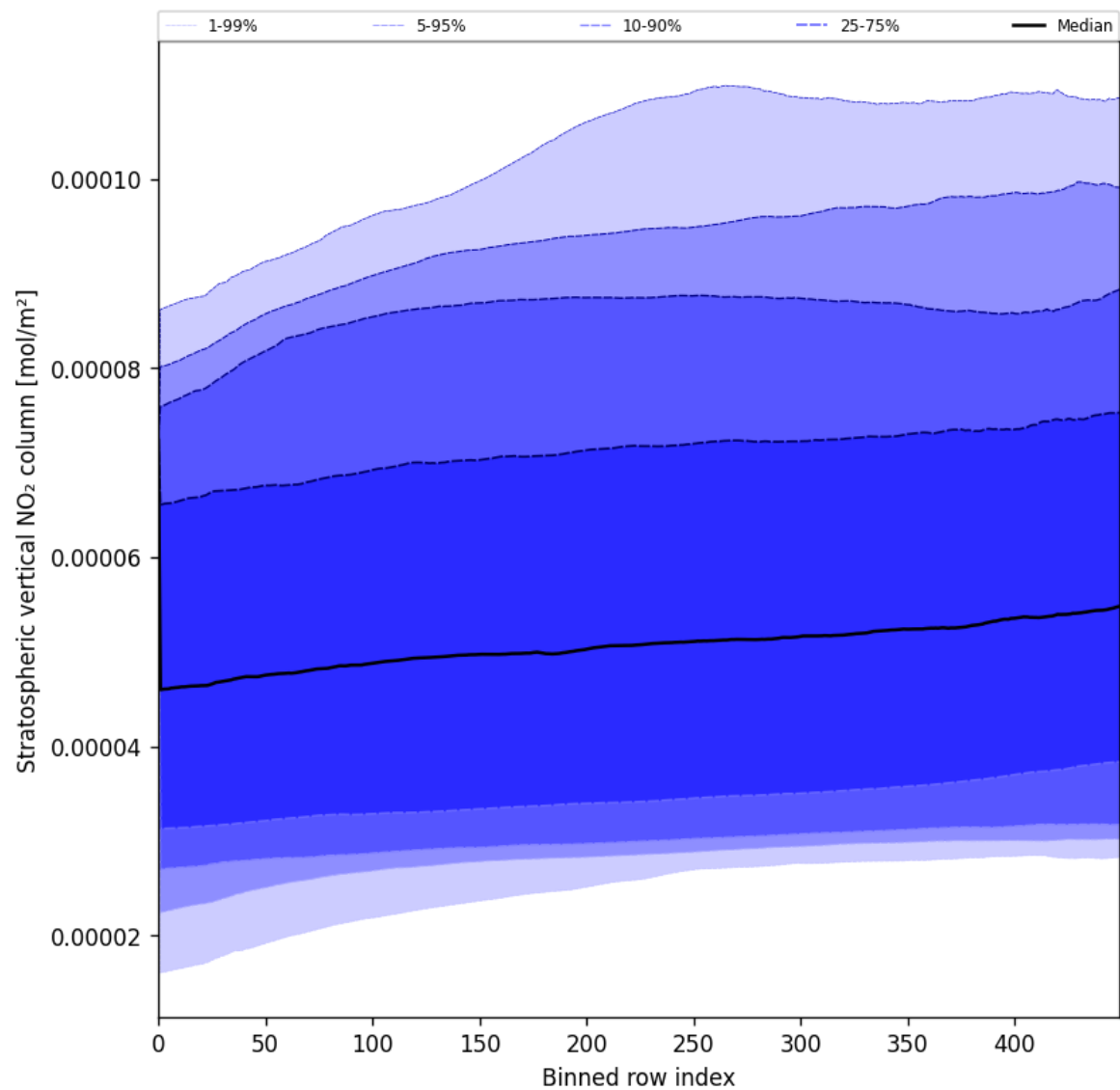
Figure 53: Along track statistics of “Stratospheric vertical NO 2 column” for 2025-05-26 to 2025-05-27
