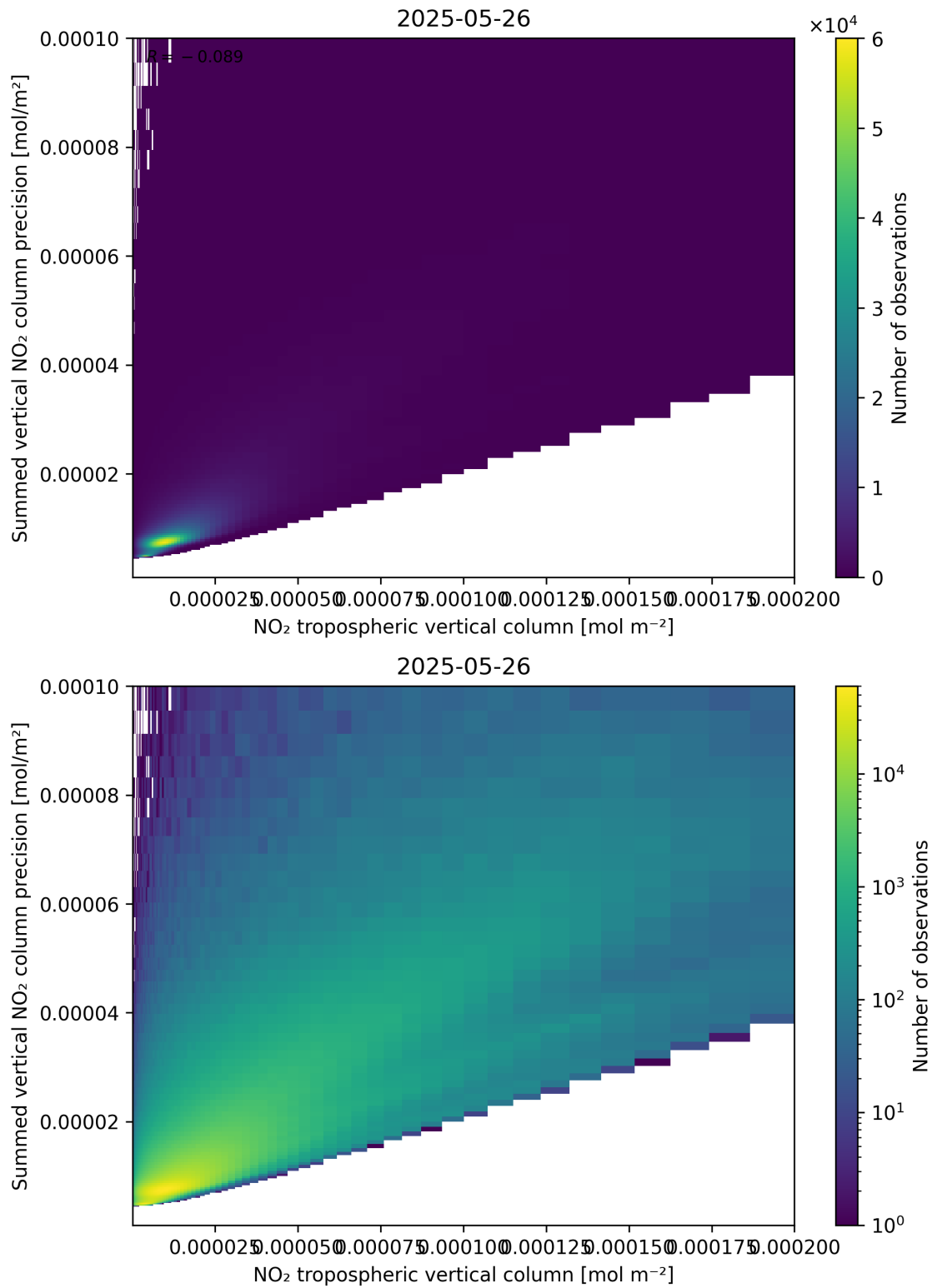
Figure 127: Scatter density plot of “NO 2 tropospheric vertical column” against “Summed vertical NO 2 column precision” for 2025-05-26 to 2025-05-27.
