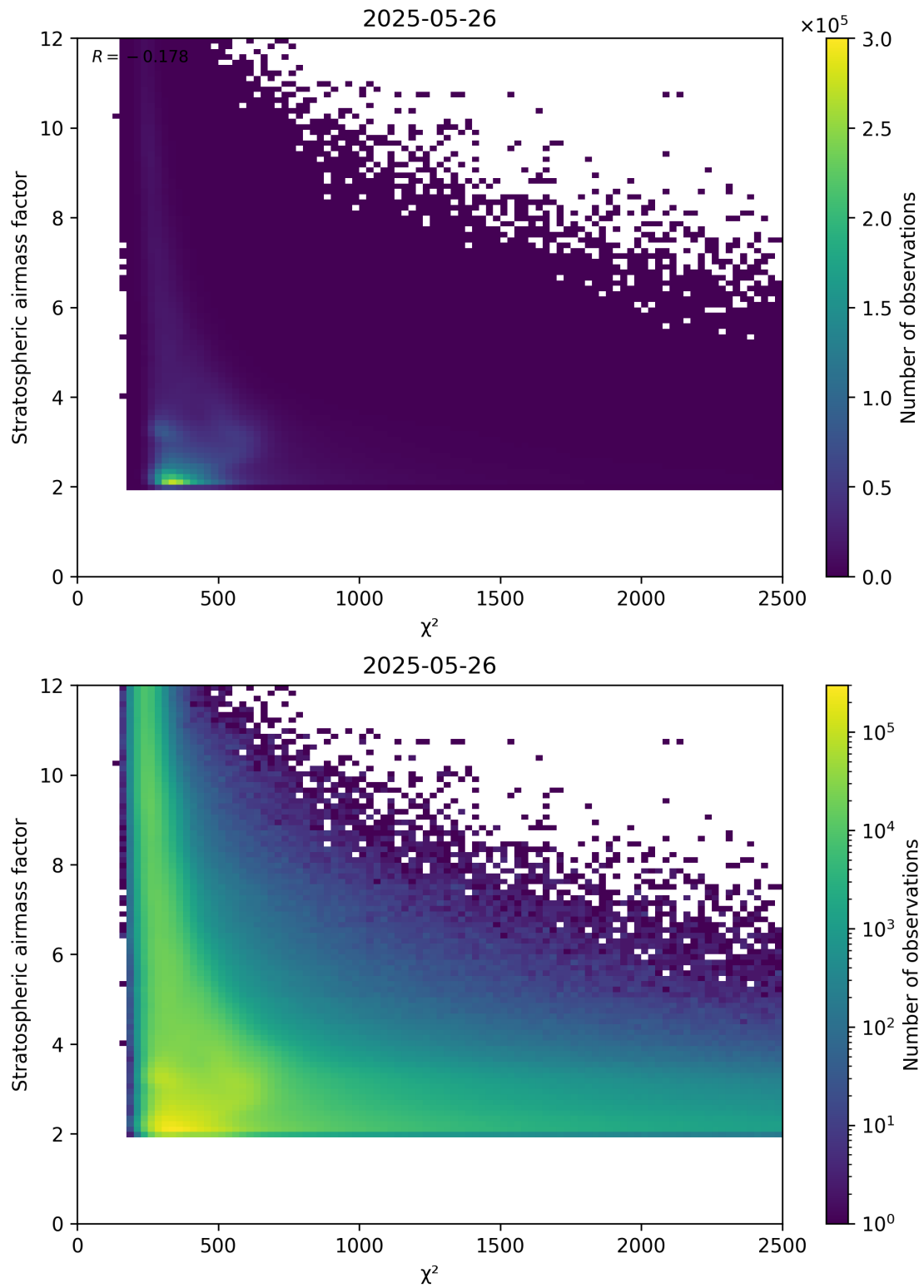
Figure 81: Scatter density plot of “ \chi^2 ” against “Stratospheric airmass factor” for 2025-05-26 to 2025-05-27.
