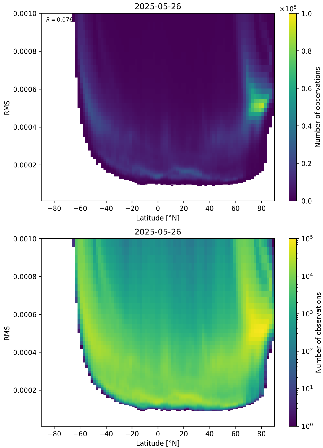
Figure 94: Scatter density plot of “Latitude” against “RMS” for 2025-05-26 to 2025-05-27.
