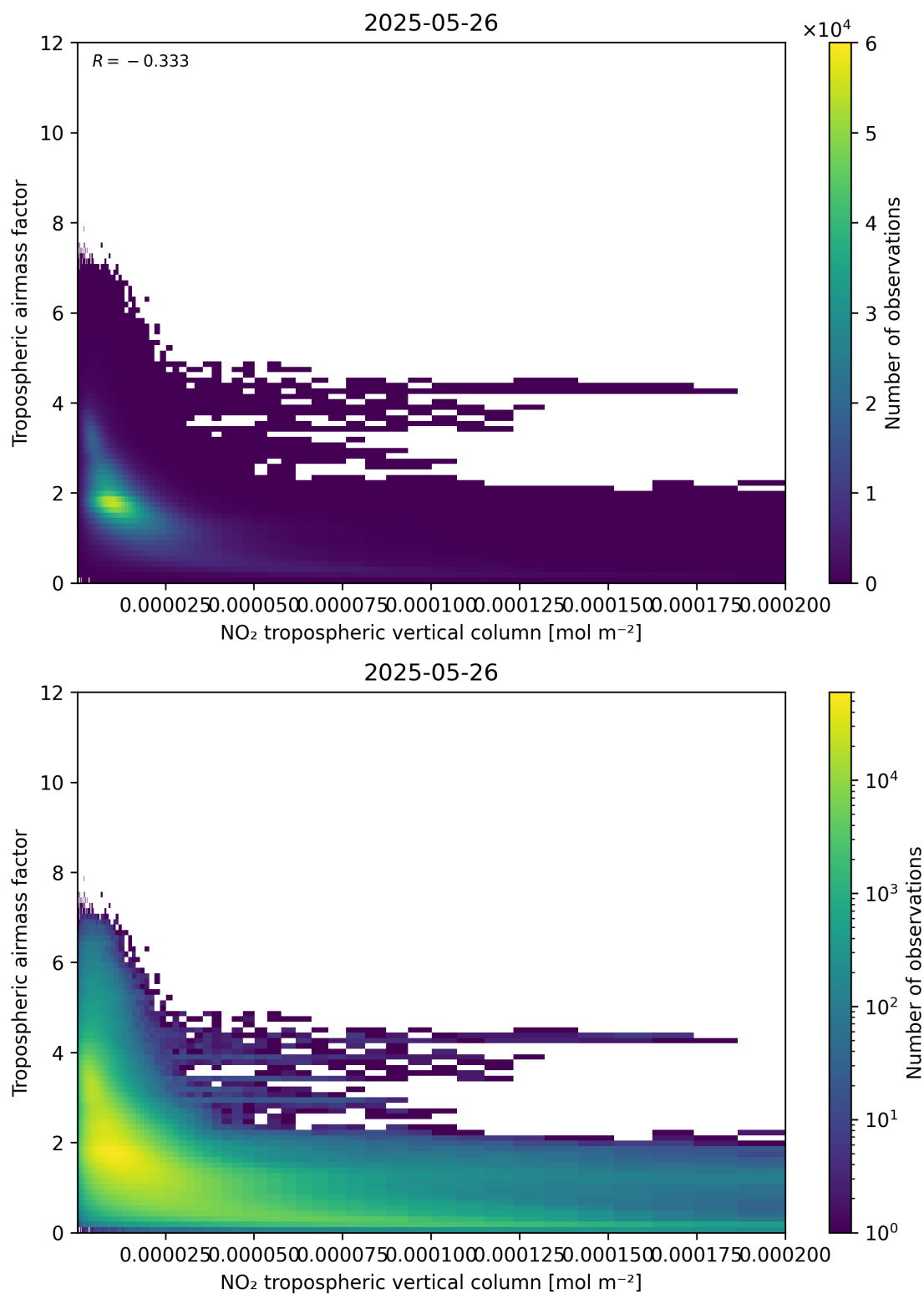
Figure 123: Scatter density plot of “NO 2 tropospheric vertical column” against “Tropospheric air mass factor” for 2025-05-26 to 2025-05-27.
