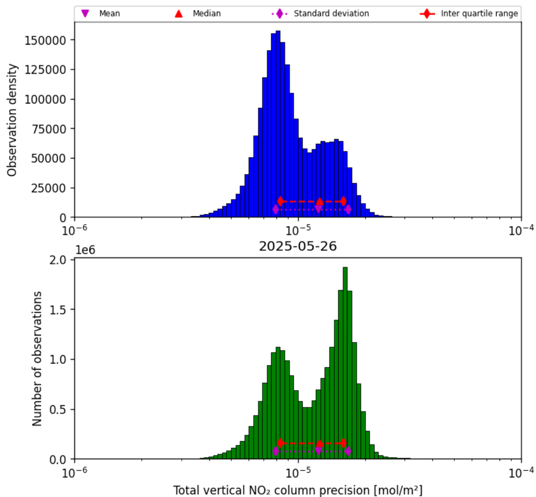
Figure 39: Histogram of “Total vertical NO 2 column precision” for 2025-05-26 to 2025-05-27
