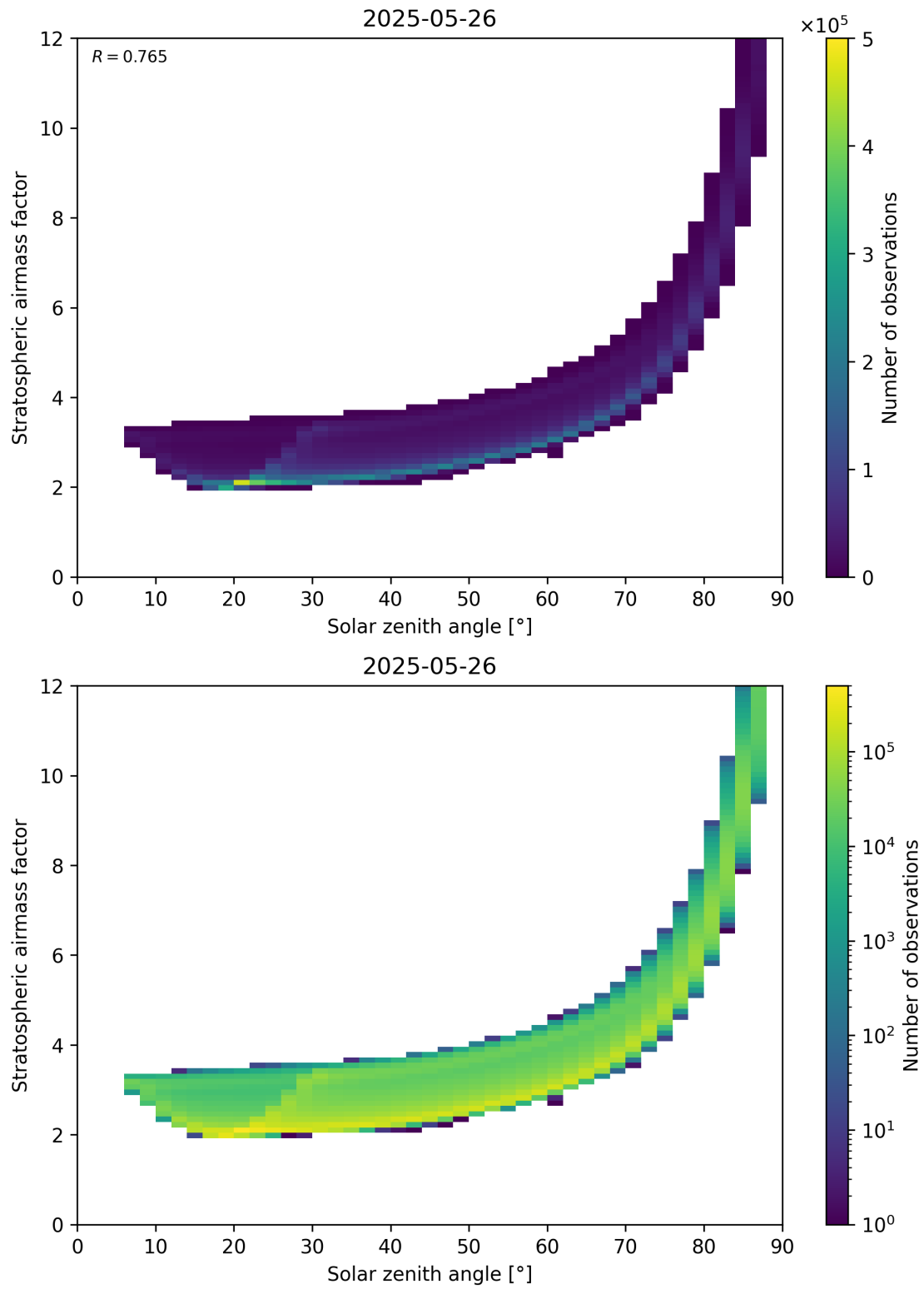
Figure 145: Scatter density plot of “Solar zenith angle” against “Stratospheric airmass factor” for 2025-05-26 to 2025-05-27.
