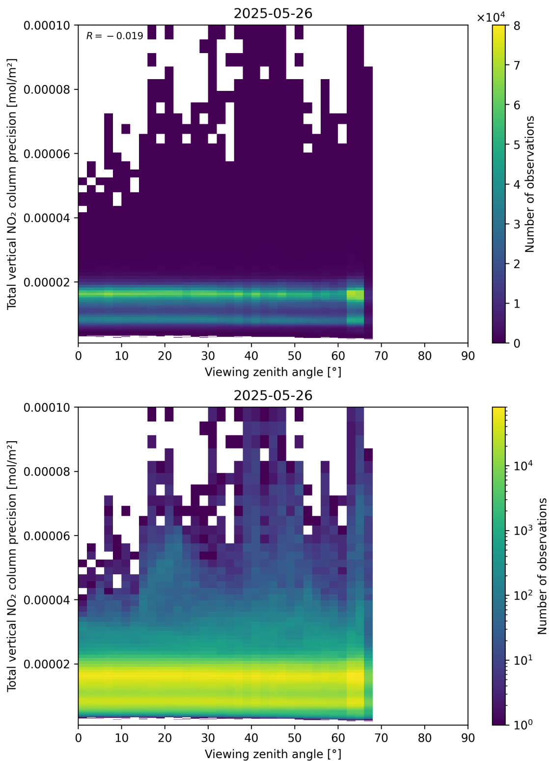
Figure 168: Scatter density plot of “Viewing zenith angle” against “Total vertical NO 2 column precision” for 2025-05-26 to 2025-05-27.
