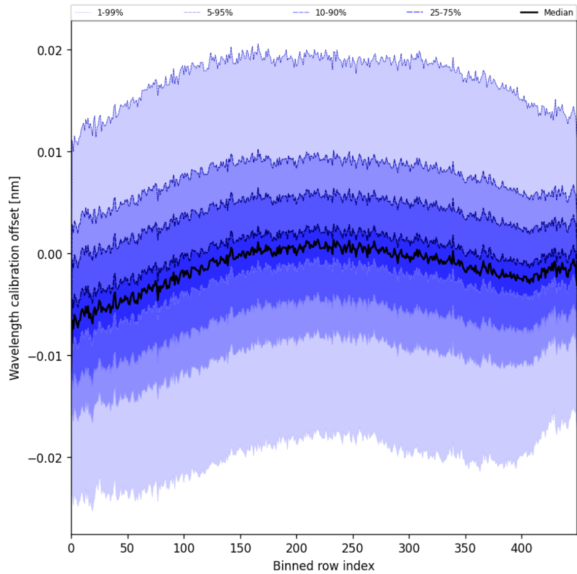
Figure 52: Along track statistics of “Wavelength calibration offset” for 2025-05-26 to 2025-05-27
