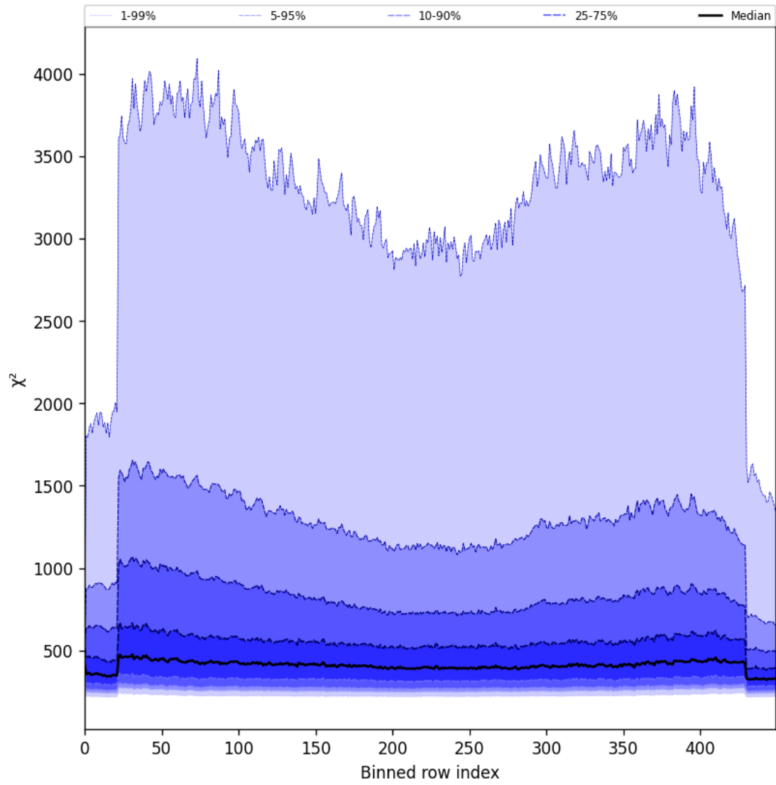
Figure 59: Along track statistics of “ \chi^2 ” for 2025-05-26 to 2025-05-27
