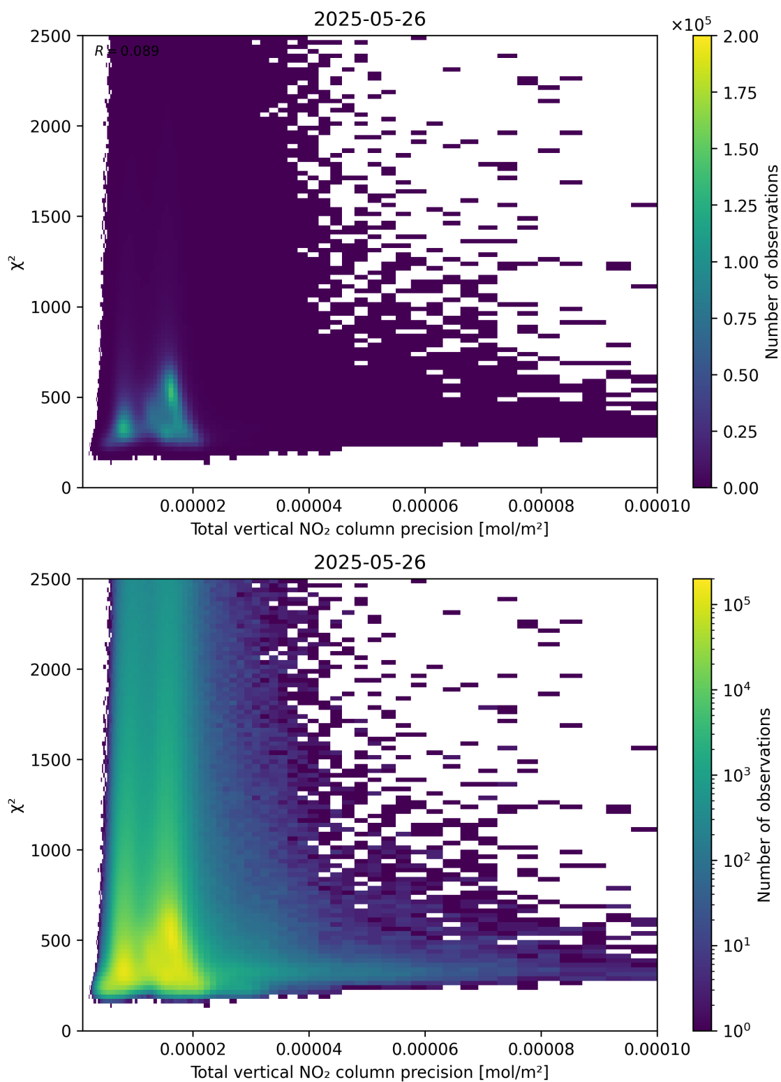
Figure 116: Scatter density plot of “Total vertical NO 2 column precision” against “ \chi^2 ” for 2025-05-26 to 2025-05-27.
