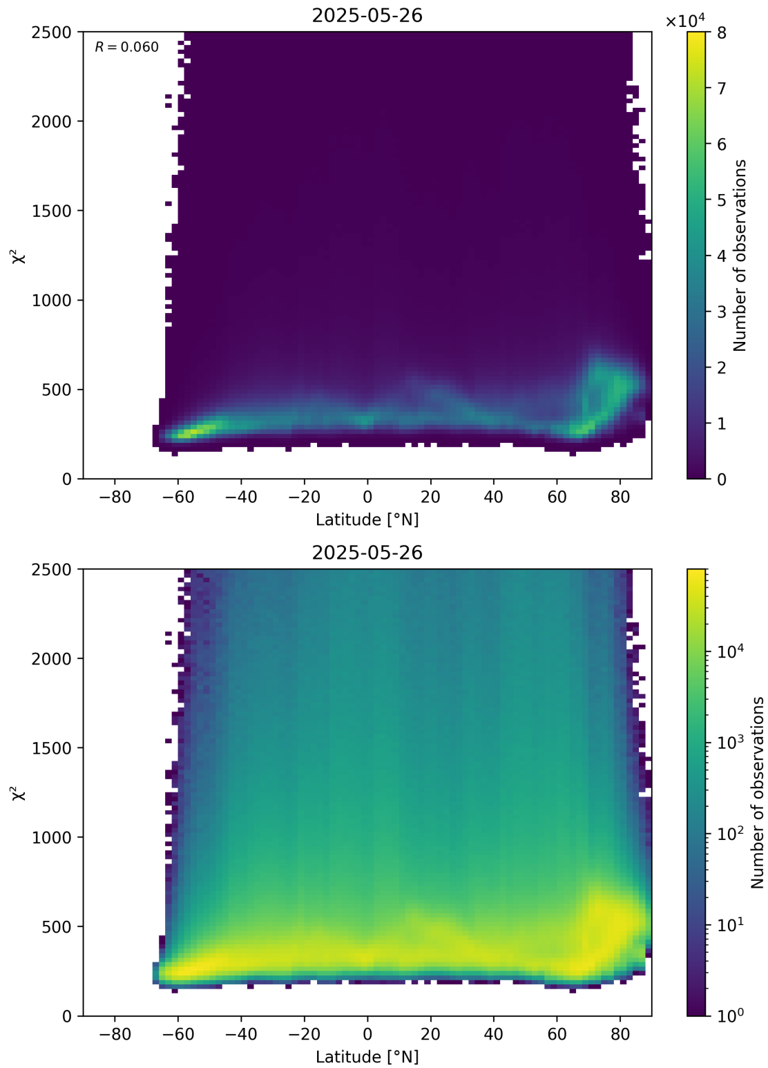
Figure 86: Scatter density plot of “Latitude” against “ \chi^2 ” for 2025-05-26 to 2025-05-27.
