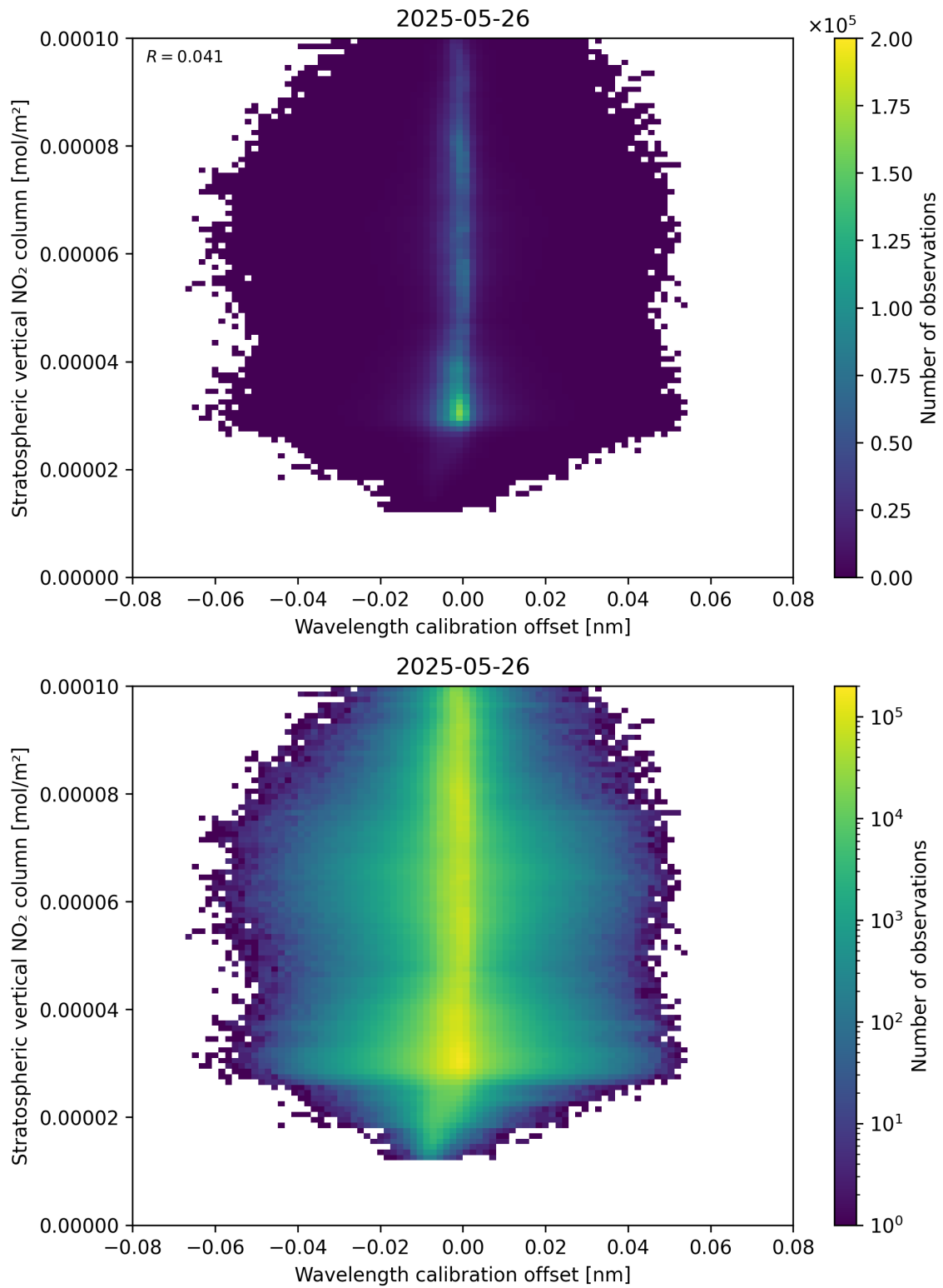
Figure 176: Scatter density plot of “Wavelength calibration offset” against “Stratospheric vertical NO 2 column” for 2025-05-26 to 2025-05-27.
