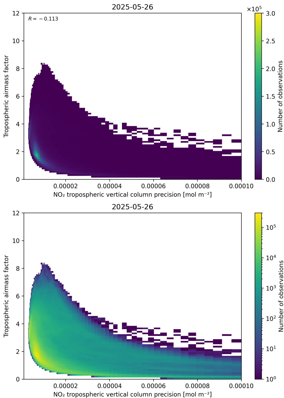
Figure 133: Scatter density plot of “NO 2 tropospheric vertical column precision” against “Tropospheric airmass factor” for 2025-05-26 to 2025-05-27.
