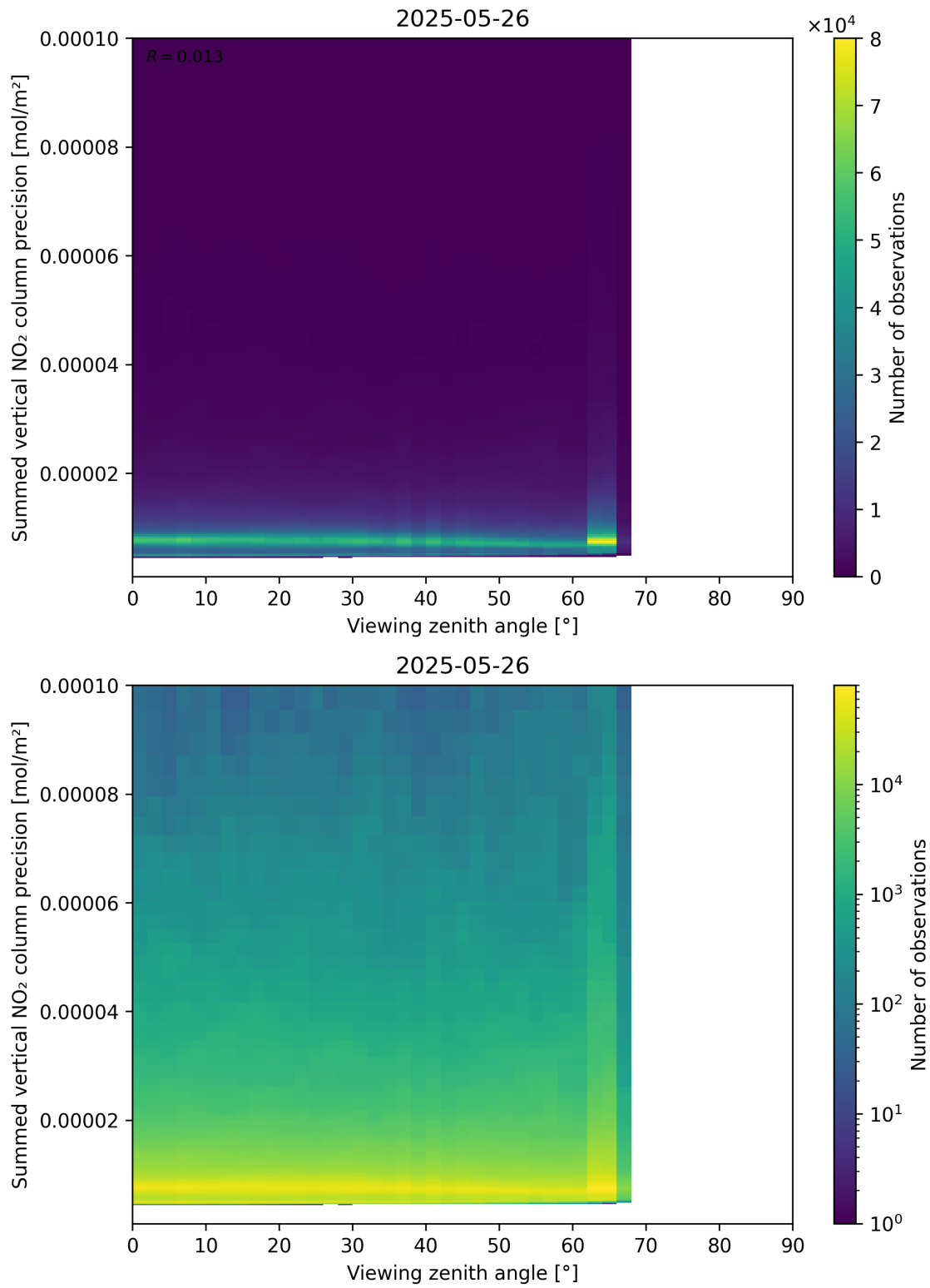
Figure 166: Scatter density plot of “Viewing zenith angle” against “Summed vertical NO 2 column precision” for 2025-05-26 to 2025-05-27.
