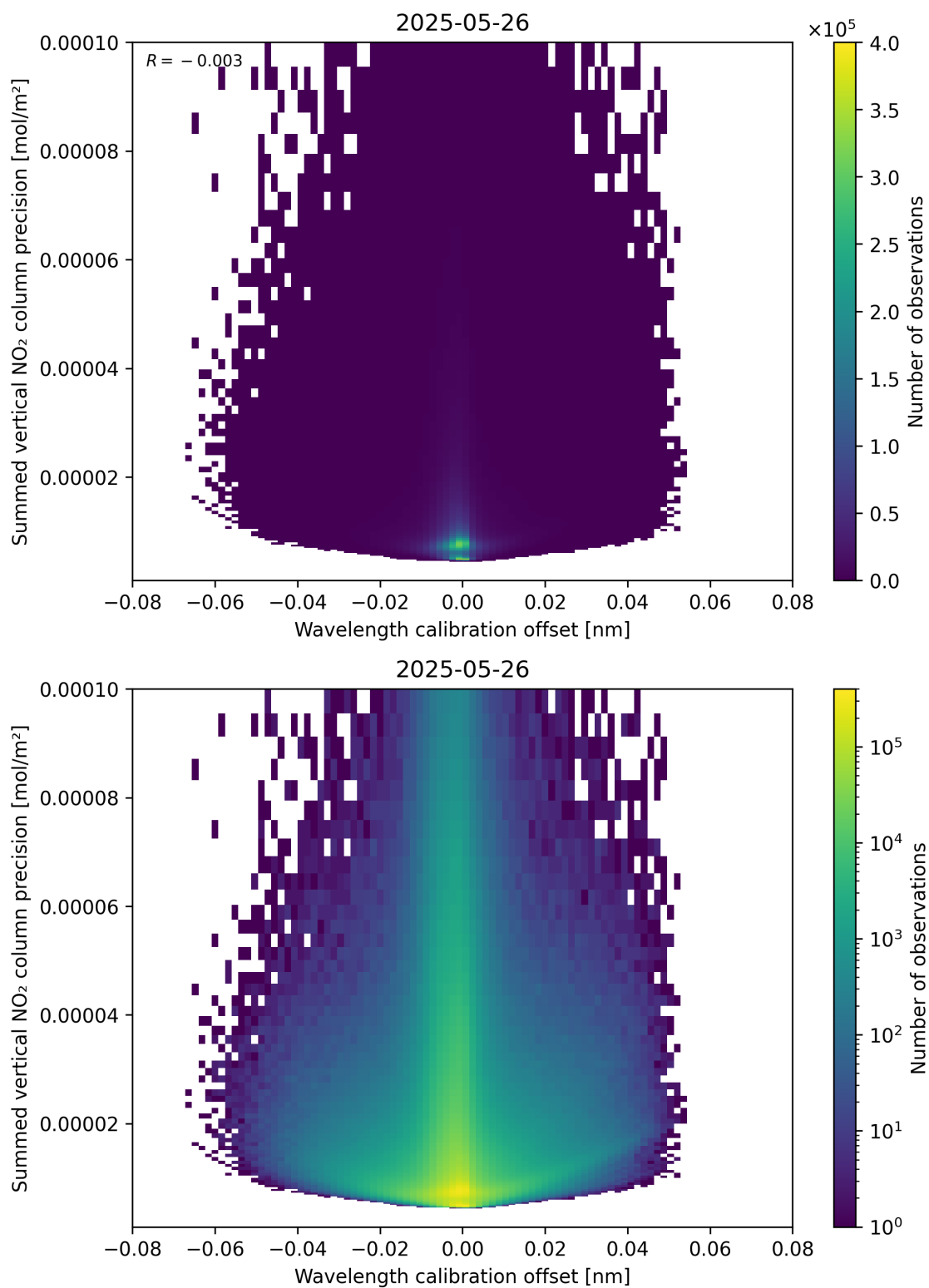
Figure 178: Scatter density plot of “Wavelength calibration offset” against “Summed vertical NO 2 column precision” for 2025-05-26 to 2025-05-27.
