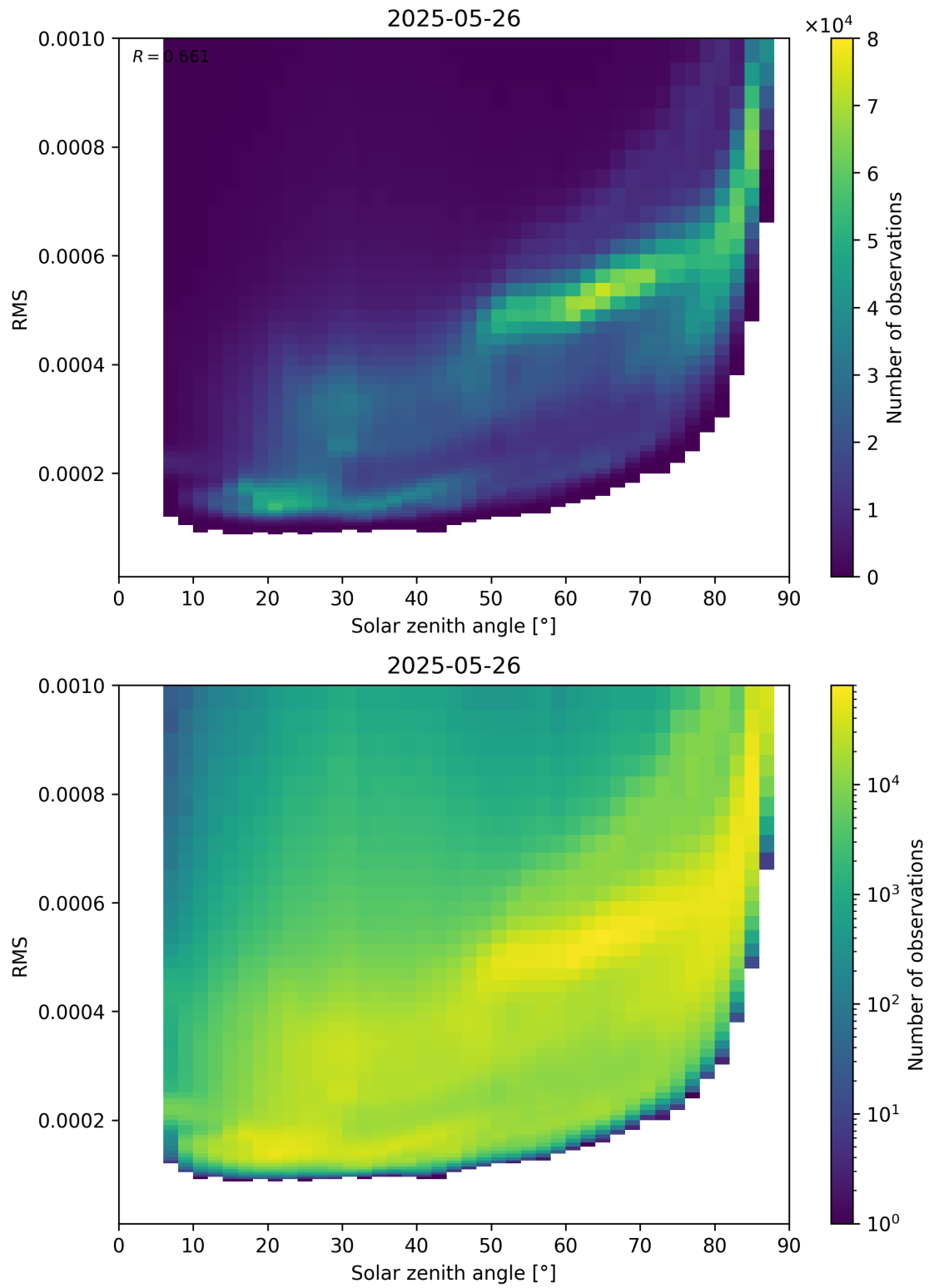
Figure 157: Scatter density plot of “Solar zenith angle” against “RMS” for 2025-05-26 to 2025-05-27.
