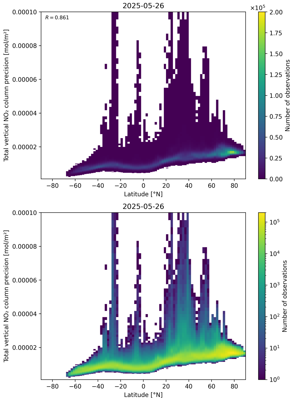
Figure 91: Scatter density plot of “Latitude” against “Total vertical NO 2 column precision” for 2025-05-26 to 2025-05-27.
