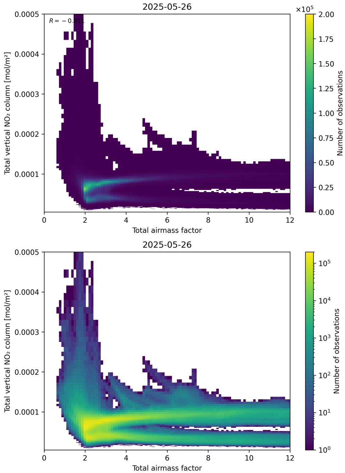
Figure 67: Scatter density plot of “Total airmass factor” against “Total vertical NO 2 column” for 2025-05-26 to 2025-05-27.
