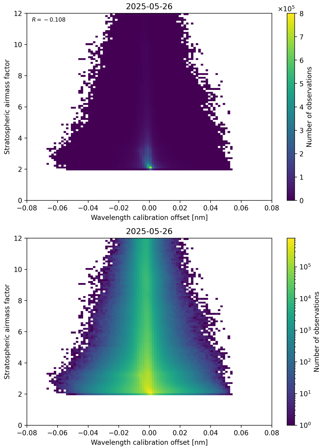
Figure 174: Scatter density plot of “Wavelength calibration offset” against “Stratospheric airmass factor” for 2025-05-26 to 2025-05-27.
