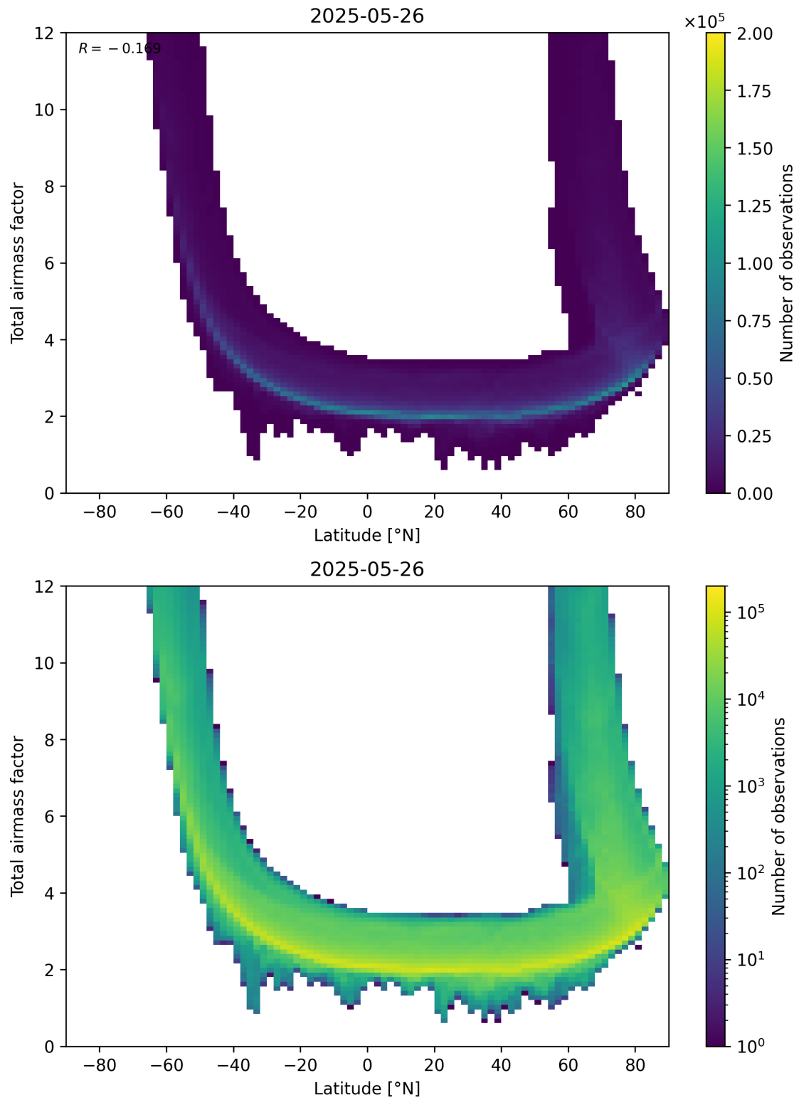
Figure 84: Scatter density plot of “Latitude” against “Total airmass factor” for 2025-05-26 to 2025-05-27.
