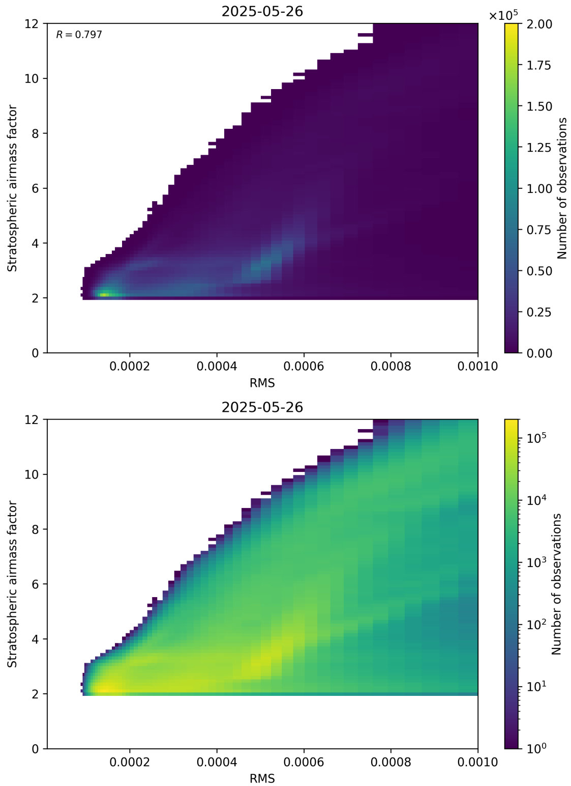
Figure 144: Scatter density plot of “RMS” against “Stratospheric airmass factor” for 2025-05-26 to 2025-05-27.
