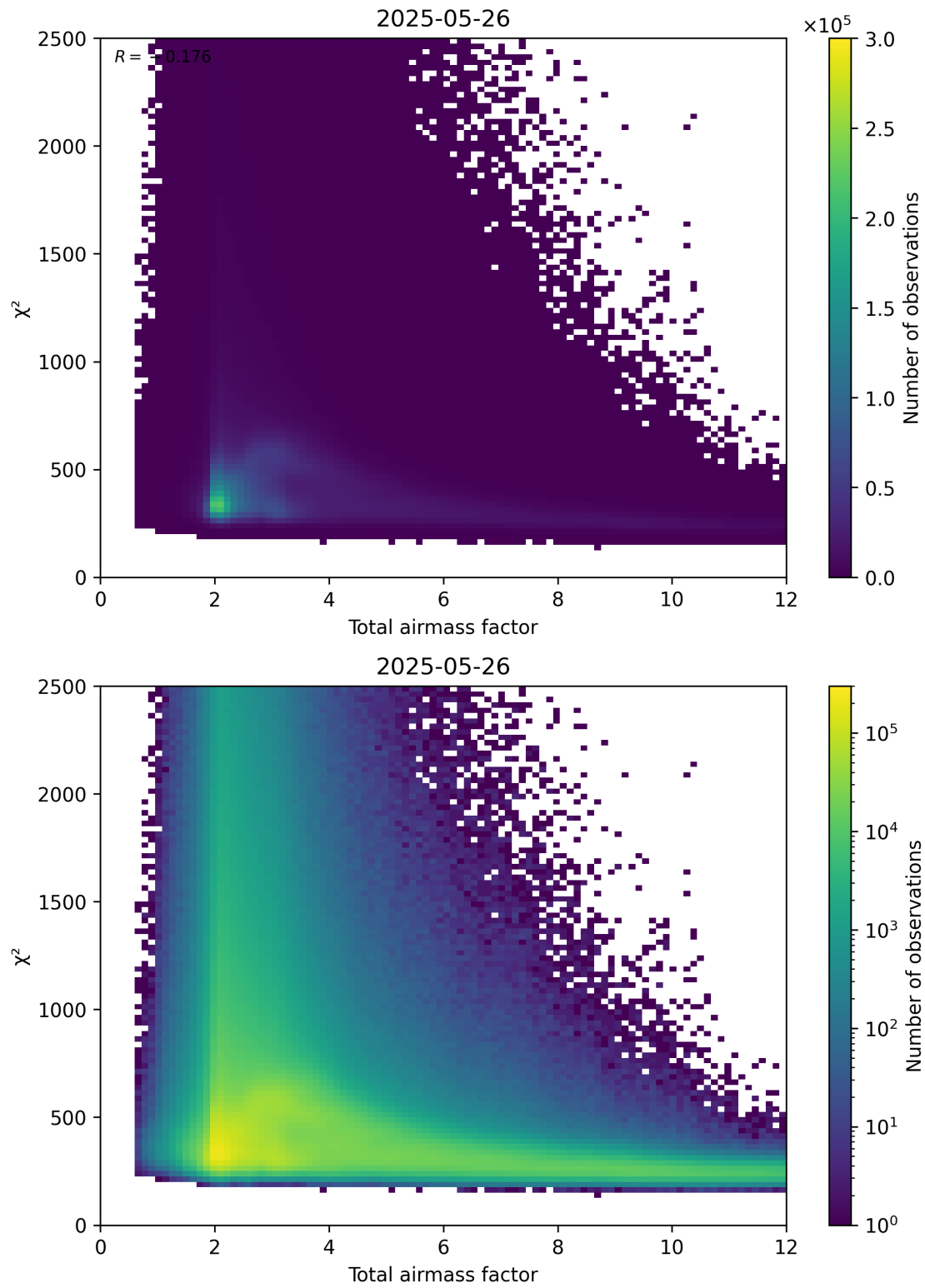
Figure 63: Scatter density plot of “Total airmass factor” against “ \chi^2 ” for 2025-05-26 to 2025-05-27.
