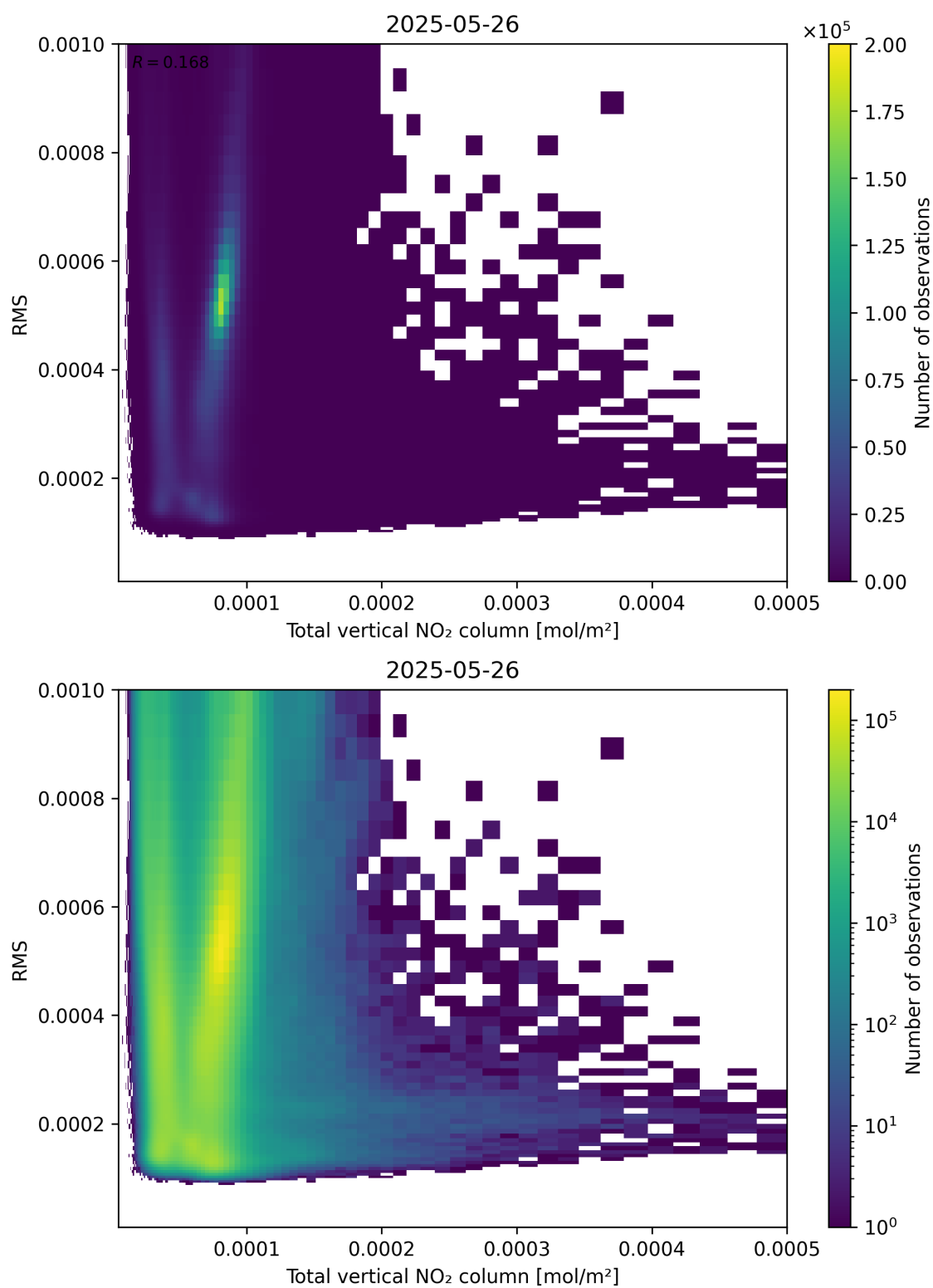
Figure 120: Scatter density plot of “Total vertical NO 2 column” against “RMS” for 2025-05-26 to 2025-05-27.
