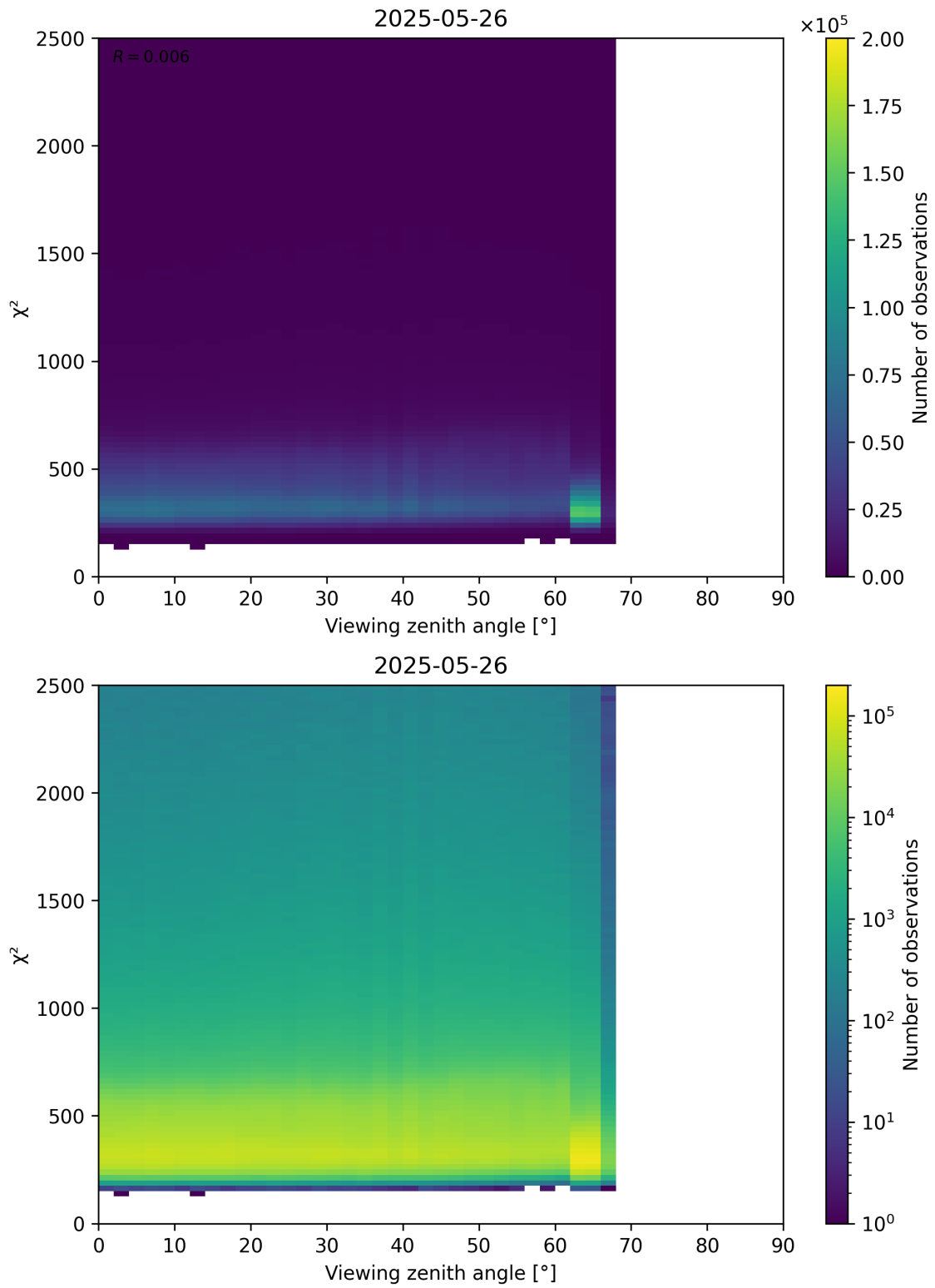
Figure 162: Scatter density plot of “Viewing zenith angle” against “ \chi^2 ” for 2025-05-26 to 2025-05-27.
