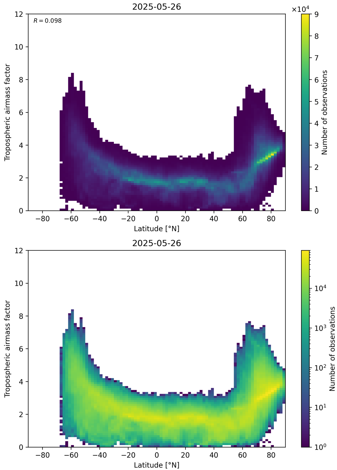
Figure 85: Scatter density plot of “Latitude” against “Tropospheric air mass factor” for 2025-05-26 to 2025-05-27.
