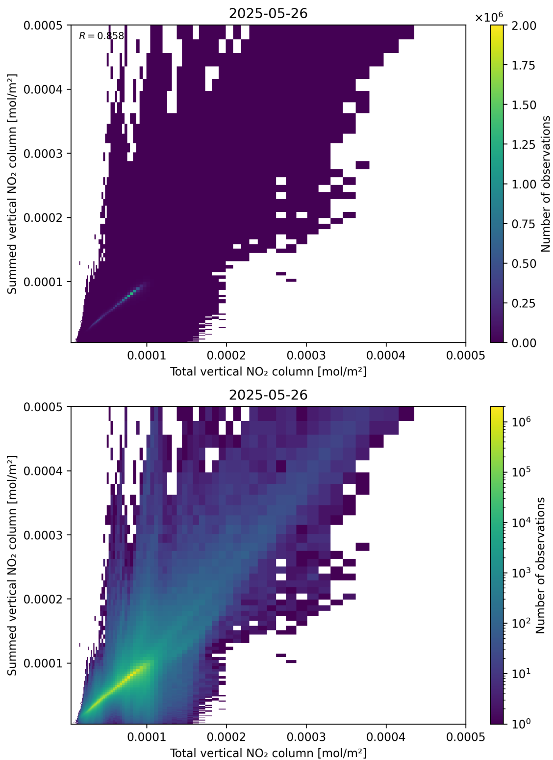
Figure 112: Scatter density plot of “Total vertical NO 2 column” against “Summed vertical NO 2 column” for 2025-05-26 to 2025-05-27.
