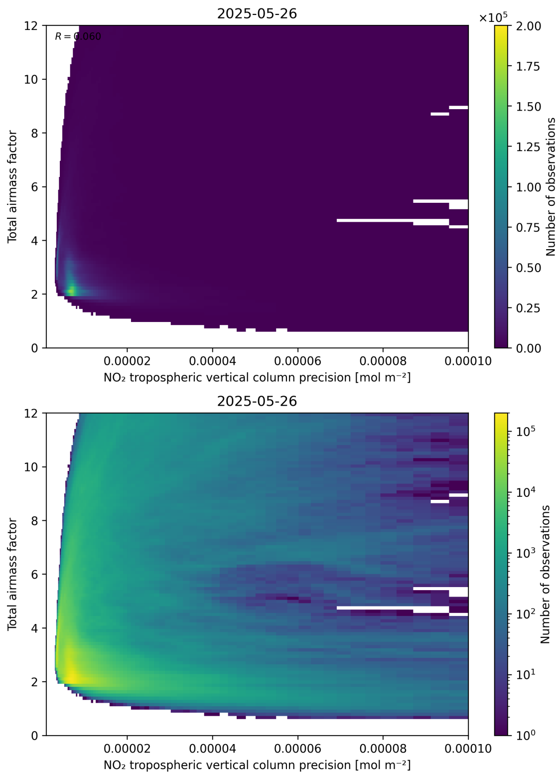
Figure 132: Scatter density plot of “NO 2 tropospheric vertical column precision” against “Total air mass factor” for 2025-05-26 to 2025-05-27.
