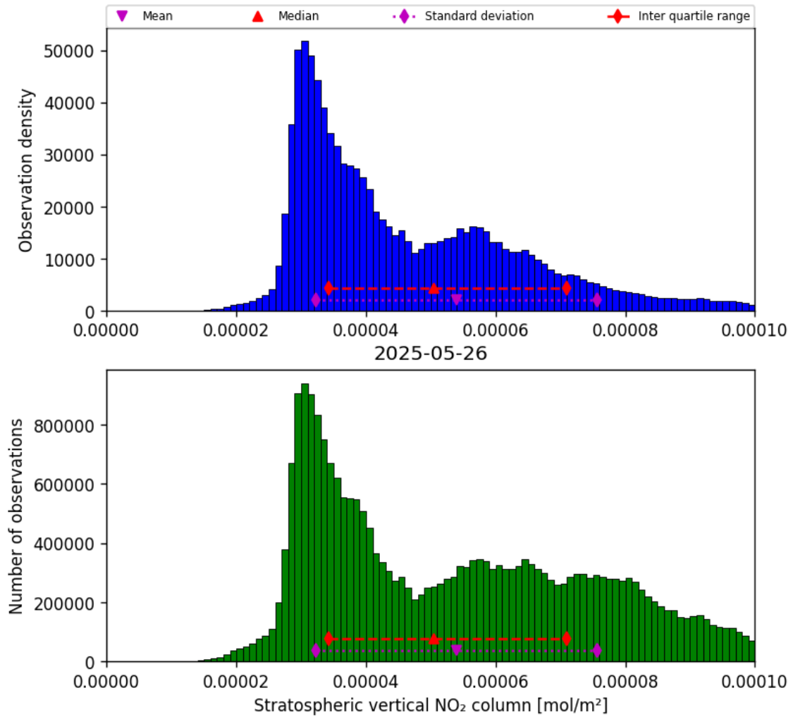
Figure 36: Histogram of “Stratospheric vertical NO 2 column” for 2025-05-26 to 2025-05-27
