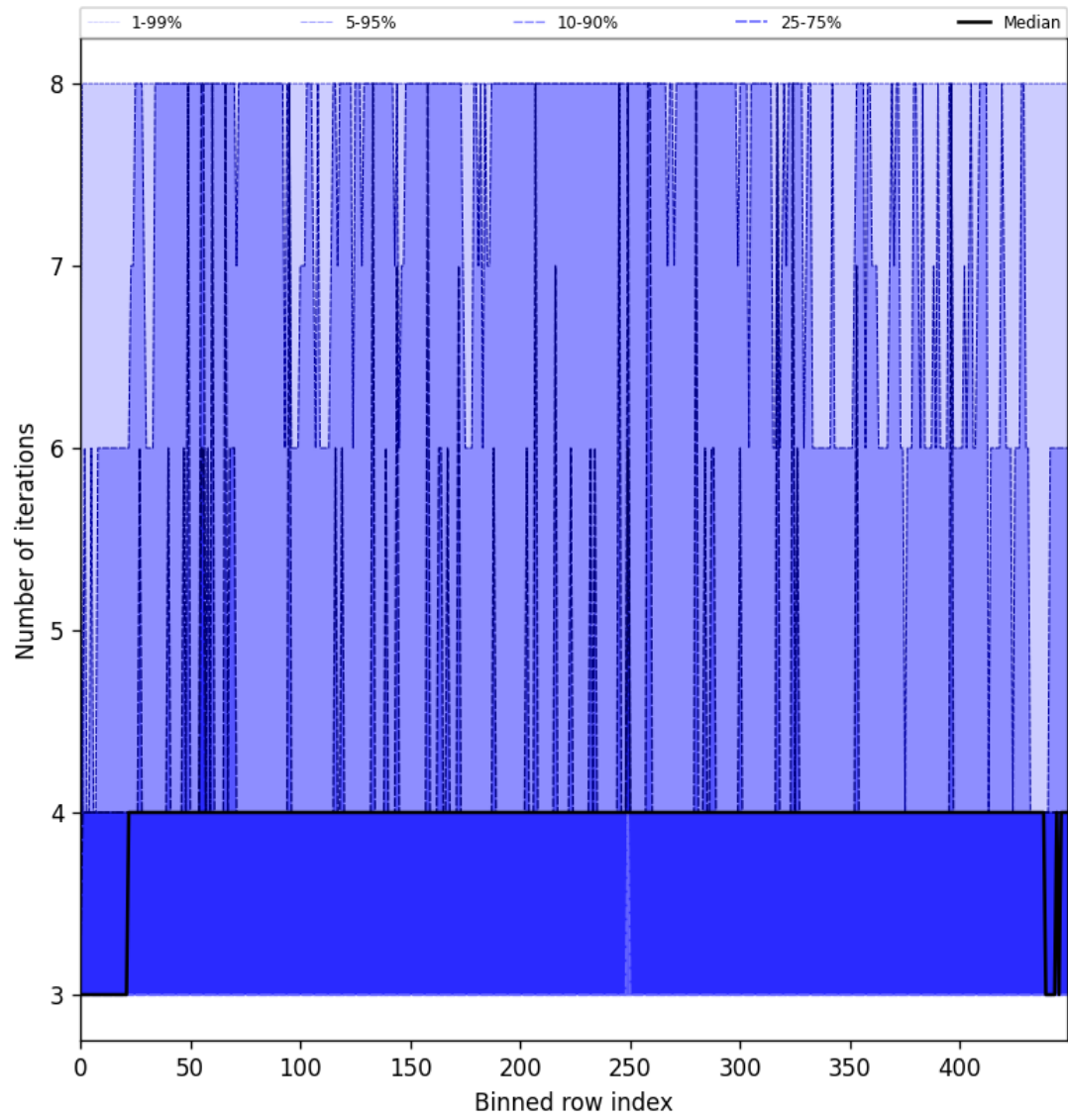
Figure 51: Along track statistics of “Number of iterations” for 2025-05-26 to 2025-05-27
