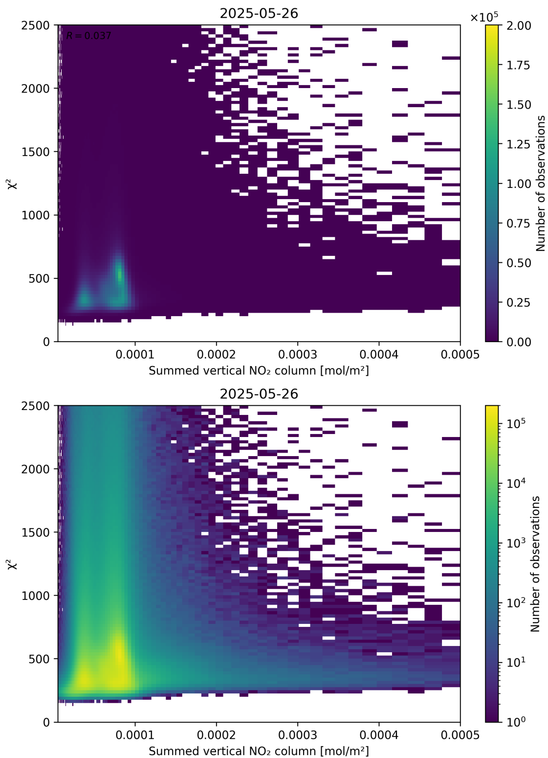
Figure 104: Scatter density plot of “Summed vertical NO 2 column” against “ \chi^2 ” for 2025-05-26 to 2025-05-27.
