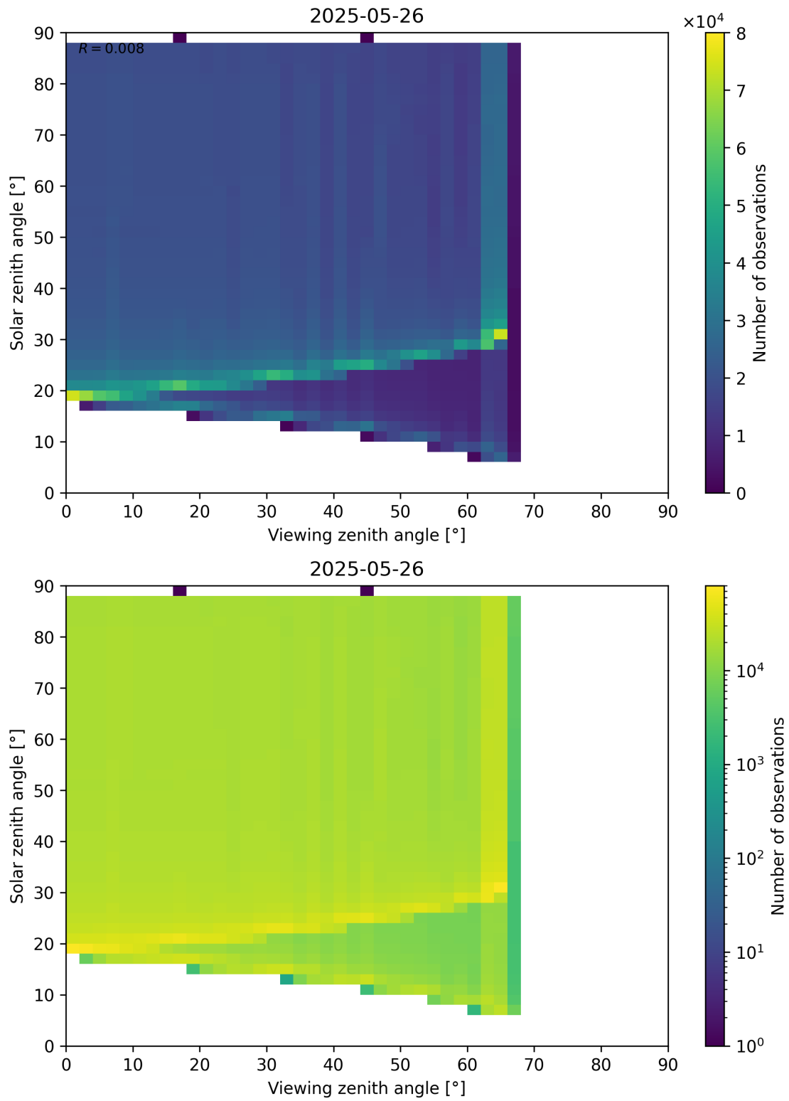
Figure 172: Scatter density plot of “Viewing zenith angle” against “Solar zenith angle” for 2025-05-26 to 2025-05-27.
