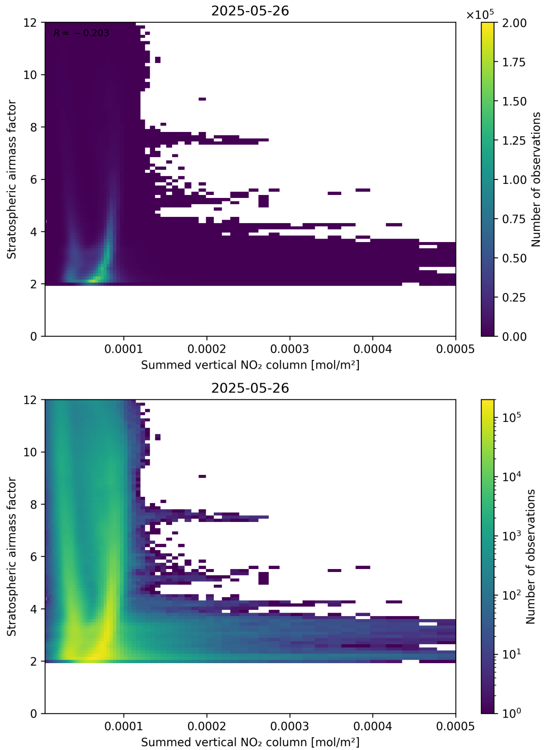
Figure 103: Scatter density plot of “Summed vertical NO 2 column” against “Stratospheric air mass factor” for 2025-05-26 to 2025-05-27.
