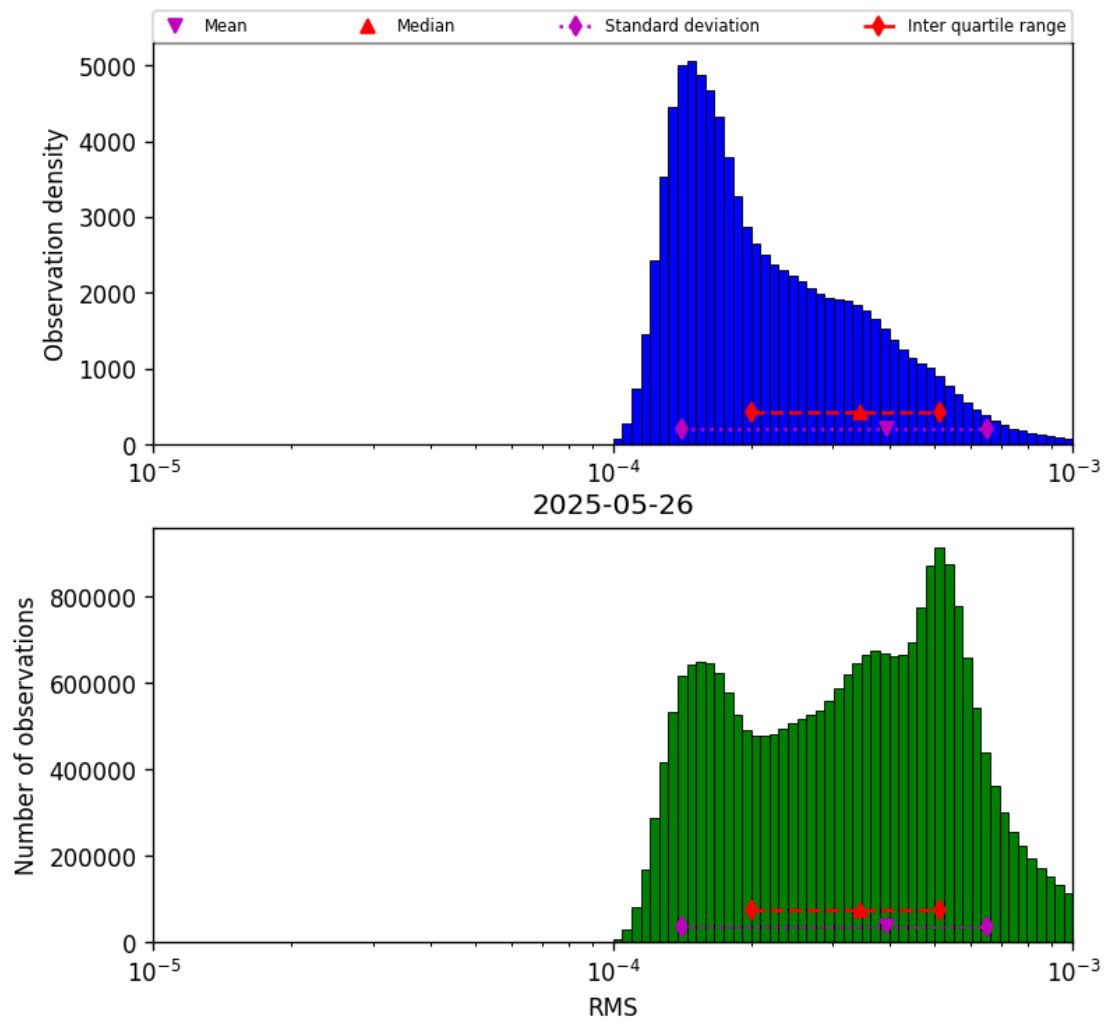
Figure 43: Histogram of “RMS” for 2025-05-26 to 2025-05-27
