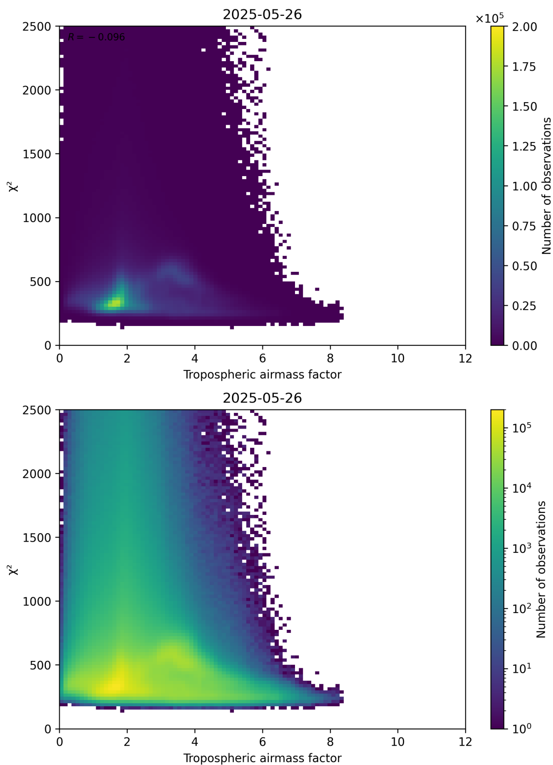
Figure 73: Scatter density plot of “Tropospheric airmass factor” against “ \chi^2 ” for 2025-05-26 to 2025-05-27.
