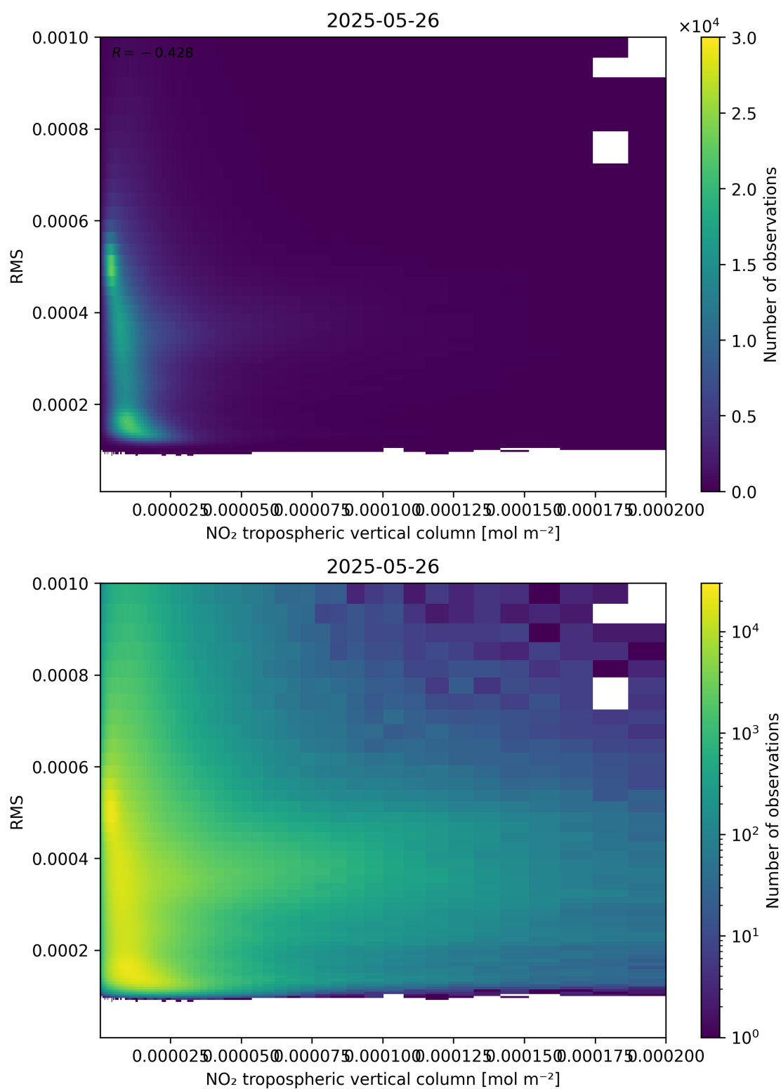
Figure 142: Scatter density plot of “NO 2 tropospheric vertical column” against “RMS” for 2025-05-26 to 2025-05-27.
