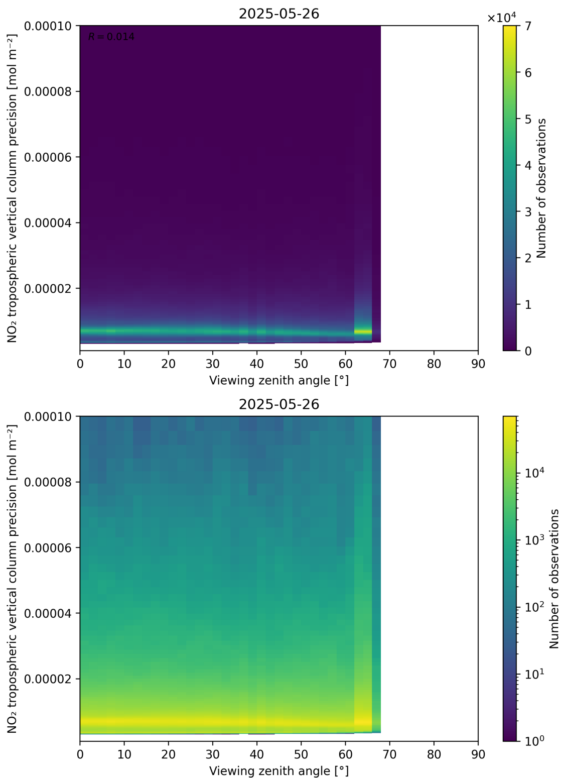
Figure 170: Scatter density plot of “Viewing zenith angle” against “NO 2 tropospheric vertical column precision” for 2025-05-26 to 2025-05-27.
