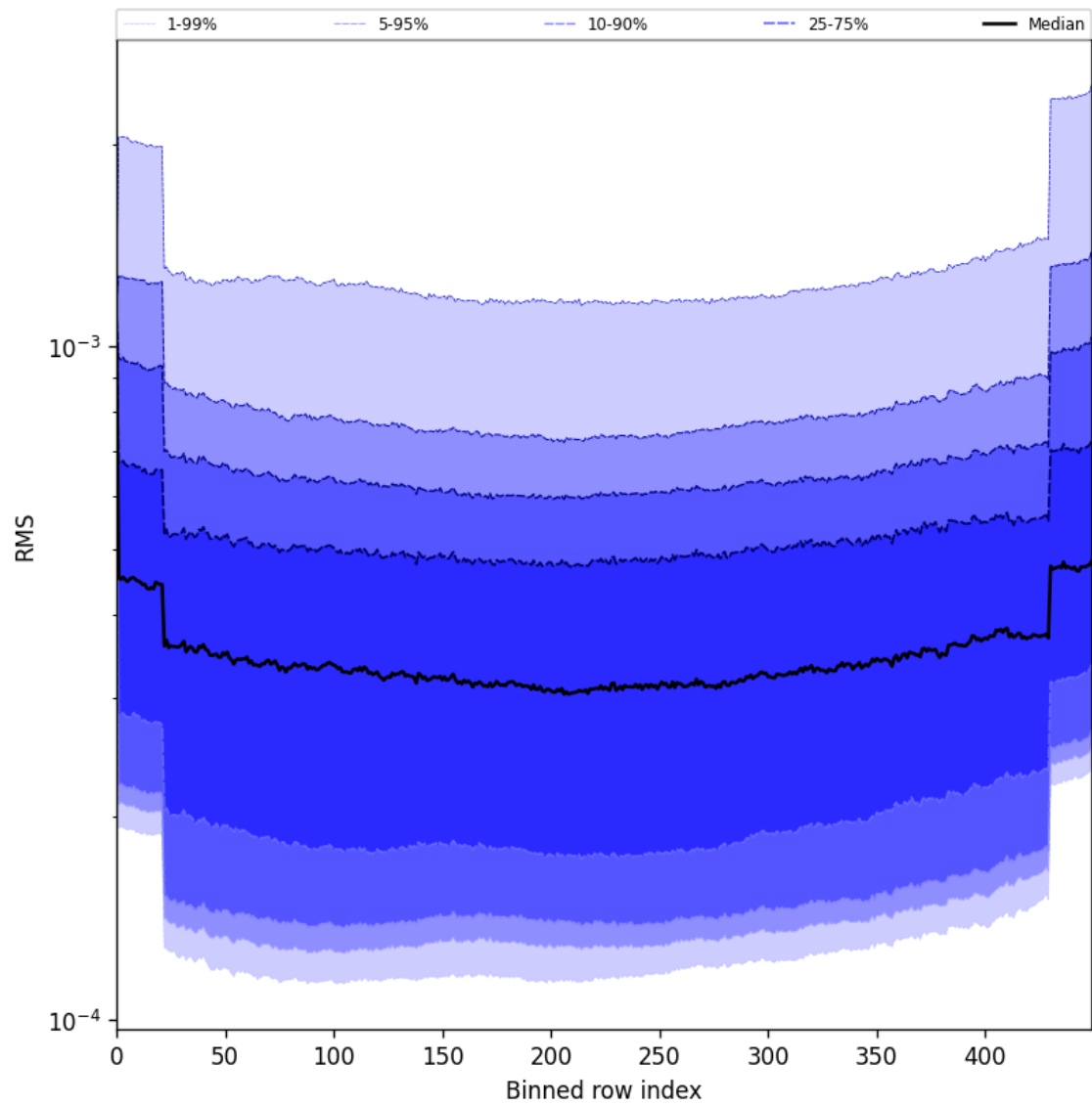
Figure 60: Along track statistics of “RMS” for 2025-05-26 to 2025-05-27
