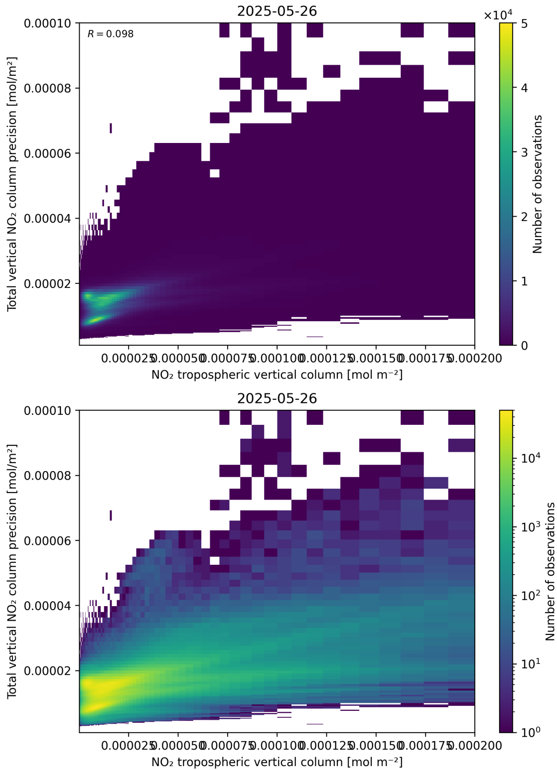
Figure 129: Scatter density plot of “NO 2 tropospheric vertical column” against “Total vertical NO 2 column precision” for 2025-05-26 to 2025-05-27.
