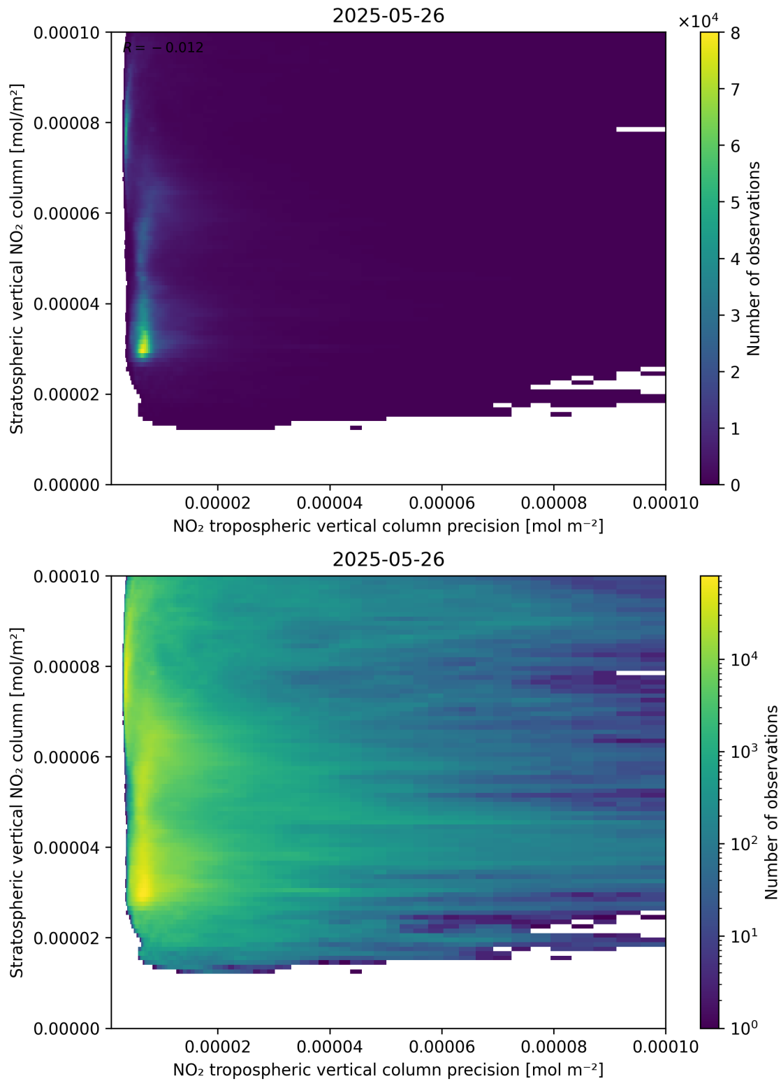
Figure 135: Scatter density plot of “NO 2 tropospheric vertical column precision” against “Stratospheric vertical NO 2 column” for 2025-05-26 to 2025-05-27.
