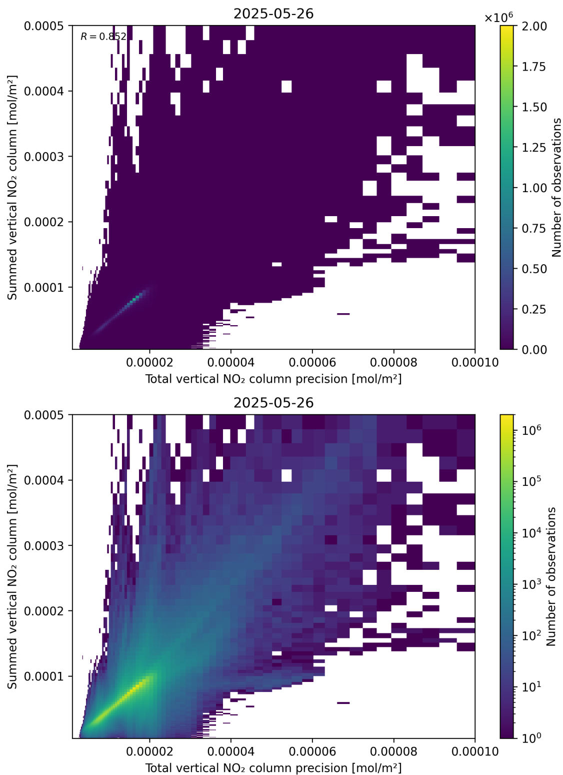
Figure 117: Scatter density plot of “Total vertical NO 2 column precision” against “Summed vertical NO 2 column” for 2025-05-26 to 2025-05-27.
