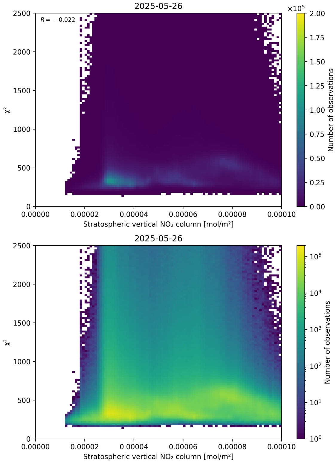
Figure 97: Scatter density plot of “Stratospheric vertical NO 2 column” against “ \chi^2 ” for 2025-05-26 to 2025-05-27.
