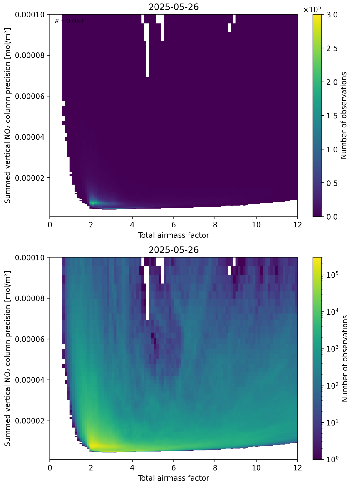
Figure 66: Scatter density plot of “Total airmass factor” against “Summed vertical NO 2 column precision” for 2025-05-26 to 2025-05-27.
