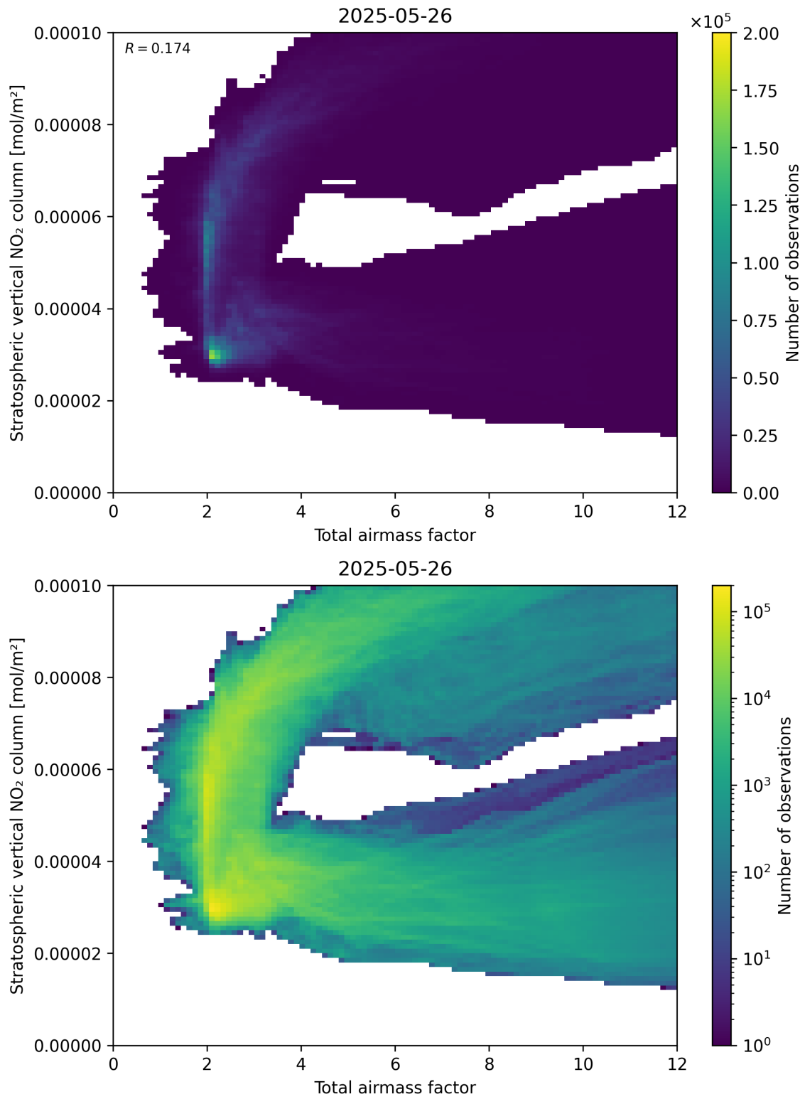
Figure 64: Scatter density plot of “Total airmass factor” against “Stratospheric vertical \text{NO}_2 column” for 2025-05-26 to 2025-05-27.
