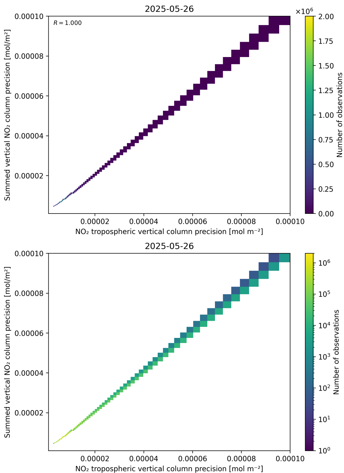
Figure 137: Scatter density plot of “NO 2 tropospheric vertical column precision” against “Summed vertical NO 2 column precision” for 2025-05-26 to 2025-05-27.
