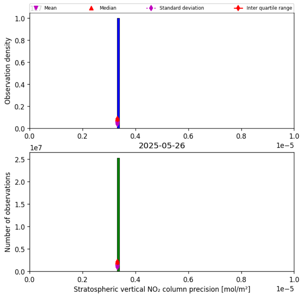
Figure 37: Histogram of “Stratospheric vertical NO 2 column precision” for 2025-05-26 to 2025-05-27
