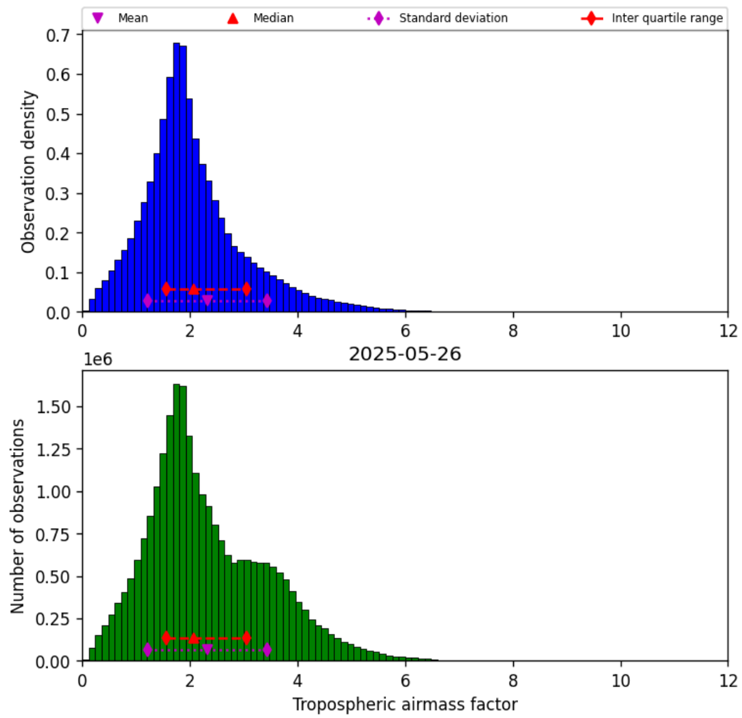
Figure 31: Histogram of “Tropospheric airmass factor” for 2025-05-26 to 2025-05-27
