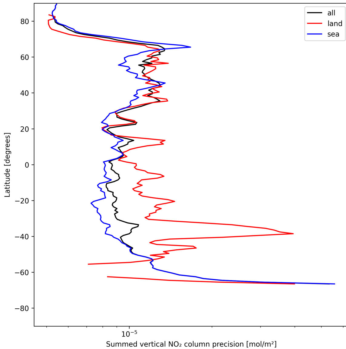
Figure 24: Zonal average of “Summed vertical NO 2 column precision” for 2025-05-26 to 2025-05-27.
