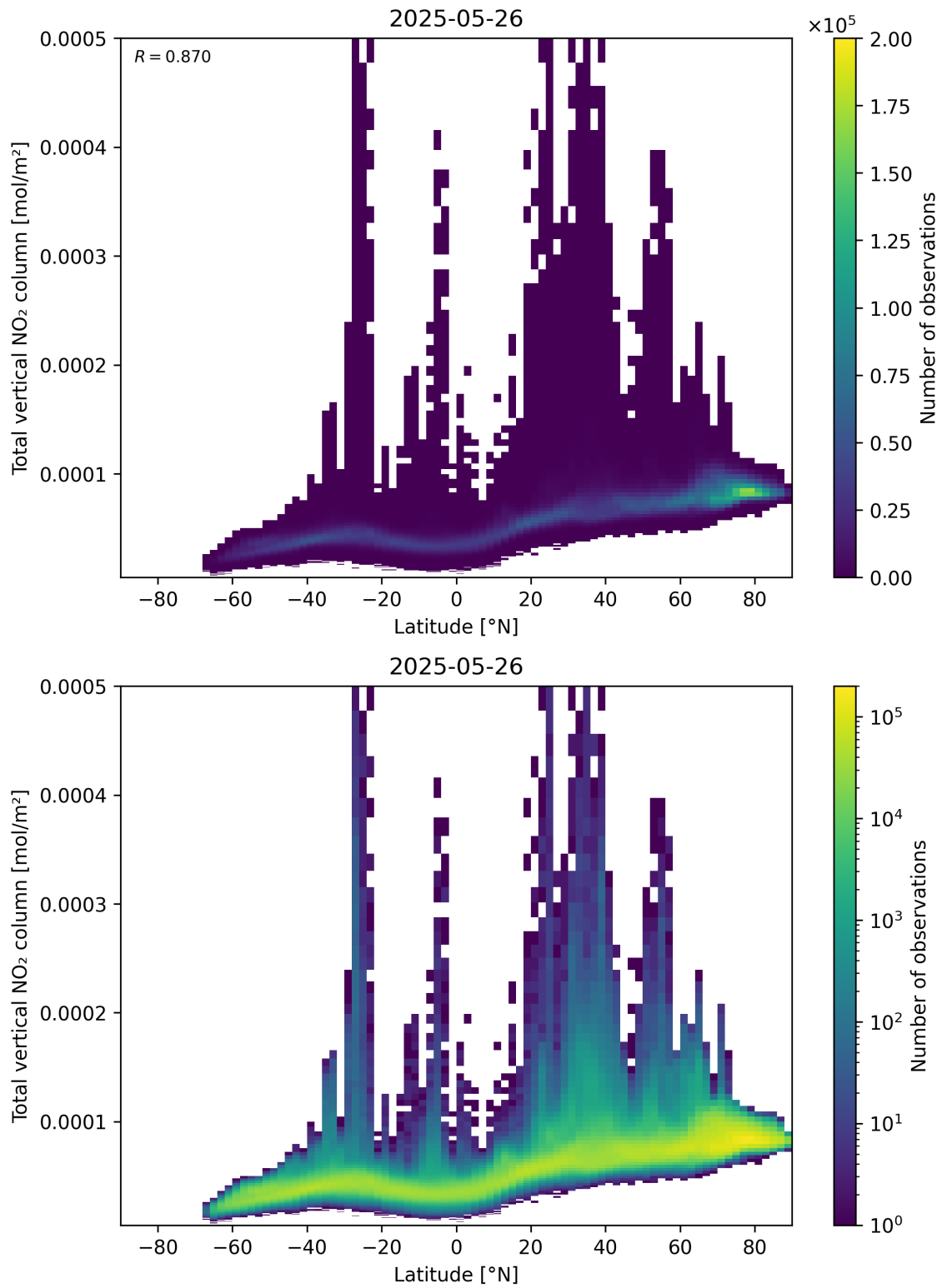
Figure 90: Scatter density plot of “Latitude” against “Total vertical NO 2 column” for 2025-05-26 to 2025-05-27.
