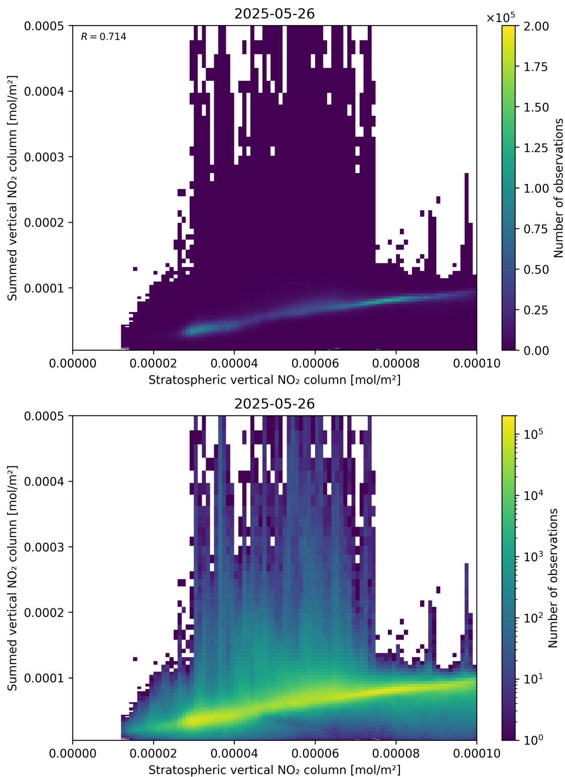
Figure 98: Scatter density plot of “Stratospheric vertical NO 2 column” against “Summed vertical NO 2 column” for 2025-05-26 to 2025-05-27.
