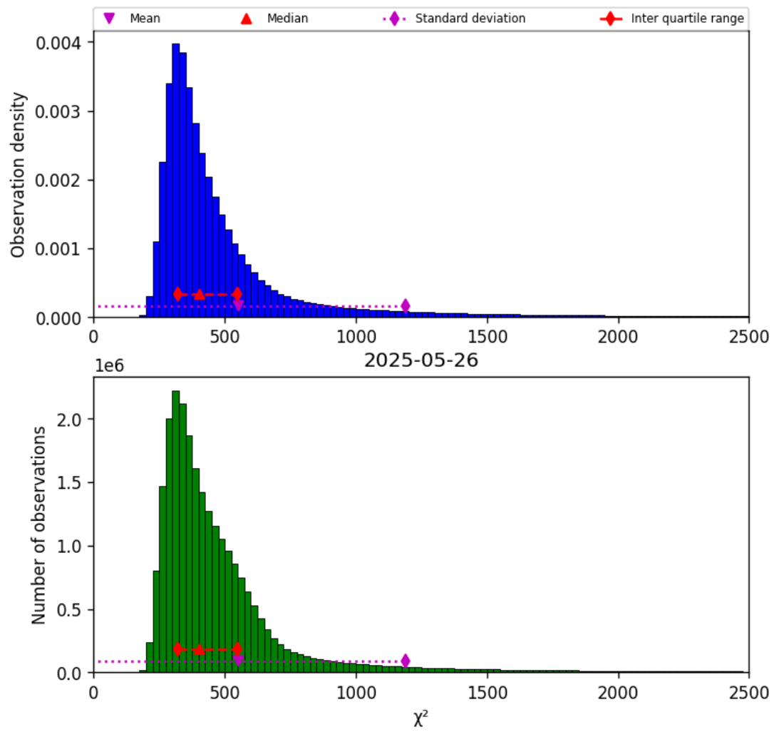
Figure 42: Histogram of “ \chi^2 ” for 2025-05-26 to 2025-05-27
