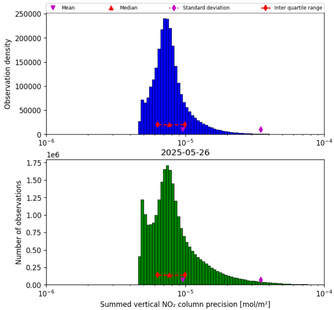
Figure 41: Histogram of “Summed vertical NO 2 column precision” for 2025-05-26 to 2025-05-27
