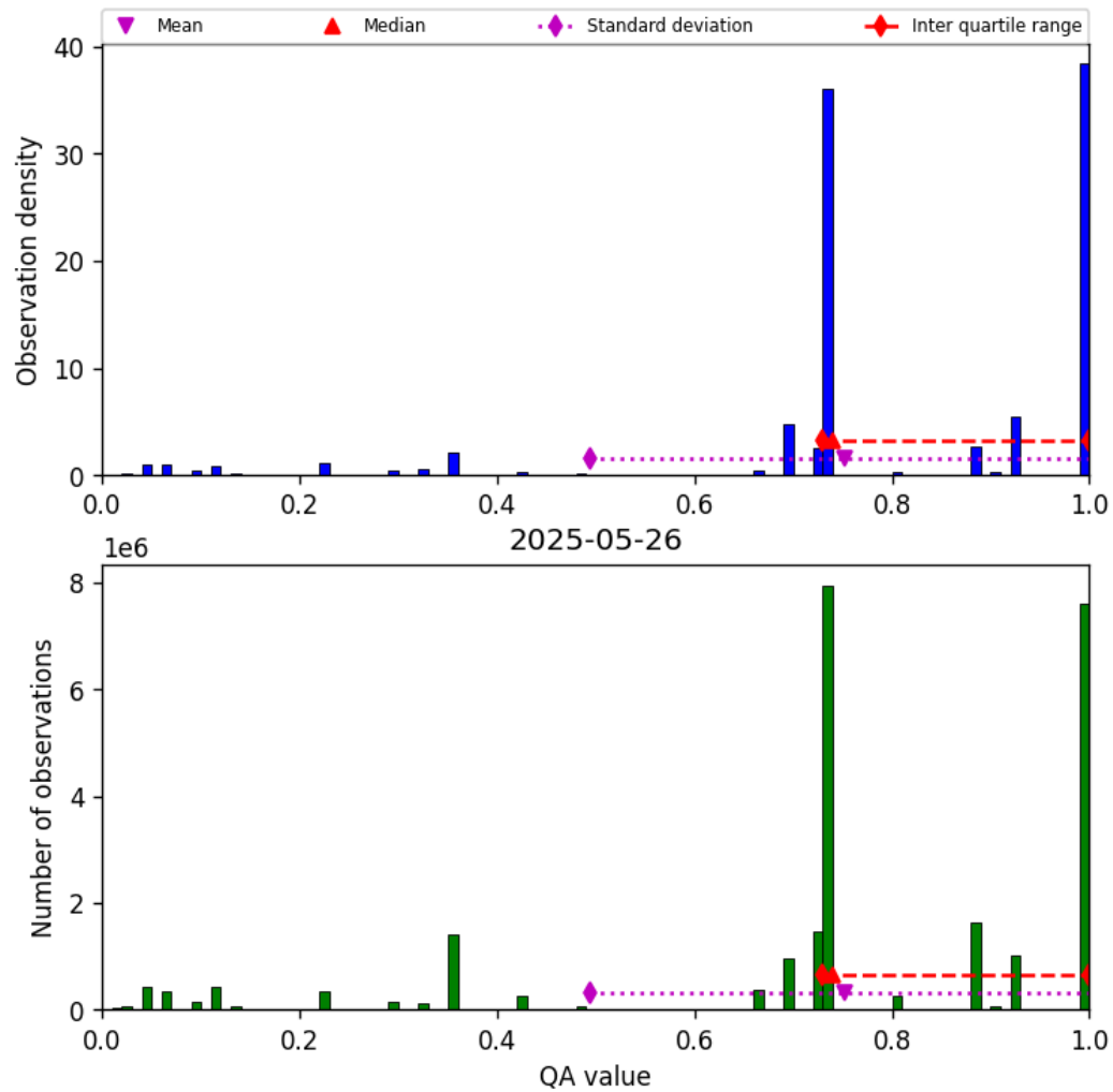
Figure 28: Histogram of “QA value” for 2025-05-26 to 2025-05-27
