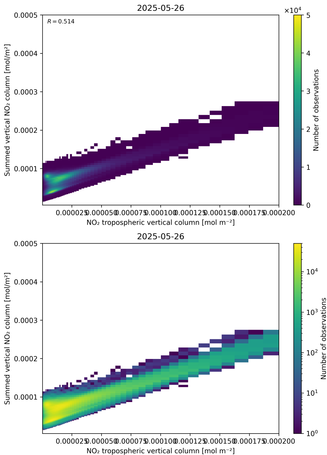
Figure 126: Scatter density plot of “NO 2 tropospheric vertical column” against “Summed vertical NO 2 column” for 2025-05-26 to 2025-05-27.
