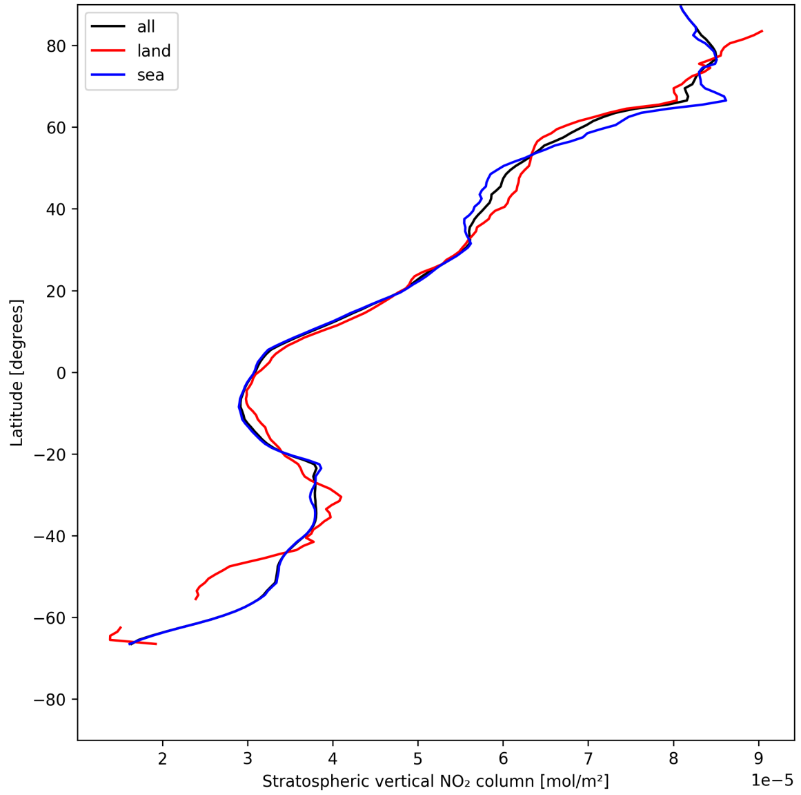
Figure 19: Zonal average of “Stratospheric vertical NO 2 column” for 2025-05-26 to 2025-05-27.
