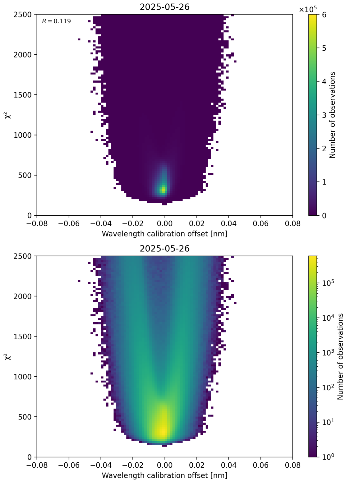
Figure 175: Scatter density plot of “Wavelength calibration offset” against “ \chi^2 ” for 2025-05-26 to 2025-05-27.
