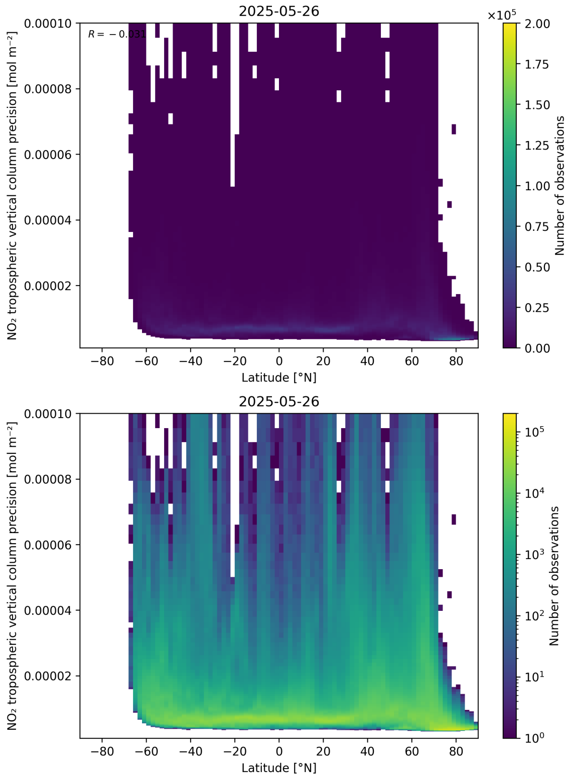
Figure 93: Scatter density plot of “Latitude” against “NO 2 tropospheric vertical column precision” for 2025-05-26 to 2025-05-27.
