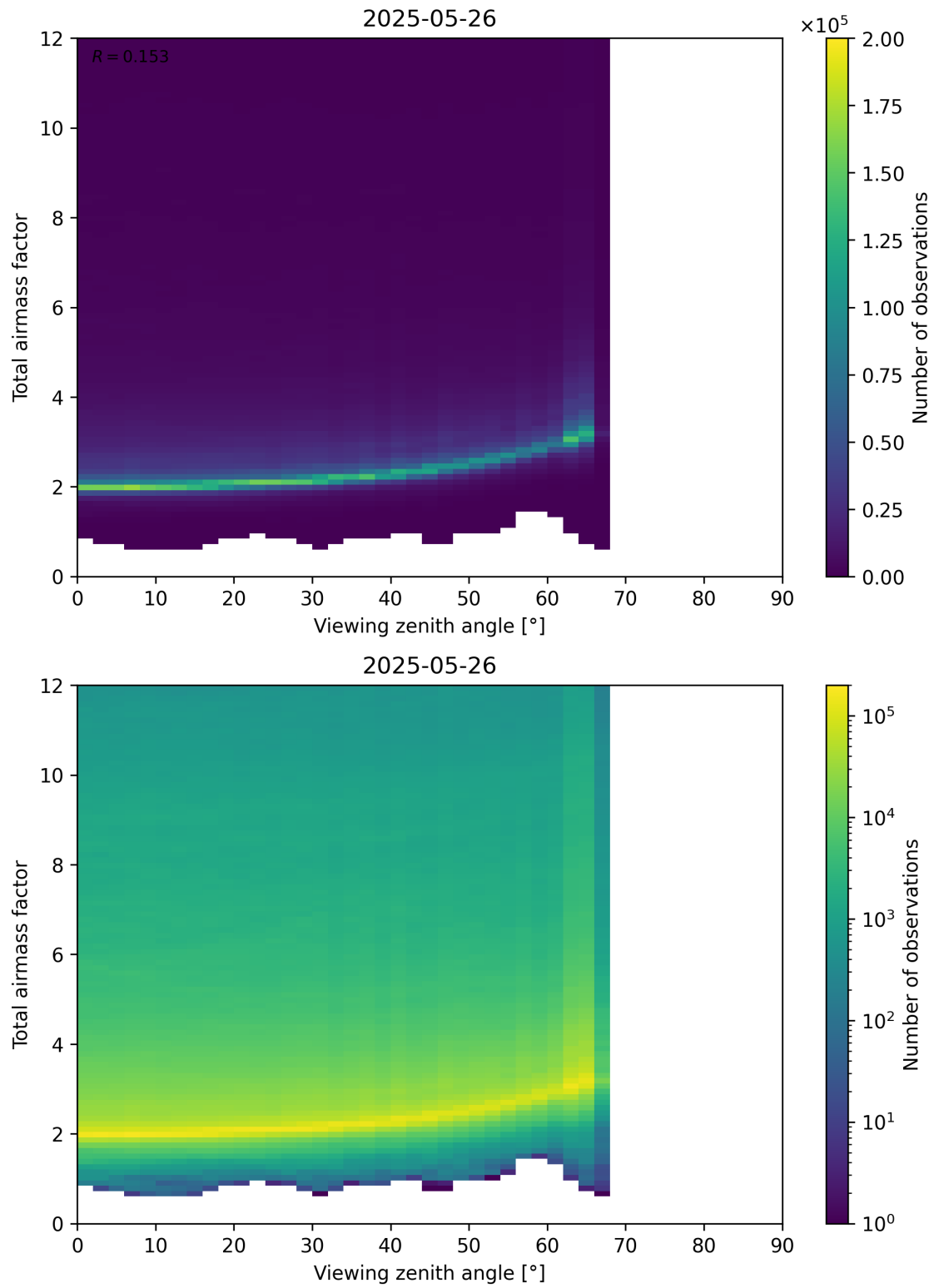
Figure 160: Scatter density plot of “Viewing zenith angle” against “Total airmass factor” for 2025-05-26 to 2025-05-27.
