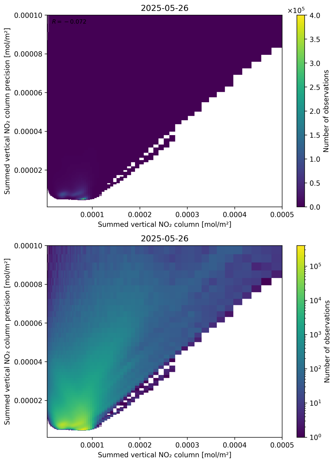
Figure 105: Scatter density plot of “Summed vertical NO 2 column” against “Summed vertical NO 2 column precision” for 2025-05-26 to 2025-05-27.
