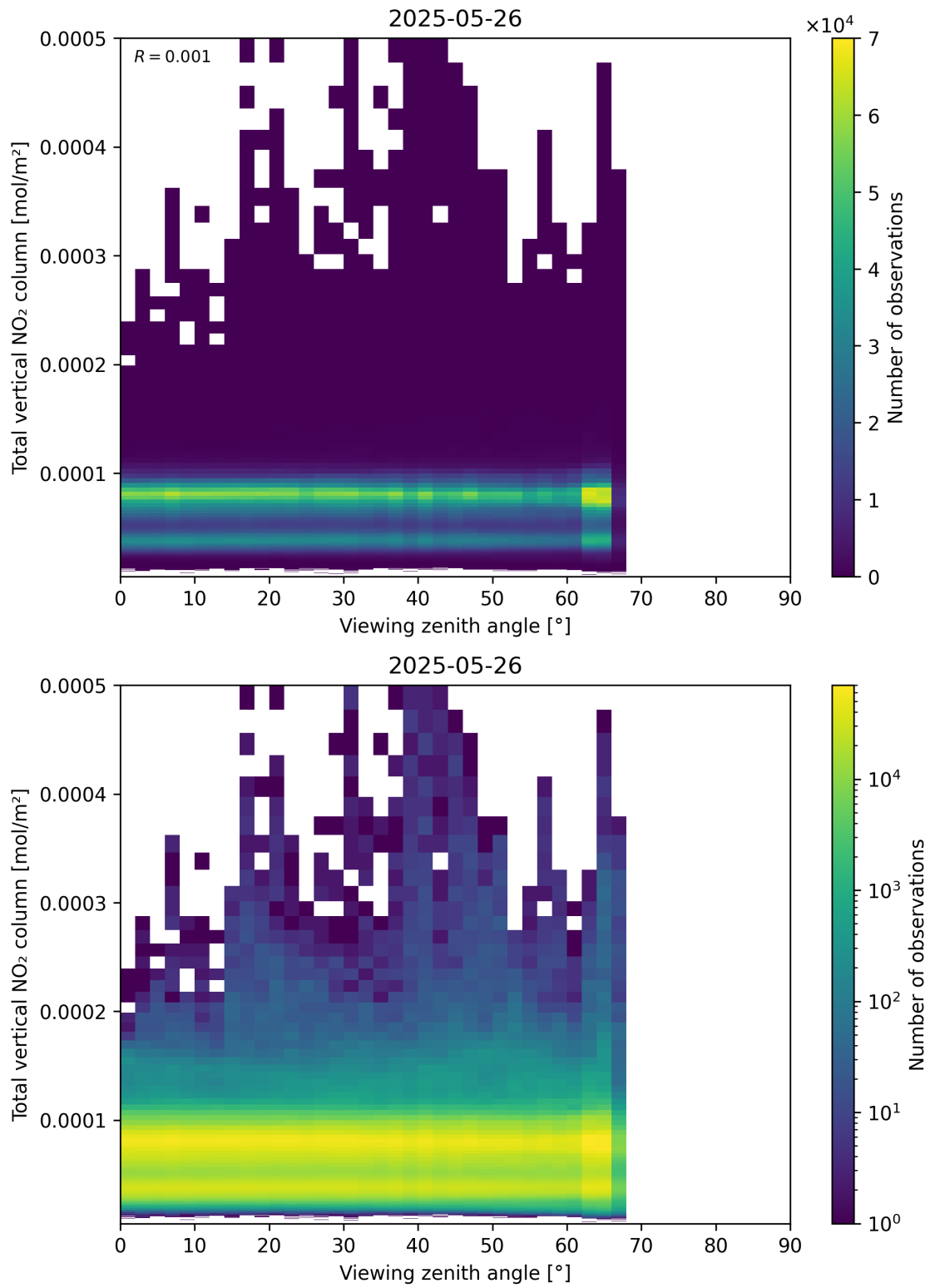
Figure 167: Scatter density plot of “Viewing zenith angle” against “Total vertical NO 2 column” for 2025-05-26 to 2025-05-27.
