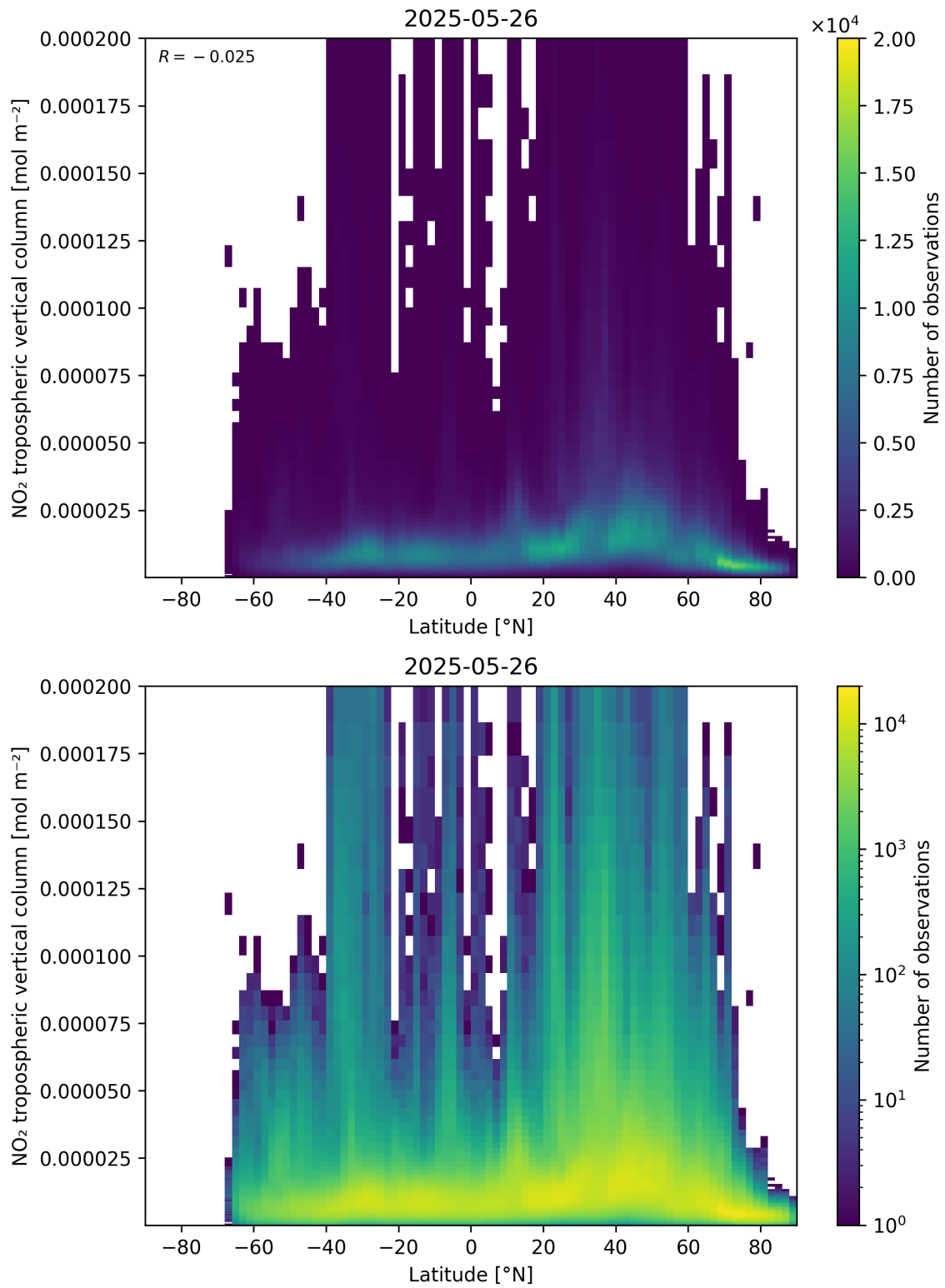
Figure 92: Scatter density plot of “Latitude” against “NO 2 tropospheric vertical column” for 2025-05-26 to 2025-05-27.
