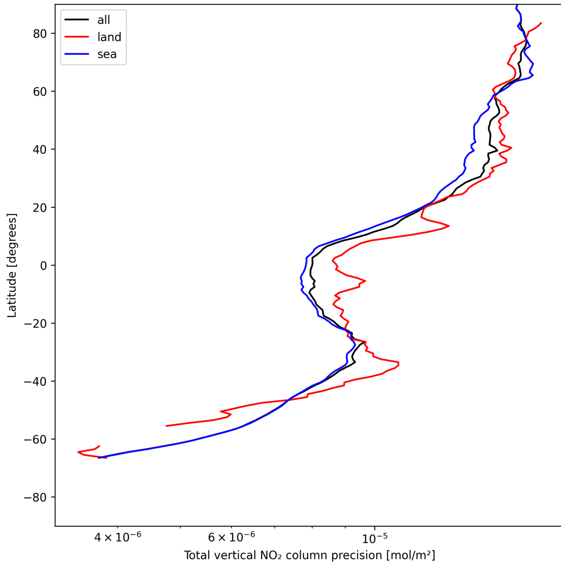
Figure 22: Zonal average of “Total vertical NO 2 column precision” for 2025-05-26 to 2025-05-27.
