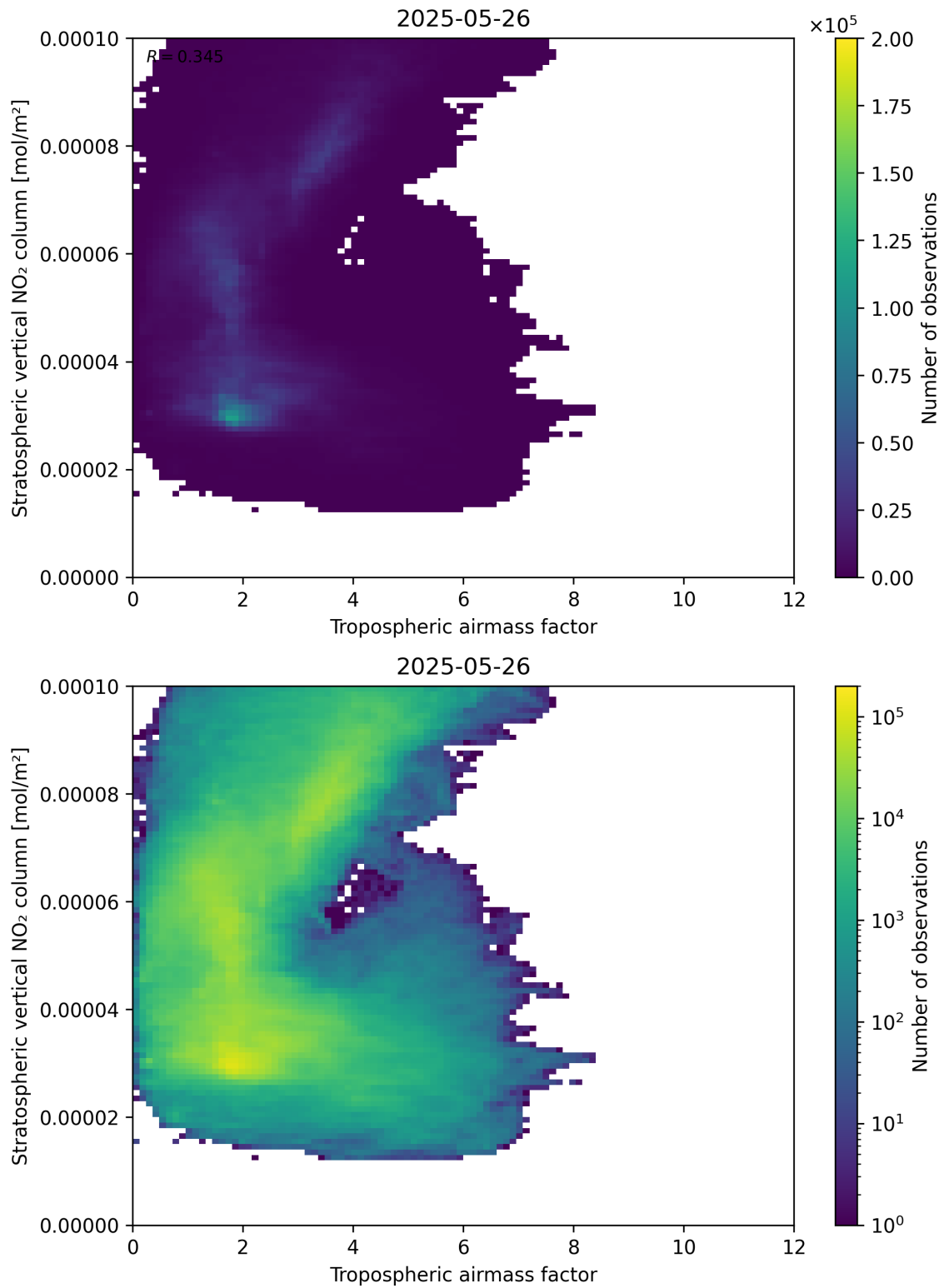
Figure 74: Scatter density plot of “Tropospheric air mass factor” against “Stratospheric vertical NO 2 column” for 2025-05-26 to 2025-05-27.
