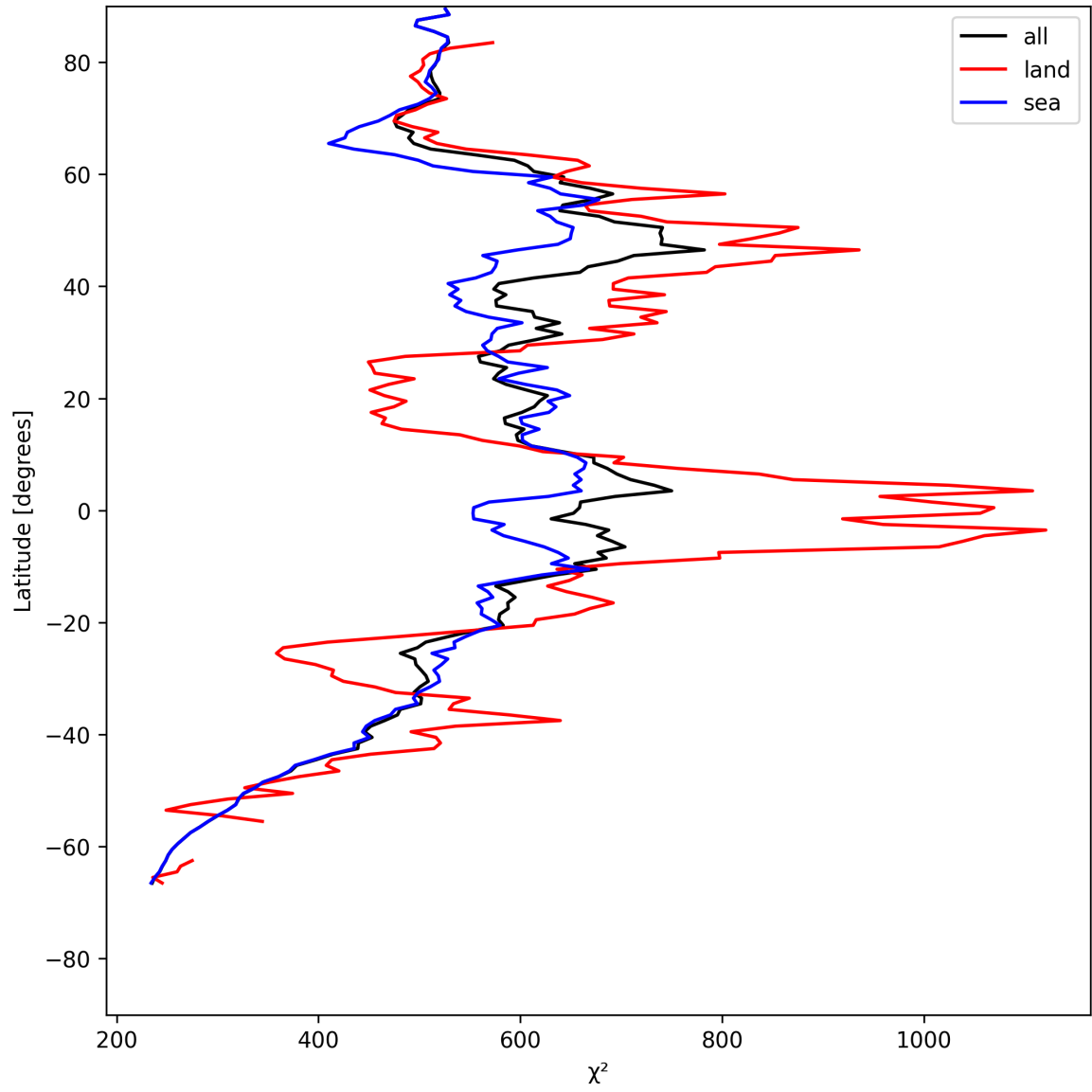
Figure 25: Zonal average of “ \chi^2 ” for 2025-05-26 to 2025-05-27.
