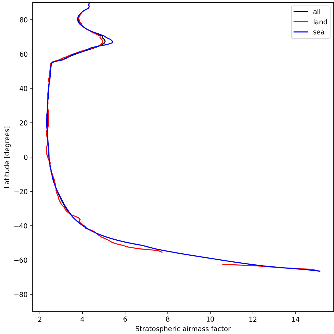
Figure 27: Zonal average of “Stratospheric air mass factor” for 2025-05-26 to 2025-05-27.
