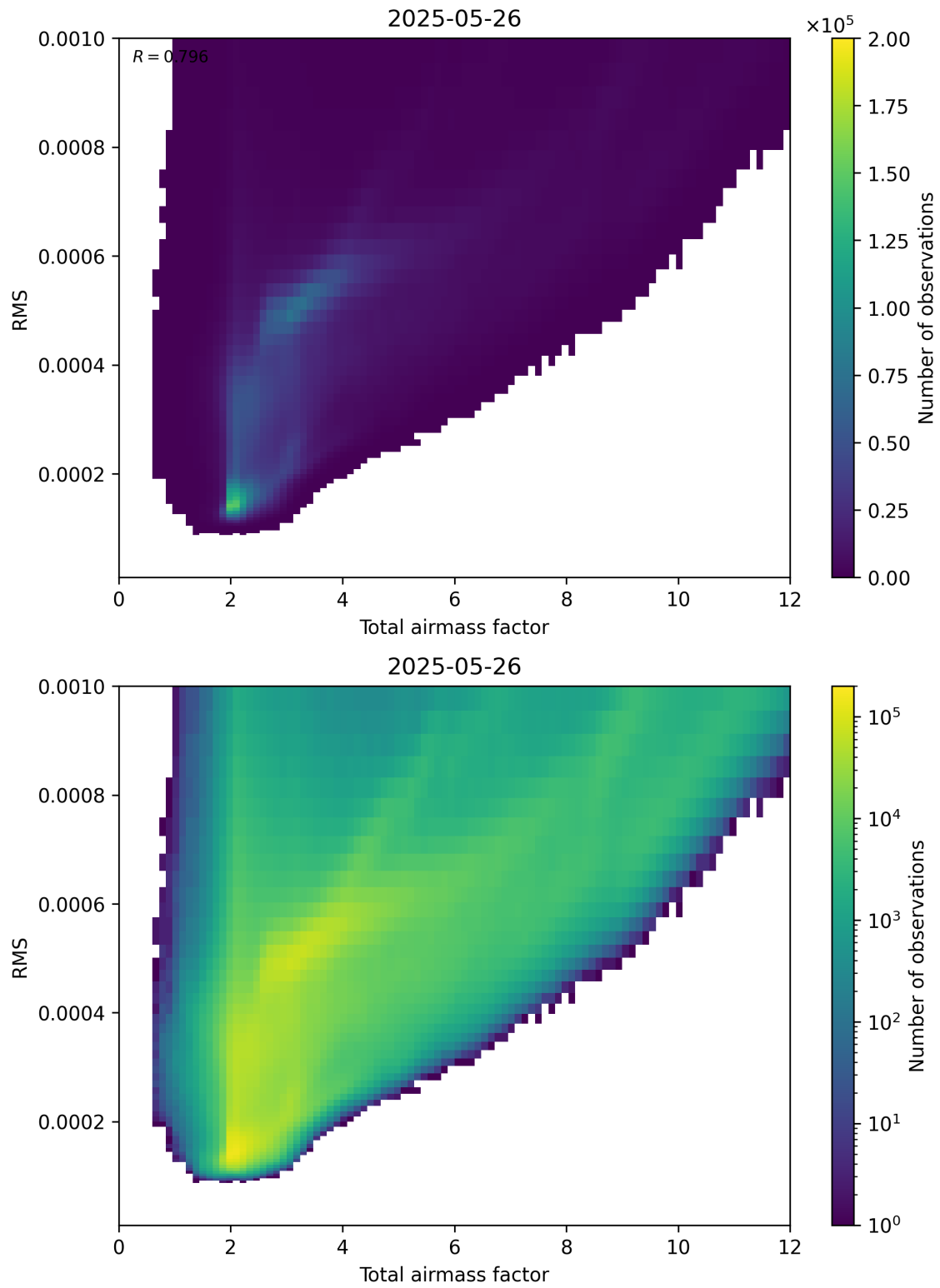
Figure 69: Scatter density plot of “Total airmass factor” against “RMS” for 2025-05-26 to 2025-05-27.
