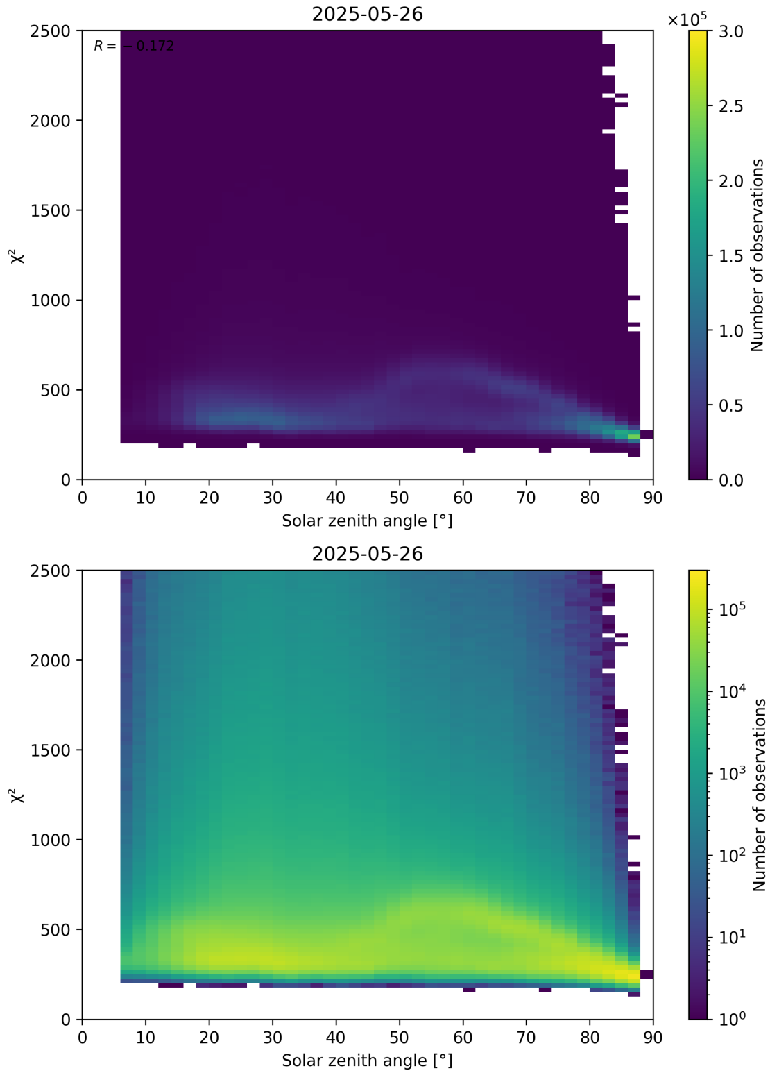
Figure 148: Scatter density plot of “Solar zenith angle” against “ \chi^2 ” for 2025-05-26 to 2025-05-27.
