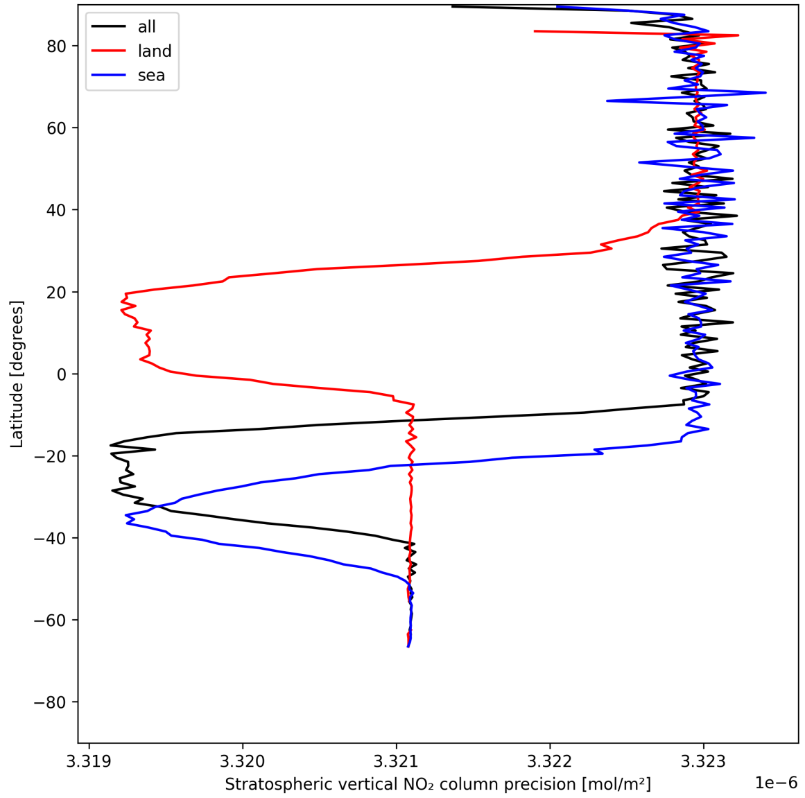
Figure 20: Zonal average of “Stratospheric vertical NO 2 column precision” for 2025-05-26 to 2025-05-27.
