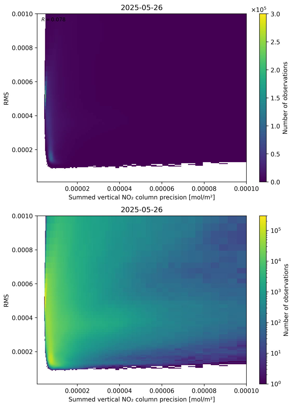
Figure 108: Scatter density plot of “Summed vertical NO 2 column precision” against “RMS” for 2025-05-26 to 2025-05-27.
