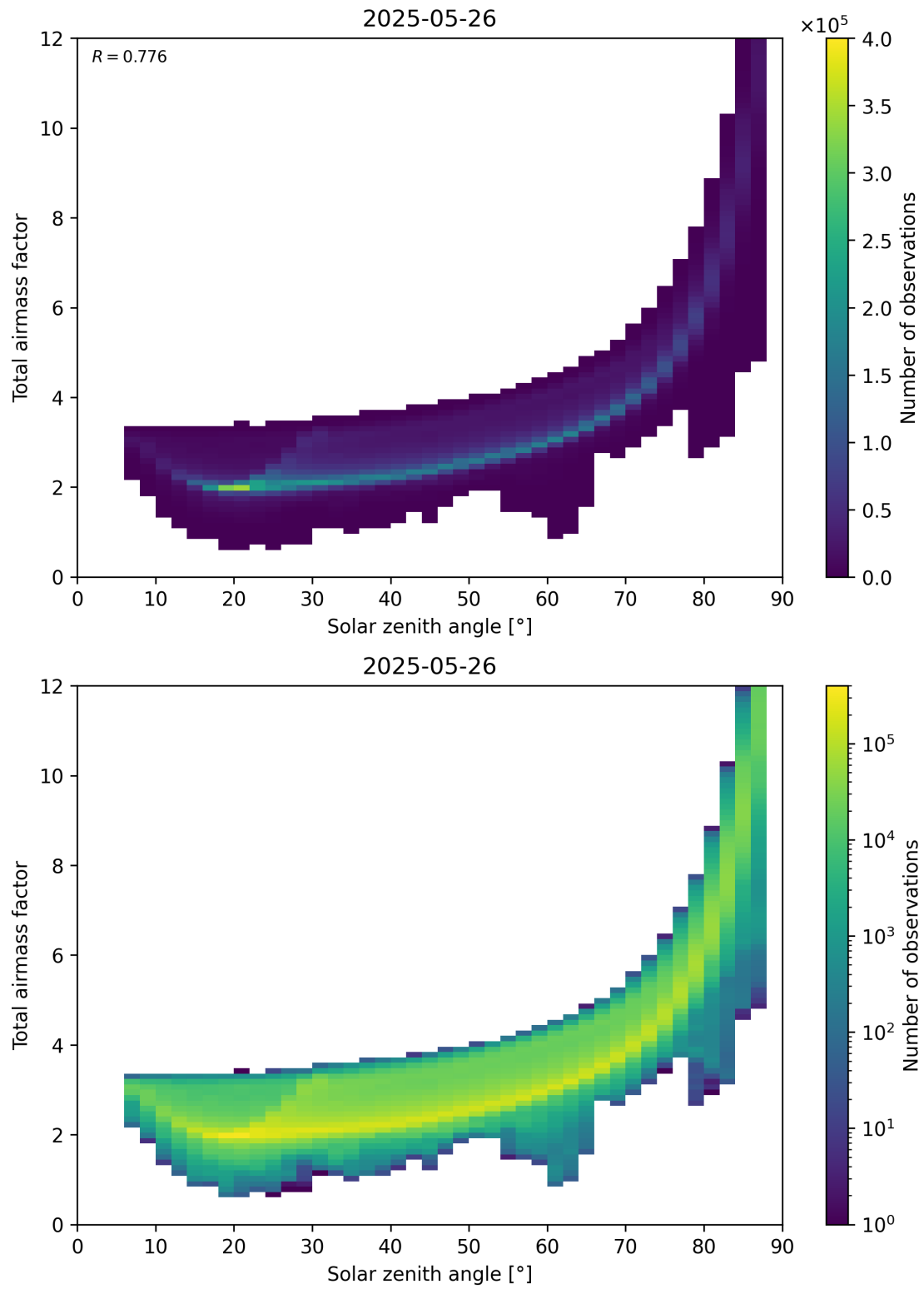
Figure 146: Scatter density plot of “Solar zenith angle” against “Total airmass factor” for 2025-05-26 to 2025-05-27.
