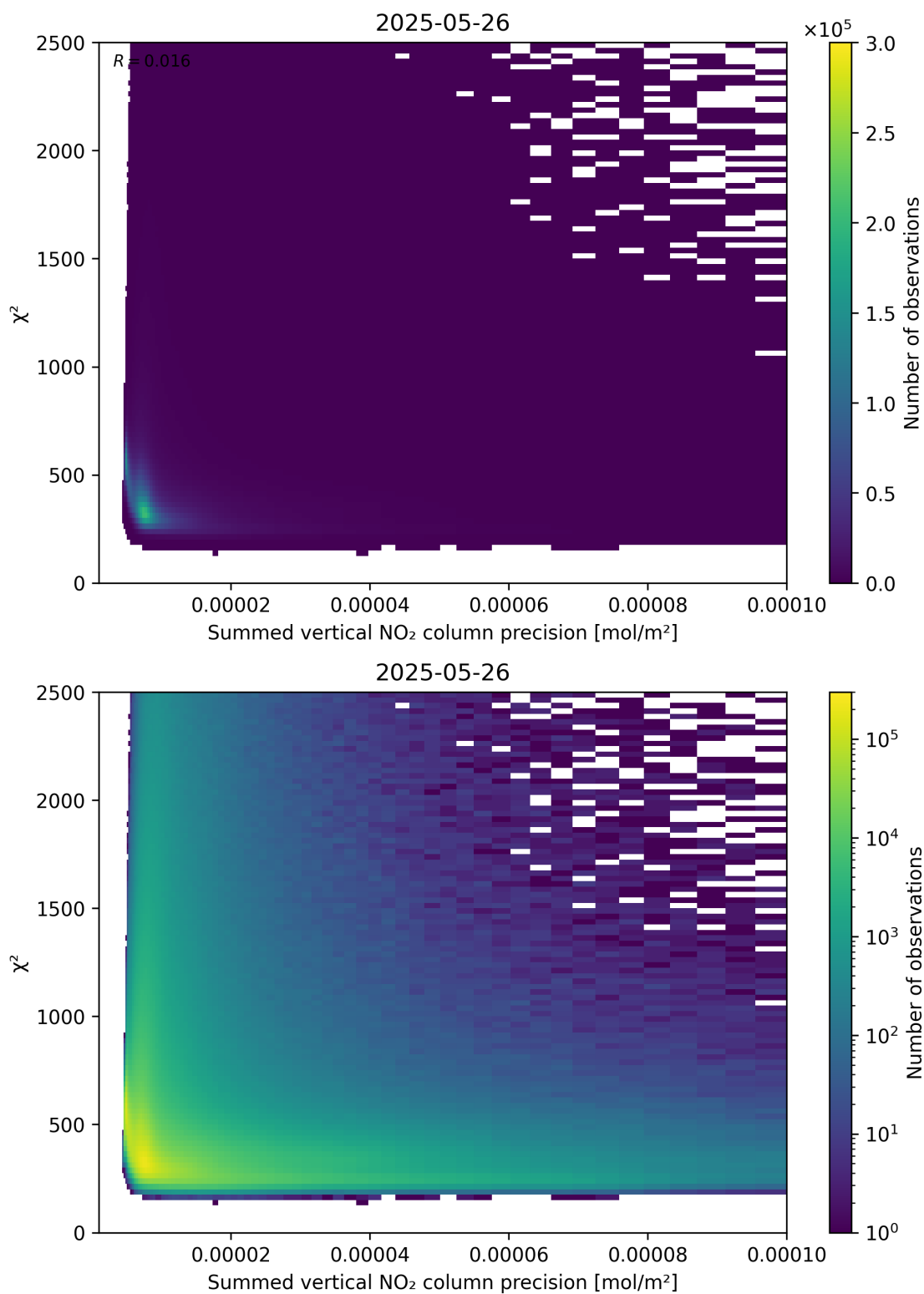
Figure 107: Scatter density plot of “Summed vertical NO 2 column precision” against “ \chi^2 ” for 2025-05-26 to 2025-05-27.
