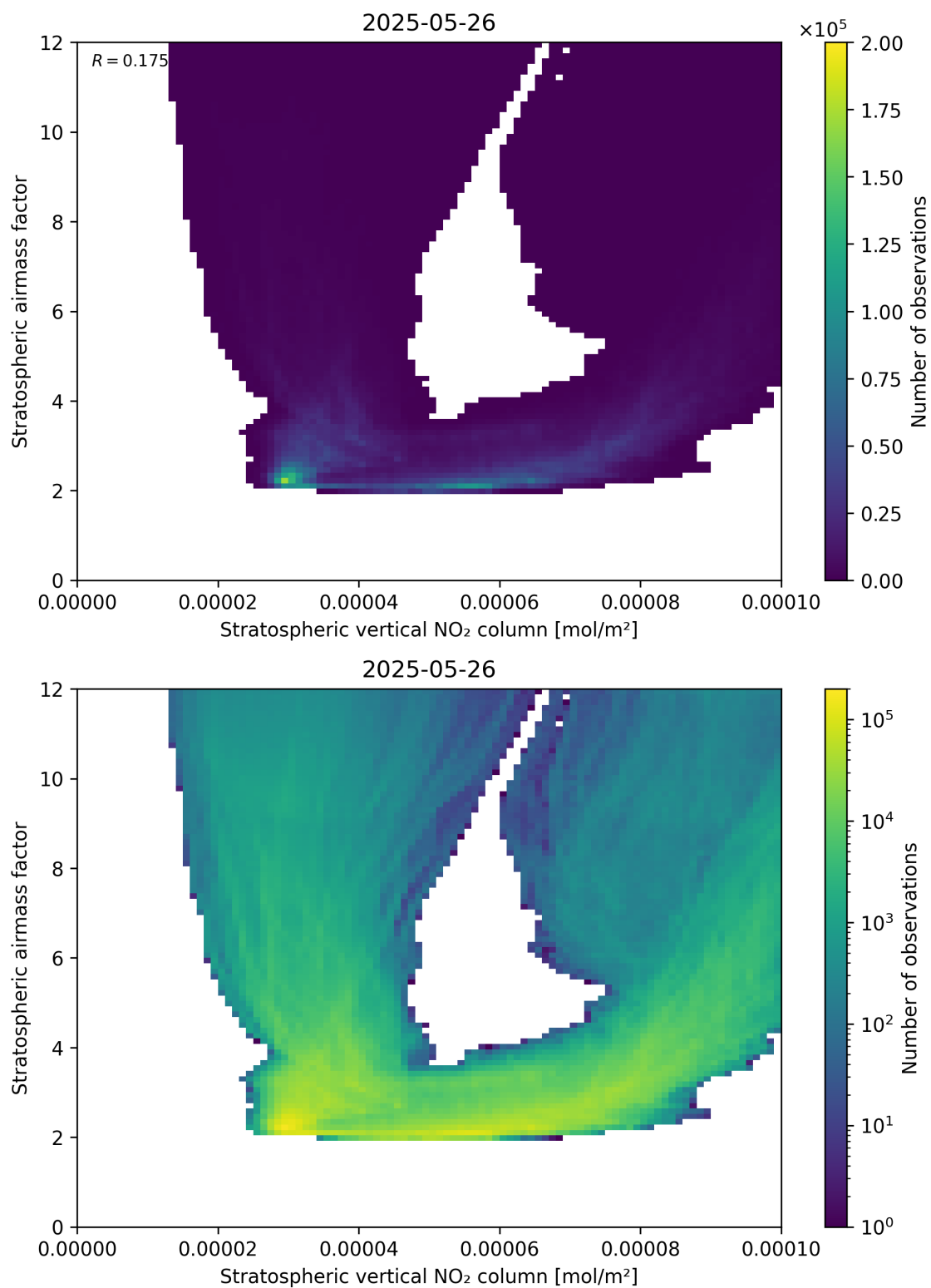
Figure 96: Scatter density plot of “Stratospheric vertical NO 2 column” against “Stratospheric airmass factor” for 2025-05-26 to 2025-05-27.
