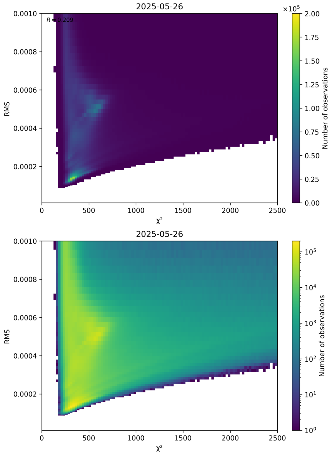
Figure 82: Scatter density plot of “ \chi^2 ” against “RMS” for 2025-05-26 to 2025-05-27.
