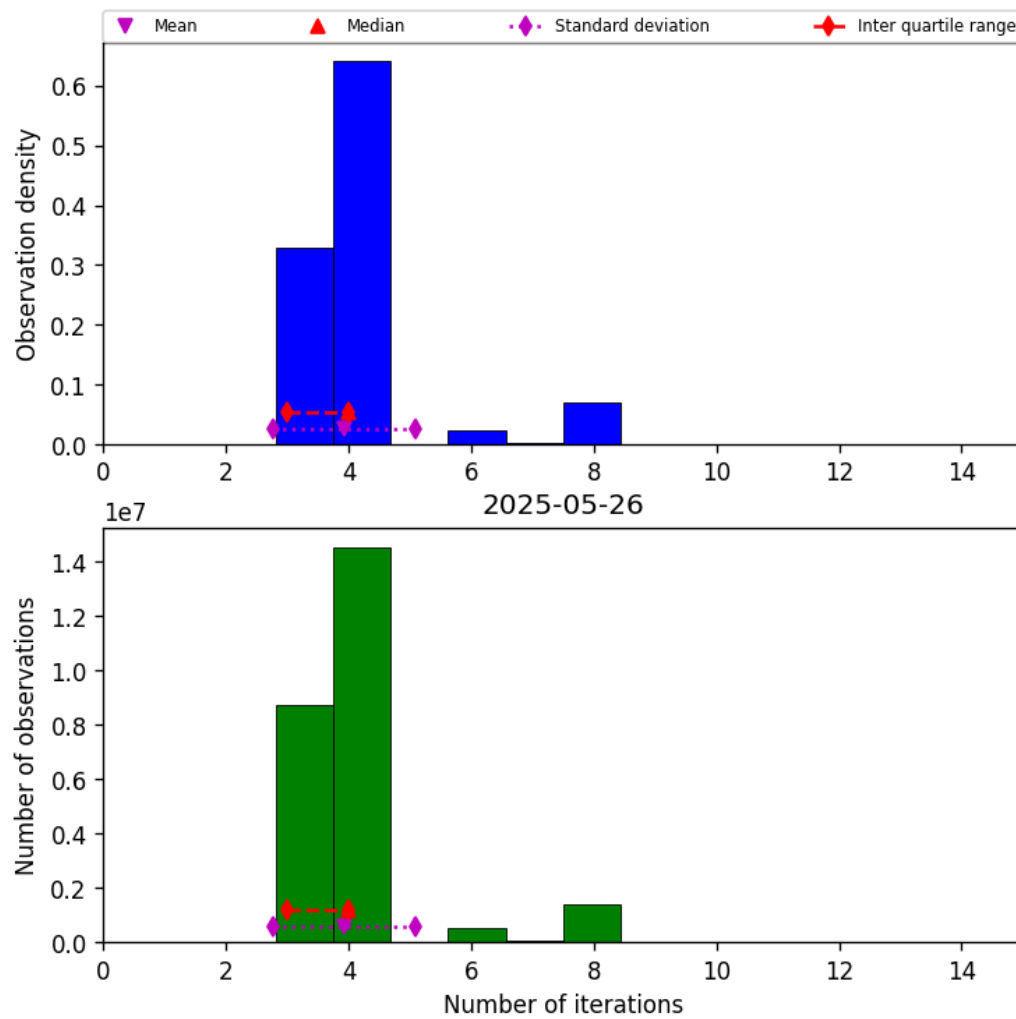
Figure 34: Histogram of “Number of iterations” for 2025-05-26 to 2025-05-27
