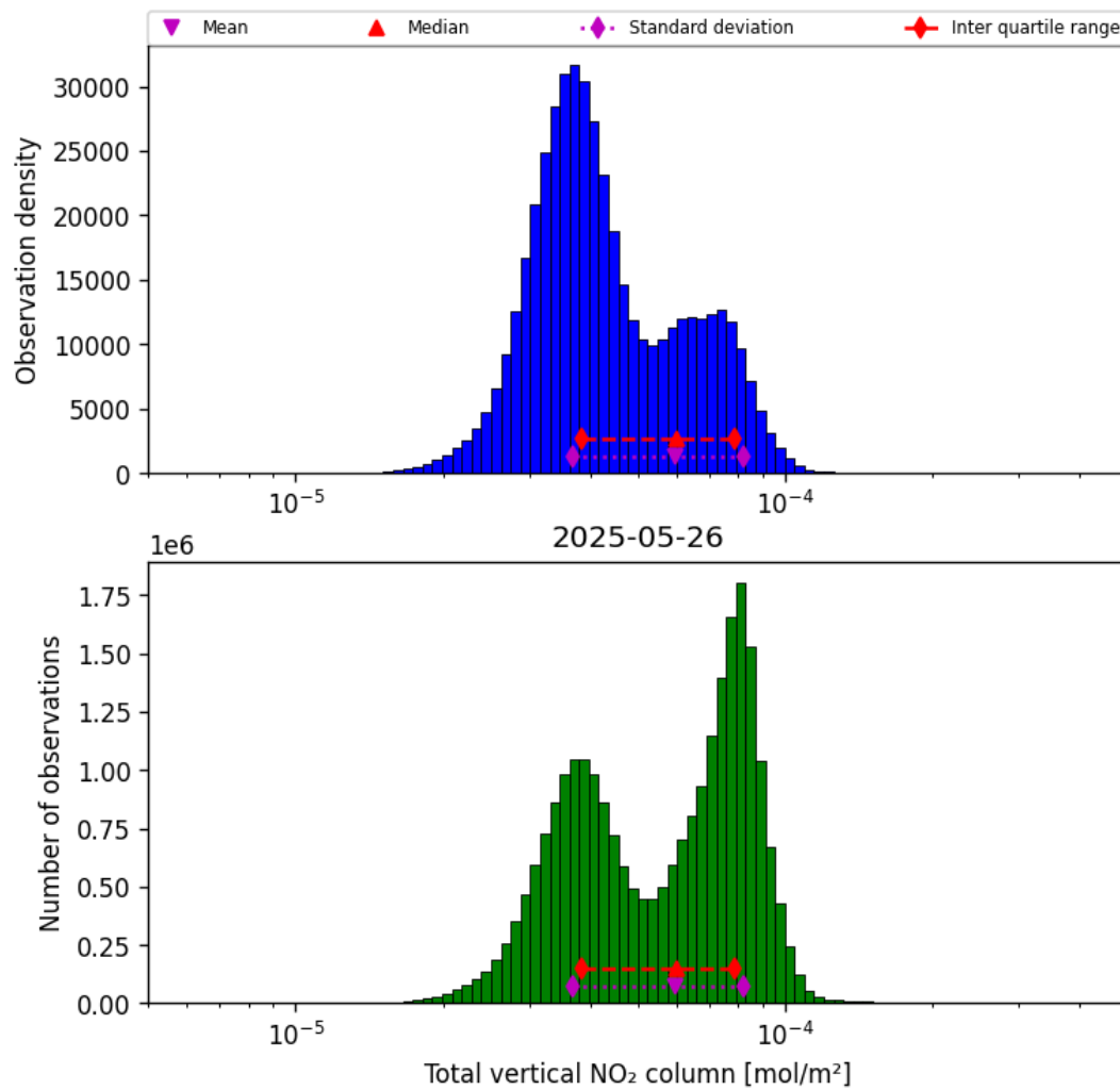
Figure 38: Histogram of “Total vertical NO 2 column” for 2025-05-26 to 2025-05-27
