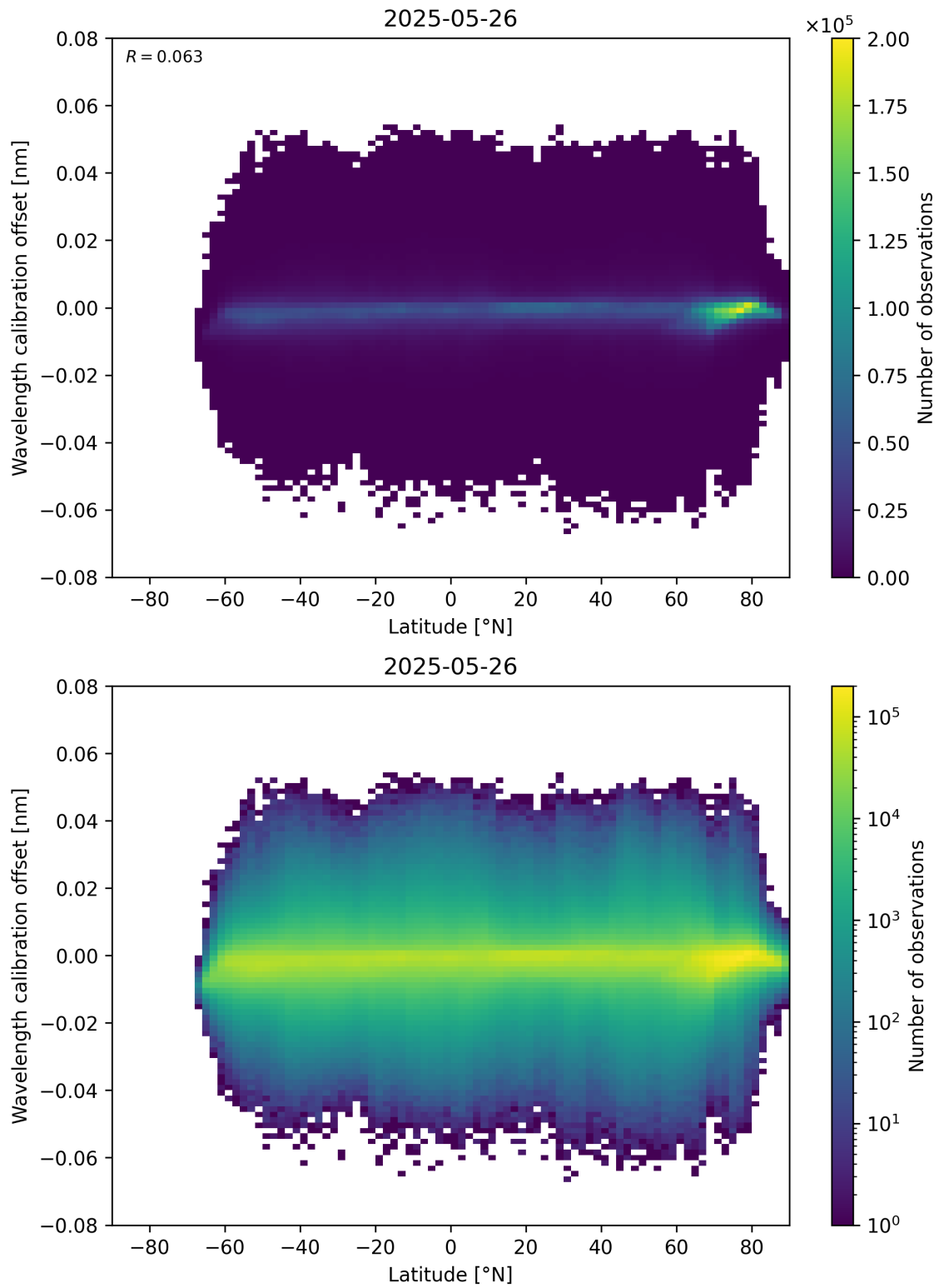
Figure 95: Scatter density plot of “Latitude” against “Wavelength calibration offset” for 2025-05-26 to 2025-05-27.
