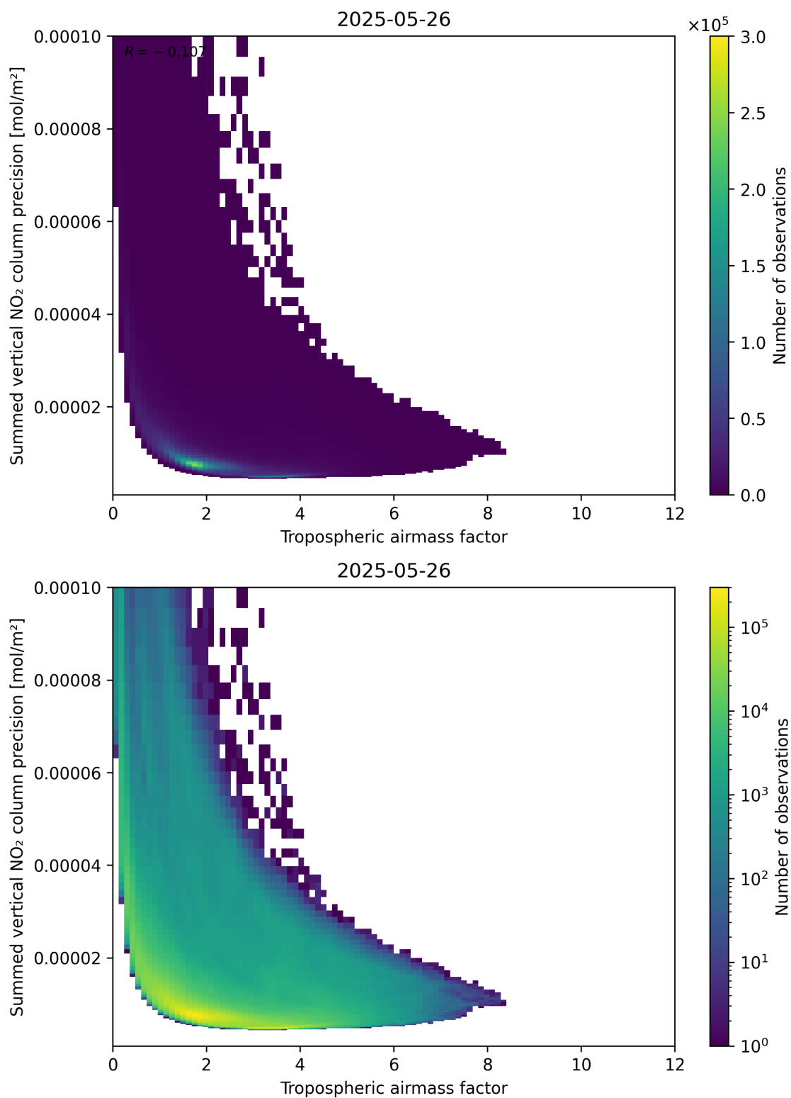
Figure 76: Scatter density plot of “Tropospheric air mass factor” against “Summed vertical NO 2 column precision” for 2025-05-26 to 2025-05-27.
