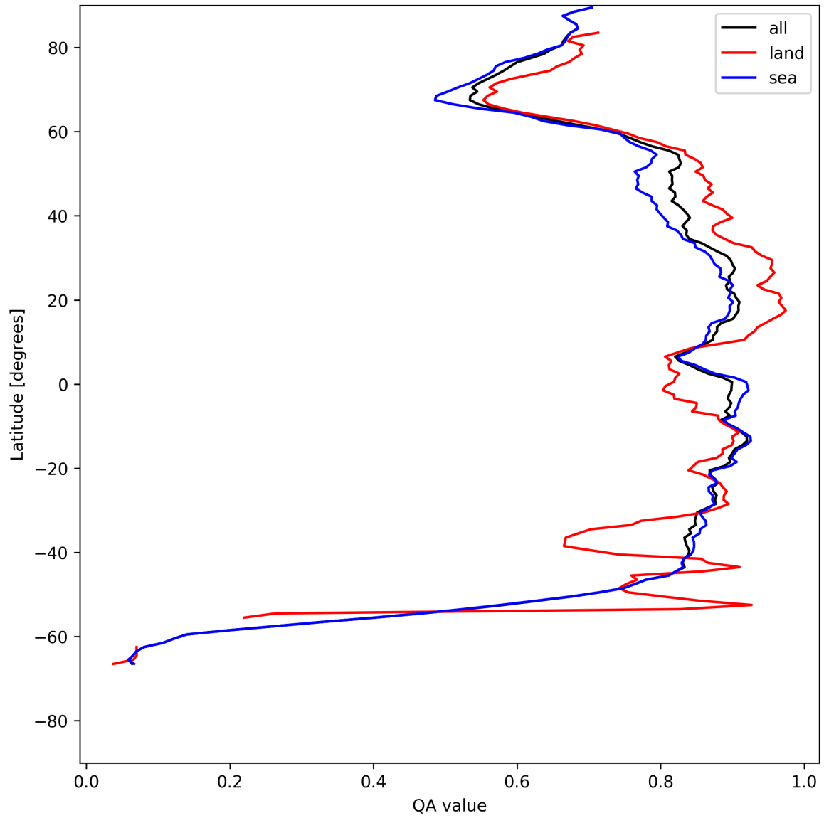
Figure 11: Zonal average of “QA value” for 2025-05-26 to 2025-05-27.
