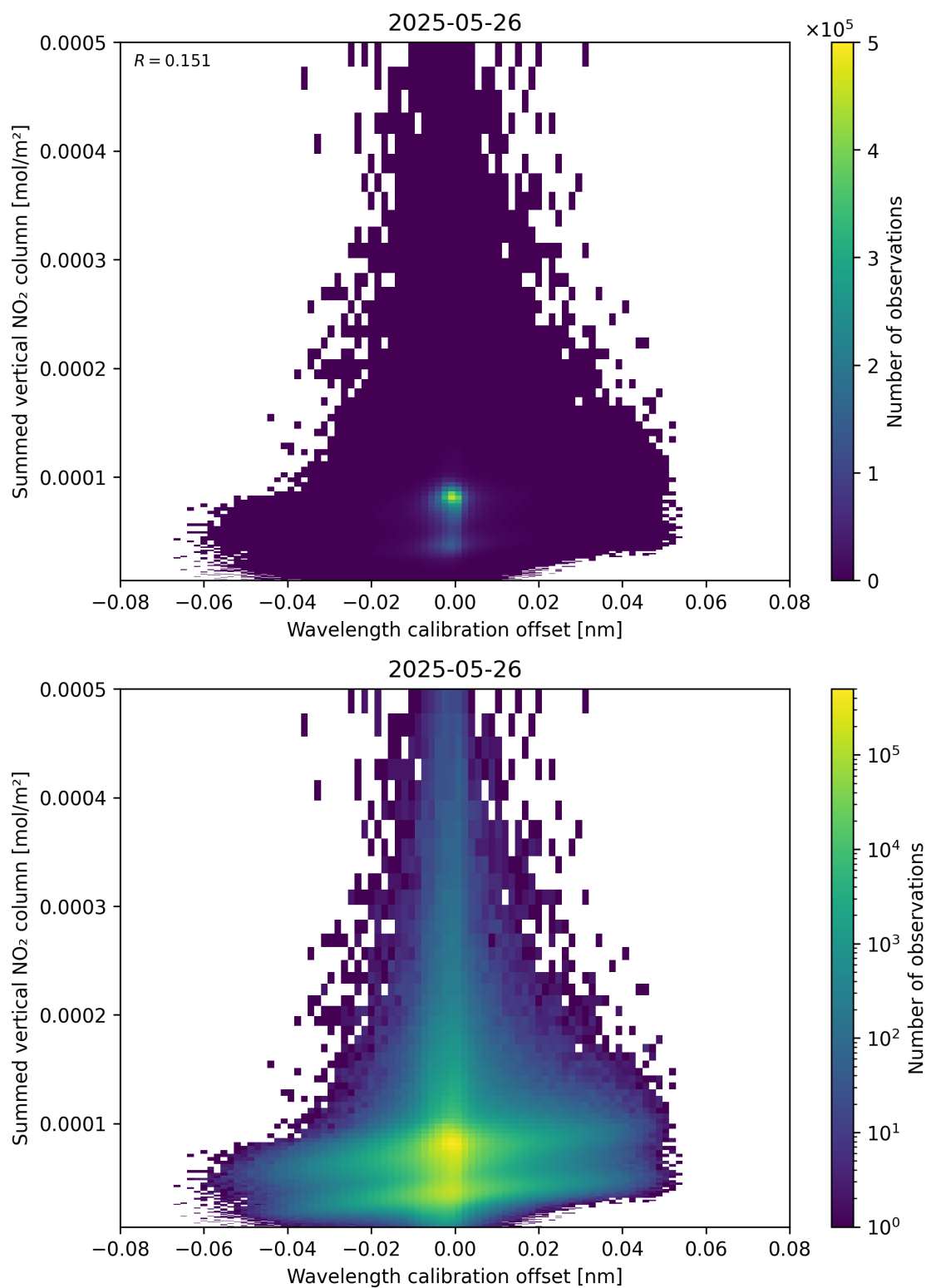
Figure 177: Scatter density plot of “Wavelength calibration offset” against “Summed vertical NO 2 column” for 2025-05-26 to 2025-05-27.
