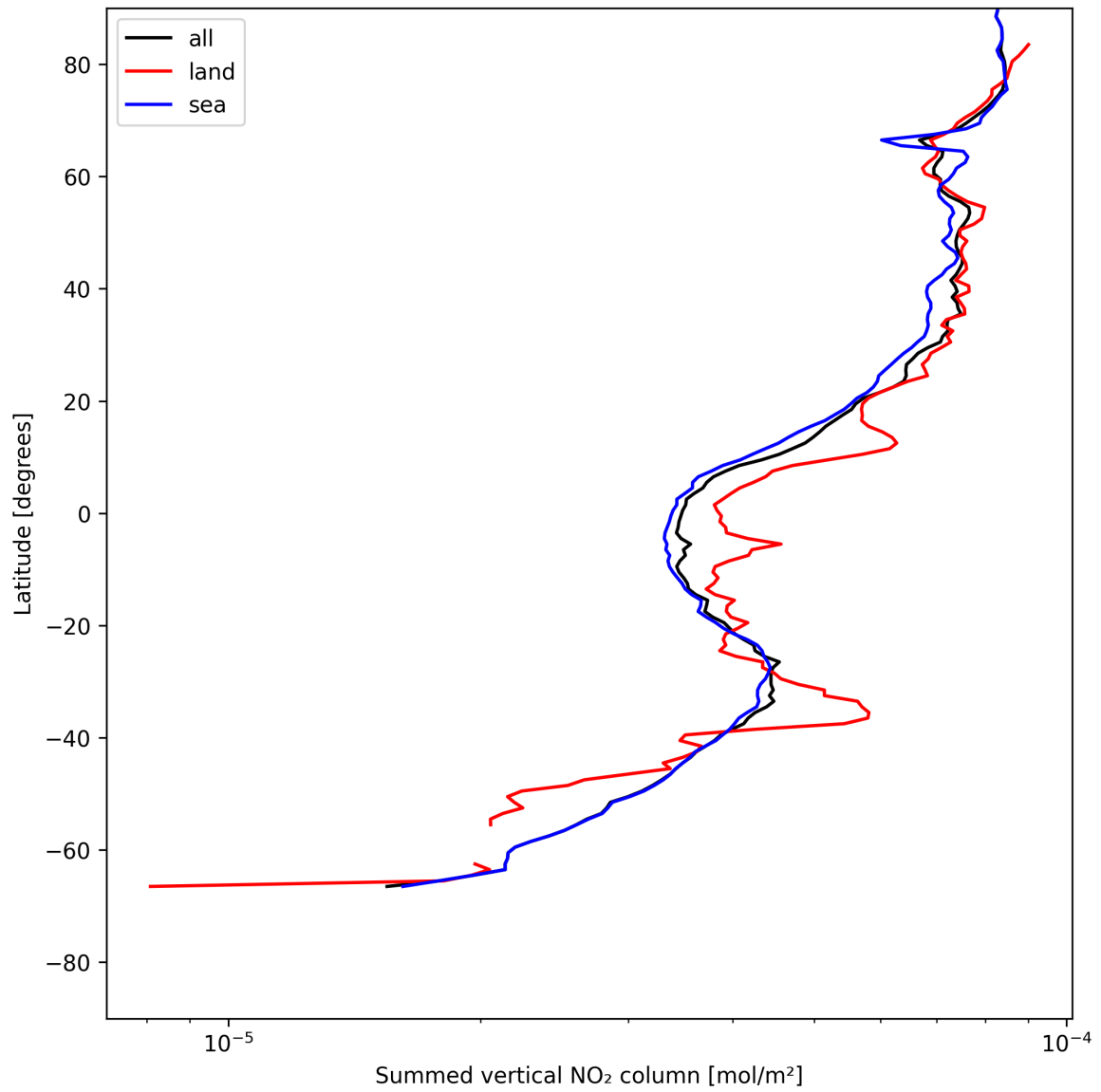
Figure 23: Zonal average of “Summed vertical NO 2 column” for 2025-05-26 to 2025-05-27.
