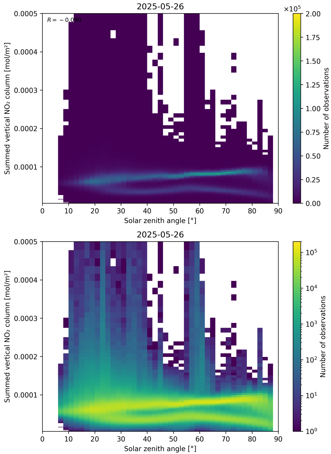
Figure 151: Scatter density plot of “Solar zenith angle” against “Summed vertical NO 2 column” for 2025-05-26 to 2025-05-27.
