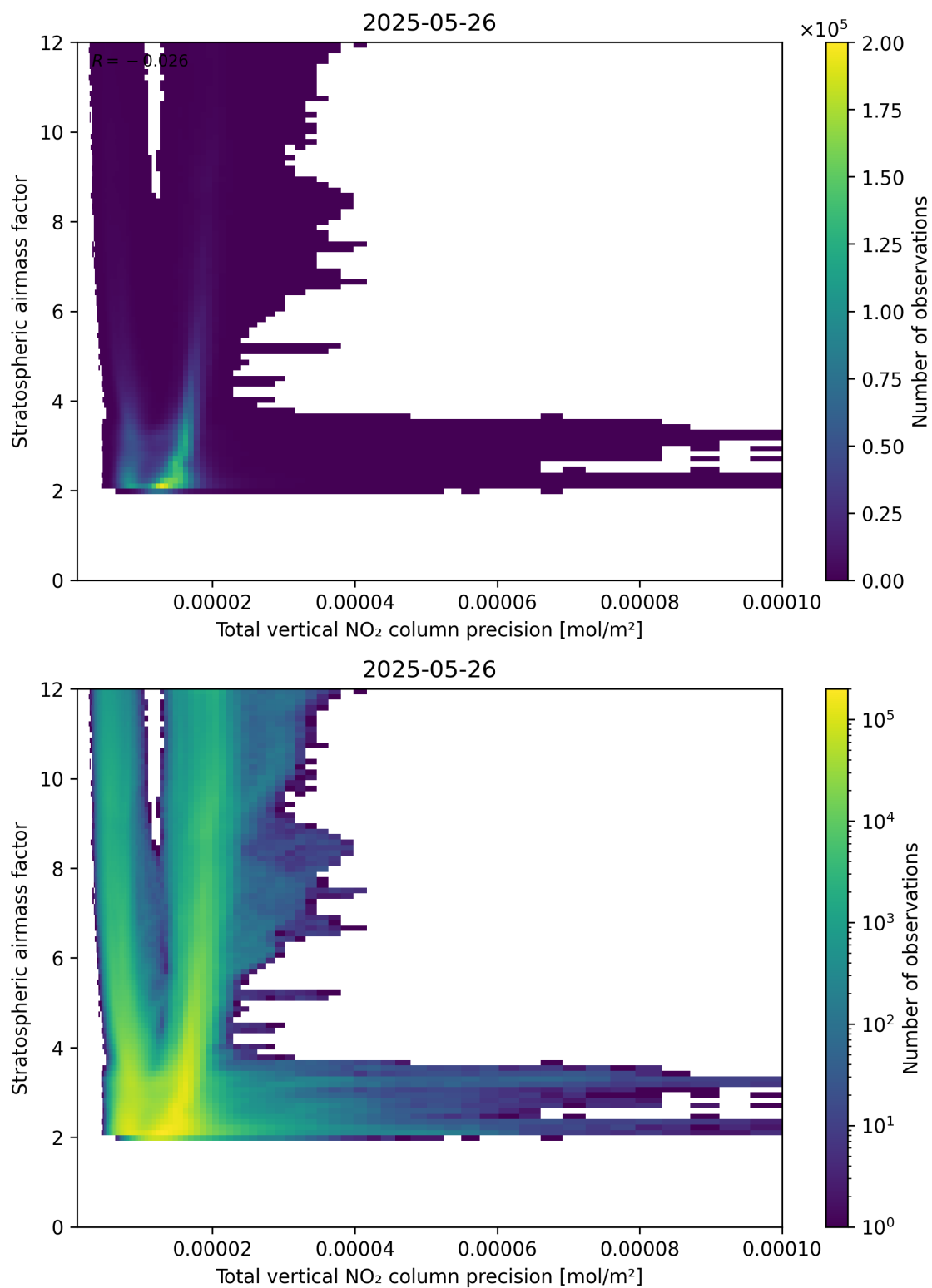
Figure 115: Scatter density plot of “Total vertical NO 2 column precision” against “Stratospheric air mass factor” for 2025-05-26 to 2025-05-27.
