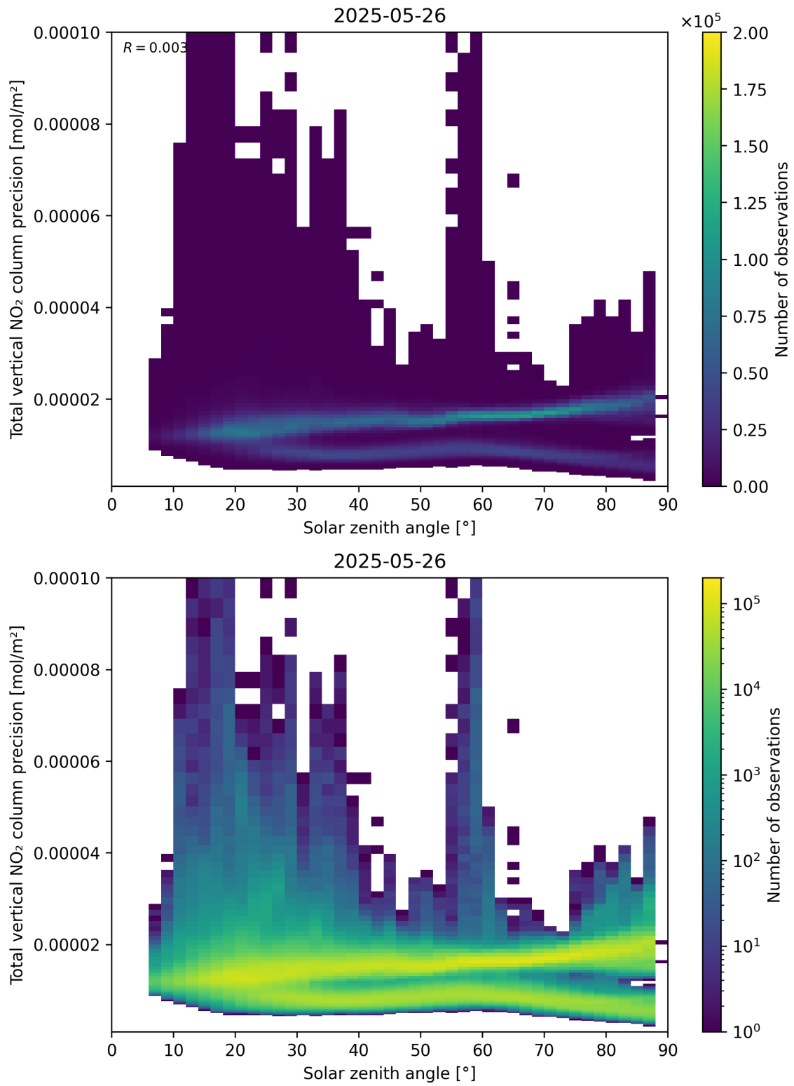
Figure 154: Scatter density plot of “Solar zenith angle” against “Total vertical NO 2 column precision” for 2025-05-26 to 2025-05-27.
