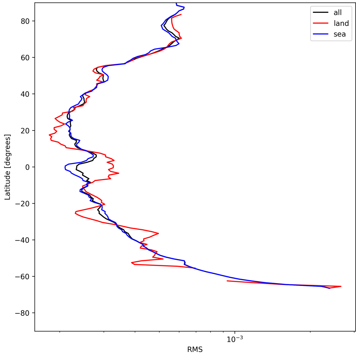
Figure 26: Zonal average of “RMS” for 2025-05-26 to 2025-05-27.
