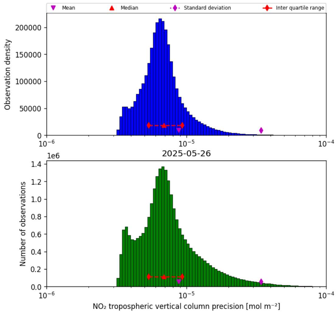
Figure 30: Histogram of “NO 2 tropospheric vertical column precision” for 2025-05-26 to 2025-05-27
