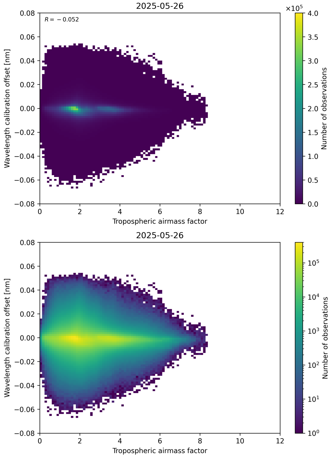
Figure 80: Scatter density plot of “Tropospheric airmass factor” against “Wavelength calibration offset” for 2025-05-26 to 2025-05-27.
