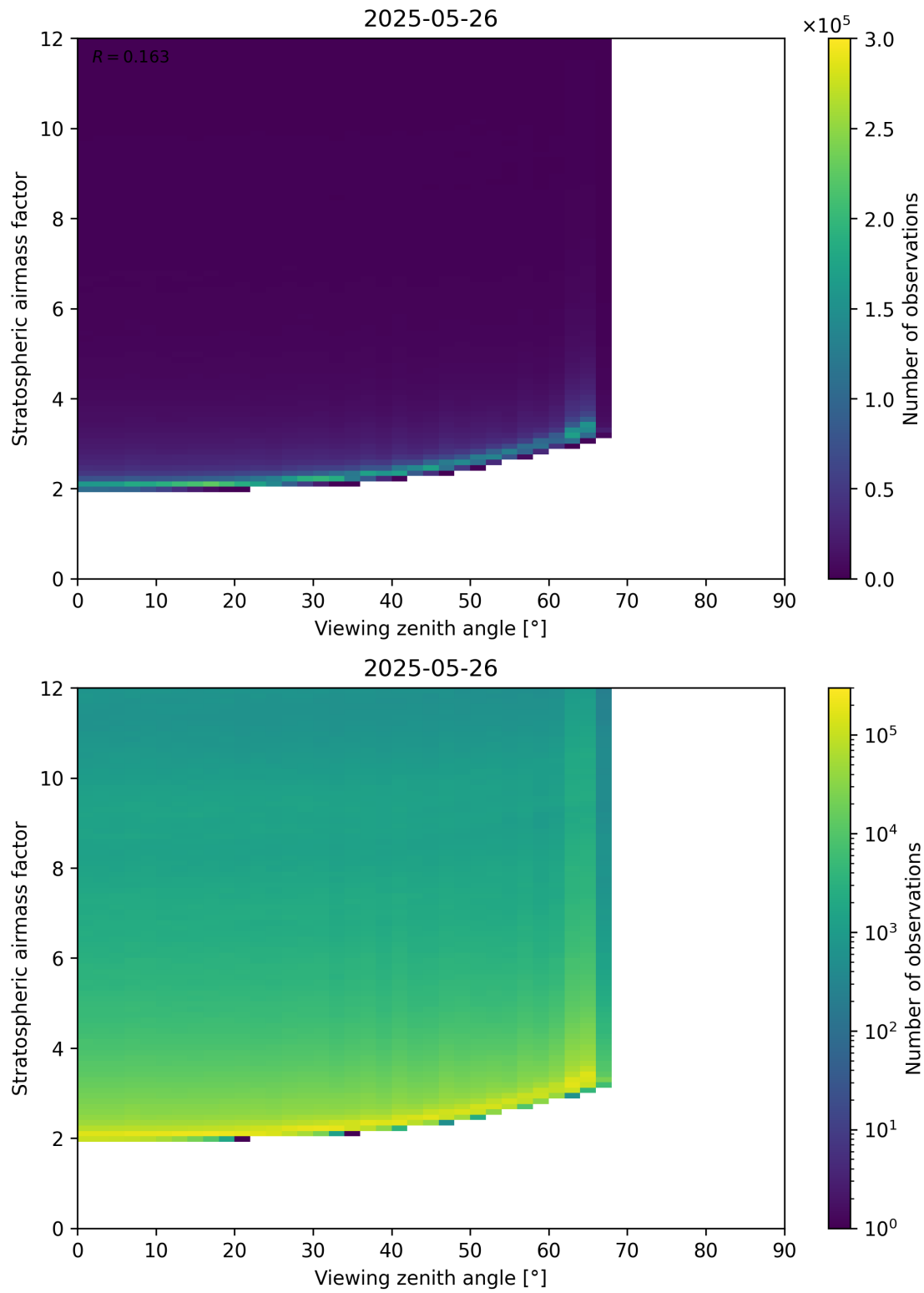
Figure 159: Scatter density plot of “Viewing zenith angle” against “Stratospheric airmass factor” for 2025-05-26 to 2025-05-27.
