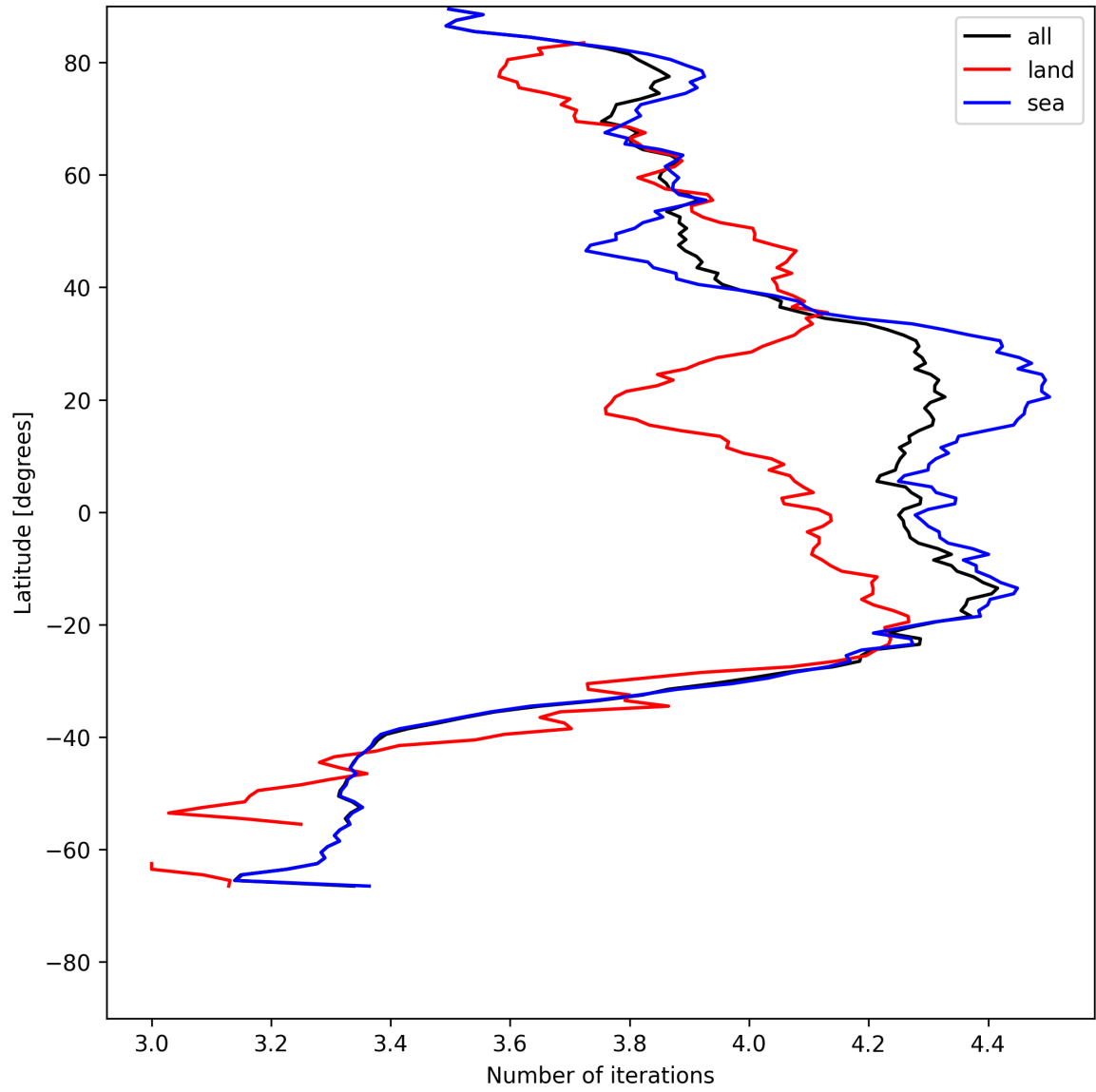
Figure 17: Zonal average of “Number of iterations” for 2025-05-26 to 2025-05-27.
