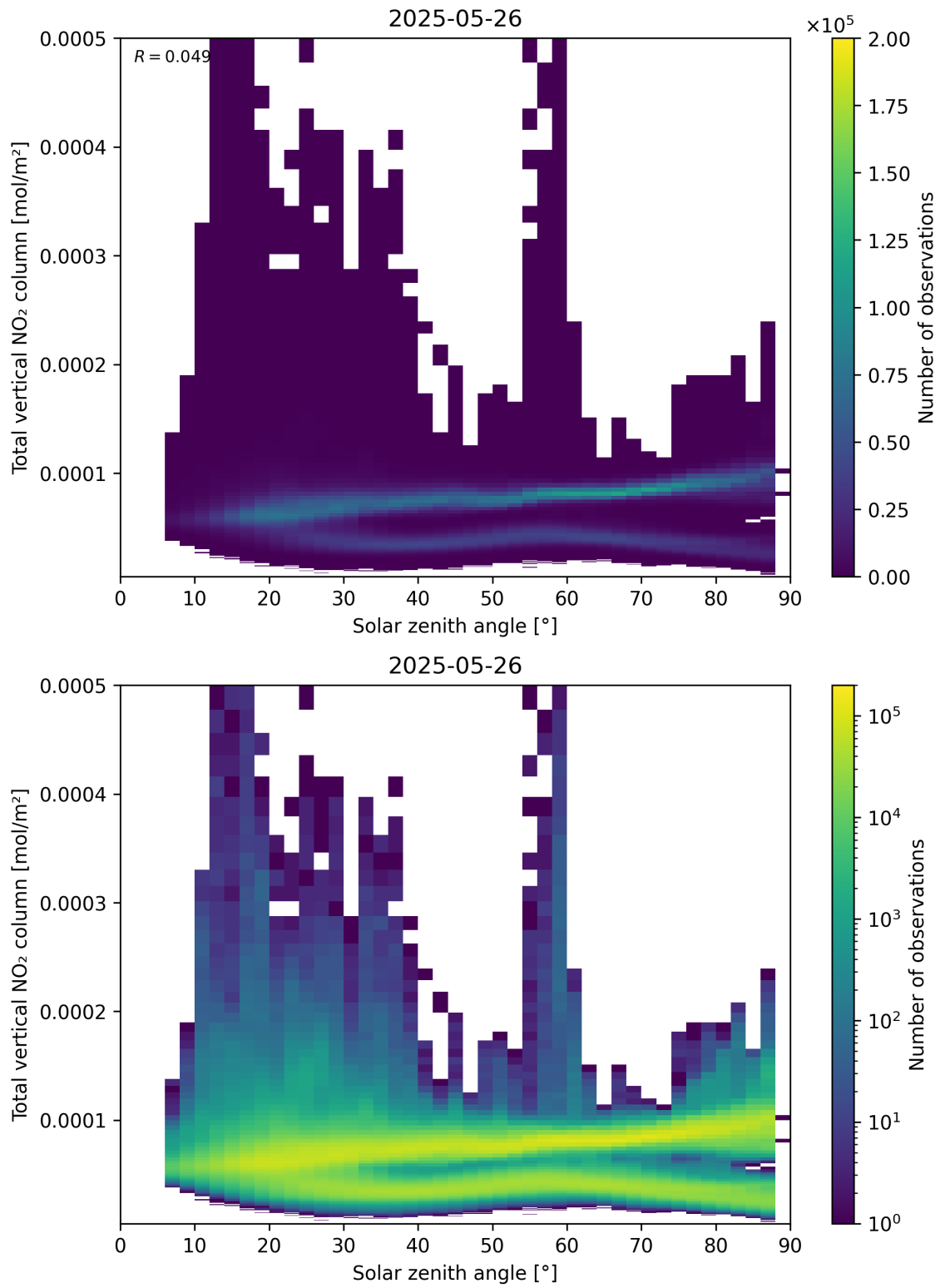
Figure 153: Scatter density plot of “Solar zenith angle” against “Total vertical NO 2 column” for 2025-05-26 to 2025-05-27.
