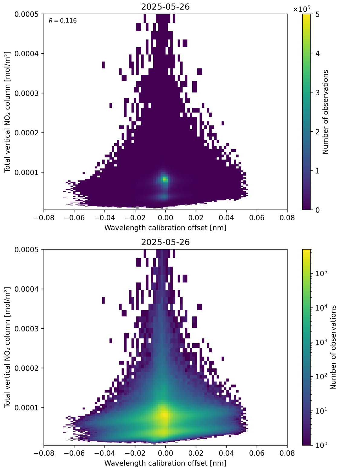
Figure 179: Scatter density plot of “Wavelength calibration offset” against “Total vertical NO 2 column” for 2025-05-26 to 2025-05-27.
