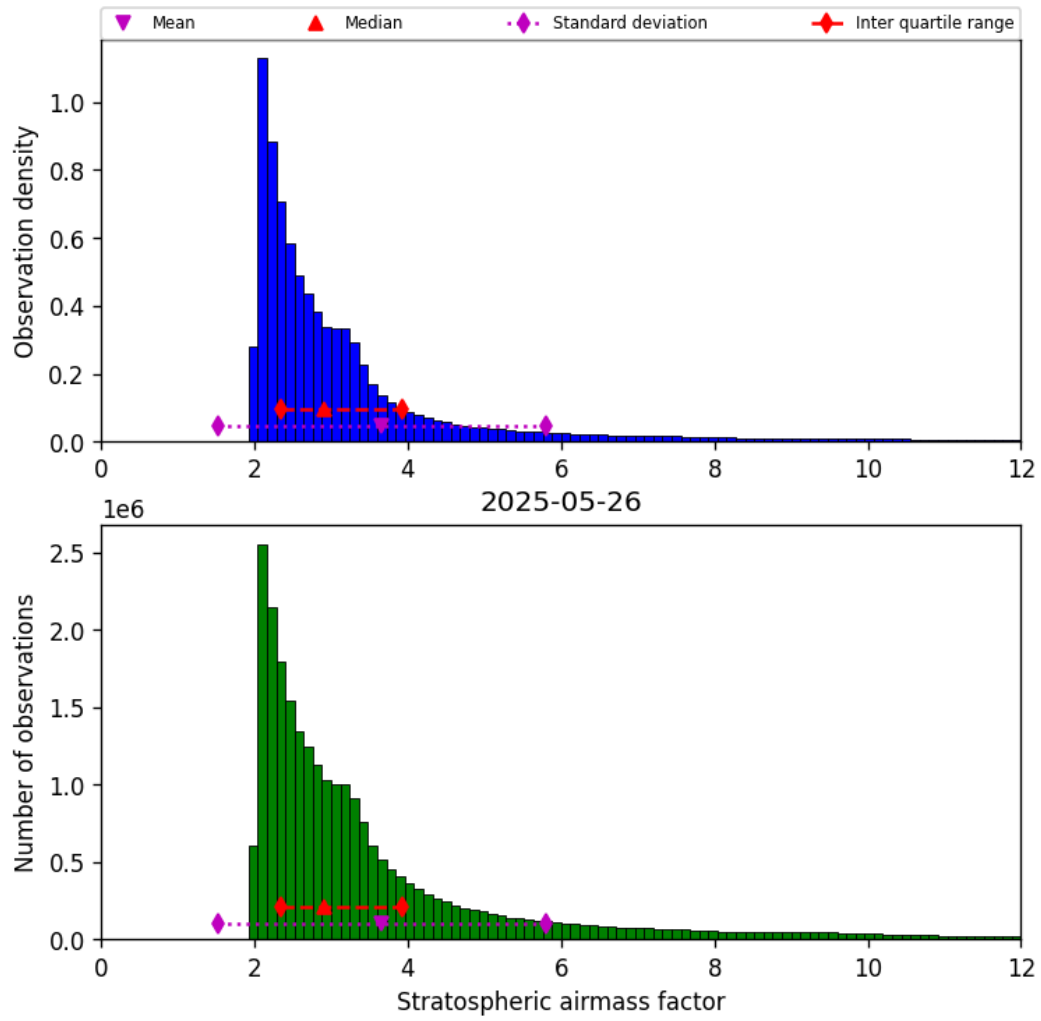
Figure 44: Histogram of “Stratospheric airmass factor” for 2025-05-26 to 2025-05-27
