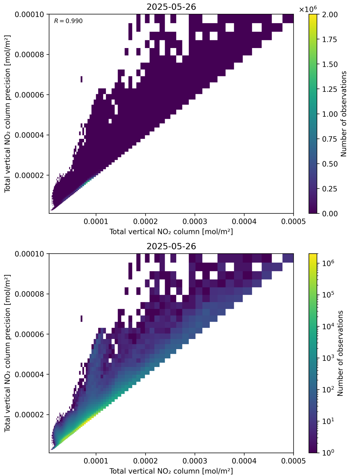
Figure 114: Scatter density plot of “Total vertical NO 2 column” against “Total vertical NO 2 column precision” for 2025-05-26 to 2025-05-27.
