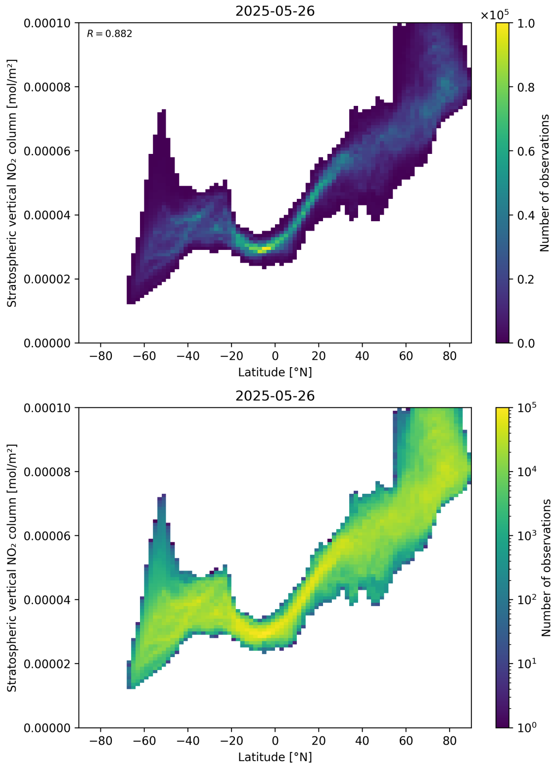
Figure 87: Scatter density plot of “Latitude” against “Stratospheric vertical NO 2 column” for 2025-05-26 to 2025-05-27.
