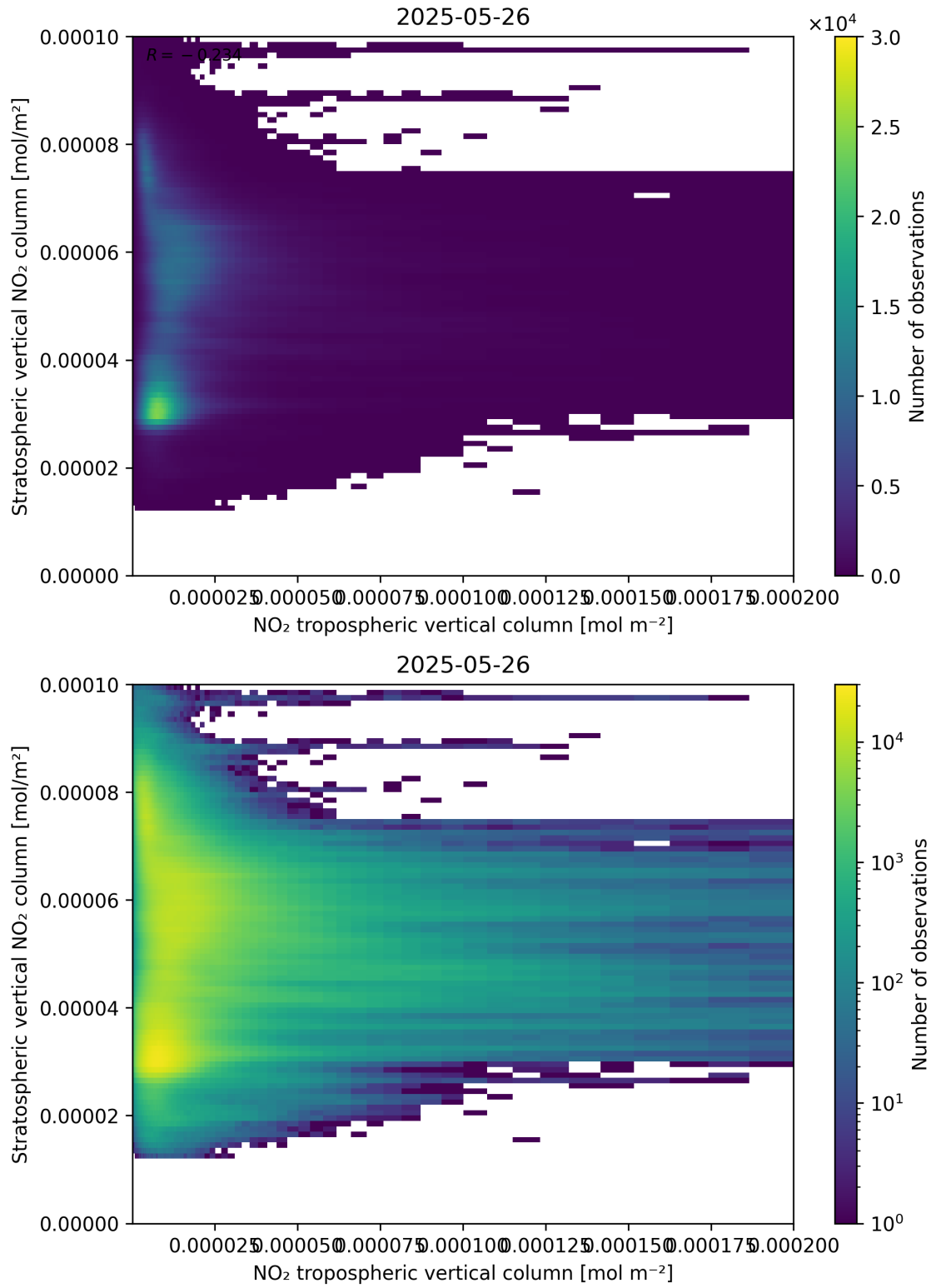
Figure 125: Scatter density plot of “NO 2 tropospheric vertical column” against “Stratospheric vertical NO 2 column” for 2025-05-26 to 2025-05-27.
