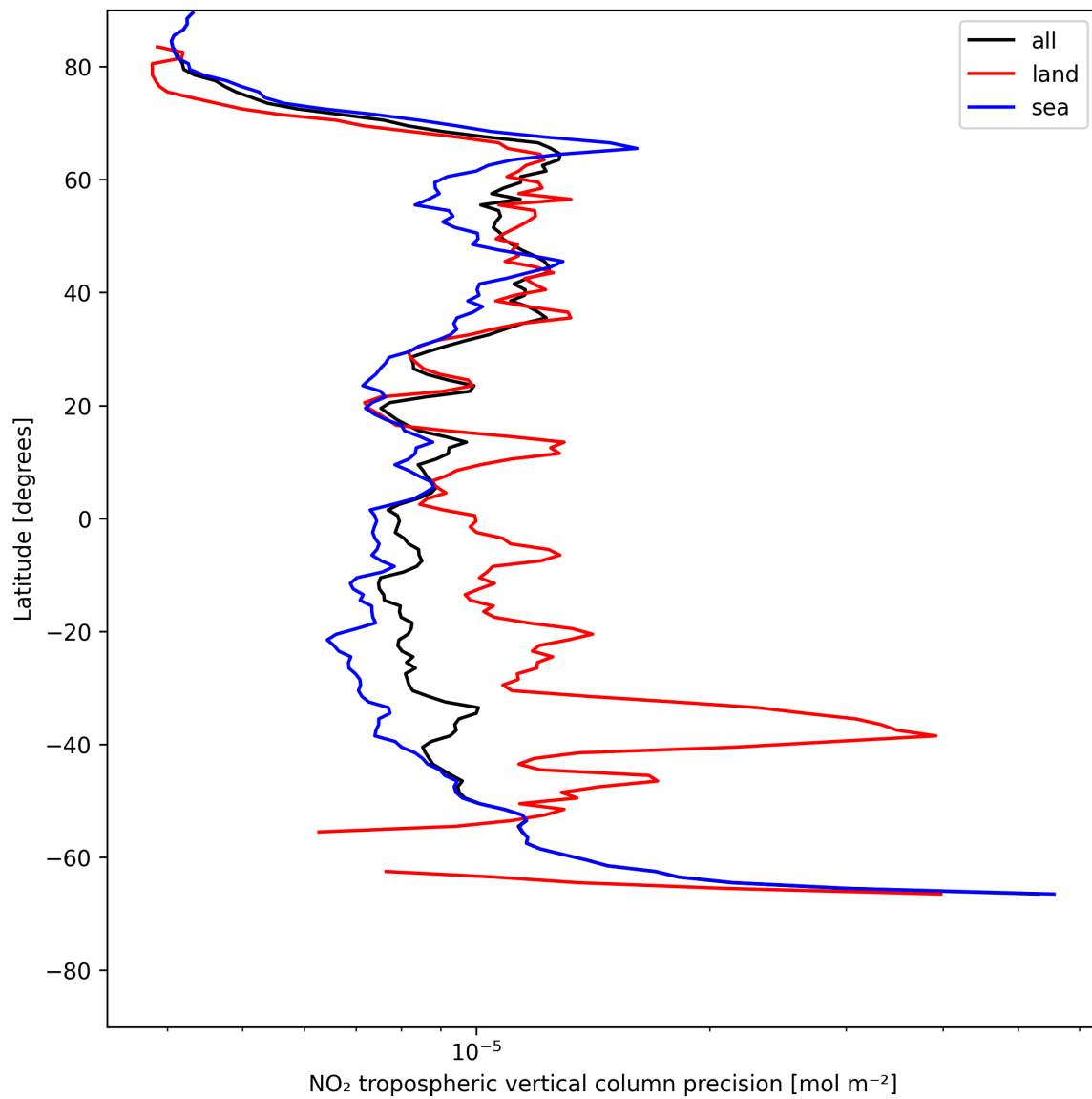
Figure 13: Zonal average of “NO 2 tropospheric vertical column precision” for 2025-05-26 to 2025-05-27.
