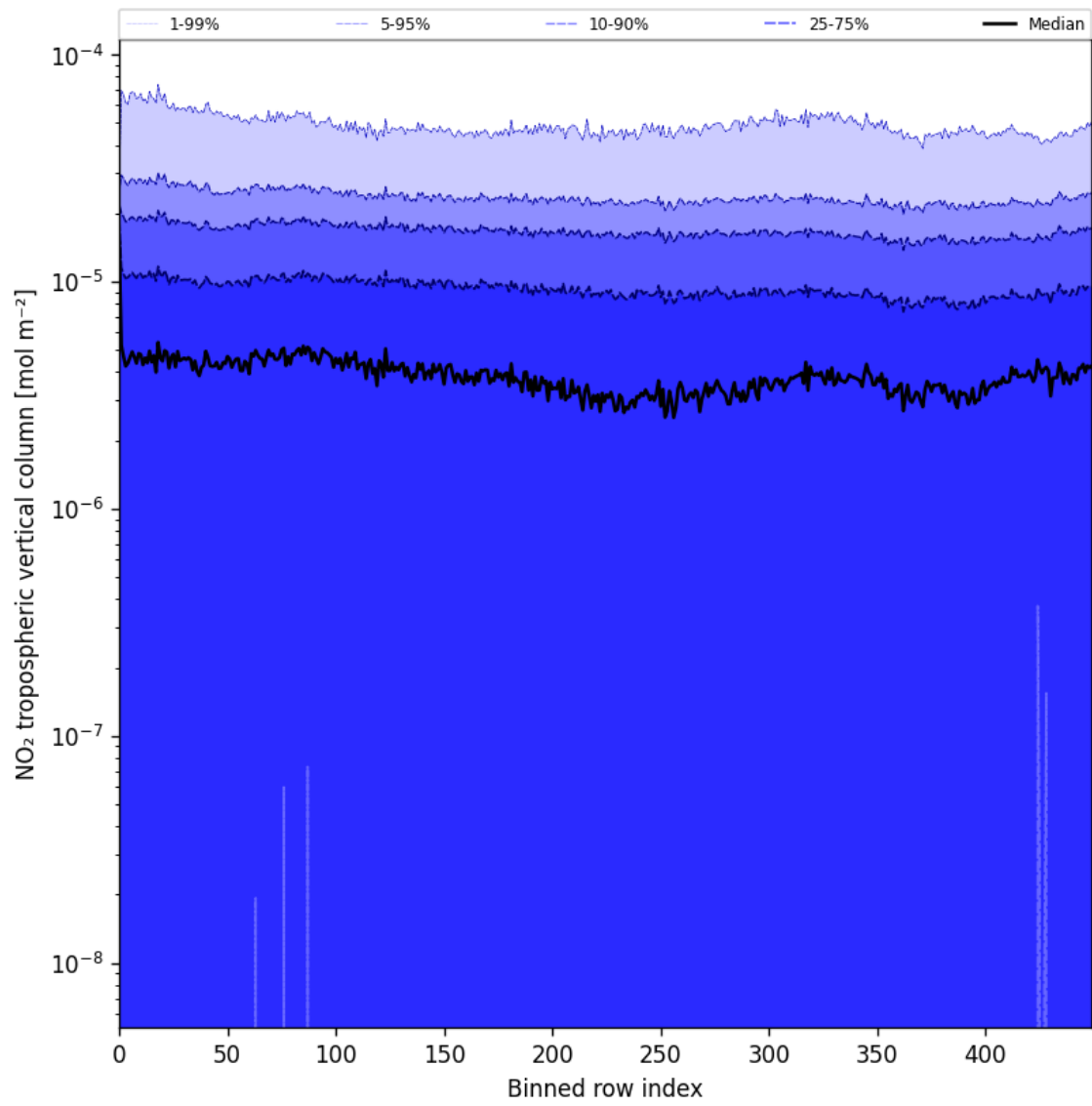
Figure 46: Along track statistics of “NO 2 tropospheric vertical column” for 2025-05-26 to 2025-05-27
