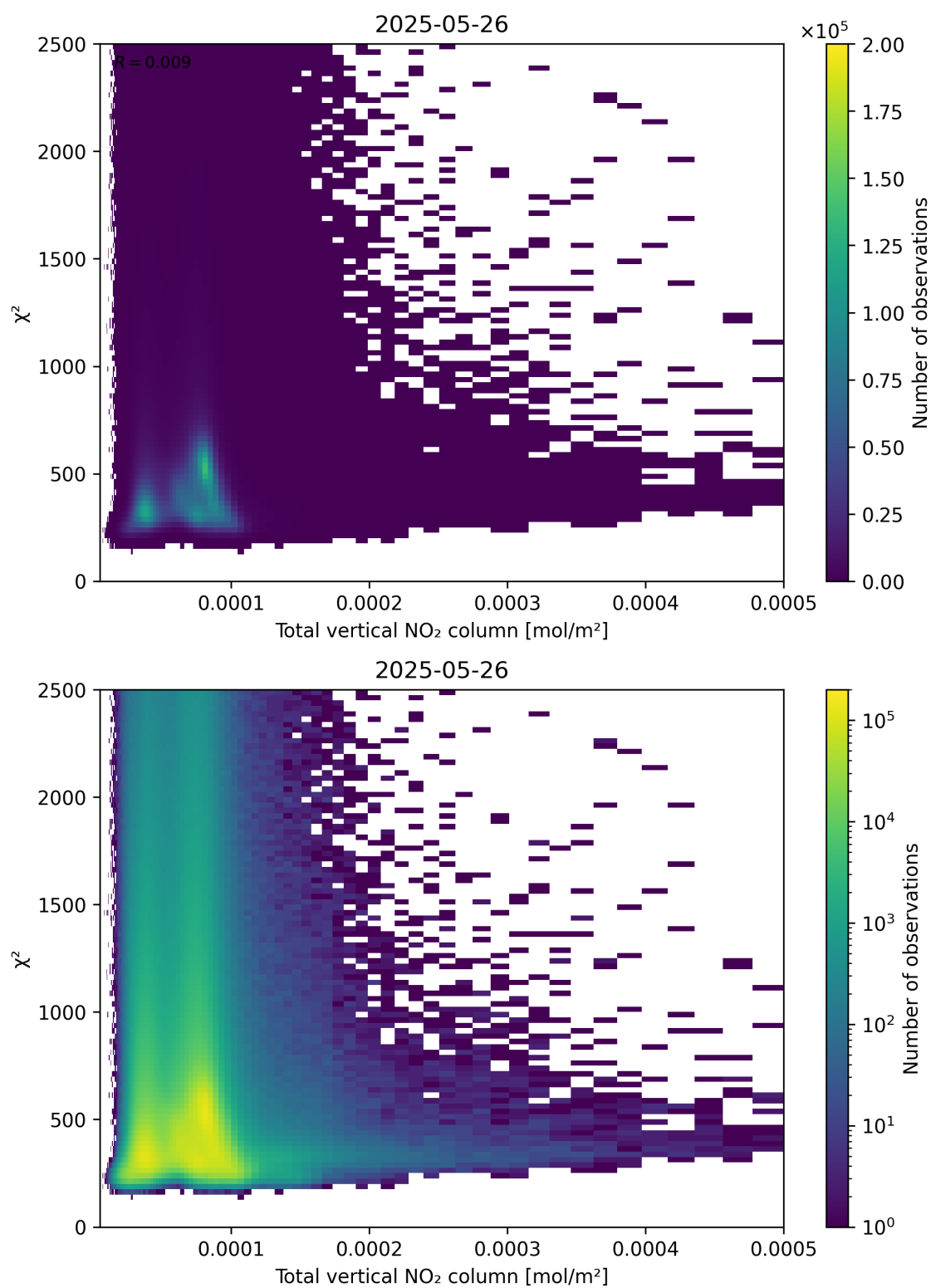
Figure 111: Scatter density plot of “Total vertical NO 2 column” against “ \chi^2 ” for 2025-05-26 to 2025-05-27.
