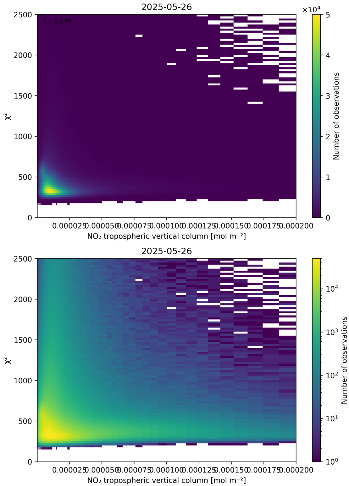
Figure 124: Scatter density plot of “NO 2 tropospheric vertical column” against “ \chi^2 ” for 2025-05-26 to 2025-05-27.
