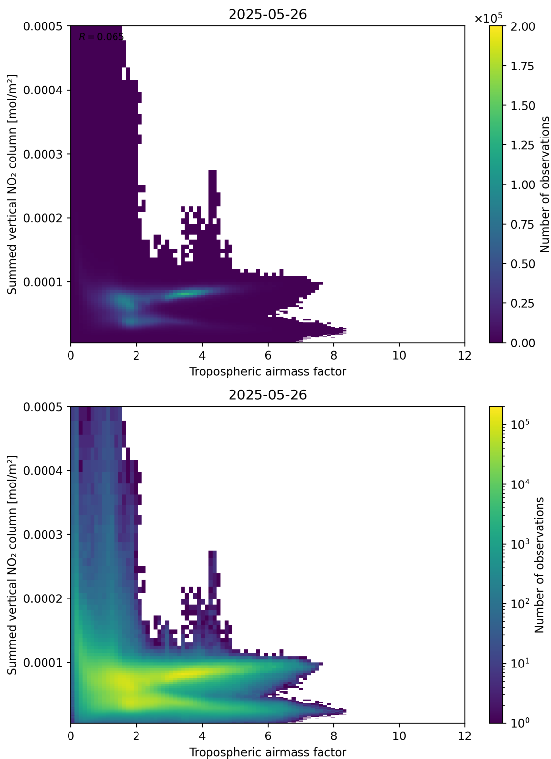
Figure 75: Scatter density plot of “Tropospheric airmass factor” against “Summed vertical NO 2 column” for 2025-05-26 to 2025-05-27.
