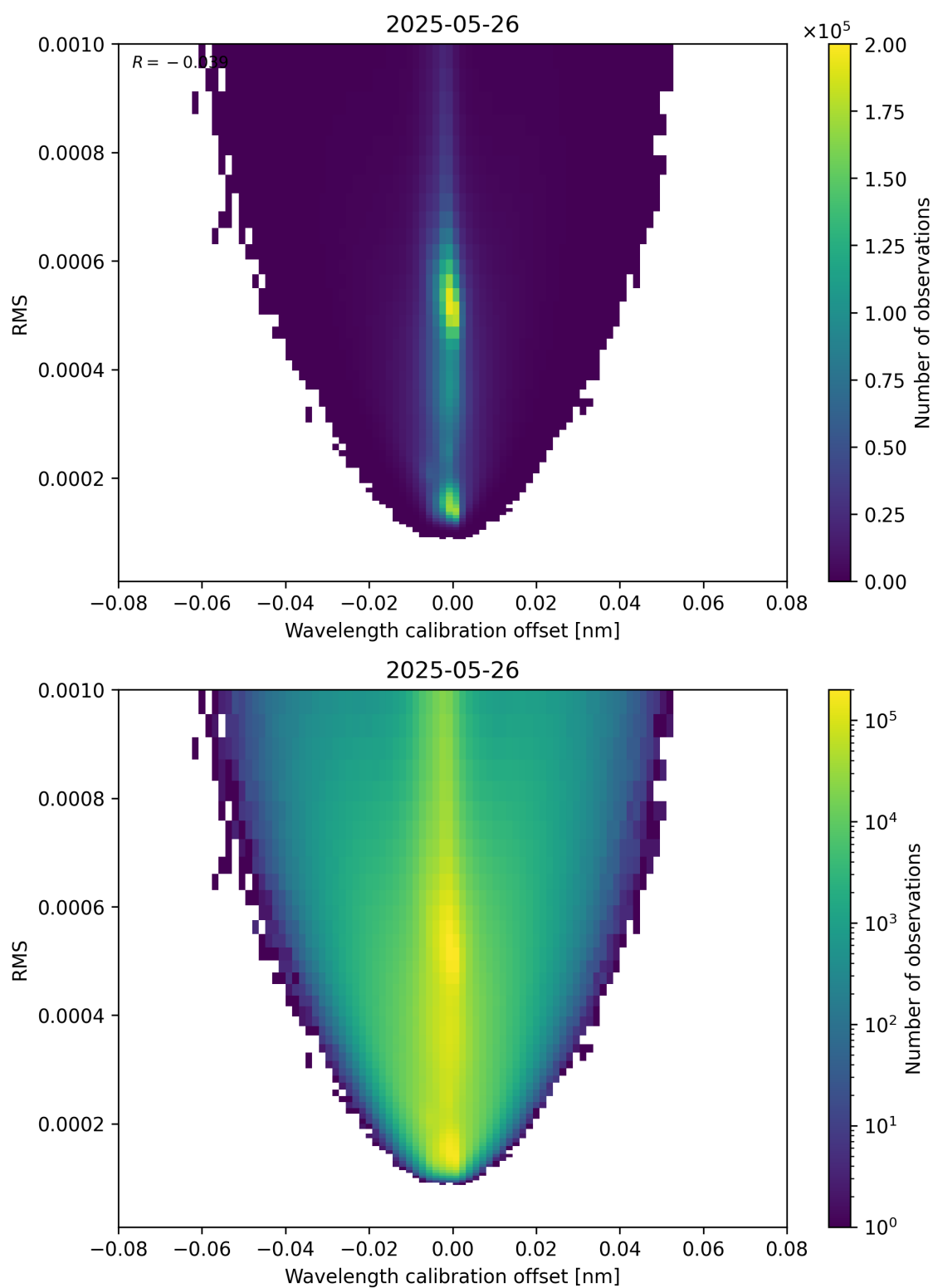
Figure 181: Scatter density plot of “Wavelength calibration offset” against “RMS” for 2025-05-26 to 2025-05-27.
