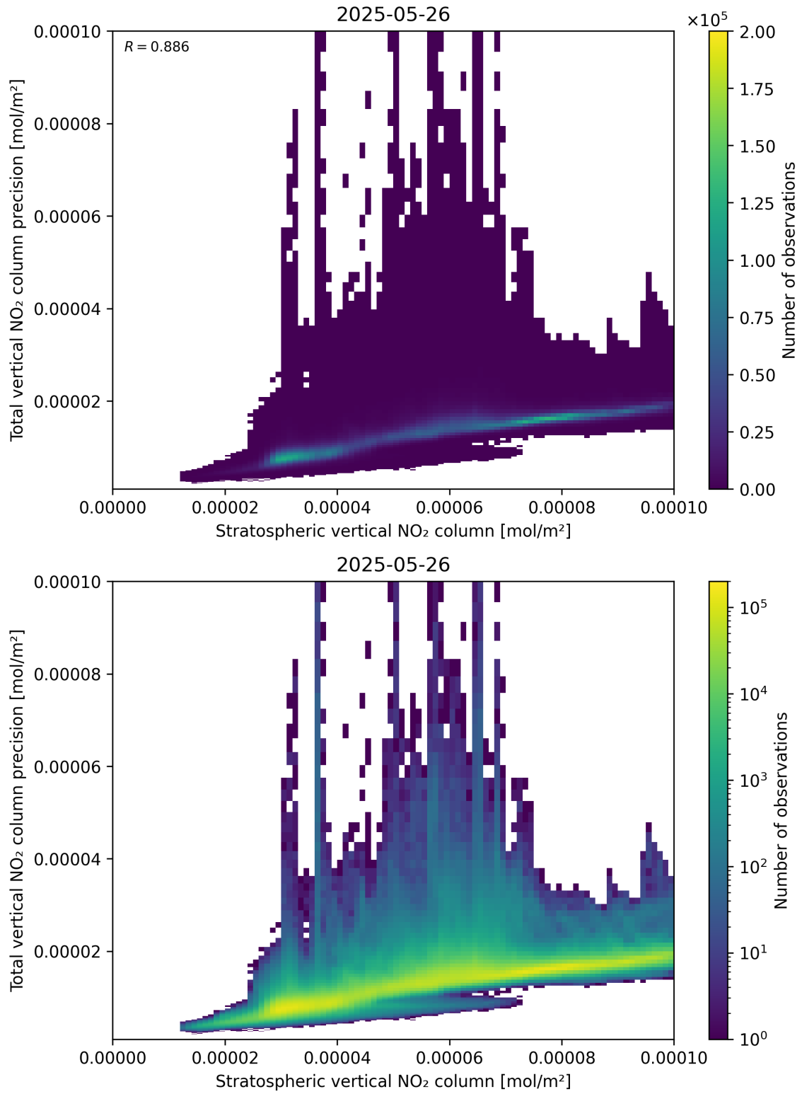
Figure 101: Scatter density plot of “Stratospheric vertical NO 2 column” against “Total vertical NO 2 column precision” for 2025-05-26 to 2025-05-27.
