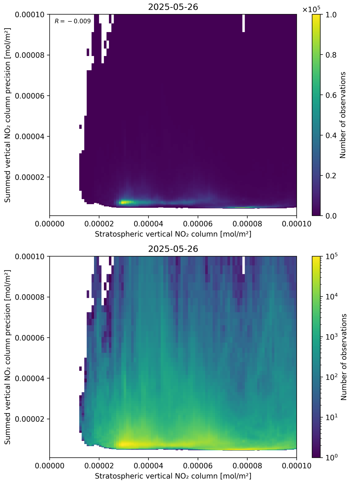
Figure 99: Scatter density plot of “Stratospheric vertical NO 2 column” against “Summed vertical NO 2 column precision” for 2025-05-26 to 2025-05-27.
