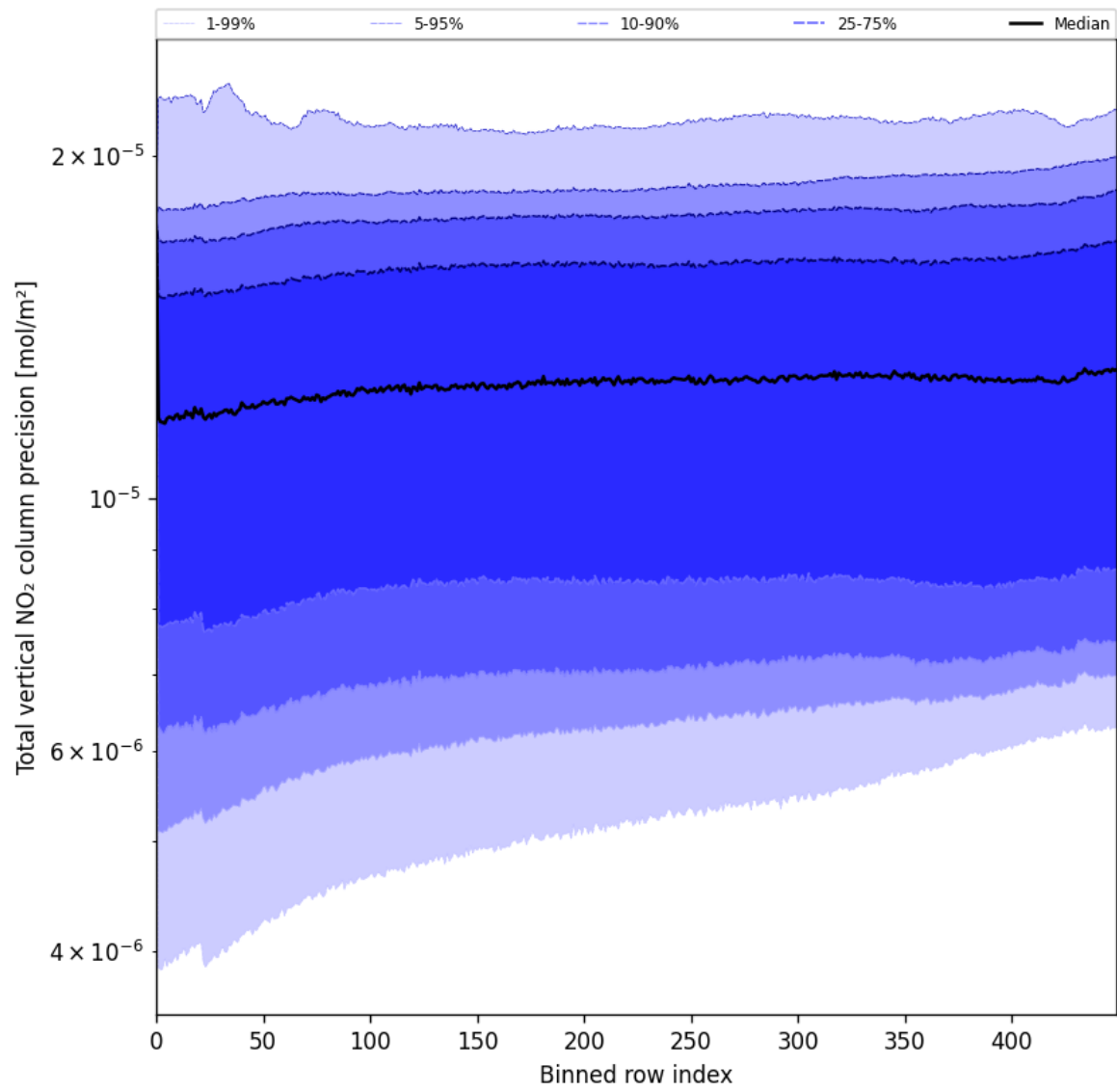
Figure 56: Along track statistics of "Total vertical NO 2 column precision" for 2025-05-26 to 2025-05-27
