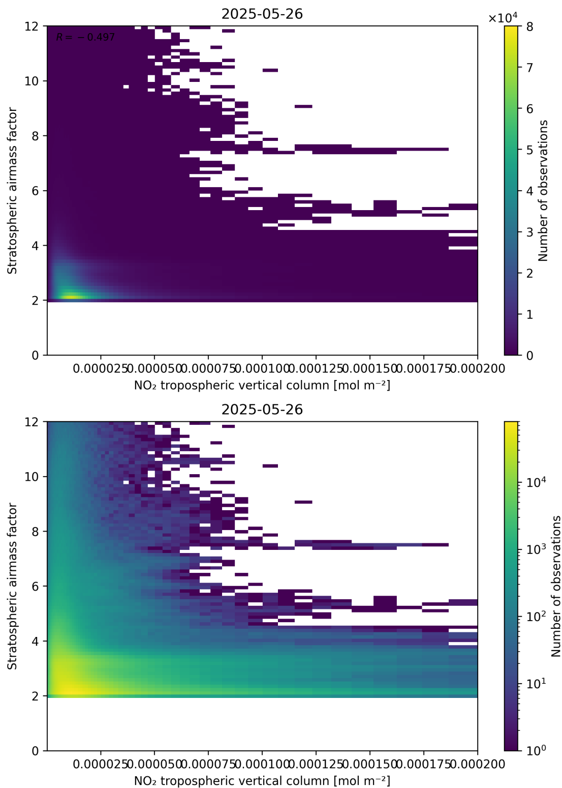
Figure 121: Scatter density plot of “NO 2 tropospheric vertical column” against “Stratospheric air mass factor” for 2025-05-26 to 2025-05-27.
