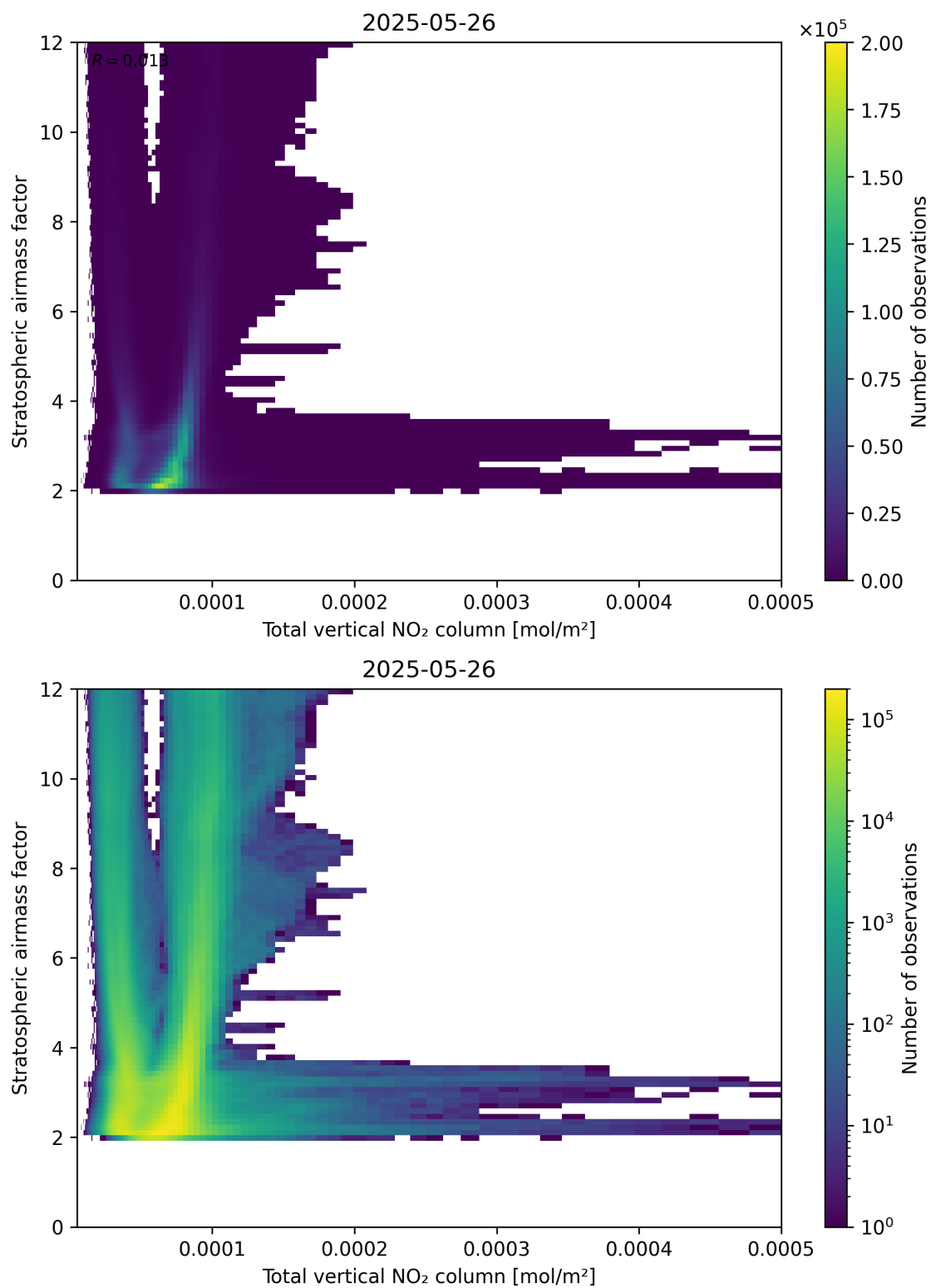
Figure 110: Scatter density plot of “Total vertical NO 2 column” against “Stratospheric airmass factor” for 2025-05-26 to 2025-05-27.
