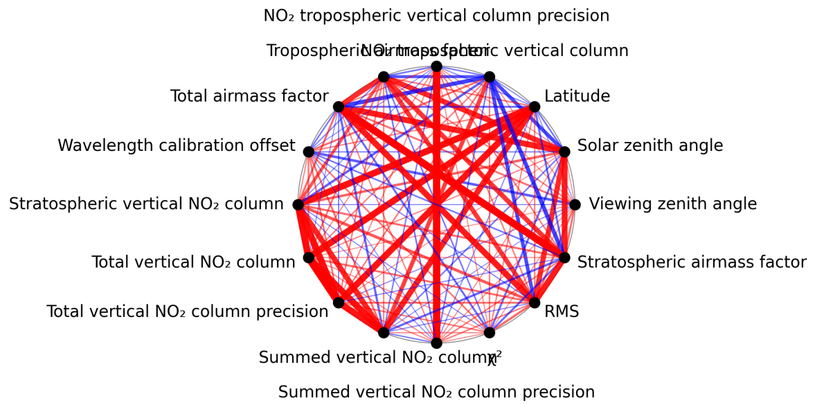
Figure 1: Map of correlation graph for 2025-05-26 to 2025-05-27.
