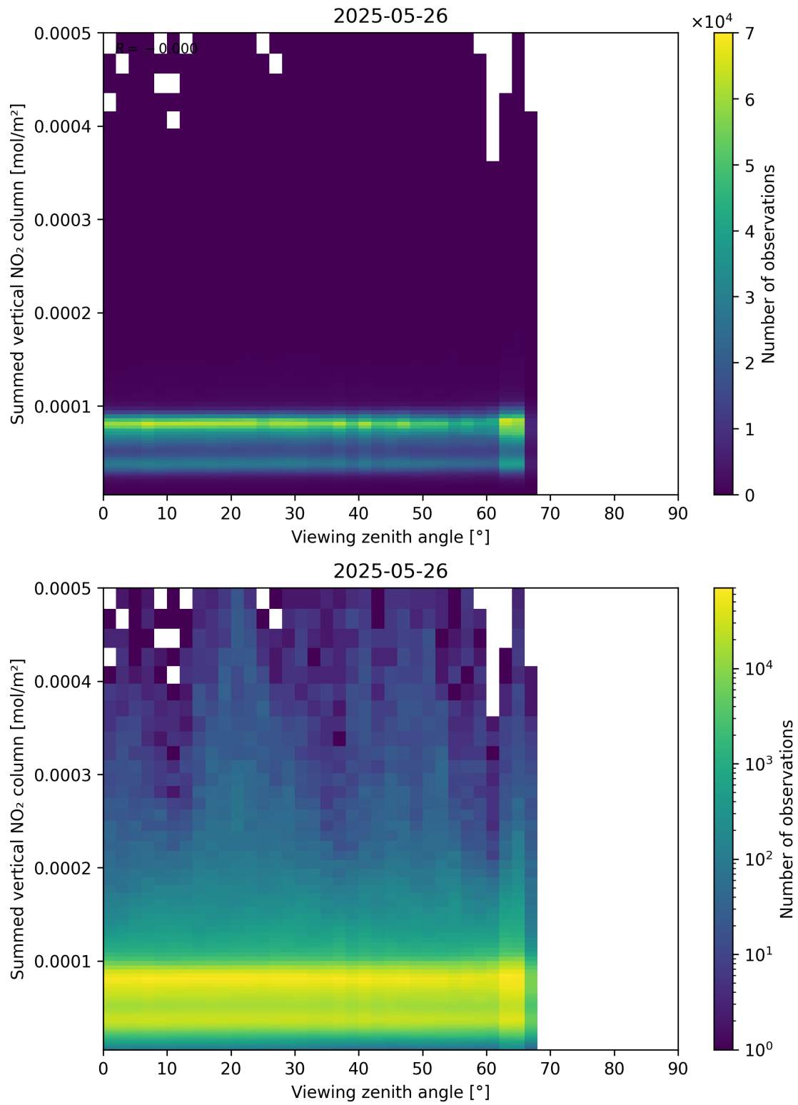
Figure 165: Scatter density plot of “Viewing zenith angle” against “Summed vertical NO 2 column” for 2025-05-26 to 2025-05-27.
