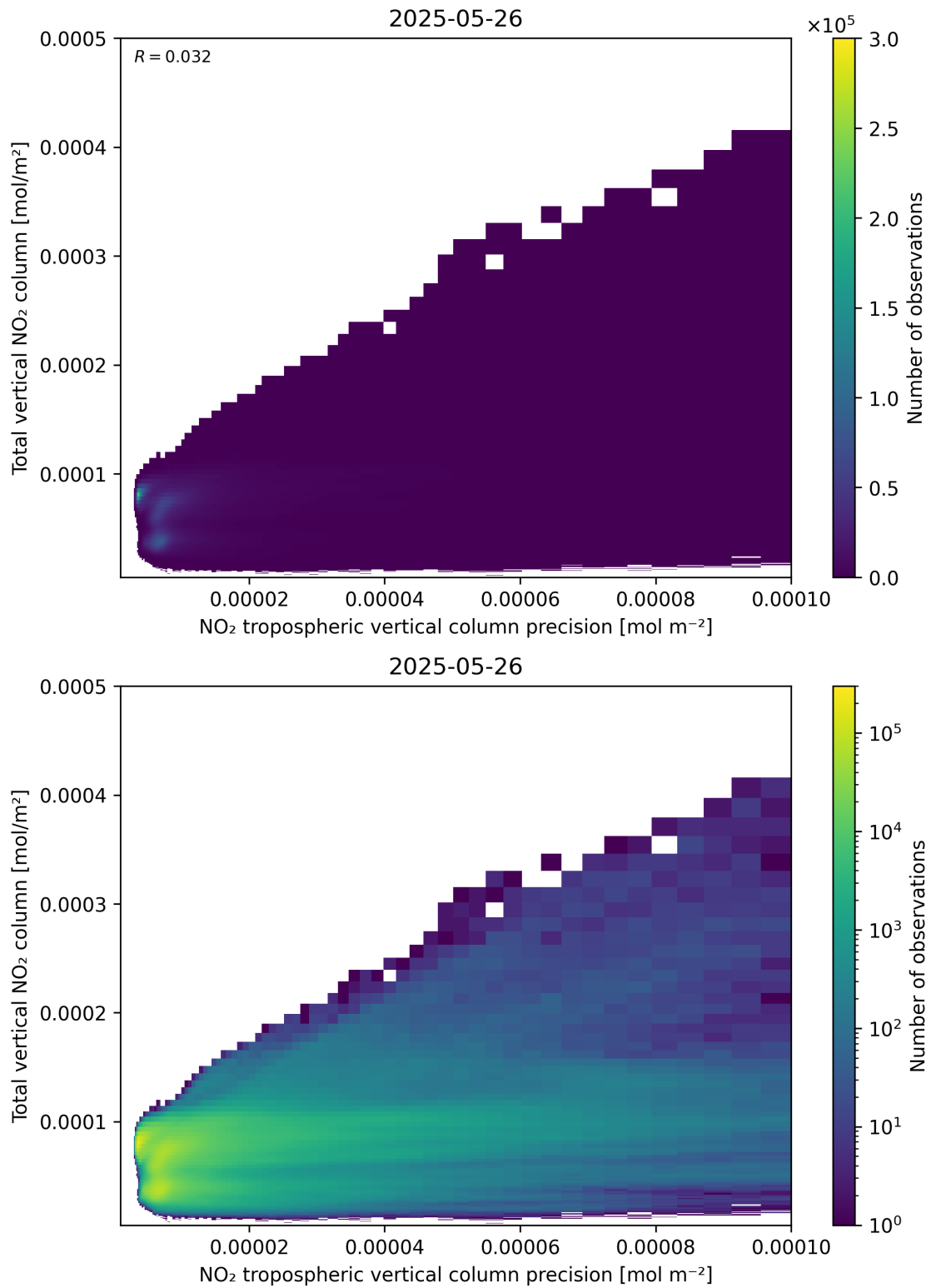
Figure 138: Scatter density plot of “NO 2 tropospheric vertical column precision” against “Total vertical NO 2 column” for 2025-05-26 to 2025-05-27.
