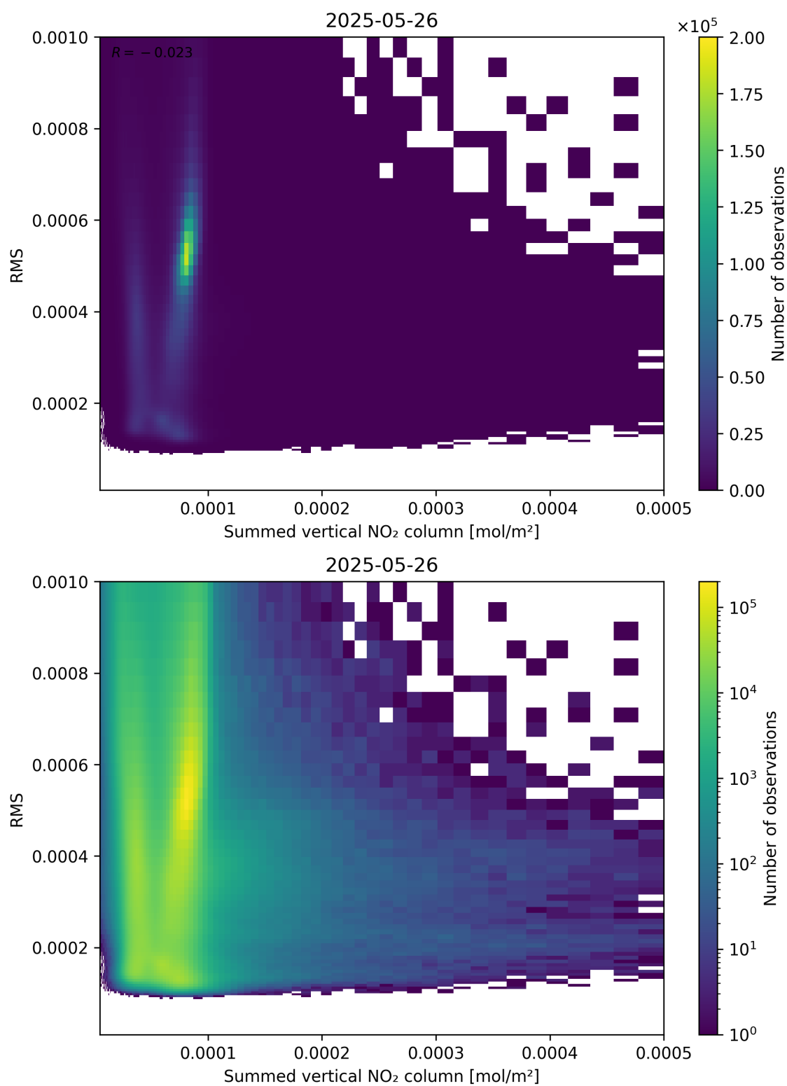
Figure 109: Scatter density plot of “Summed vertical NO 2 column” against “RMS” for 2025-05-26 to 2025-05-27.
