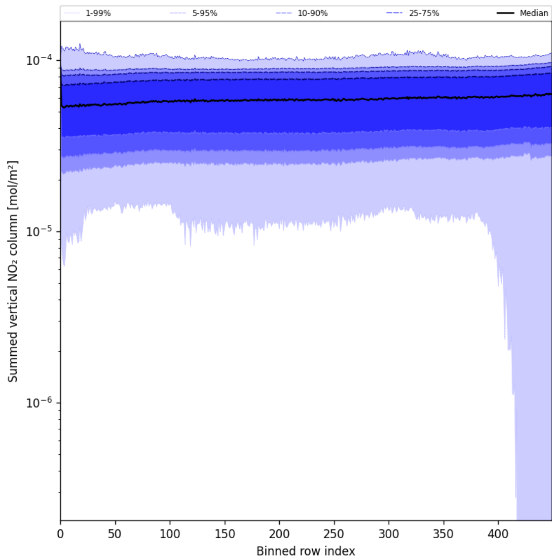
Figure 57: Along track statistics of “Summed vertical NO 2 column” for 2025-05-26 to 2025-05-27
