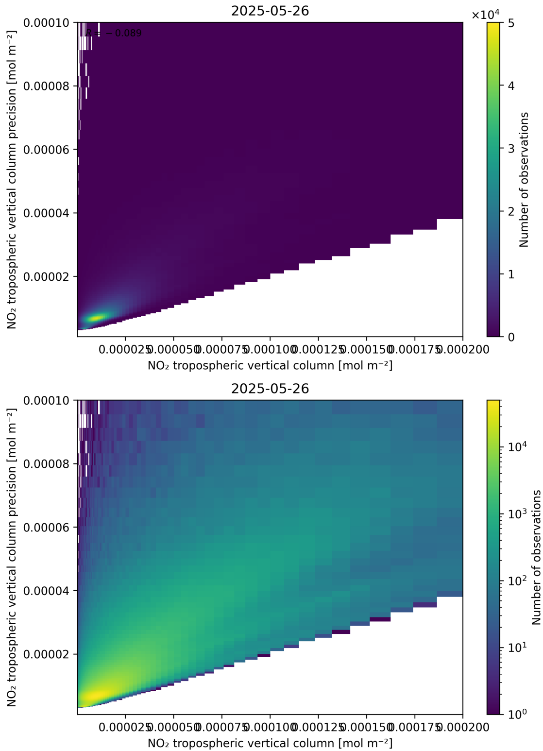
Figure 130: Scatter density plot of “NO 2 tropospheric vertical column” against “NO 2 tropospheric vertical column precision” for 2025-05-26 to 2025-05-27.
