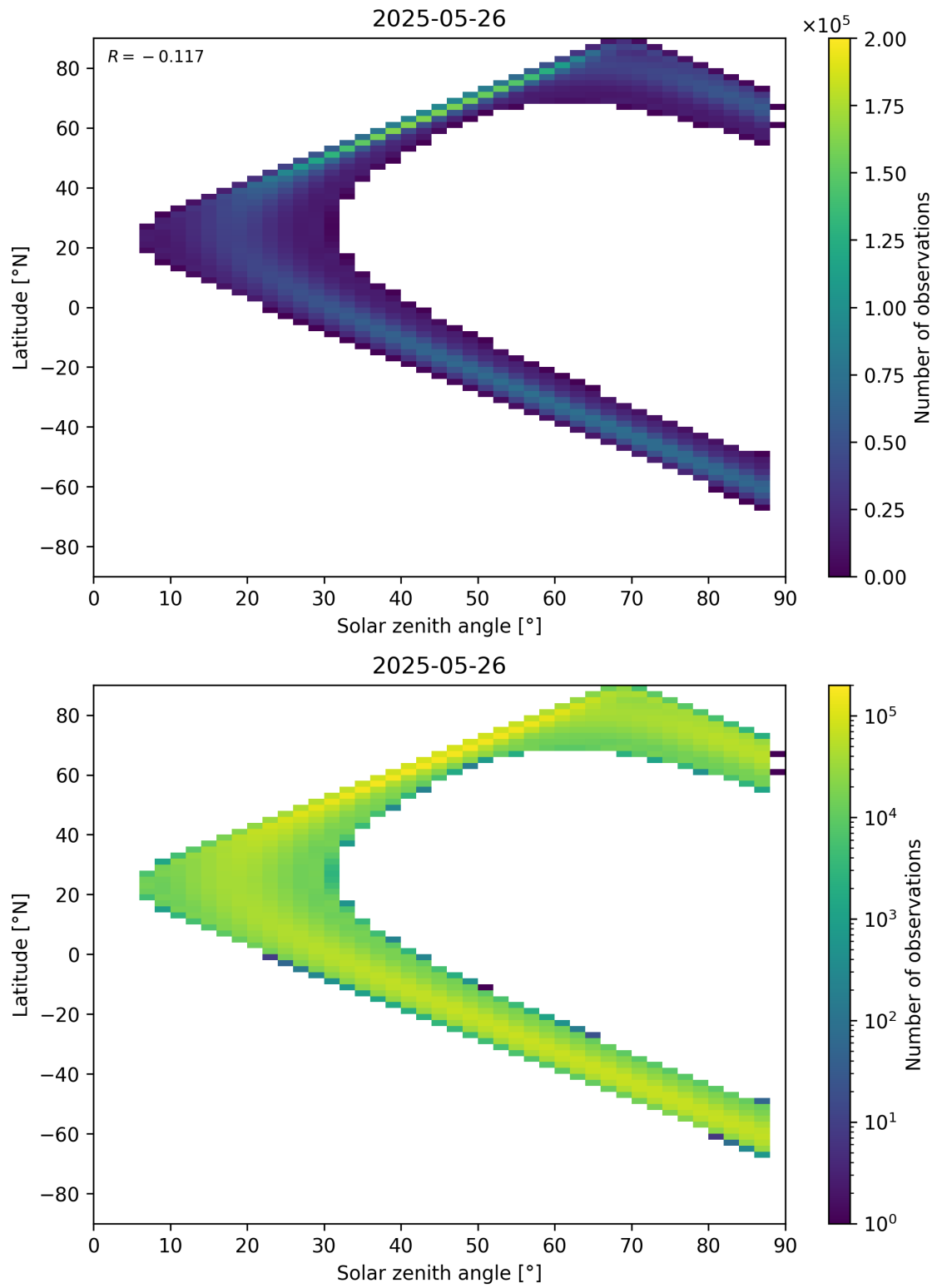
Figure 149: Scatter density plot of “Solar zenith angle” against “Latitude” for 2025-05-26 to 2025-05-27.
