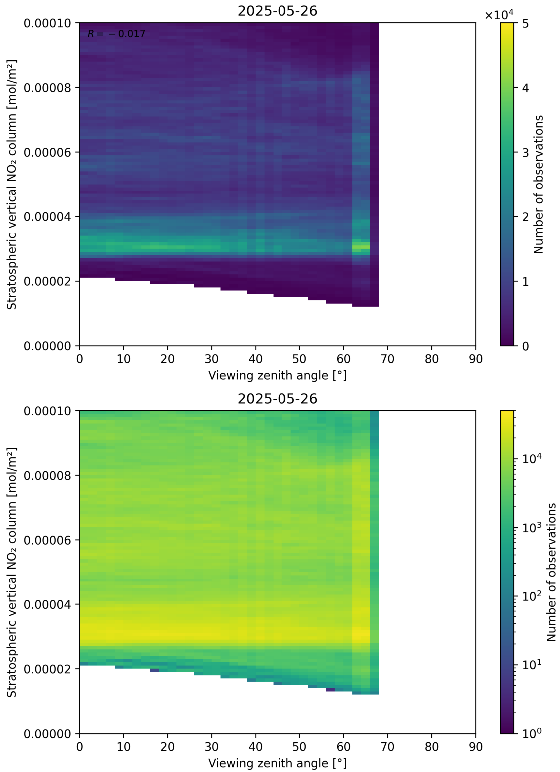
Figure 164: Scatter density plot of “Viewing zenith angle” against “Stratospheric vertical NO 2 column” for 2025-05-26 to 2025-05-27.
