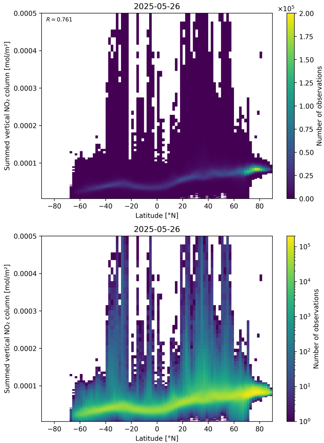
Figure 88: Scatter density plot of “Latitude” against “Summed vertical NO 2 column” for 2025-05-26 to 2025-05-27.
