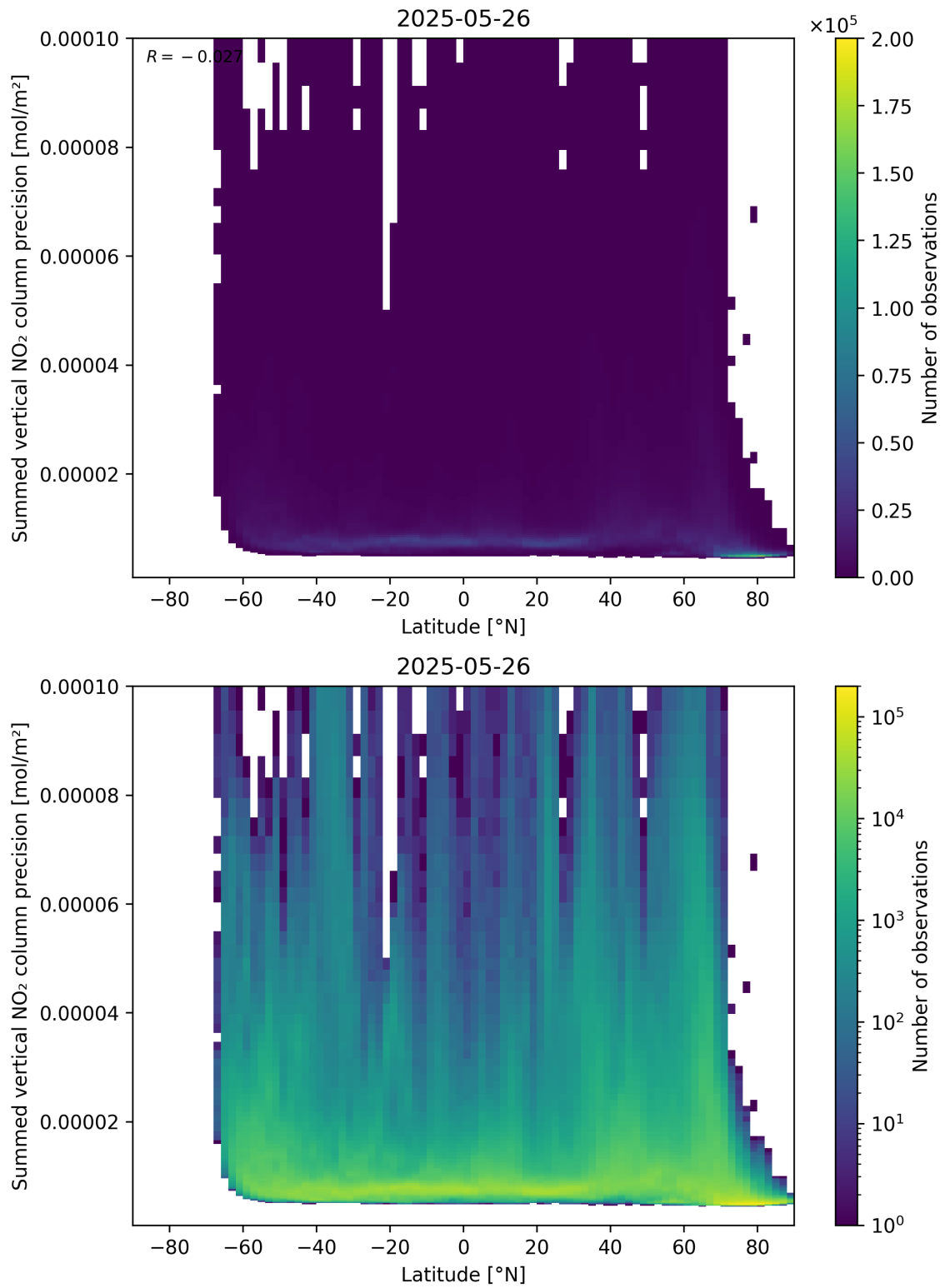
Figure 89: Scatter density plot of “Latitude” against “Summed vertical NO 2 column precision” for 2025-05-26 to 2025-05-27.
