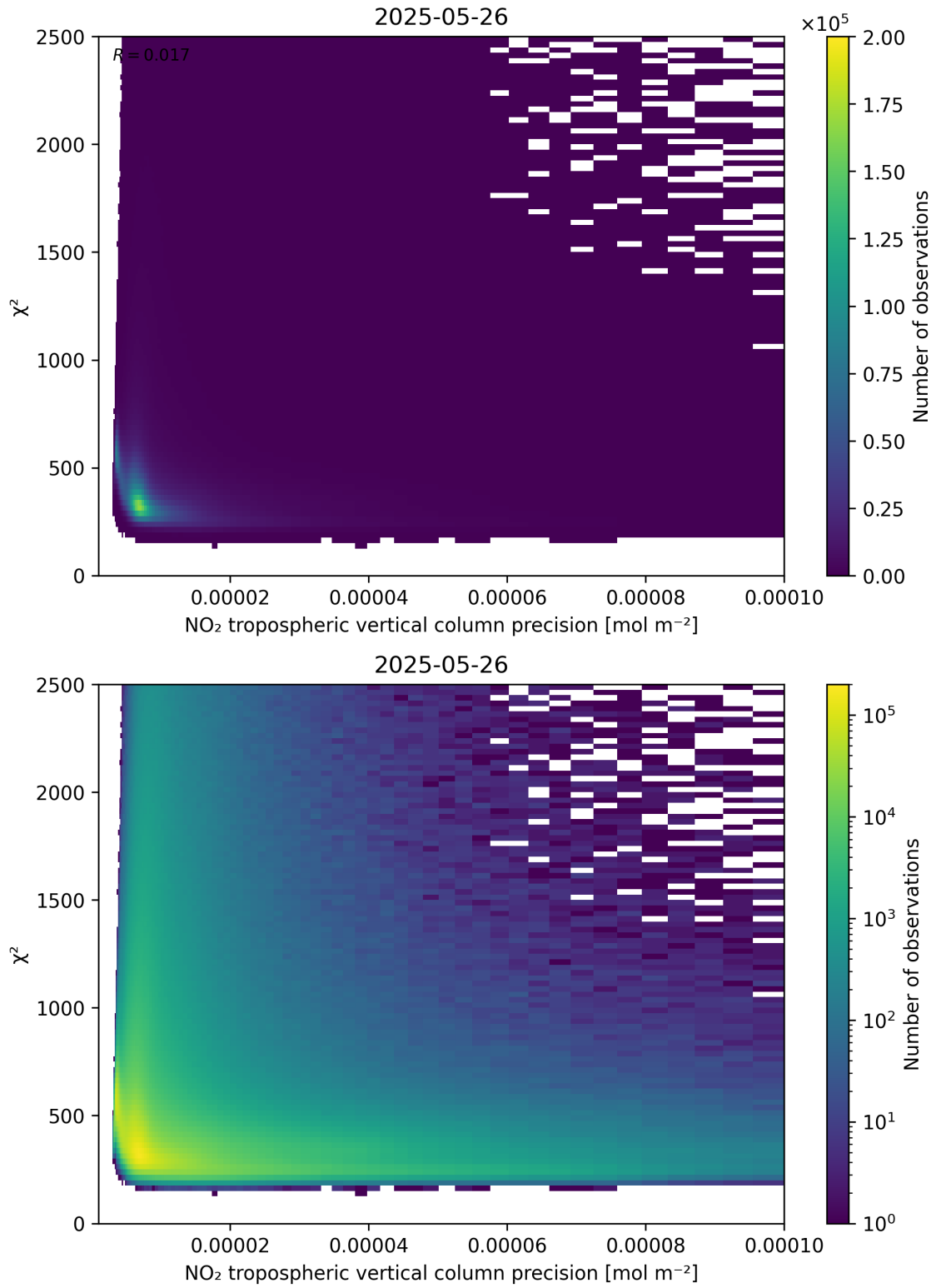
Figure 134: Scatter density plot of “NO 2 tropospheric vertical column precision” against “ \chi^2 ” for 2025-05-26 to 2025-05-27.
