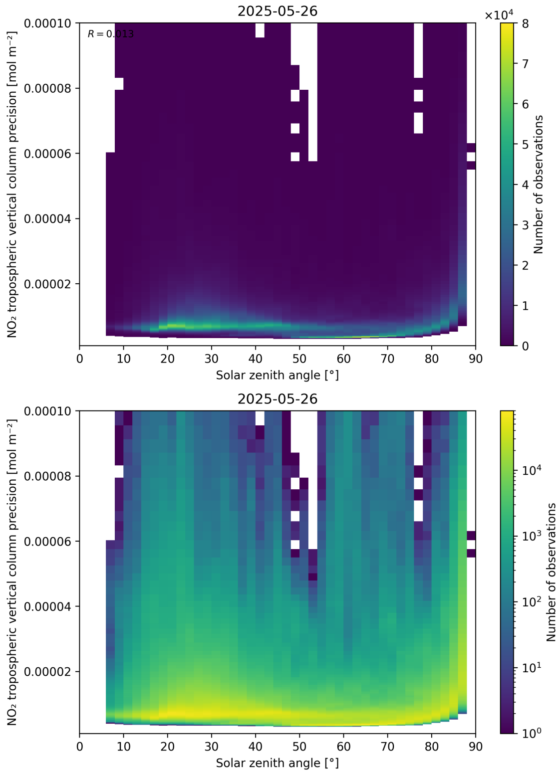
Figure 156: Scatter density plot of “Solar zenith angle” against “NO 2 tropospheric vertical column precision” for 2025-05-26 to 2025-05-27.
