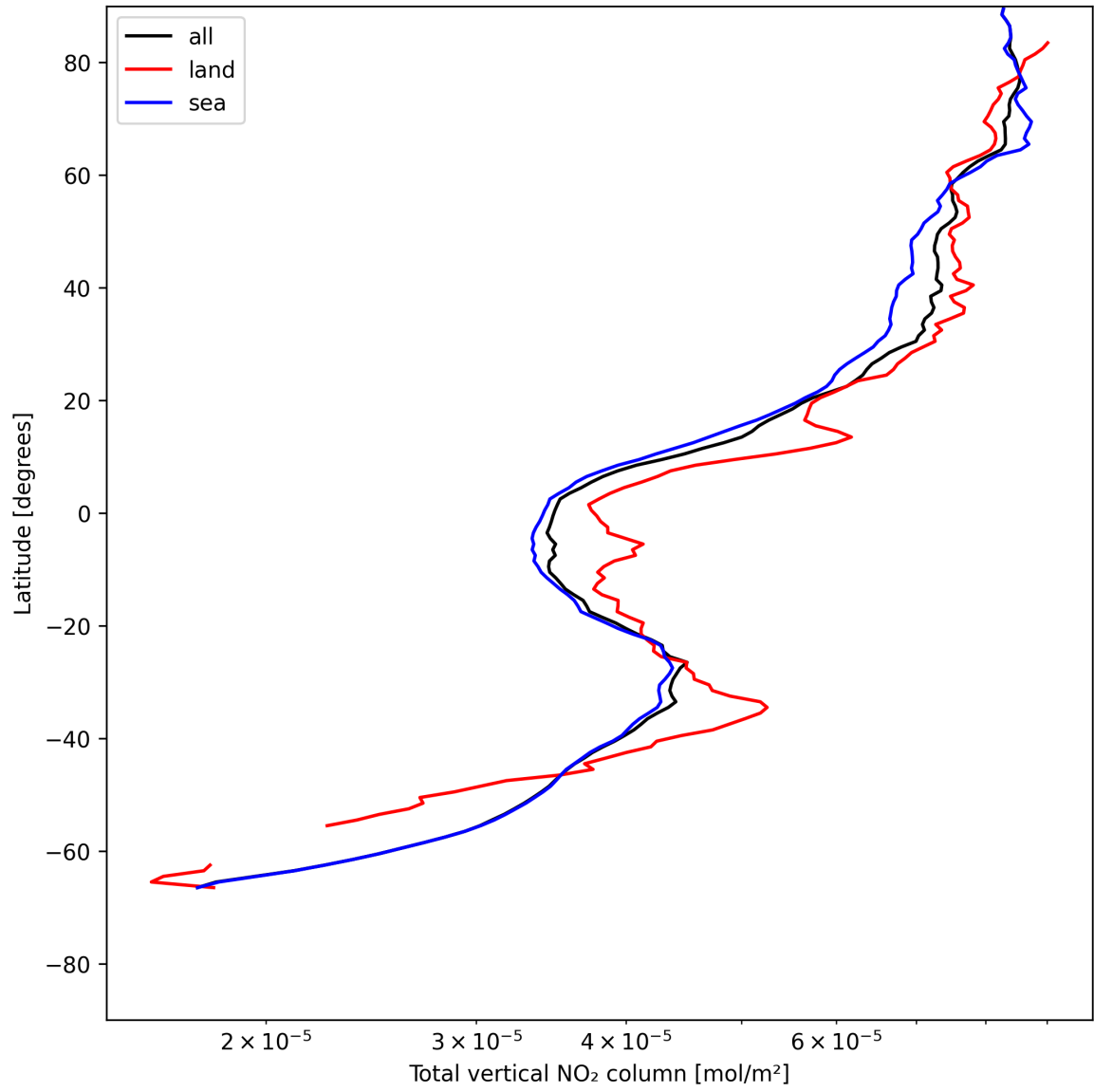
Figure 21: Zonal average of “Total vertical NO 2 column” for 2025-05-26 to 2025-05-27.
