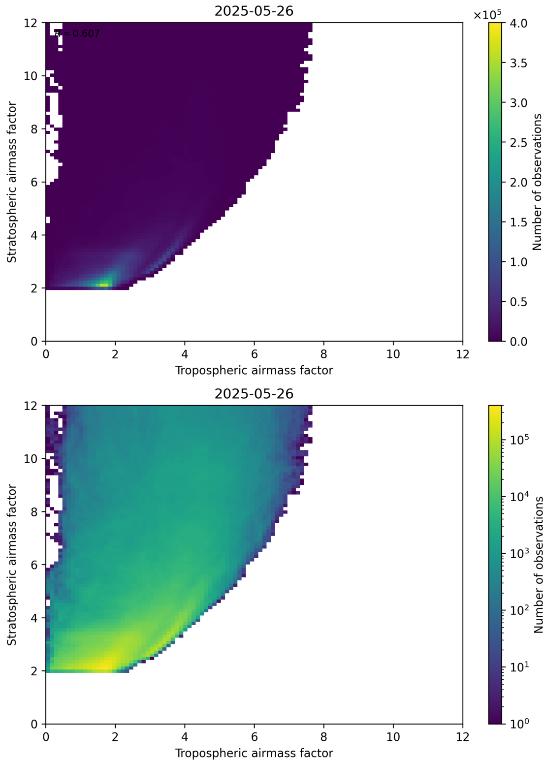
Figure 71: Scatter density plot of “Tropospheric airmass factor” against “Stratospheric airmass factor” for 2025-05-26 to 2025-05-27.
