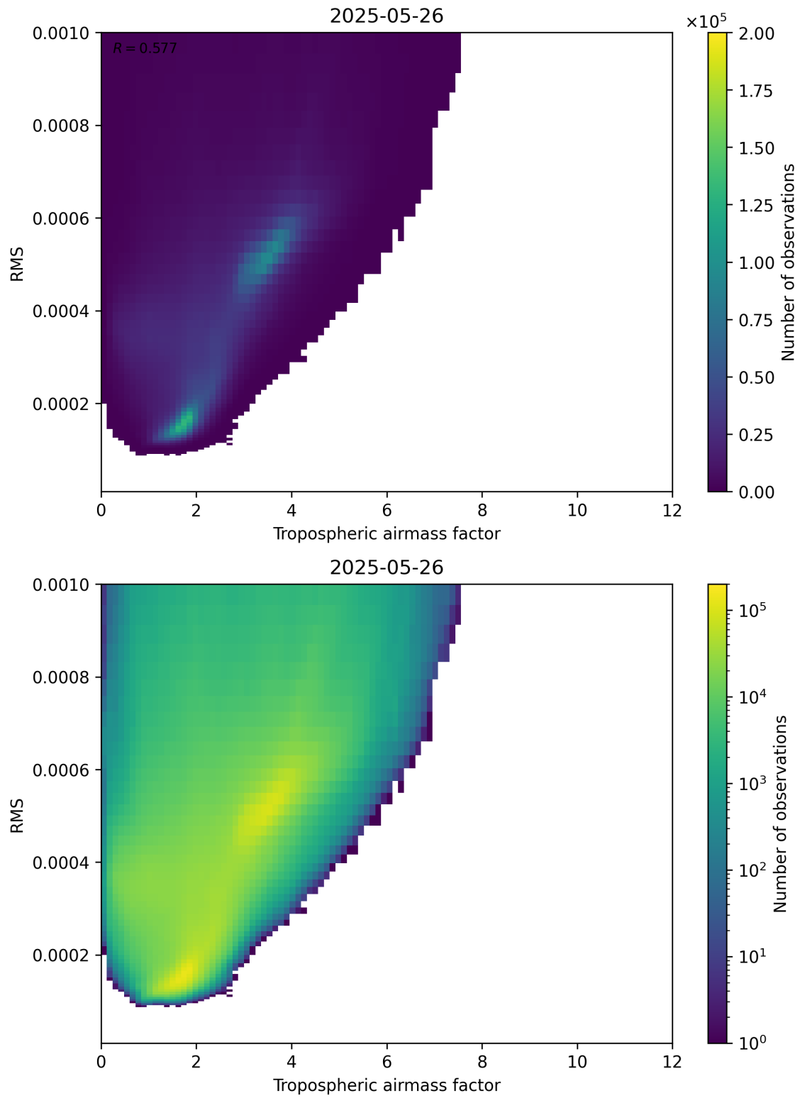
Figure 79: Scatter density plot of “Tropospheric airmass factor” against “RMS” for 2025-05-26 to 2025-05-27.
