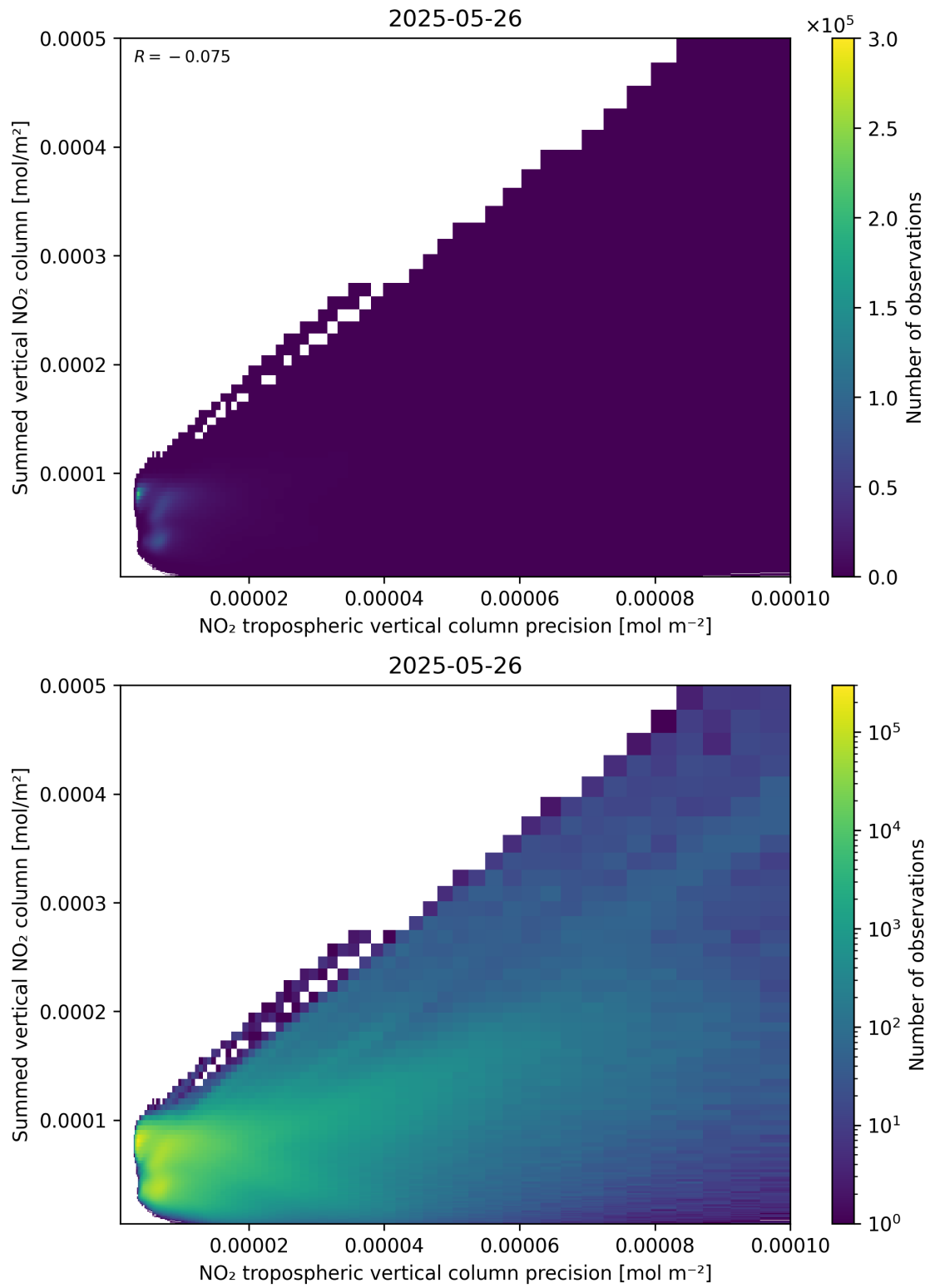
Figure 136: Scatter density plot of “NO 2 tropospheric vertical column precision” against “Summed vertical NO 2 column” for 2025-05-26 to 2025-05-27.
