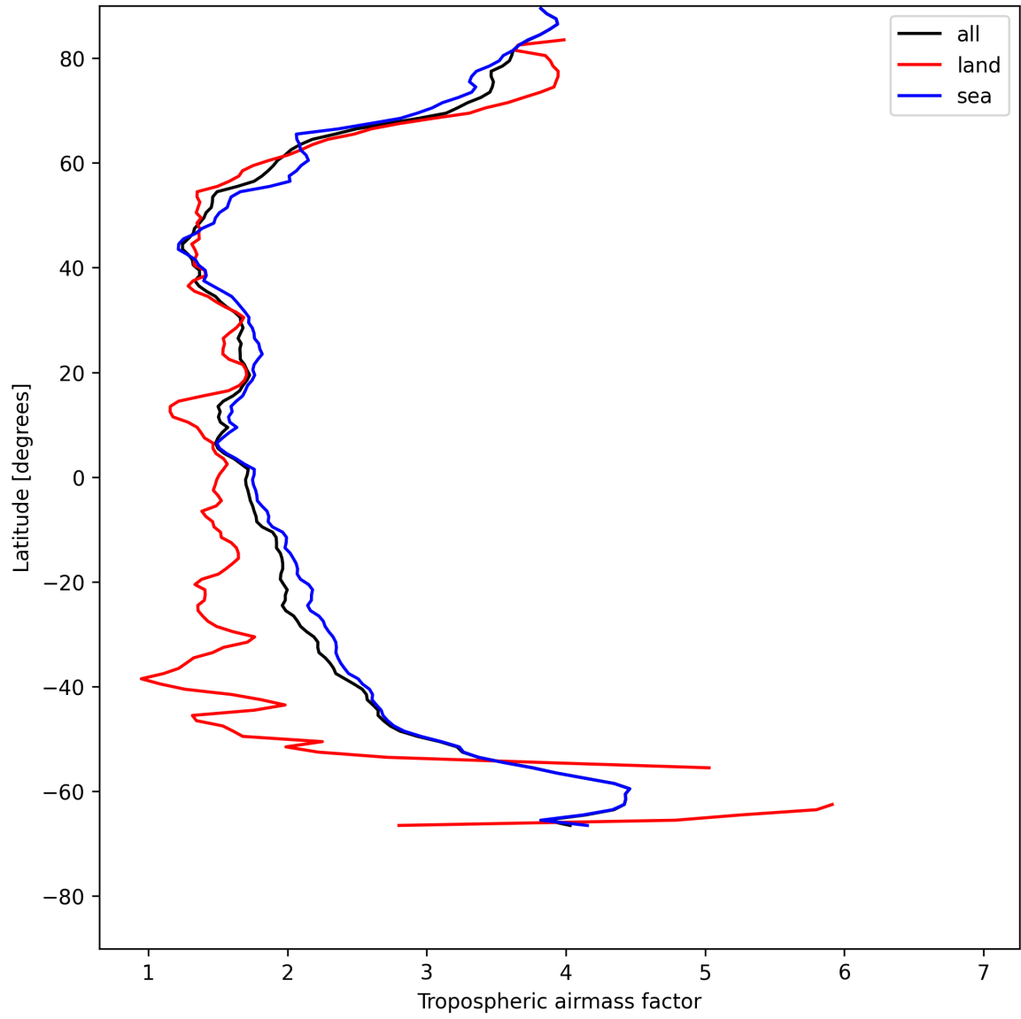
Figure 14: Zonal average of “Tropospheric airmass factor” for 2025-05-26 to 2025-05-27.
