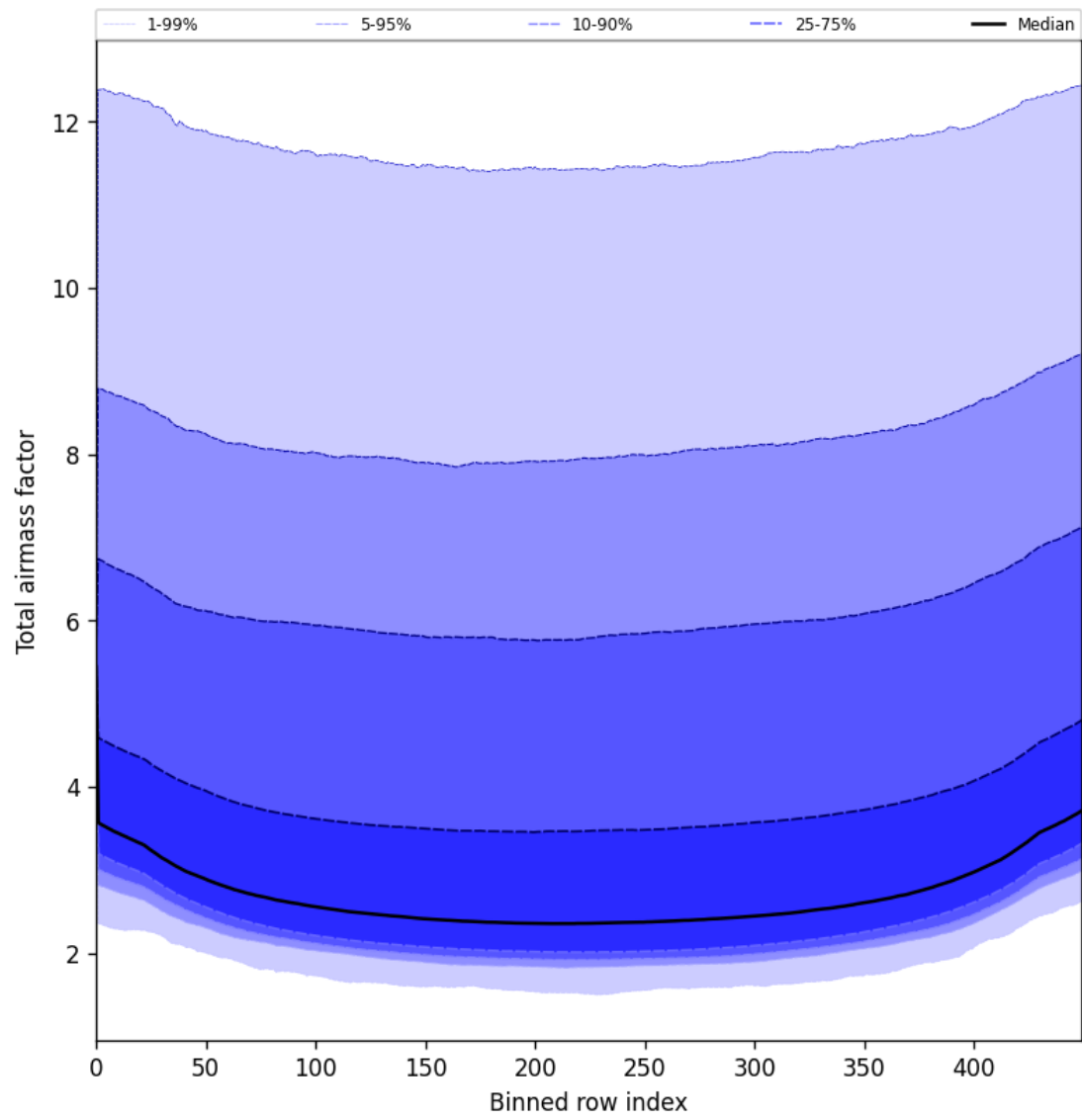
Figure 49: Along track statistics of “Total airmass factor” for 2025-05-26 to 2025-05-27
