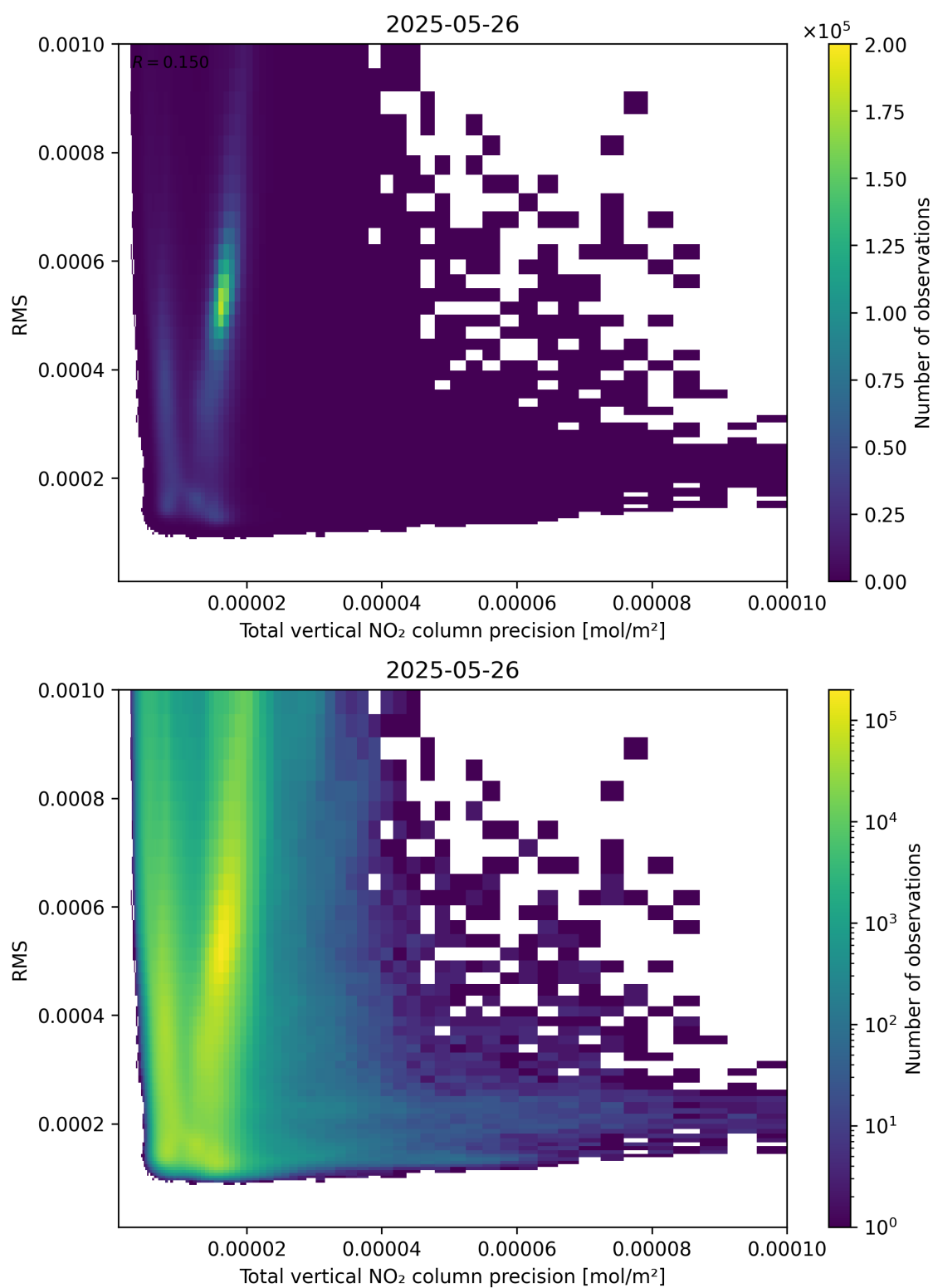
Figure 119: Scatter density plot of “Total vertical NO 2 column precision” against “RMS” for 2025-05-26 to 2025-05-27.
