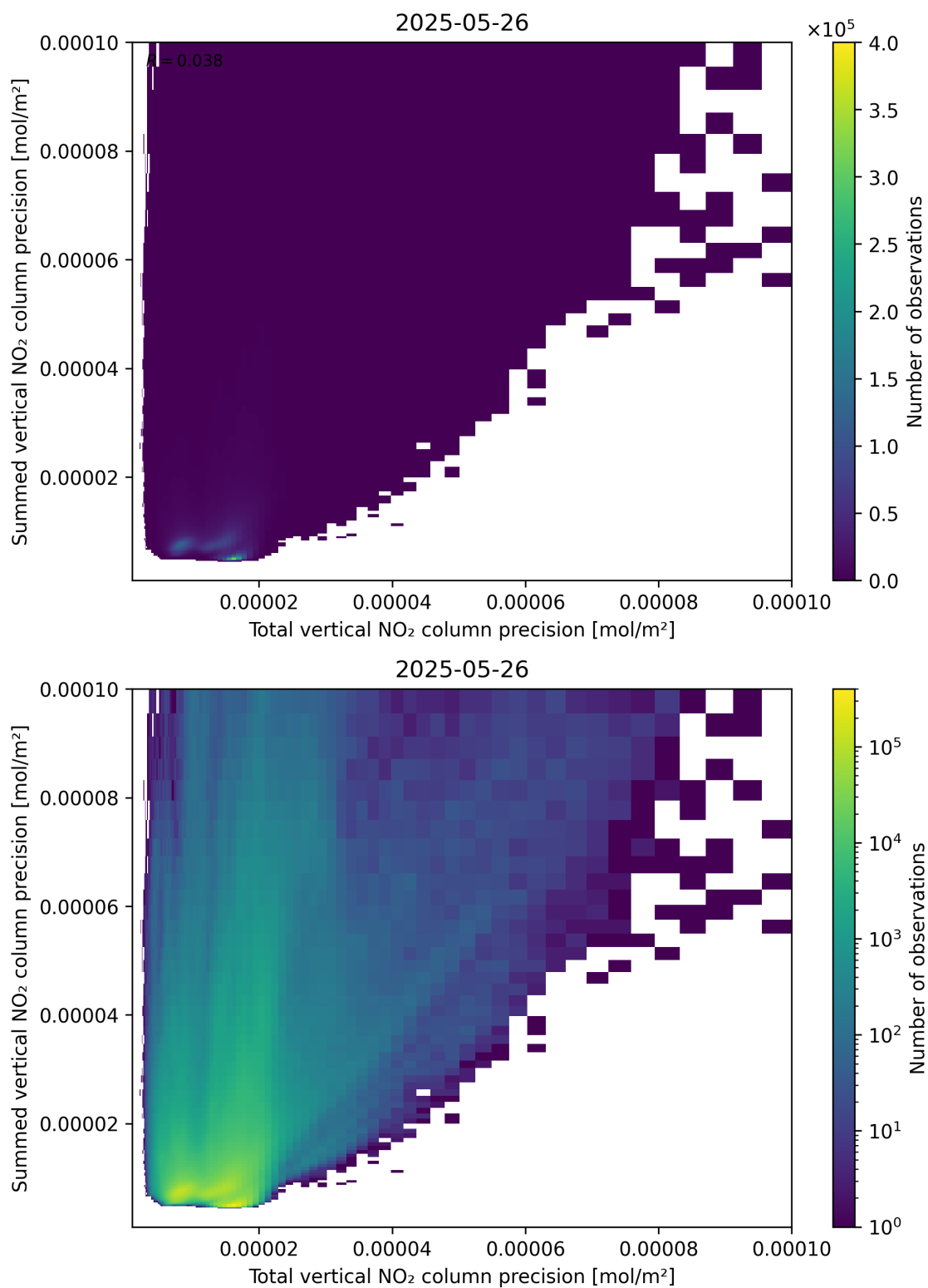
Figure 118: Scatter density plot of “Total vertical NO 2 column precision” against “Summed vertical NO 2 column precision” for 2025-05-26 to 2025-05-27.
