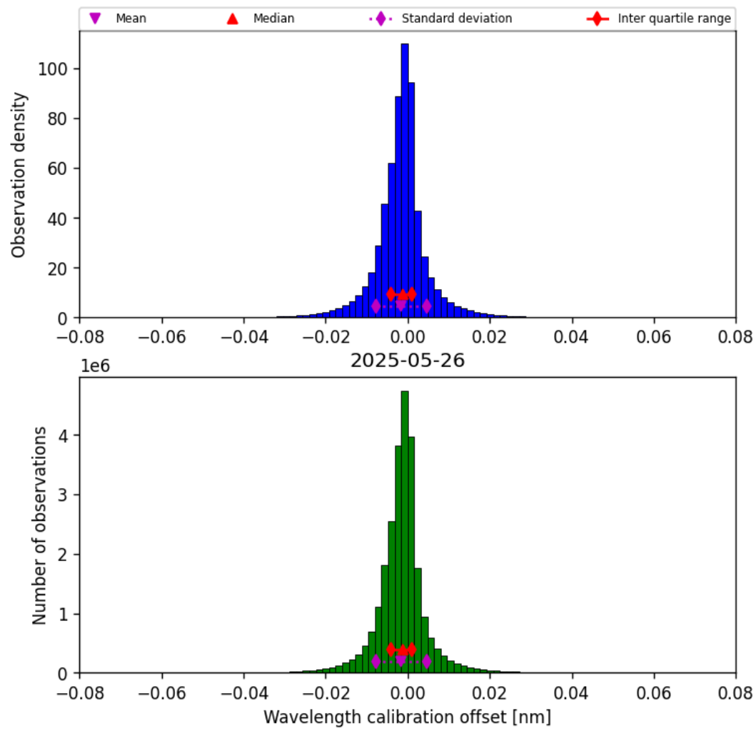
Figure 35: Histogram of “Wavelength calibration offset” for 2025-05-26 to 2025-05-27
