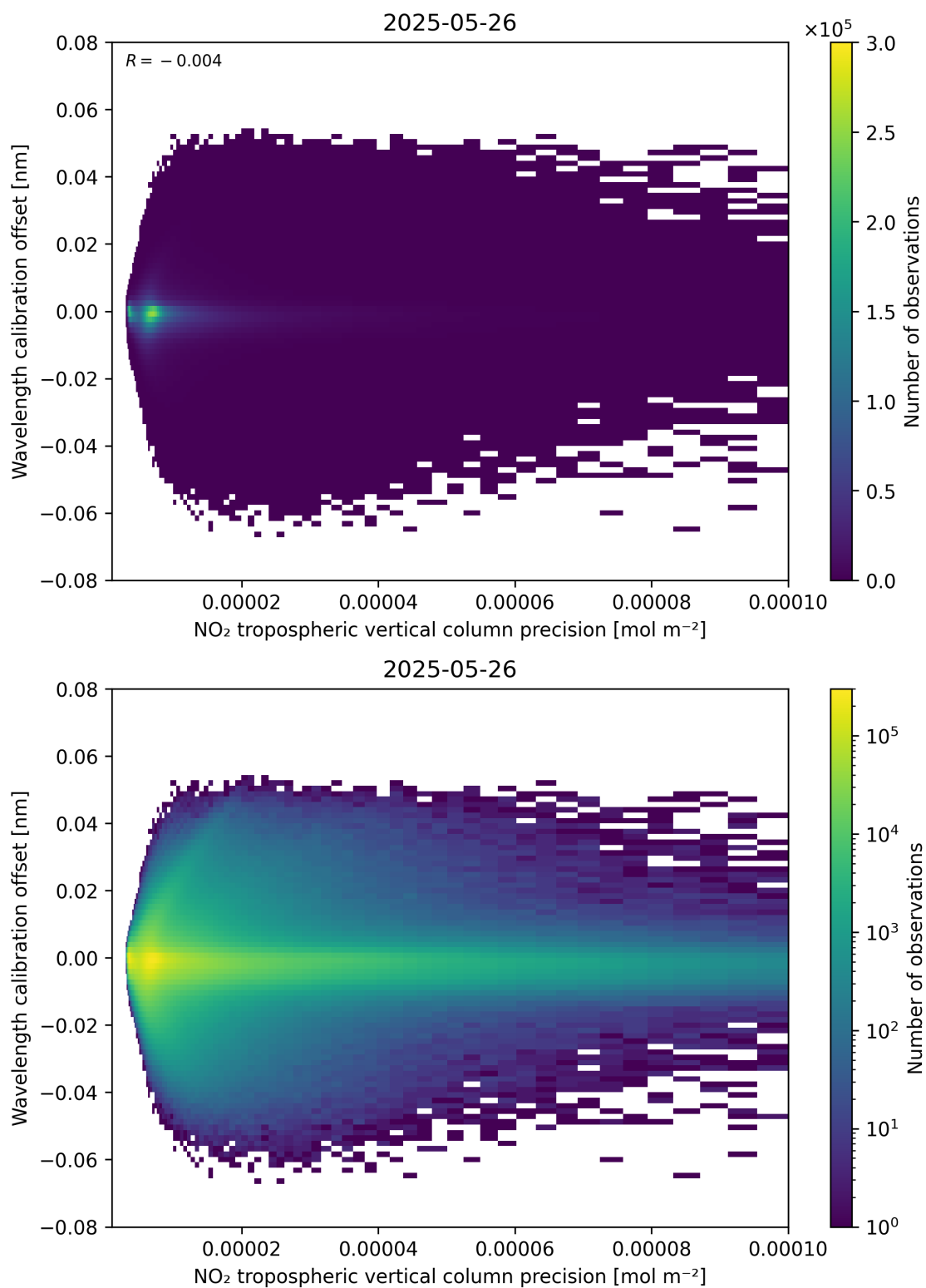
Figure 141: Scatter density plot of “NO 2 tropospheric vertical column precision” against “Wavelength calibration offset” for 2025-05-26 to 2025-05-27.
