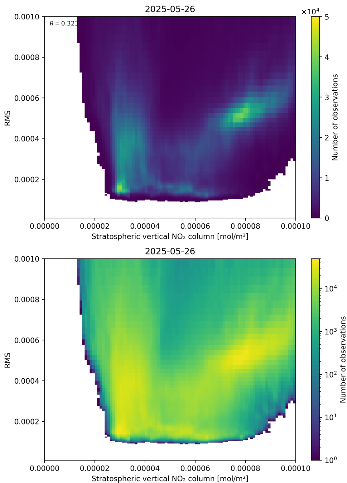
Figure 102: Scatter density plot of “Stratospheric vertical NO 2 column” against “RMS” for 2025-05-26 to 2025-05-27.
