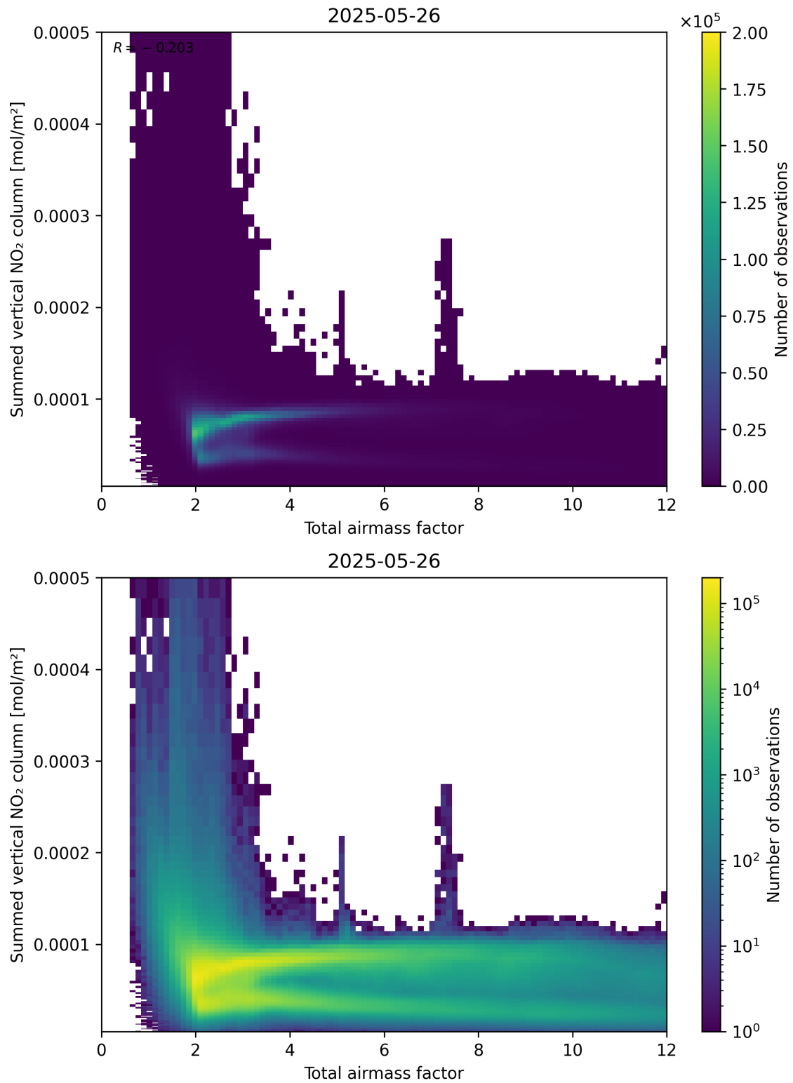
Figure 65: Scatter density plot of “Total airmass factor” against “Summed vertical NO 2 column” for 2025-05-26 to 2025-05-27.
