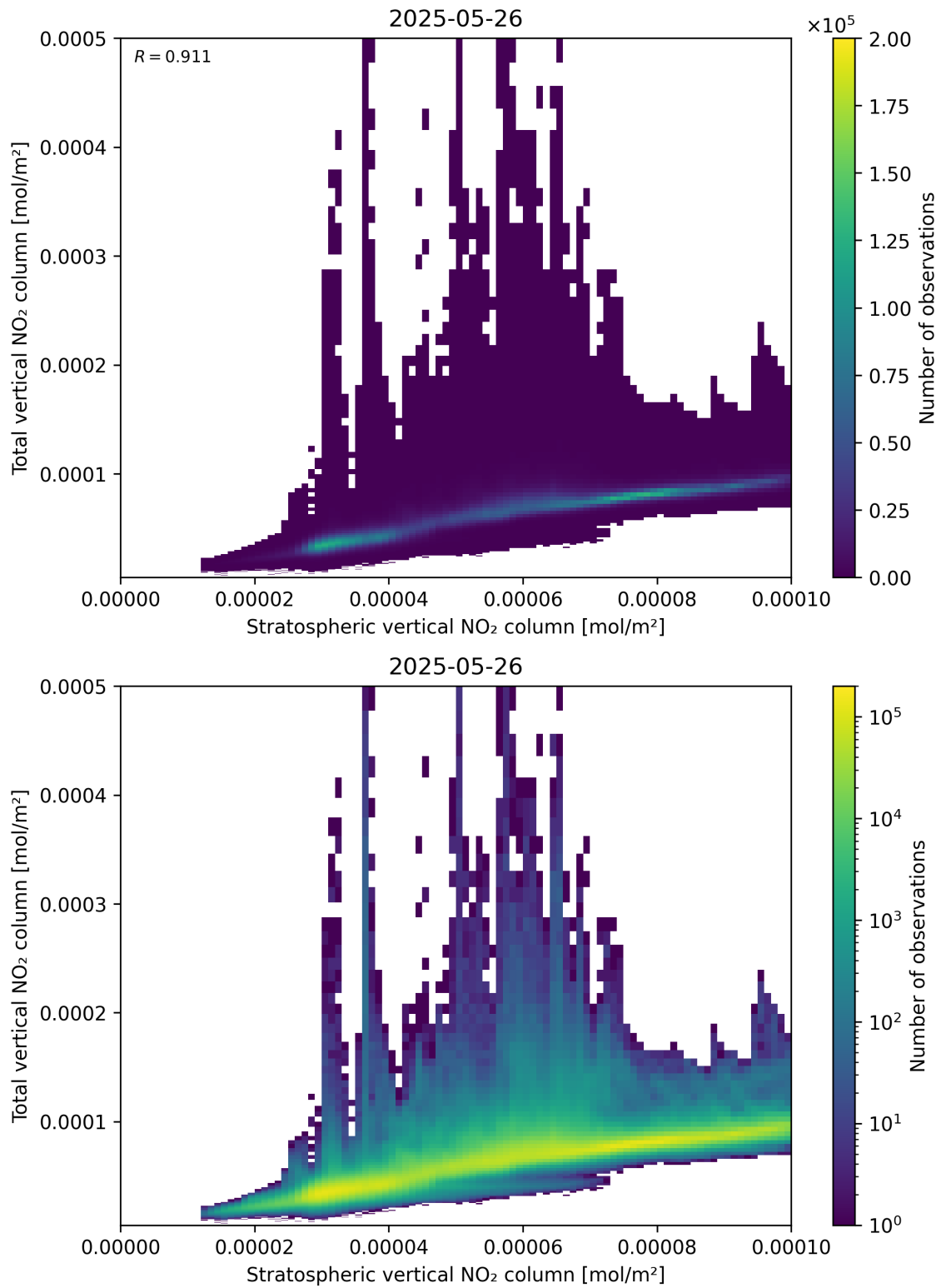
Figure 100: Scatter density plot of “Stratospheric vertical NO 2 column” against “Total vertical NO 2 column” for 2025-05-26 to 2025-05-27.
