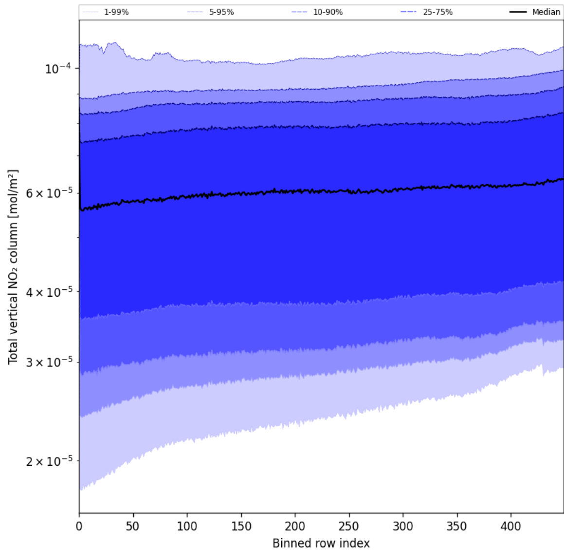
Figure 55: Along track statistics of “Total vertical NO 2 column” for 2025-05-26 to 2025-05-27
