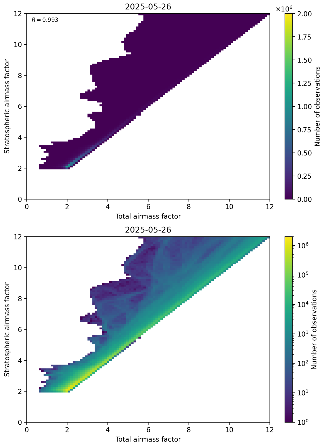
Figure 62: Scatter density plot of “Total airmass factor” against “Stratospheric airmass factor” for 2025-05-26 to 2025-05-27.
