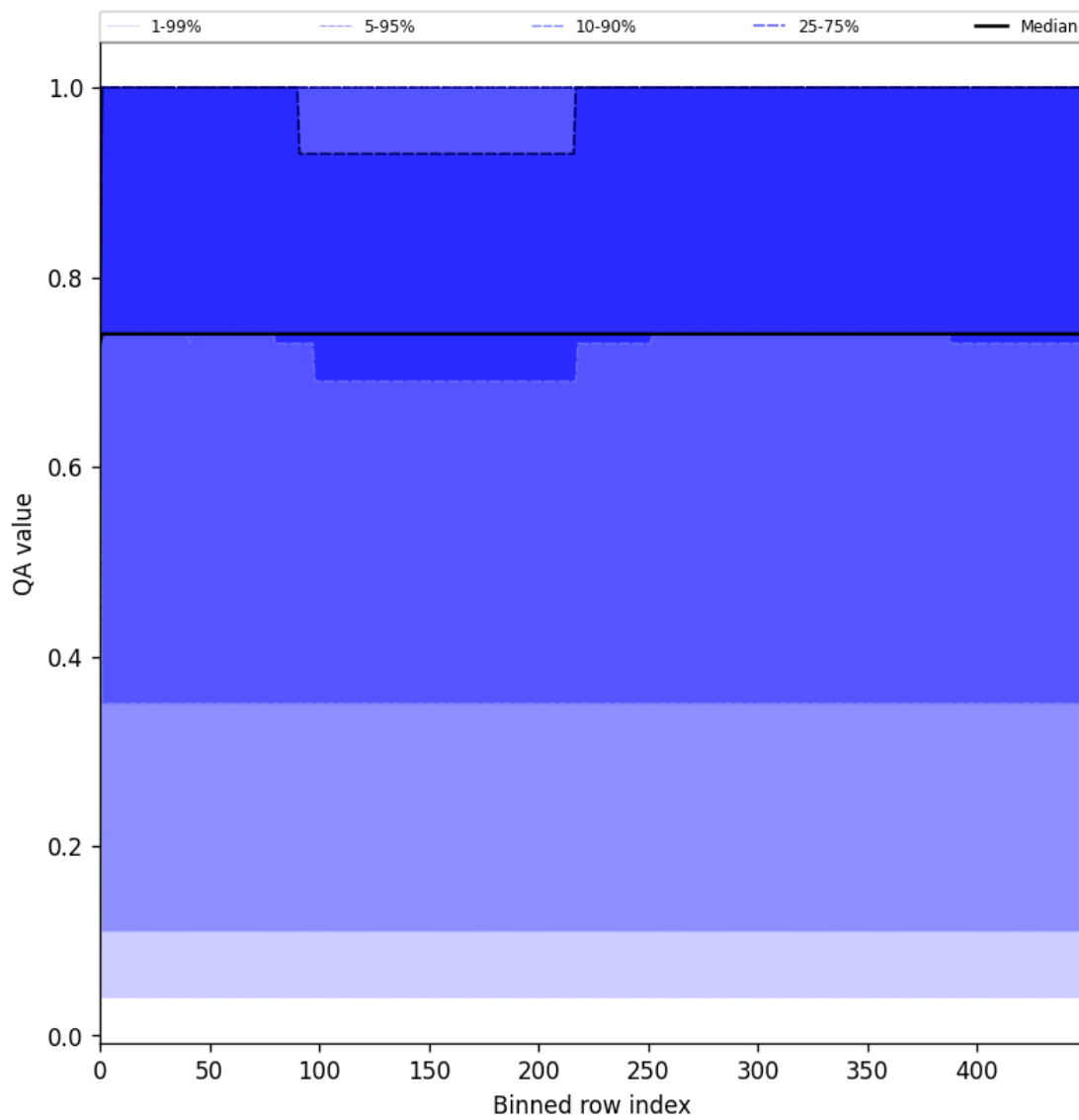
Figure 45: Along track statistics of “QA value” for 2025-05-26 to 2025-05-27
