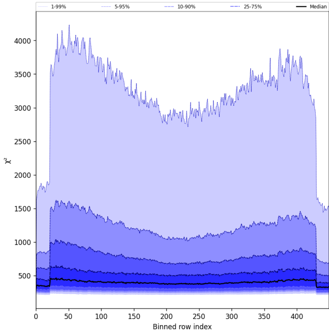
Figure 59: Along track statistics of “ \chi^2 ” for 2025-05-27 to 2025-05-29
