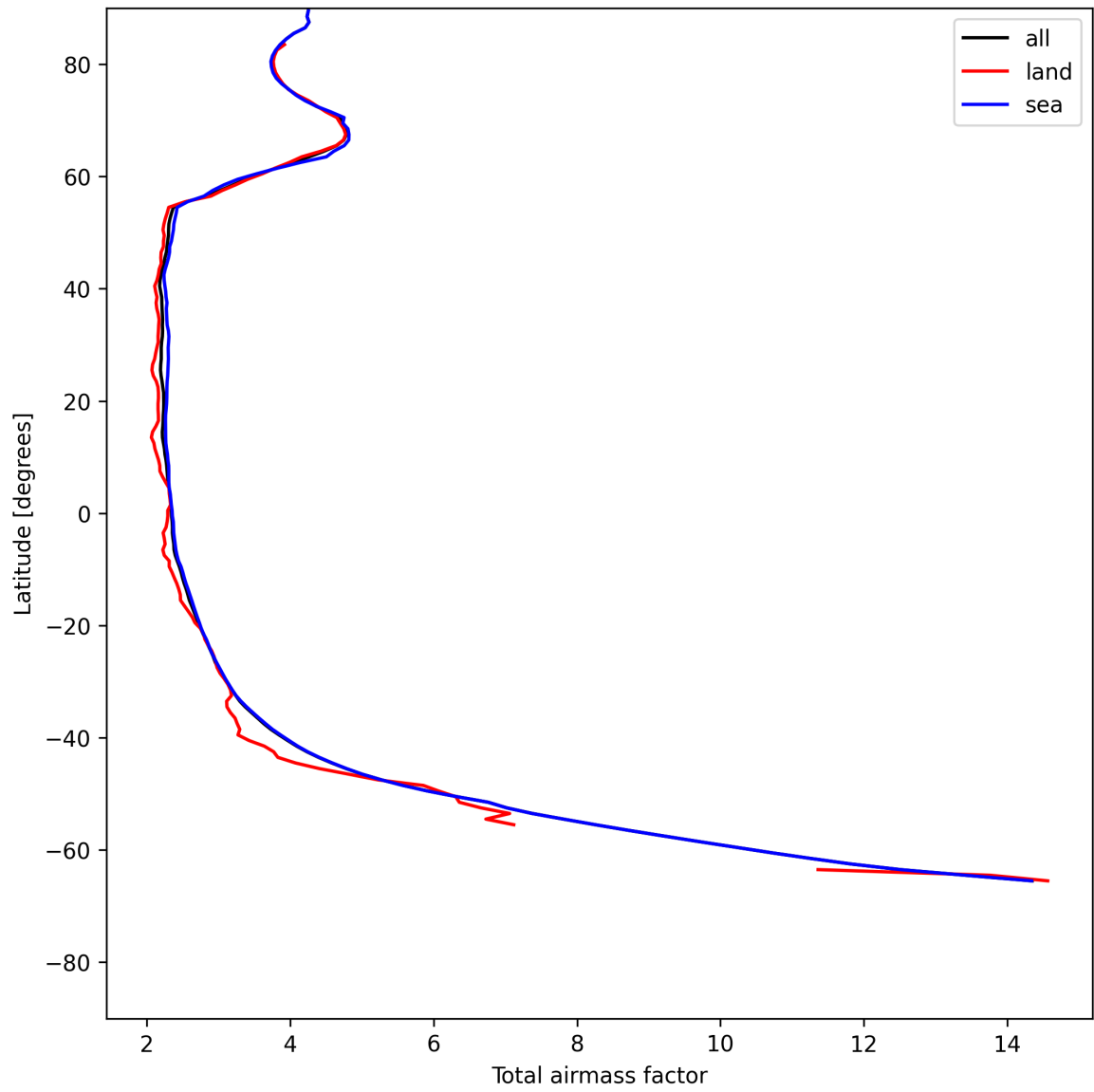
Figure 15: Zonal average of “Total airmass factor” for 2025-05-27 to 2025-05-29.
