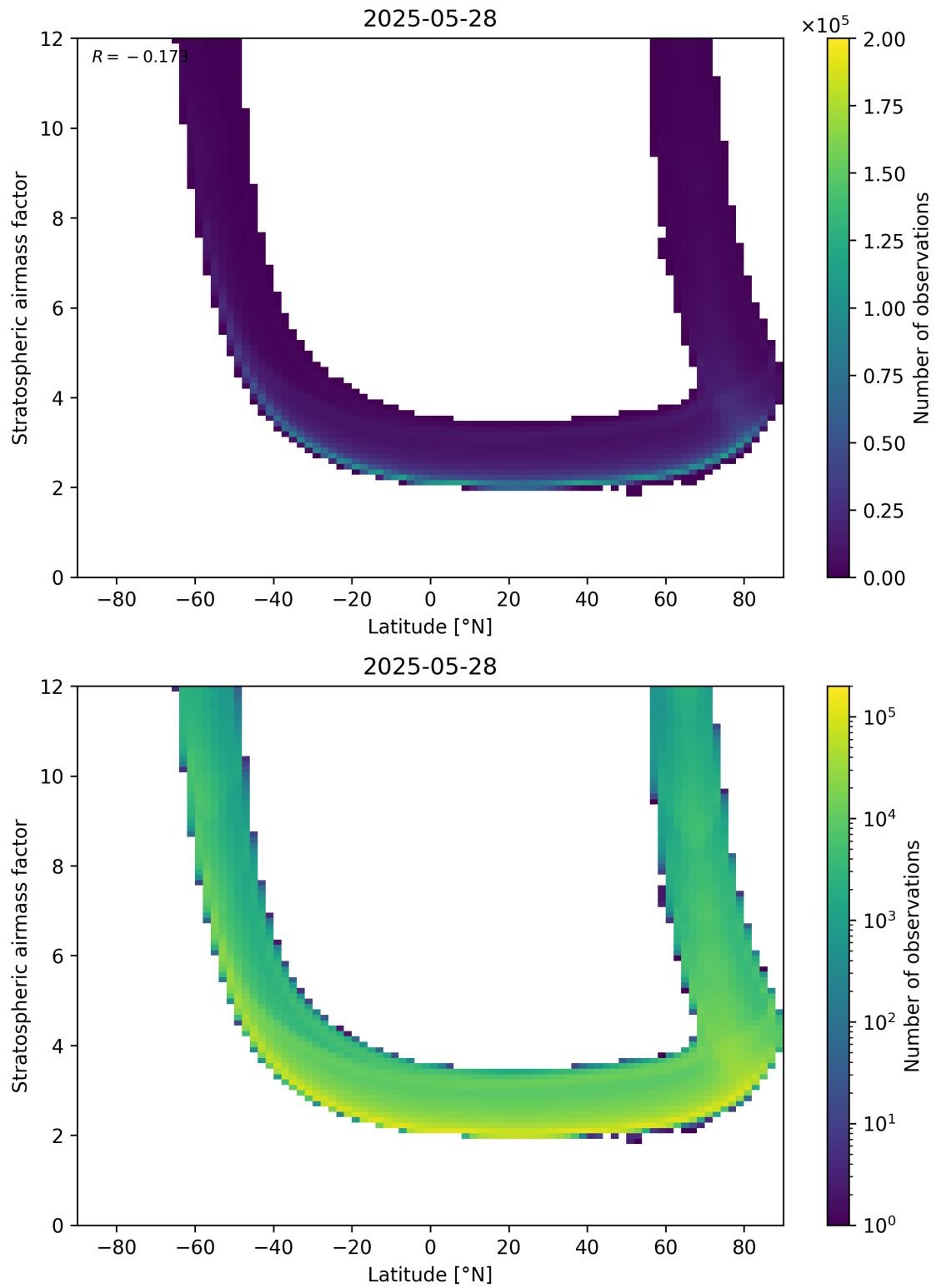
Figure 83: Scatter density plot of “Latitude” against “Stratospheric air mass factor” for 2025-05-27 to 2025-05-29.
