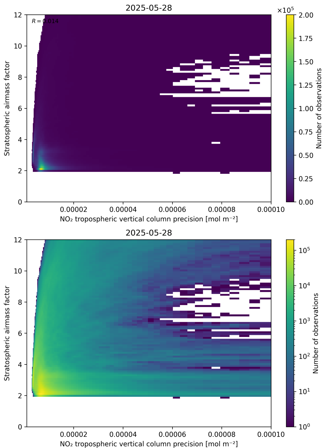
Figure 131: Scatter density plot of “NO 2 tropospheric vertical column precision” against “Stratospheric airmass factor” for 2025-05-27 to 2025-05-29.
