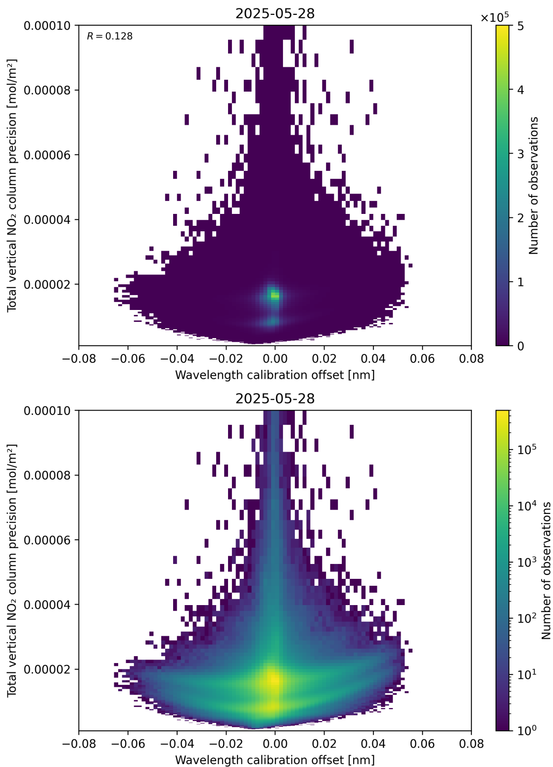
Figure 180: Scatter density plot of “Wavelength calibration offset” against “Total vertical NO 2 column precision” for 2025-05-27 to 2025-05-29.
