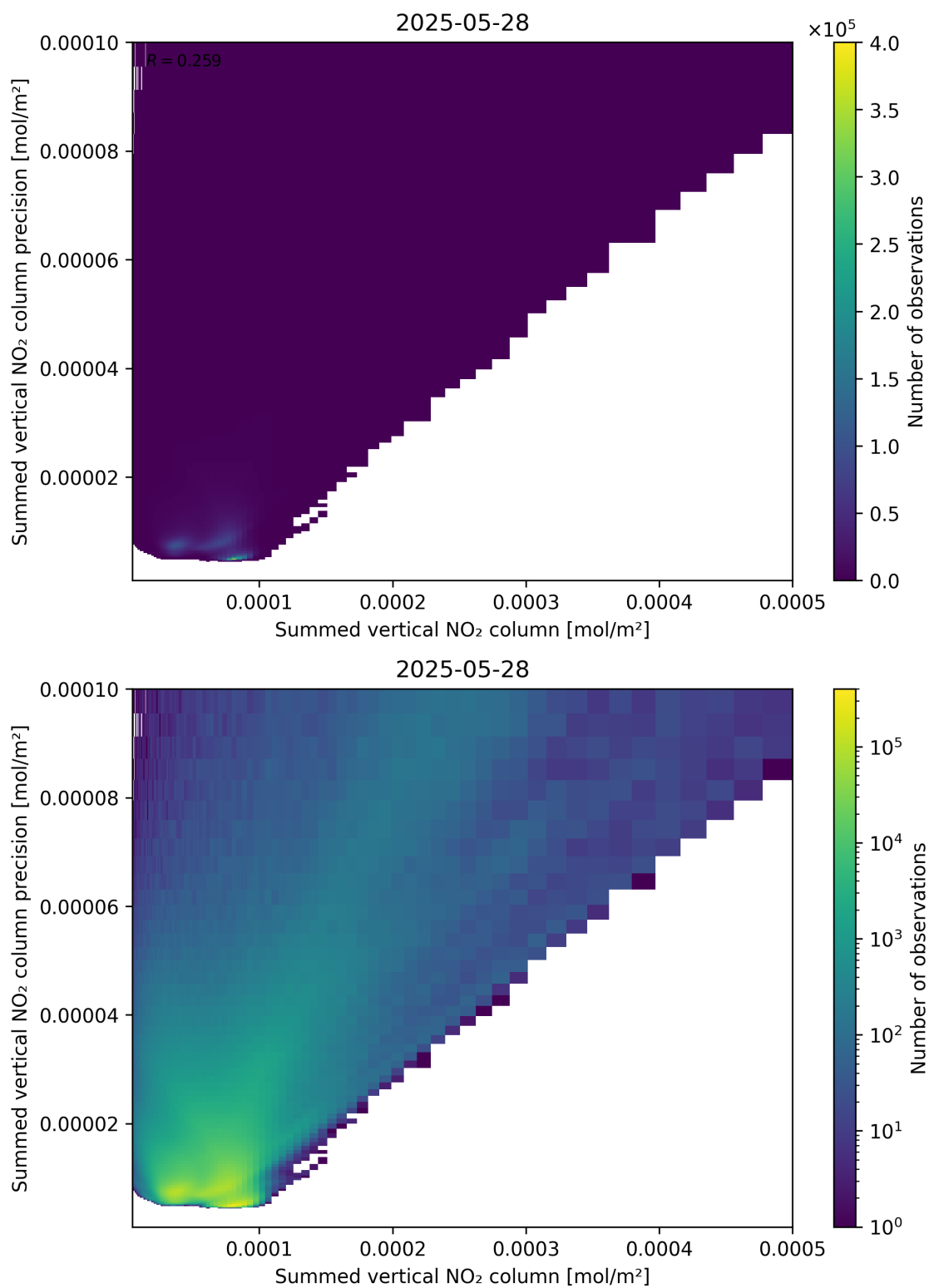
Figure 105: Scatter density plot of “Summed vertical NO 2 column” against “Summed vertical NO 2 column precision” for 2025-05-27 to 2025-05-29.
