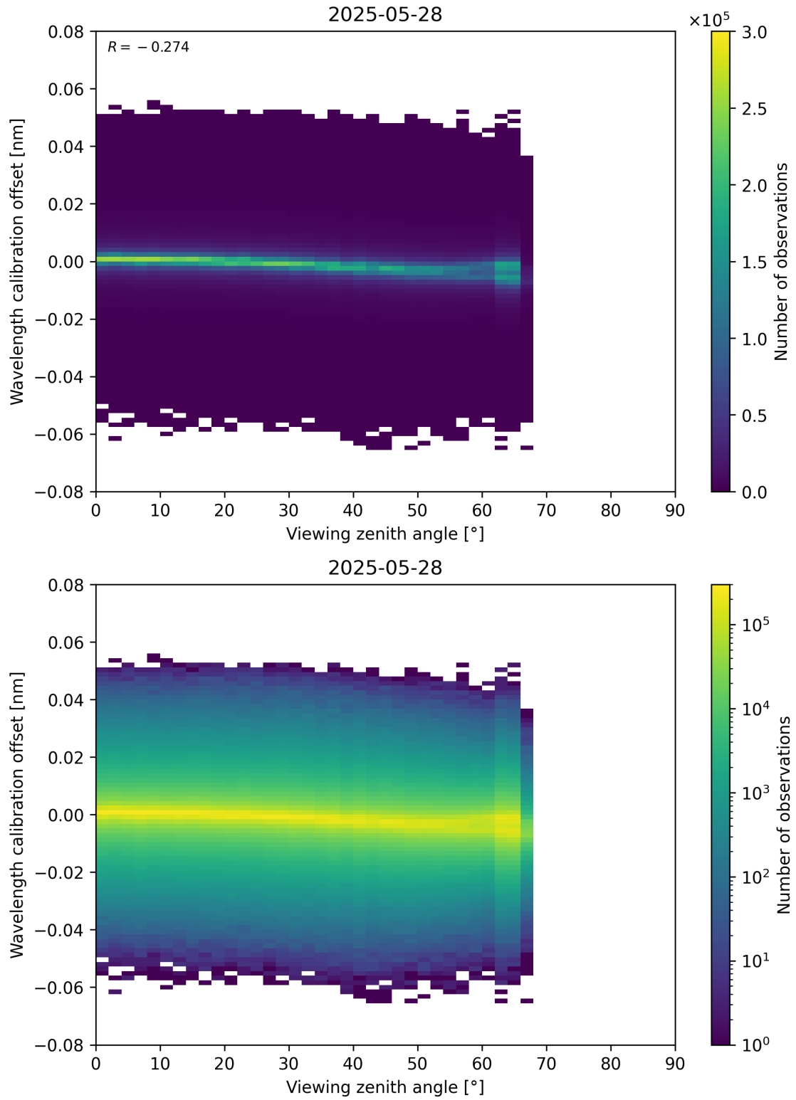
Figure 173: Scatter density plot of “Viewing zenith angle” against “Wavelength calibration offset” for 2025-05-27 to 2025-05-29.
