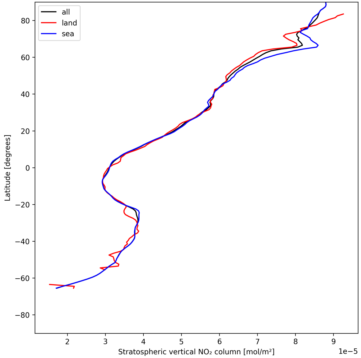
Figure 19: Zonal average of “Stratospheric vertical NO 2 column” for 2025-05-27 to 2025-05-29.
