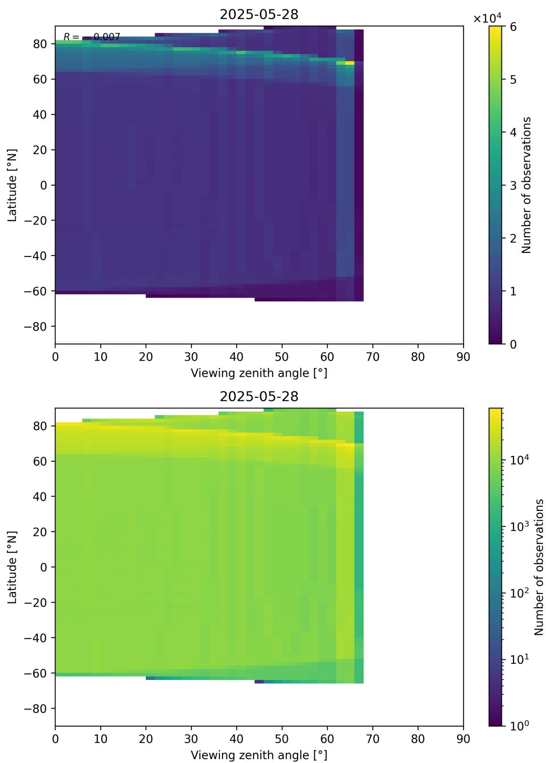
Figure 163: Scatter density plot of “Viewing zenith angle” against “Latitude” for 2025-05-27 to 2025-05-29.
