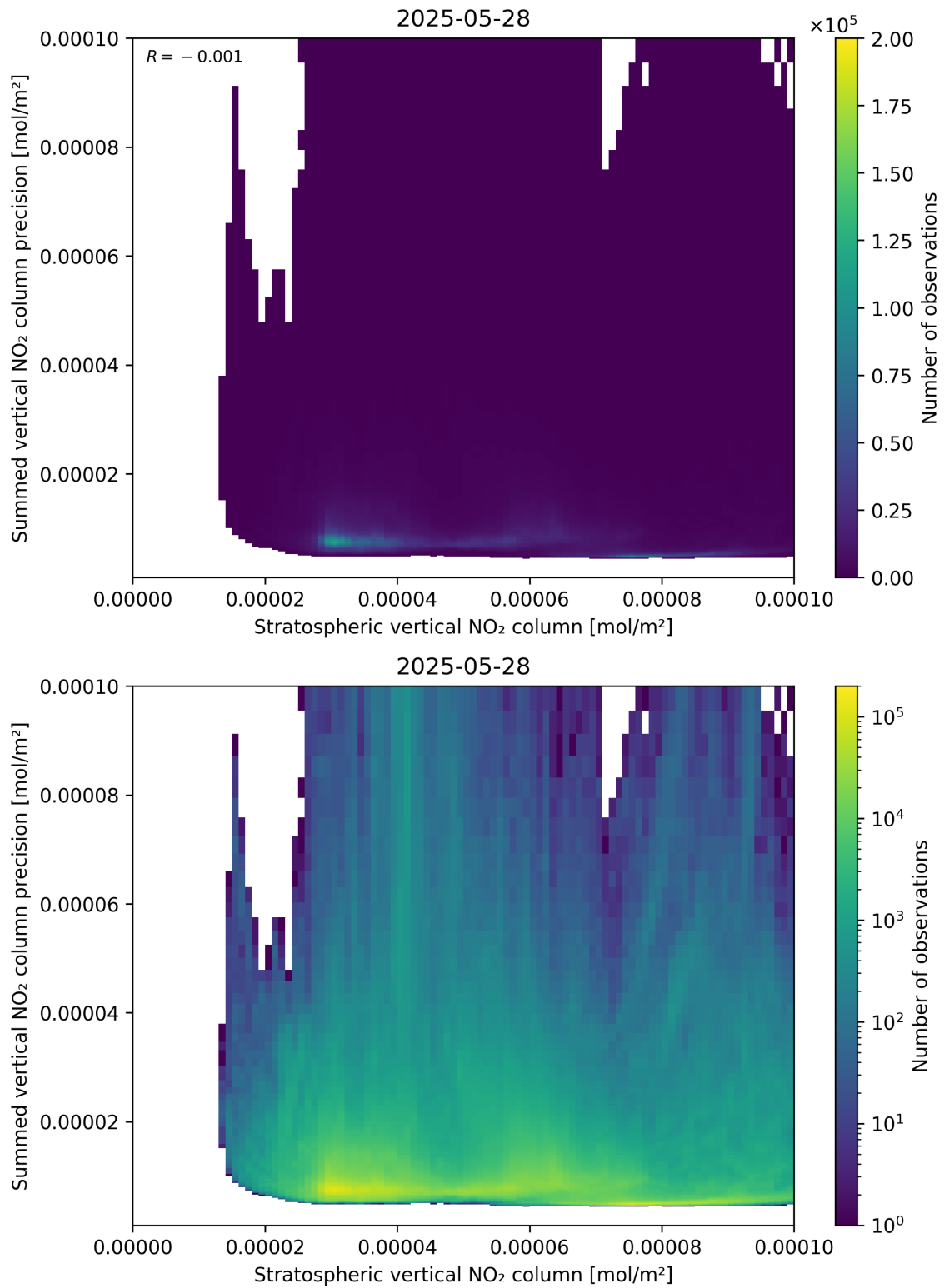
Figure 99: Scatter density plot of “Stratospheric vertical NO 2 column” against “Summed vertical NO 2 column precision” for 2025-05-27 to 2025-05-29.
