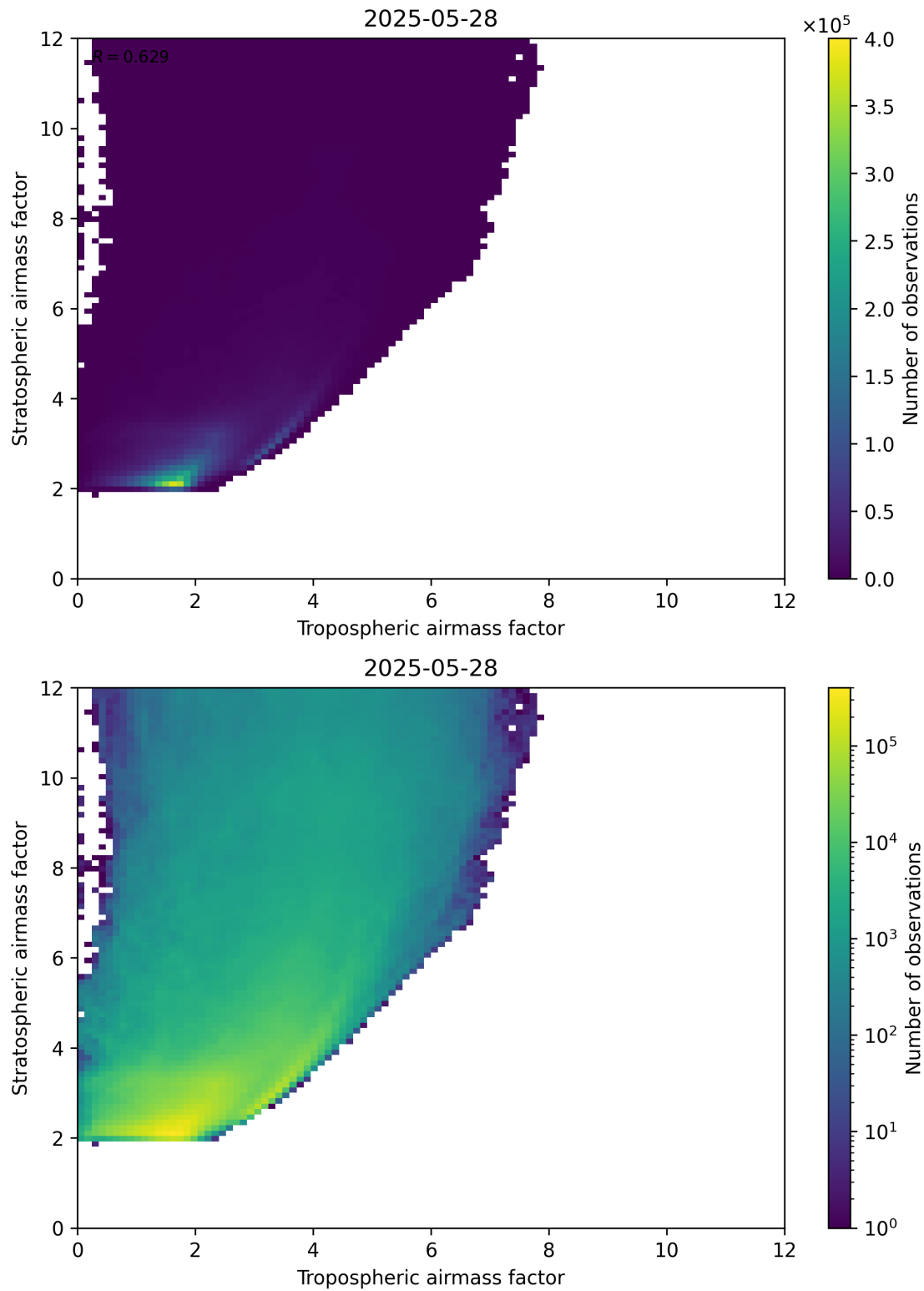
Figure 71: Scatter density plot of “Tropospheric airmass factor” against “Stratospheric airmass factor” for 2025-05-27 to 2025-05-29.
