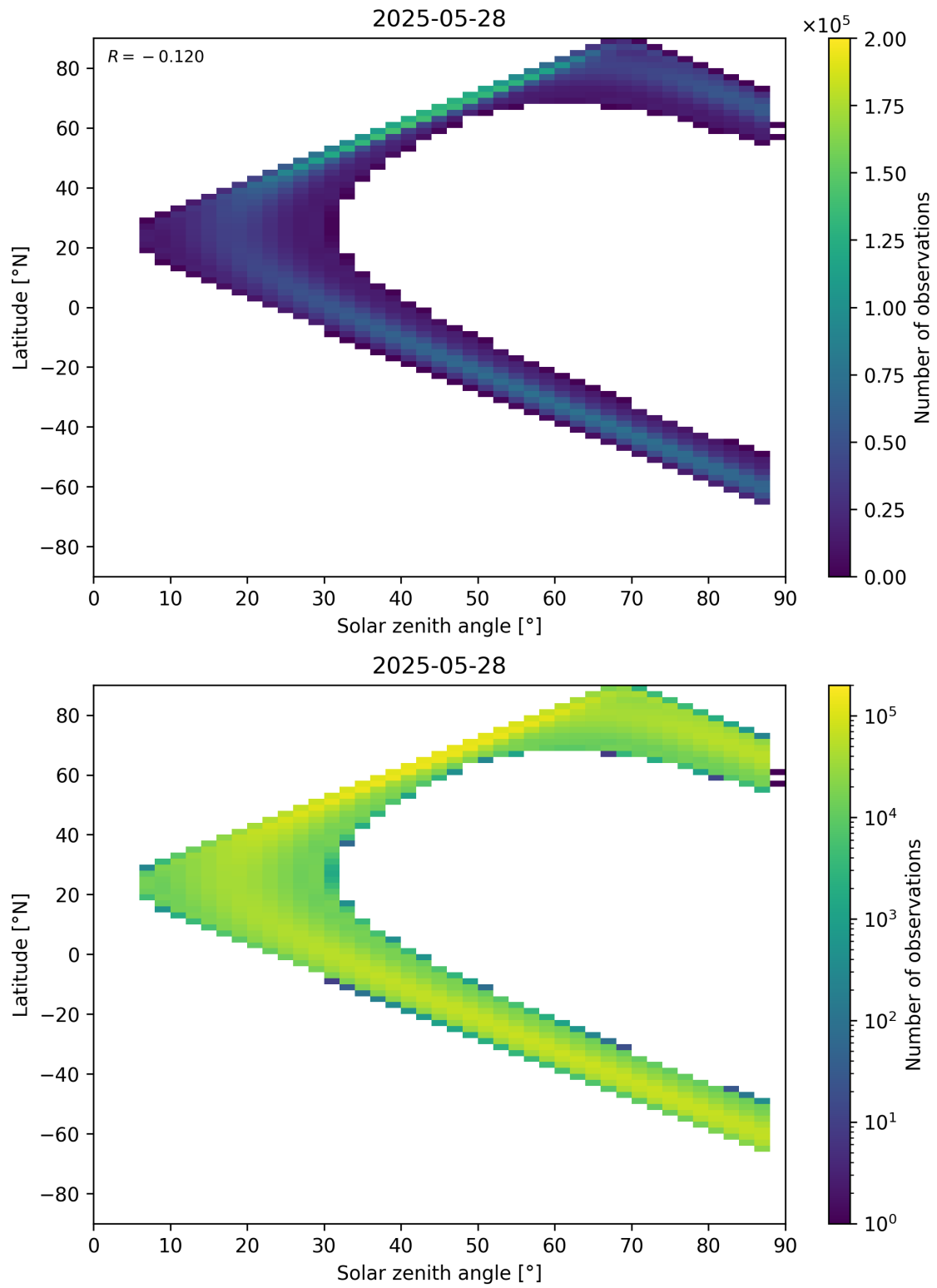
Figure 149: Scatter density plot of “Solar zenith angle” against “Latitude” for 2025-05-27 to 2025-05-29.
