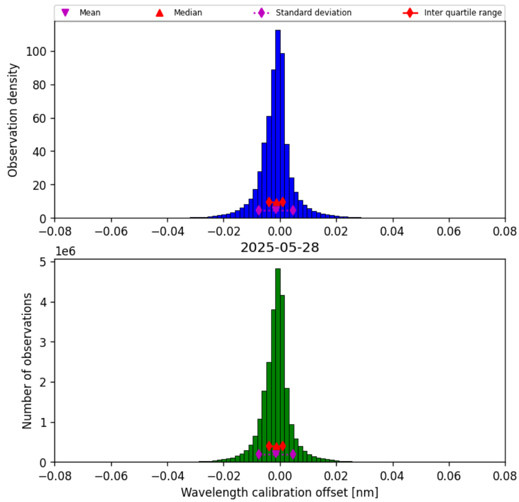
Figure 35: Histogram of “Wavelength calibration offset” for 2025-05-27 to 2025-05-29
