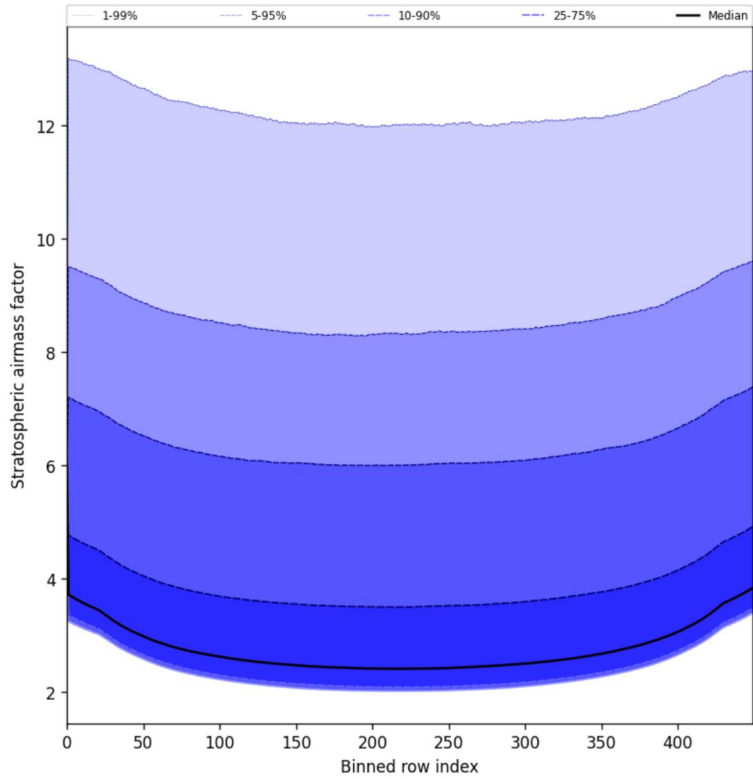
Figure 61: Along track statistics of “Stratospheric airmass factor” for 2025-05-27 to 2025-05-29
