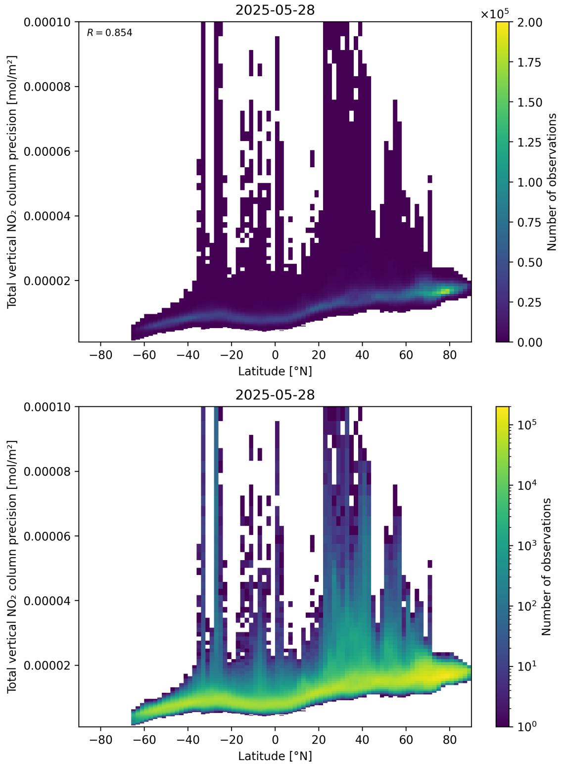
Figure 91: Scatter density plot of “Latitude” against “Total vertical NO 2 column precision” for 2025-05-27 to 2025-05-29.
