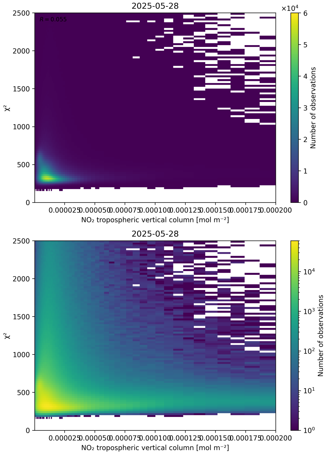
Figure 124: Scatter density plot of “NO 2 tropospheric vertical column” against “ \chi^2 ” for 2025-05-27 to 2025-05-29.
