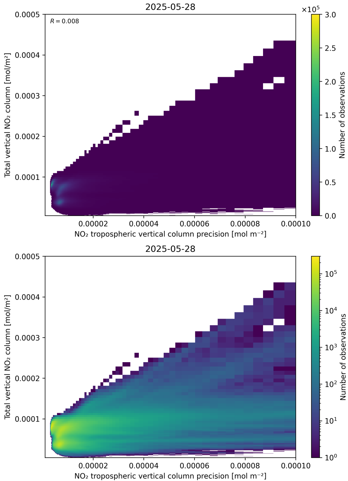
Figure 138: Scatter density plot of “NO 2 tropospheric vertical column precision” against “Total vertical NO 2 column” for 2025-05-27 to 2025-05-29.
