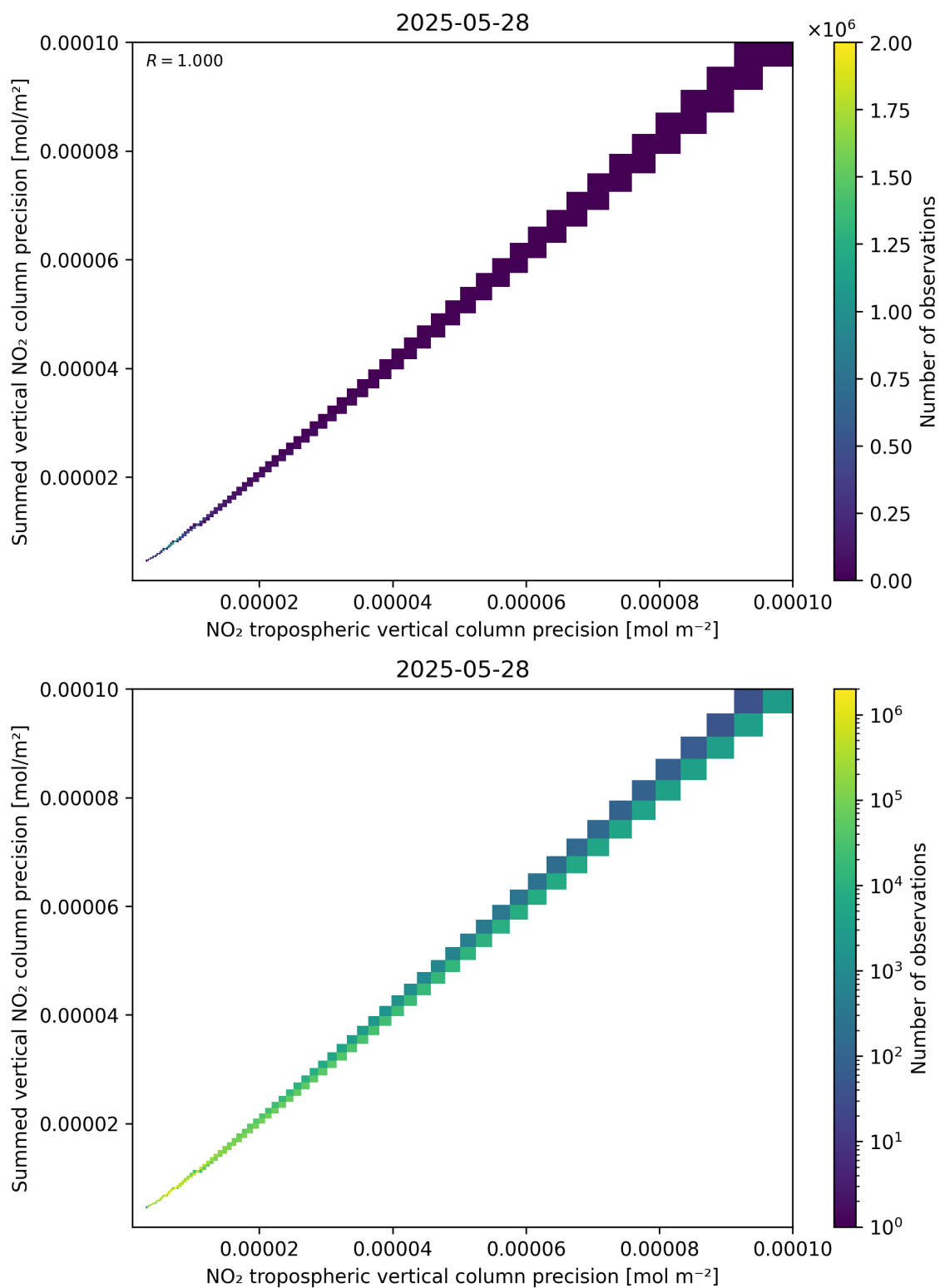
Figure 137: Scatter density plot of “NO 2 tropospheric vertical column precision” against “Summed vertical NO 2 column precision” for 2025-05-27 to 2025-05-29.
