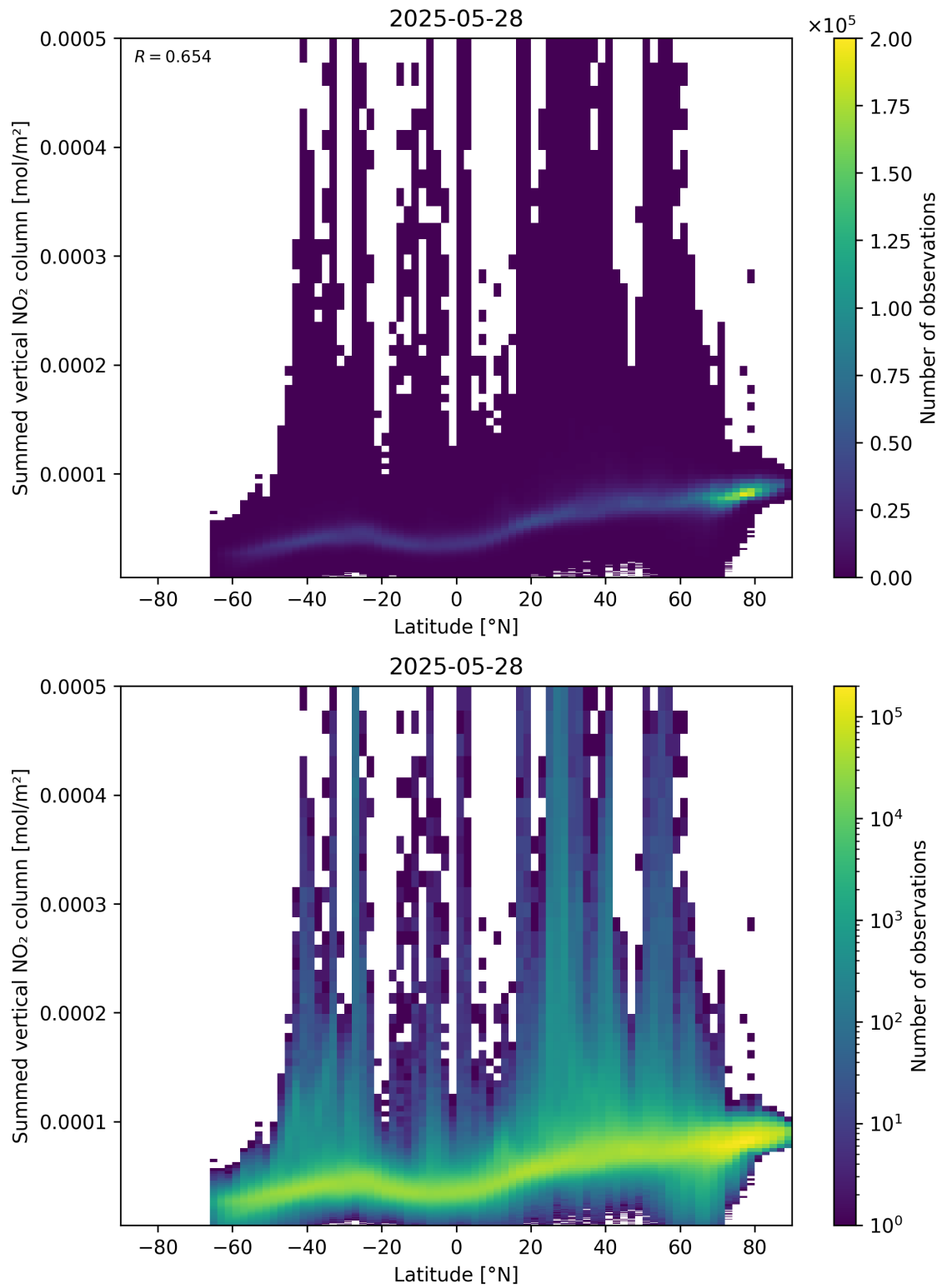
Figure 88: Scatter density plot of “Latitude” against “Summed vertical NO 2 column” for 2025-05-27 to 2025-05-29.
