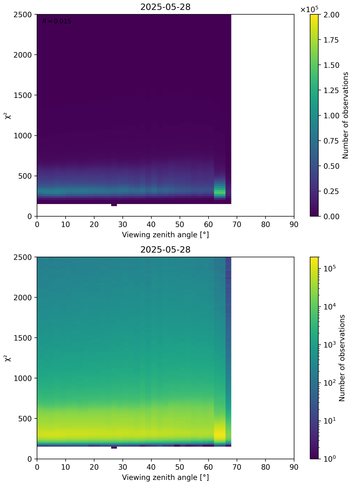
Figure 162: Scatter density plot of “Viewing zenith angle” against “ \chi^2 ” for 2025-05-27 to 2025-05-29.
