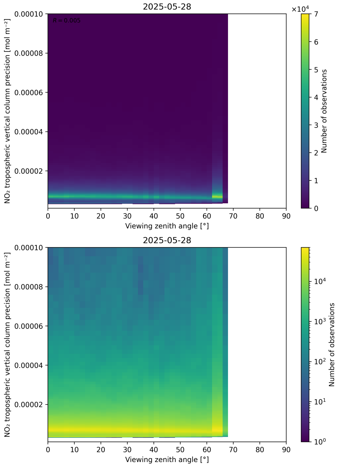
Figure 170: Scatter density plot of “Viewing zenith angle” against “NO 2 tropospheric vertical column precision” for 2025-05-27 to 2025-05-29.
