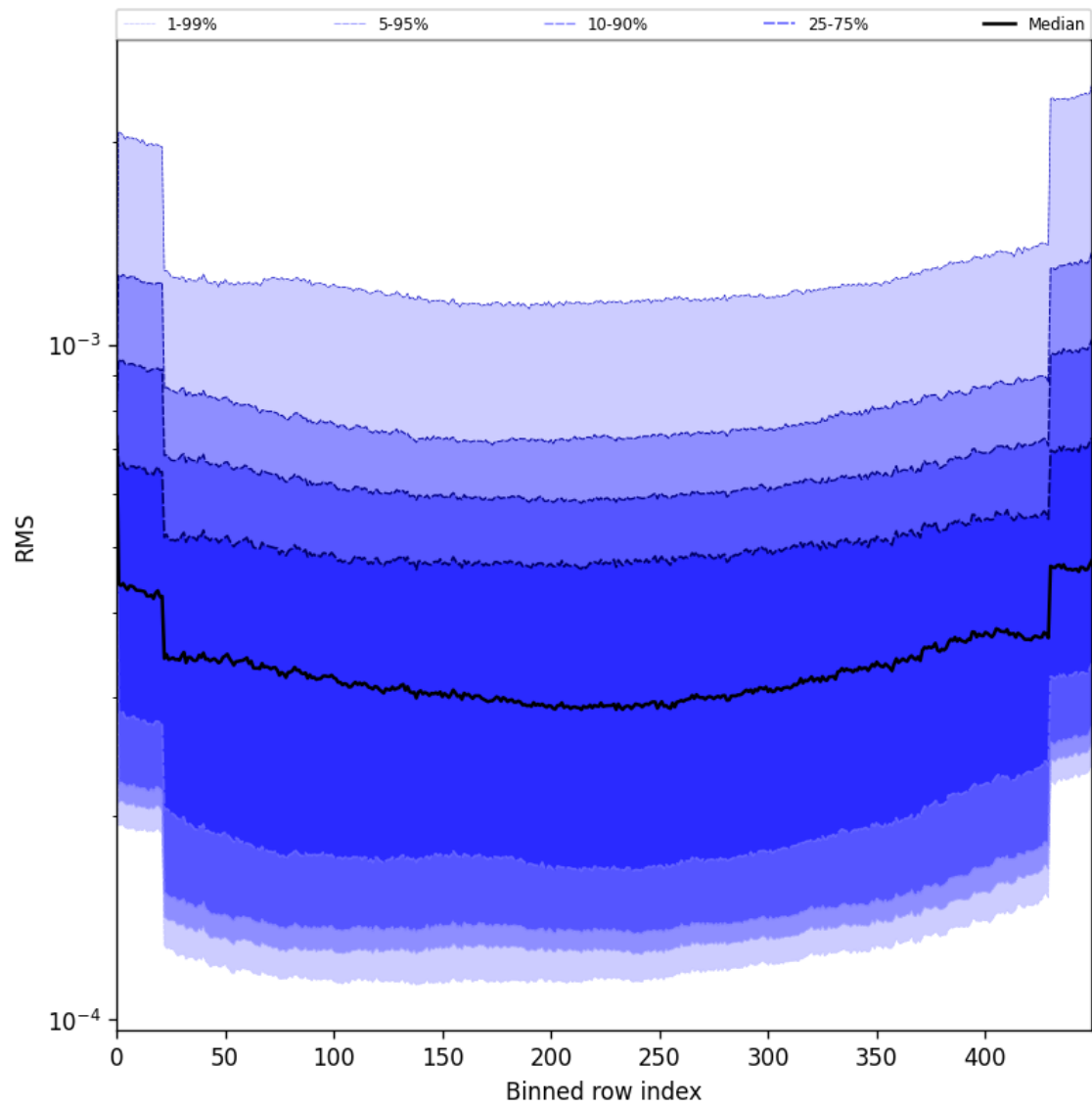
Figure 60: Along track statistics of “RMS” for 2025-05-27 to 2025-05-29
