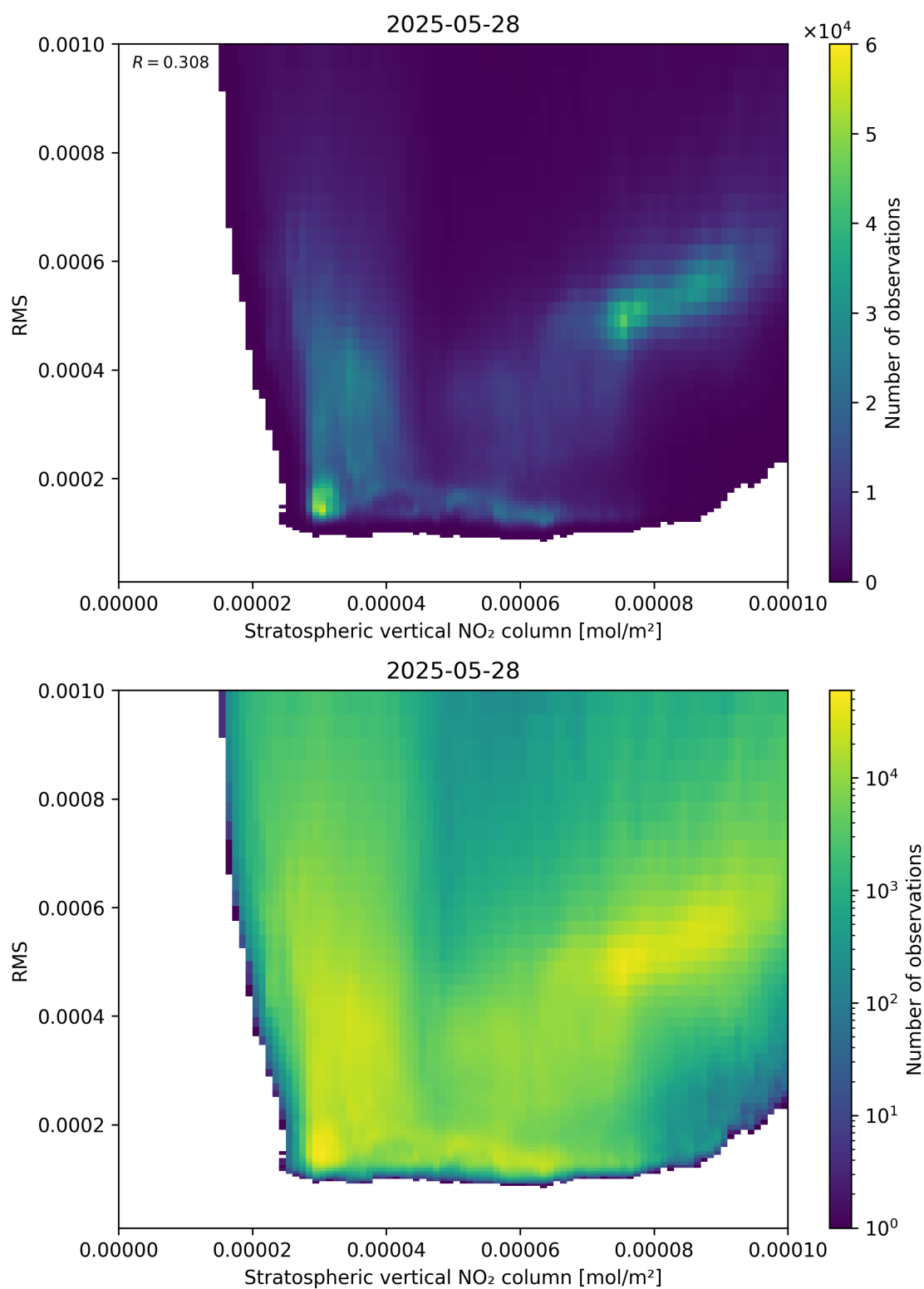
Figure 102: Scatter density plot of “Stratospheric vertical NO 2 column” against “RMS” for 2025-05-27 to 2025-05-29.
