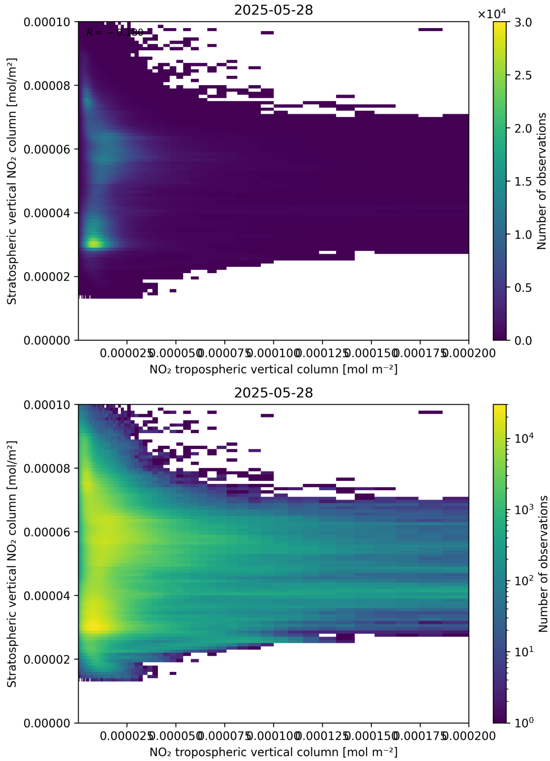
Figure 125: Scatter density plot of “NO 2 tropospheric vertical column” against “Stratospheric vertical NO 2 column” for 2025-05-27 to 2025-05-29.
