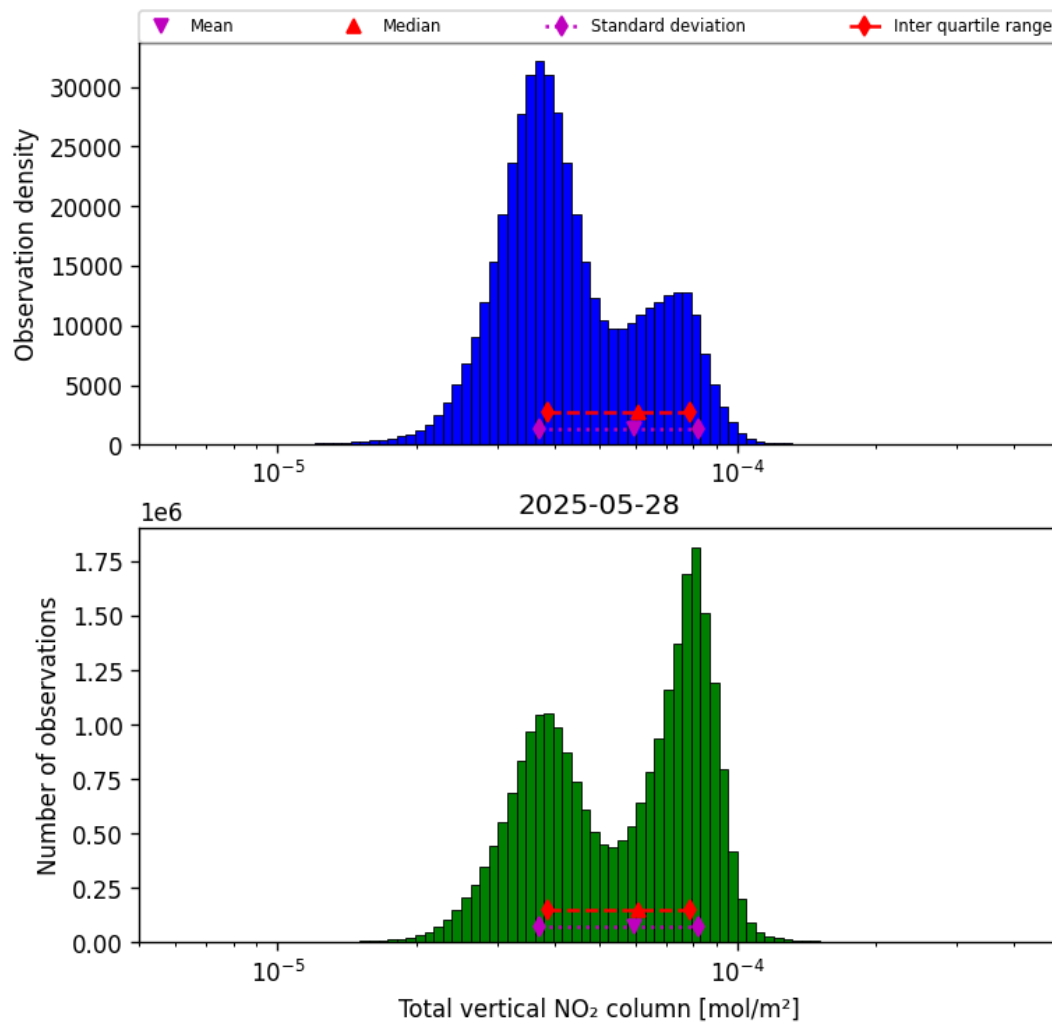
Figure 38: Histogram of “Total vertical NO 2 column” for 2025-05-27 to 2025-05-29
