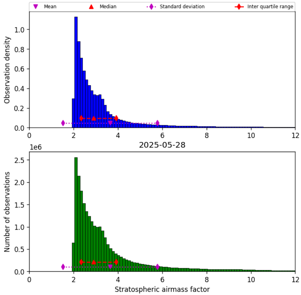
Figure 44: Histogram of “Stratospheric airmass factor” for 2025-05-27 to 2025-05-29
