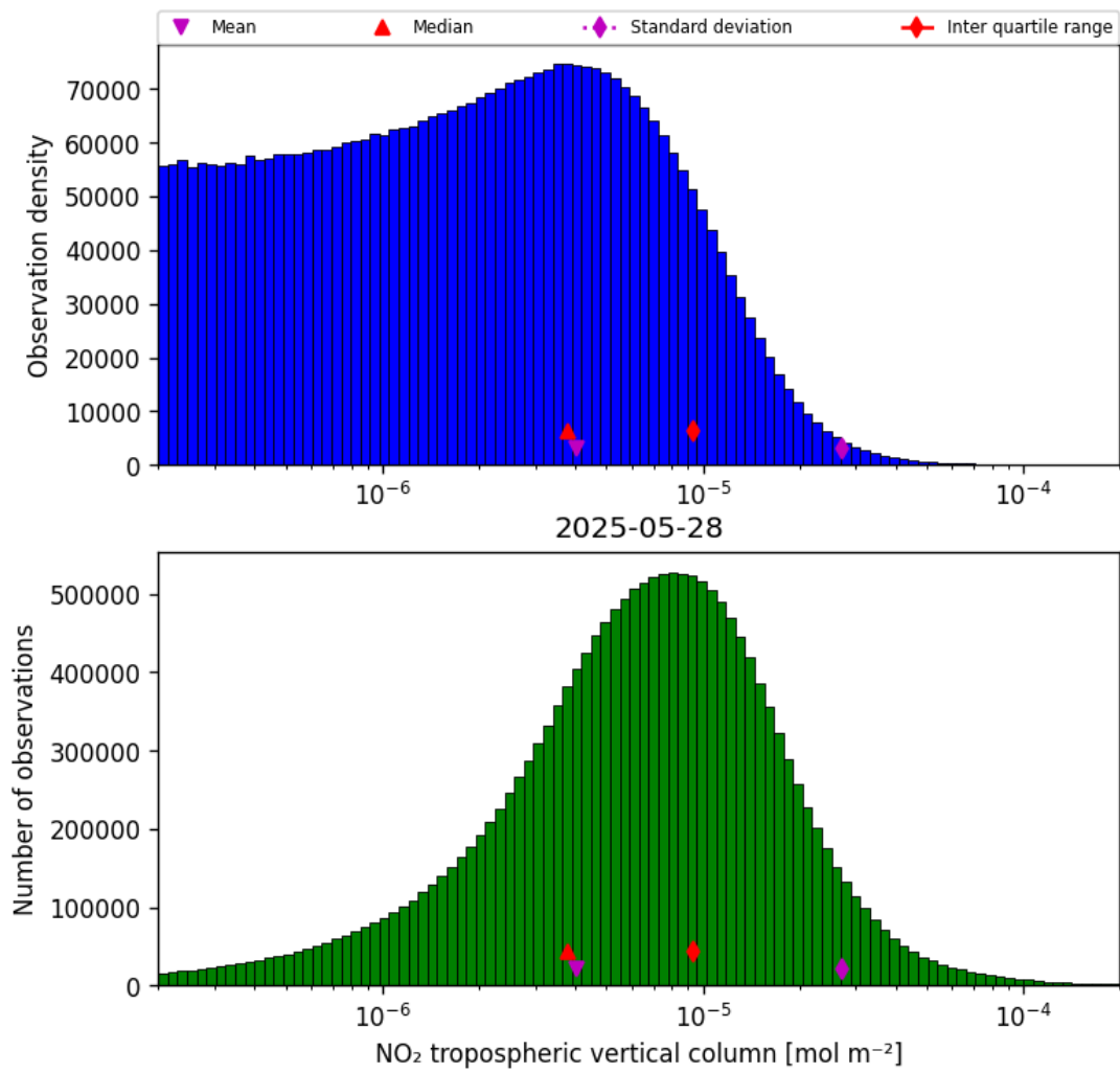
Figure 29: Histogram of “NO 2 tropospheric vertical column” for 2025-05-27 to 2025-05-29
