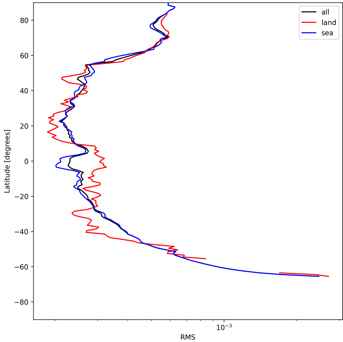
Figure 26: Zonal average of “RMS” for 2025-05-27 to 2025-05-29.
