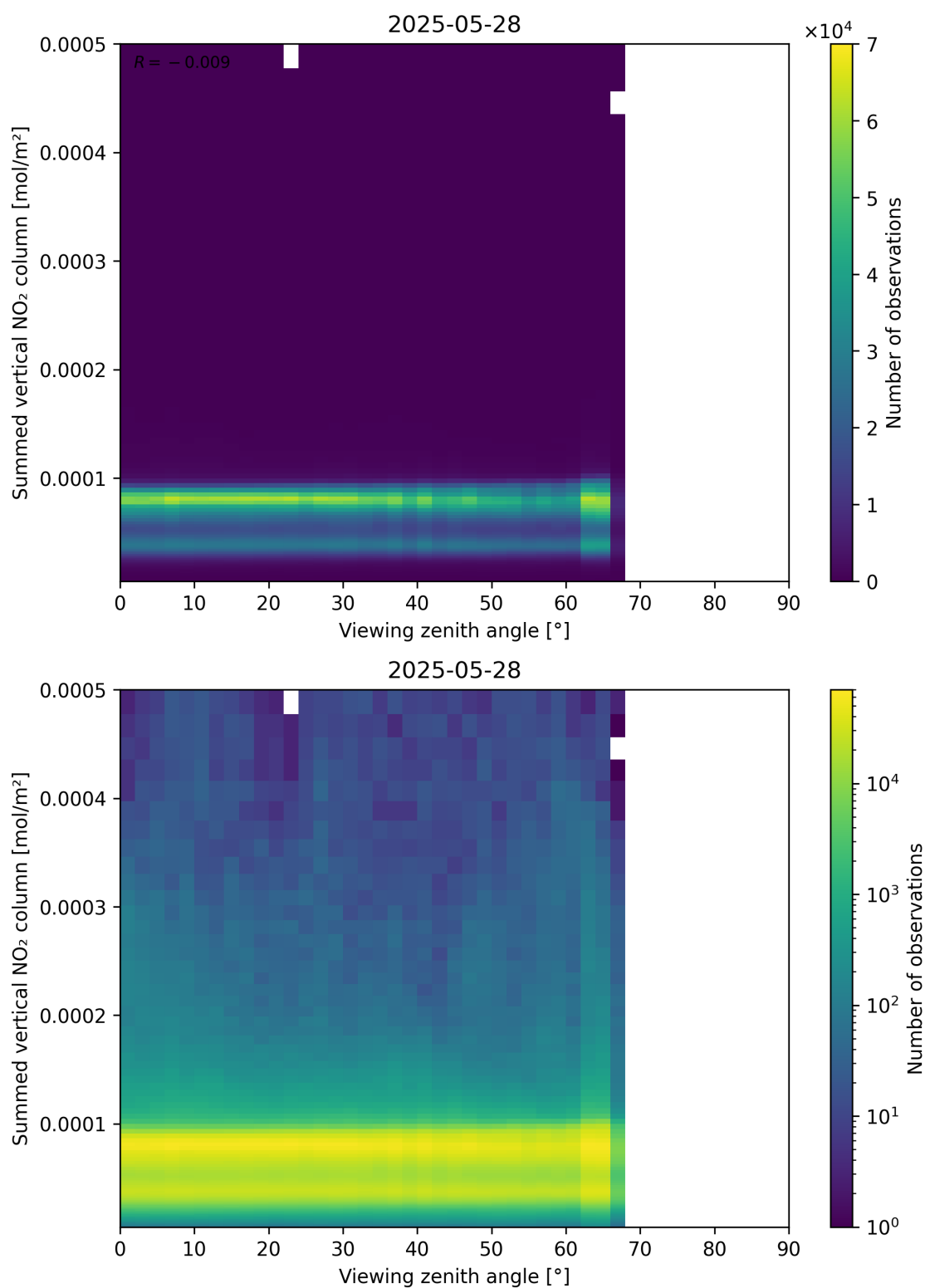
Figure 165: Scatter density plot of “Viewing zenith angle” against “Summed vertical NO 2 column” for 2025-05-27 to 2025-05-29.
