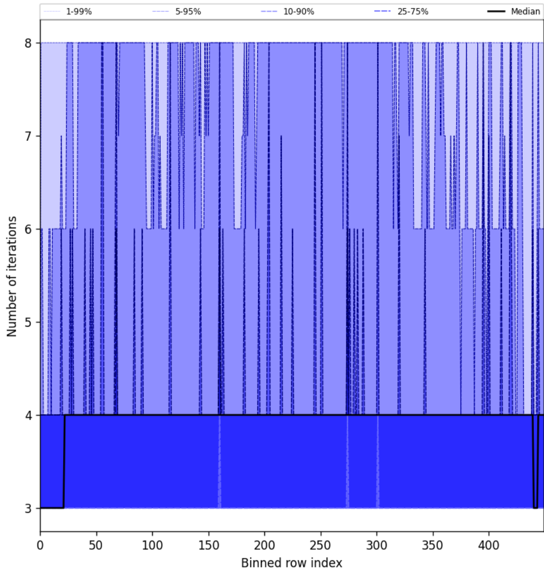
Figure 51: Along track statistics of “Number of iterations” for 2025-05-27 to 2025-05-29
