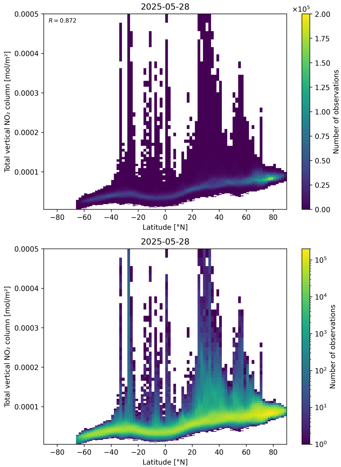
Figure 90: Scatter density plot of “Latitude” against “Total vertical NO 2 column” for 2025-05-27 to 2025-05-29.
