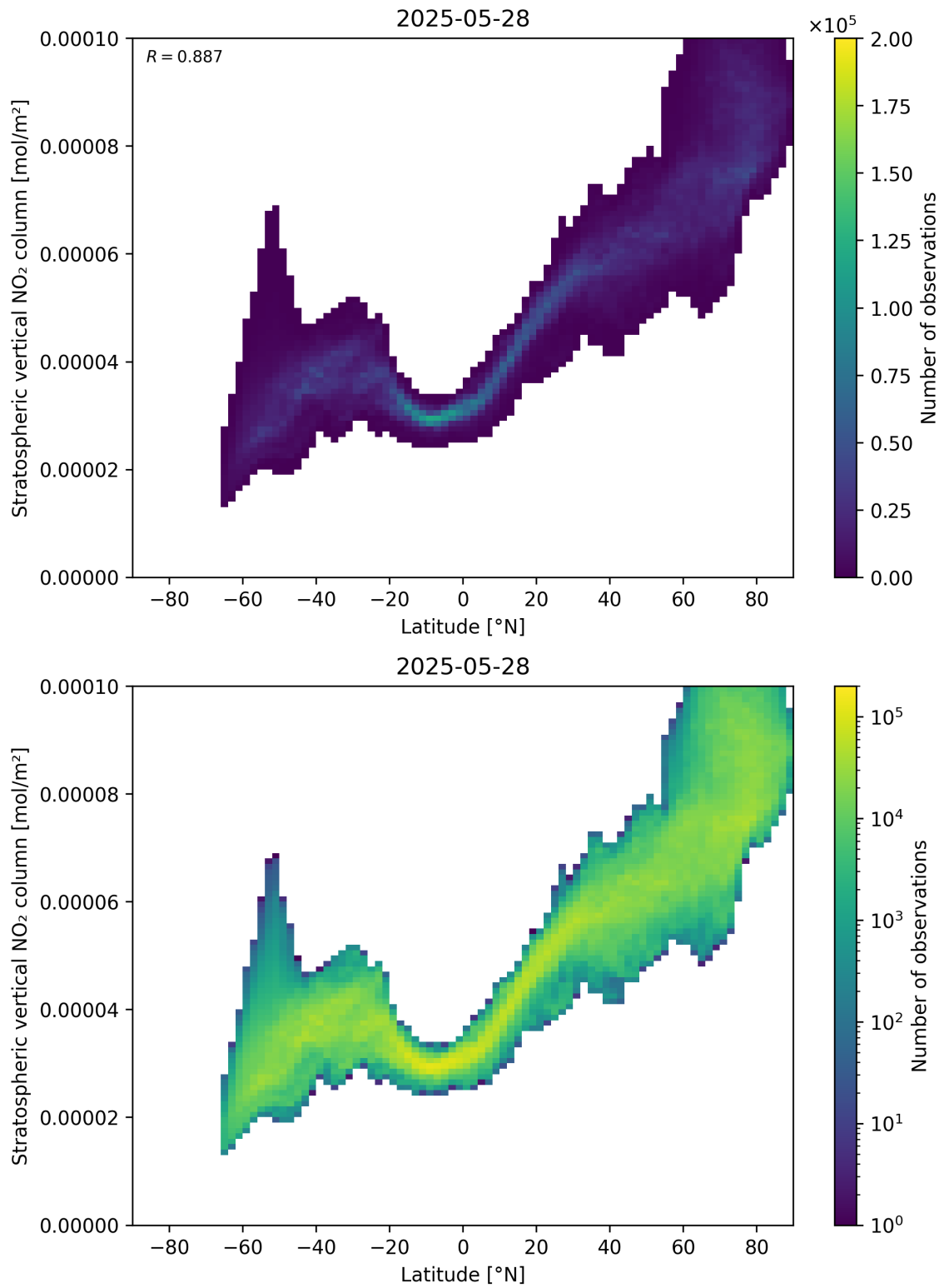
Figure 87: Scatter density plot of “Latitude” against “Stratospheric vertical \text{NO}_2 column” for 2025-05-27 to 2025-05-29.
