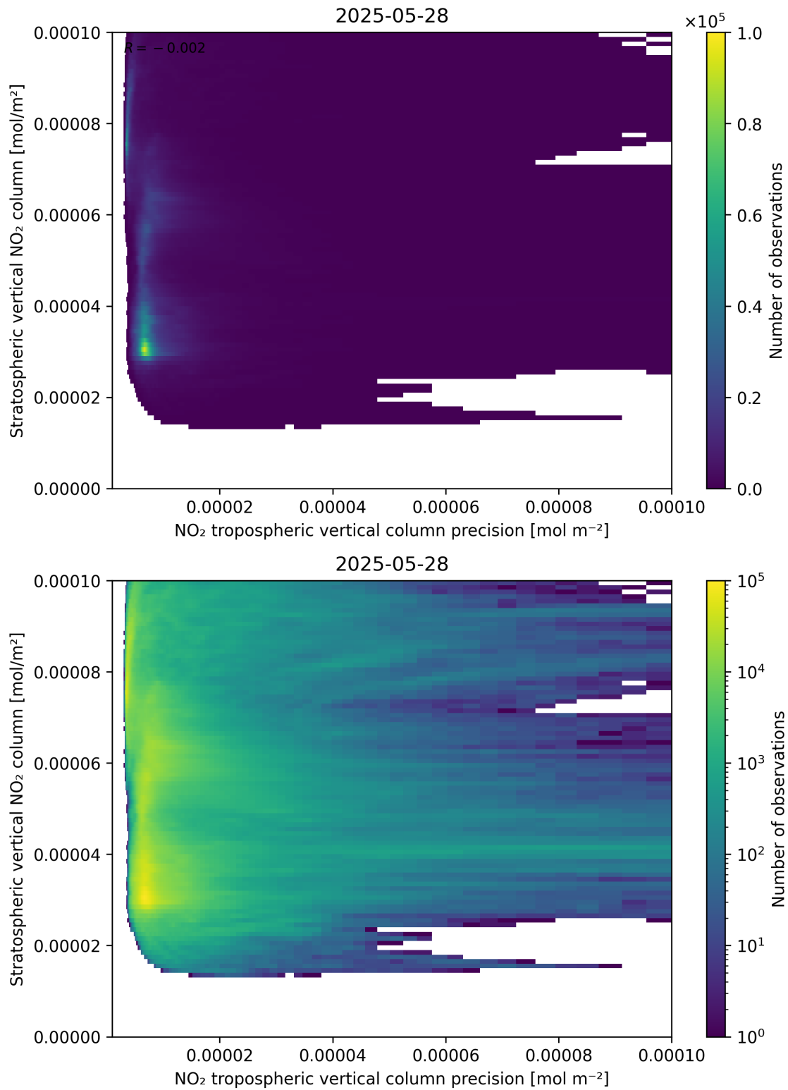
Figure 135: Scatter density plot of “NO 2 tropospheric vertical column precision” against “Stratospheric vertical NO 2 column” for 2025-05-27 to 2025-05-29.
