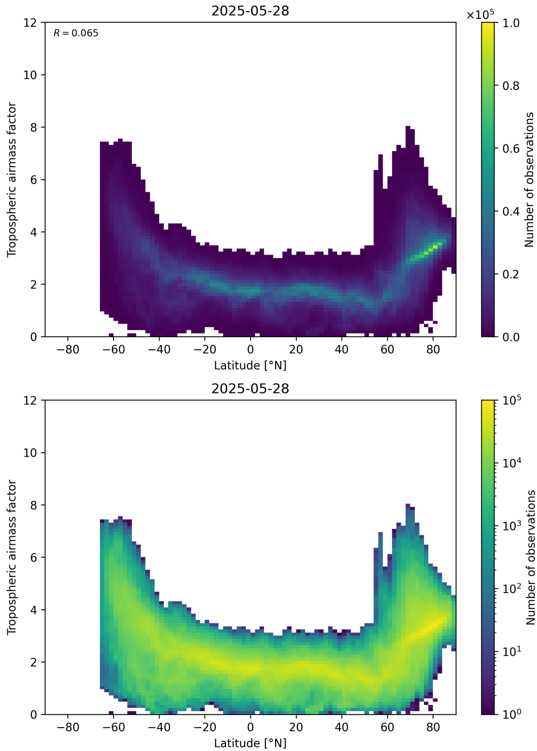
Figure 85: Scatter density plot of “Latitude” against “Tropospheric air mass factor” for 2025-05-27 to 2025-05-29.
