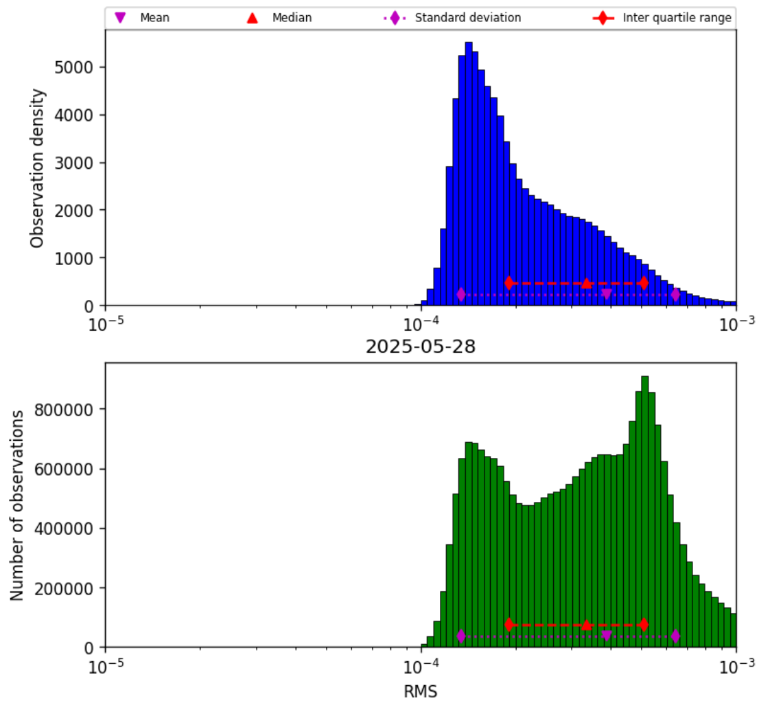
Figure 43: Histogram of “RMS” for 2025-05-27 to 2025-05-29
