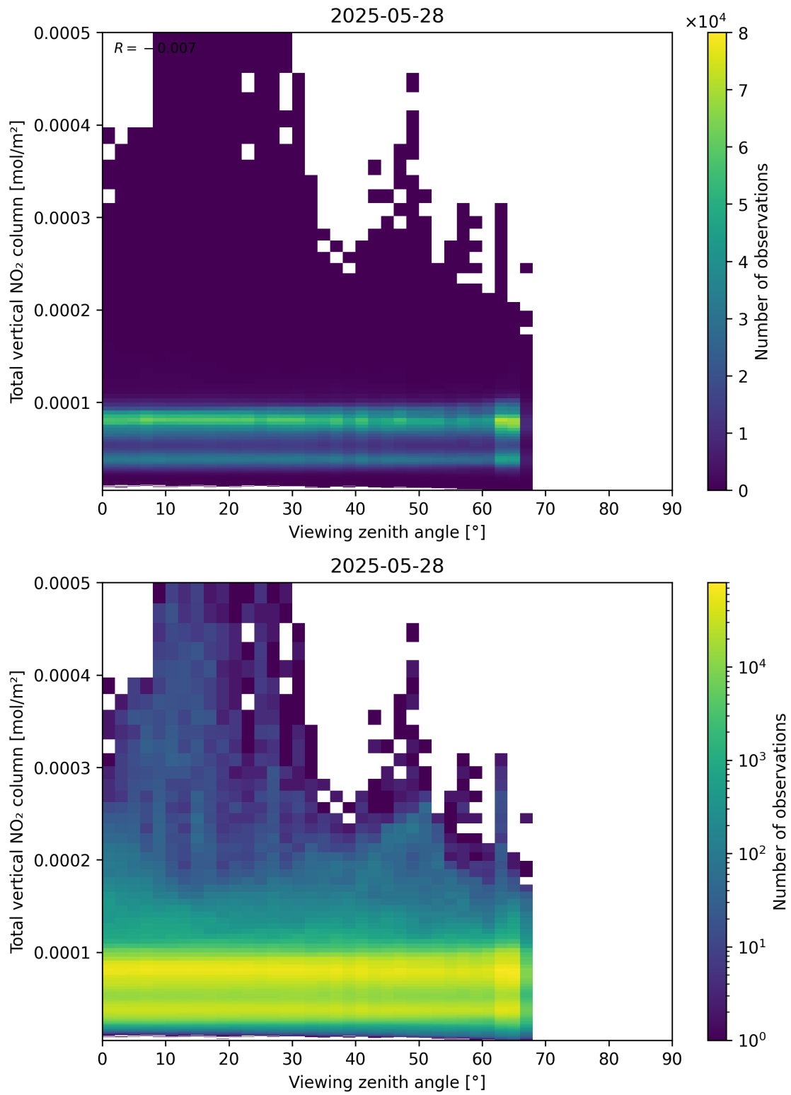
Figure 167: Scatter density plot of “Viewing zenith angle” against “Total vertical NO 2 column” for 2025-05-27 to 2025-05-29.
