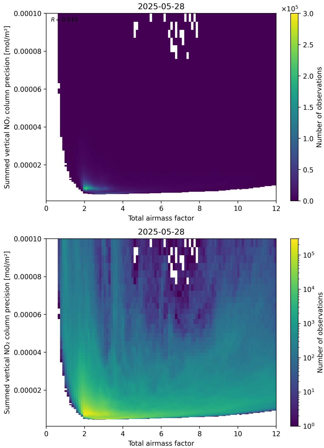
Figure 66: Scatter density plot of “Total airmass factor” against “Summed vertical NO 2 column precision” for 2025-05-27 to 2025-05-29.
