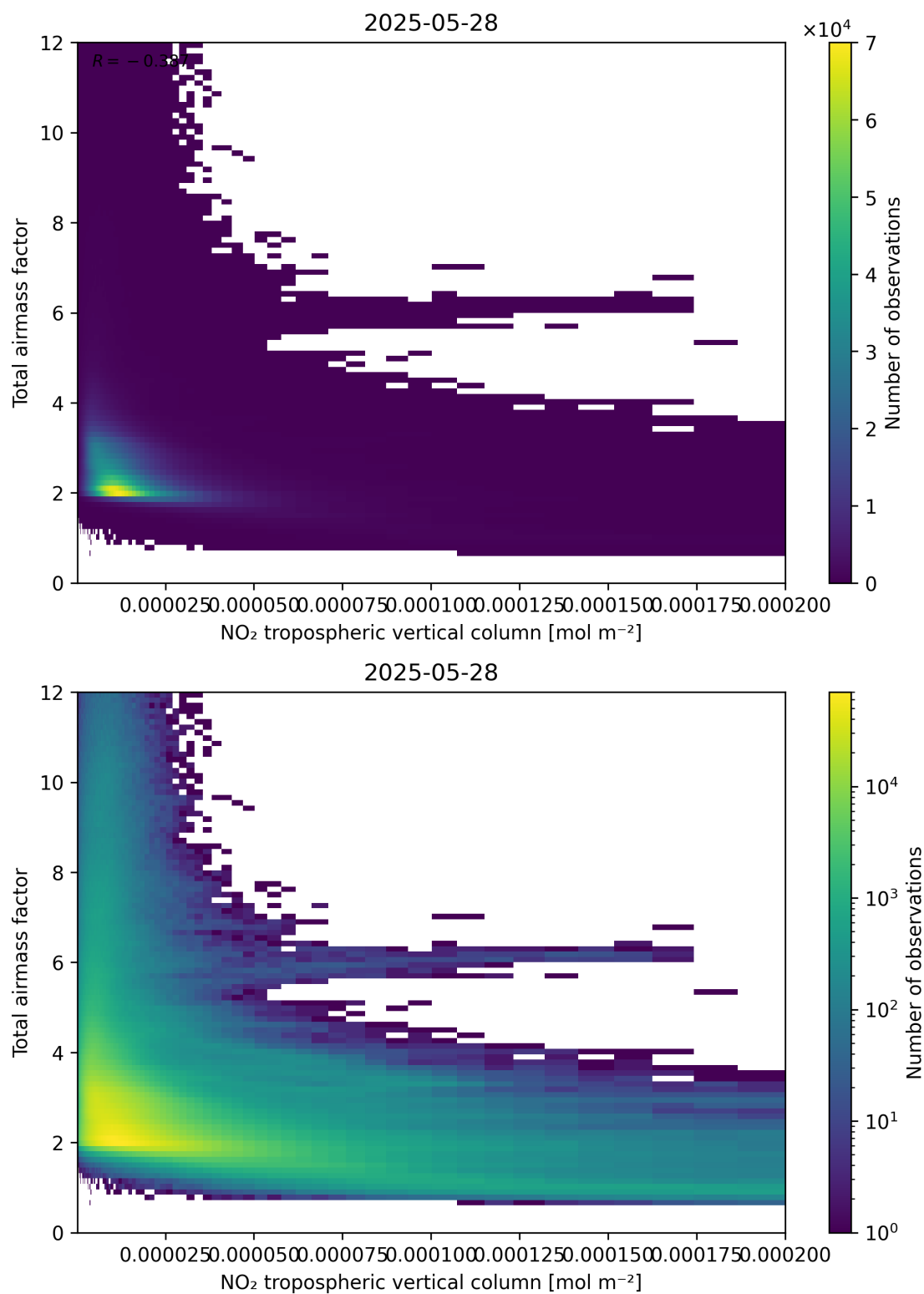
Figure 122: Scatter density plot of “NO 2 tropospheric vertical column” against “Total air mass factor” for 2025-05-27 to 2025-05-29.
