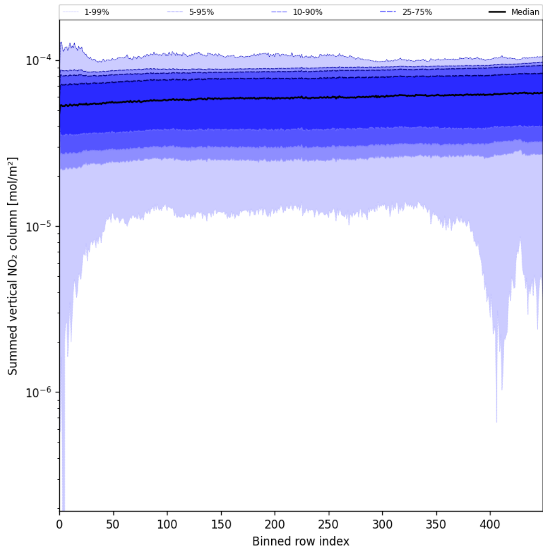
Figure 57: Along track statistics of “Summed vertical NO 2 column” for 2025-05-27 to 2025-05-29
