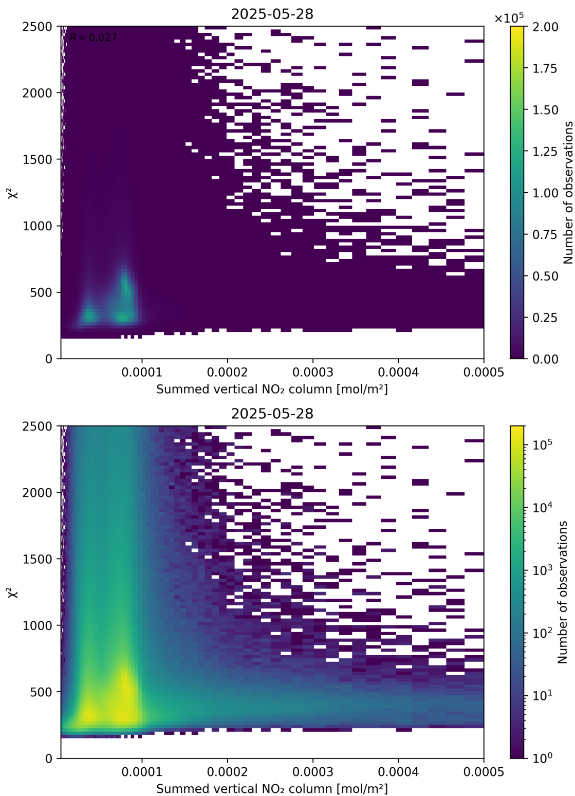
Figure 104: Scatter density plot of “Summed vertical NO 2 column” against “ \chi^2 ” for 2025-05-27 to 2025-05-29.
