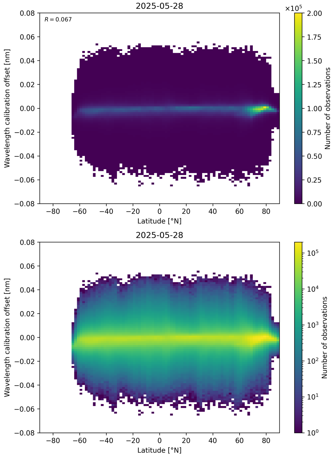
Figure 95: Scatter density plot of “Latitude” against “Wavelength calibration offset” for 2025-05-27 to 2025-05-29.
