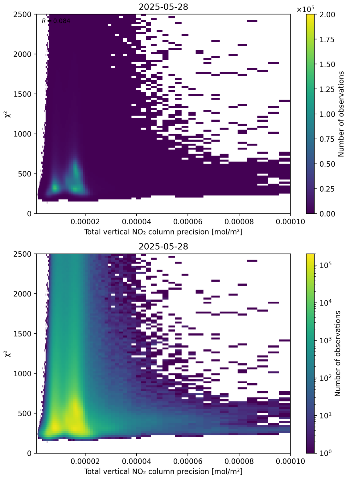
Figure 116: Scatter density plot of “Total vertical NO 2 column precision” against “ \chi^2 ” for 2025-05-27 to 2025-05-29.
