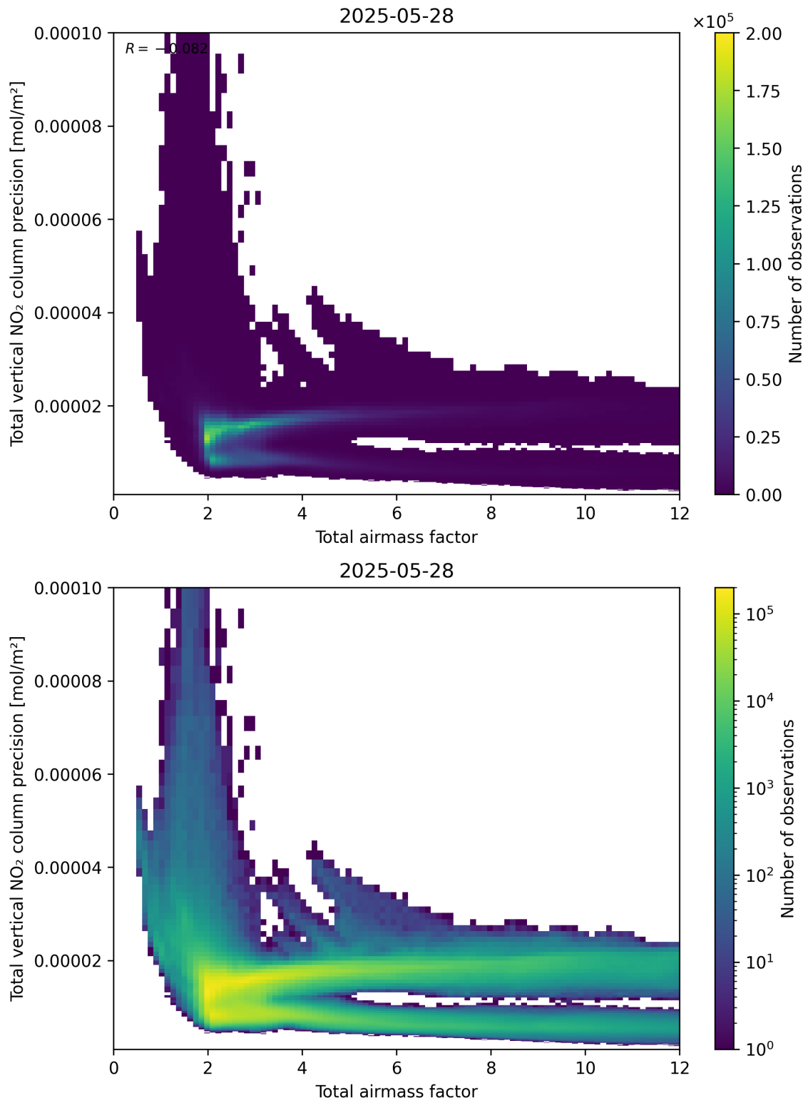
Figure 68: Scatter density plot of “Total airmass factor” against “Total vertical NO 2 column precision” for 2025-05-27 to 2025-05-29.
