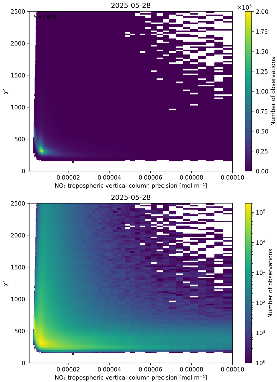
Figure 134: Scatter density plot of “NO 2 tropospheric vertical column precision” against “ \chi^2 ” for 2025-05-27 to 2025-05-29.
