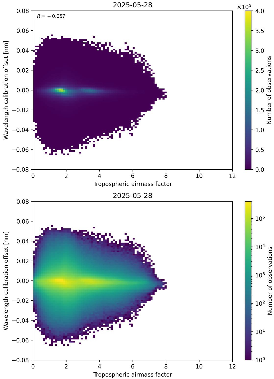
Figure 80: Scatter density plot of “Tropospheric airmass factor” against “Wavelength calibration offset” for 2025-05-27 to 2025-05-29.
