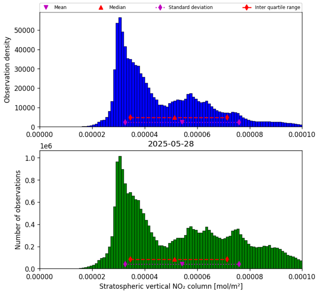
Figure 36: Histogram of “Stratospheric vertical NO 2 column” for 2025-05-27 to 2025-05-29
