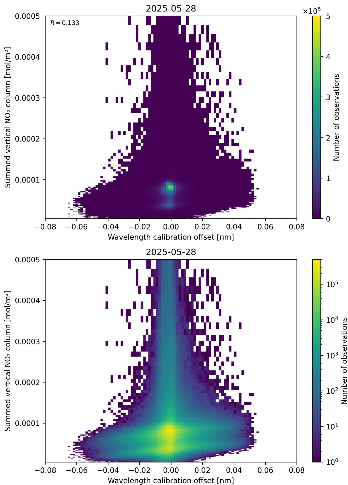
Figure 177: Scatter density plot of “Wavelength calibration offset” against “Summed vertical NO 2 column” for 2025-05-27 to 2025-05-29.
