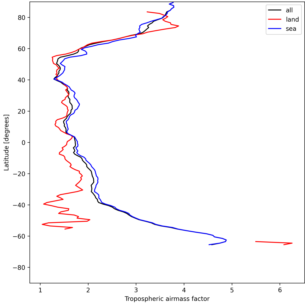
Figure 14: Zonal average of “Tropospheric airmass factor” for 2025-05-27 to 2025-05-29.
