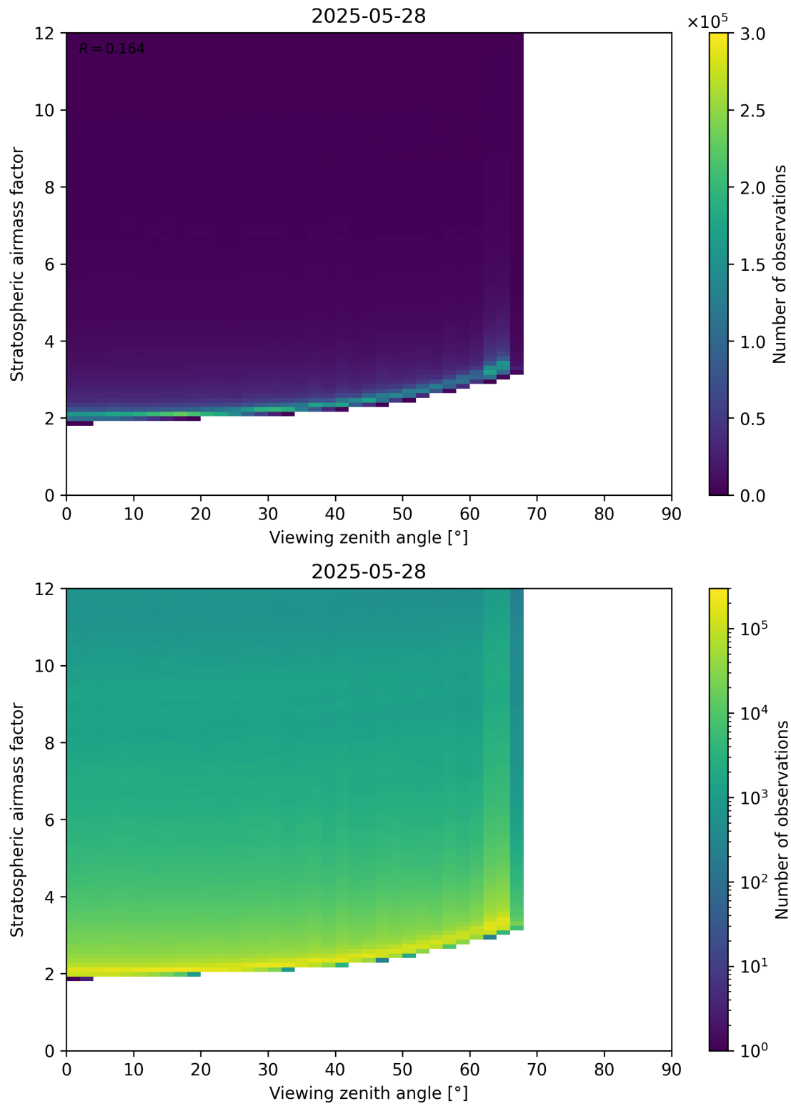
Figure 159: Scatter density plot of “Viewing zenith angle” against “Stratospheric airmass factor” for 2025-05-27 to 2025-05-29.
