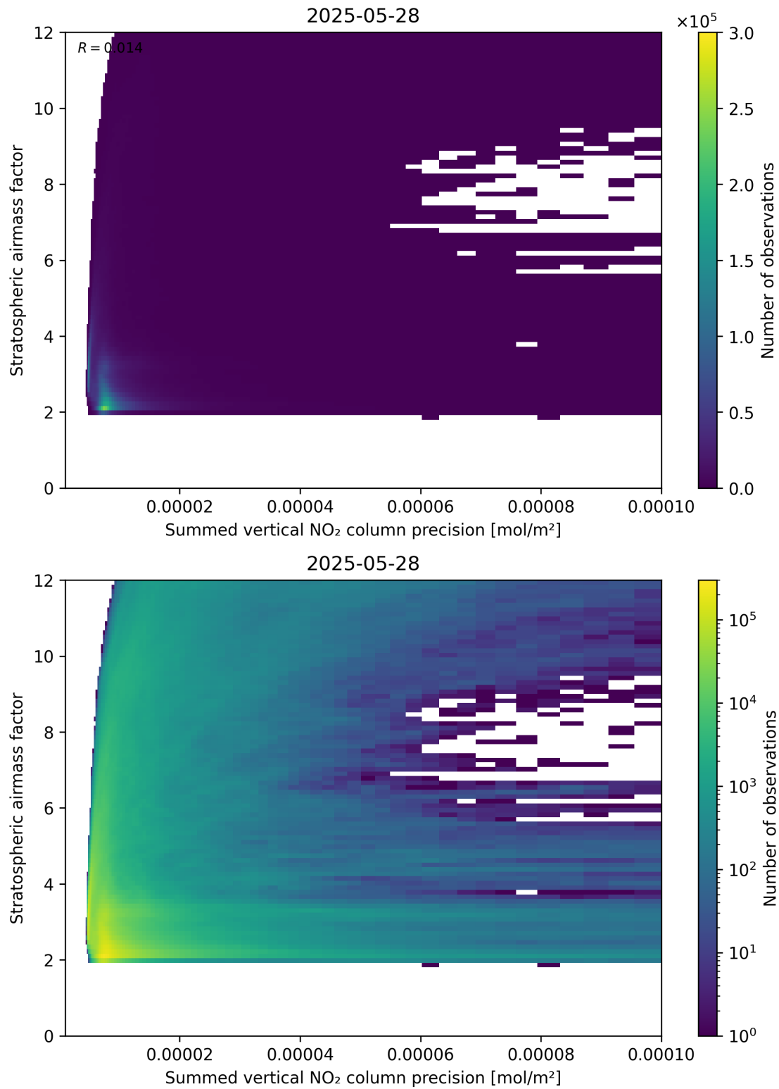
Figure 106: Scatter density plot of “Summed vertical NO 2 column precision” against “Stratospheric airmass factor” for 2025-05-27 to 2025-05-29.
