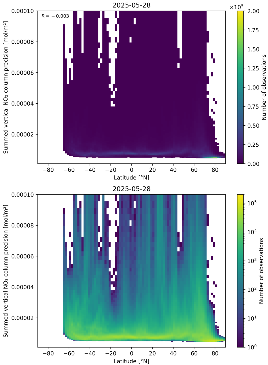
Figure 89: Scatter density plot of “Latitude” against “Summed vertical NO 2 column precision” for 2025-05-27 to 2025-05-29.
