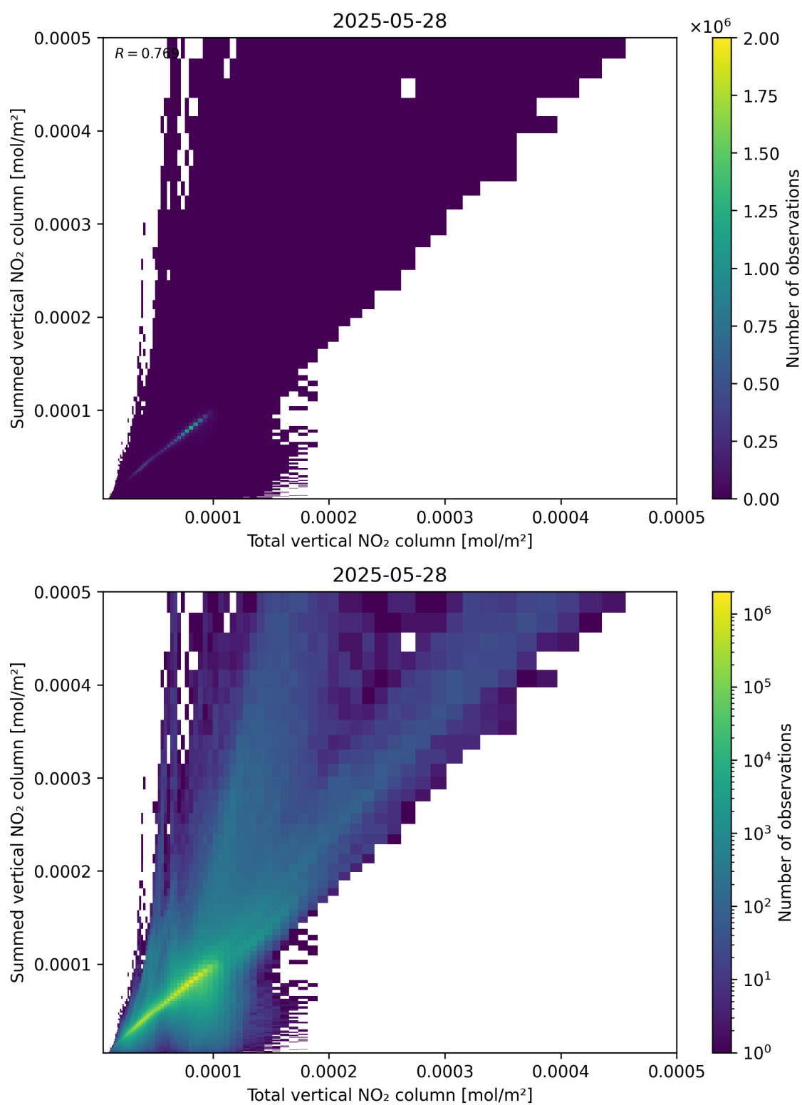
Figure 112: Scatter density plot of “Total vertical NO 2 column” against “Summed vertical NO 2 column” for 2025-05-27 to 2025-05-29.
