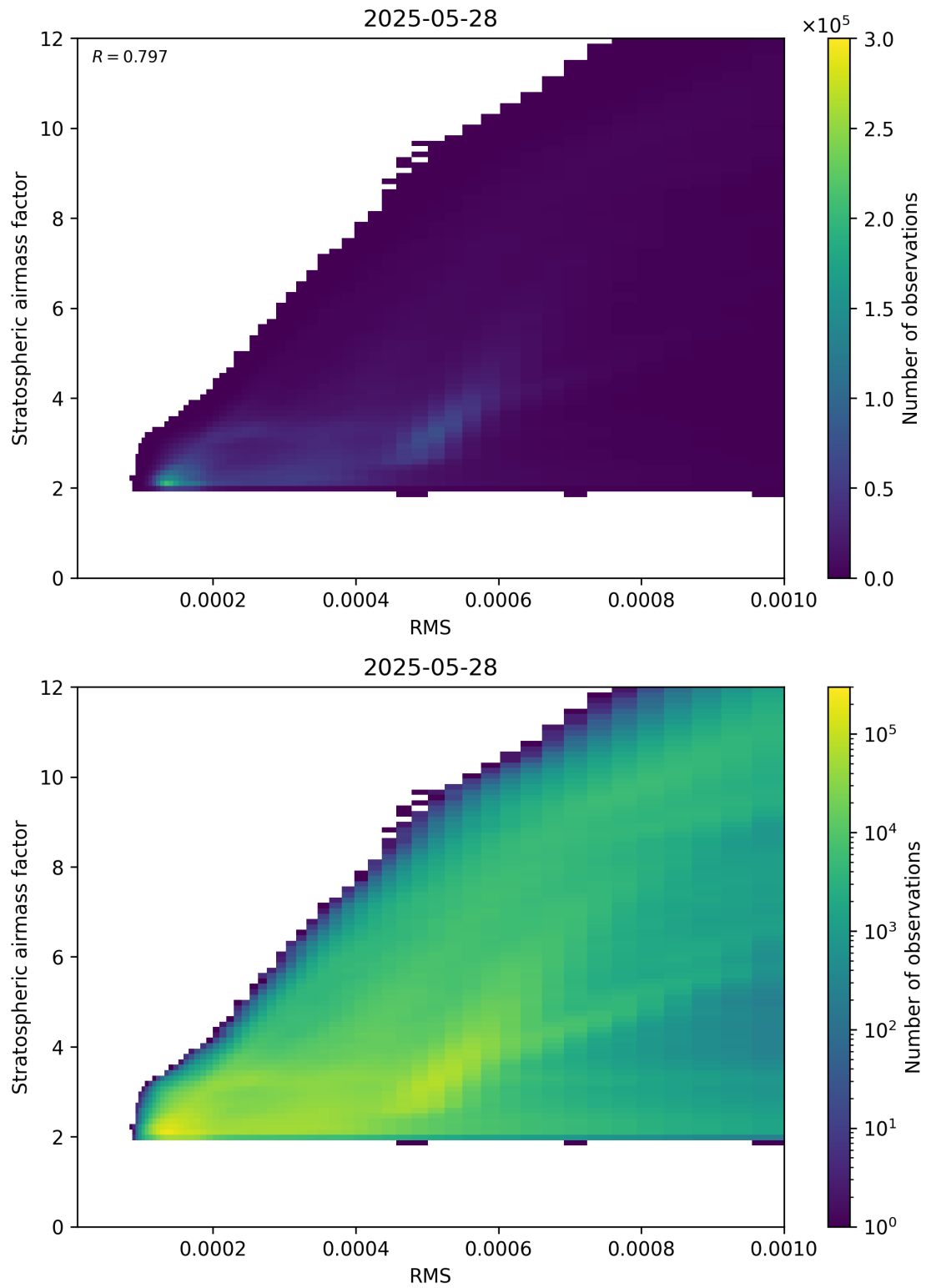
Figure 144: Scatter density plot of “RMS” against “Stratospheric airmass factor” for 2025-05-27 to 2025-05-29.
