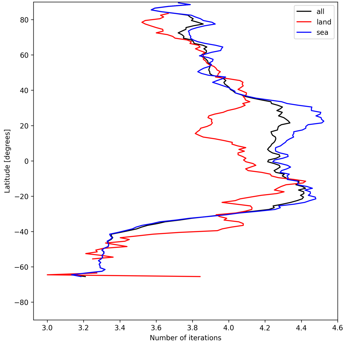
Figure 17: Zonal average of “Number of iterations” for 2025-05-27 to 2025-05-29.
