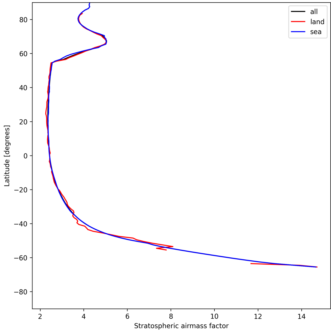
Figure 27: Zonal average of “Stratospheric air mass factor” for 2025-05-27 to 2025-05-29.
