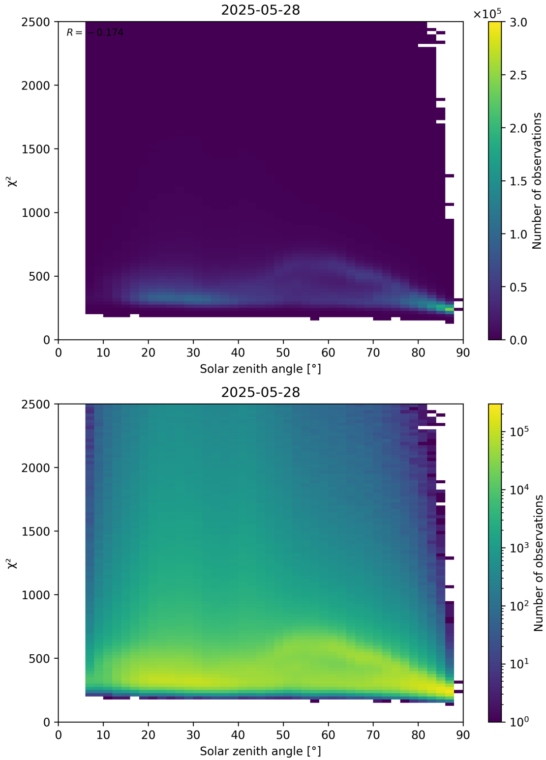
Figure 148: Scatter density plot of “Solar zenith angle” against “ \chi^2 ” for 2025-05-27 to 2025-05-29.
