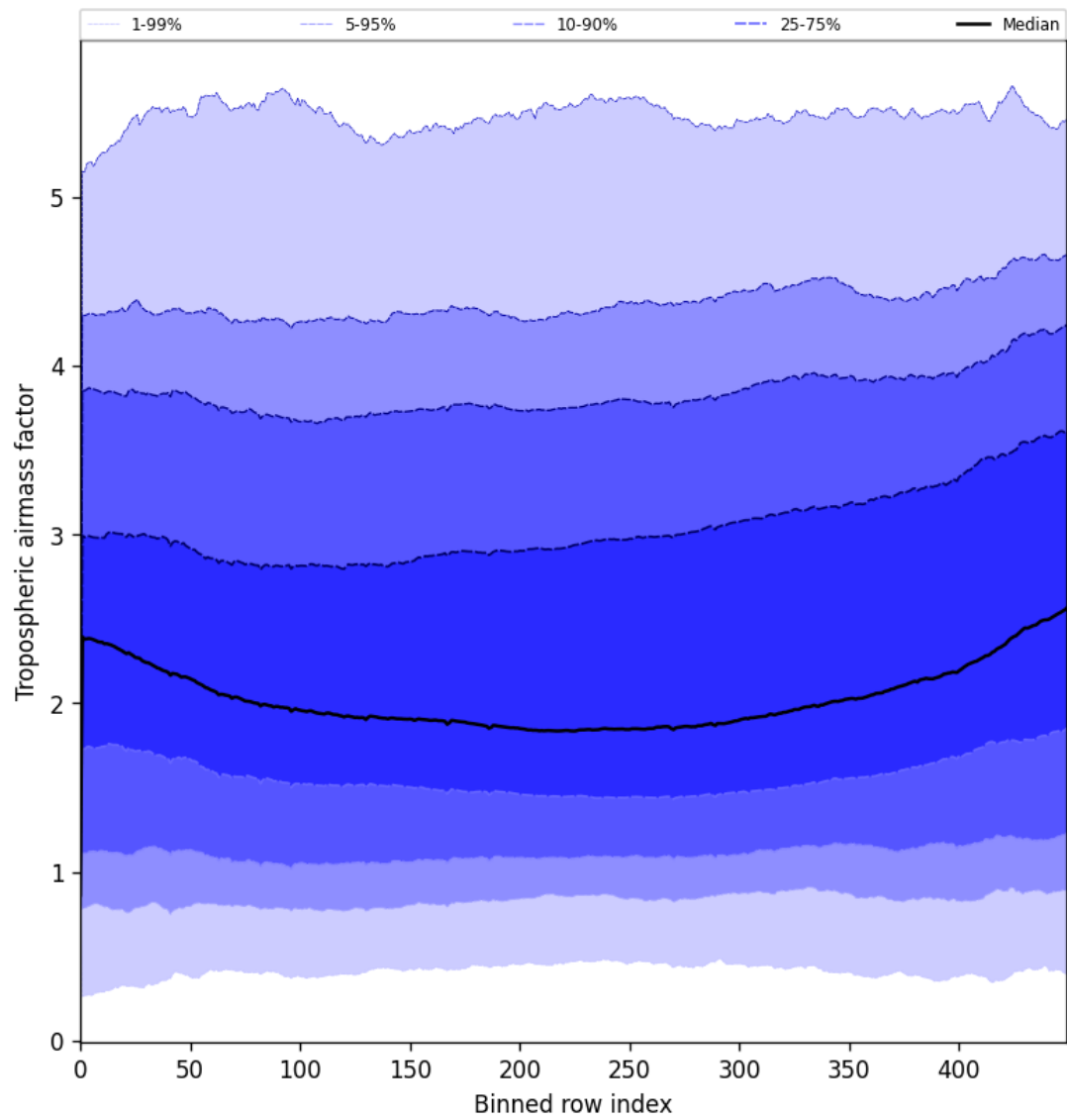
Figure 48: Along track statistics of “Tropospheric airmass factor” for 2025-05-27 to 2025-05-29
