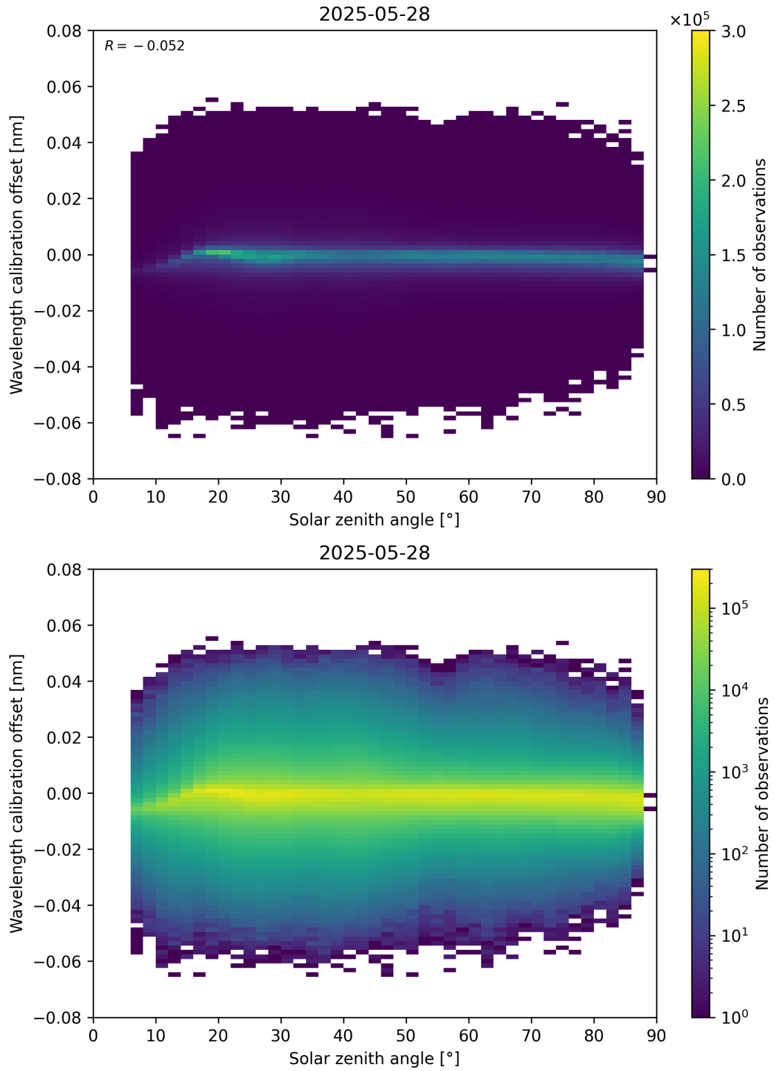
Figure 158: Scatter density plot of “Solar zenith angle” against “Wavelength calibration offset” for 2025-05-27 to 2025-05-29.
