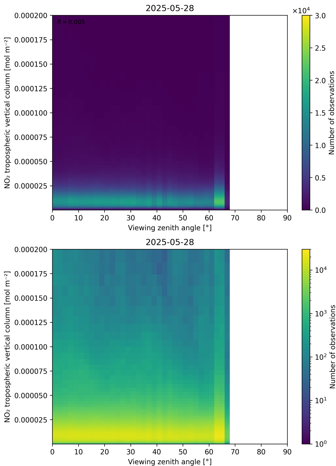
Figure 169: Scatter density plot of “Viewing zenith angle” against “NO 2 tropospheric vertical column” for 2025-05-27 to 2025-05-29.
