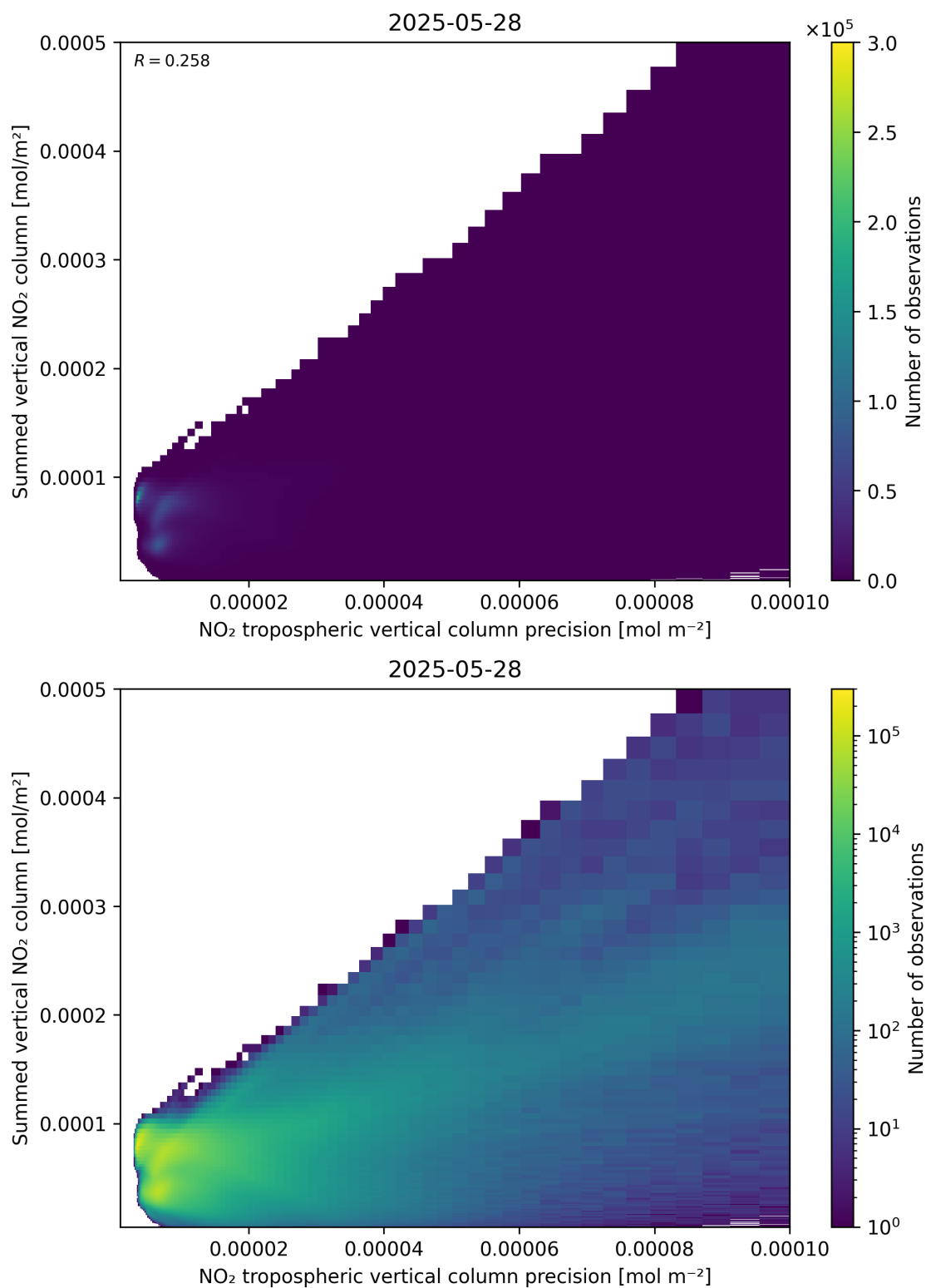
Figure 136: Scatter density plot of “NO 2 tropospheric vertical column precision” against “Summed vertical NO 2 column” for 2025-05-27 to 2025-05-29.
