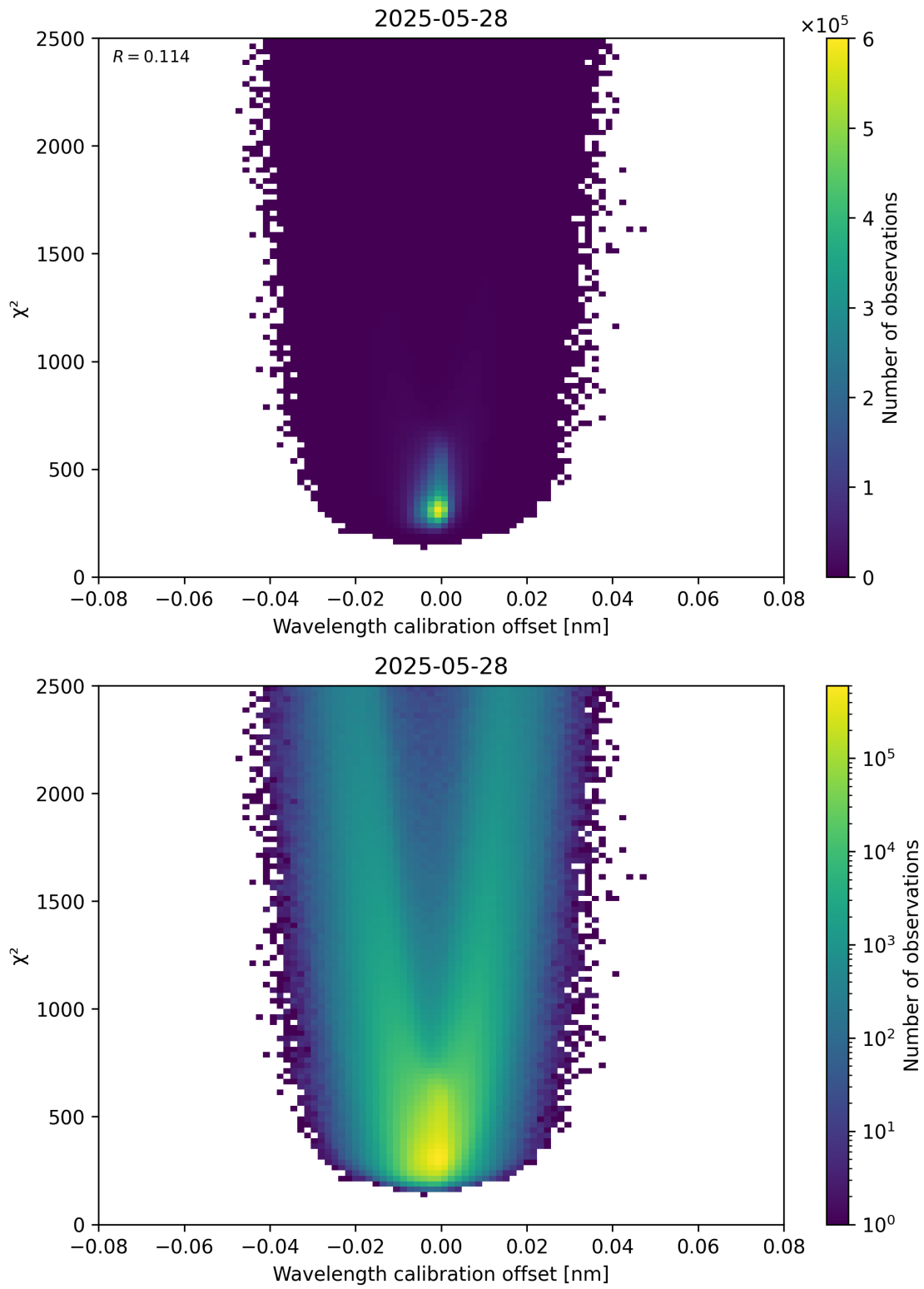
Figure 175: Scatter density plot of “Wavelength calibration offset” against “ \chi^2 ” for 2025-05-27 to 2025-05-29.
