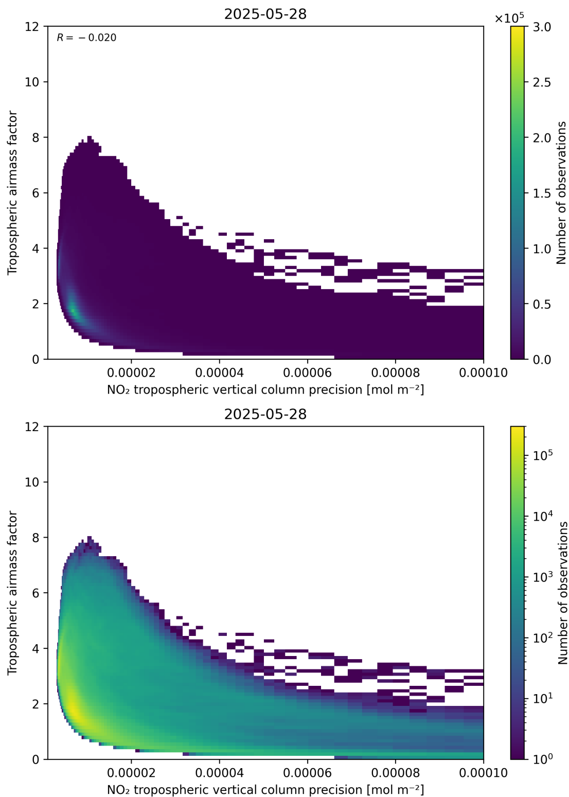
Figure 133: Scatter density plot of “NO 2 tropospheric vertical column precision” against “Tropospheric airmass factor” for 2025-05-27 to 2025-05-29.
