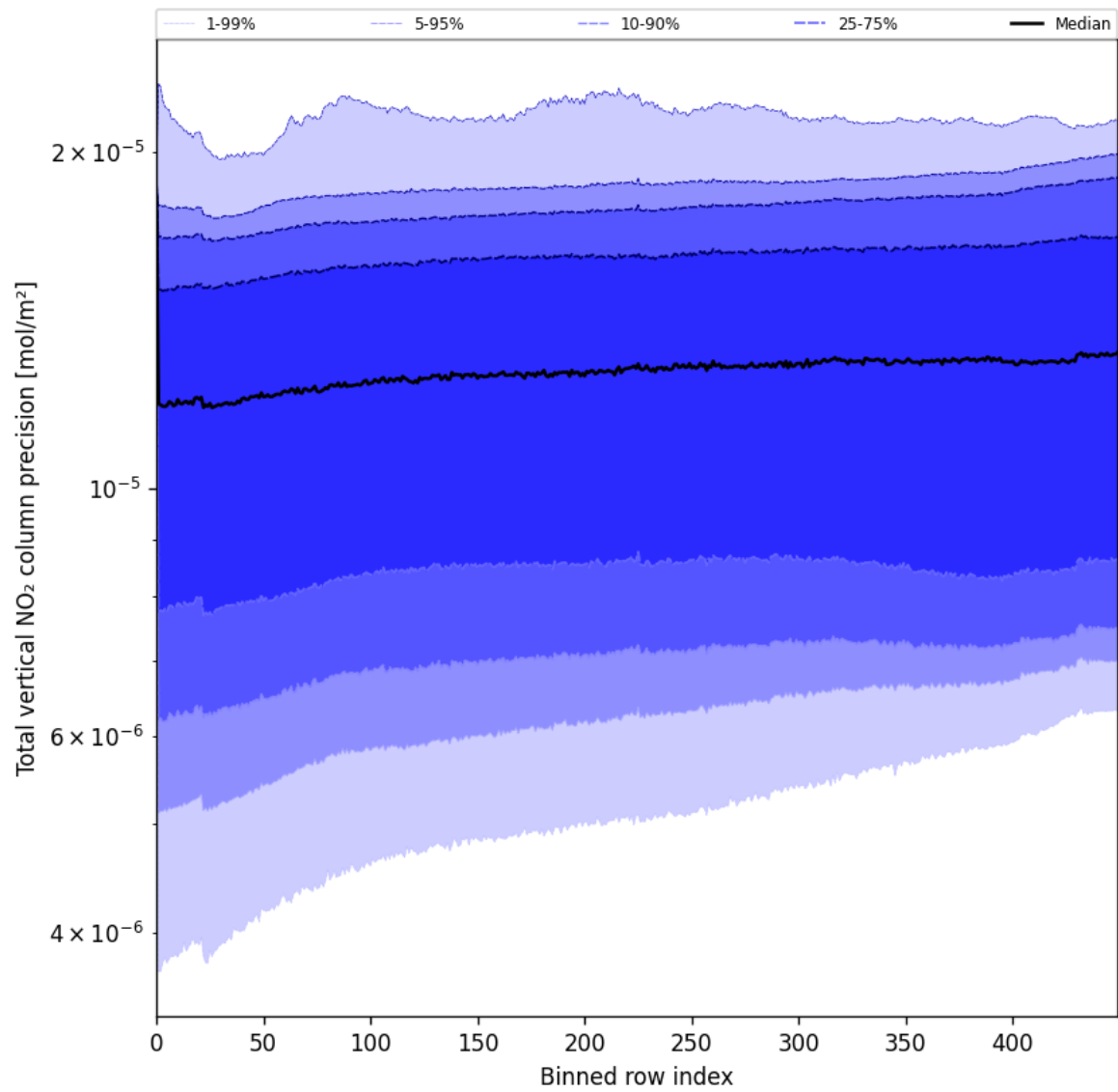
Figure 56: Along track statistics of “Total vertical NO 2 column precision” for 2025-05-27 to 2025-05-29
