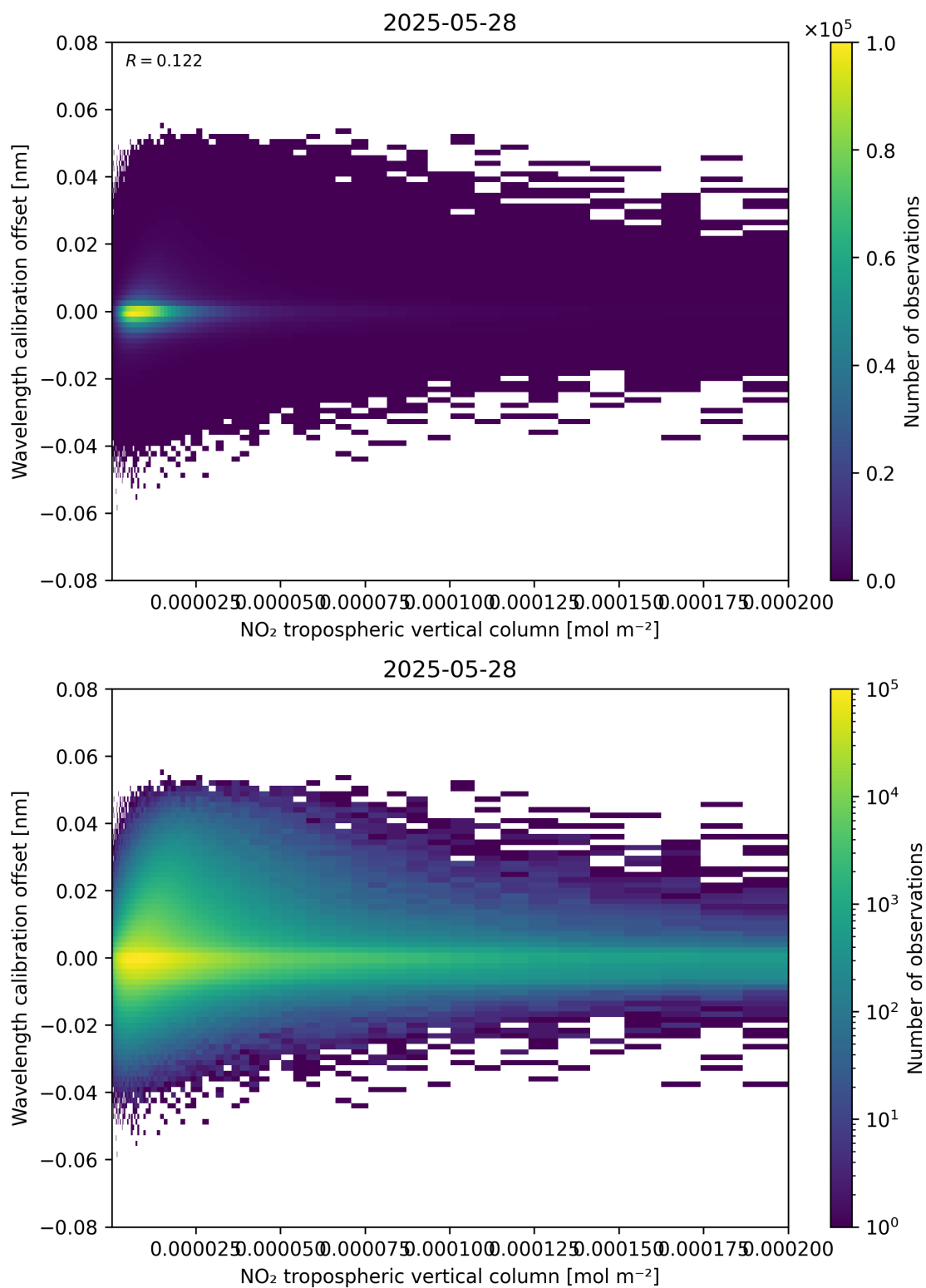
Figure 143: Scatter density plot of “NO 2 tropospheric vertical column” against “Wavelength calibration offset” for 2025-05-27 to 2025-05-29.
