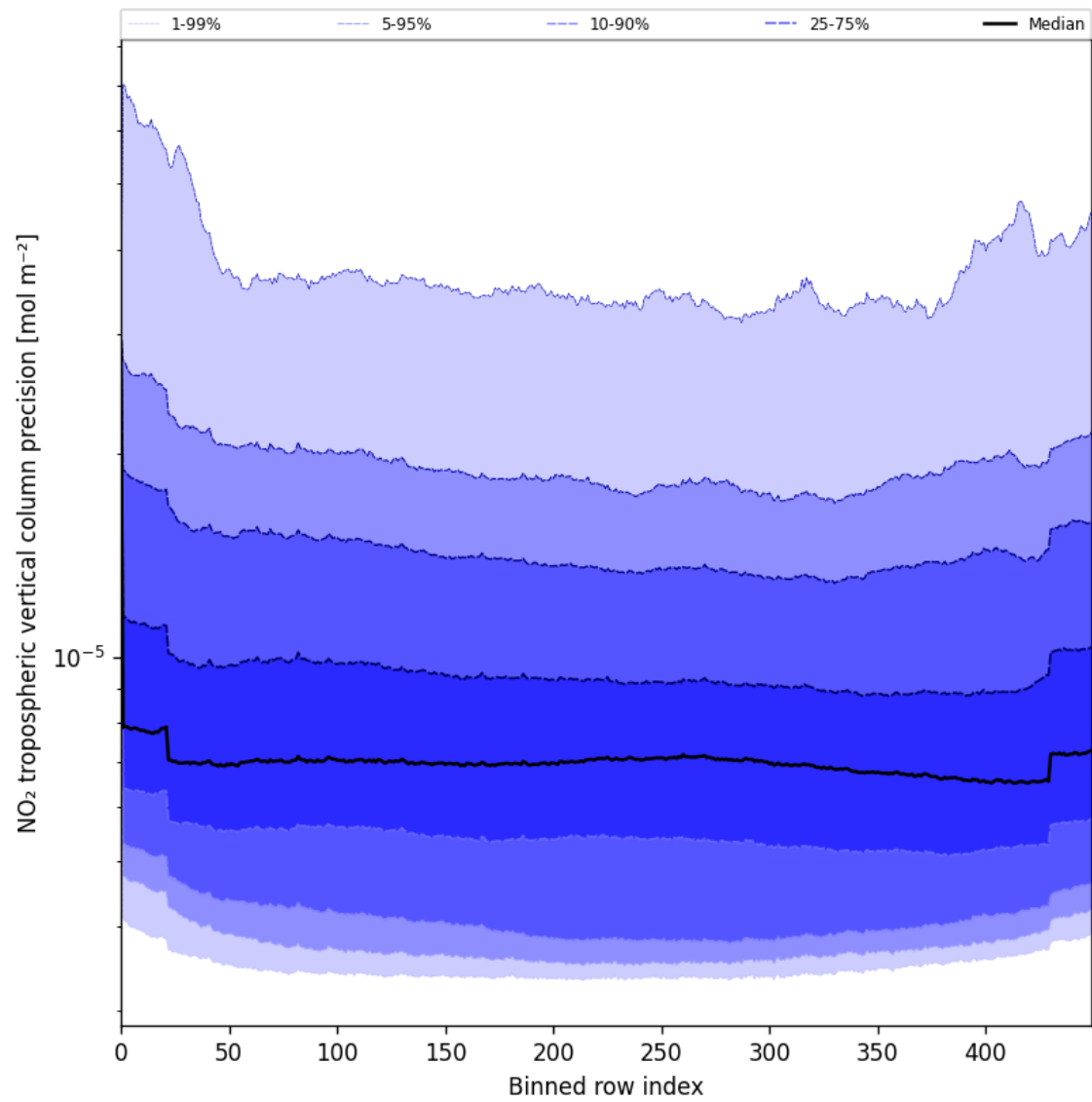
Figure 47: Along track statistics of “NO 2 tropospheric vertical column precision” for 2025-05-27 to 2025-05-29
