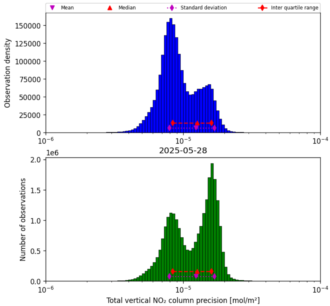
Figure 39: Histogram of “Total vertical NO 2 column precision” for 2025-05-27 to 2025-05-29
