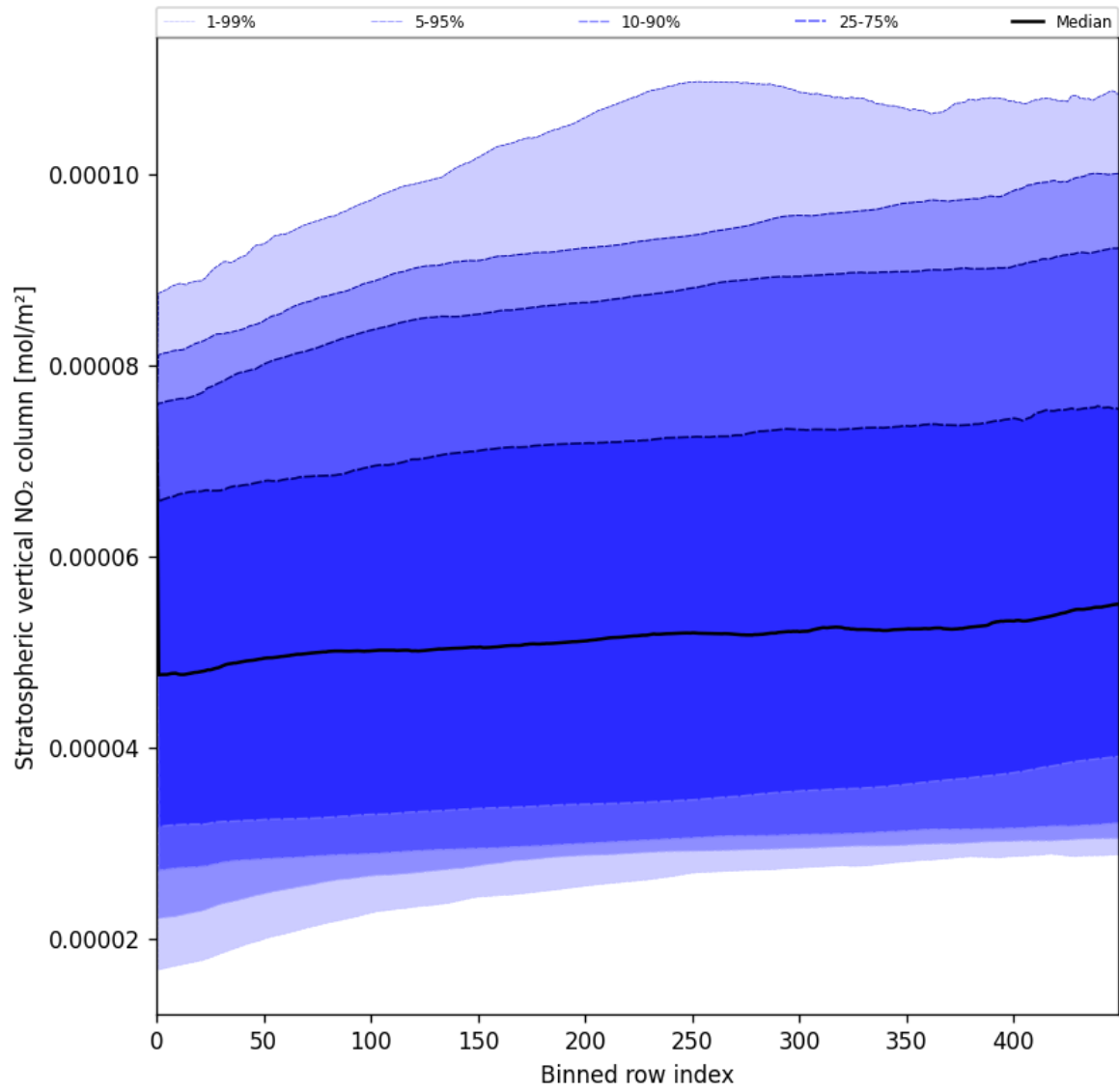
Figure 53: Along track statistics of “Stratospheric vertical NO 2 column” for 2025-05-27 to 2025-05-29
