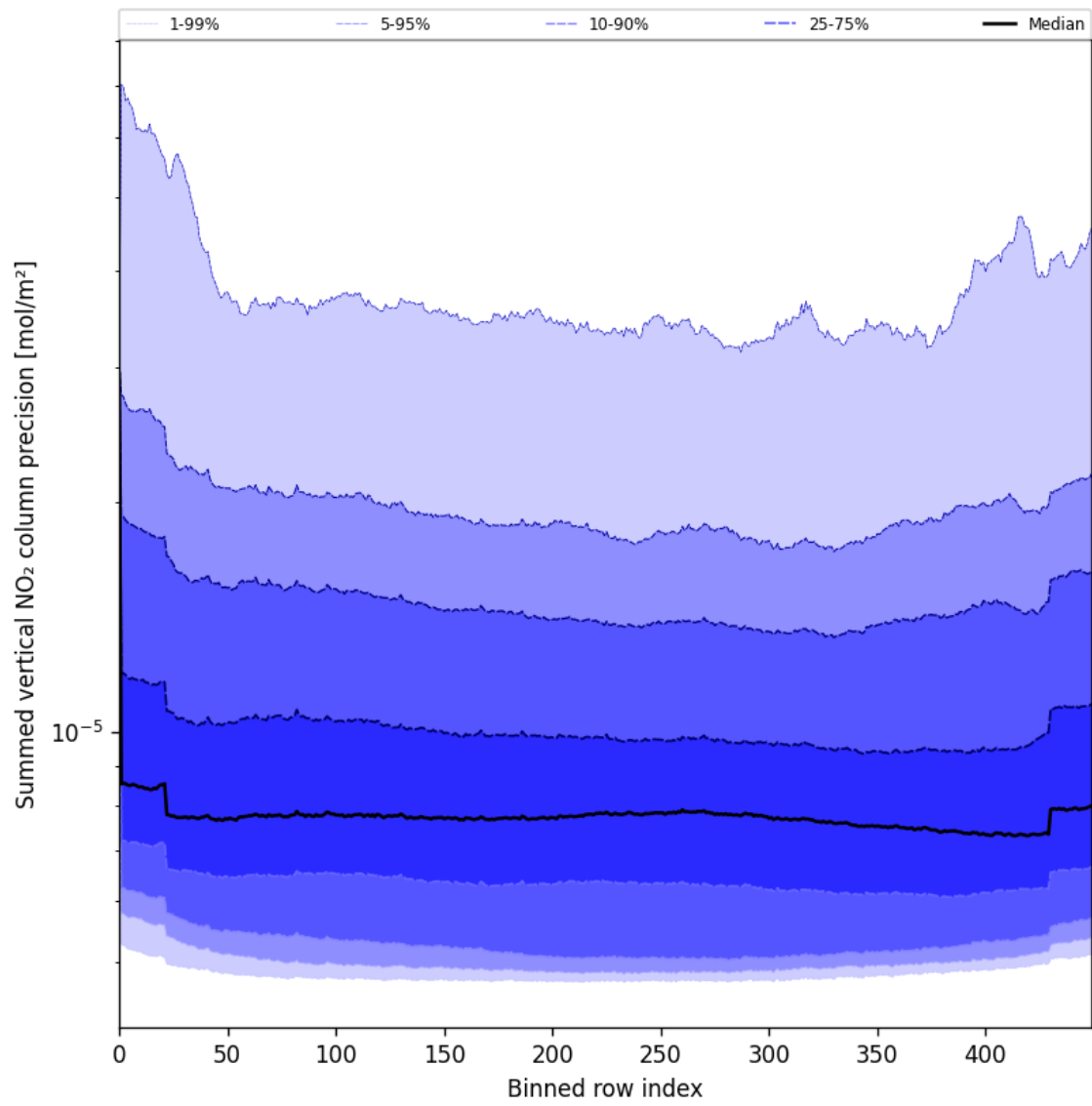
Figure 58: Along track statistics of “Summed vertical NO 2 column precision” for 2025-05-27 to 2025-05-29
