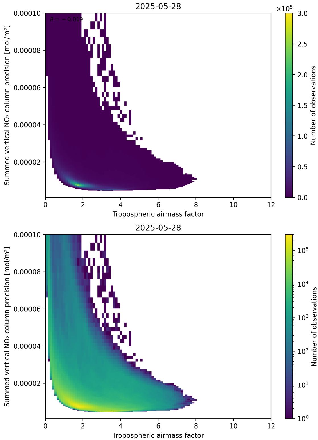
Figure 76: Scatter density plot of “Tropospheric air mass factor” against “Summed vertical NO 2 column precision” for 2025-05-27 to 2025-05-29.
