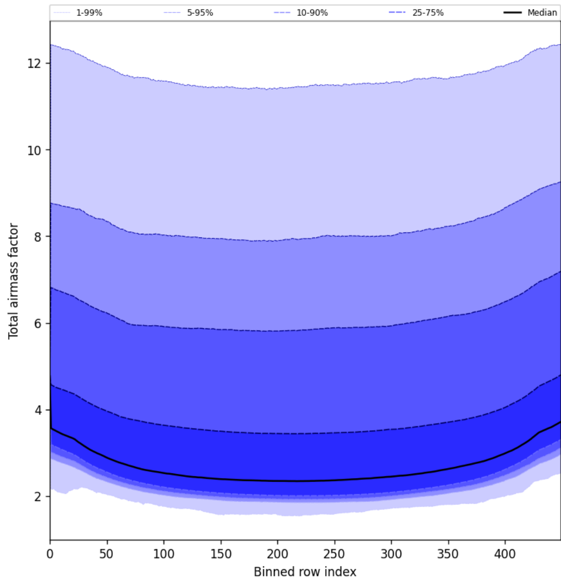
Figure 49: Along track statistics of “Total airmass factor” for 2025-05-27 to 2025-05-29
