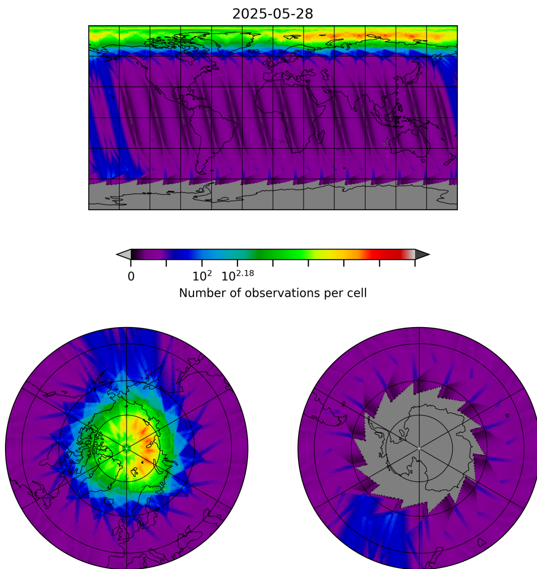
Figure 10: Map of the number of observations for 2025-05-27 to 2025-05-29
