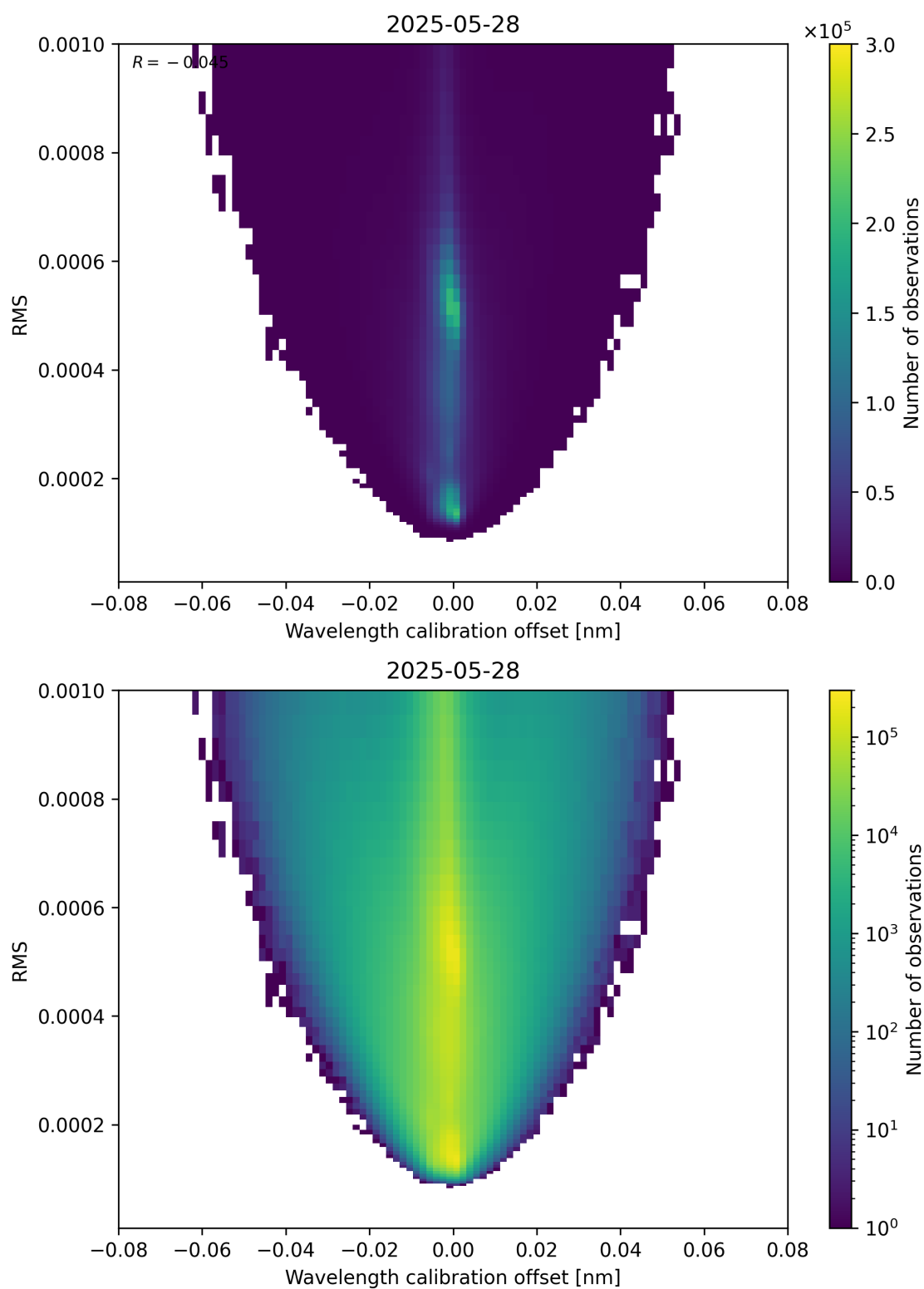
Figure 181: Scatter density plot of “Wavelength calibration offset” against “RMS” for 2025-05-27 to 2025-05-29.
