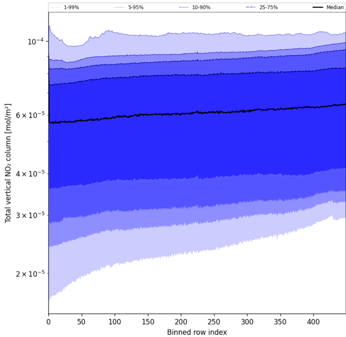
Figure 55: Along track statistics of “Total vertical NO 2 column” for 2025-05-27 to 2025-05-29
