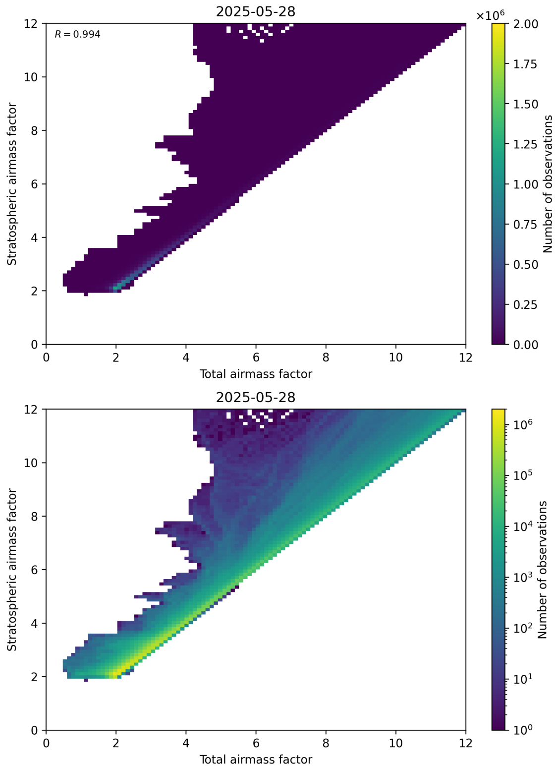
Figure 62: Scatter density plot of “Total airmass factor” against “Stratospheric airmass factor” for 2025-05-27 to 2025-05-29.
