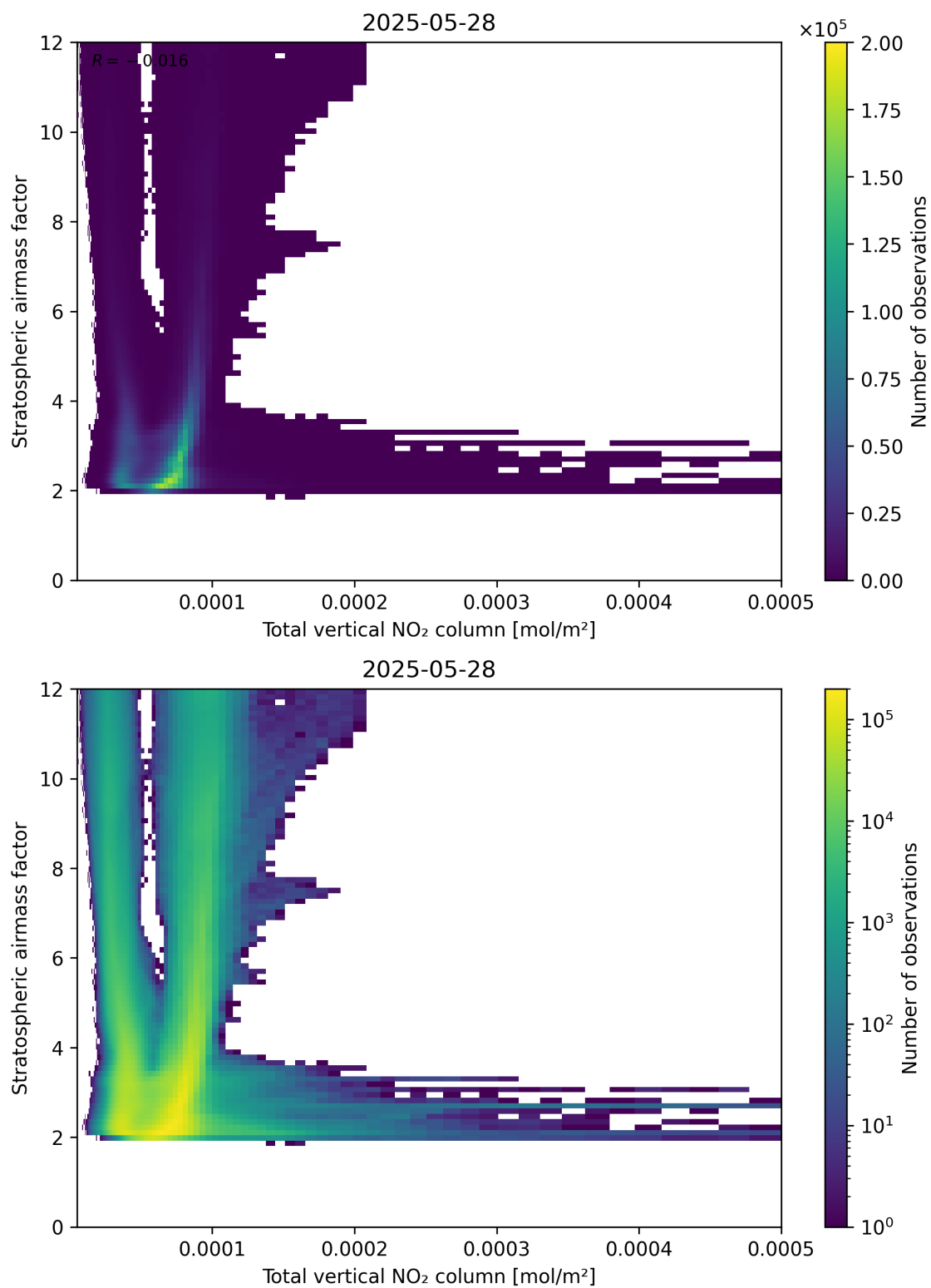
Figure 110: Scatter density plot of “Total vertical NO 2 column” against “Stratospheric air mass factor” for 2025-05-27 to 2025-05-29.
