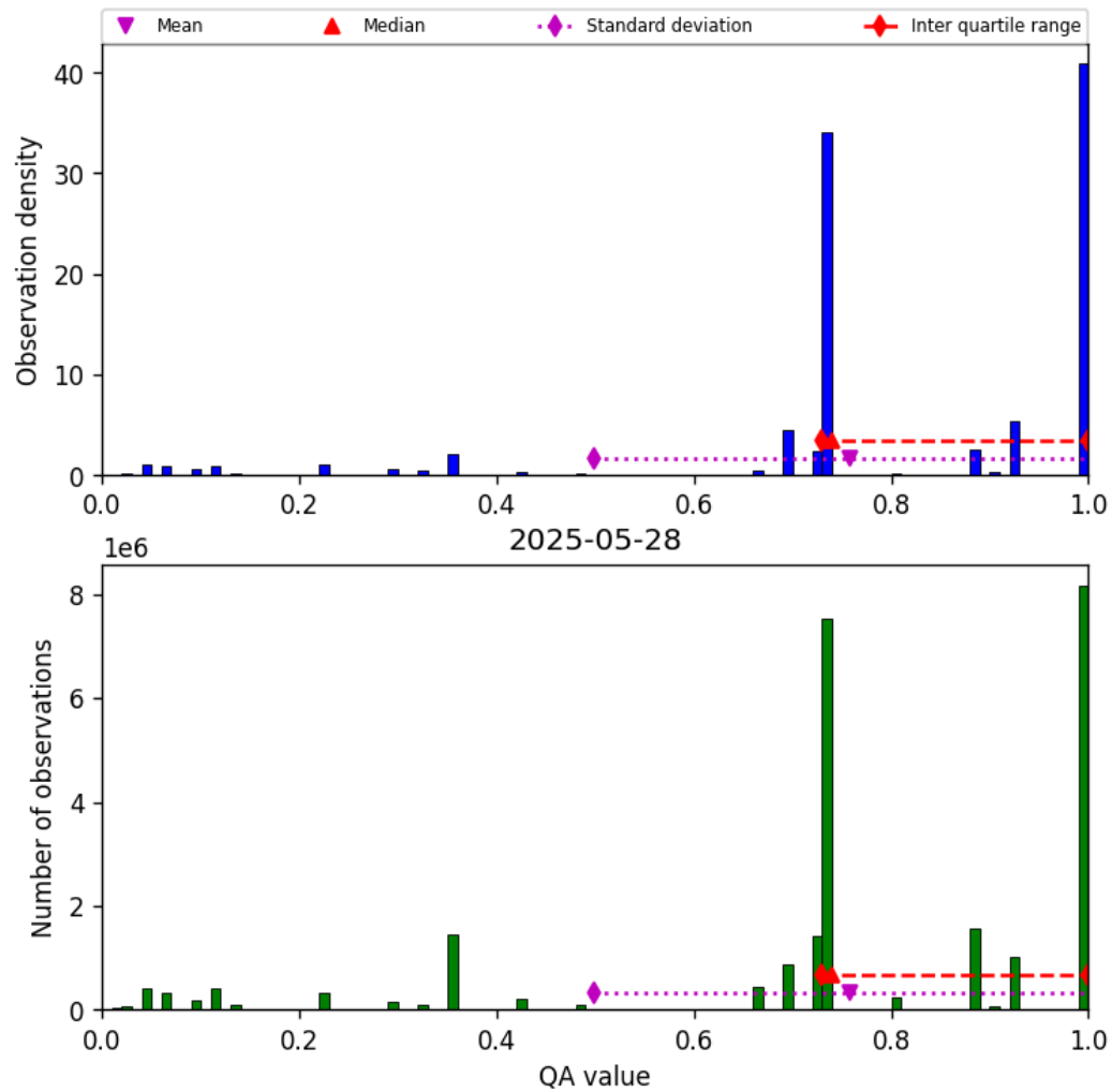
Figure 28: Histogram of “QA value” for 2025-05-27 to 2025-05-29
