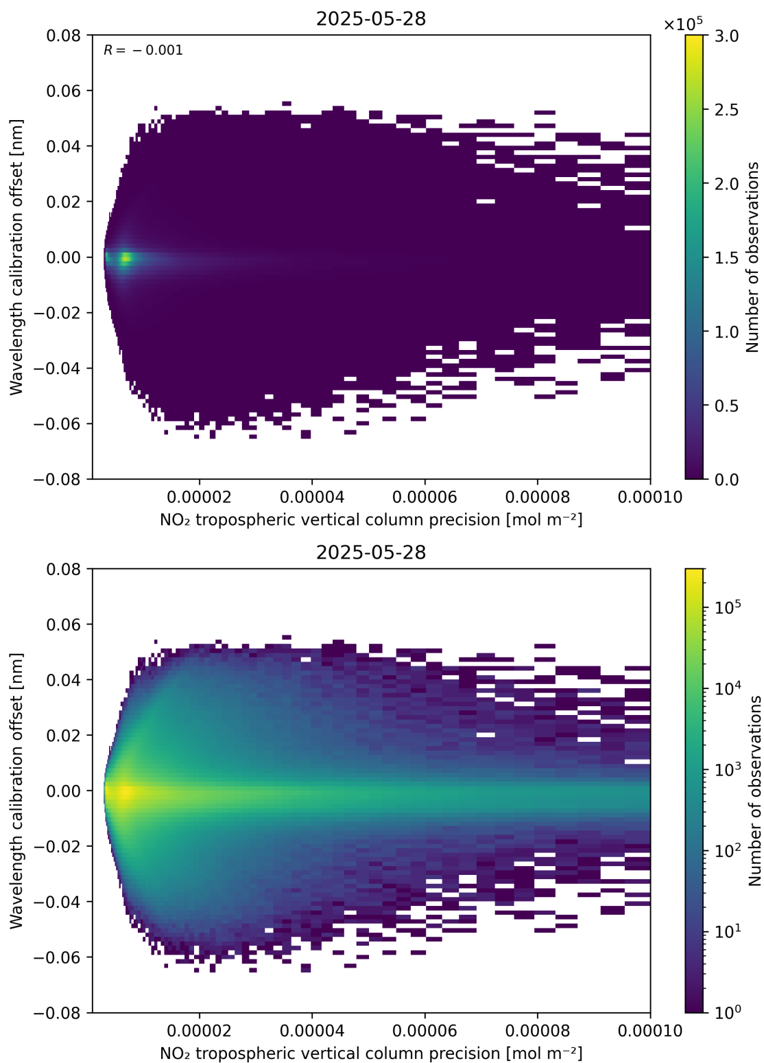
Figure 141: Scatter density plot of “NO 2 tropospheric vertical column precision” against “Wavelength calibration offset” for 2025-05-27 to 2025-05-29.
