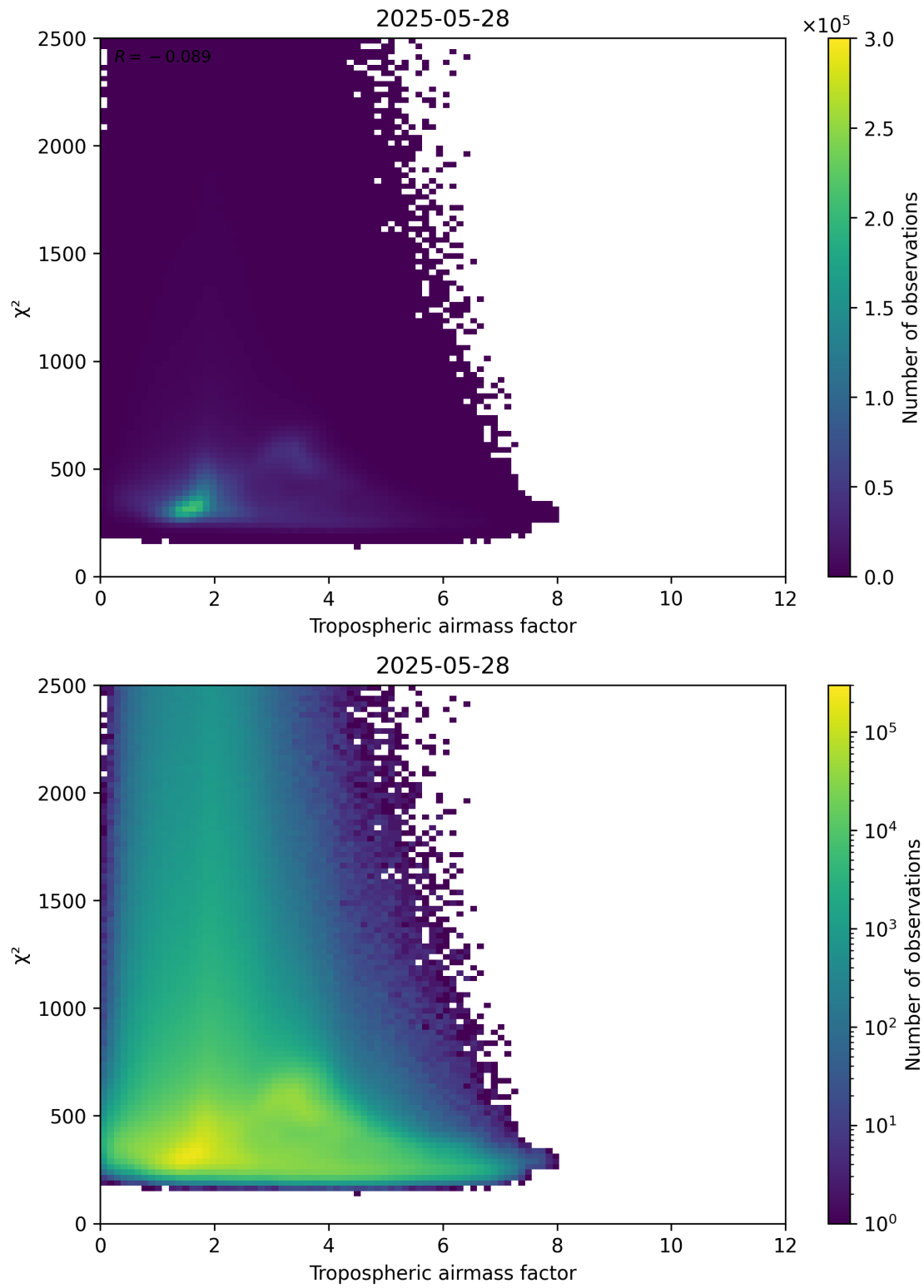
Figure 73: Scatter density plot of “Tropospheric airmass factor” against “ \chi^2 ” for 2025-05-27 to 2025-05-29.
