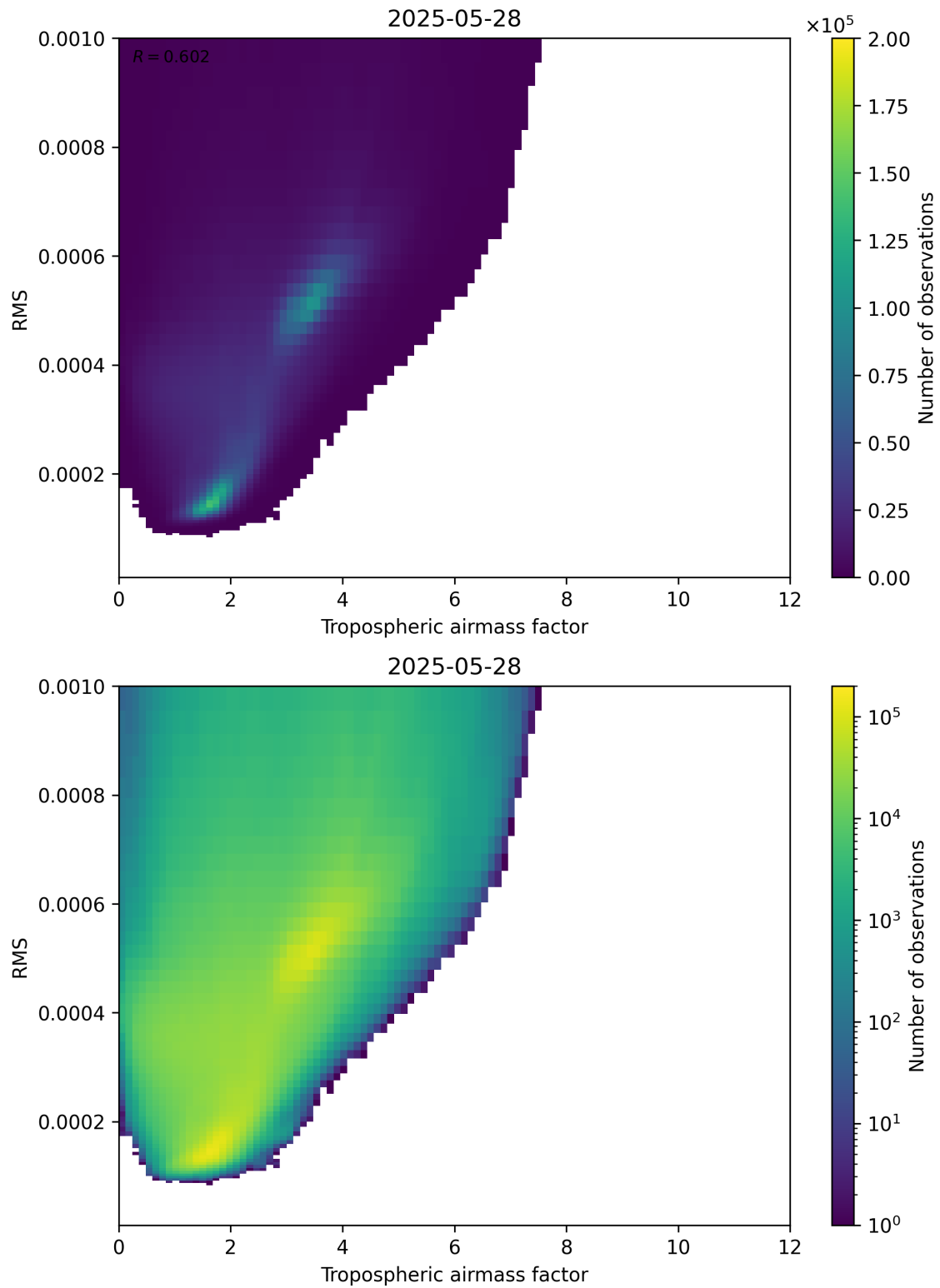
Figure 79: Scatter density plot of “Tropospheric airmass factor” against “RMS” for 2025-05-27 to 2025-05-29.
