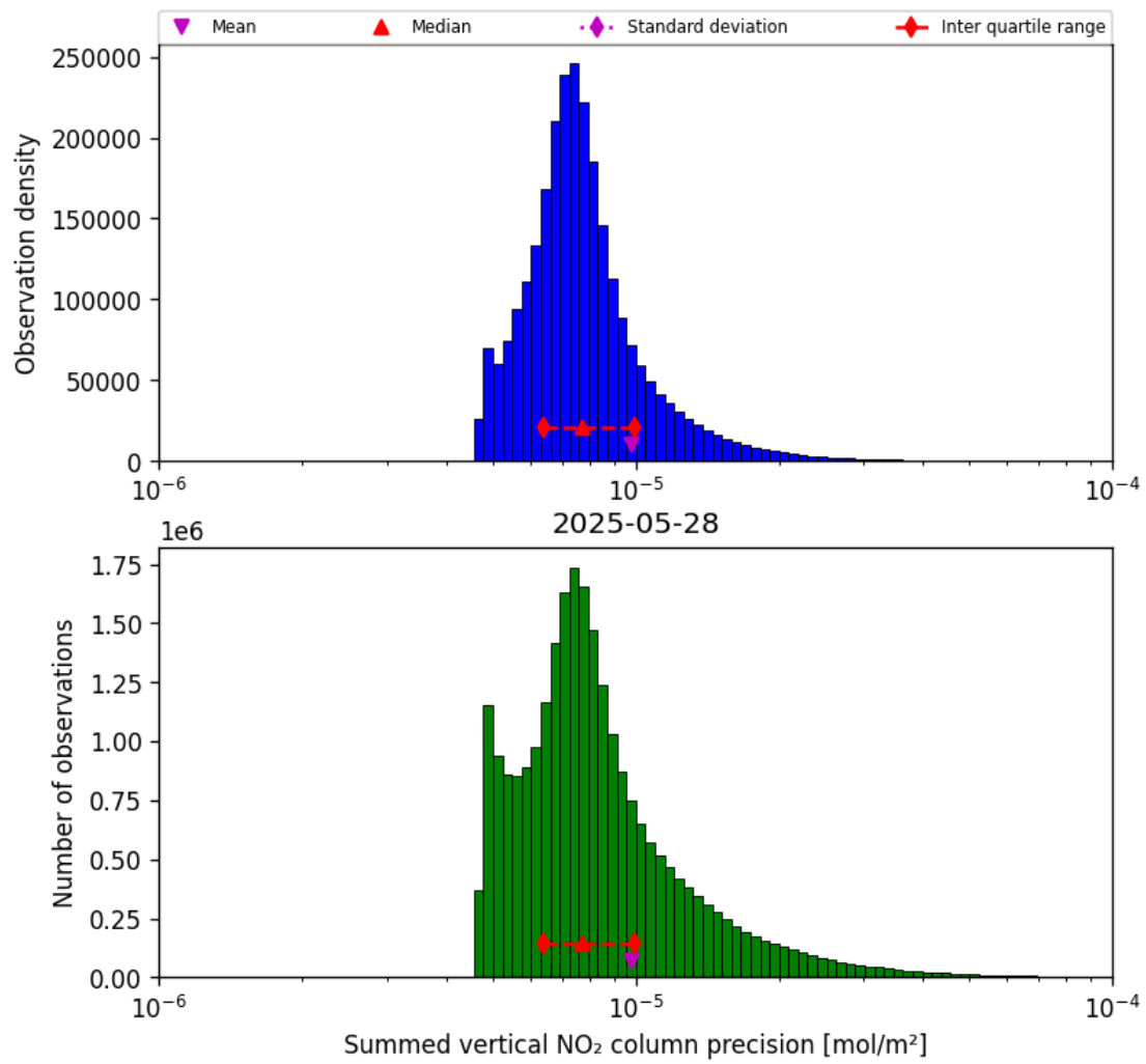
Figure 41: Histogram of “Summed vertical NO 2 column precision” for 2025-05-27 to 2025-05-29
