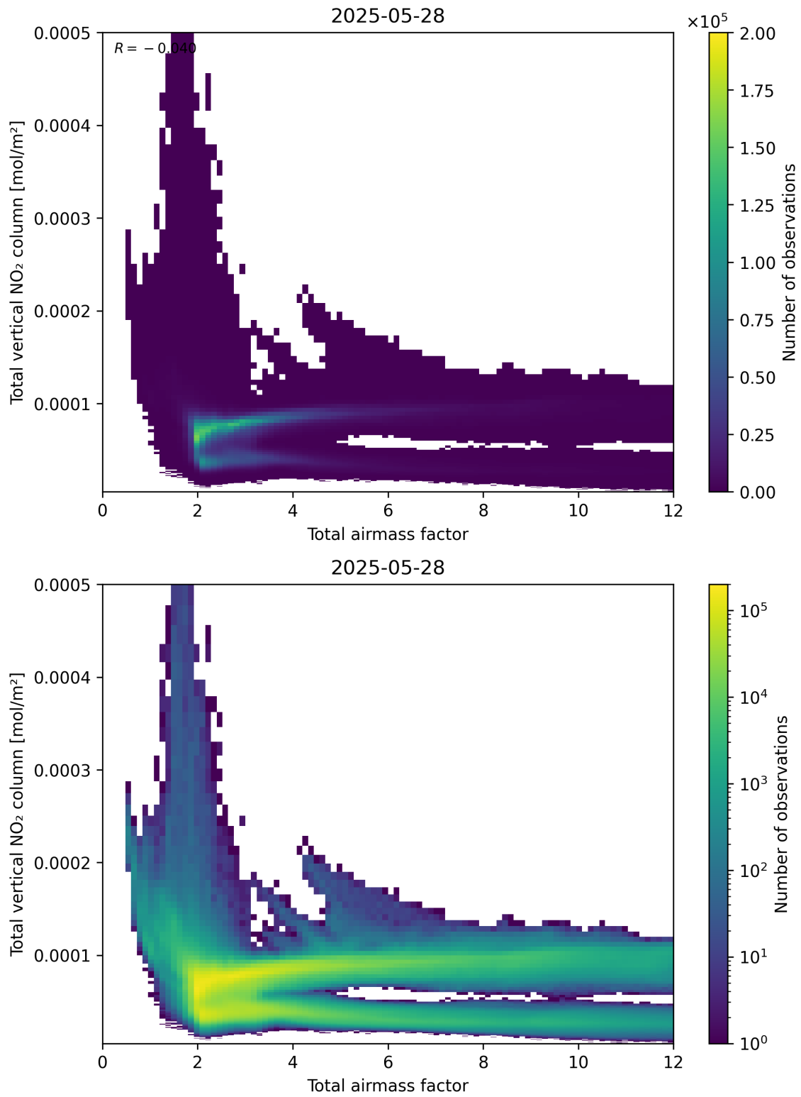
Figure 67: Scatter density plot of “Total airmass factor” against “Total vertical NO 2 column” for 2025-05-27 to 2025-05-29.
