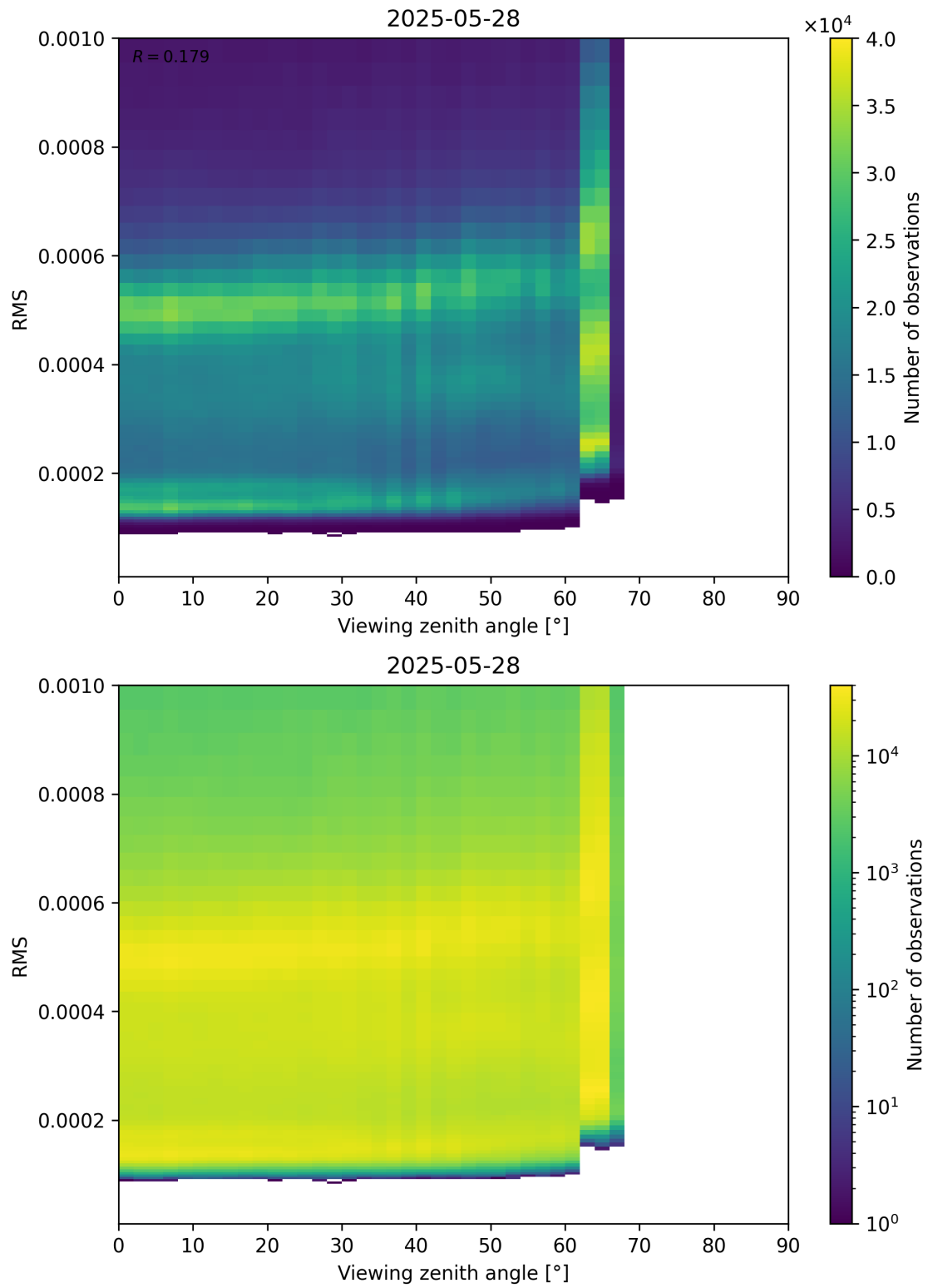
Figure 171: Scatter density plot of “Viewing zenith angle” against “RMS” for 2025-05-27 to 2025-05-29.
