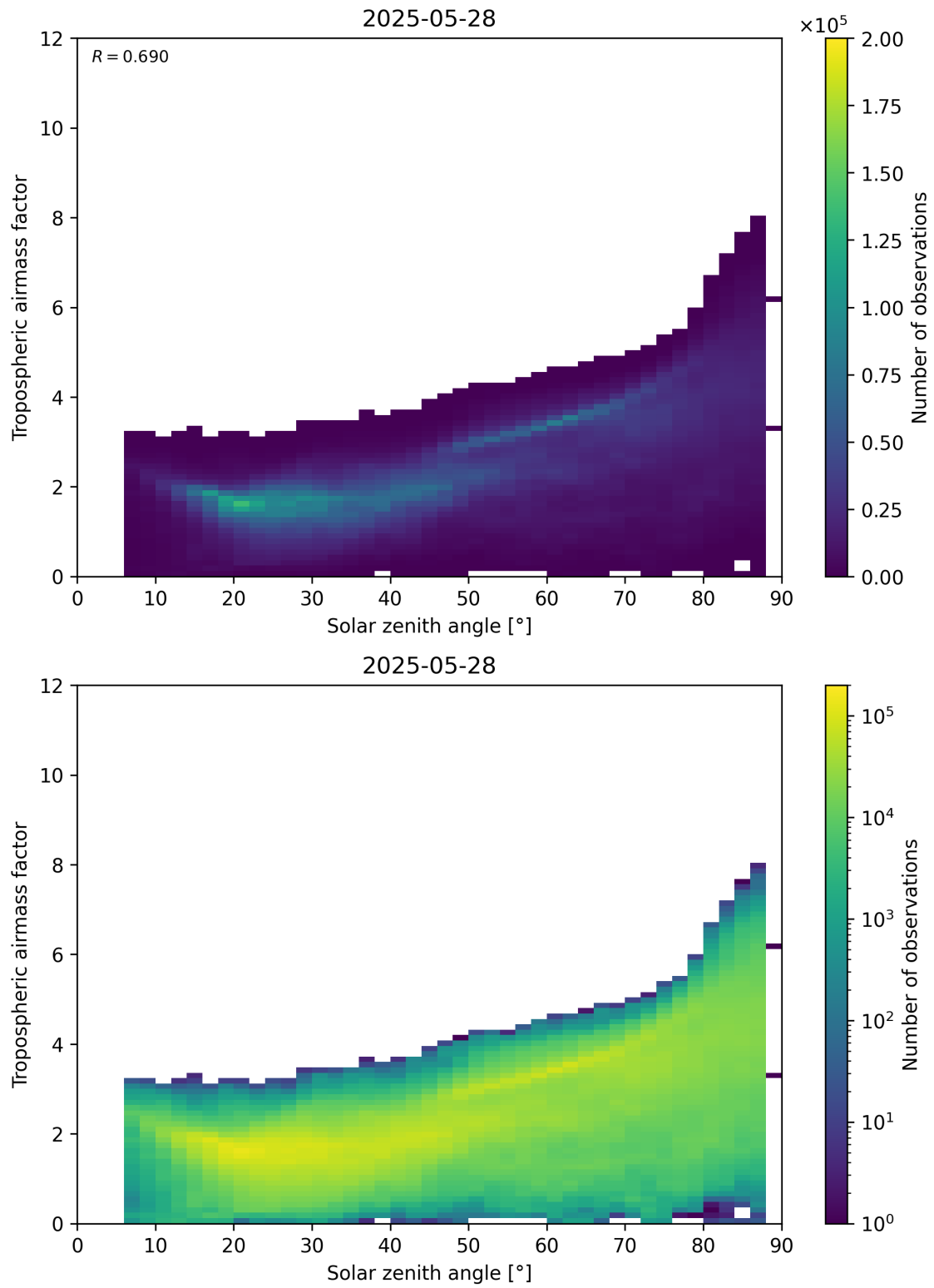
Figure 147: Scatter density plot of “Solar zenith angle” against “Tropospheric airmass factor” for 2025-05-27 to 2025-05-29.
