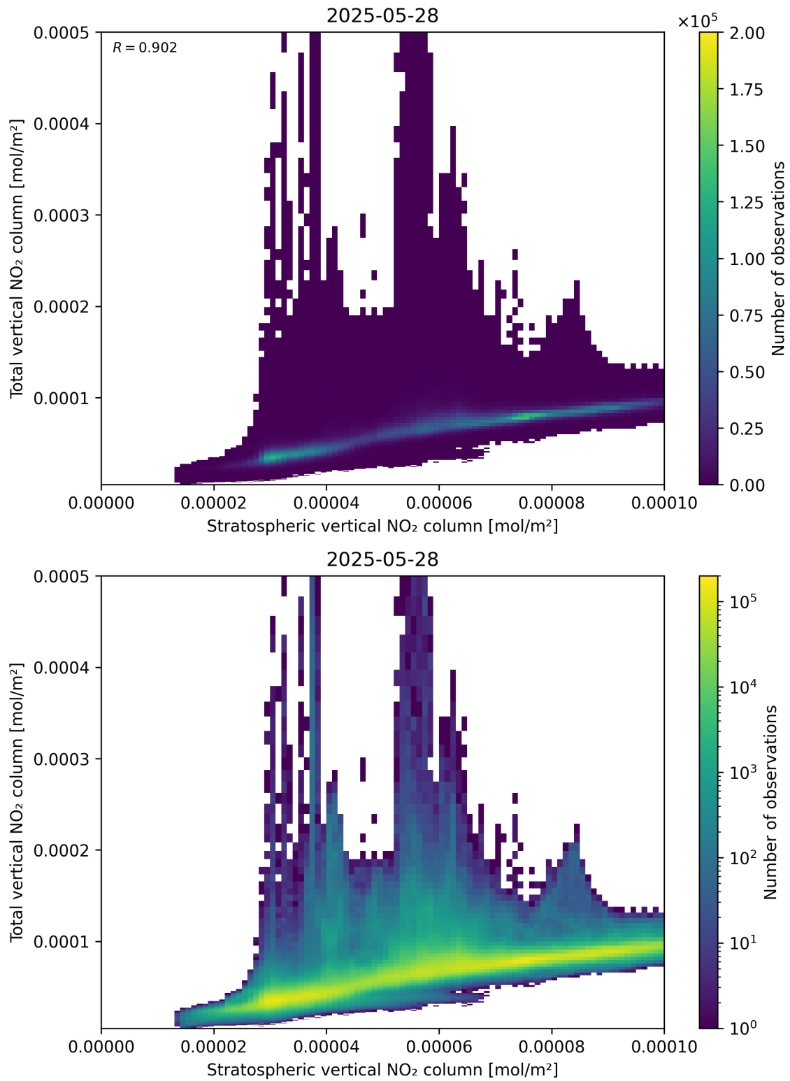
Figure 100: Scatter density plot of “Stratospheric vertical NO 2 column” against “Total vertical NO 2 column” for 2025-05-27 to 2025-05-29.
