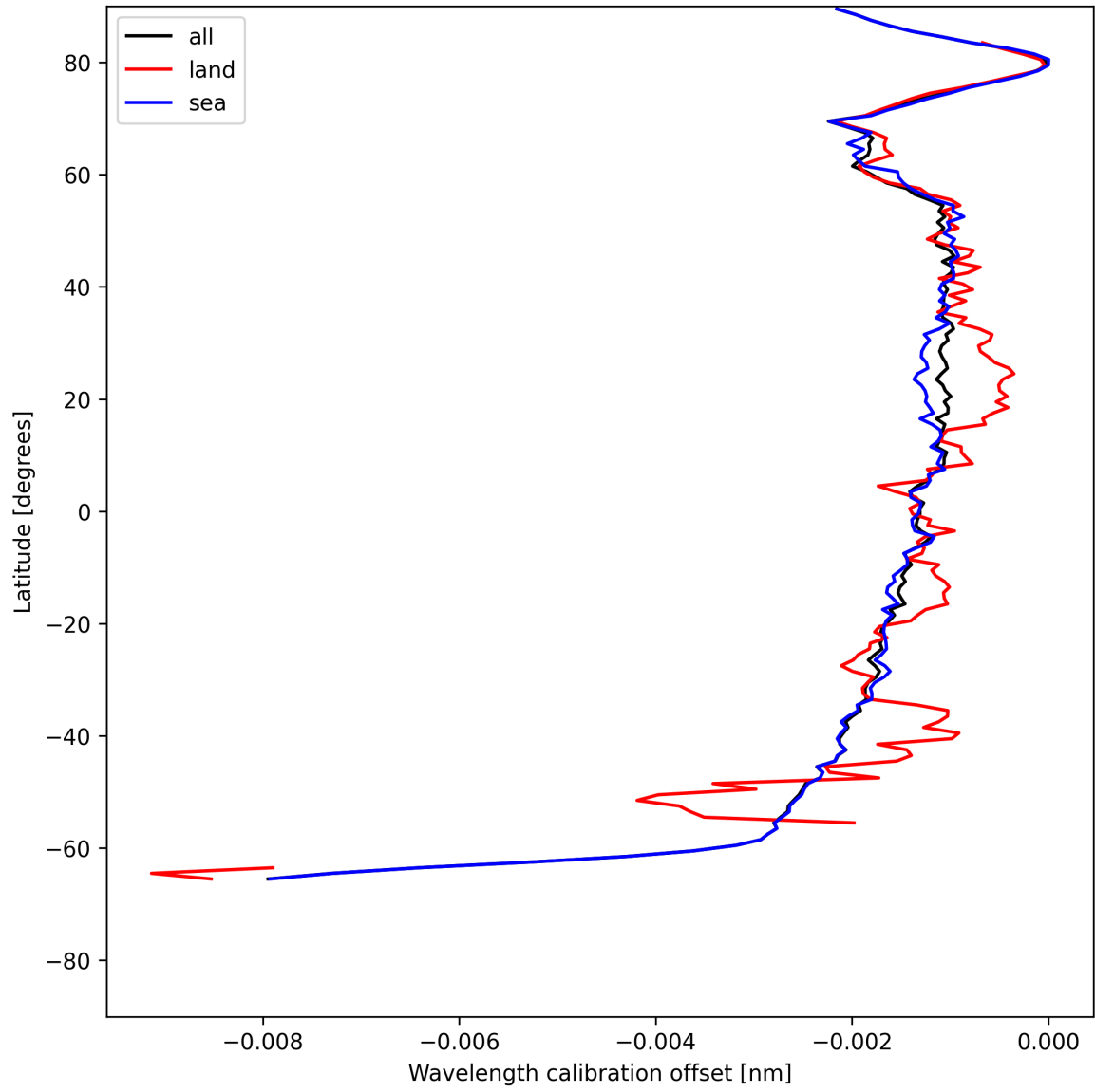
Figure 18: Zonal average of “Wavelength calibration offset” for 2025-05-27 to 2025-05-29.
