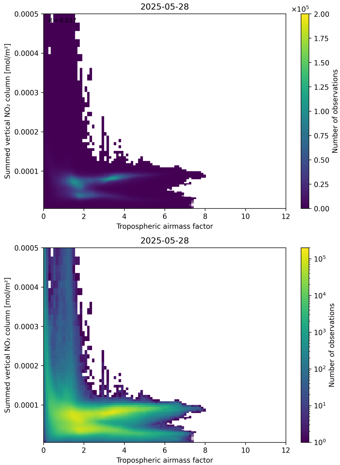
Figure 75: Scatter density plot of “Tropospheric airmass factor” against “Summed vertical NO 2 column” for 2025-05-27 to 2025-05-29.
