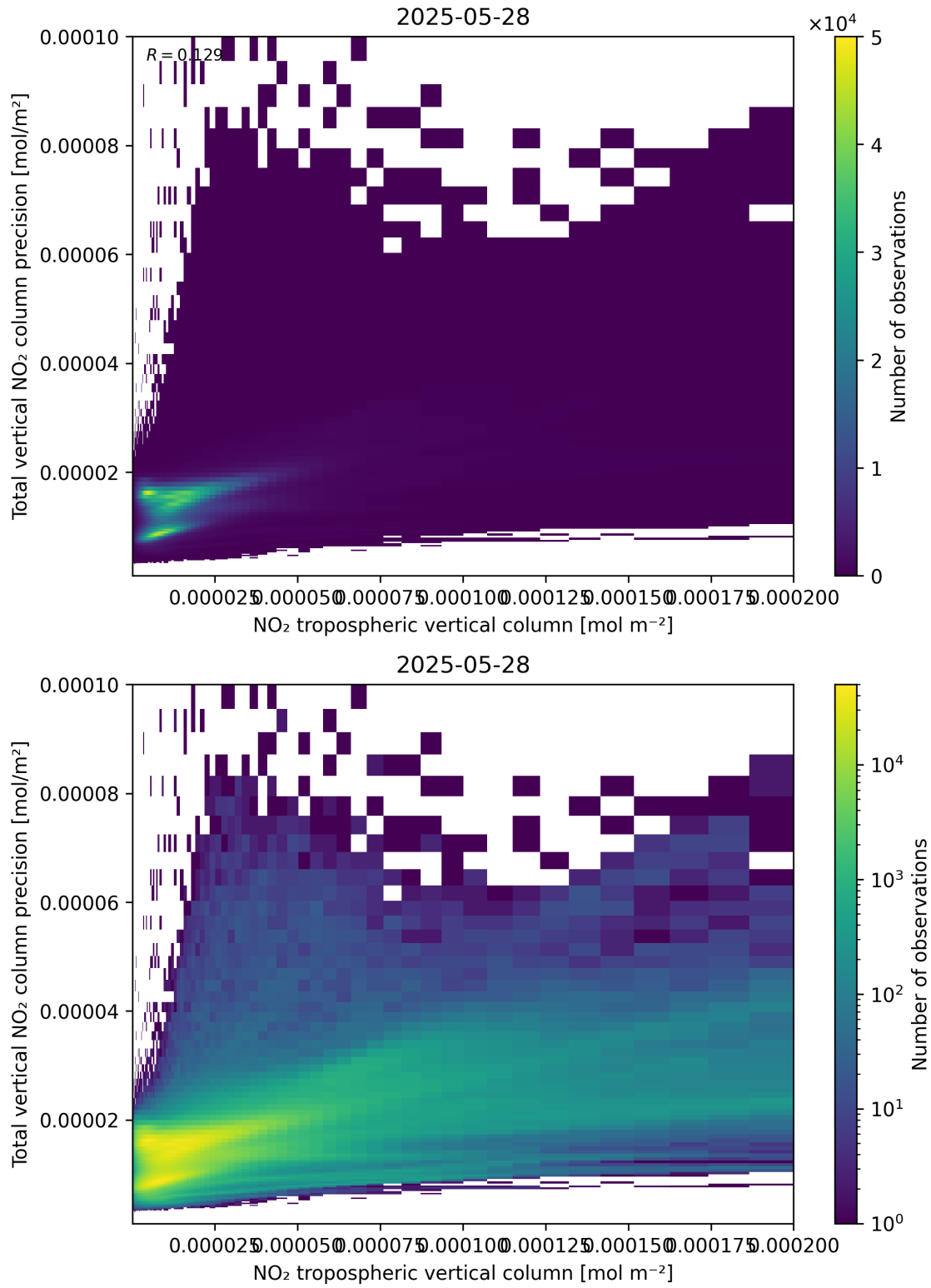
Figure 129: Scatter density plot of “NO 2 tropospheric vertical column” against “Total vertical NO 2 column precision” for 2025-05-27 to 2025-05-29.
