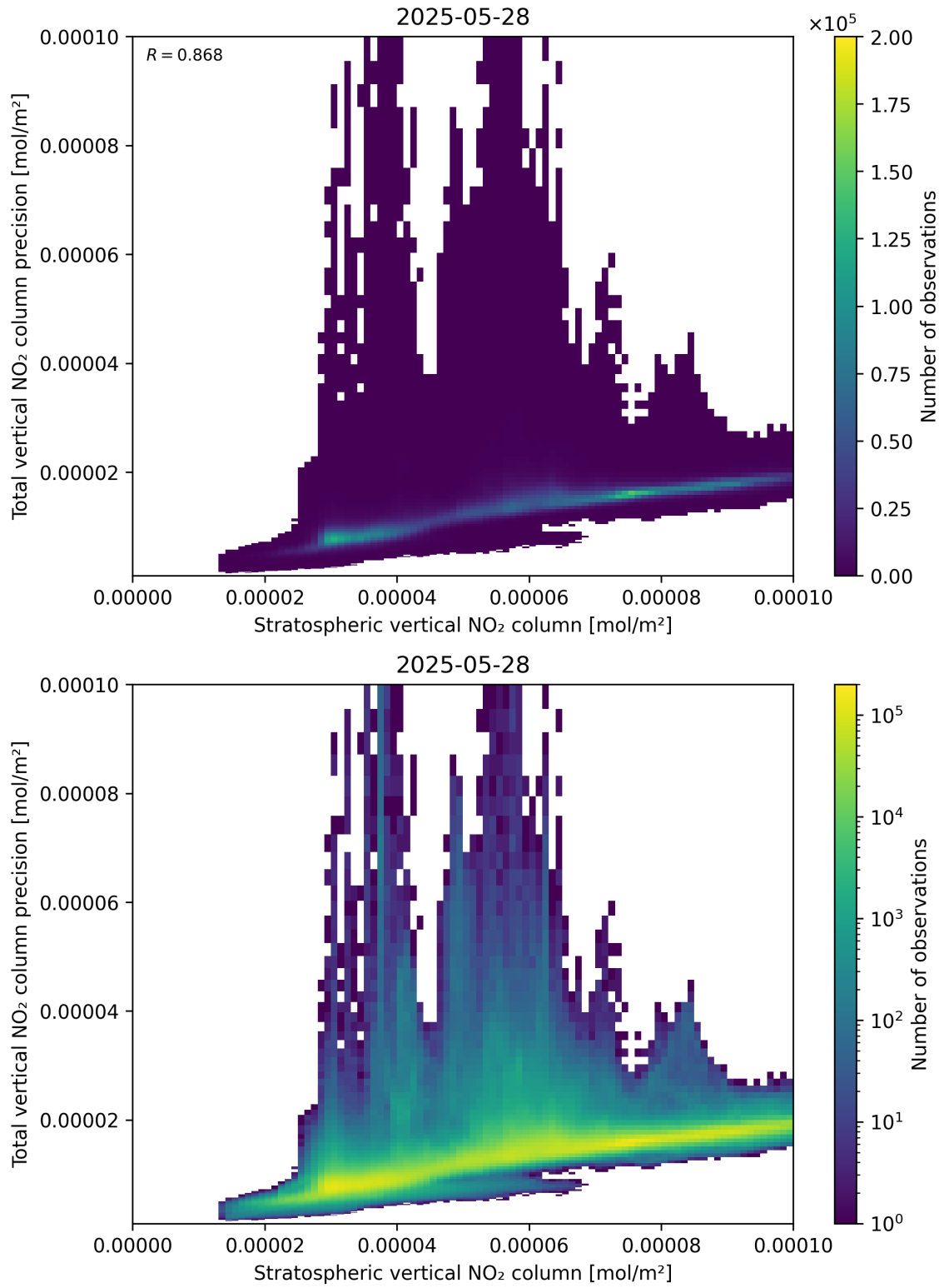
Figure 101: Scatter density plot of “Stratospheric vertical NO 2 column” against “Total vertical NO 2 column precision” for 2025-05-27 to 2025-05-29.
