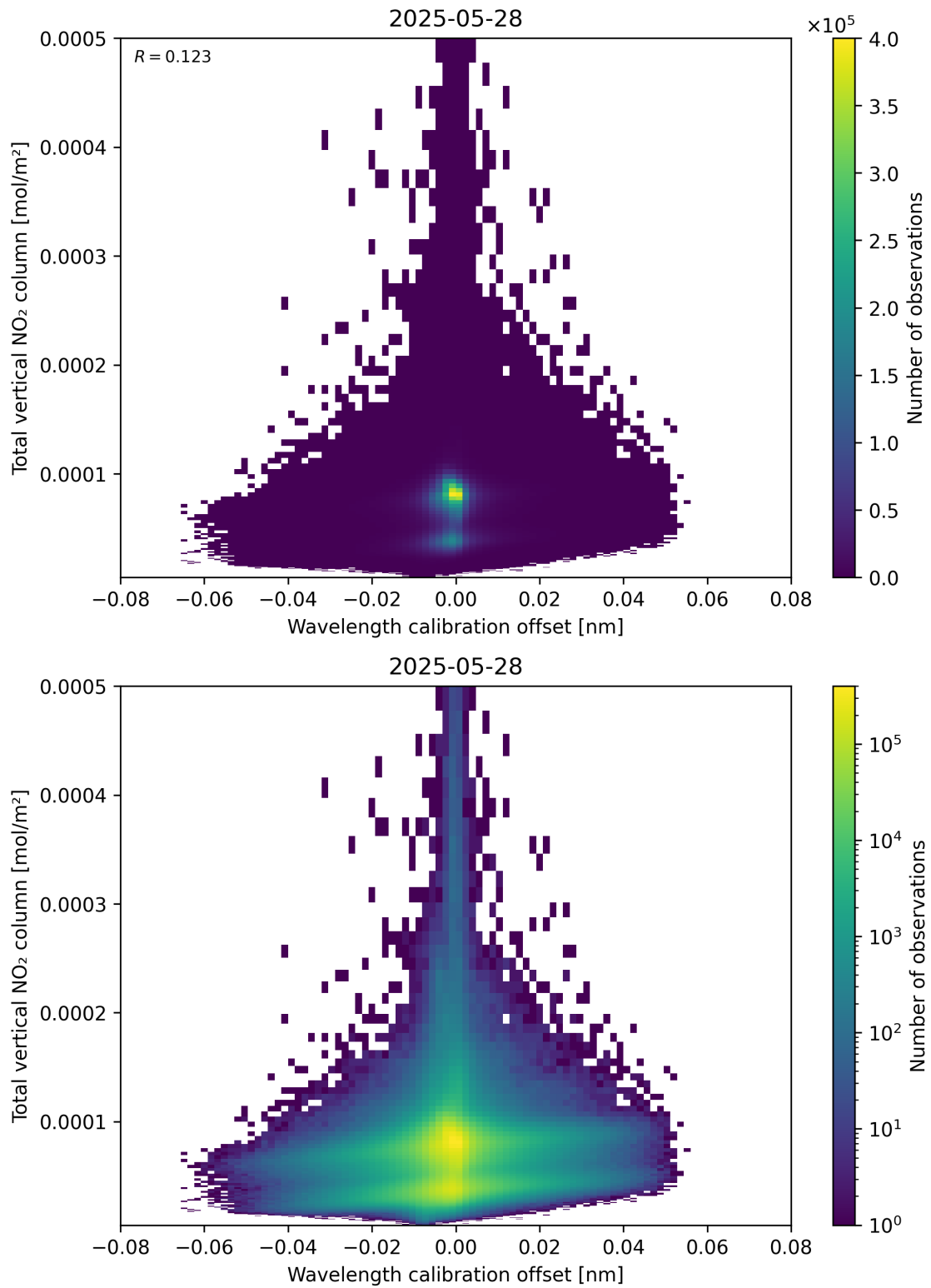
Figure 179: Scatter density plot of “Wavelength calibration offset” against “Total vertical NO 2 column” for 2025-05-27 to 2025-05-29.
