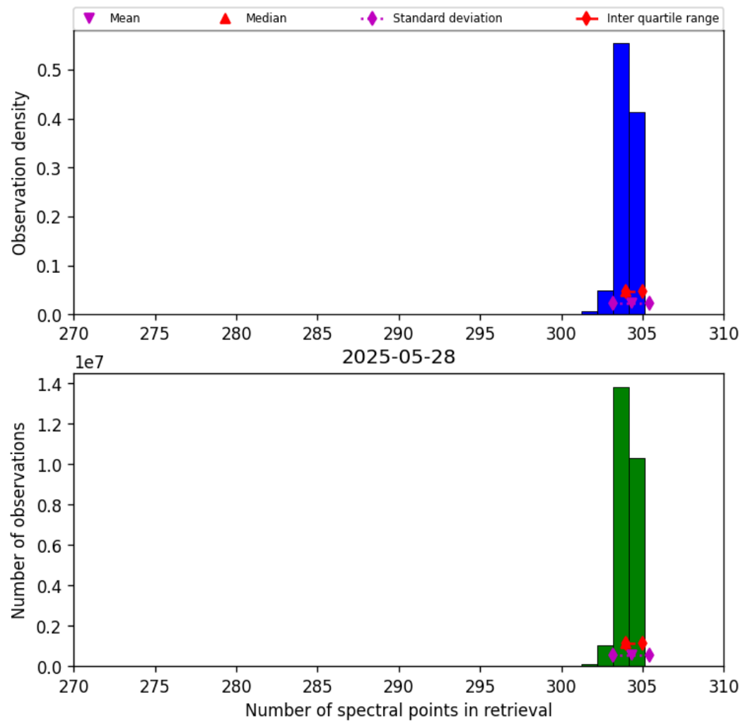
Figure 33: Histogram of “Number of spectral points in retrieval” for 2025-05-27 to 2025-05-29
