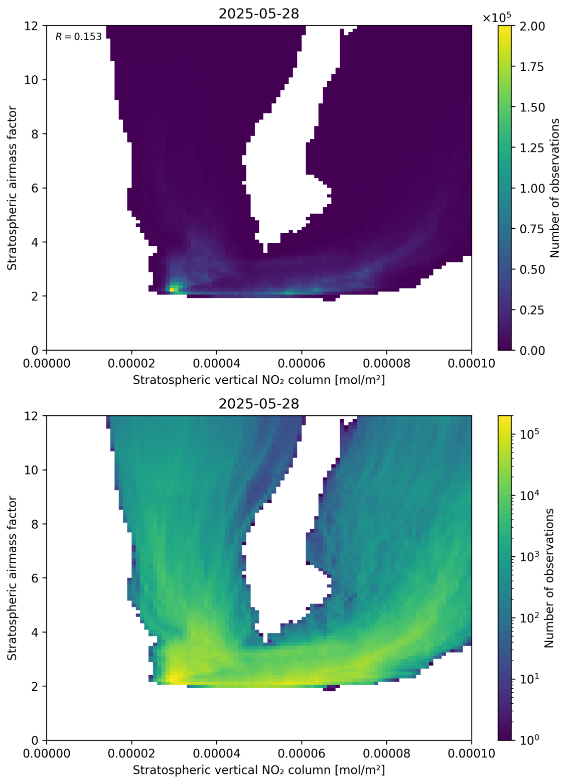
Figure 96: Scatter density plot of “Stratospheric vertical NO 2 column” against “Stratospheric airmass factor” for 2025-05-27 to 2025-05-29.
