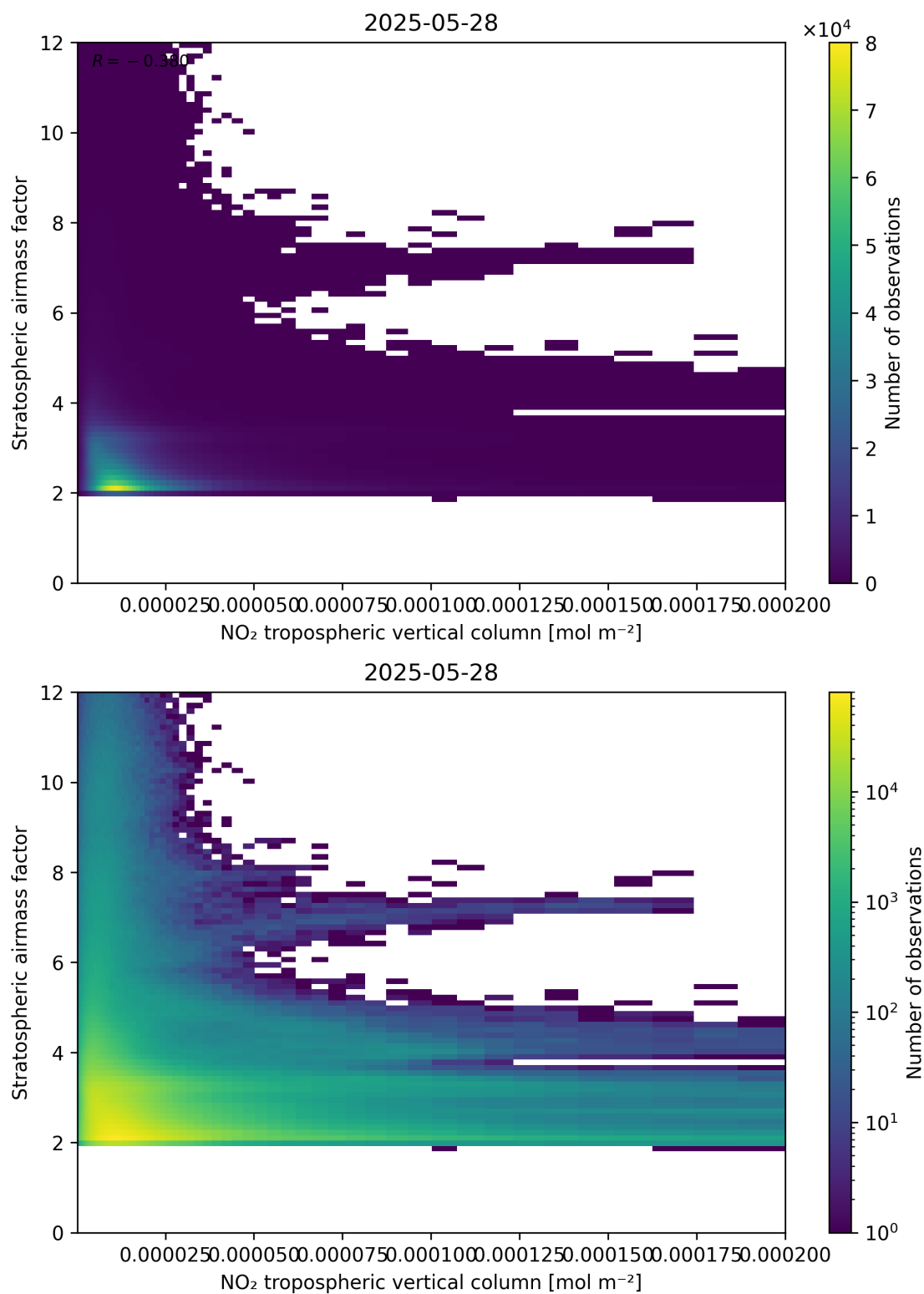
Figure 121: Scatter density plot of “NO 2 tropospheric vertical column” against “Stratospheric air mass factor” for 2025-05-27 to 2025-05-29.
