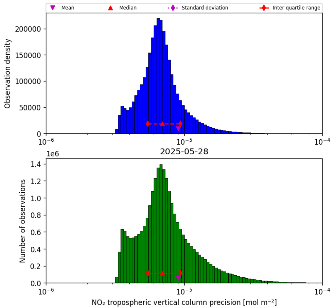
Figure 30: Histogram of “NO 2 tropospheric vertical column precision” for 2025-05-27 to 2025-05-29
