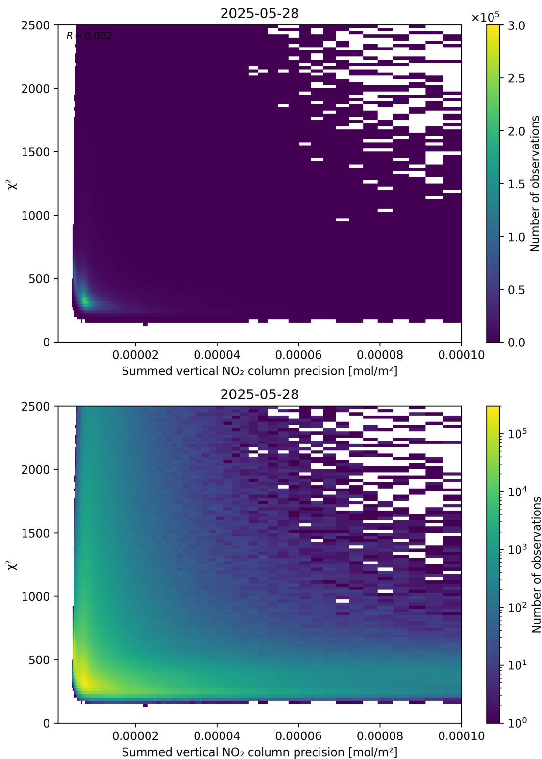
Figure 107: Scatter density plot of “Summed vertical NO 2 column precision” against “ \chi^2 ” for 2025-05-27 to 2025-05-29.
