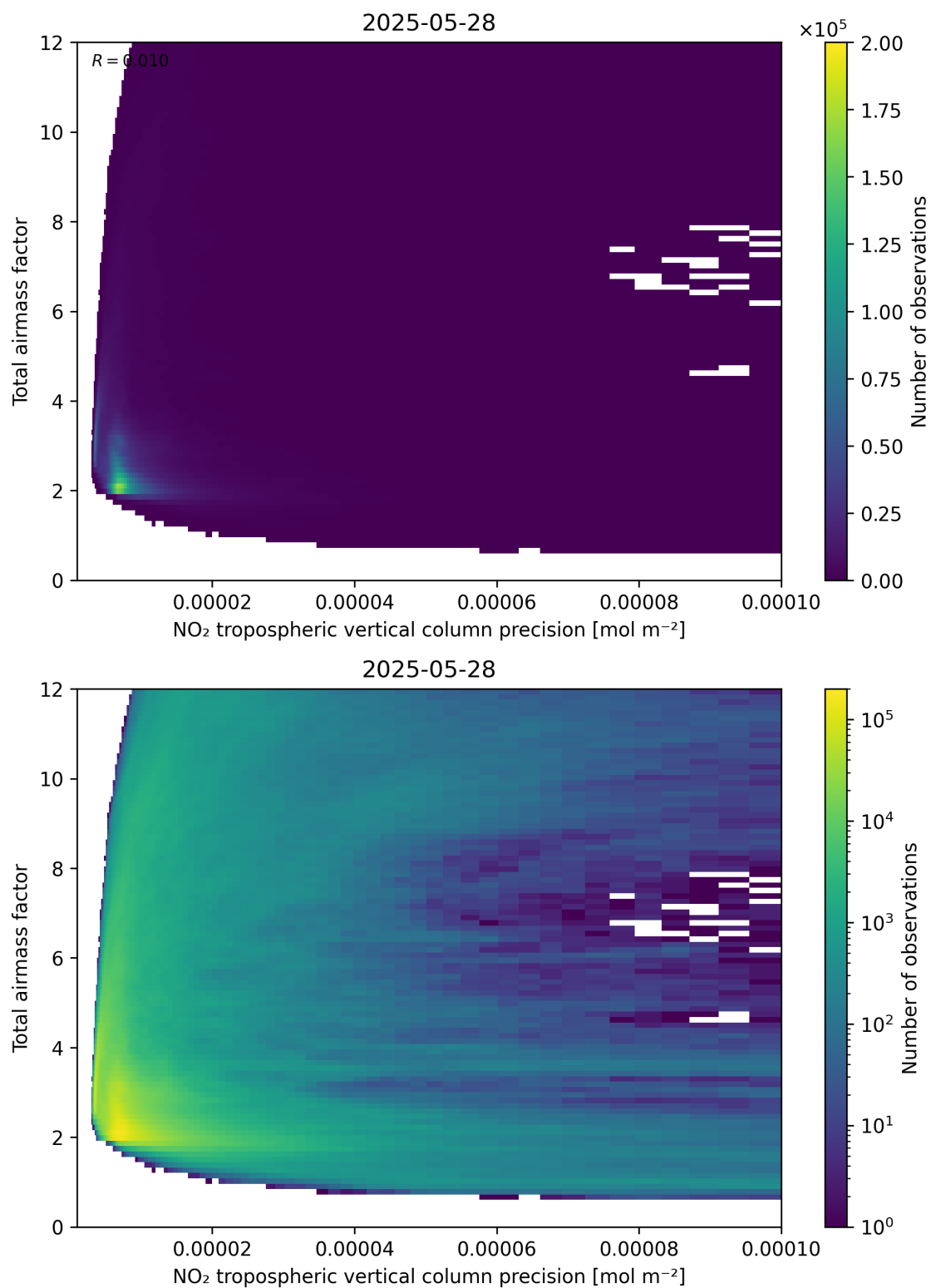
Figure 132: Scatter density plot of “NO 2 tropospheric vertical column precision” against “Total air mass factor” for 2025-05-27 to 2025-05-29.
