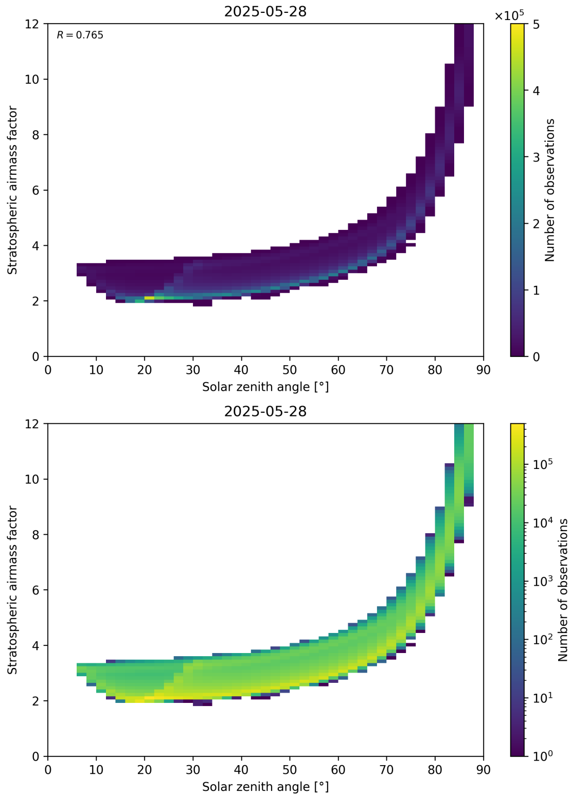
Figure 145: Scatter density plot of “Solar zenith angle” against “Stratospheric airmass factor” for 2025-05-27 to 2025-05-29.
