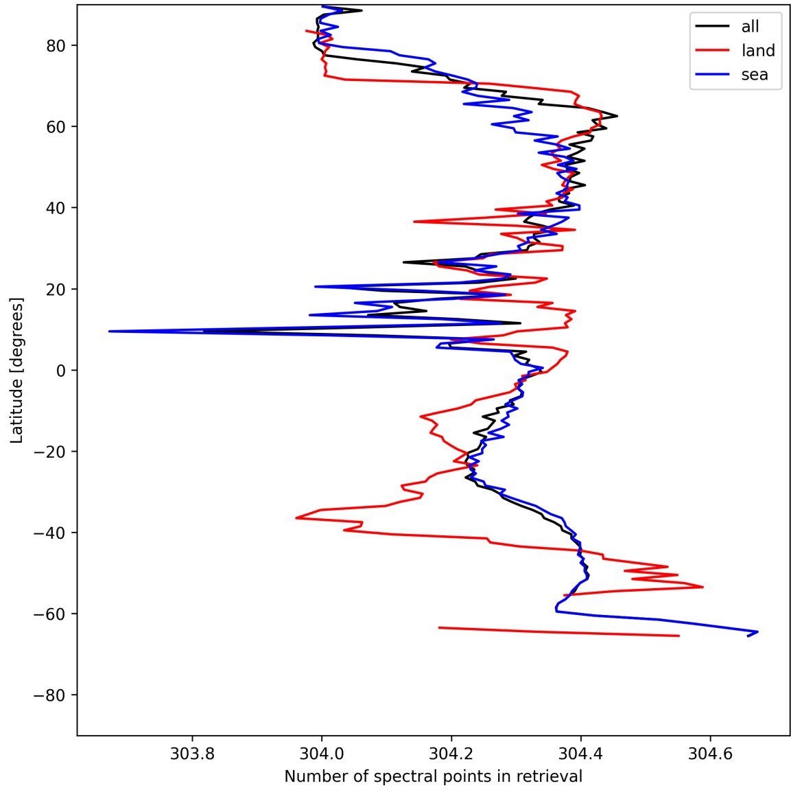
Figure 16: Zonal average of “Number of spectral points in retrieval” for 2025-05-27 to 2025-05-29.
