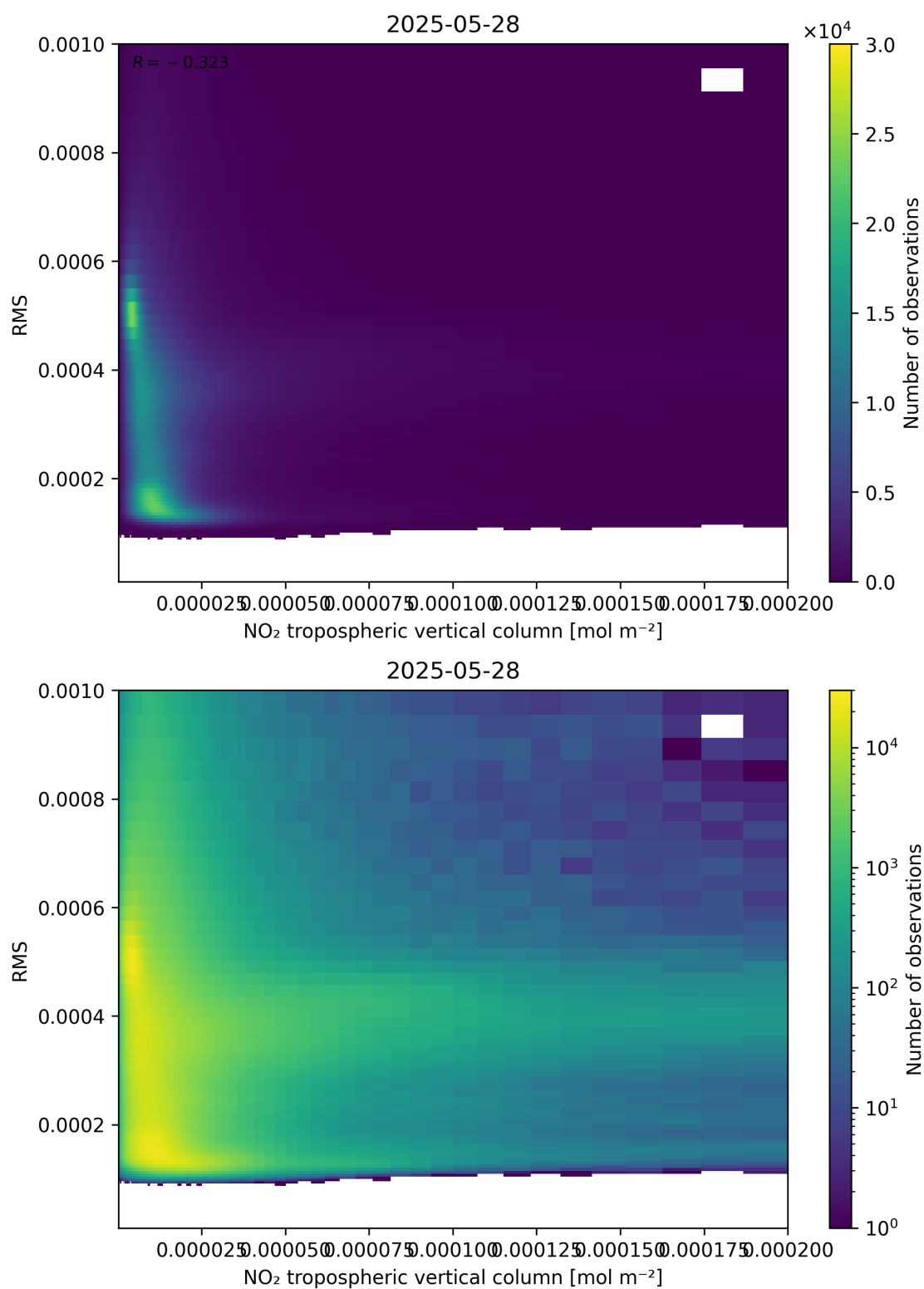
Figure 142: Scatter density plot of “NO 2 tropospheric vertical column” against “RMS” for 2025-05-27 to 2025-05-29.
