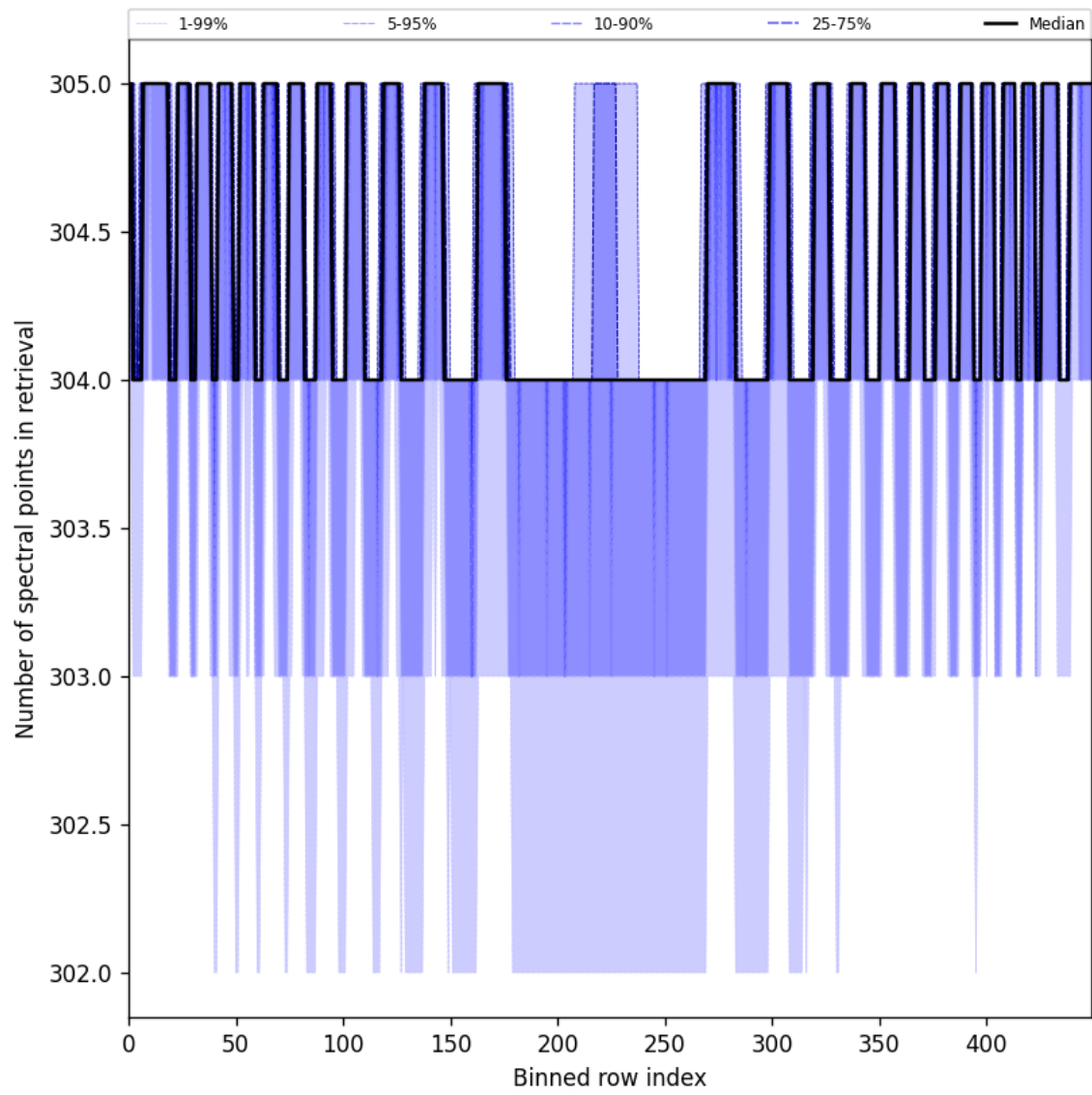
Figure 50: Along track statistics of “Number of spectral points in retrieval” for 2025-05-27 to 2025-05-29
