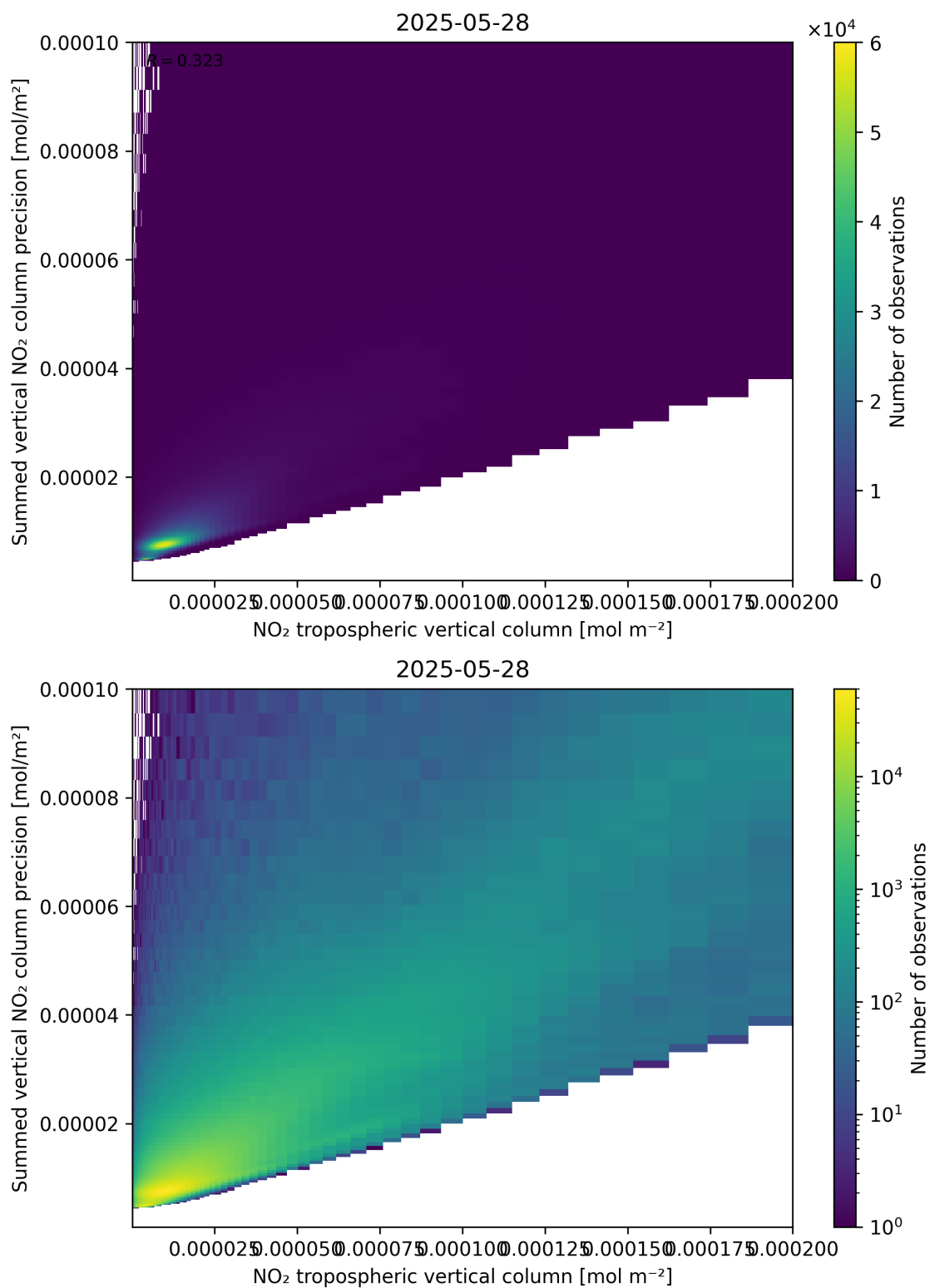
Figure 127: Scatter density plot of “NO 2 tropospheric vertical column” against “Summed vertical NO 2 column precision” for 2025-05-27 to 2025-05-29.
