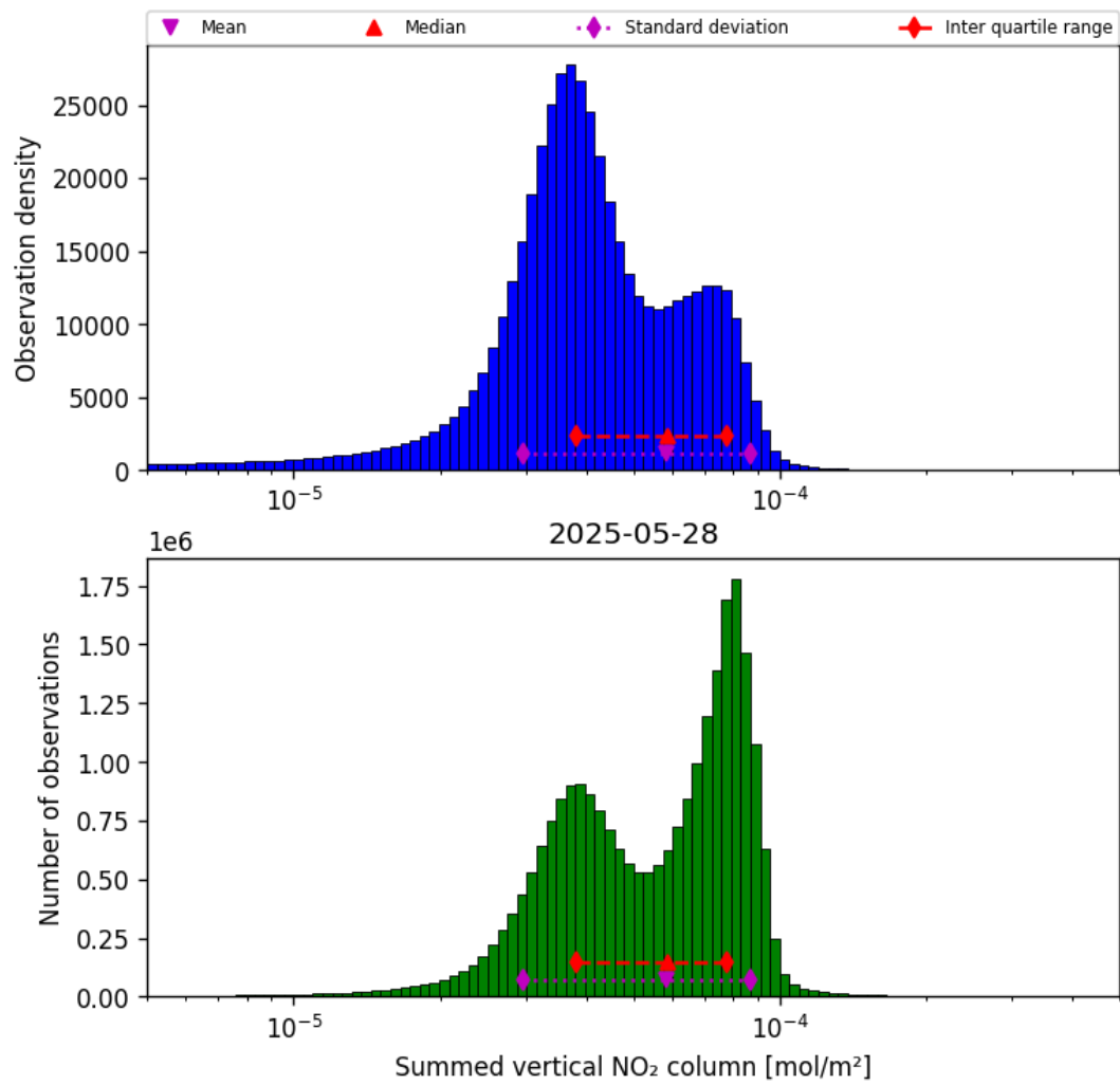
Figure 40: Histogram of “Summed vertical NO 2 column” for 2025-05-27 to 2025-05-29
