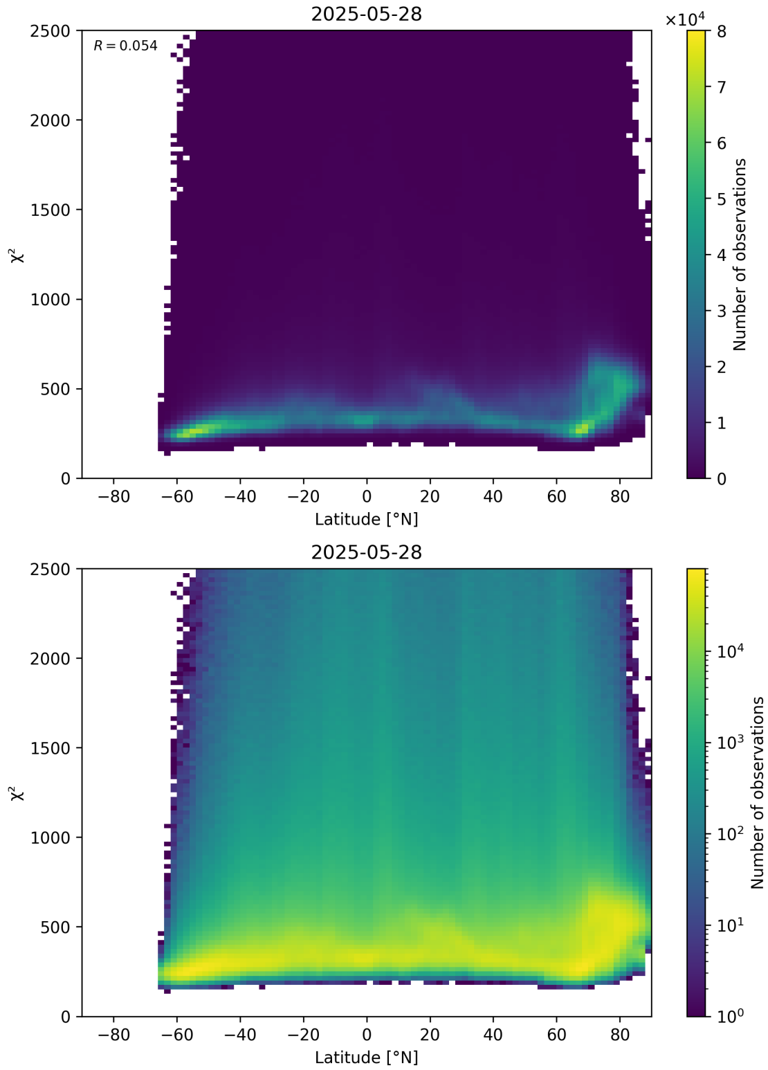
Figure 86: Scatter density plot of “Latitude” against “ \chi^2 ” for 2025-05-27 to 2025-05-29.
