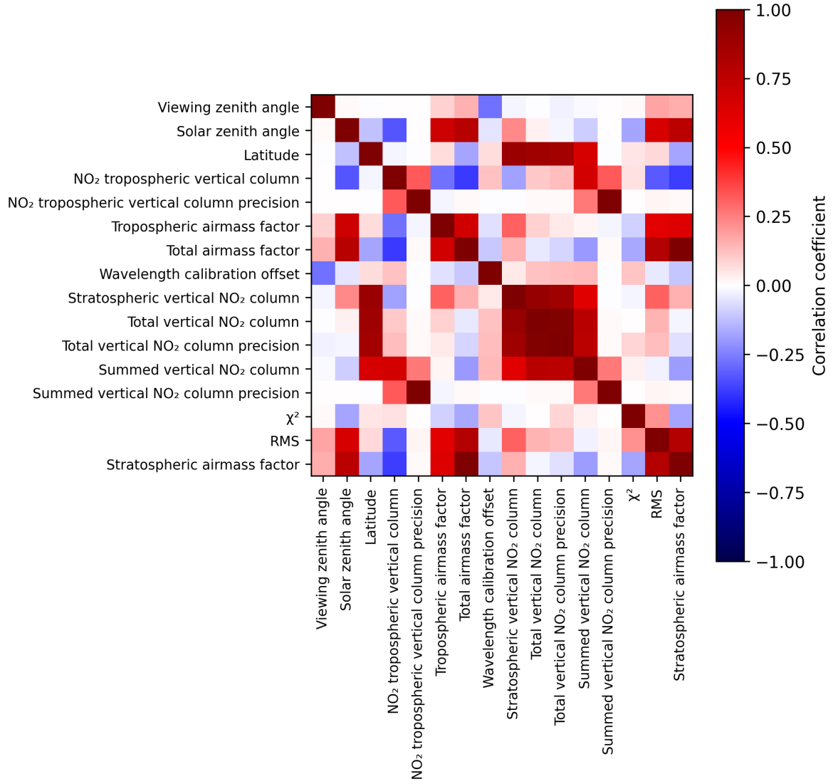
Figure 2: Map of correlation matrix for 2025-05-27 to 2025-05-29.
