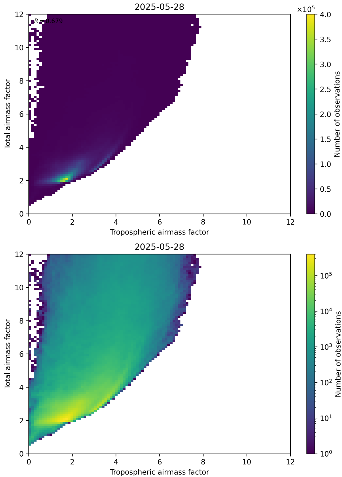
Figure 72: Scatter density plot of “Tropospheric airmass factor” against “Total airmass factor” for 2025-05-27 to 2025-05-29.
