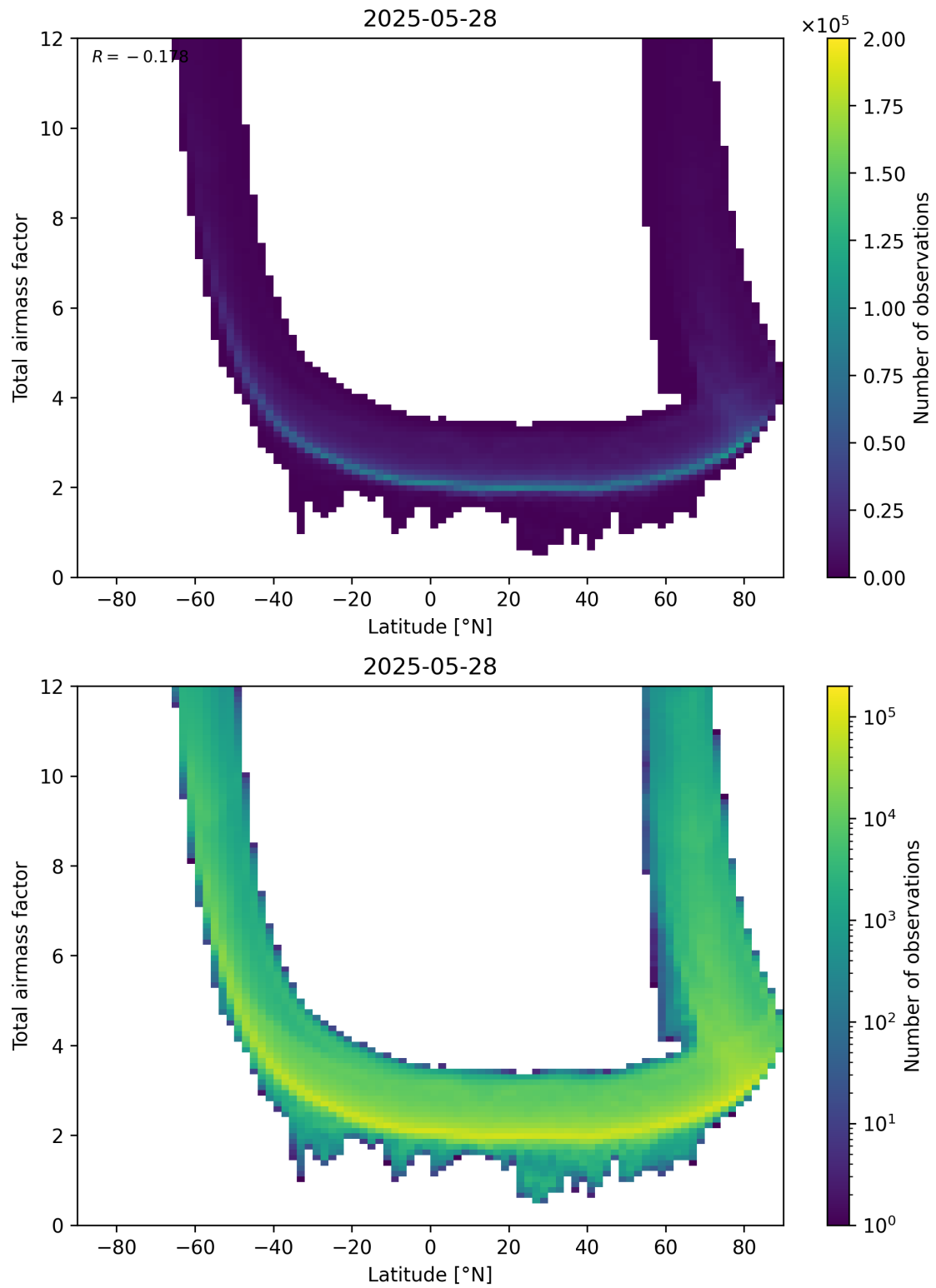
Figure 84: Scatter density plot of “Latitude” against “Total airmass factor” for 2025-05-27 to 2025-05-29.
