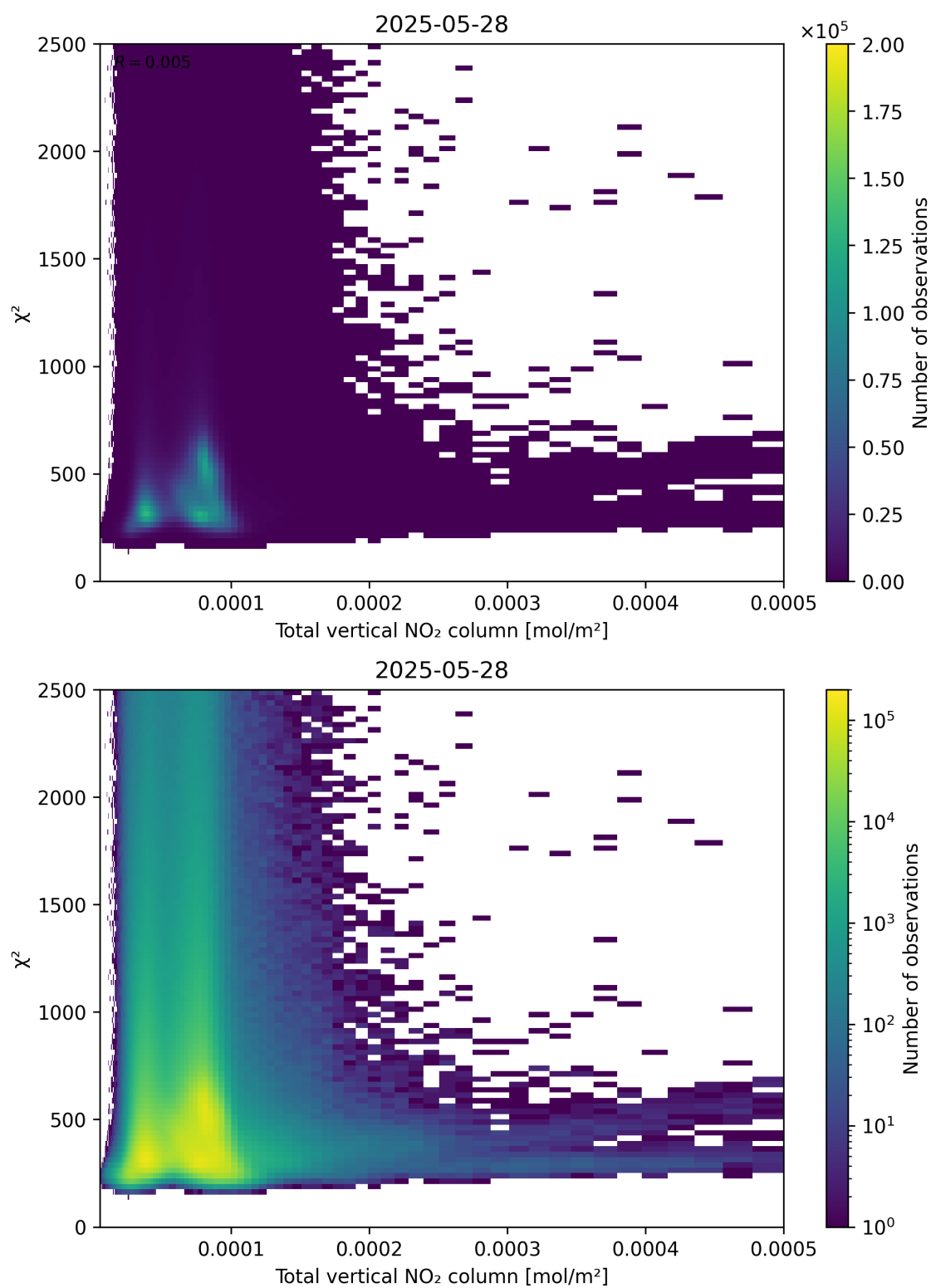
Figure 111: Scatter density plot of “Total vertical NO 2 column” against “ \chi^2 ” for 2025-05-27 to 2025-05-29.
