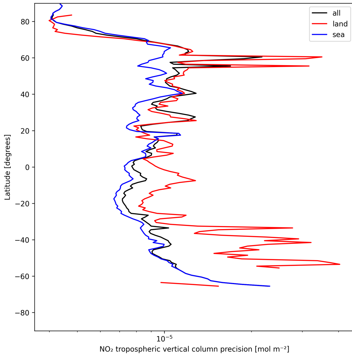
Figure 13: Zonal average of “NO 2 tropospheric vertical column precision” for 2025-05-27 to 2025-05-29.
