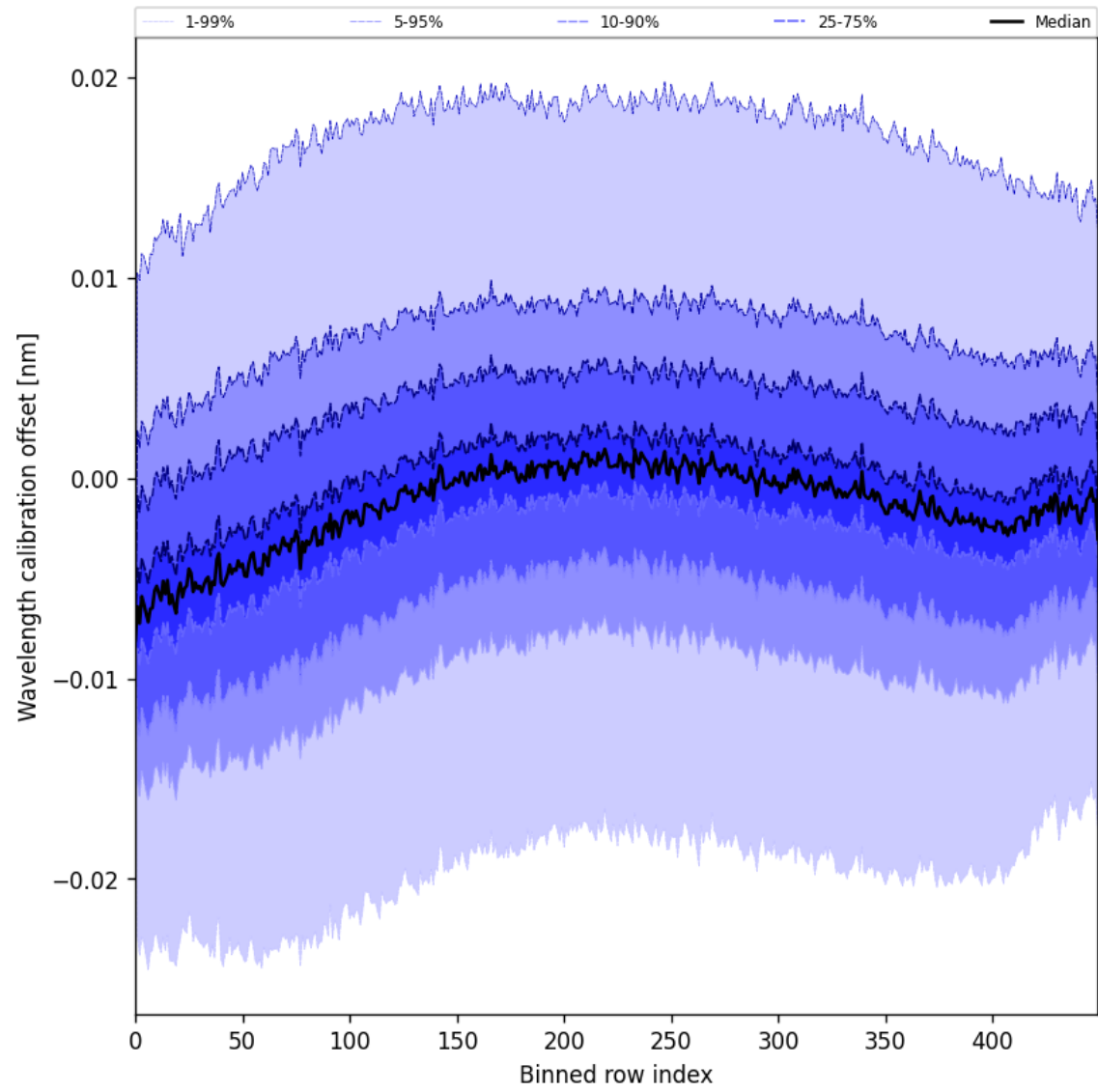
Figure 52: Along track statistics of “Wavelength calibration offset” for 2025-05-27 to 2025-05-29
