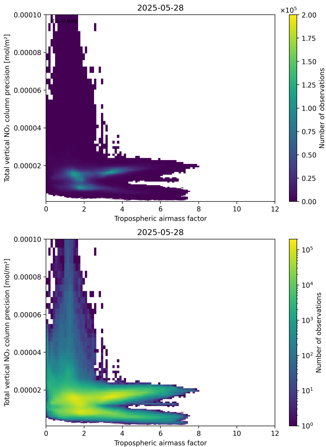
Figure 78: Scatter density plot of “Tropospheric air mass factor” against “Total vertical NO 2 column precision” for 2025-05-27 to 2025-05-29.
