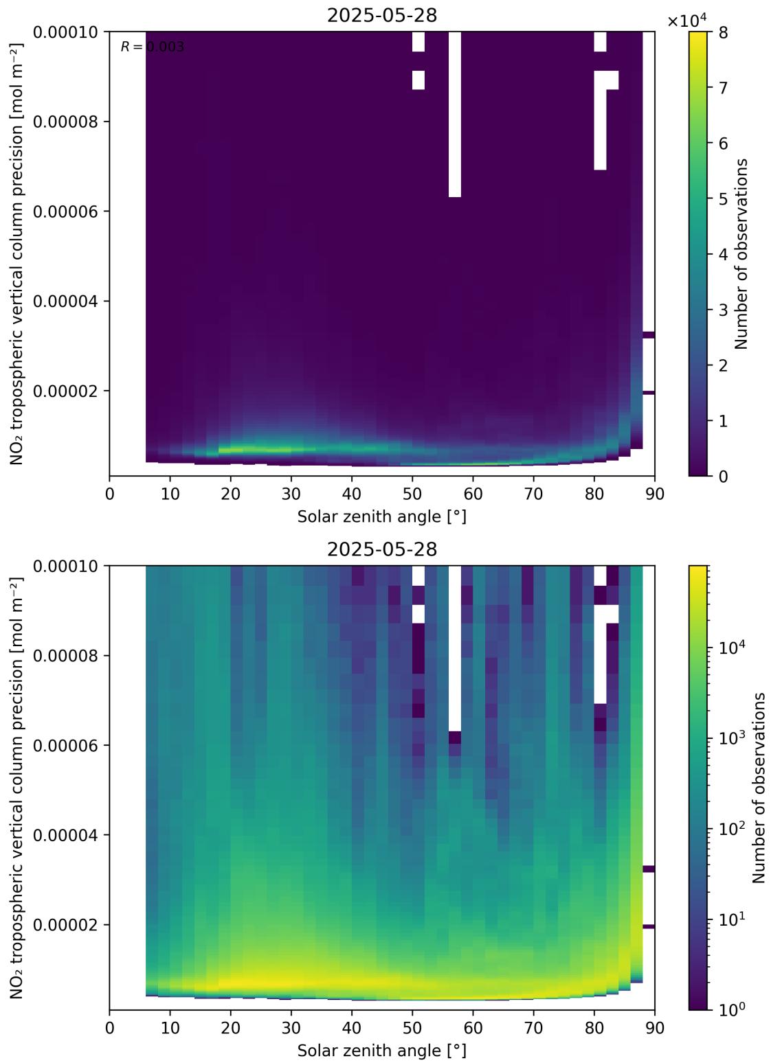
Figure 156: Scatter density plot of “Solar zenith angle” against “NO 2 tropospheric vertical column precision” for 2025-05-27 to 2025-05-29.
