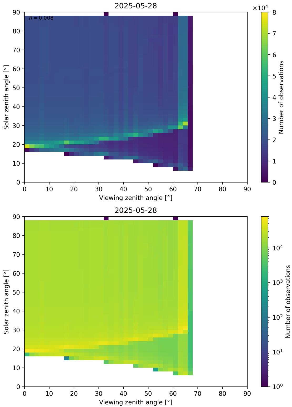
Figure 172: Scatter density plot of “Viewing zenith angle” against “Solar zenith angle” for 2025-05-27 to 2025-05-29.
