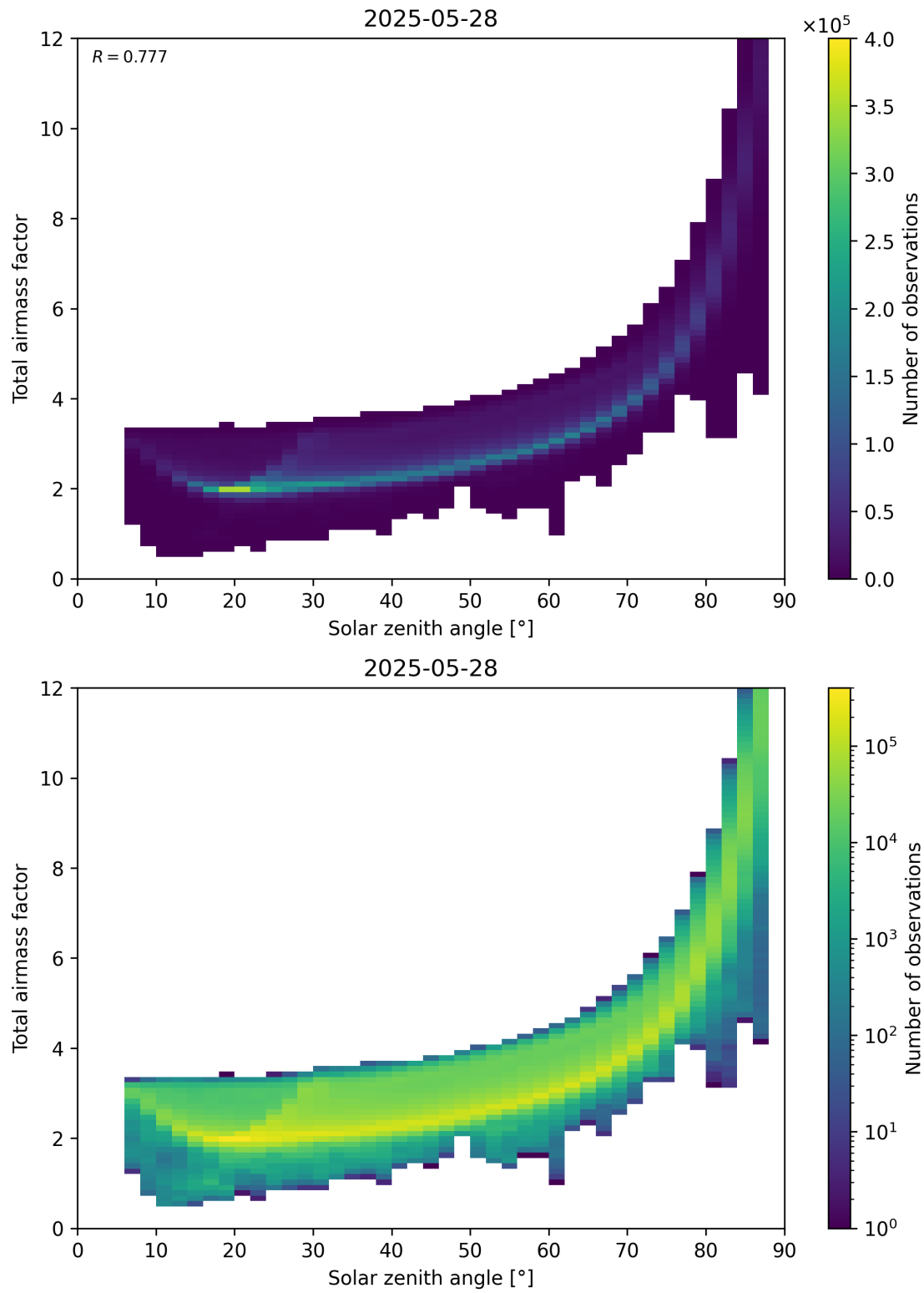
Figure 146: Scatter density plot of “Solar zenith angle” against “Total air mass factor” for 2025-05-27 to 2025-05-29.
