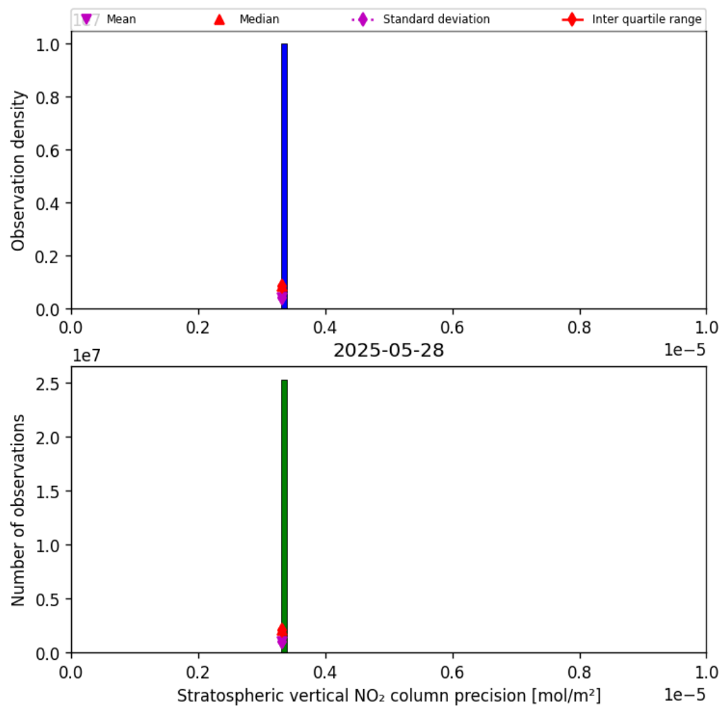
Figure 37: Histogram of “Stratospheric vertical NO 2 column precision” for 2025-05-27 to 2025-05-29
