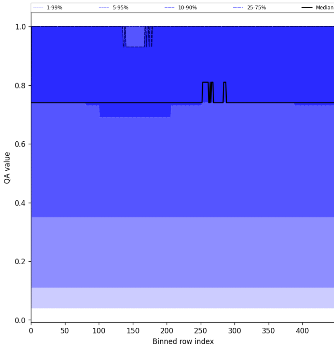
Figure 45: Along track statistics of “QA value” for 2025-05-27 to 2025-05-29
