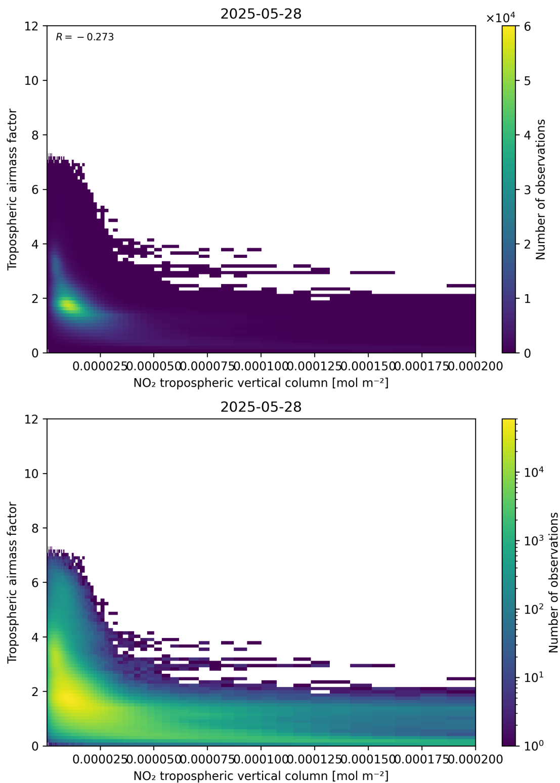
Figure 123: Scatter density plot of “NO 2 tropospheric vertical column” against “Tropospheric air mass factor” for 2025-05-27 to 2025-05-29.
