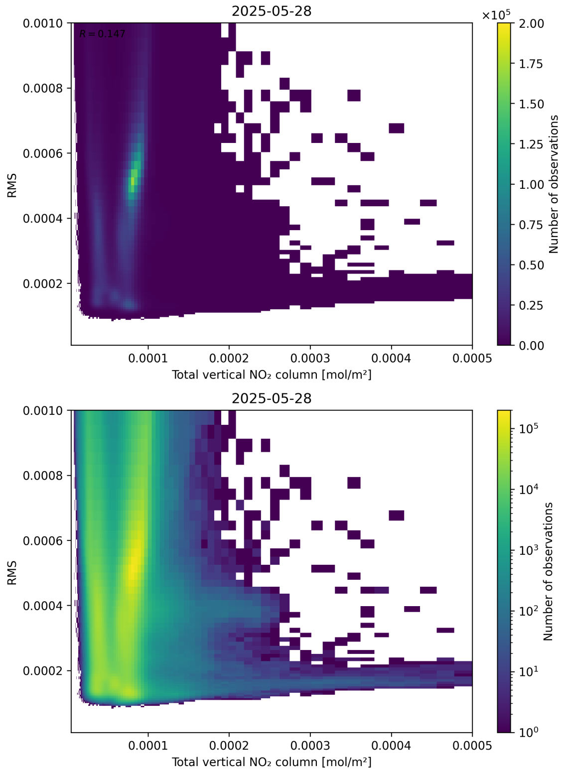
Figure 120: Scatter density plot of “Total vertical NO 2 column” against “RMS” for 2025-05-27 to 2025-05-29.
