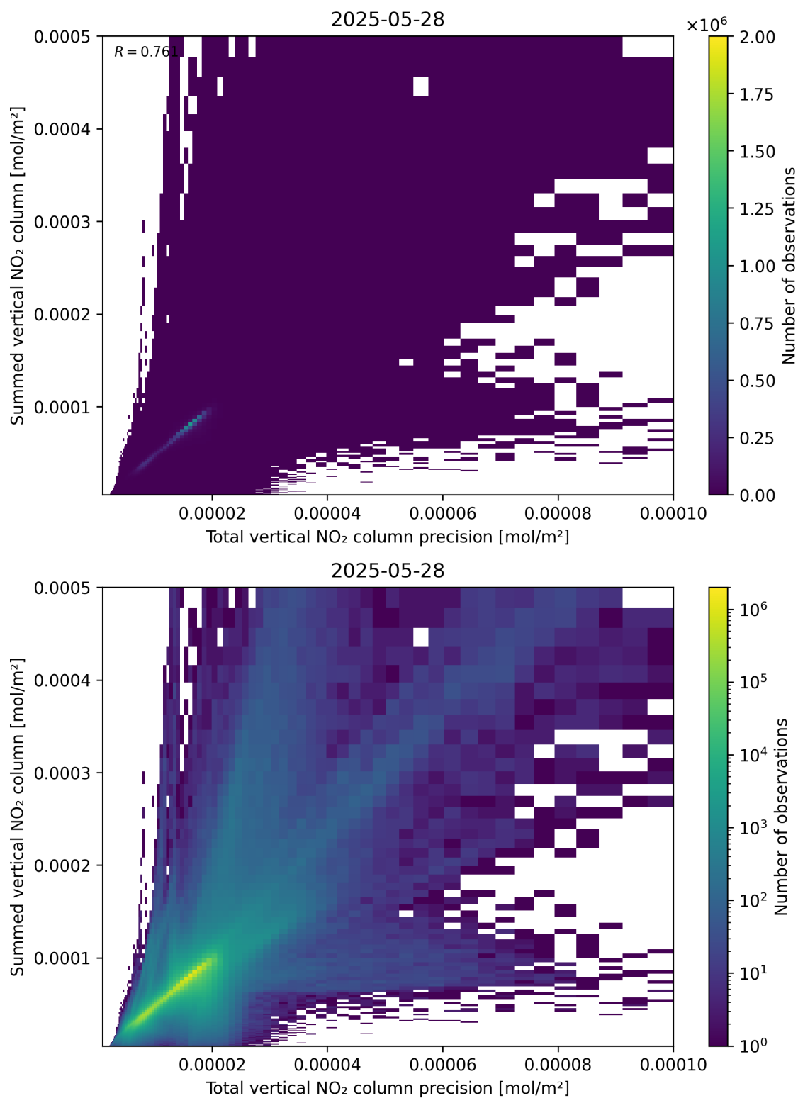
Figure 117: Scatter density plot of “Total vertical NO 2 column precision” against “Summed vertical NO 2 column” for 2025-05-27 to 2025-05-29.
