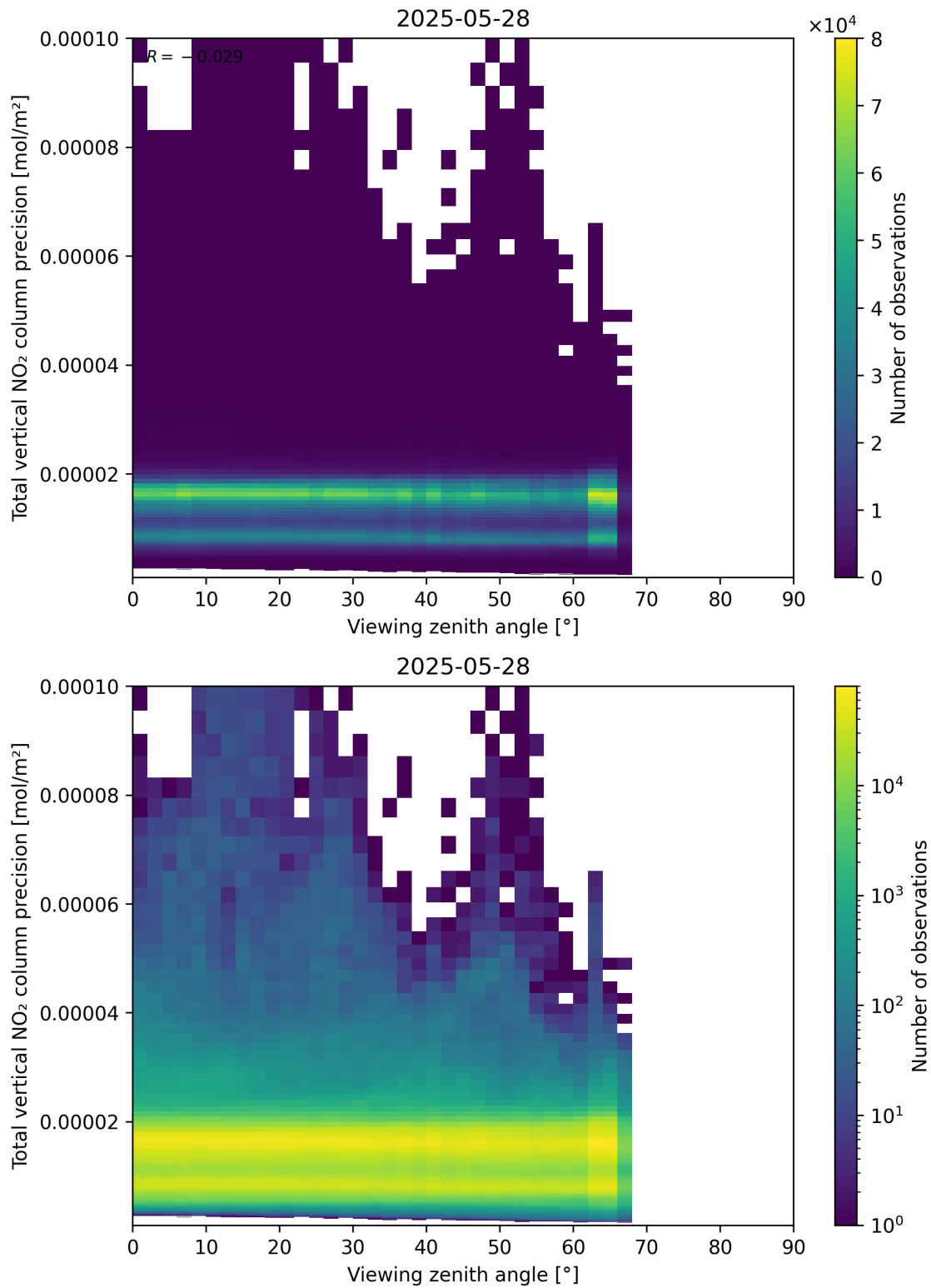
Figure 168: Scatter density plot of “Viewing zenith angle” against “Total vertical NO 2 column precision” for 2025-05-27 to 2025-05-29.
