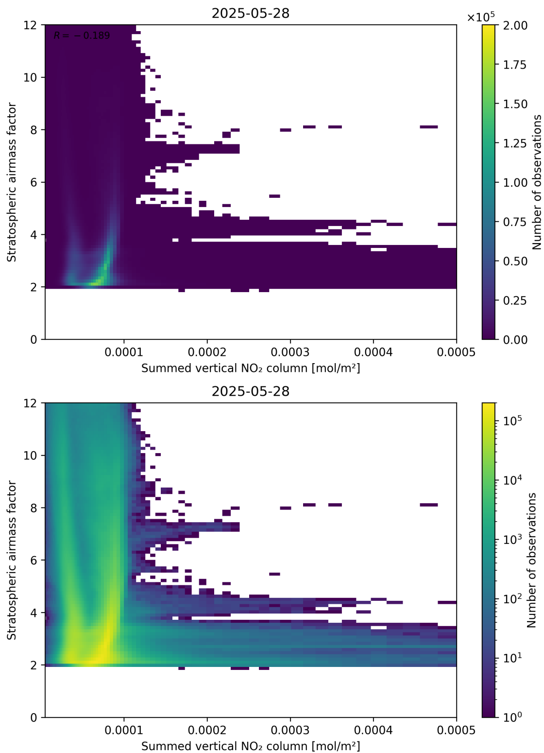
Figure 103: Scatter density plot of “Summed vertical NO 2 column” against “Stratospheric airmass factor” for 2025-05-27 to 2025-05-29.
