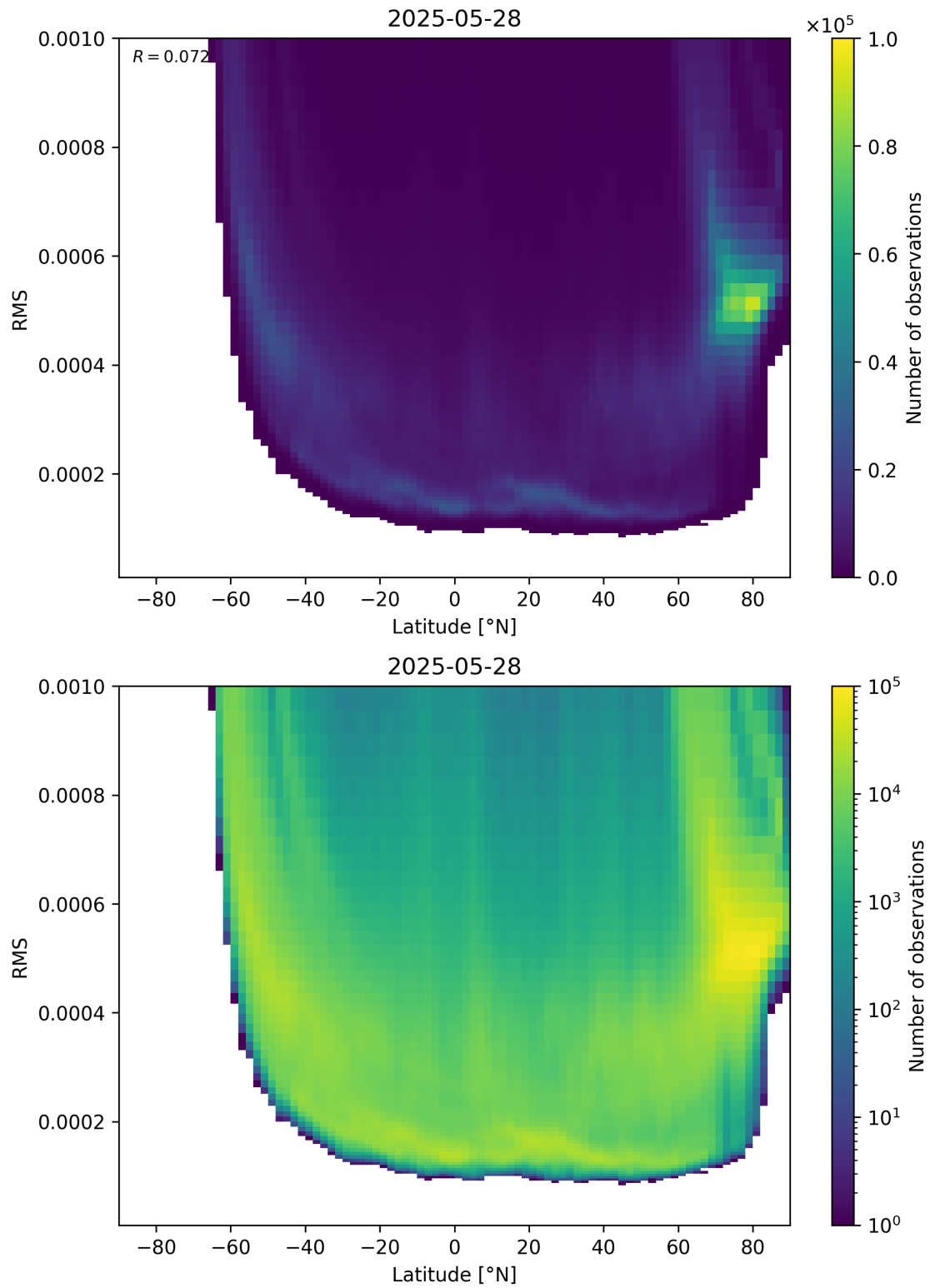
Figure 94: Scatter density plot of “Latitude” against “RMS” for 2025-05-27 to 2025-05-29.
