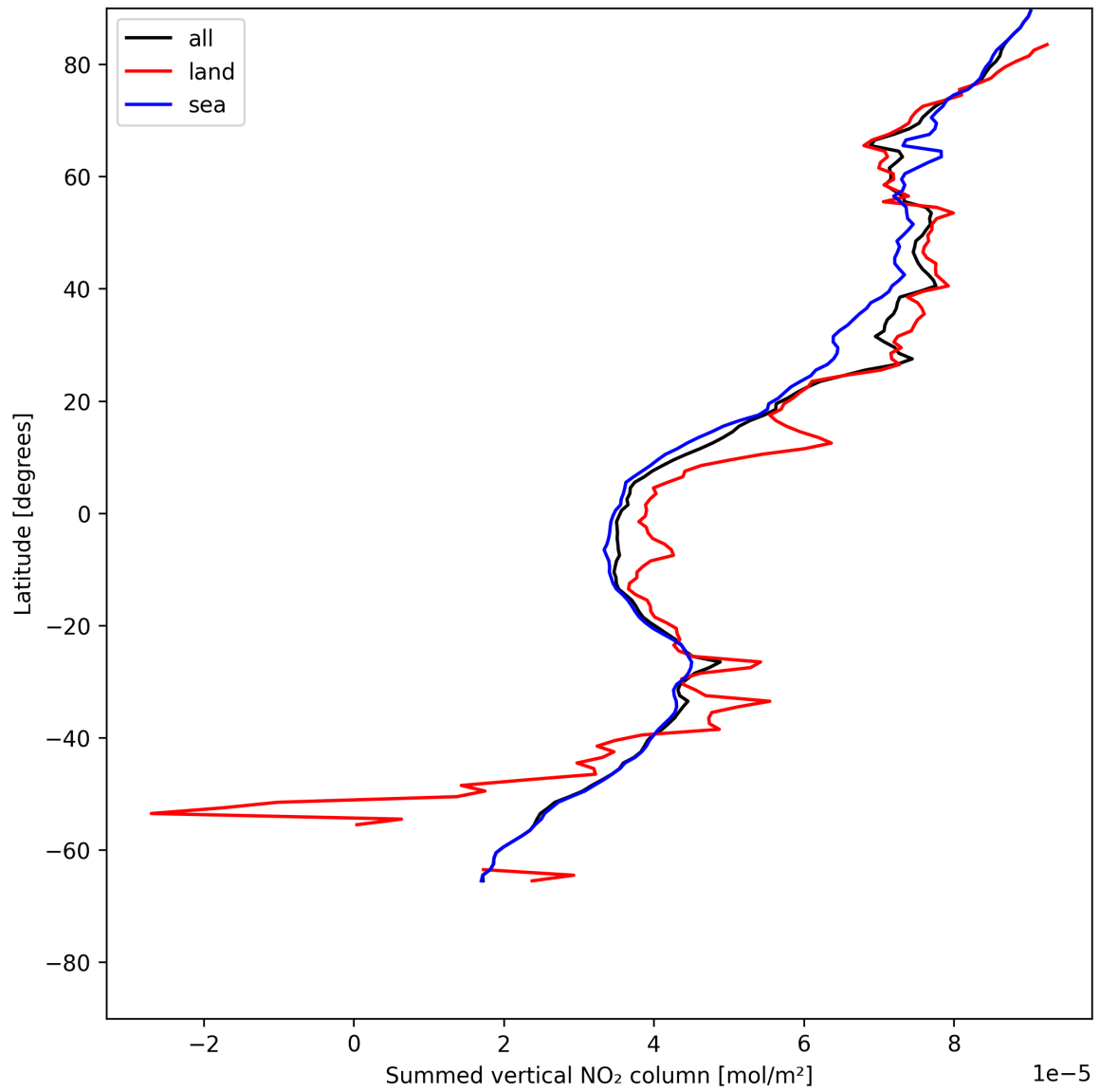
Figure 23: Zonal average of “Summed vertical NO 2 column” for 2025-05-27 to 2025-05-29.
