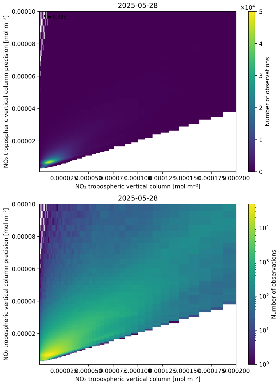
Figure 130: Scatter density plot of “NO 2 tropospheric vertical column” against “NO 2 tropospheric vertical column precision” for 2025-05-27 to 2025-05-29.
