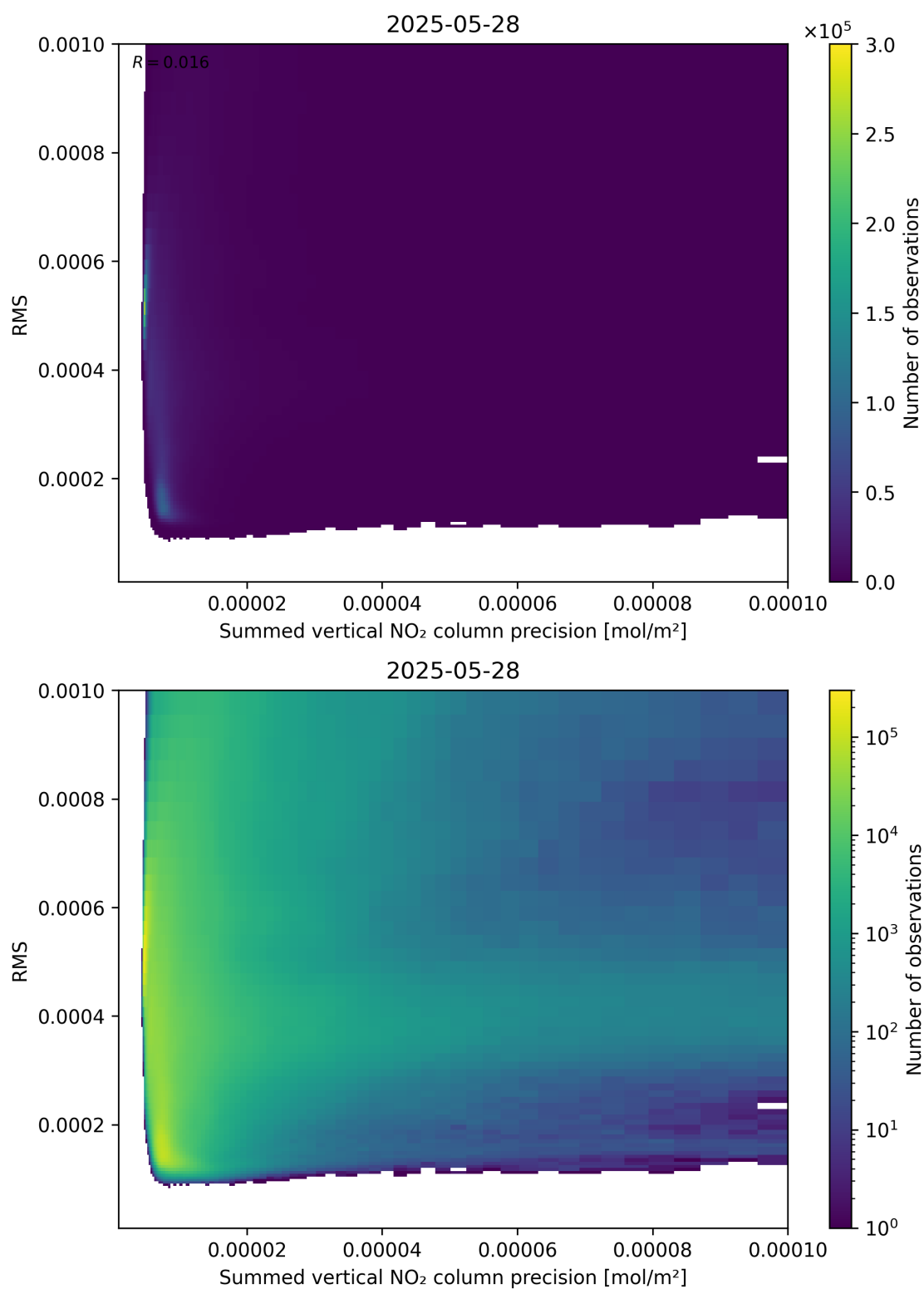
Figure 108: Scatter density plot of “Summed vertical NO 2 column precision” against “RMS” for 2025-05-27 to 2025-05-29.
