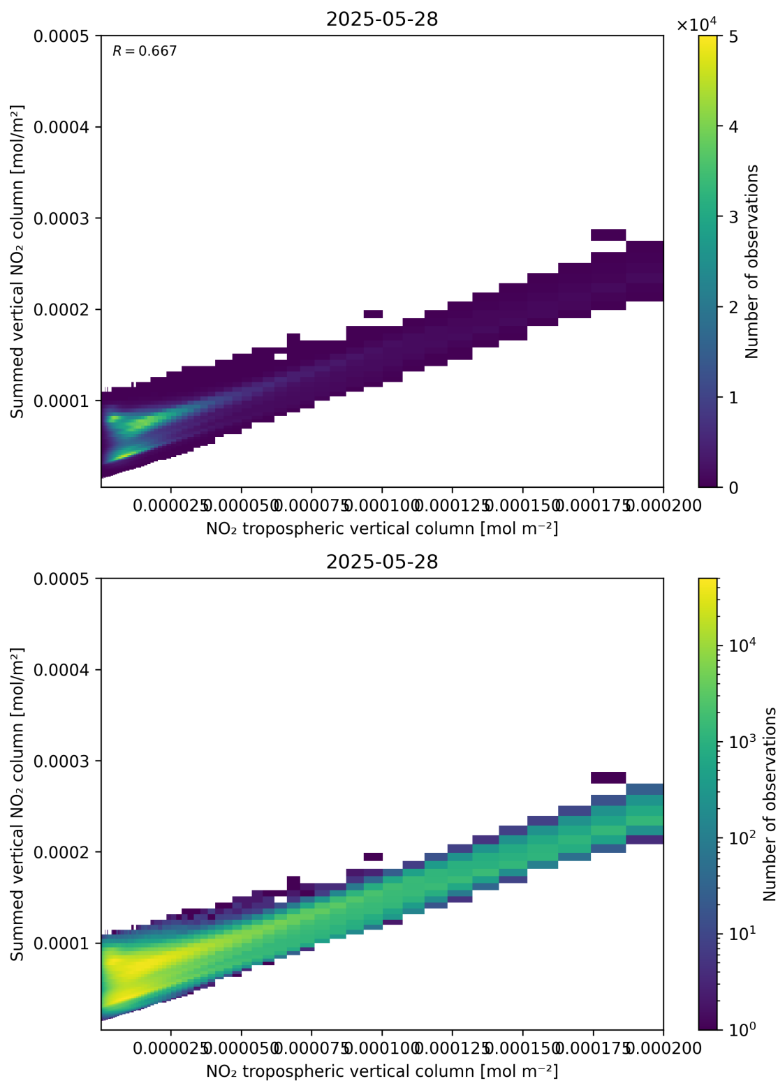
Figure 126: Scatter density plot of “NO 2 tropospheric vertical column” against “Summed vertical NO 2 column” for 2025-05-27 to 2025-05-29.
