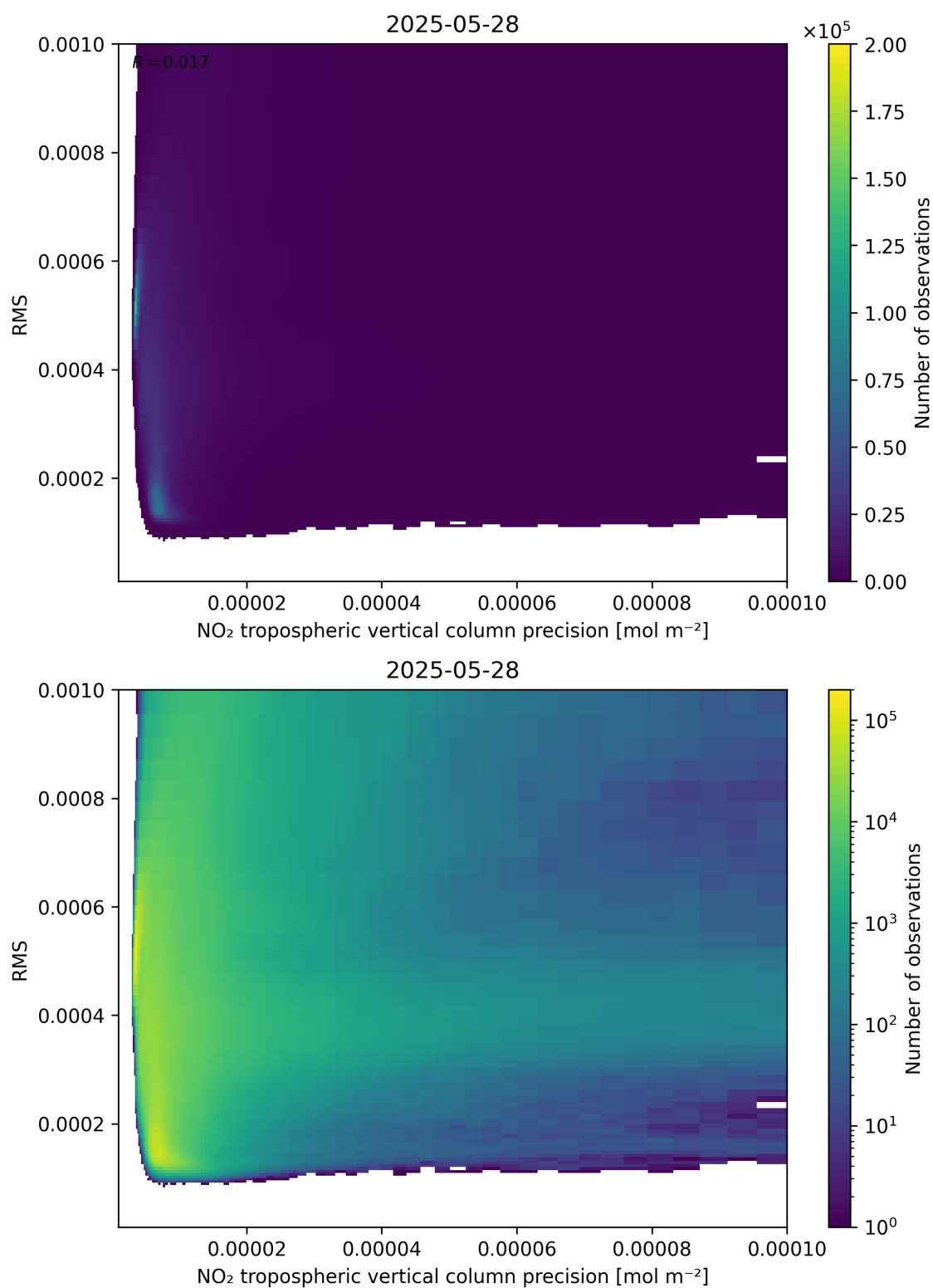
Figure 140: Scatter density plot of “NO 2 tropospheric vertical column precision” against “RMS” for 2025-05-27 to 2025-05-29.
