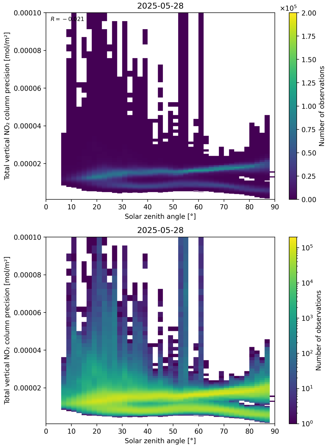
Figure 154: Scatter density plot of “Solar zenith angle” against “Total vertical NO 2 column precision” for 2025-05-27 to 2025-05-29.
