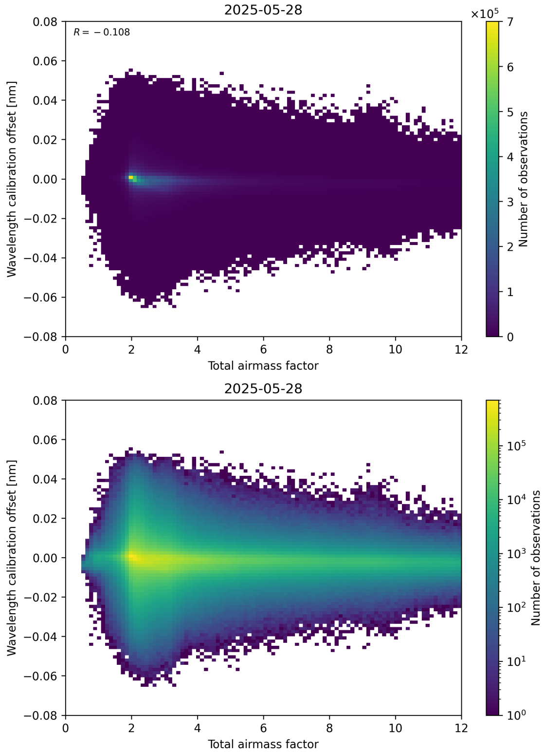
Figure 70: Scatter density plot of “Total airmass factor” against “Wavelength calibration offset” for 2025-05-27 to 2025-05-29.
