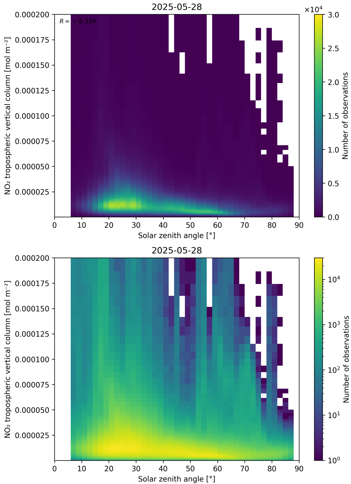
Figure 155: Scatter density plot of “Solar zenith angle” against “NO 2 tropospheric vertical column” for 2025-05-27 to 2025-05-29.
