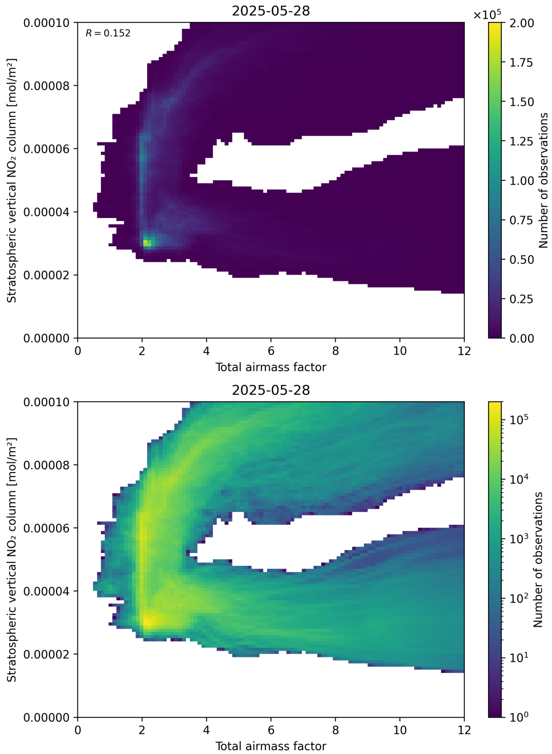
Figure 64: Scatter density plot of “Total airmass factor” against “Stratospheric vertical \text{NO}_2 column” for 2025-05-27 to 2025-05-29.
