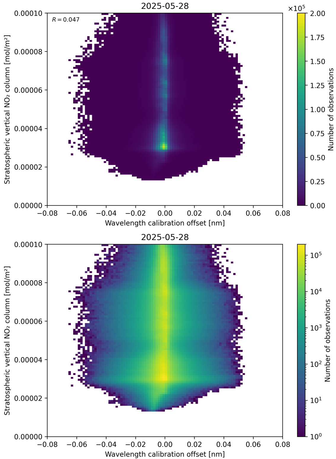
Figure 176: Scatter density plot of “Wavelength calibration offset” against “Stratospheric vertical NO 2 column” for 2025-05-27 to 2025-05-29.
