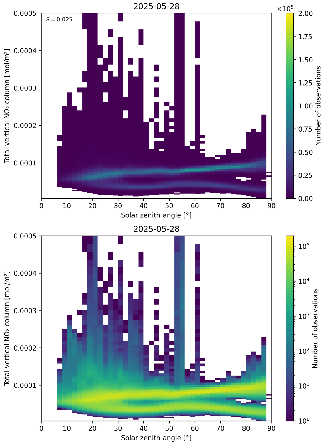
Figure 153: Scatter density plot of “Solar zenith angle” against “Total vertical NO 2 column” for 2025-05-27 to 2025-05-29.
