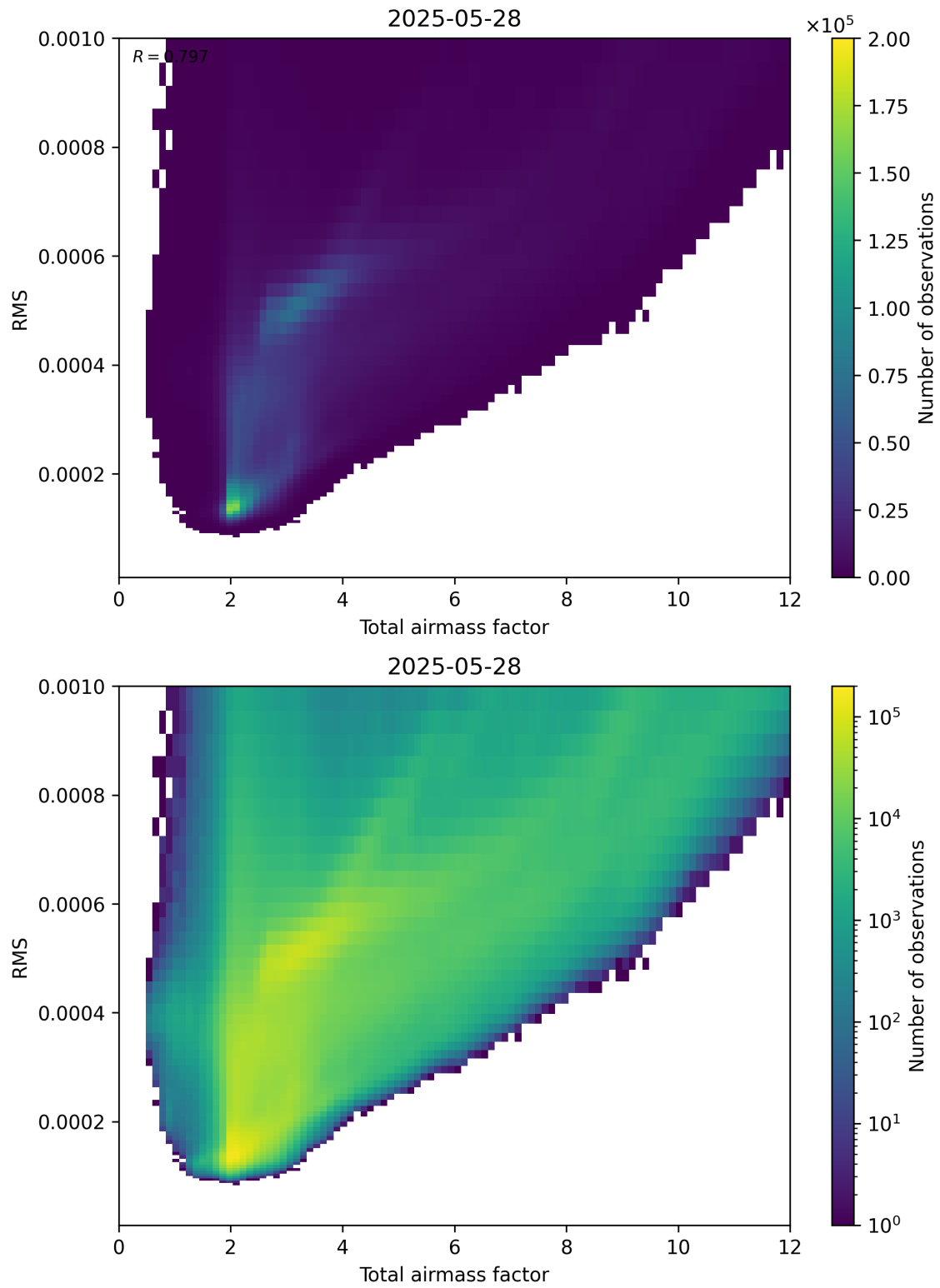
Figure 69: Scatter density plot of “Total airmass factor” against “RMS” for 2025-05-27 to 2025-05-29.
