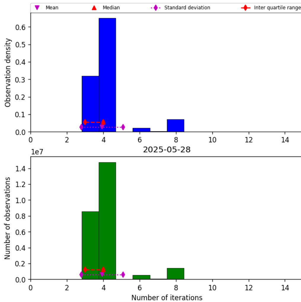
Figure 34: Histogram of “Number of iterations” for 2025-05-27 to 2025-05-29
