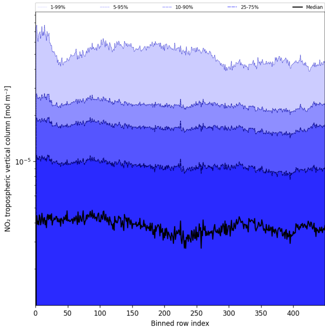
Figure 46: Along track statistics of “NO 2 tropospheric vertical column” for 2025-05-27 to 2025-05-29
