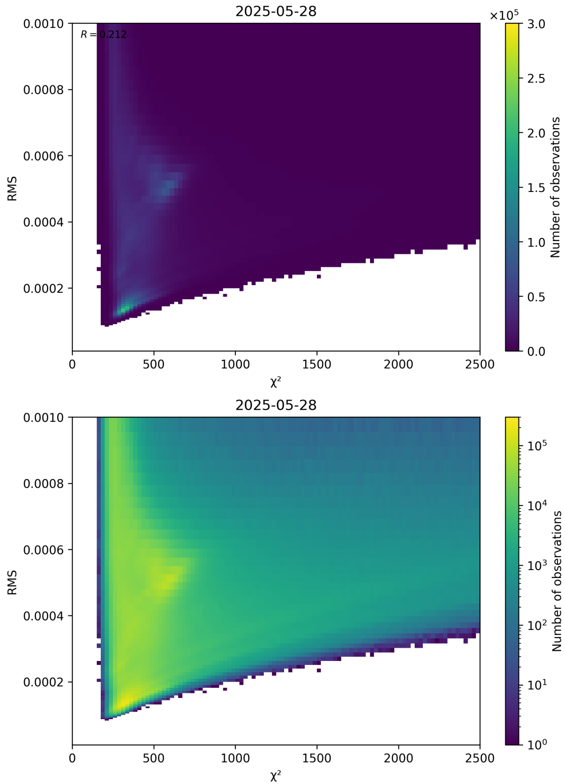
Figure 82: Scatter density plot of “ \chi^2 ” against “RMS” for 2025-05-27 to 2025-05-29.
