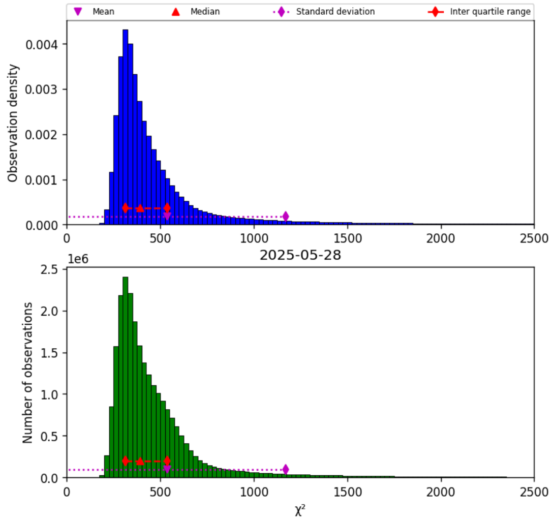
Figure 42: Histogram of “ \chi^2 ” for 2025-05-27 to 2025-05-29
