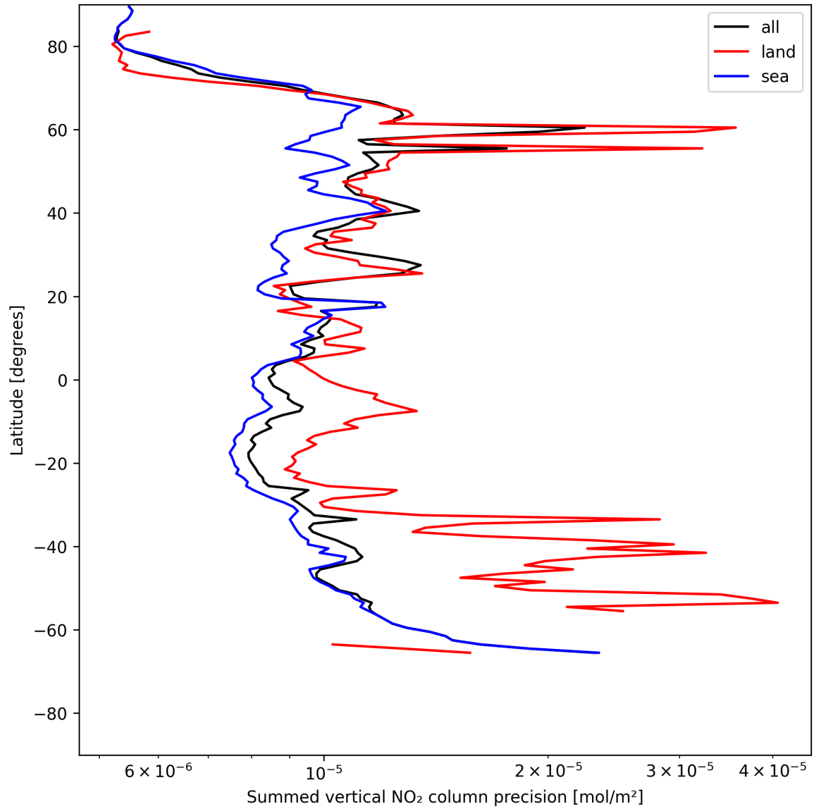
Figure 24: Zonal average of “Summed vertical NO 2 column precision” for 2025-05-27 to 2025-05-29.
