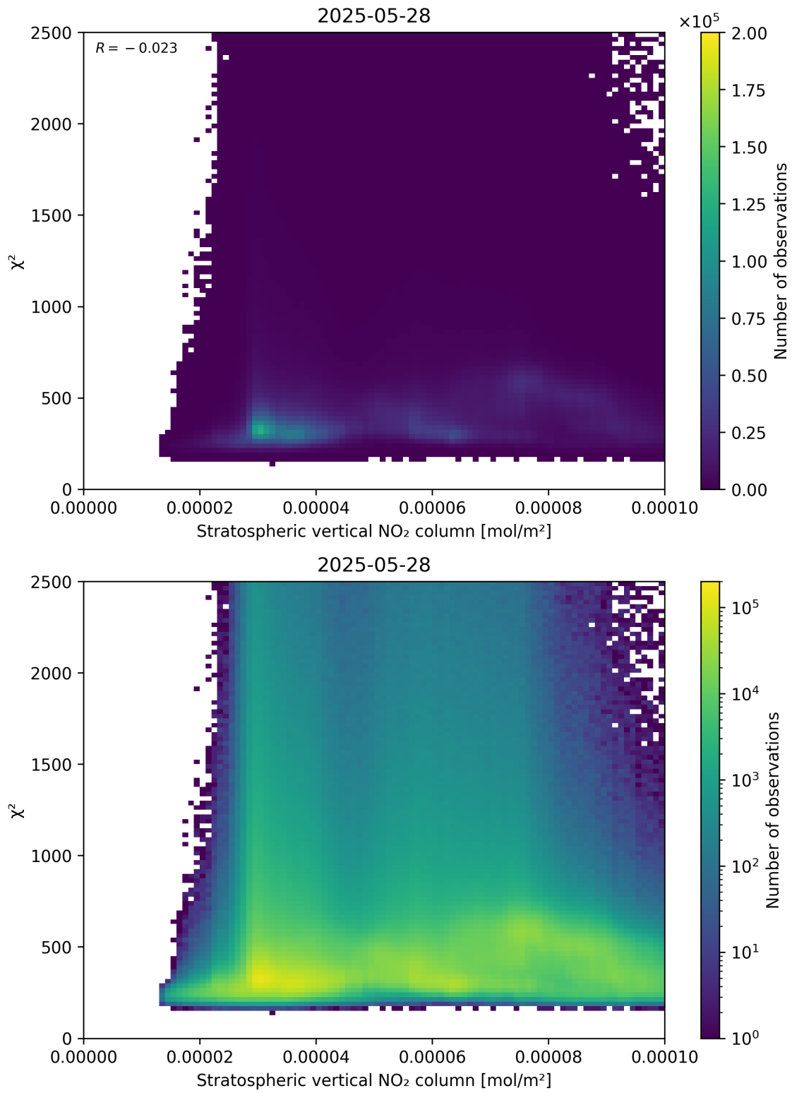
Figure 97: Scatter density plot of “Stratospheric vertical NO 2 column” against “ \chi^2 ” for 2025-05-27 to 2025-05-29.
