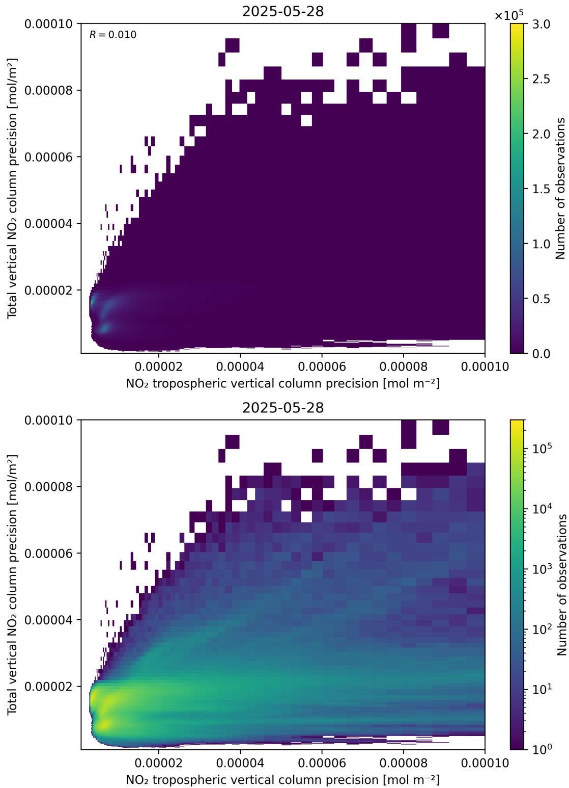
Figure 139: Scatter density plot of “NO 2 tropospheric vertical column precision” against “Total vertical NO 2 column precision” for 2025-05-27 to 2025-05-29.
