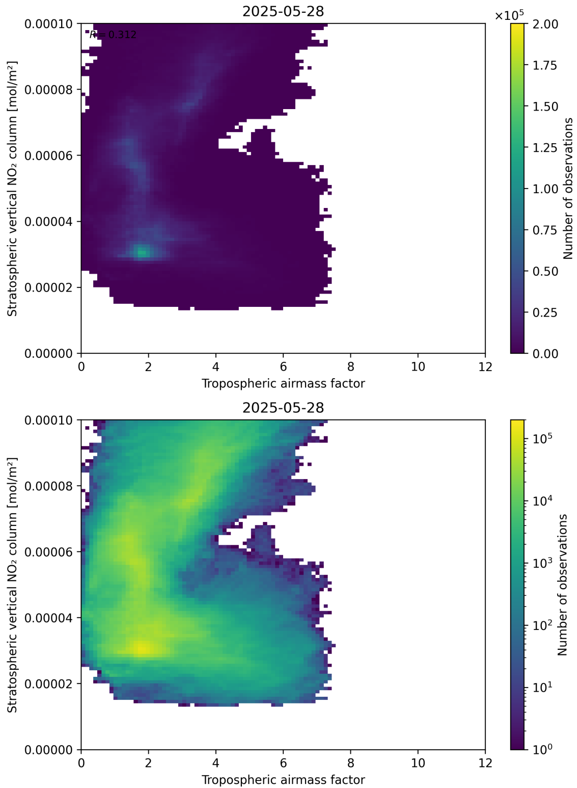
Figure 74: Scatter density plot of “Tropospheric airmass factor” against “Stratospheric vertical NO 2 column” for 2025-05-27 to 2025-05-29.
