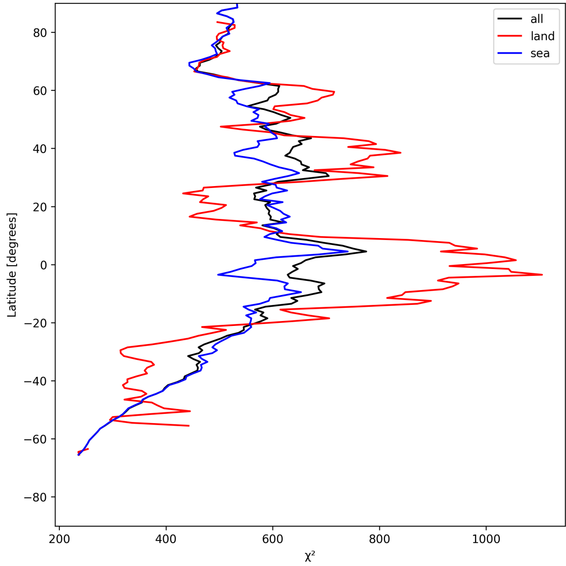
Figure 25: Zonal average of “ \chi^2 ” for 2025-05-27 to 2025-05-29.
