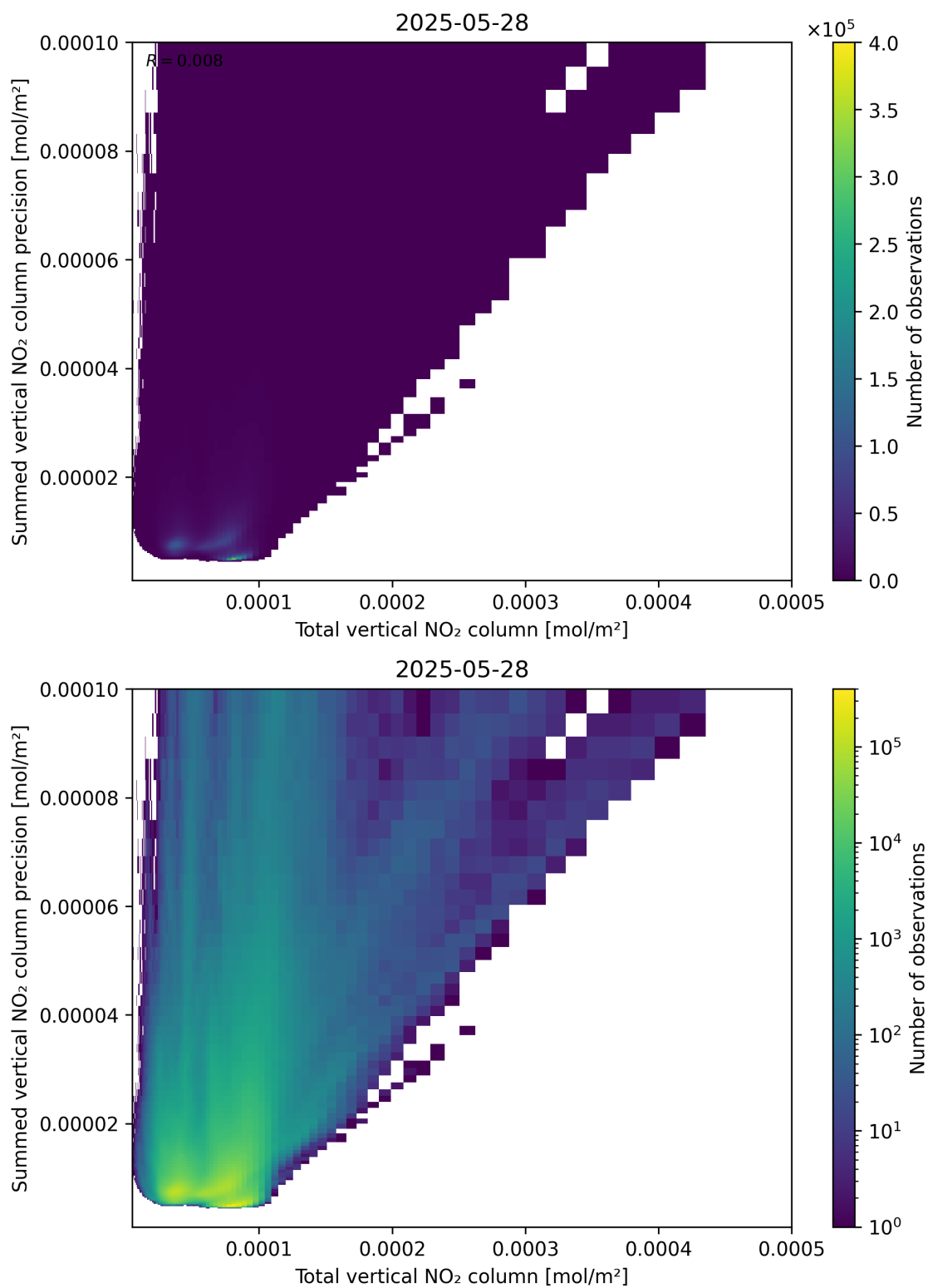
Figure 113: Scatter density plot of “Total vertical NO 2 column” against “Summed vertical NO 2 column precision” for 2025-05-27 to 2025-05-29.
