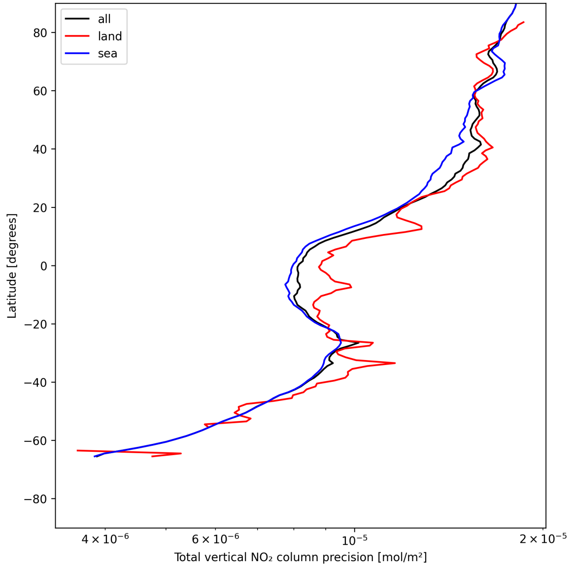
Figure 22: Zonal average of “Total vertical NO 2 column precision” for 2025-05-27 to 2025-05-29.
