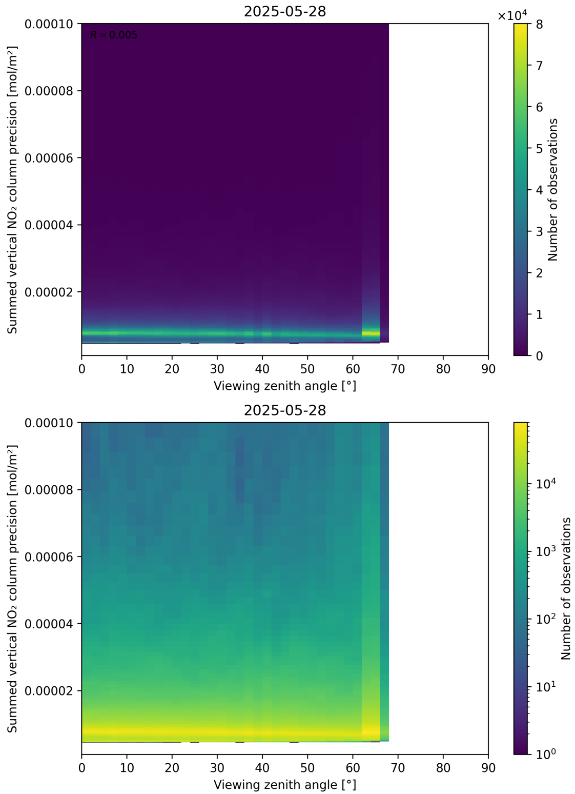
Figure 166: Scatter density plot of “Viewing zenith angle” against “Summed vertical NO 2 column precision” for 2025-05-27 to 2025-05-29.
