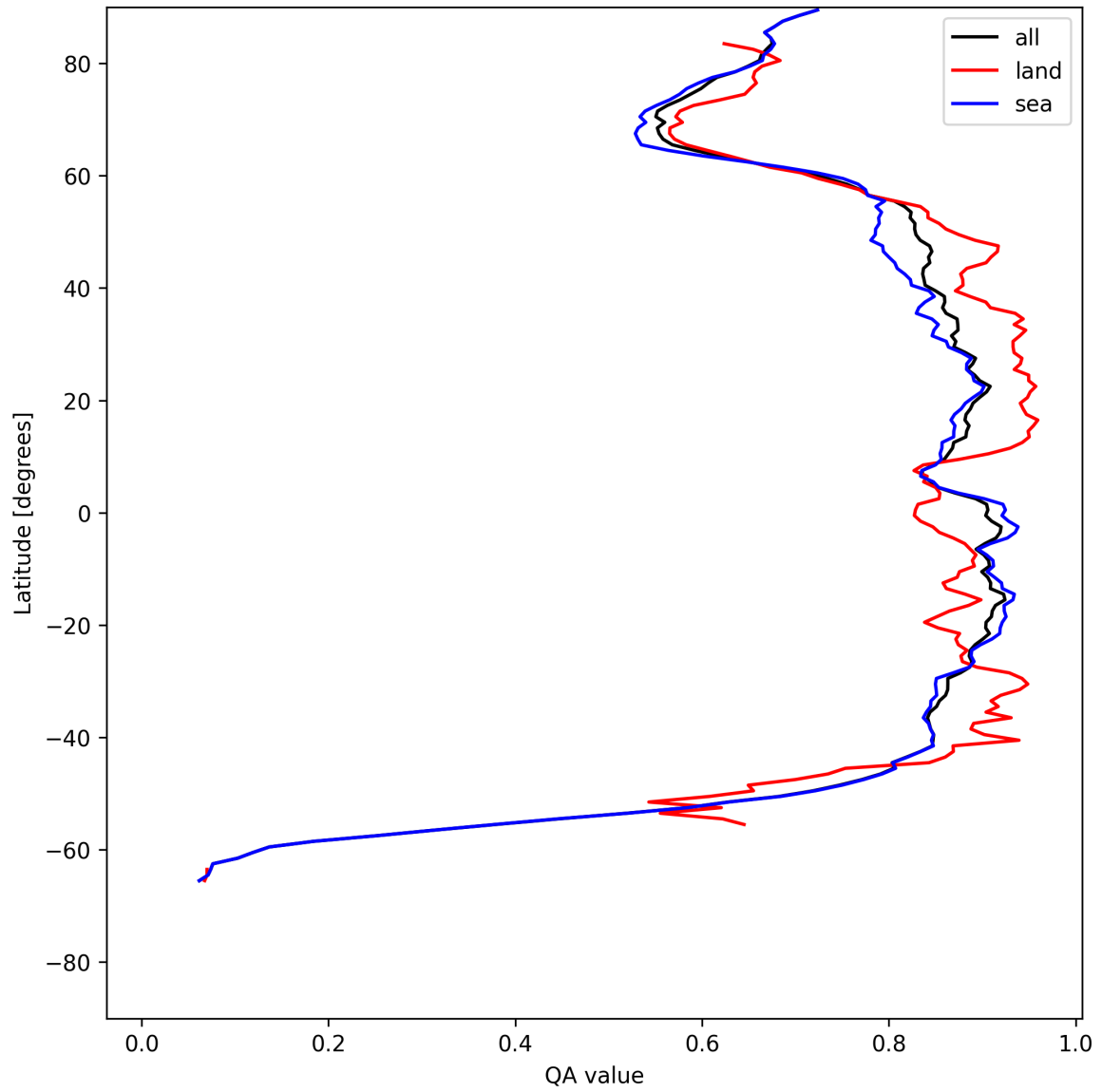
Figure 11: Zonal average of “QA value” for 2025-05-27 to 2025-05-29.
