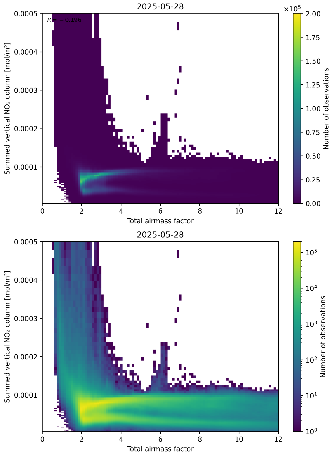
Figure 65: Scatter density plot of “Total airmass factor” against “Summed vertical NO 2 column” for 2025-05-27 to 2025-05-29.
