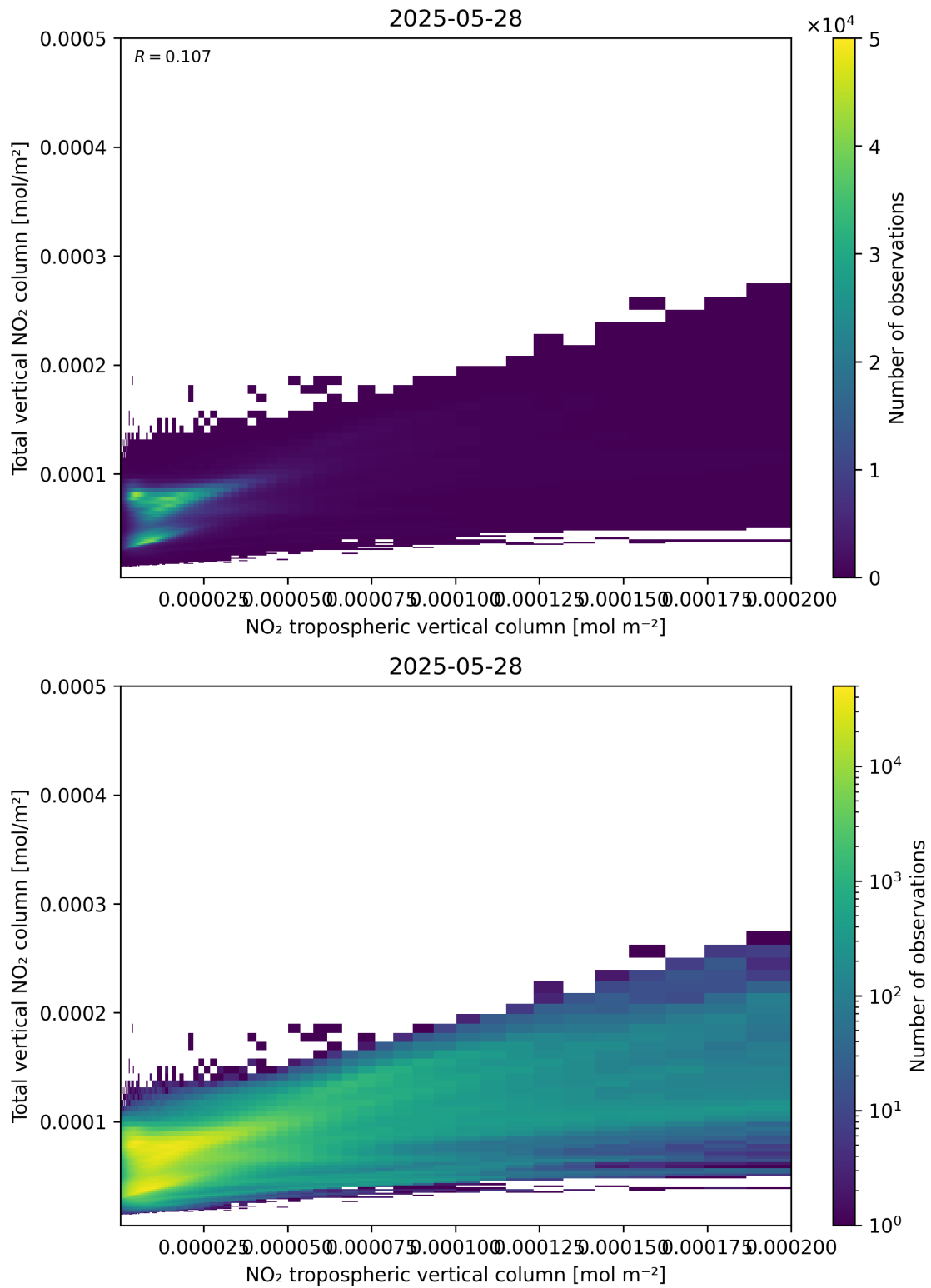
Figure 128: Scatter density plot of “NO 2 tropospheric vertical column” against “Total vertical NO 2 column” for 2025-05-27 to 2025-05-29.
