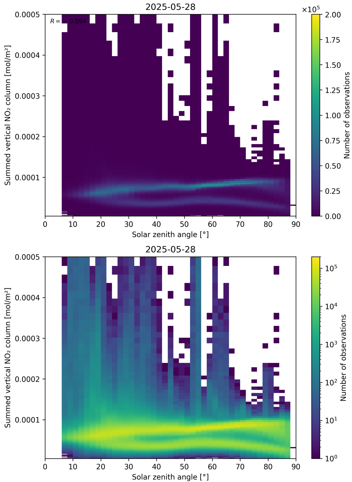
Figure 151: Scatter density plot of “Solar zenith angle” against “Summed vertical NO 2 column” for 2025-05-27 to 2025-05-29.
