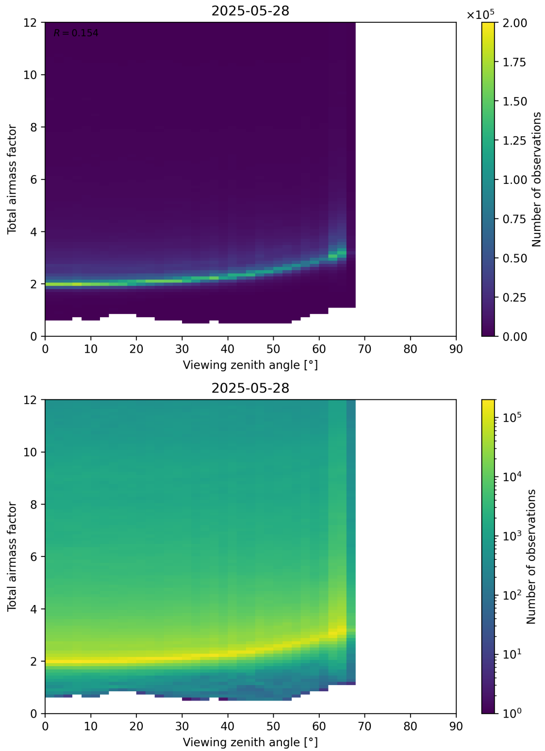
Figure 160: Scatter density plot of “Viewing zenith angle” against “Total airmass factor” for 2025-05-27 to 2025-05-29.
