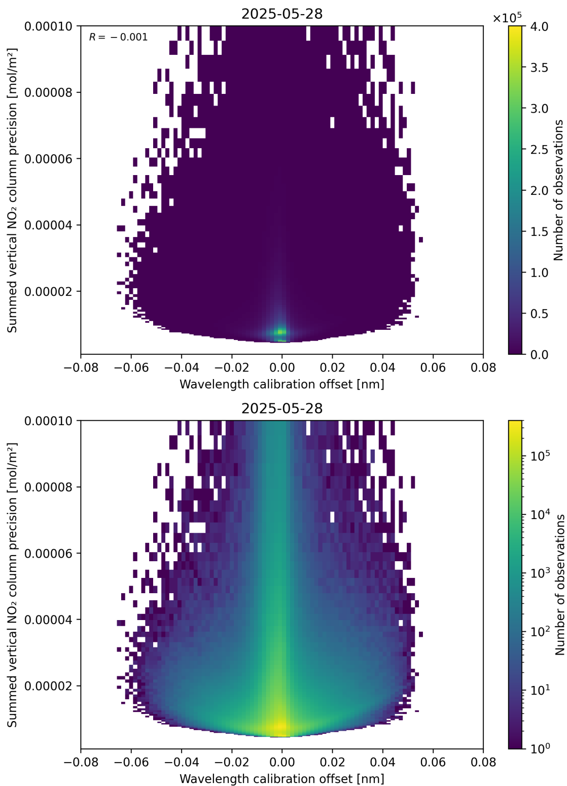
Figure 178: Scatter density plot of “Wavelength calibration offset” against “Summed vertical NO 2 column precision” for 2025-05-27 to 2025-05-29.
