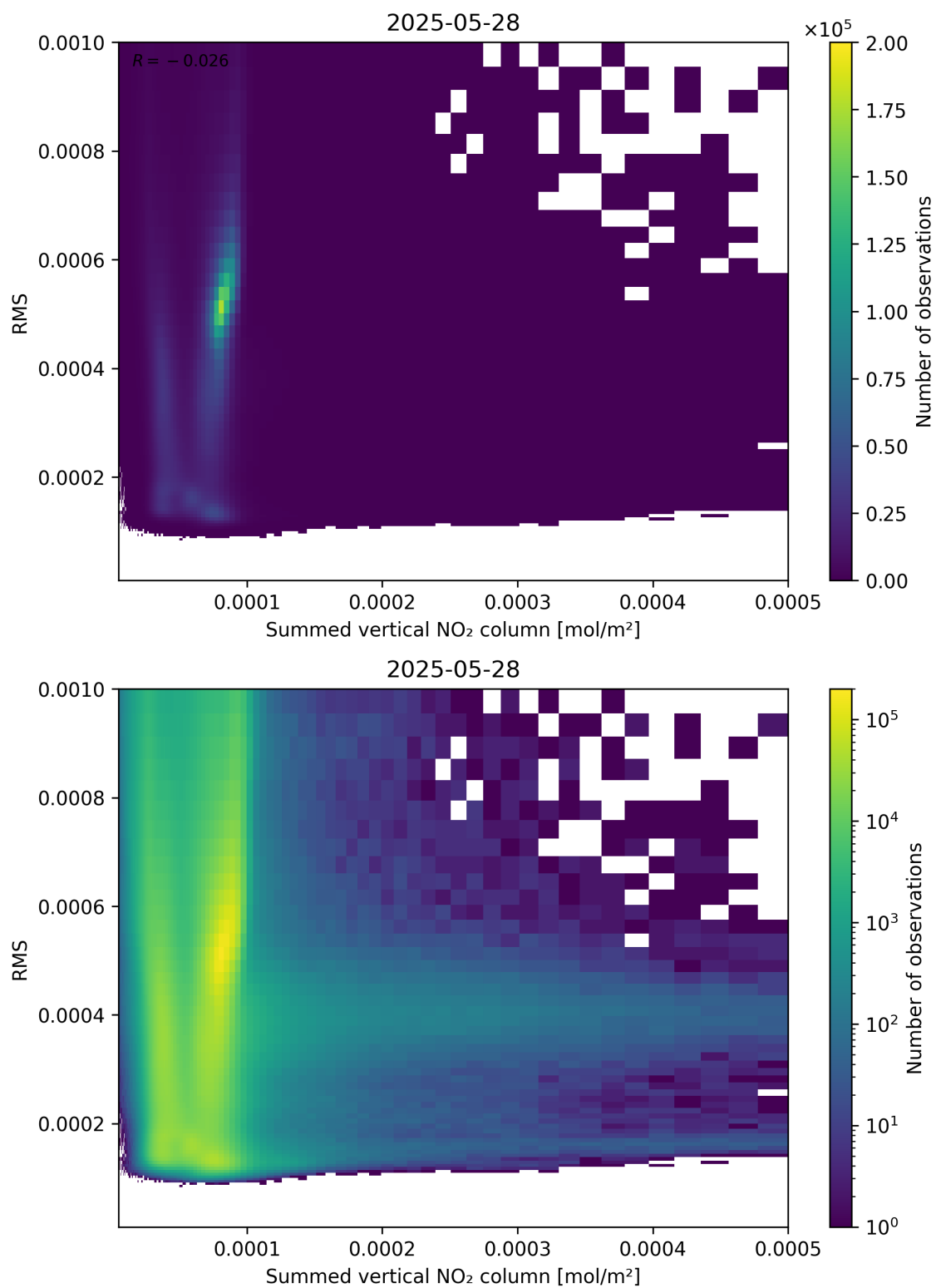
Figure 109: Scatter density plot of “Summed vertical NO 2 column” against “RMS” for 2025-05-27 to 2025-05-29.
