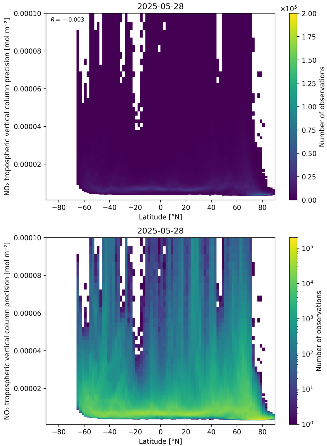
Figure 93: Scatter density plot of “Latitude” against “NO 2 tropospheric vertical column precision” for 2025-05-27 to 2025-05-29.
