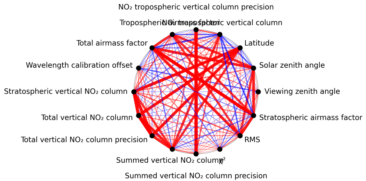
Figure 1: Map of correlation graph for 2025-05-27 to 2025-05-29.
