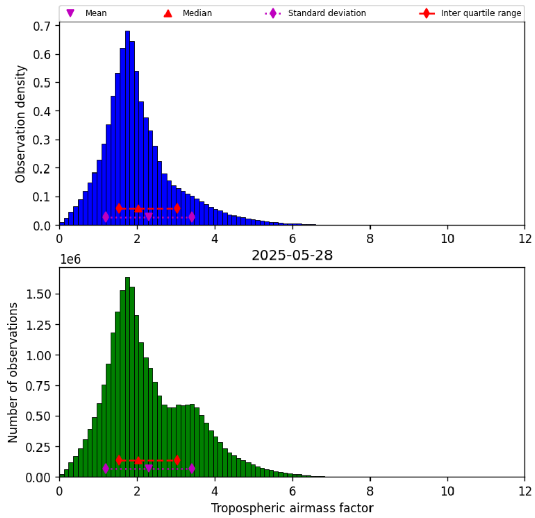
Figure 31: Histogram of “Tropospheric air mass factor” for 2025-05-27 to 2025-05-29
