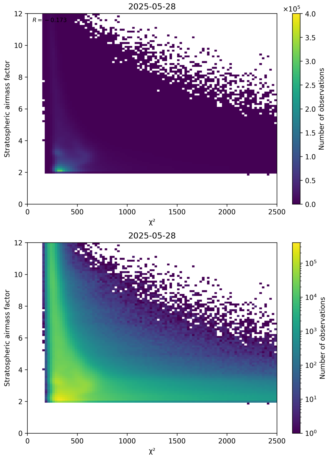
Figure 81: Scatter density plot of “ \chi^2 ” against “Stratospheric airmass factor” for 2025-05-27 to 2025-05-29.
