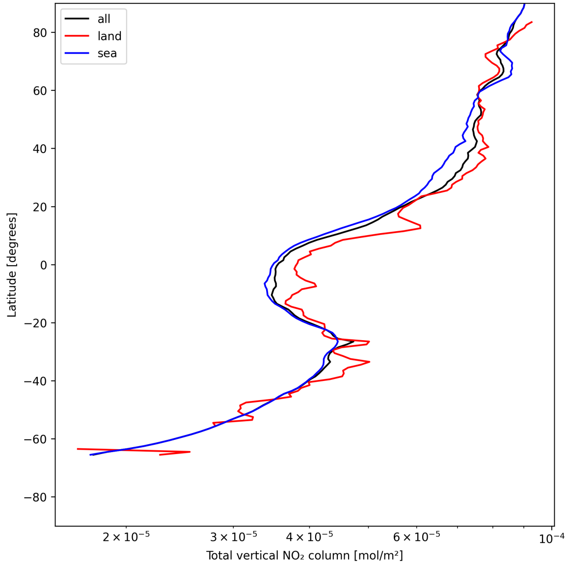
Figure 21: Zonal average of “Total vertical NO 2 column” for 2025-05-27 to 2025-05-29.
