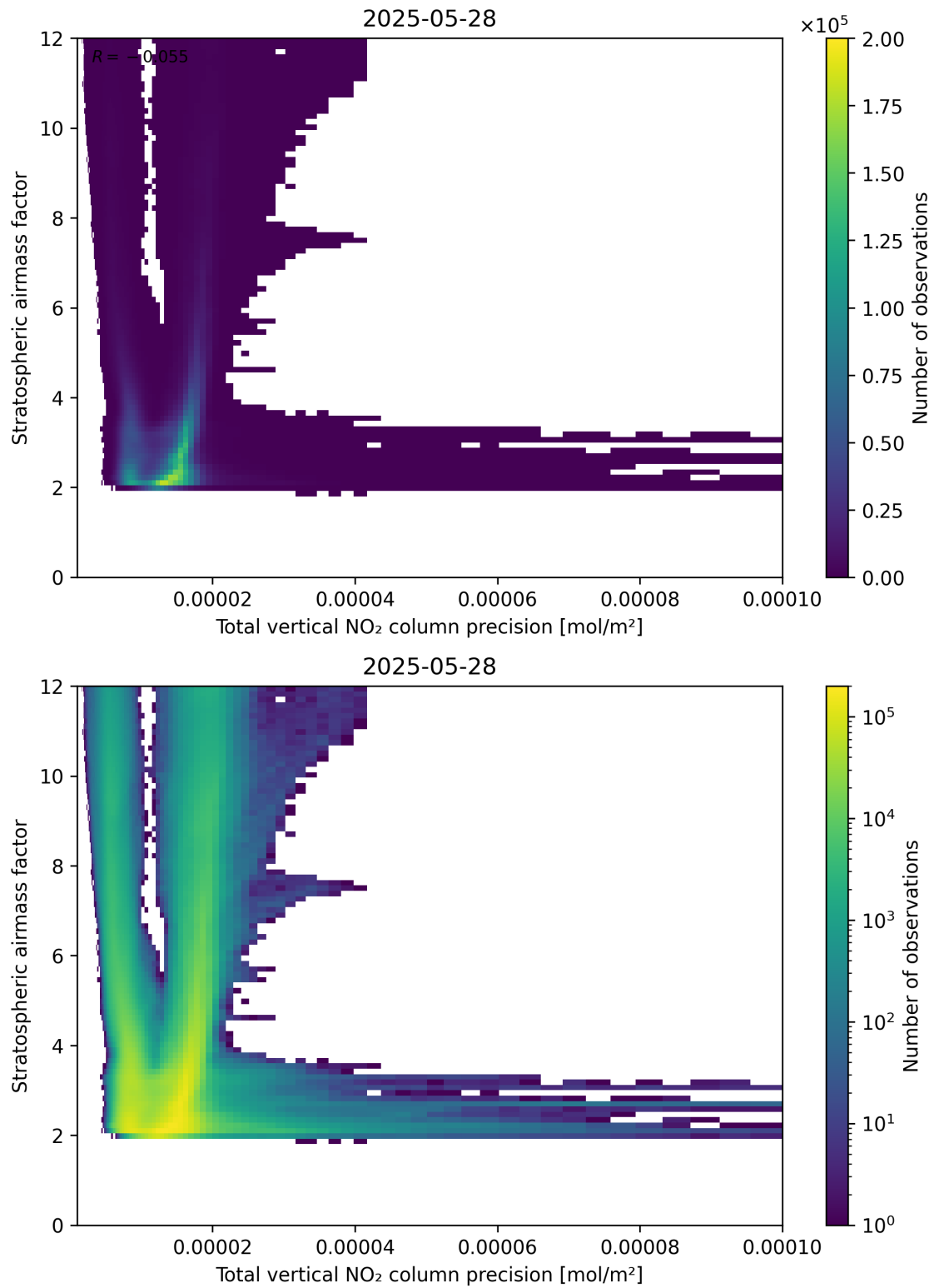
Figure 115: Scatter density plot of “Total vertical NO 2 column precision” against “Stratospheric air mass factor” for 2025-05-27 to 2025-05-29.
