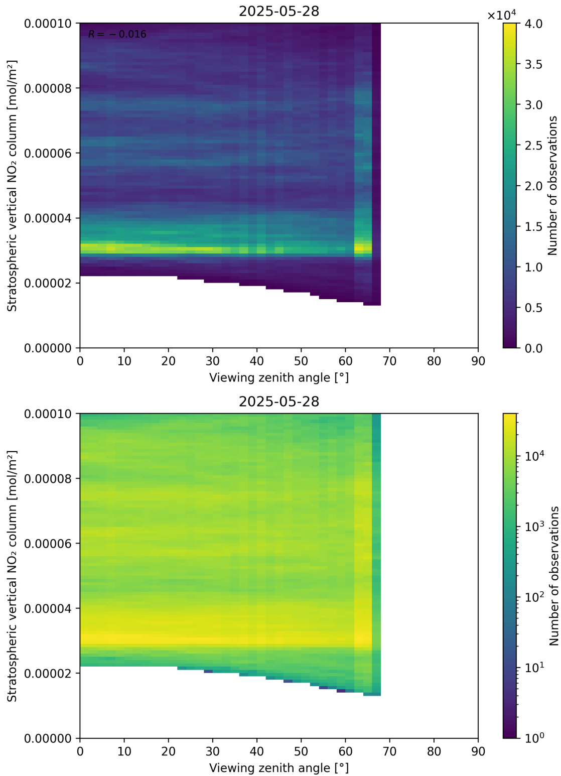
Figure 164: Scatter density plot of “Viewing zenith angle” against “Stratospheric vertical NO 2 column” for 2025-05-27 to 2025-05-29.
