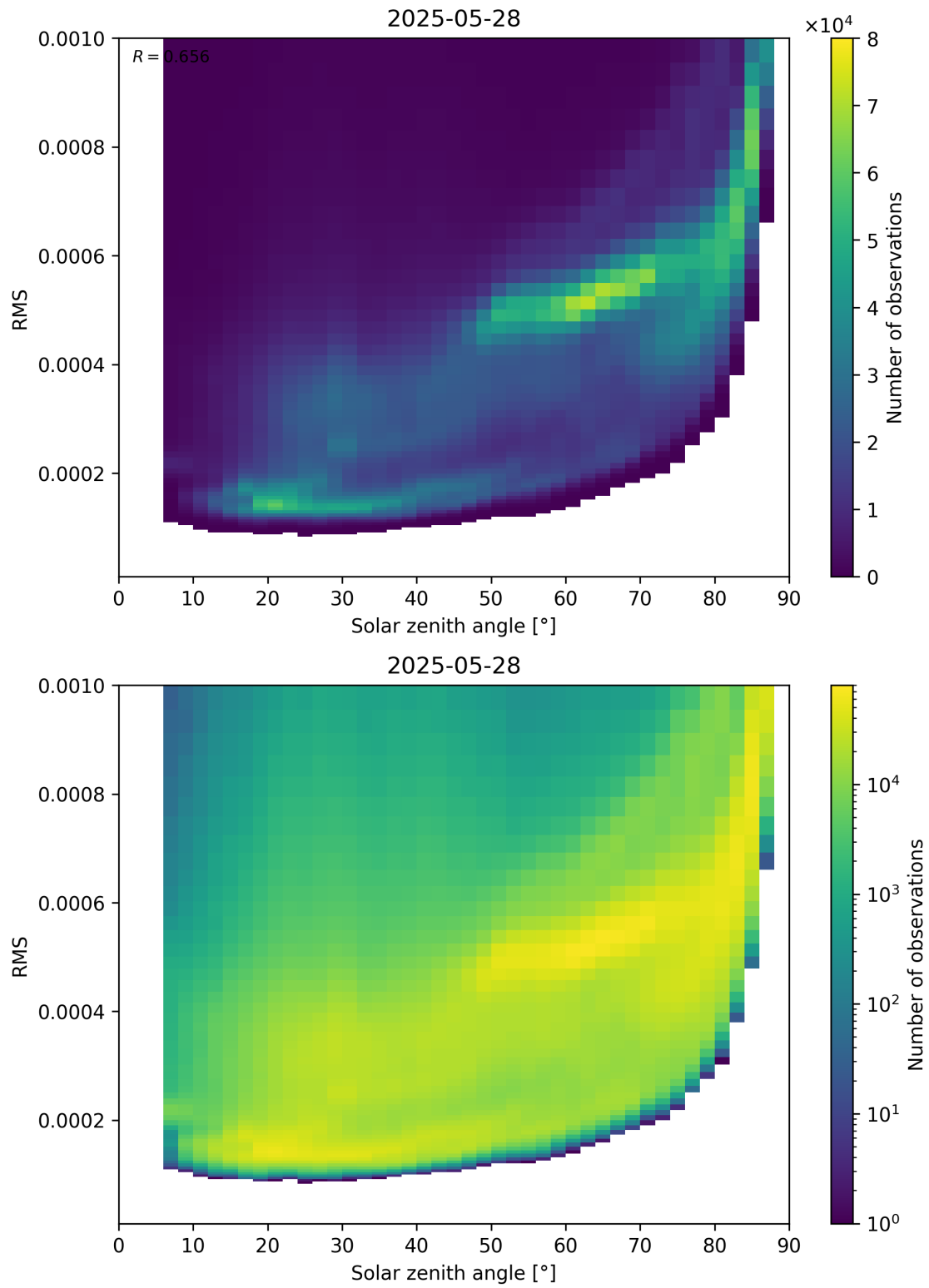
Figure 157: Scatter density plot of “Solar zenith angle” against “RMS” for 2025-05-27 to 2025-05-29.
