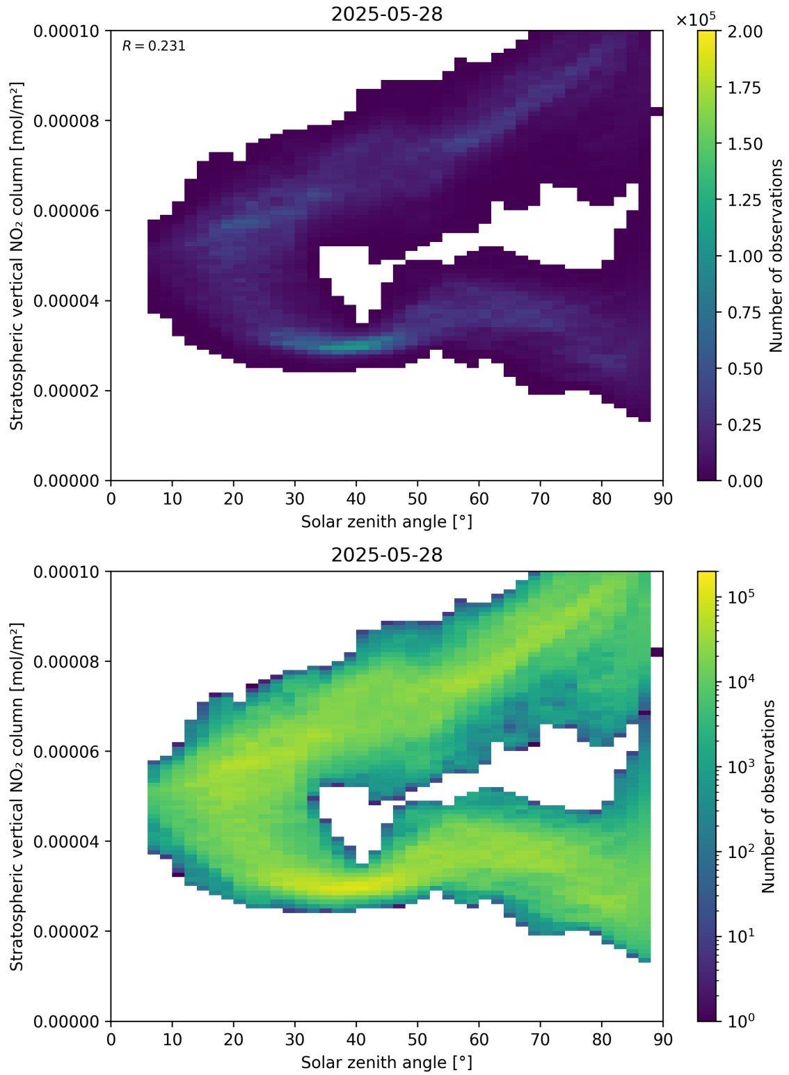
Figure 150: Scatter density plot of “Solar zenith angle” against “Stratospheric vertical NO 2 column” for 2025-05-27 to 2025-05-29.
