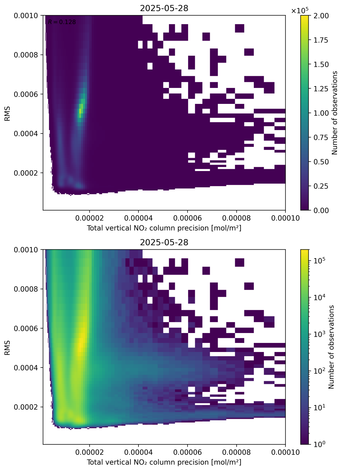
Figure 119: Scatter density plot of “Total vertical NO 2 column precision” against “RMS” for 2025-05-27 to 2025-05-29.
