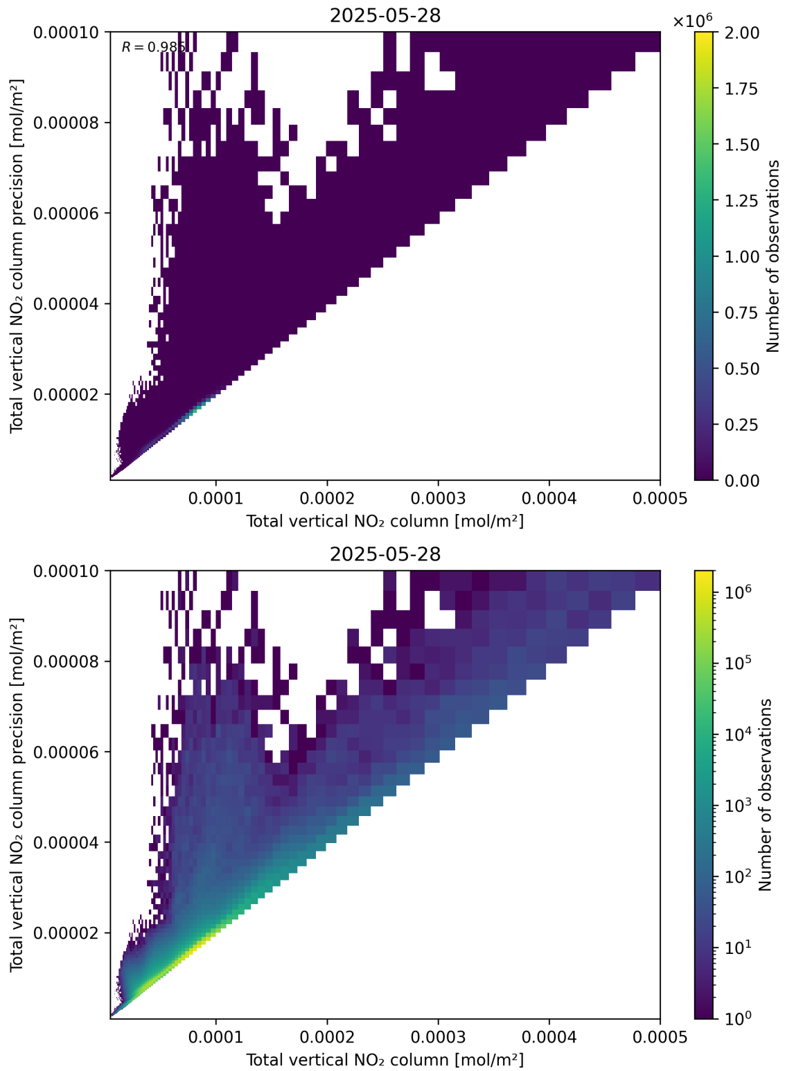
Figure 114: Scatter density plot of “Total vertical NO 2 column” against “Total vertical NO 2 column precision” for 2025-05-27 to 2025-05-29.
