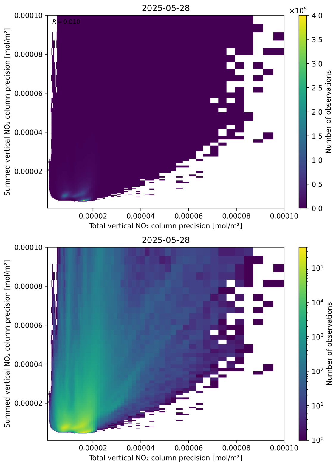
Figure 118: Scatter density plot of “Total vertical NO 2 column precision” against “Summed vertical NO 2 column precision” for 2025-05-27 to 2025-05-29.
