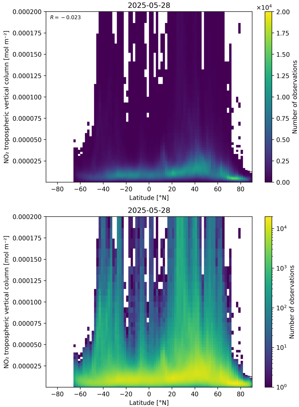
Figure 92: Scatter density plot of “Latitude” against “NO 2 tropospheric vertical column” for 2025-05-27 to 2025-05-29.
