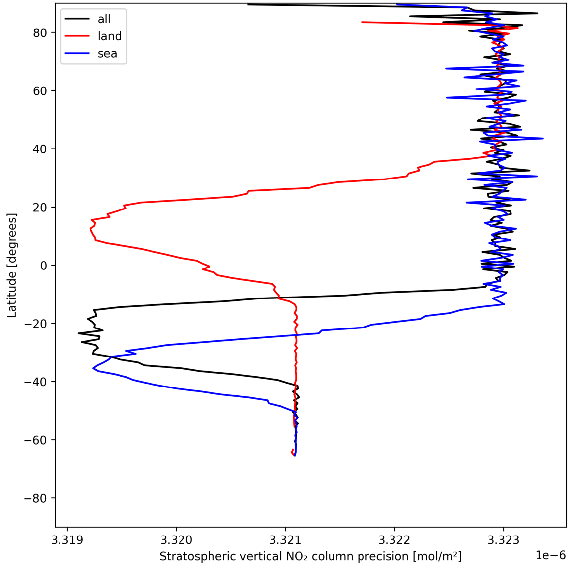
Figure 20: Zonal average of “Stratospheric vertical NO 2 column precision” for 2025-05-27 to 2025-05-29.
