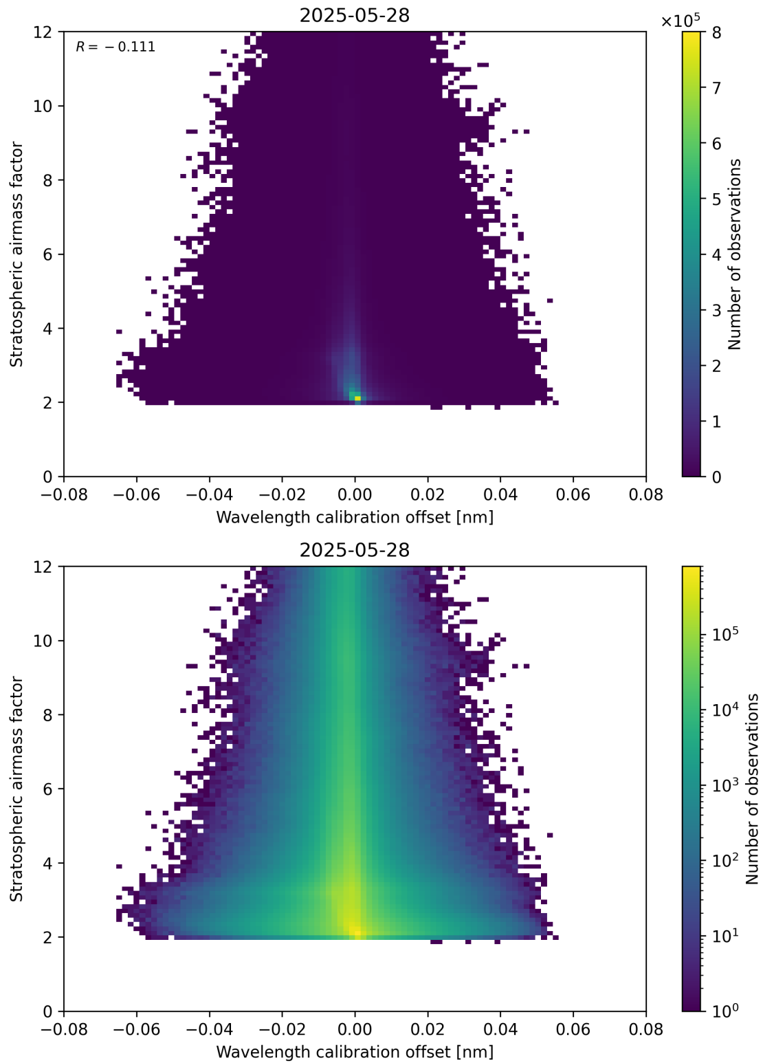
Figure 174: Scatter density plot of “Wavelength calibration offset” against “Stratospheric air mass factor” for 2025-05-27 to 2025-05-29.
