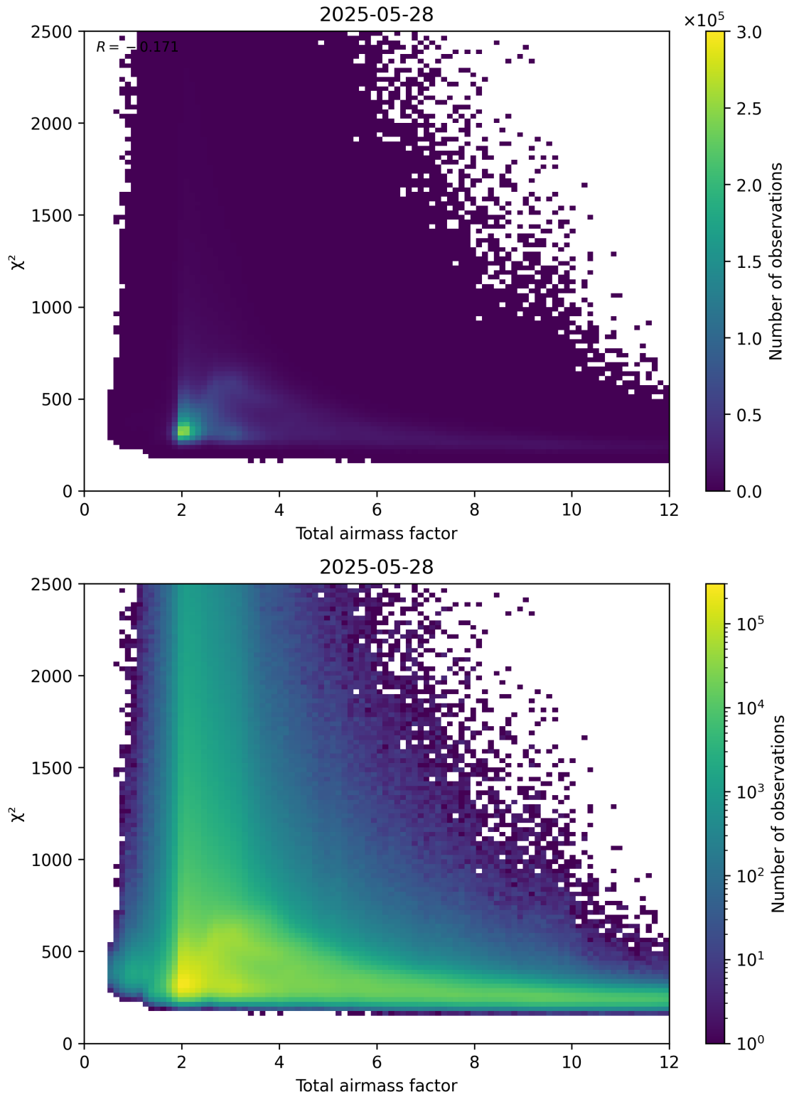
Figure 63: Scatter density plot of “Total airmass factor” against “ \chi^2 ” for 2025-05-27 to 2025-05-29.
