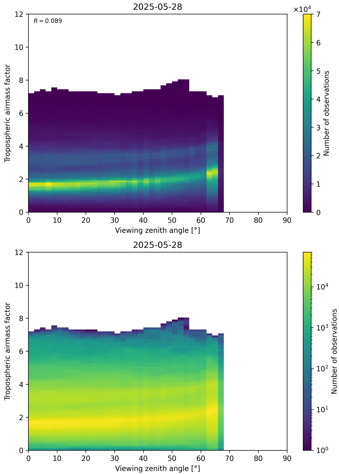
Figure 161: Scatter density plot of “Viewing zenith angle” against “Tropospheric airmass factor” for 2025-05-27 to 2025-05-29.
