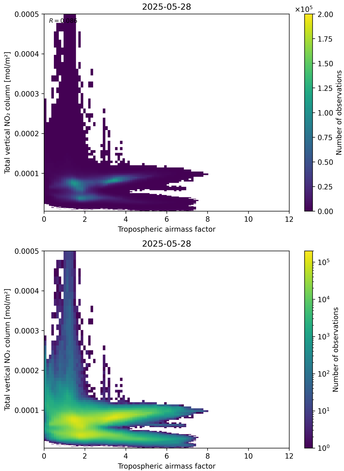
Figure 77: Scatter density plot of “Tropospheric airmass factor” against “Total vertical \text{NO}_2 column” for 2025-05-27 to 2025-05-29.
