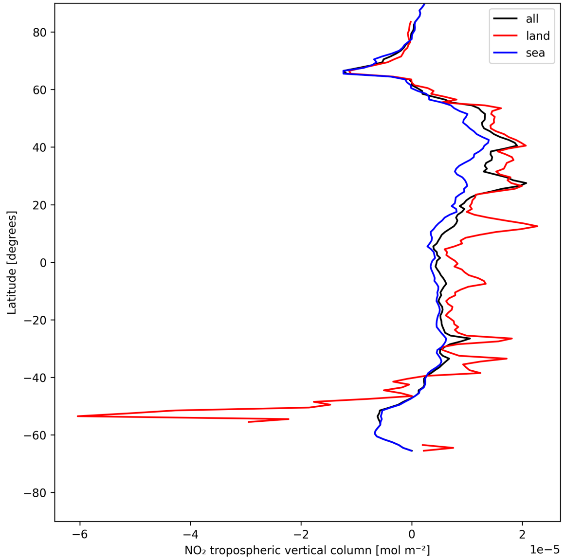
Figure 12: Zonal average of “NO 2 tropospheric vertical column” for 2025-05-27 to 2025-05-29.
