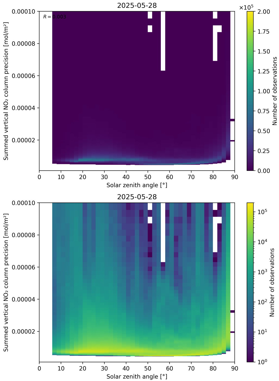
Figure 152: Scatter density plot of “Solar zenith angle” against “Summed vertical NO 2 column precision” for 2025-05-27 to 2025-05-29.
