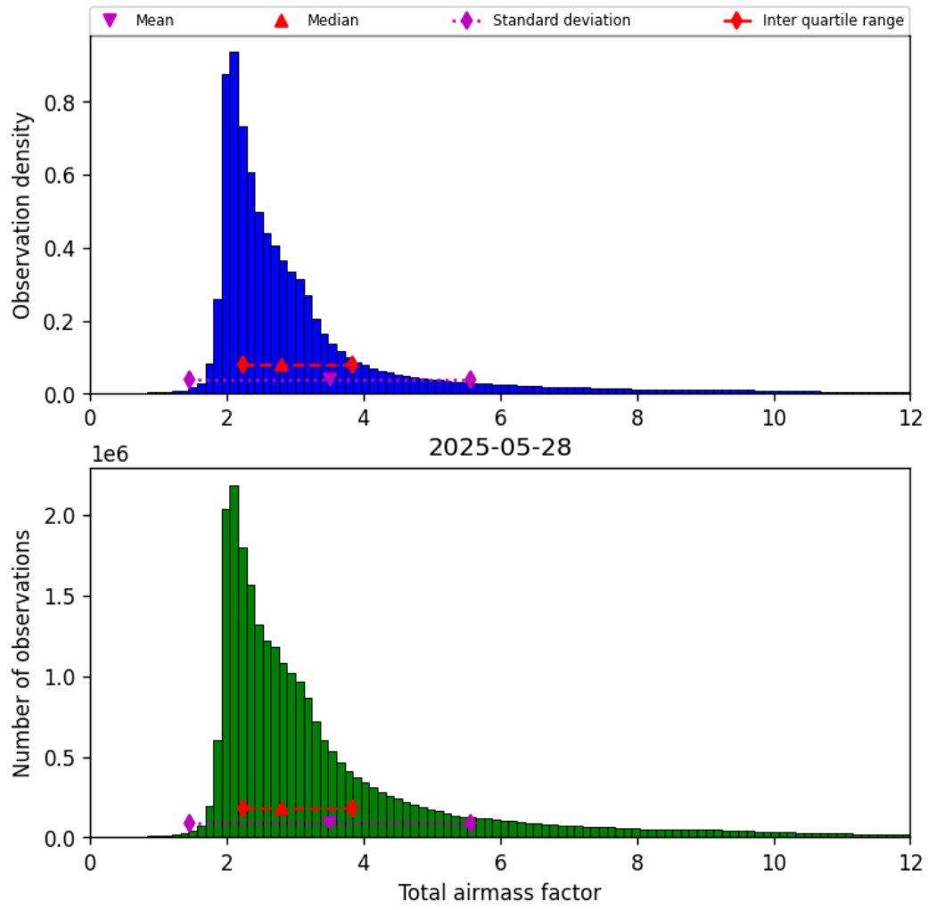
Figure 32: Histogram of “Total airmass factor” for 2025-05-27 to 2025-05-29
