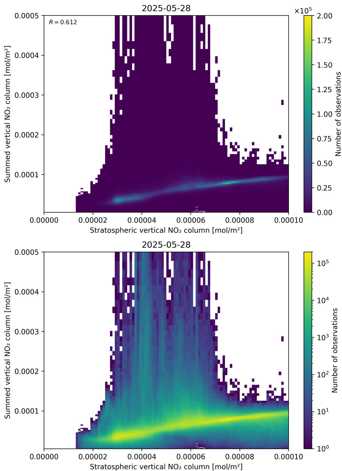
Figure 98: Scatter density plot of “Stratospheric vertical NO 2 column” against “Summed vertical NO 2 column” for 2025-05-27 to 2025-05-29.
