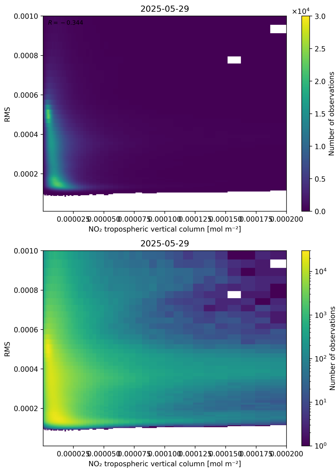
Figure 142: Scatter density plot of “NO 2 tropospheric vertical column” against “RMS” for 2025-05-28 to 2025-05-30.
