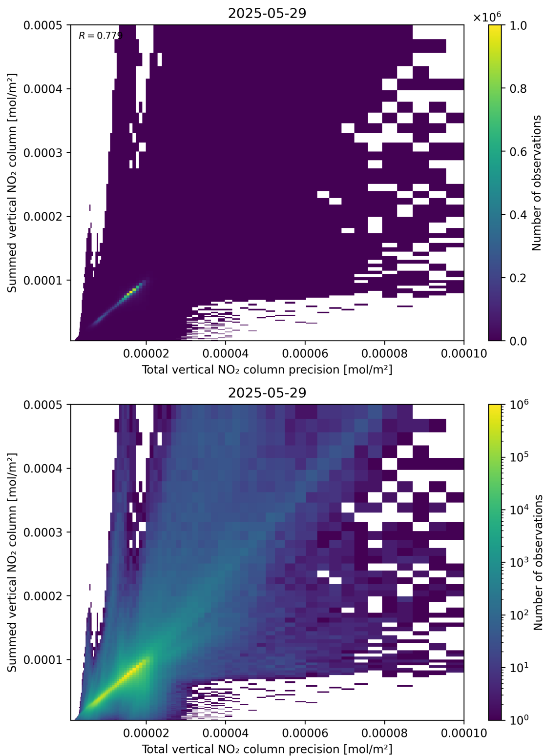
Figure 117: Scatter density plot of “Total vertical NO 2 column precision” against “Summed vertical NO 2 column” for 2025-05-28 to 2025-05-30.
