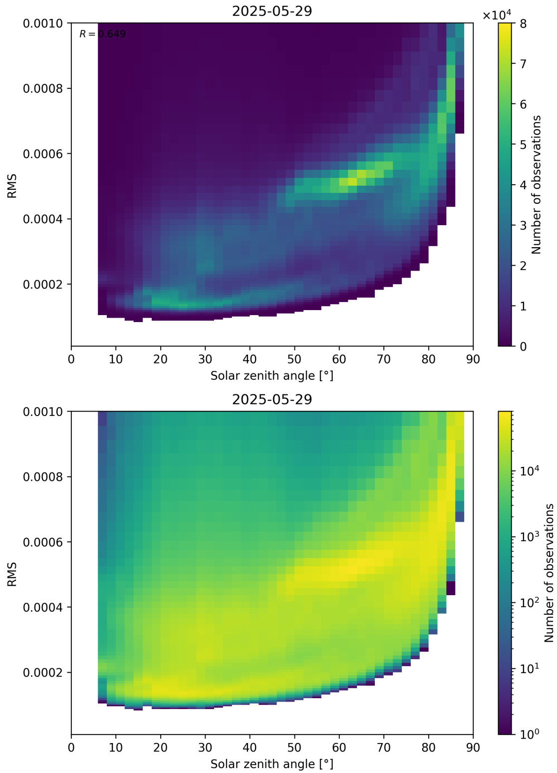
Figure 157: Scatter density plot of “Solar zenith angle” against “RMS” for 2025-05-28 to 2025-05-30.
