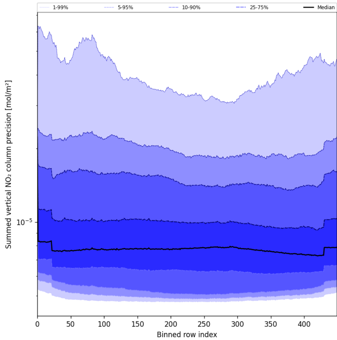
Figure 58: Along track statistics of “Summed vertical NO 2 column precision” for 2025-05-28 to 2025-05-30
