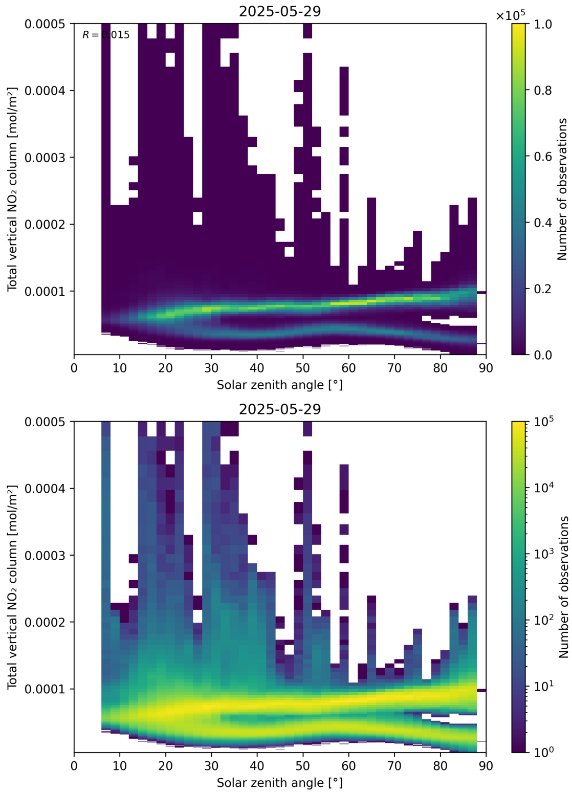
Figure 153: Scatter density plot of “Solar zenith angle” against “Total vertical NO 2 column” for 2025-05-28 to 2025-05-30.
