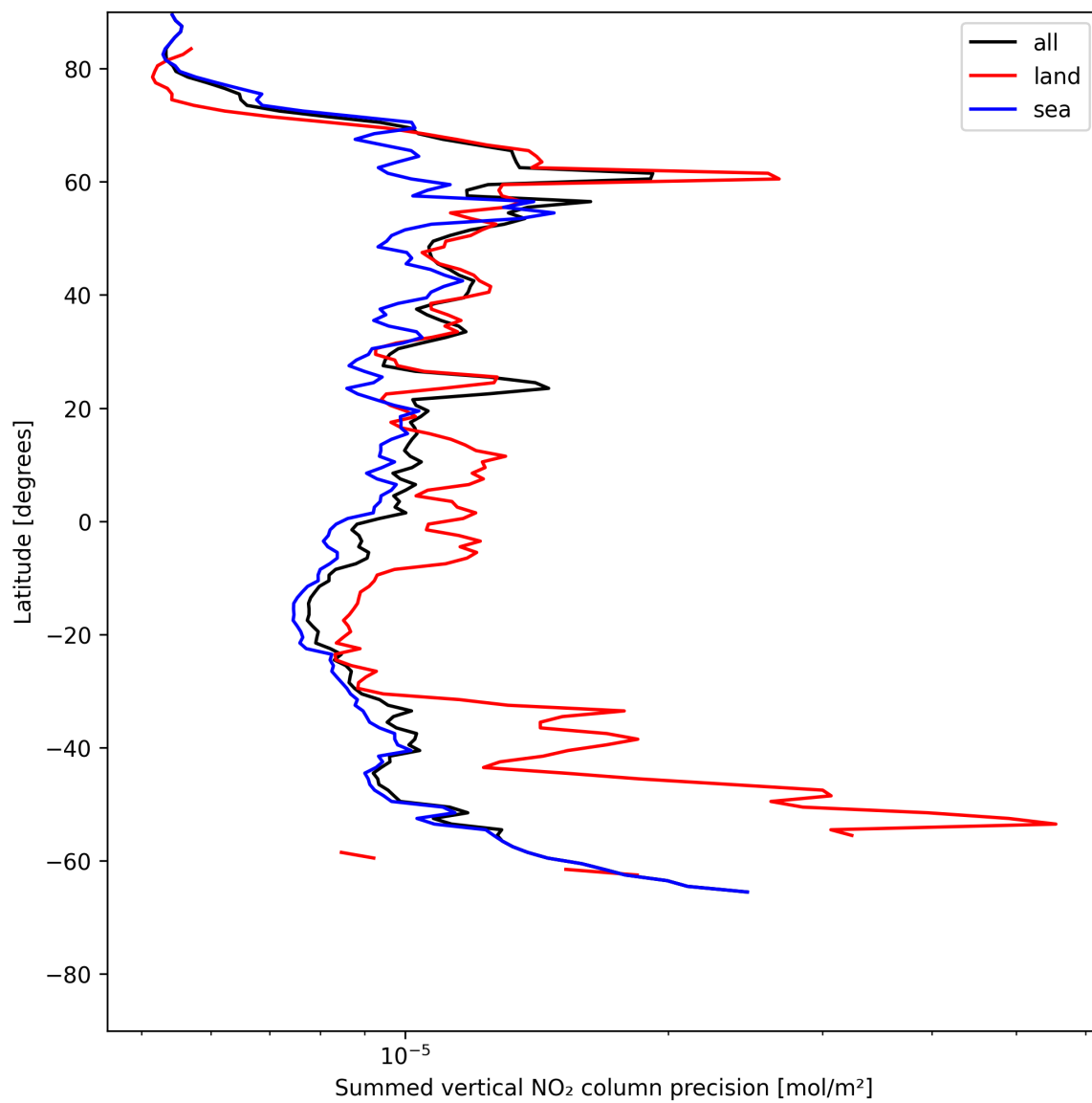
Figure 24: Zonal average of “Summed vertical NO 2 column precision” for 2025-05-28 to 2025-05-30.
