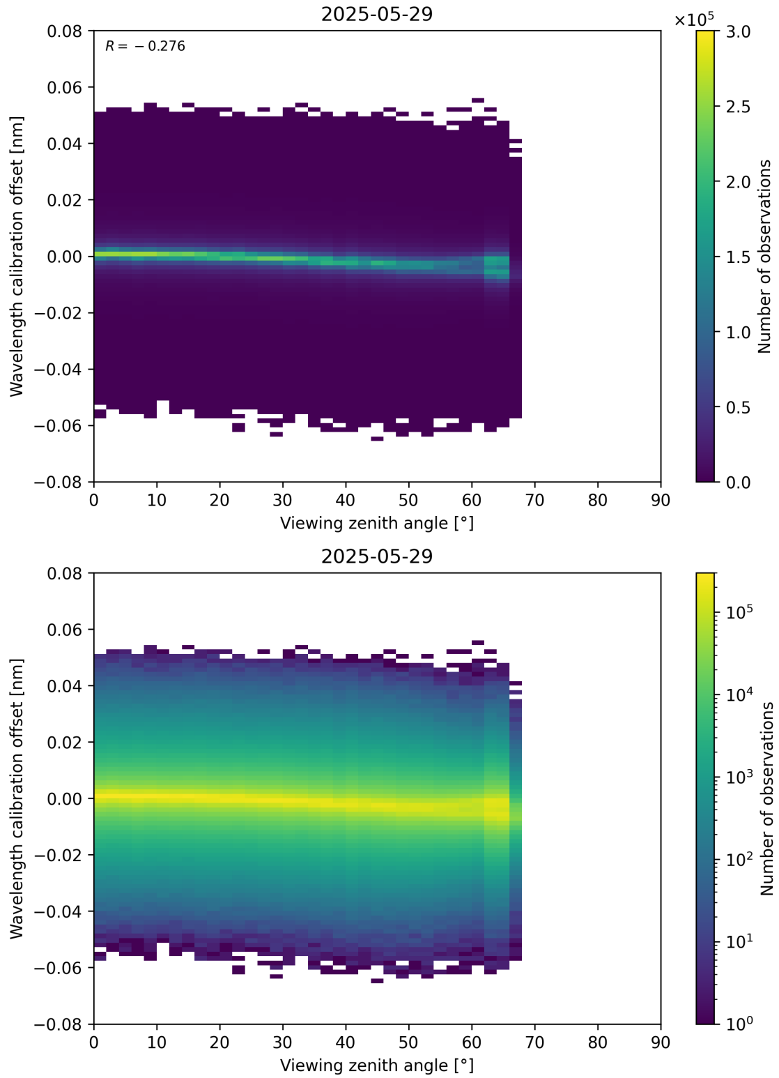
Figure 173: Scatter density plot of “Viewing zenith angle” against “Wavelength calibration offset” for 2025-05-28 to 2025-05-30.
