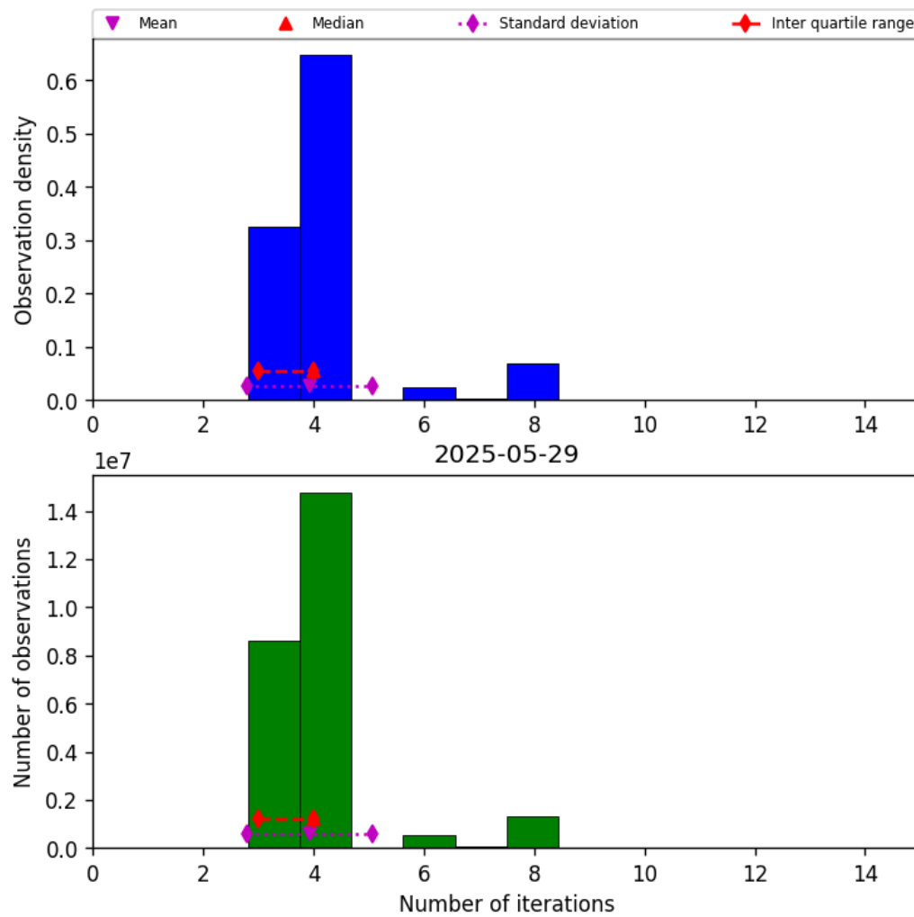
Figure 34: Histogram of “Number of iterations” for 2025-05-28 to 2025-05-30
