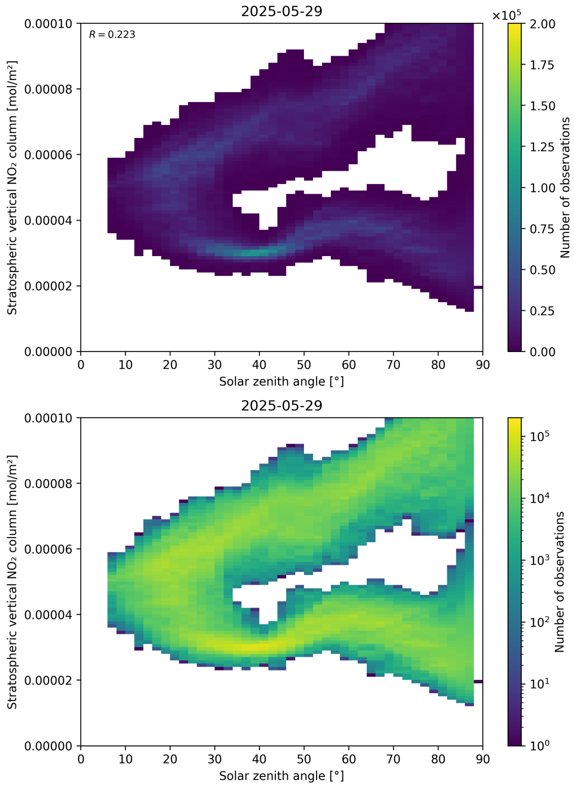
Figure 150: Scatter density plot of “Solar zenith angle” against “Stratospheric vertical NO 2 column” for 2025-05-28 to 2025-05-30.
