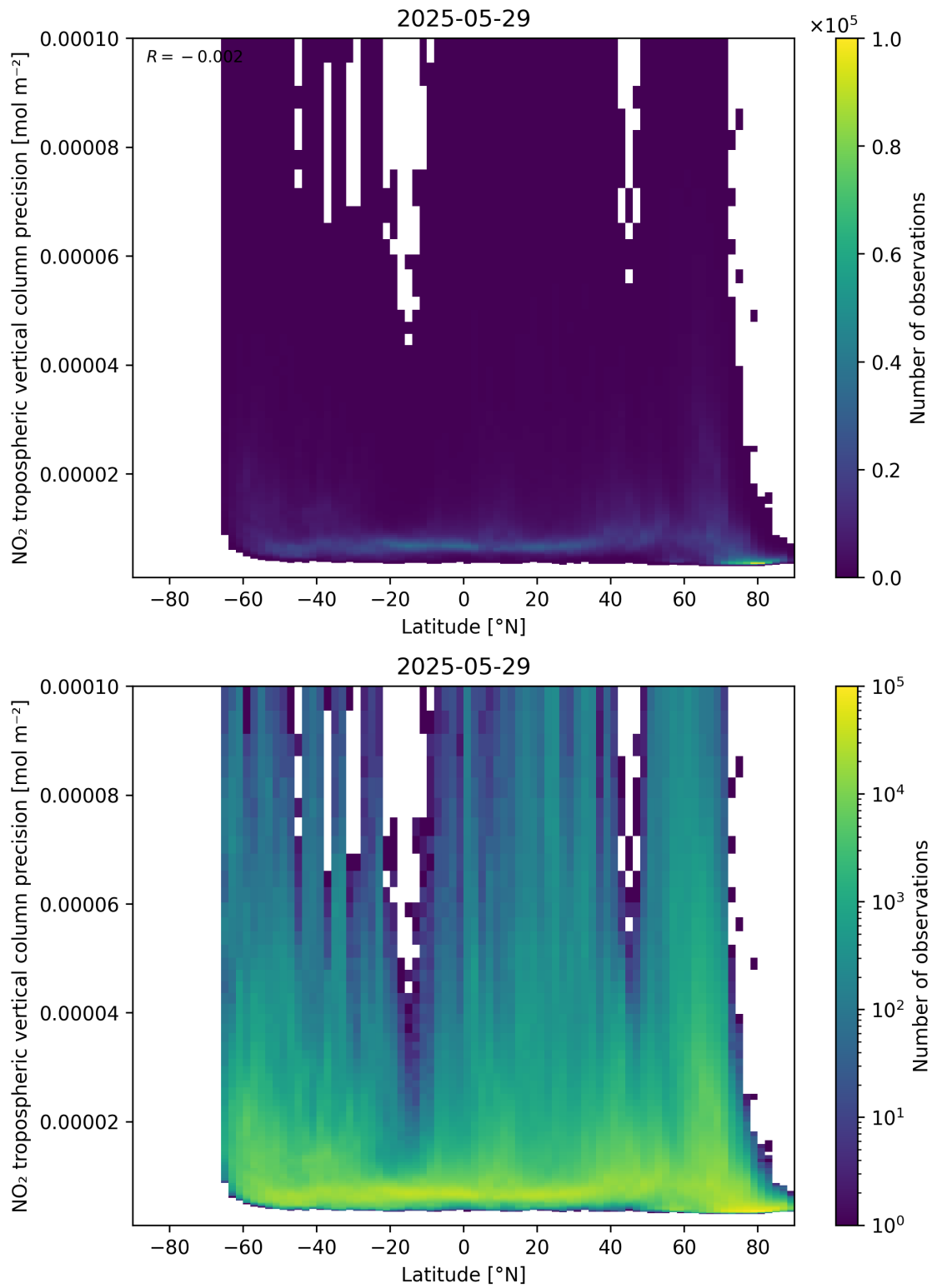
Figure 93: Scatter density plot of “Latitude” against “NO 2 tropospheric vertical column precision” for 2025-05-28 to 2025-05-30.
