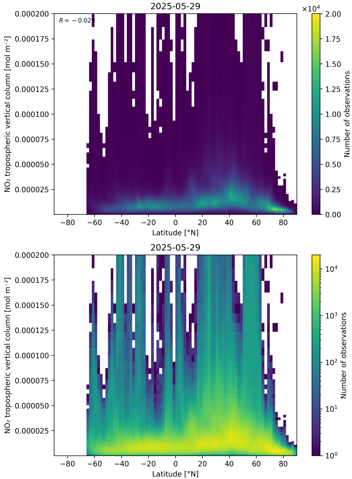
Figure 92: Scatter density plot of “Latitude” against “NO 2 tropospheric vertical column” for 2025-05-28 to 2025-05-30.
