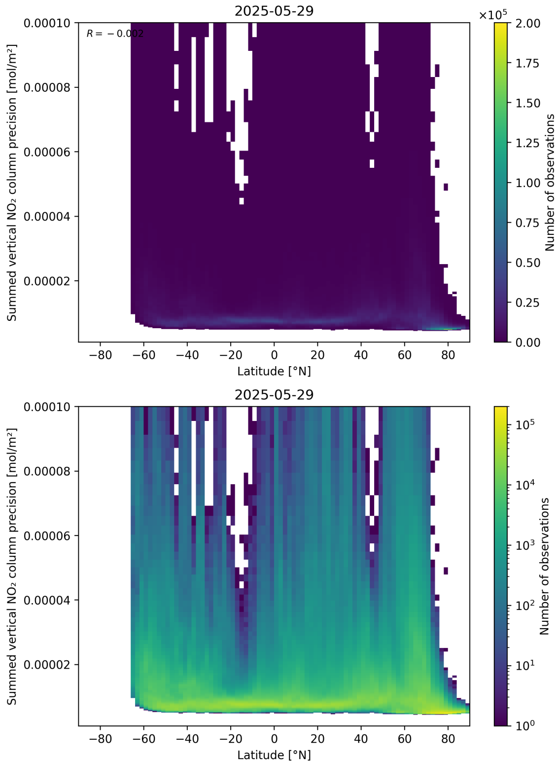
Figure 89: Scatter density plot of “Latitude” against “Summed vertical NO 2 column precision” for 2025-05-28 to 2025-05-30.
