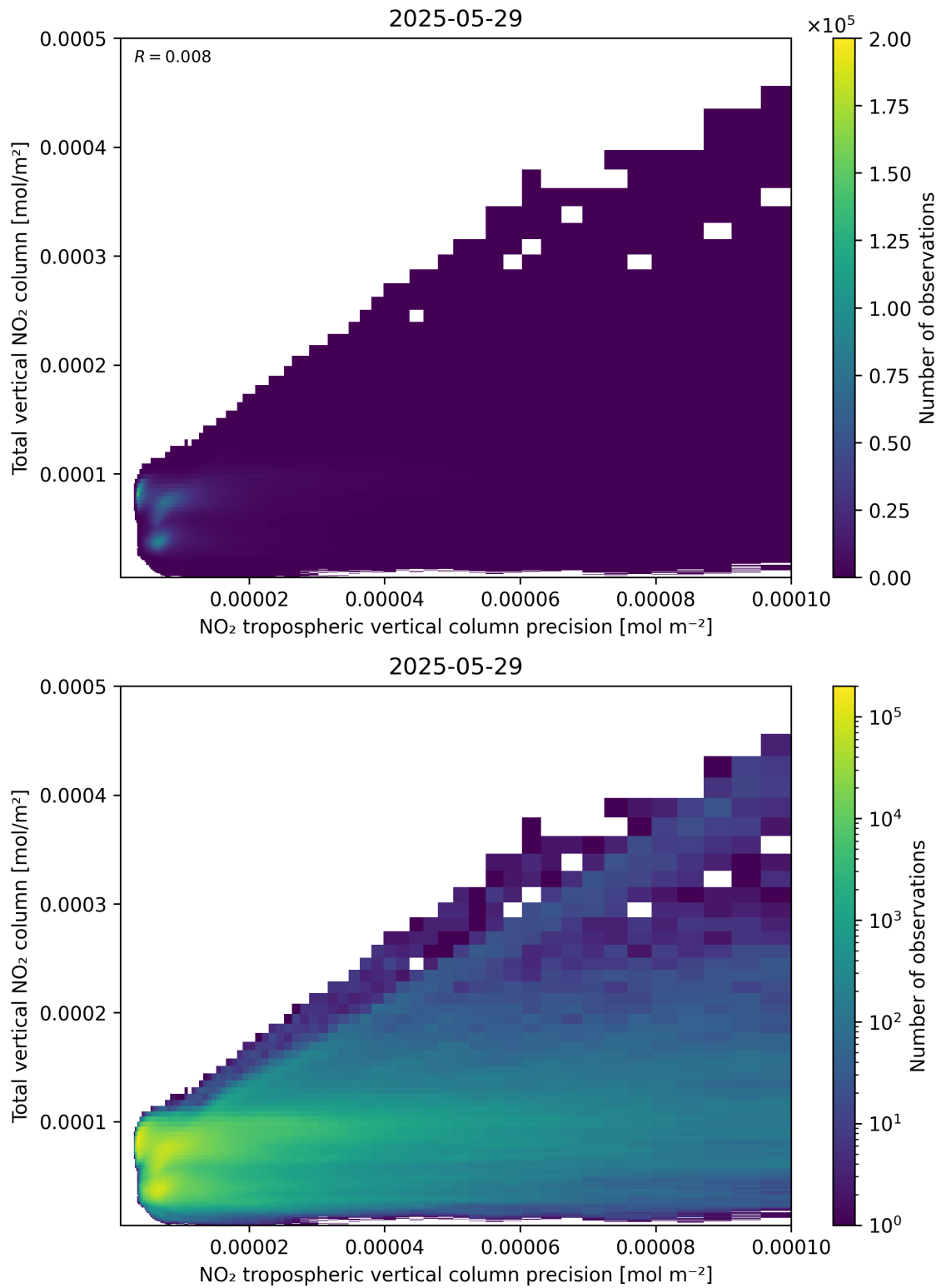
Figure 138: Scatter density plot of “NO 2 tropospheric vertical column precision” against “Total vertical NO 2 column” for 2025-05-28 to 2025-05-30.
