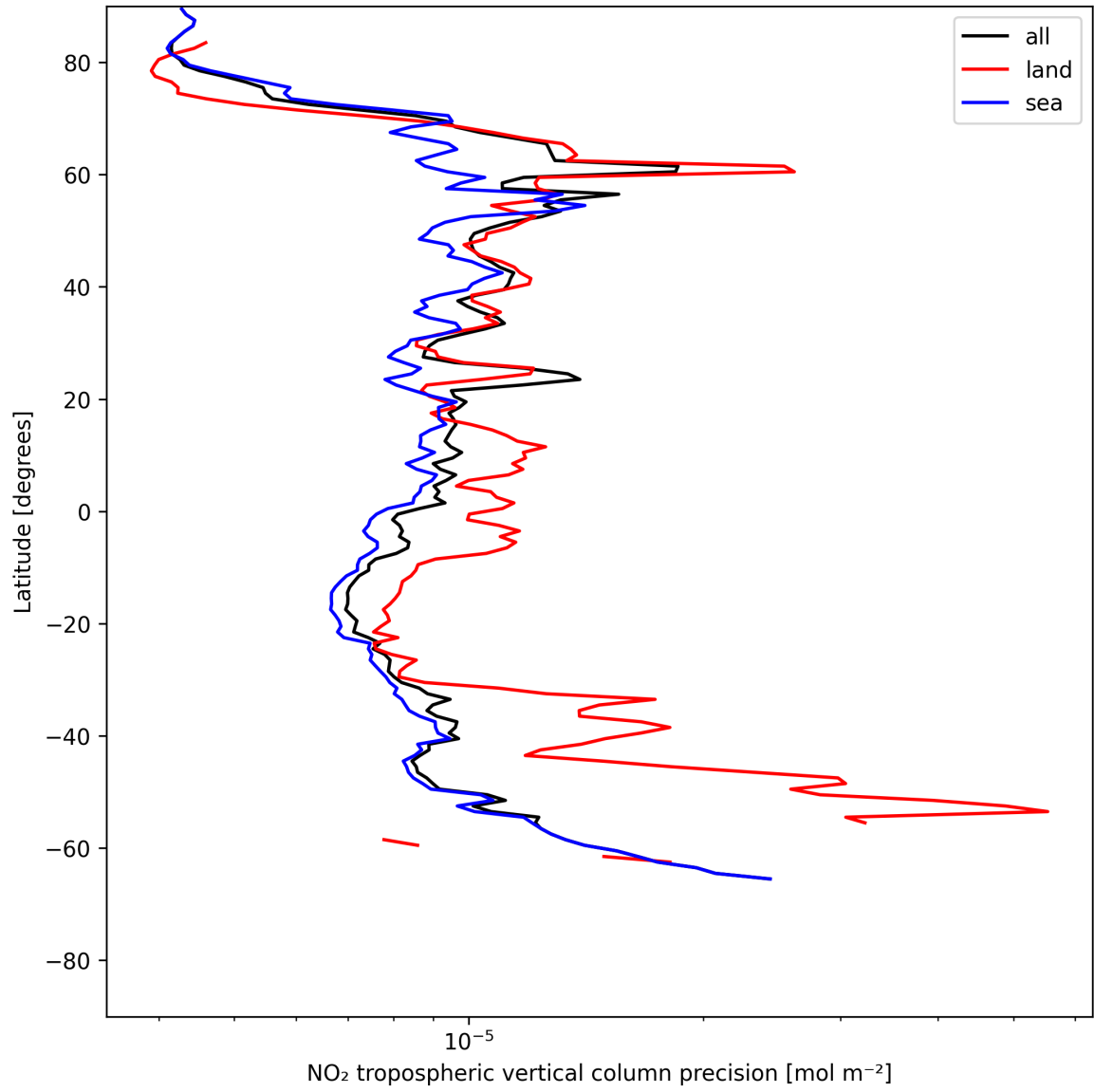
Figure 13: Zonal average of “NO 2 tropospheric vertical column precision” for 2025-05-28 to 2025-05-30.
