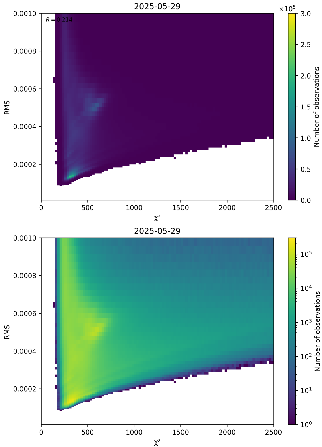
Figure 82: Scatter density plot of “ \chi^2 ” against “RMS” for 2025-05-28 to 2025-05-30.
