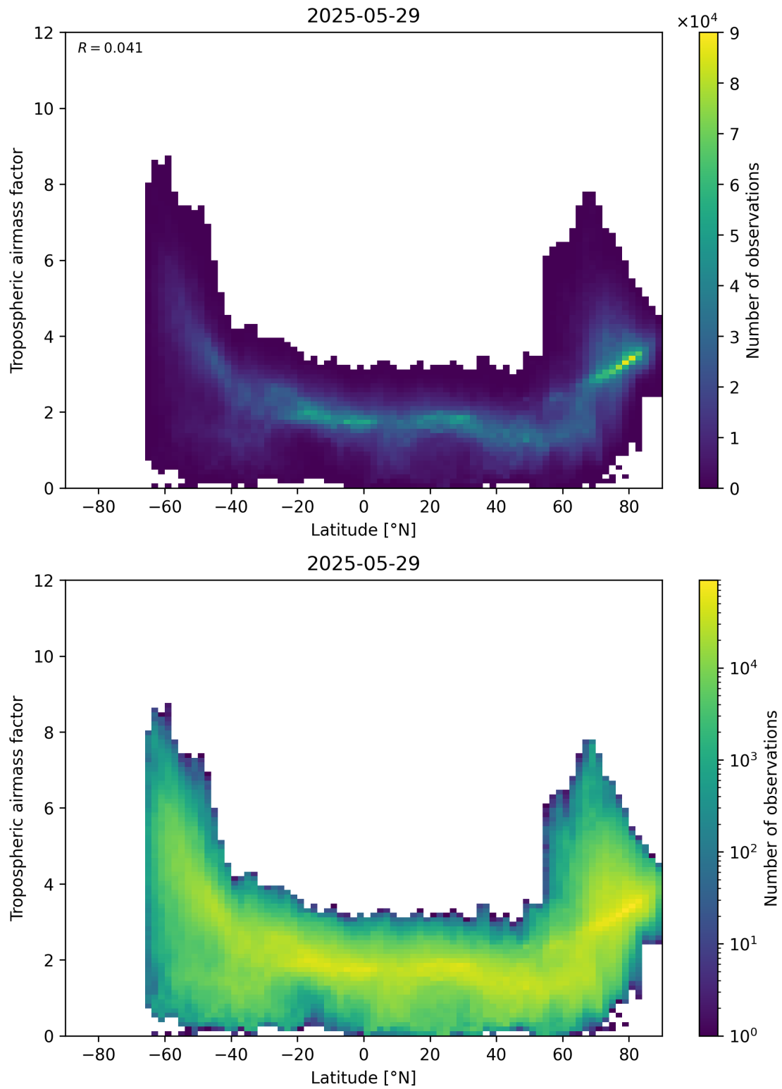
Figure 85: Scatter density plot of “Latitude” against “Tropospheric air mass factor” for 2025-05-28 to 2025-05-30.
