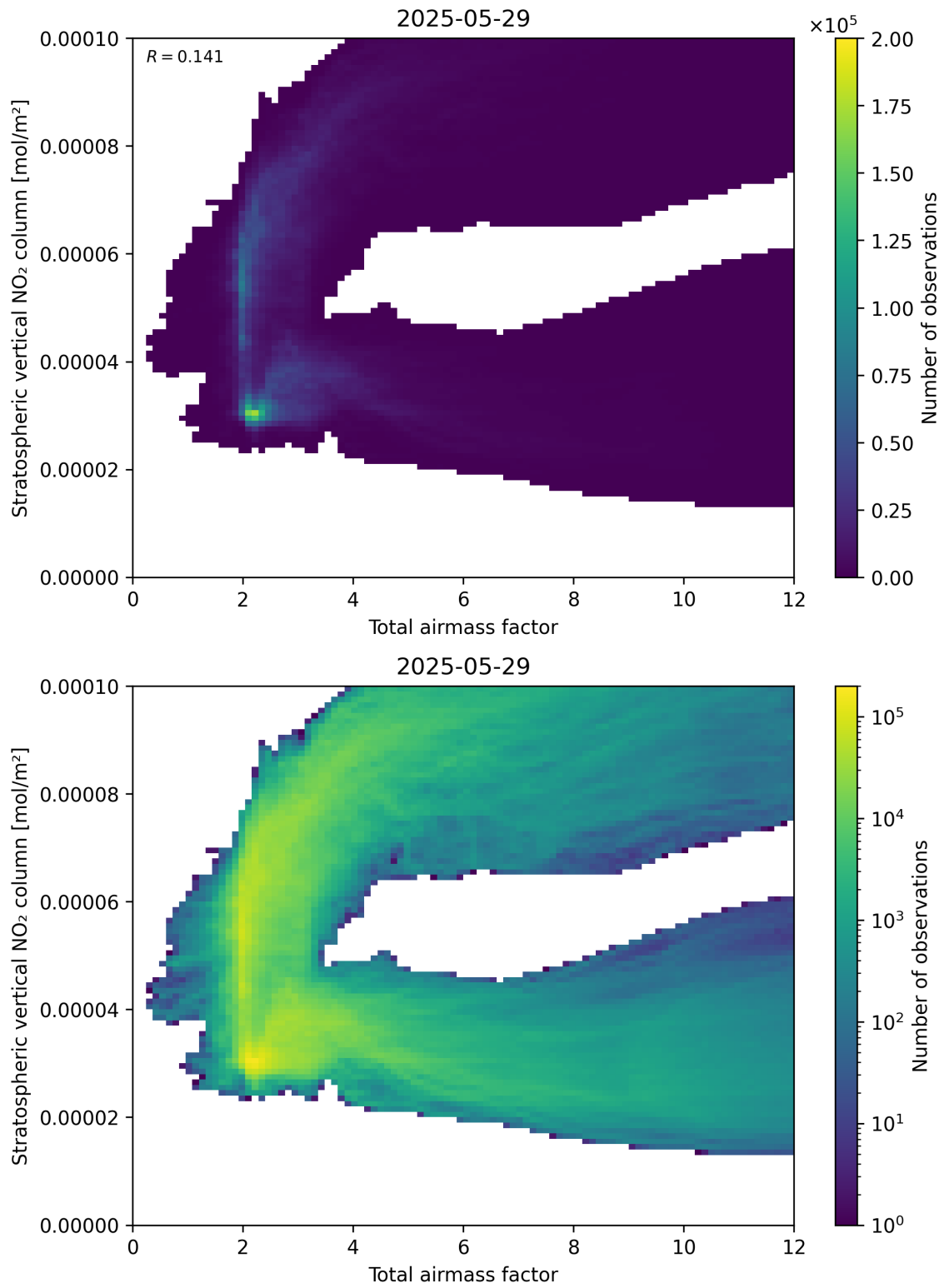
Figure 64: Scatter density plot of “Total airmass factor” against “Stratospheric vertical NO 2 column” for 2025-05-28 to 2025-05-30.
