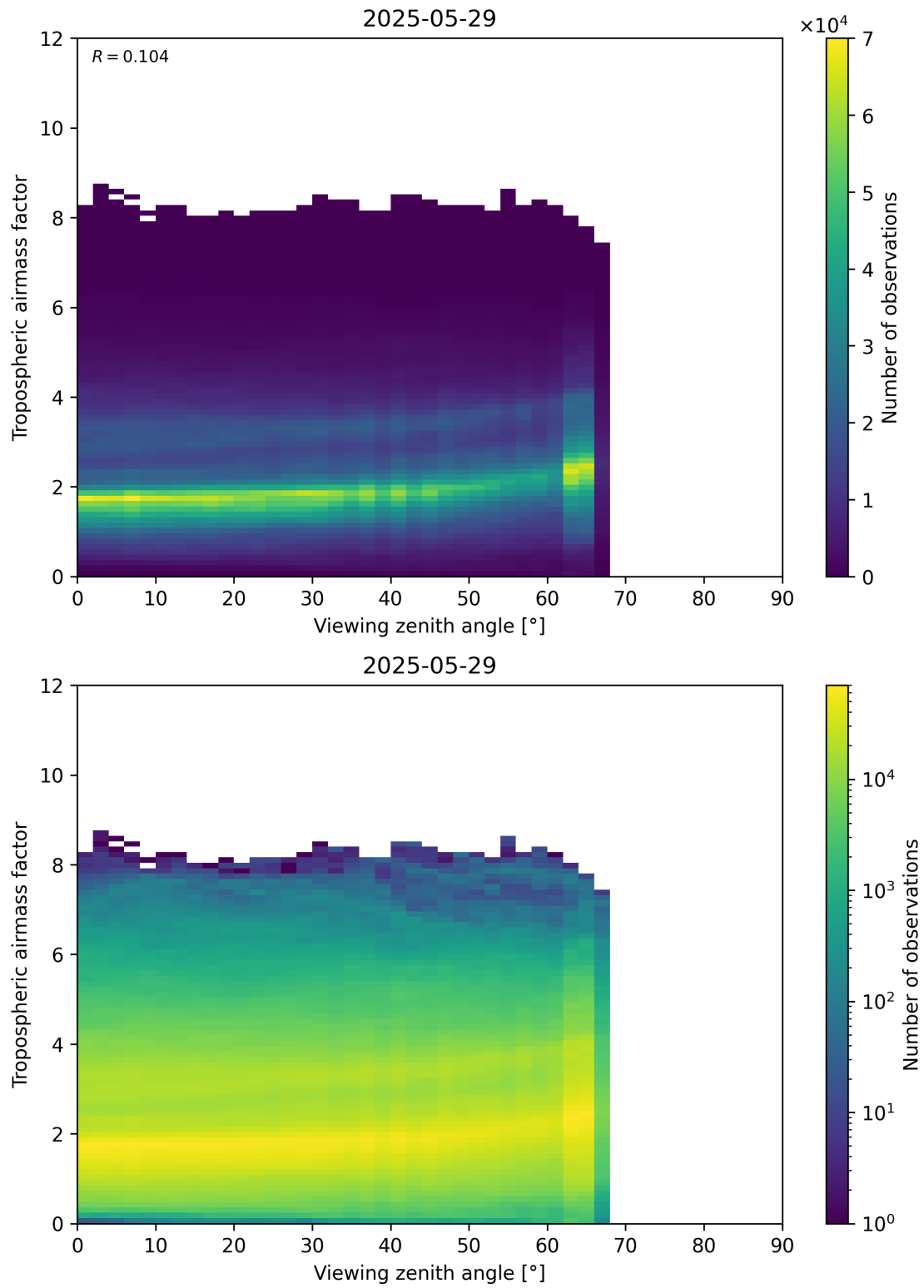
Figure 161: Scatter density plot of “Viewing zenith angle” against “Tropospheric airmass factor” for 2025-05-28 to 2025-05-30.
