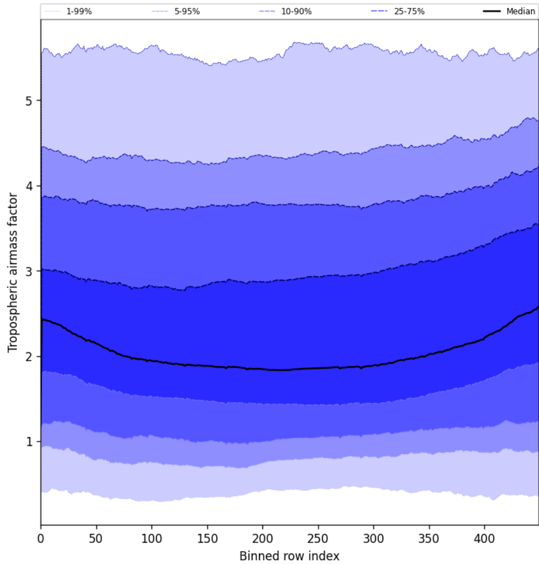
Figure 48: Along track statistics of “Tropospheric airmass factor” for 2025-05-28 to 2025-05-30
