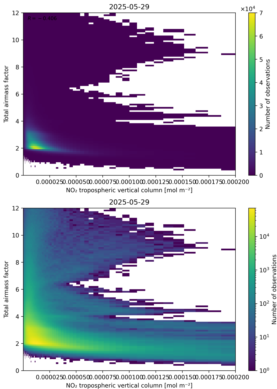
Figure 122: Scatter density plot of “NO 2 tropospheric vertical column” against “Total air mass factor” for 2025-05-28 to 2025-05-30.
