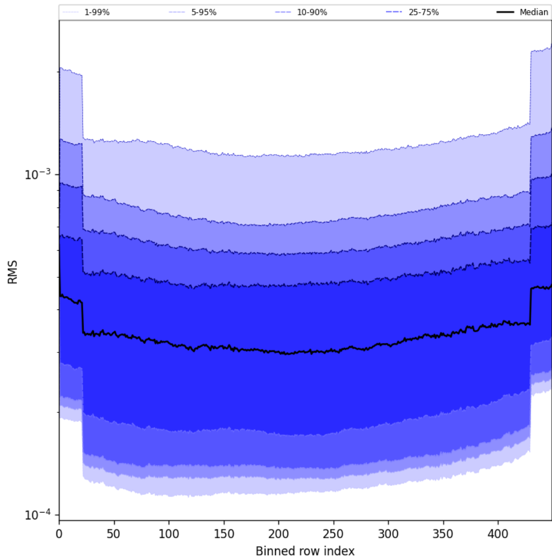
Figure 60: Along track statistics of “RMS” for 2025-05-28 to 2025-05-30
