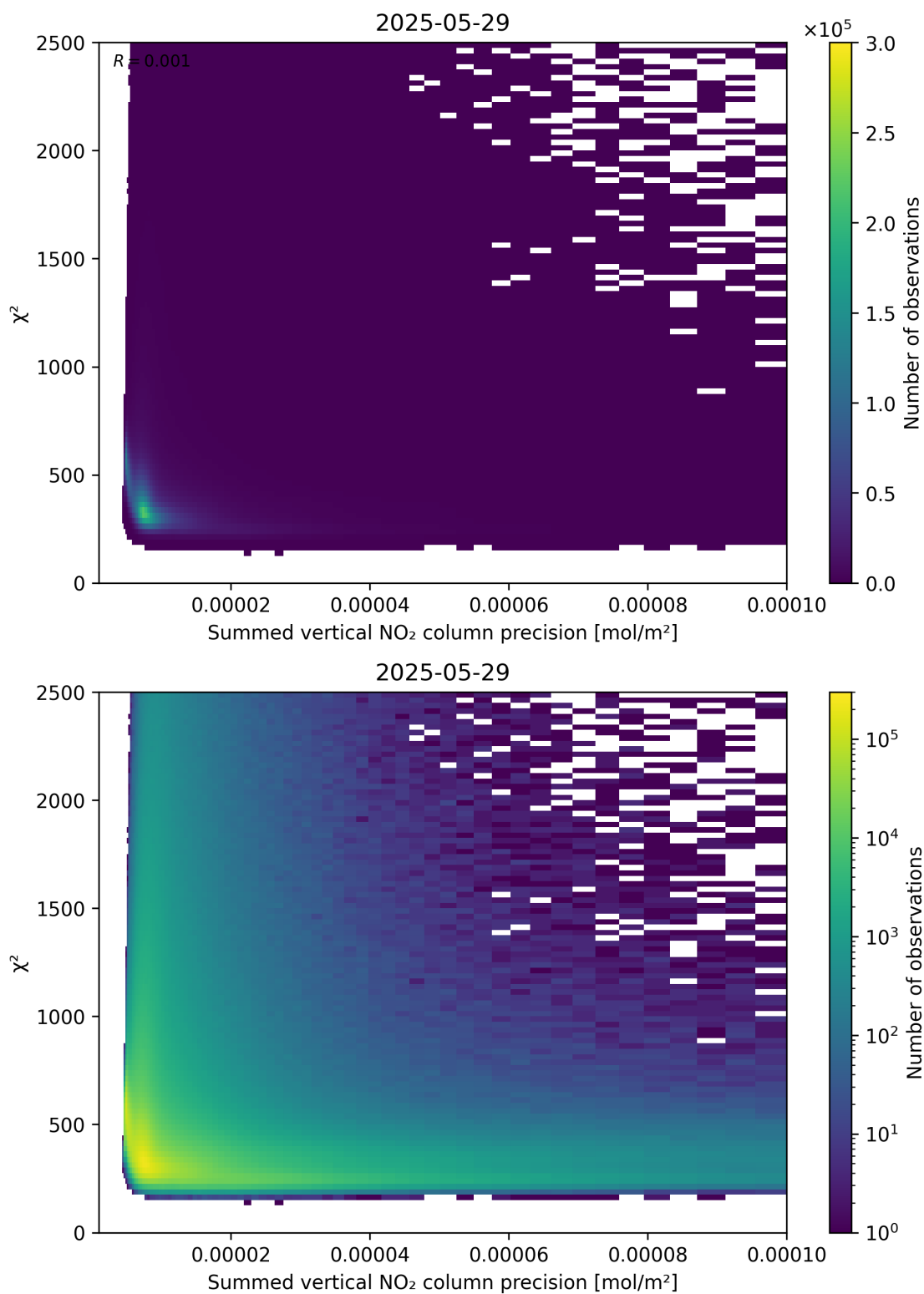
Figure 107: Scatter density plot of “Summed vertical NO 2 column precision” against “ \chi^2 ” for 2025-05-28 to 2025-05-30.
