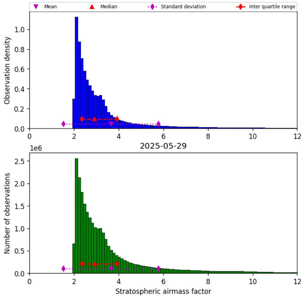
Figure 44: Histogram of “Stratospheric airmass factor” for 2025-05-28 to 2025-05-30
