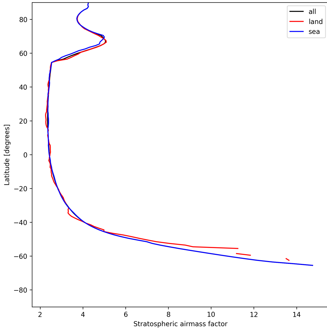
Figure 27: Zonal average of “Stratospheric air mass factor” for 2025-05-28 to 2025-05-30.
