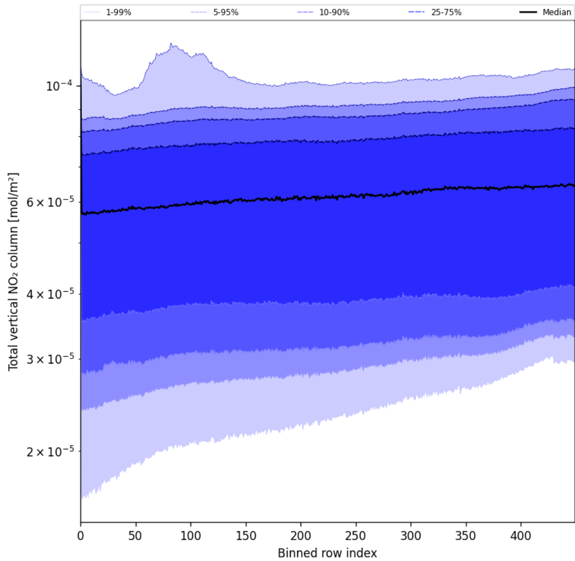
Figure 55: Along track statistics of “Total vertical NO 2 column” for 2025-05-28 to 2025-05-30
