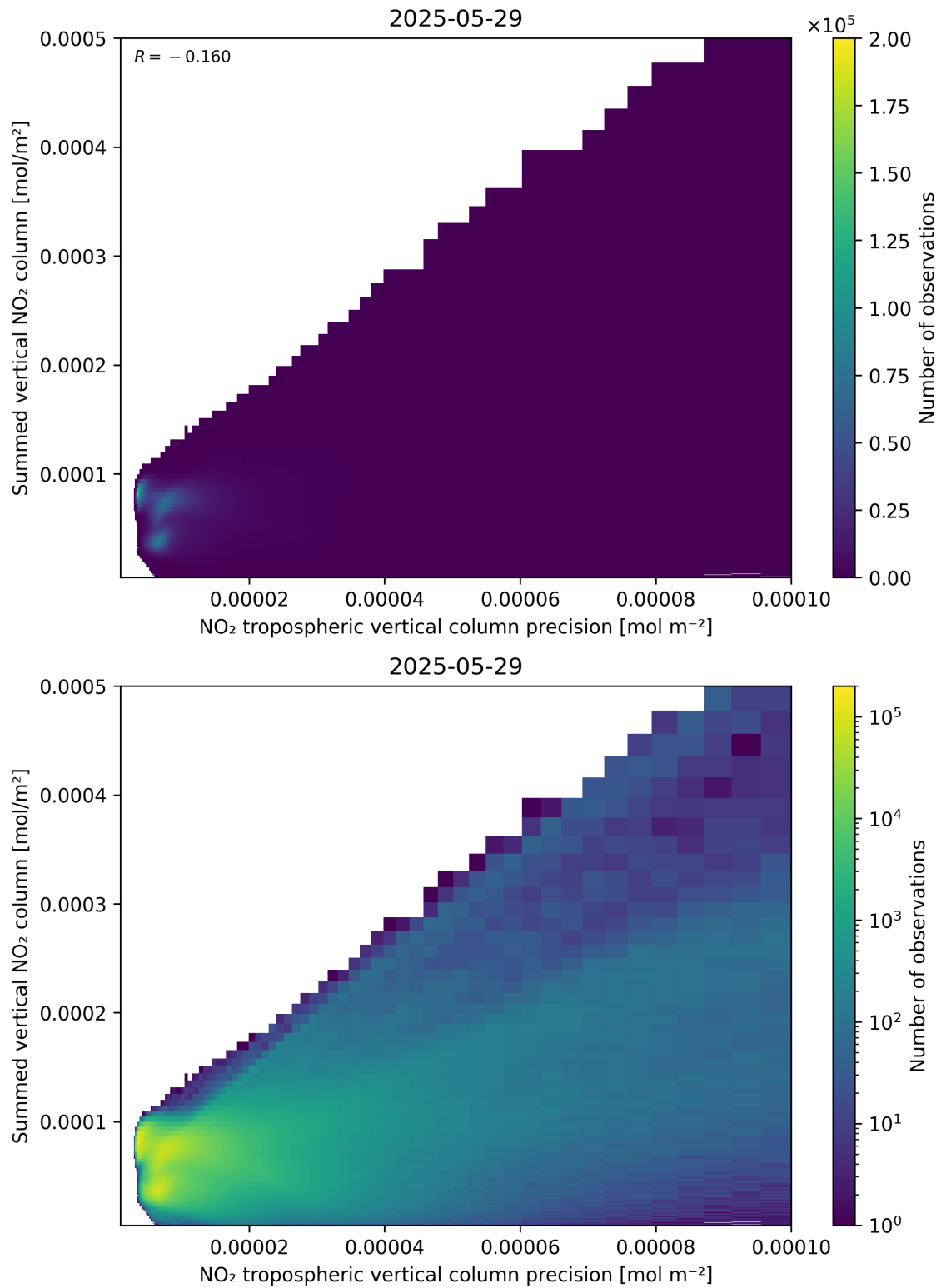
Figure 136: Scatter density plot of “NO 2 tropospheric vertical column precision” against “Summed vertical NO 2 column” for 2025-05-28 to 2025-05-30.
