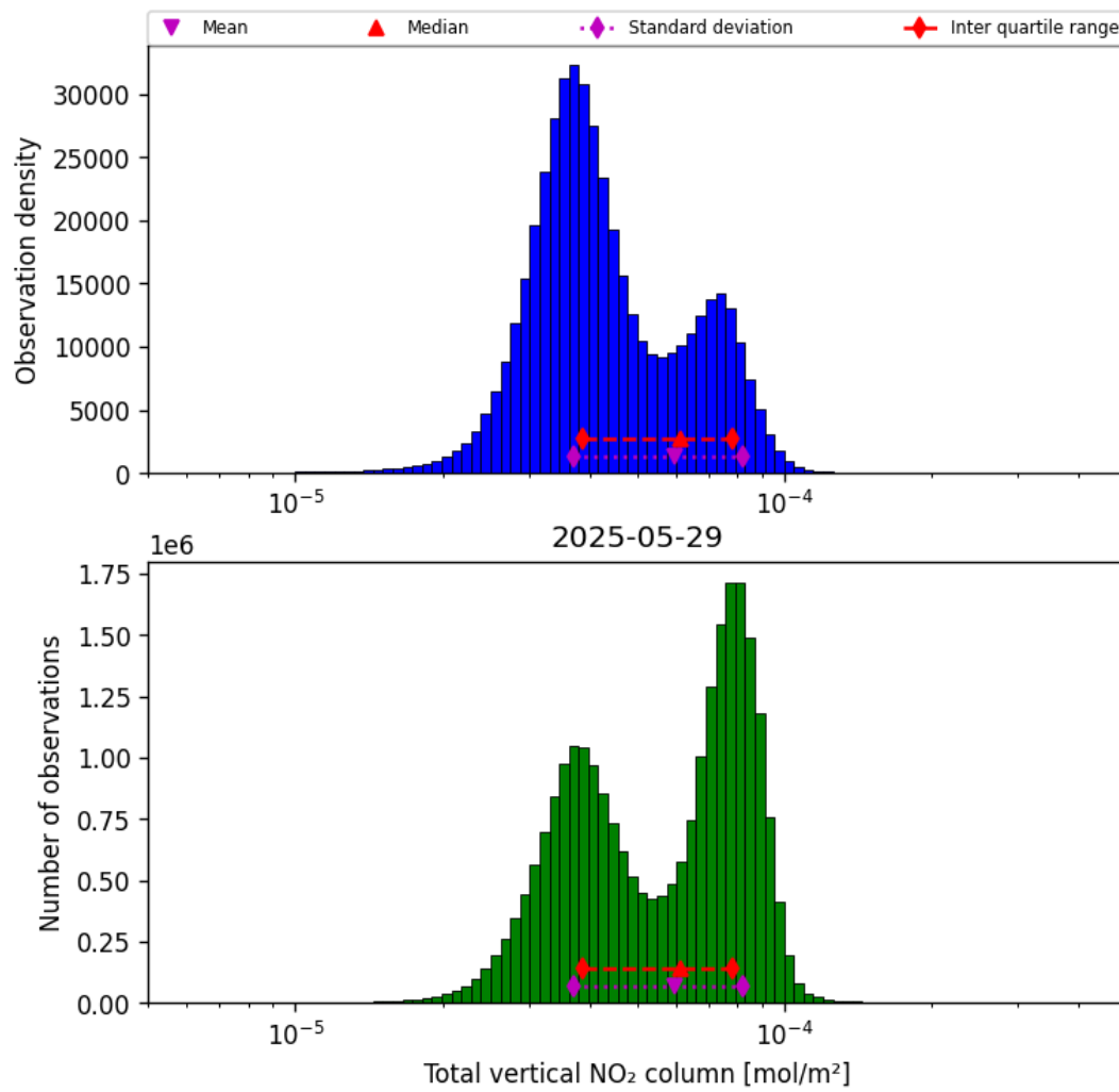
Figure 38: Histogram of “Total vertical NO 2 column” for 2025-05-28 to 2025-05-30
