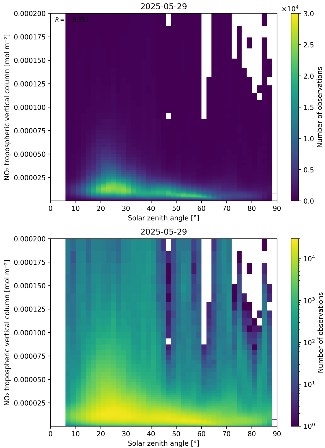
Figure 155: Scatter density plot of “Solar zenith angle” against “NO 2 tropospheric vertical column” for 2025-05-28 to 2025-05-30.
