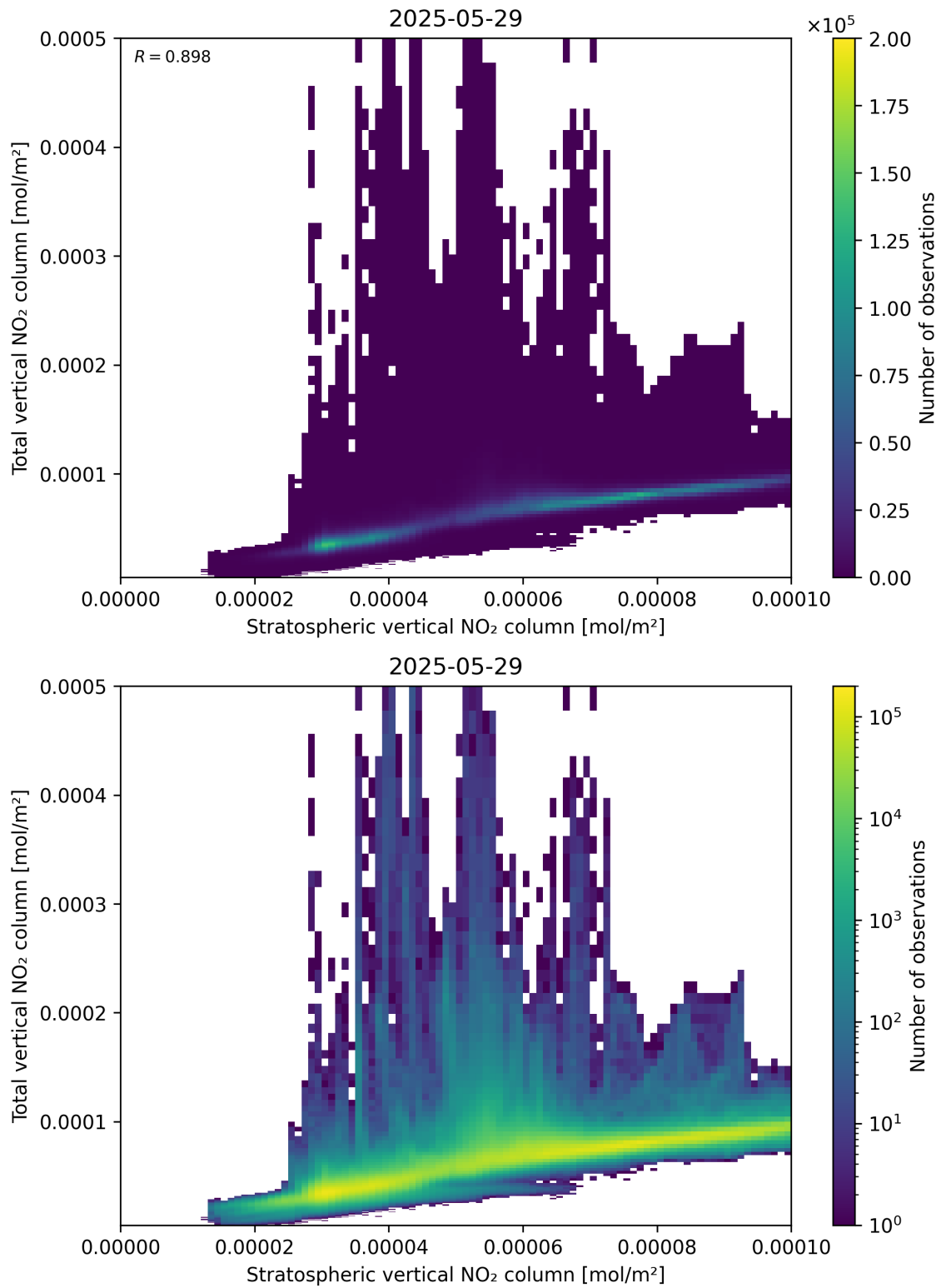
Figure 100: Scatter density plot of “Stratospheric vertical NO 2 column” against “Total vertical NO 2 column” for 2025-05-28 to 2025-05-30.
