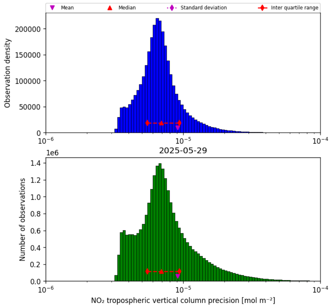
Figure 30: Histogram of “NO 2 tropospheric vertical column precision” for 2025-05-28 to 2025-05-30
