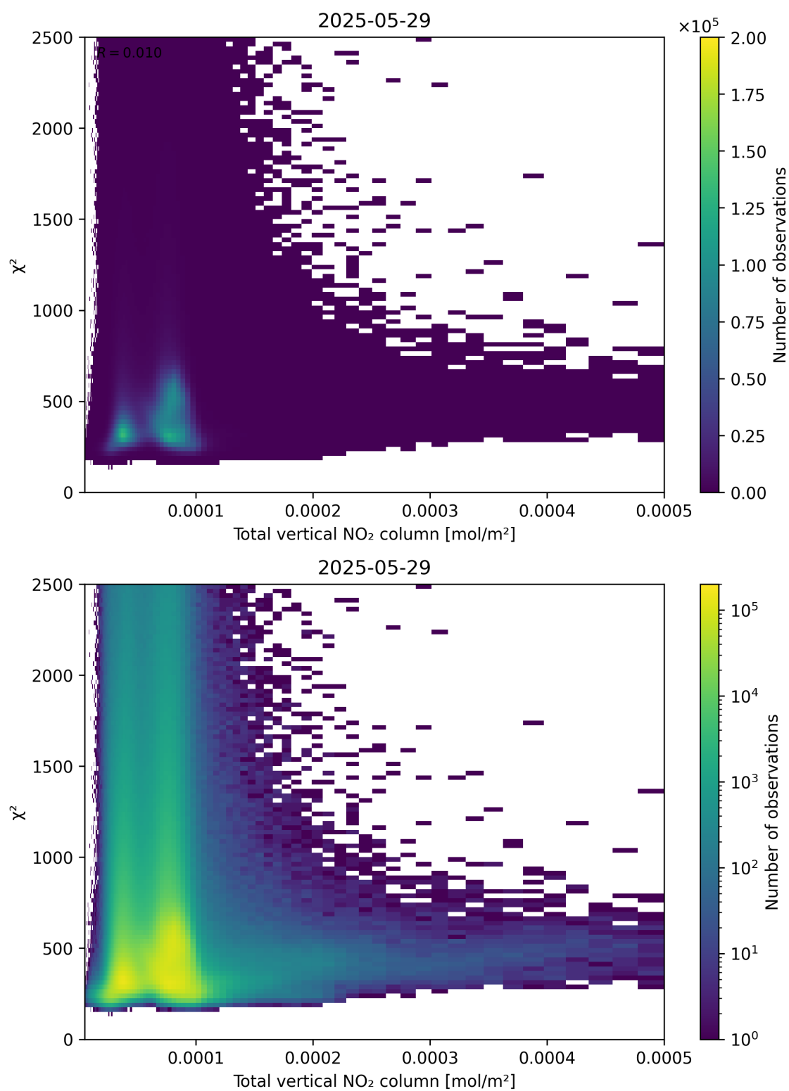
Figure 111: Scatter density plot of “Total vertical NO 2 column” against “ \chi^2 ” for 2025-05-28 to 2025-05-30.
