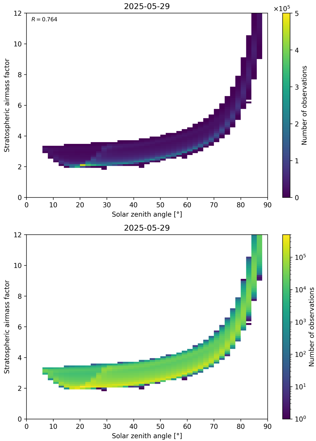
Figure 145: Scatter density plot of “Solar zenith angle” against “Stratospheric airmass factor” for 2025-05-28 to 2025-05-30.
