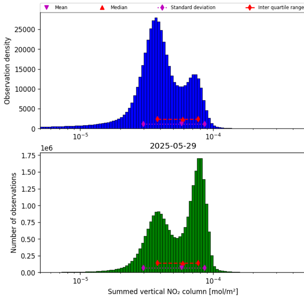
Figure 40: Histogram of “Summed vertical NO 2 column” for 2025-05-28 to 2025-05-30
