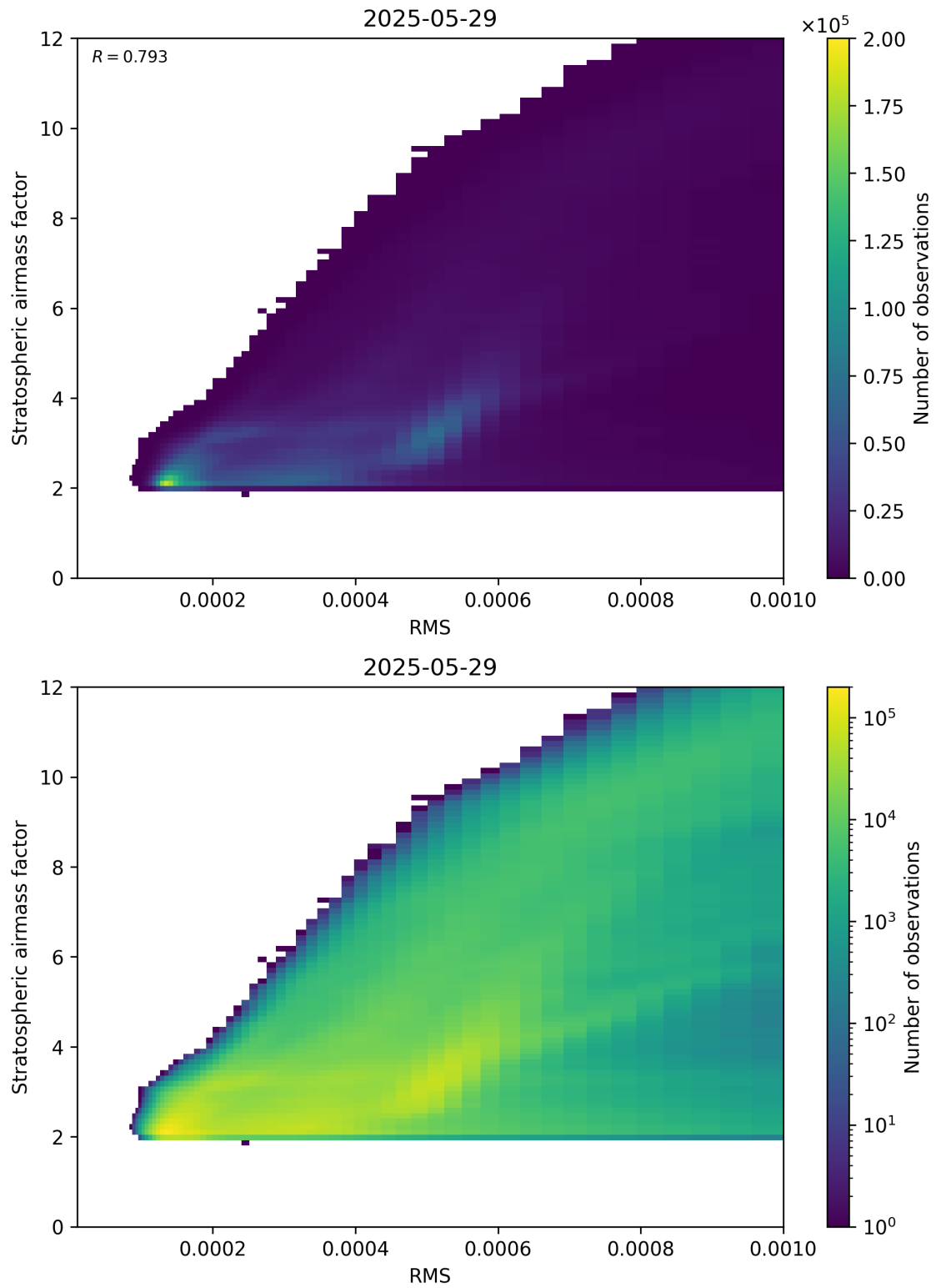
Figure 144: Scatter density plot of “RMS” against “Stratospheric airmass factor” for 2025-05-28 to 2025-05-30.
