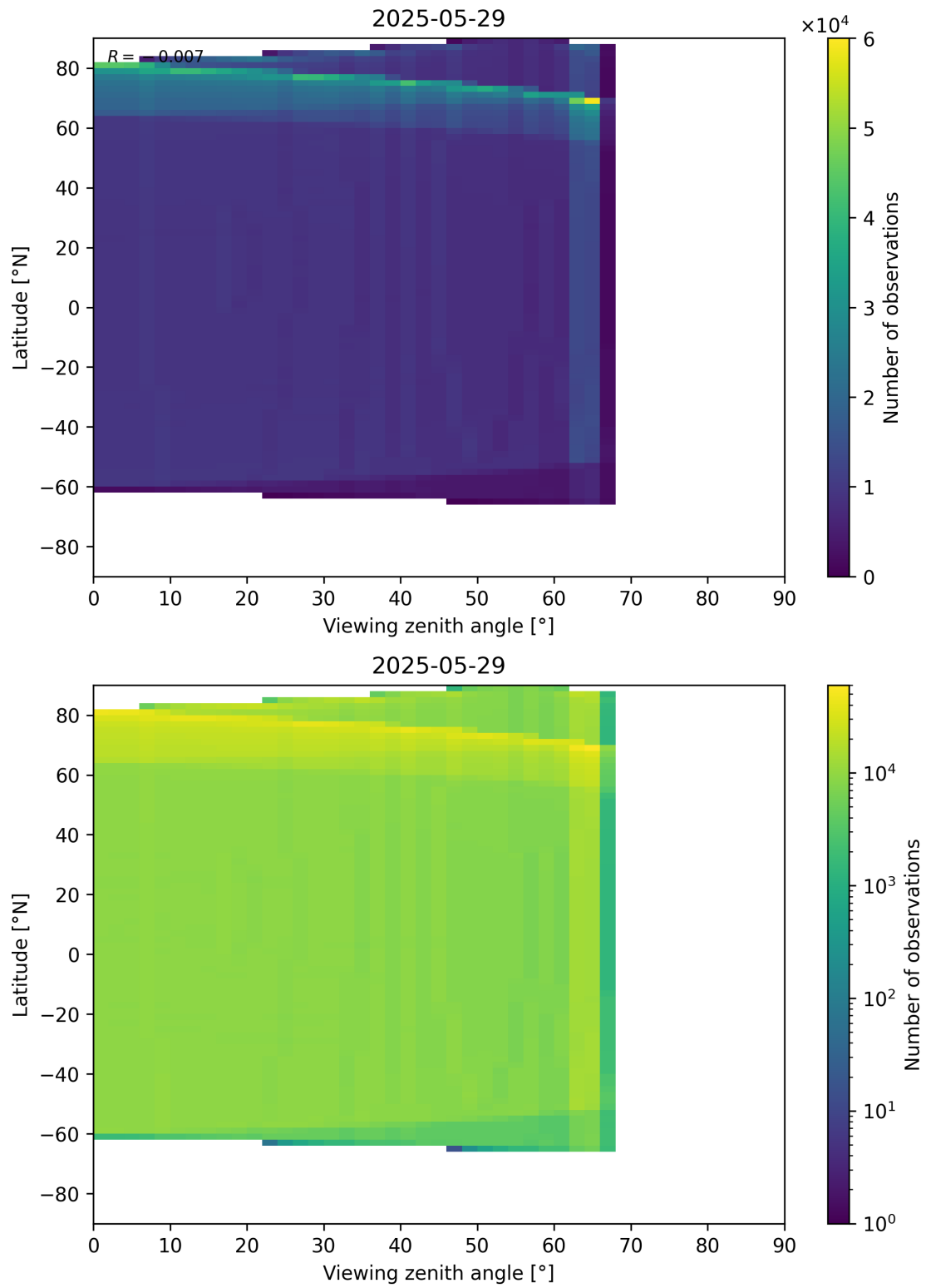
Figure 163: Scatter density plot of “Viewing zenith angle” against “Latitude” for 2025-05-28 to 2025-05-30.
