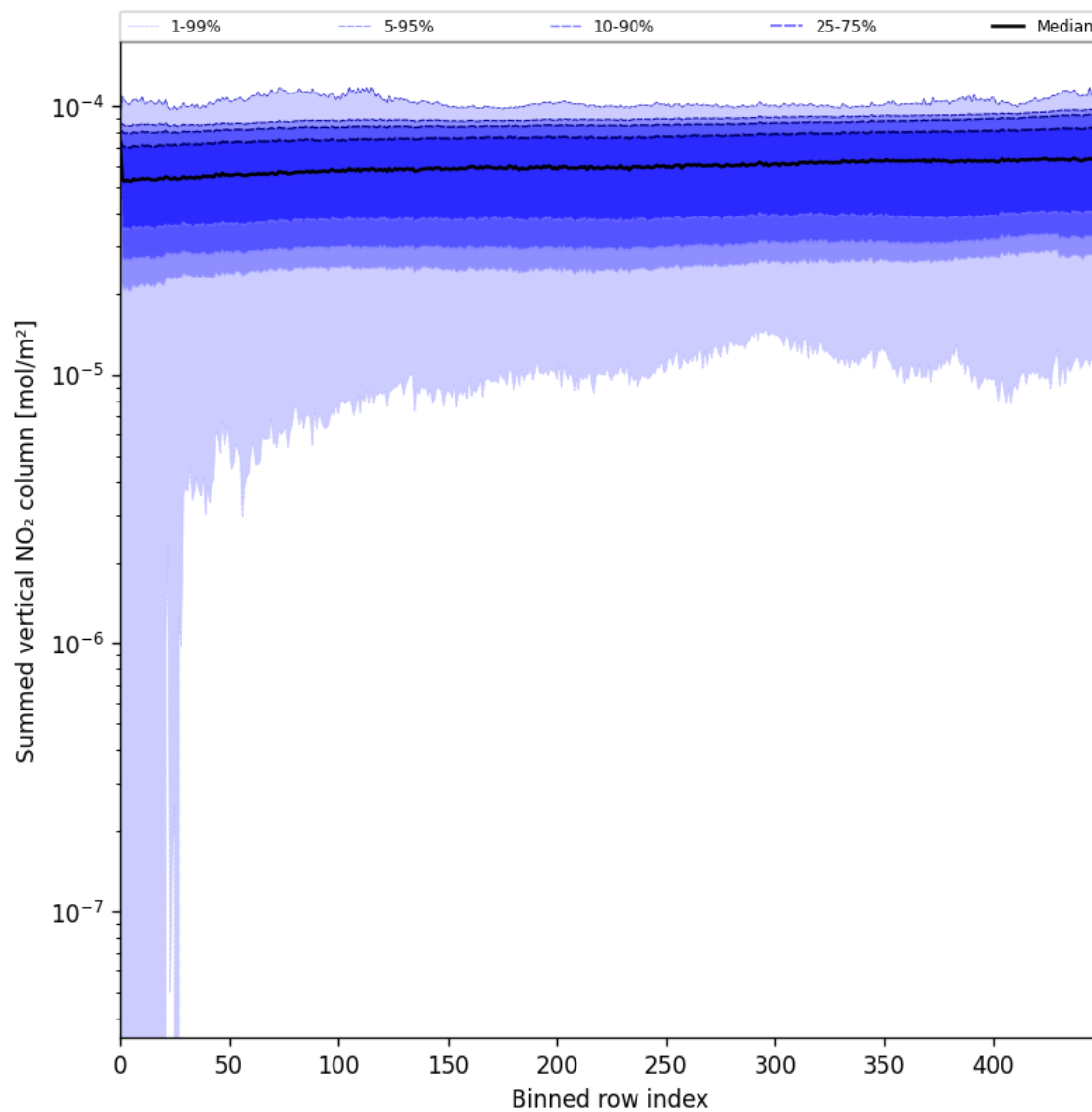
Figure 57: Along track statistics of “Summed vertical NO 2 column” for 2025-05-28 to 2025-05-30
