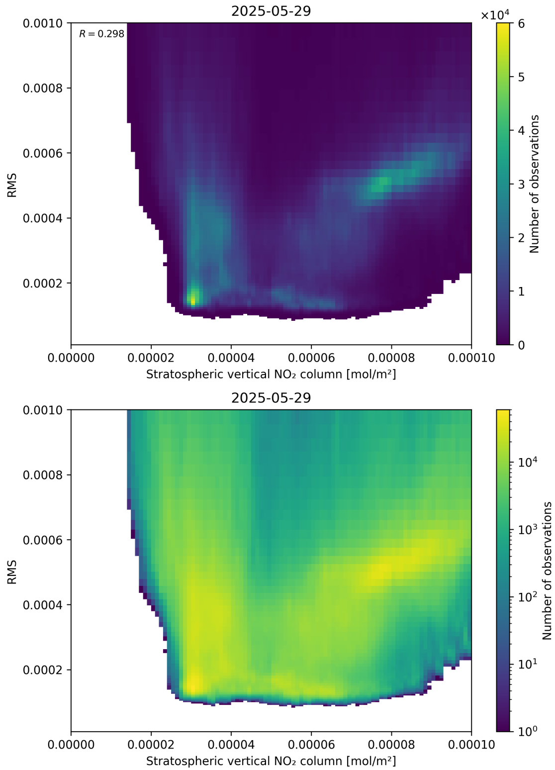
Figure 102: Scatter density plot of “Stratospheric vertical NO 2 column” against “RMS” for 2025-05-28 to 2025-05-30.
