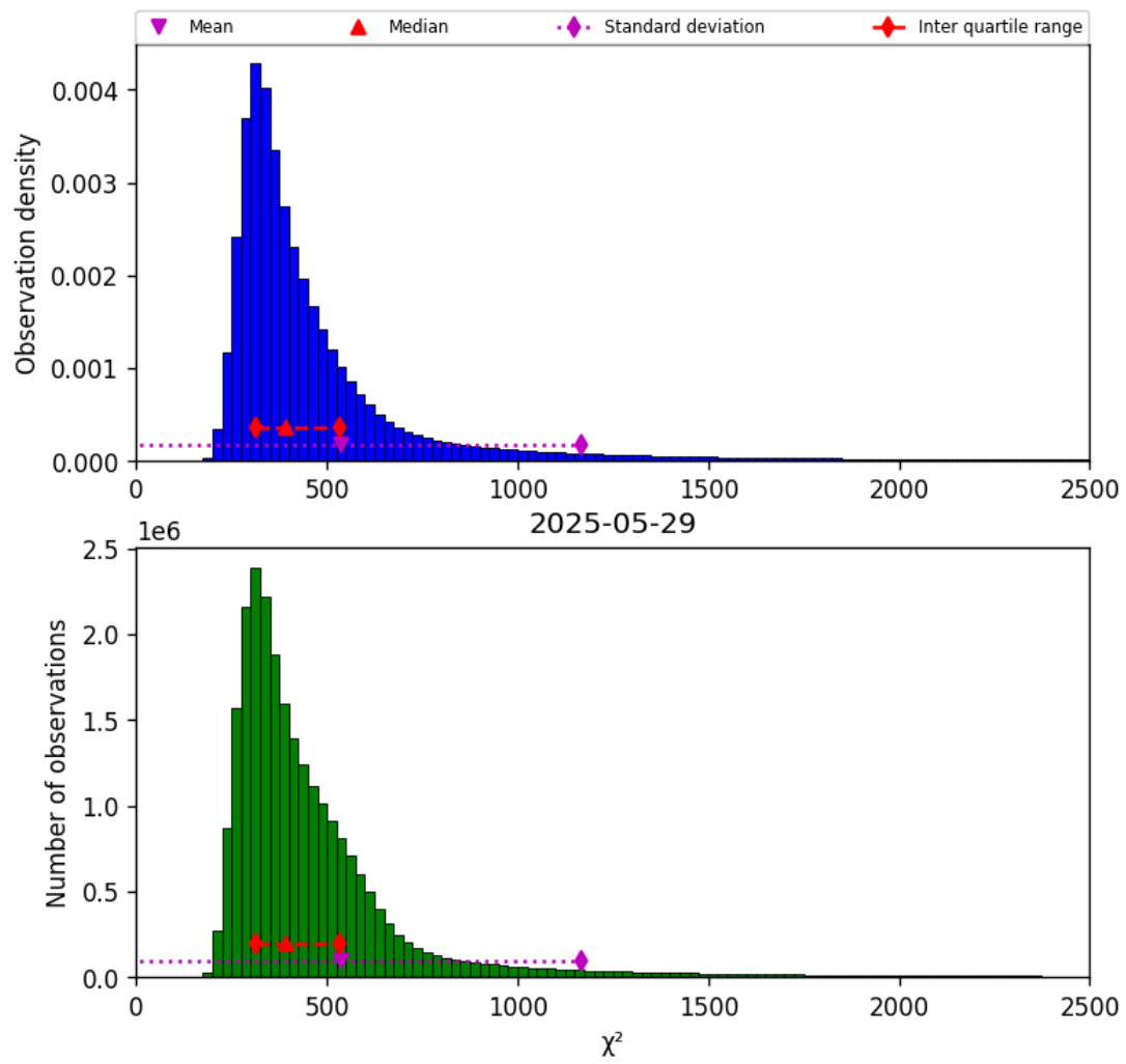
Figure 42: Histogram of “ \chi^2 ” for 2025-05-28 to 2025-05-30
