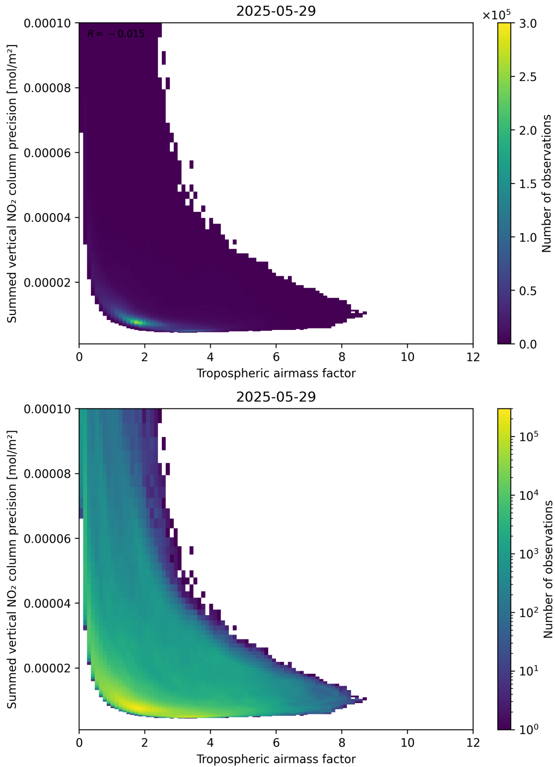
Figure 76: Scatter density plot of “Tropospheric air mass factor” against “Summed vertical NO 2 column precision” for 2025-05-28 to 2025-05-30.
