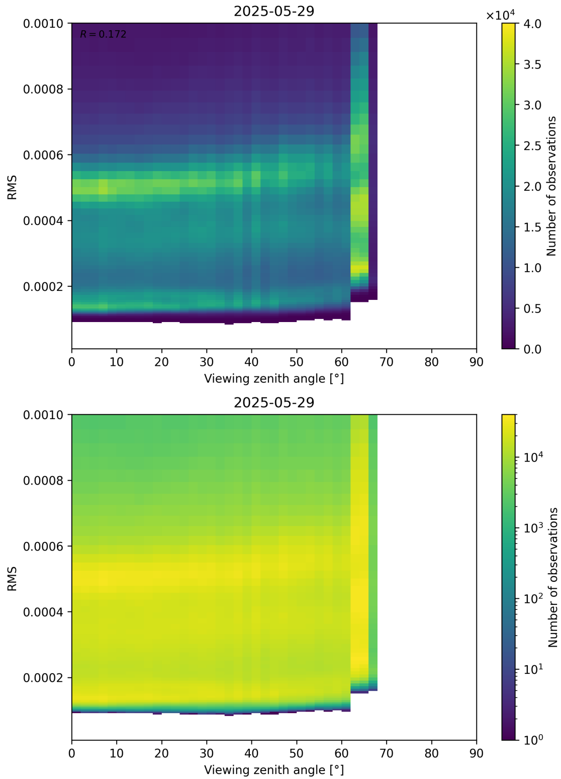
Figure 171: Scatter density plot of “Viewing zenith angle” against “RMS” for 2025-05-28 to 2025-05-30.
