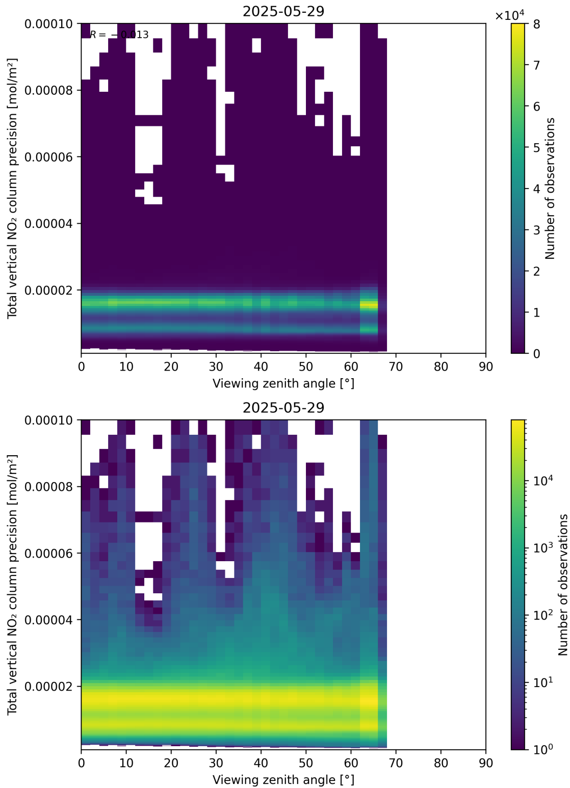
Figure 168: Scatter density plot of “Viewing zenith angle” against “Total vertical NO 2 column precision” for 2025-05-28 to 2025-05-30.
