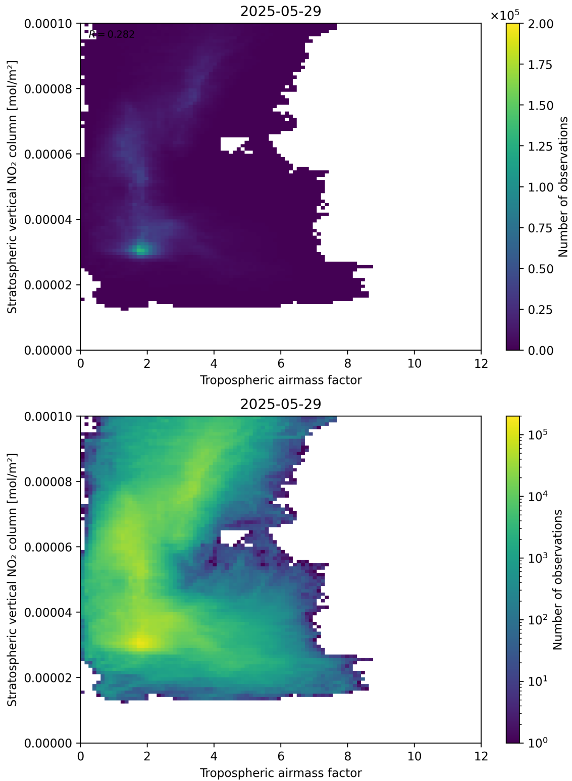
Figure 74: Scatter density plot of “Tropospheric air mass factor” against “Stratospheric vertical NO 2 column” for 2025-05-28 to 2025-05-30.
