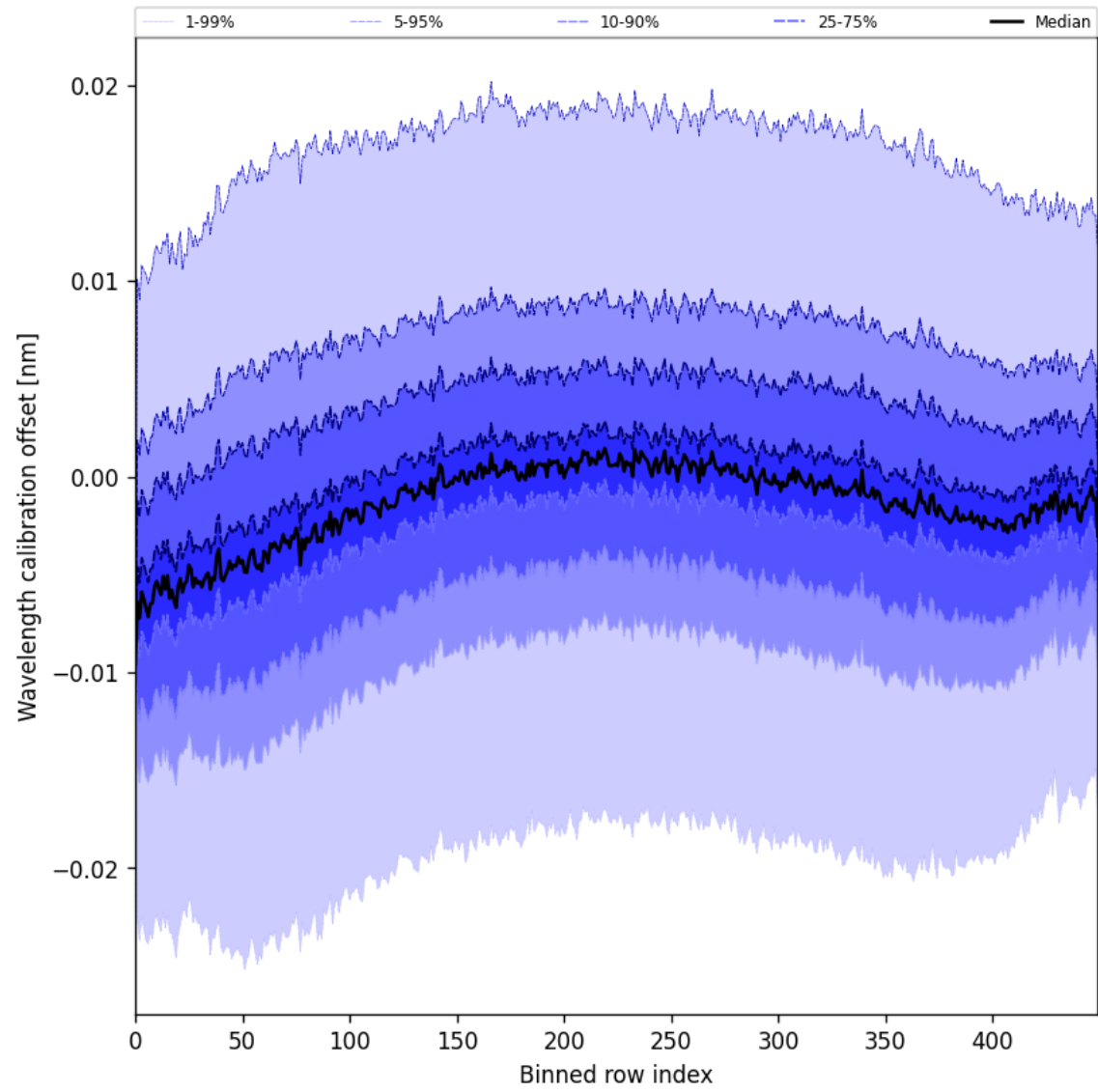
Figure 52: Along track statistics of “Wavelength calibration offset” for 2025-05-28 to 2025-05-30
