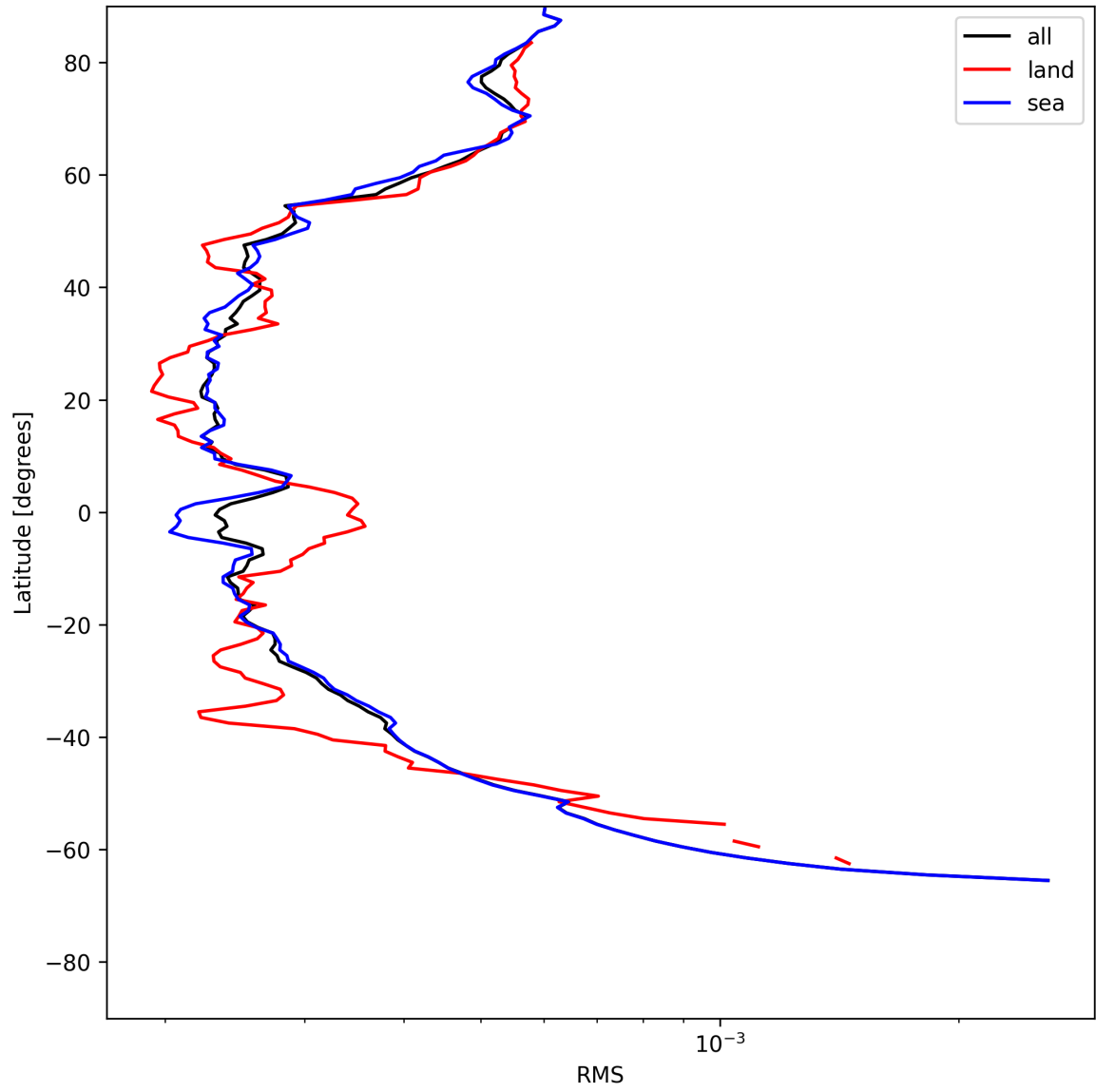
Figure 26: Zonal average of “RMS” for 2025-05-28 to 2025-05-30.
