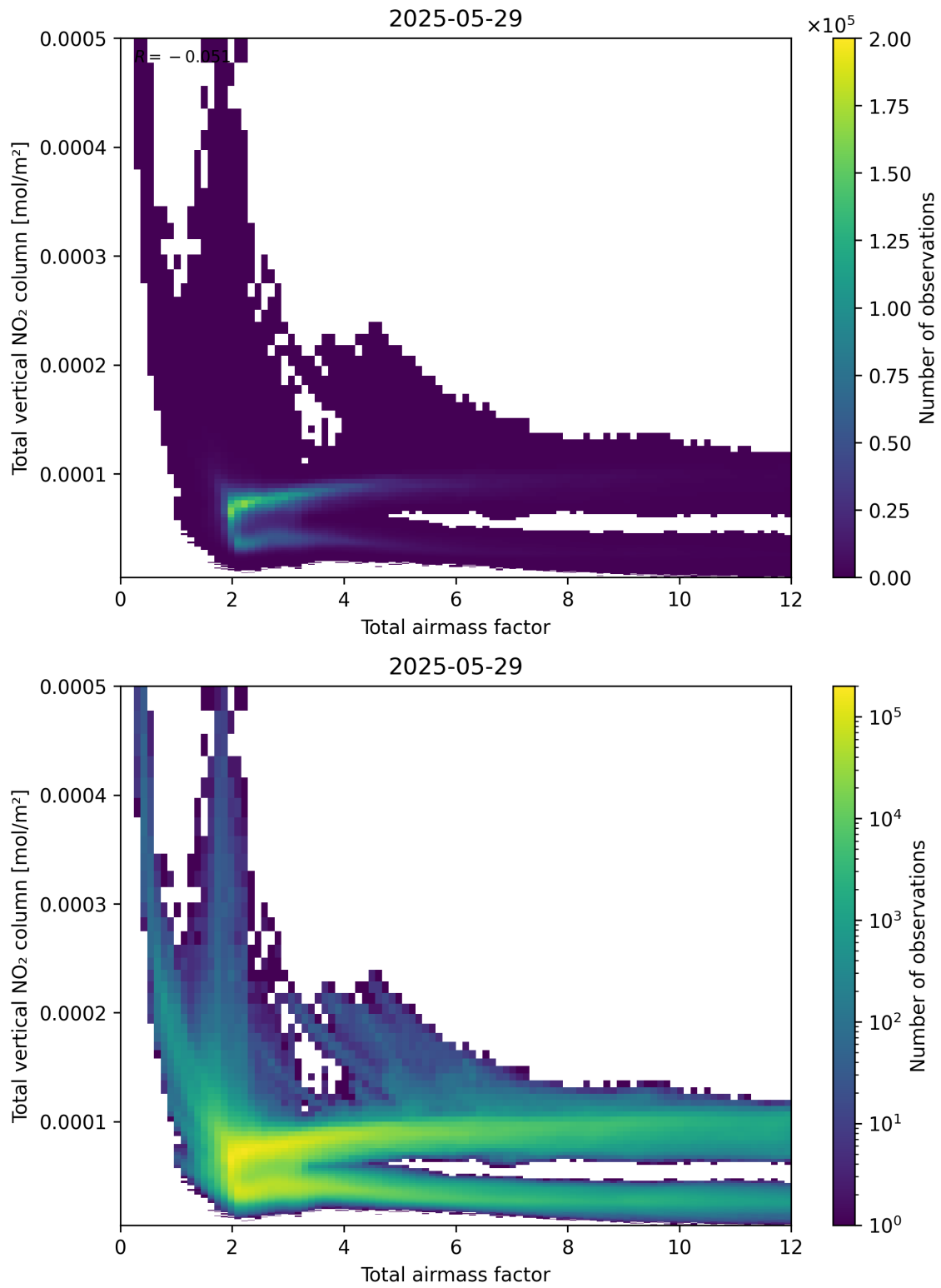
Figure 67: Scatter density plot of “Total airmass factor” against “Total vertical NO 2 column” for 2025-05-28 to 2025-05-30.
