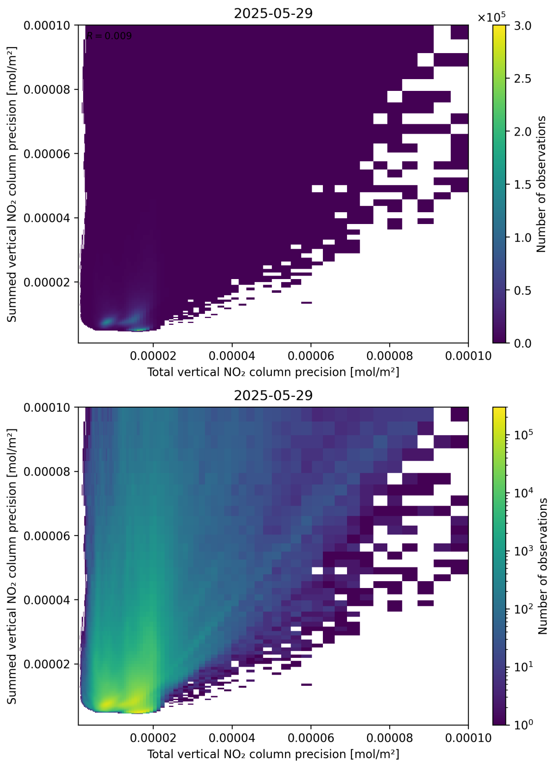
Figure 118: Scatter density plot of “Total vertical NO 2 column precision” against “Summed vertical NO 2 column precision” for 2025-05-28 to 2025-05-30.
