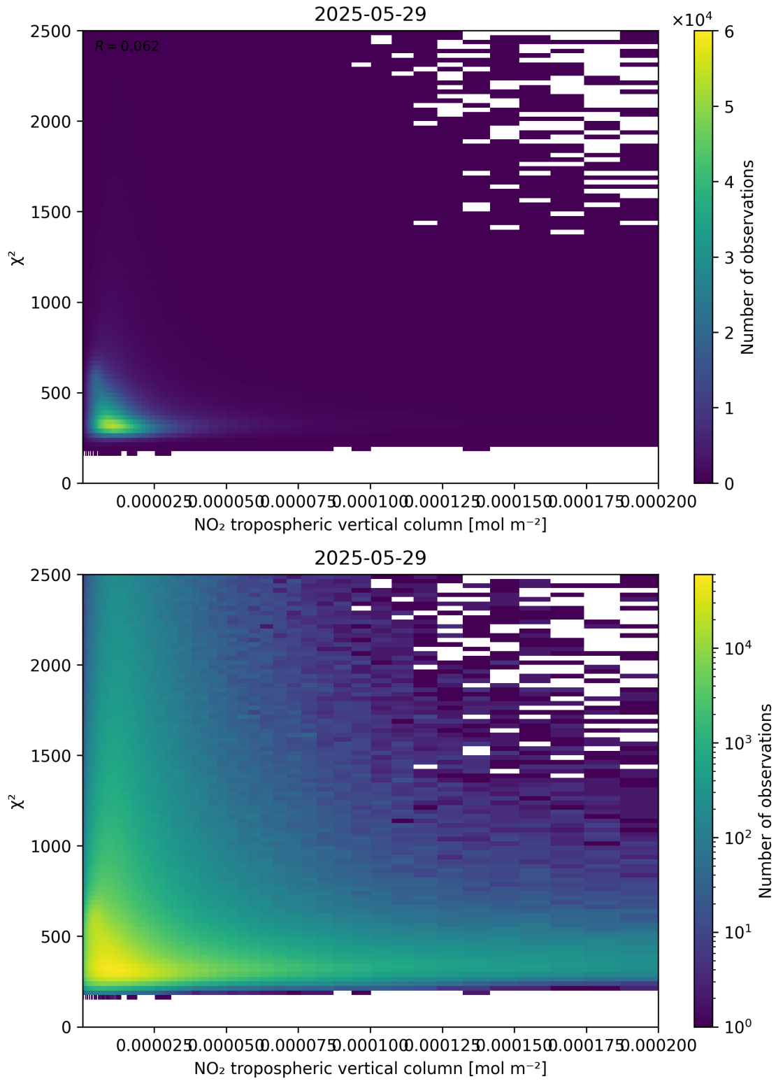
Figure 124: Scatter density plot of “NO 2 tropospheric vertical column” against “ \chi^2 ” for 2025-05-28 to 2025-05-30.
