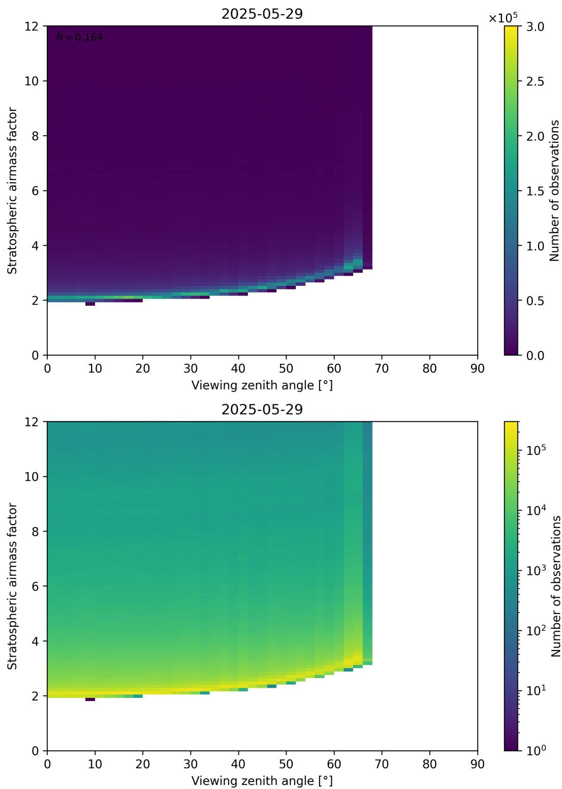
Figure 159: Scatter density plot of “Viewing zenith angle” against “Stratospheric airmass factor” for 2025-05-28 to 2025-05-30.
