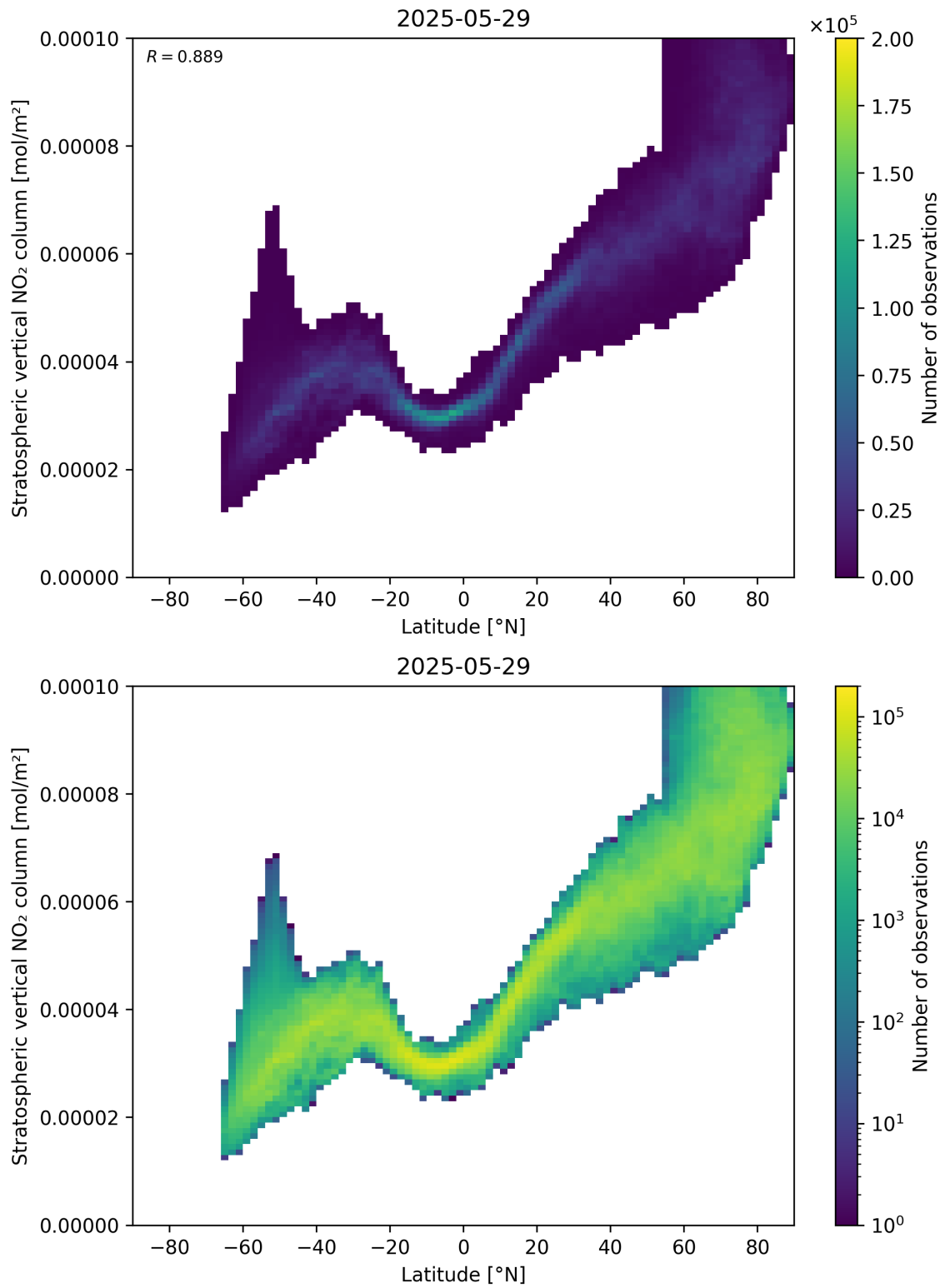
Figure 87: Scatter density plot of “Latitude” against “Stratospheric vertical \text{NO}_2 column” for 2025-05-28 to 2025-05-30.
