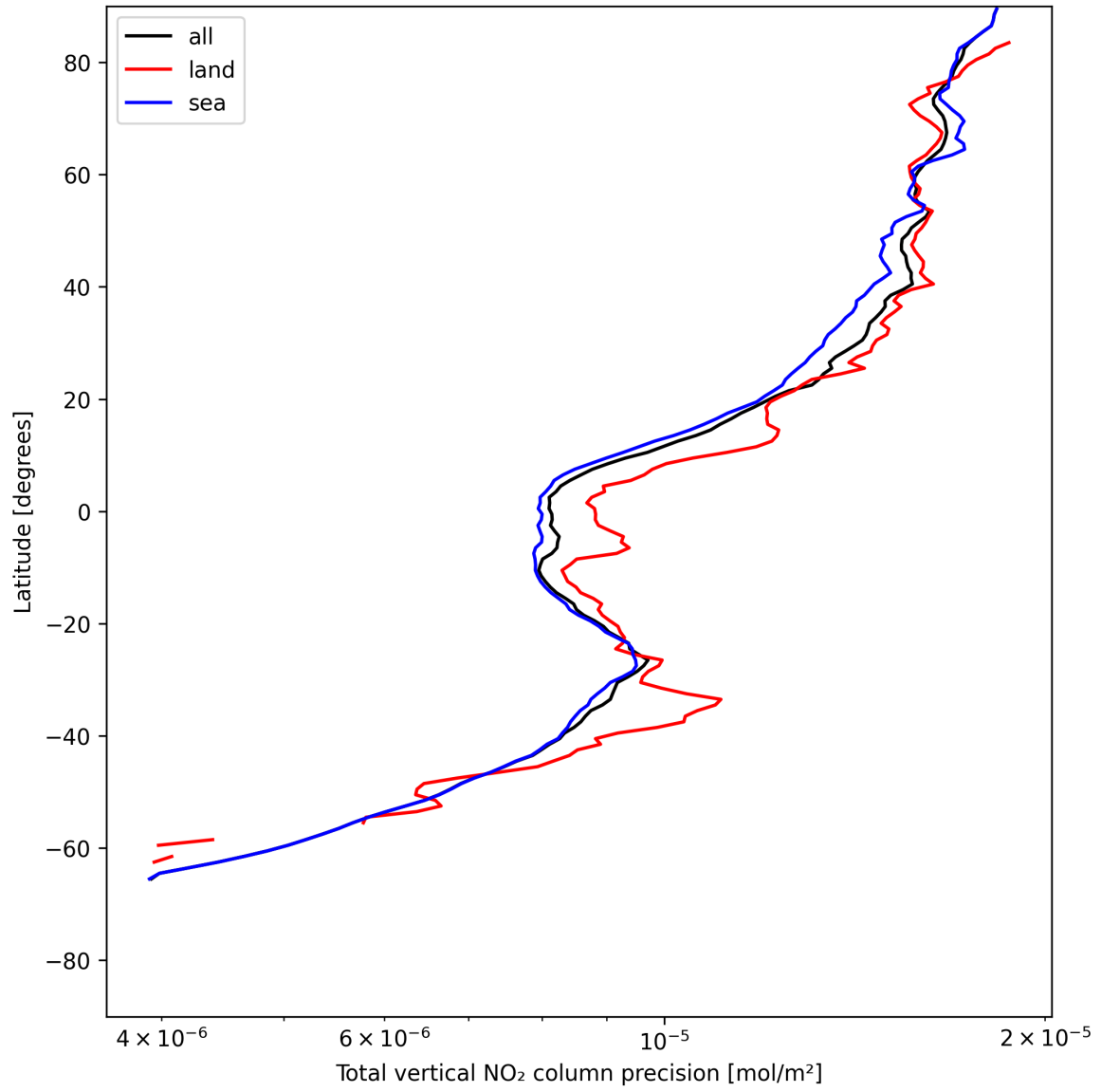
Figure 22: Zonal average of “Total vertical NO 2 column precision” for 2025-05-28 to 2025-05-30.
