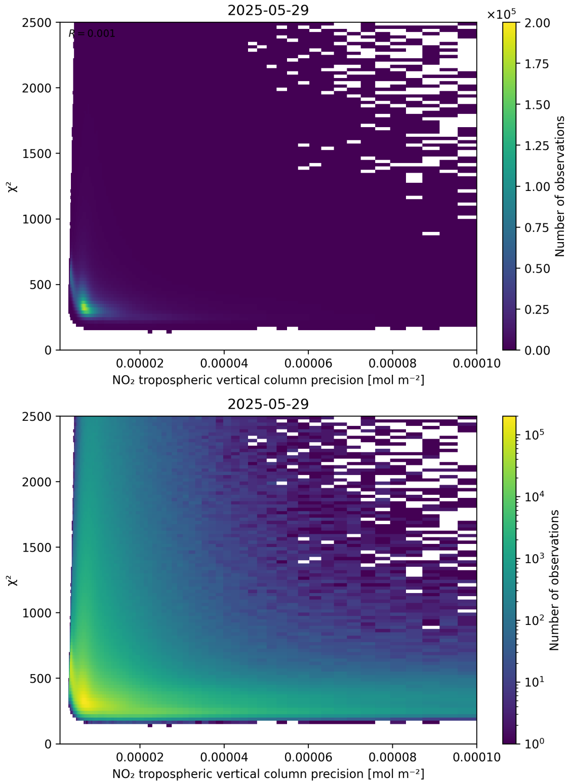
Figure 134: Scatter density plot of “NO 2 tropospheric vertical column precision” against “ \chi^2 ” for 2025-05-28 to 2025-05-30.
