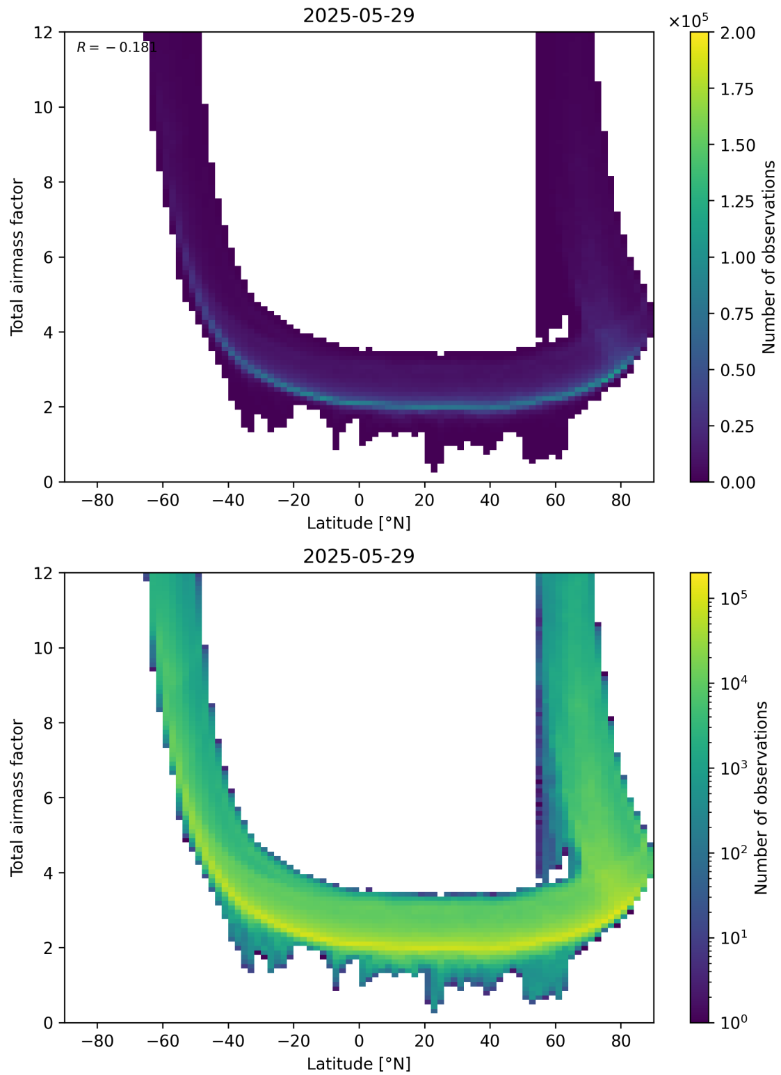
Figure 84: Scatter density plot of “Latitude” against “Total airmass factor” for 2025-05-28 to 2025-05-30.
