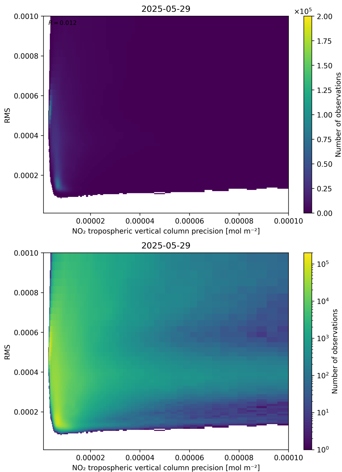
Figure 140: Scatter density plot of “NO 2 tropospheric vertical column precision” against “RMS” for 2025-05-28 to 2025-05-30.
