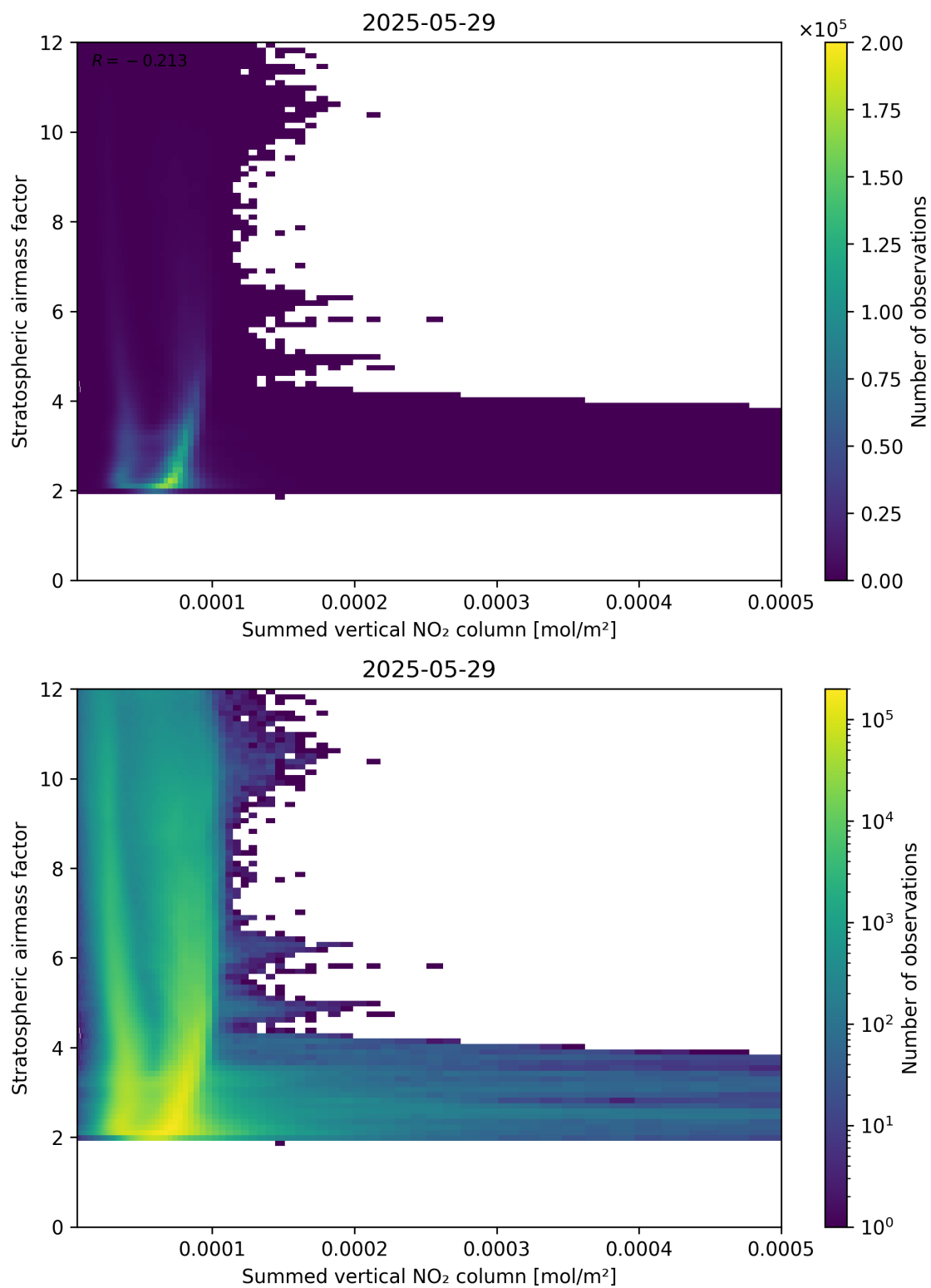
Figure 103: Scatter density plot of “Summed vertical NO 2 column” against “Stratospheric air mass factor” for 2025-05-28 to 2025-05-30.
