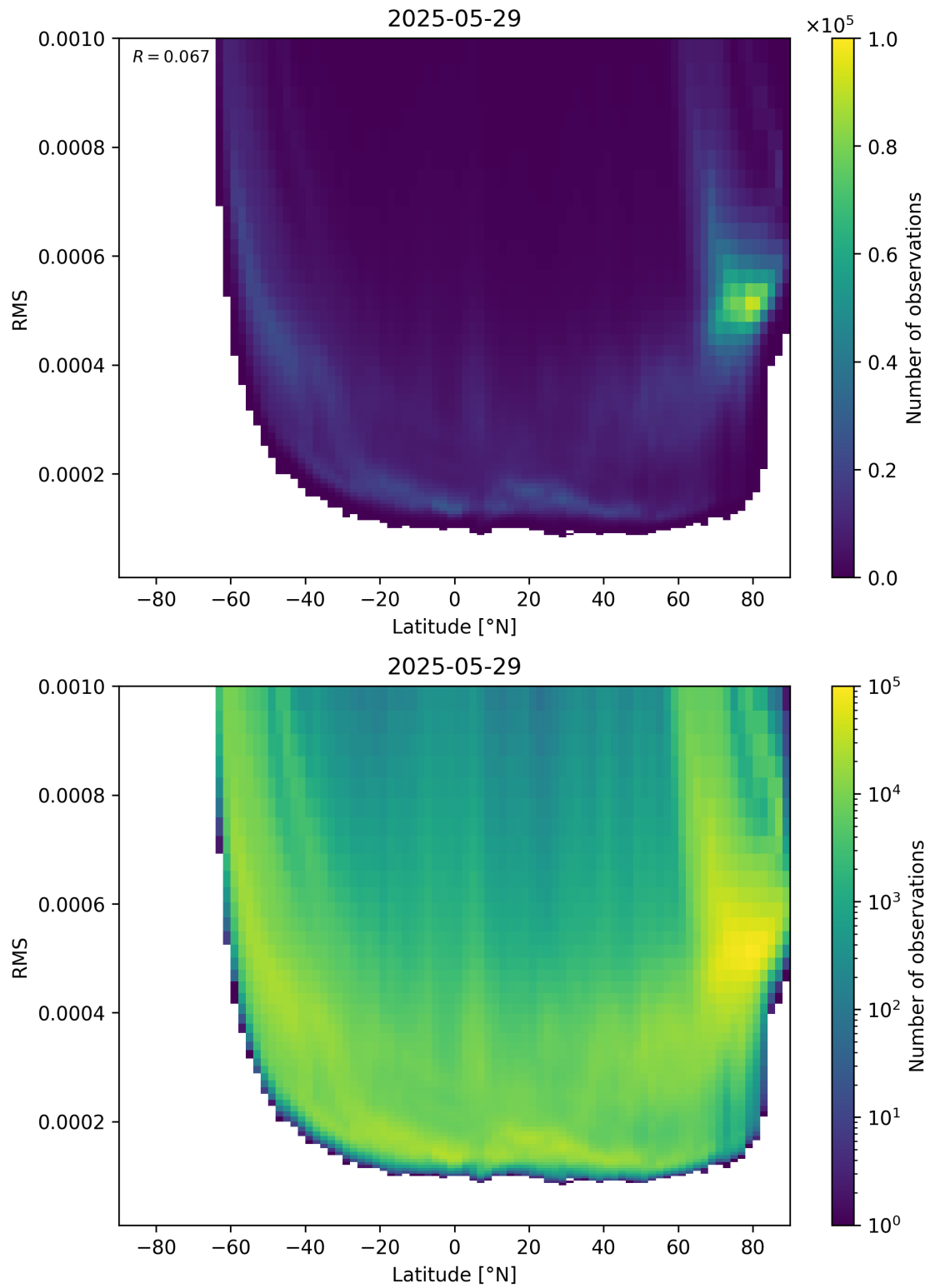
Figure 94: Scatter density plot of “Latitude” against “RMS” for 2025-05-28 to 2025-05-30.
