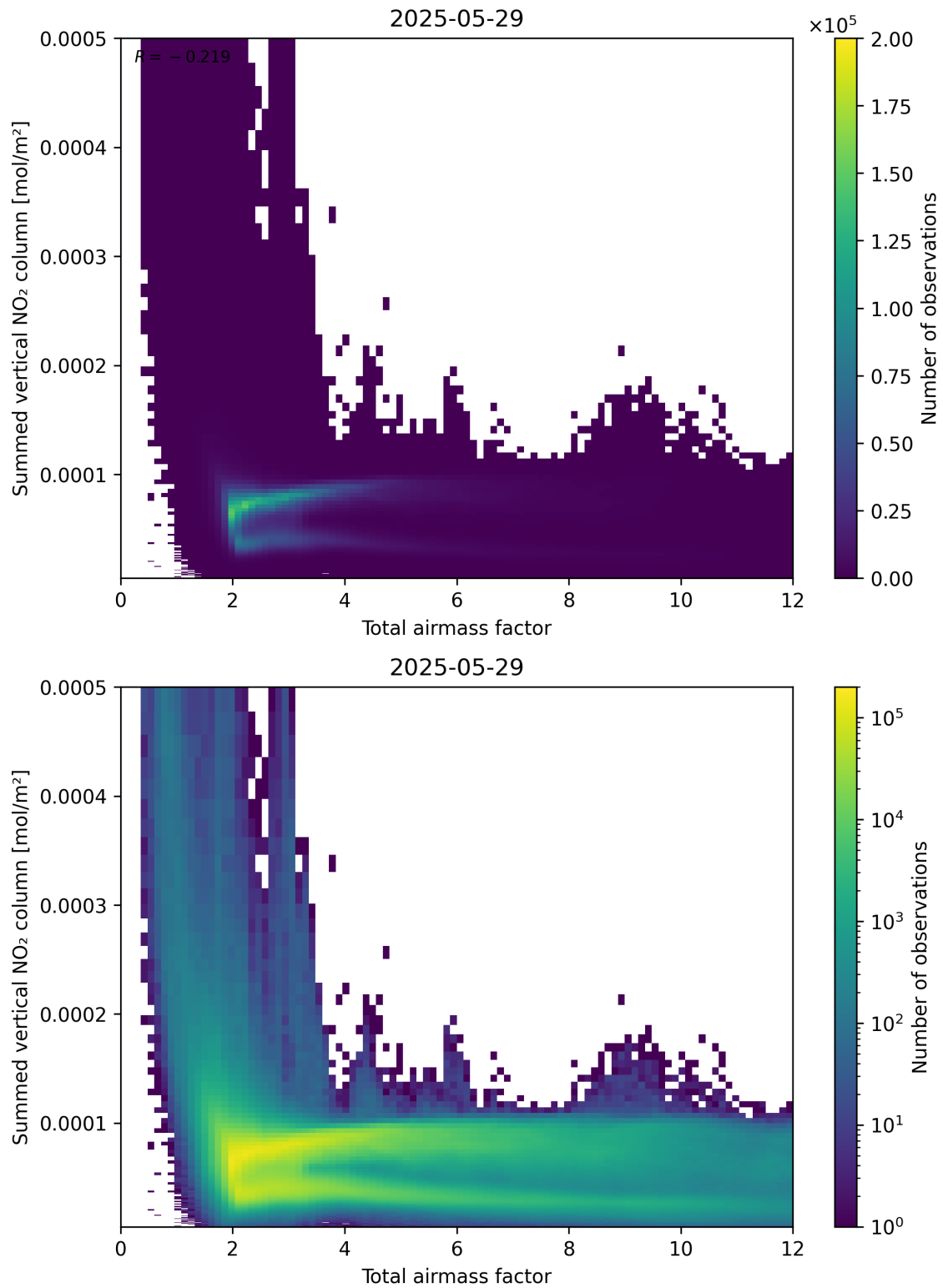
Figure 65: Scatter density plot of “Total airmass factor” against “Summed vertical NO 2 column” for 2025-05-28 to 2025-05-30.
