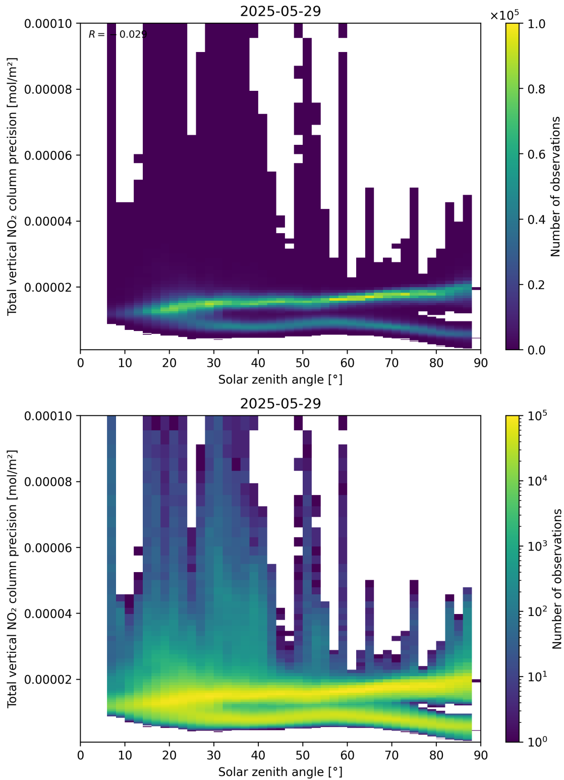
Figure 154: Scatter density plot of “Solar zenith angle” against “Total vertical NO 2 column precision” for 2025-05-28 to 2025-05-30.
