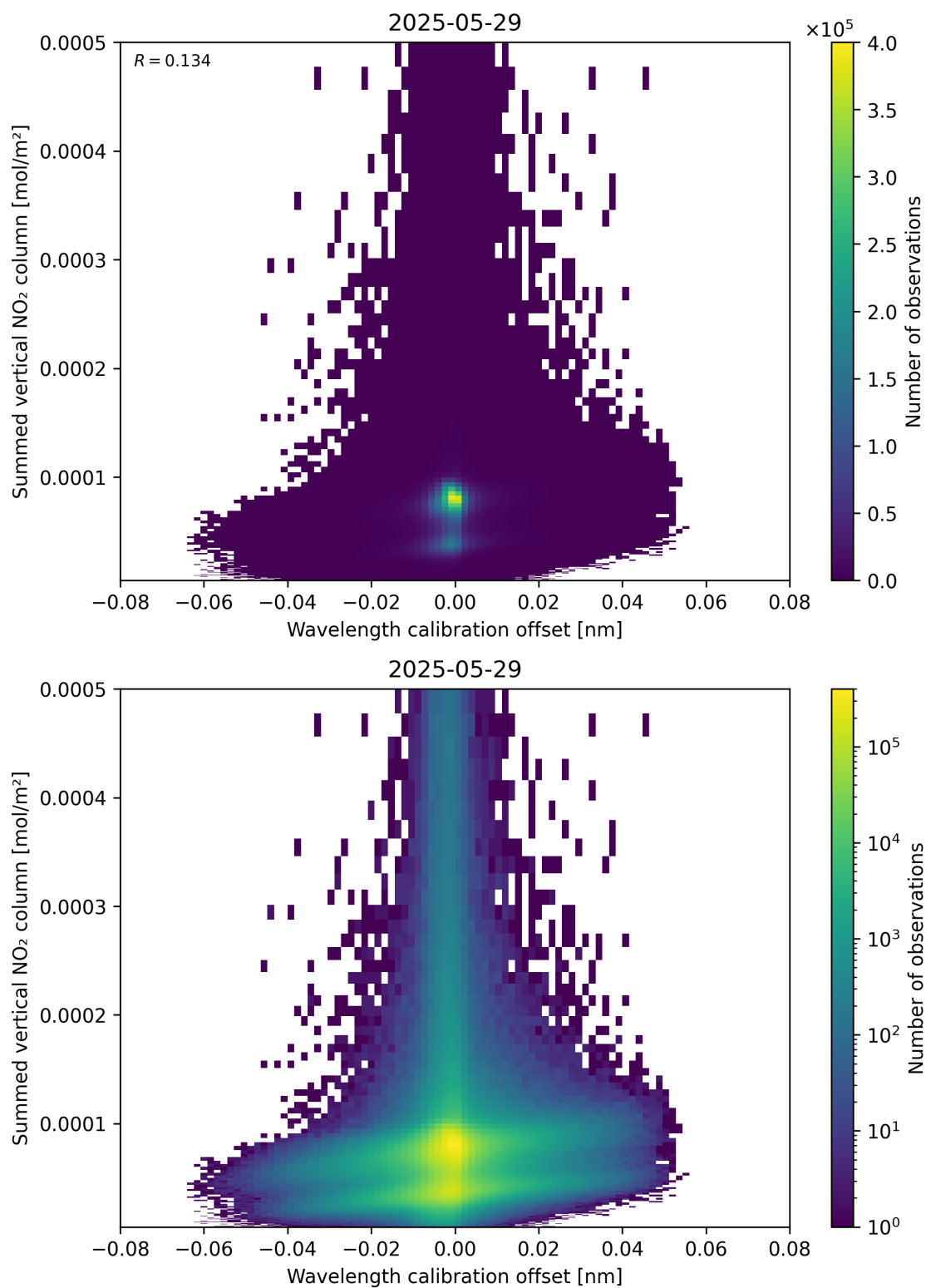
Figure 177: Scatter density plot of “Wavelength calibration offset” against “Summed vertical NO 2 column” for 2025-05-28 to 2025-05-30.
