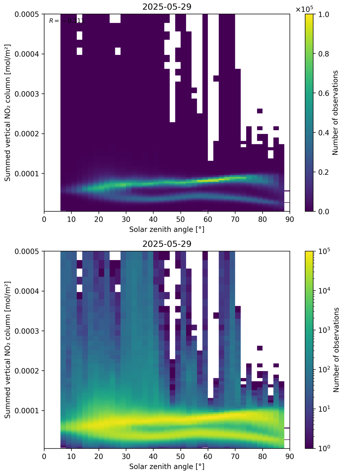
Figure 151: Scatter density plot of “Solar zenith angle” against “Summed vertical NO 2 column” for 2025-05-28 to 2025-05-30.
