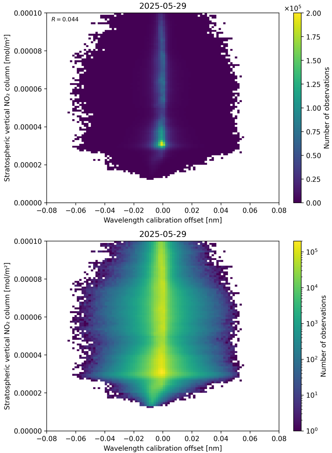
Figure 176: Scatter density plot of “Wavelength calibration offset” against “Stratospheric vertical NO 2 column” for 2025-05-28 to 2025-05-30.
