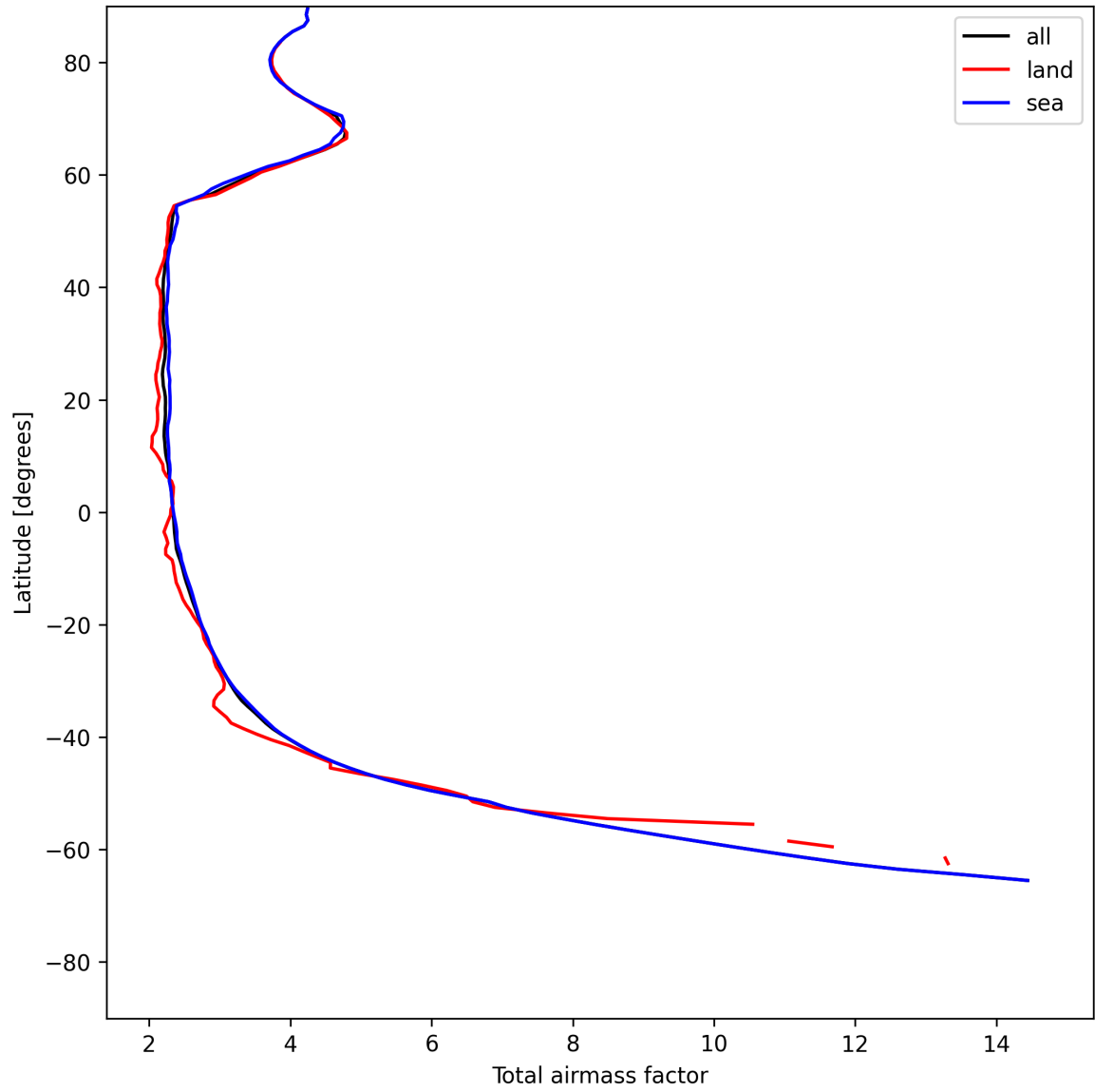
Figure 15: Zonal average of “Total airmass factor” for 2025-05-28 to 2025-05-30.
