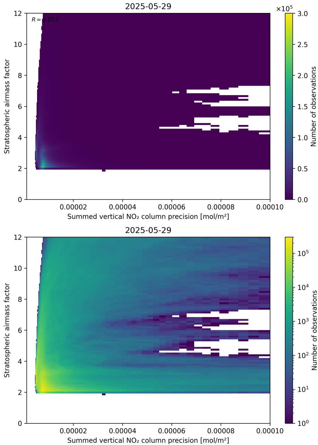
Figure 106: Scatter density plot of “Summed vertical NO 2 column precision” against “Stratospheric airmass factor” for 2025-05-28 to 2025-05-30.
