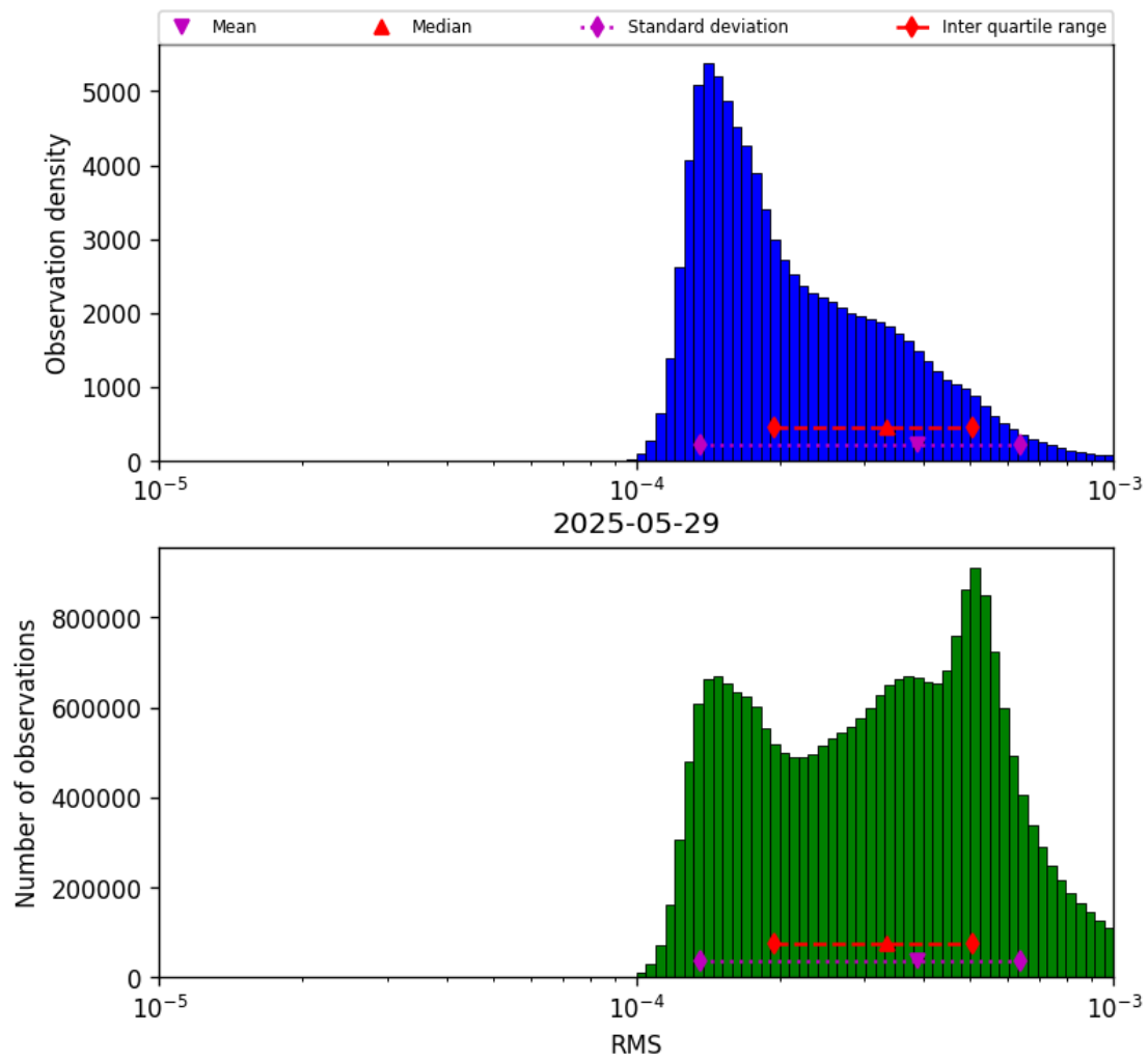
Figure 43: Histogram of “RMS” for 2025-05-28 to 2025-05-30
