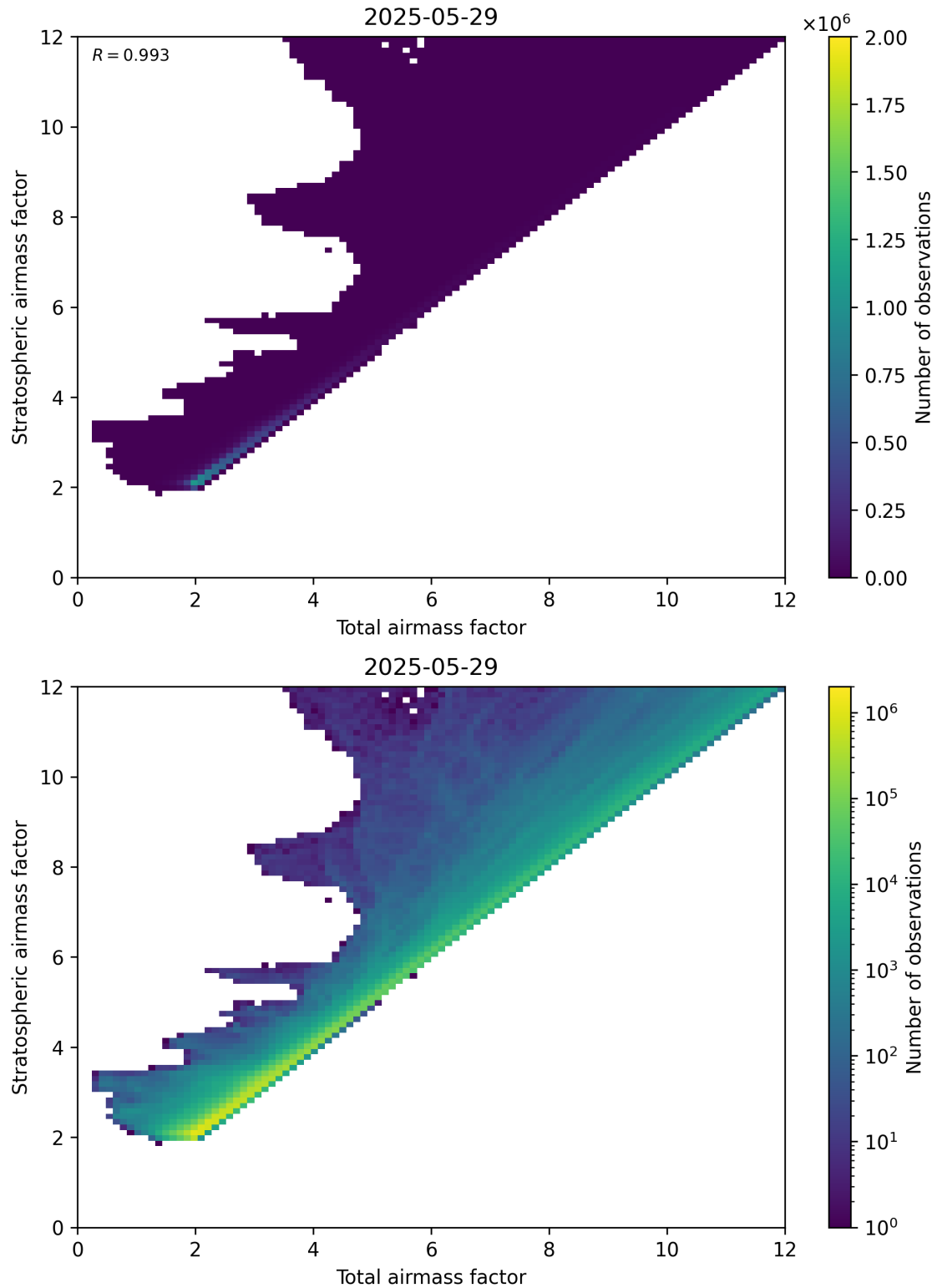
Figure 62: Scatter density plot of “Total airmass factor” against “Stratospheric airmass factor” for 2025-05-28 to 2025-05-30.
