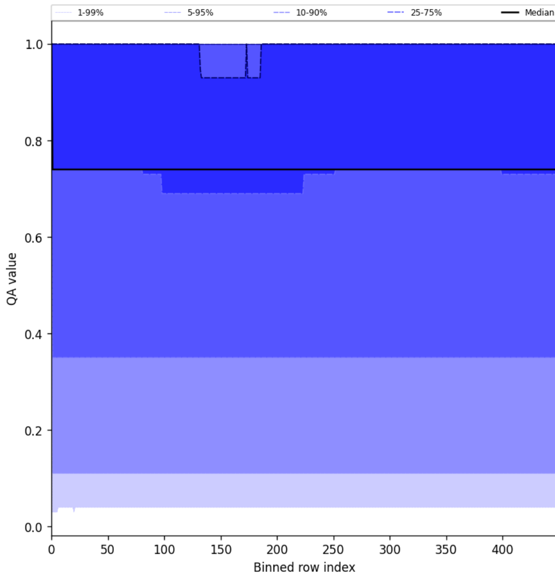
Figure 45: Along track statistics of “QA value” for 2025-05-28 to 2025-05-30
