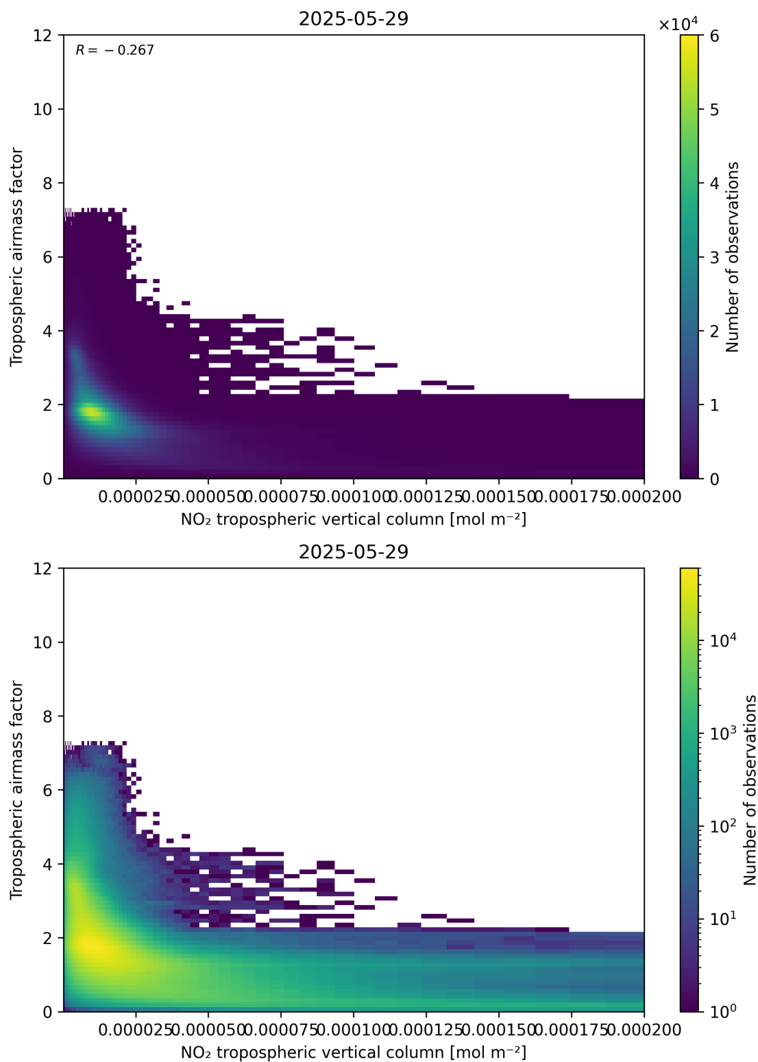
Figure 123: Scatter density plot of “NO 2 tropospheric vertical column” against “Tropospheric air mass factor” for 2025-05-28 to 2025-05-30.
