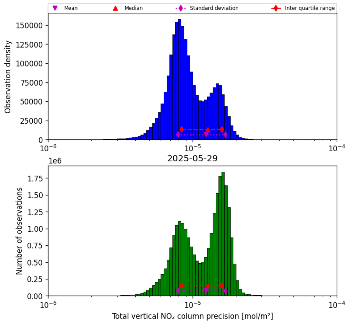
Figure 39: Histogram of "Total vertical NO 2 column precision" for 2025-05-28 to 2025-05-30
