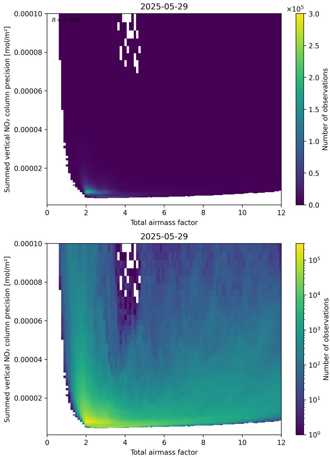
Figure 66: Scatter density plot of “Total airmass factor” against “Summed vertical NO 2 column precision” for 2025-05-28 to 2025-05-30.
