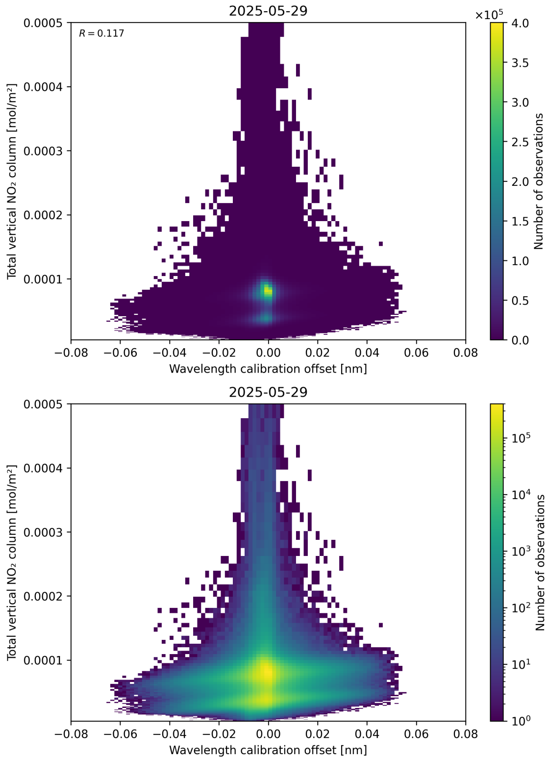
Figure 179: Scatter density plot of “Wavelength calibration offset” against “Total vertical NO 2 column” for 2025-05-28 to 2025-05-30.
