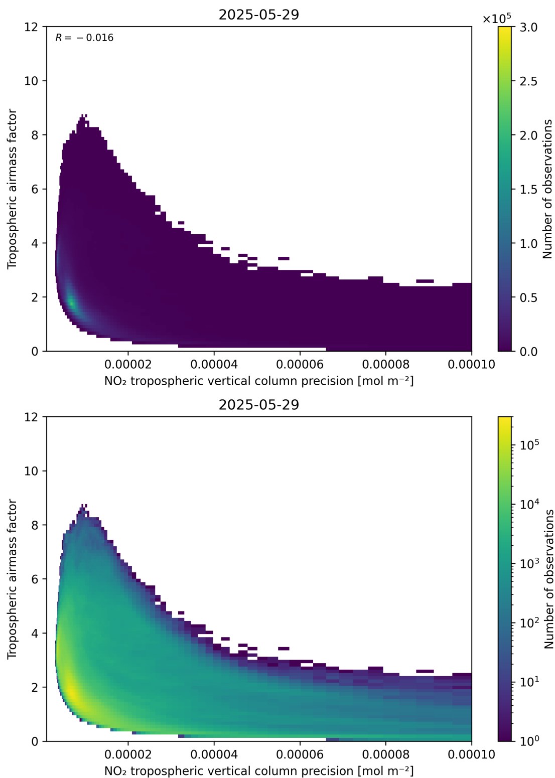
Figure 133: Scatter density plot of “NO 2 tropospheric vertical column precision” against “Tropospheric airmass factor” for 2025-05-28 to 2025-05-30.
