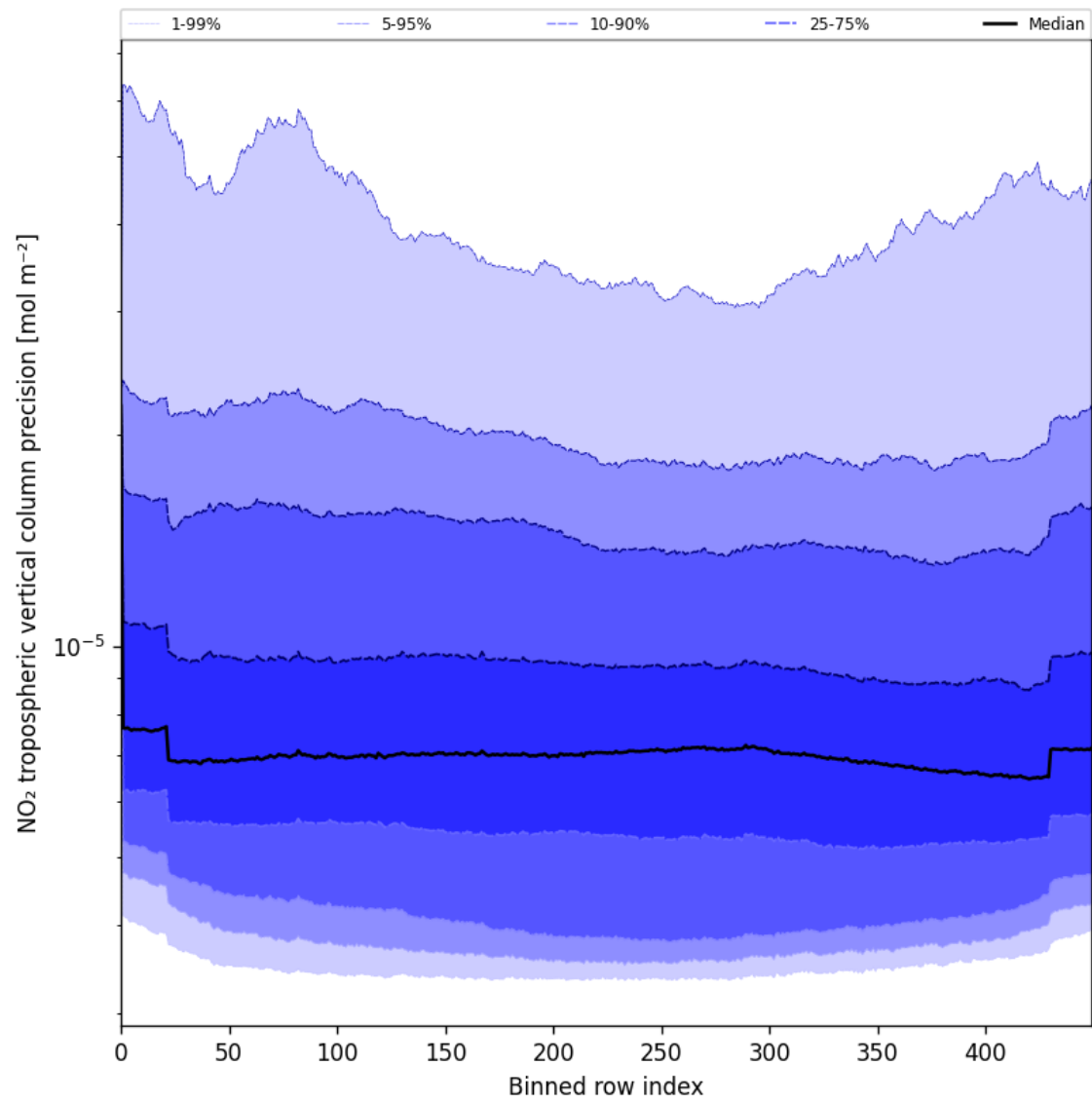
Figure 47: Along track statistics of “NO 2 tropospheric vertical column precision” for 2025-05-28 to 2025-05-30
