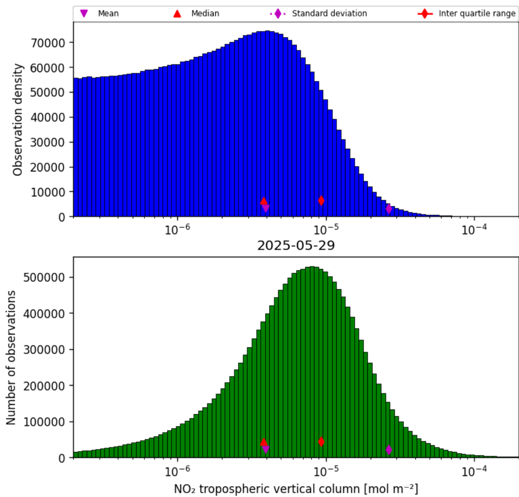
Figure 29: Histogram of “NO 2 tropospheric vertical column” for 2025-05-28 to 2025-05-30
