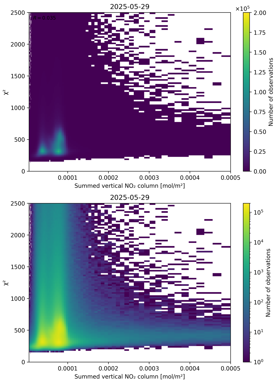
Figure 104: Scatter density plot of “Summed vertical NO 2 column” against “ \chi^2 ” for 2025-05-28 to 2025-05-30.
