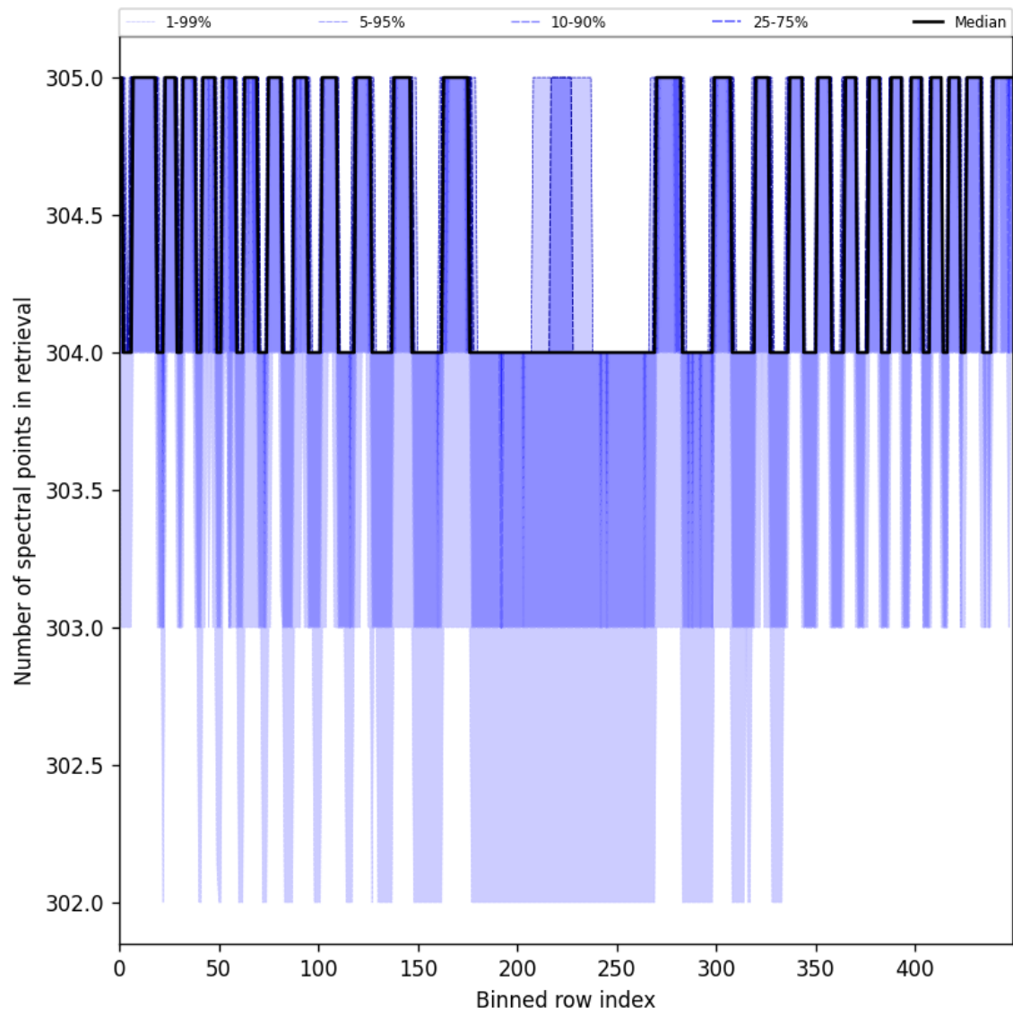
Figure 50: Along track statistics of “Number of spectral points in retrieval” for 2025-05-28 to 2025-05-30
