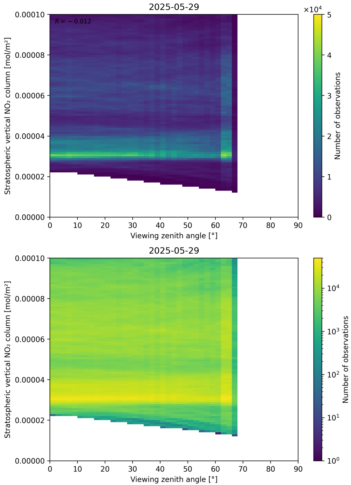
Figure 164: Scatter density plot of “Viewing zenith angle” against “Stratospheric vertical NO 2 column” for 2025-05-28 to 2025-05-30.
