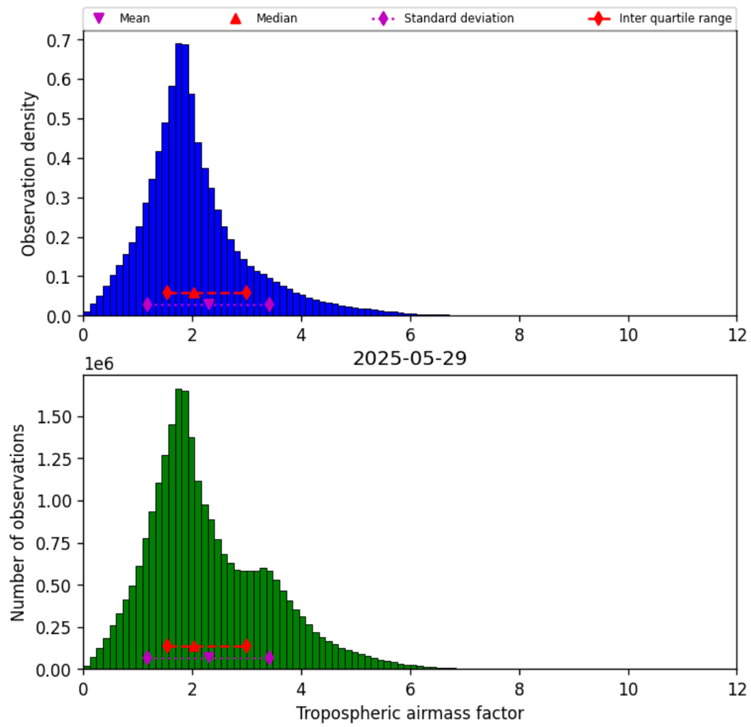
Figure 31: Histogram of “Tropospheric airmass factor” for 2025-05-28 to 2025-05-30
