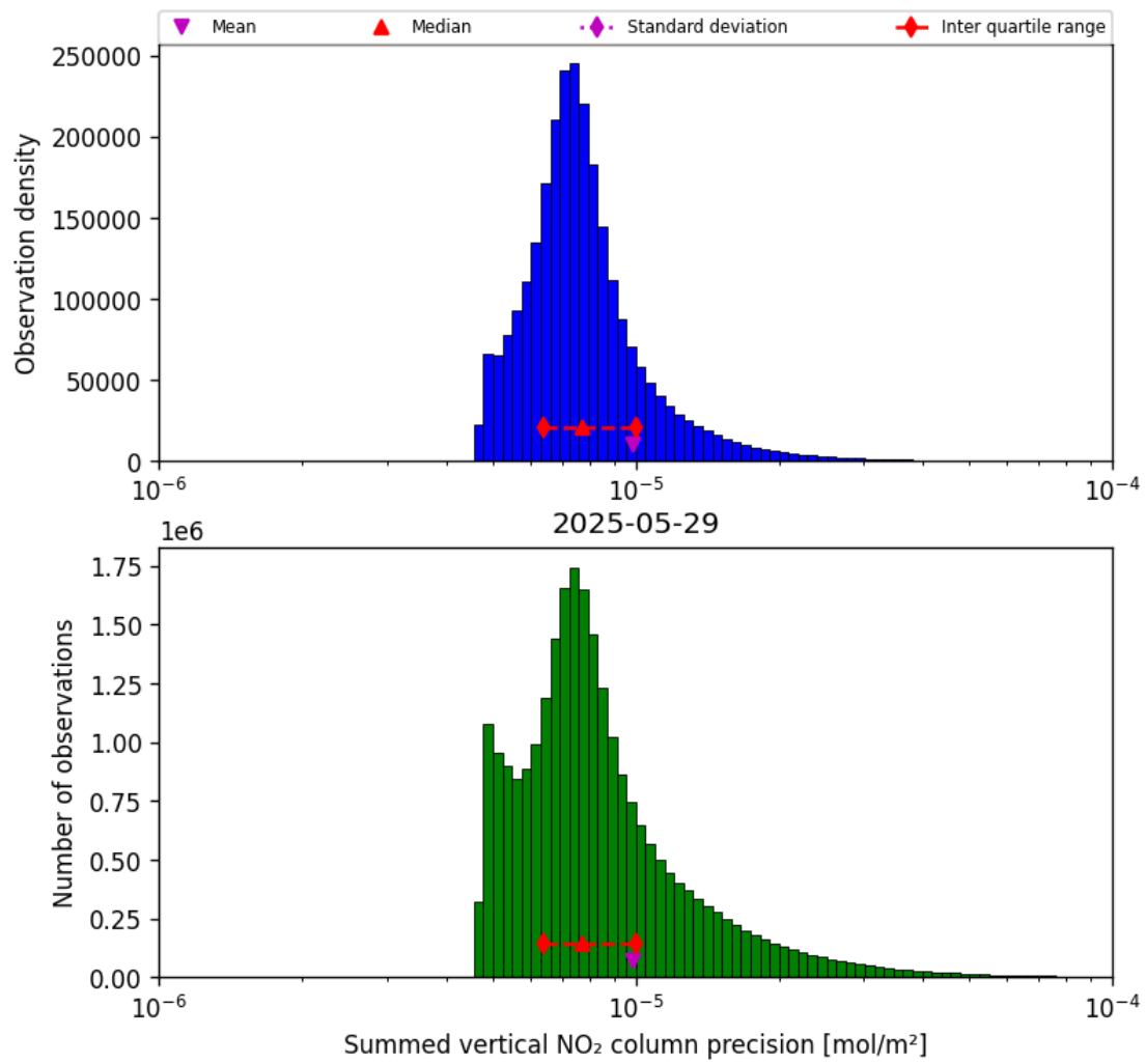
Figure 41: Histogram of "Summed vertical NO 2 column precision" for 2025-05-28 to 2025-05-30
