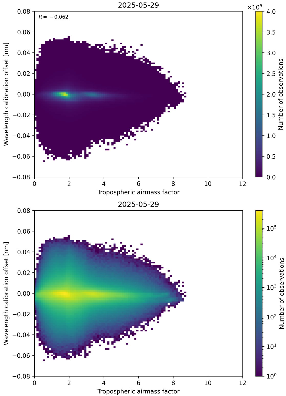
Figure 80: Scatter density plot of “Tropospheric airmass factor” against “Wavelength calibration offset” for 2025-05-28 to 2025-05-30.
