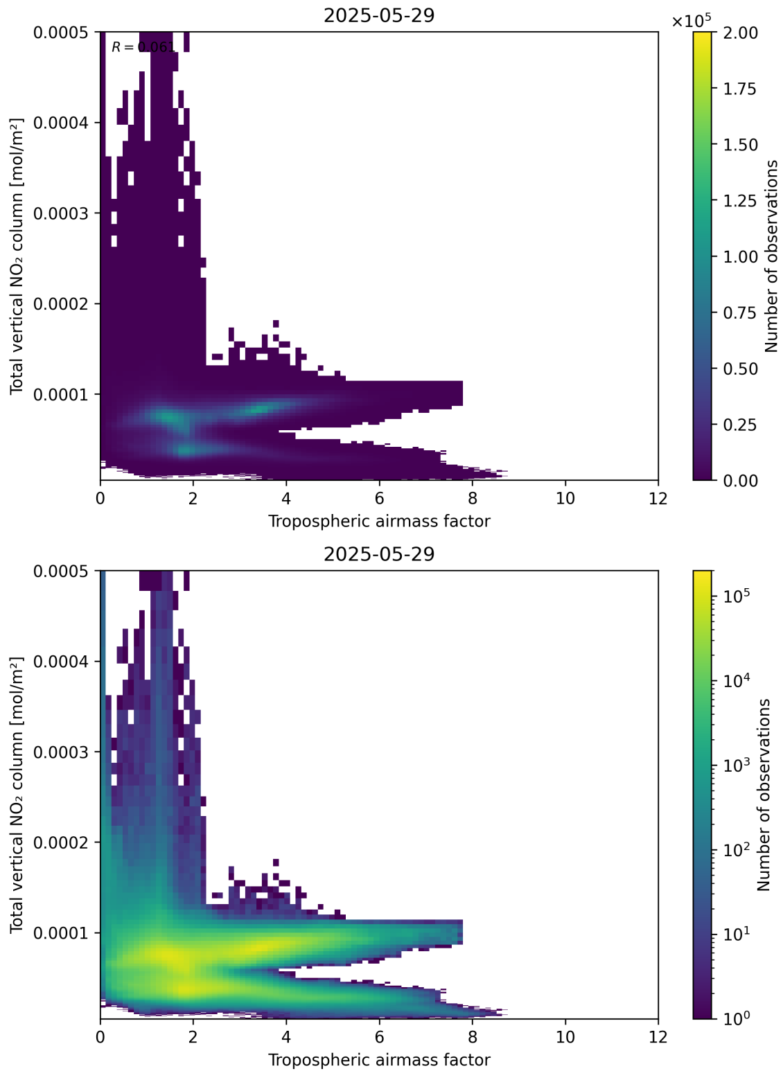
Figure 77: Scatter density plot of “Tropospheric airmass factor” against “Total vertical NO 2 column” for 2025-05-28 to 2025-05-30.
