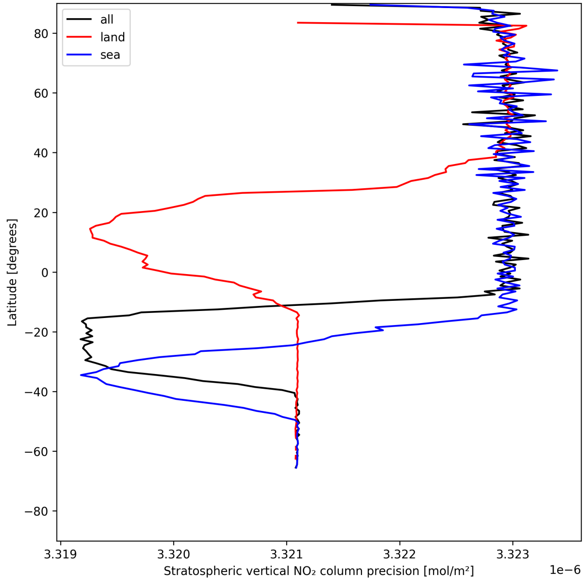
Figure 20: Zonal average of “Stratospheric vertical NO 2 column precision” for 2025-05-28 to 2025-05-30.
