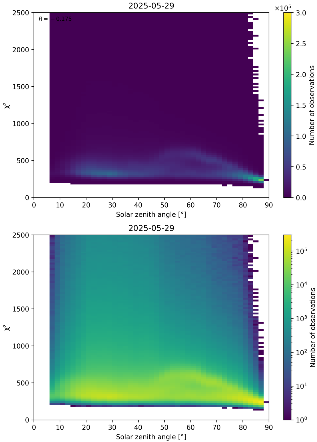
Figure 148: Scatter density plot of “Solar zenith angle” against “ \chi^2 ” for 2025-05-28 to 2025-05-30.
