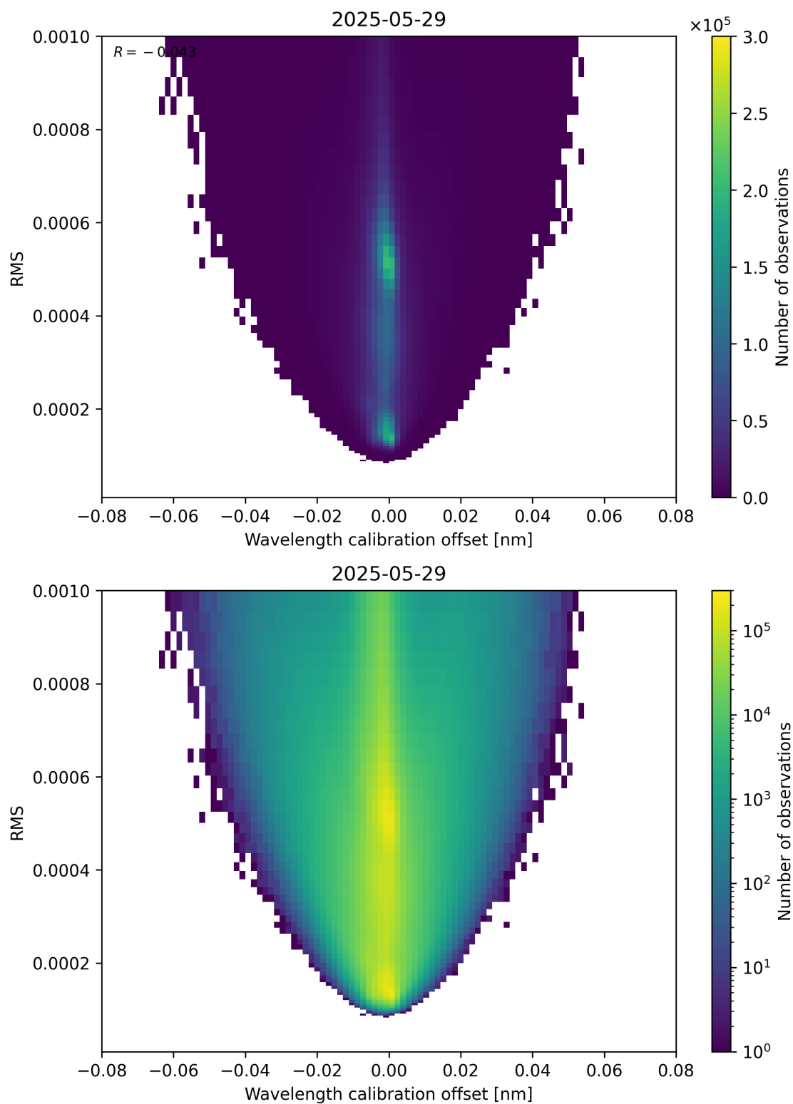
Figure 181: Scatter density plot of “Wavelength calibration offset” against “RMS” for 2025-05-28 to 2025-05-30.
