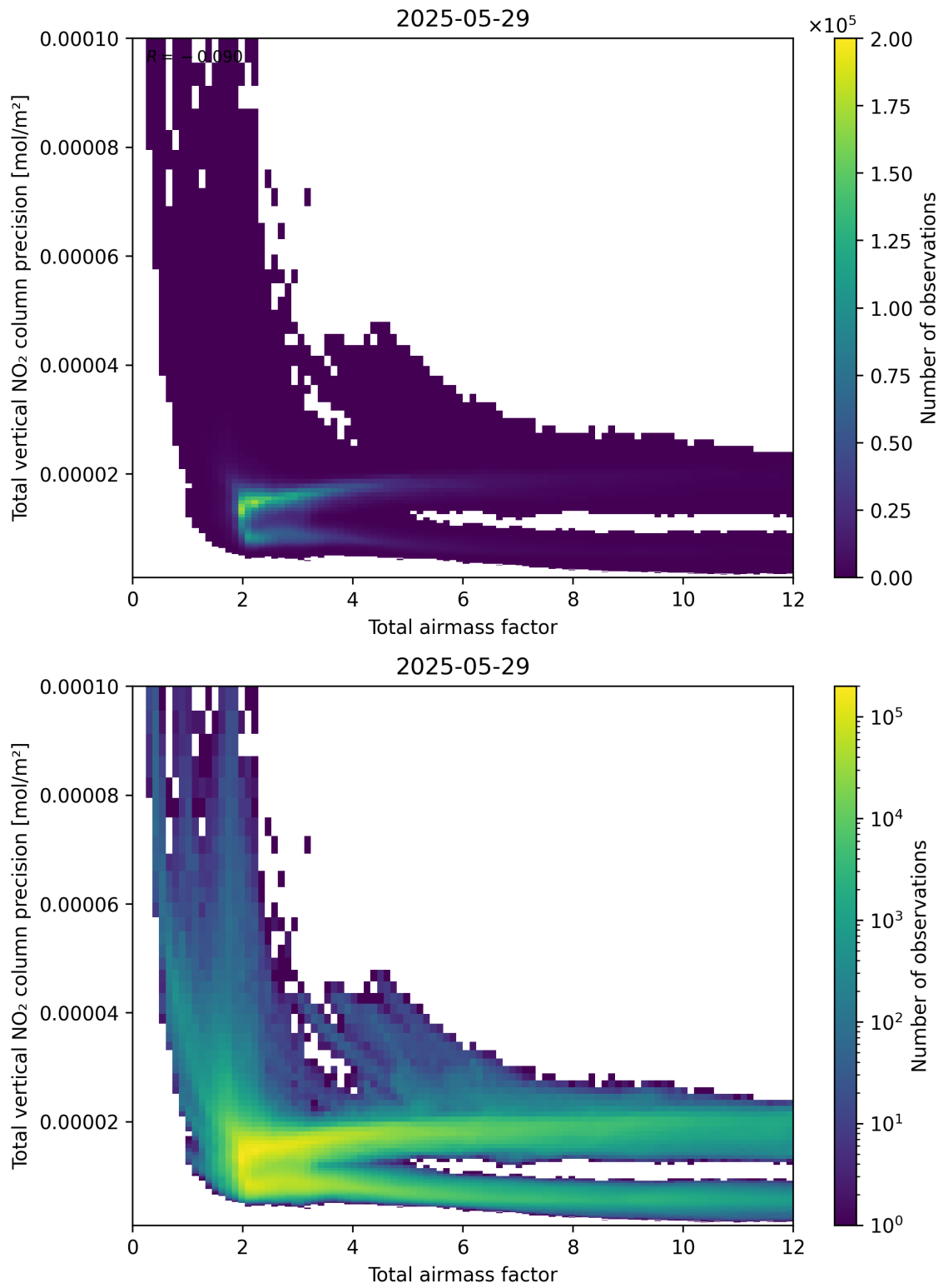
Figure 68: Scatter density plot of “Total airmass factor” against “Total vertical NO 2 column precision” for 2025-05-28 to 2025-05-30.
