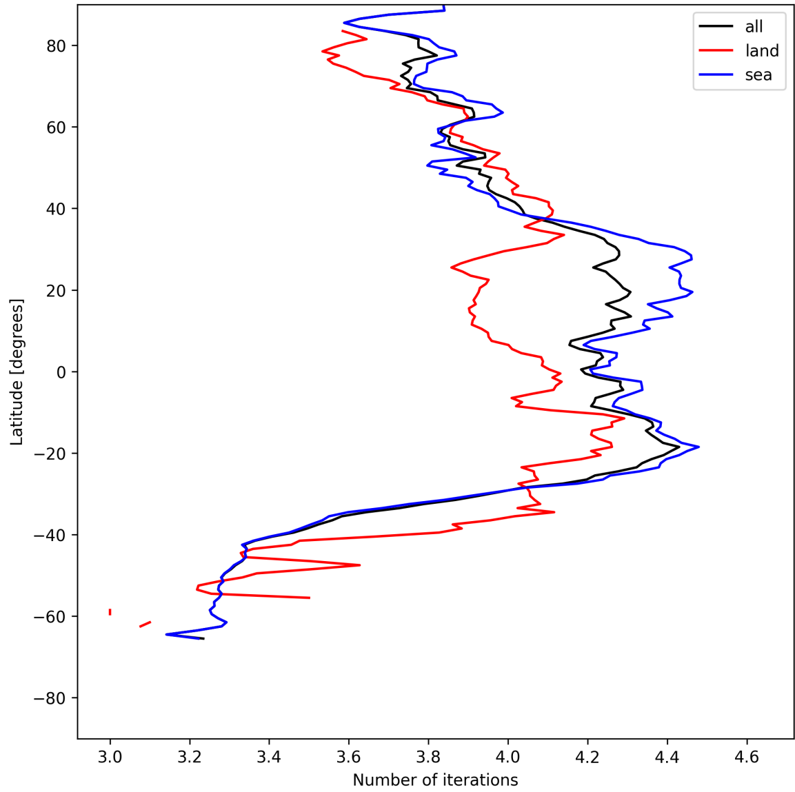
Figure 17: Zonal average of “Number of iterations” for 2025-05-28 to 2025-05-30.
