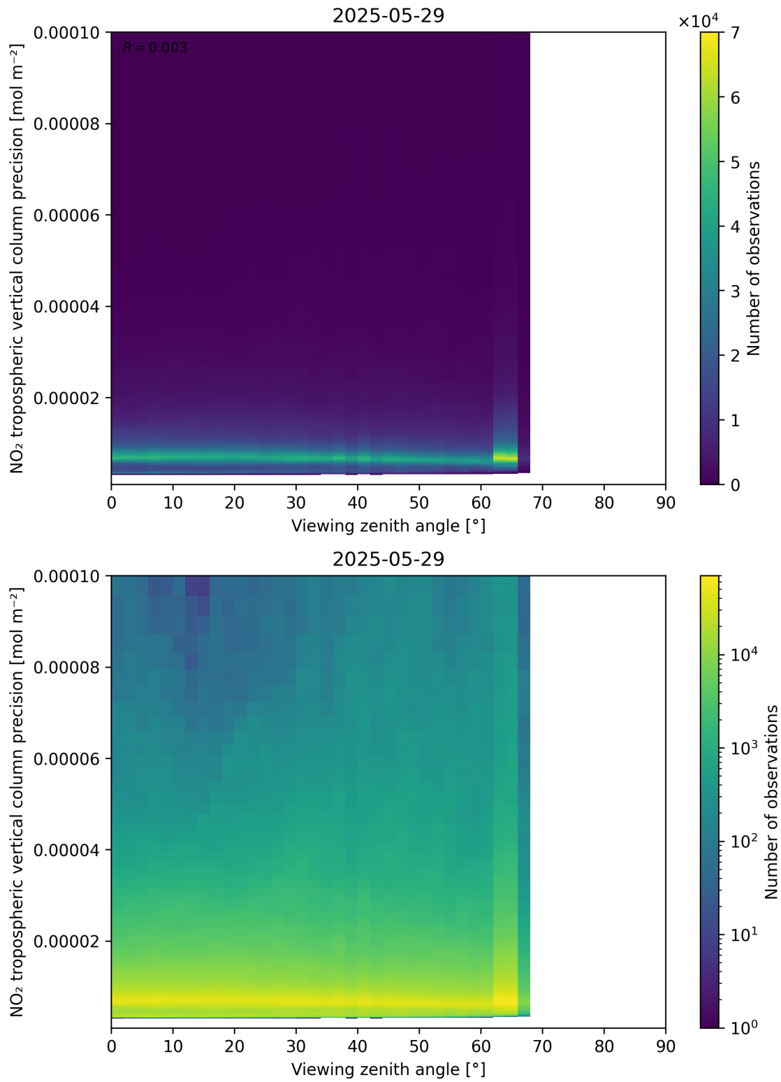
Figure 170: Scatter density plot of “Viewing zenith angle” against “NO 2 tropospheric vertical column precision” for 2025-05-28 to 2025-05-30.
