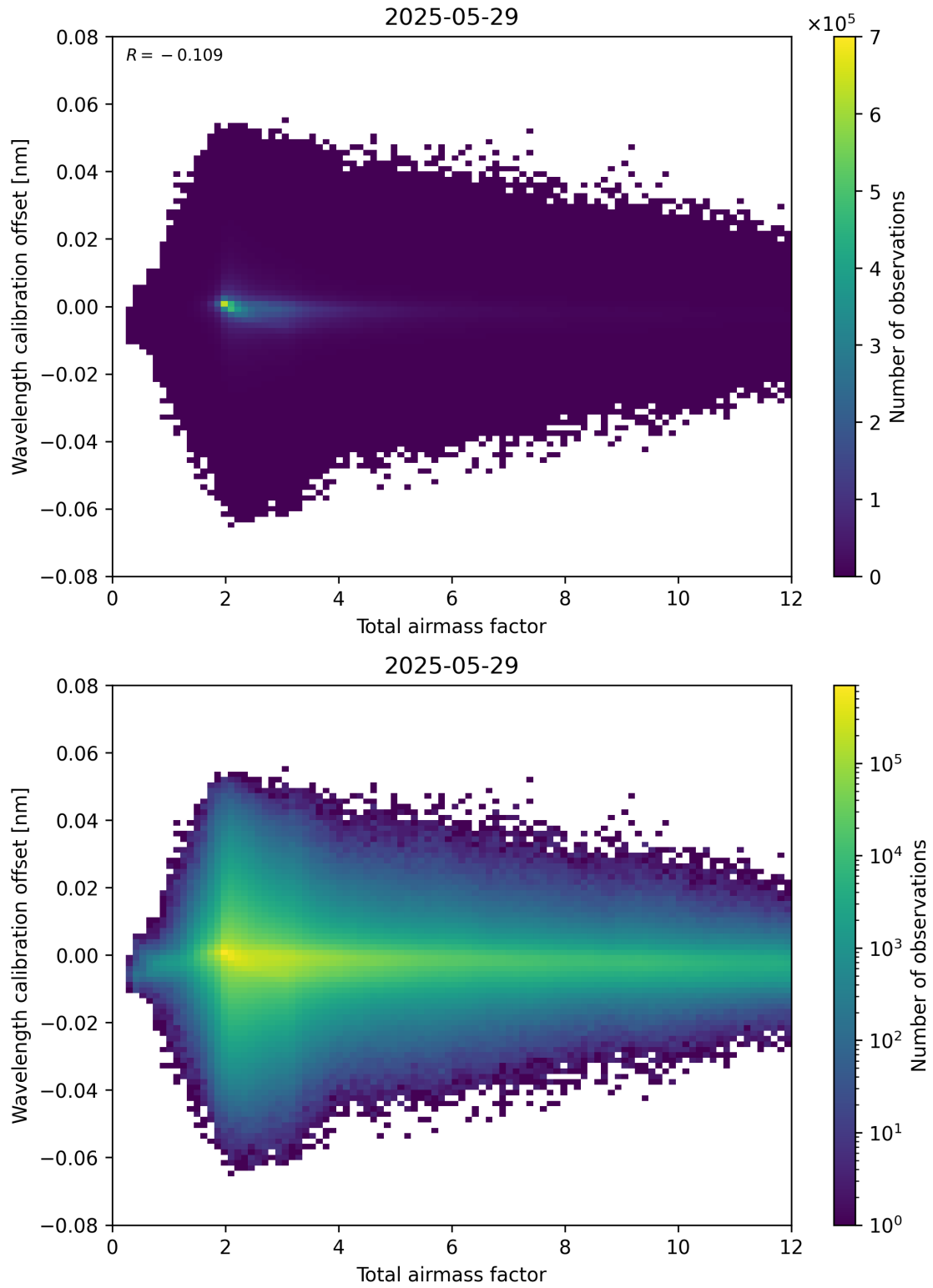
Figure 70: Scatter density plot of “Total airmass factor” against “Wavelength calibration offset” for 2025-05-28 to 2025-05-30.
