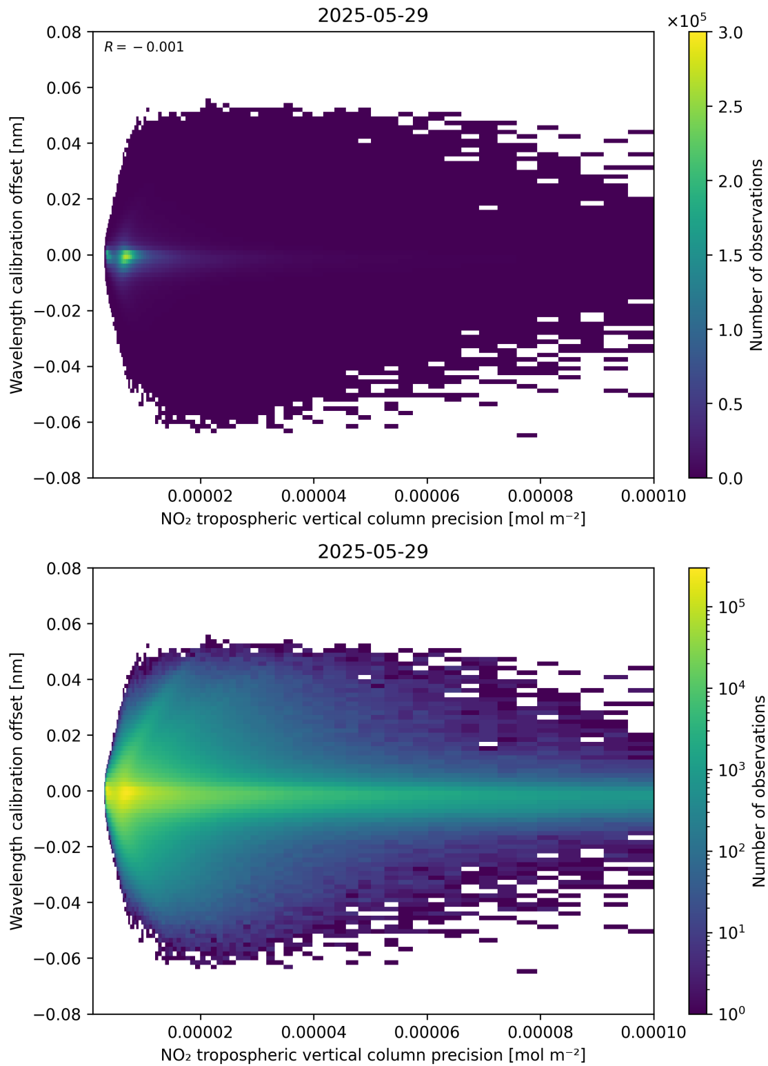
Figure 141: Scatter density plot of “NO 2 tropospheric vertical column precision” against “Wavelength calibration offset” for 2025-05-28 to 2025-05-30.
