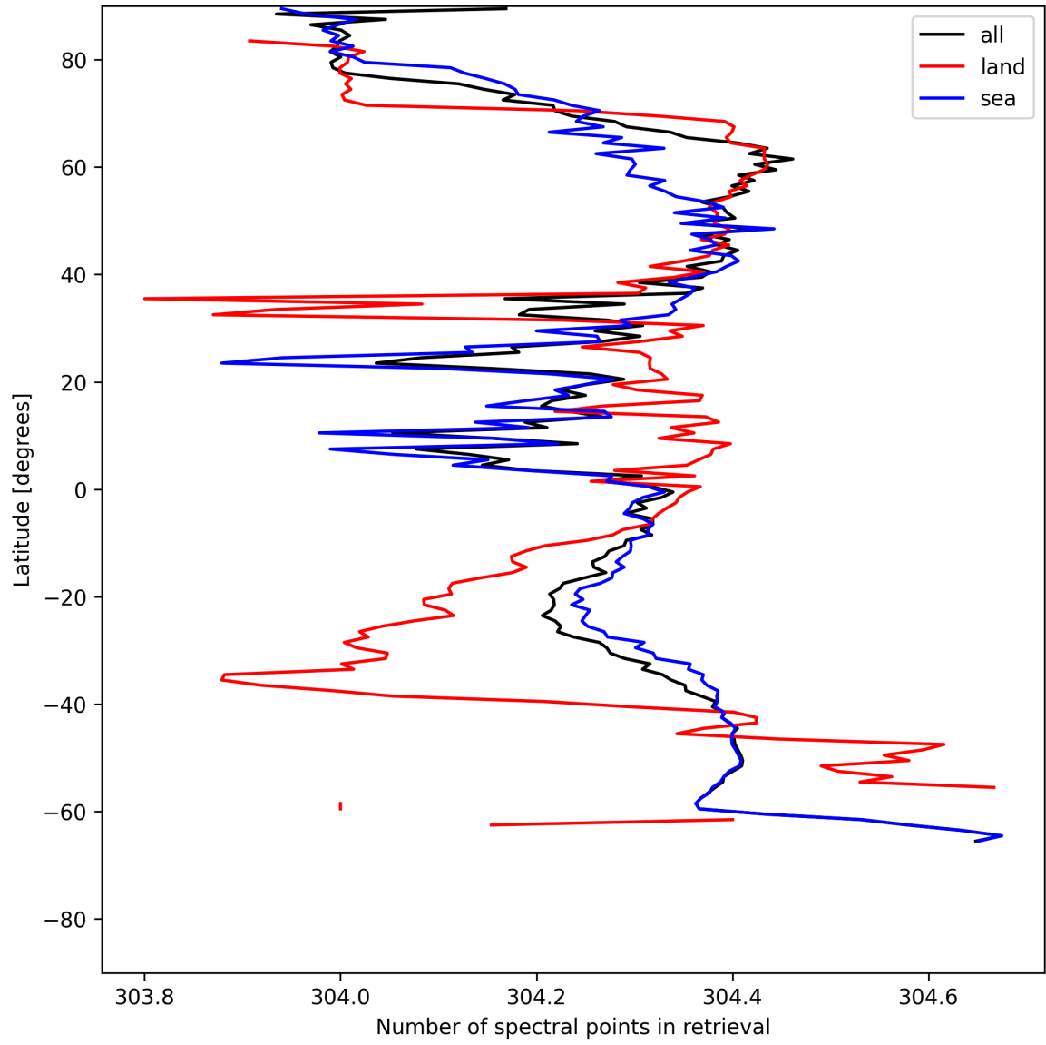
Figure 16: Zonal average of “Number of spectral points in retrieval” for 2025-05-28 to 2025-05-30.
