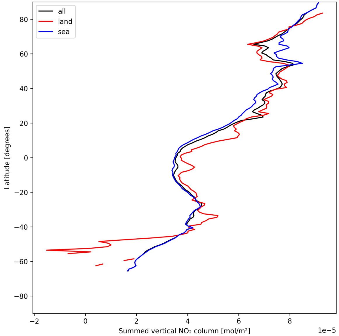
Figure 23: Zonal average of “Summed vertical NO 2 column” for 2025-05-28 to 2025-05-30.
