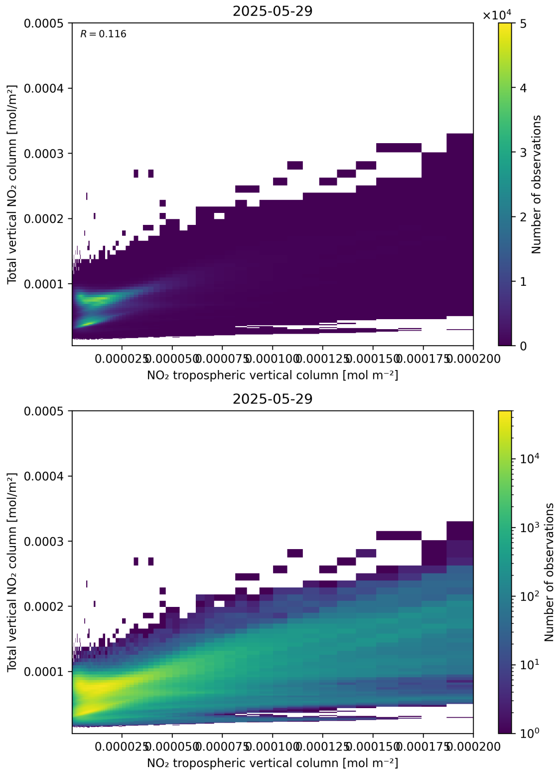
Figure 128: Scatter density plot of “NO 2 tropospheric vertical column” against “Total vertical NO 2 column” for 2025-05-28 to 2025-05-30.
