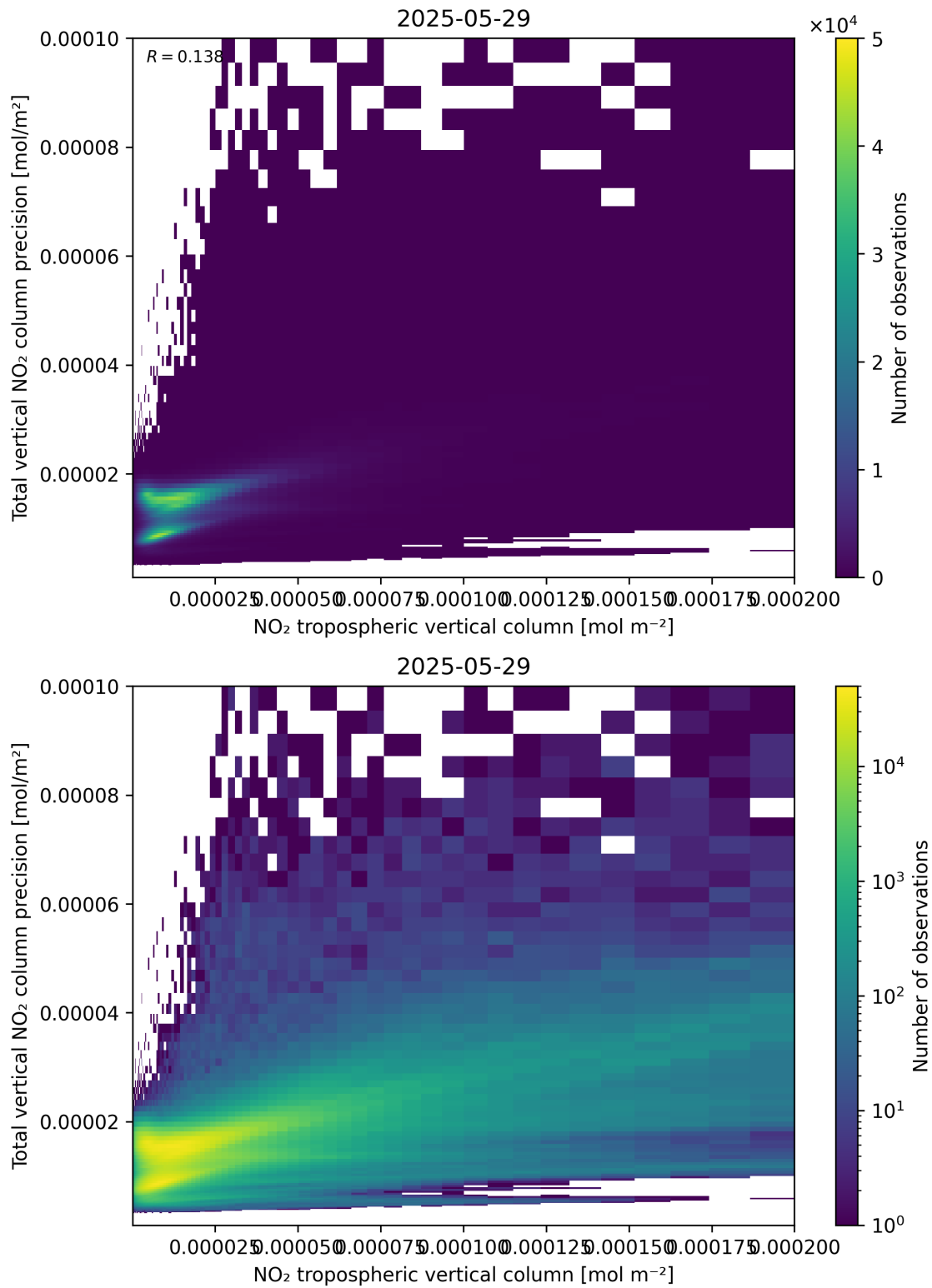
Figure 129: Scatter density plot of “NO 2 tropospheric vertical column” against “Total vertical NO 2 column precision” for 2025-05-28 to 2025-05-30.
