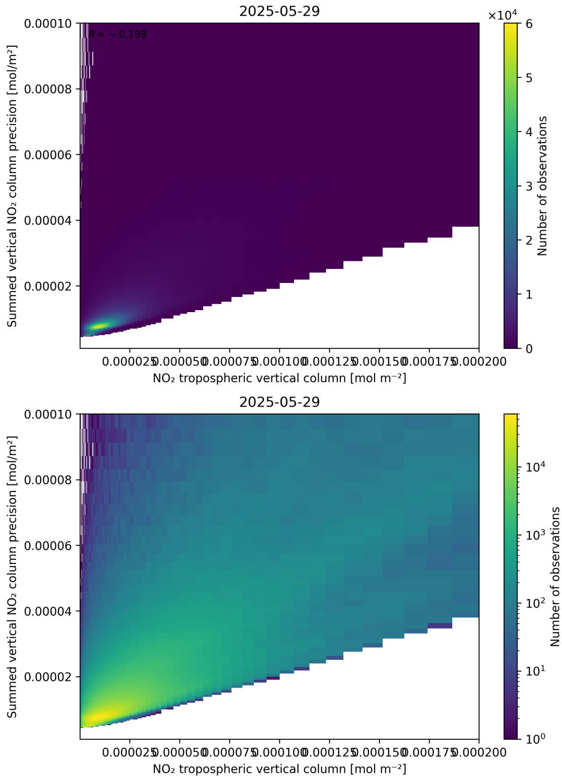
Figure 127: Scatter density plot of “NO 2 tropospheric vertical column” against “Summed vertical NO 2 column precision” for 2025-05-28 to 2025-05-30.
