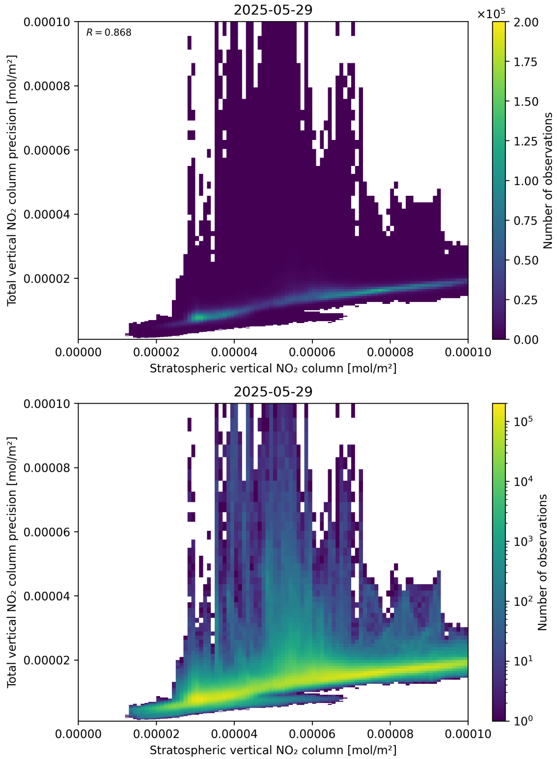
Figure 101: Scatter density plot of “Stratospheric vertical NO 2 column” against “Total vertical NO 2 column precision” for 2025-05-28 to 2025-05-30.
