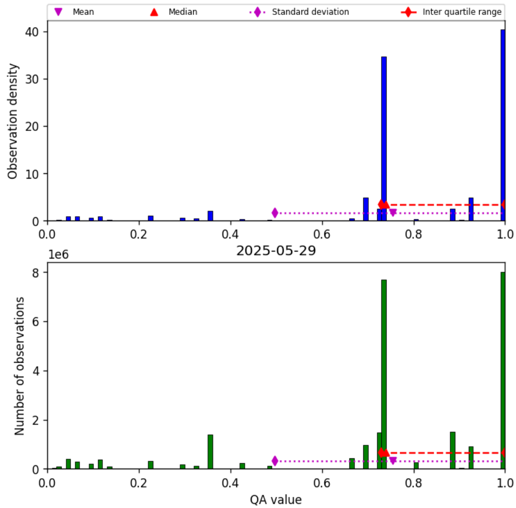
Figure 28: Histogram of “QA value” for 2025-05-28 to 2025-05-30
