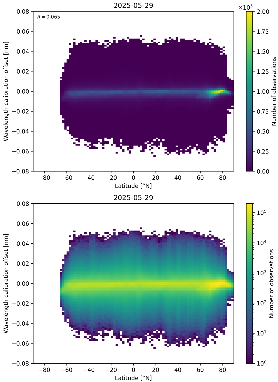
Figure 95: Scatter density plot of “Latitude” against “Wavelength calibration offset” for 2025-05-28 to 2025-05-30.
