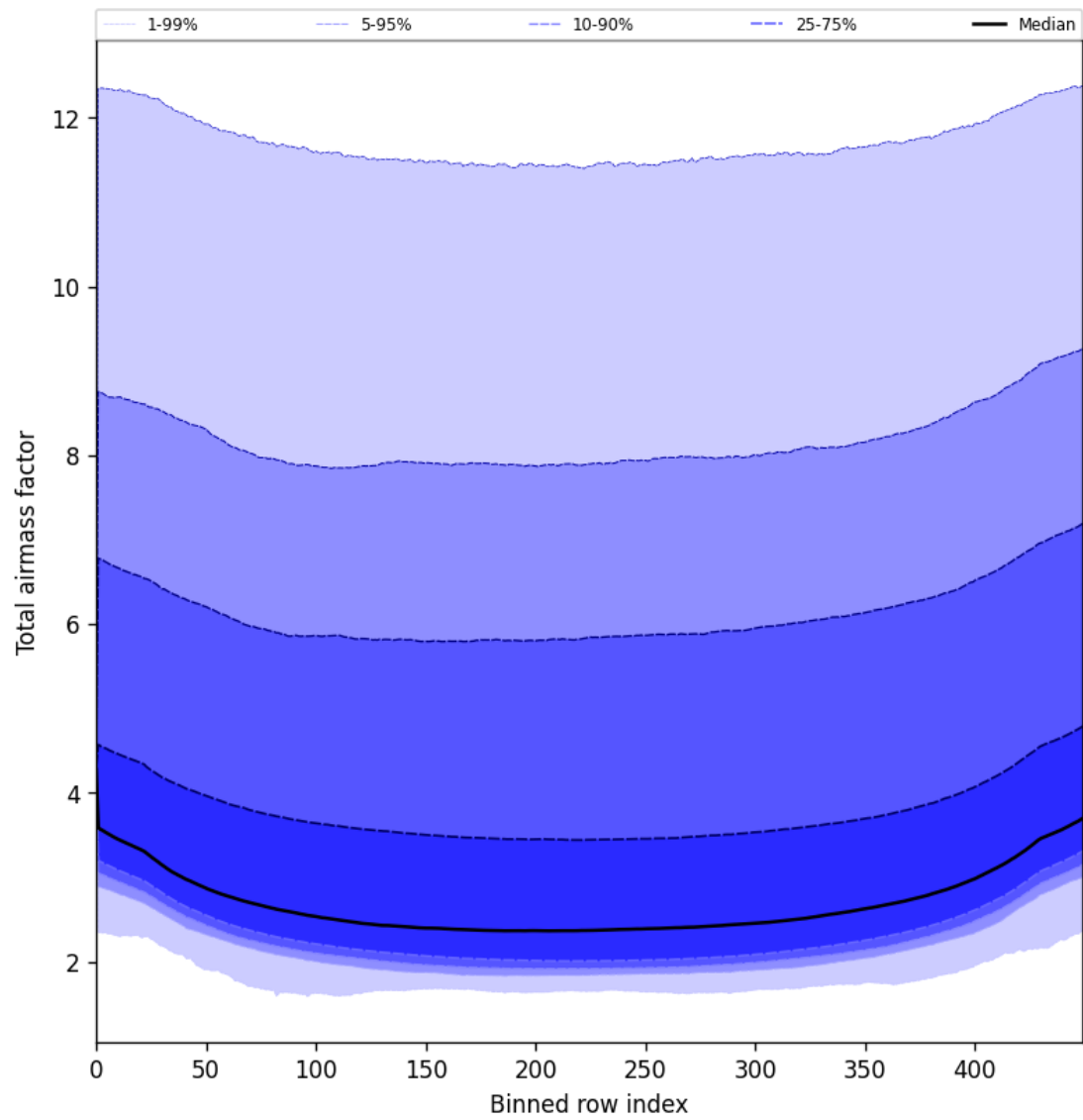
Figure 49: Along track statistics of “Total airmass factor” for 2025-05-28 to 2025-05-30
