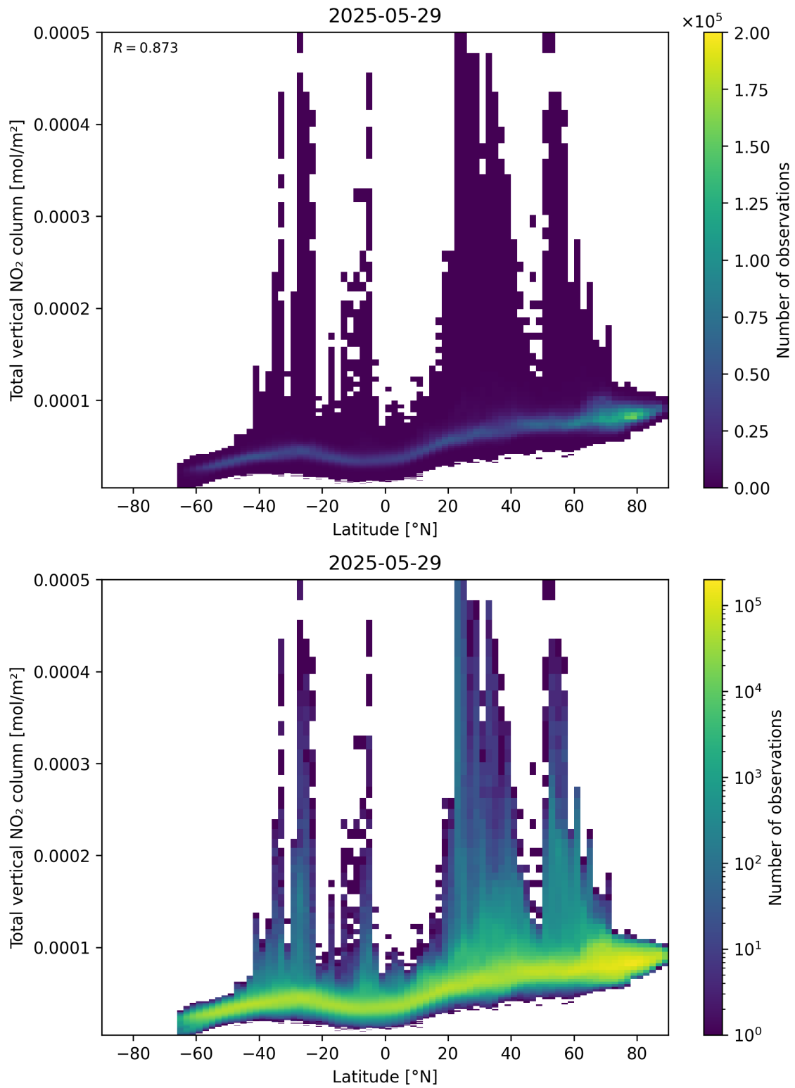
Figure 90: Scatter density plot of “Latitude” against “Total vertical NO 2 column” for 2025-05-28 to 2025-05-30.
