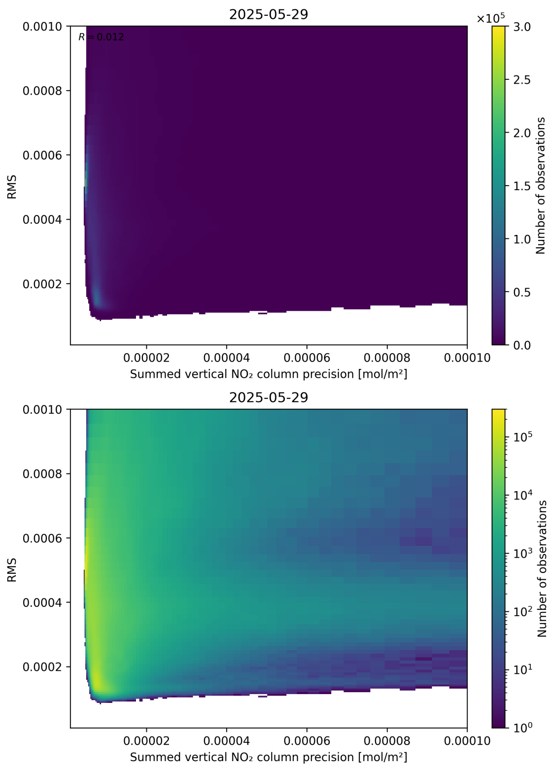
Figure 108: Scatter density plot of “Summed vertical NO 2 column precision” against “RMS” for 2025-05-28 to 2025-05-30.
