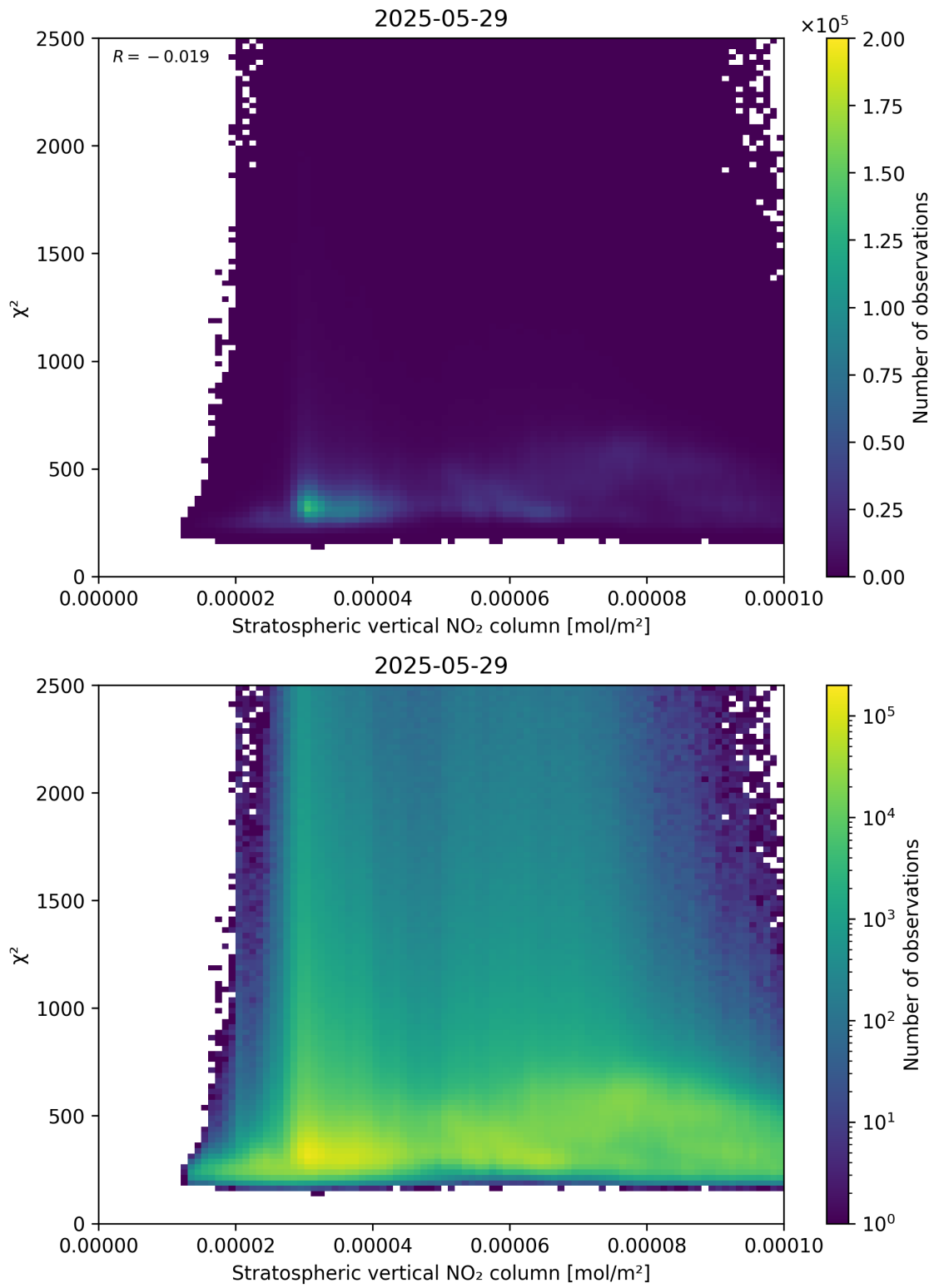
Figure 97: Scatter density plot of “Stratospheric vertical NO 2 column” against “ \chi^2 ” for 2025-05-28 to 2025-05-30.
