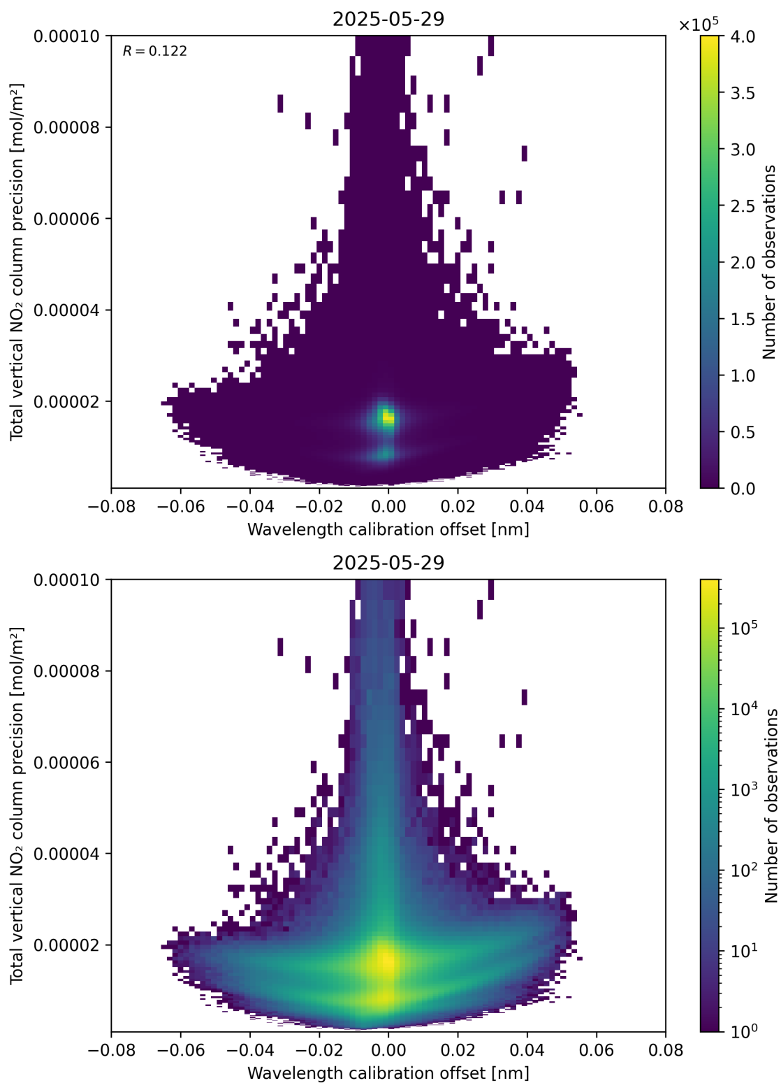
Figure 180: Scatter density plot of “Wavelength calibration offset” against “Total vertical NO 2 column precision” for 2025-05-28 to 2025-05-30.
