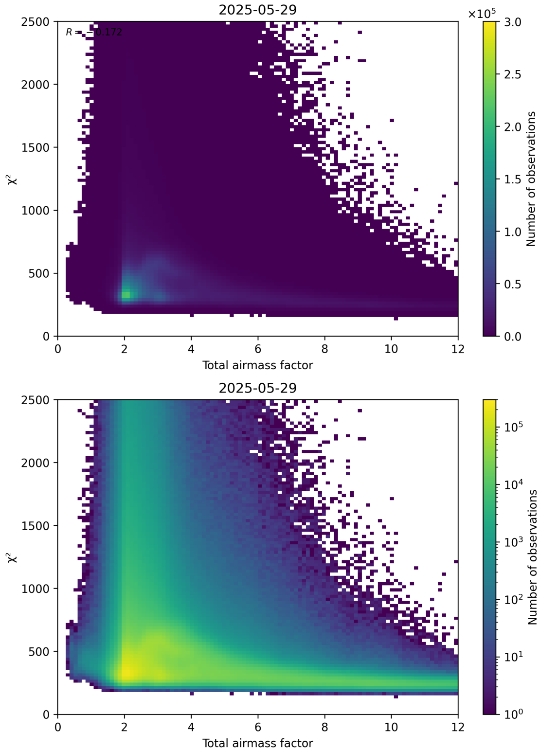
Figure 63: Scatter density plot of “Total airmass factor” against “ \chi^2 ” for 2025-05-28 to 2025-05-30.
