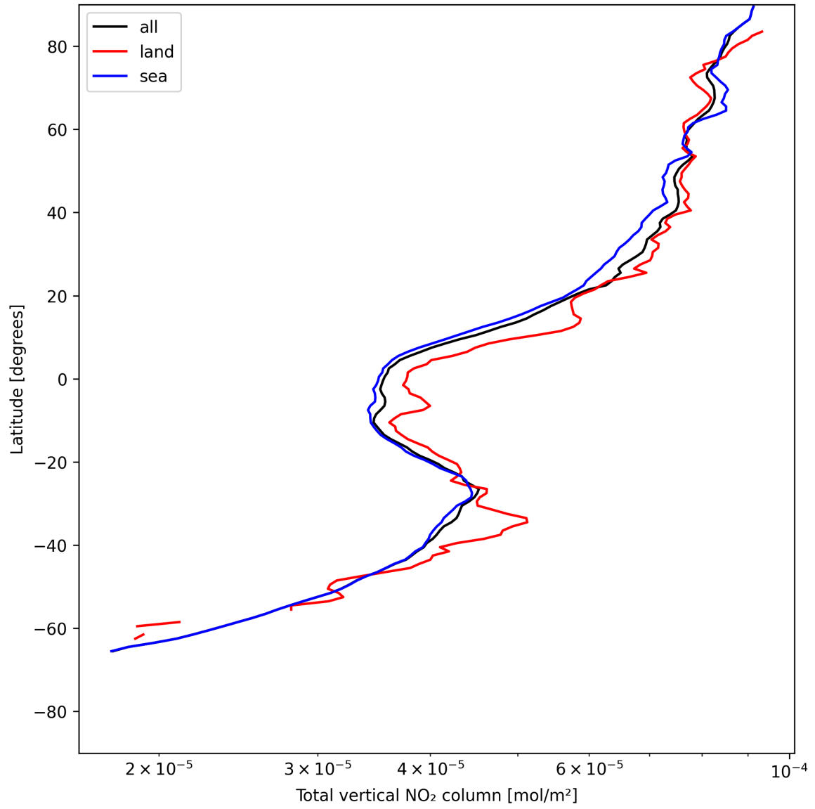
Figure 21: Zonal average of “Total vertical NO 2 column” for 2025-05-28 to 2025-05-30.
