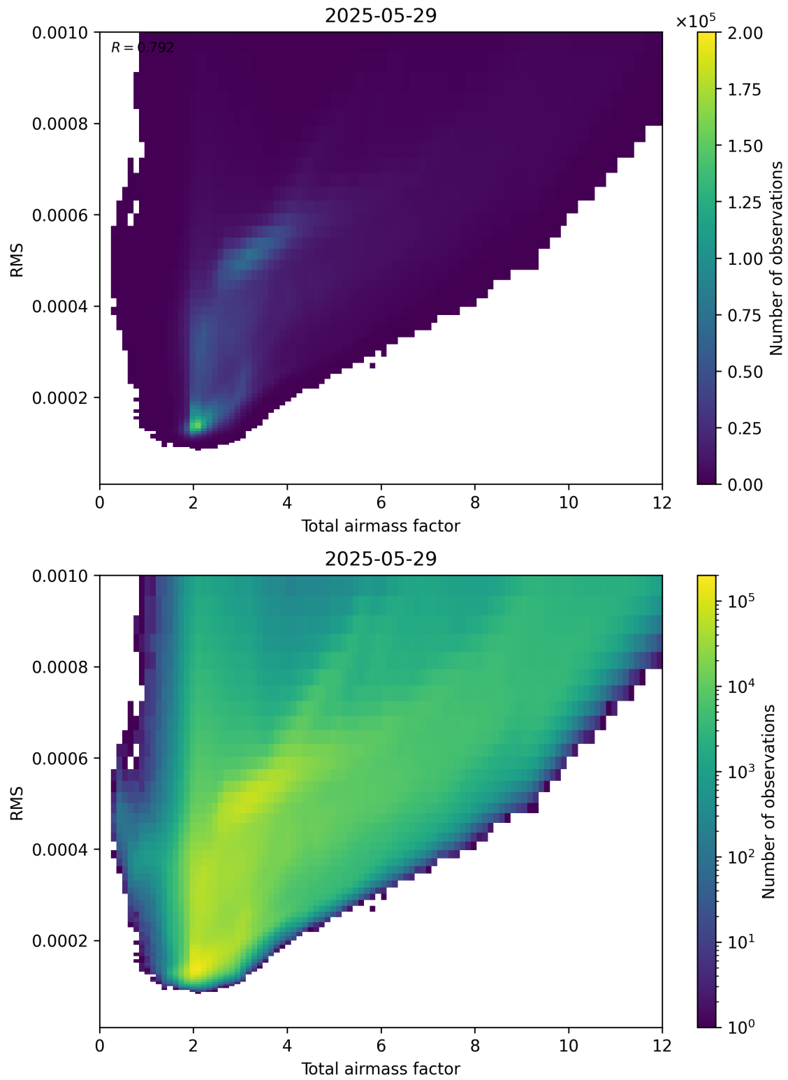
Figure 69: Scatter density plot of “Total airmass factor” against “RMS” for 2025-05-28 to 2025-05-30.
