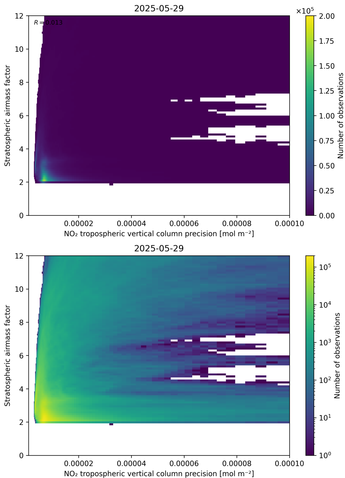
Figure 131: Scatter density plot of “NO 2 tropospheric vertical column precision” against “Stratospheric airmass factor” for 2025-05-28 to 2025-05-30.
