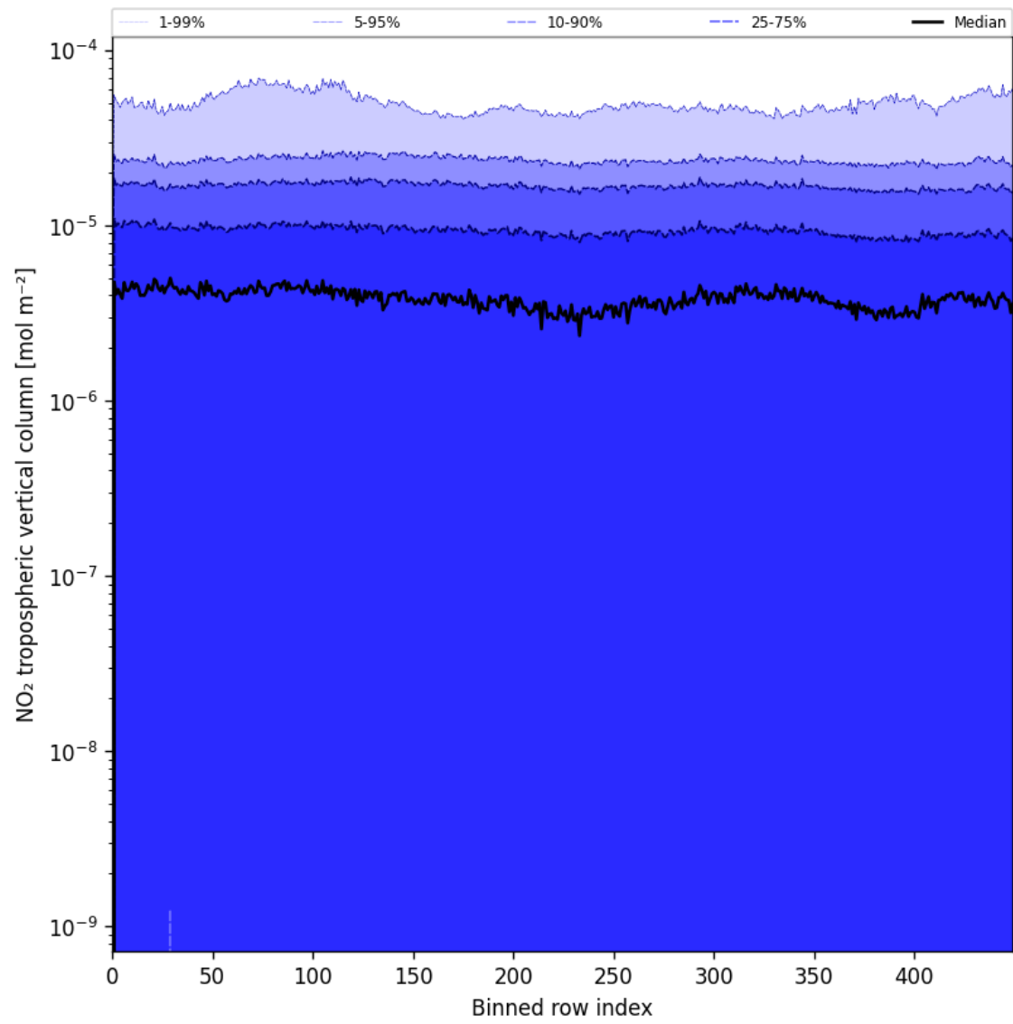
Figure 46: Along track statistics of “NO 2 tropospheric vertical column” for 2025-05-28 to 2025-05-30
