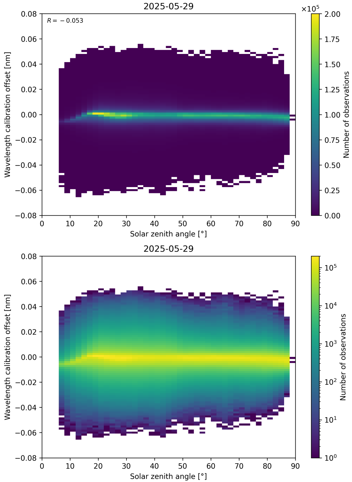
Figure 158: Scatter density plot of “Solar zenith angle” against “Wavelength calibration offset” for 2025-05-28 to 2025-05-30.
