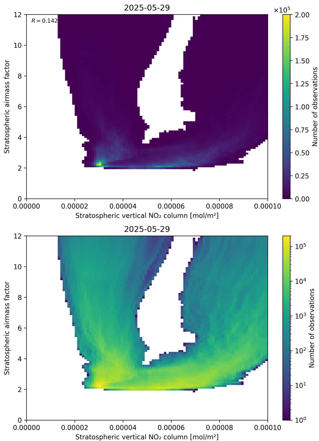
Figure 96: Scatter density plot of “Stratospheric vertical NO 2 column” against “Stratospheric airmass factor” for 2025-05-28 to 2025-05-30.
