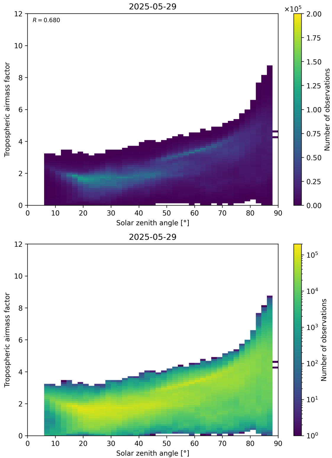
Figure 147: Scatter density plot of “Solar zenith angle” against “Tropospheric airmass factor” for 2025-05-28 to 2025-05-30.
