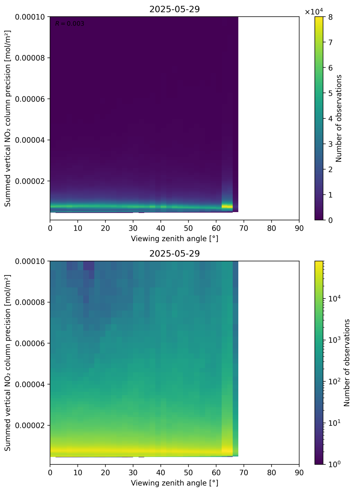
Figure 166: Scatter density plot of “Viewing zenith angle” against “Summed vertical NO 2 column precision” for 2025-05-28 to 2025-05-30.
