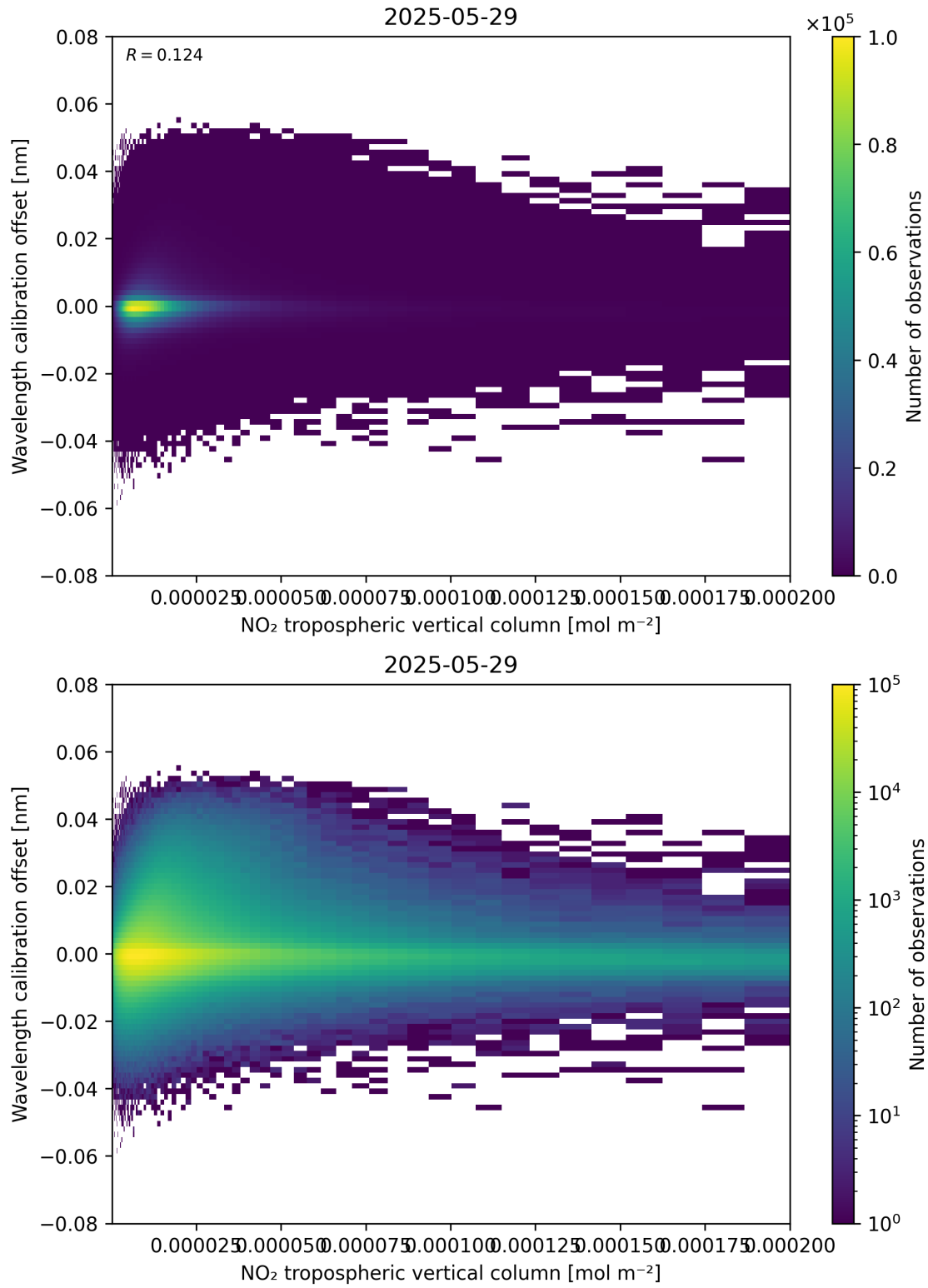
Figure 143: Scatter density plot of “NO 2 tropospheric vertical column” against “Wavelength calibration offset” for 2025-05-28 to 2025-05-30.
