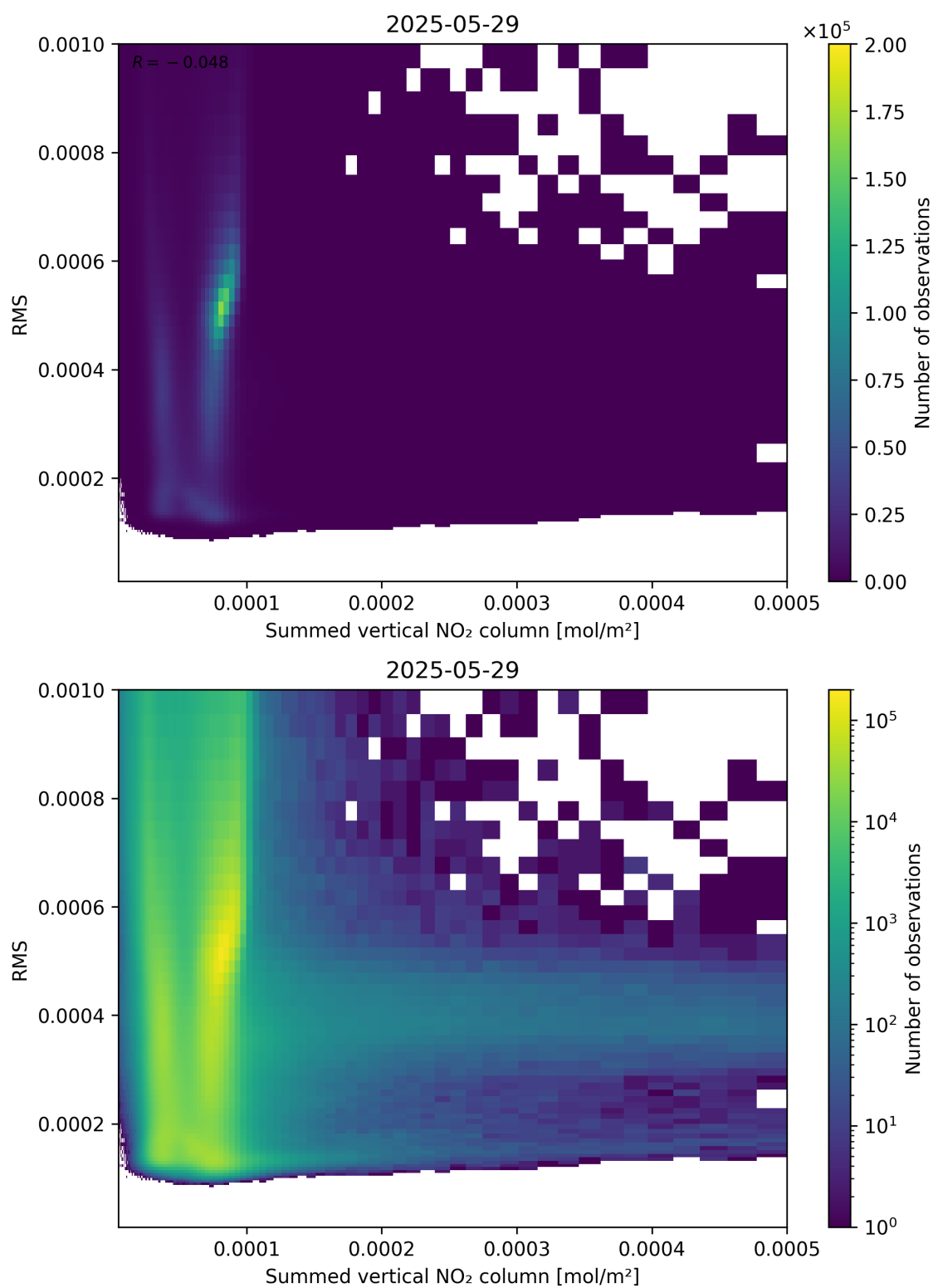
Figure 109: Scatter density plot of “Summed vertical NO 2 column” against “RMS” for 2025-05-28 to 2025-05-30.
