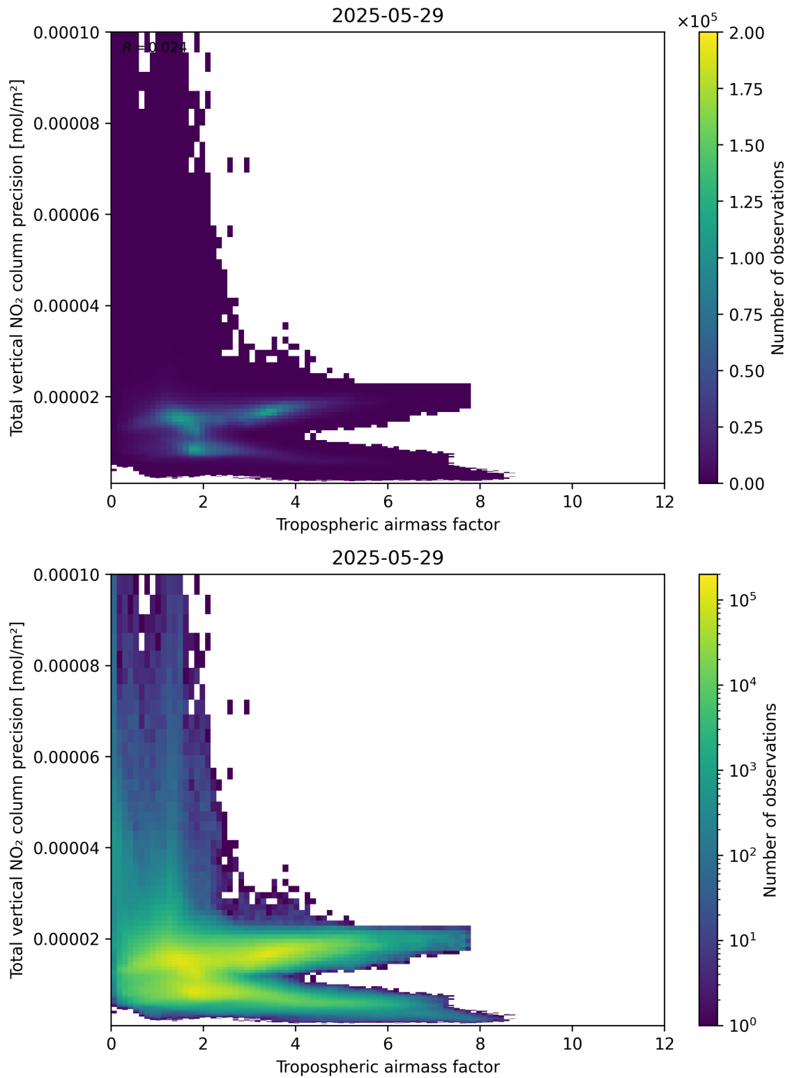
Figure 78: Scatter density plot of “Tropospheric air mass factor” against “Total vertical NO 2 column precision” for 2025-05-28 to 2025-05-30.
