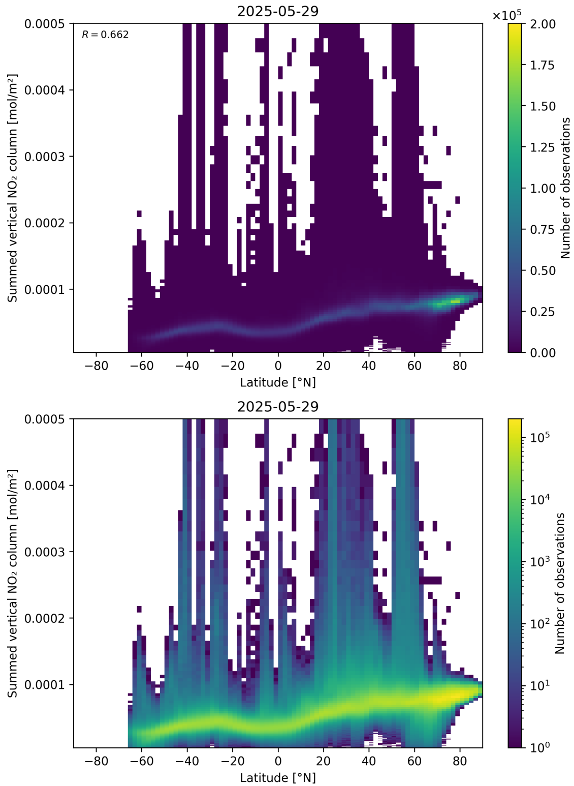
Figure 88: Scatter density plot of “Latitude” against “Summed vertical NO 2 column” for 2025-05-28 to 2025-05-30.
