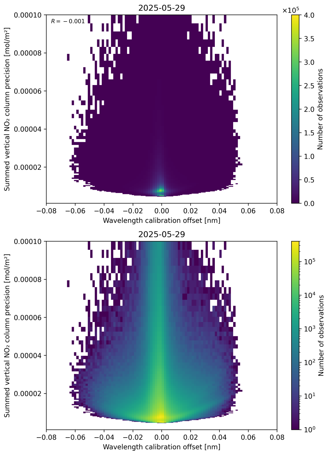
Figure 178: Scatter density plot of “Wavelength calibration offset” against “Summed vertical NO 2 column precision” for 2025-05-28 to 2025-05-30.
