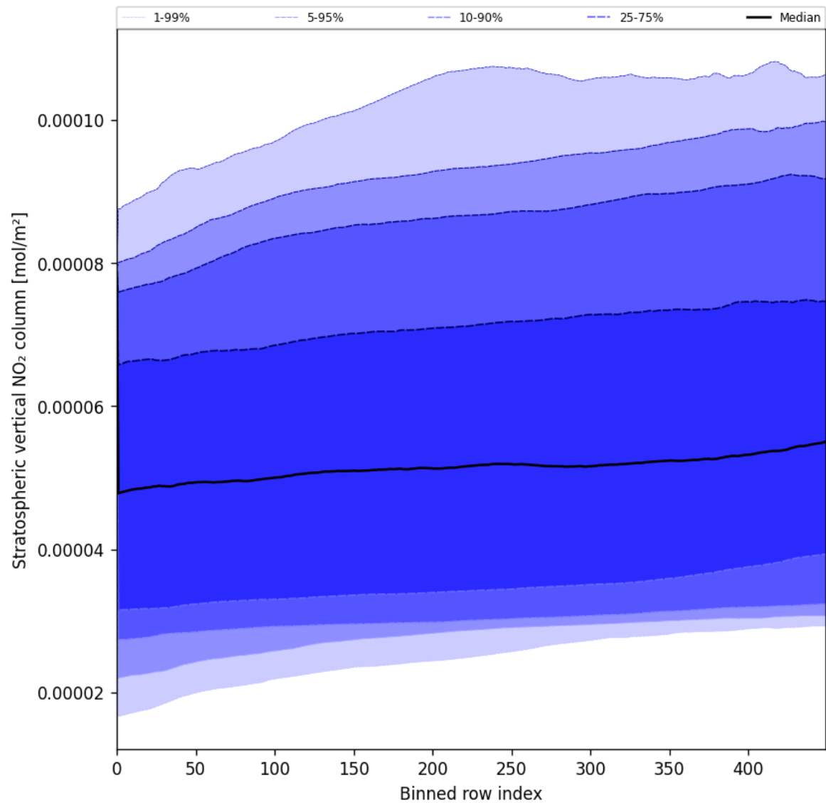
Figure 53: Along track statistics of “Stratospheric vertical NO 2 column” for 2025-05-28 to 2025-05-30
