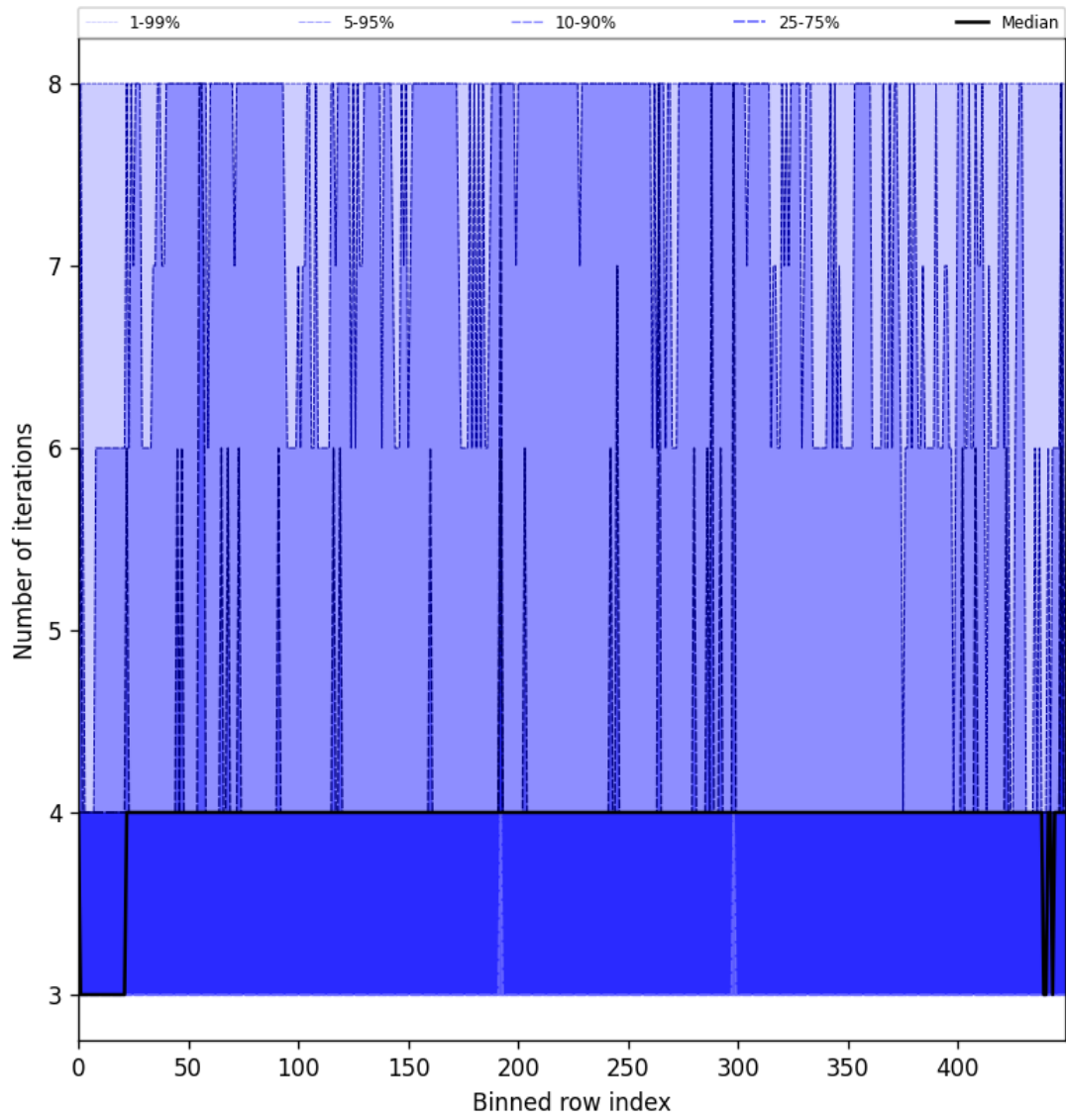
Figure 51: Along track statistics of “Number of iterations” for 2025-05-28 to 2025-05-30
