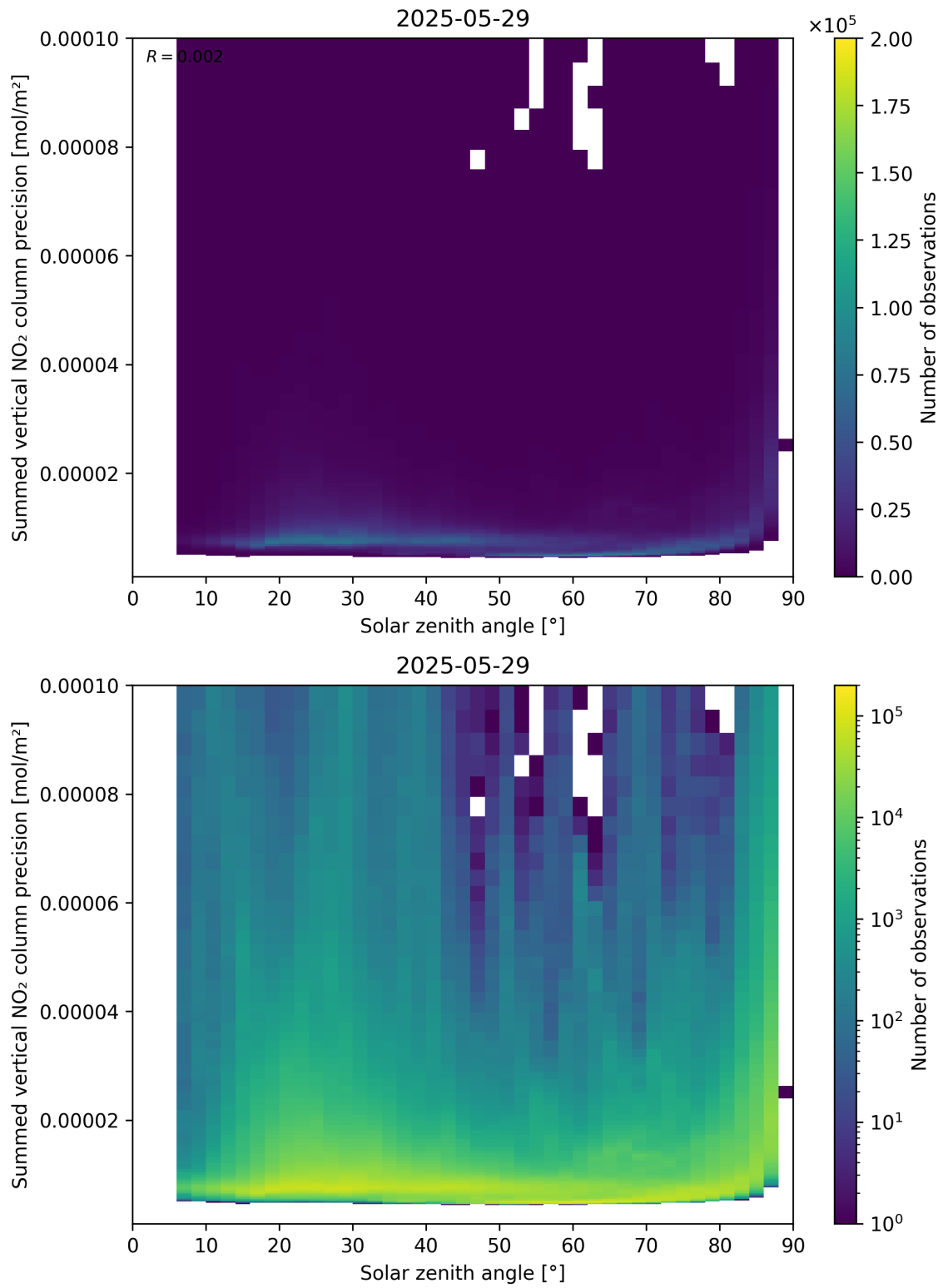
Figure 152: Scatter density plot of “Solar zenith angle” against “Summed vertical NO 2 column precision” for 2025-05-28 to 2025-05-30.
