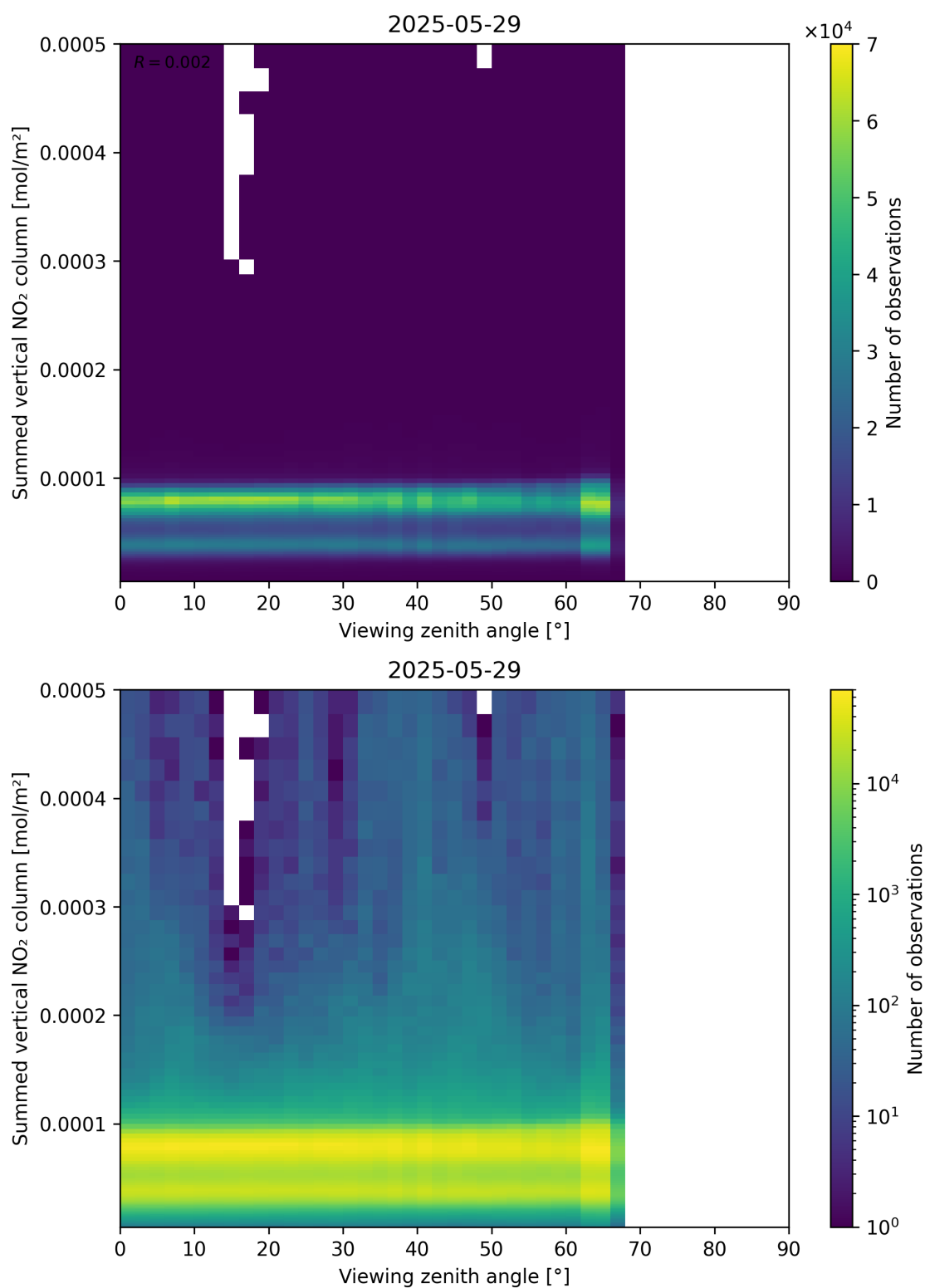
Figure 165: Scatter density plot of “Viewing zenith angle” against “Summed vertical NO 2 column” for 2025-05-28 to 2025-05-30.
