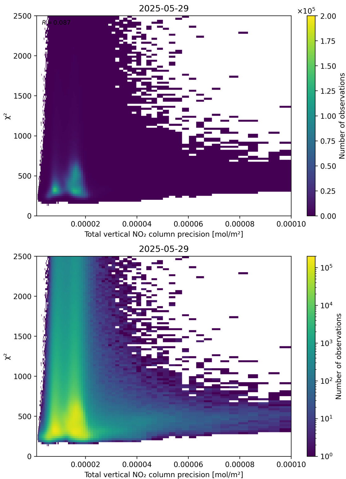
Figure 116: Scatter density plot of “Total vertical NO 2 column precision” against “ \chi^2 ” for 2025-05-28 to 2025-05-30.
