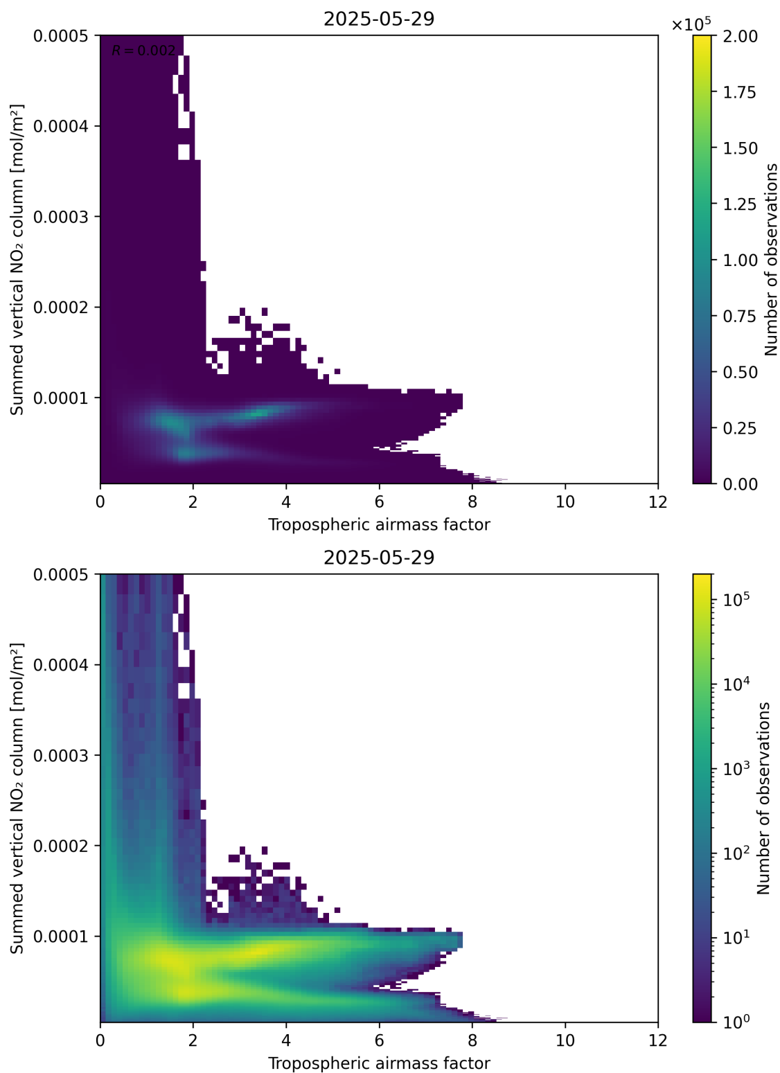
Figure 75: Scatter density plot of “Tropospheric air mass factor” against “Summed vertical NO 2 column” for 2025-05-28 to 2025-05-30.
