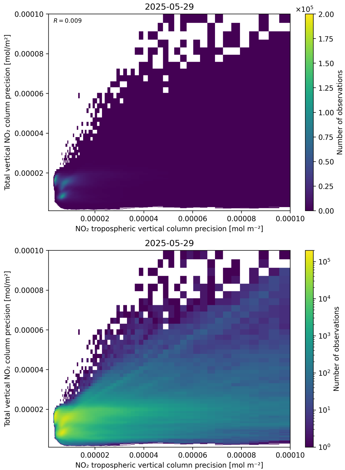
Figure 139: Scatter density plot of “NO 2 tropospheric vertical column precision” against “Total vertical NO 2 column precision” for 2025-05-28 to 2025-05-30.
