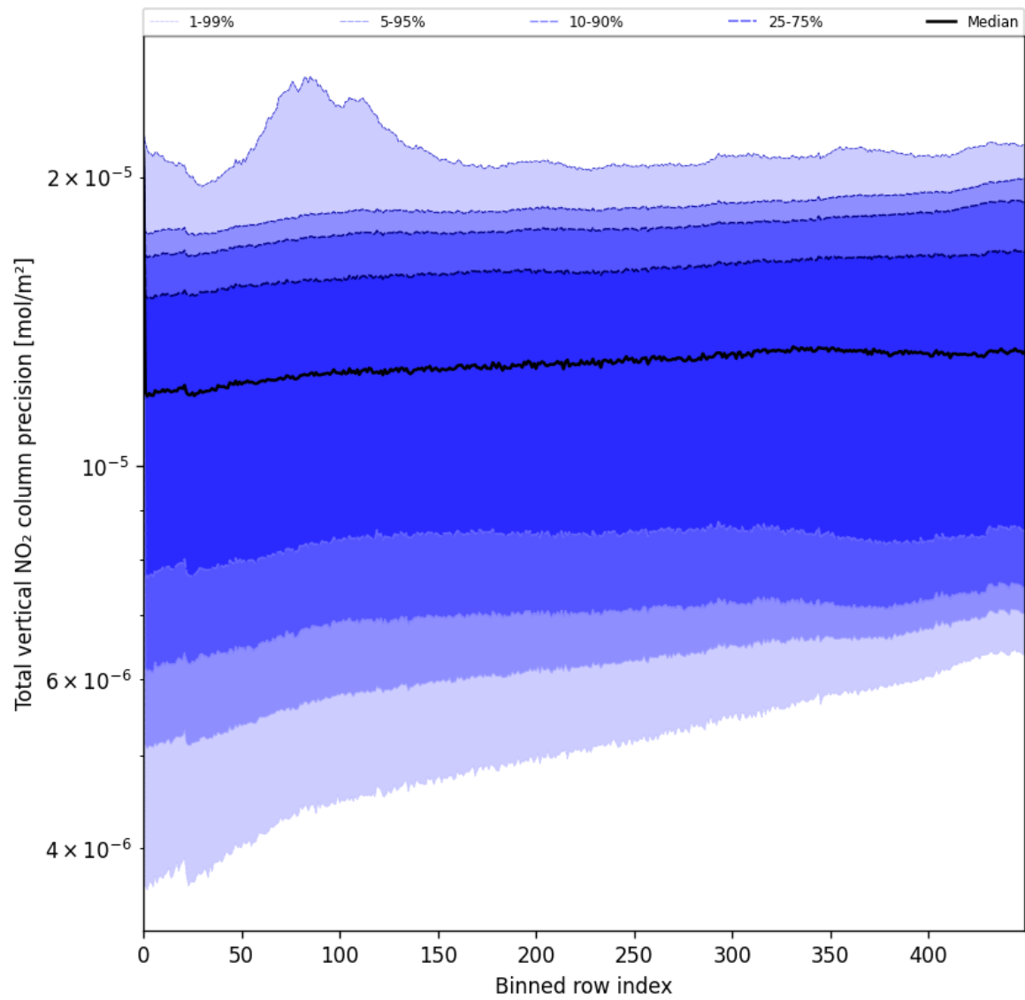
Figure 56: Along track statistics of “Total vertical NO 2 column precision” for 2025-05-28 to 2025-05-30
