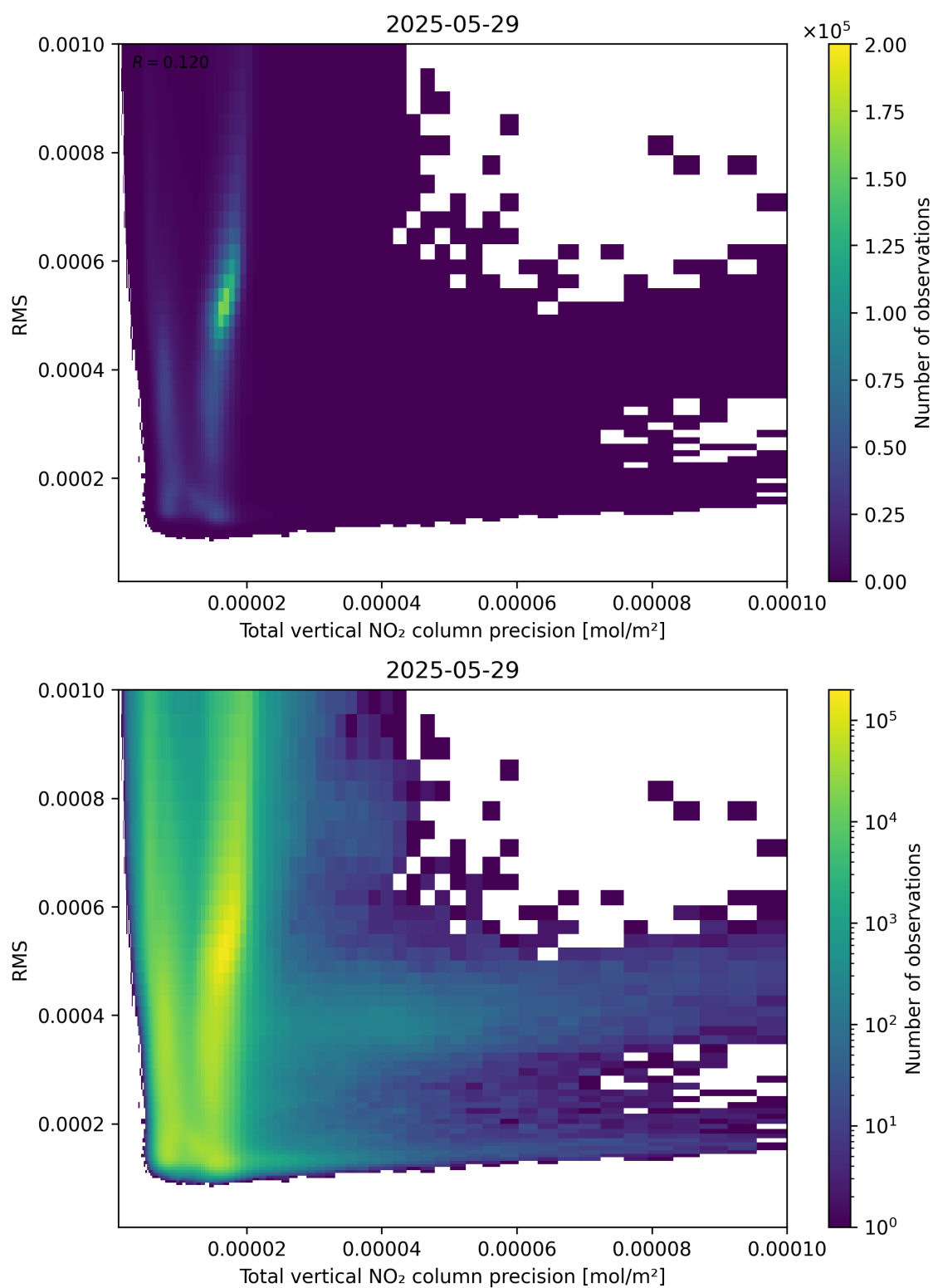
Figure 119: Scatter density plot of “Total vertical NO 2 column precision” against “RMS” for 2025-05-28 to 2025-05-30.
