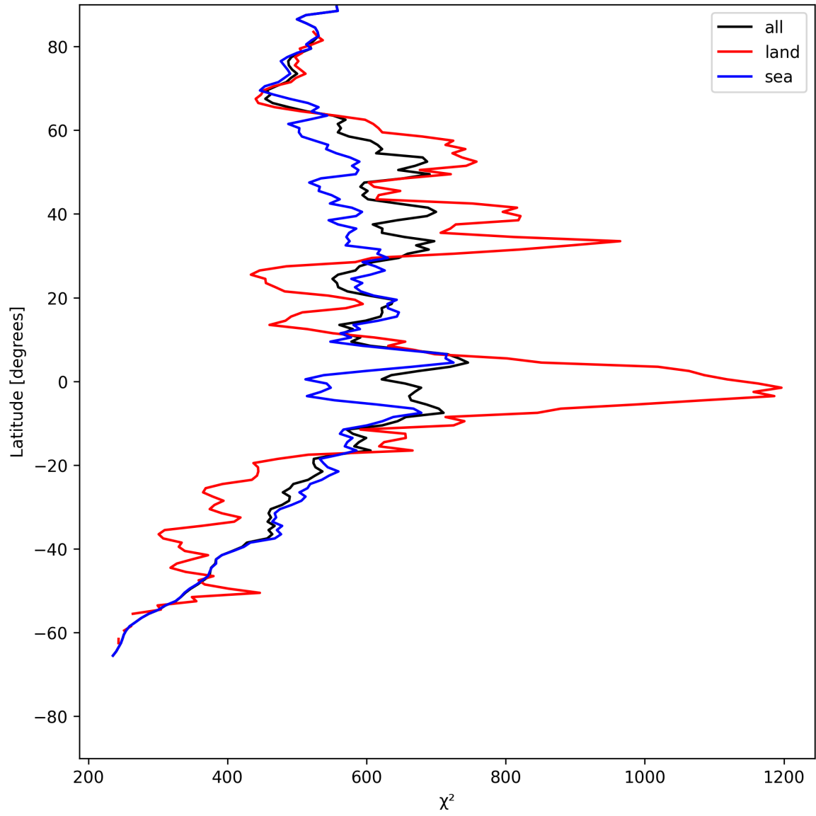
Figure 25: Zonal average of “ \chi^2 ” for 2025-05-28 to 2025-05-30.
