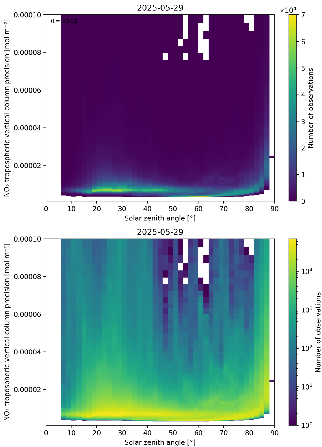
Figure 156: Scatter density plot of “Solar zenith angle” against “NO 2 tropospheric vertical column precision” for 2025-05-28 to 2025-05-30.
