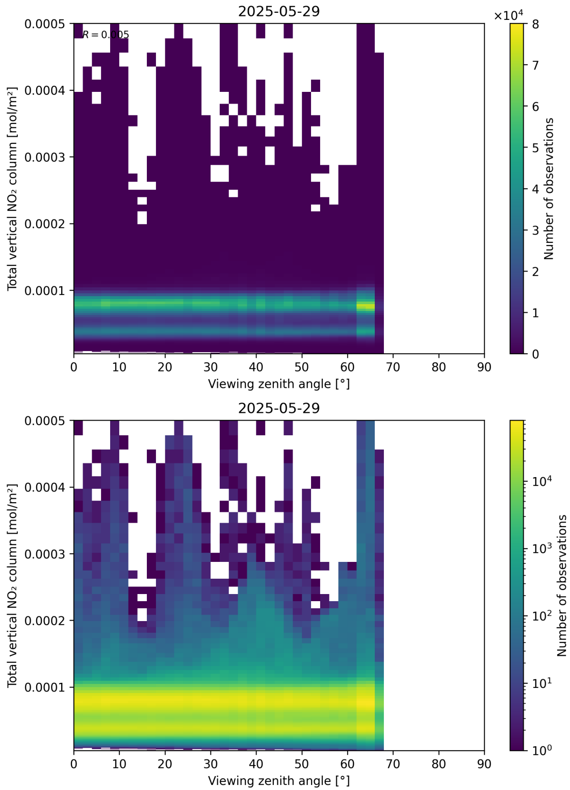
Figure 167: Scatter density plot of “Viewing zenith angle” against “Total vertical NO 2 column” for 2025-05-28 to 2025-05-30.
