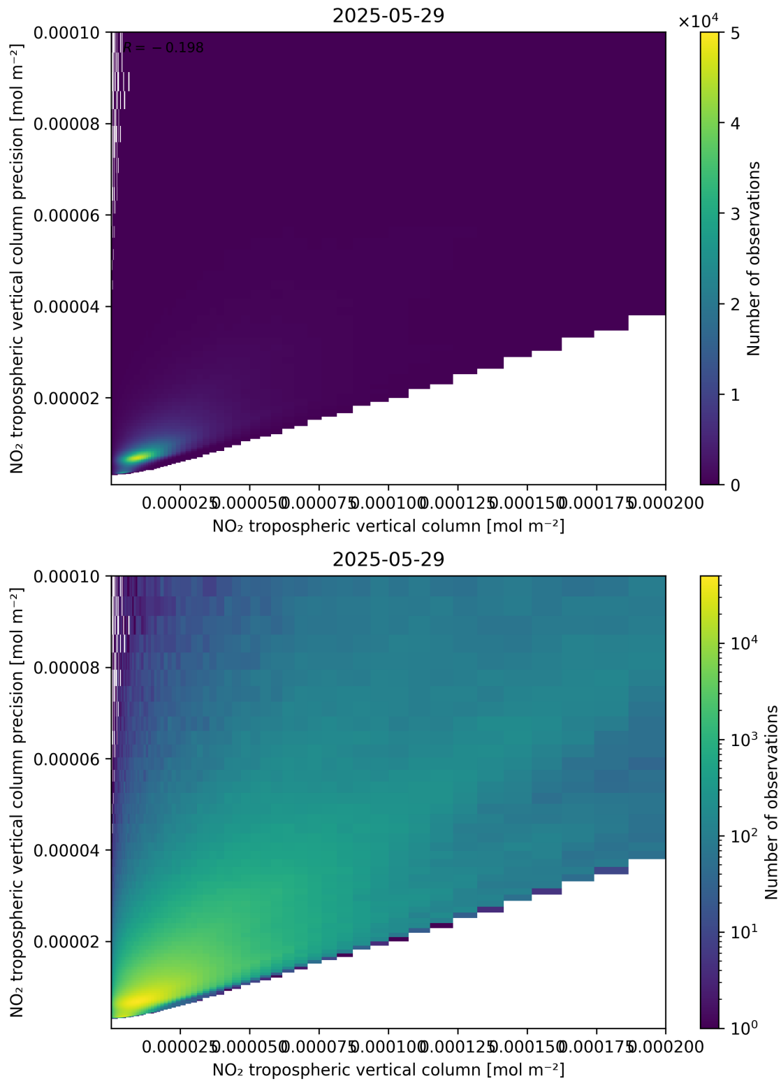
Figure 130: Scatter density plot of “NO 2 tropospheric vertical column” against “NO 2 tropospheric vertical column precision” for 2025-05-28 to 2025-05-30.
