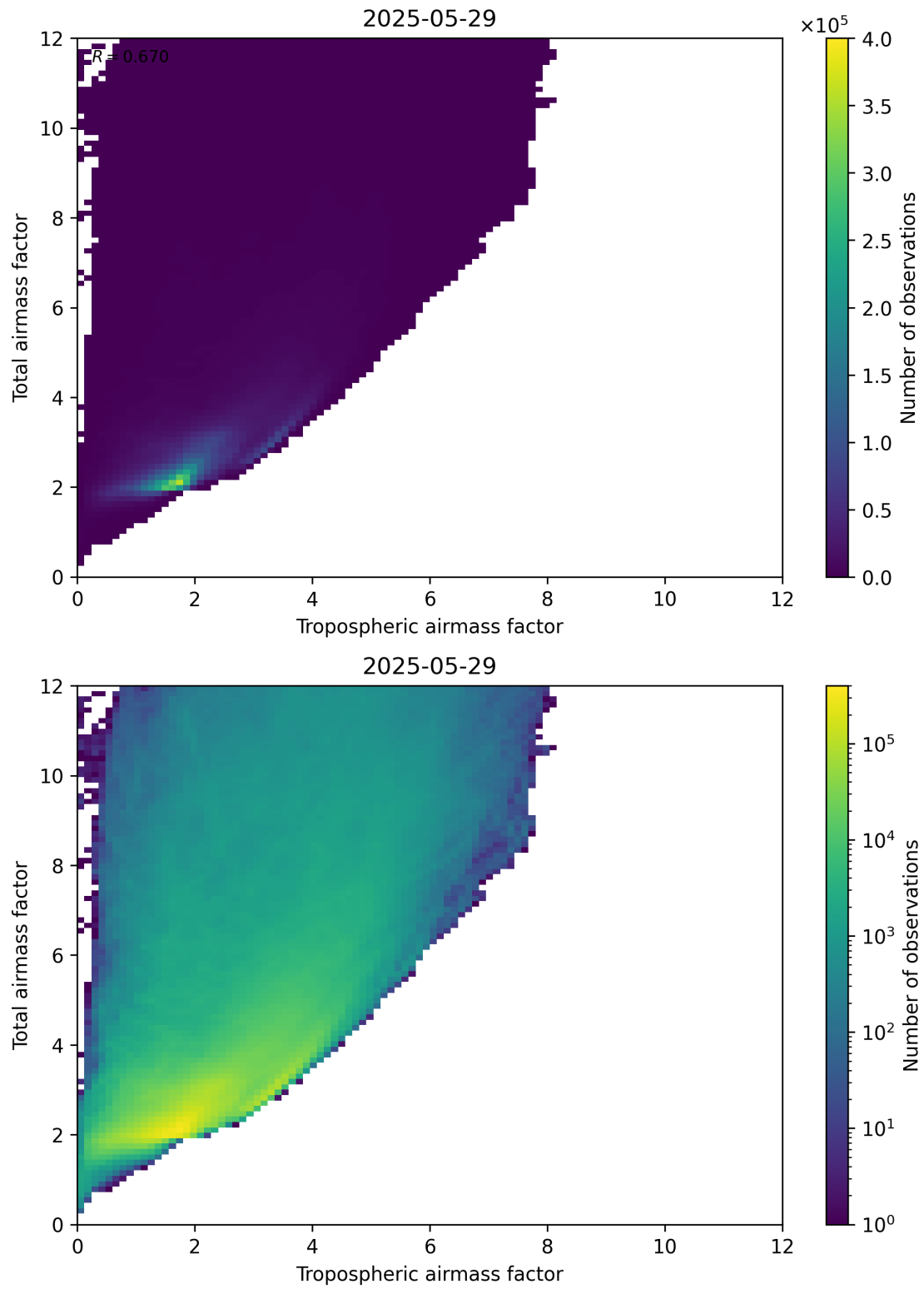
Figure 72: Scatter density plot of “Tropospheric airmass factor” against “Total airmass factor” for 2025-05-28 to 2025-05-30.
