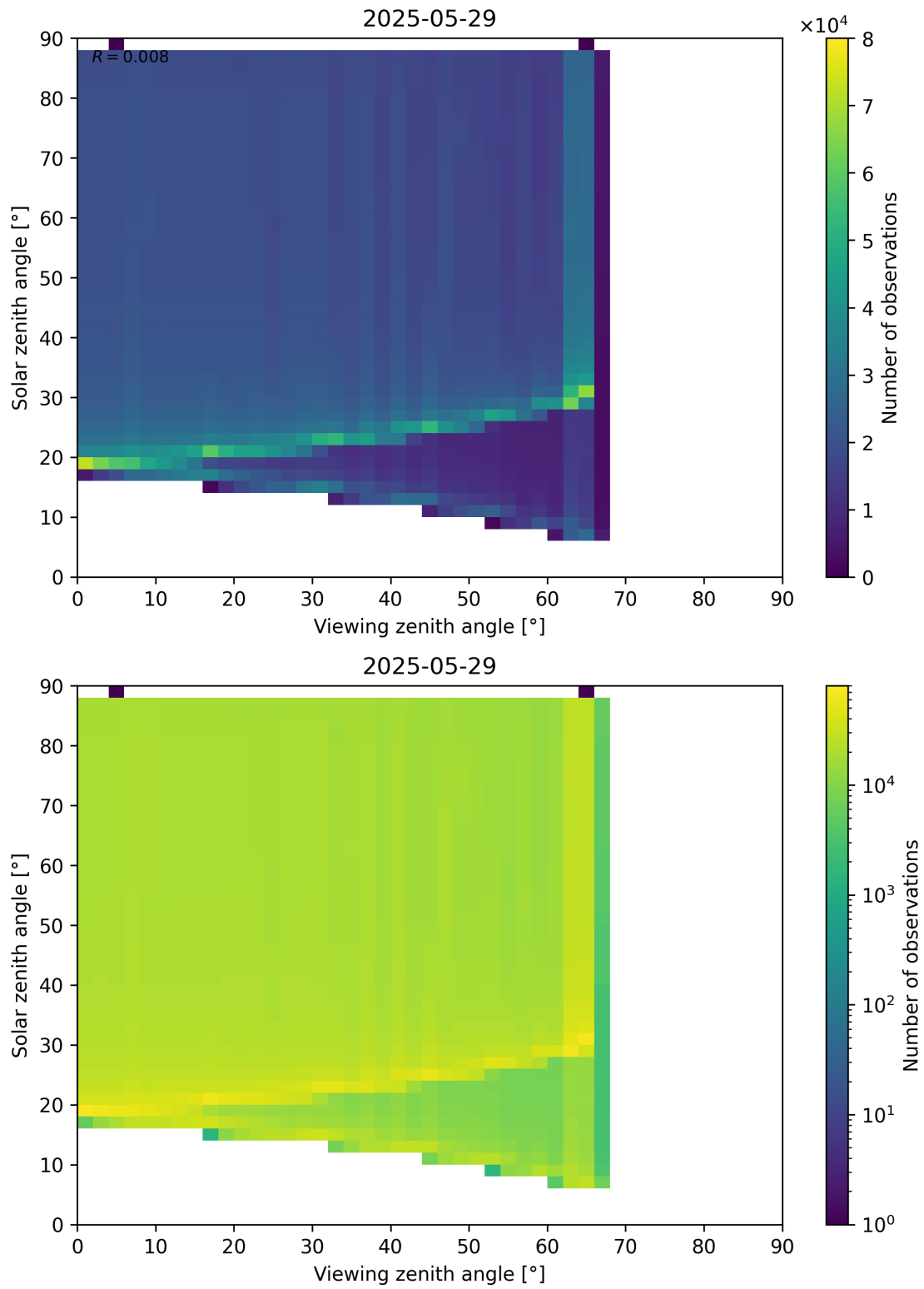
Figure 172: Scatter density plot of “Viewing zenith angle” against “Solar zenith angle” for 2025-05-28 to 2025-05-30.
