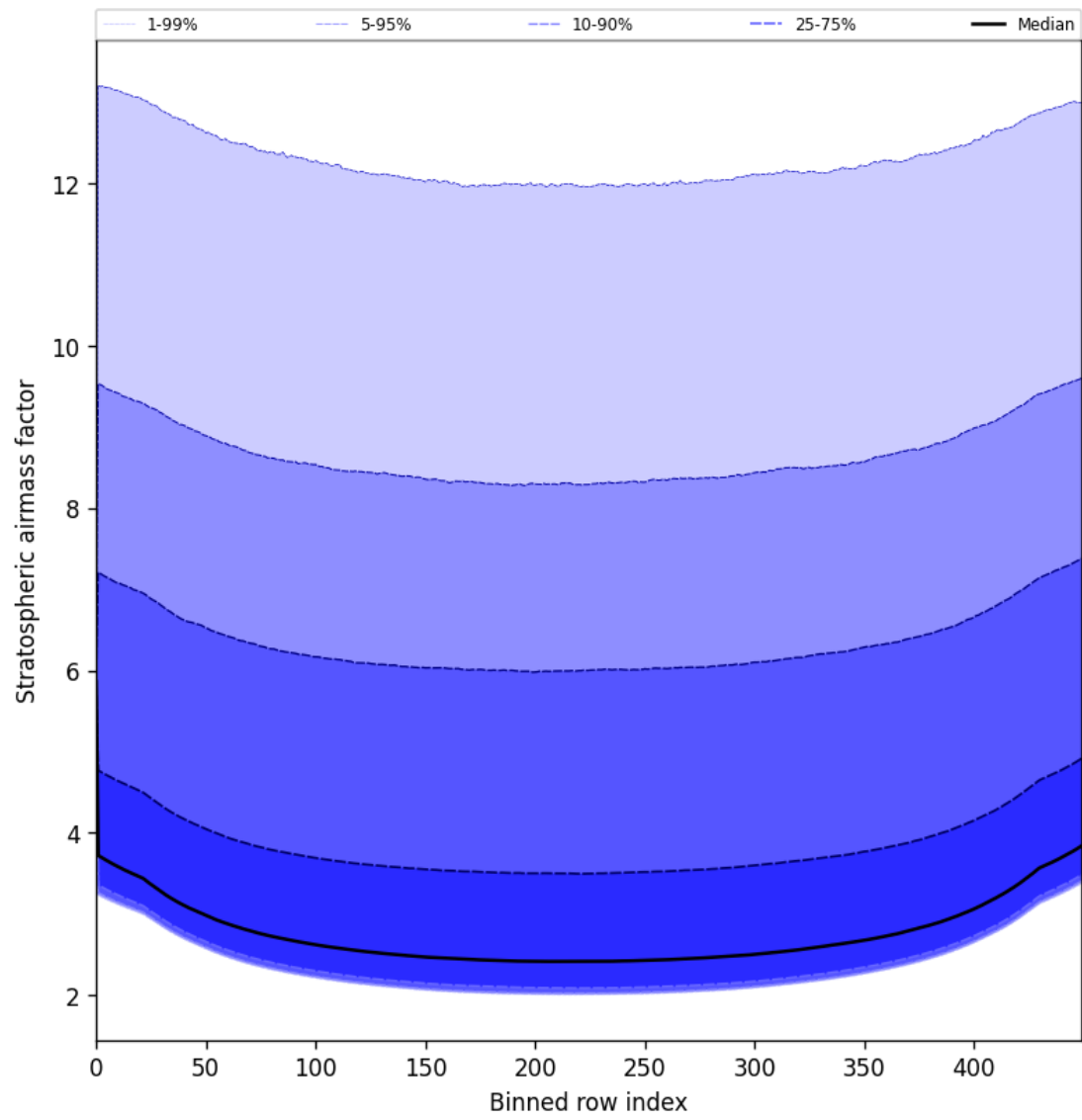
Figure 61: Along track statistics of “Stratospheric airmass factor” for 2025-05-28 to 2025-05-30
