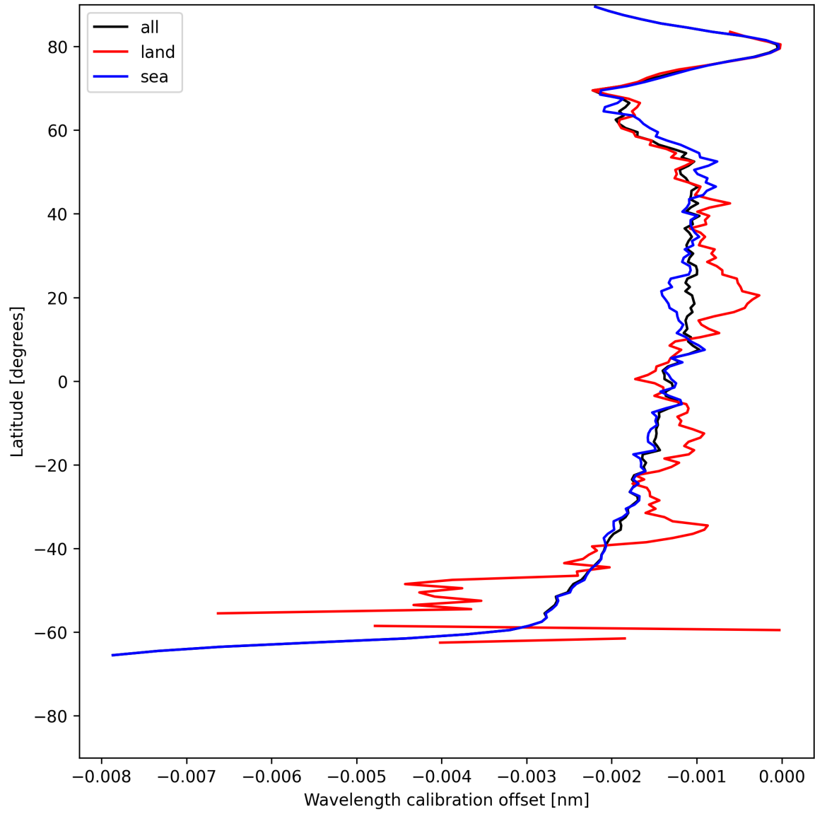
Figure 18: Zonal average of “Wavelength calibration offset” for 2025-05-28 to 2025-05-30.
