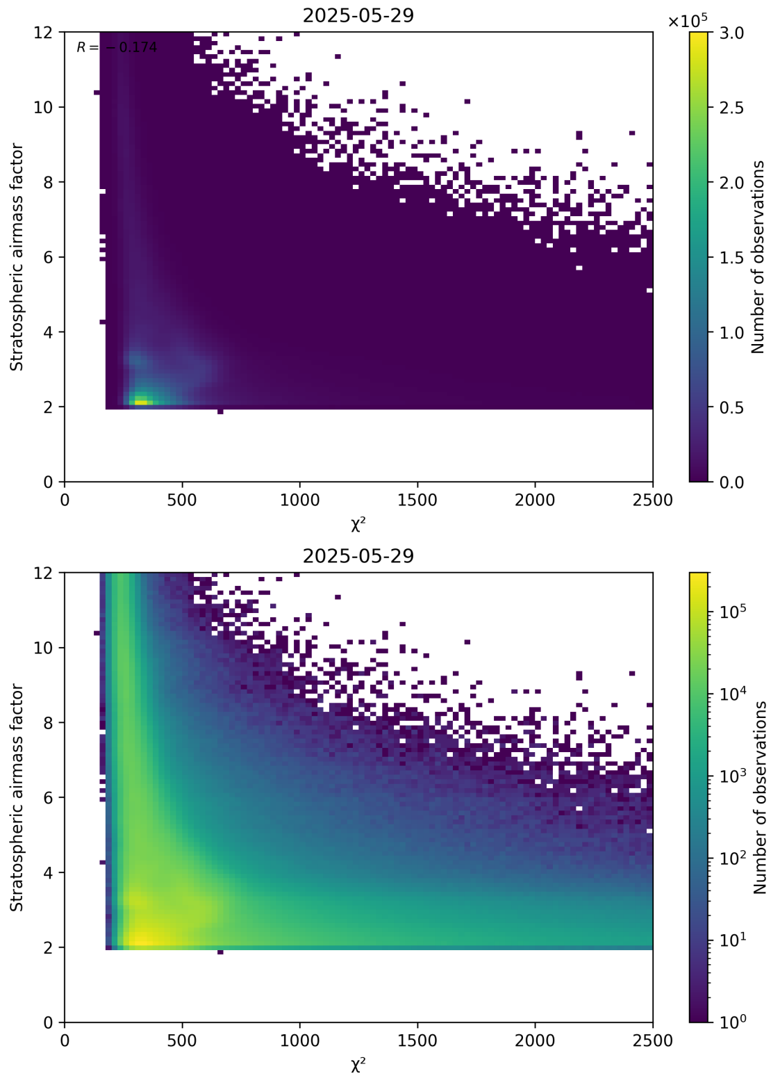
Figure 81: Scatter density plot of “ \chi^2 ” against “Stratospheric airmass factor” for 2025-05-28 to 2025-05-30.
