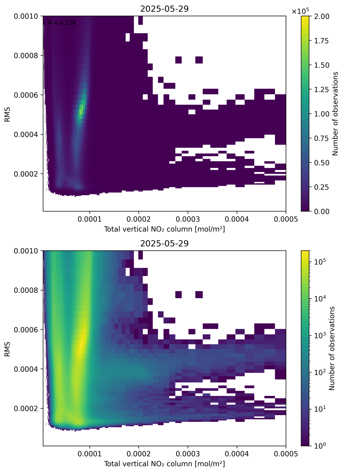
Figure 120: Scatter density plot of “Total vertical NO 2 column” against “RMS” for 2025-05-28 to 2025-05-30.
