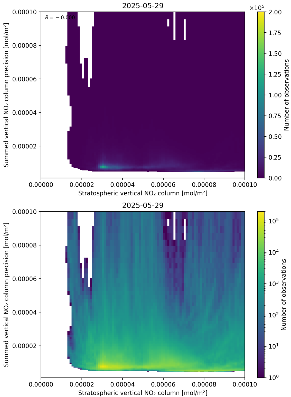
Figure 99: Scatter density plot of “Stratospheric vertical NO 2 column” against “Summed vertical NO 2 column precision” for 2025-05-28 to 2025-05-30.
