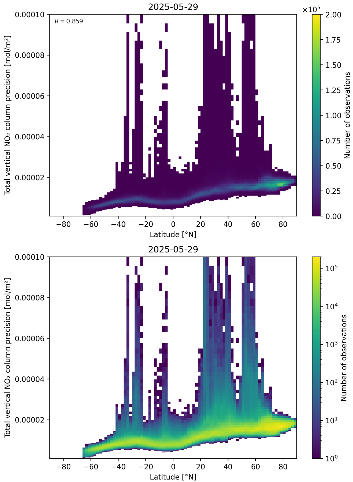
Figure 91: Scatter density plot of “Latitude” against “Total vertical NO 2 column precision” for 2025-05-28 to 2025-05-30.
