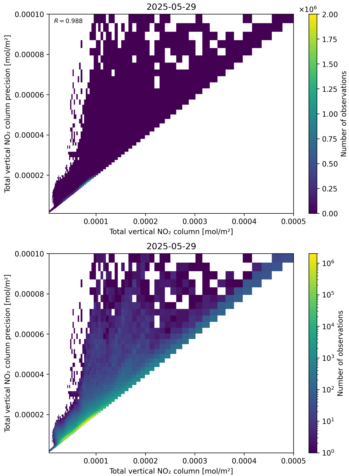
Figure 114: Scatter density plot of “Total vertical NO 2 column” against “Total vertical NO 2 column precision” for 2025-05-28 to 2025-05-30.
