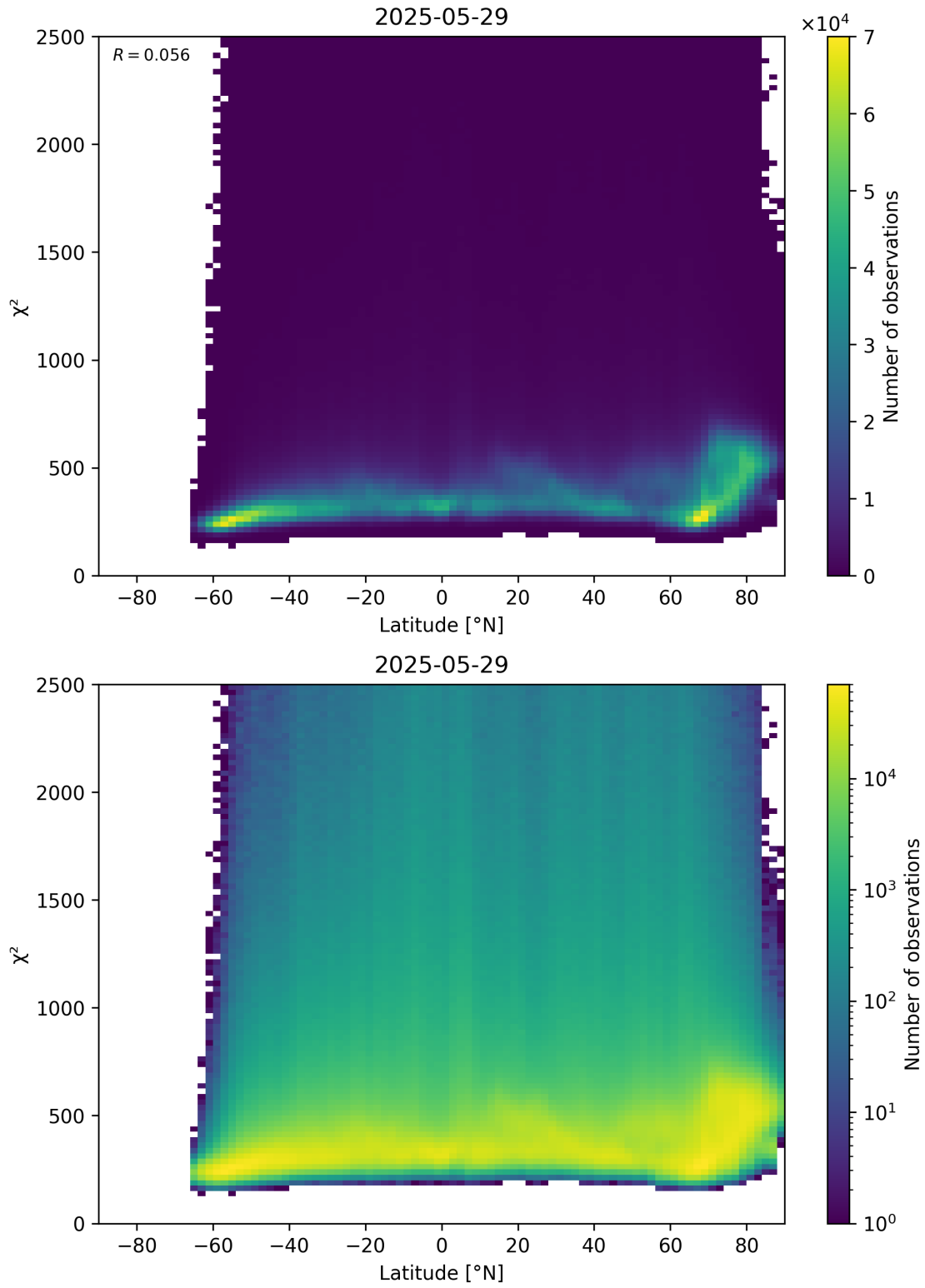
Figure 86: Scatter density plot of “Latitude” against “ \chi^2 ” for 2025-05-28 to 2025-05-30.
