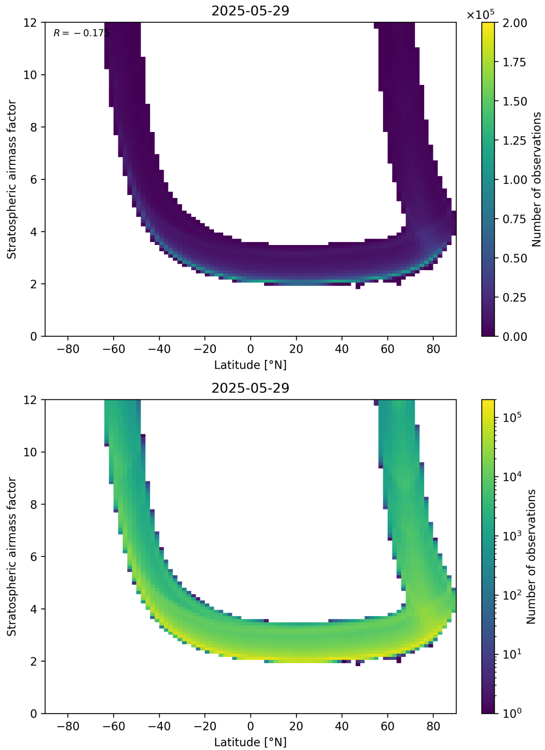
Figure 83: Scatter density plot of “Latitude” against “Stratospheric air mass factor” for 2025-05-28 to 2025-05-30.
