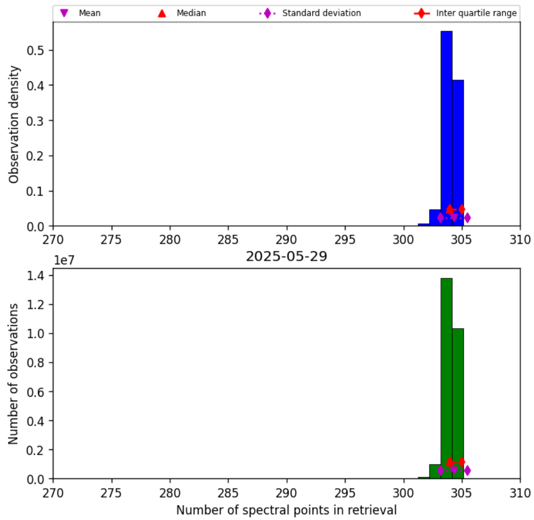
Figure 33: Histogram of “Number of spectral points in retrieval” for 2025-05-28 to 2025-05-30
