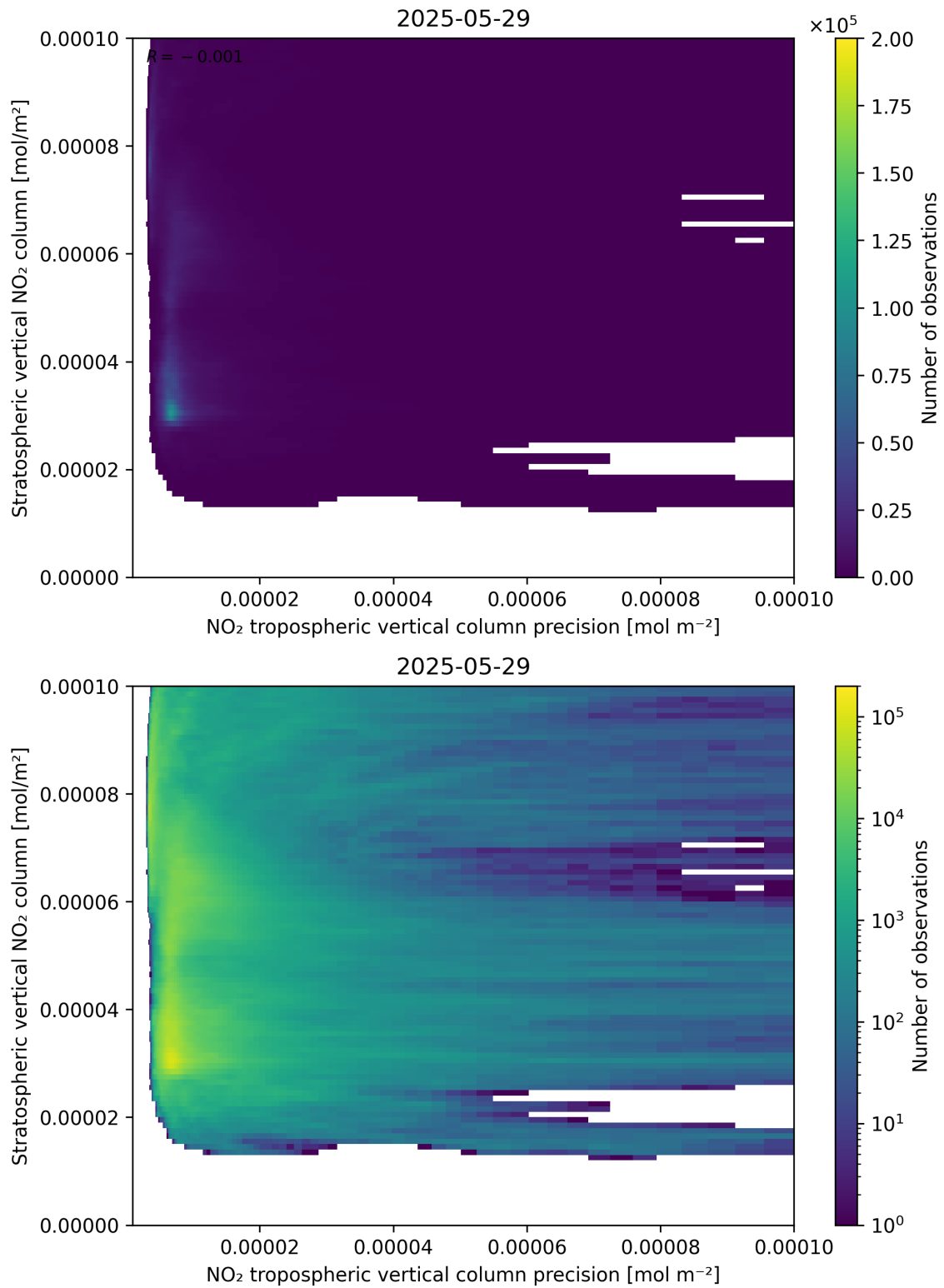
Figure 135: Scatter density plot of “NO 2 tropospheric vertical column precision” against “Stratospheric vertical NO 2 column” for 2025-05-28 to 2025-05-30.
