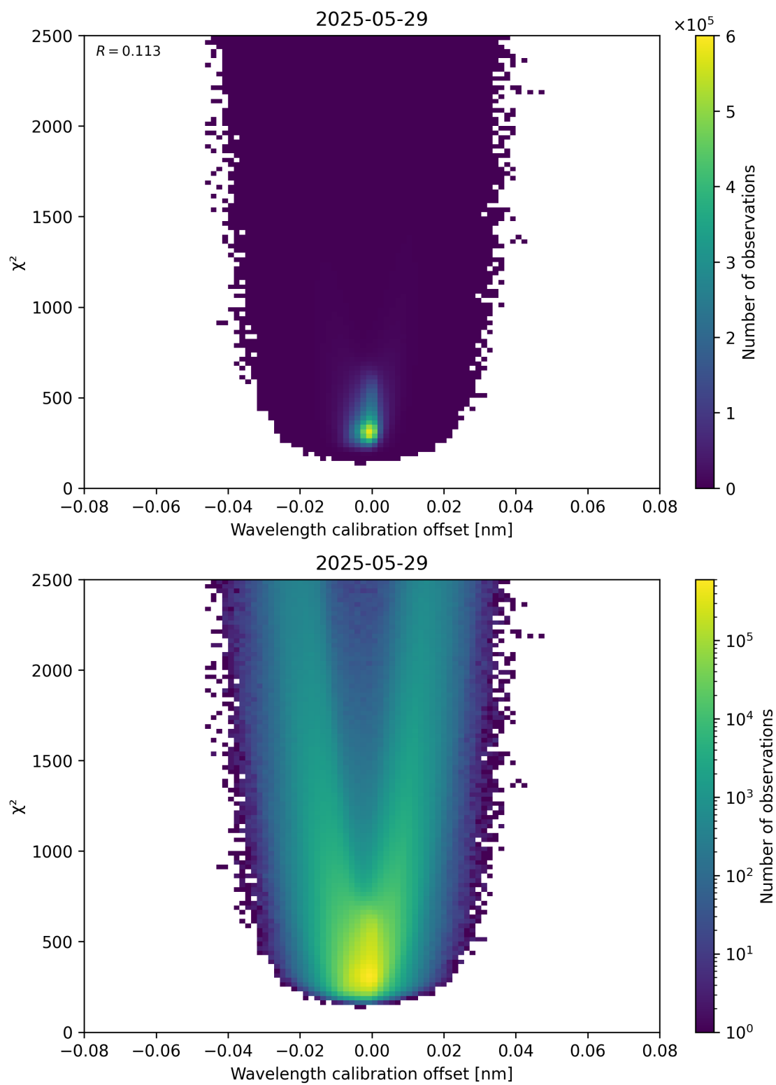
Figure 175: Scatter density plot of “Wavelength calibration offset” against “ \chi^2 ” for 2025-05-28 to 2025-05-30.
