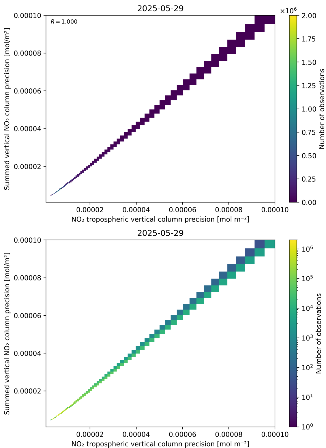
Figure 137: Scatter density plot of “NO 2 tropospheric vertical column precision” against “Summed vertical NO 2 column precision” for 2025-05-28 to 2025-05-30.
