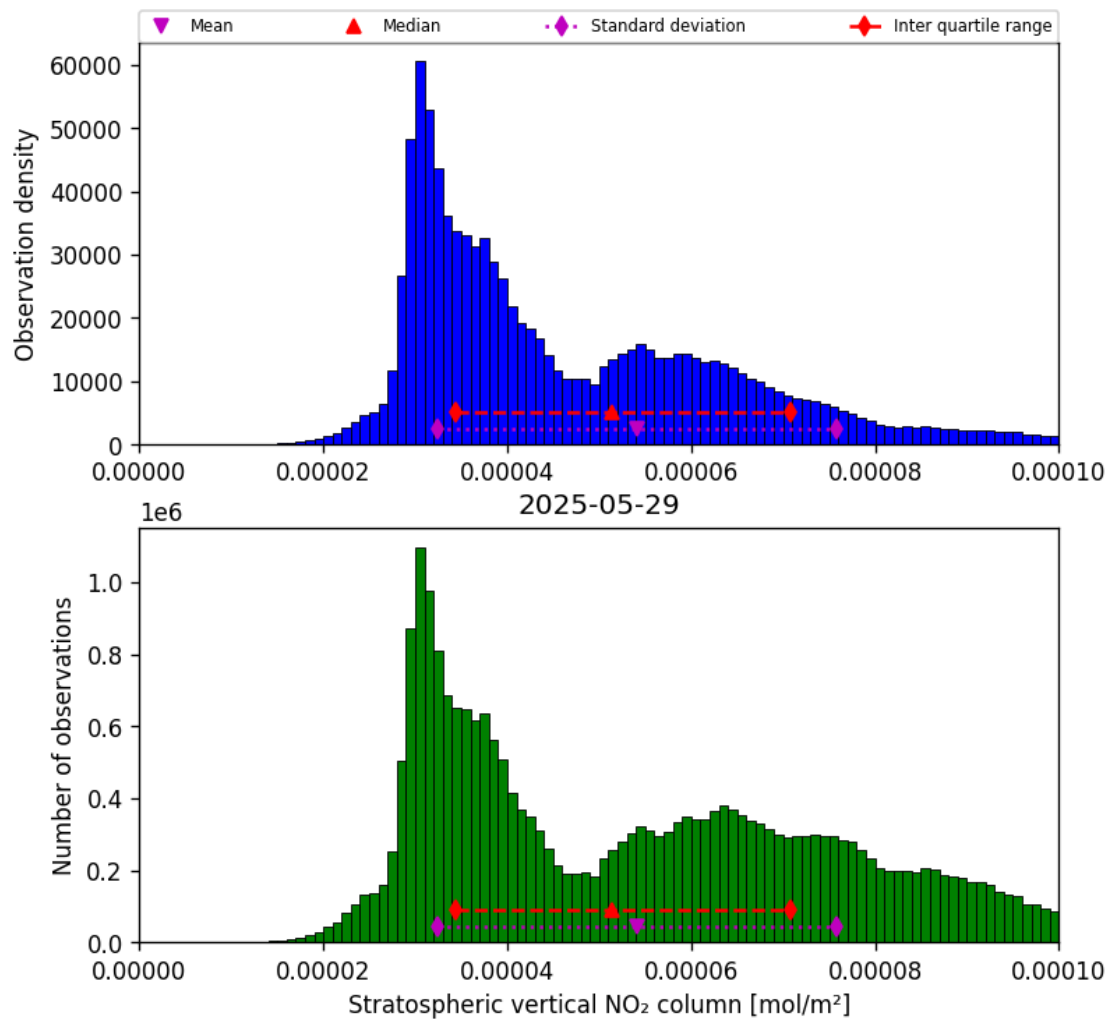
Figure 36: Histogram of “Stratospheric vertical NO 2 column” for 2025-05-28 to 2025-05-30
