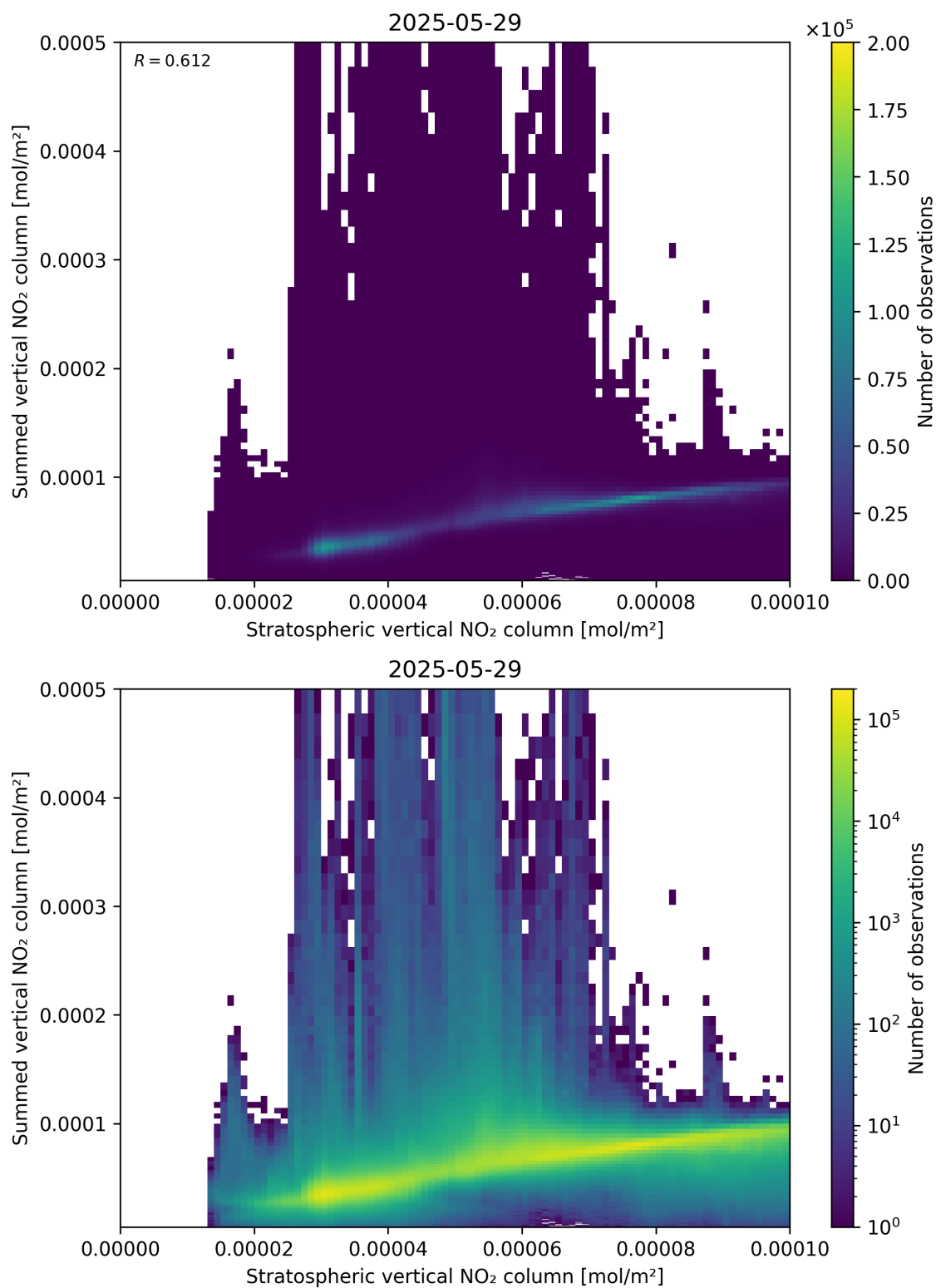
Figure 98: Scatter density plot of “Stratospheric vertical NO 2 column” against “Summed vertical NO 2 column” for 2025-05-28 to 2025-05-30.
