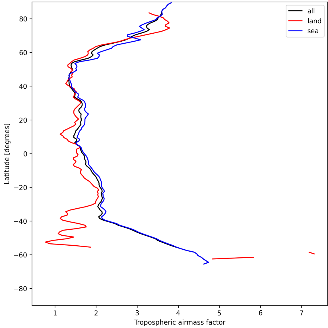
Figure 14: Zonal average of “Tropospheric airmass factor” for 2025-05-28 to 2025-05-30.
