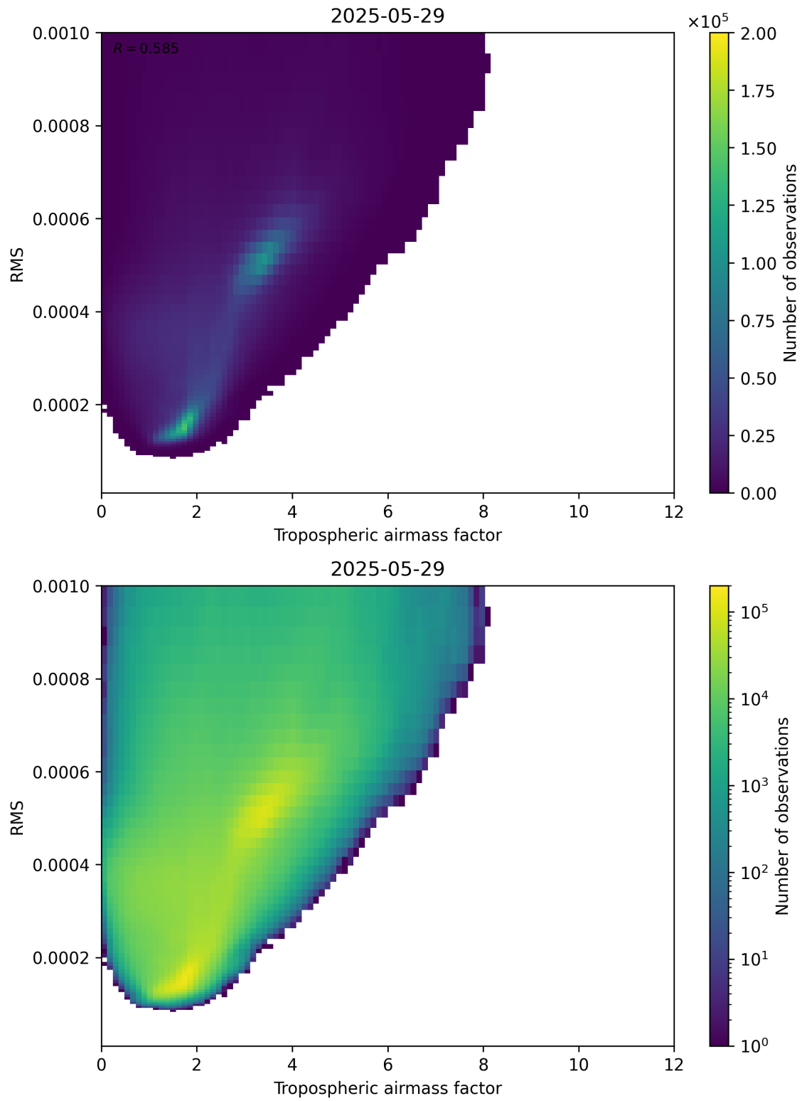
Figure 79: Scatter density plot of “Tropospheric airmass factor” against “RMS” for 2025-05-28 to 2025-05-30.
