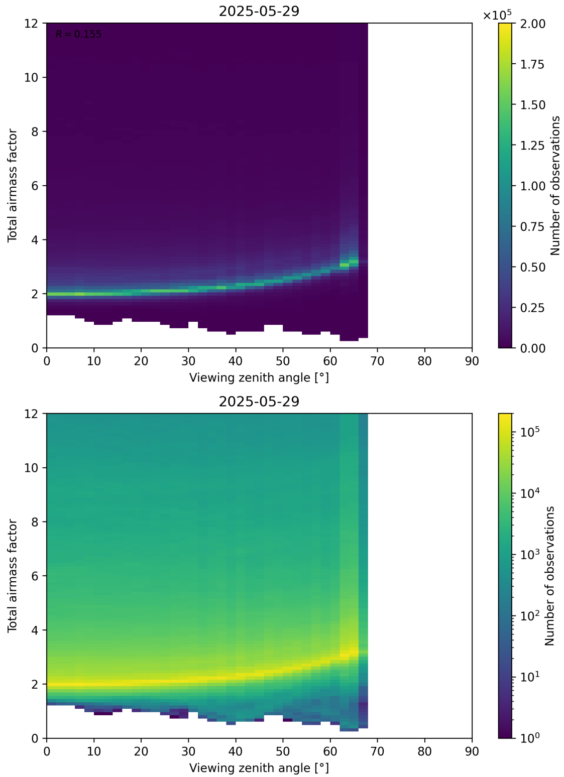
Figure 160: Scatter density plot of “Viewing zenith angle” against “Total airmass factor” for 2025-05-28 to 2025-05-30.
