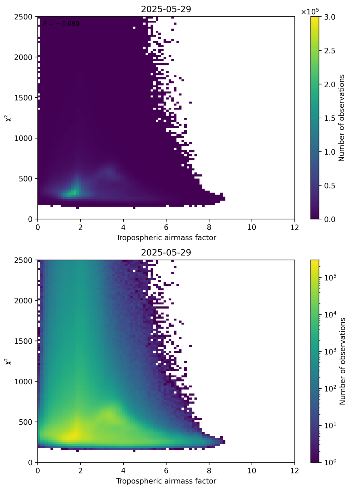
Figure 73: Scatter density plot of “Tropospheric airmass factor” against “ \chi^2 ” for 2025-05-28 to 2025-05-30.
