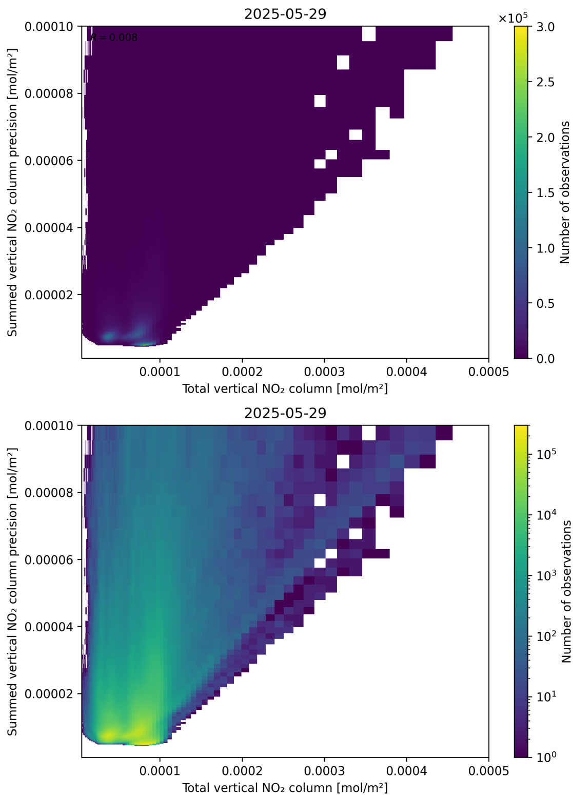
Figure 113: Scatter density plot of “Total vertical NO 2 column” against “Summed vertical NO 2 column precision” for 2025-05-28 to 2025-05-30.
