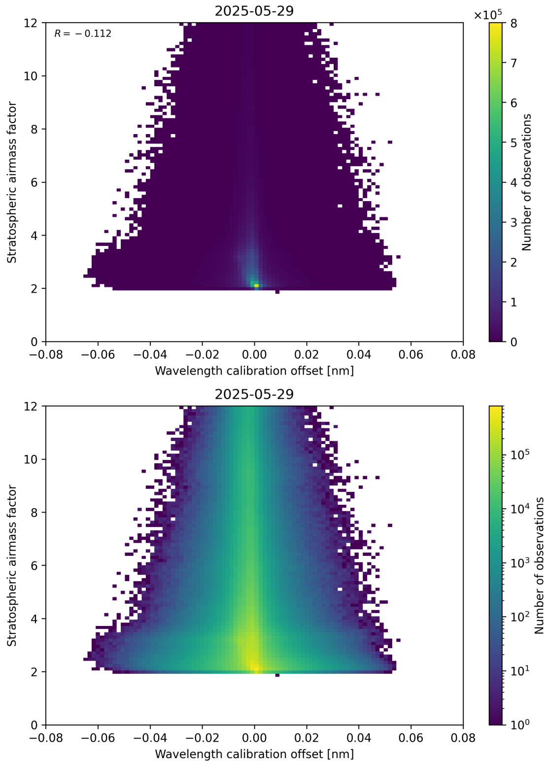
Figure 174: Scatter density plot of “Wavelength calibration offset” against “Stratospheric airmass factor” for 2025-05-28 to 2025-05-30.
