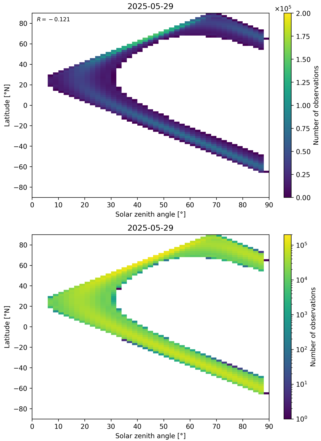
Figure 149: Scatter density plot of “Solar zenith angle” against “Latitude” for 2025-05-28 to 2025-05-30.
