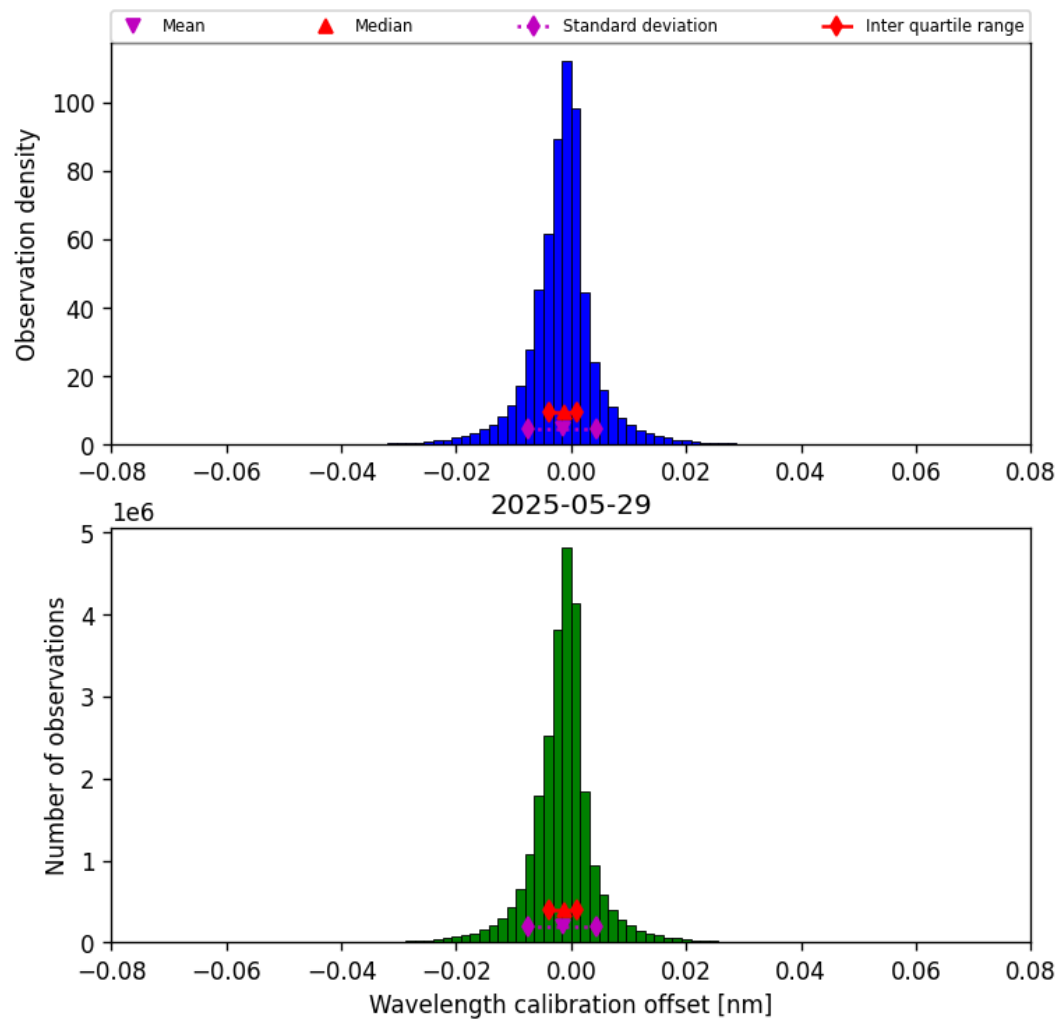
Figure 35: Histogram of “Wavelength calibration offset” for 2025-05-28 to 2025-05-30
