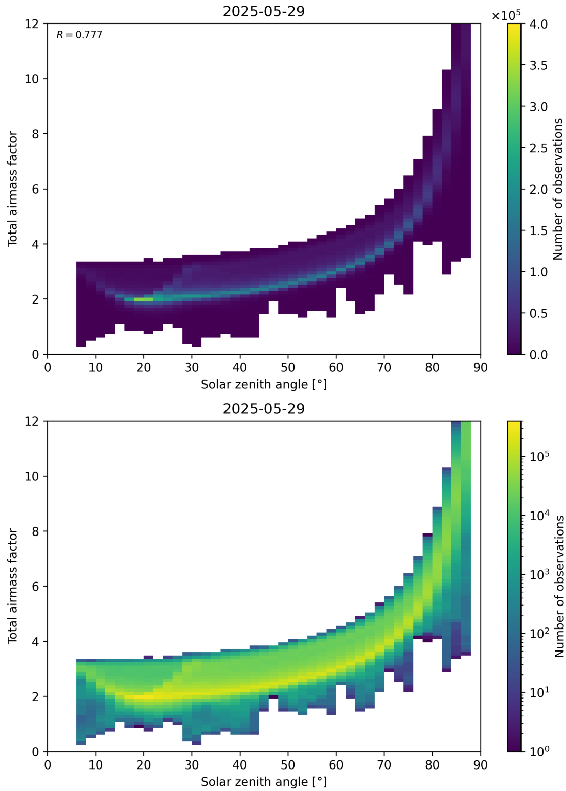
Figure 146: Scatter density plot of “Solar zenith angle” against “Total air mass factor” for 2025-05-28 to 2025-05-30.
