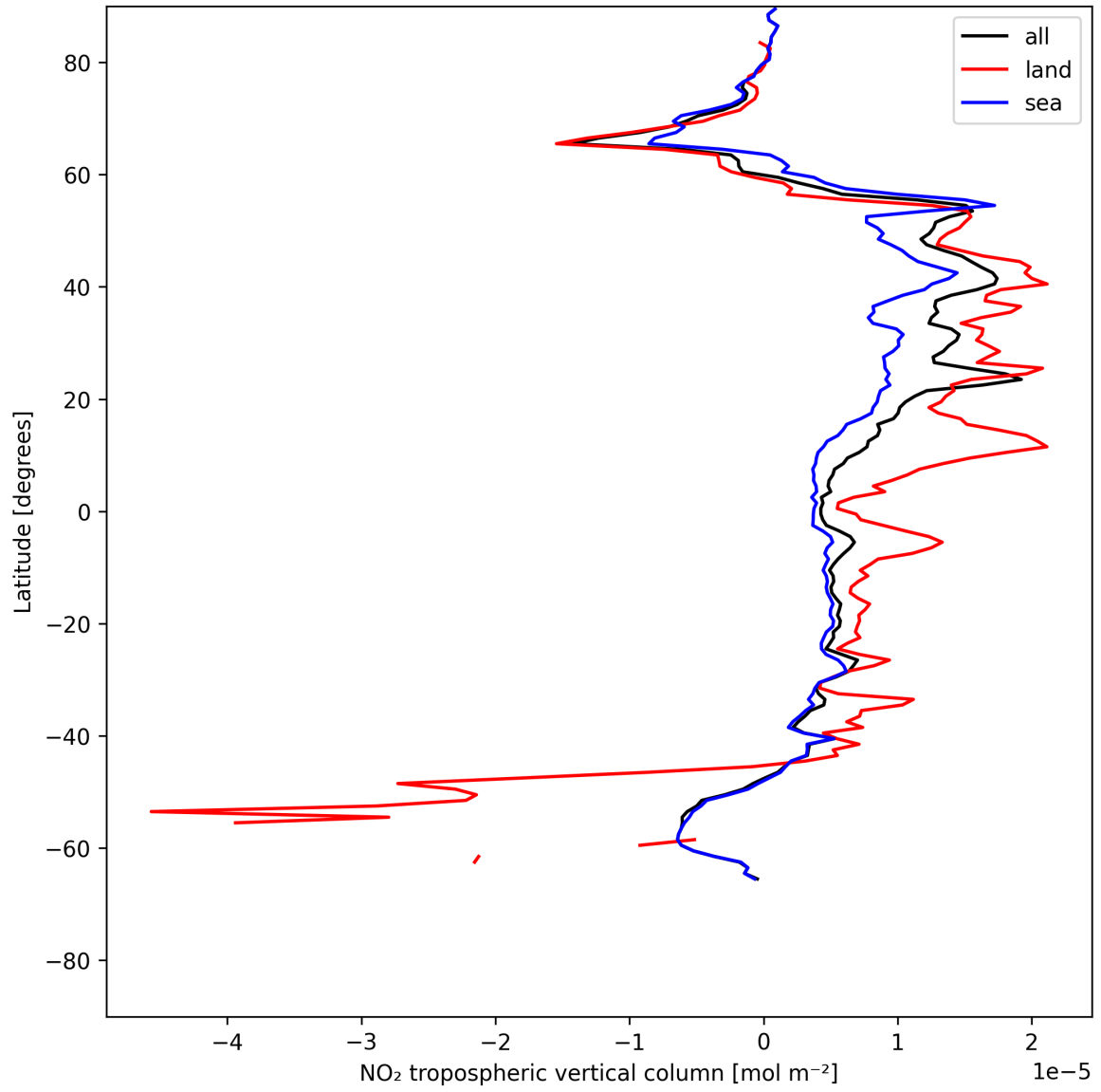
Figure 12: Zonal average of “NO 2 tropospheric vertical column” for 2025-05-28 to 2025-05-30.
