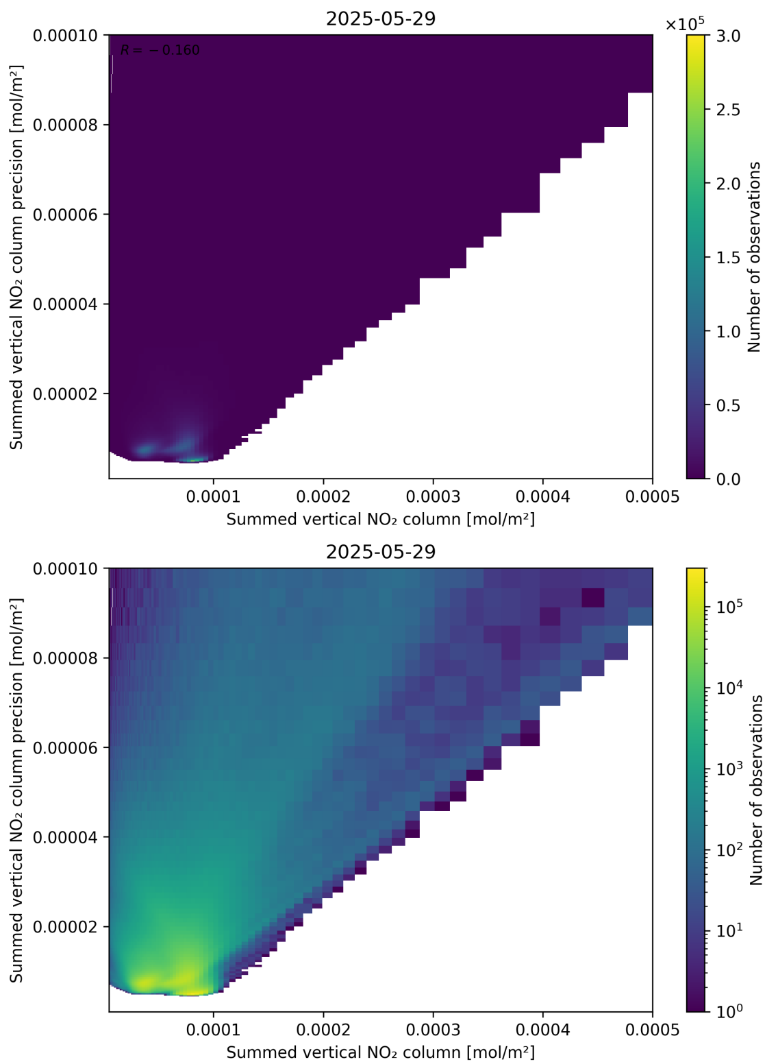
Figure 105: Scatter density plot of “Summed vertical NO 2 column” against “Summed vertical NO 2 column precision” for 2025-05-28 to 2025-05-30.
