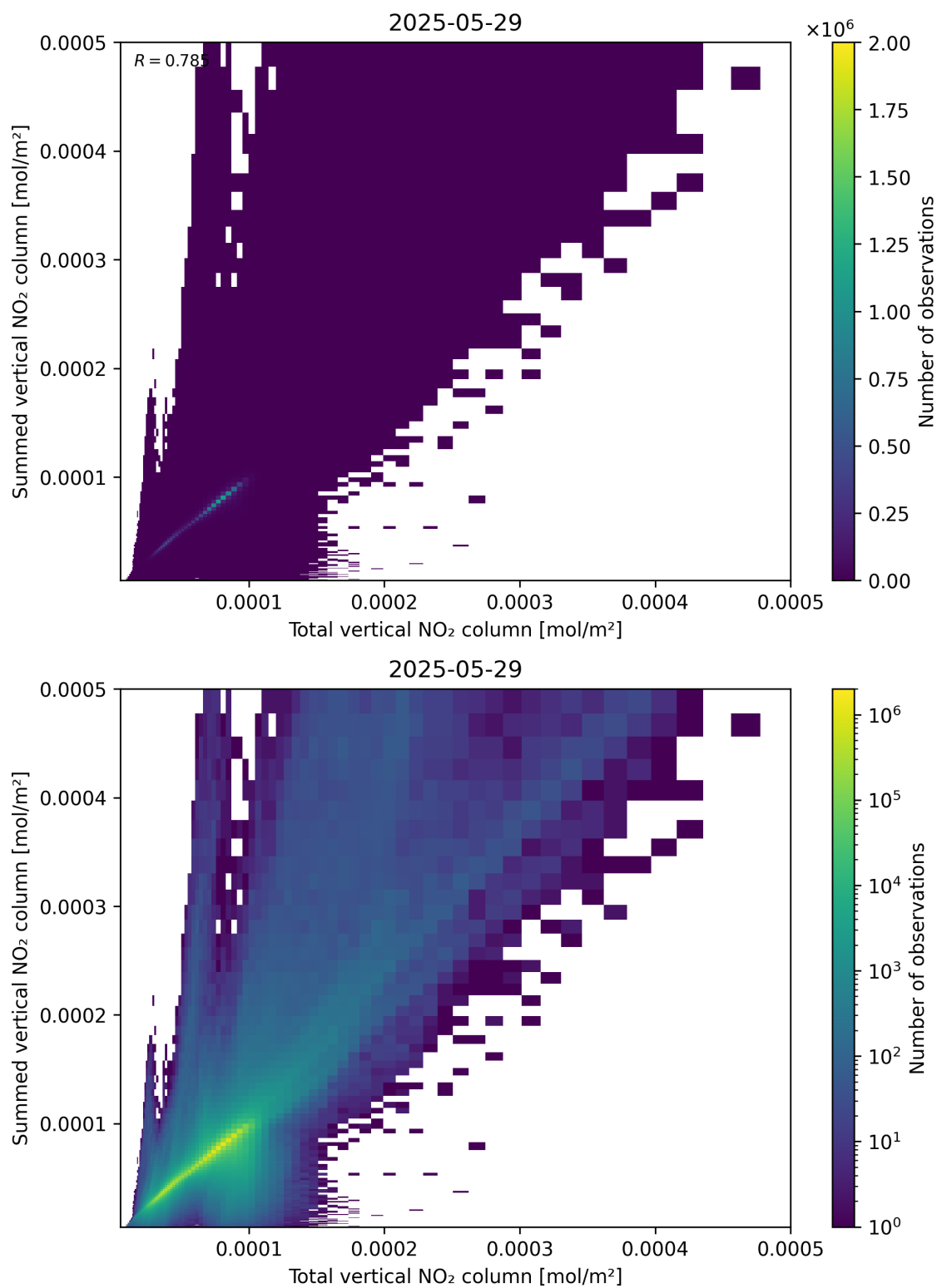
Figure 112: Scatter density plot of “Total vertical NO 2 column” against “Summed vertical NO 2 column” for 2025-05-28 to 2025-05-30.
