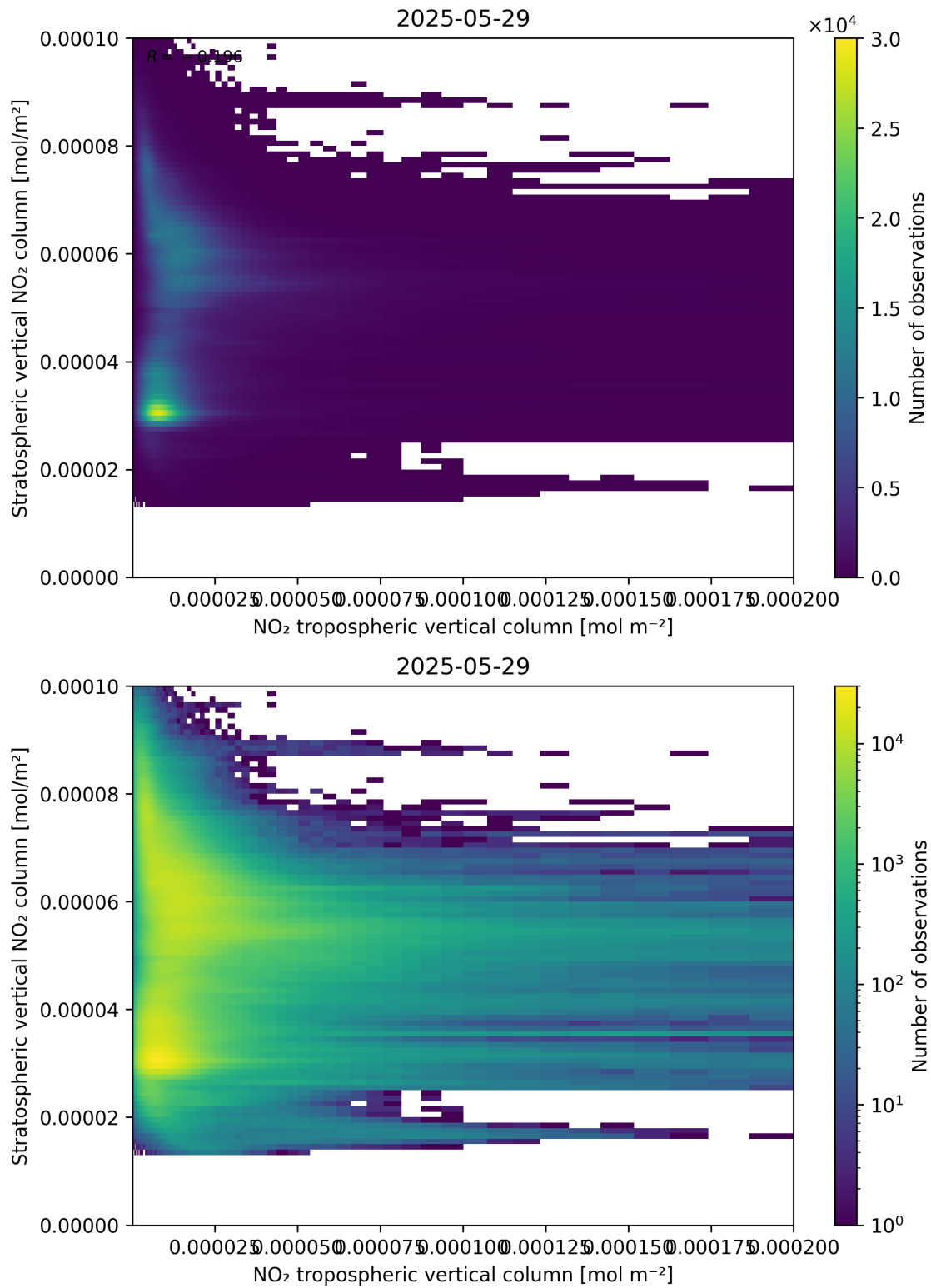
Figure 125: Scatter density plot of “NO 2 tropospheric vertical column” against “Stratospheric vertical NO 2 column” for 2025-05-28 to 2025-05-30.
