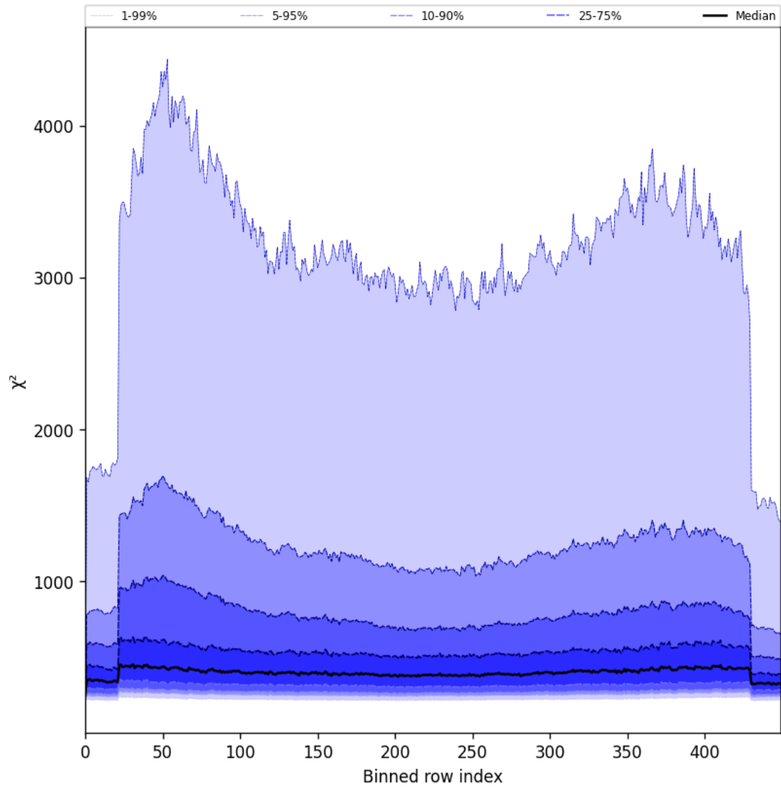
Figure 59: Along track statistics of “ \chi^2 ” for 2025-05-28 to 2025-05-30
