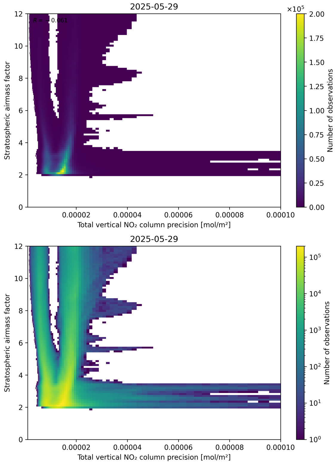
Figure 115: Scatter density plot of “Total vertical NO 2 column precision” against “Stratospheric air mass factor” for 2025-05-28 to 2025-05-30.
