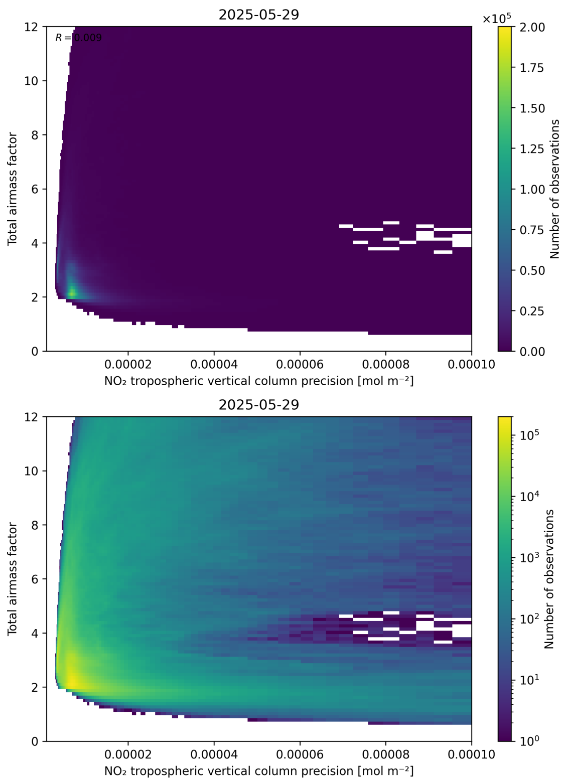
Figure 132: Scatter density plot of “NO 2 tropospheric vertical column precision” against “Total air mass factor” for 2025-05-28 to 2025-05-30.
