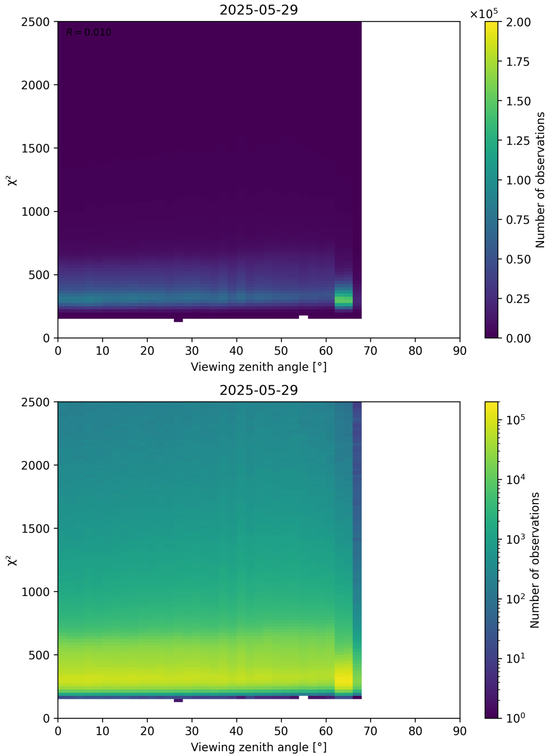
Figure 162: Scatter density plot of “Viewing zenith angle” against “ \chi^2 ” for 2025-05-28 to 2025-05-30.
