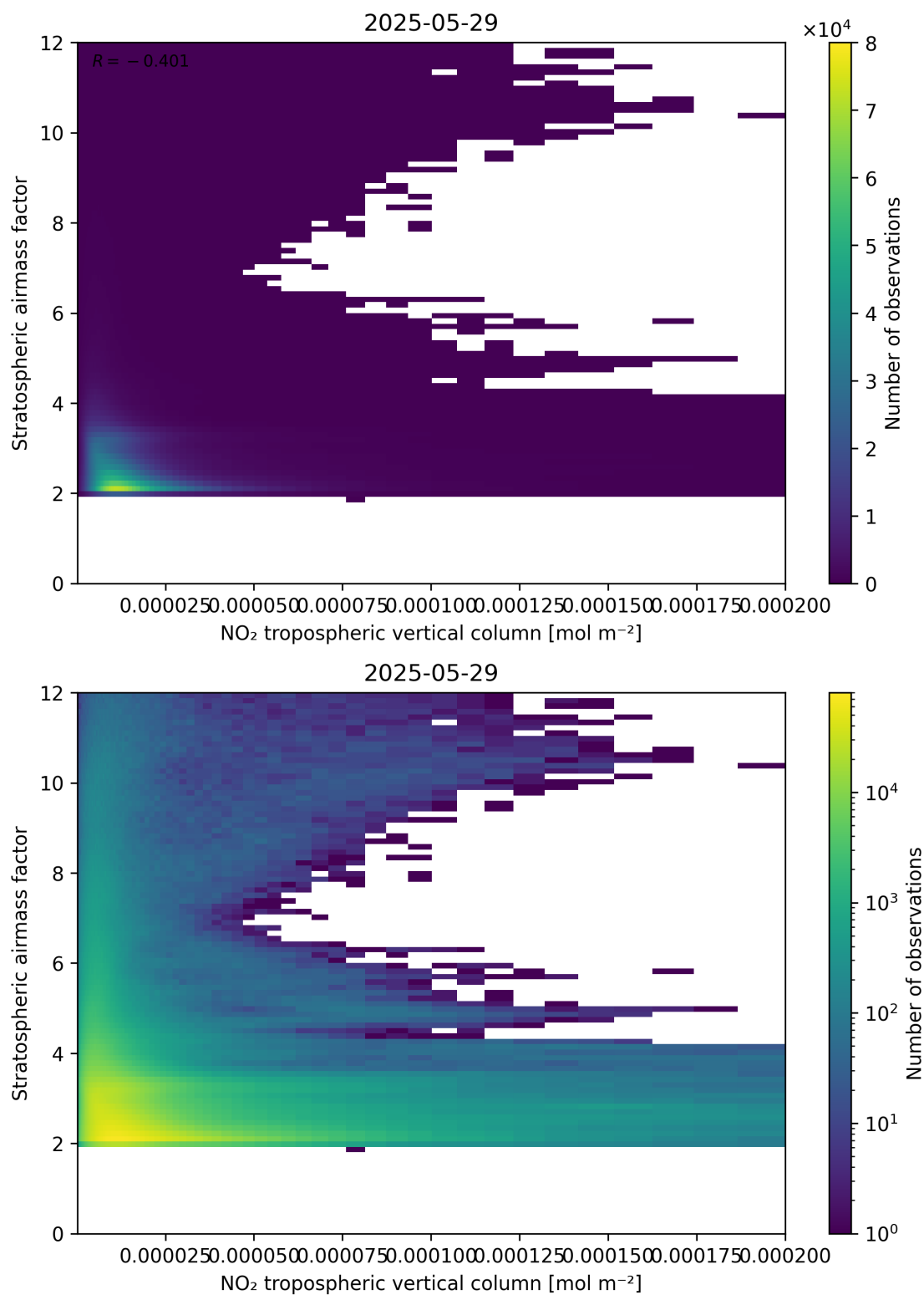
Figure 121: Scatter density plot of “NO 2 tropospheric vertical column” against “Stratospheric air mass factor” for 2025-05-28 to 2025-05-30.
