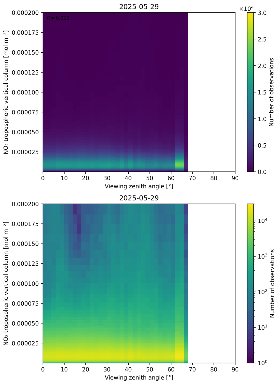
Figure 169: Scatter density plot of “Viewing zenith angle” against “NO 2 tropospheric vertical column” for 2025-05-28 to 2025-05-30.
