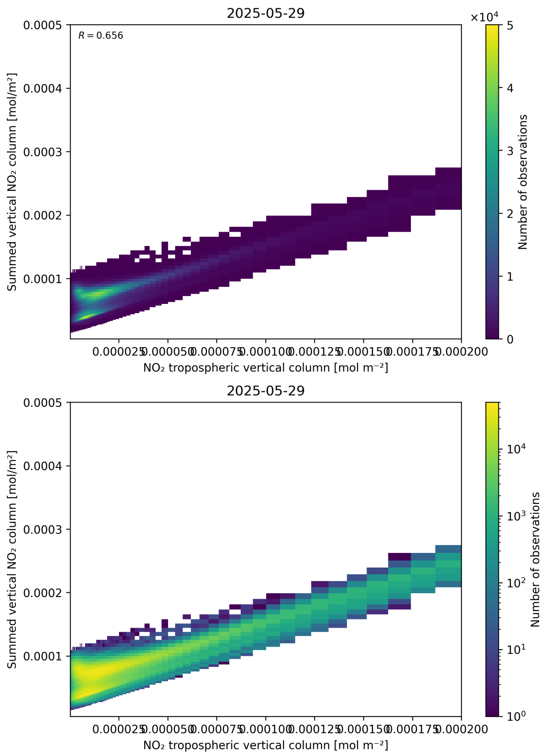
Figure 126: Scatter density plot of “NO 2 tropospheric vertical column” against “Summed vertical NO 2 column” for 2025-05-28 to 2025-05-30.
