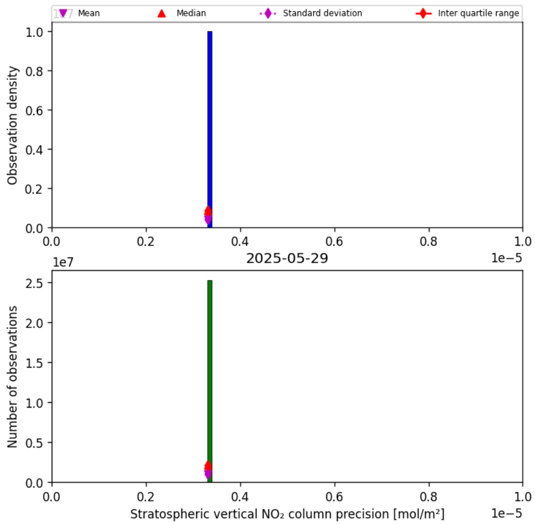
Figure 37: Histogram of “Stratospheric vertical NO 2 column precision” for 2025-05-28 to 2025-05-30
