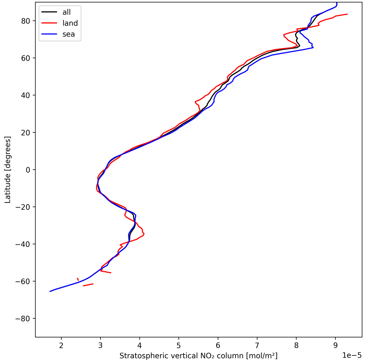
Figure 19: Zonal average of “Stratospheric vertical NO 2 column” for 2025-05-28 to 2025-05-30.
