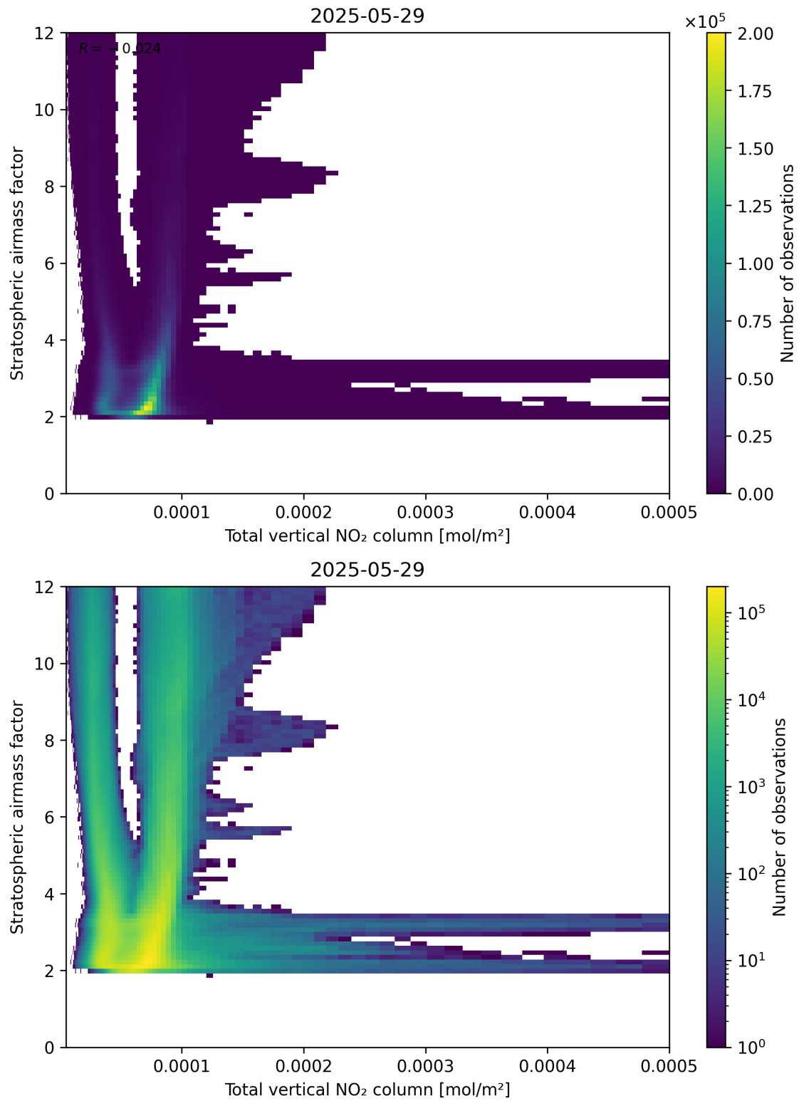
Figure 110: Scatter density plot of “Total vertical NO 2 column” against “Stratospheric airmass factor” for 2025-05-28 to 2025-05-30.
