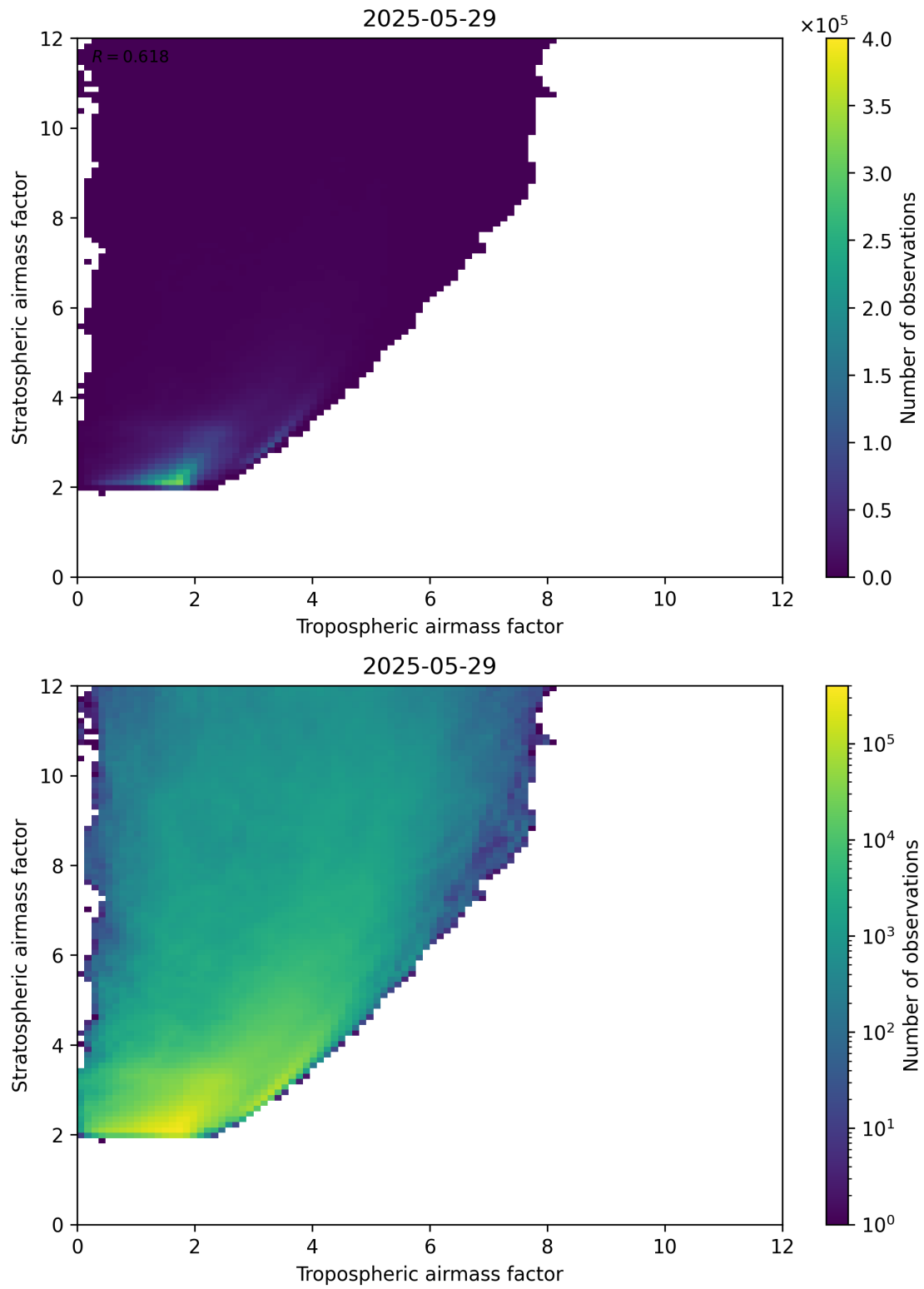
Figure 71: Scatter density plot of “Tropospheric airmass factor” against “Stratospheric airmass factor” for 2025-05-28 to 2025-05-30.
