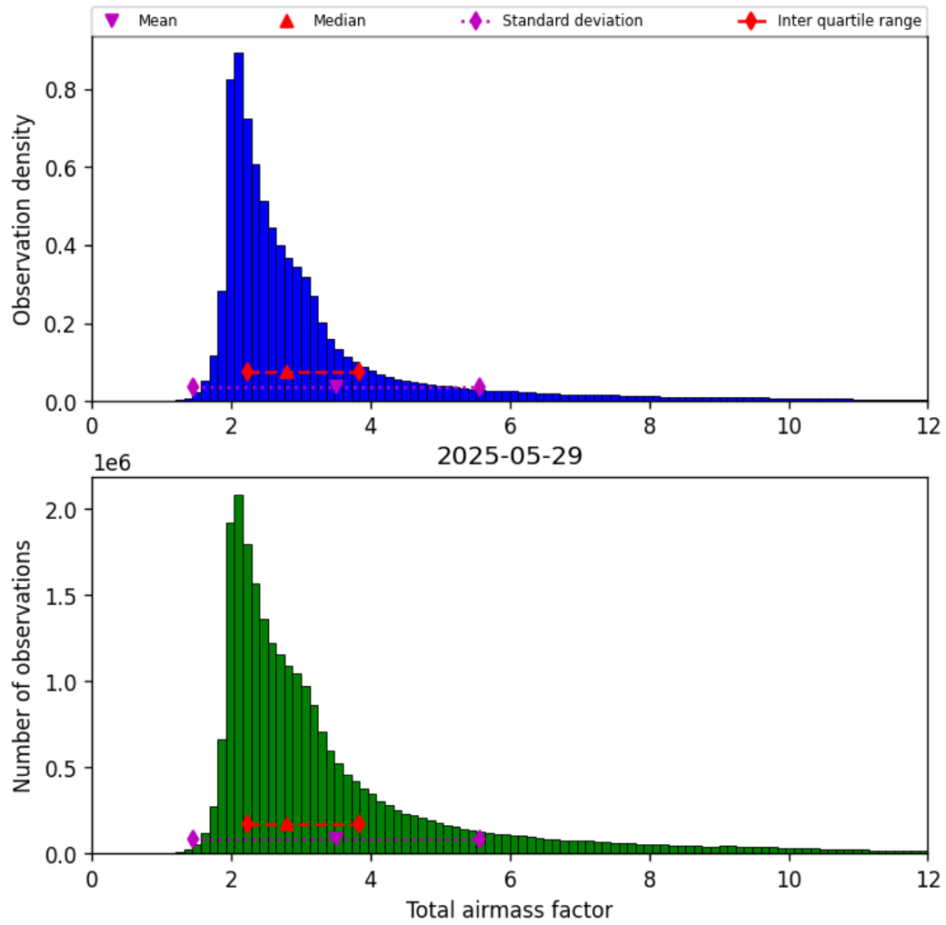
Figure 32: Histogram of “Total airmass factor” for 2025-05-28 to 2025-05-30
