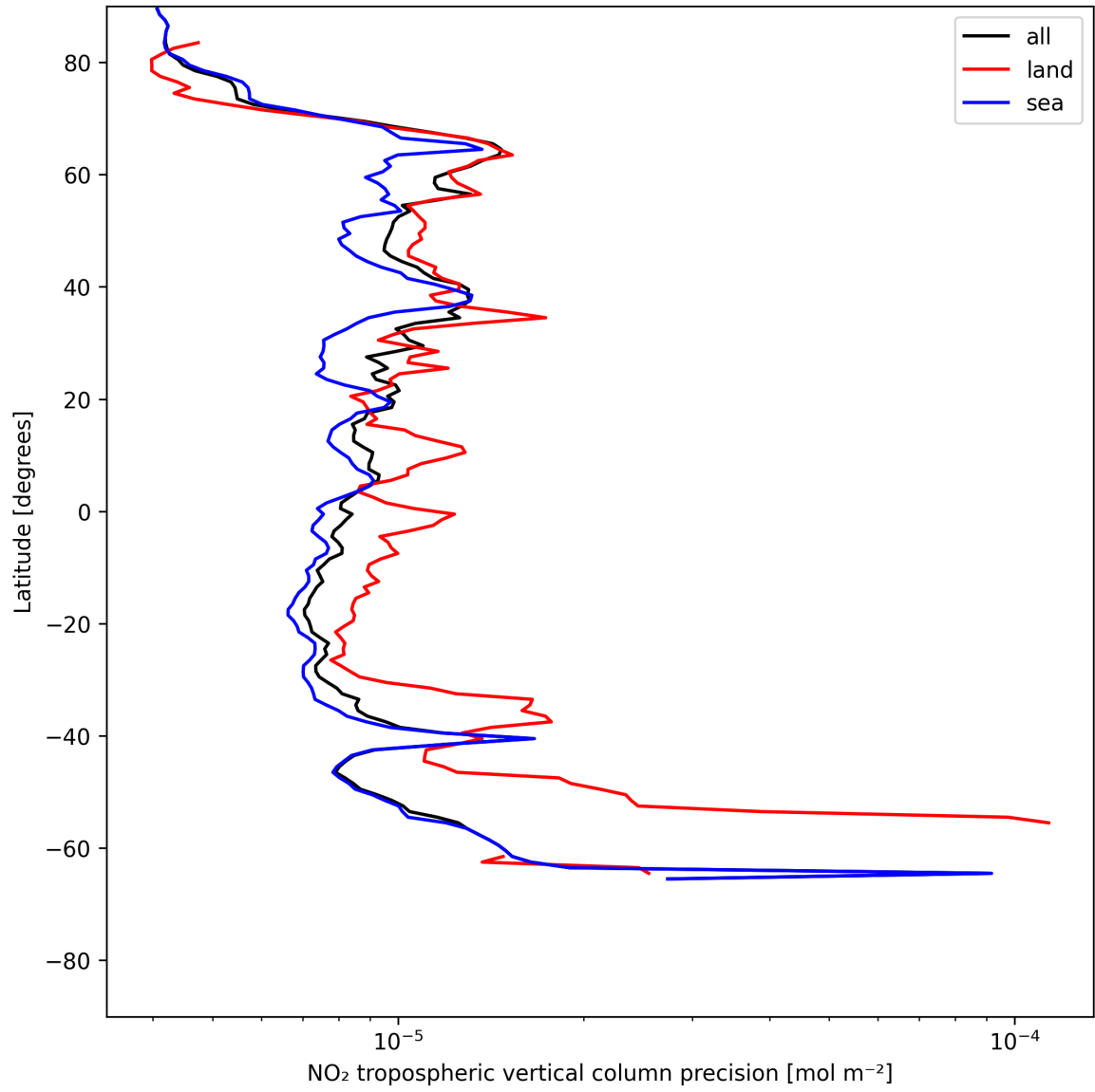
Figure 13: Zonal average of “NO 2 tropospheric vertical column precision” for 2025-05-29 to 2025-05-31.
