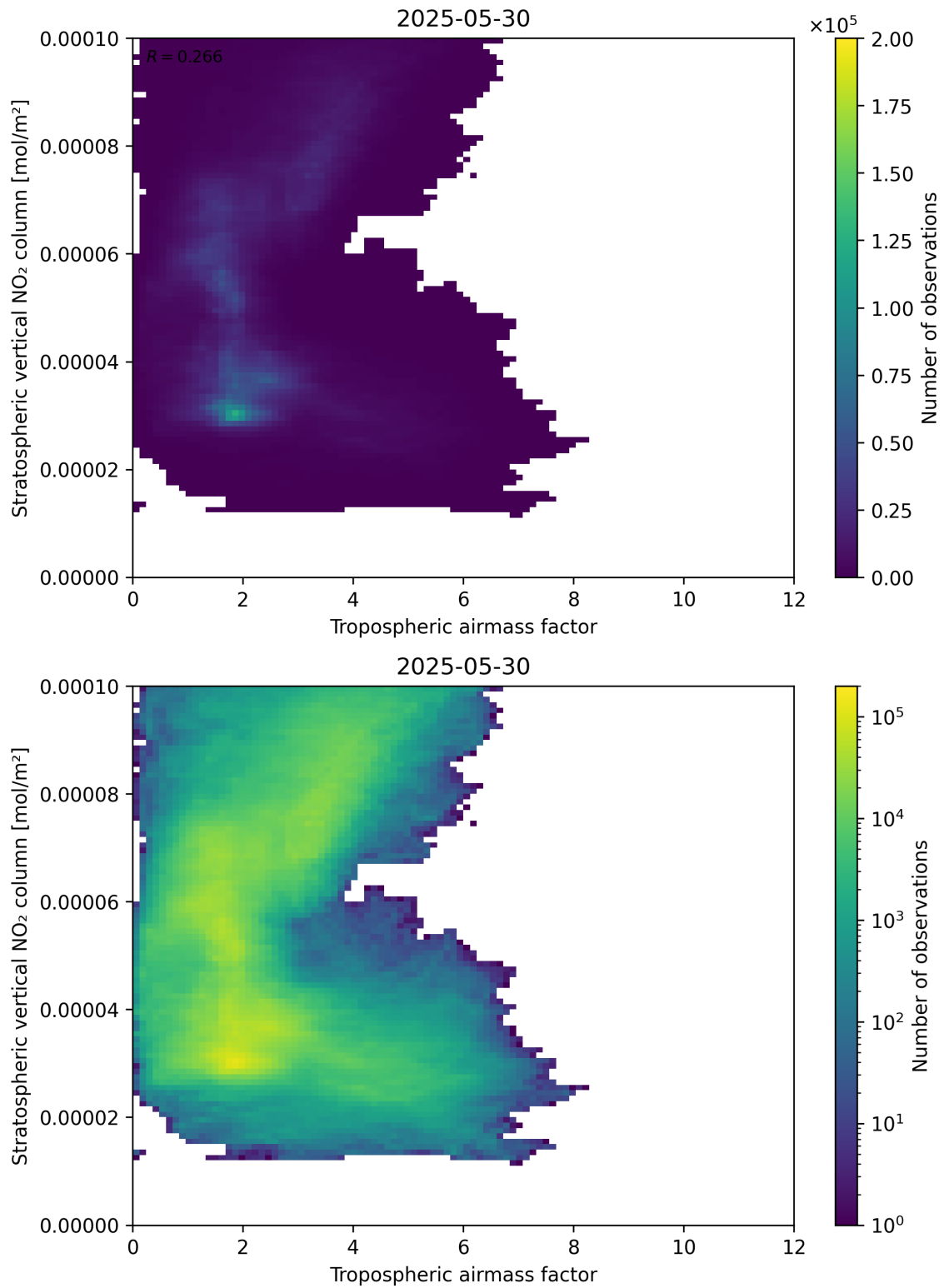
Figure 74: Scatter density plot of “Tropospheric airmass factor” against “Stratospheric vertical NO 2 column” for 2025-05-29 to 2025-05-31.
