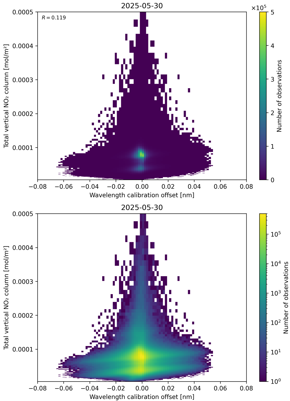
Figure 179: Scatter density plot of “Wavelength calibration offset” against “Total vertical NO 2 column” for 2025-05-29 to 2025-05-31.
