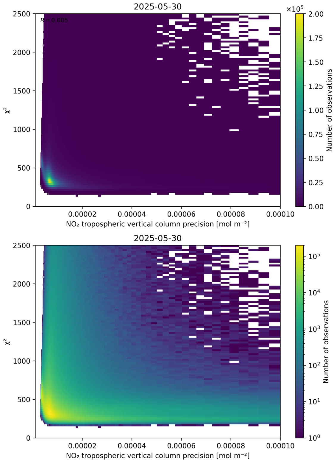
Figure 134: Scatter density plot of “NO 2 tropospheric vertical column precision” against “ \chi^2 ” for 2025-05-29 to 2025-05-31.
