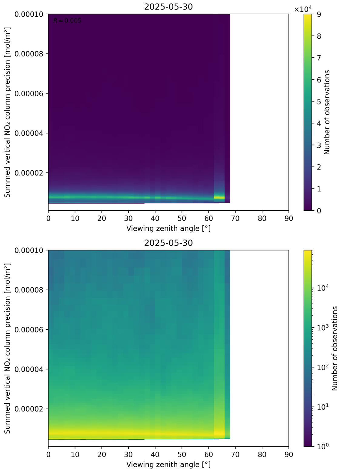
Figure 166: Scatter density plot of “Viewing zenith angle” against “Summed vertical NO 2 column precision” for 2025-05-29 to 2025-05-31.
