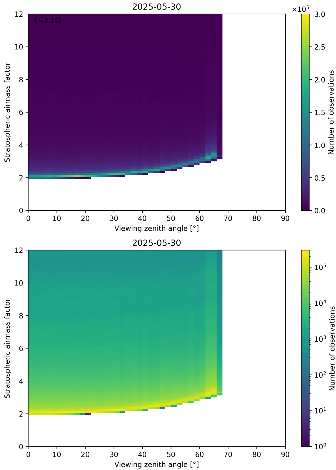
Figure 159: Scatter density plot of “Viewing zenith angle” against “Stratospheric airmass factor” for 2025-05-29 to 2025-05-31.
