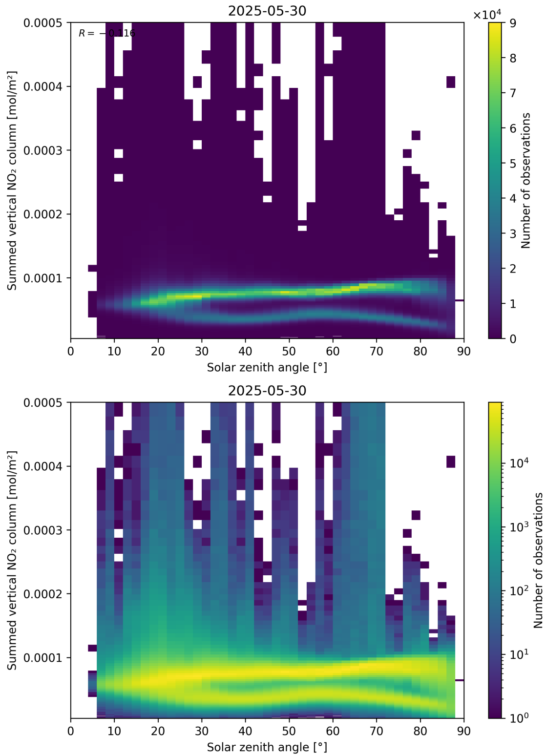
Figure 151: Scatter density plot of “Solar zenith angle” against “Summed vertical NO 2 column” for 2025-05-29 to 2025-05-31.
