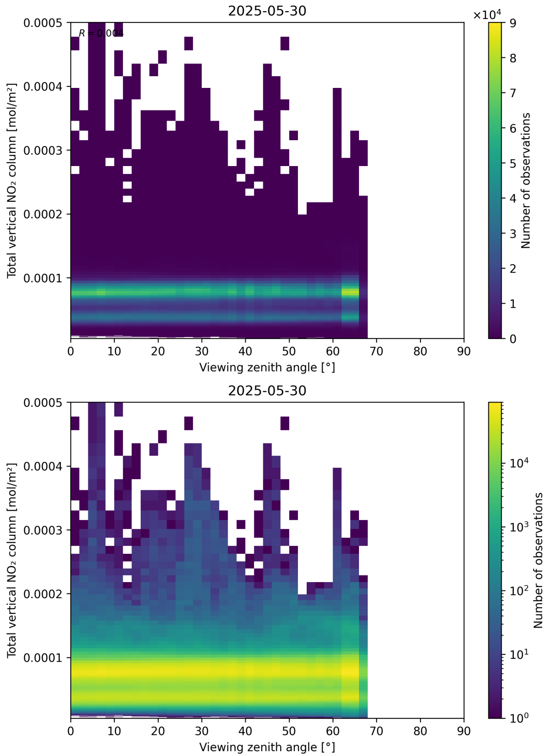
Figure 167: Scatter density plot of “Viewing zenith angle” against “Total vertical NO 2 column” for 2025-05-29 to 2025-05-31.
