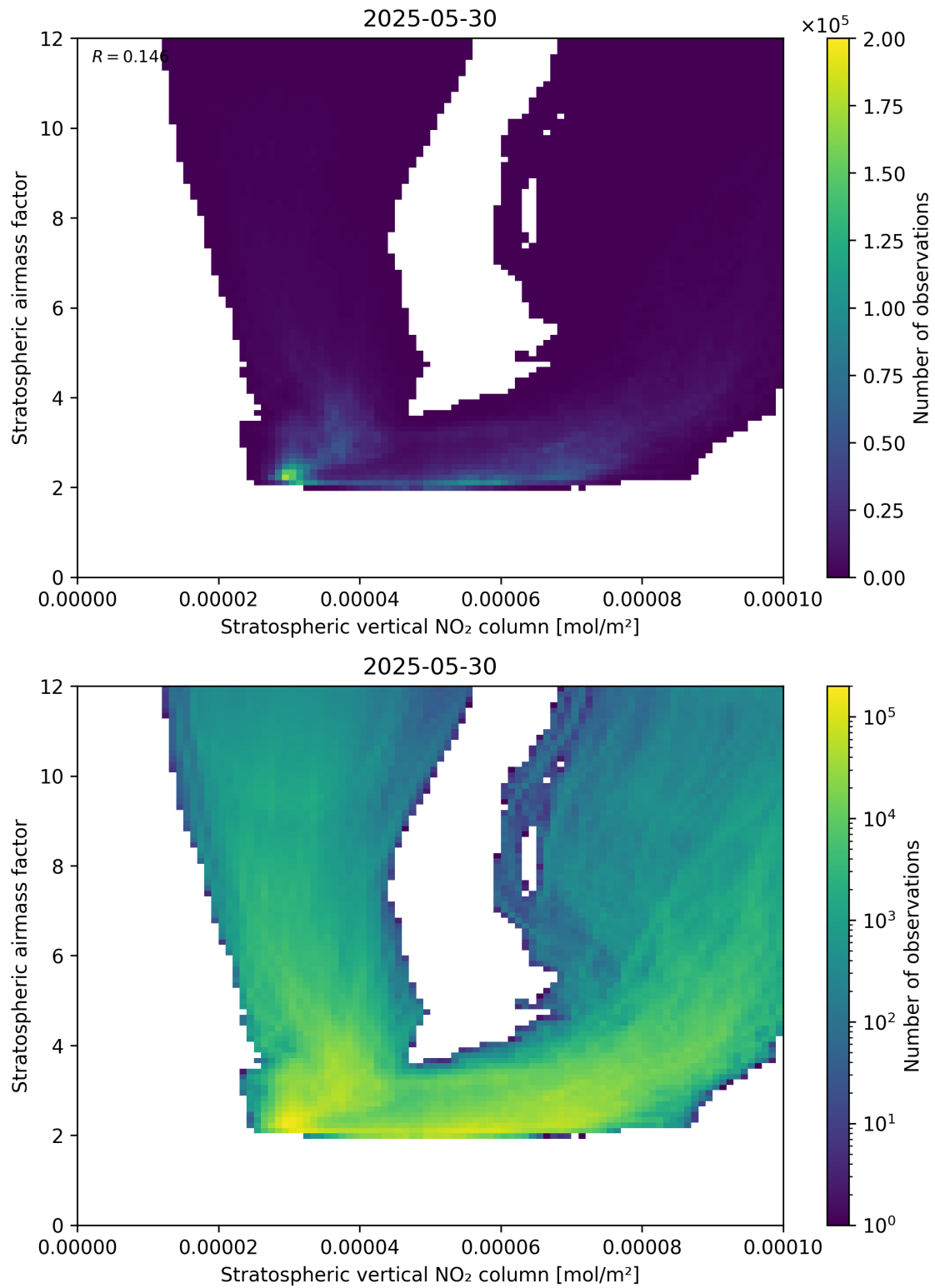
Figure 96: Scatter density plot of “Stratospheric vertical NO 2 column” against “Stratospheric airmass factor” for 2025-05-29 to 2025-05-31.
