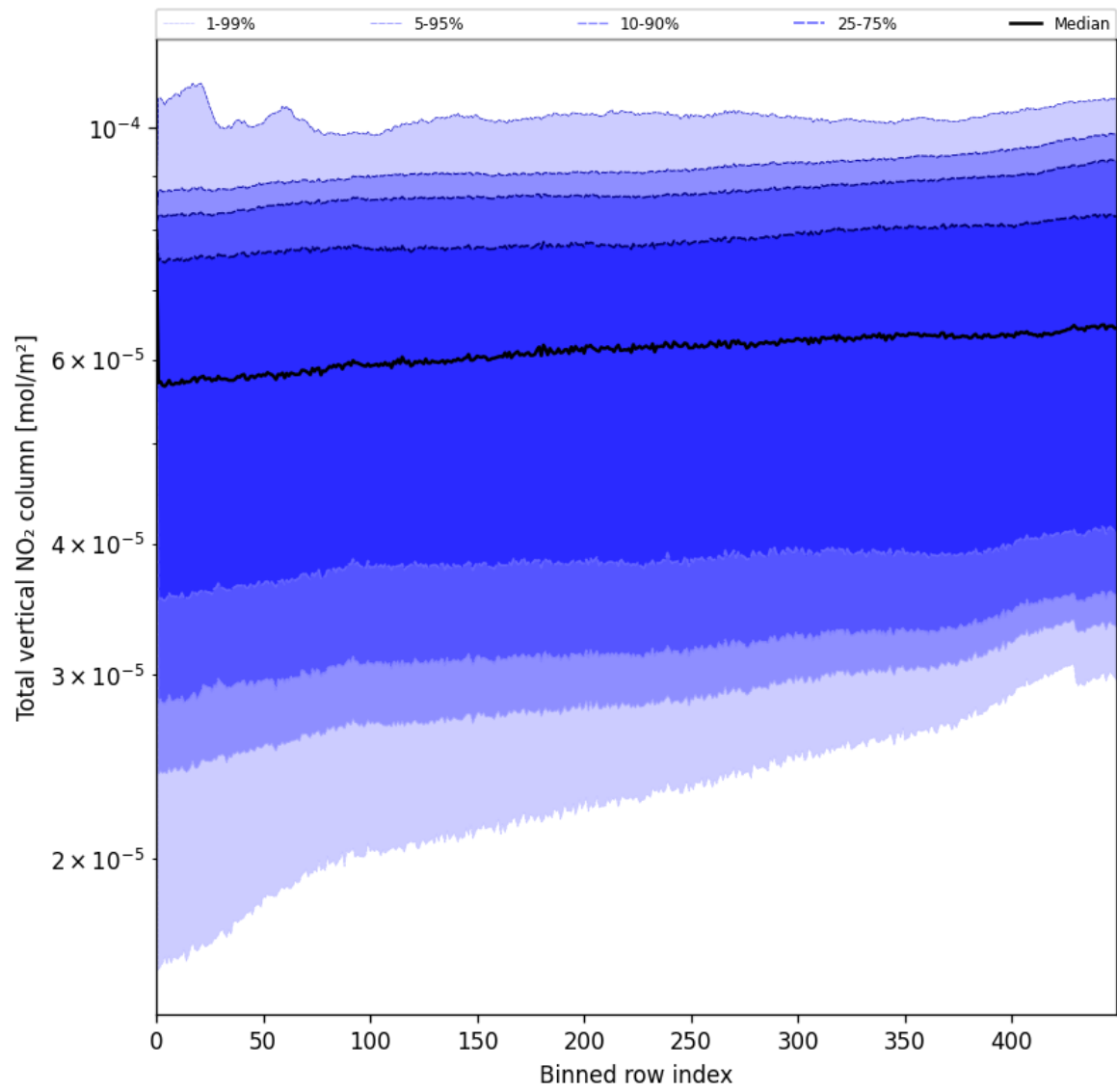
Figure 55: Along track statistics of “Total vertical NO 2 column” for 2025-05-29 to 2025-05-31
