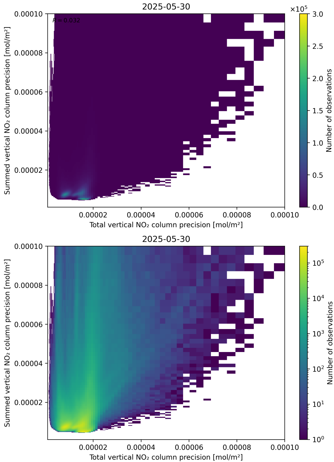
Figure 118: Scatter density plot of “Total vertical NO 2 column precision” against “Summed vertical NO 2 column precision” for 2025-05-29 to 2025-05-31.
