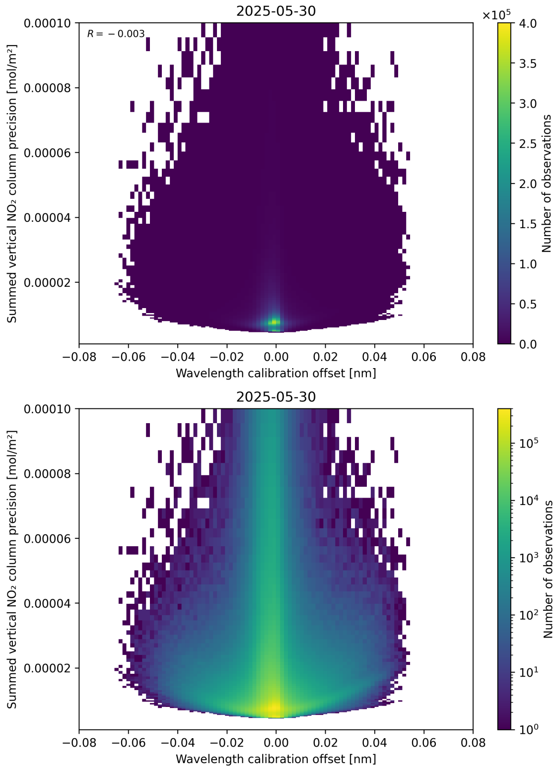
Figure 178: Scatter density plot of “Wavelength calibration offset” against “Summed vertical NO 2 column precision” for 2025-05-29 to 2025-05-31.
