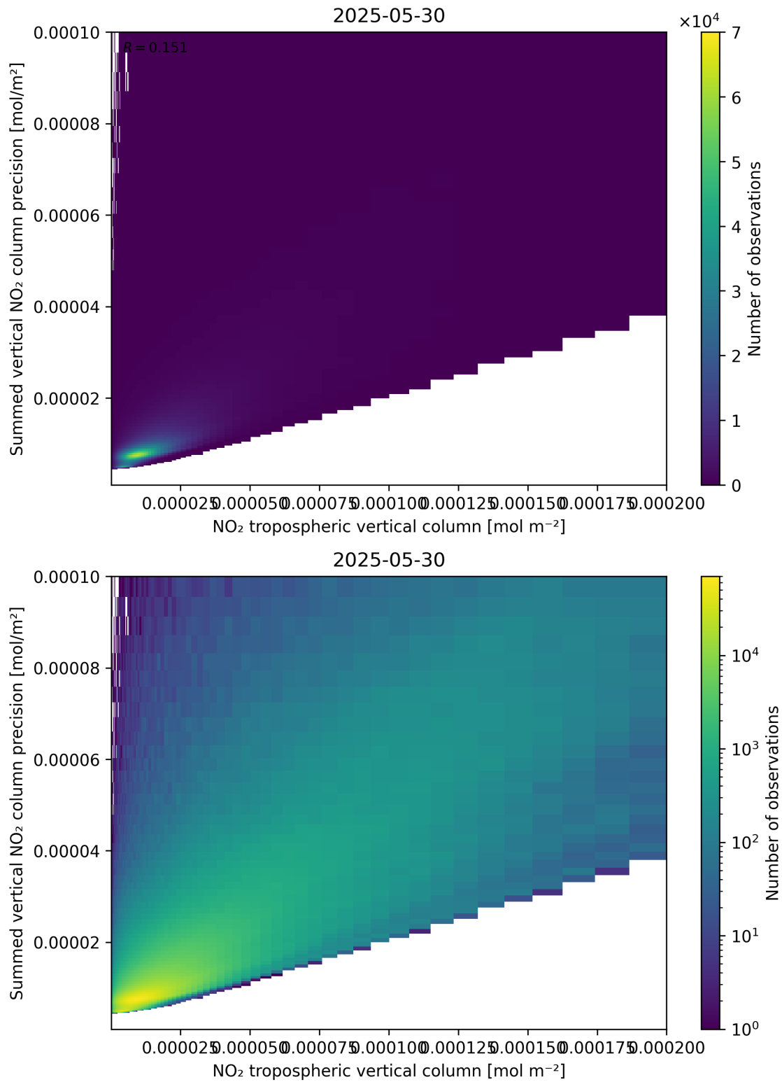
Figure 127: Scatter density plot of “NO 2 tropospheric vertical column” against “Summed vertical NO 2 column precision” for 2025-05-29 to 2025-05-31.
