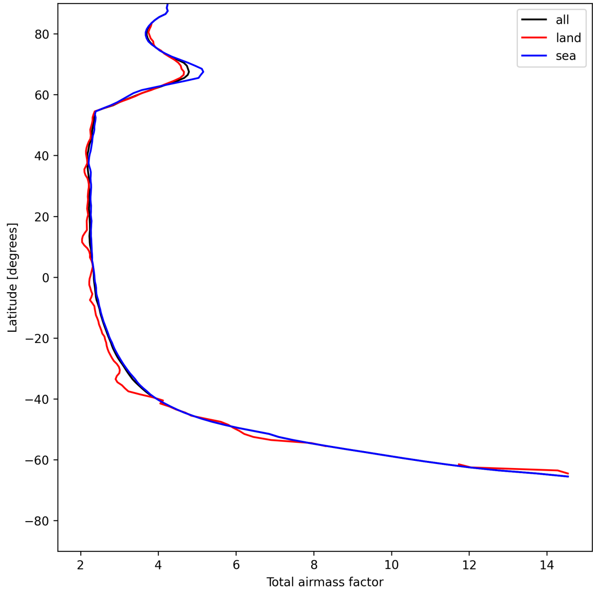
Figure 15: Zonal average of “Total airmass factor” for 2025-05-29 to 2025-05-31.
