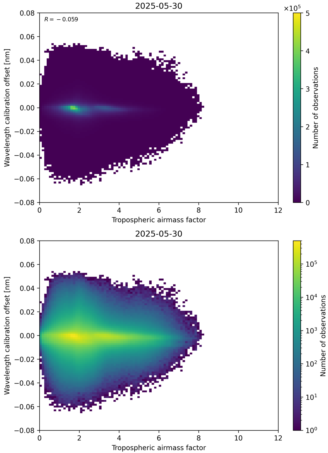
Figure 80: Scatter density plot of “Tropospheric airmass factor” against “Wavelength calibration offset” for 2025-05-29 to 2025-05-31.
