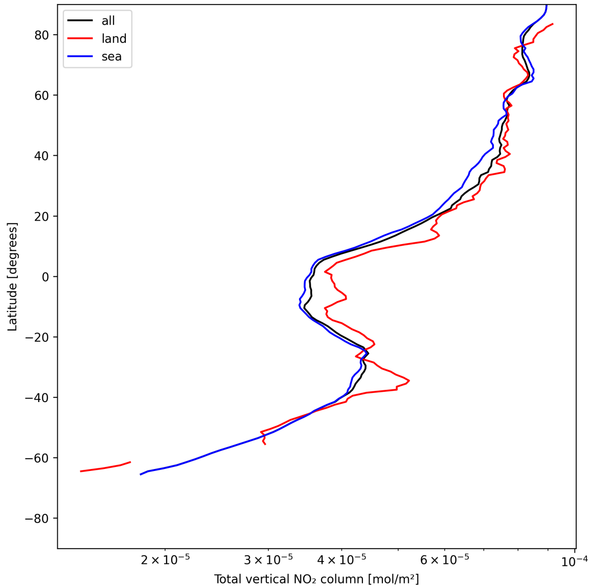
Figure 21: Zonal average of “Total vertical NO 2 column” for 2025-05-29 to 2025-05-31.
