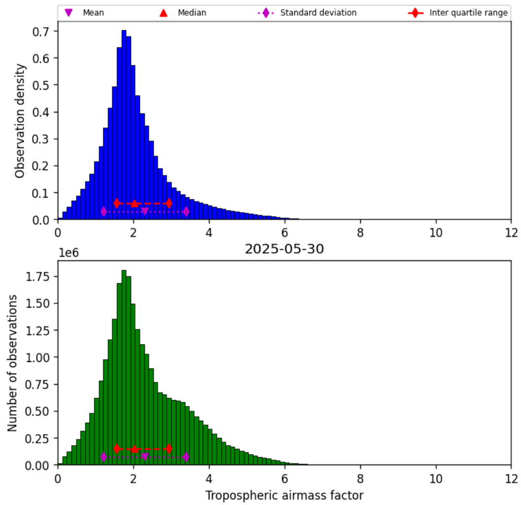
Figure 31: Histogram of “Tropospheric airmass factor” for 2025-05-29 to 2025-05-31
