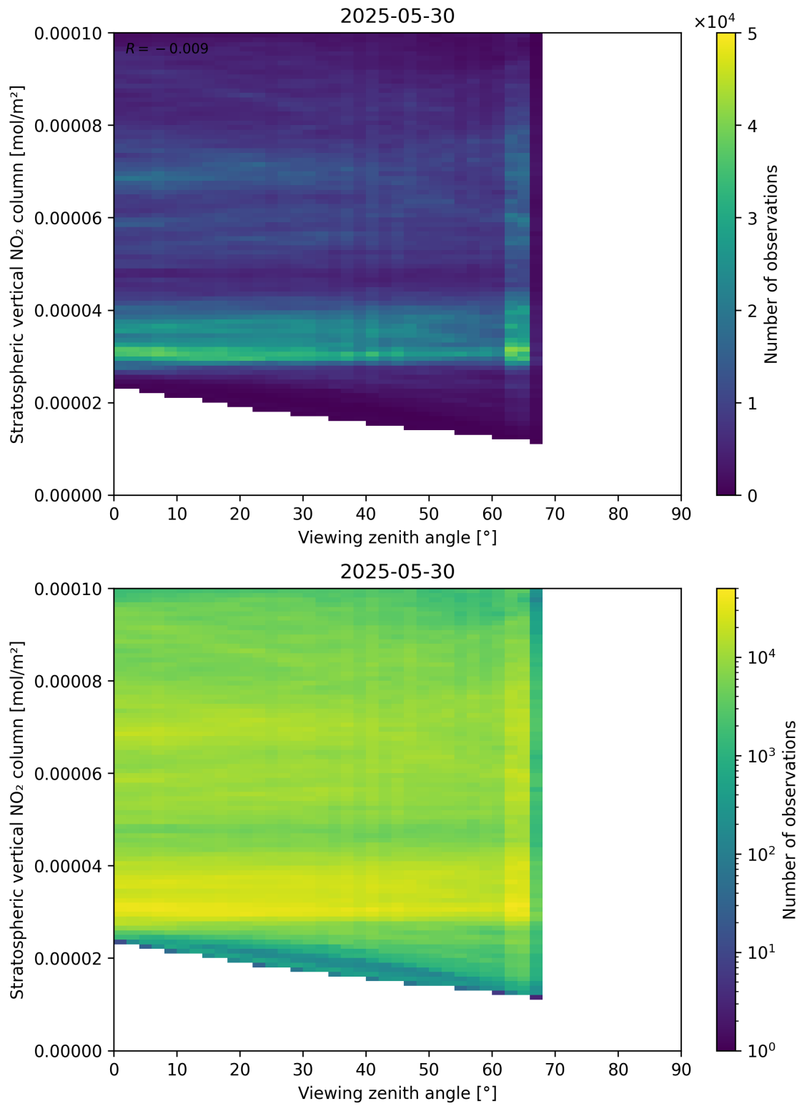
Figure 164: Scatter density plot of “Viewing zenith angle” against “Stratospheric vertical NO 2 column” for 2025-05-29 to 2025-05-31.
