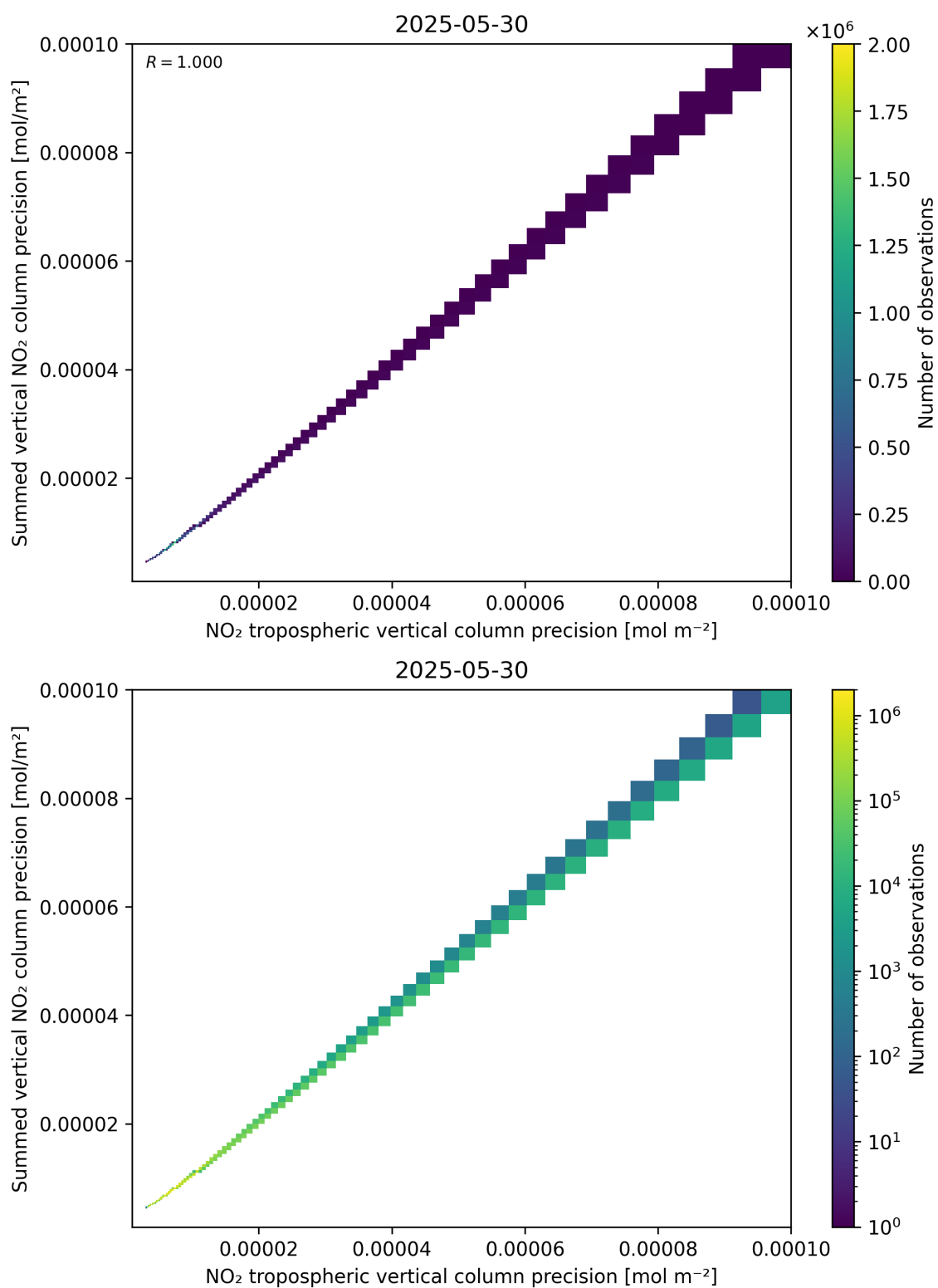
Figure 137: Scatter density plot of “NO 2 tropospheric vertical column precision” against “Summed vertical NO 2 column precision” for 2025-05-29 to 2025-05-31.
