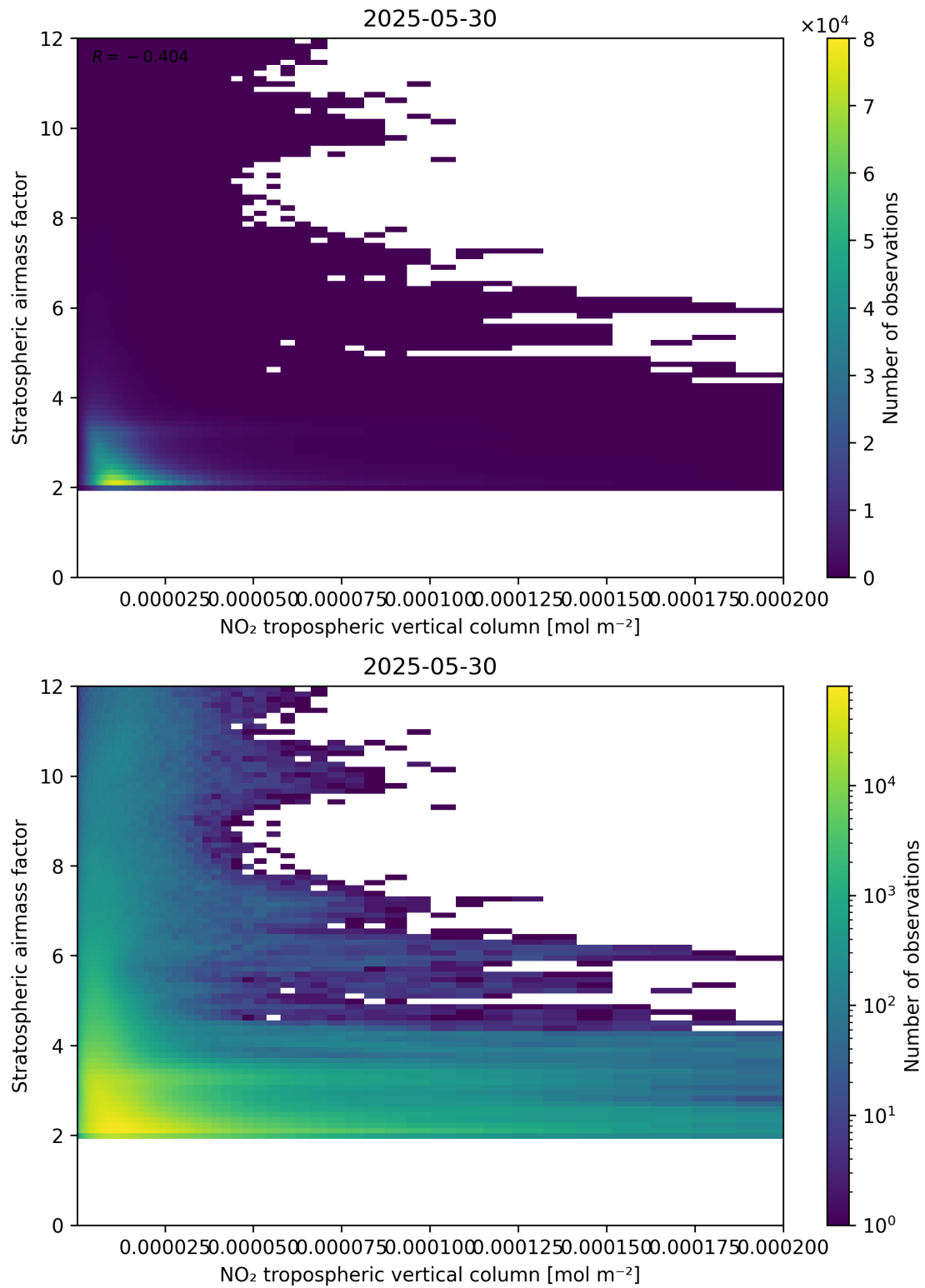
Figure 121: Scatter density plot of “NO 2 tropospheric vertical column” against “Stratospheric air mass factor” for 2025-05-29 to 2025-05-31.
