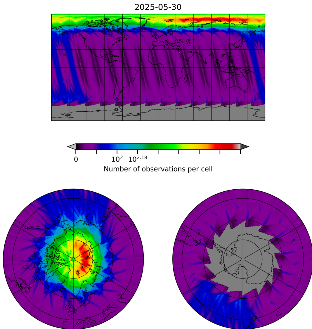
Figure 10: Map of the number of observations for 2025-05-29 to 2025-05-31
