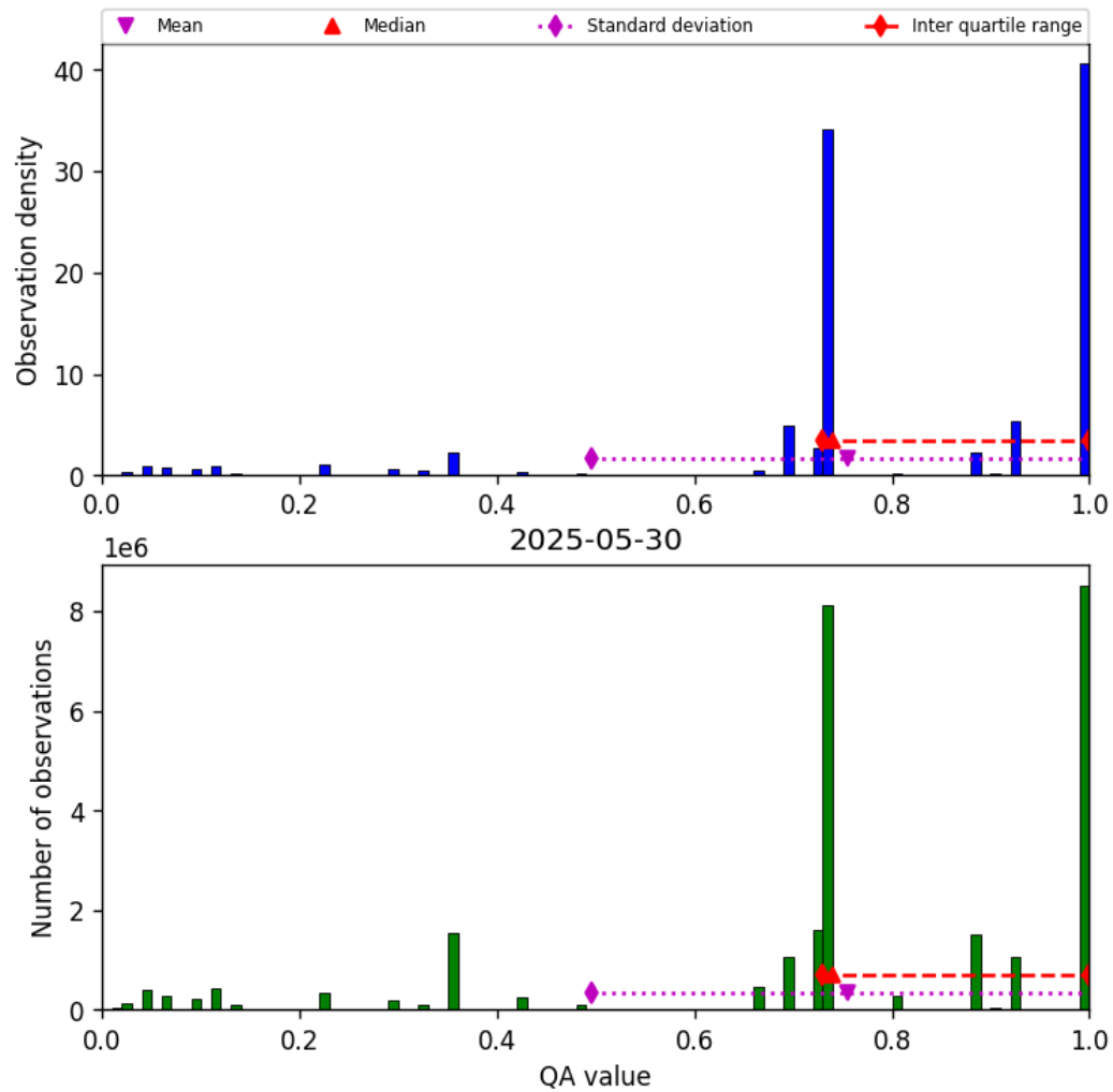
Figure 28: Histogram of “QA value” for 2025-05-29 to 2025-05-31
