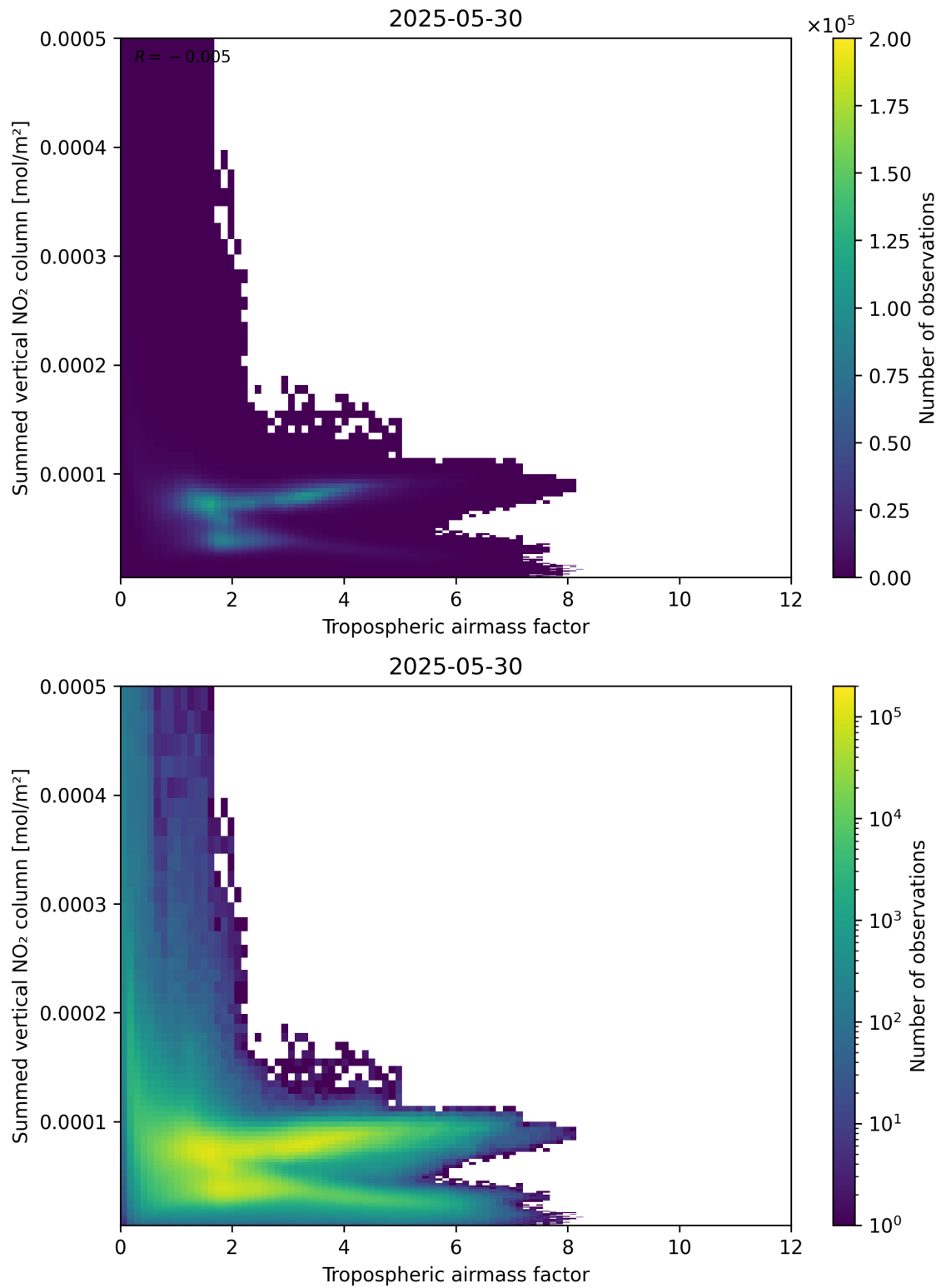
Figure 75: Scatter density plot of “Tropospheric airmass factor” against “Summed vertical NO 2 column” for 2025-05-29 to 2025-05-31.
