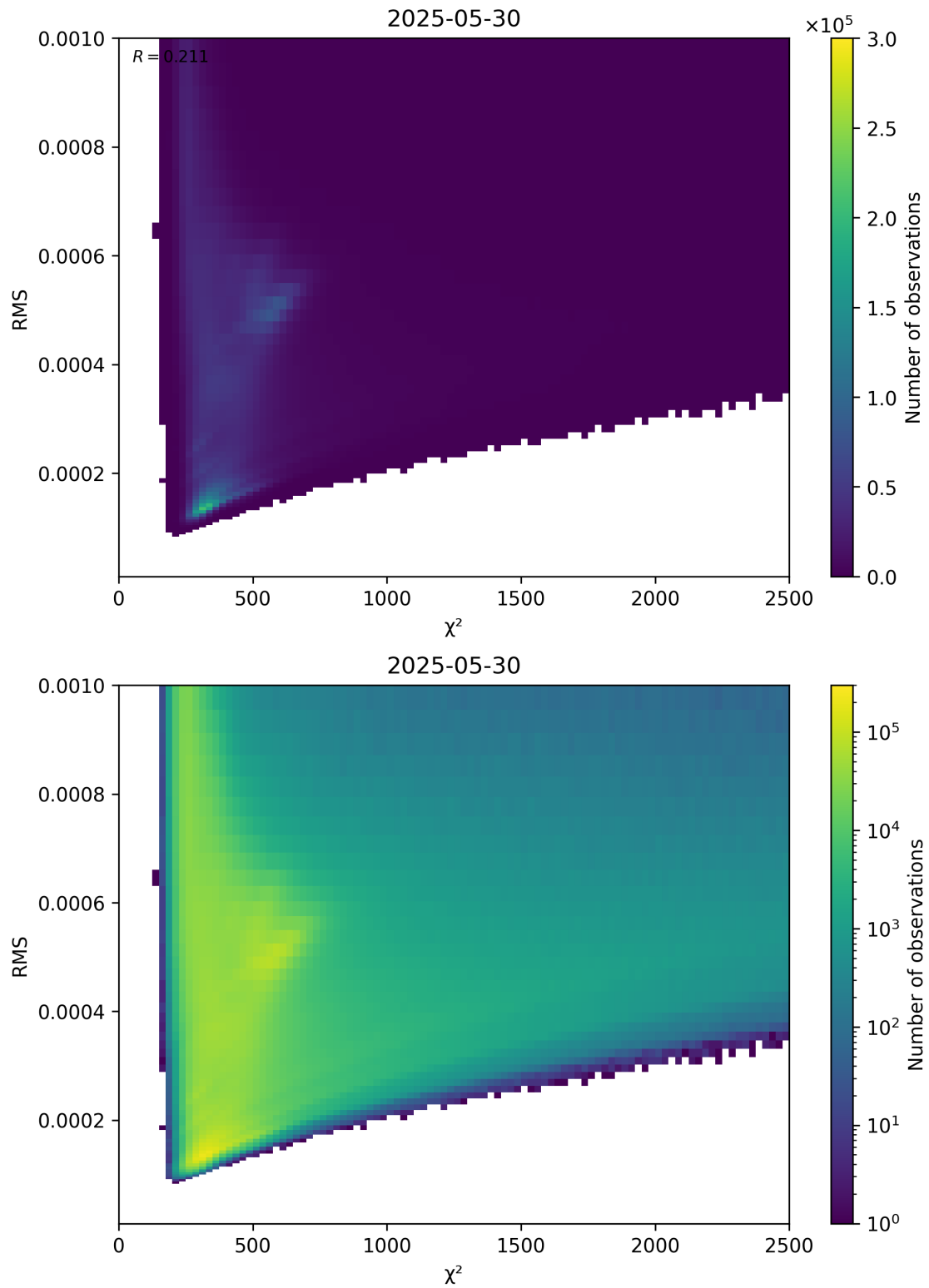
Figure 82: Scatter density plot of “ \chi^2 ” against “RMS” for 2025-05-29 to 2025-05-31.
