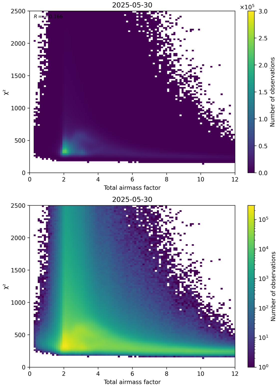
Figure 63: Scatter density plot of “Total airmass factor” against “ \chi^2 ” for 2025-05-29 to 2025-05-31.
