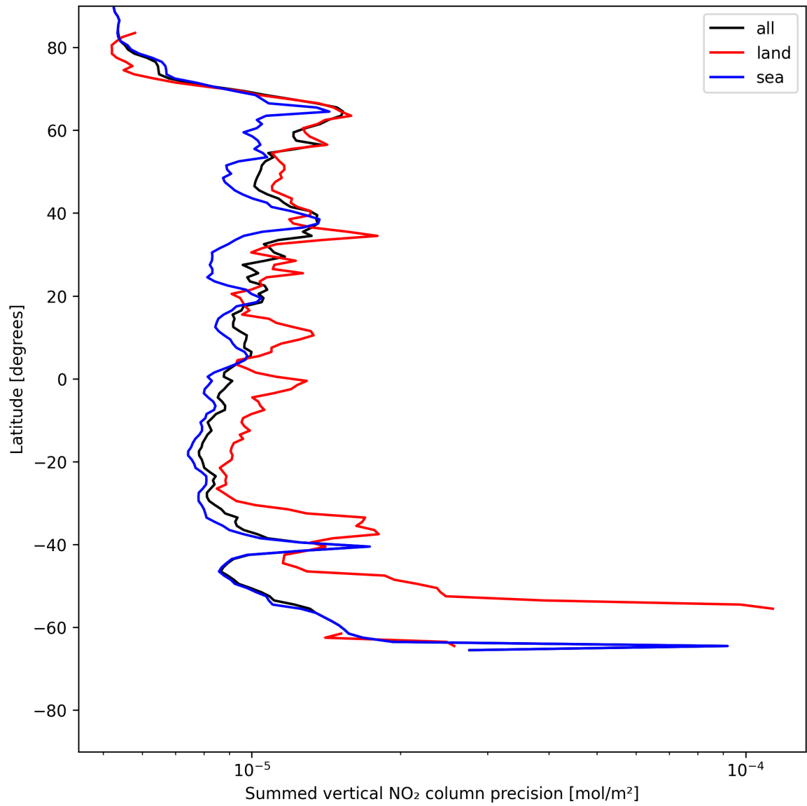
Figure 24: Zonal average of “Summed vertical NO 2 column precision” for 2025-05-29 to 2025-05-31.
