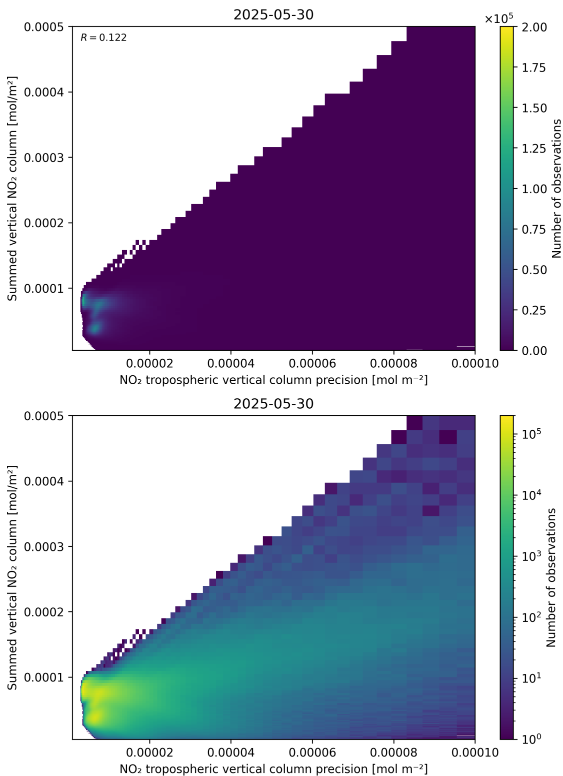
Figure 136: Scatter density plot of “NO 2 tropospheric vertical column precision” against “Summed vertical NO 2 column” for 2025-05-29 to 2025-05-31.
