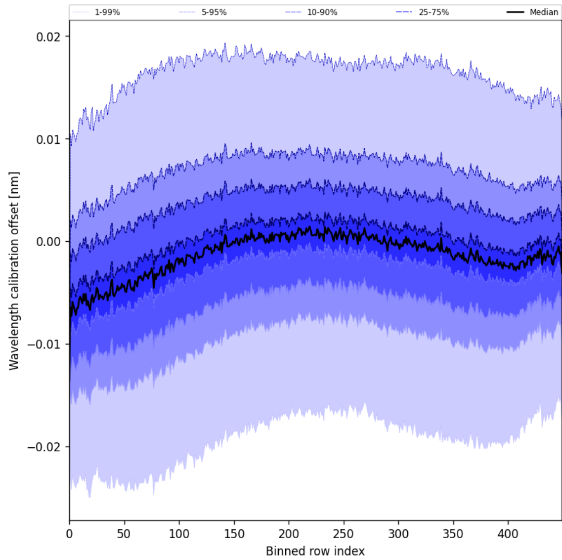
Figure 52: Along track statistics of “Wavelength calibration offset” for 2025-05-29 to 2025-05-31
