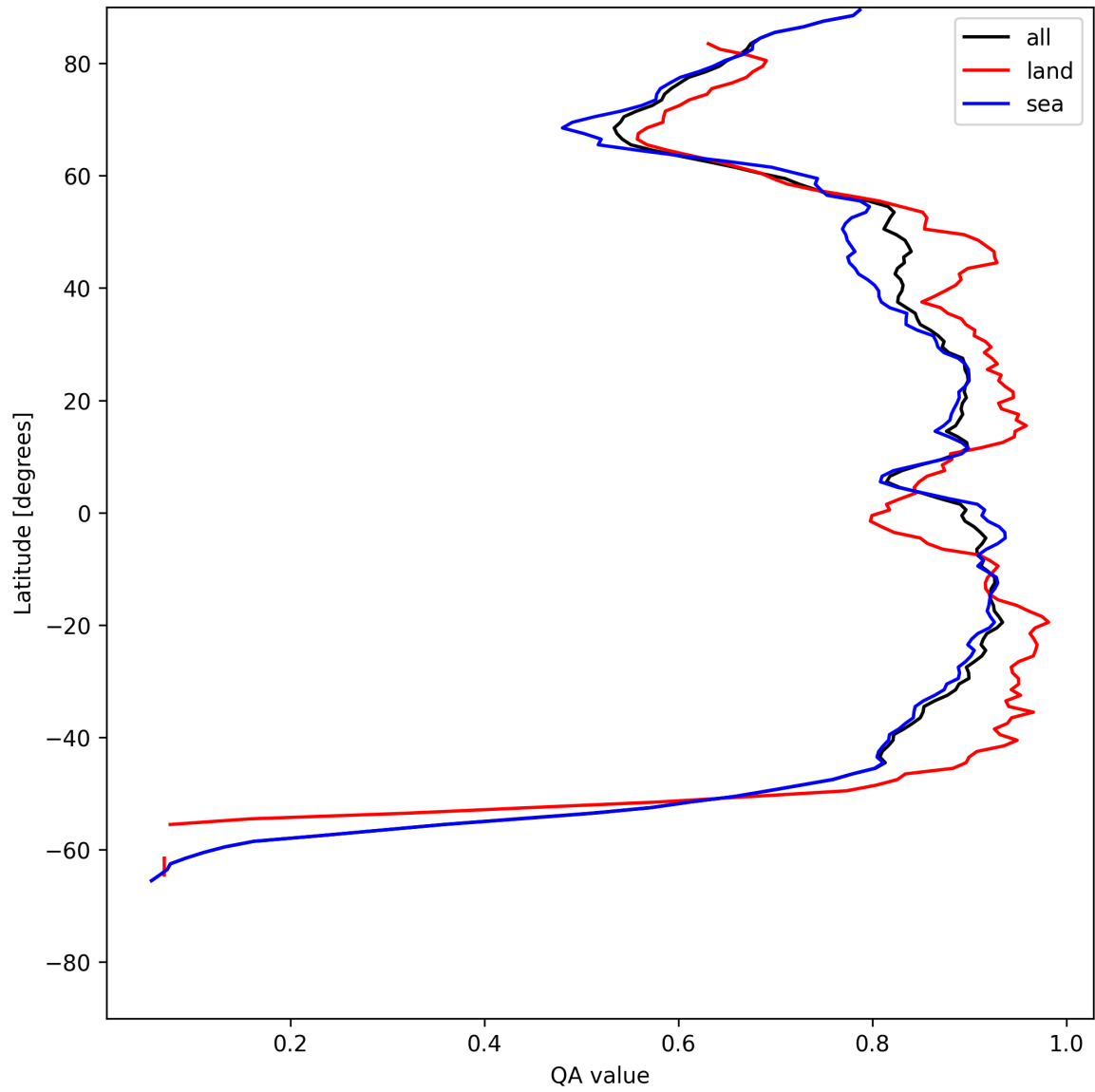
Figure 11: Zonal average of “QA value” for 2025-05-29 to 2025-05-31.
