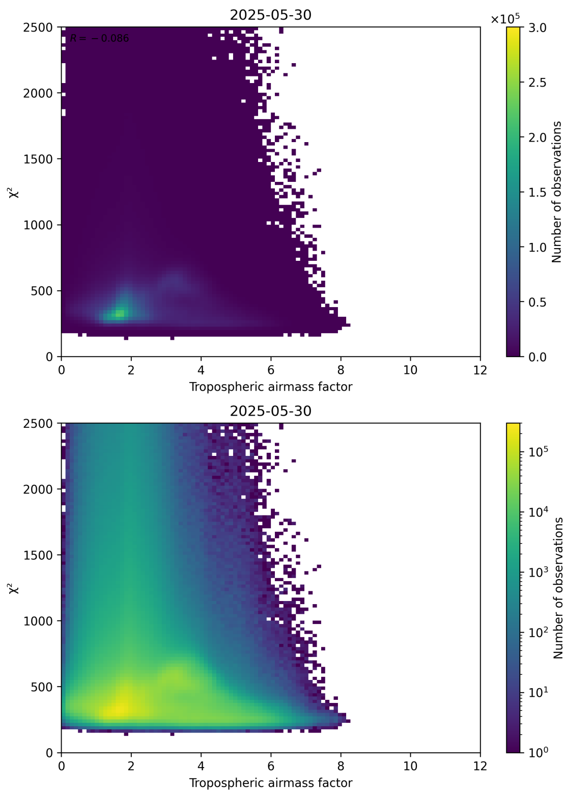
Figure 73: Scatter density plot of “Tropospheric airmass factor” against “ \chi^2 ” for 2025-05-29 to 2025-05-31.
