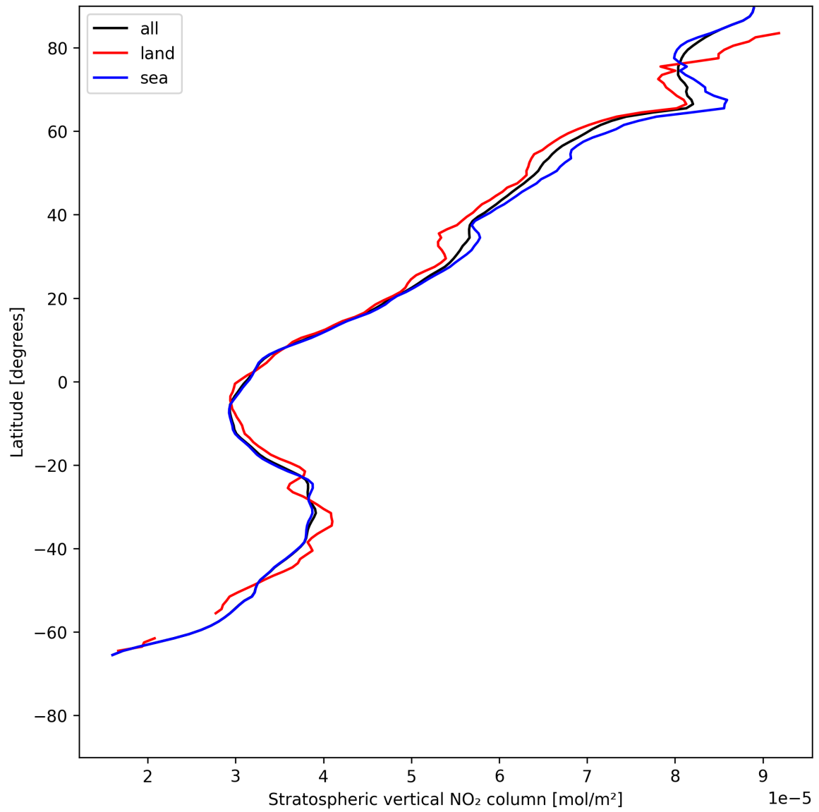
Figure 19: Zonal average of “Stratospheric vertical NO 2 column” for 2025-05-29 to 2025-05-31.
