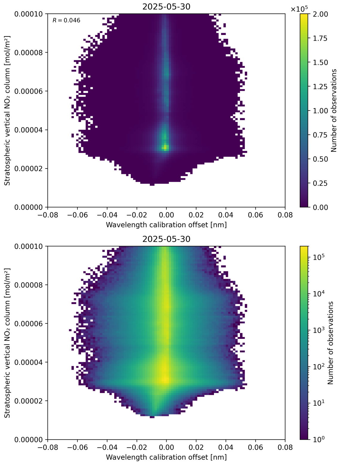
Figure 176: Scatter density plot of “Wavelength calibration offset” against “Stratospheric vertical NO 2 column” for 2025-05-29 to 2025-05-31.
