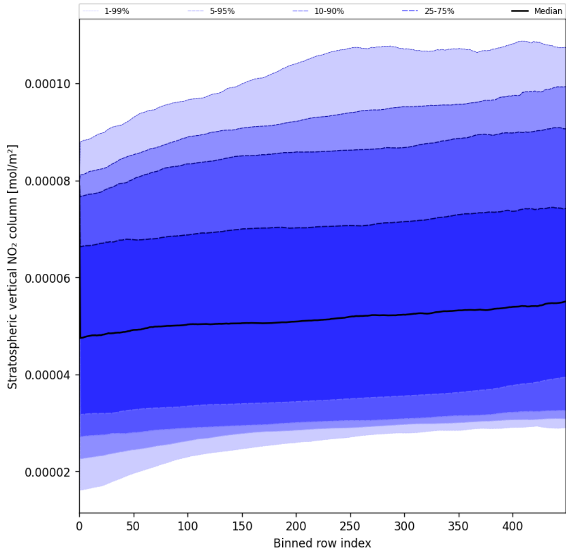
Figure 53: Along track statistics of “Stratospheric vertical NO 2 column” for 2025-05-29 to 2025-05-31
