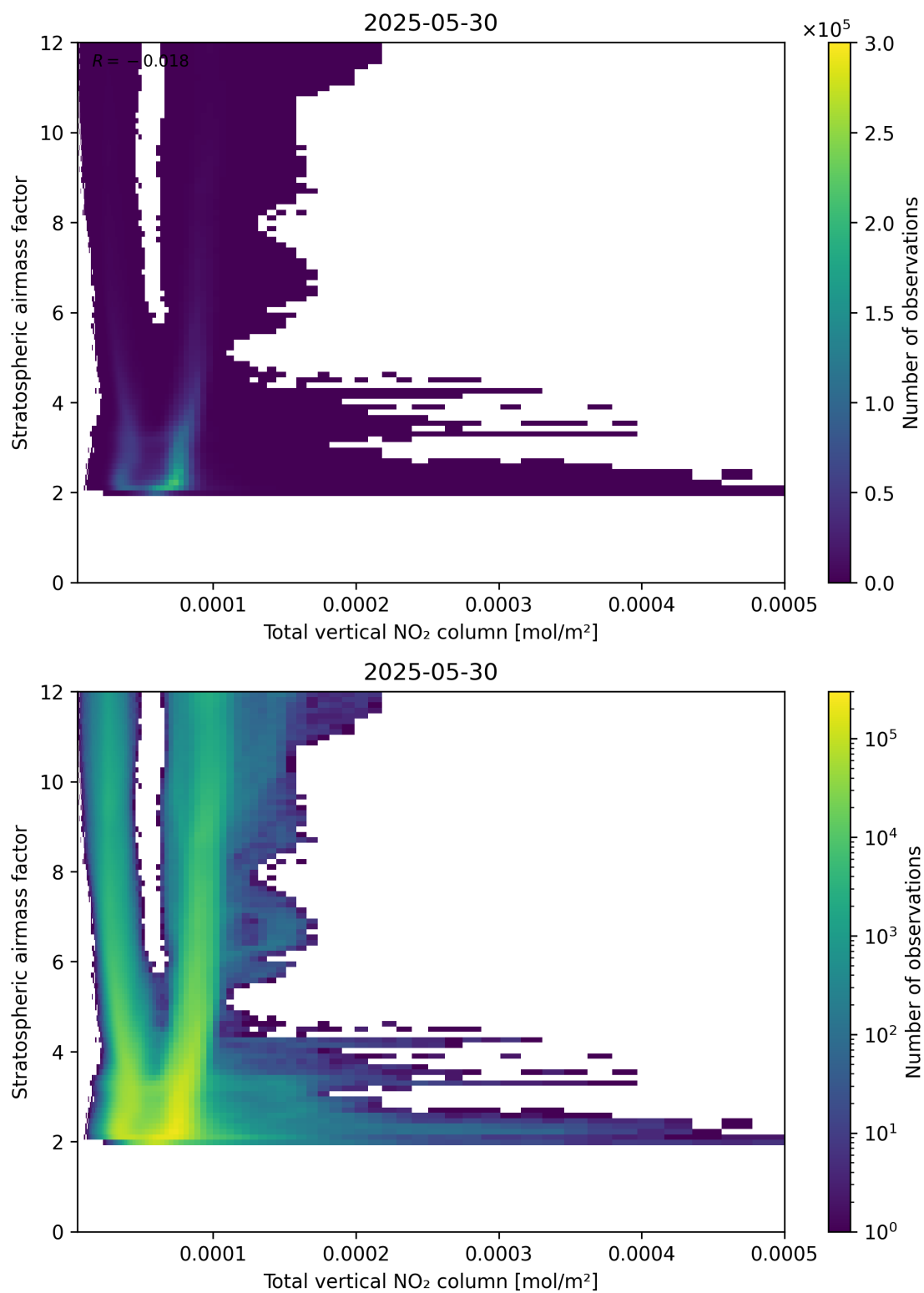
Figure 110: Scatter density plot of “Total vertical NO 2 column” against “Stratospheric airmass factor” for 2025-05-29 to 2025-05-31.
