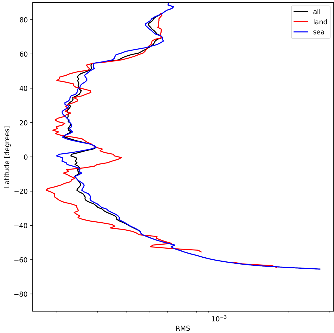
Figure 26: Zonal average of “RMS” for 2025-05-29 to 2025-05-31.
