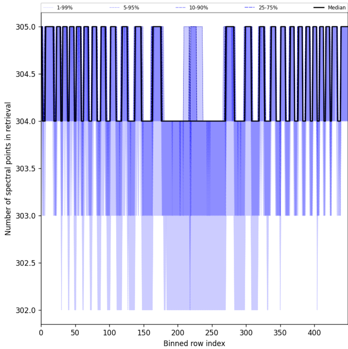
Figure 50: Along track statistics of “Number of spectral points in retrieval” for 2025-05-29 to 2025-05-31
