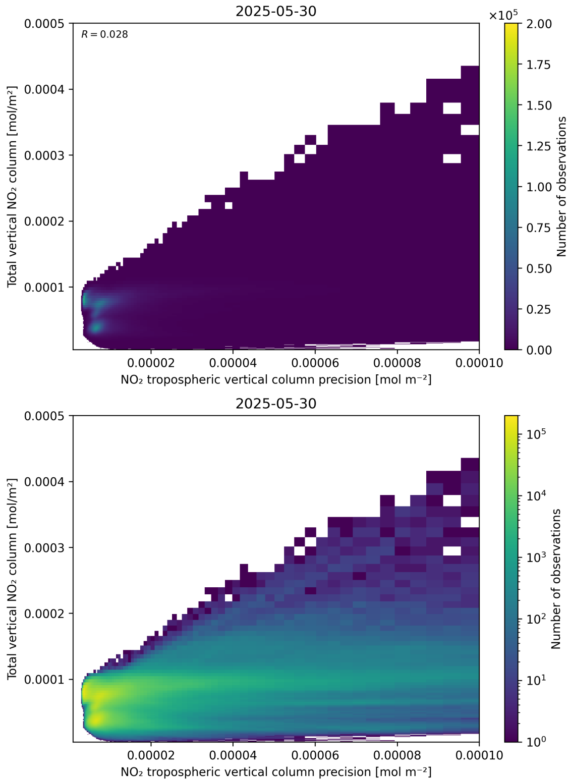
Figure 138: Scatter density plot of “NO 2 tropospheric vertical column precision” against “Total vertical NO 2 column” for 2025-05-29 to 2025-05-31.
