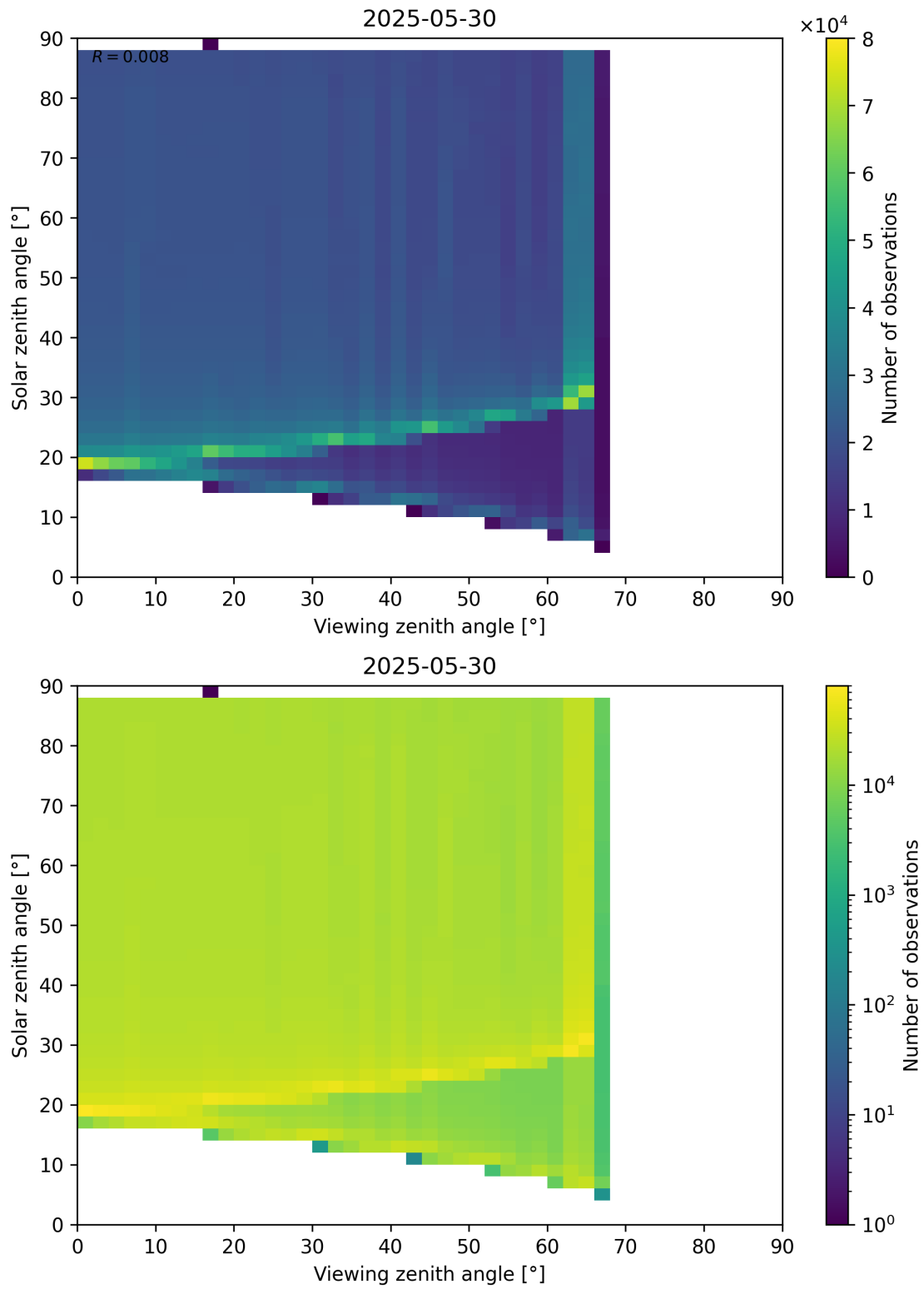
Figure 172: Scatter density plot of “Viewing zenith angle” against “Solar zenith angle” for 2025-05-29 to 2025-05-31.
