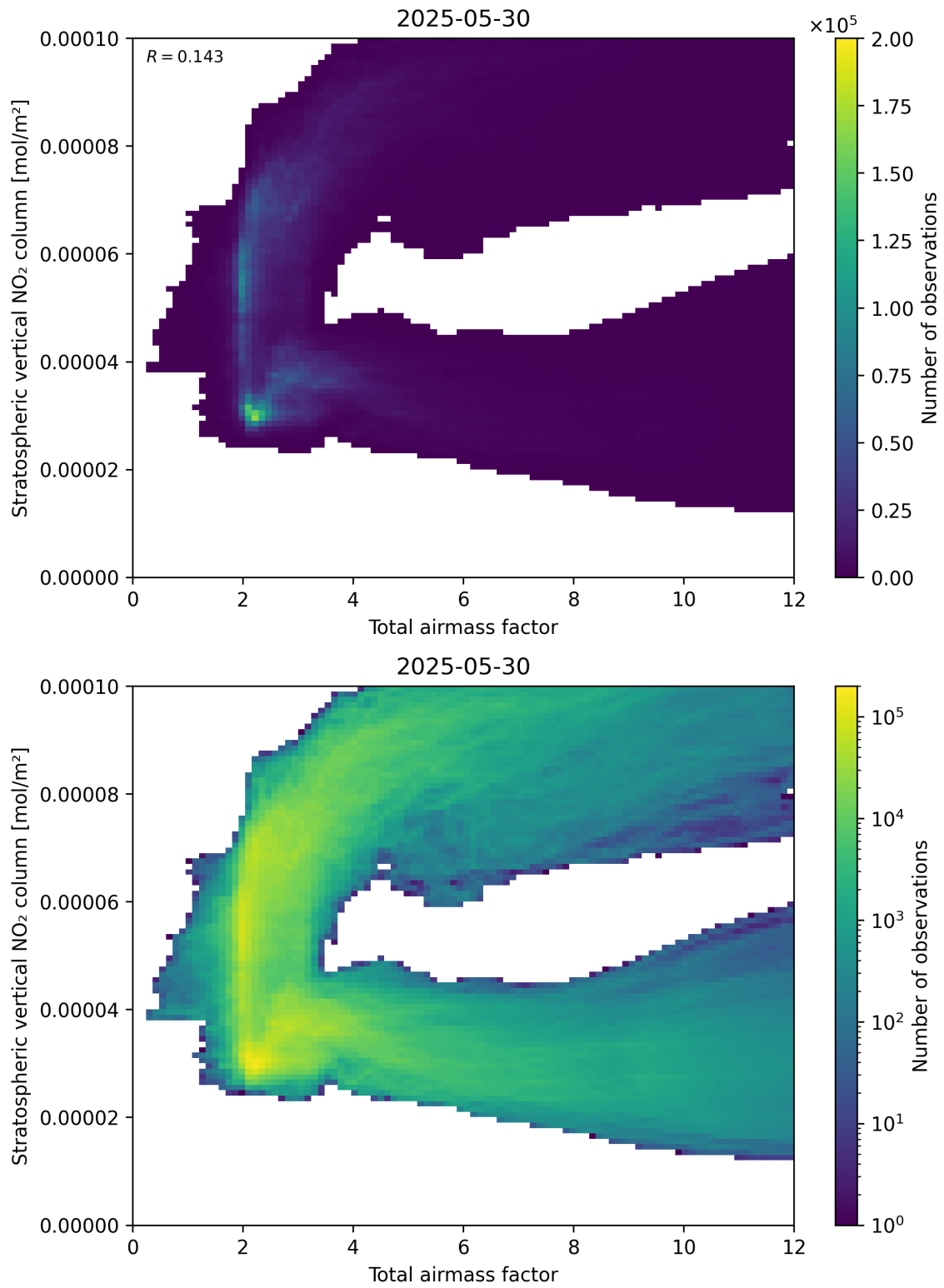
Figure 64: Scatter density plot of “Total airmass factor” against “Stratospheric vertical NO 2 column” for 2025-05-29 to 2025-05-31.
