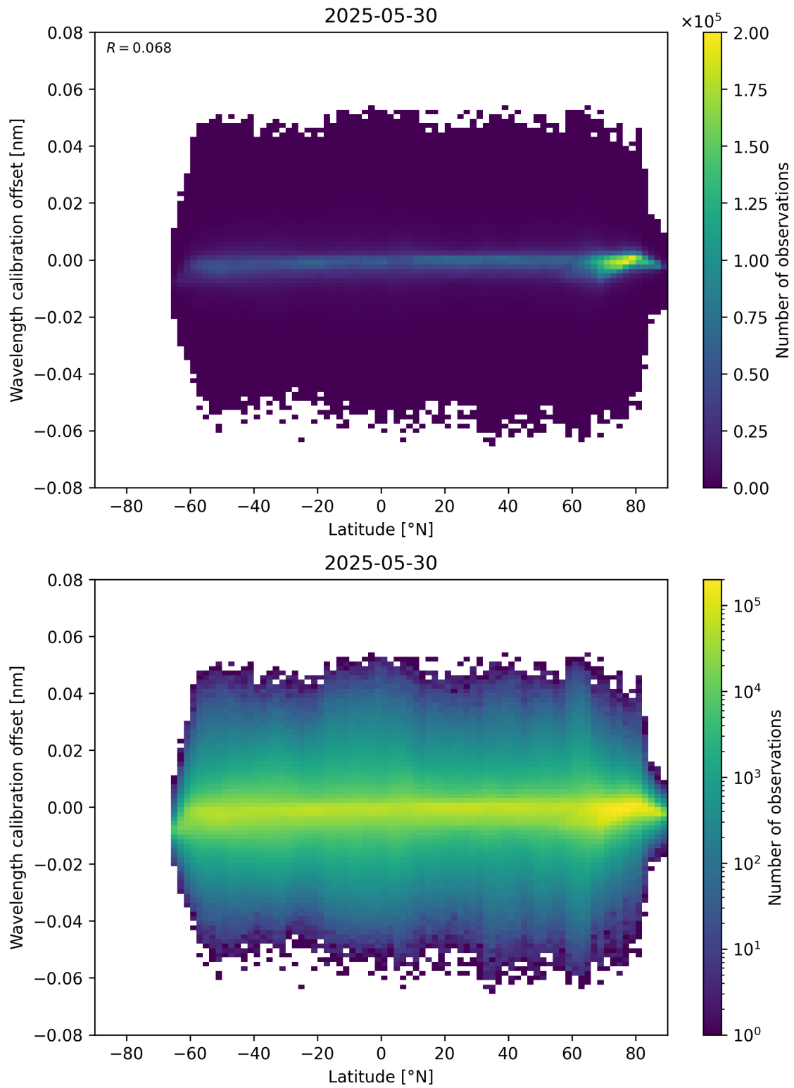
Figure 95: Scatter density plot of “Latitude” against “Wavelength calibration offset” for 2025-05-29 to 2025-05-31.
