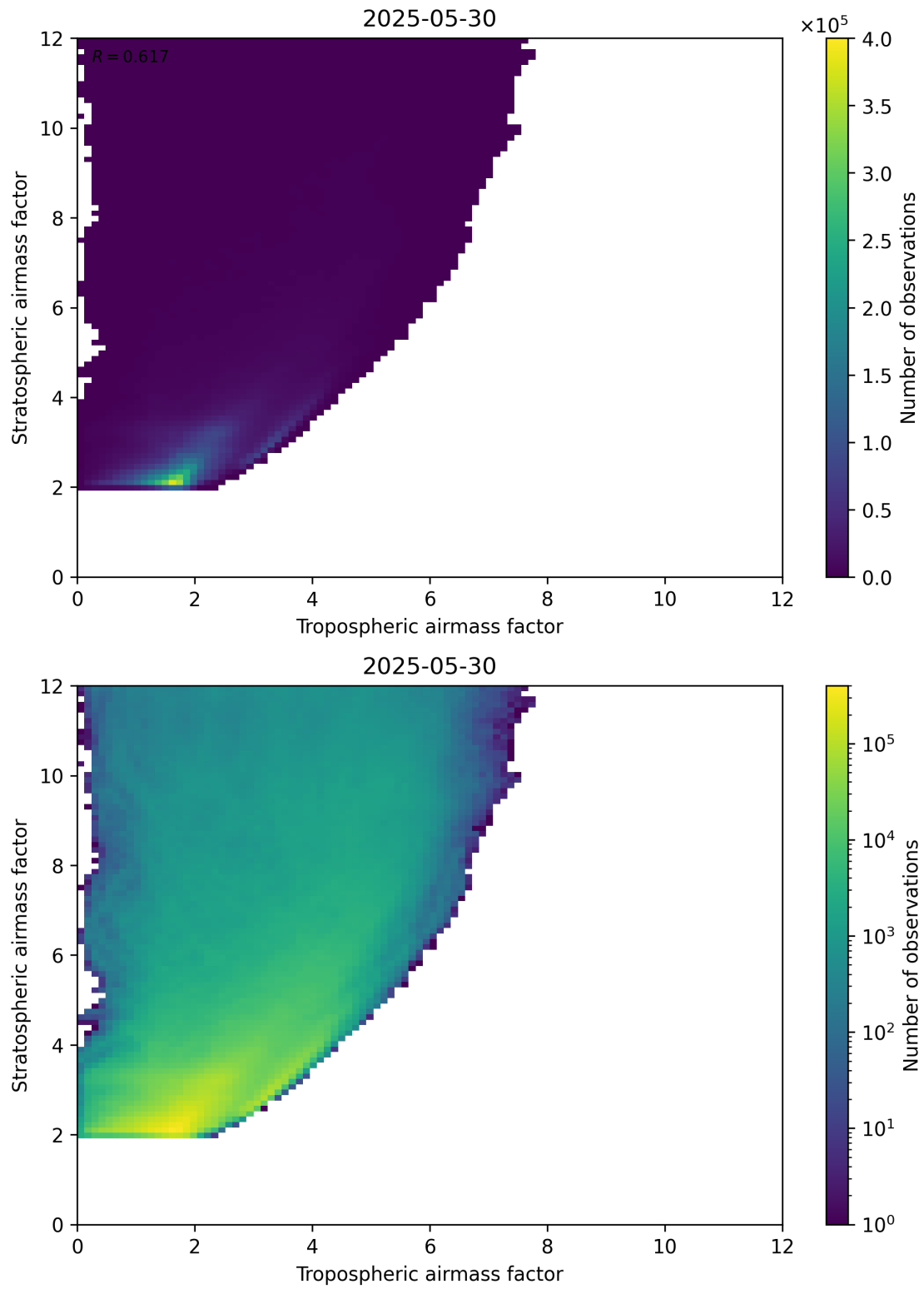
Figure 71: Scatter density plot of “Tropospheric airmass factor” against “Stratospheric airmass factor” for 2025-05-29 to 2025-05-31.
