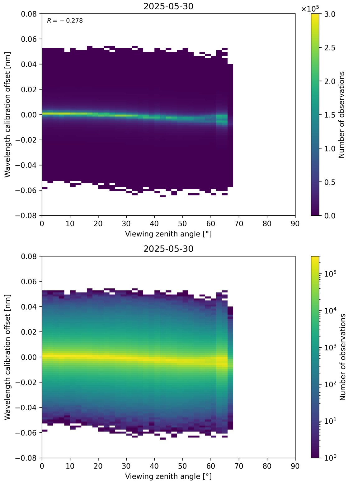
Figure 173: Scatter density plot of “Viewing zenith angle” against “Wavelength calibration offset” for 2025-05-29 to 2025-05-31.
