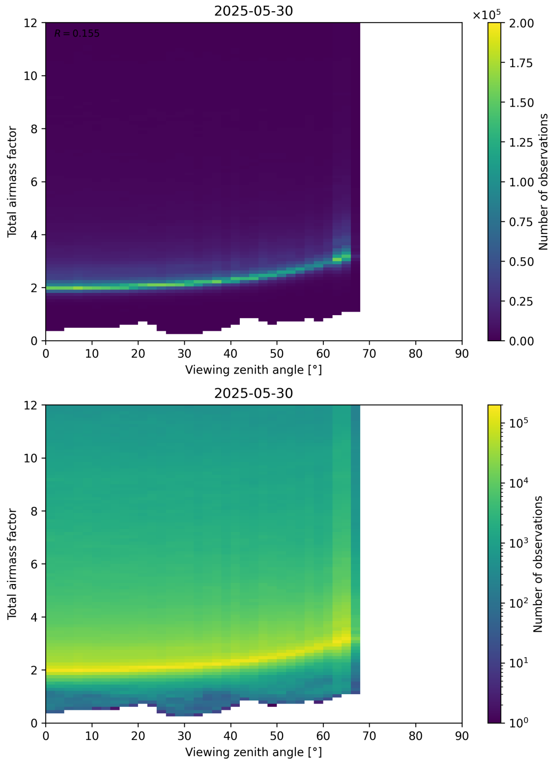
Figure 160: Scatter density plot of “Viewing zenith angle” against “Total airmass factor” for 2025-05-29 to 2025-05-31.
