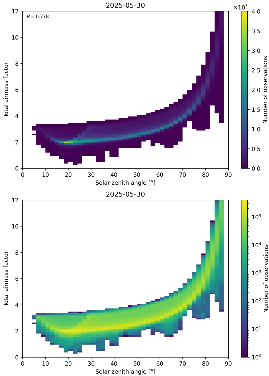
Figure 146: Scatter density plot of “Solar zenith angle” against “Total air mass factor” for 2025-05-29 to 2025-05-31.
