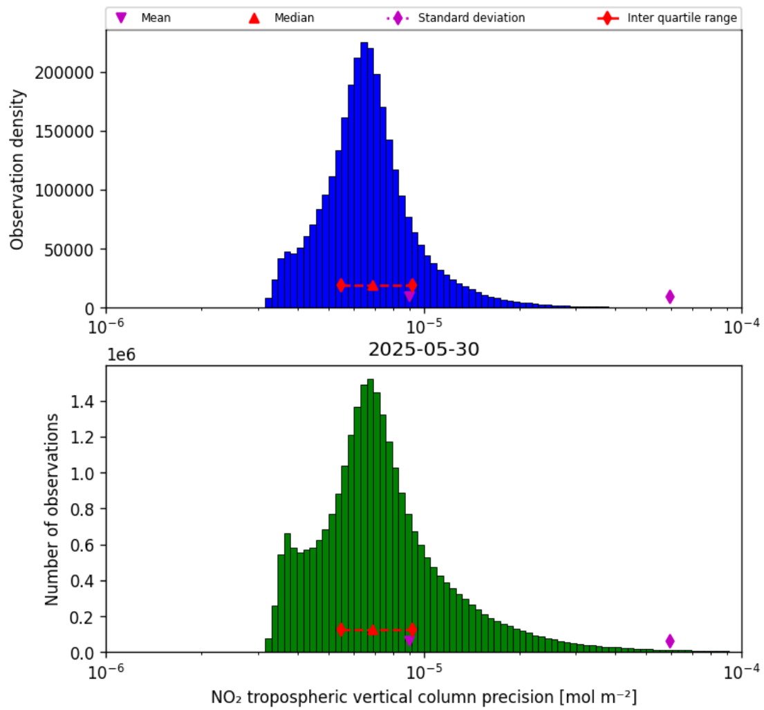
Figure 30: Histogram of “NO 2 tropospheric vertical column precision” for 2025-05-29 to 2025-05-31
