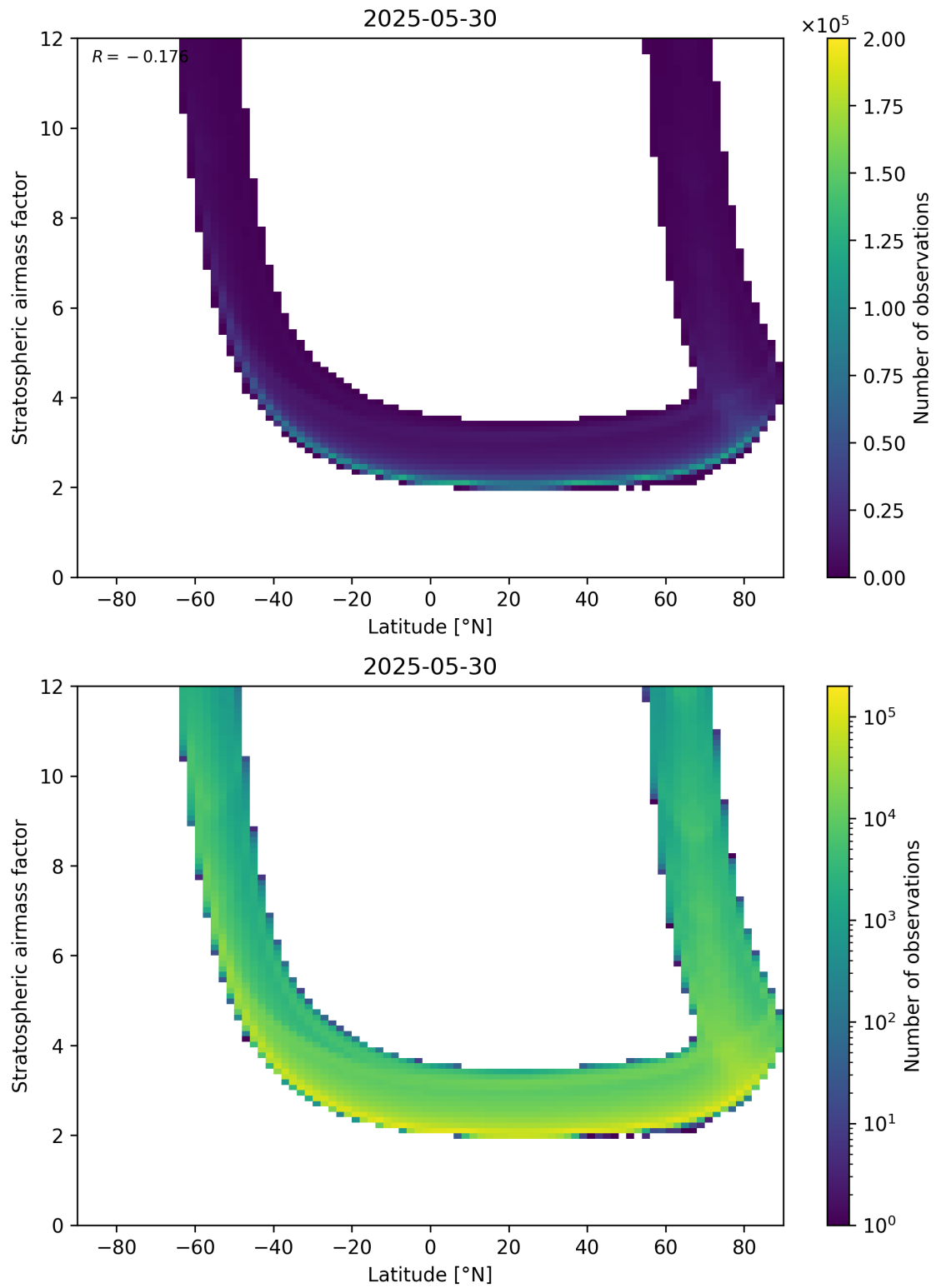
Figure 83: Scatter density plot of “Latitude” against “Stratospheric air mass factor” for 2025-05-29 to 2025-05-31.
