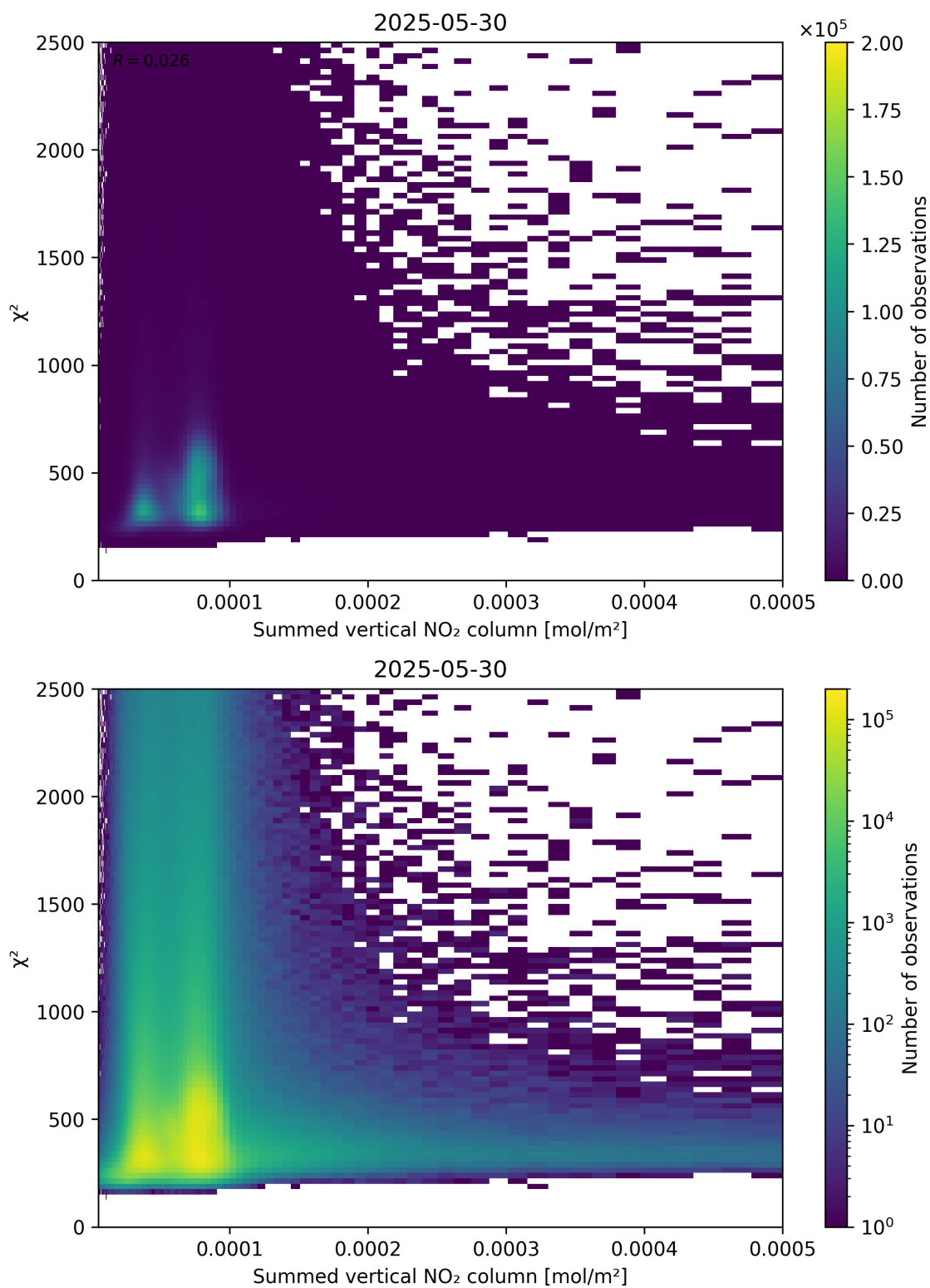
Figure 104: Scatter density plot of “Summed vertical NO 2 column” against “ \chi^2 ” for 2025-05-29 to 2025-05-31.
