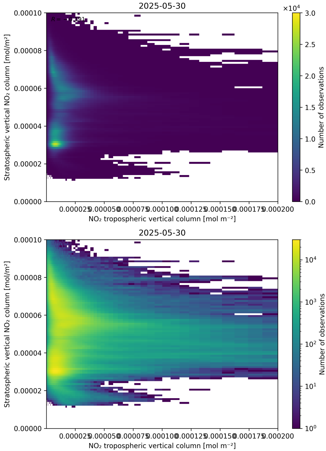
Figure 125: Scatter density plot of “NO 2 tropospheric vertical column” against “Stratospheric vertical NO 2 column” for 2025-05-29 to 2025-05-31.
