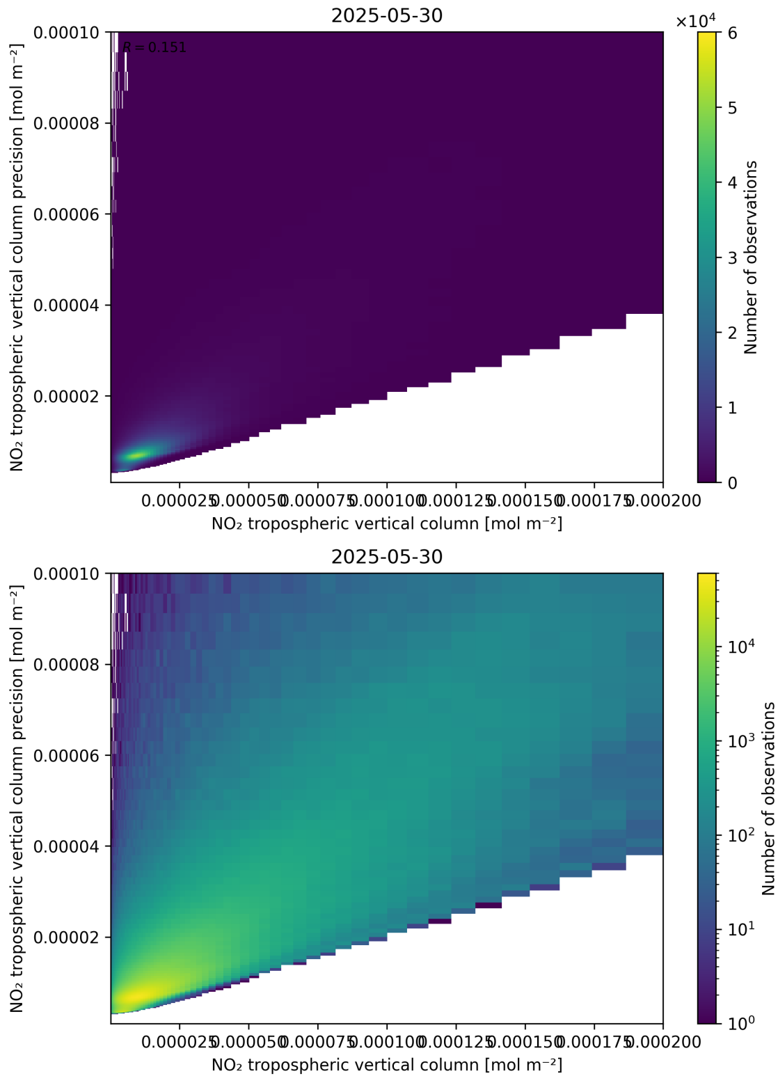
Figure 130: Scatter density plot of “NO 2 tropospheric vertical column” against “NO 2 tropospheric vertical column precision” for 2025-05-29 to 2025-05-31.
