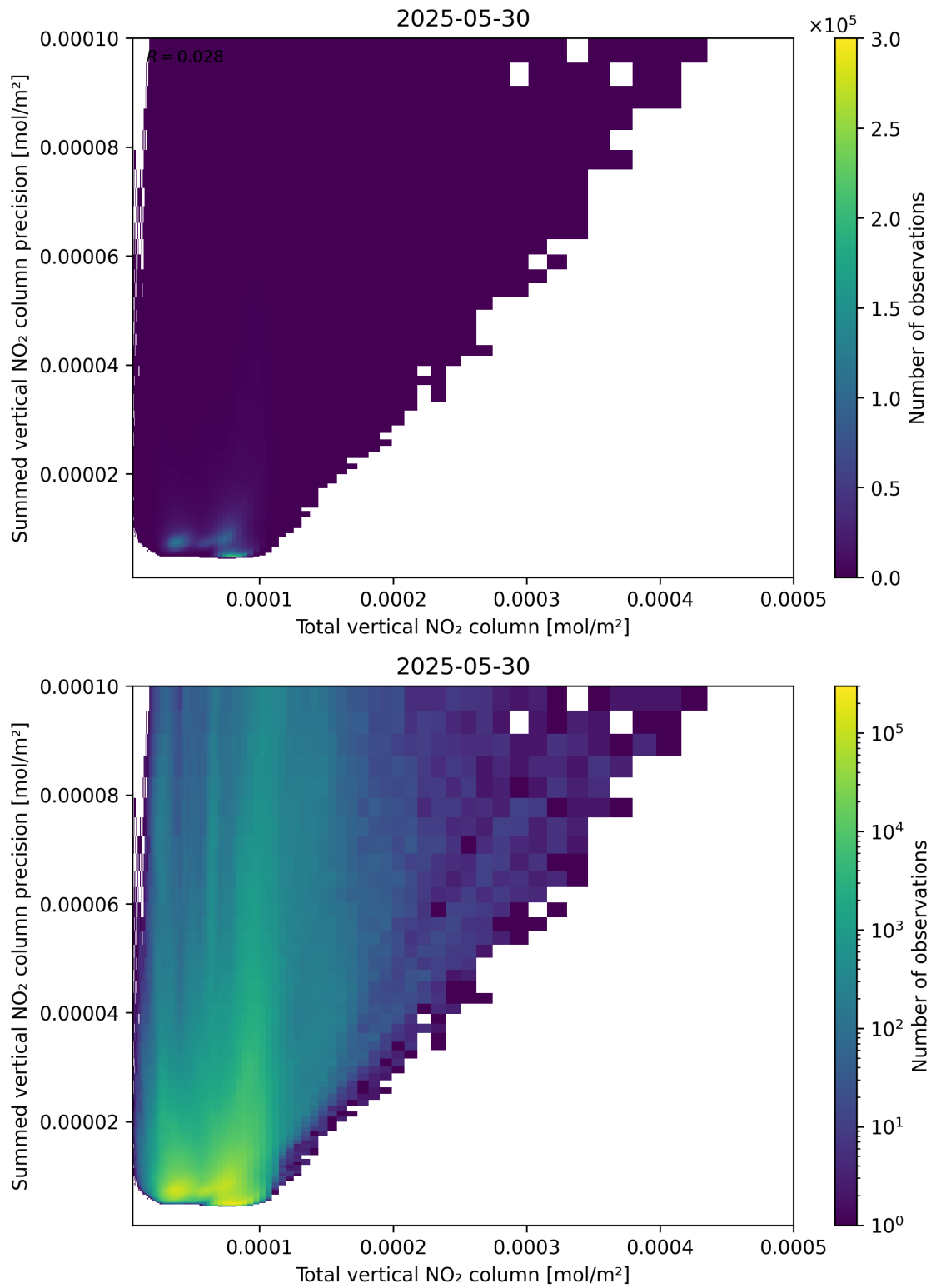
Figure 113: Scatter density plot of “Total vertical NO 2 column” against “Summed vertical NO 2 column precision” for 2025-05-29 to 2025-05-31.
