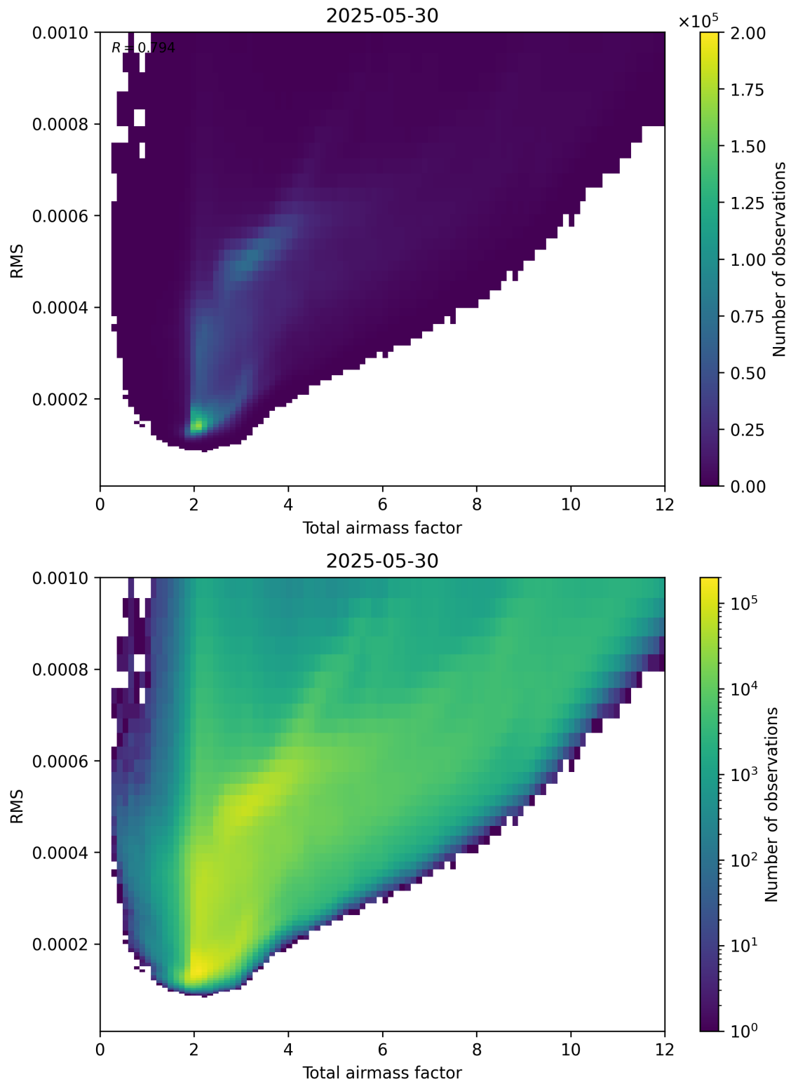
Figure 69: Scatter density plot of “Total airmass factor” against “RMS” for 2025-05-29 to 2025-05-31.
