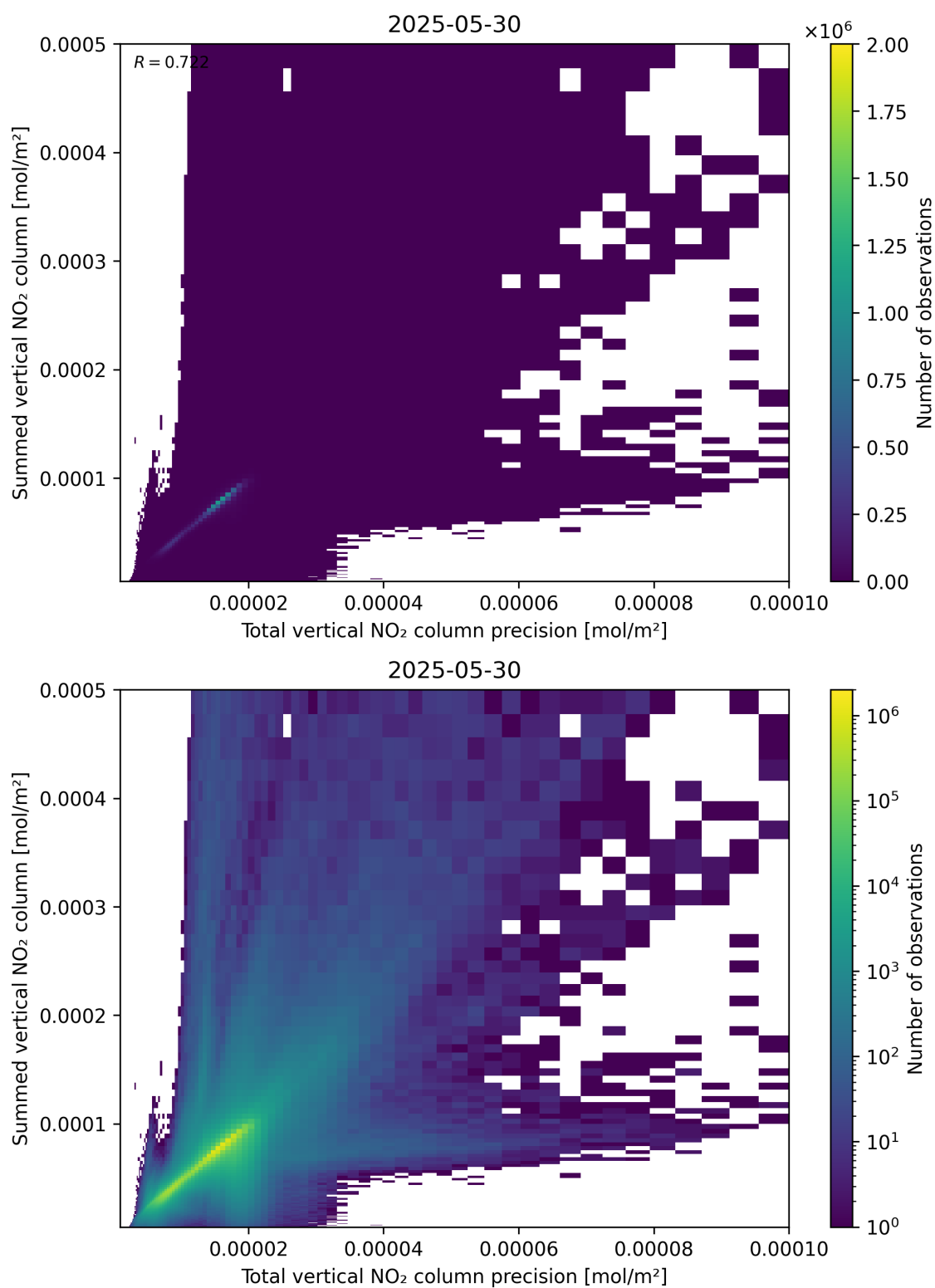
Figure 117: Scatter density plot of “Total vertical NO 2 column precision” against “Summed vertical NO 2 column” for 2025-05-29 to 2025-05-31.
