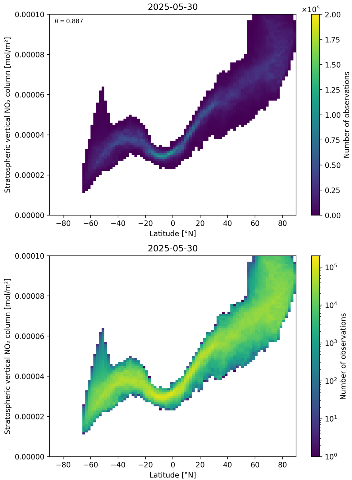
Figure 87: Scatter density plot of “Latitude” against “Stratospheric vertical \text{NO}_2 column” for 2025-05-29 to 2025-05-31.
