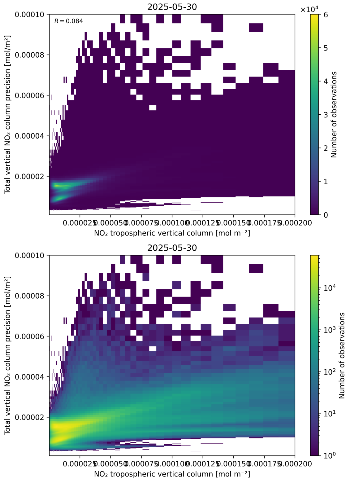
Figure 129: Scatter density plot of “NO 2 tropospheric vertical column” against “Total vertical NO 2 column precision” for 2025-05-29 to 2025-05-31.
