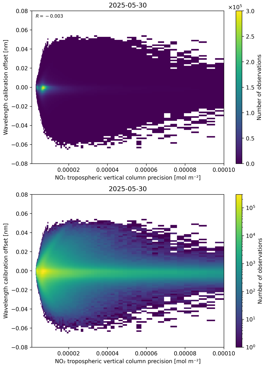
Figure 141: Scatter density plot of “NO 2 tropospheric vertical column precision” against “Wavelength calibration offset” for 2025-05-29 to 2025-05-31.
