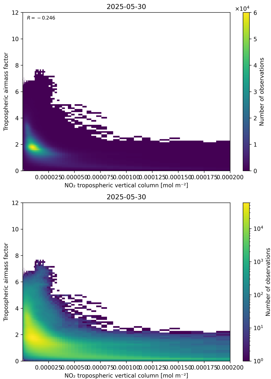
Figure 123: Scatter density plot of “NO 2 tropospheric vertical column” against “Tropospheric air mass factor” for 2025-05-29 to 2025-05-31.
