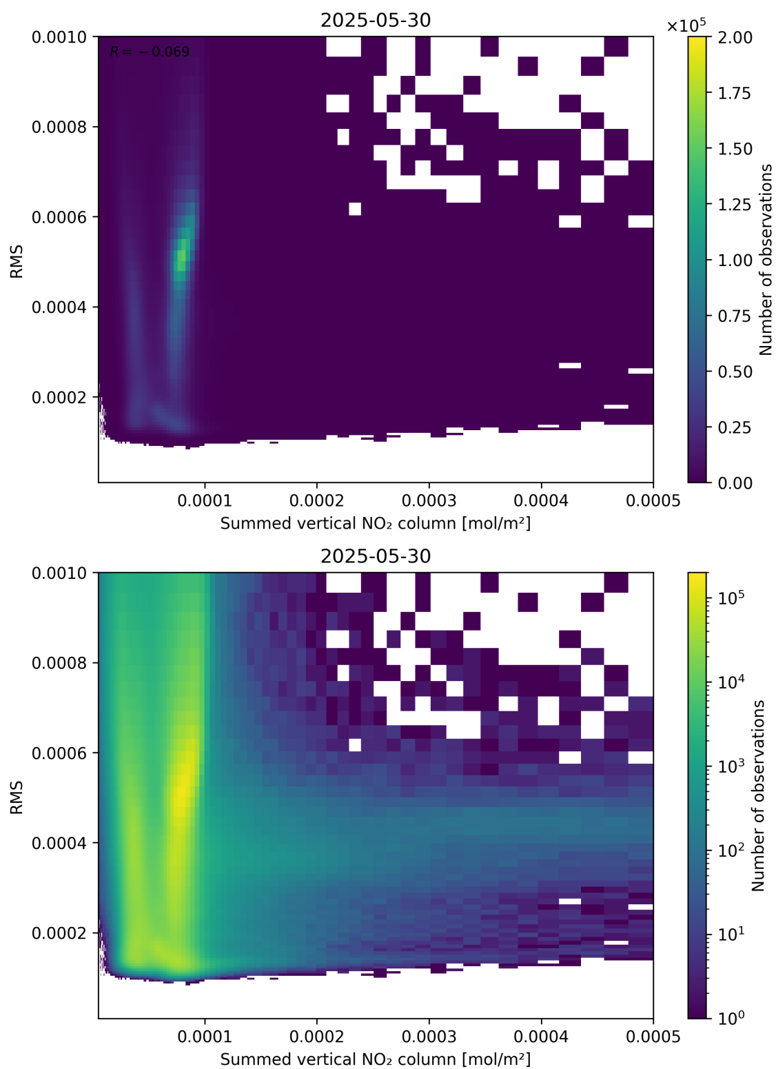
Figure 109: Scatter density plot of “Summed vertical NO 2 column” against “RMS” for 2025-05-29 to 2025-05-31.
