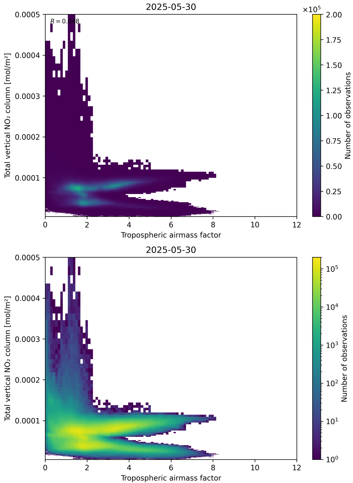
Figure 77: Scatter density plot of “Tropospheric airmass factor” against “Total vertical NO 2 column” for 2025-05-29 to 2025-05-31.
