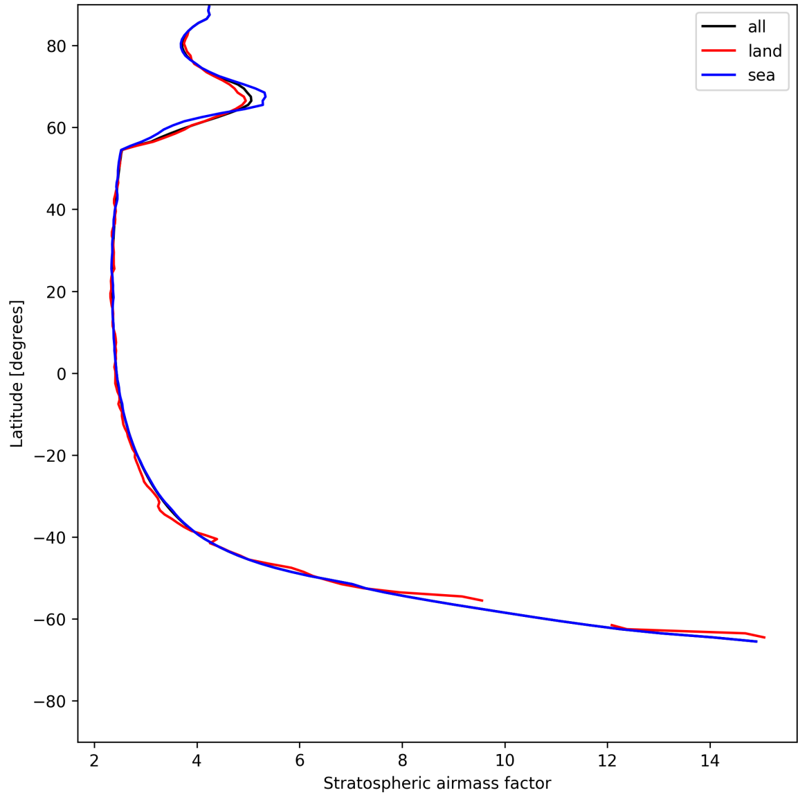
Figure 27: Zonal average of “Stratospheric air mass factor” for 2025-05-29 to 2025-05-31.
