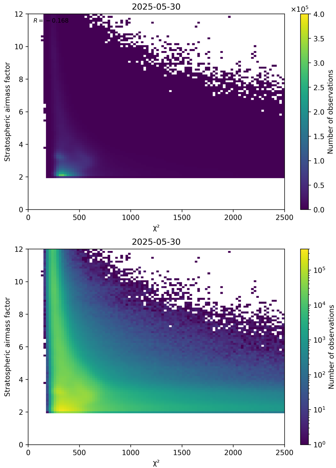
Figure 81: Scatter density plot of “ \chi^2 ” against “Stratospheric airmass factor” for 2025-05-29 to 2025-05-31.
