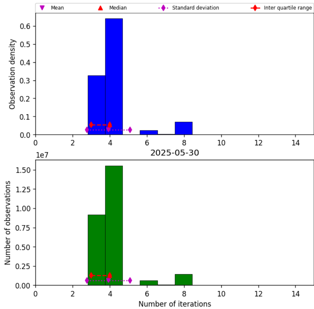
Figure 34: Histogram of "Number of iterations" for 2025-05-29 to 2025-05-31
