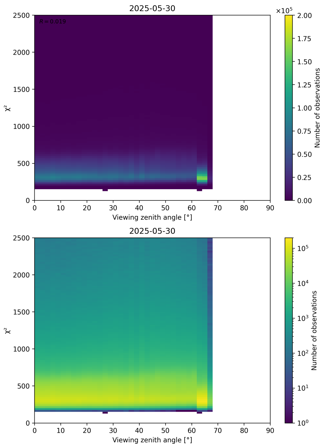
Figure 162: Scatter density plot of “Viewing zenith angle” against “ \chi^2 ” for 2025-05-29 to 2025-05-31.
