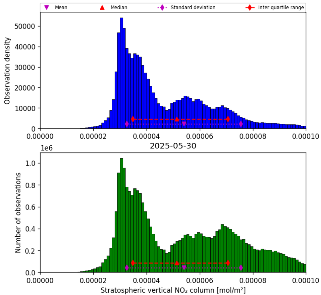
Figure 36: Histogram of “Stratospheric vertical NO 2 column” for 2025-05-29 to 2025-05-31
