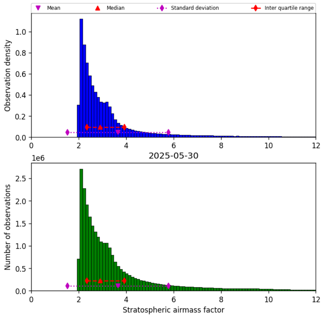
Figure 44: Histogram of “Stratospheric airmass factor” for 2025-05-29 to 2025-05-31
