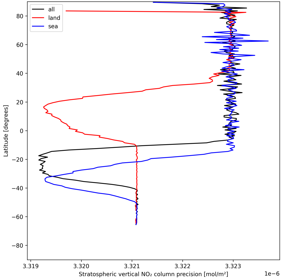
Figure 20: Zonal average of “Stratospheric vertical NO 2 column precision” for 2025-05-29 to 2025-05-31.
