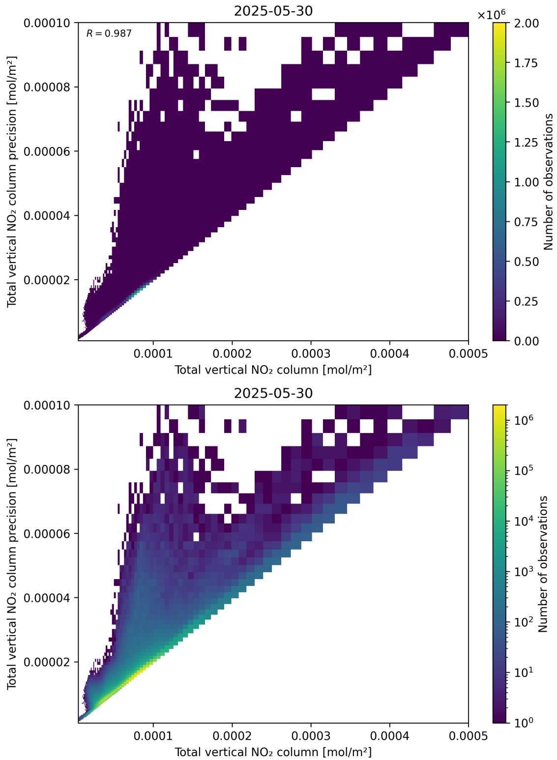
Figure 114: Scatter density plot of “Total vertical NO 2 column” against “Total vertical NO 2 column precision” for 2025-05-29 to 2025-05-31.
