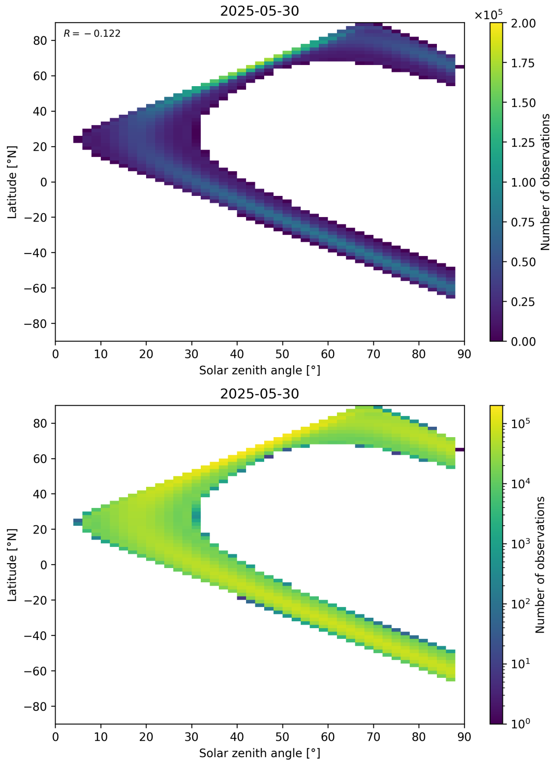
Figure 149: Scatter density plot of “Solar zenith angle” against “Latitude” for 2025-05-29 to 2025-05-31.
