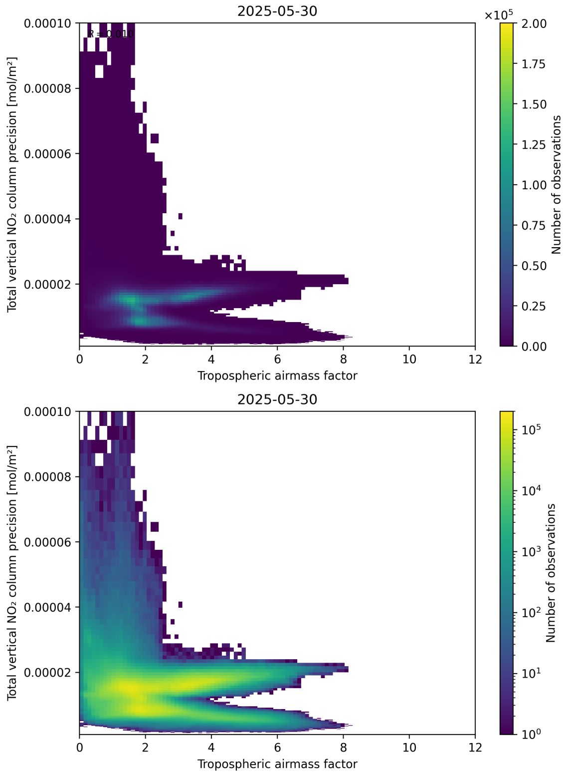
Figure 78: Scatter density plot of “Tropospheric air mass factor” against “Total vertical NO 2 column precision” for 2025-05-29 to 2025-05-31.
