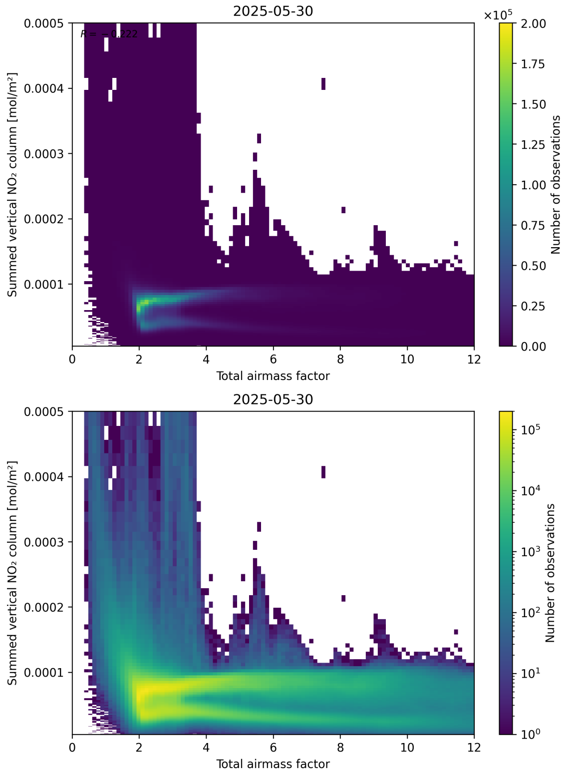
Figure 65: Scatter density plot of “Total airmass factor” against “Summed vertical NO 2 column” for 2025-05-29 to 2025-05-31.
