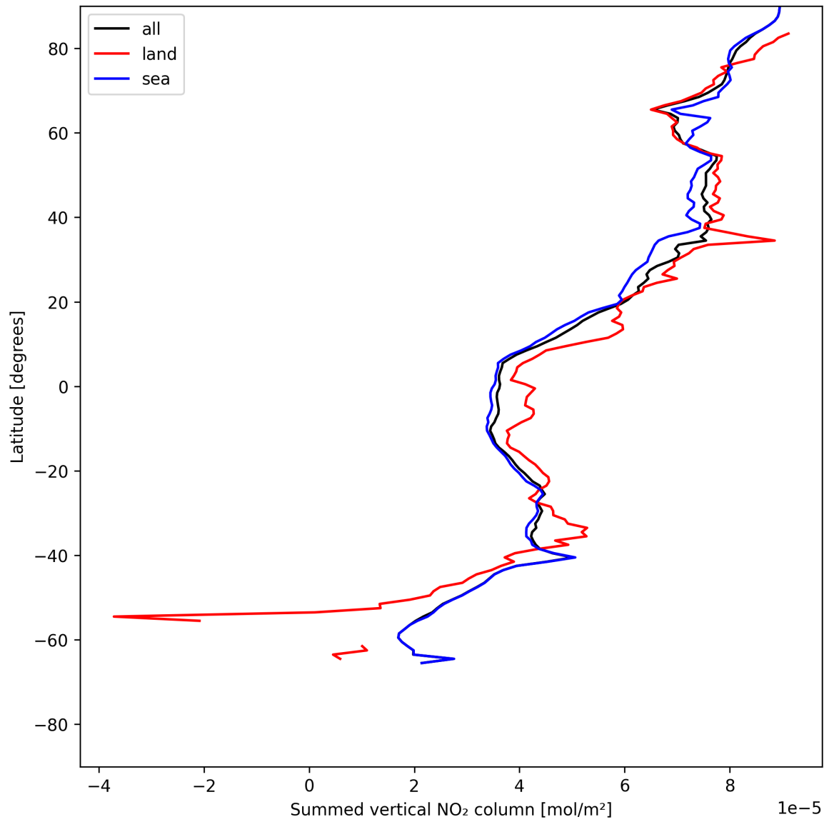
Figure 23: Zonal average of “Summed vertical NO 2 column” for 2025-05-29 to 2025-05-31.
