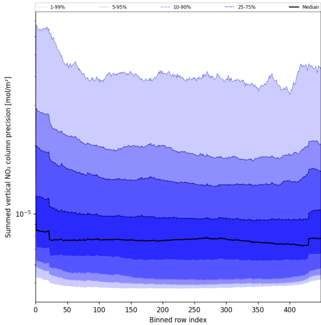
Figure 58: Along track statistics of “Summed vertical NO 2 column precision” for 2025-05-29 to 2025-05-31
