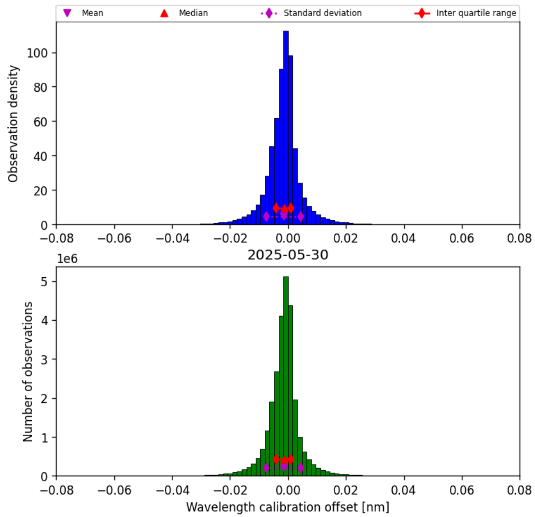
Figure 35: Histogram of “Wavelength calibration offset” for 2025-05-29 to 2025-05-31
