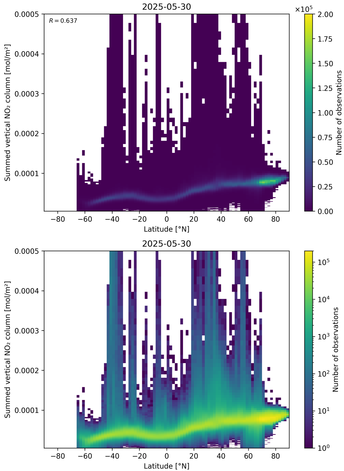
Figure 88: Scatter density plot of “Latitude” against “Summed vertical NO 2 column” for 2025-05-29 to 2025-05-31.
