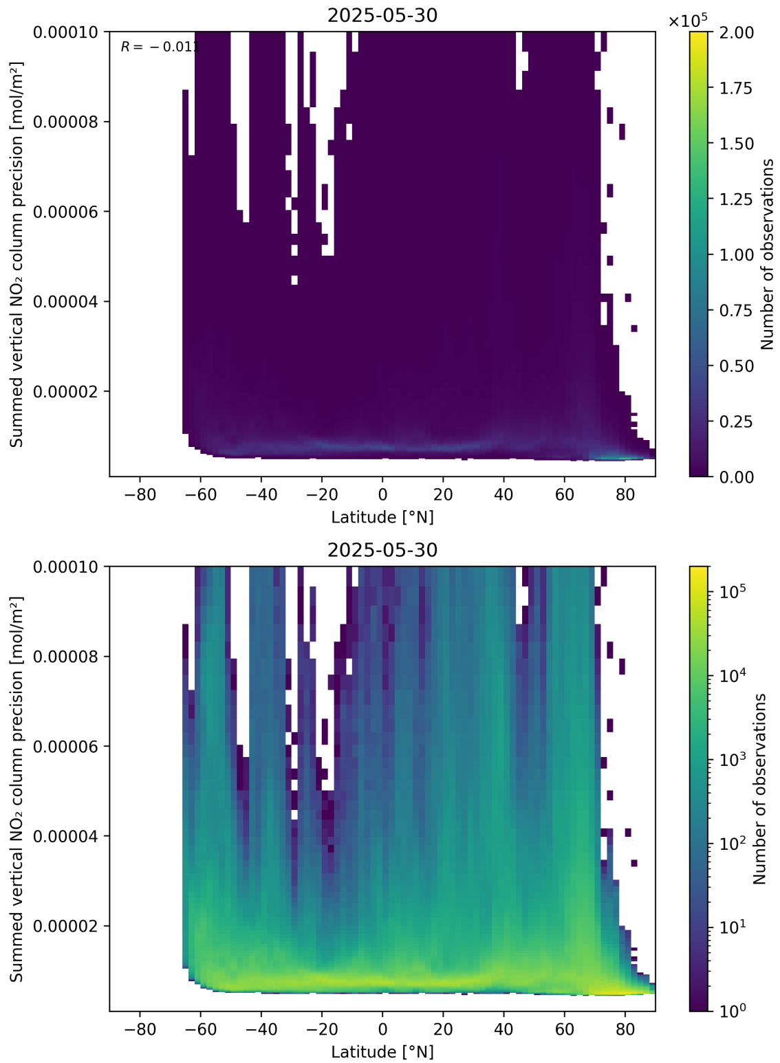
Figure 89: Scatter density plot of “Latitude” against “Summed vertical NO 2 column precision” for 2025-05-29 to 2025-05-31.
