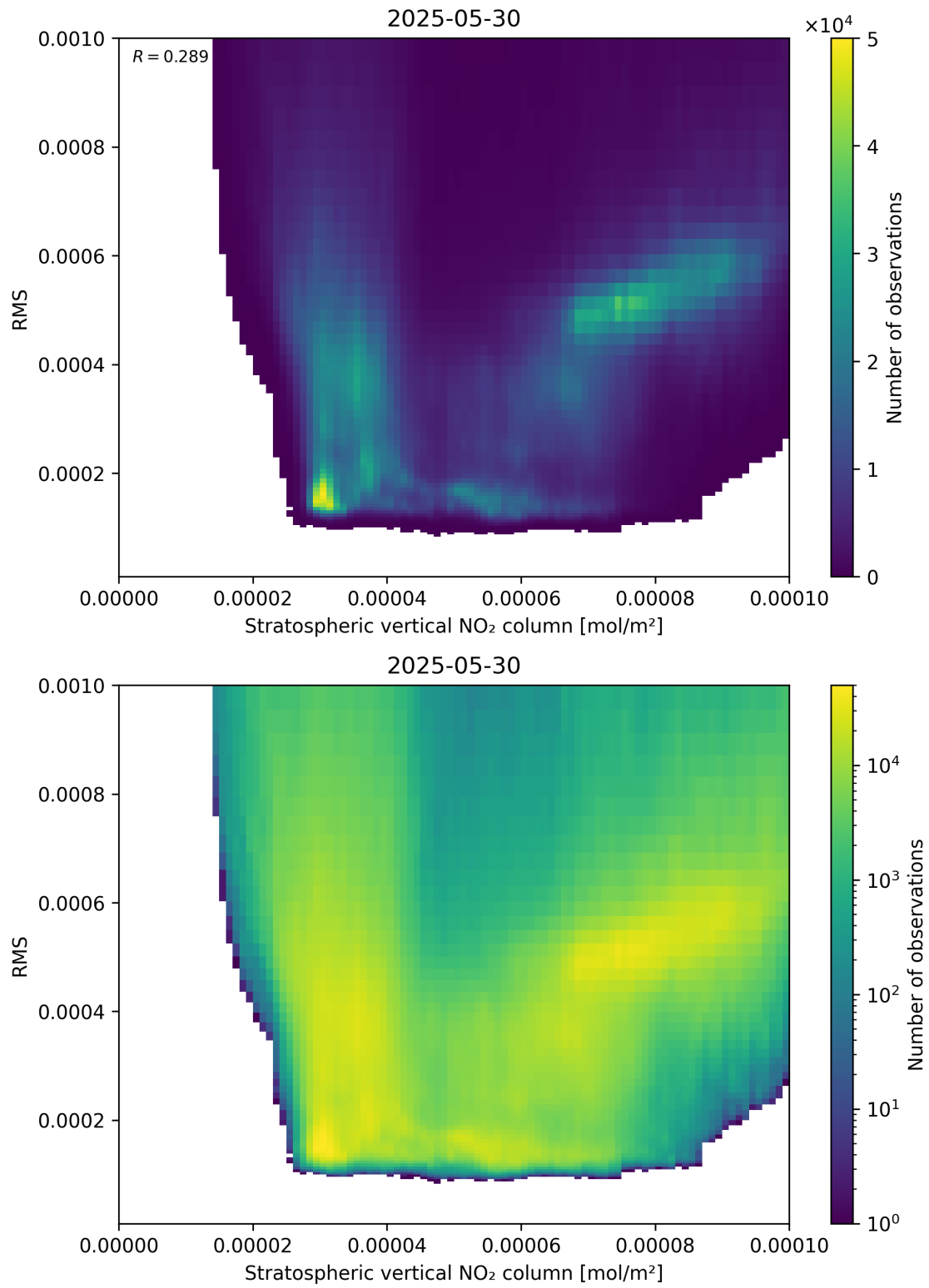
Figure 102: Scatter density plot of “Stratospheric vertical NO 2 column” against “RMS” for 2025-05-29 to 2025-05-31.
