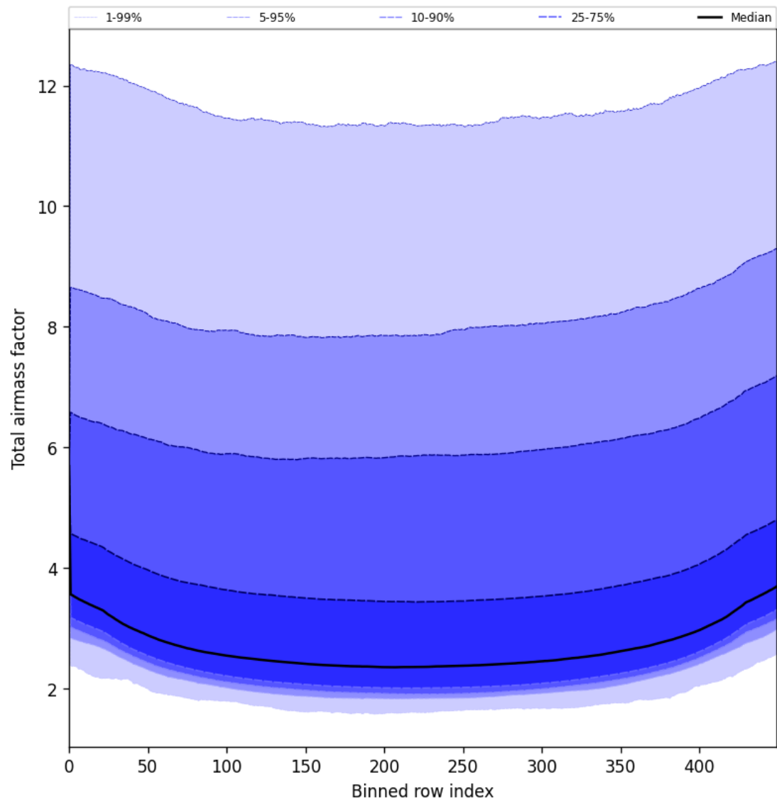
Figure 49: Along track statistics of “Total airmass factor” for 2025-05-29 to 2025-05-31
