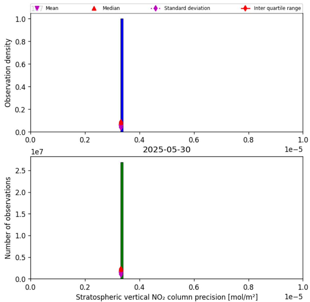
Figure 37: Histogram of “Stratospheric vertical NO 2 column precision” for 2025-05-29 to 2025-05-31
