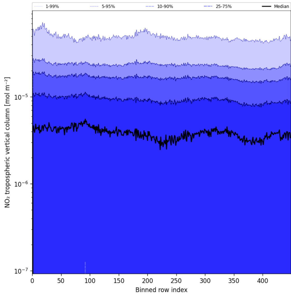
Figure 46: Along track statistics of “NO 2 tropospheric vertical column” for 2025-05-29 to 2025-05-31
