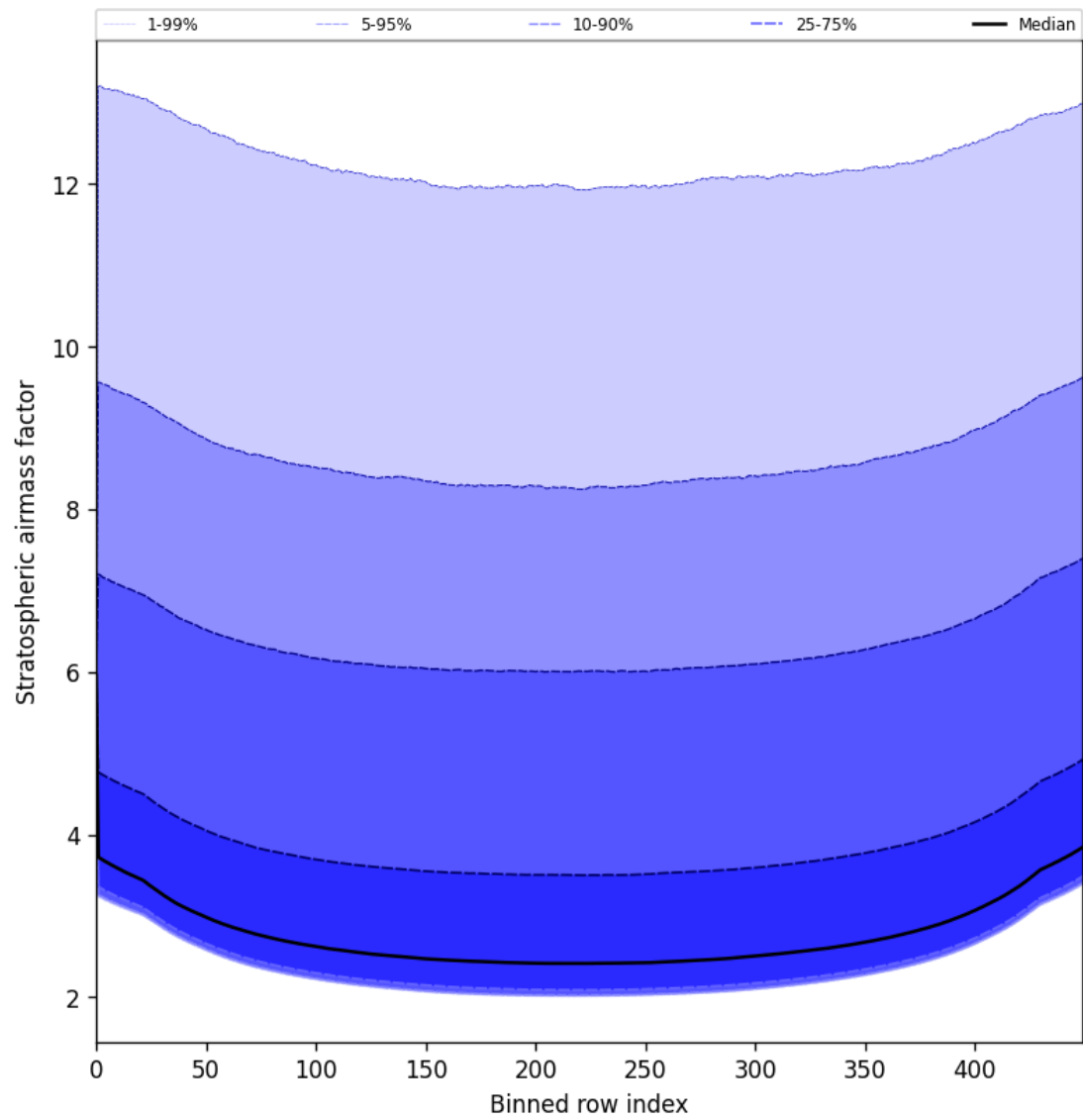
Figure 61: Along track statistics of “Stratospheric airmass factor” for 2025-05-29 to 2025-05-31
