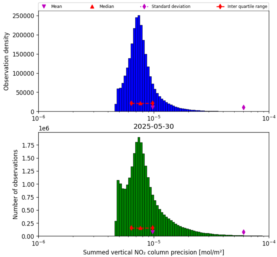
Figure 41: Histogram of "Summed vertical NO 2 column precision" for 2025-05-29 to 2025-05-31
