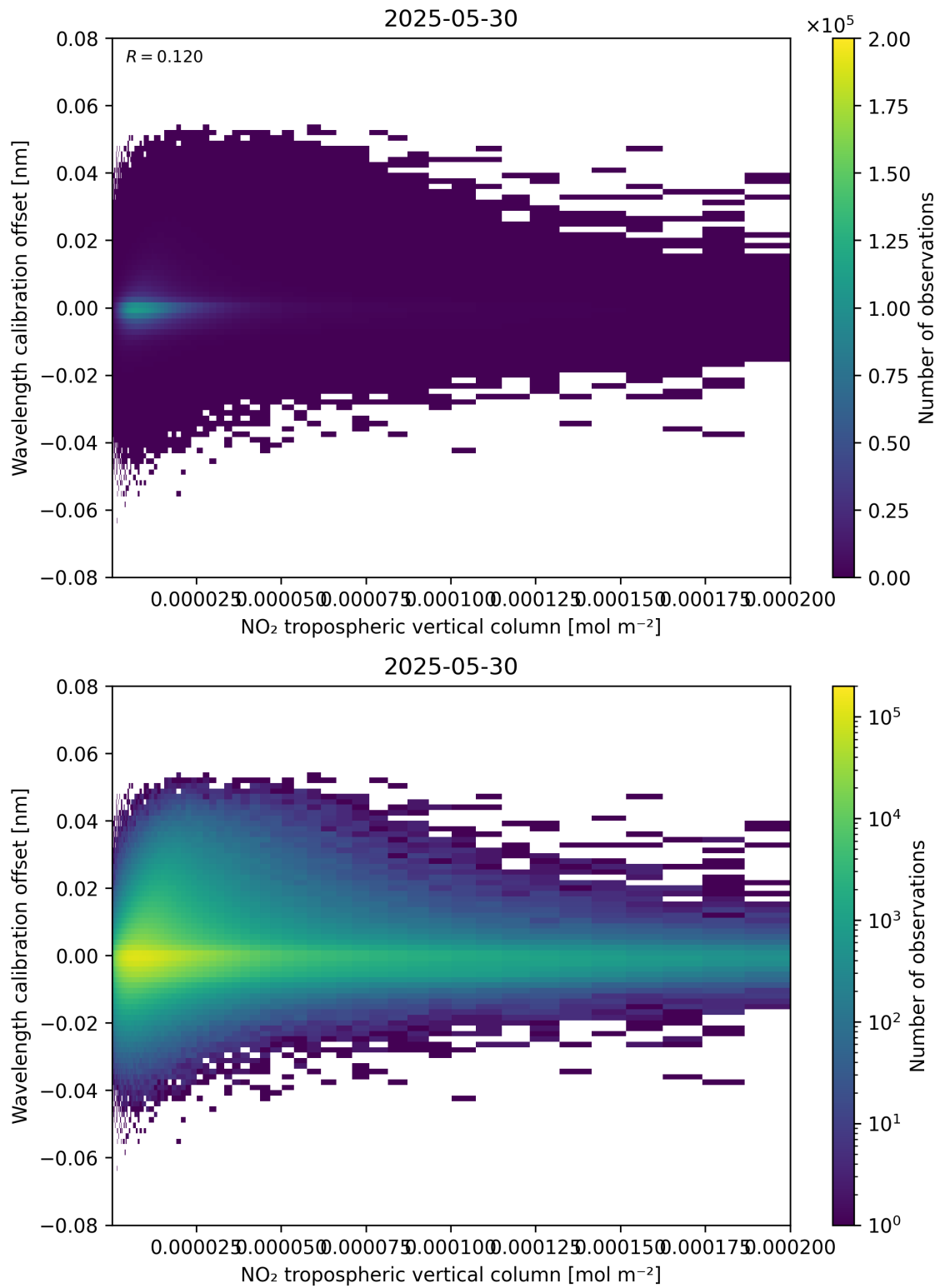
Figure 143: Scatter density plot of “NO 2 tropospheric vertical column” against “Wavelength calibration offset” for 2025-05-29 to 2025-05-31.
