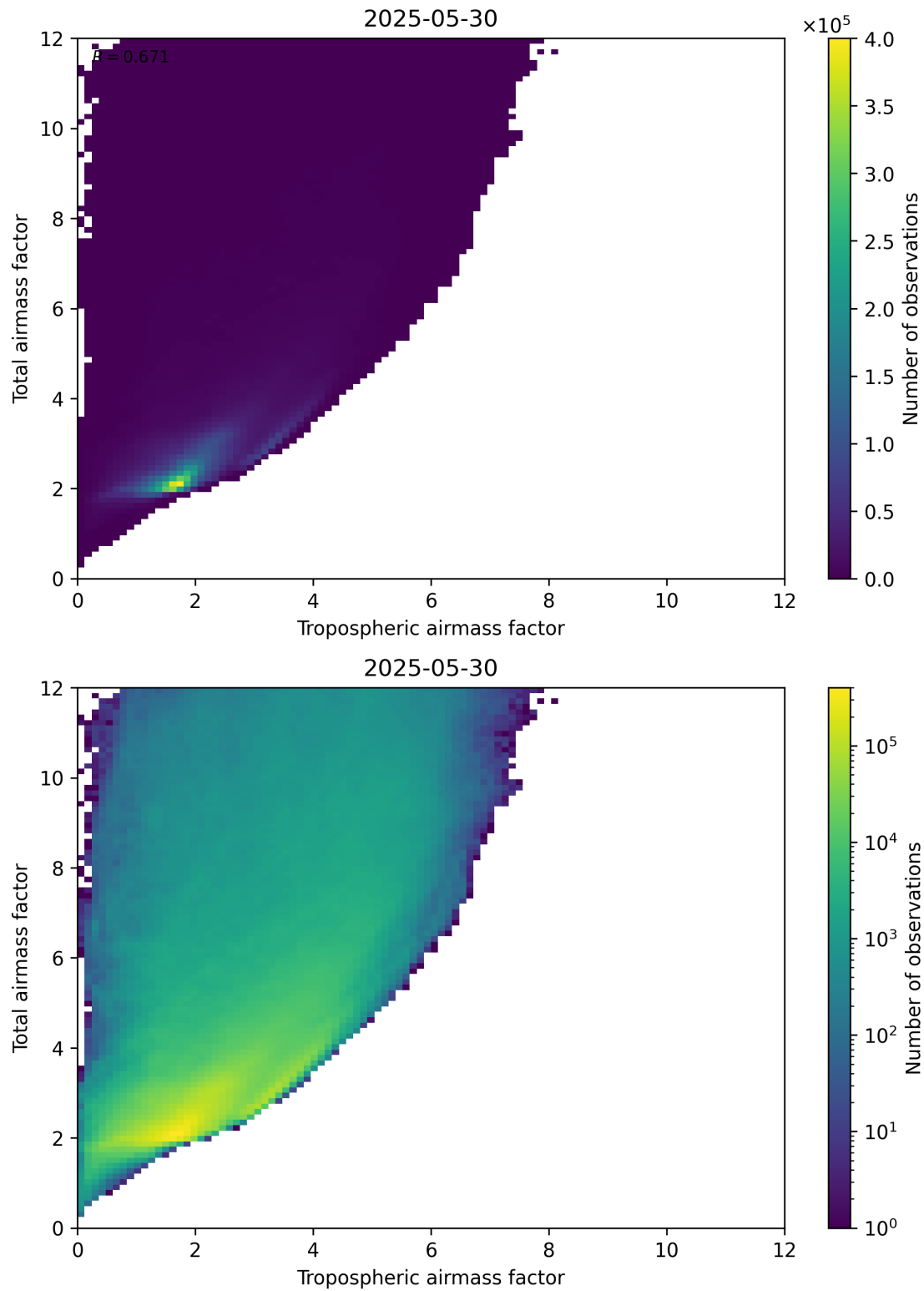
Figure 72: Scatter density plot of “Tropospheric airmass factor” against “Total airmass factor” for 2025-05-29 to 2025-05-31.
