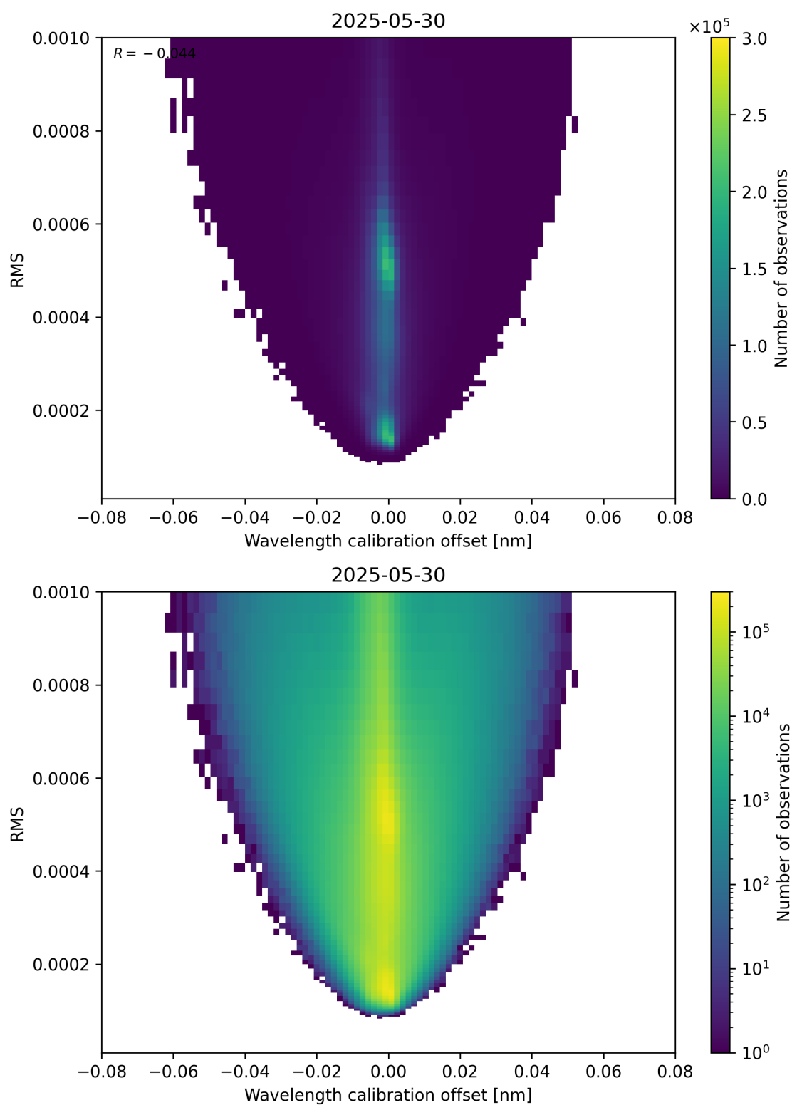
Figure 181: Scatter density plot of “Wavelength calibration offset” against “RMS” for 2025-05-29 to 2025-05-31.
