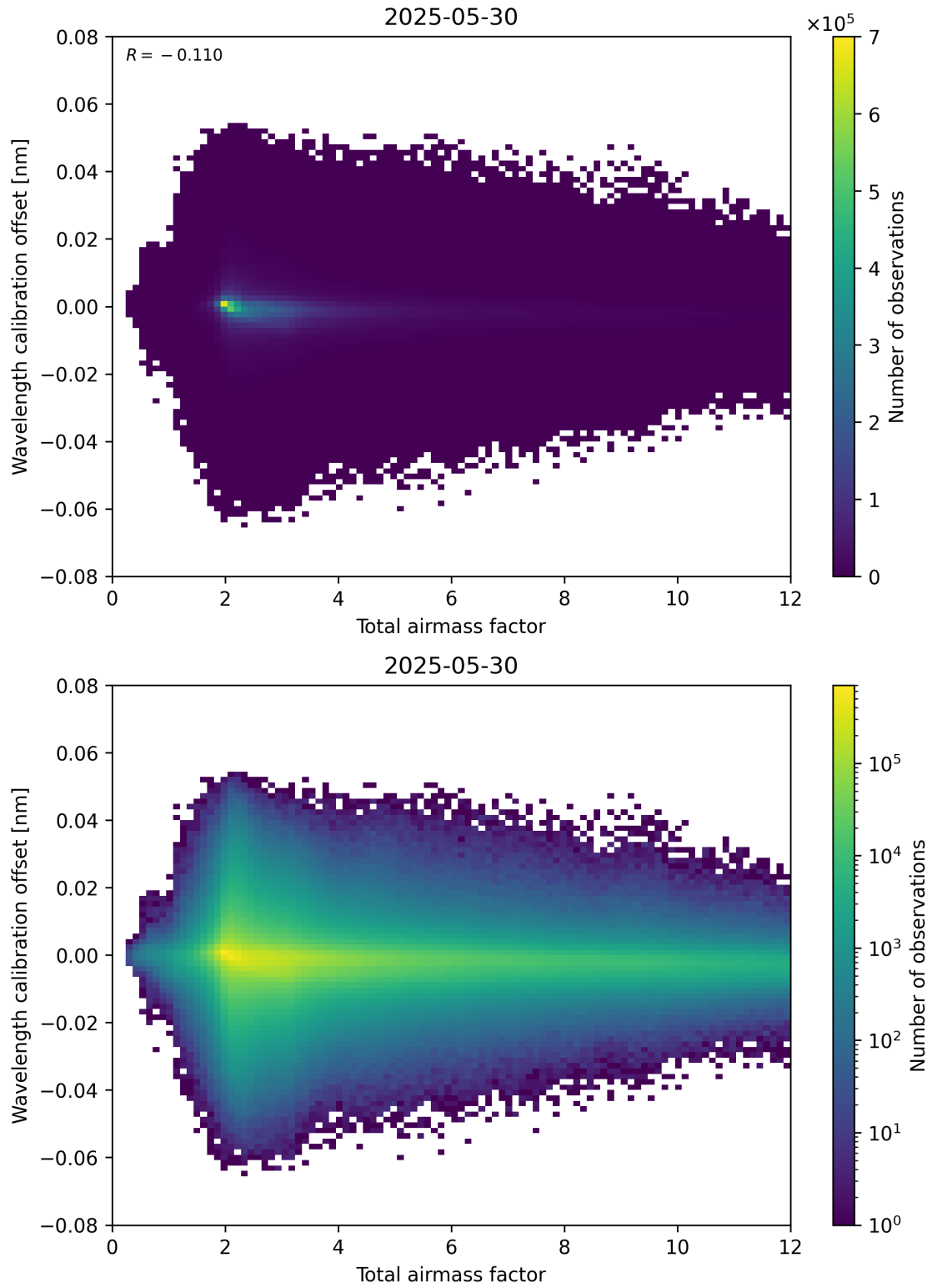
Figure 70: Scatter density plot of “Total airmass factor” against “Wavelength calibration offset” for 2025-05-29 to 2025-05-31.
