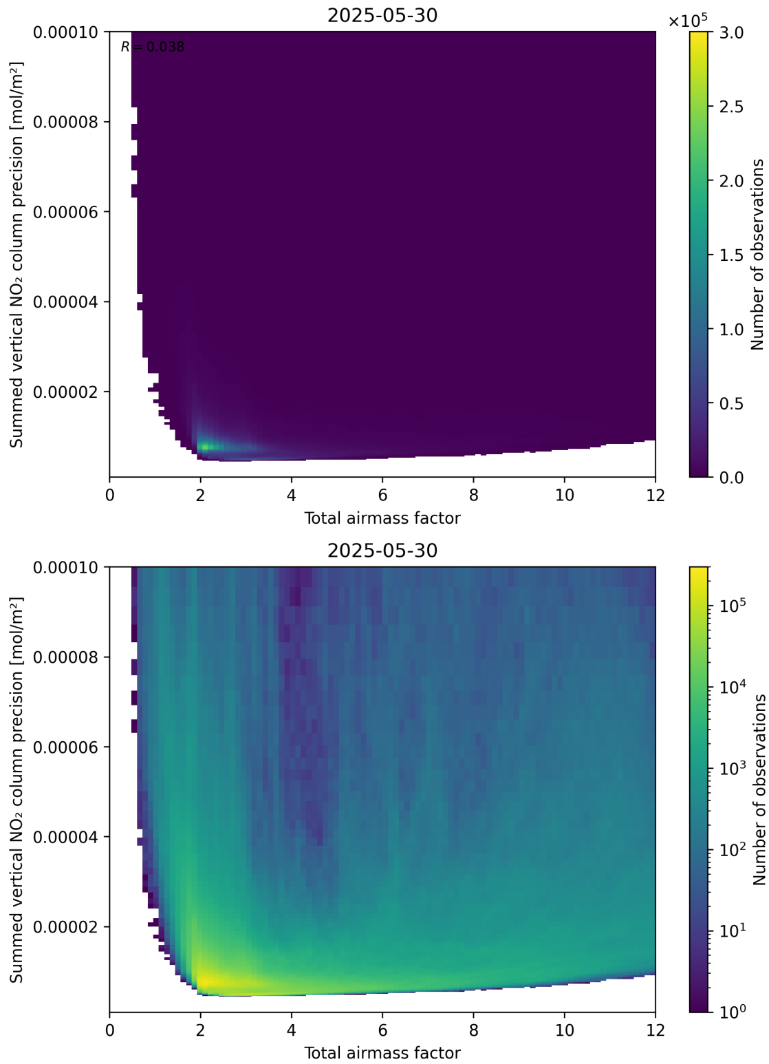
Figure 66: Scatter density plot of “Total airmass factor” against “Summed vertical NO 2 column precision” for 2025-05-29 to 2025-05-31.
