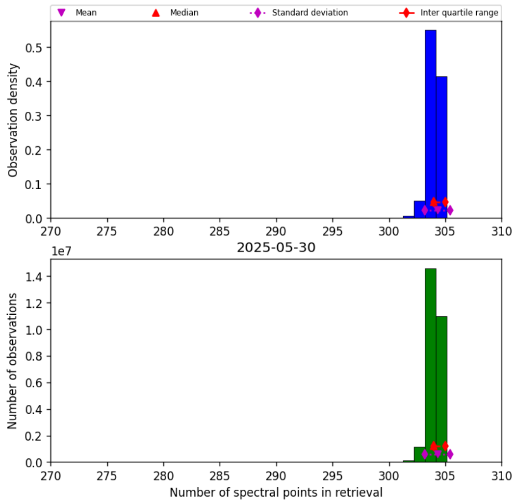
Figure 33: Histogram of “Number of spectral points in retrieval” for 2025-05-29 to 2025-05-31
