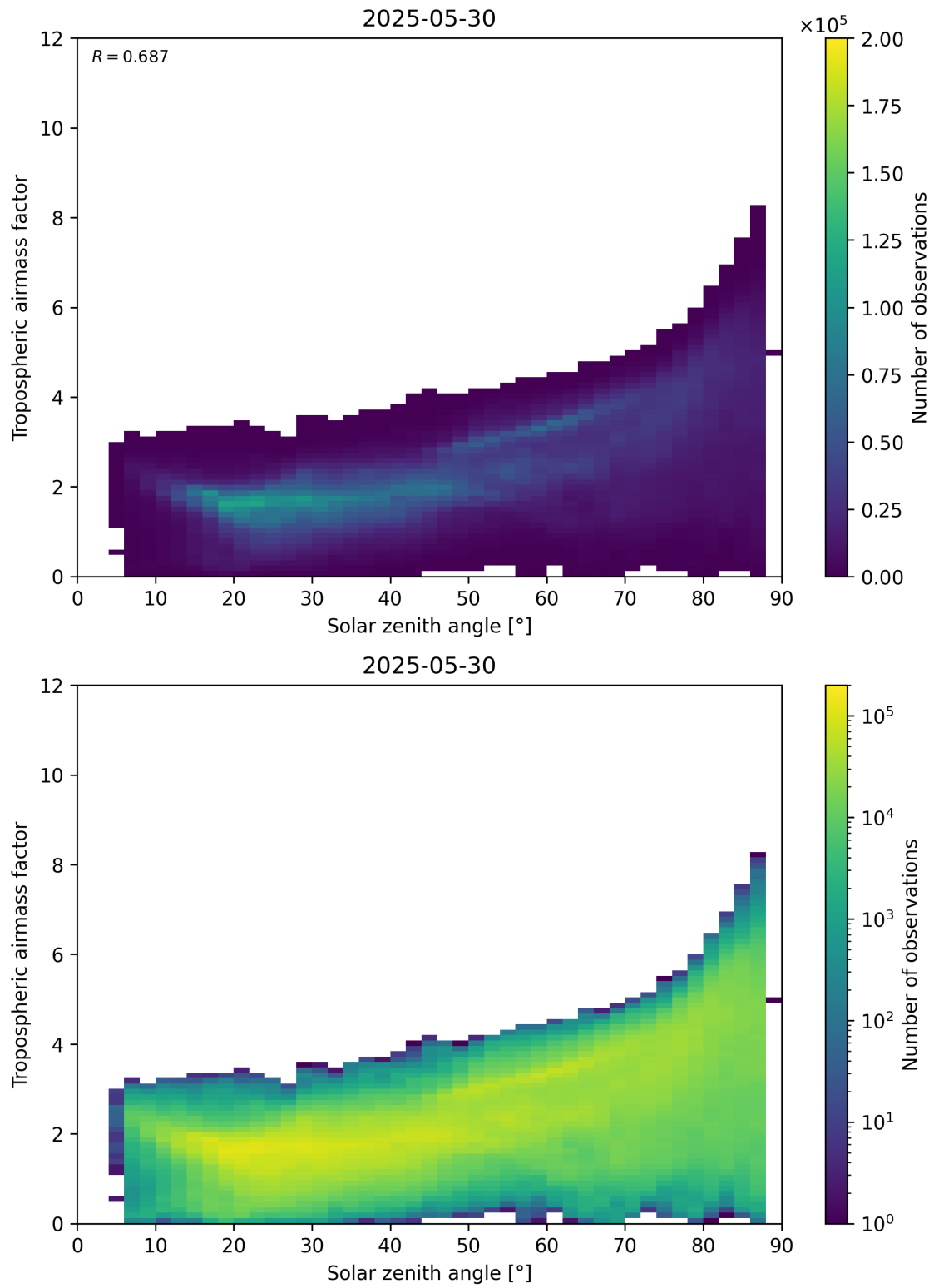
Figure 147: Scatter density plot of “Solar zenith angle” against “Tropospheric airmass factor” for 2025-05-29 to 2025-05-31.
