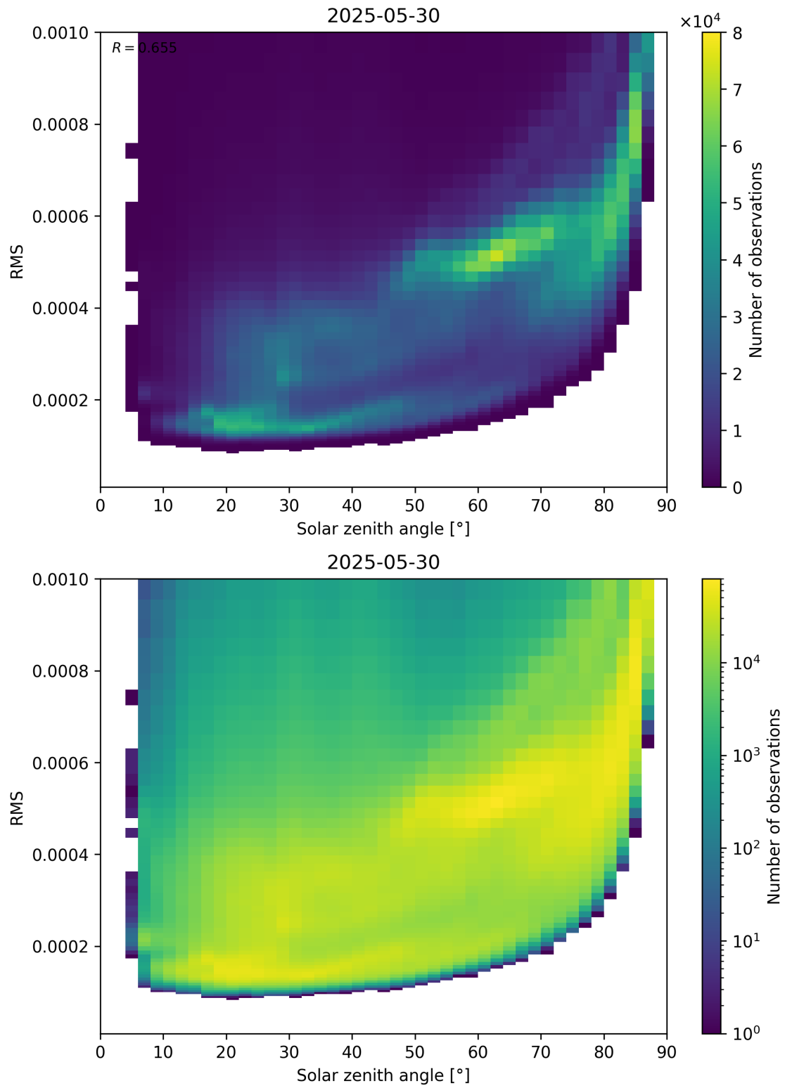
Figure 157: Scatter density plot of “Solar zenith angle” against “RMS” for 2025-05-29 to 2025-05-31.
