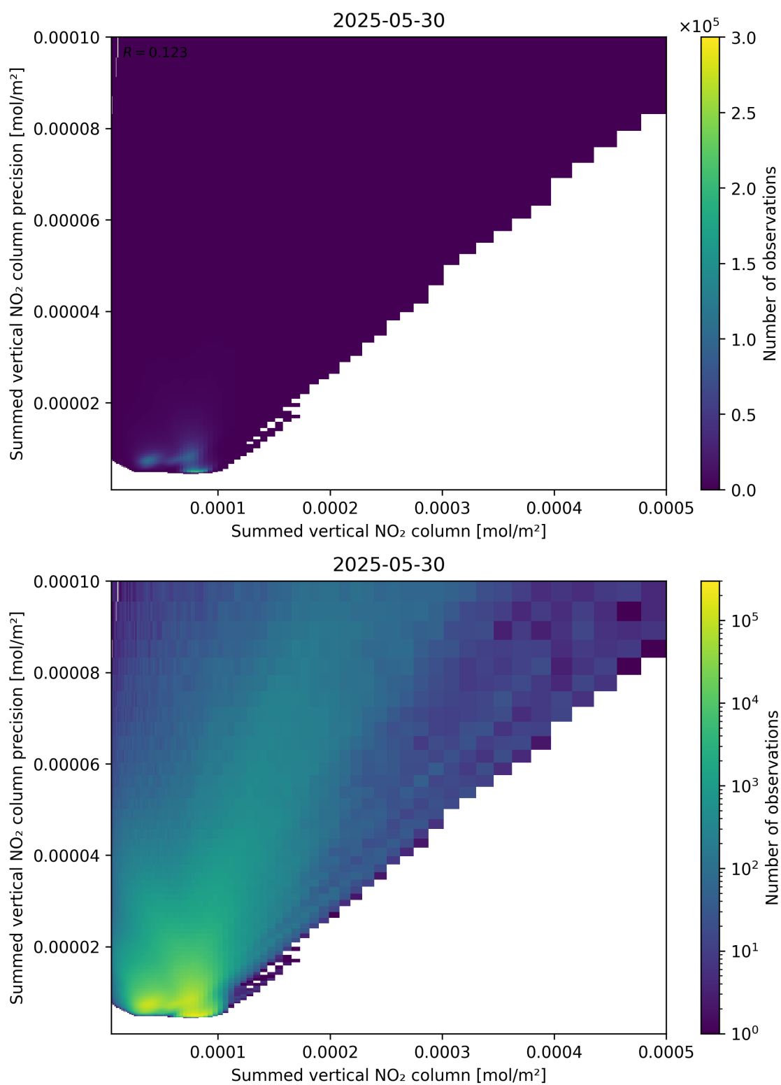
Figure 105: Scatter density plot of “Summed vertical NO 2 column” against “Summed vertical NO 2 column precision” for 2025-05-29 to 2025-05-31.
