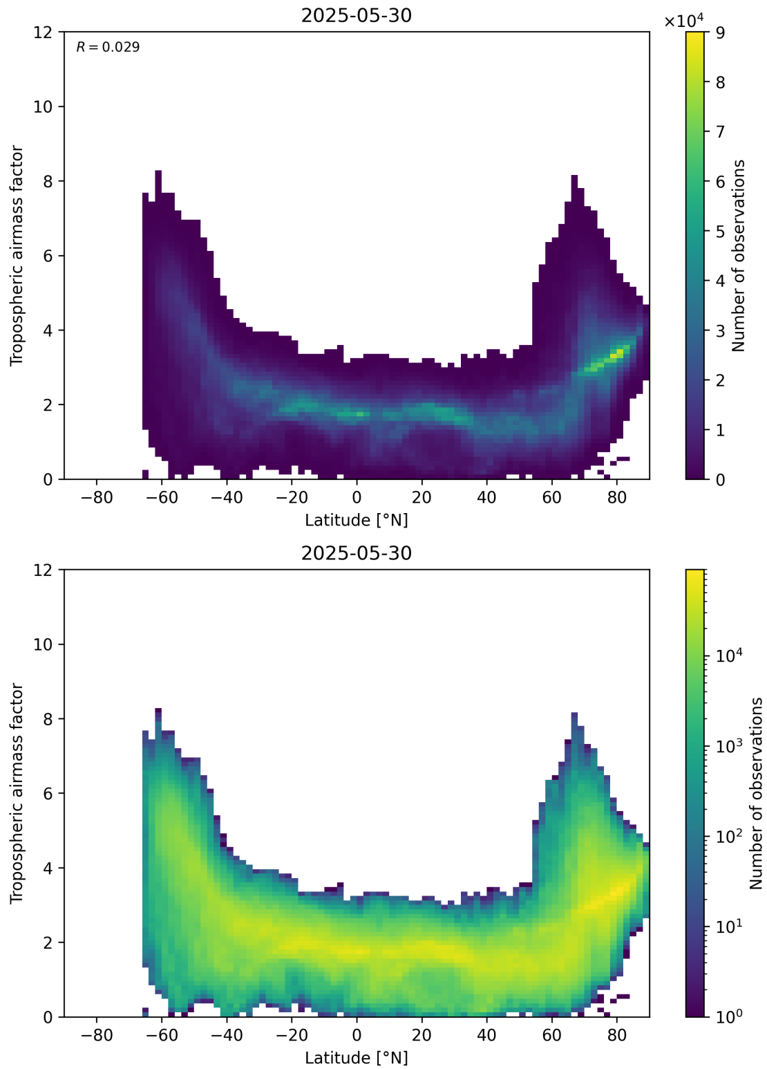
Figure 85: Scatter density plot of “Latitude” against “Tropospheric air mass factor” for 2025-05-29 to 2025-05-31.
