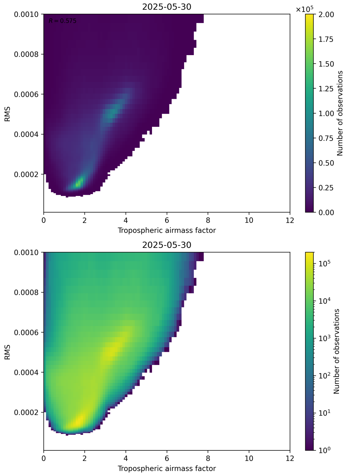
Figure 79: Scatter density plot of “Tropospheric airmass factor” against “RMS” for 2025-05-29 to 2025-05-31.
