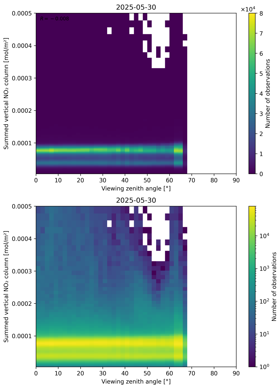
Figure 165: Scatter density plot of “Viewing zenith angle” against “Summed vertical NO 2 column” for 2025-05-29 to 2025-05-31.
