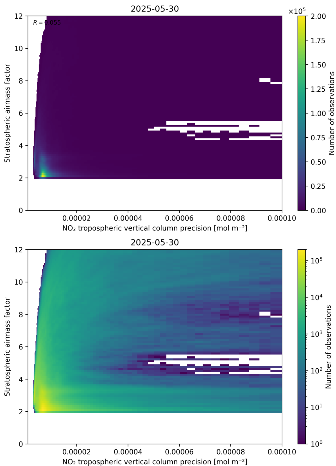
Figure 131: Scatter density plot of “NO 2 tropospheric vertical column precision” against “Stratospheric airmass factor” for 2025-05-29 to 2025-05-31.
