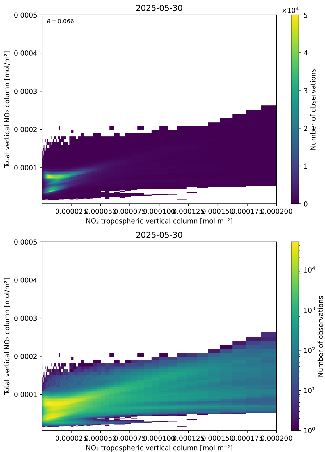
Figure 128: Scatter density plot of “NO 2 tropospheric vertical column” against “Total vertical NO 2 column” for 2025-05-29 to 2025-05-31.
