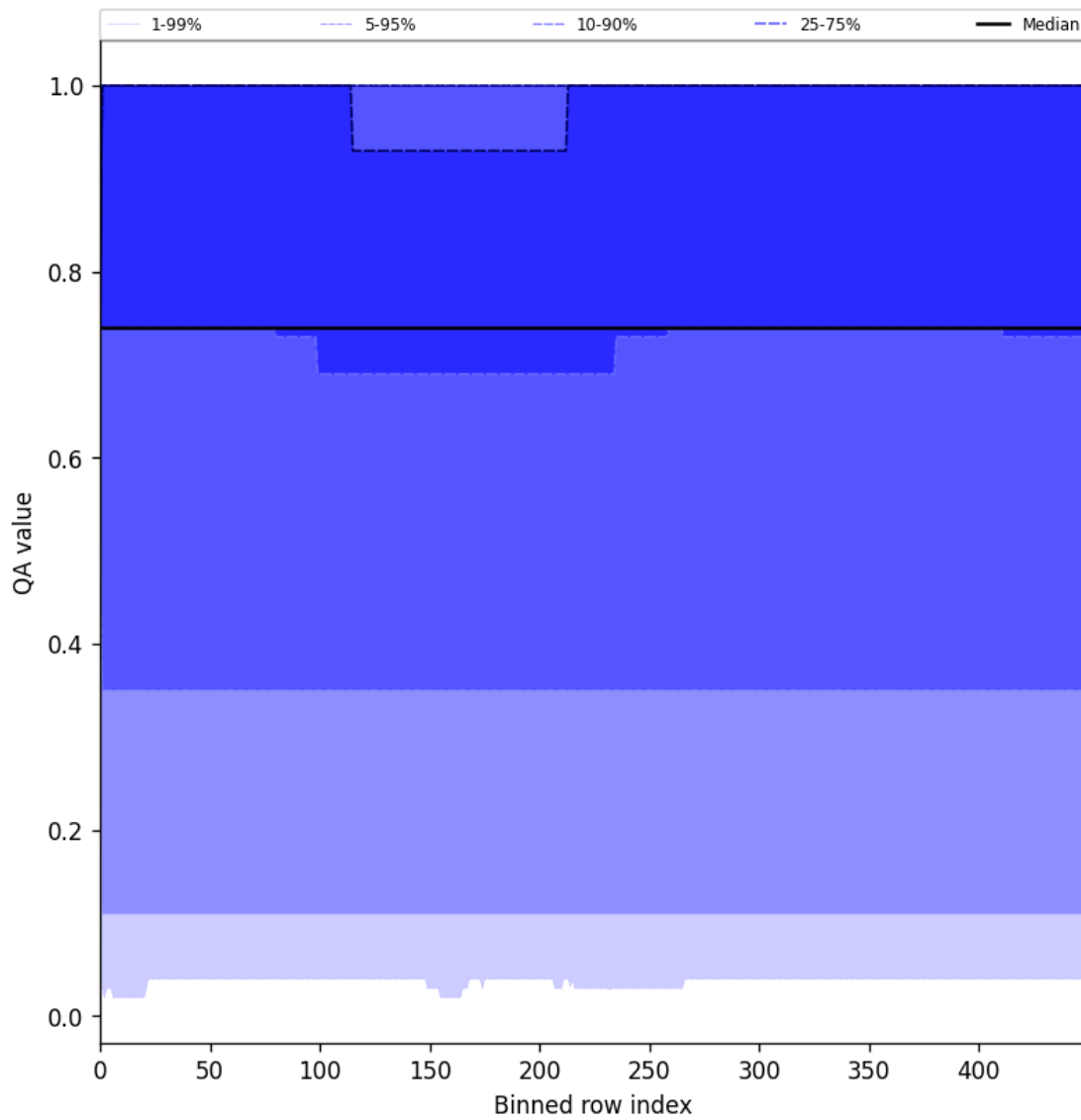
Figure 45: Along track statistics of “QA value” for 2025-05-29 to 2025-05-31
