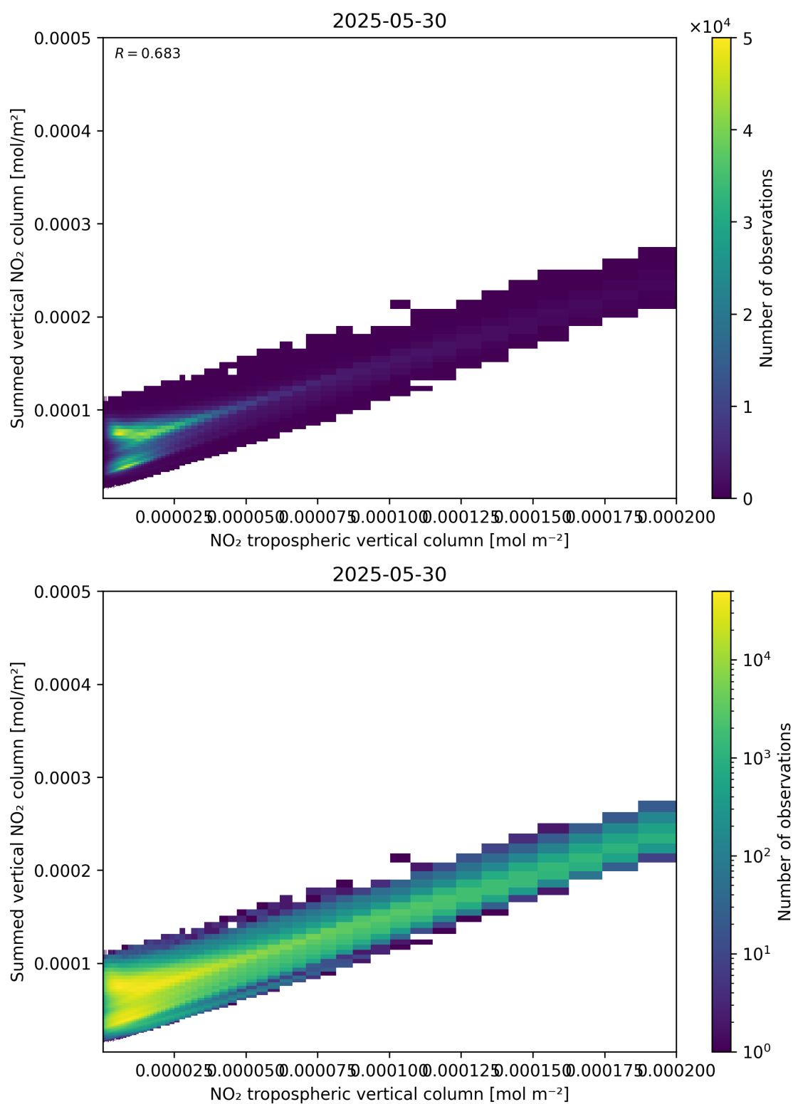
Figure 126: Scatter density plot of “NO 2 tropospheric vertical column” against “Summed vertical NO 2 column” for 2025-05-29 to 2025-05-31.
