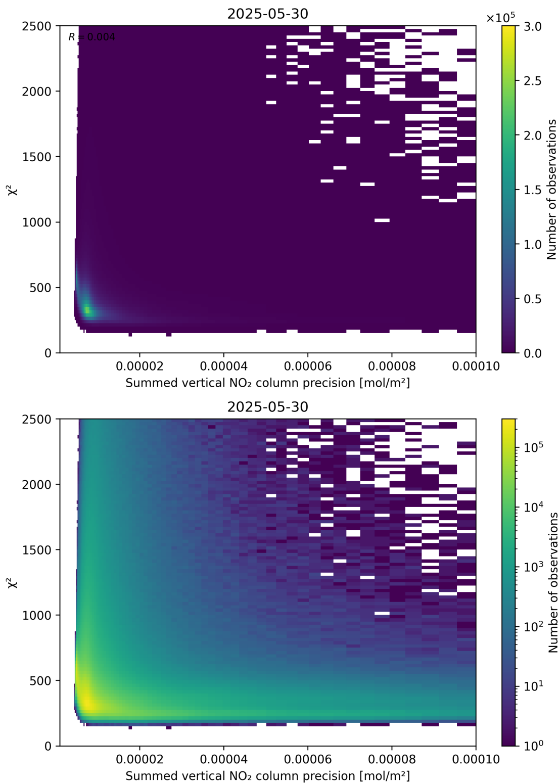
Figure 107: Scatter density plot of “Summed vertical NO 2 column precision” against “ \chi^2 ” for 2025-05-29 to 2025-05-31.
