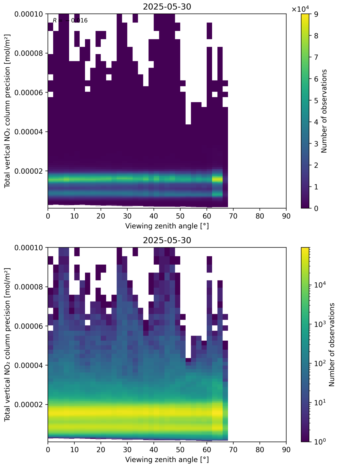
Figure 168: Scatter density plot of “Viewing zenith angle” against “Total vertical NO 2 column precision” for 2025-05-29 to 2025-05-31.
