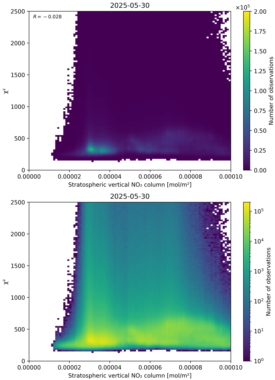
Figure 97: Scatter density plot of “Stratospheric vertical NO 2 column” against “ \chi^2 ” for 2025-05-29 to 2025-05-31.
