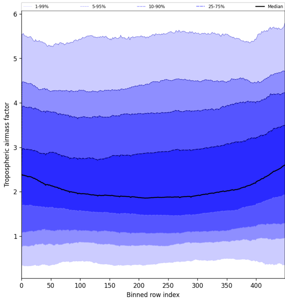
Figure 48: Along track statistics of “Tropospheric air mass factor” for 2025-05-29 to 2025-05-31
