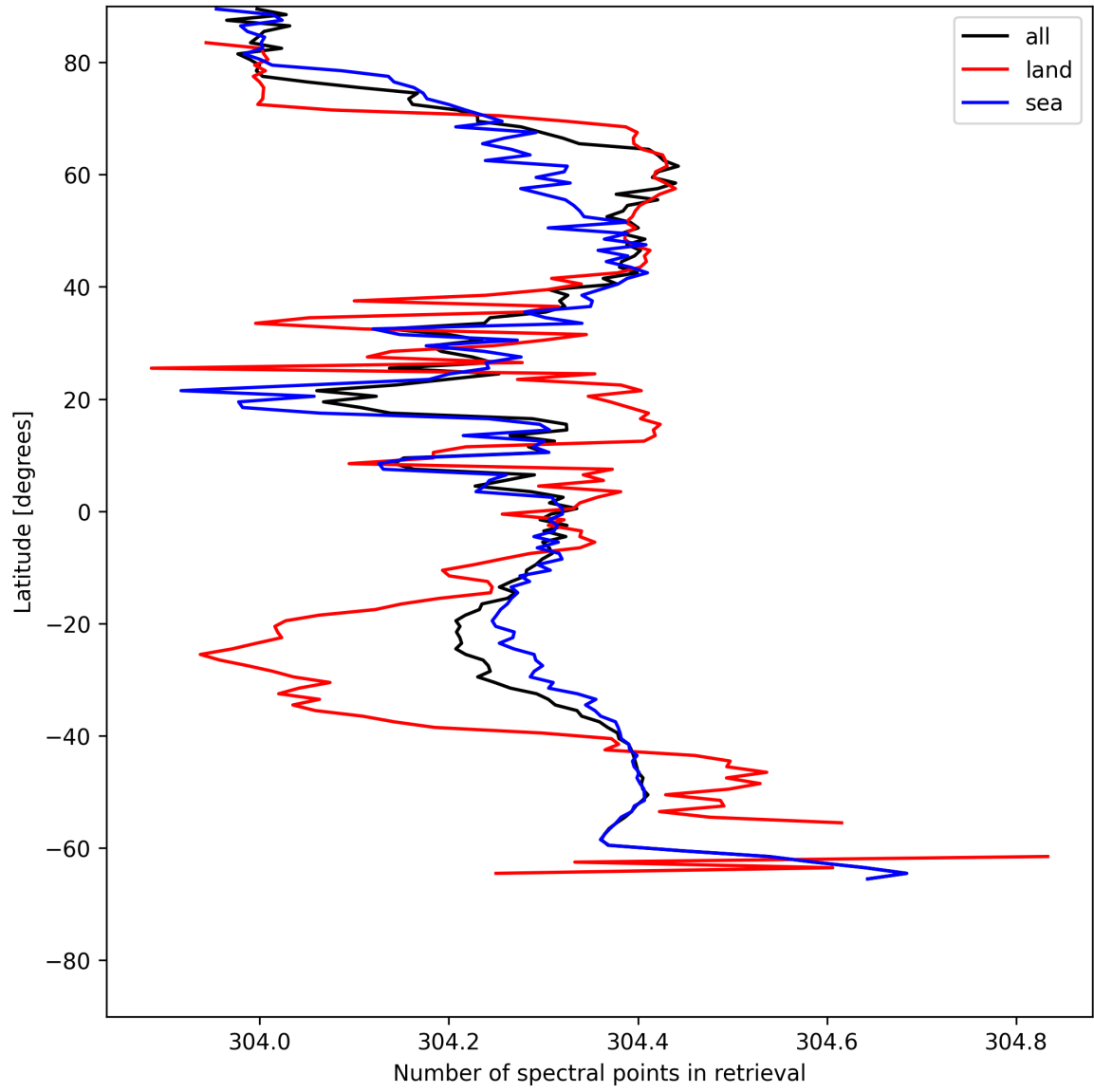
Figure 16: Zonal average of “Number of spectral points in retrieval” for 2025-05-29 to 2025-05-31.
