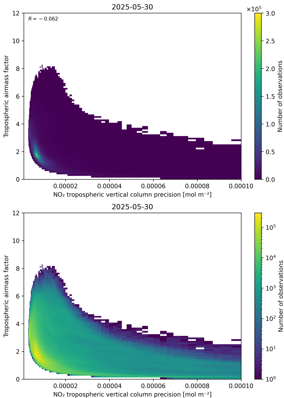
Figure 133: Scatter density plot of “NO 2 tropospheric vertical column precision” against “Tropospheric airmass factor” for 2025-05-29 to 2025-05-31.
