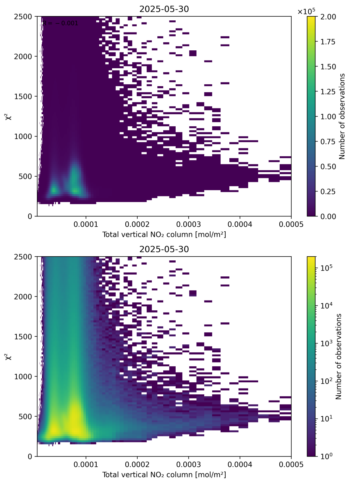
Figure 111: Scatter density plot of “Total vertical NO 2 column” against “ \chi^2 ” for 2025-05-29 to 2025-05-31.
