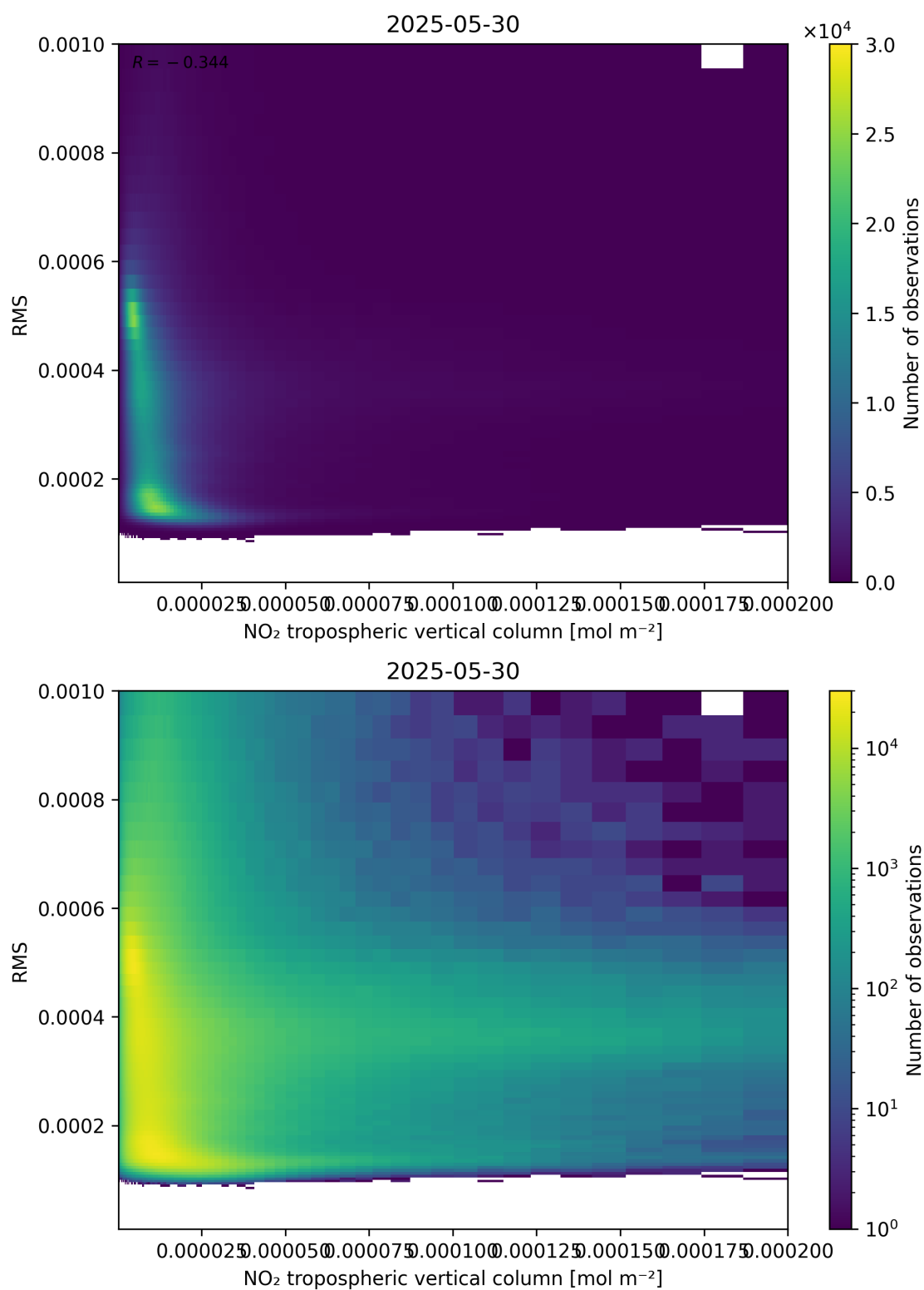
Figure 142: Scatter density plot of “NO 2 tropospheric vertical column” against “RMS” for 2025-05-29 to 2025-05-31.
