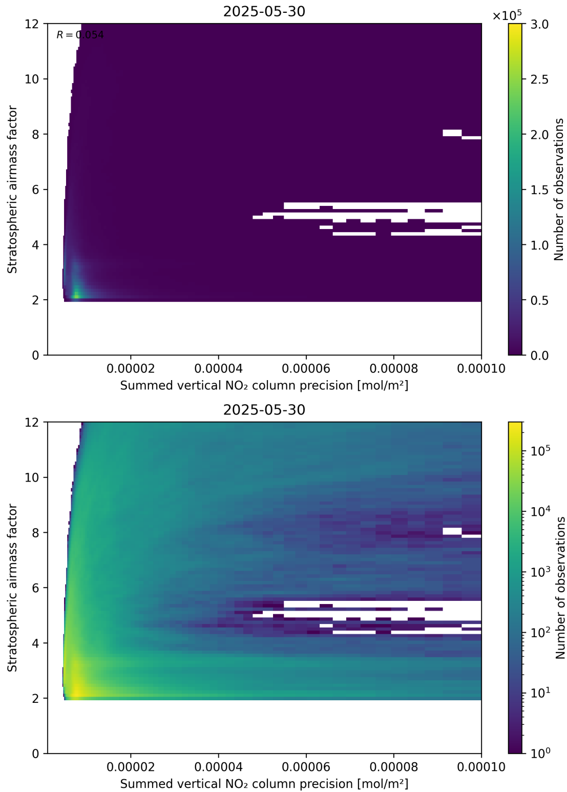
Figure 106: Scatter density plot of “Summed vertical NO 2 column precision” against “Stratospheric airmass factor” for 2025-05-29 to 2025-05-31.
