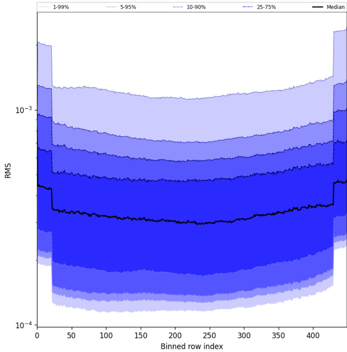
Figure 60: Along track statistics of “RMS” for 2025-05-29 to 2025-05-31
