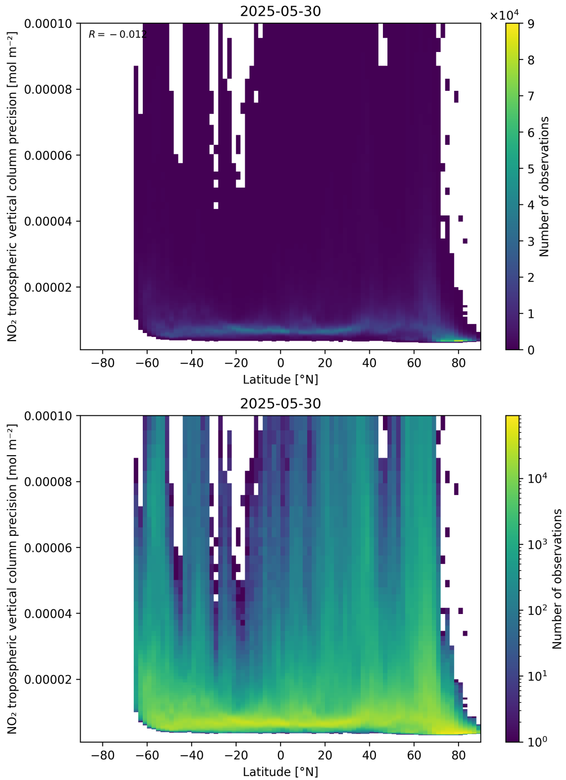
Figure 93: Scatter density plot of “Latitude” against “NO 2 tropospheric vertical column precision” for 2025-05-29 to 2025-05-31.
