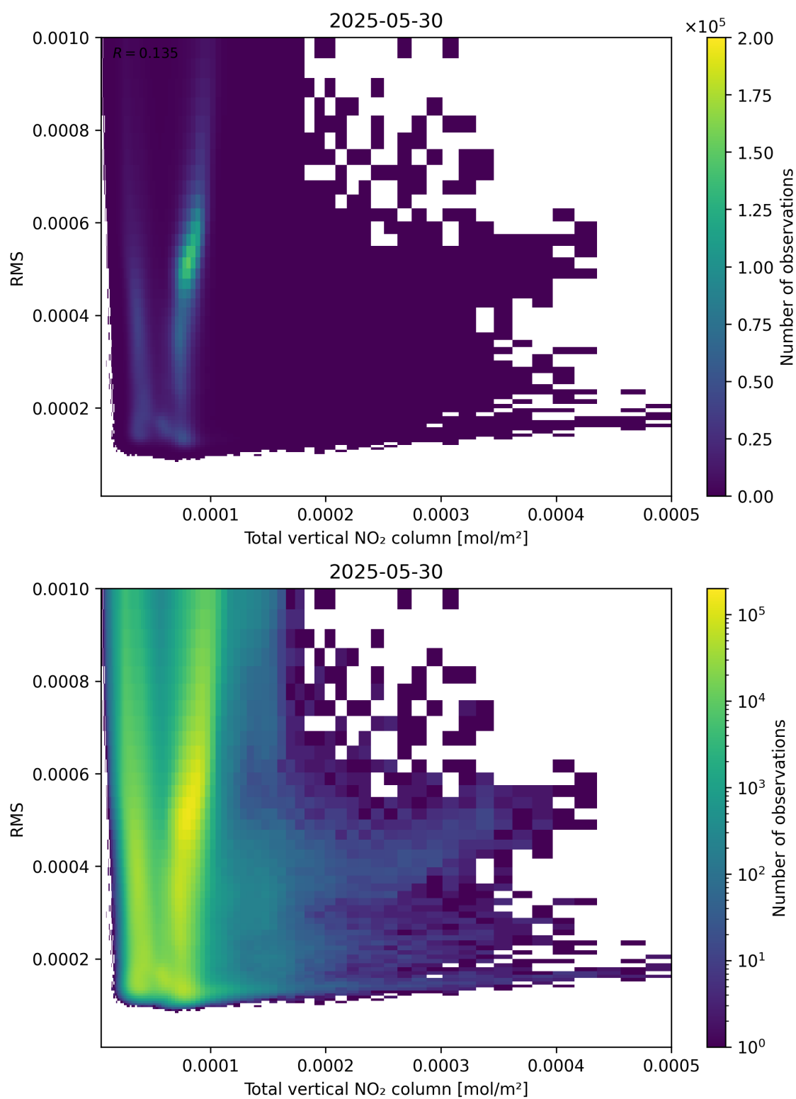
Figure 120: Scatter density plot of “Total vertical NO 2 column” against “RMS” for 2025-05-29 to 2025-05-31.
