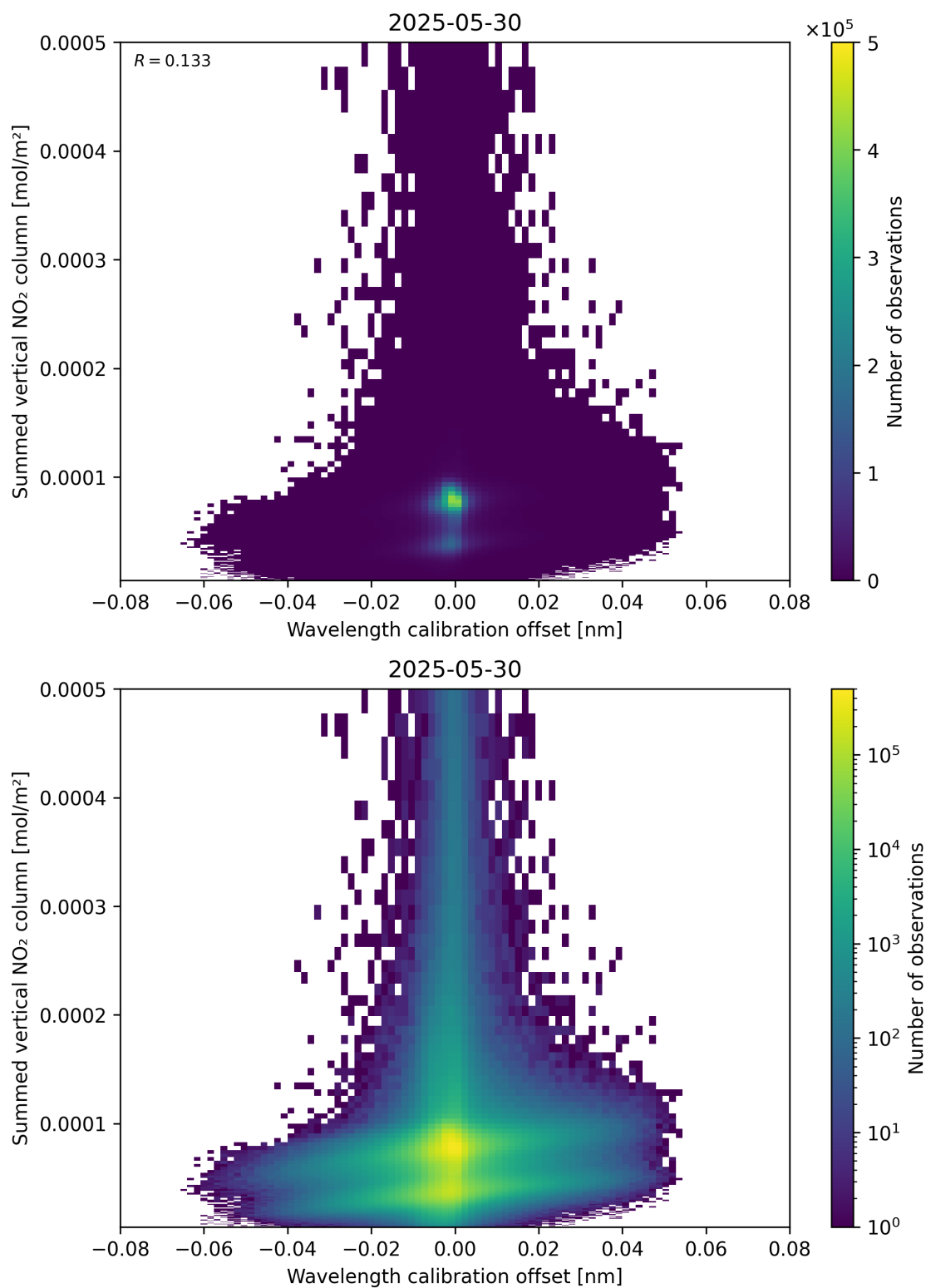
Figure 177: Scatter density plot of “Wavelength calibration offset” against “Summed vertical NO 2 column” for 2025-05-29 to 2025-05-31.
