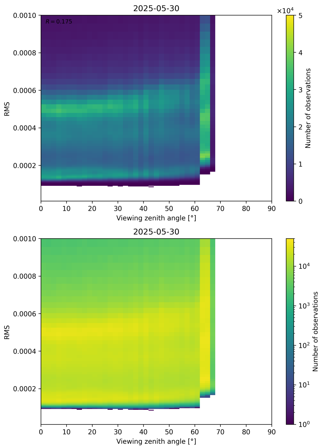
Figure 171: Scatter density plot of “Viewing zenith angle” against “RMS” for 2025-05-29 to 2025-05-31.
