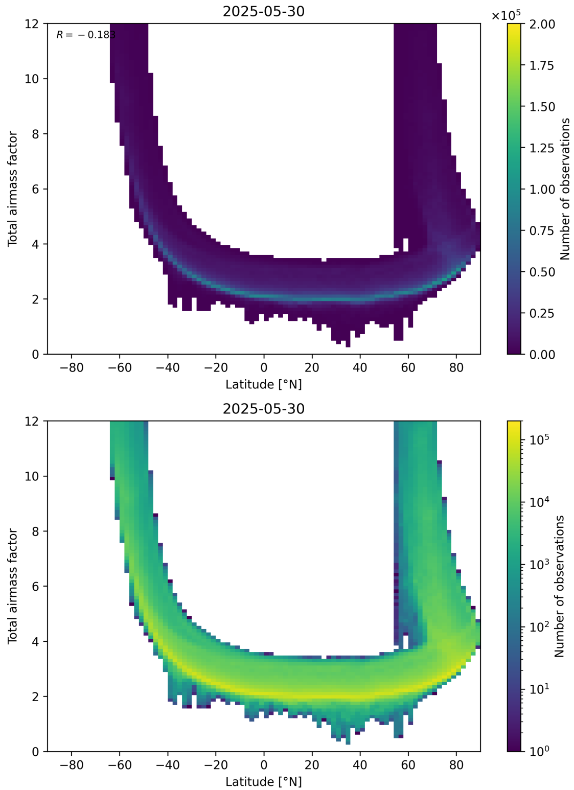
Figure 84: Scatter density plot of “Latitude” against “Total airmass factor” for 2025-05-29 to 2025-05-31.
