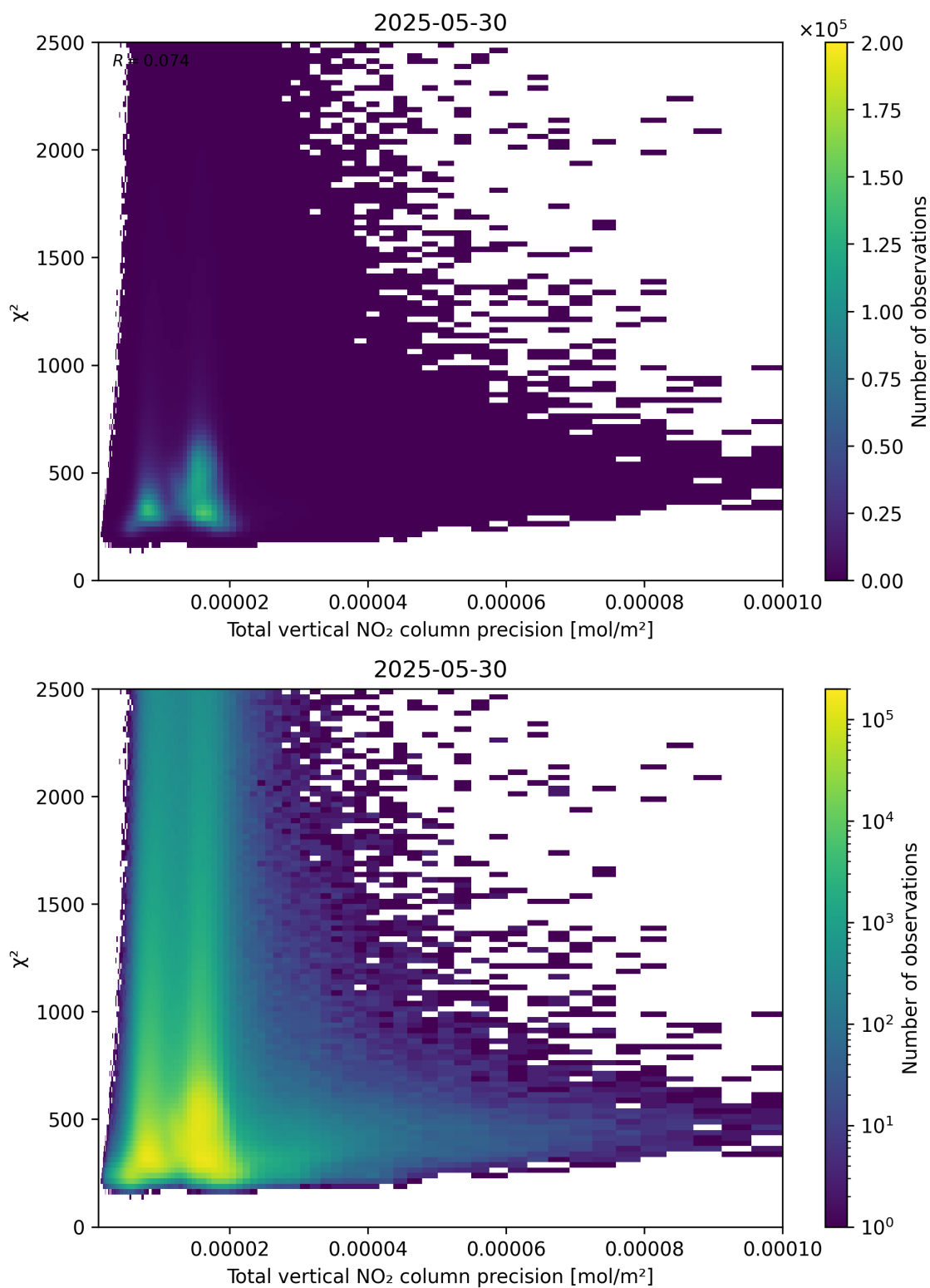
Figure 116: Scatter density plot of “Total vertical NO 2 column precision” against “ \chi^2 ” for 2025-05-29 to 2025-05-31.
