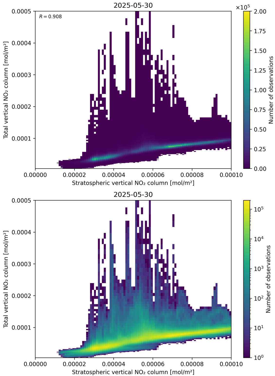
Figure 100: Scatter density plot of “Stratospheric vertical NO 2 column” against “Total vertical NO 2 column” for 2025-05-29 to 2025-05-31.
