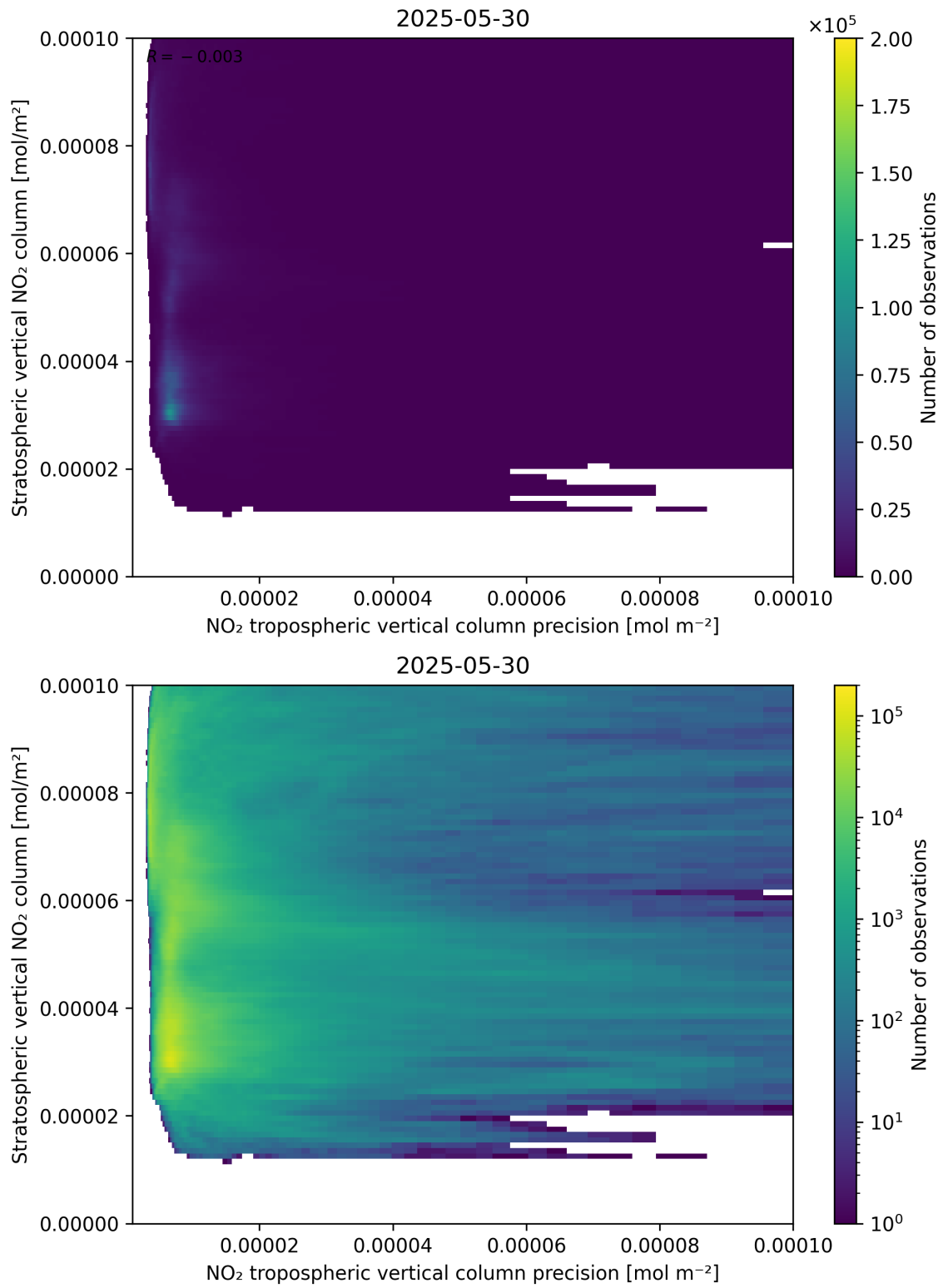
Figure 135: Scatter density plot of “NO 2 tropospheric vertical column precision” against “Stratospheric vertical NO 2 column” for 2025-05-29 to 2025-05-31.
