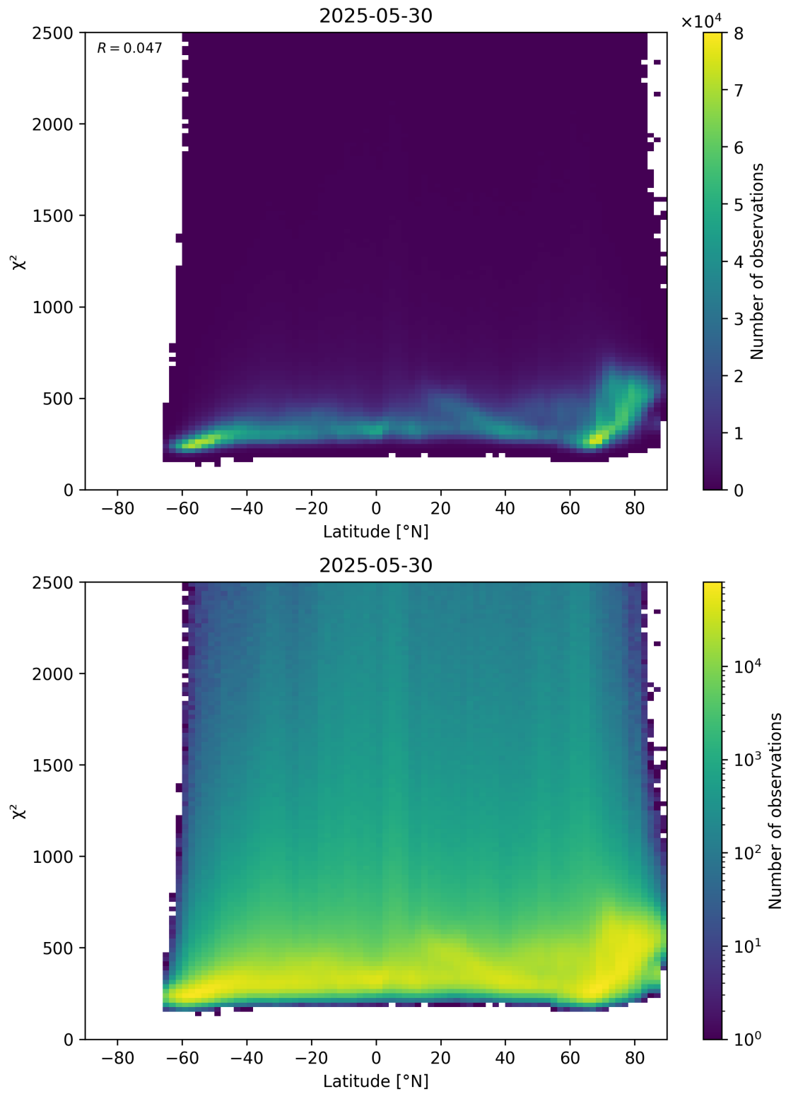
Figure 86: Scatter density plot of “Latitude” against “ \chi^2 ” for 2025-05-29 to 2025-05-31.
