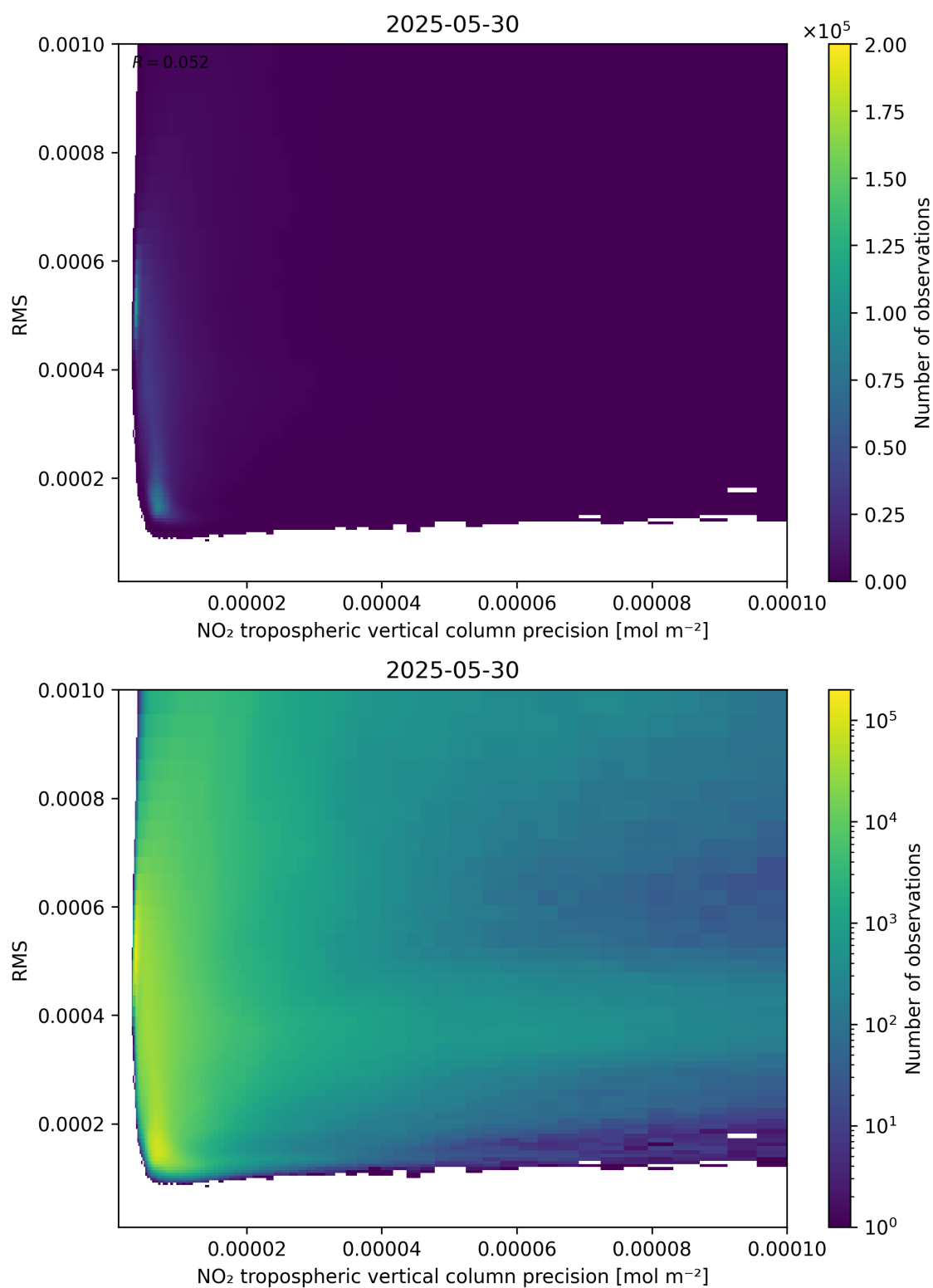
Figure 140: Scatter density plot of “NO 2 tropospheric vertical column precision” against “RMS” for 2025-05-29 to 2025-05-31.
