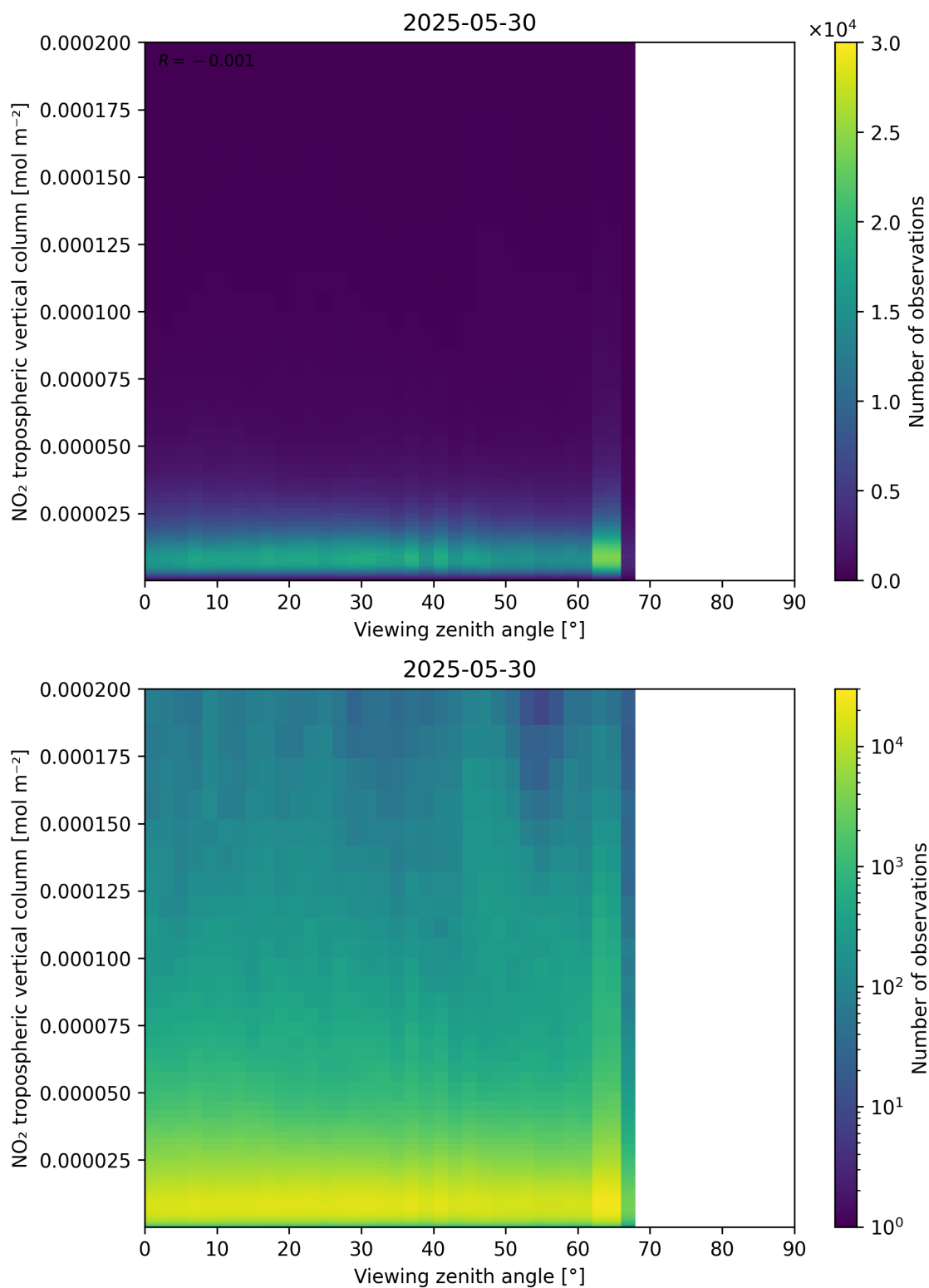
Figure 169: Scatter density plot of “Viewing zenith angle” against “NO 2 tropospheric vertical column” for 2025-05-29 to 2025-05-31.
