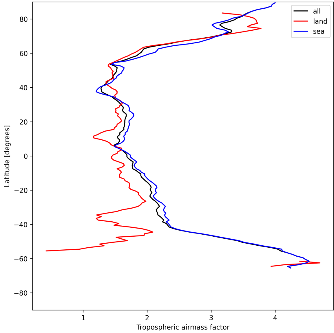
Figure 14: Zonal average of “Tropospheric airmass factor” for 2025-05-29 to 2025-05-31.
