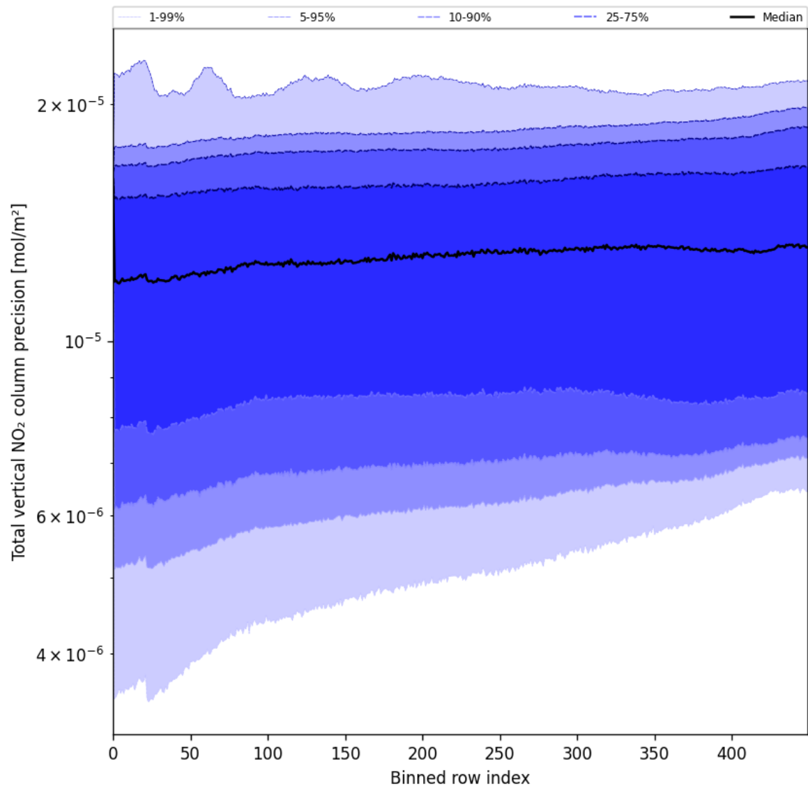
Figure 56: Along track statistics of “Total vertical NO 2 column precision” for 2025-05-29 to 2025-05-31
