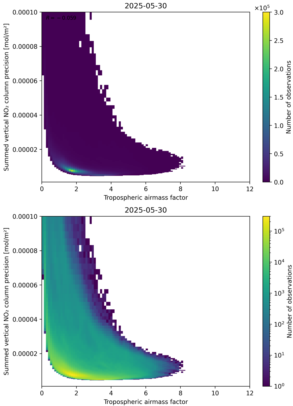
Figure 76: Scatter density plot of “Tropospheric air mass factor” against “Summed vertical NO 2 column precision” for 2025-05-29 to 2025-05-31.
