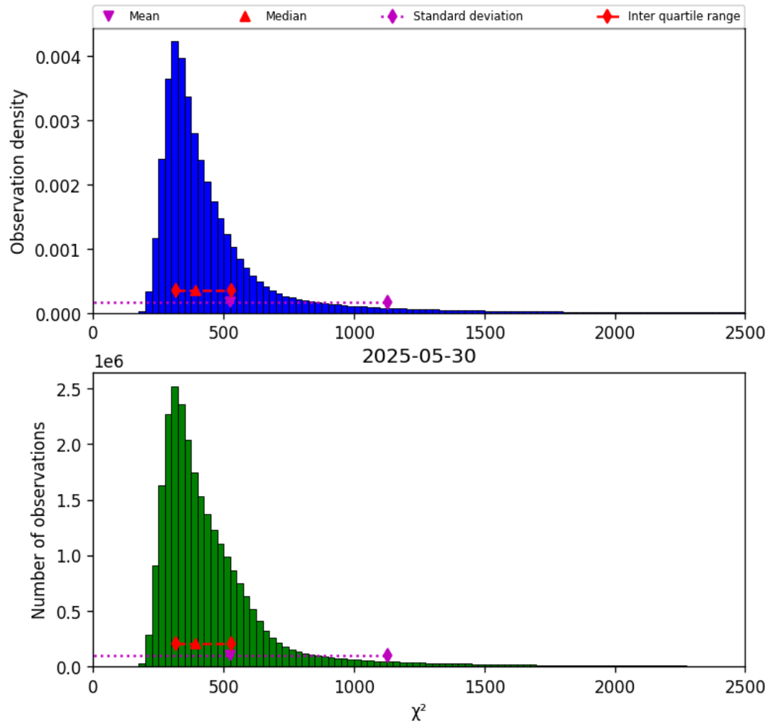
Figure 42: Histogram of " \chi^2 " for 2025-05-29 to 2025-05-31
