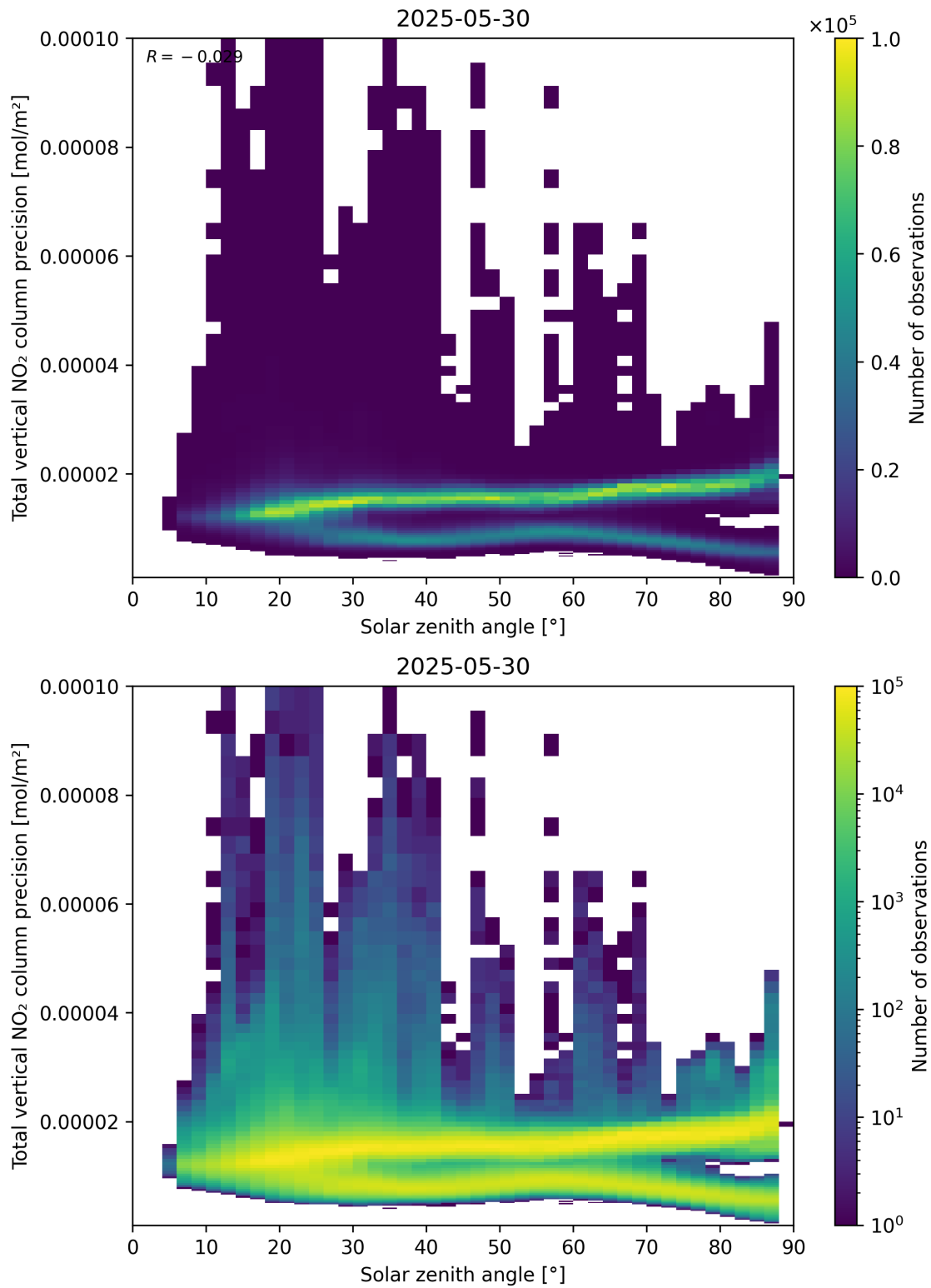
Figure 154: Scatter density plot of “Solar zenith angle” against “Total vertical NO 2 column precision” for 2025-05-29 to 2025-05-31.
