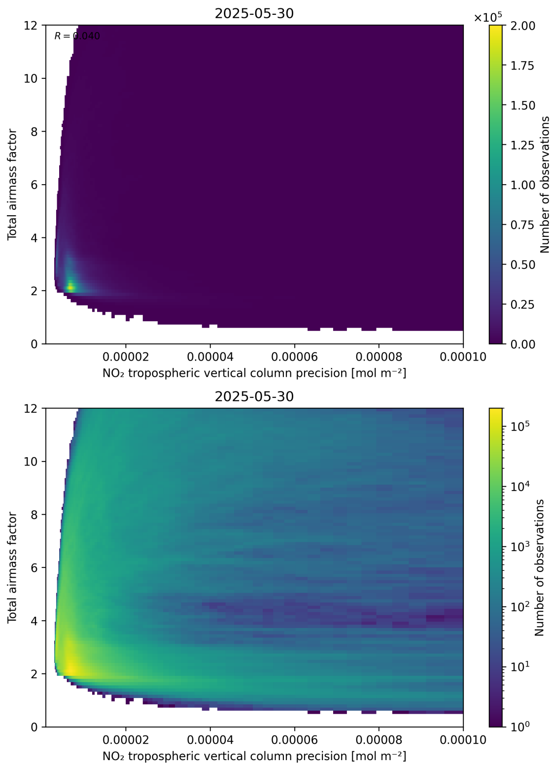
Figure 132: Scatter density plot of “NO 2 tropospheric vertical column precision” against “Total air mass factor” for 2025-05-29 to 2025-05-31.
