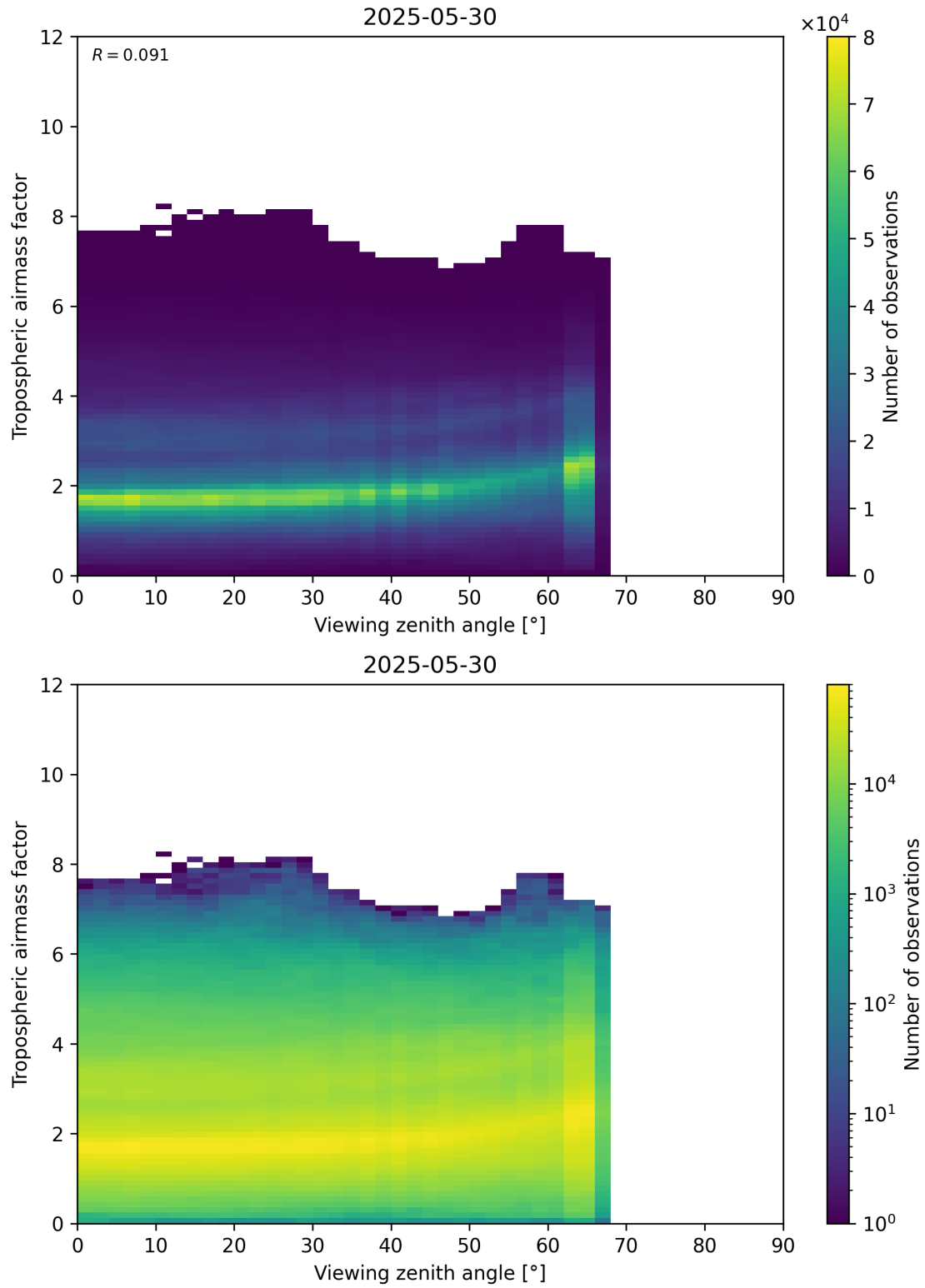
Figure 161: Scatter density plot of “Viewing zenith angle” against “Tropospheric airmass factor” for 2025-05-29 to 2025-05-31.
