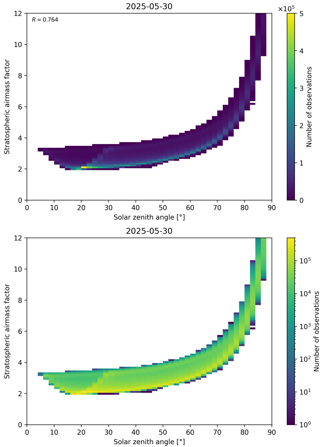
Figure 145: Scatter density plot of “Solar zenith angle” against “Stratospheric airmass factor” for 2025-05-29 to 2025-05-31.
