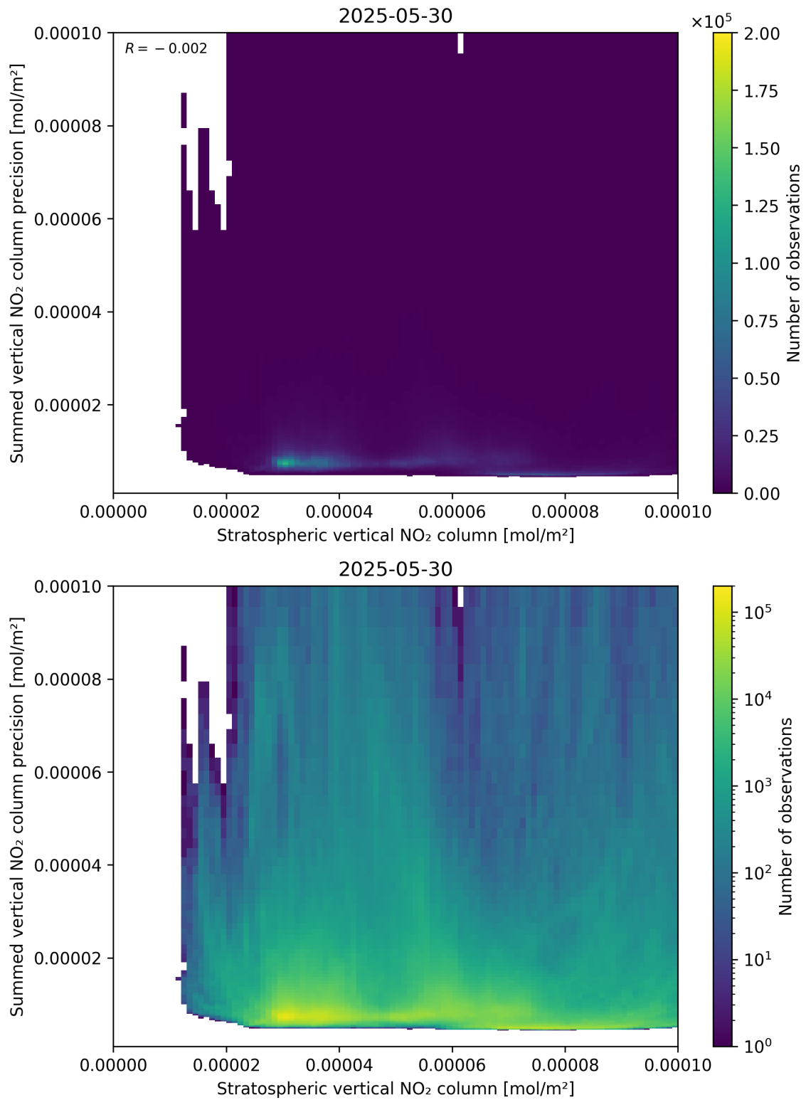
Figure 99: Scatter density plot of “Stratospheric vertical NO 2 column” against “Summed vertical NO 2 column precision” for 2025-05-29 to 2025-05-31.
