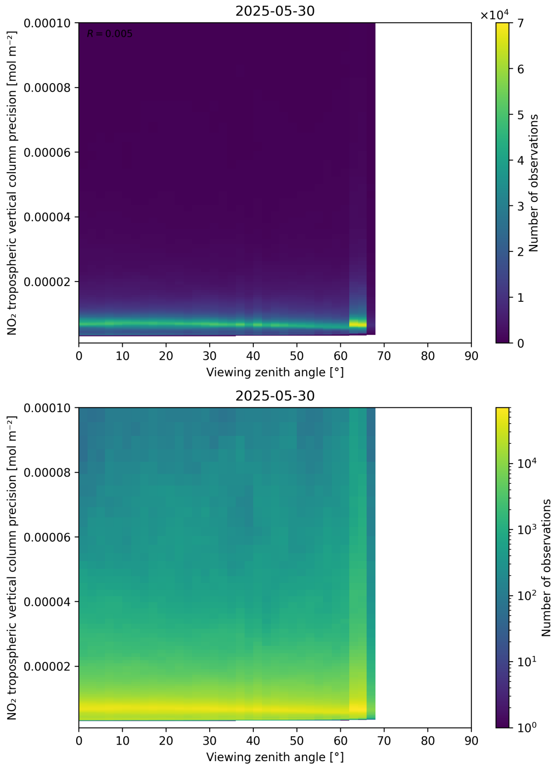
Figure 170: Scatter density plot of “Viewing zenith angle” against “NO 2 tropospheric vertical column precision” for 2025-05-29 to 2025-05-31.
