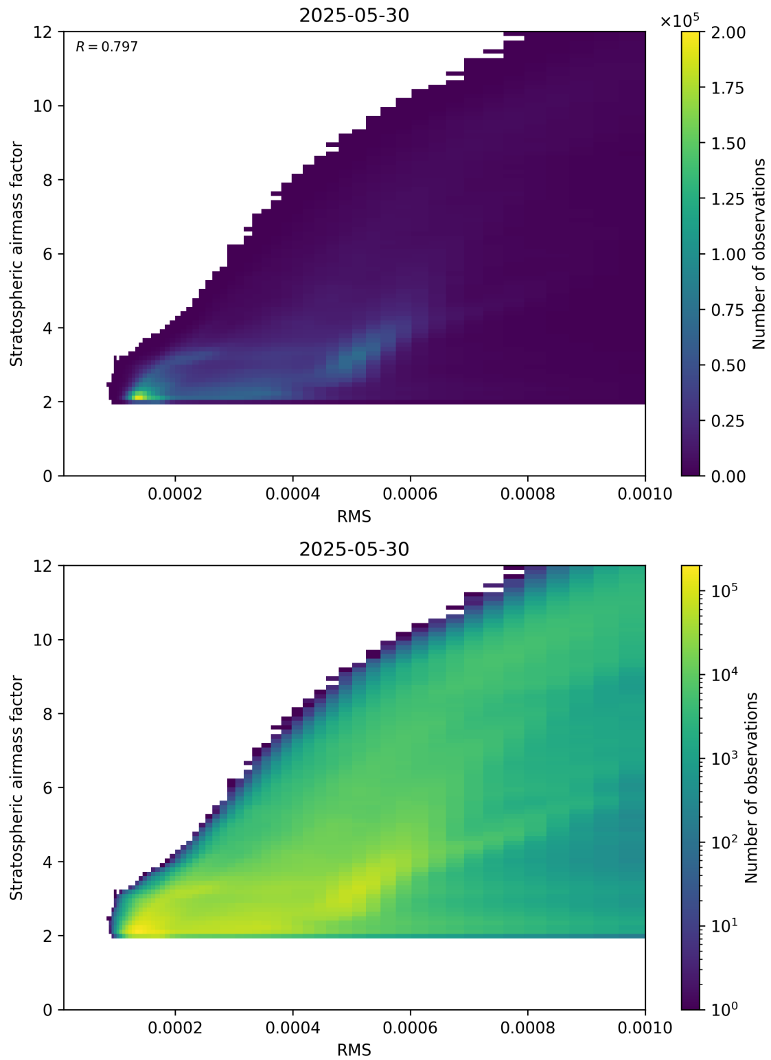
Figure 144: Scatter density plot of “RMS” against “Stratospheric airmass factor” for 2025-05-29 to 2025-05-31.
