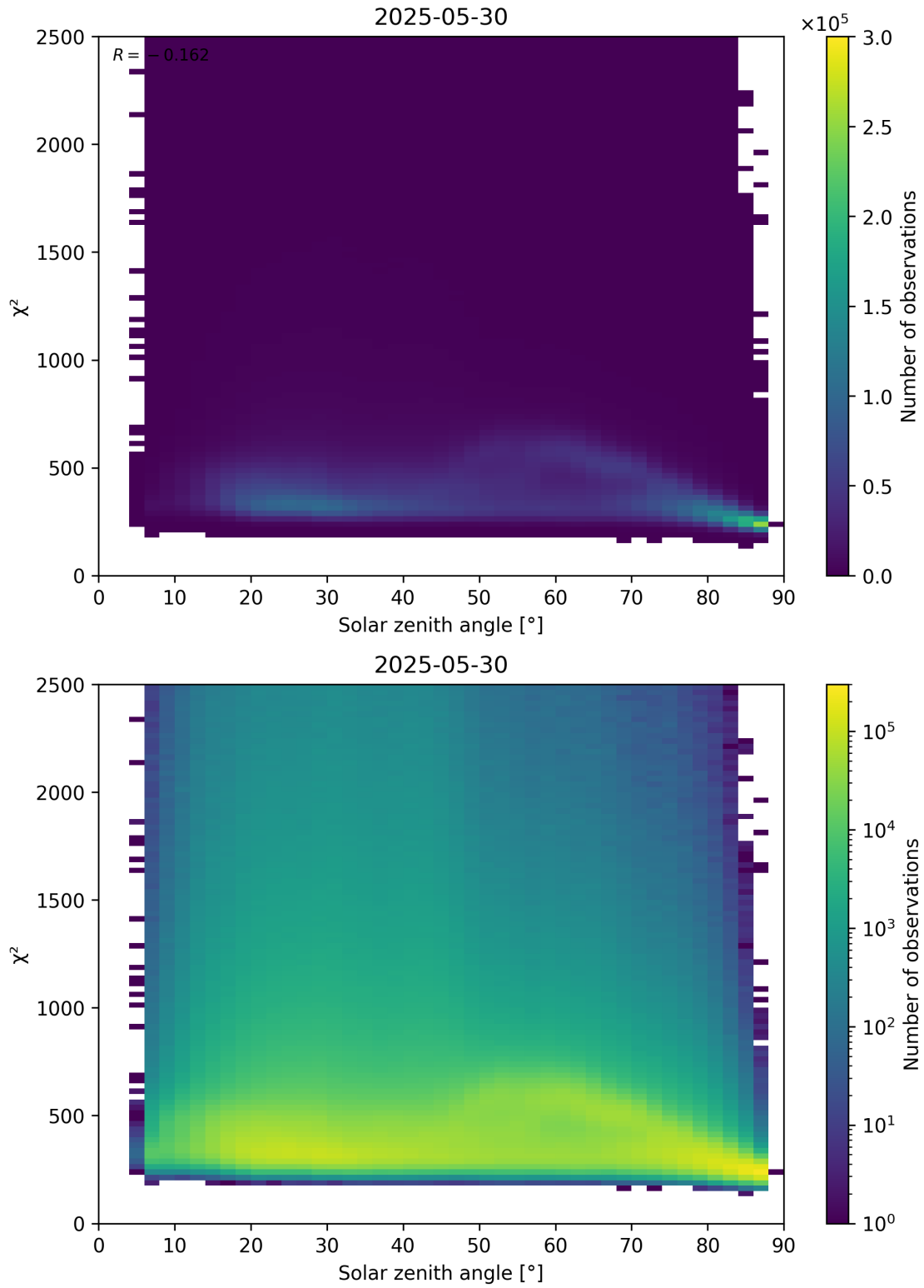
Figure 148: Scatter density plot of “Solar zenith angle” against “ \chi^2 ” for 2025-05-29 to 2025-05-31.
