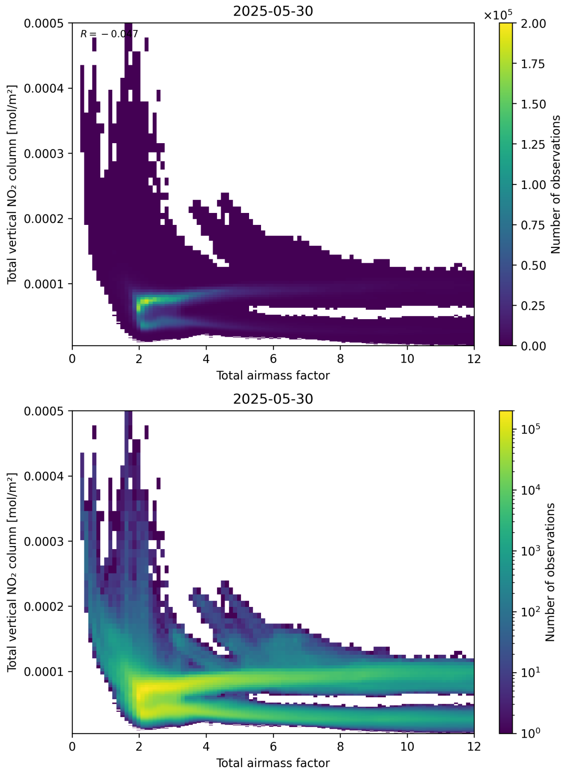
Figure 67: Scatter density plot of “Total airmass factor” against “Total vertical NO 2 column” for 2025-05-29 to 2025-05-31.
