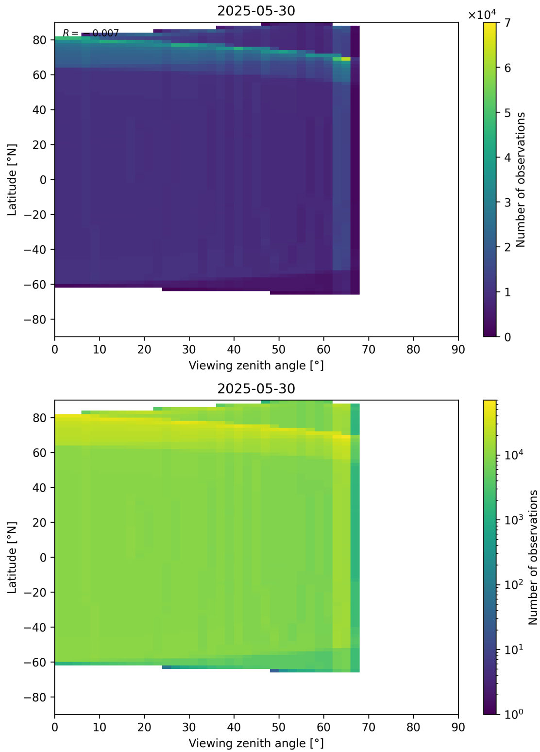
Figure 163: Scatter density plot of “Viewing zenith angle” against “Latitude” for 2025-05-29 to 2025-05-31.
