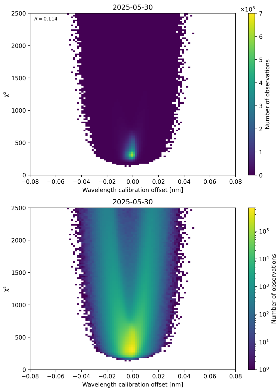
Figure 175: Scatter density plot of “Wavelength calibration offset” against “ \chi^2 ” for 2025-05-29 to 2025-05-31.
