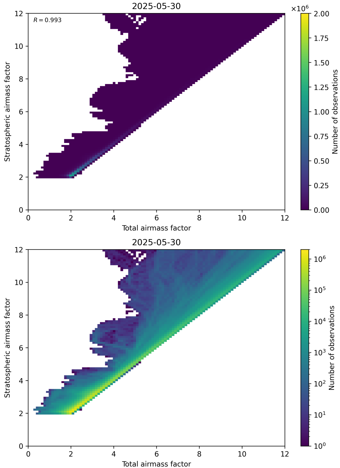
Figure 62: Scatter density plot of “Total airmass factor” against “Stratospheric airmass factor” for 2025-05-29 to 2025-05-31.
