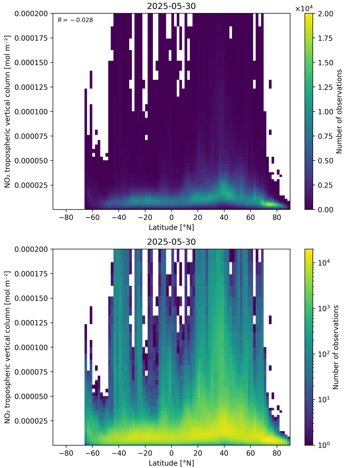
Figure 92: Scatter density plot of “Latitude” against “NO 2 tropospheric vertical column” for 2025-05-29 to 2025-05-31.
