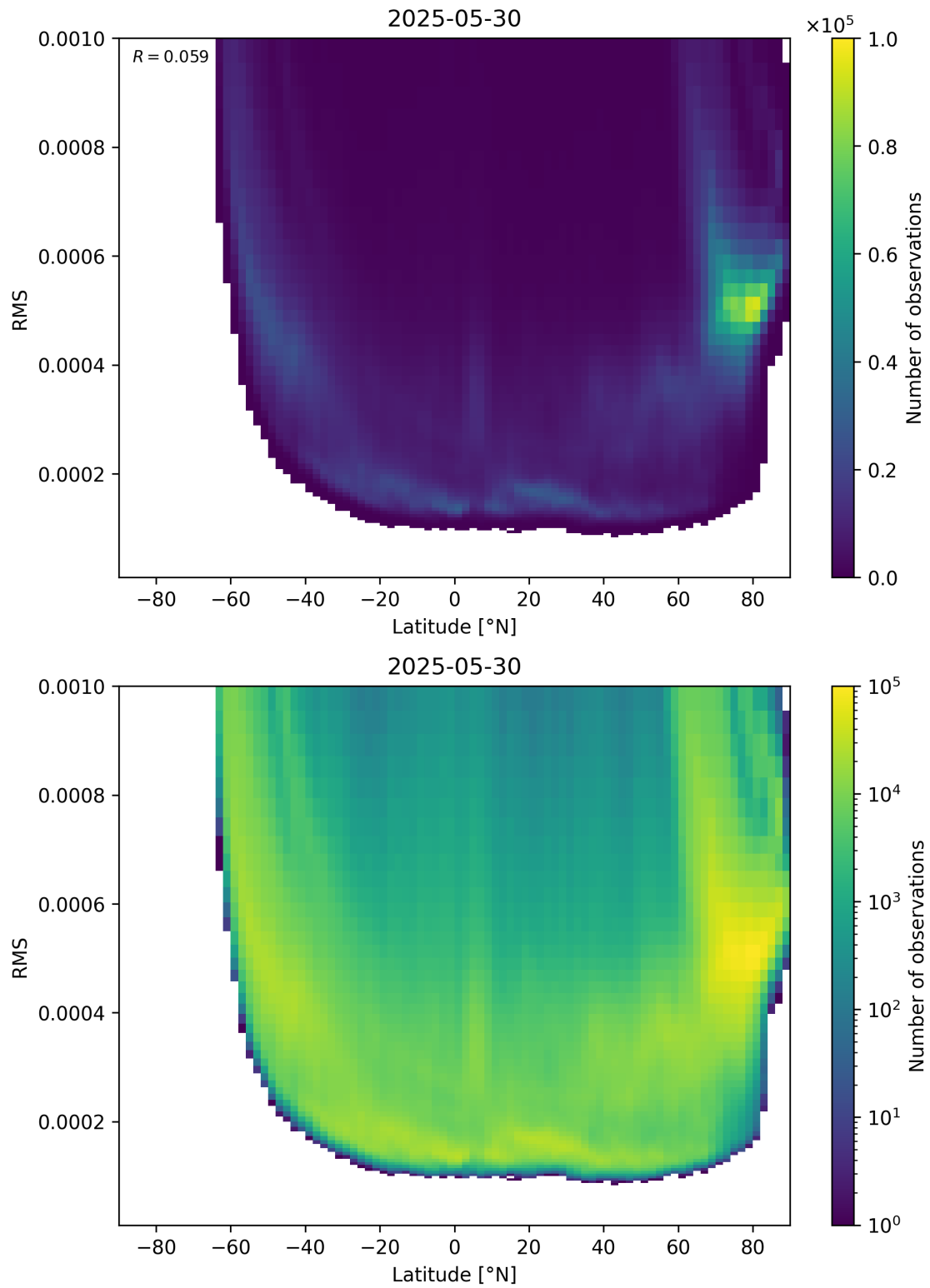
Figure 94: Scatter density plot of “Latitude” against “RMS” for 2025-05-29 to 2025-05-31.
