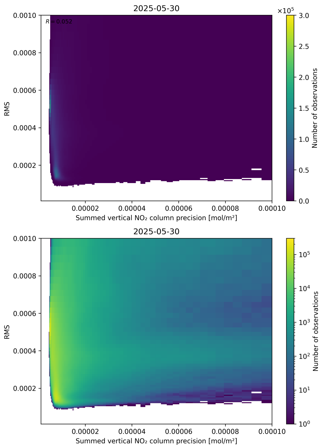
Figure 108: Scatter density plot of “Summed vertical NO 2 column precision” against “RMS” for 2025-05-29 to 2025-05-31.
