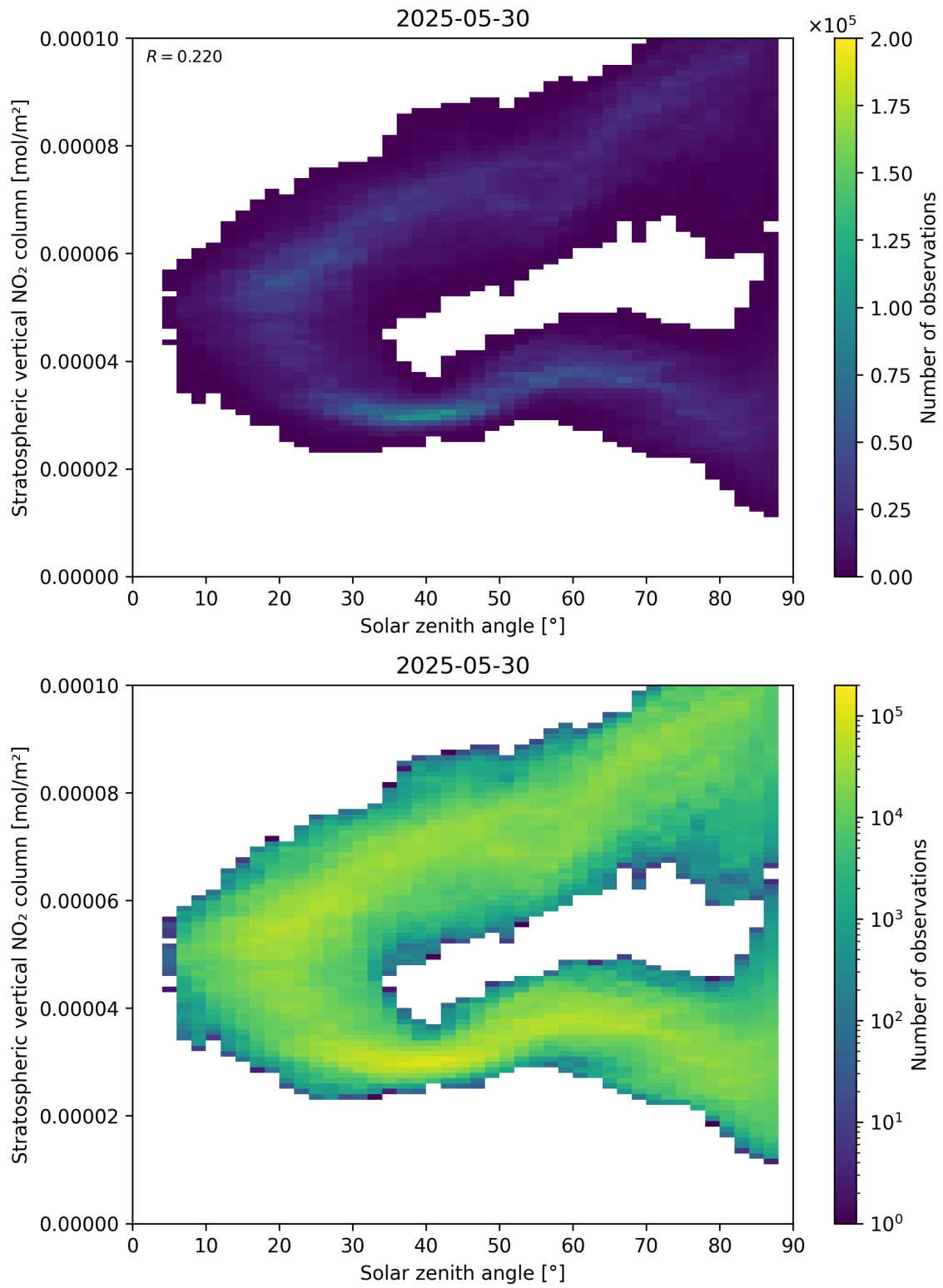
Figure 150: Scatter density plot of “Solar zenith angle” against “Stratospheric vertical NO 2 column” for 2025-05-29 to 2025-05-31.
