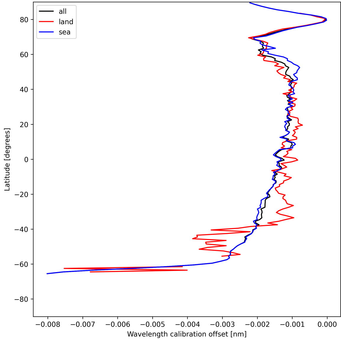
Figure 18: Zonal average of “Wavelength calibration offset” for 2025-05-29 to 2025-05-31.
