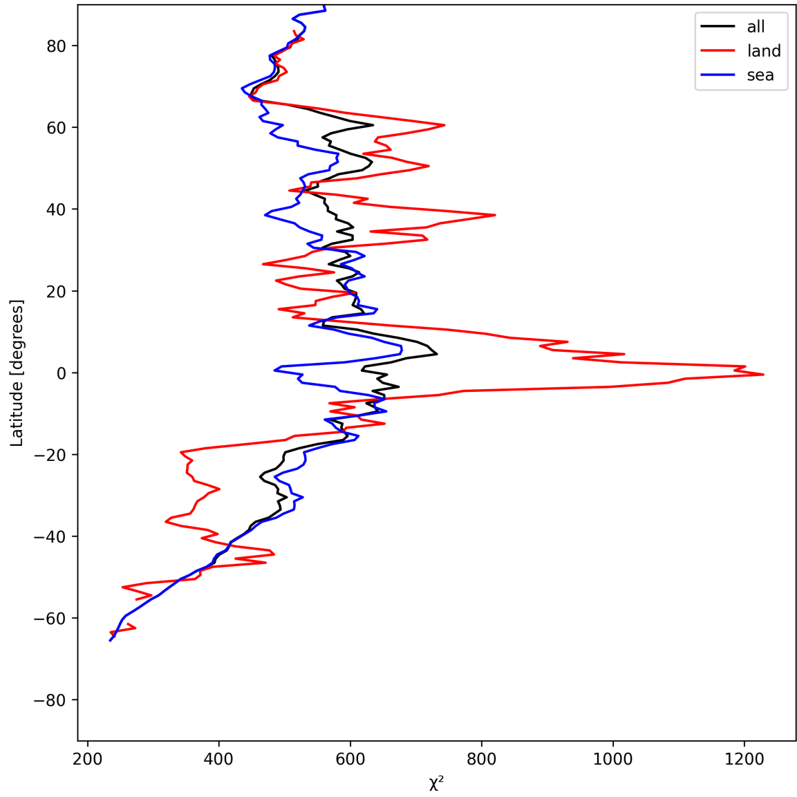
Figure 25: Zonal average of “ \chi^2 ” for 2025-05-29 to 2025-05-31.
