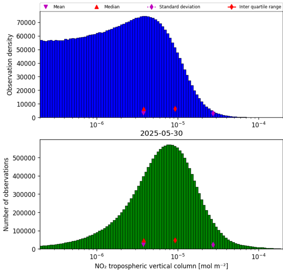
Figure 29: Histogram of “NO 2 tropospheric vertical column” for 2025-05-29 to 2025-05-31
