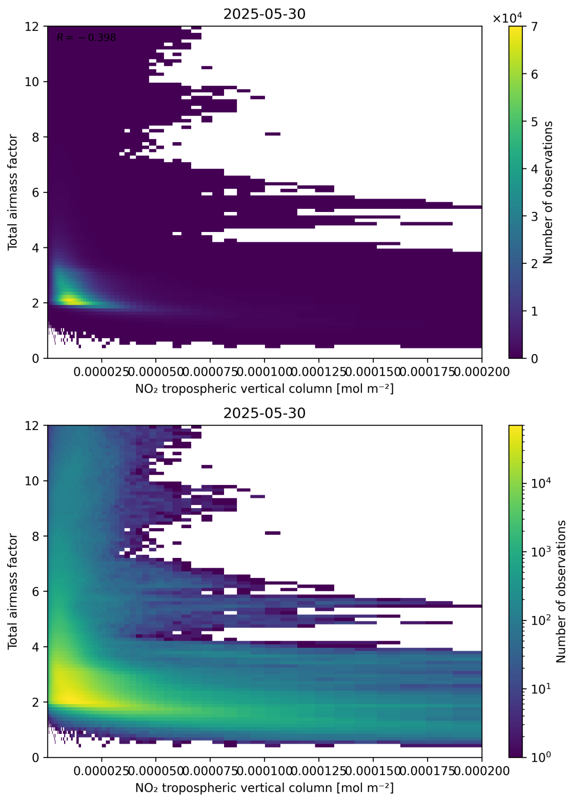
Figure 122: Scatter density plot of “NO 2 tropospheric vertical column” against “Total air mass factor” for 2025-05-29 to 2025-05-31.
