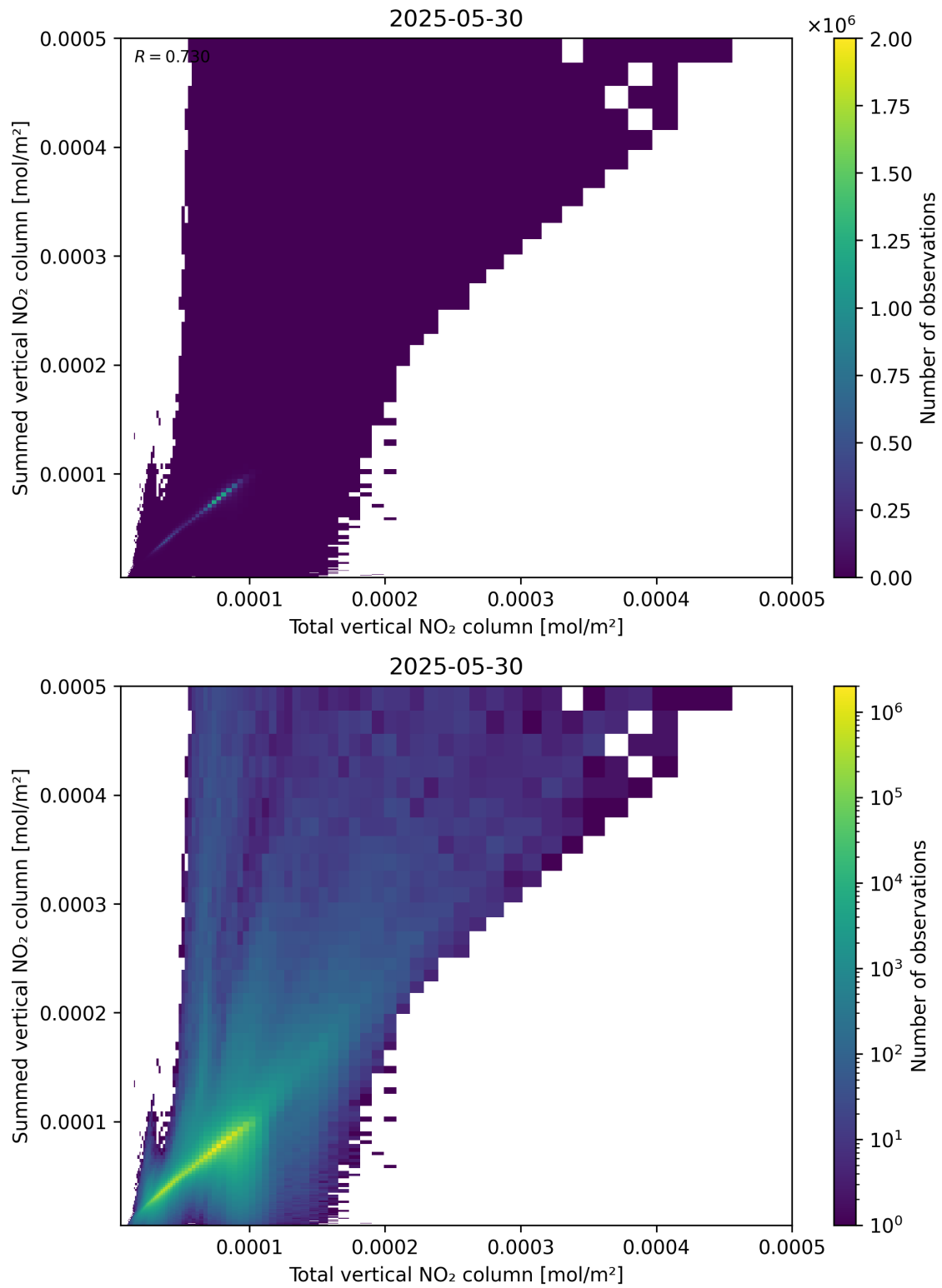
Figure 112: Scatter density plot of “Total vertical NO 2 column” against “Summed vertical NO 2 column” for 2025-05-29 to 2025-05-31.
