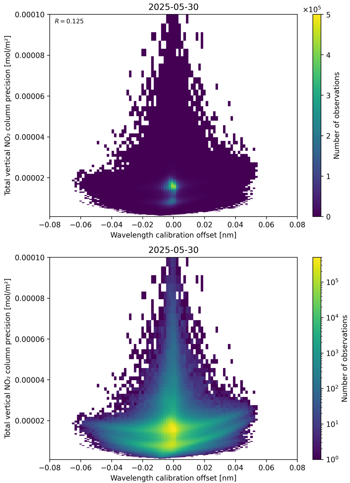
Figure 180: Scatter density plot of “Wavelength calibration offset” against “Total vertical NO 2 column precision” for 2025-05-29 to 2025-05-31.
