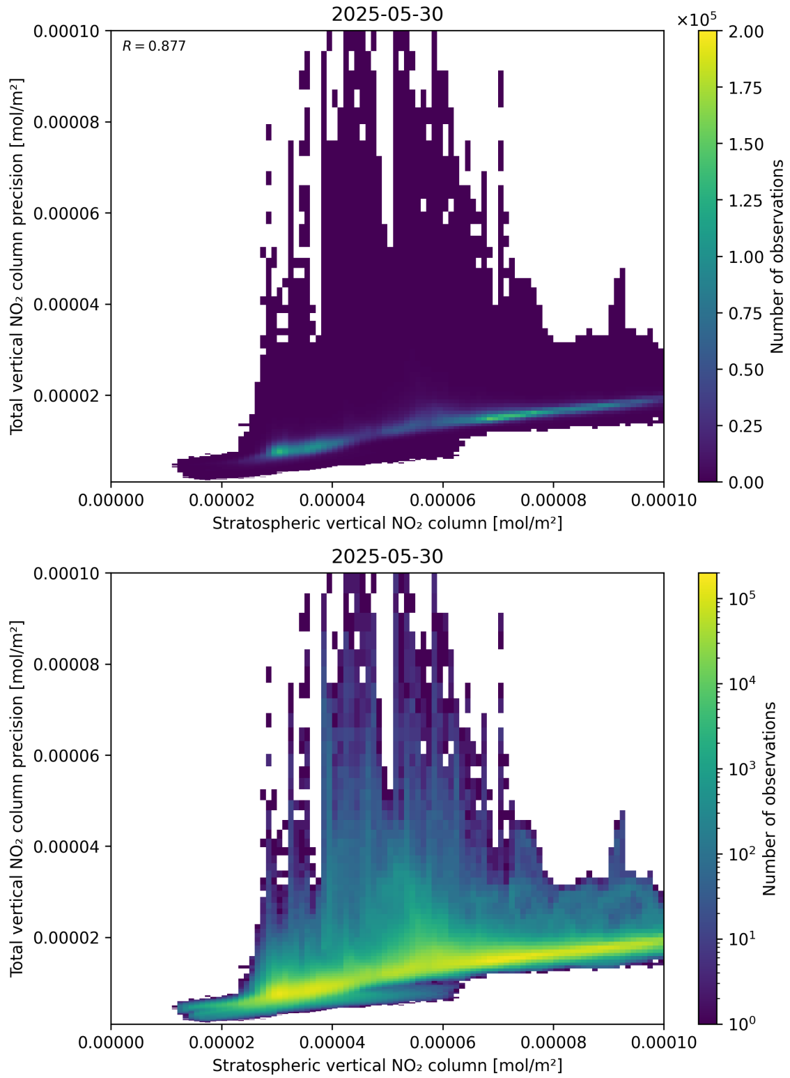
Figure 101: Scatter density plot of “Stratospheric vertical NO 2 column” against “Total vertical NO 2 column precision” for 2025-05-29 to 2025-05-31.
