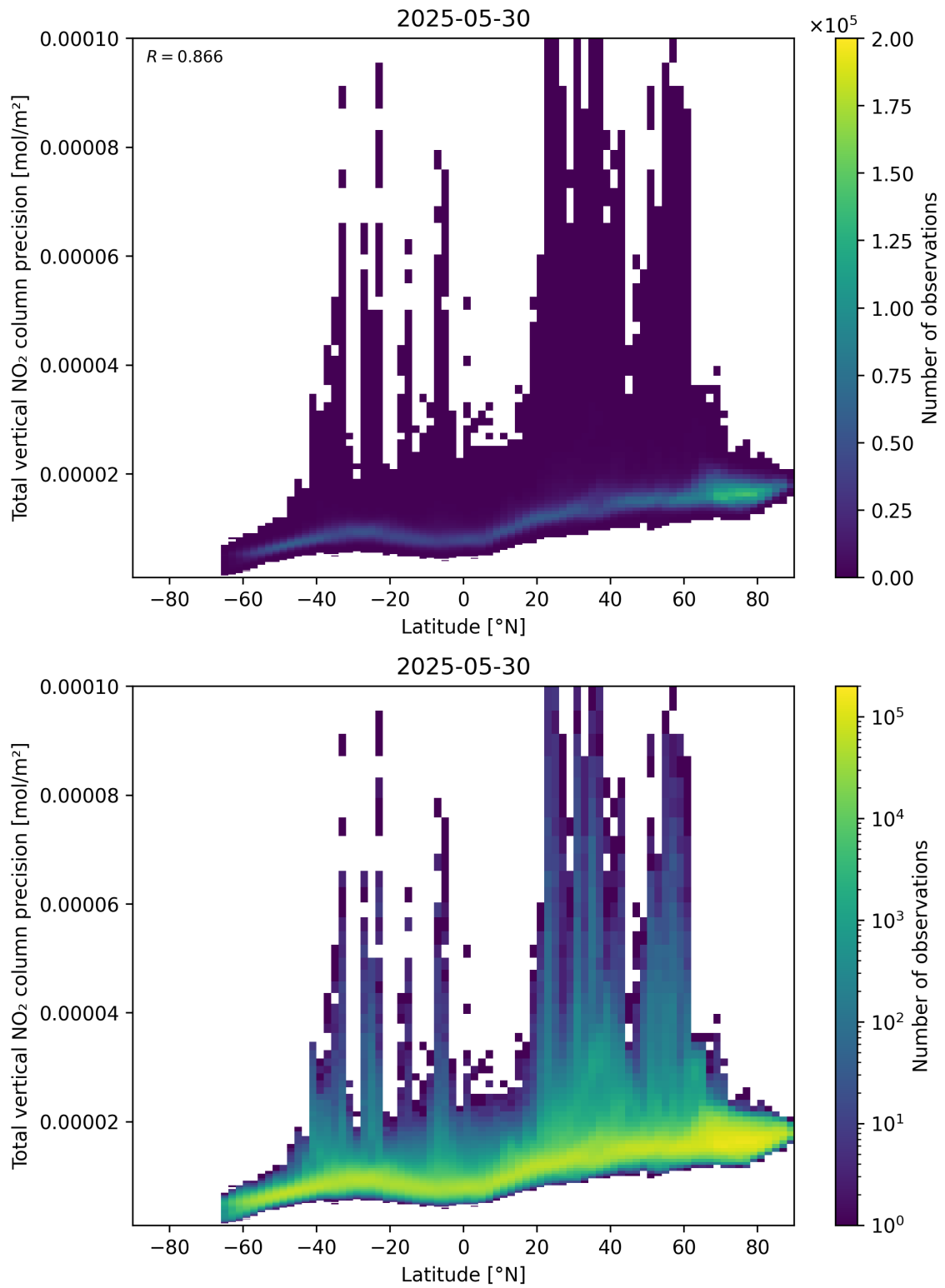
Figure 91: Scatter density plot of “Latitude” against “Total vertical NO 2 column precision” for 2025-05-29 to 2025-05-31.
