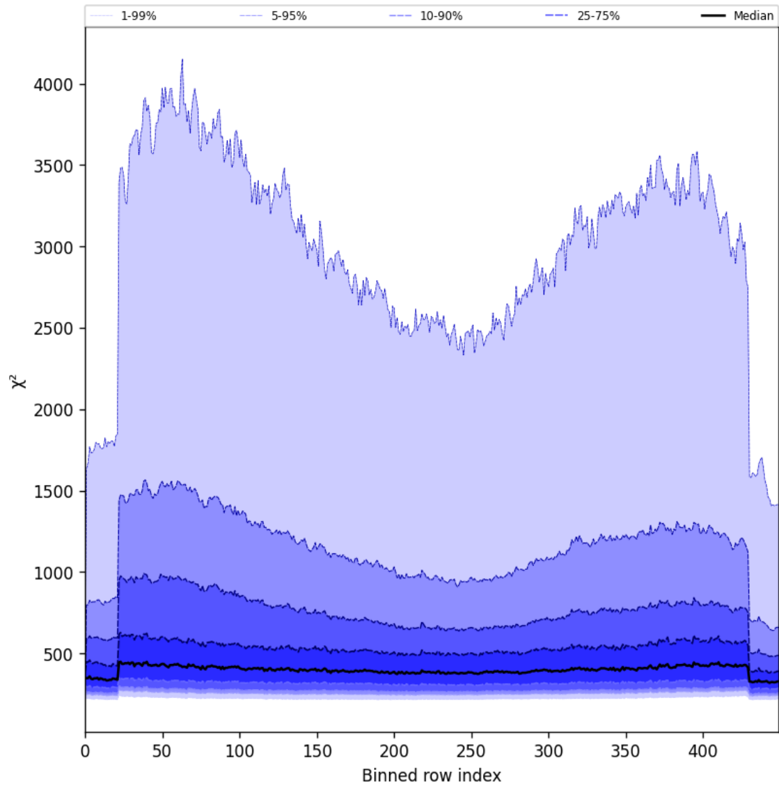
Figure 59: Along track statistics of “ \chi^2 ” for 2025-05-29 to 2025-05-31
