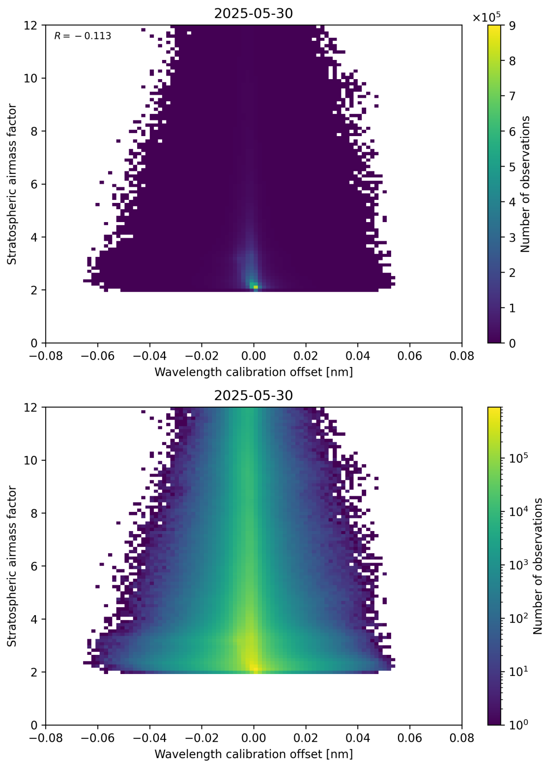
Figure 174: Scatter density plot of “Wavelength calibration offset” against “Stratospheric airmass factor” for 2025-05-29 to 2025-05-31.
