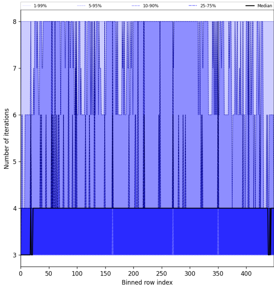
Figure 51: Along track statistics of “Number of iterations” for 2025-05-29 to 2025-05-31
