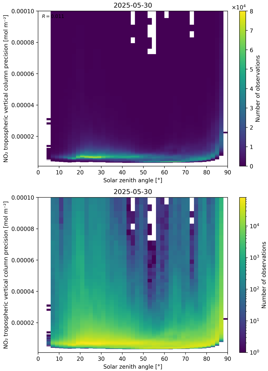
Figure 156: Scatter density plot of “Solar zenith angle” against “NO 2 tropospheric vertical column precision” for 2025-05-29 to 2025-05-31.
