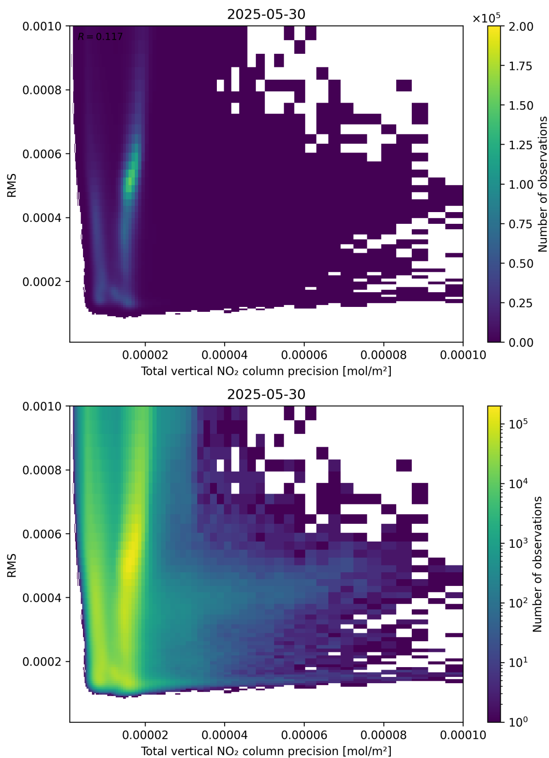
Figure 119: Scatter density plot of “Total vertical NO 2 column precision” against “RMS” for 2025-05-29 to 2025-05-31.
