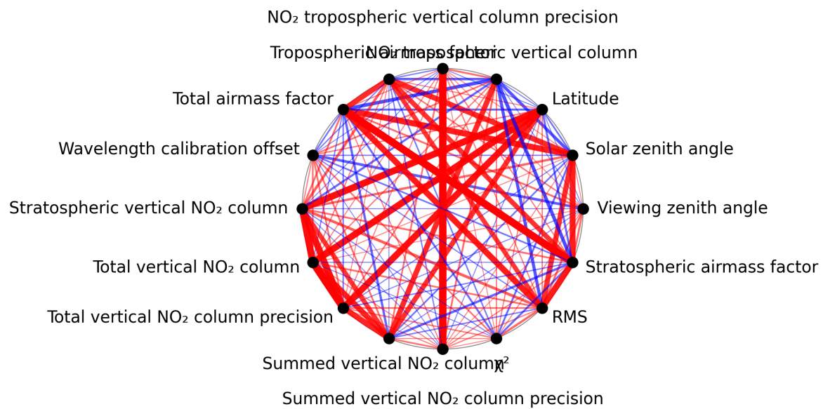
Figure 1: Map of correlation graph for 2025-05-29 to 2025-05-31.
