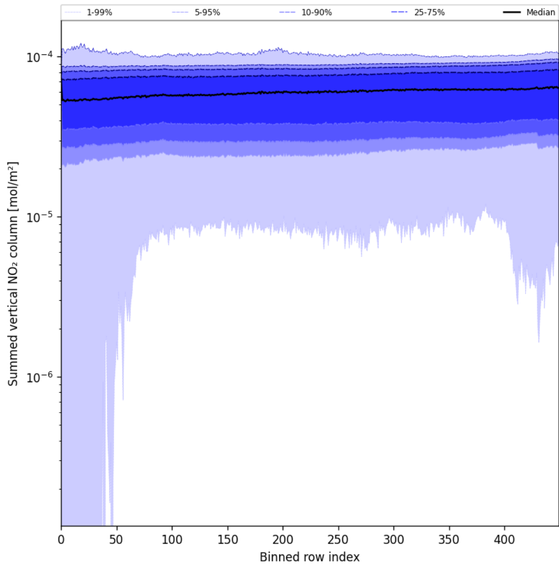
Figure 57: Along track statistics of “Summed vertical NO 2 column” for 2025-05-29 to 2025-05-31
