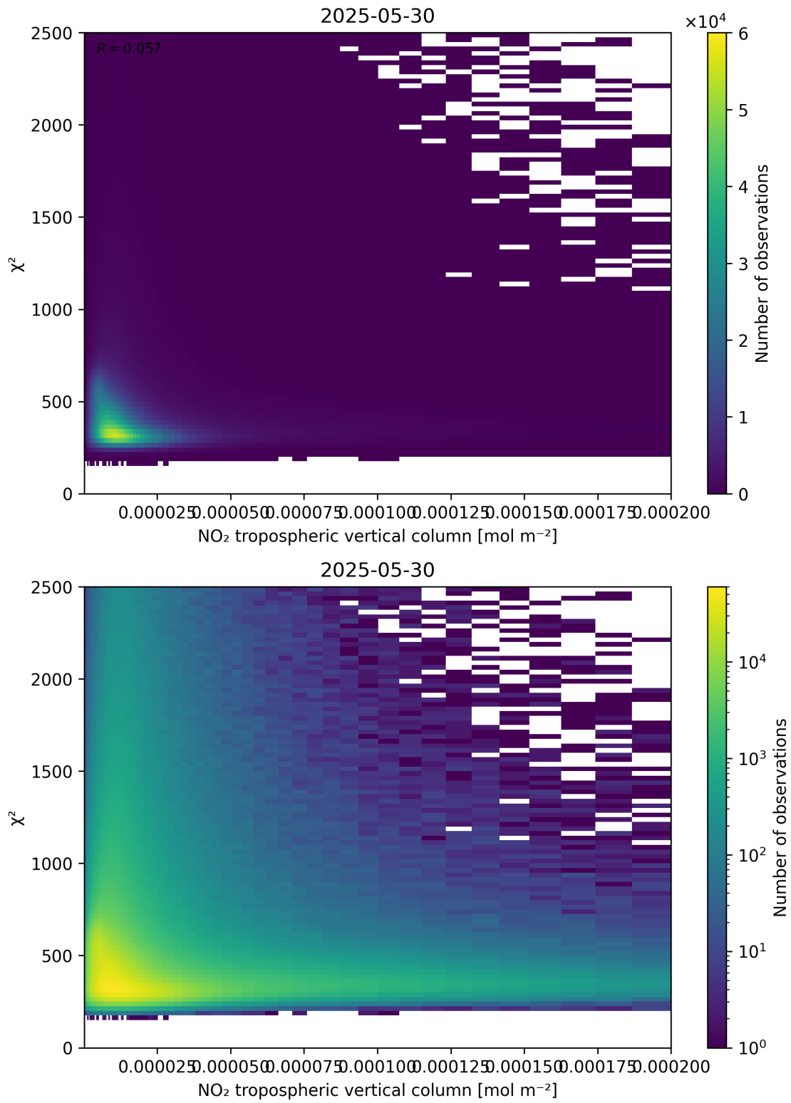
Figure 124: Scatter density plot of “NO 2 tropospheric vertical column” against “ \chi^2 ” for 2025-05-29 to 2025-05-31.
