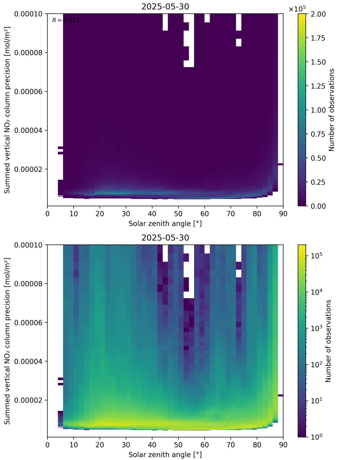
Figure 152: Scatter density plot of “Solar zenith angle” against “Summed vertical NO 2 column precision” for 2025-05-29 to 2025-05-31.
