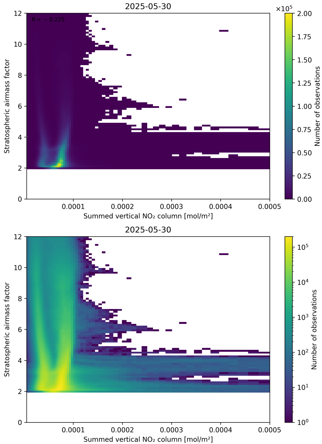
Figure 103: Scatter density plot of “Summed vertical NO 2 column” against “Stratospheric air mass factor” for 2025-05-29 to 2025-05-31.
