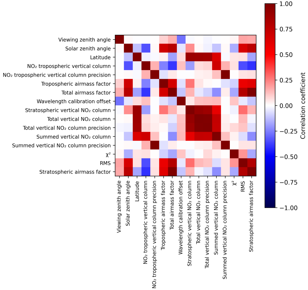
Figure 2: Map of correlation matrix for 2025-05-29 to 2025-05-31.
