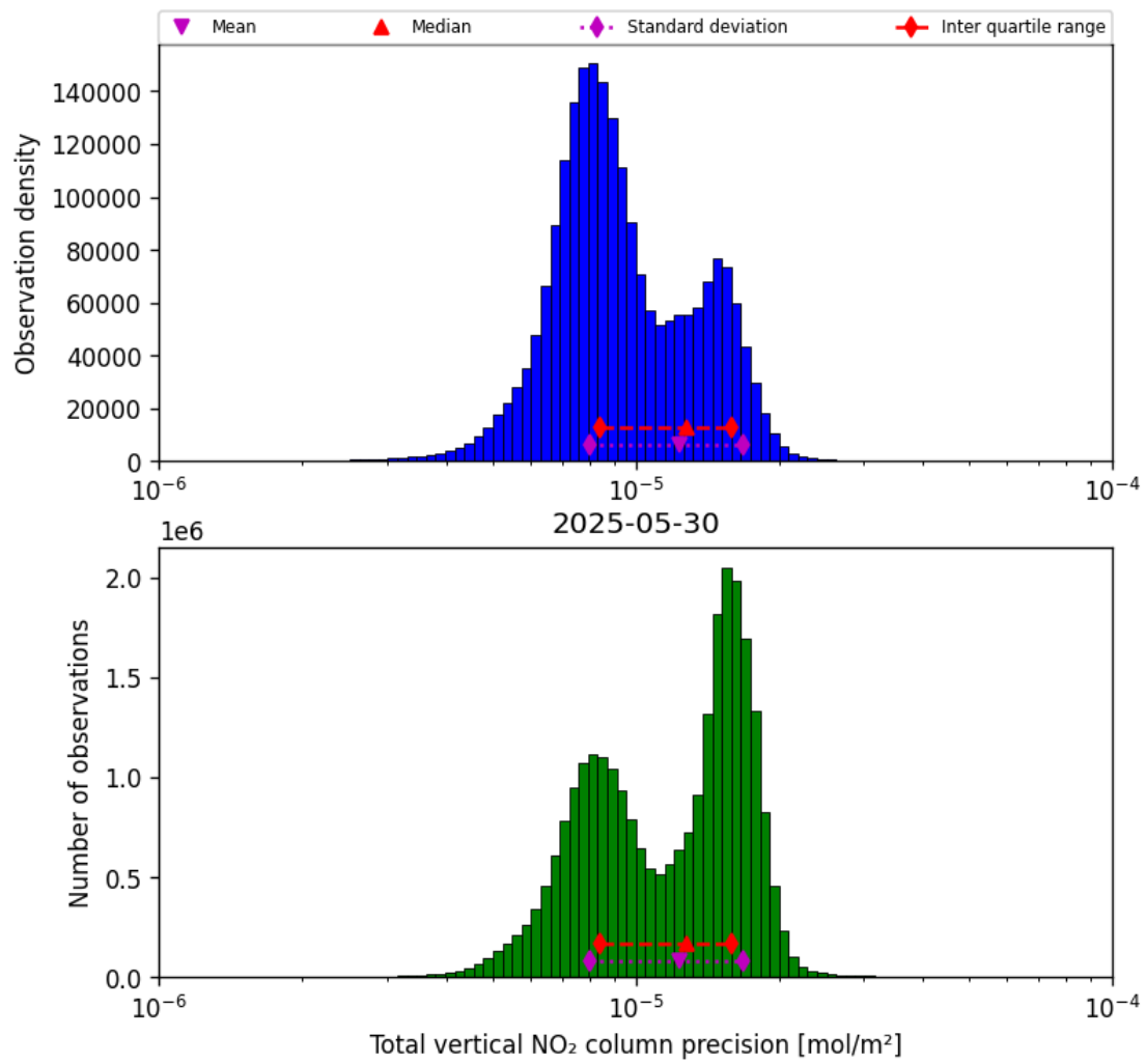
Figure 39: Histogram of “Total vertical NO 2 column precision” for 2025-05-29 to 2025-05-31
