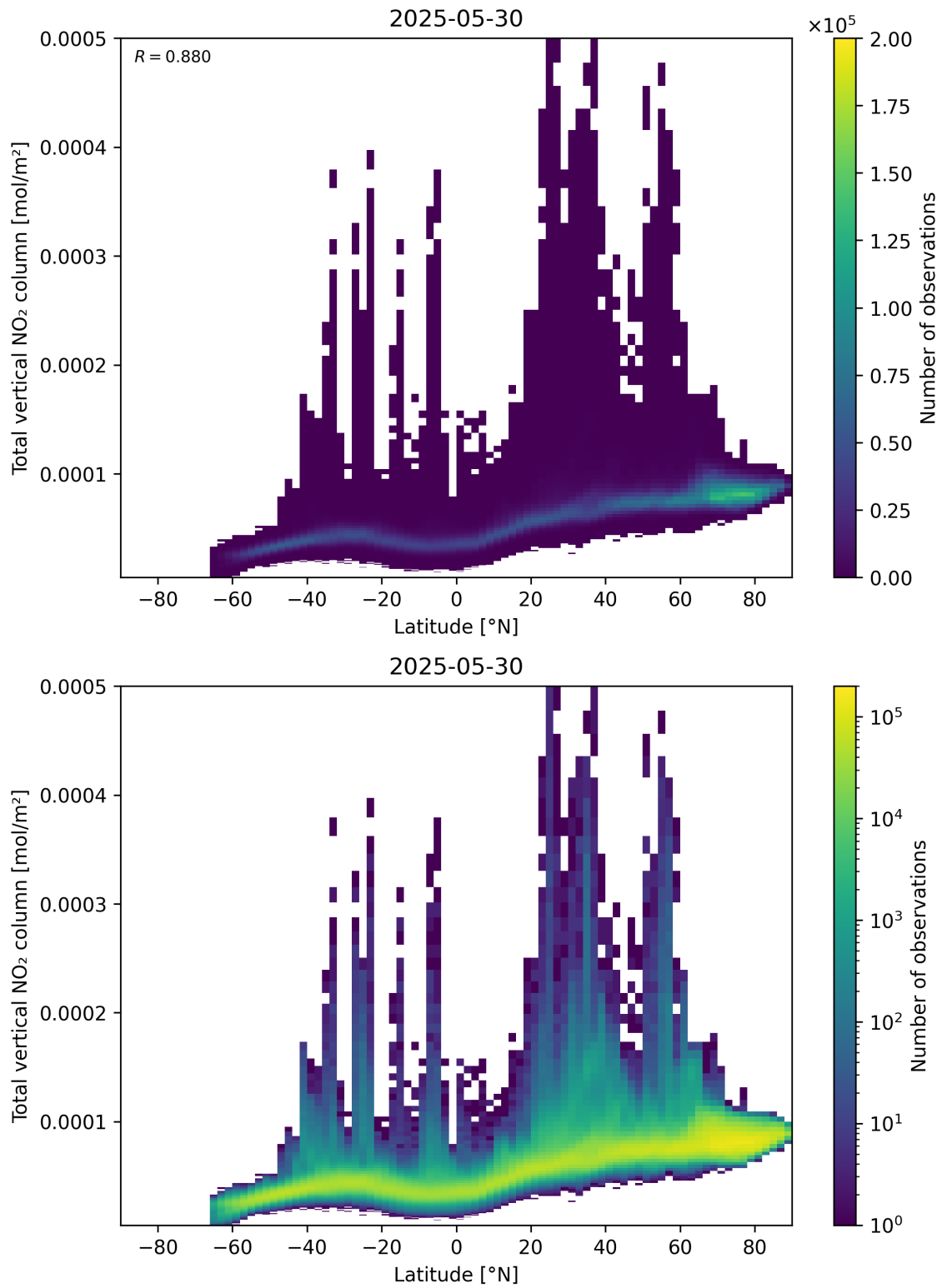
Figure 90: Scatter density plot of “Latitude” against “Total vertical NO 2 column” for 2025-05-29 to 2025-05-31.
