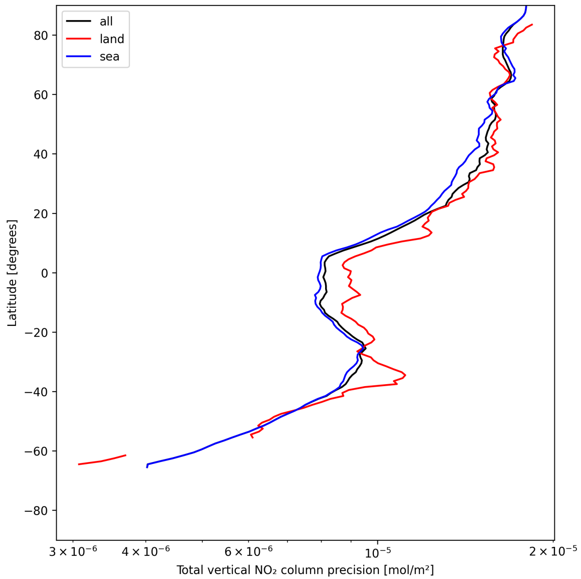
Figure 22: Zonal average of “Total vertical NO 2 column precision” for 2025-05-29 to 2025-05-31.
