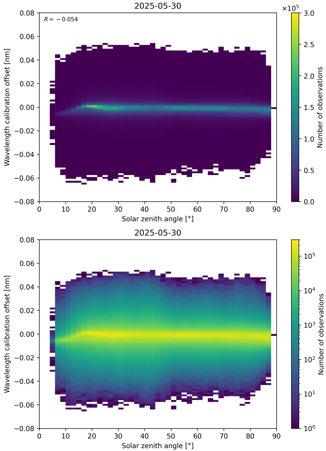
Figure 158: Scatter density plot of “Solar zenith angle” against “Wavelength calibration offset” for 2025-05-29 to 2025-05-31.
