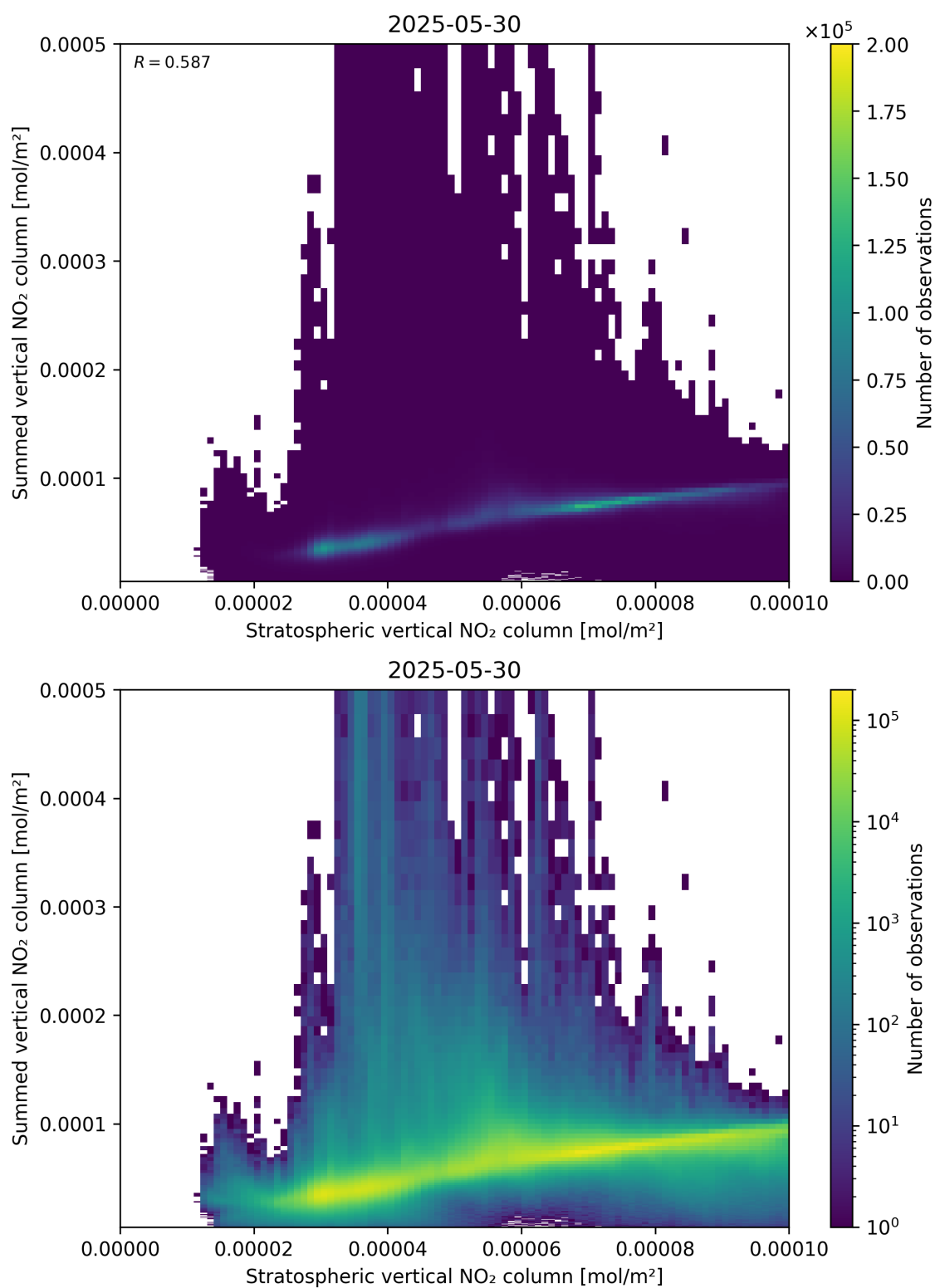
Figure 98: Scatter density plot of “Stratospheric vertical NO 2 column” against “Summed vertical NO 2 column” for 2025-05-29 to 2025-05-31.
