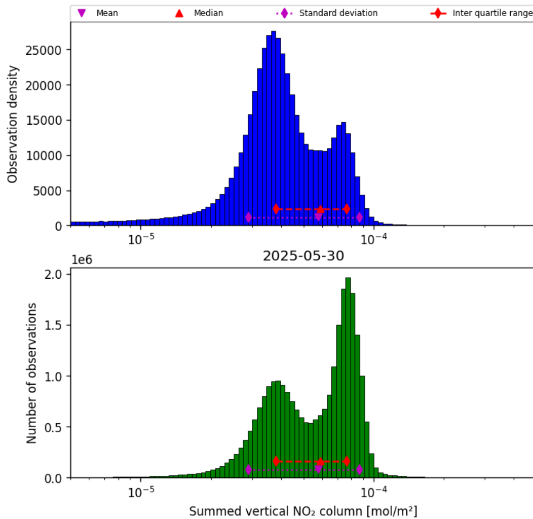
Figure 40: Histogram of “Summed vertical NO 2 column” for 2025-05-29 to 2025-05-31
