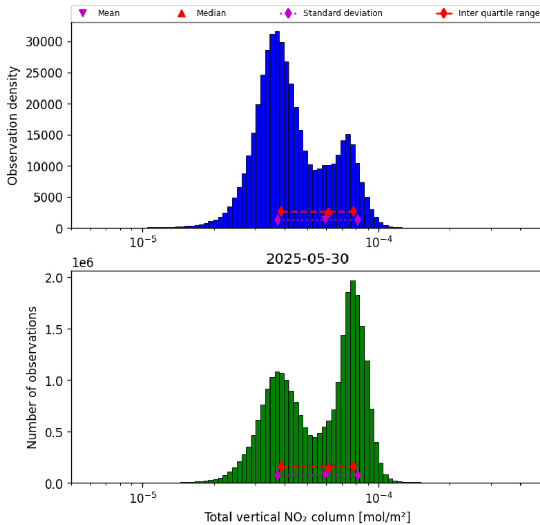
Figure 38: Histogram of “Total vertical NO 2 column” for 2025-05-29 to 2025-05-31
