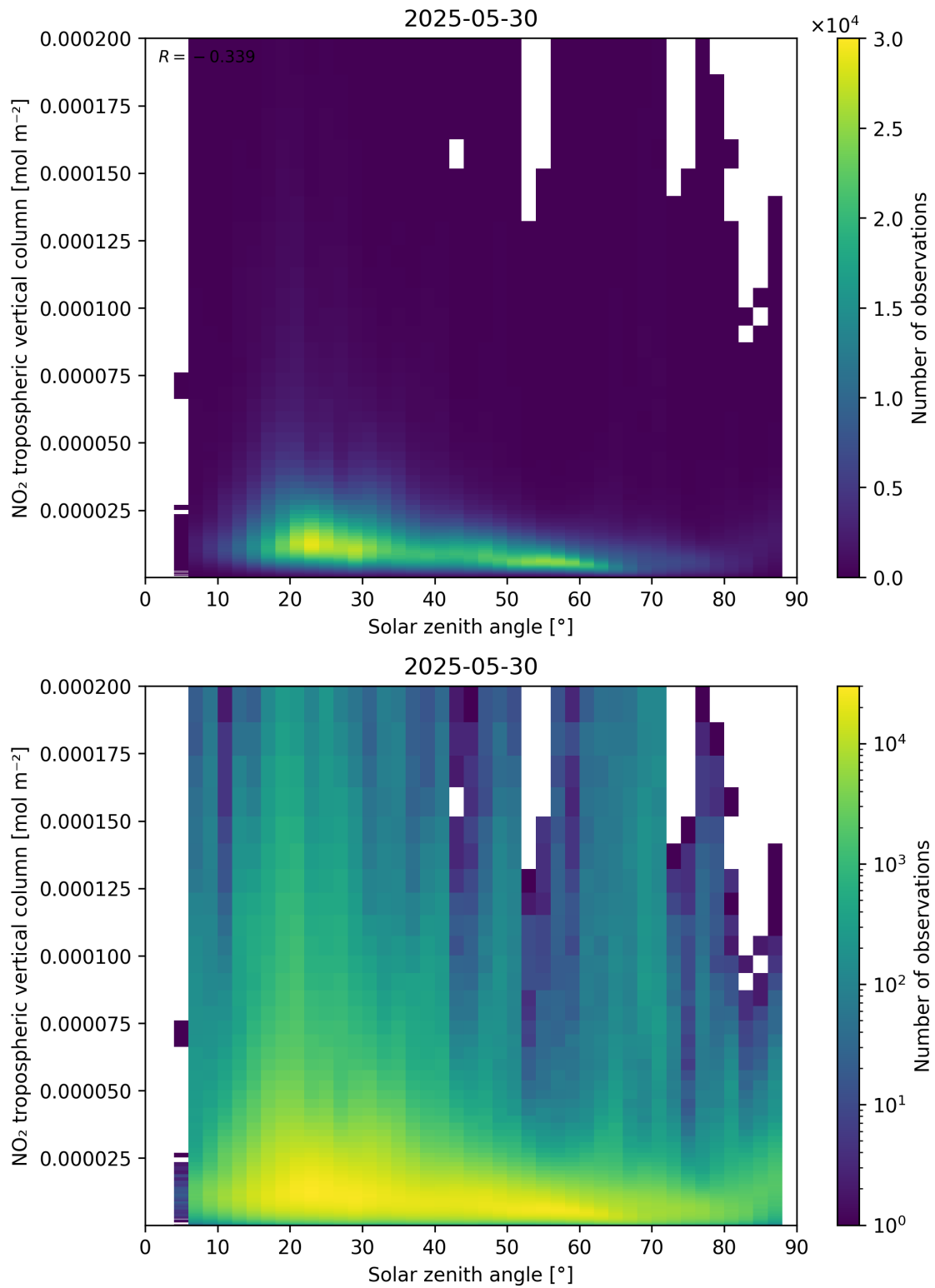
Figure 155: Scatter density plot of “Solar zenith angle” against “NO 2 tropospheric vertical column” for 2025-05-29 to 2025-05-31.
