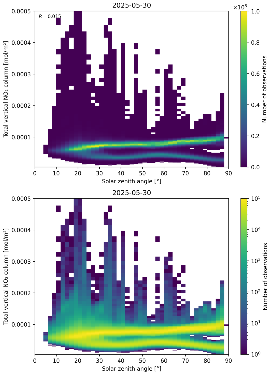
Figure 153: Scatter density plot of “Solar zenith angle” against “Total vertical NO 2 column” for 2025-05-29 to 2025-05-31.
