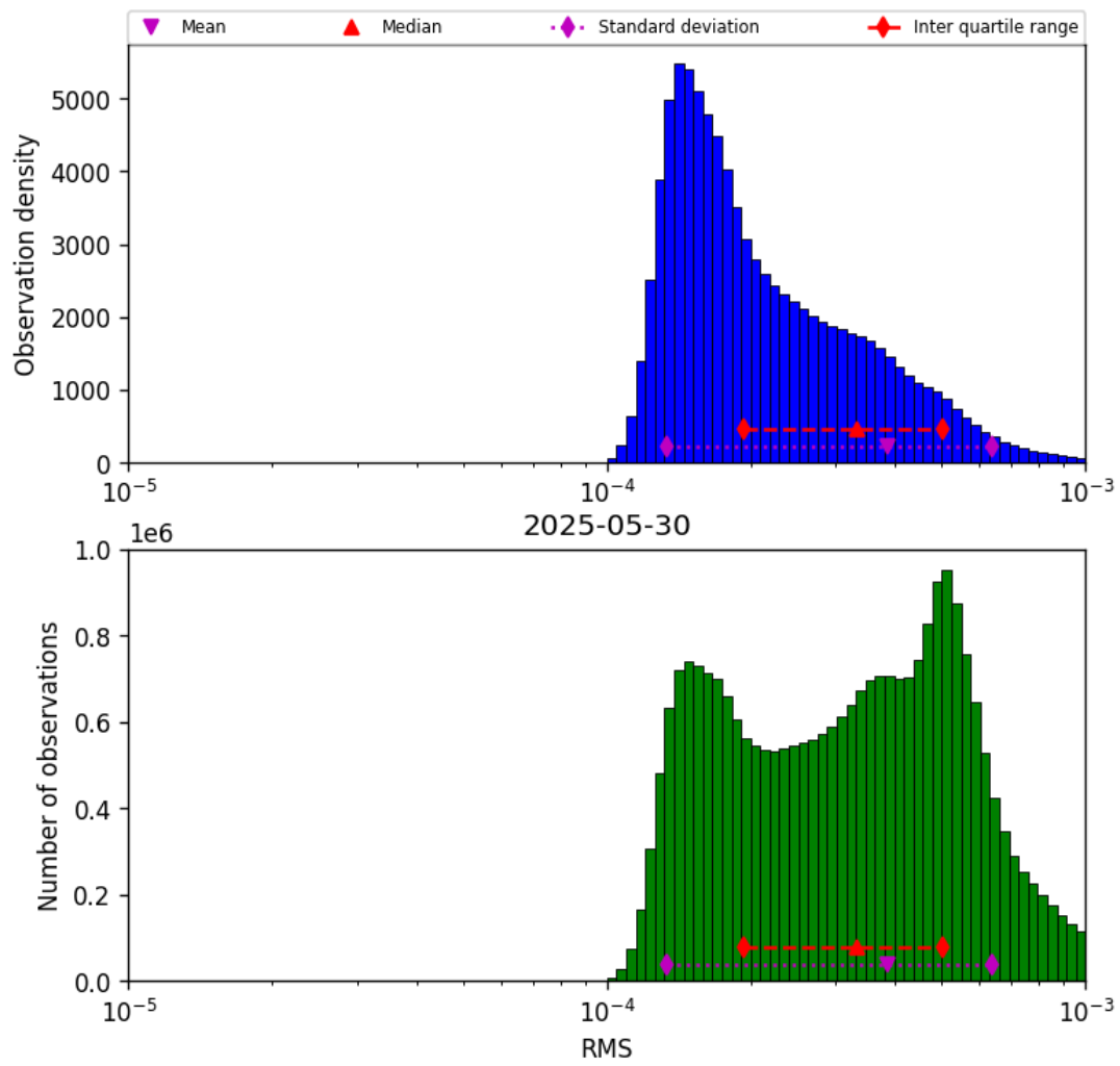
Figure 43: Histogram of “RMS” for 2025-05-29 to 2025-05-31
