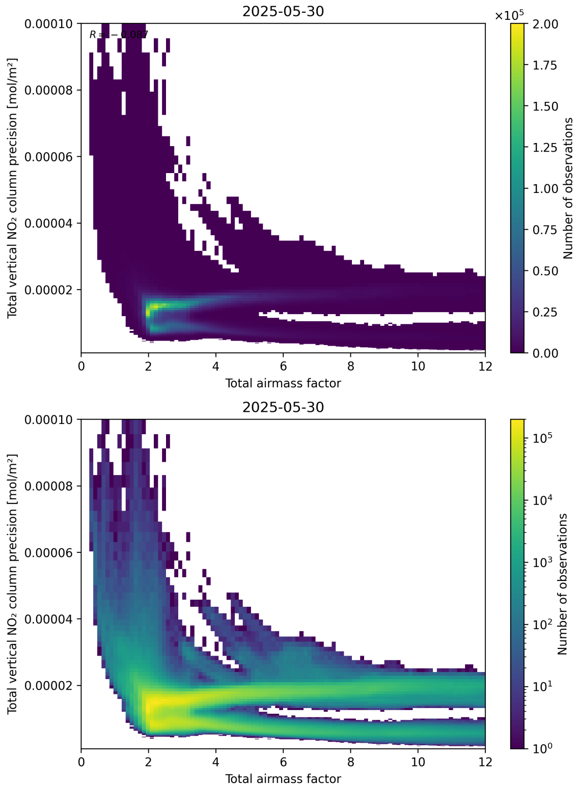
Figure 68: Scatter density plot of “Total airmass factor” against “Total vertical NO 2 column precision” for 2025-05-29 to 2025-05-31.
