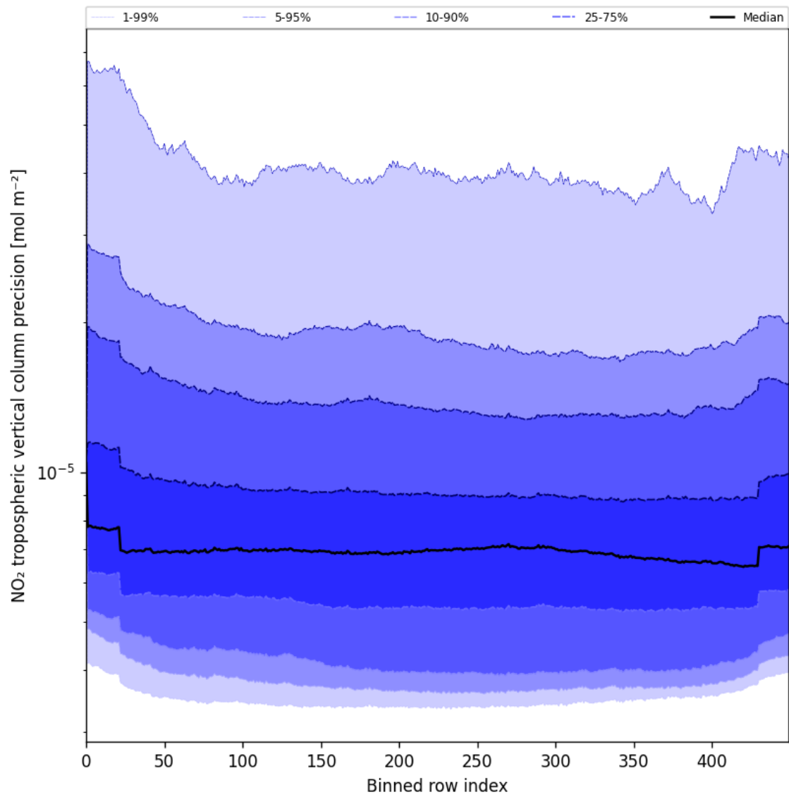
Figure 47: Along track statistics of “NO 2 tropospheric vertical column precision” for 2025-05-29 to 2025-05-31
