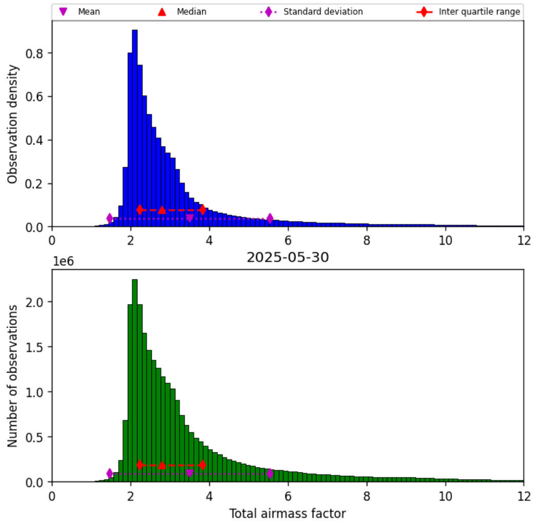
Figure 32: Histogram of “Total airmass factor” for 2025-05-29 to 2025-05-31
