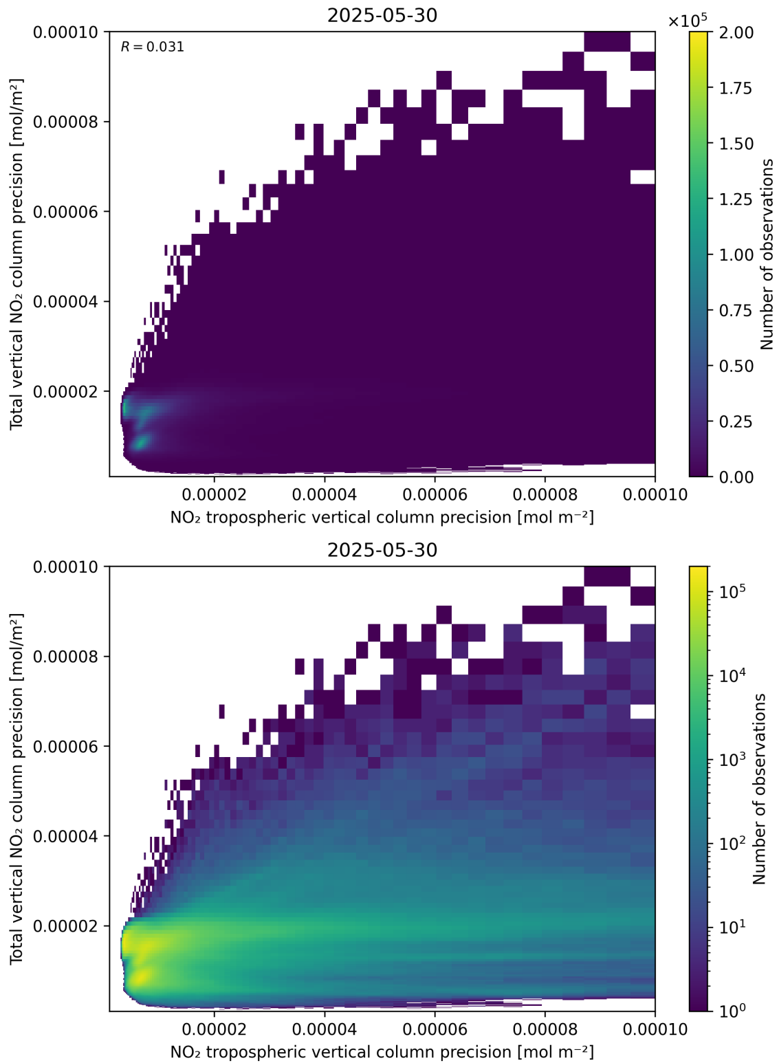
Figure 139: Scatter density plot of “NO 2 tropospheric vertical column precision” against “Total vertical NO 2 column precision” for 2025-05-29 to 2025-05-31.
