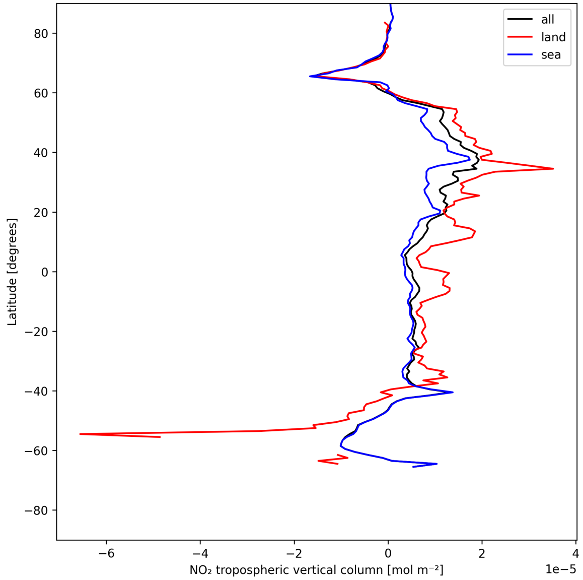
Figure 12: Zonal average of “NO 2 tropospheric vertical column” for 2025-05-29 to 2025-05-31.
