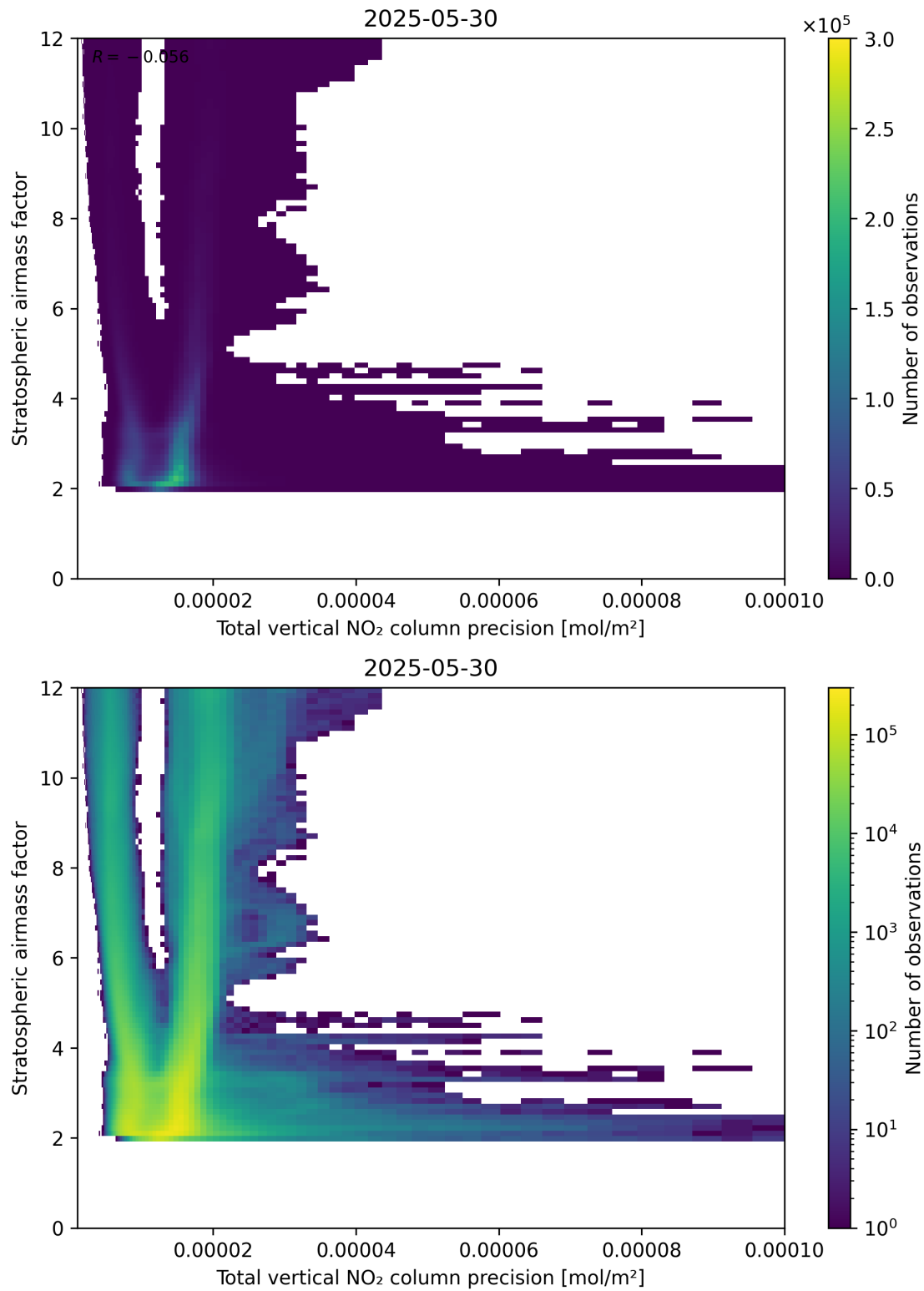
Figure 115: Scatter density plot of “Total vertical NO 2 column precision” against “Stratospheric air mass factor” for 2025-05-29 to 2025-05-31.
