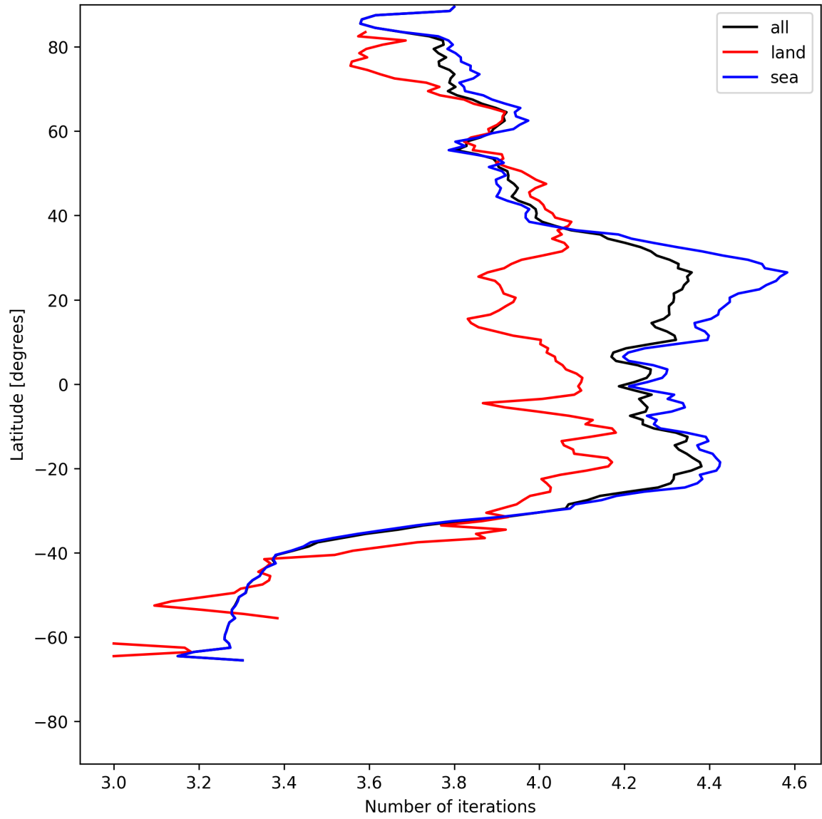
Figure 17: Zonal average of “Number of iterations” for 2025-05-29 to 2025-05-31.
