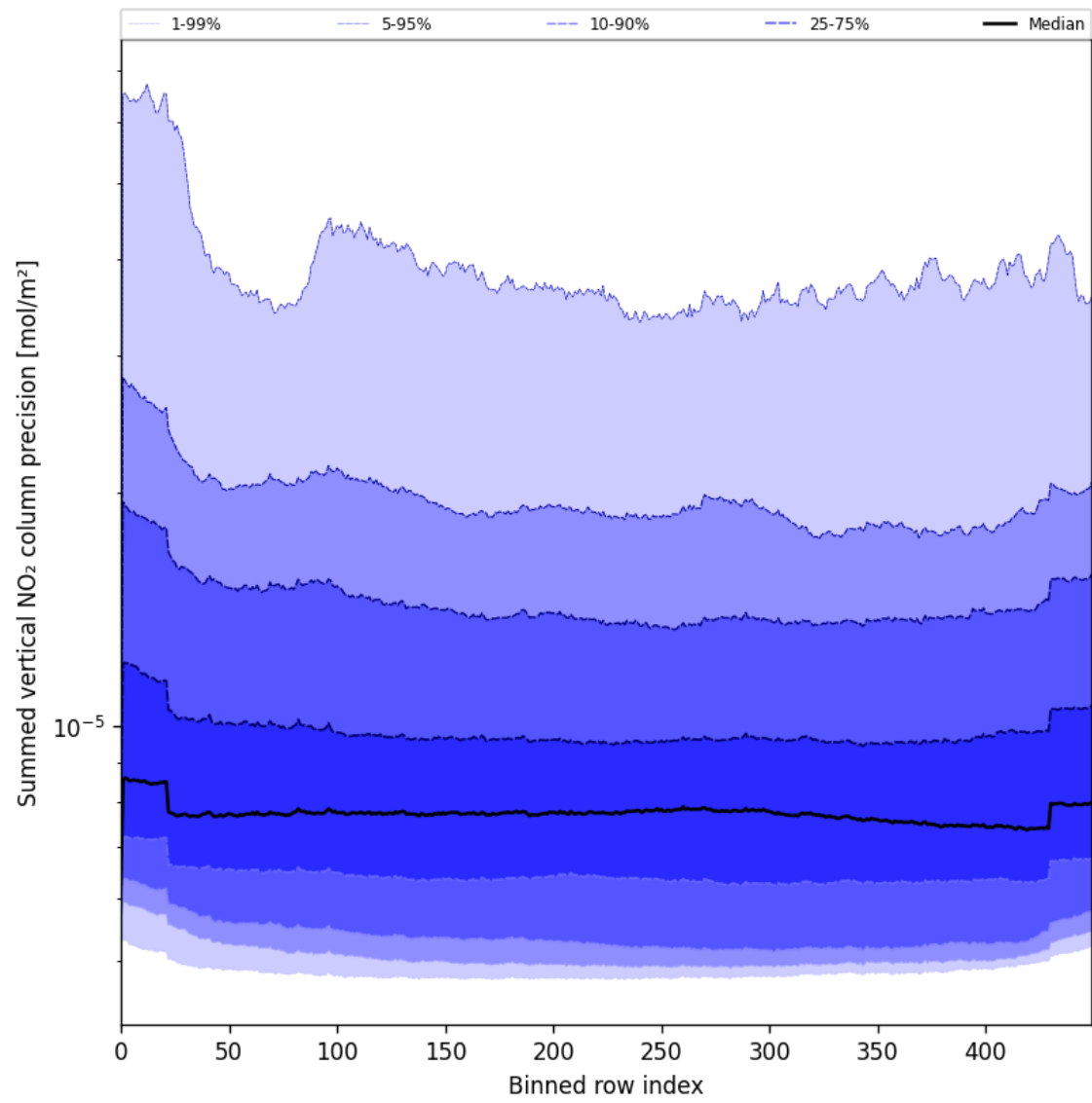
Figure 58: Along track statistics of “Summed vertical NO 2 column precision” for 2025-05-31 to 2025-06-01
