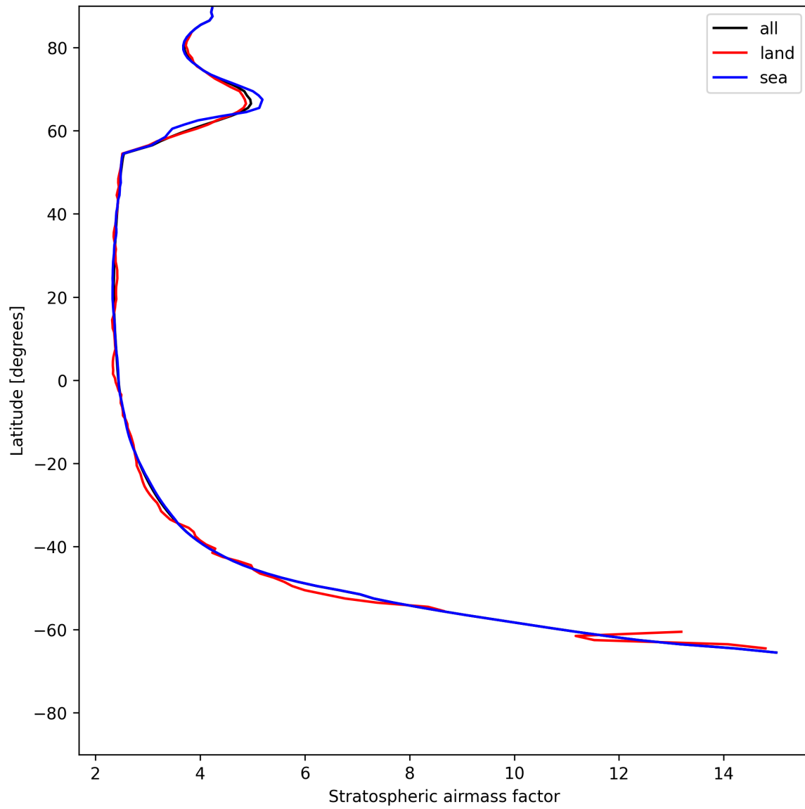
Figure 27: Zonal average of “Stratospheric air mass factor” for 2025-05-31 to 2025-06-01.
