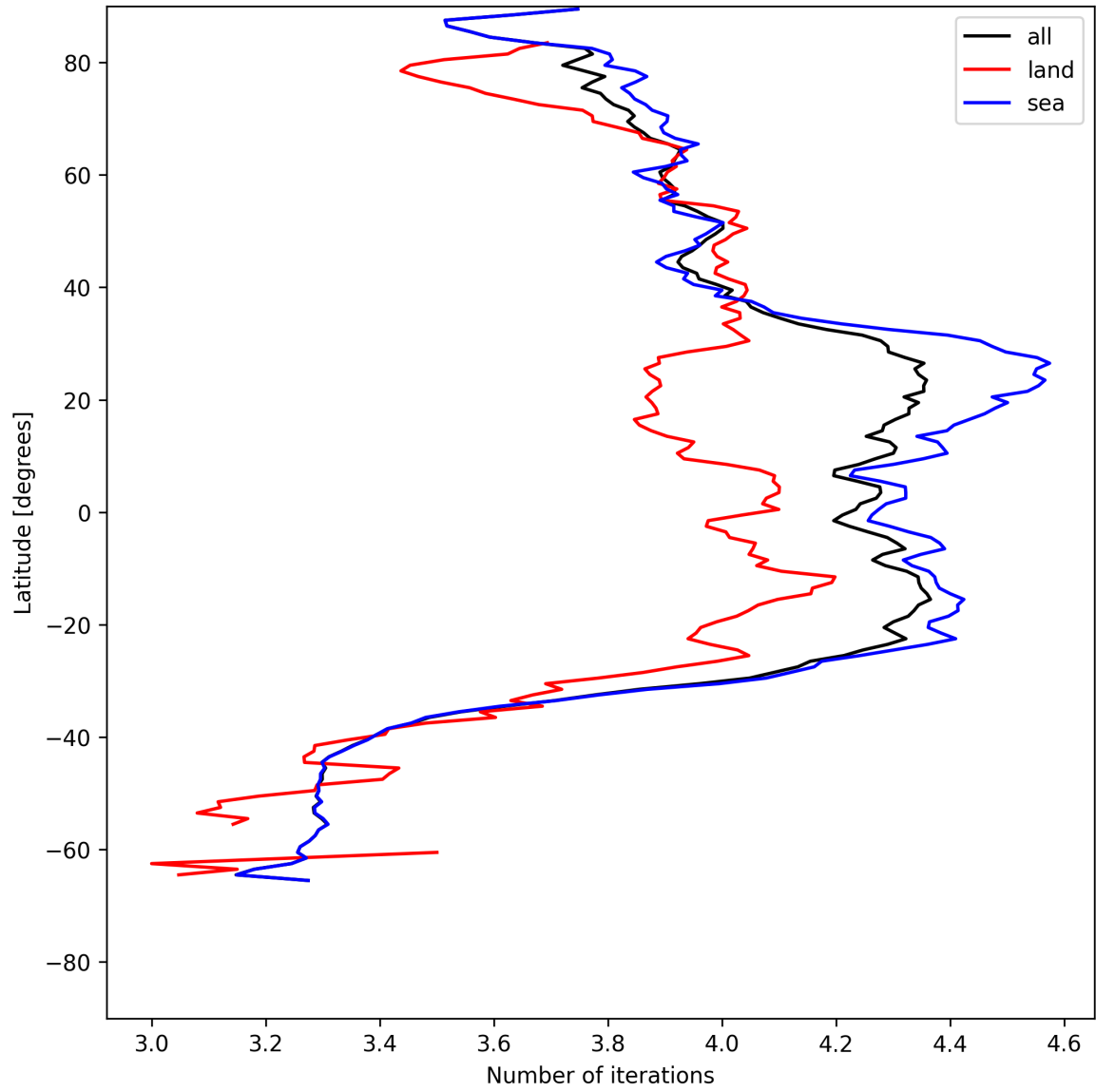
Figure 17: Zonal average of “Number of iterations” for 2025-05-31 to 2025-06-01.
