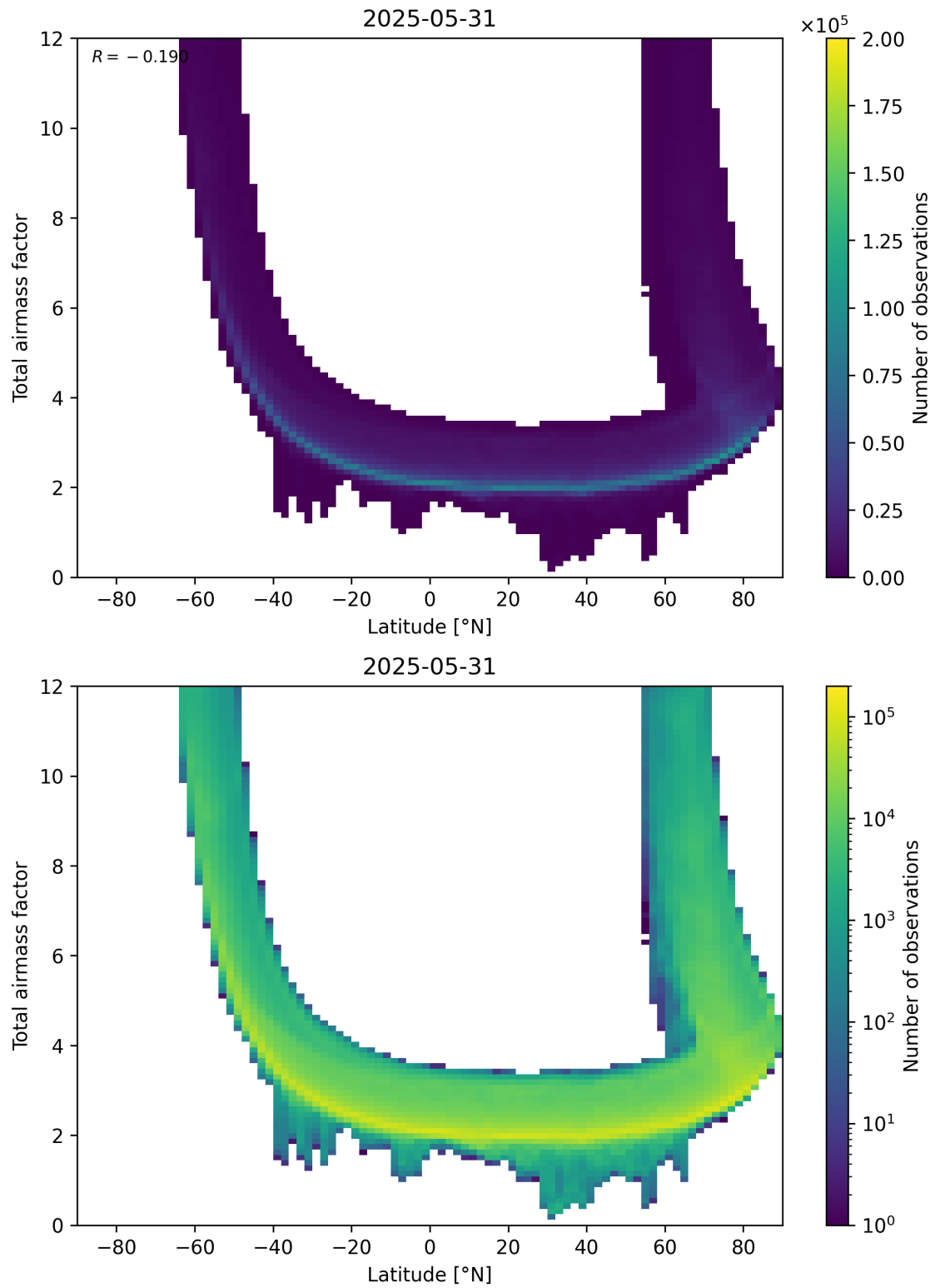
Figure 84: Scatter density plot of “Latitude” against “Total airmass factor” for 2025-05-31 to 2025-06-01.
