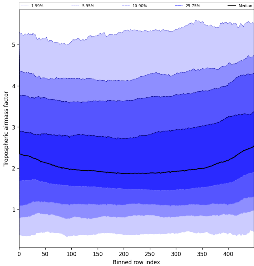
Figure 48: Along track statistics of “Tropospheric airmass factor” for 2025-05-31 to 2025-06-01
