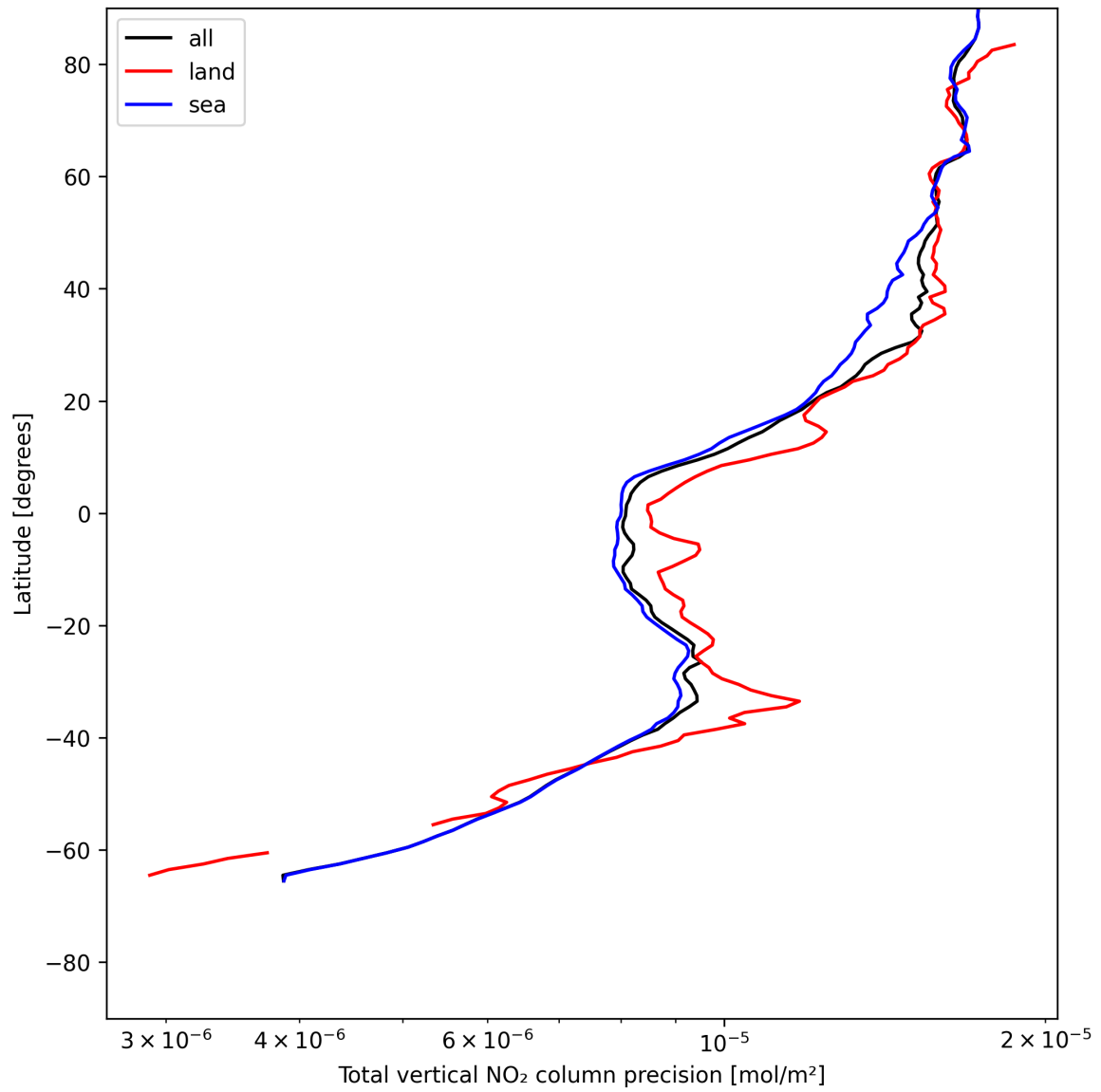
Figure 22: Zonal average of “Total vertical NO 2 column precision” for 2025-05-31 to 2025-06-01.
