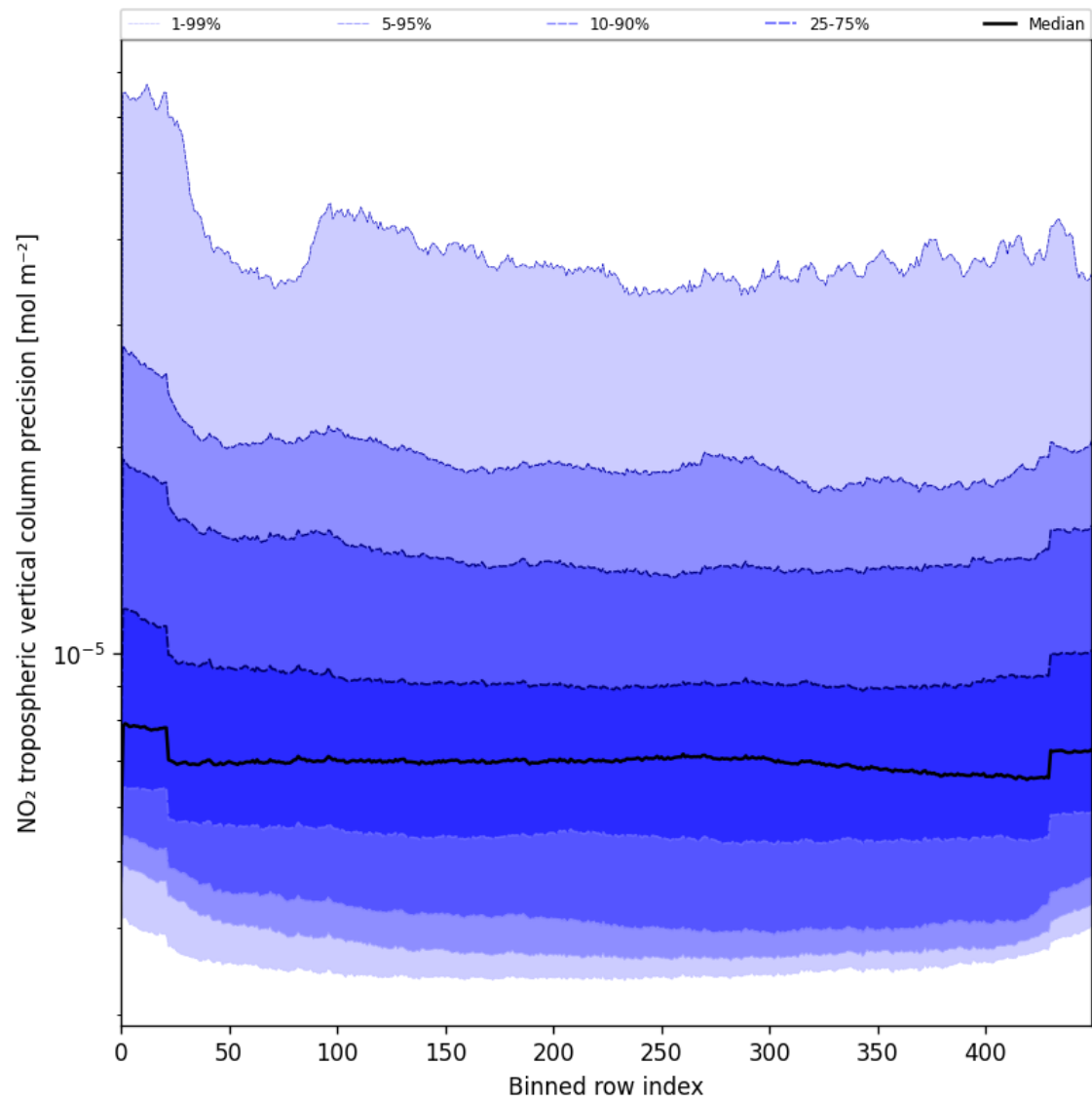
Figure 47: Along track statistics of “NO 2 tropospheric vertical column precision” for 2025-05-31 to 2025-06-01
