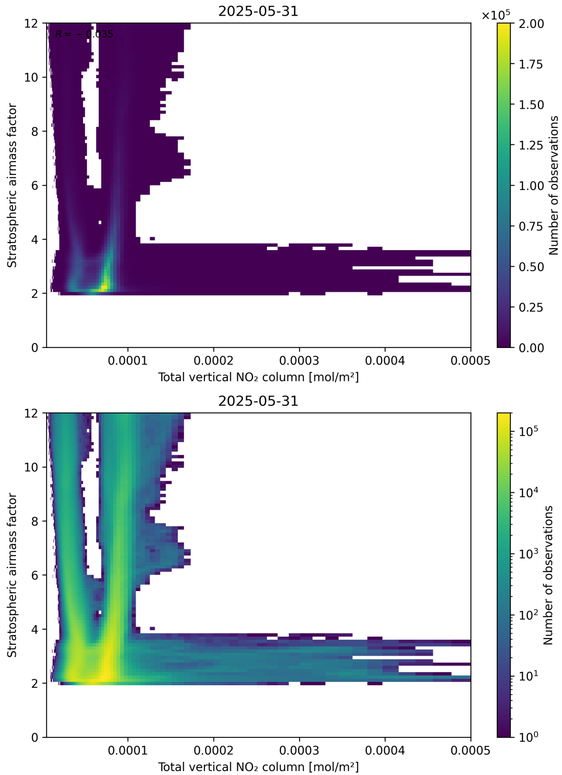
Figure 110: Scatter density plot of “Total vertical NO 2 column” against “Stratospheric airmass factor” for 2025-05-31 to 2025-06-01.
