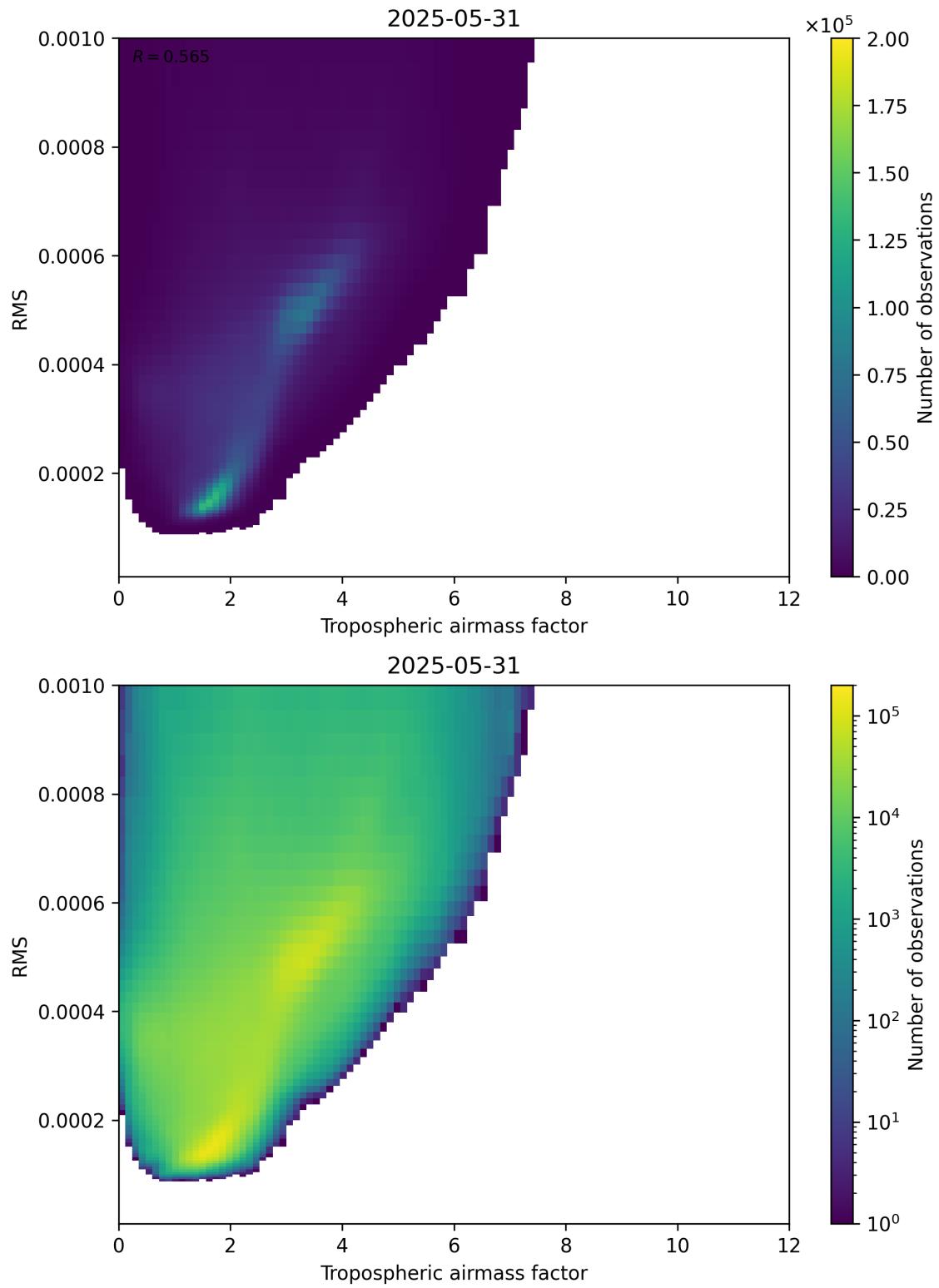
Figure 79: Scatter density plot of “Tropospheric airmass factor” against “RMS” for 2025-05-31 to 2025-06-01.
