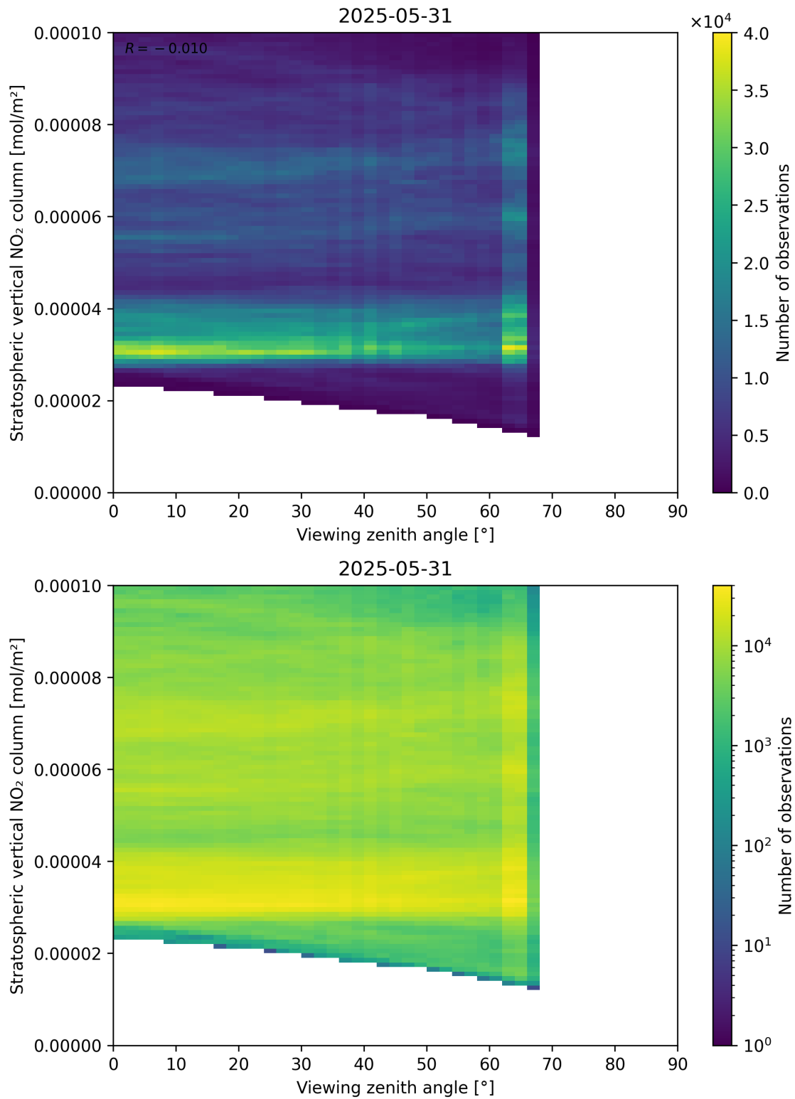
Figure 164: Scatter density plot of “Viewing zenith angle” against “Stratospheric vertical NO 2 column” for 2025-05-31 to 2025-06-01.
