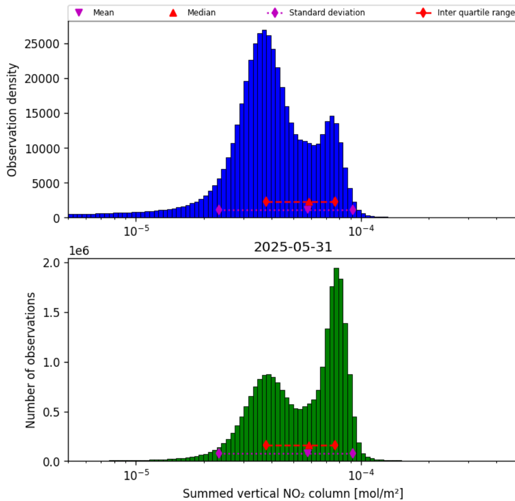
Figure 40: Histogram of “Summed vertical NO 2 column” for 2025-05-31 to 2025-06-01
