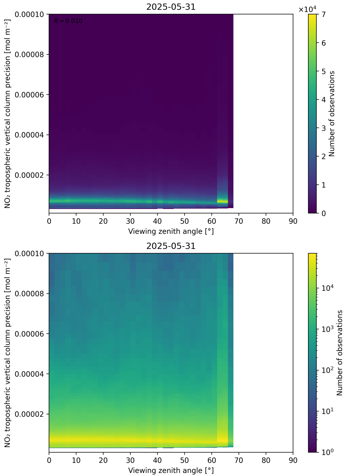
Figure 170: Scatter density plot of “Viewing zenith angle” against “NO 2 tropospheric vertical column precision” for 2025-05-31 to 2025-06-01.
