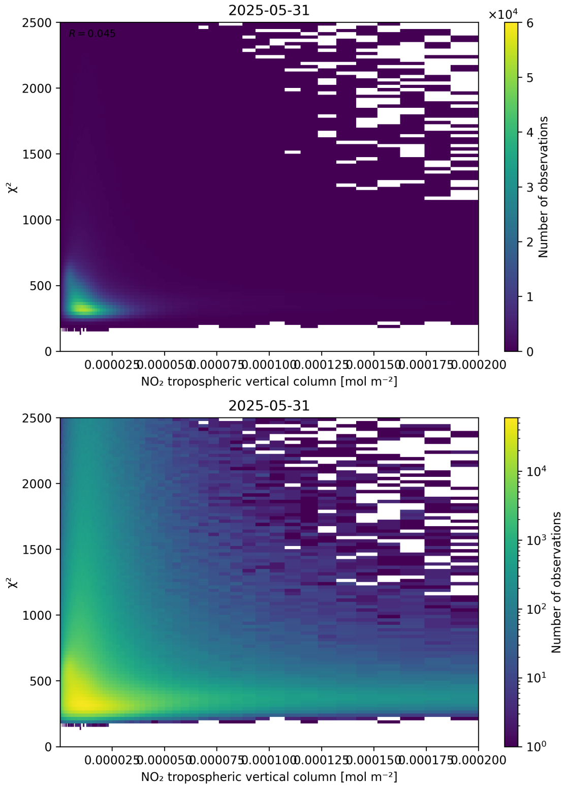
Figure 124: Scatter density plot of “NO 2 tropospheric vertical column” against “ \chi^2 ” for 2025-05-31 to 2025-06-01.
