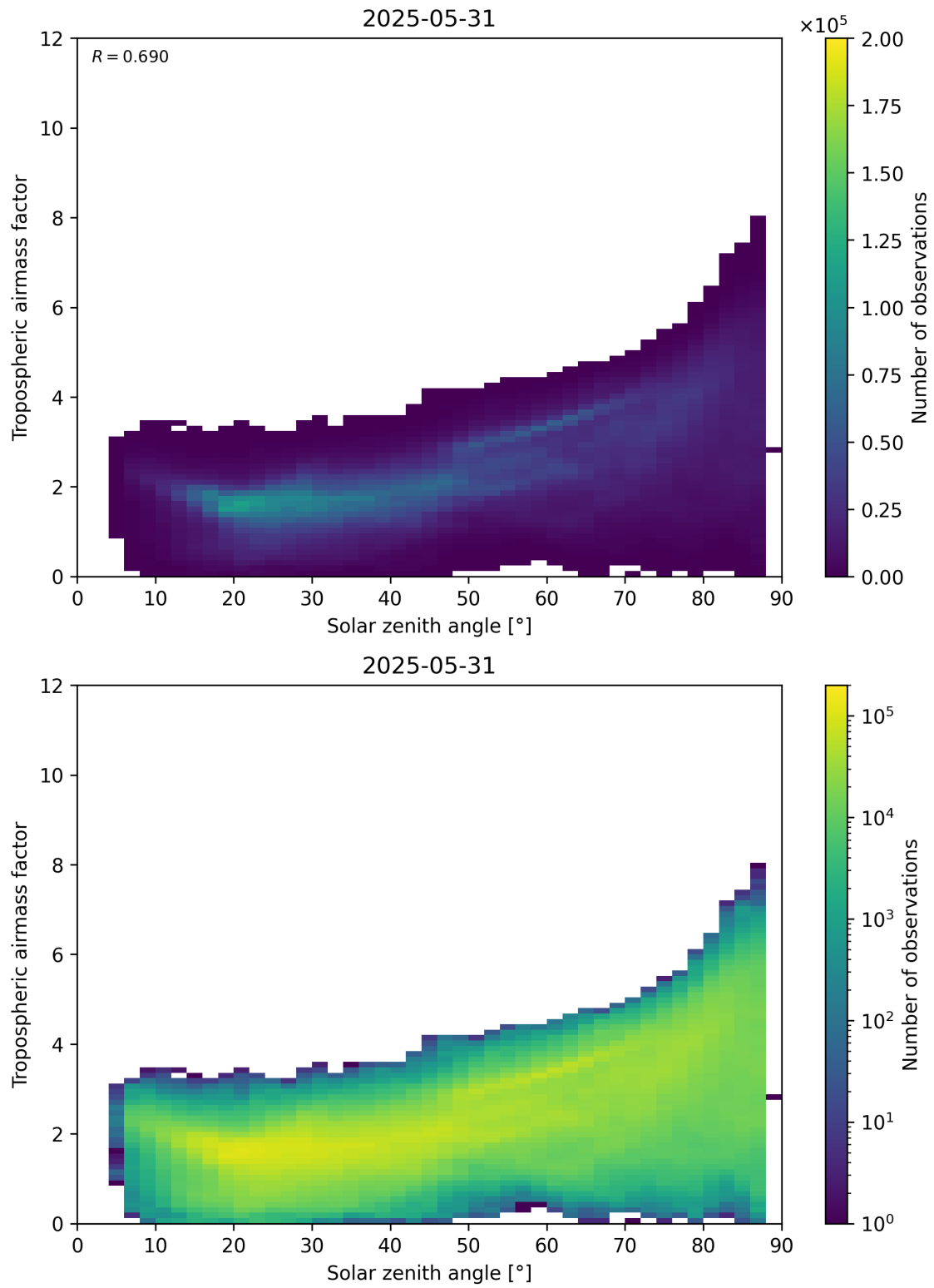
Figure 147: Scatter density plot of “Solar zenith angle” against “Tropospheric airmass factor” for 2025-05-31 to 2025-06-01.
