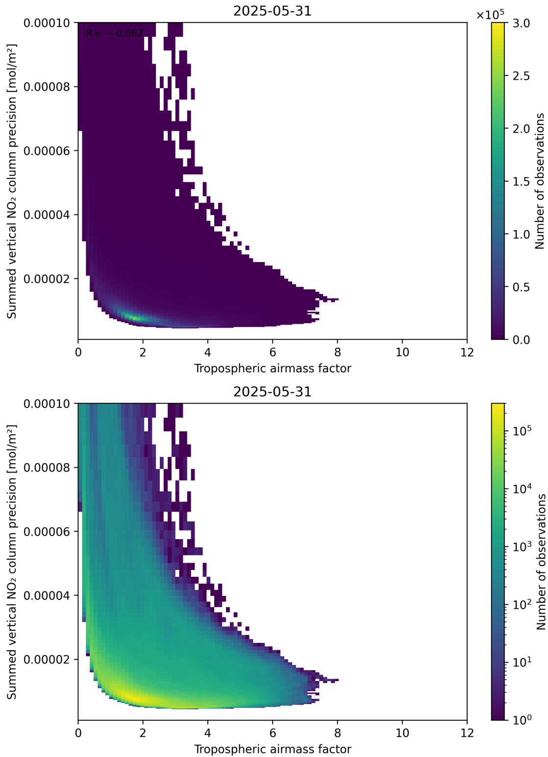
Figure 76: Scatter density plot of “Tropospheric air mass factor” against “Summed vertical NO 2 column precision” for 2025-05-31 to 2025-06-01.
