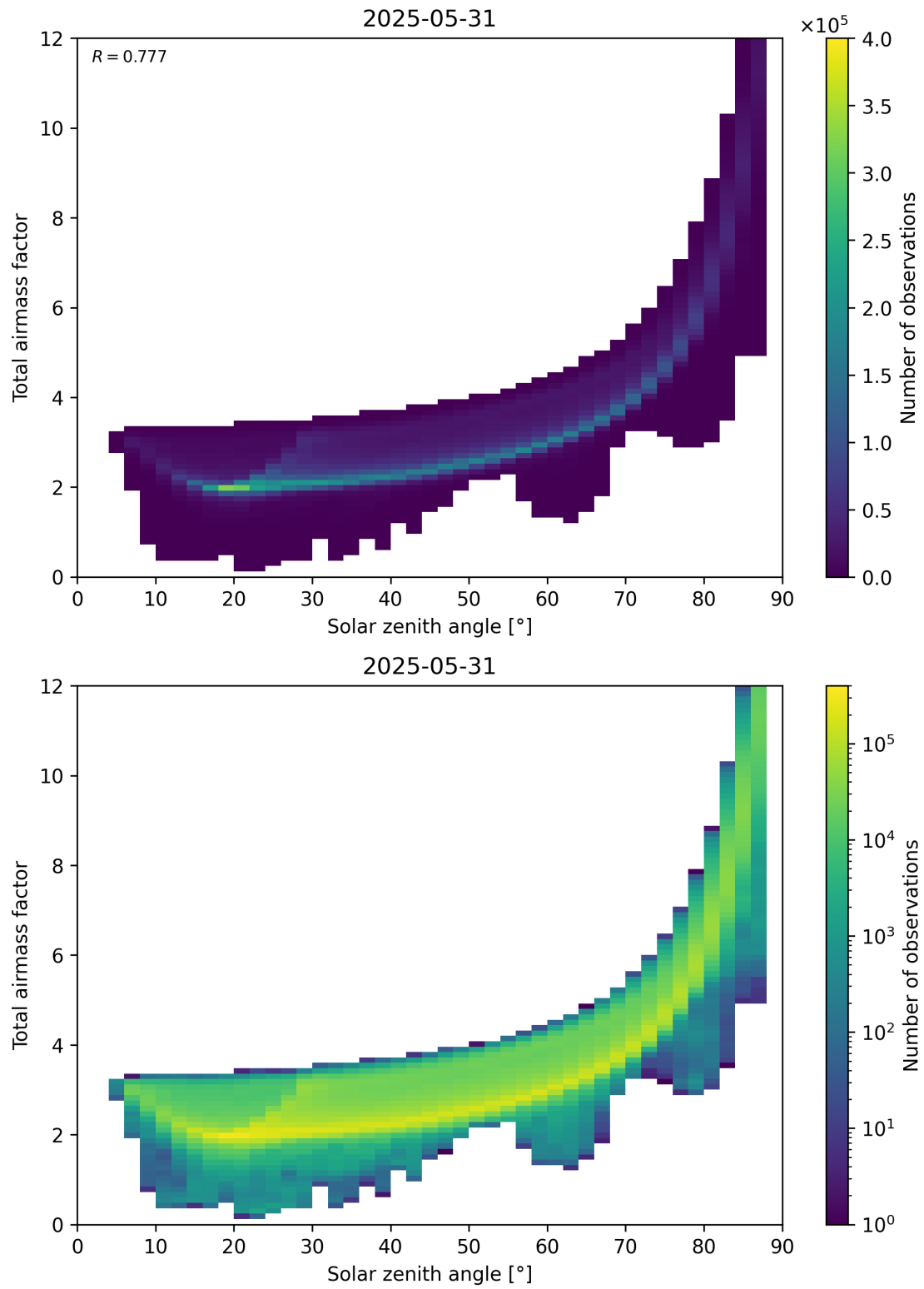
Figure 146: Scatter density plot of “Solar zenith angle” against “Total airmass factor” for 2025-05-31 to 2025-06-01.
