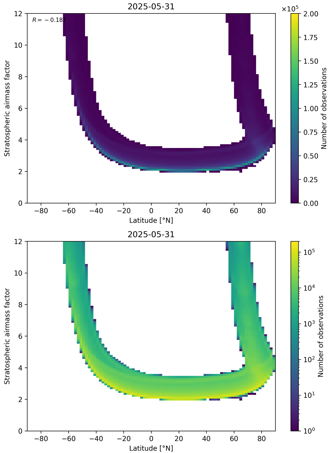
Figure 83: Scatter density plot of “Latitude” against “Stratospheric air mass factor” for 2025-05-31 to 2025-06-01.
