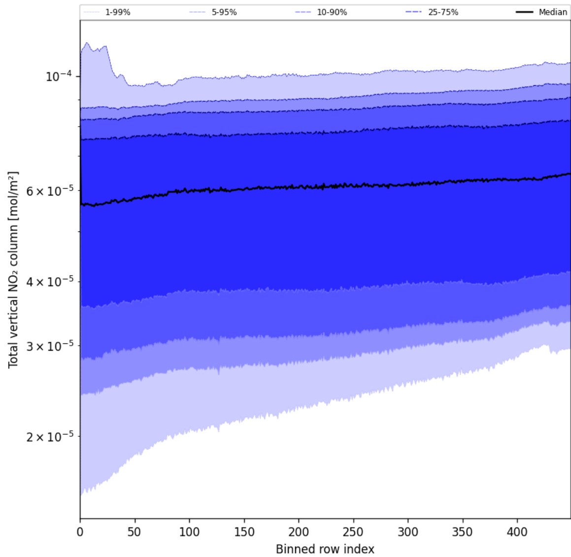
Figure 55: Along track statistics of “Total vertical NO 2 column” for 2025-05-31 to 2025-06-01
