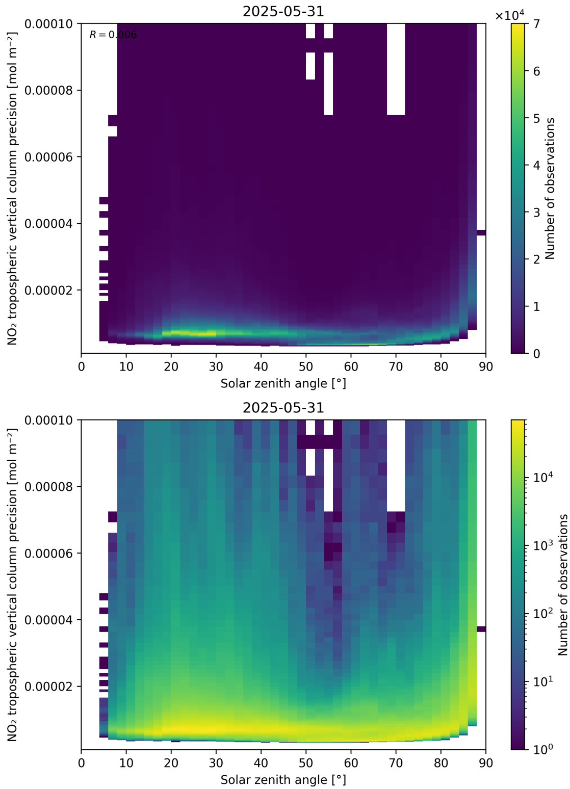
Figure 156: Scatter density plot of “Solar zenith angle” against “NO 2 tropospheric vertical column precision” for 2025-05-31 to 2025-06-01.
