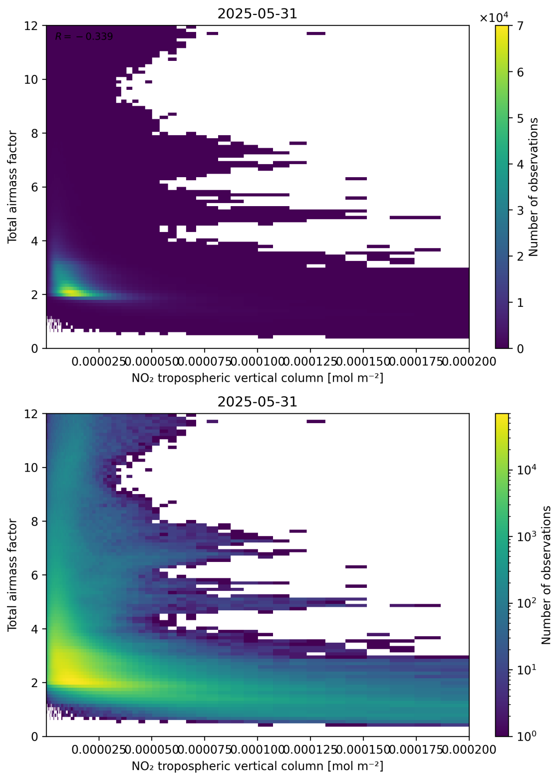
Figure 122: Scatter density plot of “NO 2 tropospheric vertical column” against “Total air mass factor” for 2025-05-31 to 2025-06-01.
