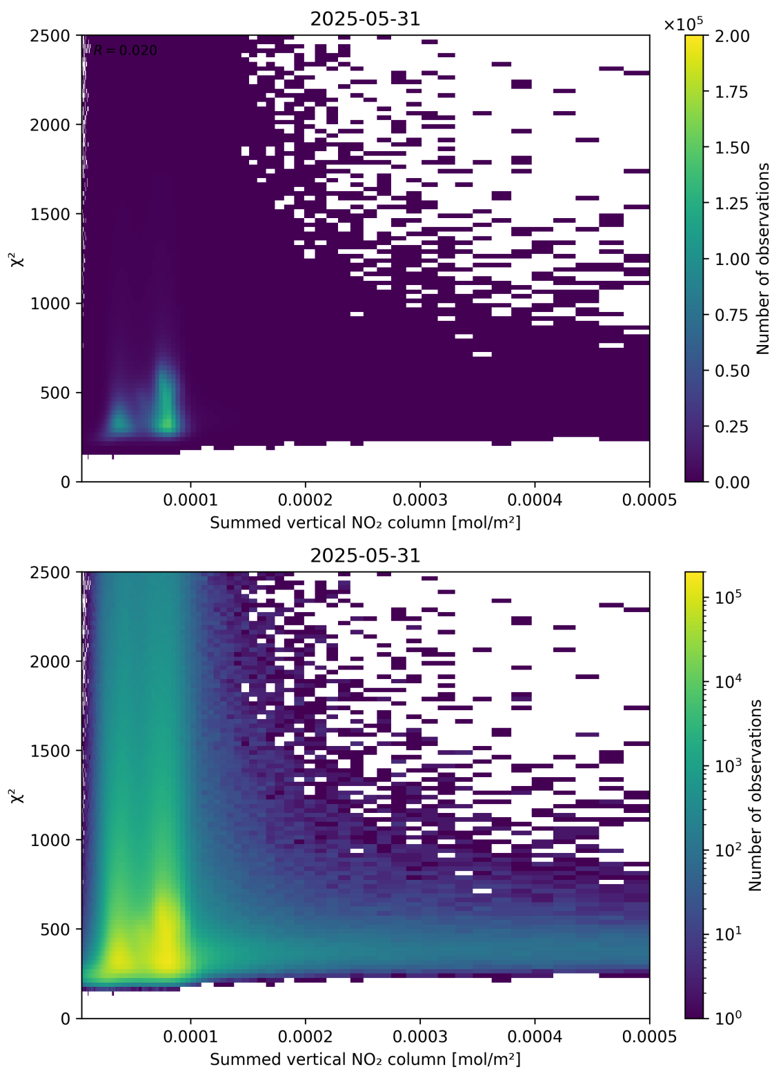
Figure 104: Scatter density plot of “Summed vertical NO 2 column” against “ \chi^2 ” for 2025-05-31 to 2025-06-01.
