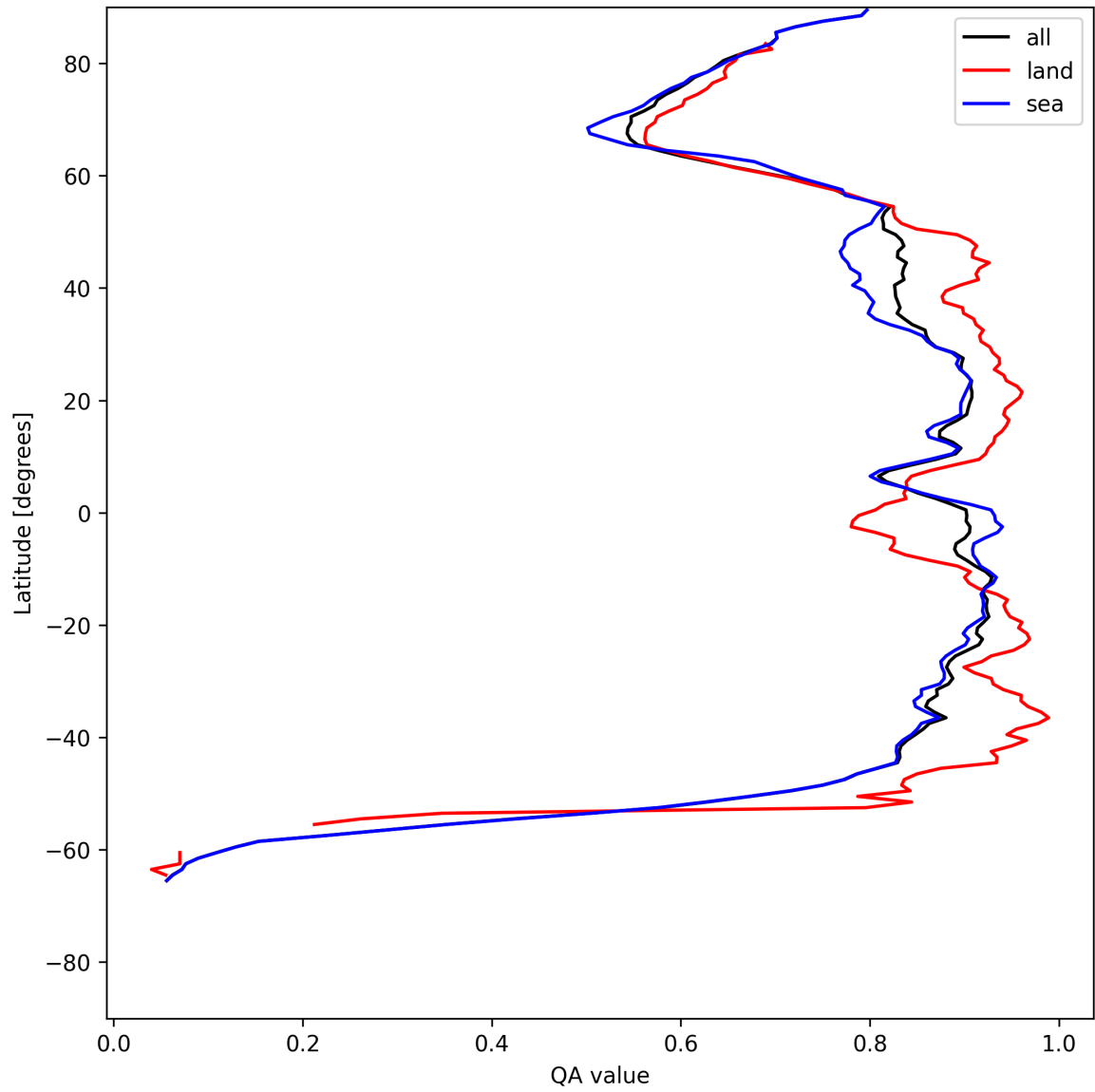
Figure 11: Zonal average of “QA value” for 2025-05-31 to 2025-06-01.
