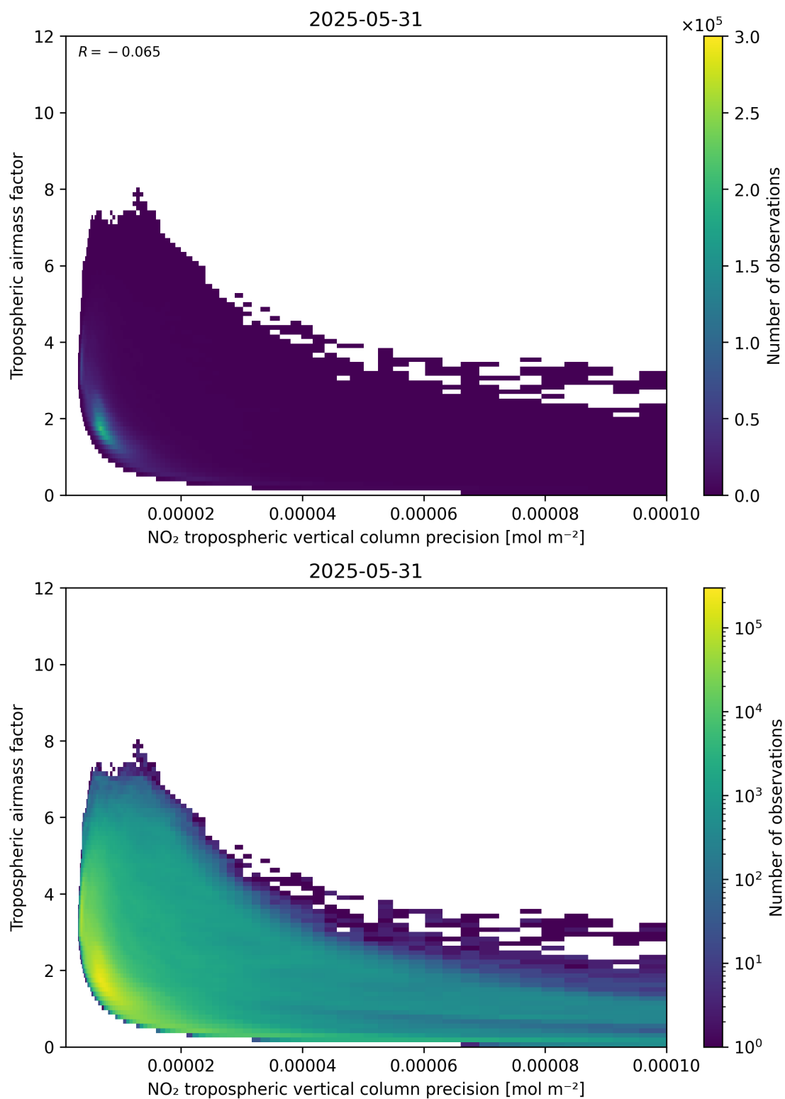
Figure 133: Scatter density plot of “NO 2 tropospheric vertical column precision” against “Tropospheric airmass factor” for 2025-05-31 to 2025-06-01.
