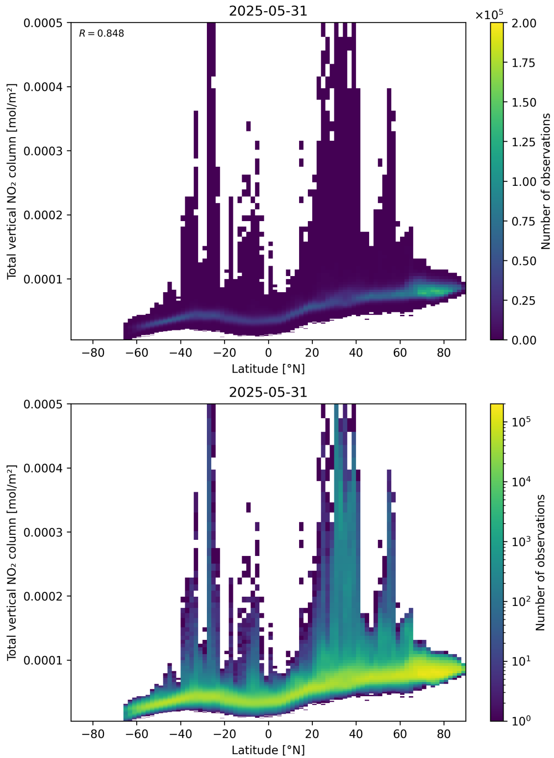
Figure 90: Scatter density plot of “Latitude” against “Total vertical NO 2 column” for 2025-05-31 to 2025-06-01.
