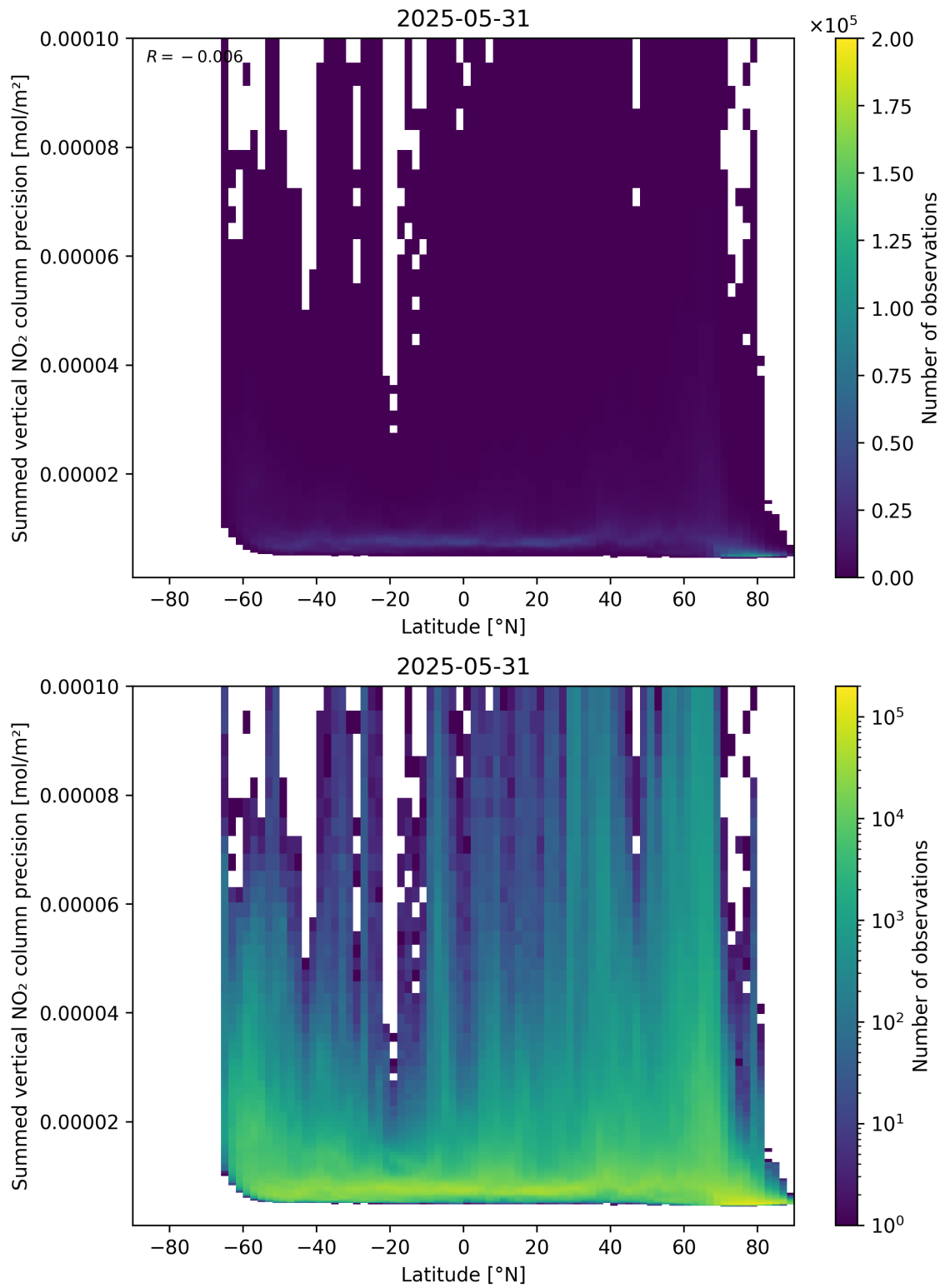
Figure 89: Scatter density plot of “Latitude” against “Summed vertical NO 2 column precision” for 2025-05-31 to 2025-06-01.
