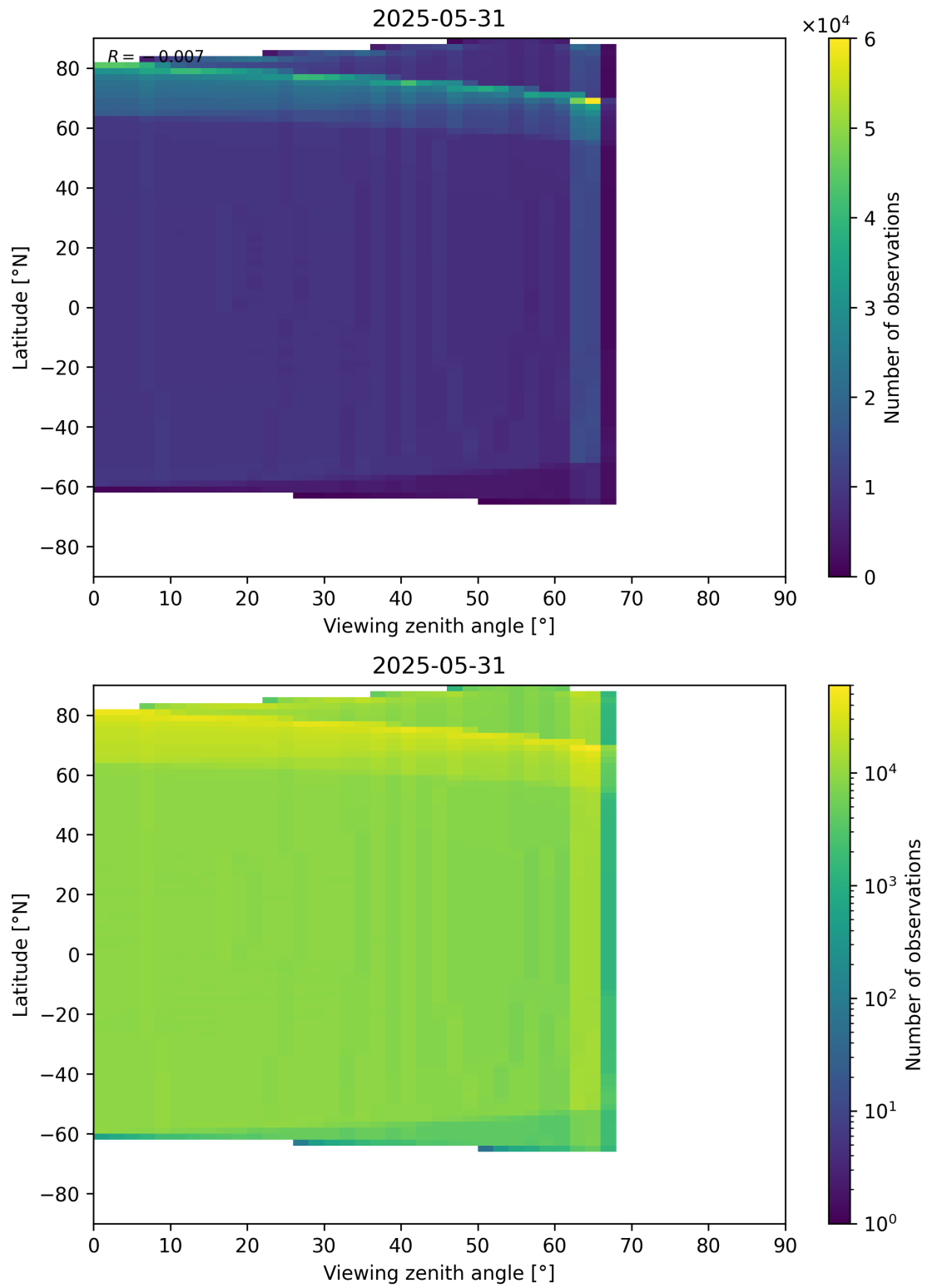
Figure 163: Scatter density plot of “Viewing zenith angle” against “Latitude” for 2025-05-31 to 2025-06-01.
