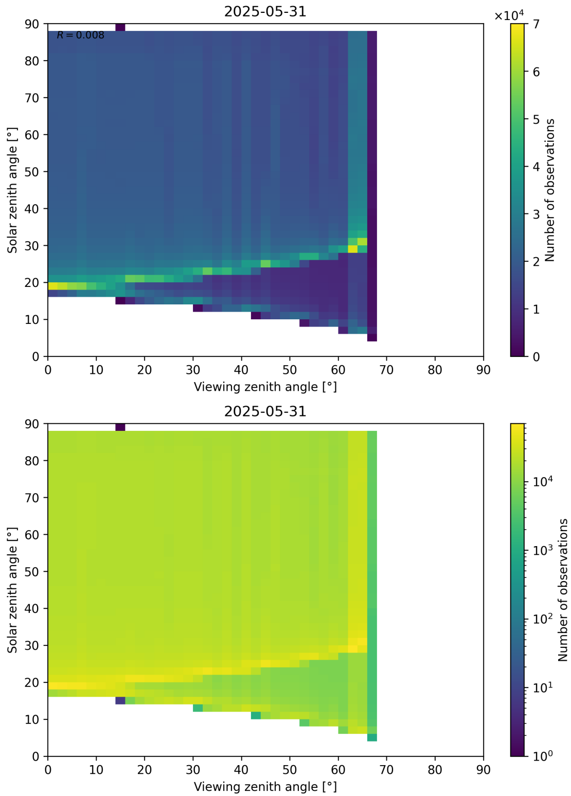
Figure 172: Scatter density plot of “Viewing zenith angle” against “Solar zenith angle” for 2025-05-31 to 2025-06-01.
