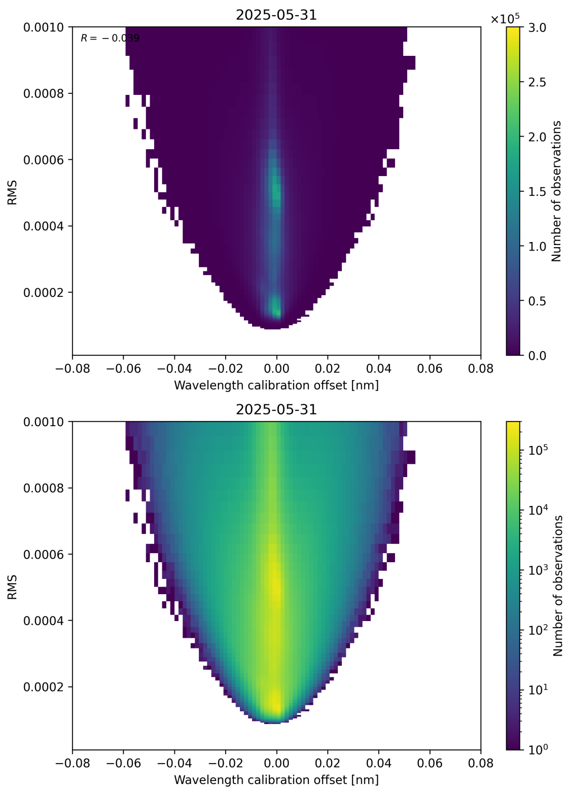
Figure 181: Scatter density plot of “Wavelength calibration offset” against “RMS” for 2025-05-31 to 2025-06-01.
