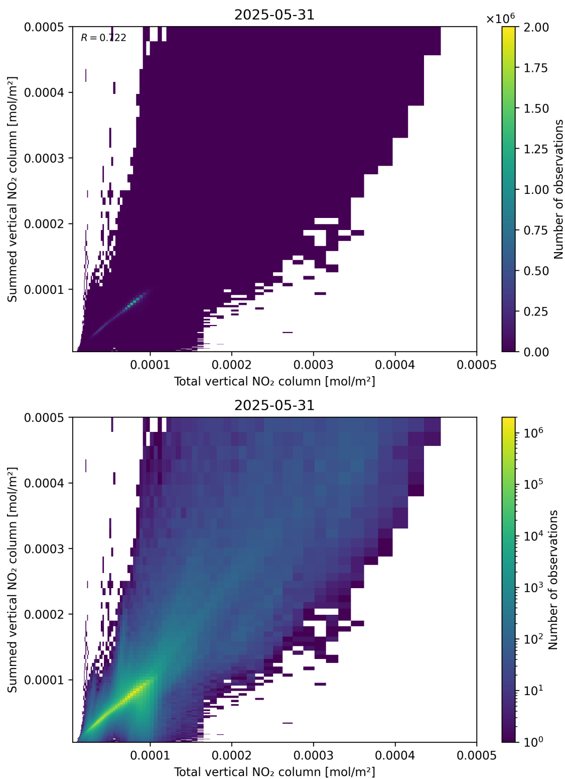
Figure 112: Scatter density plot of “Total vertical NO 2 column” against “Summed vertical NO 2 column” for 2025-05-31 to 2025-06-01.
