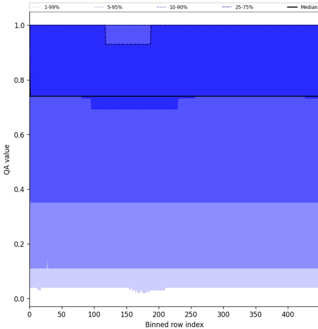
Figure 45: Along track statistics of “QA value” for 2025-05-31 to 2025-06-01
