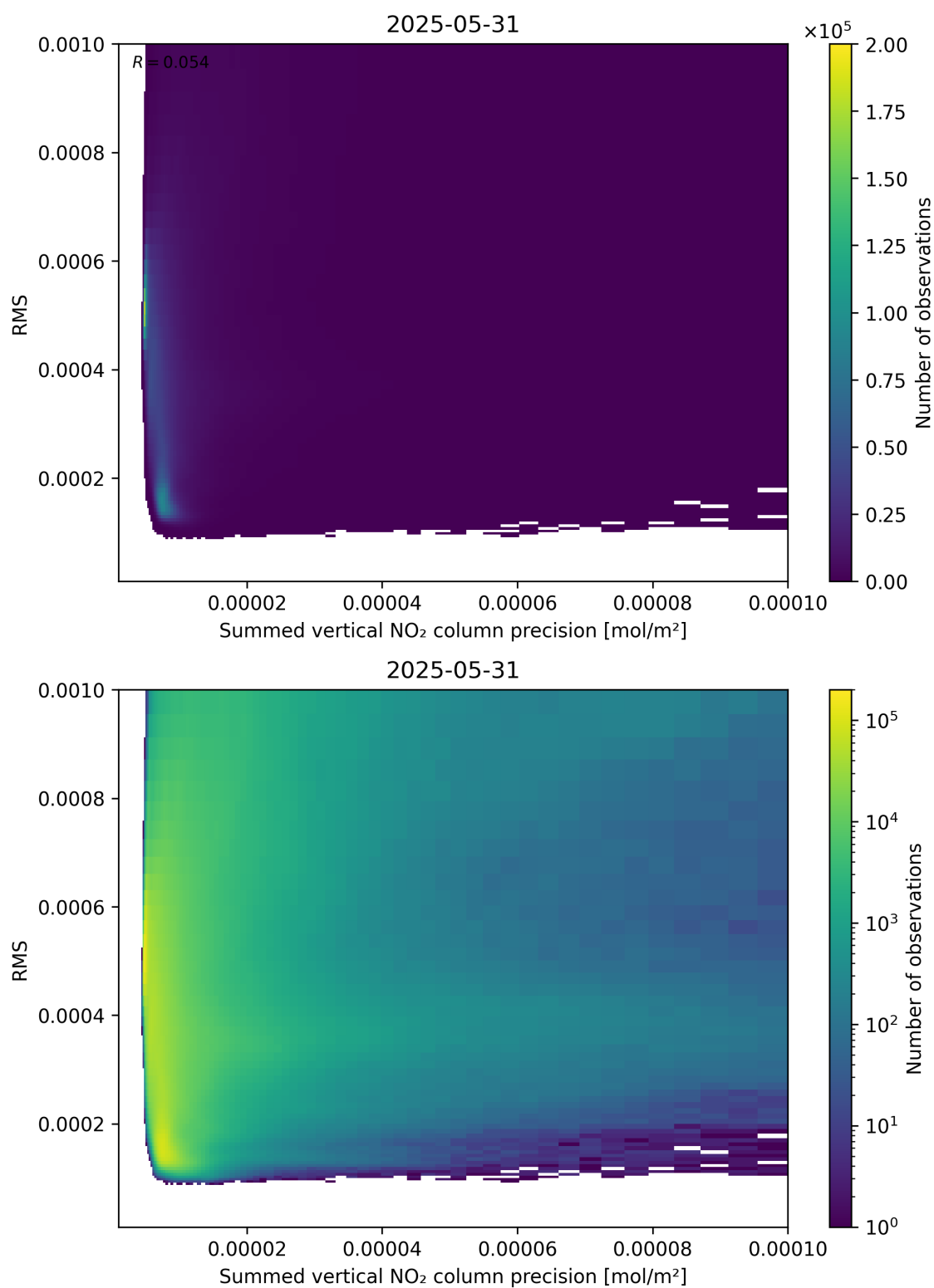
Figure 108: Scatter density plot of “Summed vertical NO 2 column precision” against “RMS” for 2025-05-31 to 2025-06-01.
