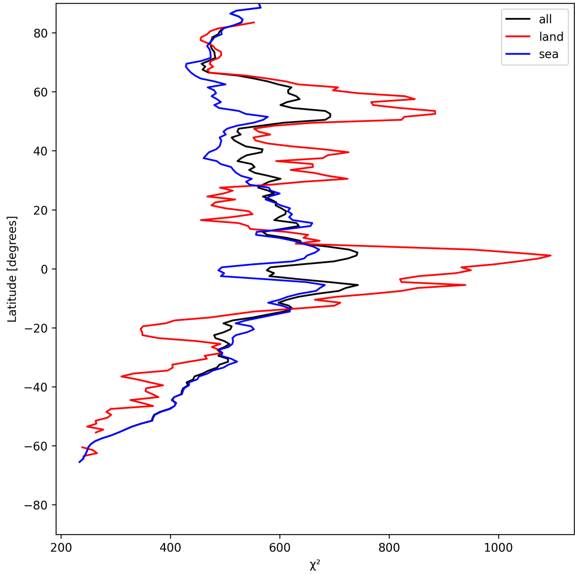
Figure 25: Zonal average of “ \chi^2 ” for 2025-05-31 to 2025-06-01.
