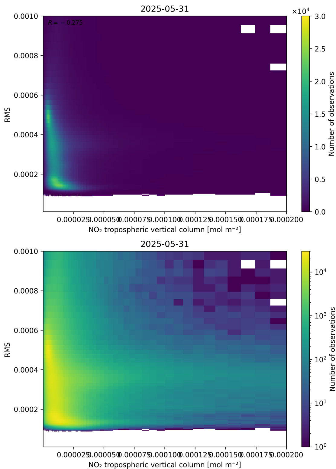
Figure 142: Scatter density plot of “NO 2 tropospheric vertical column” against “RMS” for 2025-05-31 to 2025-06-01.
