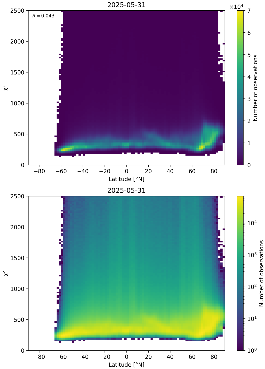
Figure 86: Scatter density plot of “Latitude” against “ \chi^2 ” for 2025-05-31 to 2025-06-01.
