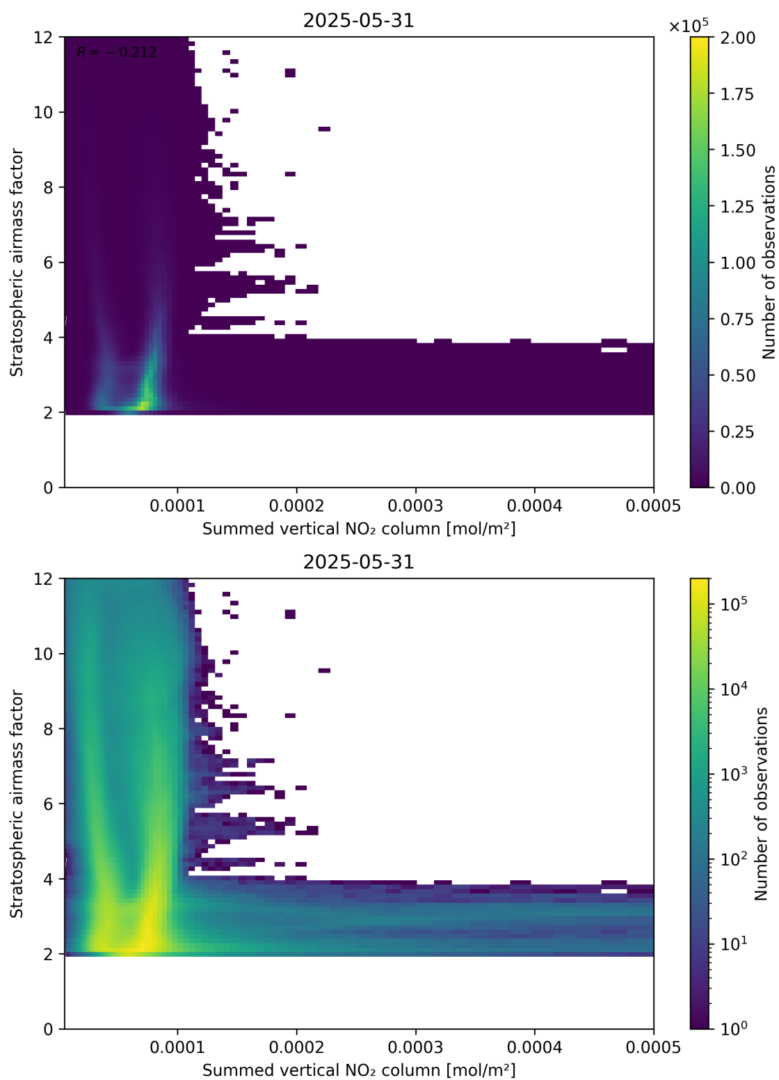
Figure 103: Scatter density plot of “Summed vertical NO 2 column” against “Stratospheric airmass factor” for 2025-05-31 to 2025-06-01.
