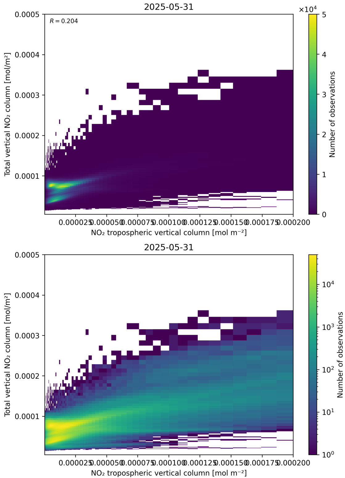
Figure 128: Scatter density plot of “NO 2 tropospheric vertical column” against “Total vertical NO 2 column” for 2025-05-31 to 2025-06-01.
