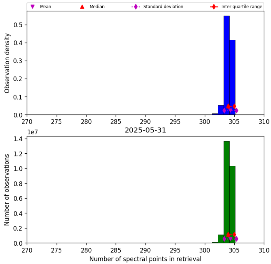
Figure 33: Histogram of “Number of spectral points in retrieval” for 2025-05-31 to 2025-06-01
