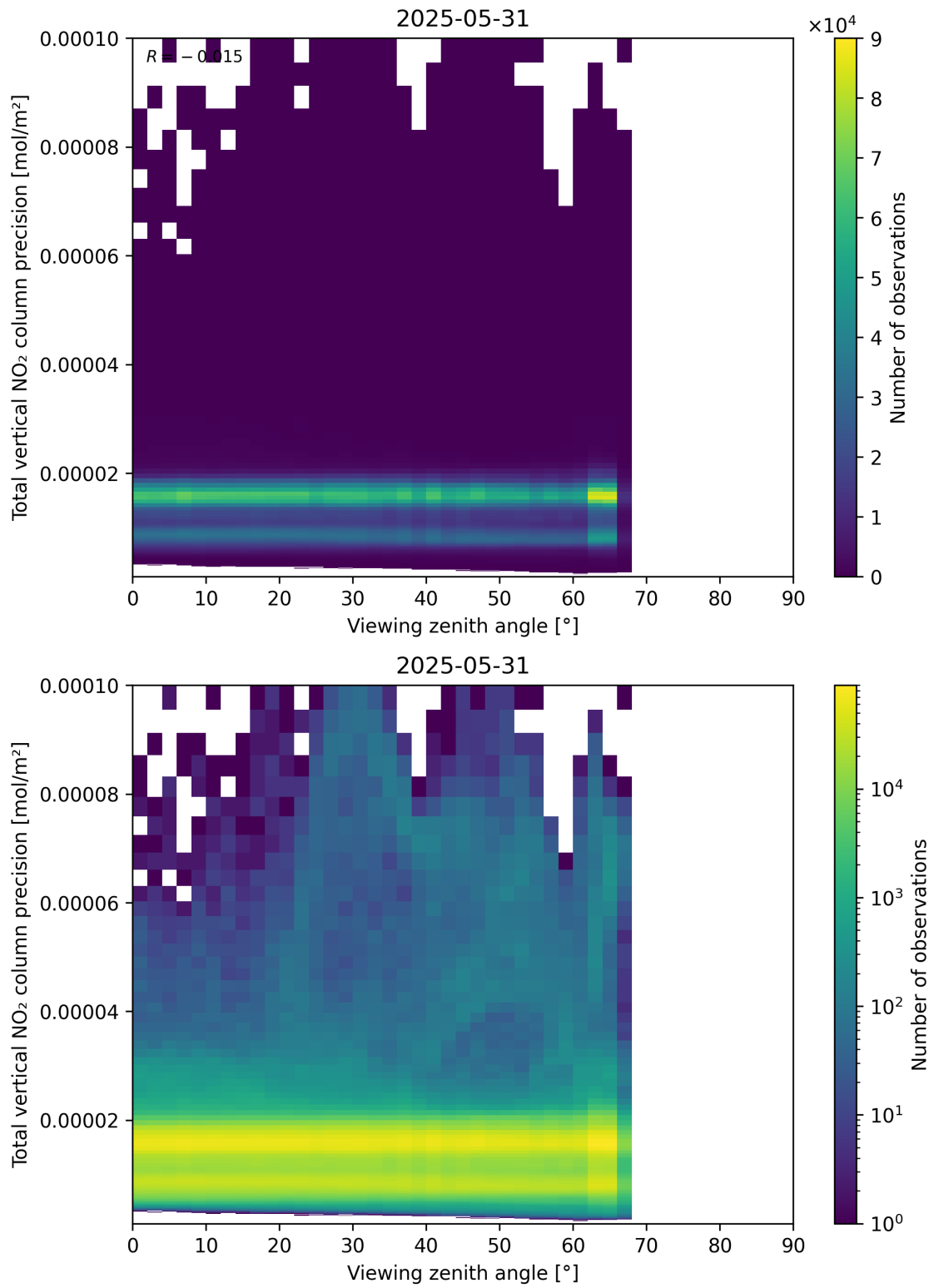
Figure 168: Scatter density plot of “Viewing zenith angle” against “Total vertical NO 2 column precision” for 2025-05-31 to 2025-06-01.
