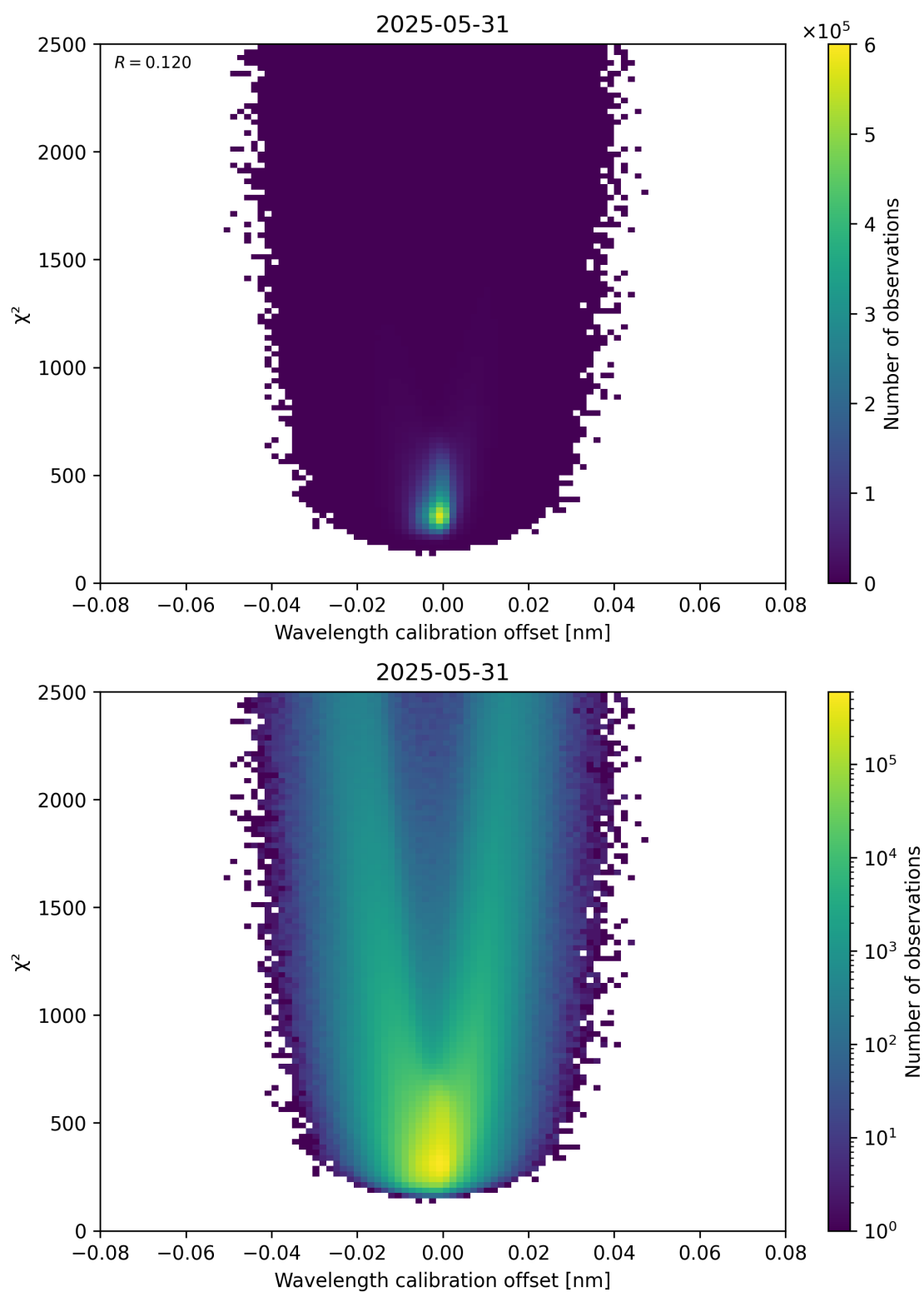
Figure 175: Scatter density plot of “Wavelength calibration offset” against “ \chi^2 ” for 2025-05-31 to 2025-06-01.
