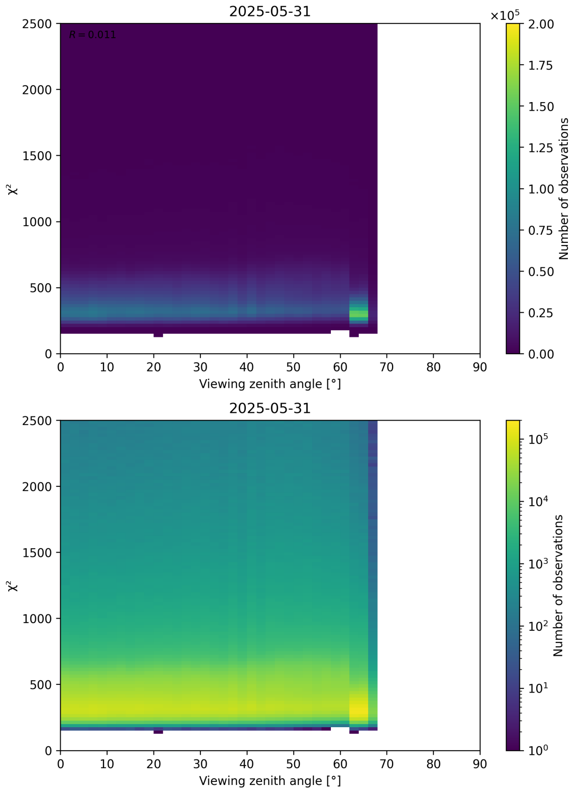
Figure 162: Scatter density plot of “Viewing zenith angle” against “ \chi^2 ” for 2025-05-31 to 2025-06-01.
