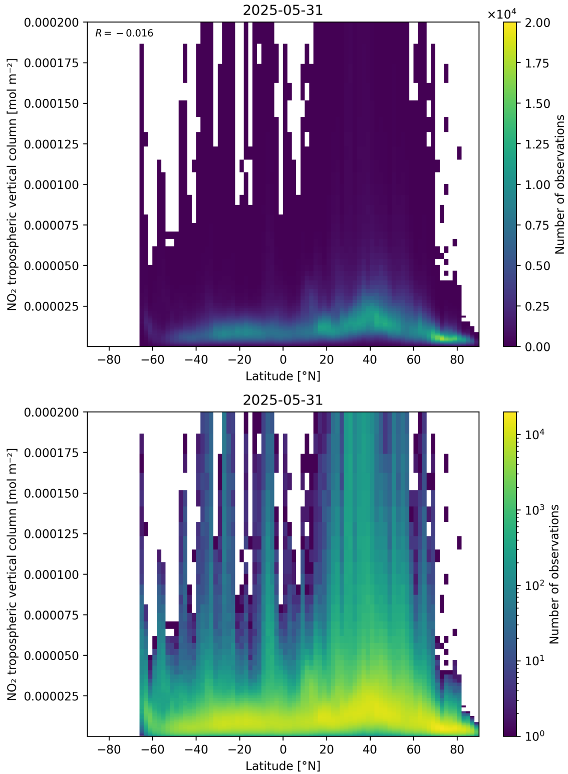
Figure 92: Scatter density plot of “Latitude” against “NO 2 tropospheric vertical column” for 2025-05-31 to 2025-06-01.
