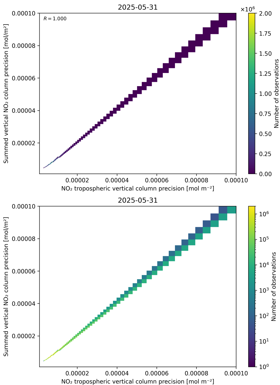
Figure 137: Scatter density plot of “NO 2 tropospheric vertical column precision” against “Summed vertical NO 2 column precision” for 2025-05-31 to 2025-06-01.
