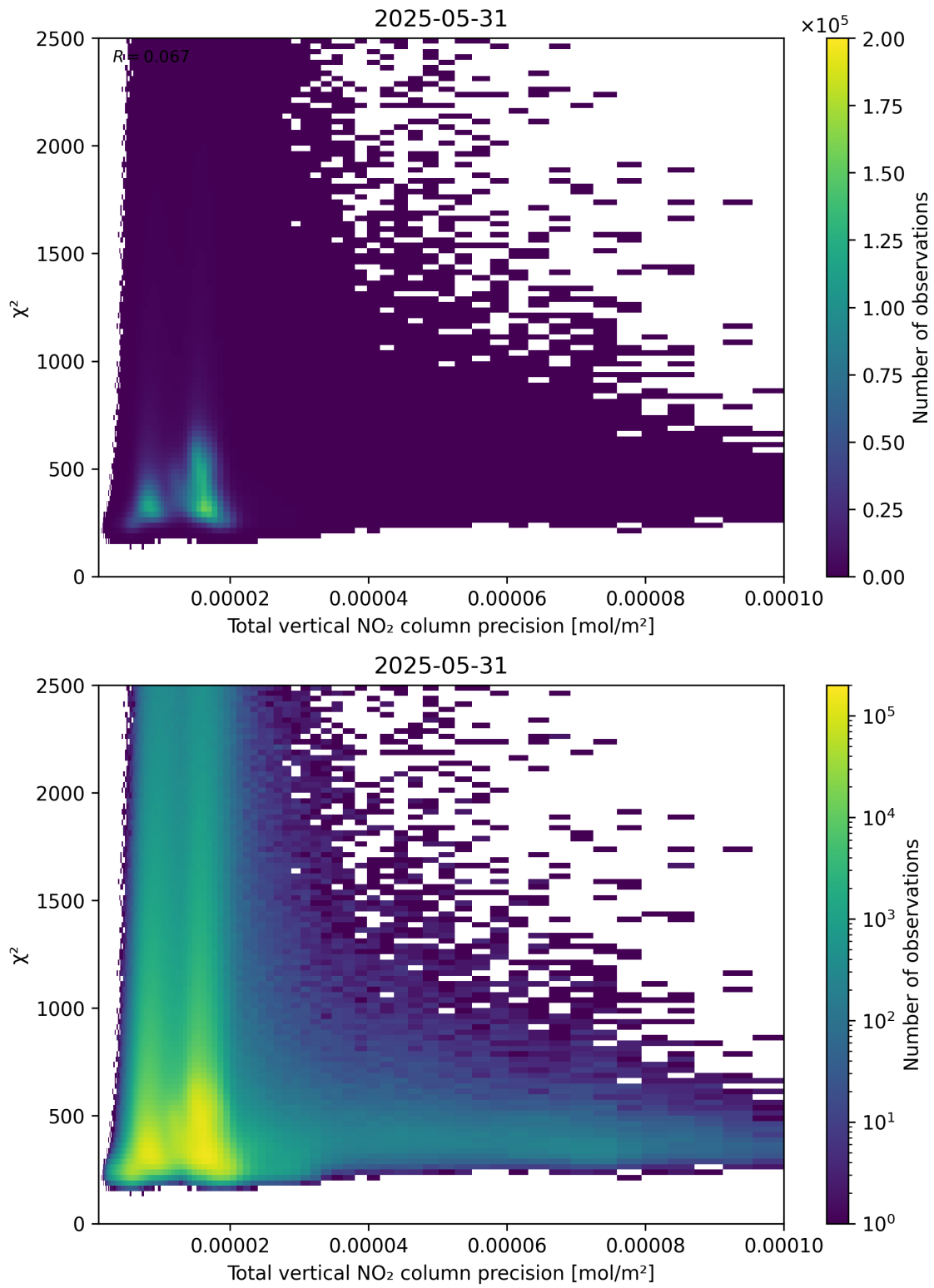
Figure 116: Scatter density plot of “Total vertical NO 2 column precision” against “ \chi^2 ” for 2025-05-31 to 2025-06-01.
