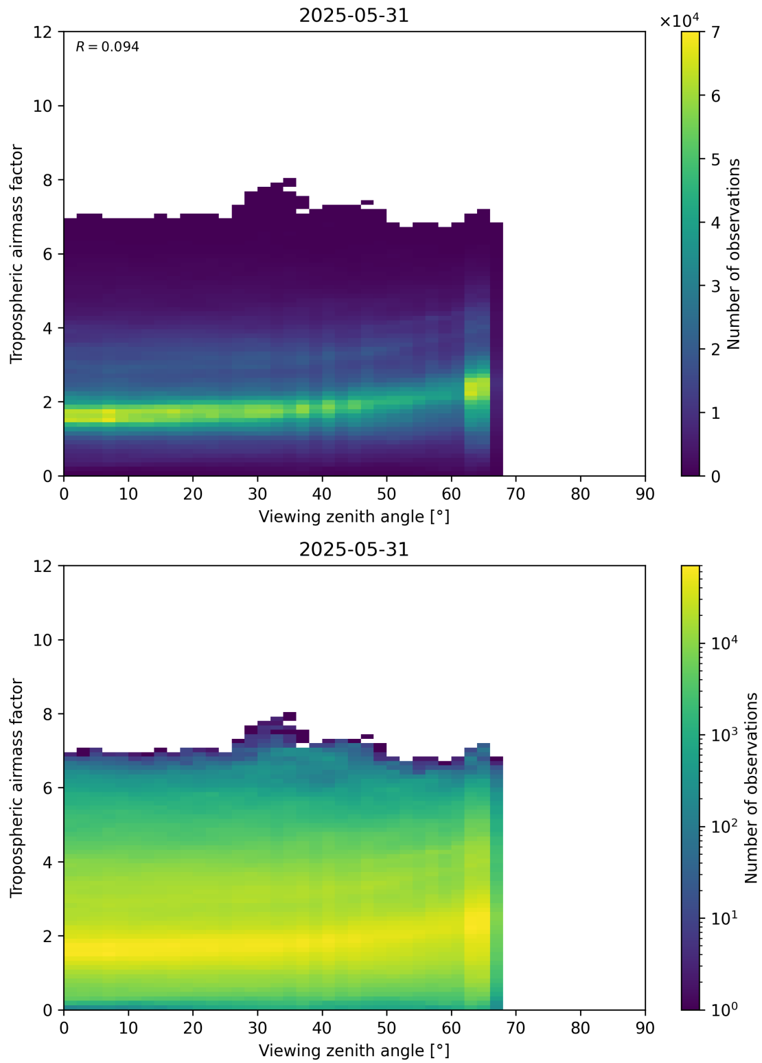
Figure 161: Scatter density plot of “Viewing zenith angle” against “Tropospheric airmass factor” for 2025-05-31 to 2025-06-01.
