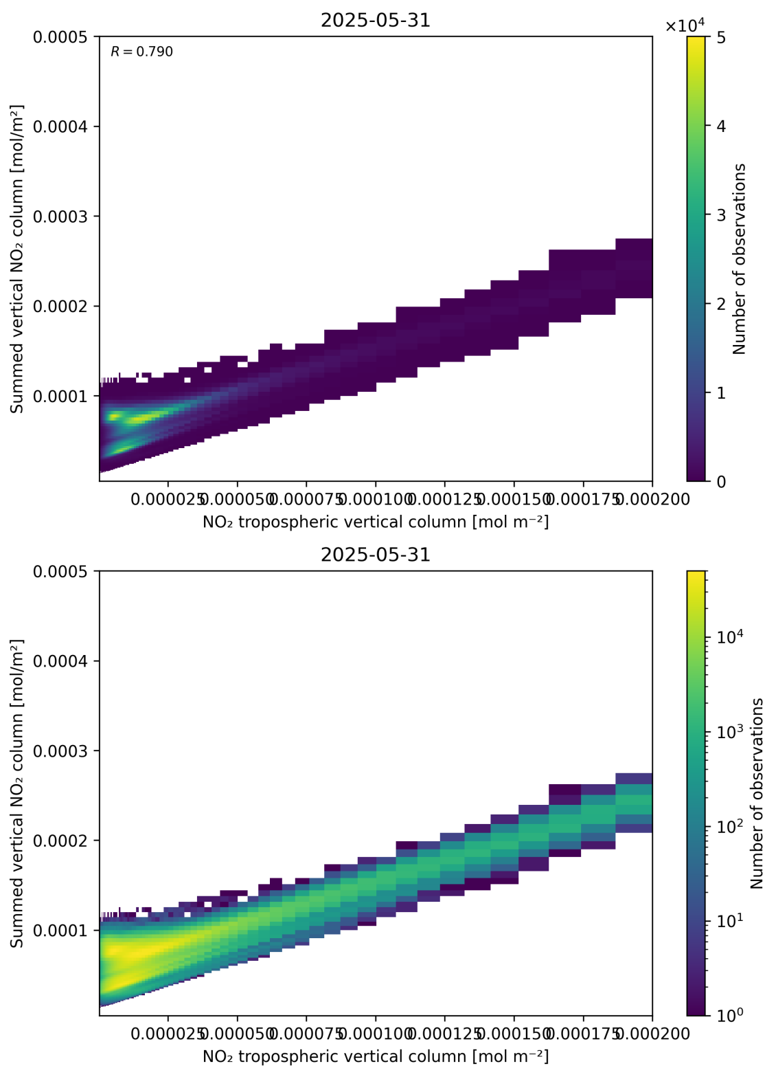
Figure 126: Scatter density plot of “NO 2 tropospheric vertical column” against “Summed vertical NO 2 column” for 2025-05-31 to 2025-06-01.
