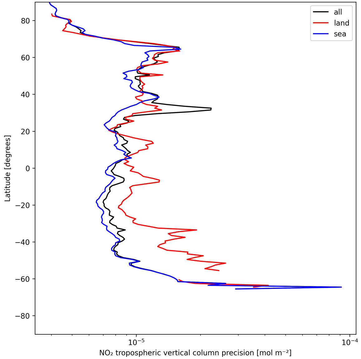
Figure 13: Zonal average of “NO 2 tropospheric vertical column precision” for 2025-05-31 to 2025-06-01.
