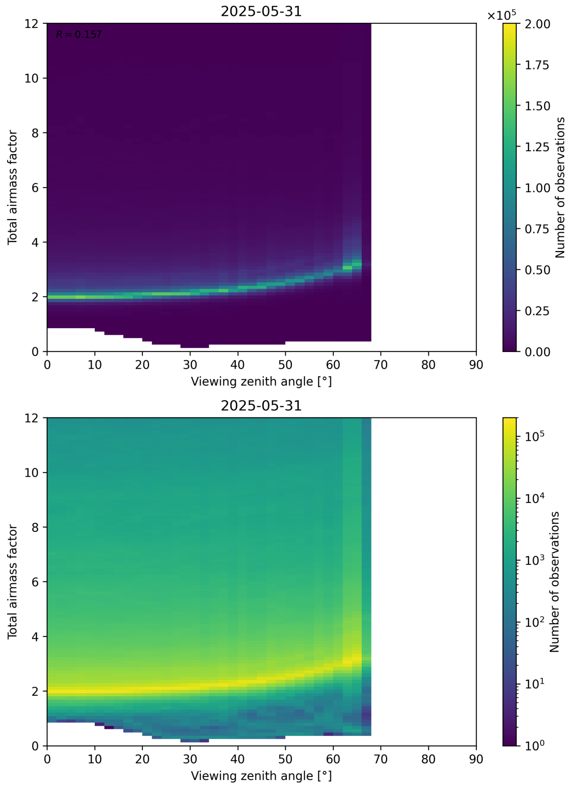
Figure 160: Scatter density plot of “Viewing zenith angle” against “Total airmass factor” for 2025-05-31 to 2025-06-01.
