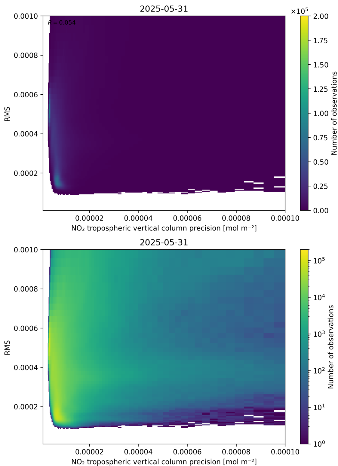
Figure 140: Scatter density plot of “NO 2 tropospheric vertical column precision” against “RMS” for 2025-05-31 to 2025-06-01.
