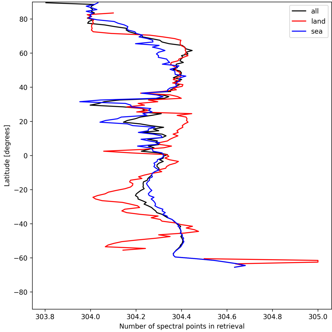
Figure 16: Zonal average of “Number of spectral points in retrieval” for 2025-05-31 to 2025-06-01.
