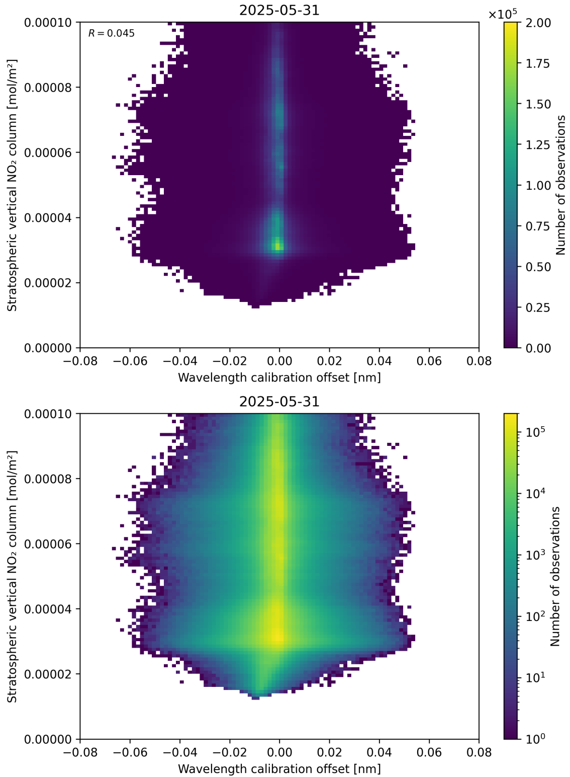
Figure 176: Scatter density plot of “Wavelength calibration offset” against “Stratospheric vertical NO 2 column” for 2025-05-31 to 2025-06-01.
