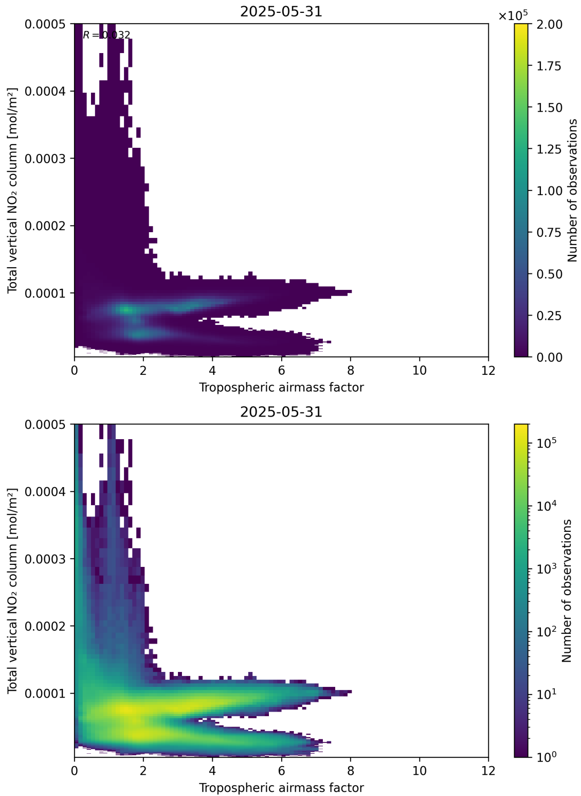
Figure 77: Scatter density plot of “Tropospheric airmass factor” against “Total vertical NO 2 column” for 2025-05-31 to 2025-06-01.
