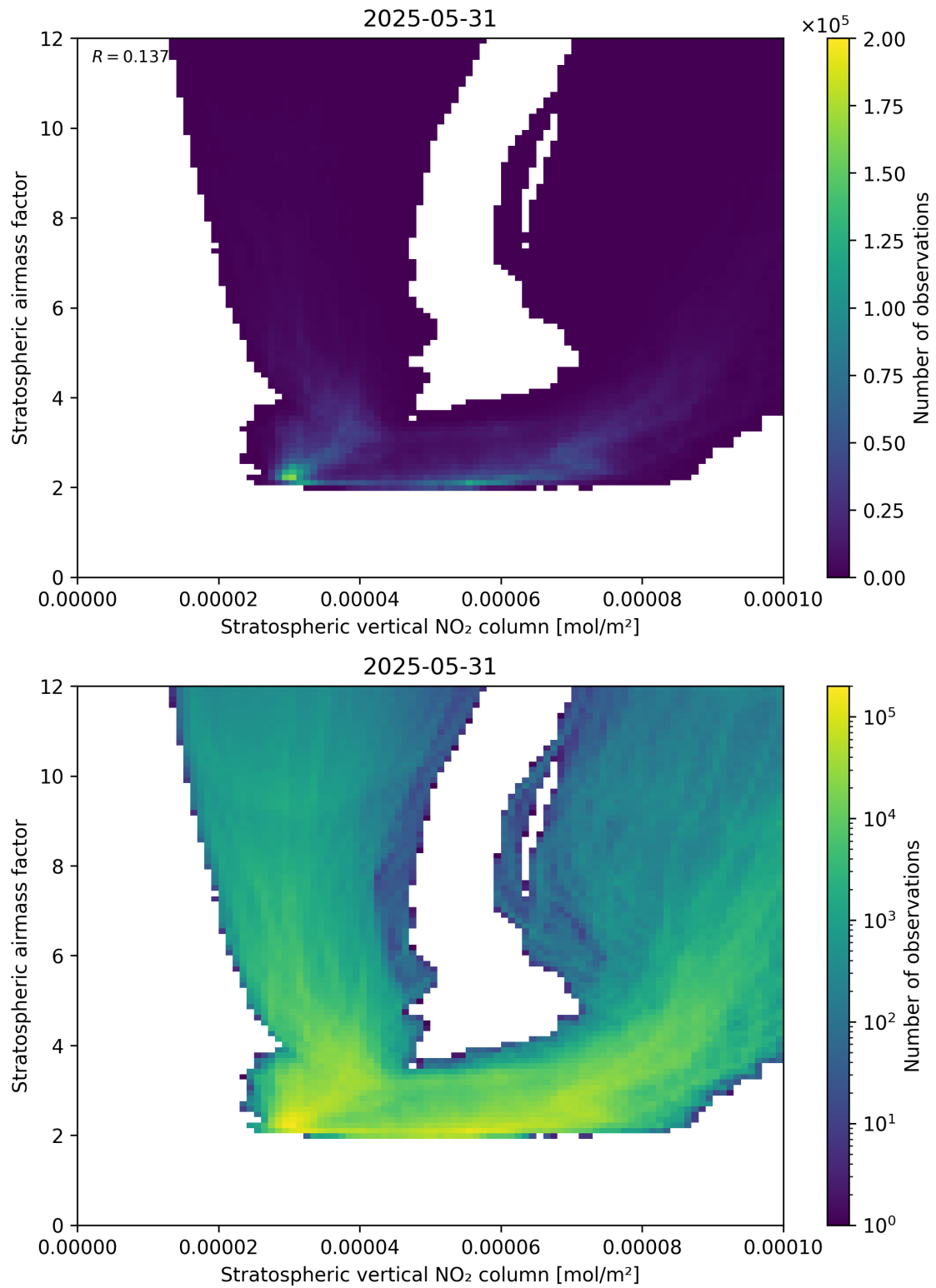
Figure 96: Scatter density plot of “Stratospheric vertical NO 2 column” against “Stratospheric airmass factor” for 2025-05-31 to 2025-06-01.
