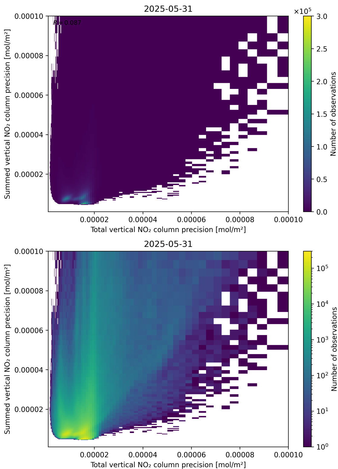
Figure 118: Scatter density plot of “Total vertical NO 2 column precision” against “Summed vertical NO 2 column precision” for 2025-05-31 to 2025-06-01.
