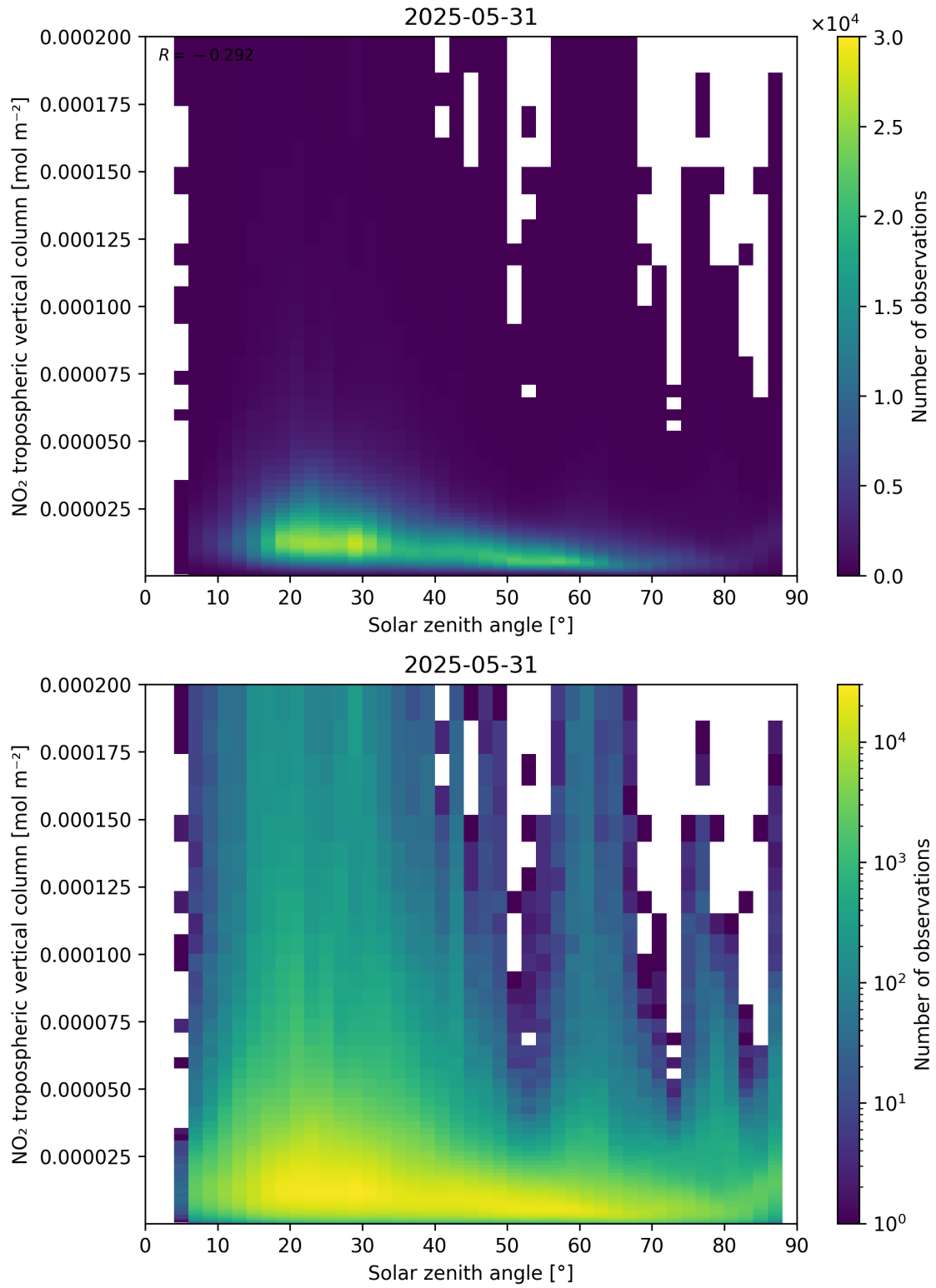
Figure 155: Scatter density plot of “Solar zenith angle” against “NO 2 tropospheric vertical column” for 2025-05-31 to 2025-06-01.
