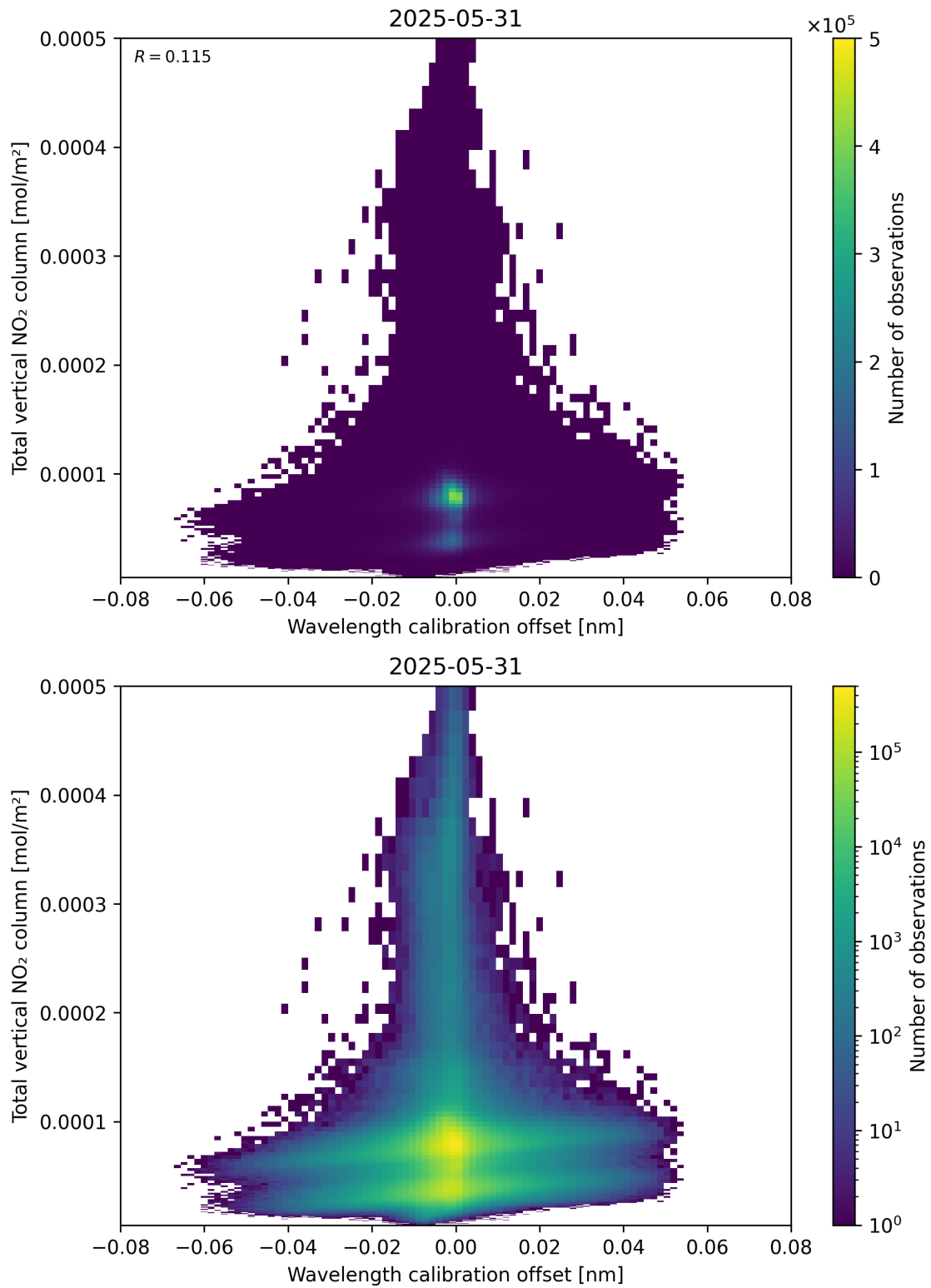
Figure 179: Scatter density plot of “Wavelength calibration offset” against “Total vertical NO 2 column” for 2025-05-31 to 2025-06-01.
