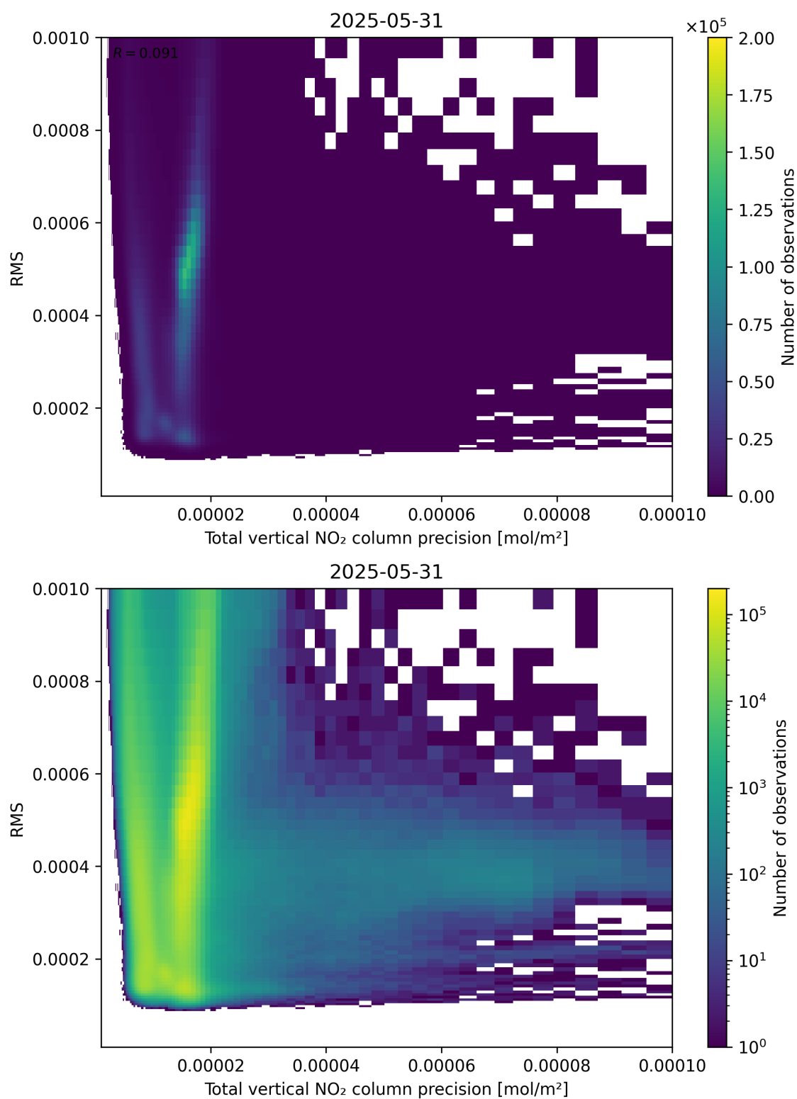
Figure 119: Scatter density plot of “Total vertical NO 2 column precision” against “RMS” for 2025-05-31 to 2025-06-01.
