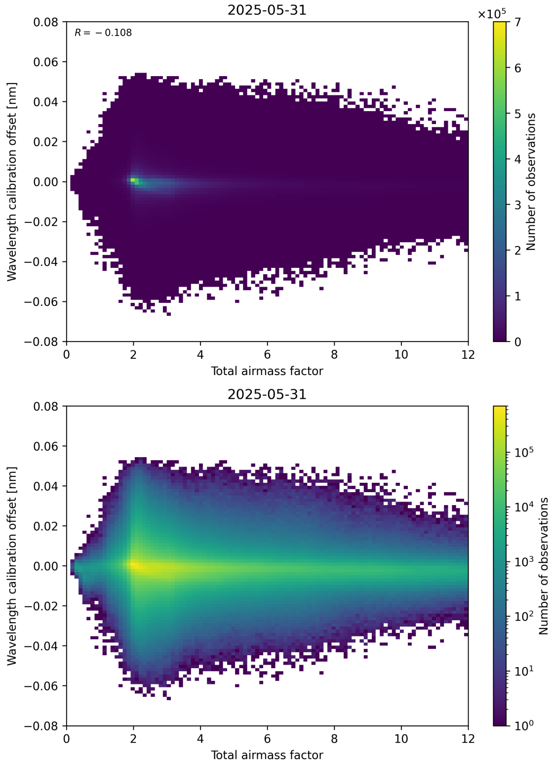
Figure 70: Scatter density plot of “Total airmass factor” against “Wavelength calibration offset” for 2025-05-31 to 2025-06-01.
