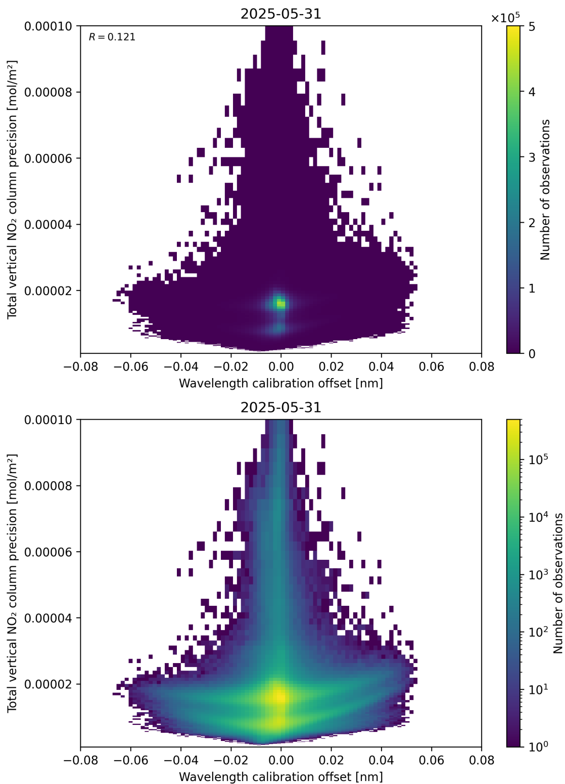
Figure 180: Scatter density plot of “Wavelength calibration offset” against “Total vertical NO 2 column precision” for 2025-05-31 to 2025-06-01.
