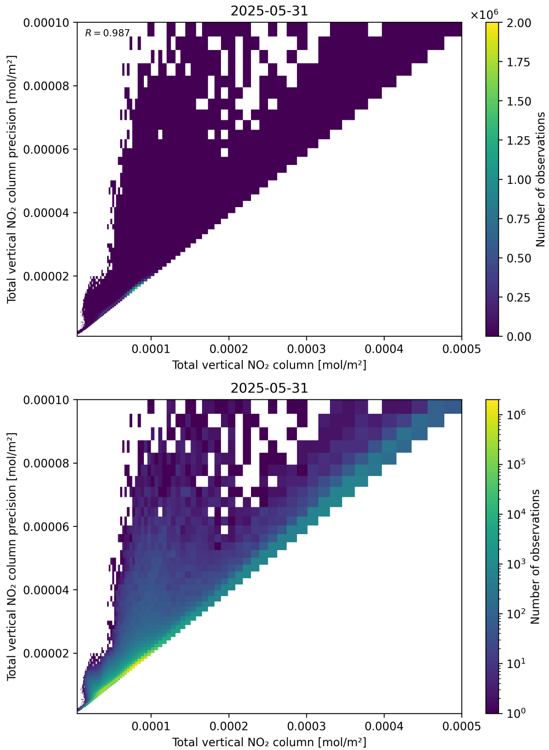
Figure 114: Scatter density plot of “Total vertical NO 2 column” against “Total vertical NO 2 column precision” for 2025-05-31 to 2025-06-01.
