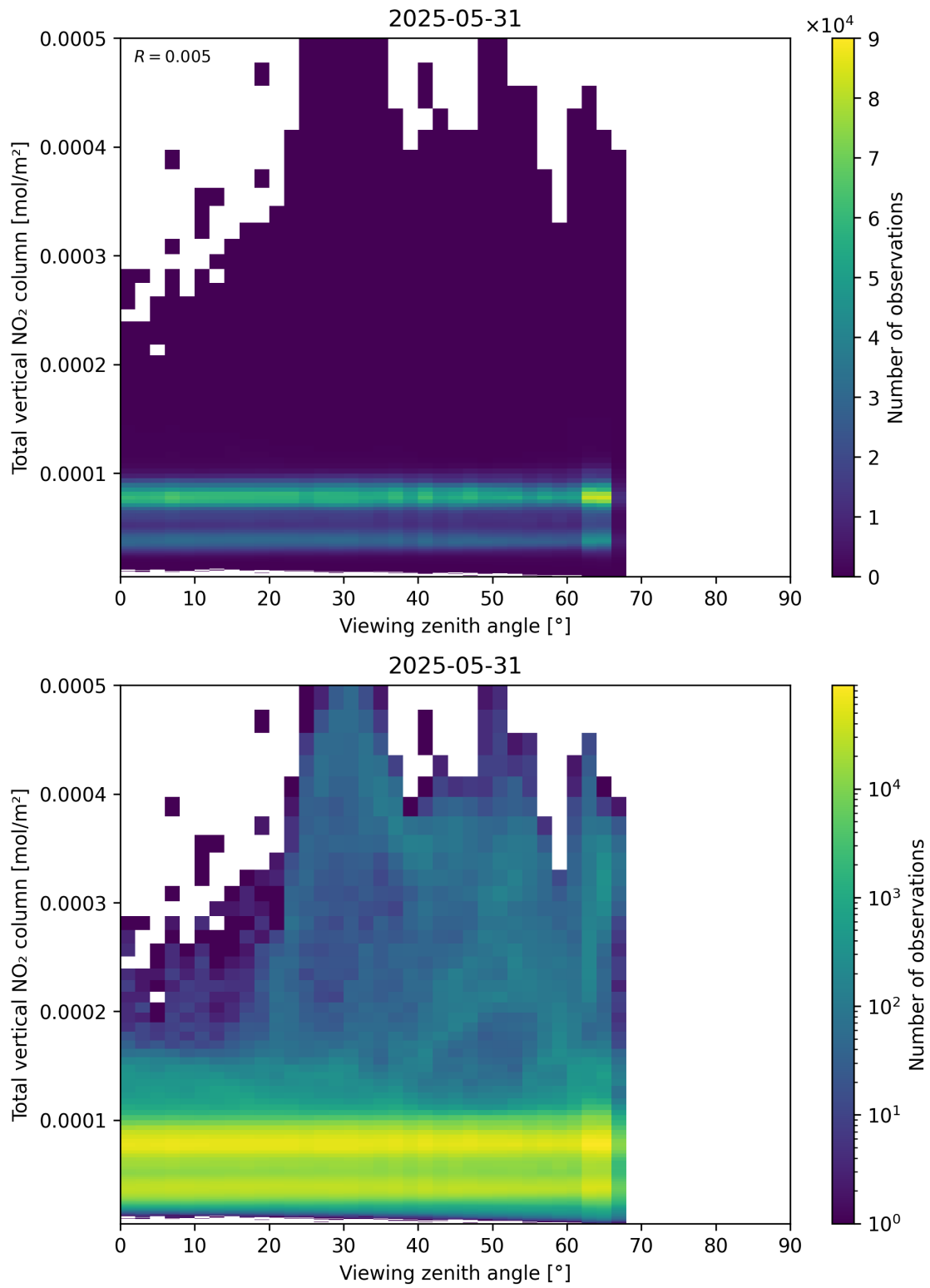
Figure 167: Scatter density plot of “Viewing zenith angle” against “Total vertical NO 2 column” for 2025-05-31 to 2025-06-01.
