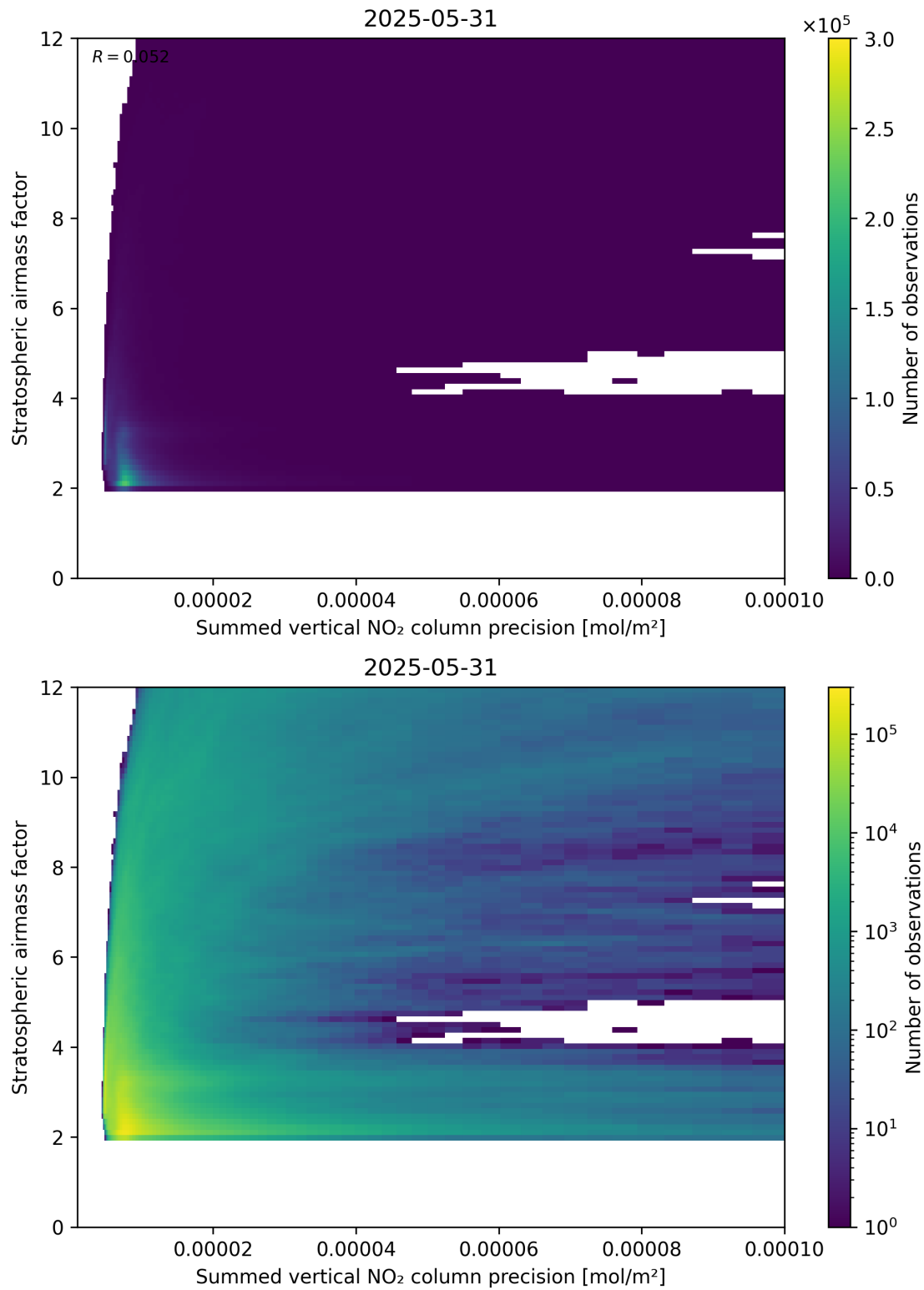
Figure 106: Scatter density plot of “Summed vertical NO 2 column precision” against “Stratospheric airmass factor” for 2025-05-31 to 2025-06-01.
