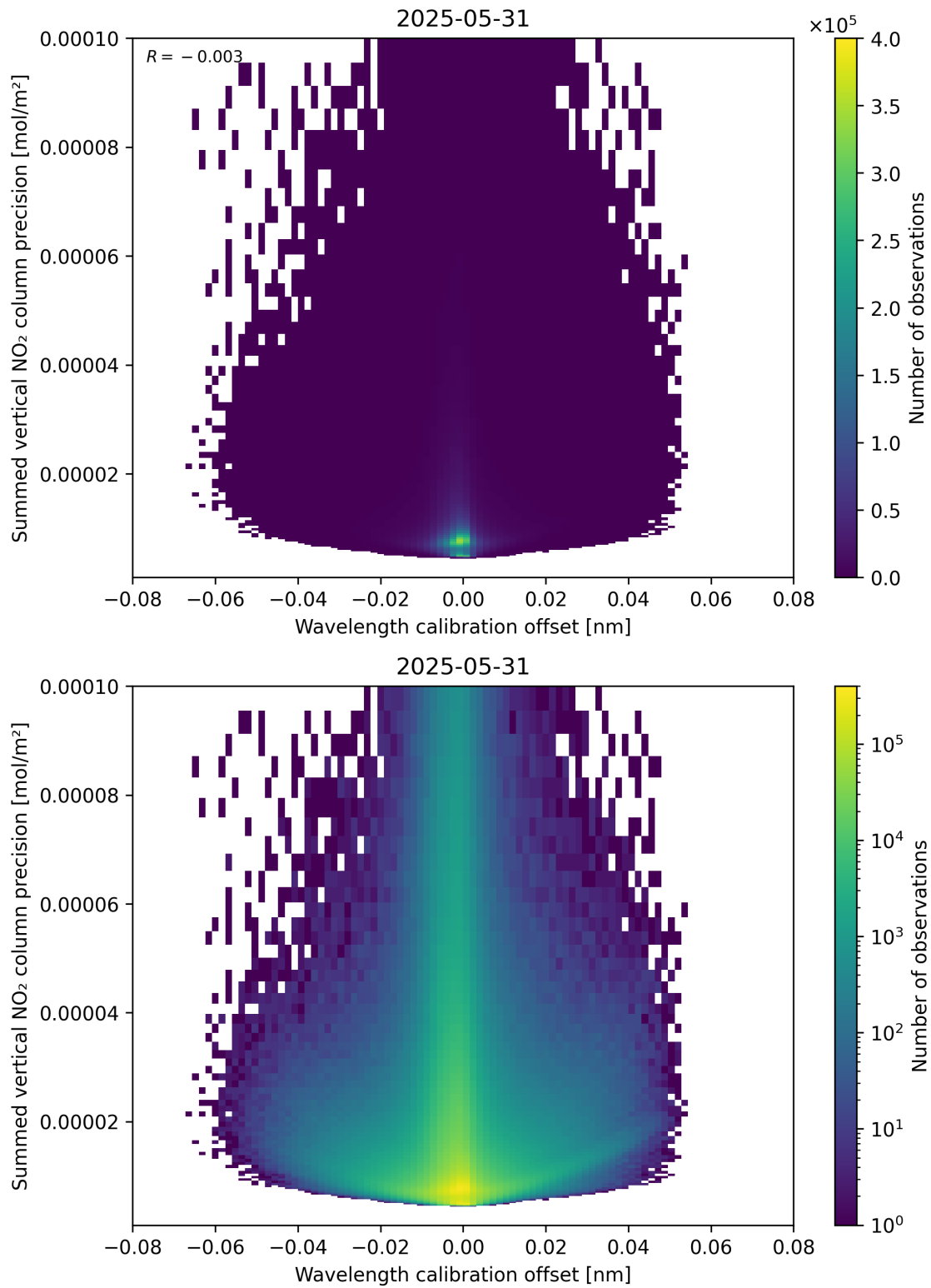
Figure 178: Scatter density plot of “Wavelength calibration offset” against “Summed vertical NO 2 column precision” for 2025-05-31 to 2025-06-01.
