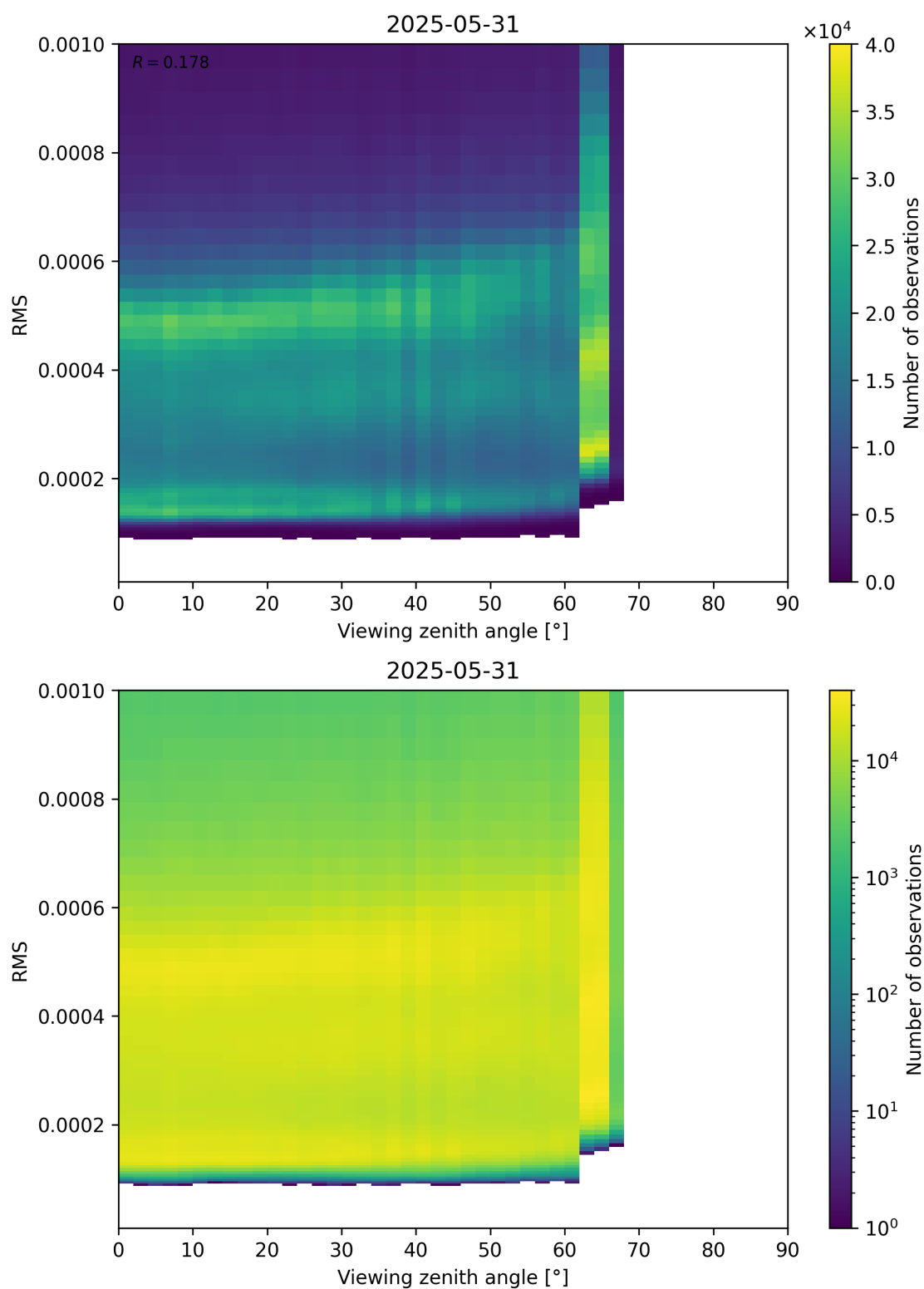
Figure 171: Scatter density plot of “Viewing zenith angle” against “RMS” for 2025-05-31 to 2025-06-01.
