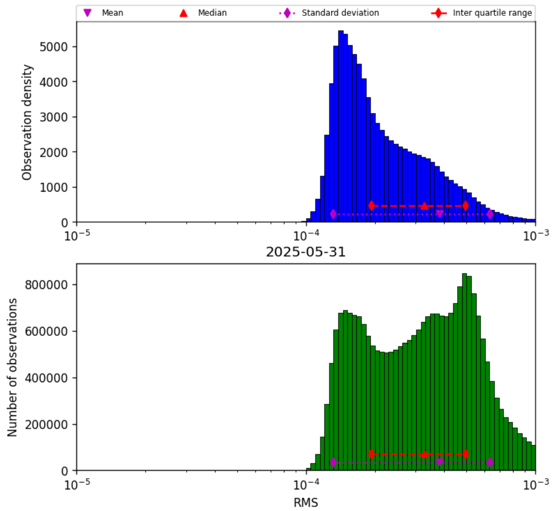
Figure 43: Histogram of “RMS” for 2025-05-31 to 2025-06-01
