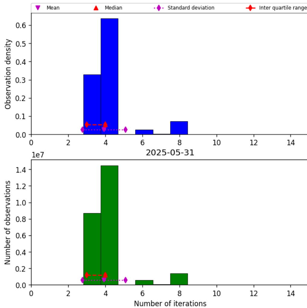
Figure 34: Histogram of “Number of iterations” for 2025-05-31 to 2025-06-01
