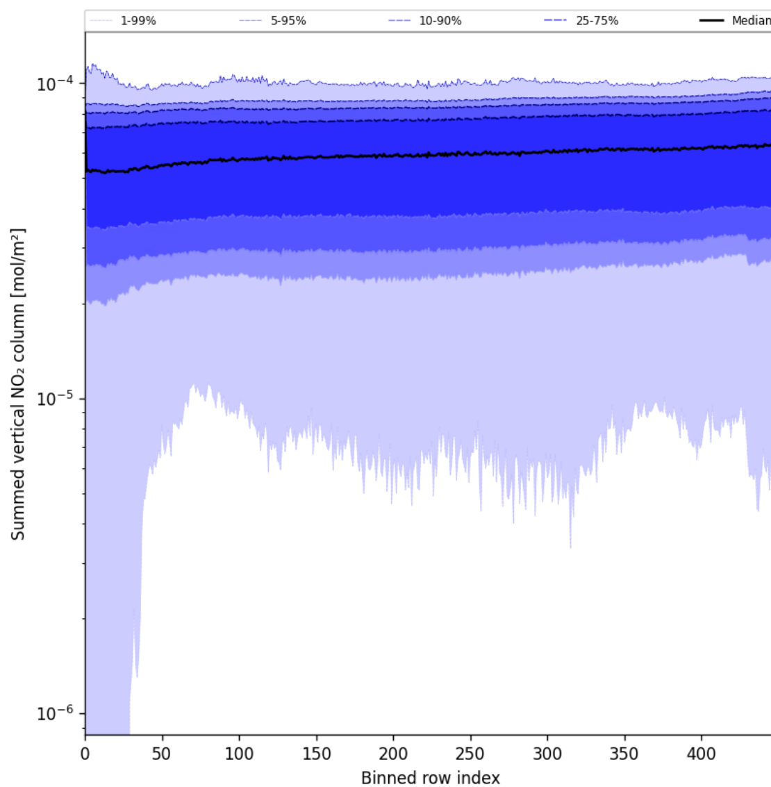
Figure 57: Along track statistics of “Summed vertical NO 2 column” for 2025-05-31 to 2025-06-01
