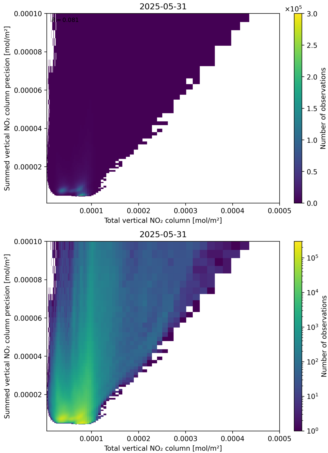
Figure 113: Scatter density plot of “Total vertical NO 2 column” against “Summed vertical NO 2 column precision” for 2025-05-31 to 2025-06-01.
