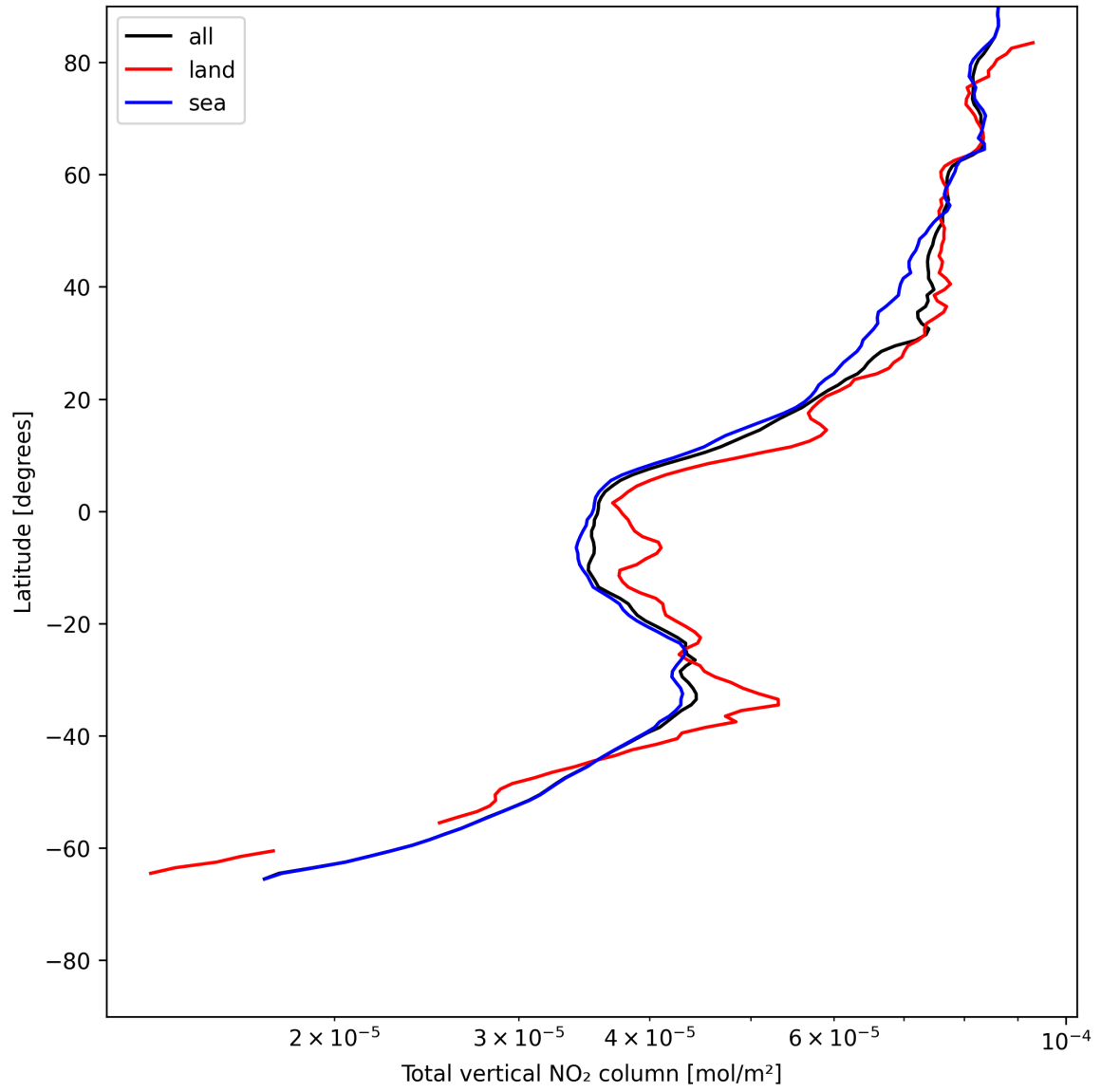
Figure 21: Zonal average of “Total vertical NO 2 column” for 2025-05-31 to 2025-06-01.
