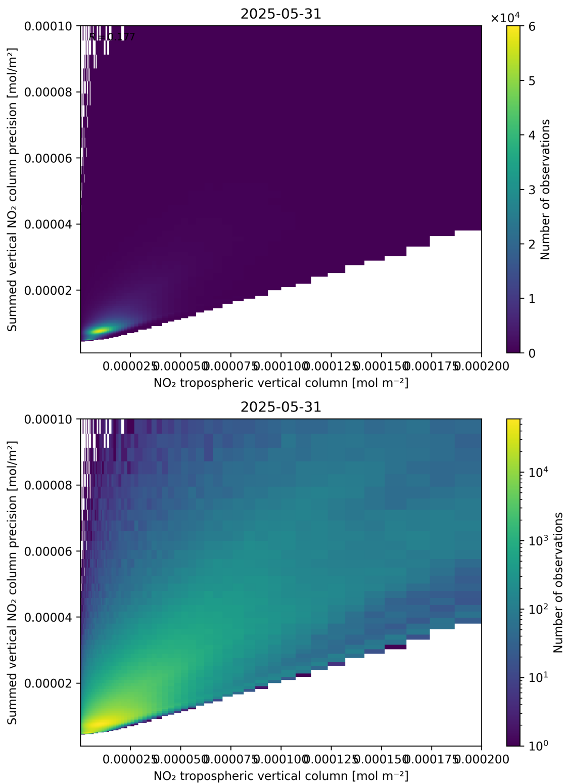
Figure 127: Scatter density plot of “NO 2 tropospheric vertical column” against “Summed vertical NO 2 column precision” for 2025-05-31 to 2025-06-01.
