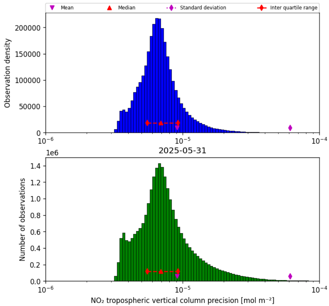
Figure 30: Histogram of “NO 2 tropospheric vertical column precision” for 2025-05-31 to 2025-06-01
