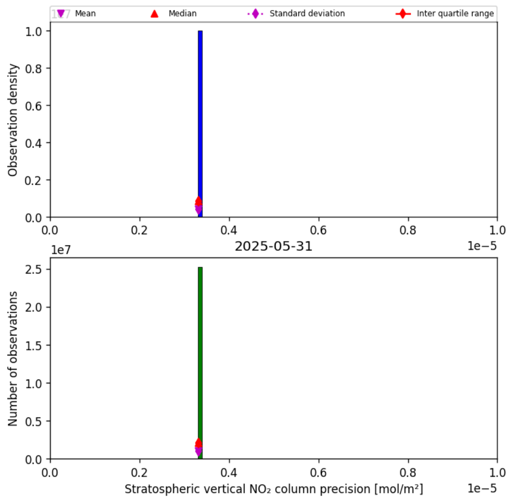
Figure 37: Histogram of “Stratospheric vertical NO 2 column precision” for 2025-05-31 to 2025-06-01
