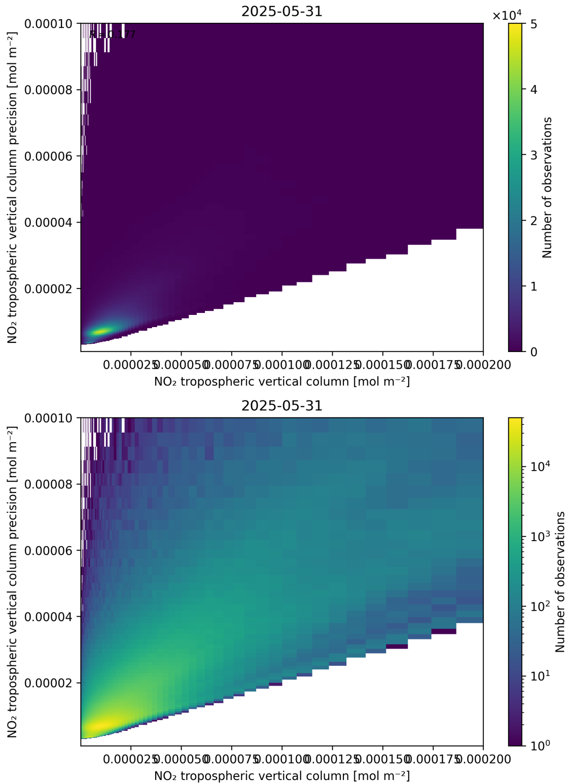
Figure 130: Scatter density plot of “NO 2 tropospheric vertical column” against “NO 2 tropospheric vertical column precision” for 2025-05-31 to 2025-06-01.
