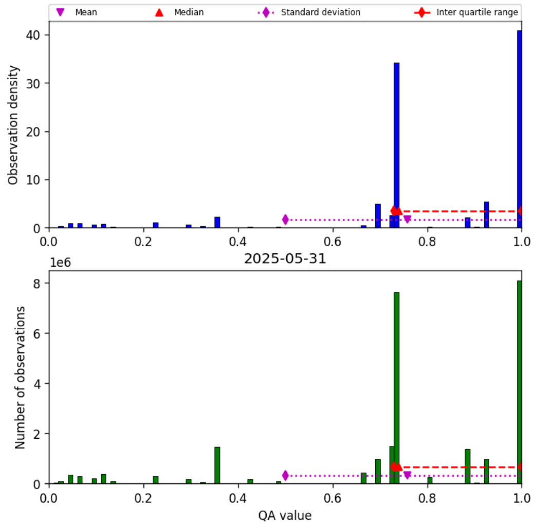
Figure 28: Histogram of “QA value” for 2025-05-31 to 2025-06-01
