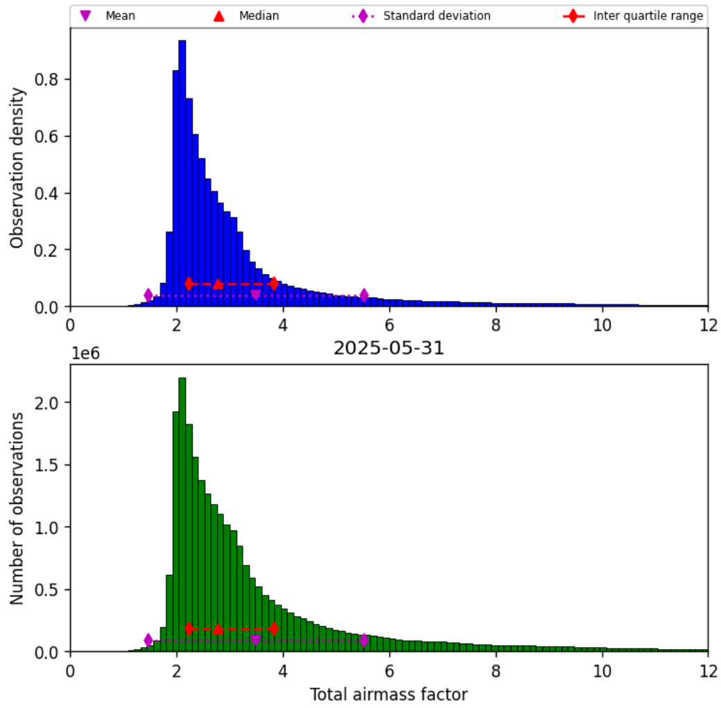
Figure 32: Histogram of “Total airmass factor” for 2025-05-31 to 2025-06-01
