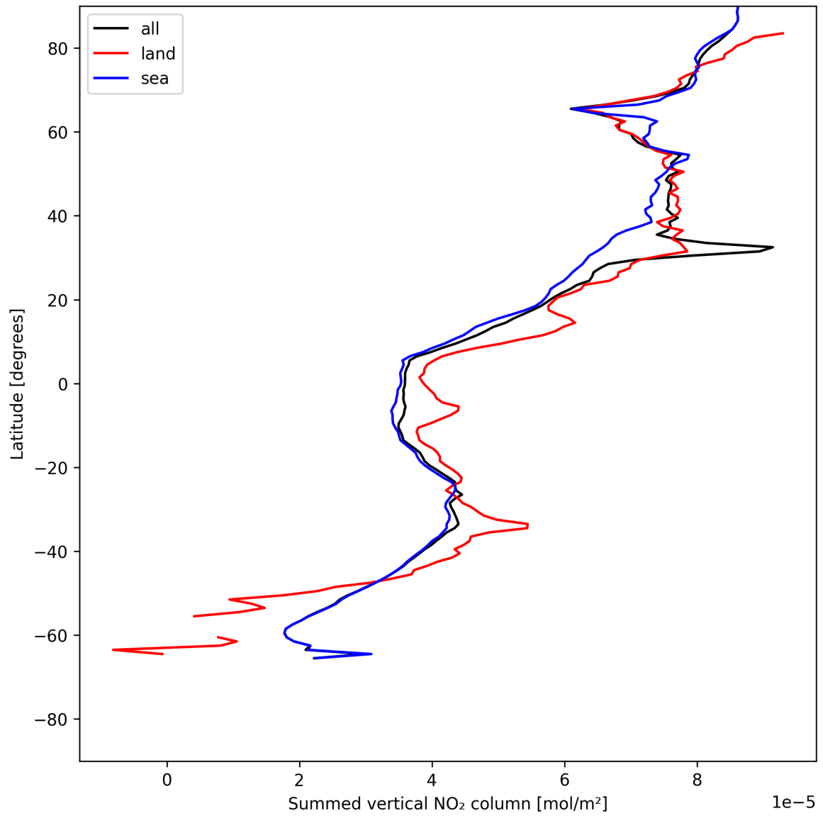
Figure 23: Zonal average of “Summed vertical NO 2 column” for 2025-05-31 to 2025-06-01.
