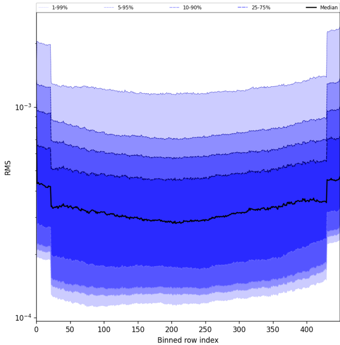
Figure 60: Along track statistics of “RMS” for 2025-05-31 to 2025-06-01
