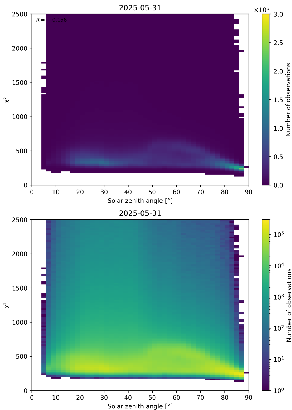
Figure 148: Scatter density plot of “Solar zenith angle” against “ \chi^2 ” for 2025-05-31 to 2025-06-01.
