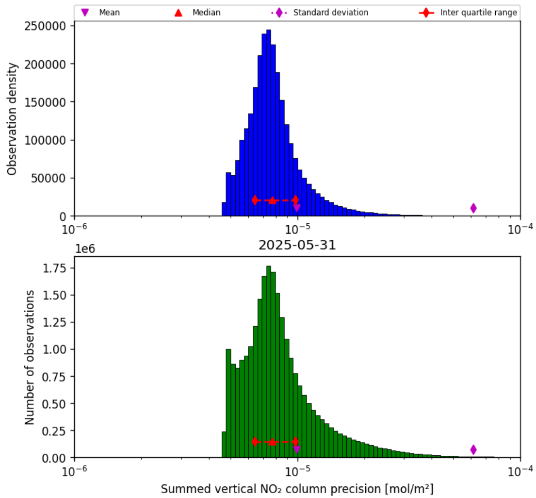
Figure 41: Histogram of "Summed vertical NO 2 column precision" for 2025-05-31 to 2025-06-01
