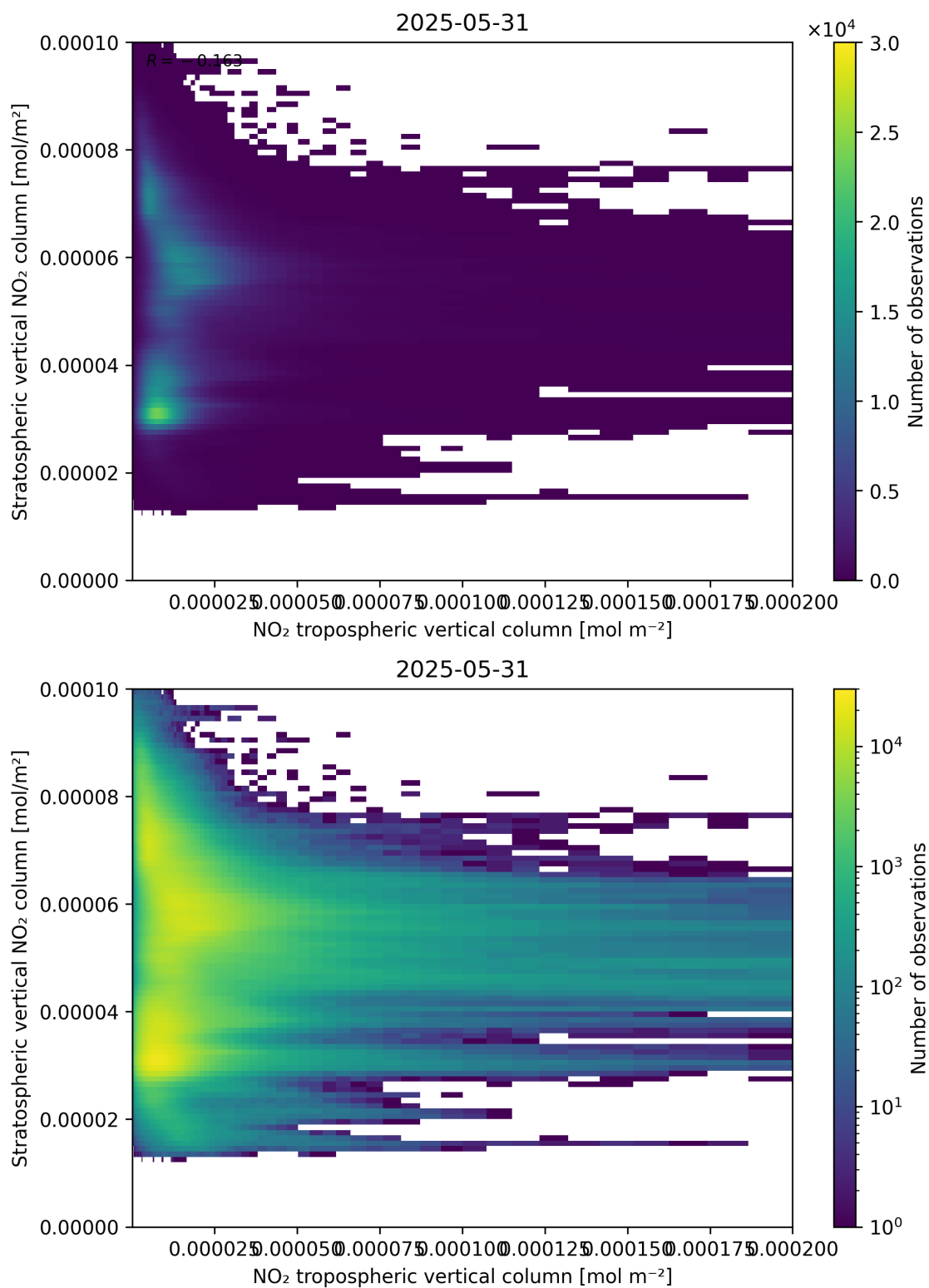
Figure 125: Scatter density plot of “NO 2 tropospheric vertical column” against “Stratospheric vertical NO 2 column” for 2025-05-31 to 2025-06-01.
