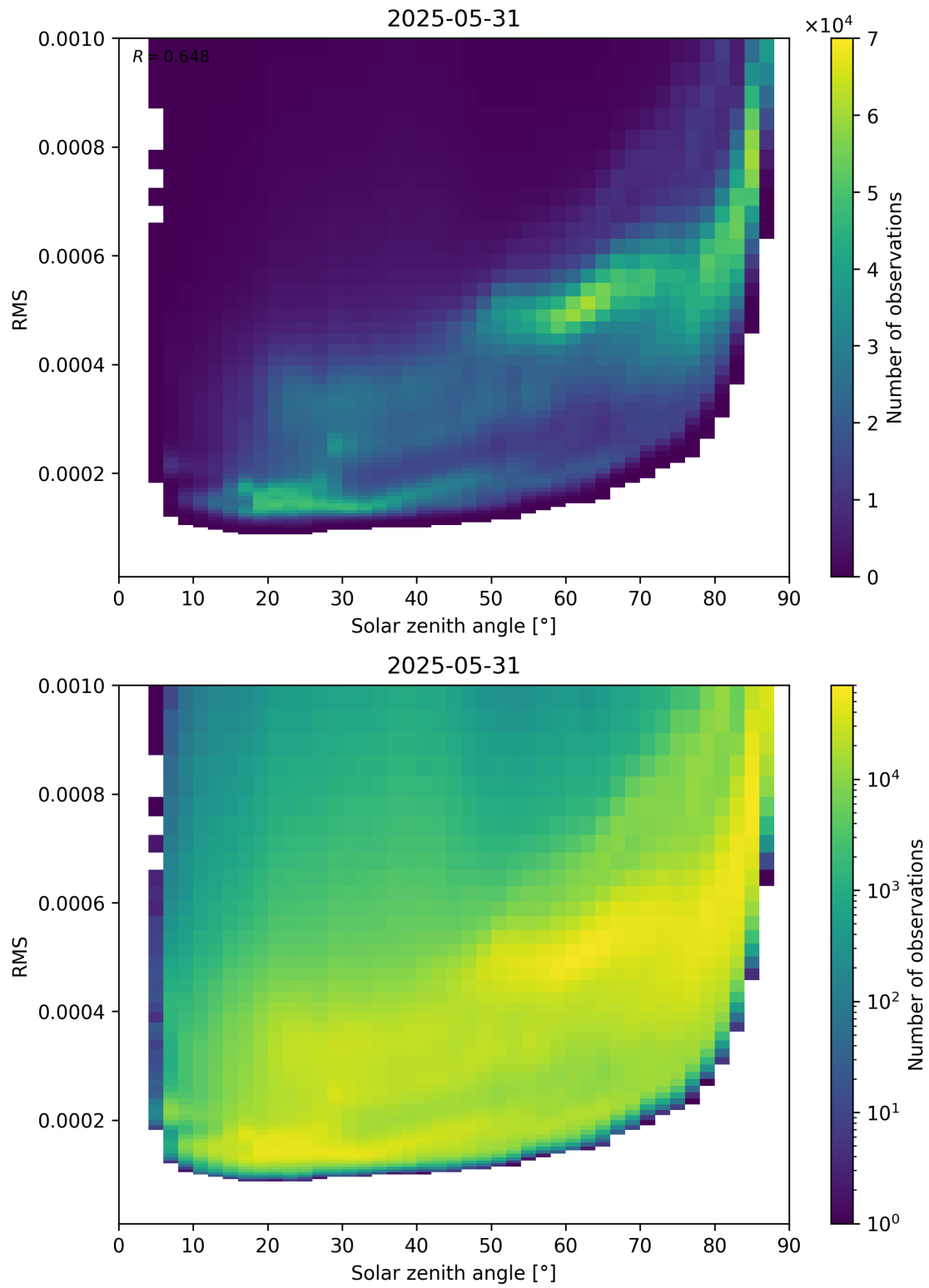
Figure 157: Scatter density plot of “Solar zenith angle” against “RMS” for 2025-05-31 to 2025-06-01.
