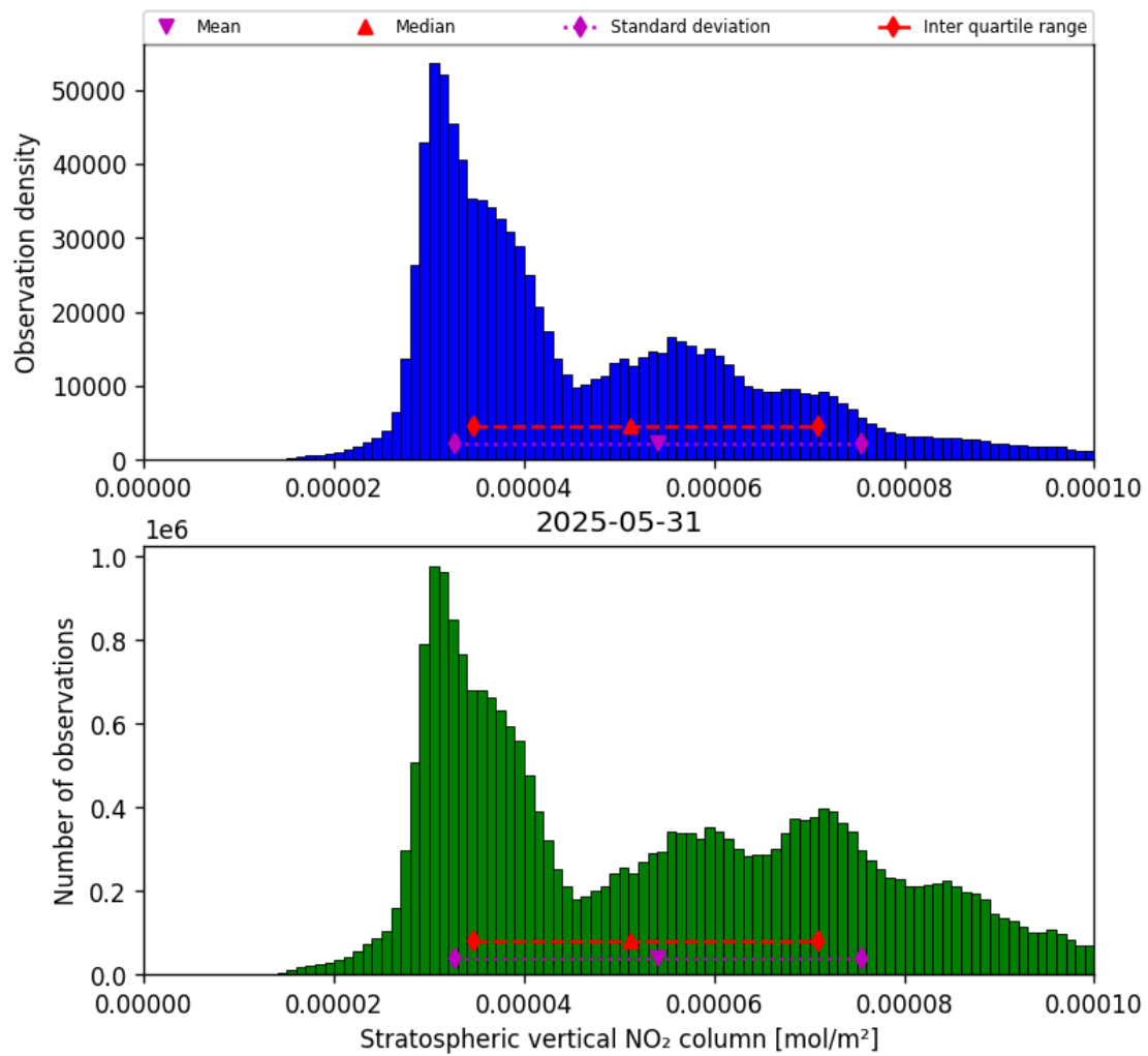
Figure 36: Histogram of “Stratospheric vertical NO 2 column” for 2025-05-31 to 2025-06-01
