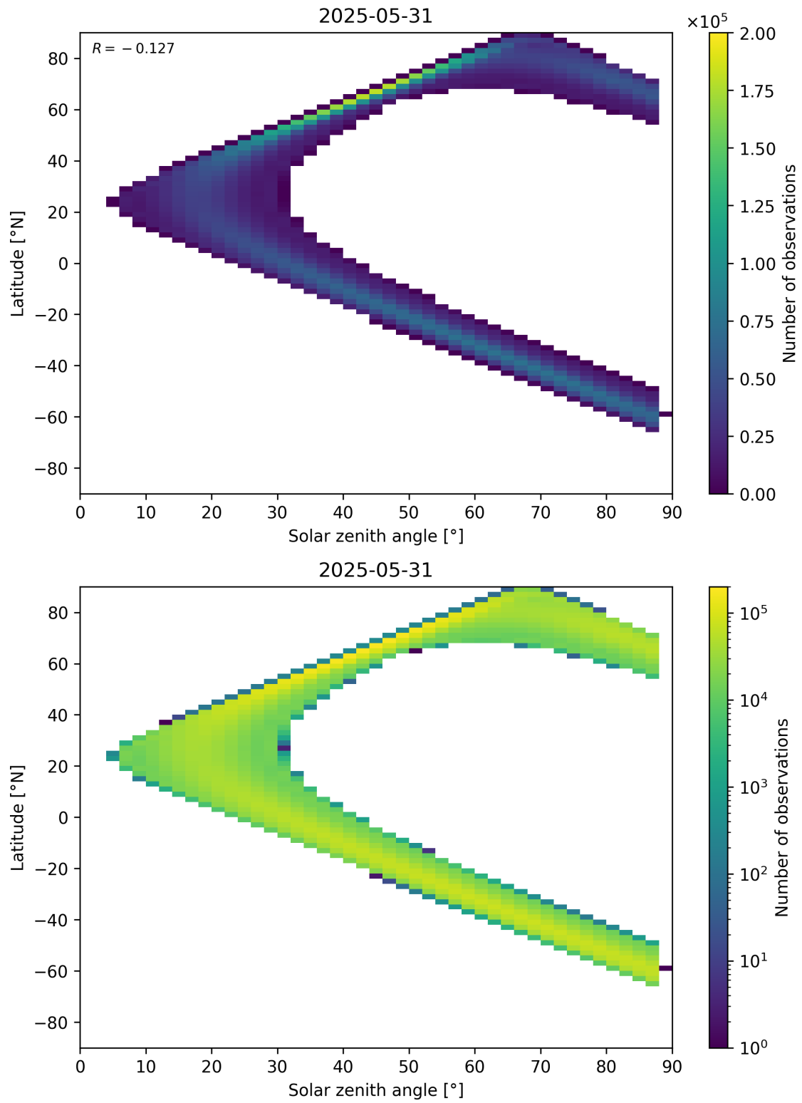
Figure 149: Scatter density plot of “Solar zenith angle” against “Latitude” for 2025-05-31 to 2025-06-01.
