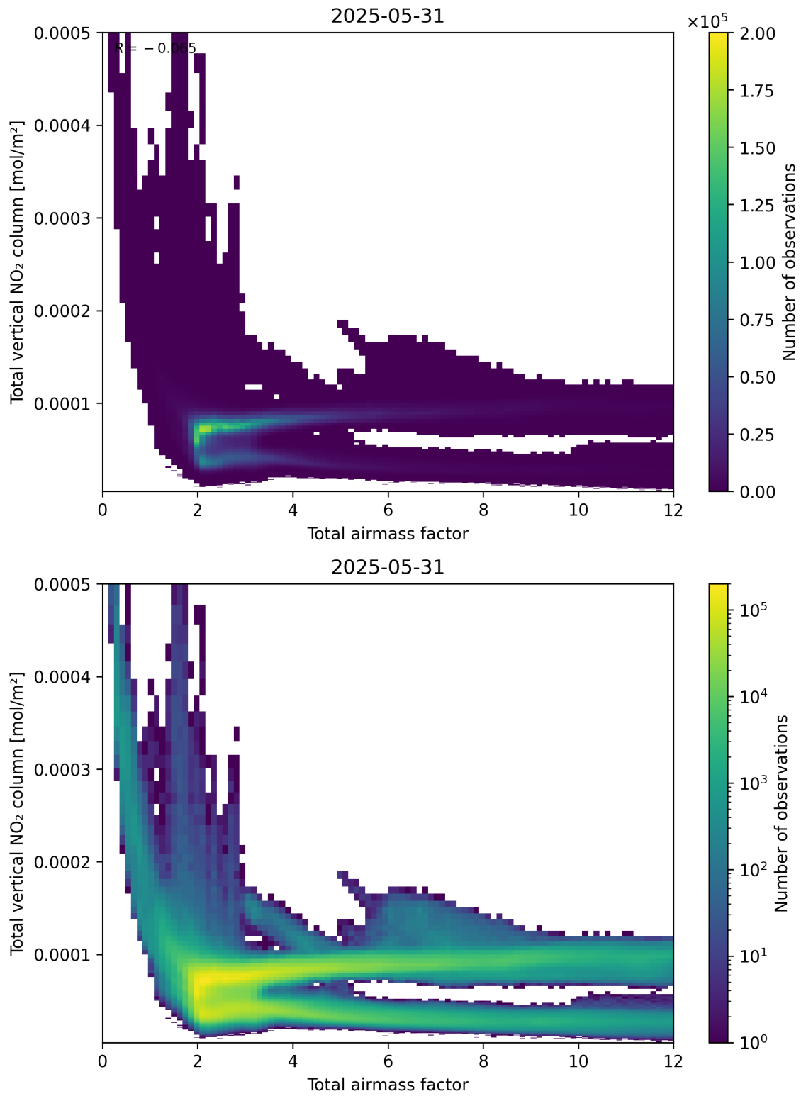
Figure 67: Scatter density plot of “Total airmass factor” against “Total vertical NO 2 column” for 2025-05-31 to 2025-06-01.
