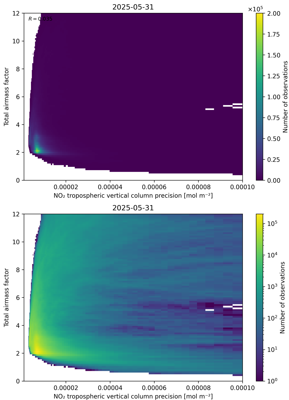
Figure 132: Scatter density plot of “NO 2 tropospheric vertical column precision” against “Total air mass factor” for 2025-05-31 to 2025-06-01.
