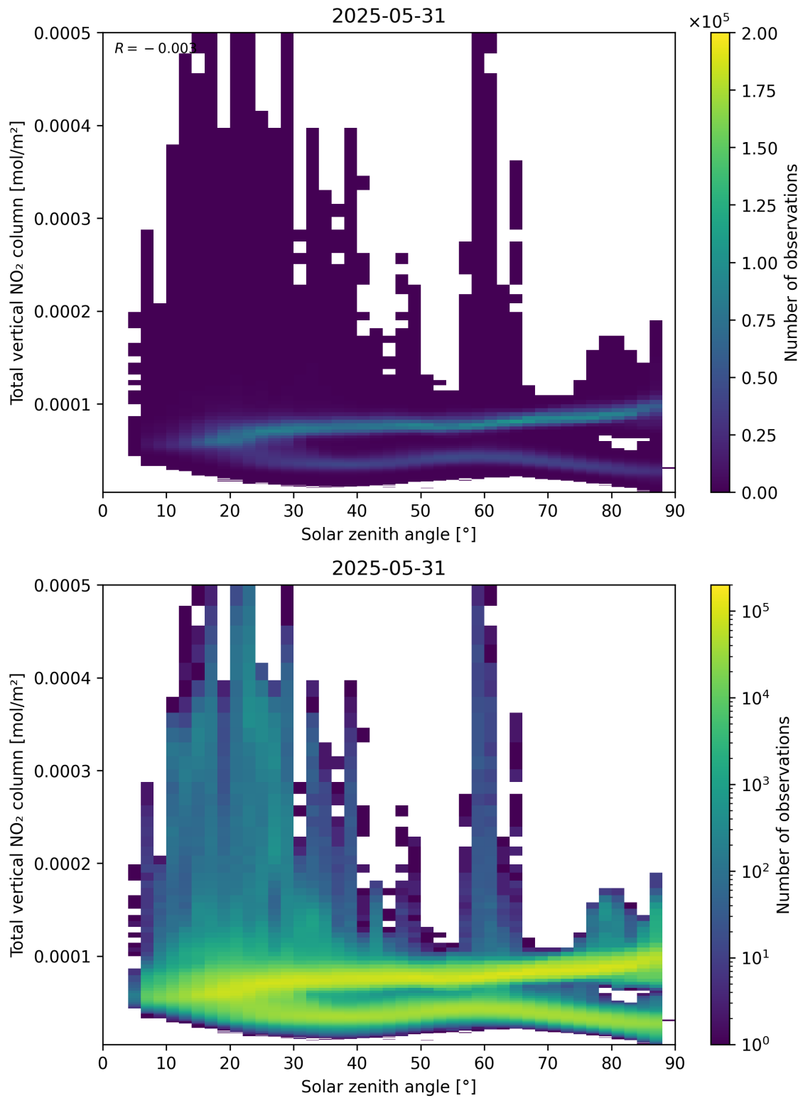
Figure 153: Scatter density plot of “Solar zenith angle” against “Total vertical NO 2 column” for 2025-05-31 to 2025-06-01.
