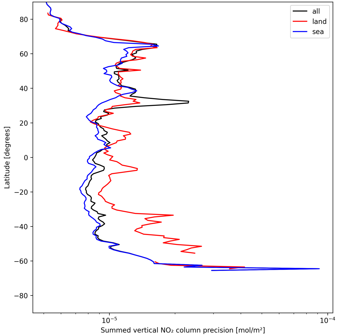
Figure 24: Zonal average of “Summed vertical NO 2 column precision” for 2025-05-31 to 2025-06-01.
