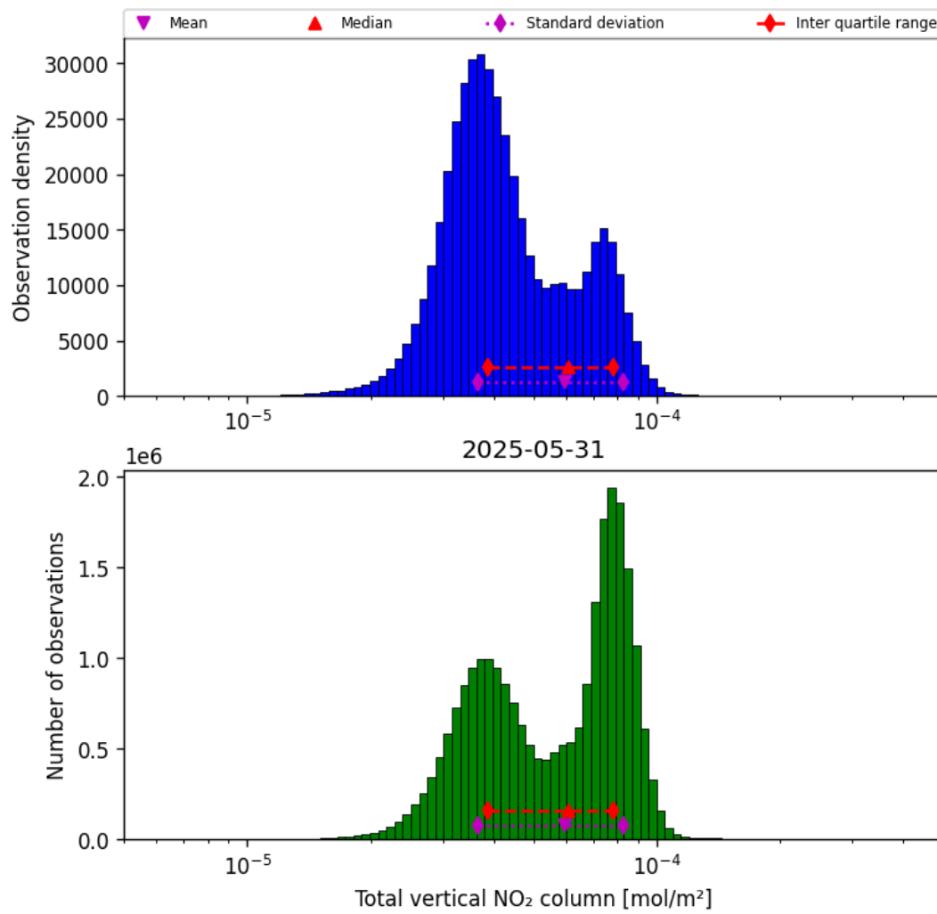
Figure 38: Histogram of “Total vertical NO 2 column” for 2025-05-31 to 2025-06-01
