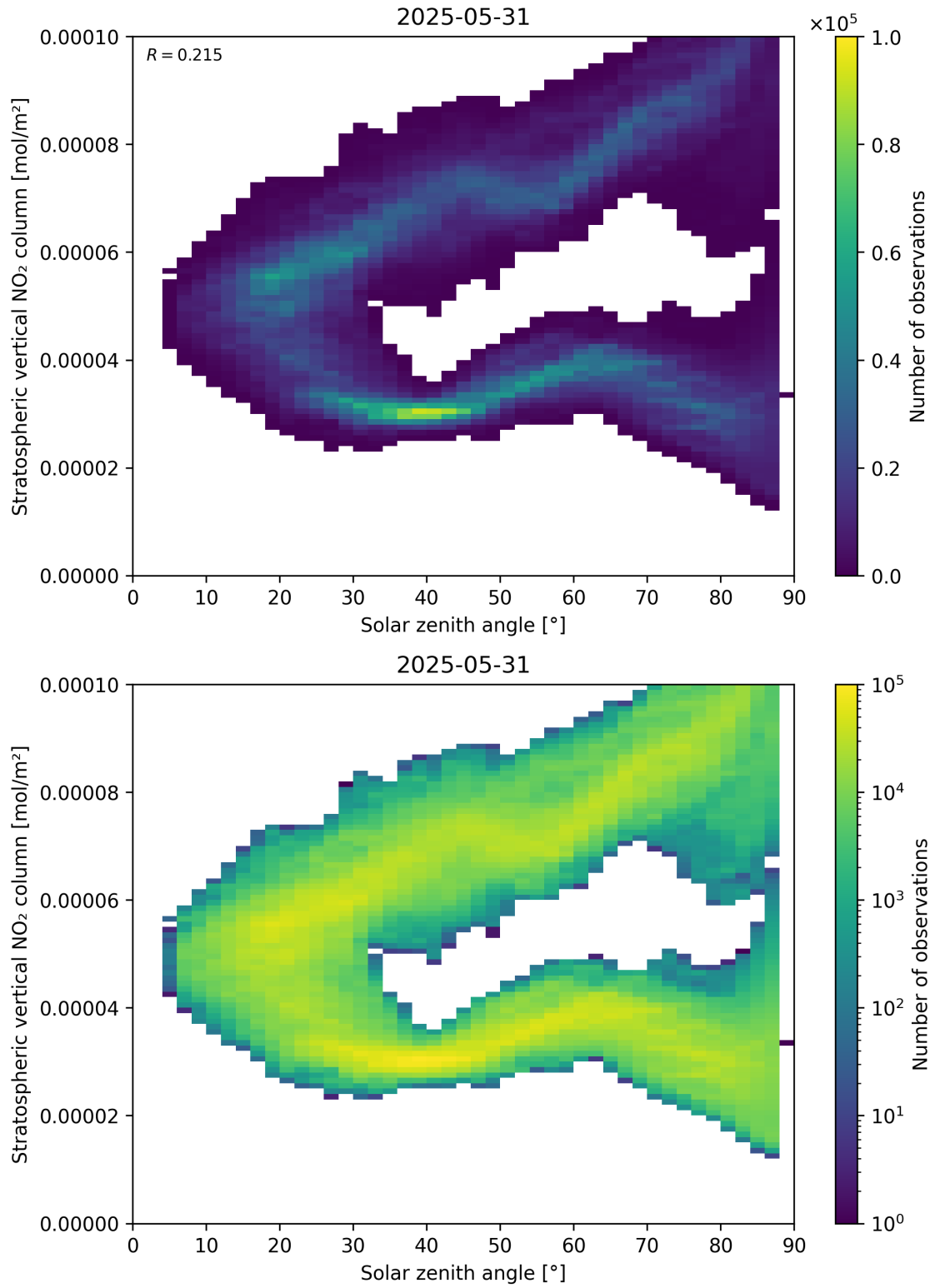
Figure 150: Scatter density plot of “Solar zenith angle” against “Stratospheric vertical NO 2 column” for 2025-05-31 to 2025-06-01.
