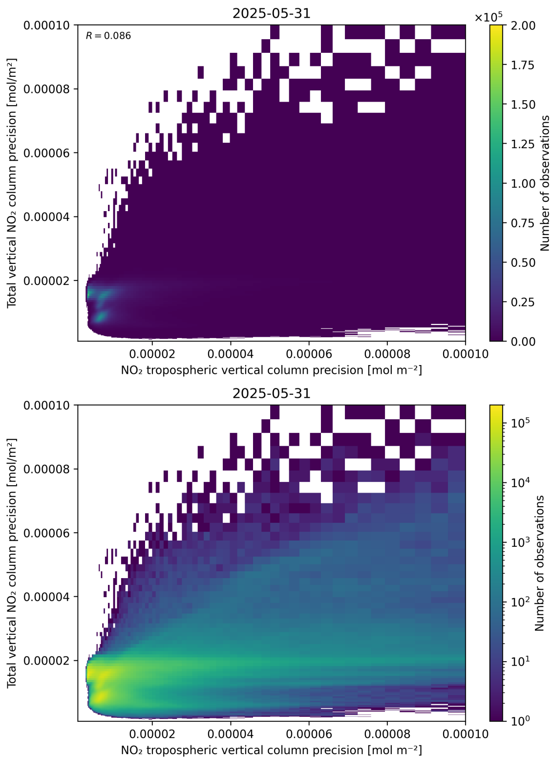
Figure 139: Scatter density plot of “NO 2 tropospheric vertical column precision” against “Total vertical NO 2 column precision” for 2025-05-31 to 2025-06-01.
