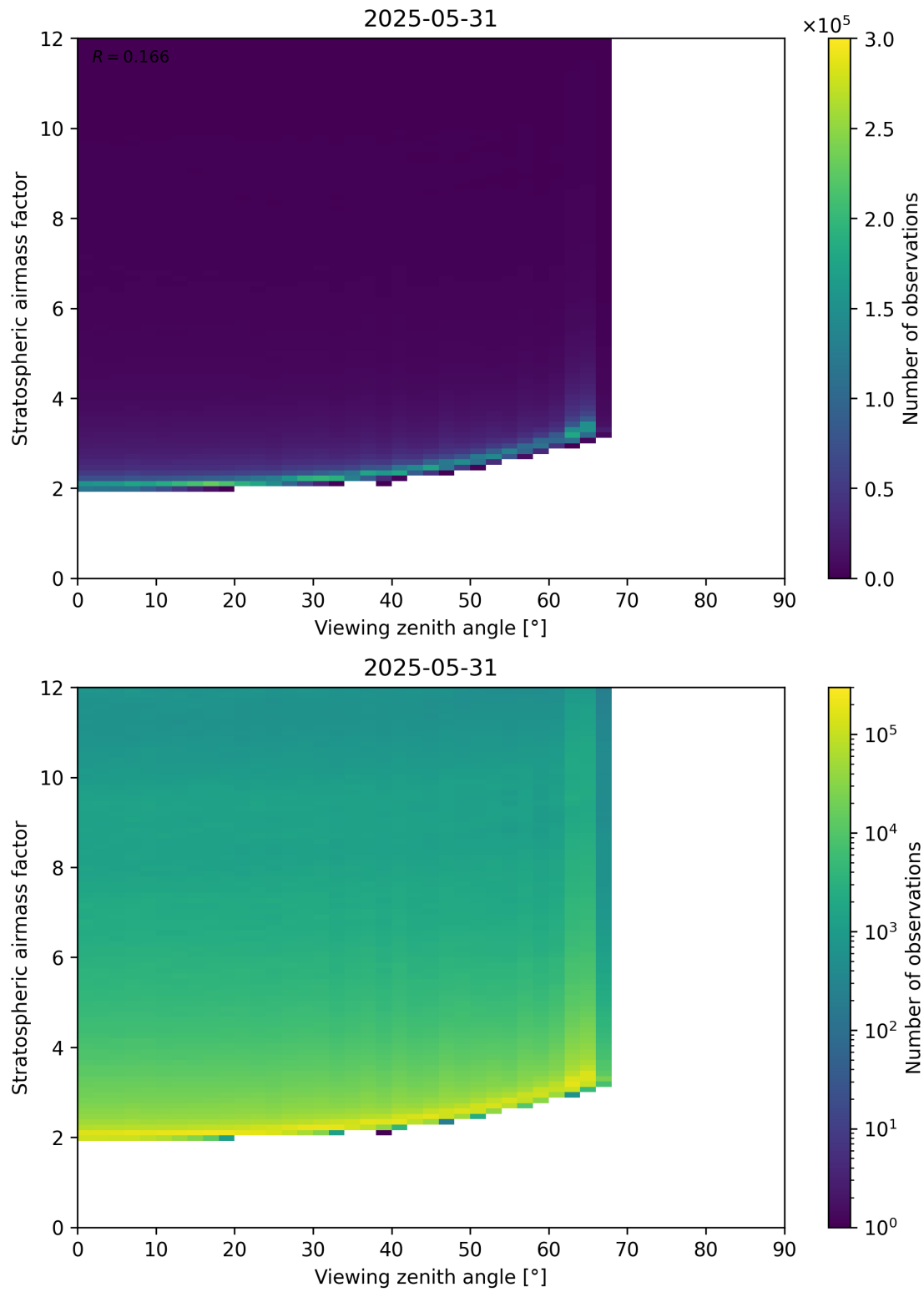
Figure 159: Scatter density plot of “Viewing zenith angle” against “Stratospheric airmass factor” for 2025-05-31 to 2025-06-01.
