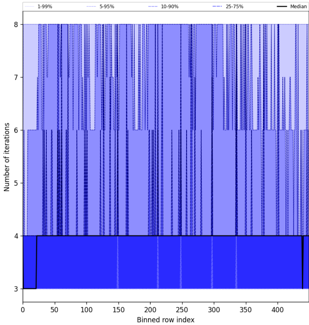
Figure 51: Along track statistics of “Number of iterations” for 2025-05-31 to 2025-06-01
