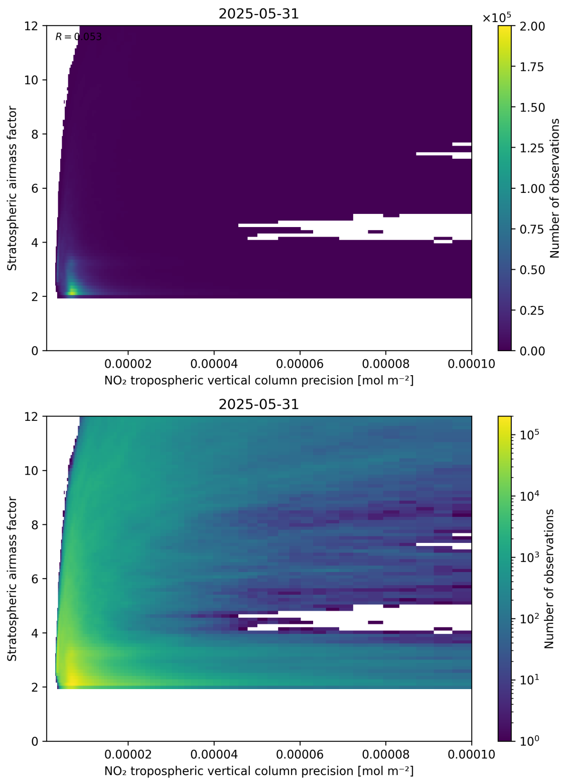
Figure 131: Scatter density plot of “NO 2 tropospheric vertical column precision” against “Stratospheric airmass factor” for 2025-05-31 to 2025-06-01.
