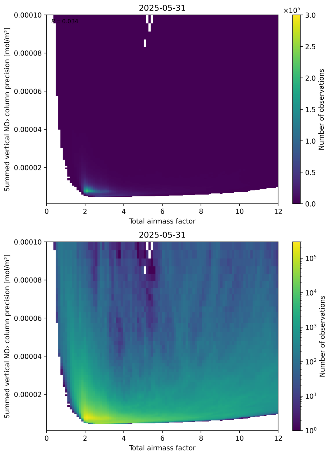
Figure 66: Scatter density plot of “Total airmass factor” against “Summed vertical NO 2 column precision” for 2025-05-31 to 2025-06-01.
