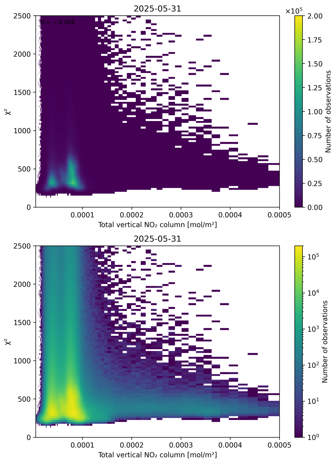
Figure 111: Scatter density plot of “Total vertical NO 2 column” against “ \chi^2 ” for 2025-05-31 to 2025-06-01.
