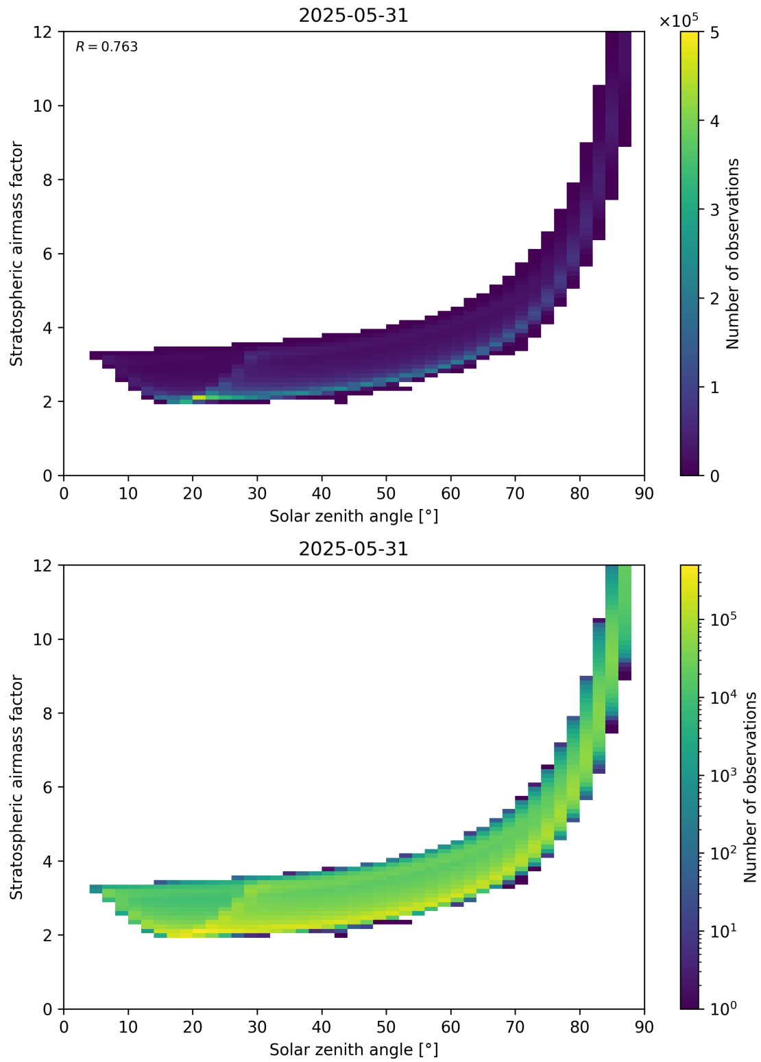
Figure 145: Scatter density plot of “Solar zenith angle” against “Stratospheric airmass factor” for 2025-05-31 to 2025-06-01.
