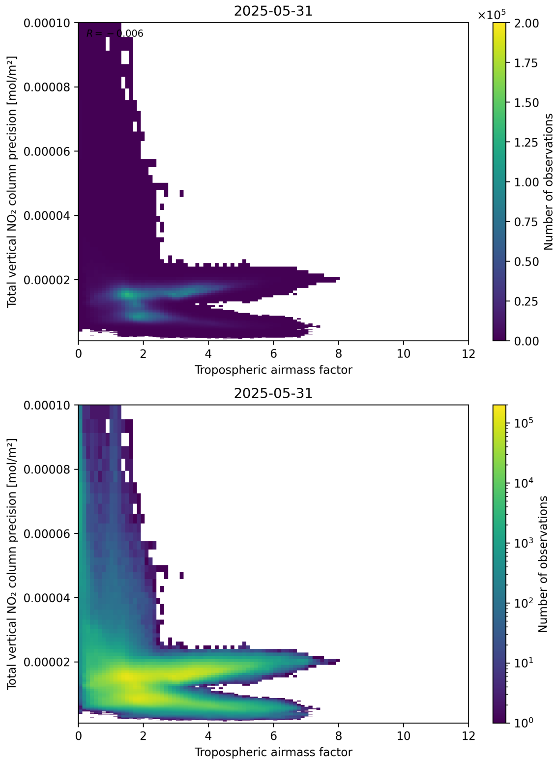
Figure 78: Scatter density plot of “Tropospheric air mass factor” against “Total vertical NO 2 column precision” for 2025-05-31 to 2025-06-01.
