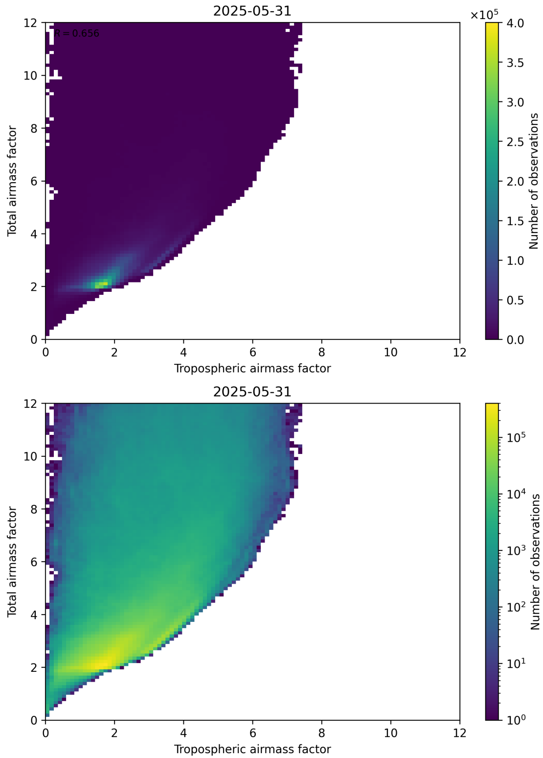
Figure 72: Scatter density plot of “Tropospheric airmass factor” against “Total airmass factor” for 2025-05-31 to 2025-06-01.
