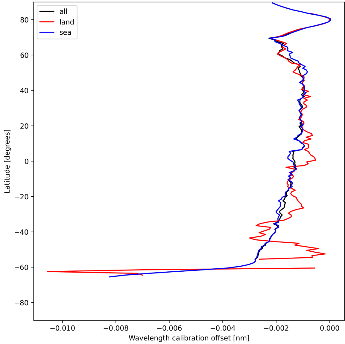
Figure 18: Zonal average of “Wavelength calibration offset” for 2025-05-31 to 2025-06-01.
