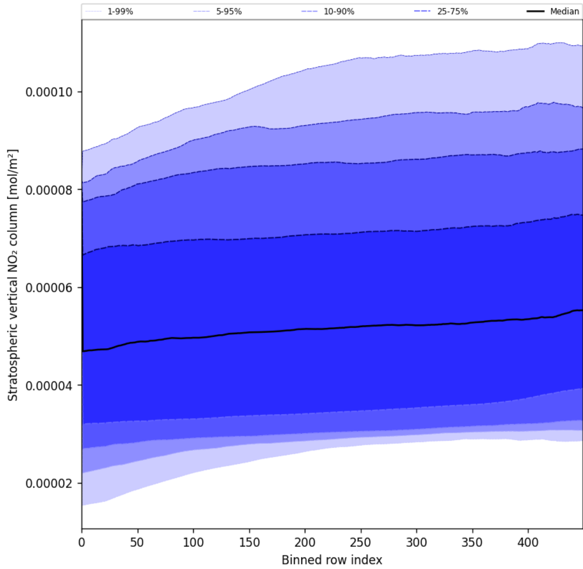
Figure 53: Along track statistics of “Stratospheric vertical NO 2 column” for 2025-05-31 to 2025-06-01
