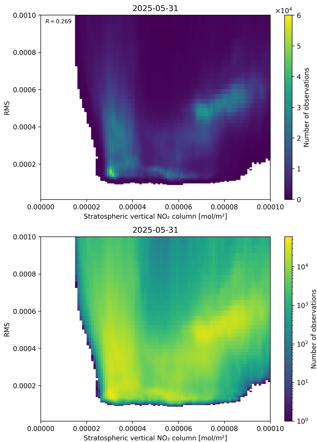
Figure 102: Scatter density plot of “Stratospheric vertical NO 2 column” against “RMS” for 2025-05-31 to 2025-06-01.
