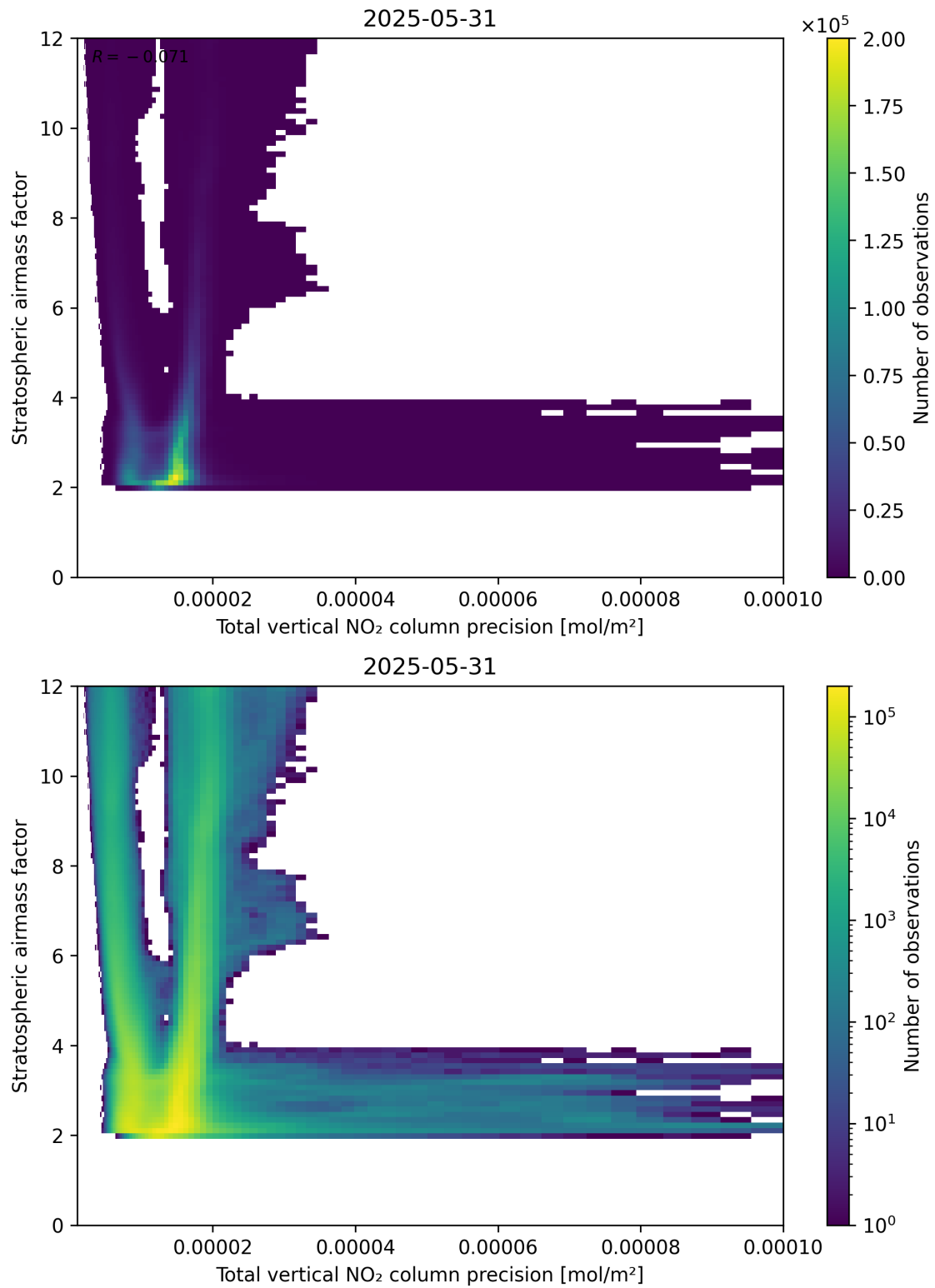
Figure 115: Scatter density plot of “Total vertical NO 2 column precision” against “Stratospheric air mass factor” for 2025-05-31 to 2025-06-01.
