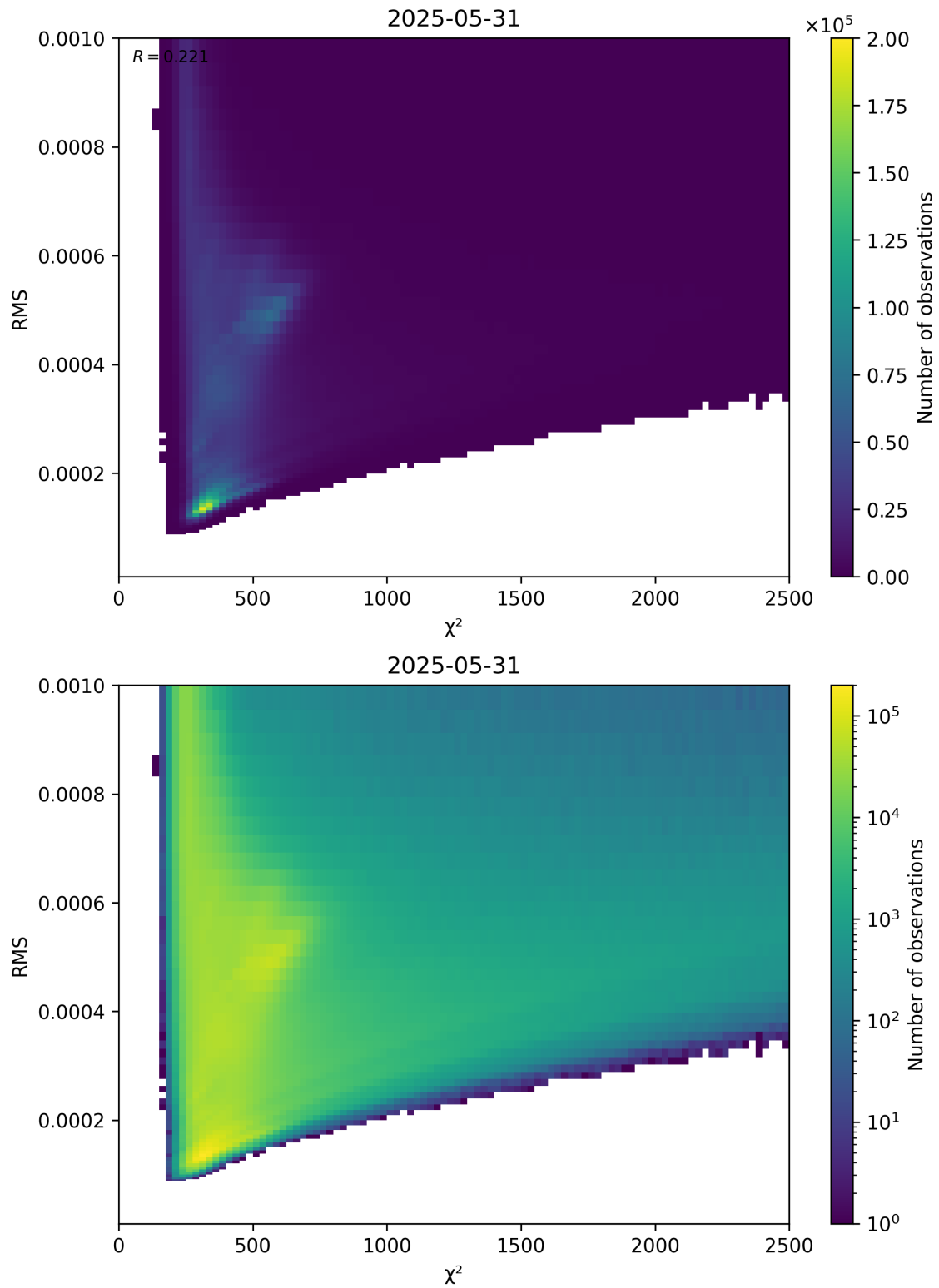
Figure 82: Scatter density plot of “ \chi^2 ” against “RMS” for 2025-05-31 to 2025-06-01.
