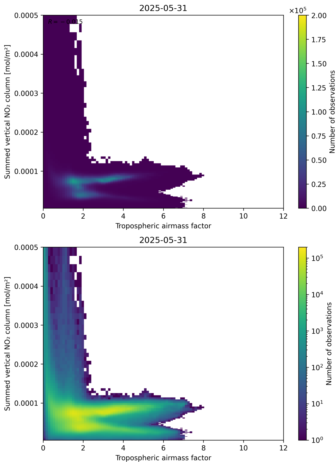
Figure 75: Scatter density plot of “Tropospheric air mass factor” against “Summed vertical NO 2 column” for 2025-05-31 to 2025-06-01.
