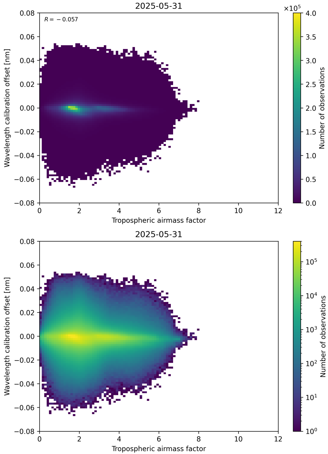
Figure 80: Scatter density plot of “Tropospheric airmass factor” against “Wavelength calibration offset” for 2025-05-31 to 2025-06-01.
