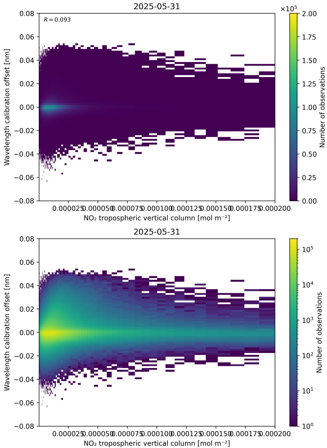
Figure 143: Scatter density plot of “NO 2 tropospheric vertical column” against “Wavelength calibration offset” for 2025-05-31 to 2025-06-01.
