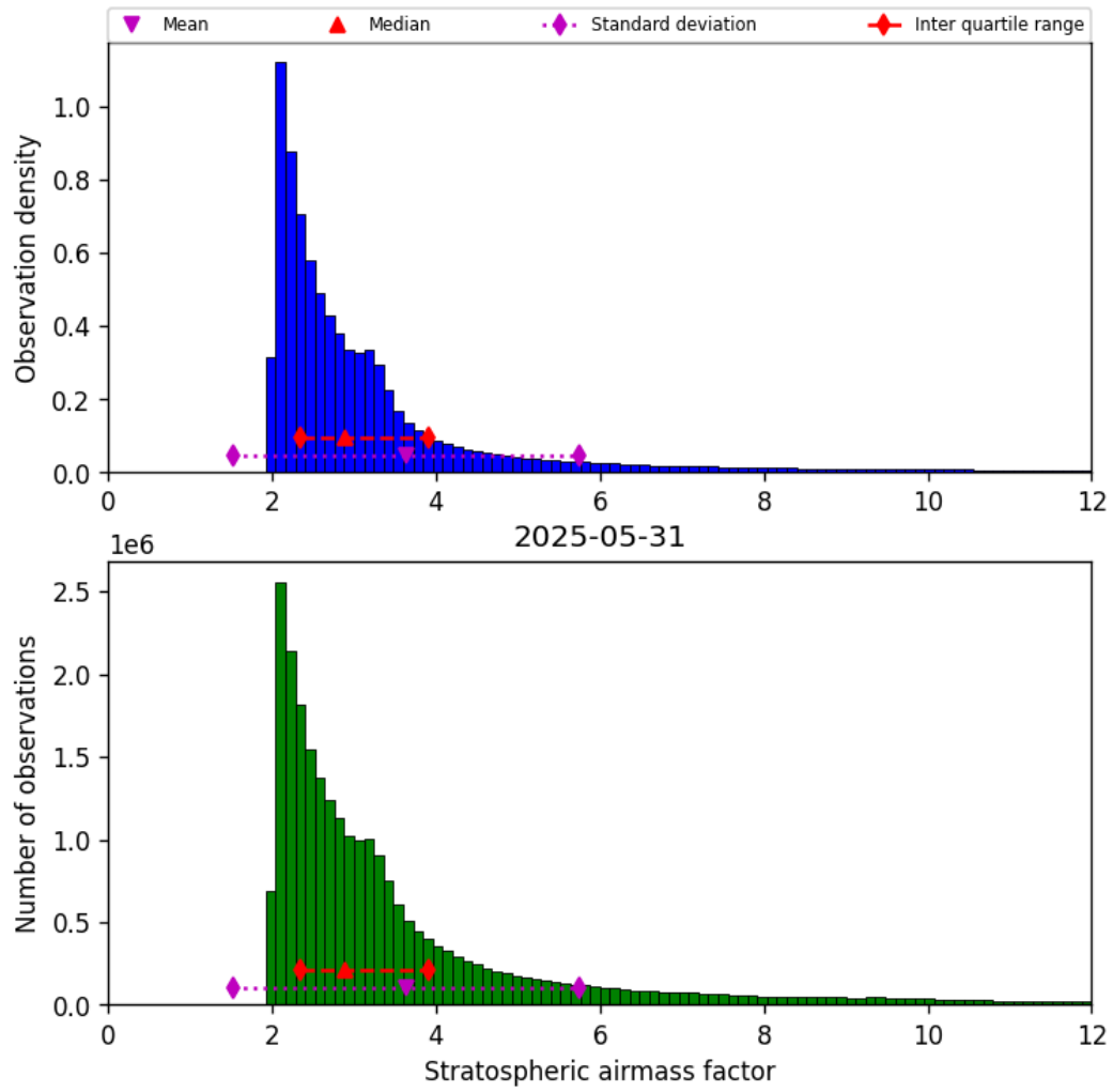
Figure 44: Histogram of “Stratospheric airmass factor” for 2025-05-31 to 2025-06-01
