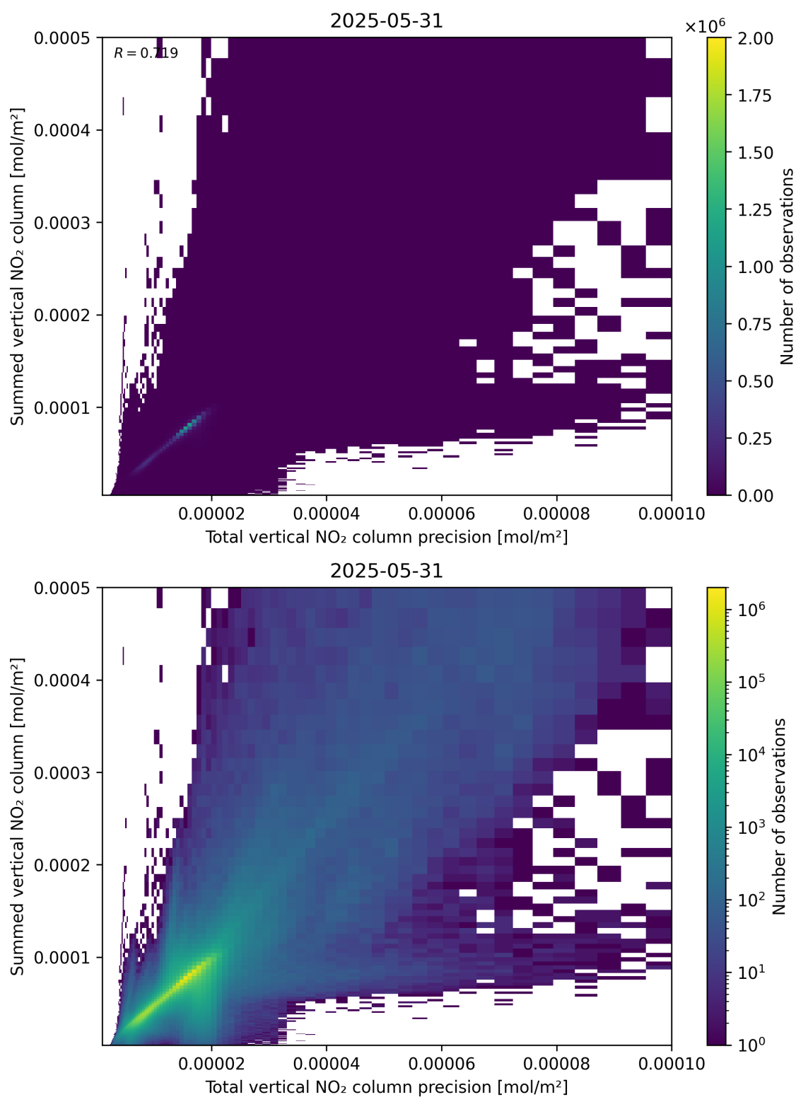
Figure 117: Scatter density plot of “Total vertical NO 2 column precision” against “Summed vertical NO 2 column” for 2025-05-31 to 2025-06-01.
