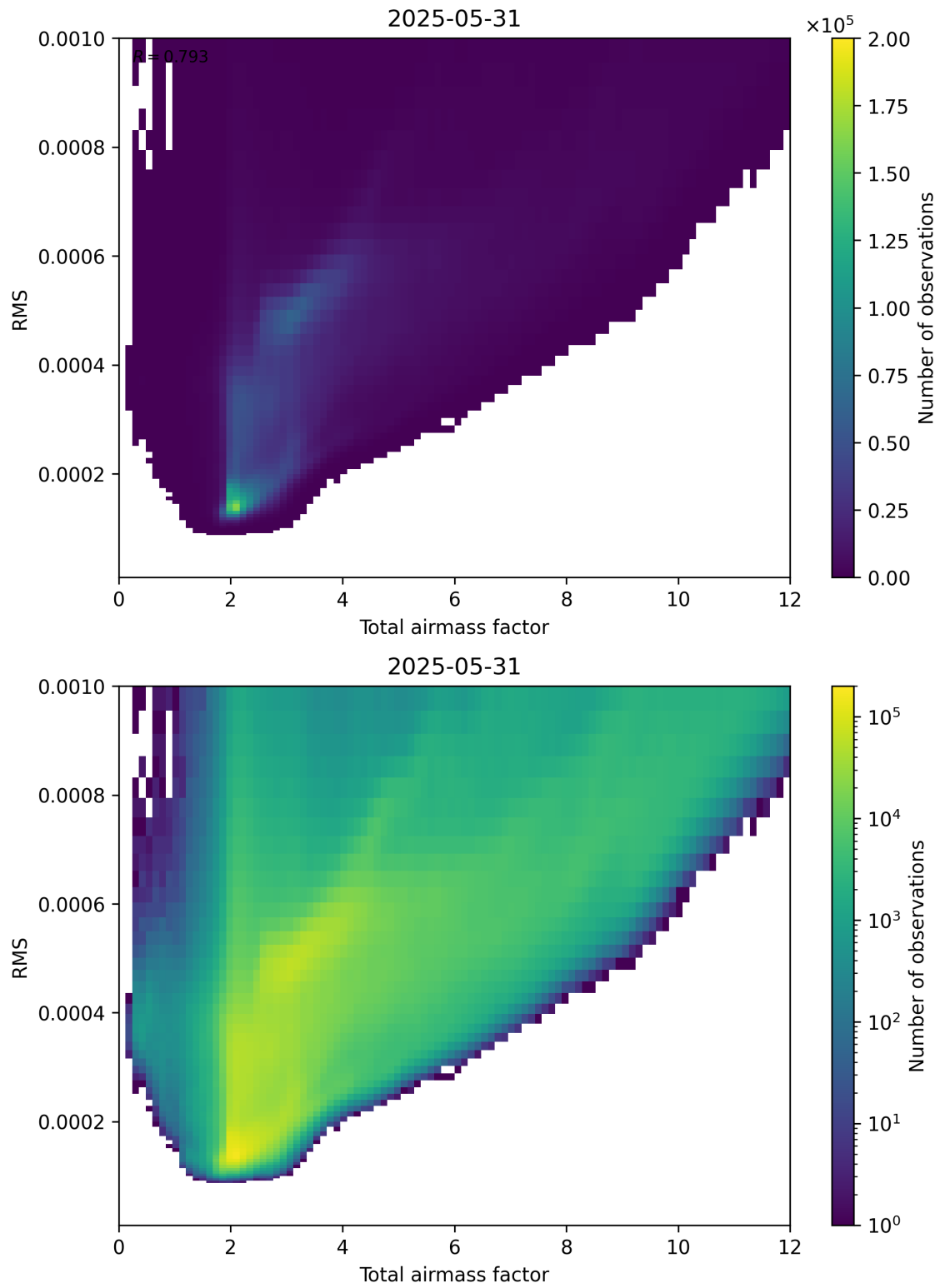
Figure 69: Scatter density plot of “Total airmass factor” against “RMS” for 2025-05-31 to 2025-06-01.
