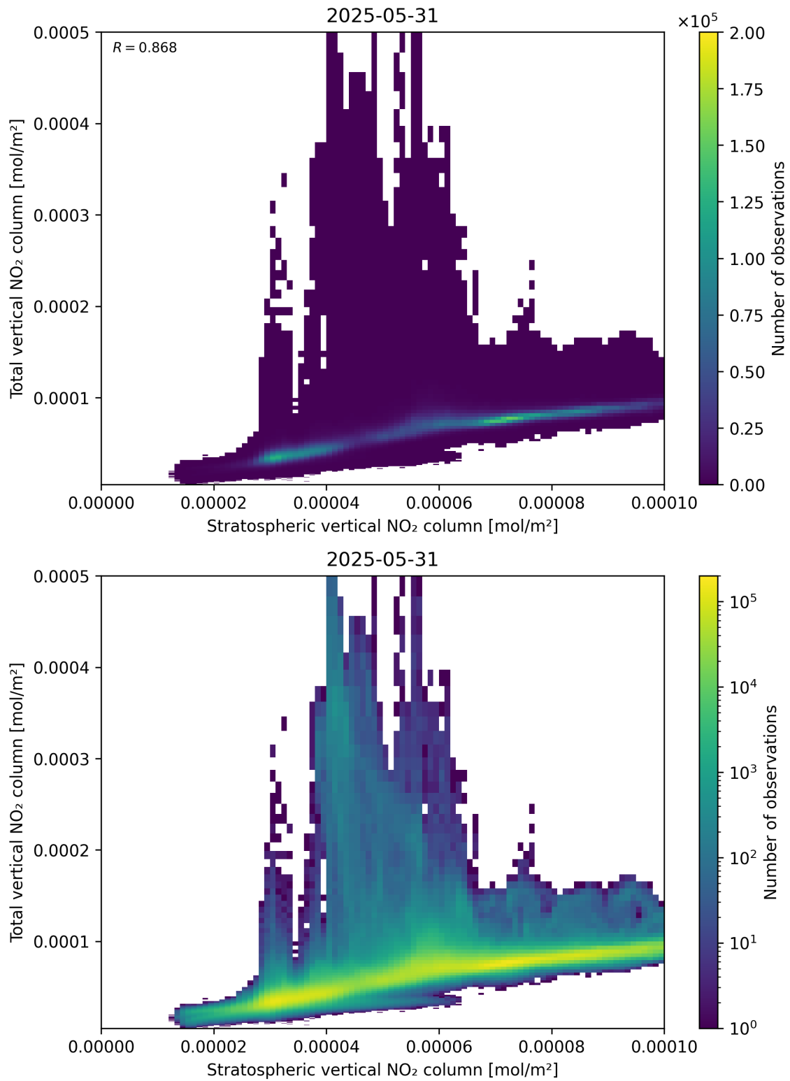
Figure 100: Scatter density plot of “Stratospheric vertical NO 2 column” against “Total vertical NO 2 column” for 2025-05-31 to 2025-06-01.
