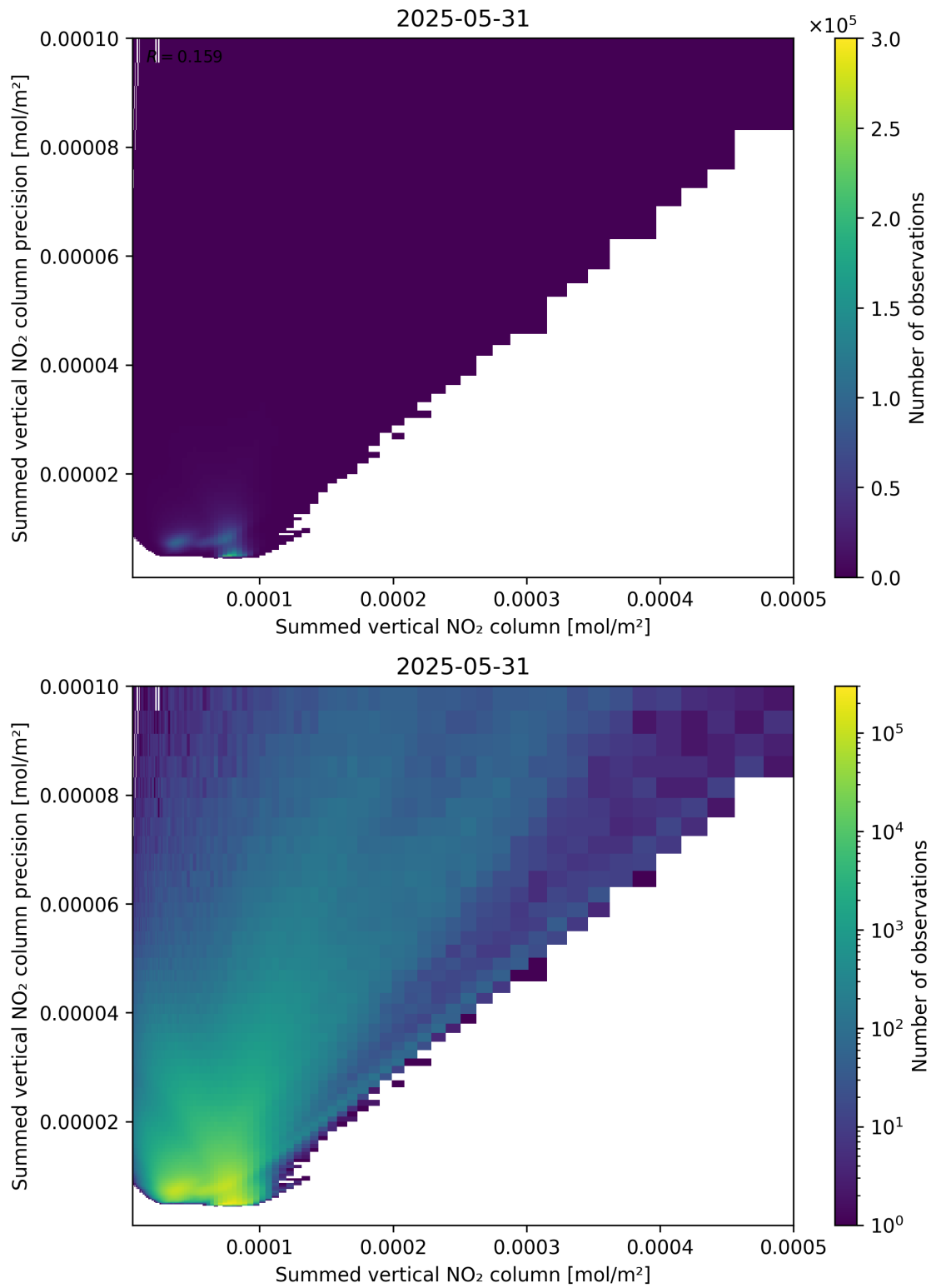
Figure 105: Scatter density plot of “Summed vertical NO 2 column” against “Summed vertical NO 2 column precision” for 2025-05-31 to 2025-06-01.
