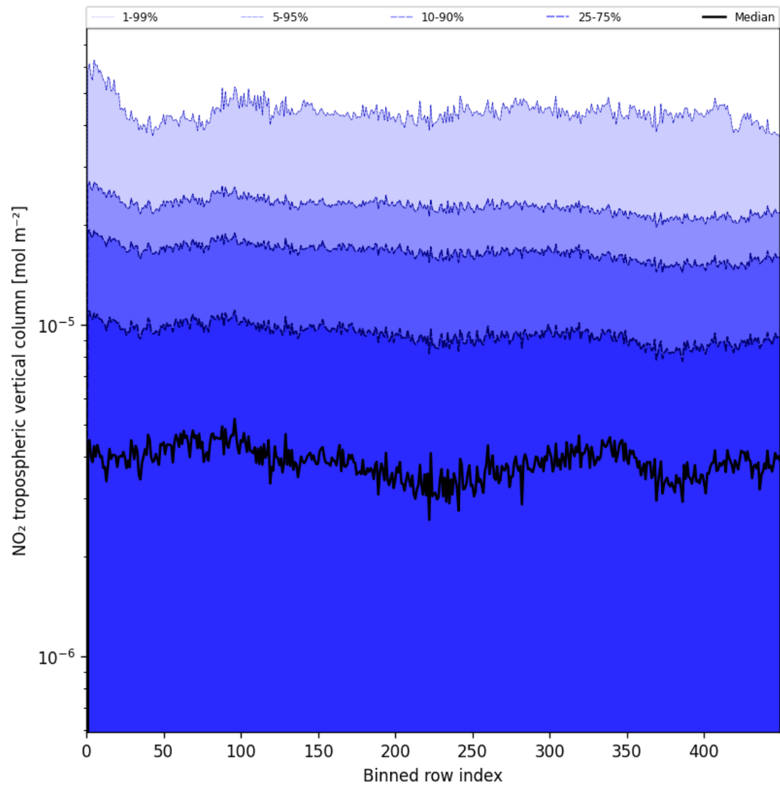
Figure 46: Along track statistics of “NO 2 tropospheric vertical column” for 2025-05-31 to 2025-06-01
