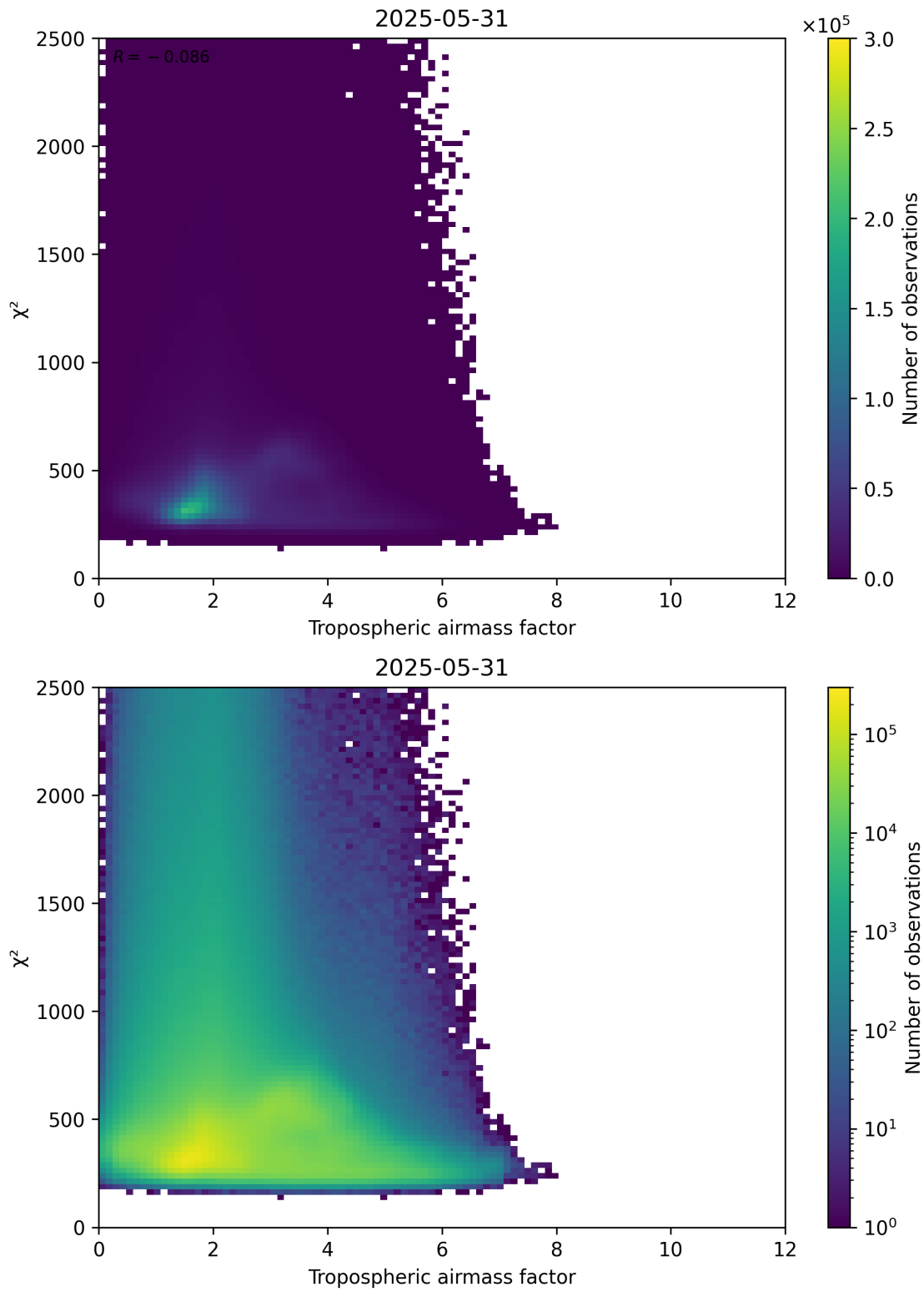
Figure 73: Scatter density plot of “Tropospheric airmass factor” against “ \chi^2 ” for 2025-05-31 to 2025-06-01.
