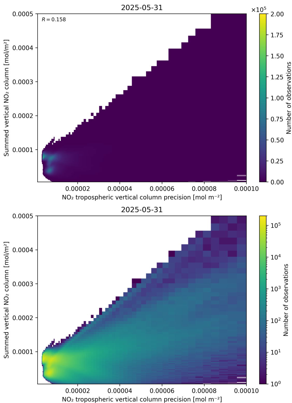
Figure 136: Scatter density plot of “NO 2 tropospheric vertical column precision” against “Summed vertical NO 2 column” for 2025-05-31 to 2025-06-01.
