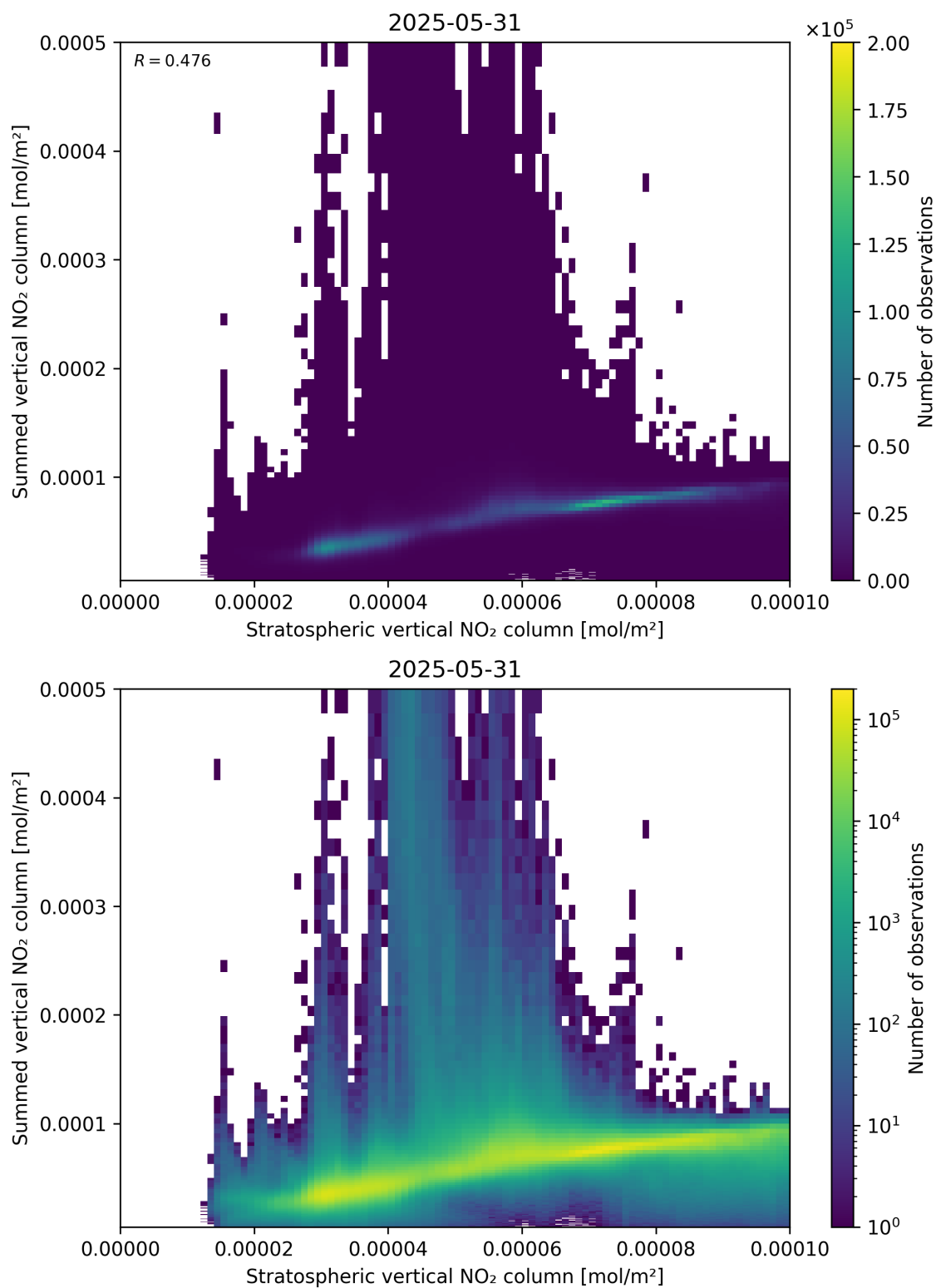
Figure 98: Scatter density plot of “Stratospheric vertical NO 2 column” against “Summed vertical NO 2 column” for 2025-05-31 to 2025-06-01.
