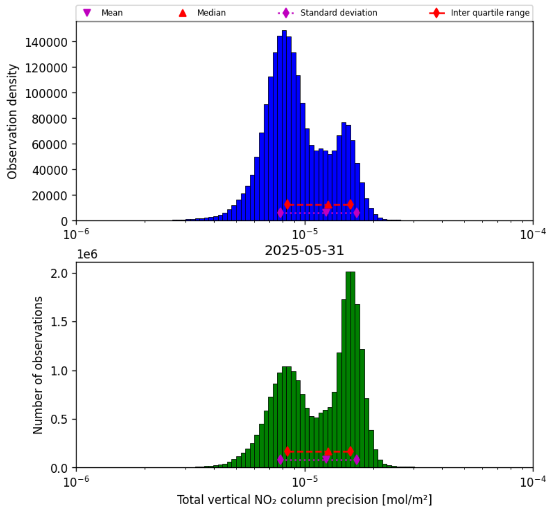
Figure 39: Histogram of “Total vertical NO 2 column precision” for 2025-05-31 to 2025-06-01
