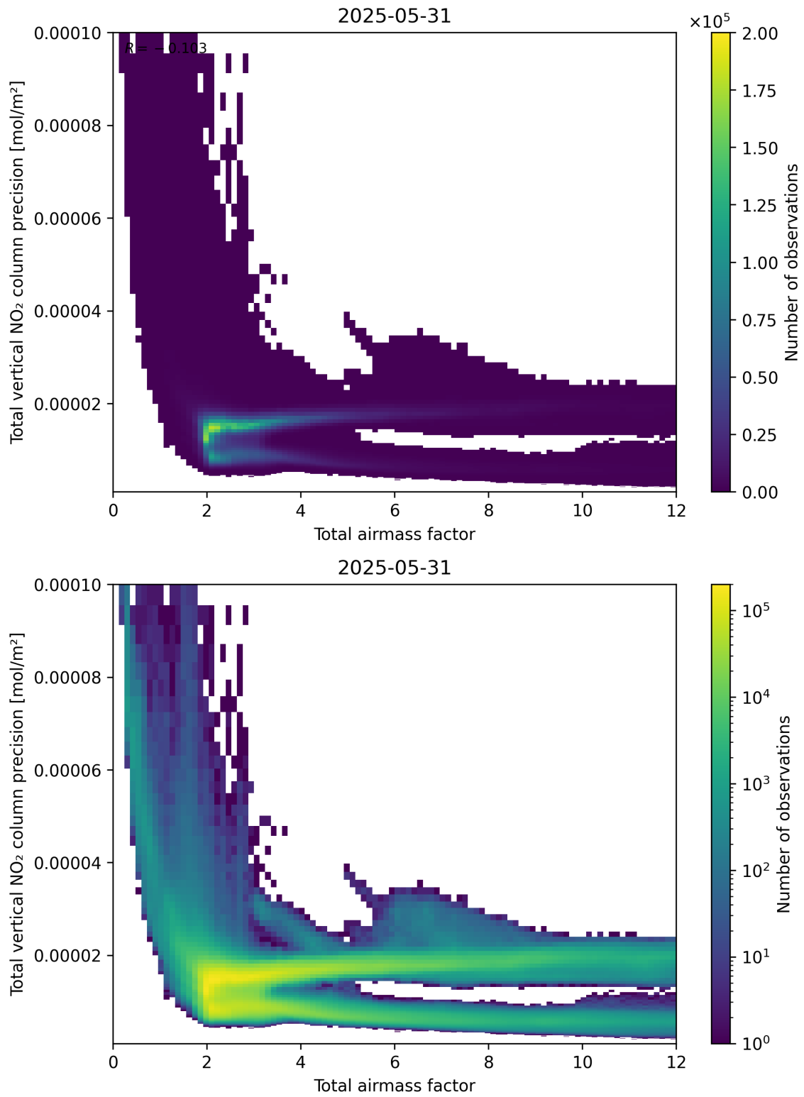
Figure 68: Scatter density plot of “Total airmass factor” against “Total vertical NO 2 column precision” for 2025-05-31 to 2025-06-01.
