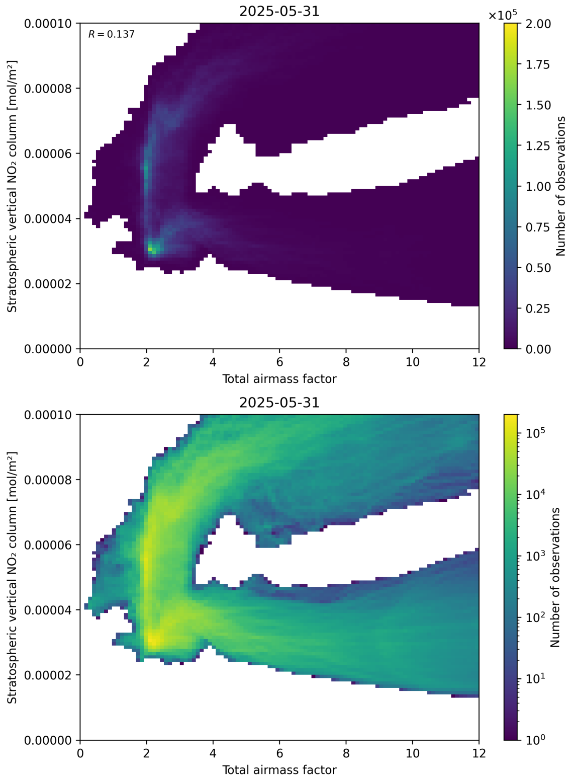
Figure 64: Scatter density plot of “Total airmass factor” against “Stratospheric vertical NO 2 column” for 2025-05-31 to 2025-06-01.
