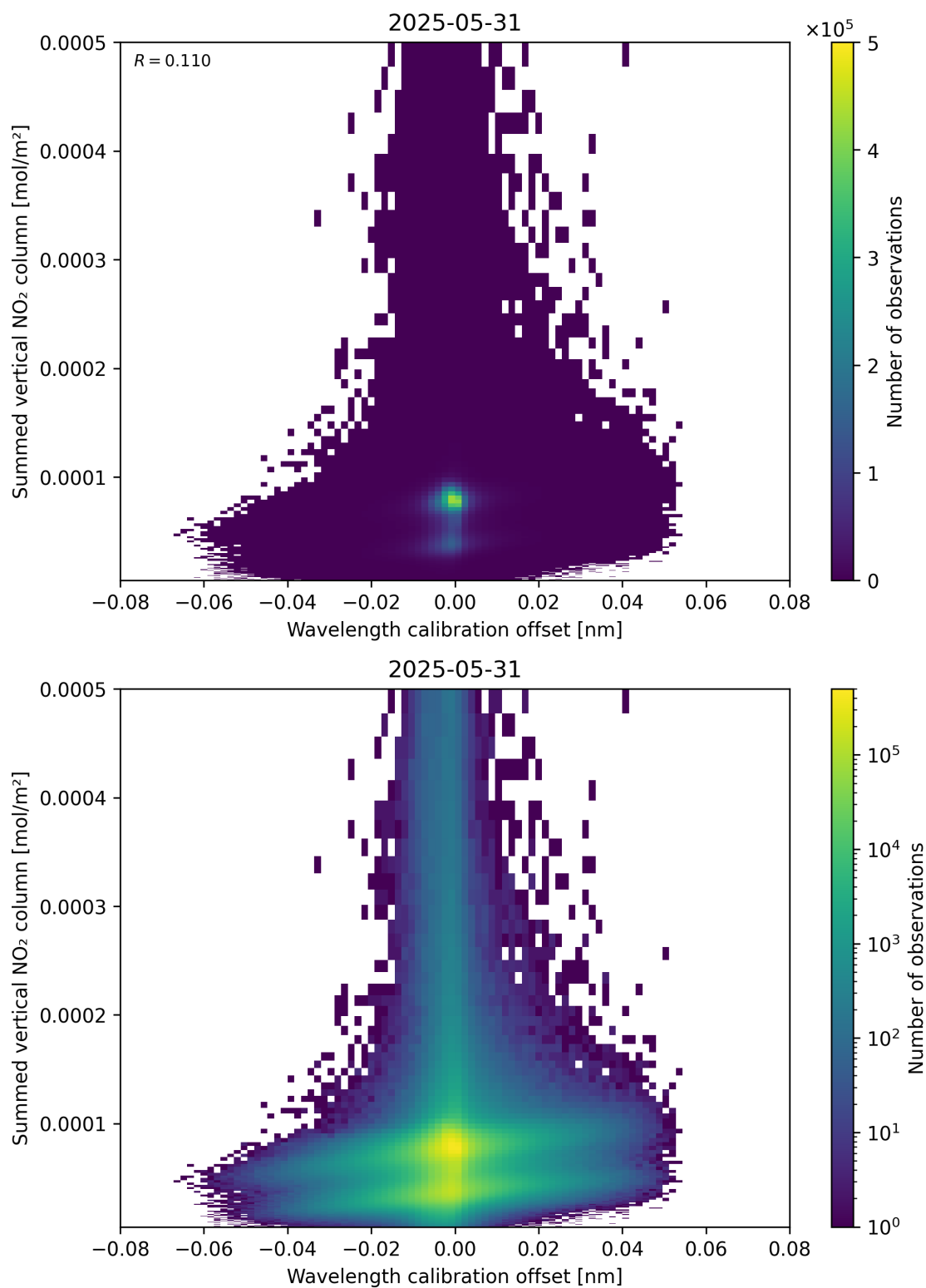
Figure 177: Scatter density plot of “Wavelength calibration offset” against “Summed vertical NO 2 column” for 2025-05-31 to 2025-06-01.
