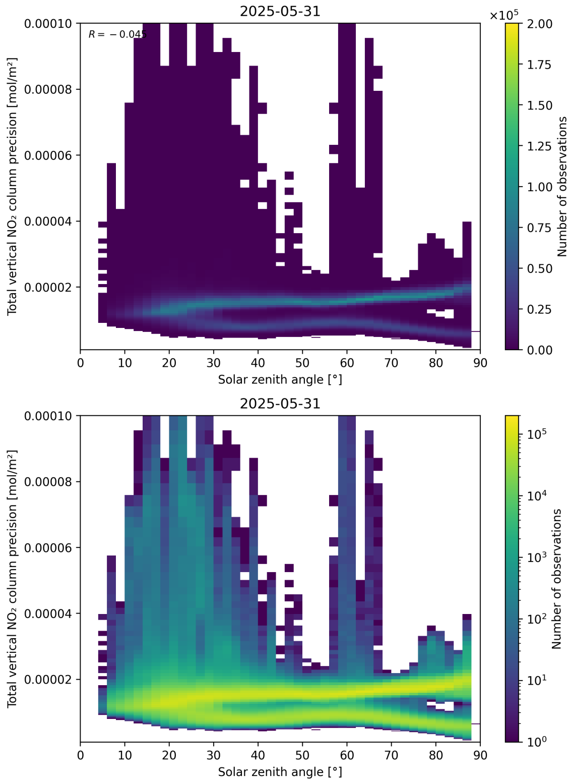
Figure 154: Scatter density plot of “Solar zenith angle” against “Total vertical NO 2 column precision” for 2025-05-31 to 2025-06-01.
