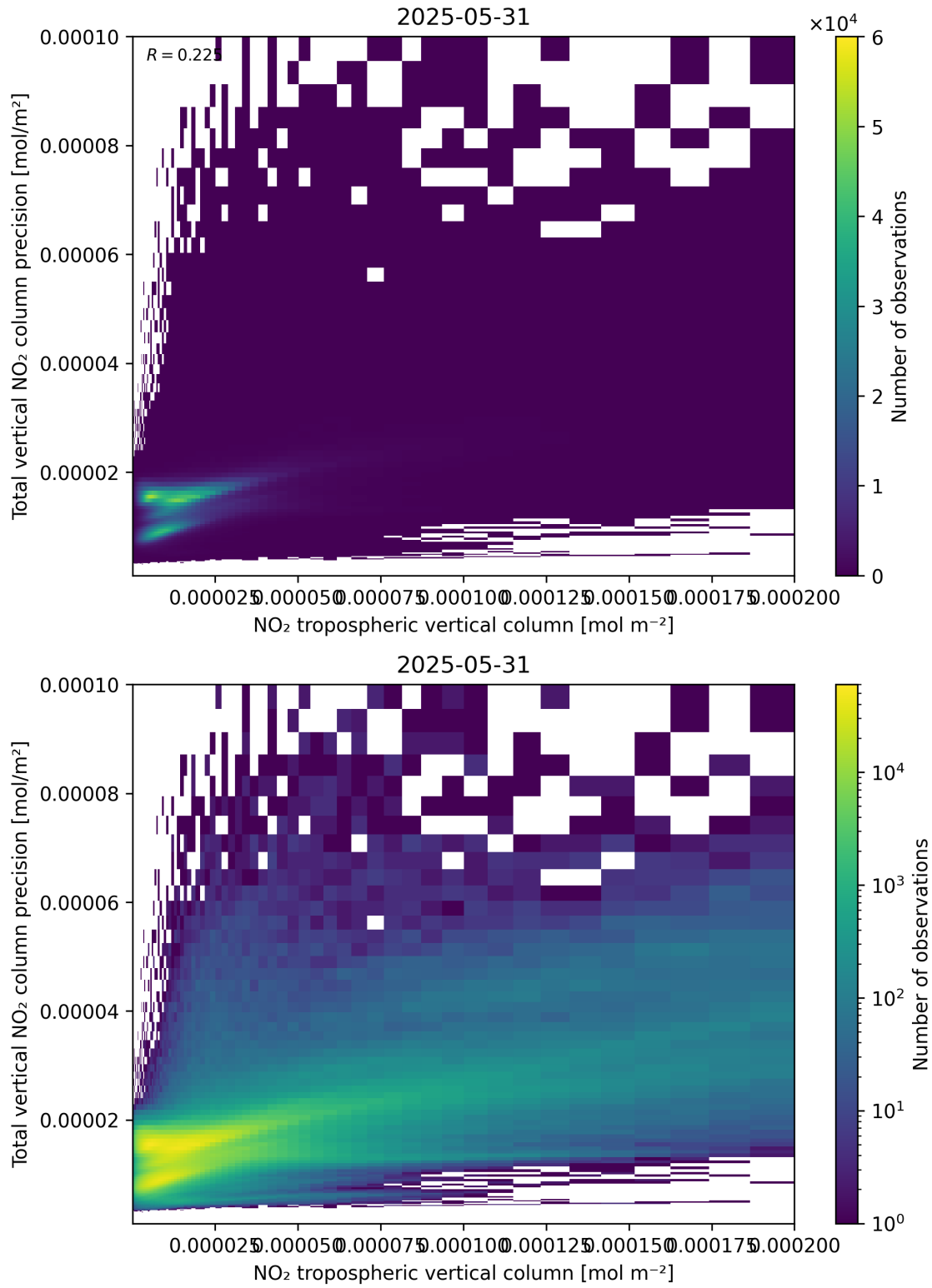
Figure 129: Scatter density plot of “NO 2 tropospheric vertical column” against “Total vertical NO 2 column precision” for 2025-05-31 to 2025-06-01.
