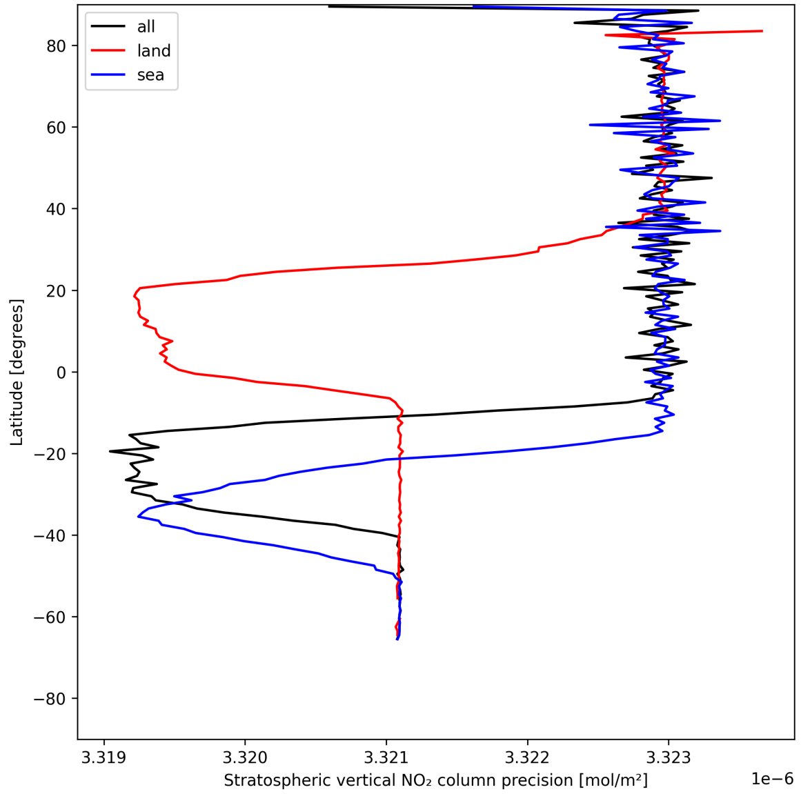
Figure 20: Zonal average of “Stratospheric vertical NO 2 column precision” for 2025-05-31 to 2025-06-01.
