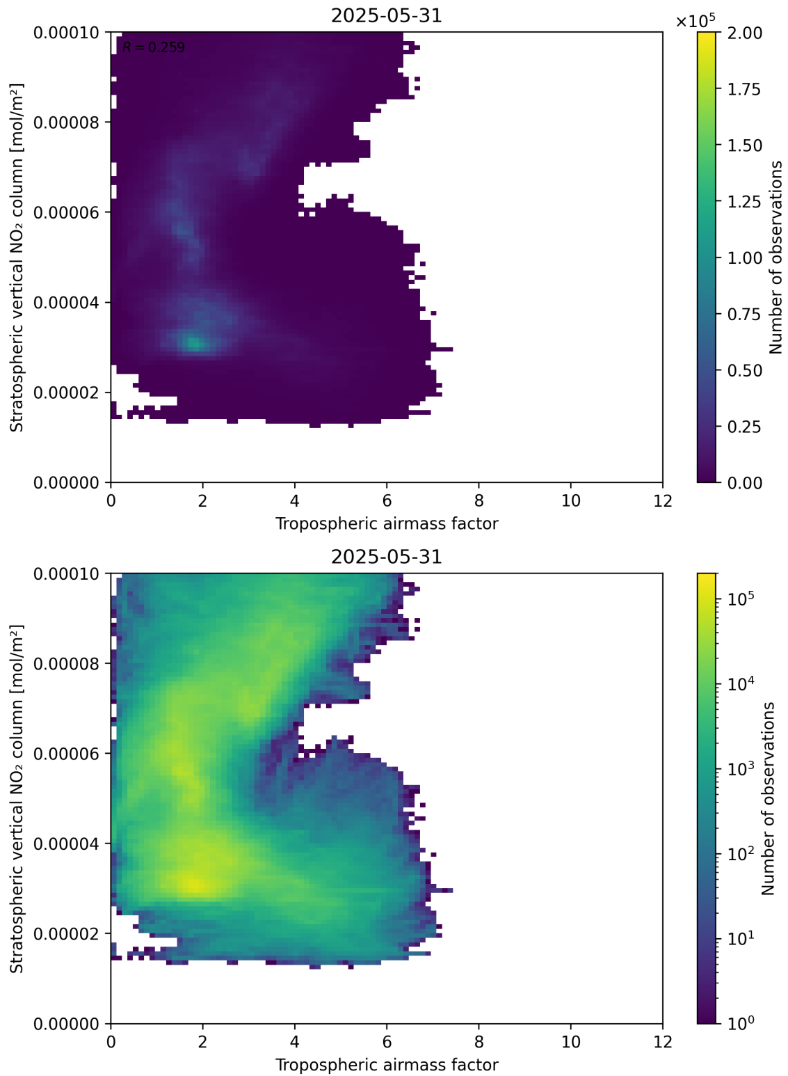
Figure 74: Scatter density plot of “Tropospheric airmass factor” against “Stratospheric vertical NO 2 column” for 2025-05-31 to 2025-06-01.
