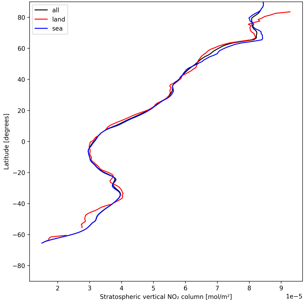
Figure 19: Zonal average of “Stratospheric vertical NO 2 column” for 2025-05-31 to 2025-06-01.
