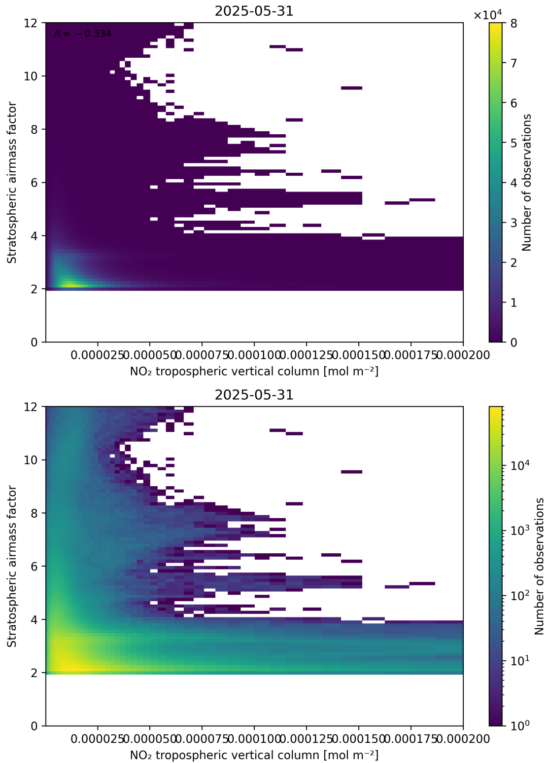
Figure 121: Scatter density plot of “NO 2 tropospheric vertical column” against “Stratospheric air mass factor” for 2025-05-31 to 2025-06-01.
