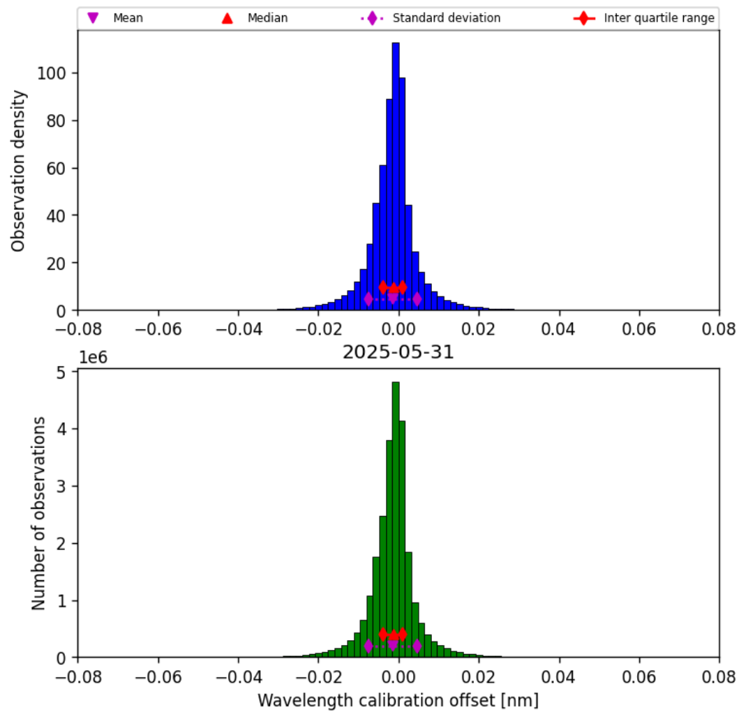
Figure 35: Histogram of “Wavelength calibration offset” for 2025-05-31 to 2025-06-01
