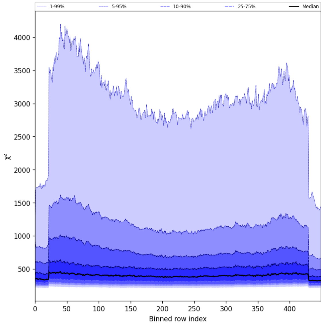
Figure 59: Along track statistics of “ \chi^2 ” for 2025-05-31 to 2025-06-01
