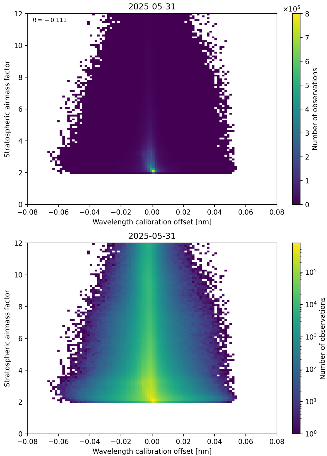
Figure 174: Scatter density plot of “Wavelength calibration offset” against “Stratospheric airmass factor” for 2025-05-31 to 2025-06-01.
