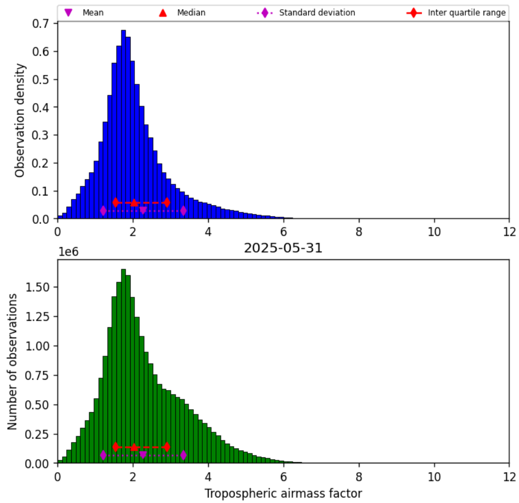
Figure 31: Histogram of “Tropospheric airmass factor” for 2025-05-31 to 2025-06-01
