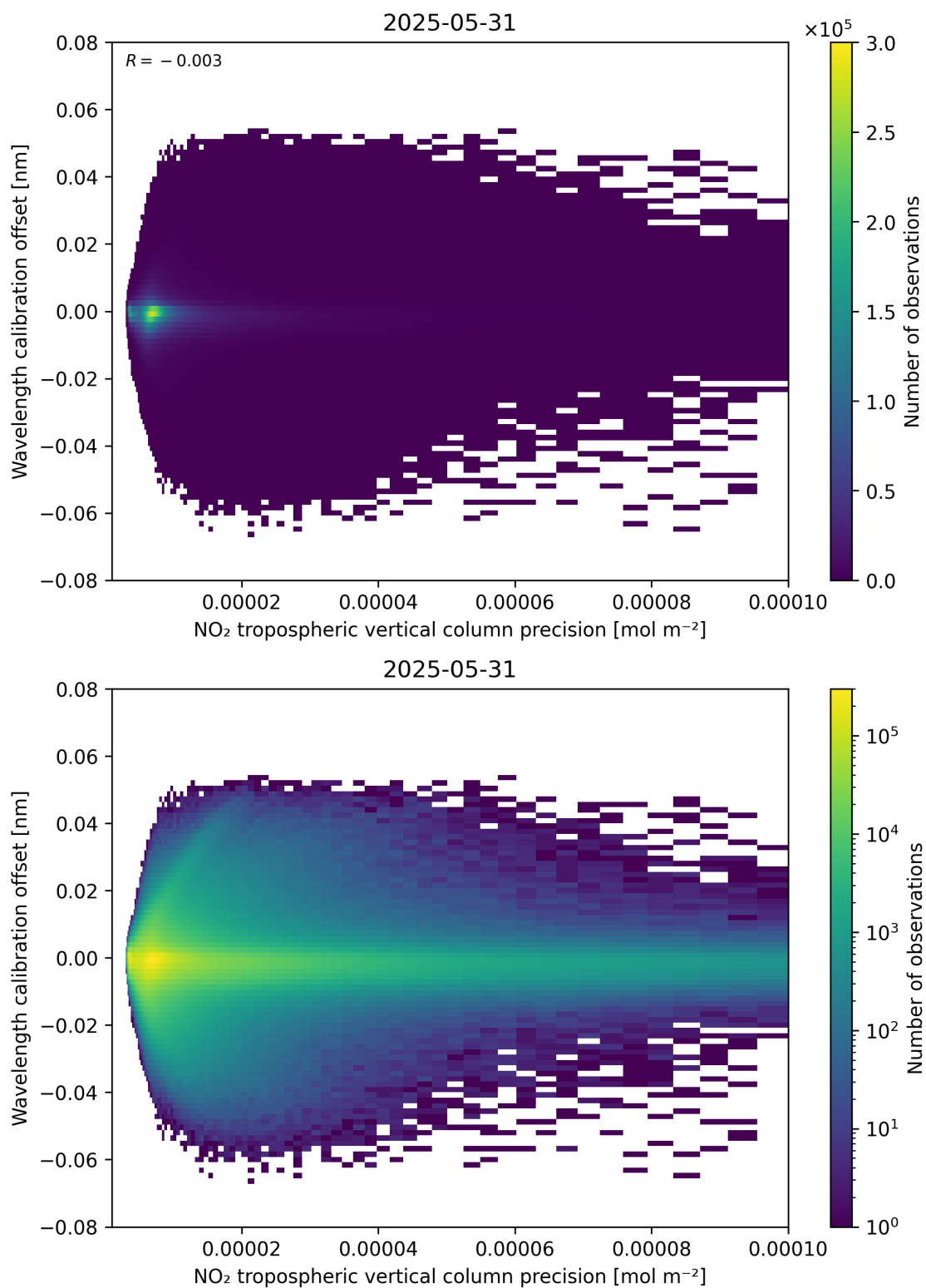
Figure 141: Scatter density plot of “NO 2 tropospheric vertical column precision” against “Wavelength calibration offset” for 2025-05-31 to 2025-06-01.
