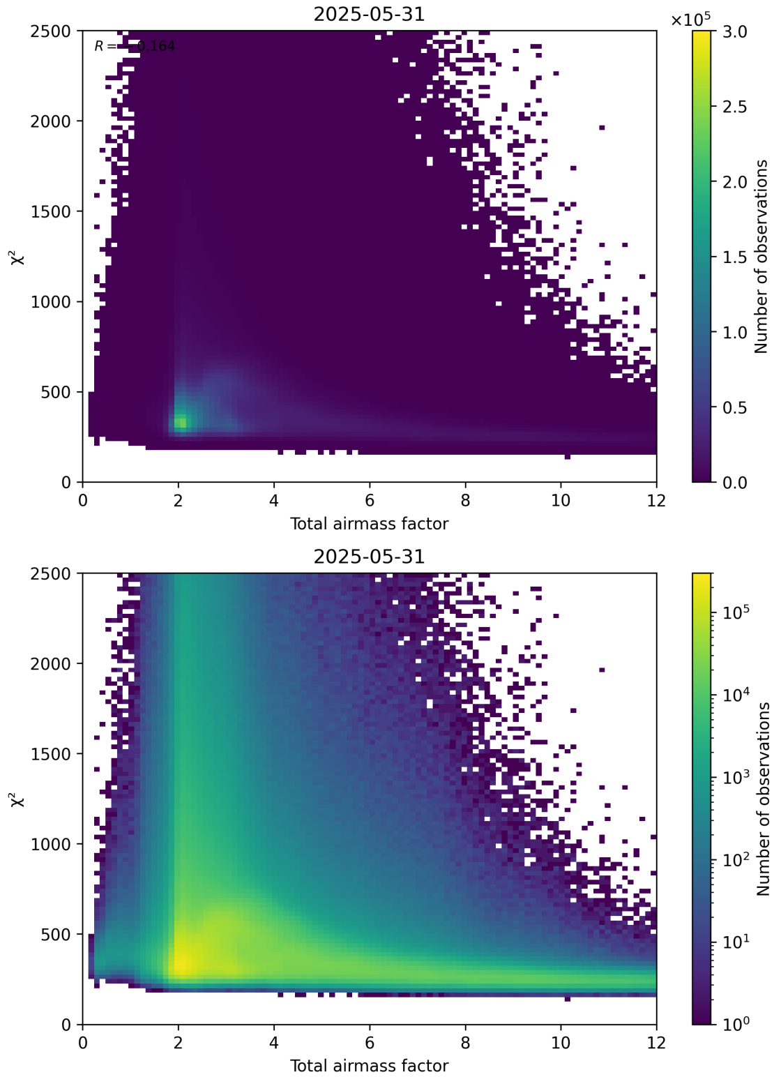
Figure 63: Scatter density plot of “Total airmass factor” against “ \chi^2 ” for 2025-05-31 to 2025-06-01.
