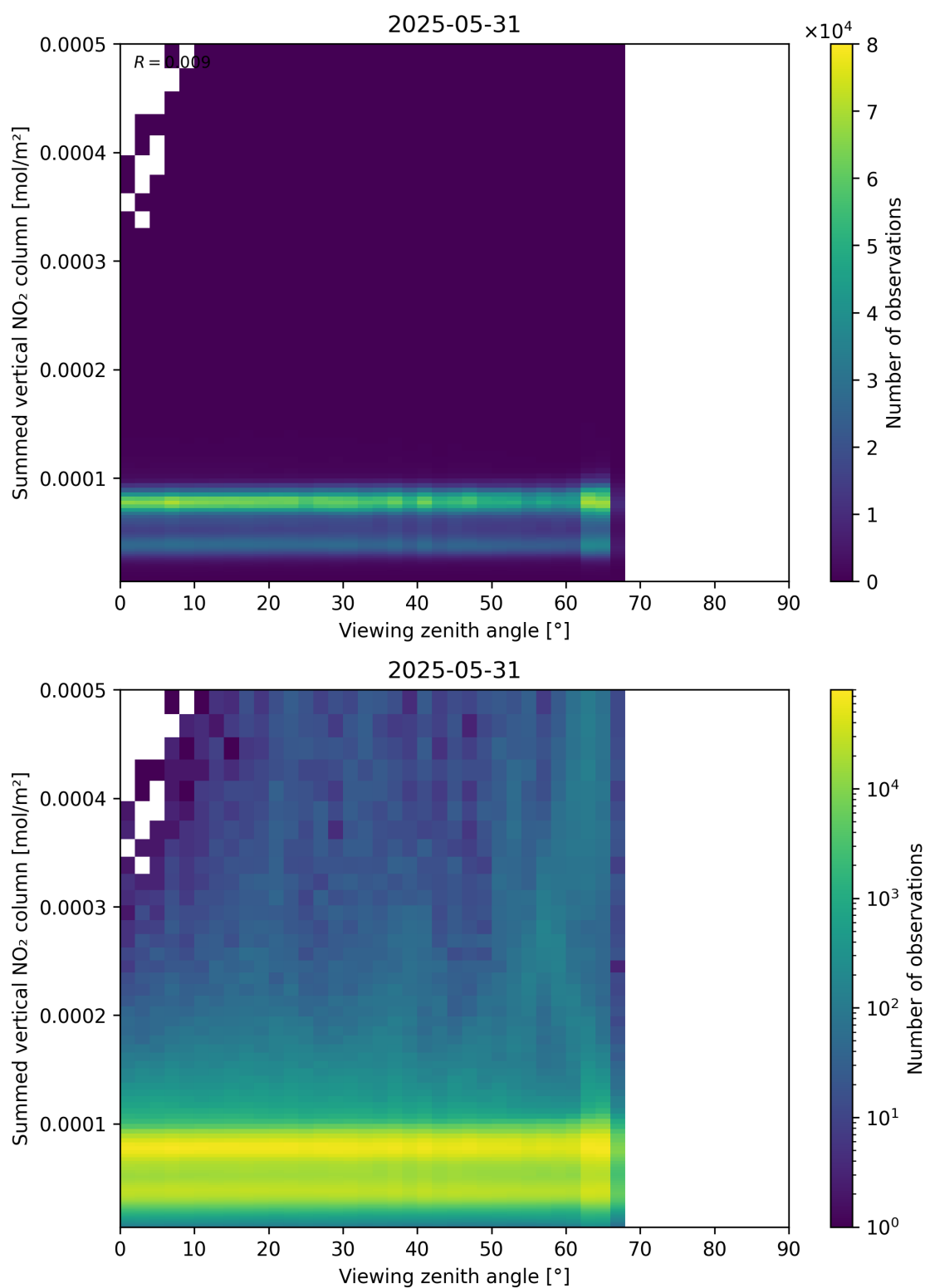
Figure 165: Scatter density plot of “Viewing zenith angle” against “Summed vertical NO 2 column” for 2025-05-31 to 2025-06-01.
