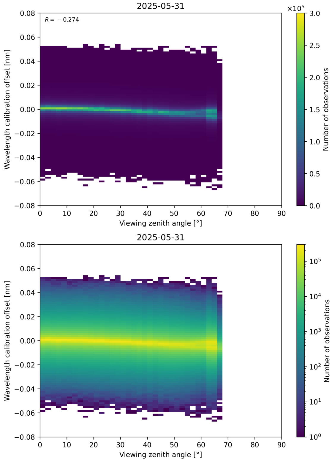
Figure 173: Scatter density plot of “Viewing zenith angle” against “Wavelength calibration offset” for 2025-05-31 to 2025-06-01.
