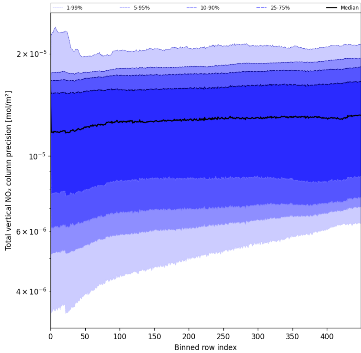
Figure 56: Along track statistics of “Total vertical NO 2 column precision” for 2025-05-31 to 2025-06-01
