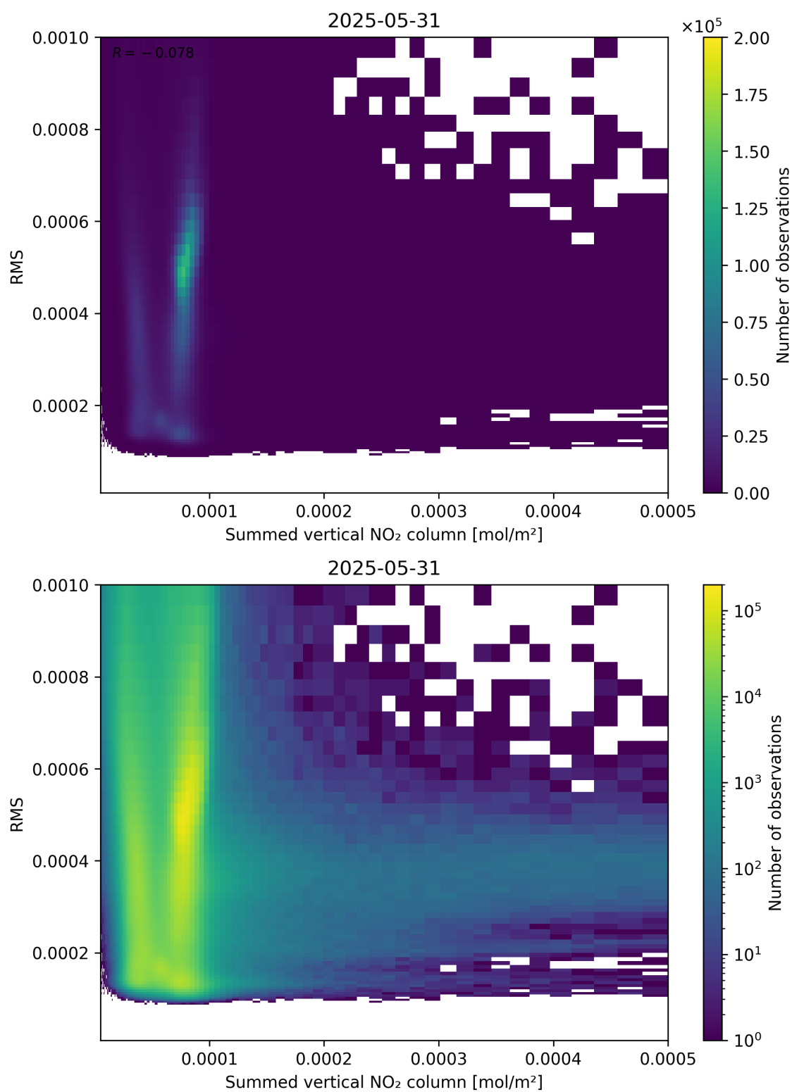
Figure 109: Scatter density plot of “Summed vertical NO 2 column” against “RMS” for 2025-05-31 to 2025-06-01.
