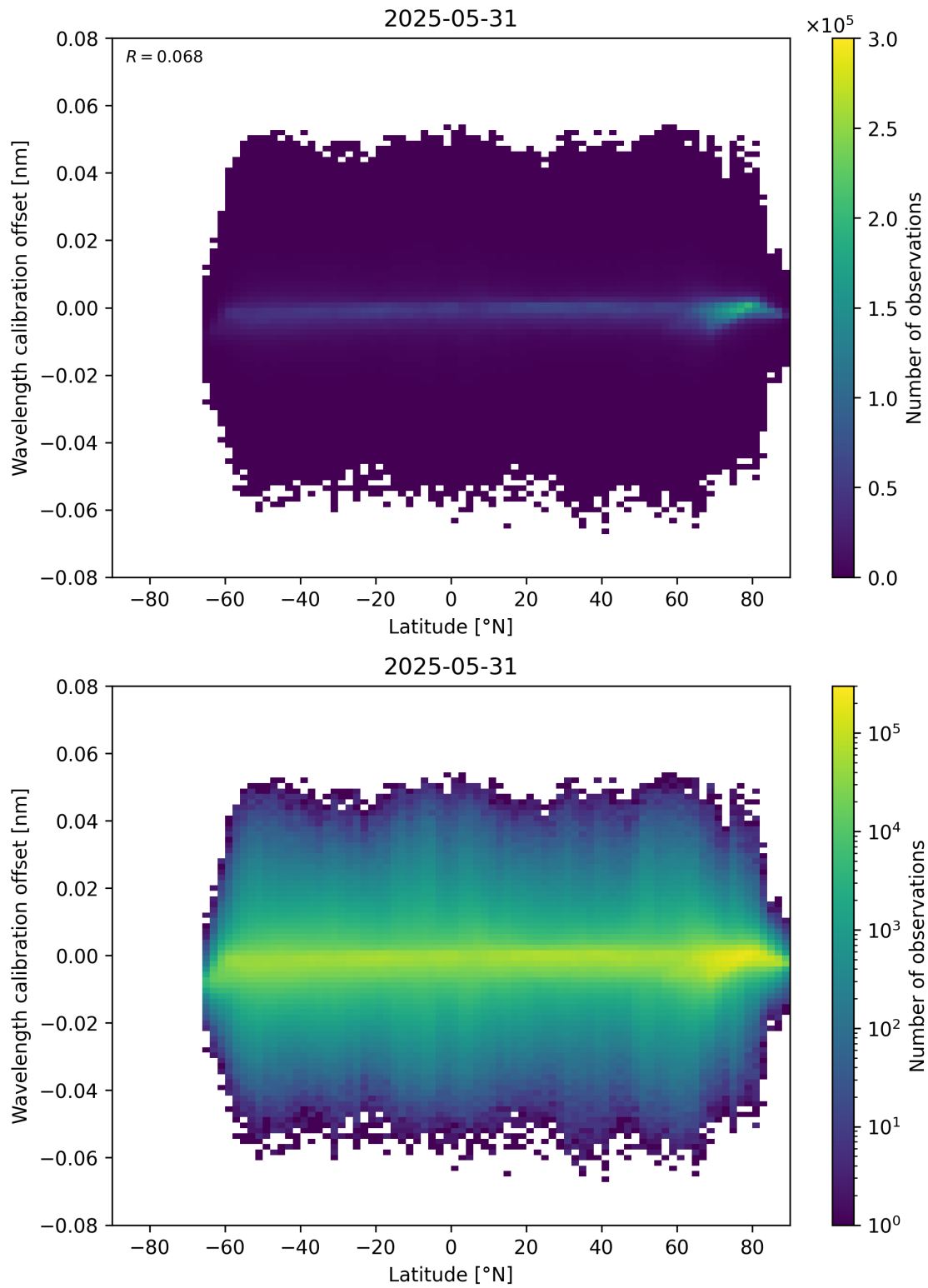
Figure 95: Scatter density plot of “Latitude” against “Wavelength calibration offset” for 2025-05-31 to 2025-06-01.
