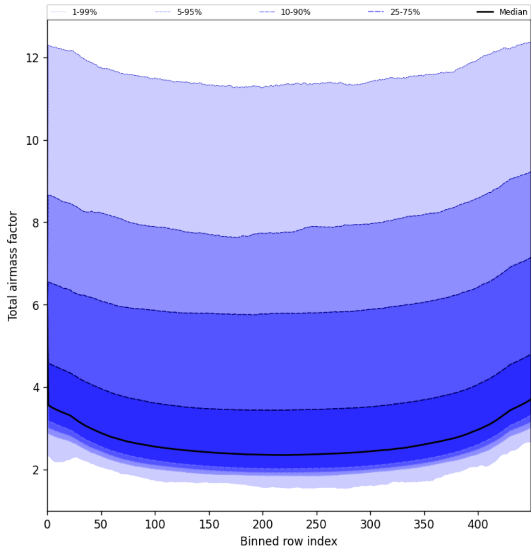
Figure 49: Along track statistics of “Total airmass factor” for 2025-05-31 to 2025-06-01
