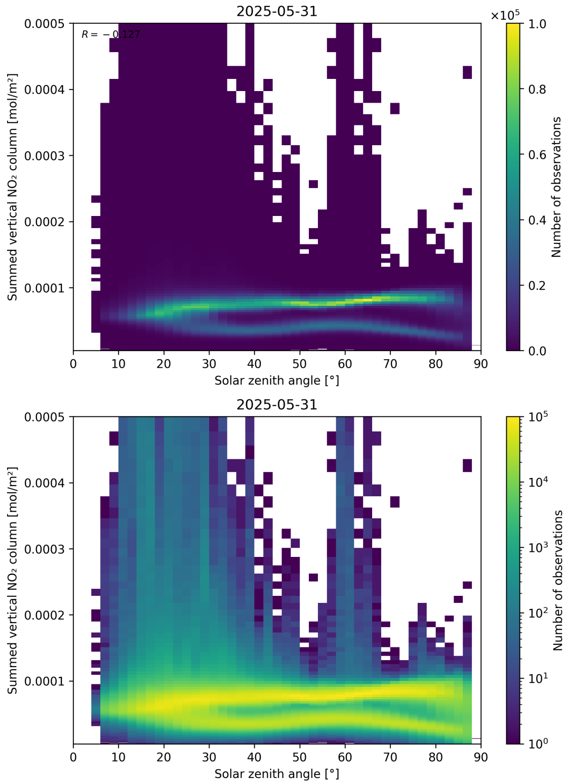
Figure 151: Scatter density plot of “Solar zenith angle” against “Summed vertical NO 2 column” for 2025-05-31 to 2025-06-01.
