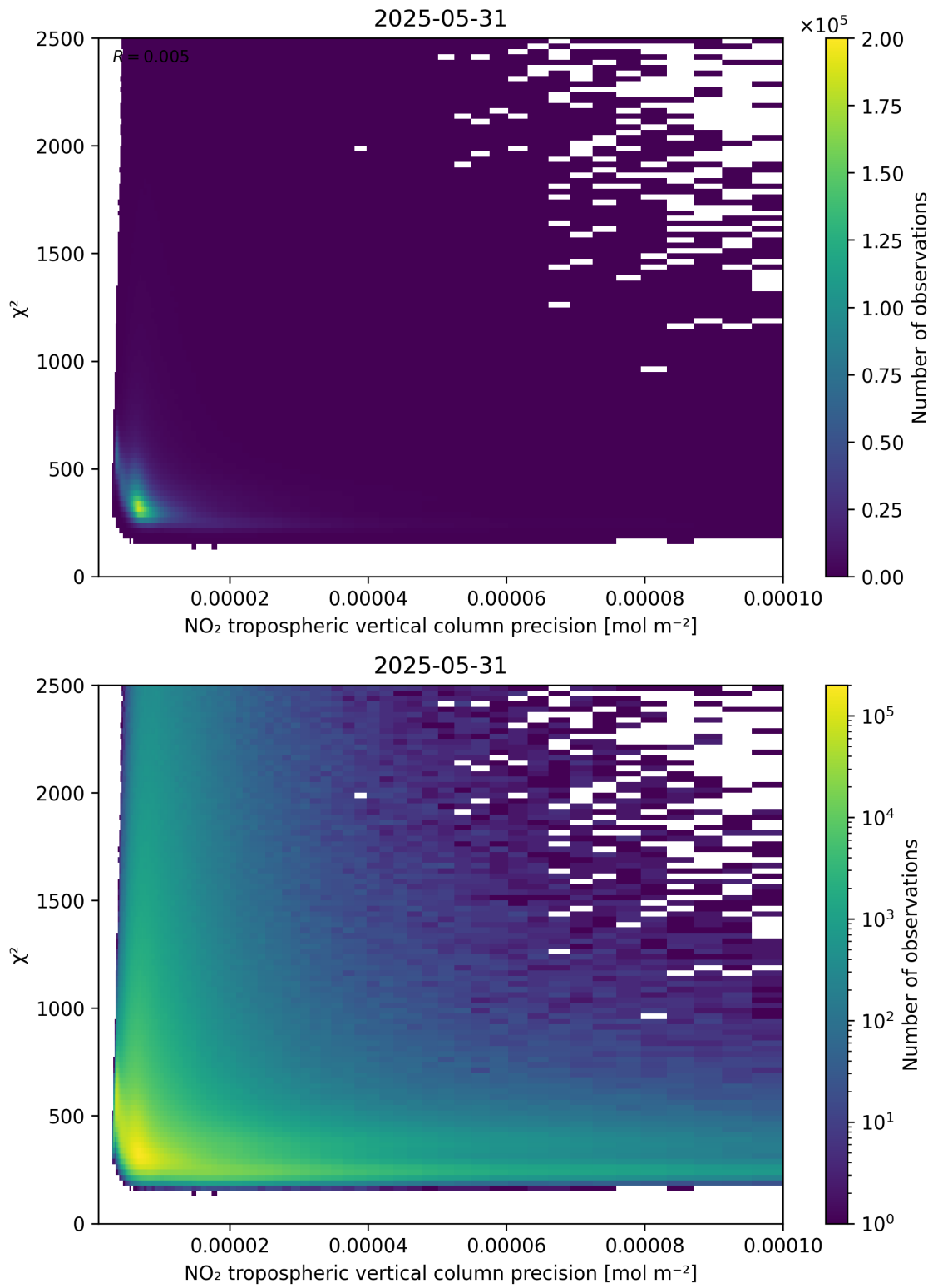
Figure 134: Scatter density plot of “NO 2 tropospheric vertical column precision” against “ \chi^2 ” for 2025-05-31 to 2025-06-01.
