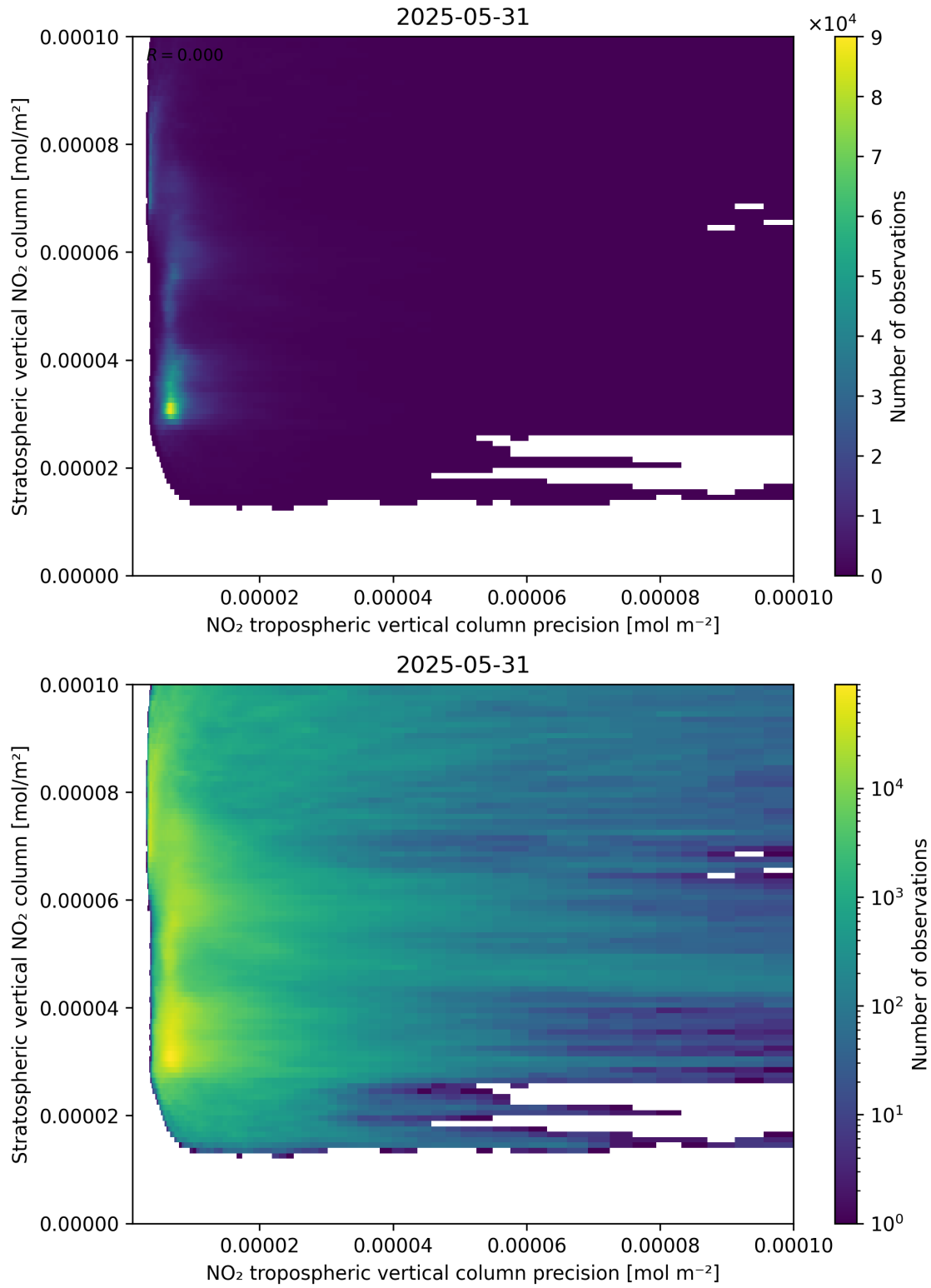
Figure 135: Scatter density plot of “NO 2 tropospheric vertical column precision” against “Stratospheric vertical NO 2 column” for 2025-05-31 to 2025-06-01.
