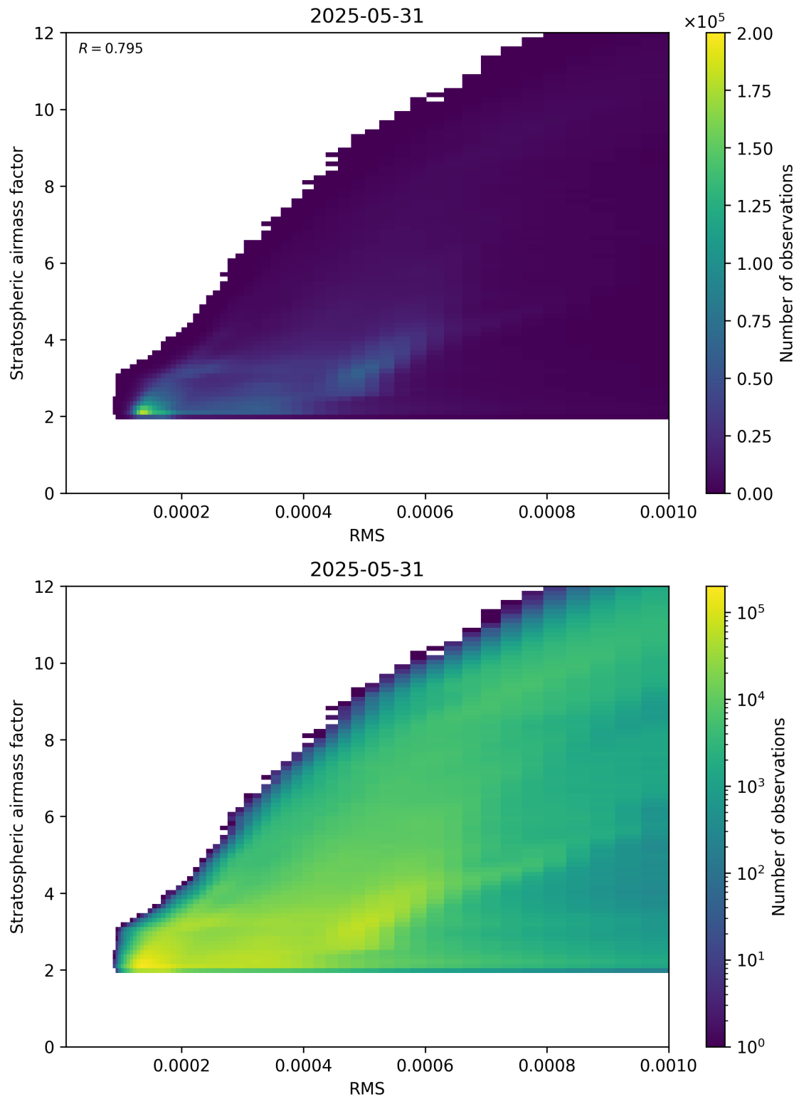
Figure 144: Scatter density plot of “RMS” against “Stratospheric airmass factor” for 2025-05-31 to 2025-06-01.
