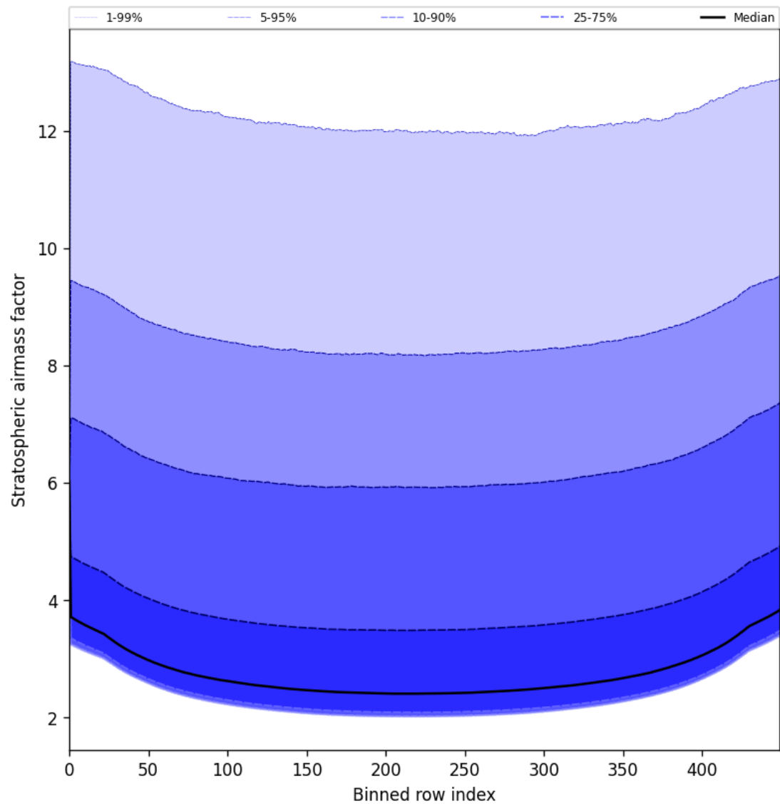
Figure 61: Along track statistics of “Stratospheric airmass factor” for 2025-05-31 to 2025-06-01
