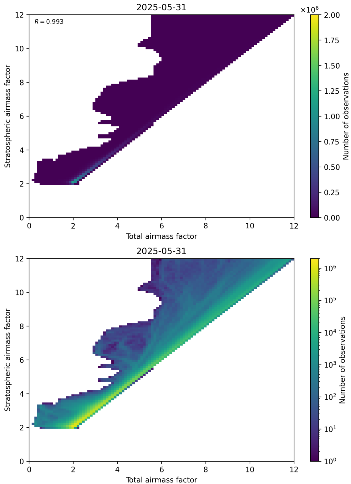
Figure 62: Scatter density plot of “Total airmass factor” against “Stratospheric airmass factor” for 2025-05-31 to 2025-06-01.
