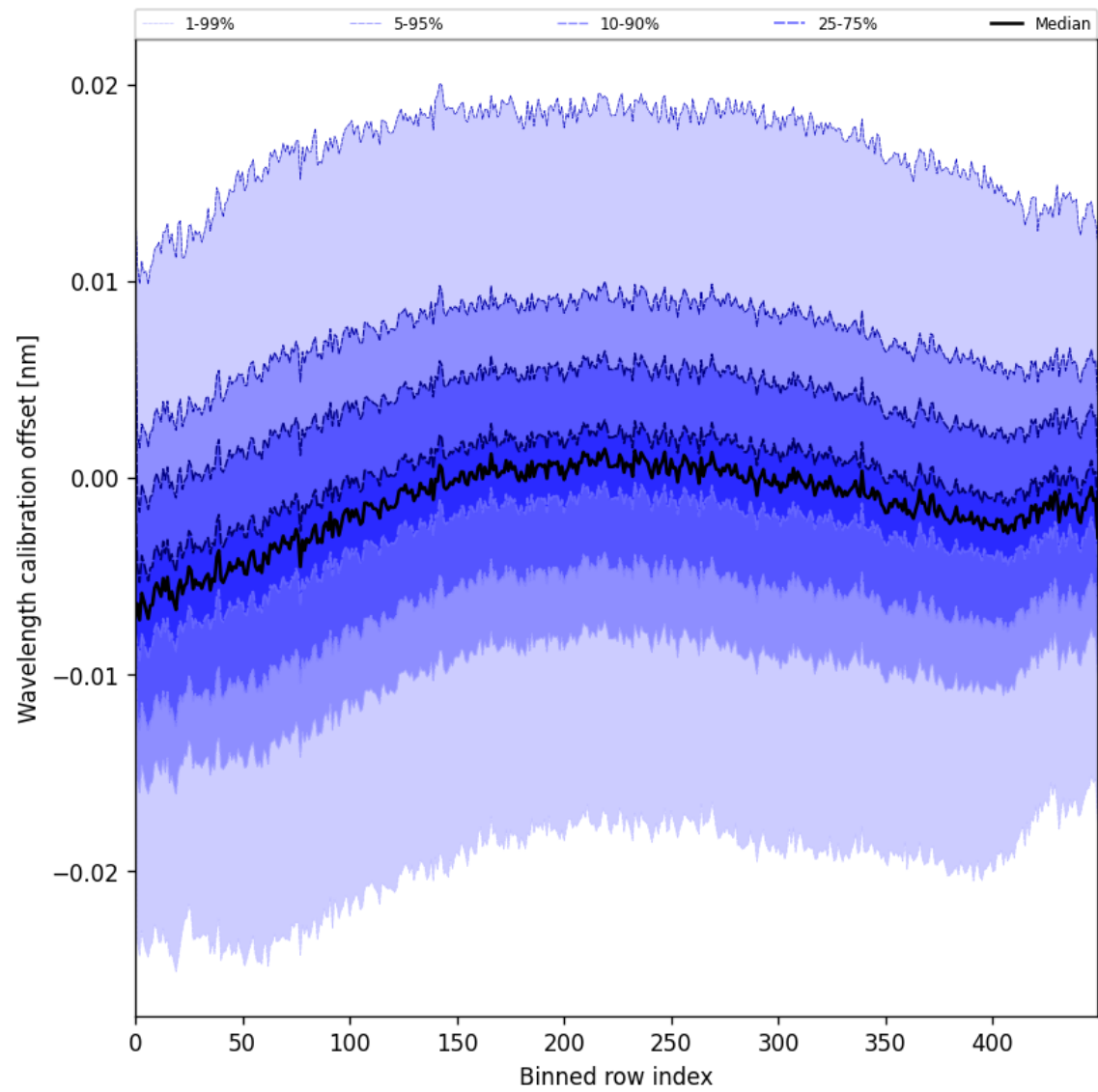
Figure 52: Along track statistics of “Wavelength calibration offset” for 2025-05-31 to 2025-06-01
