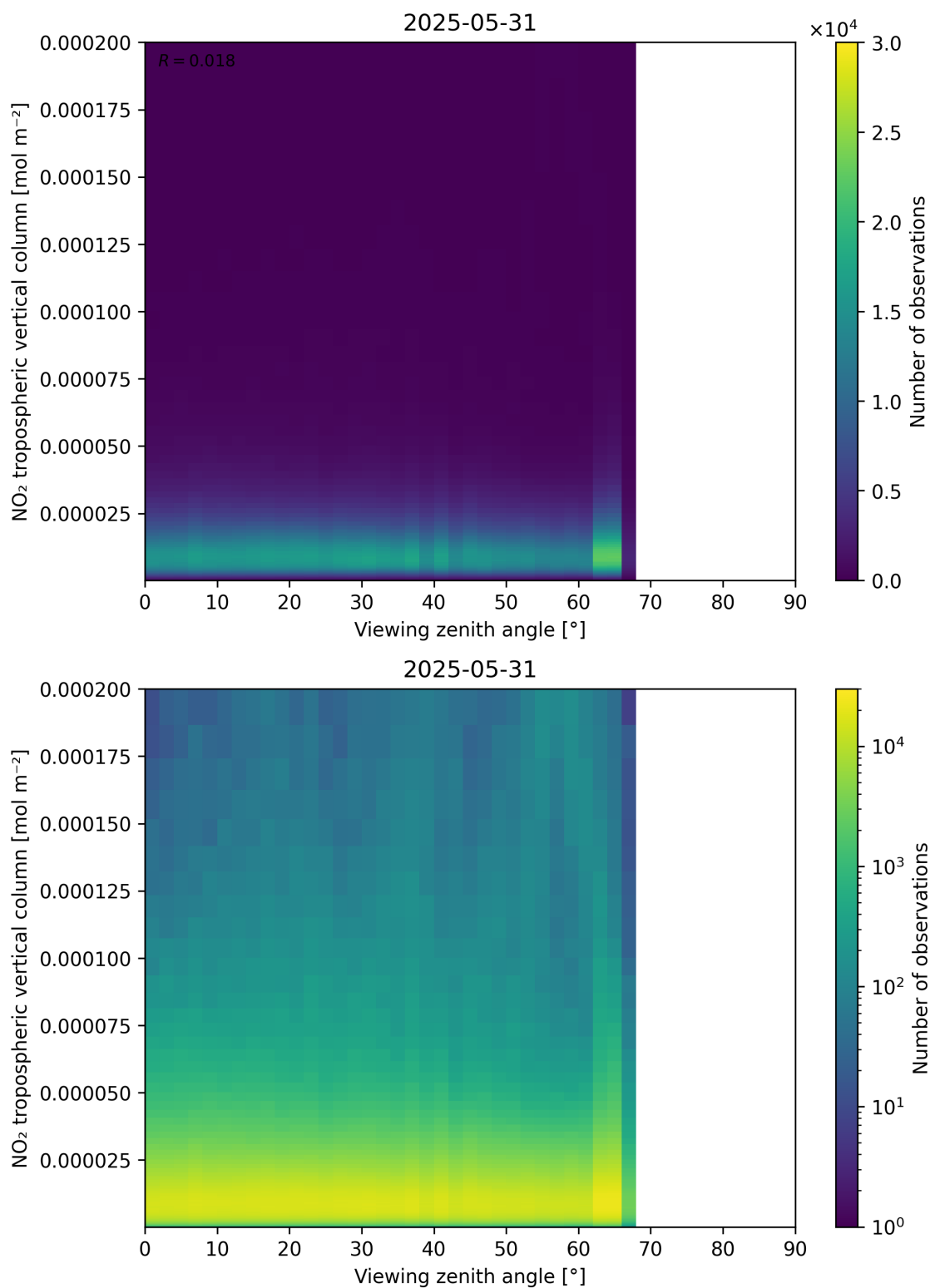
Figure 169: Scatter density plot of “Viewing zenith angle” against “NO 2 tropospheric vertical column” for 2025-05-31 to 2025-06-01.
