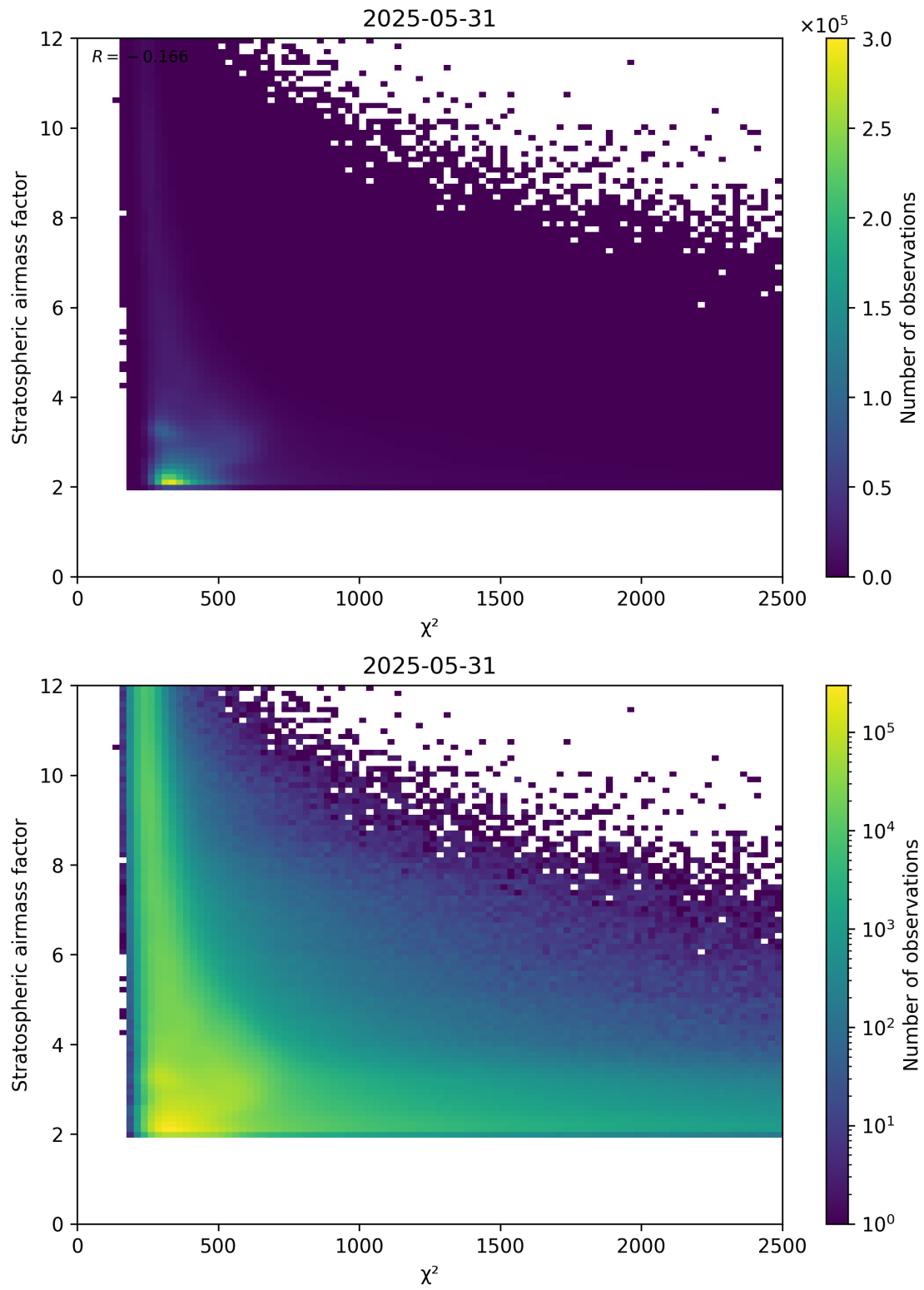
Figure 81: Scatter density plot of “ \chi^2 ” against “Stratospheric airmass factor” for 2025-05-31 to 2025-06-01.
