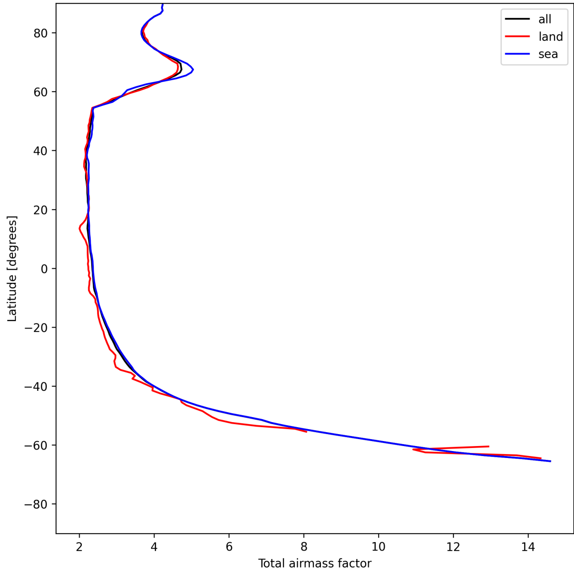
Figure 15: Zonal average of “Total airmass factor” for 2025-05-31 to 2025-06-01.
