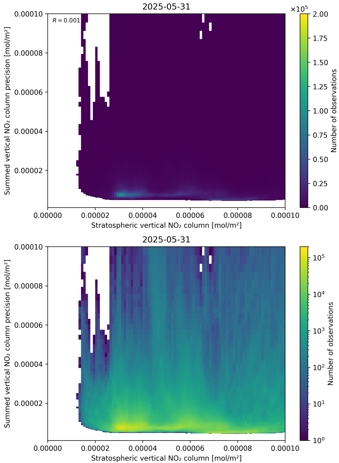
Figure 99: Scatter density plot of “Stratospheric vertical NO 2 column” against “Summed vertical NO 2 column precision” for 2025-05-31 to 2025-06-01.
