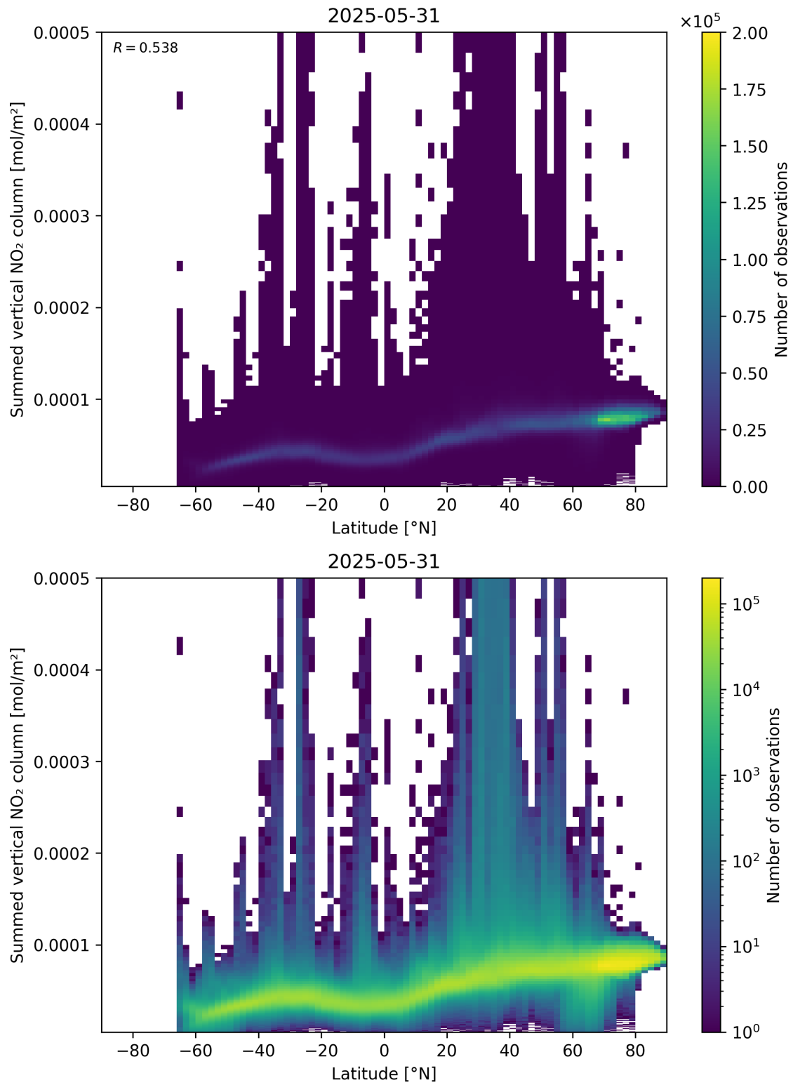
Figure 88: Scatter density plot of “Latitude” against “Summed vertical NO 2 column” for 2025-05-31 to 2025-06-01.
