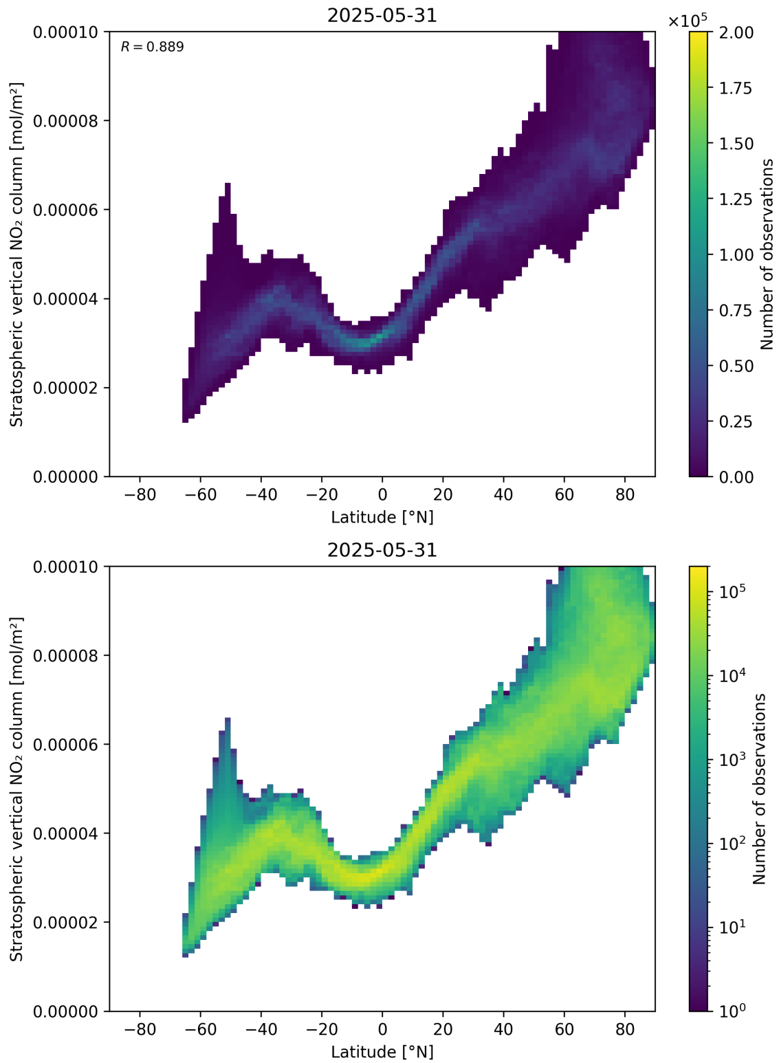
Figure 87: Scatter density plot of “Latitude” against “Stratospheric vertical \text{NO}_2 column” for 2025-05-31 to 2025-06-01.
