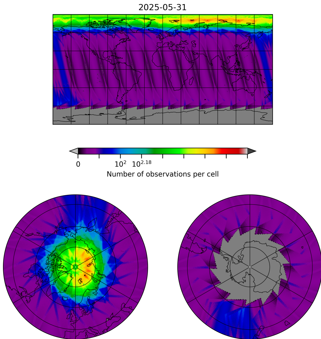
Figure 10: Map of the number of observations for 2025-05-31 to 2025-06-01
