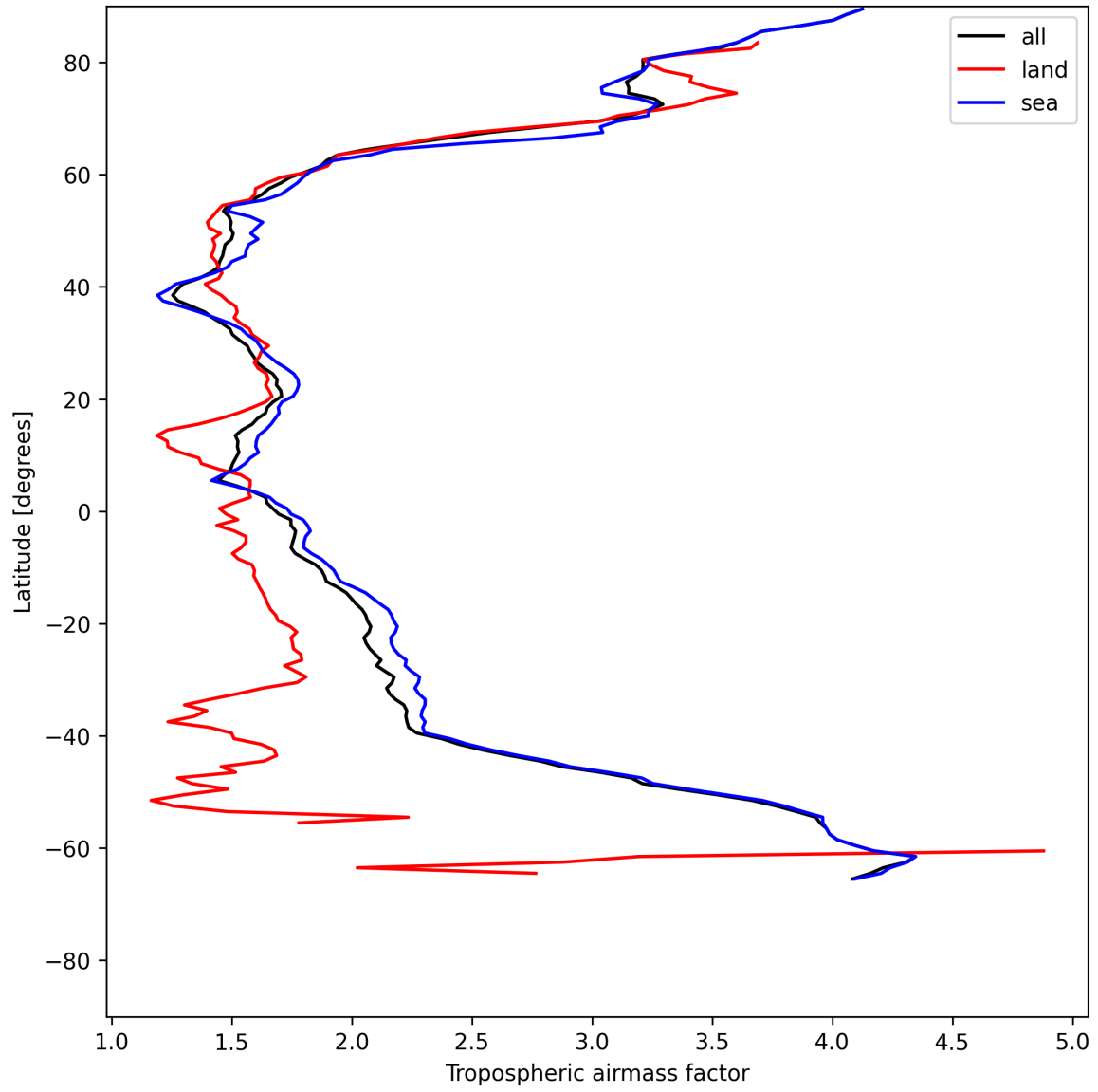
Figure 14: Zonal average of “Tropospheric airmass factor” for 2025-05-31 to 2025-06-01.
