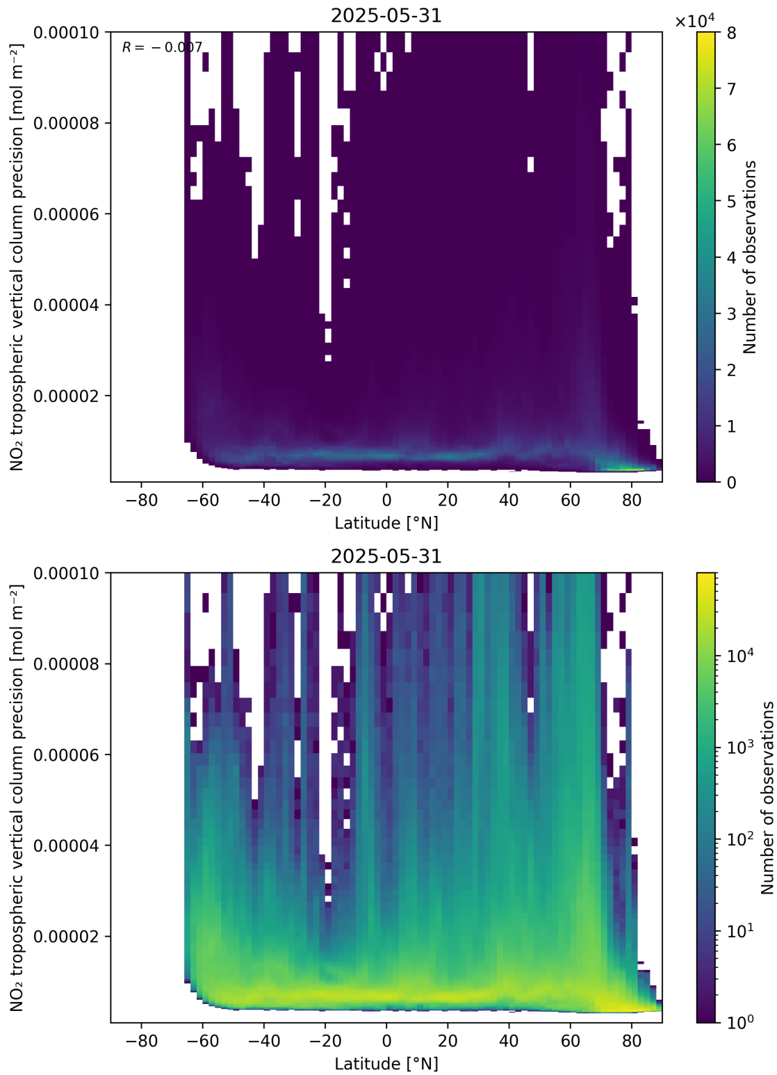
Figure 93: Scatter density plot of “Latitude” against “NO 2 tropospheric vertical column precision” for 2025-05-31 to 2025-06-01.
