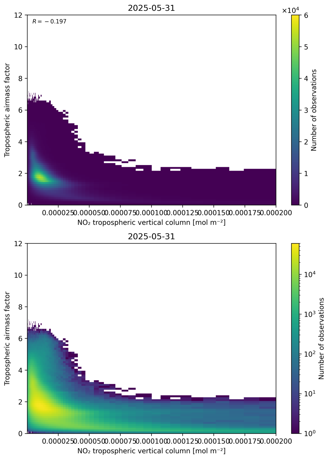
Figure 123: Scatter density plot of “NO 2 tropospheric vertical column” against “Tropospheric air mass factor” for 2025-05-31 to 2025-06-01.
