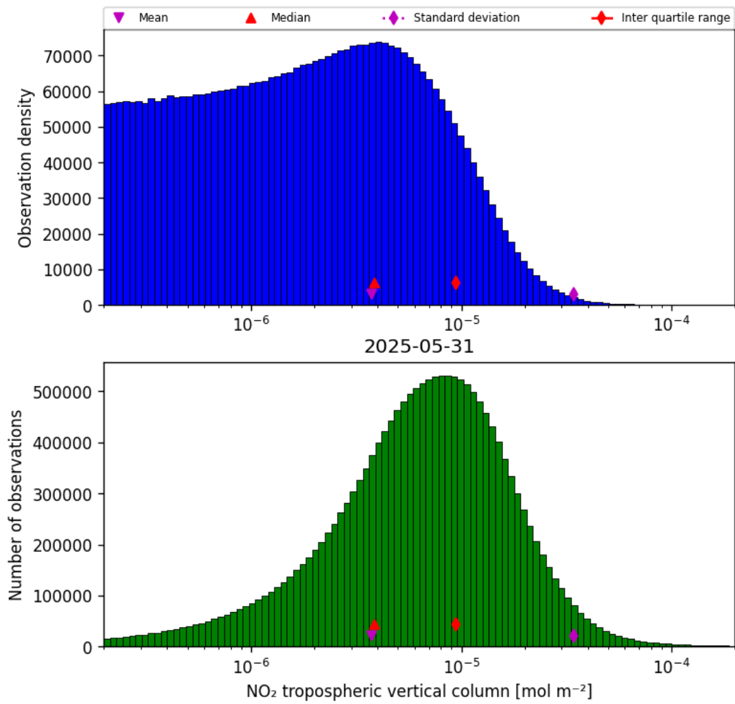
Figure 29: Histogram of “NO 2 tropospheric vertical column” for 2025-05-31 to 2025-06-01
