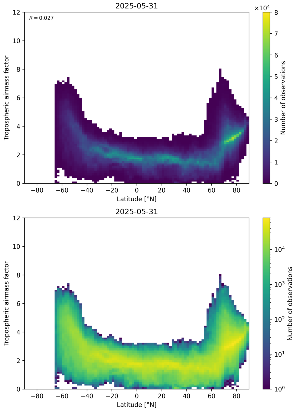
Figure 85: Scatter density plot of “Latitude” against “Tropospheric air mass factor” for 2025-05-31 to 2025-06-01.
