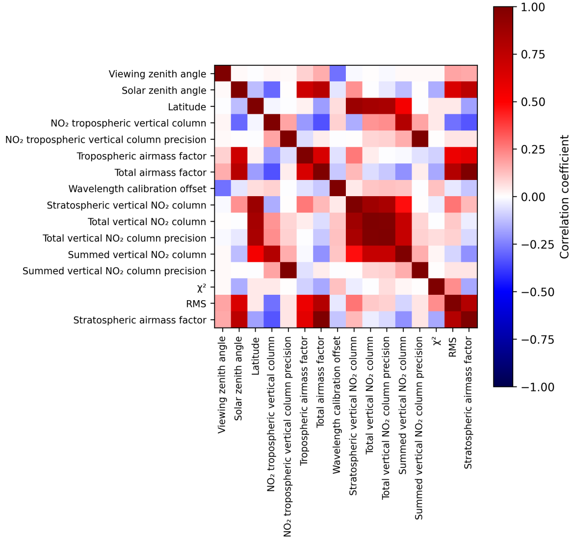
Figure 2: Map of correlation matrix for 2025-05-31 to 2025-06-01.
