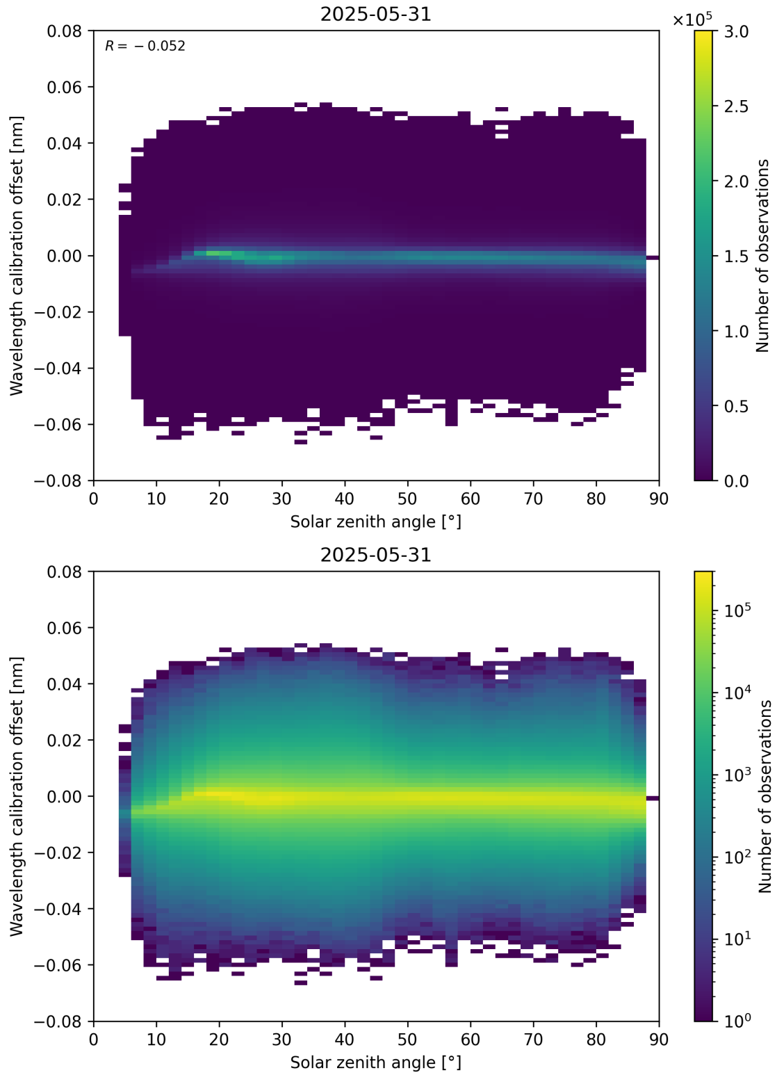
Figure 158: Scatter density plot of “Solar zenith angle” against “Wavelength calibration offset” for 2025-05-31 to 2025-06-01.
