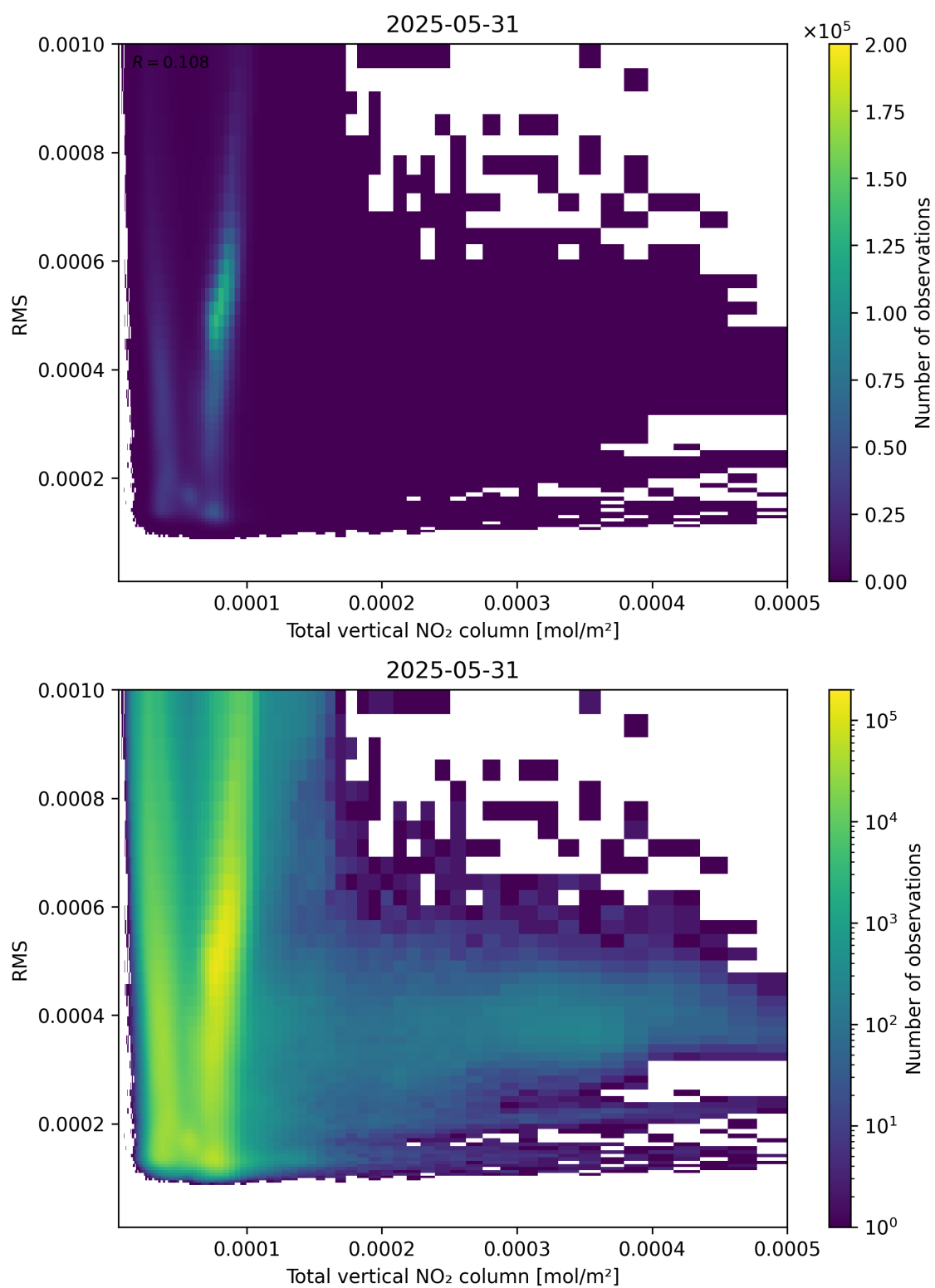
Figure 120: Scatter density plot of “Total vertical NO 2 column” against “RMS” for 2025-05-31 to 2025-06-01.
