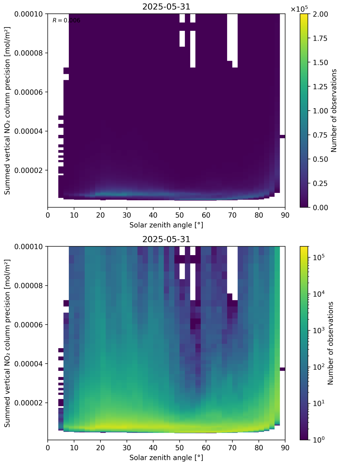
Figure 152: Scatter density plot of “Solar zenith angle” against “Summed vertical NO 2 column precision” for 2025-05-31 to 2025-06-01.
