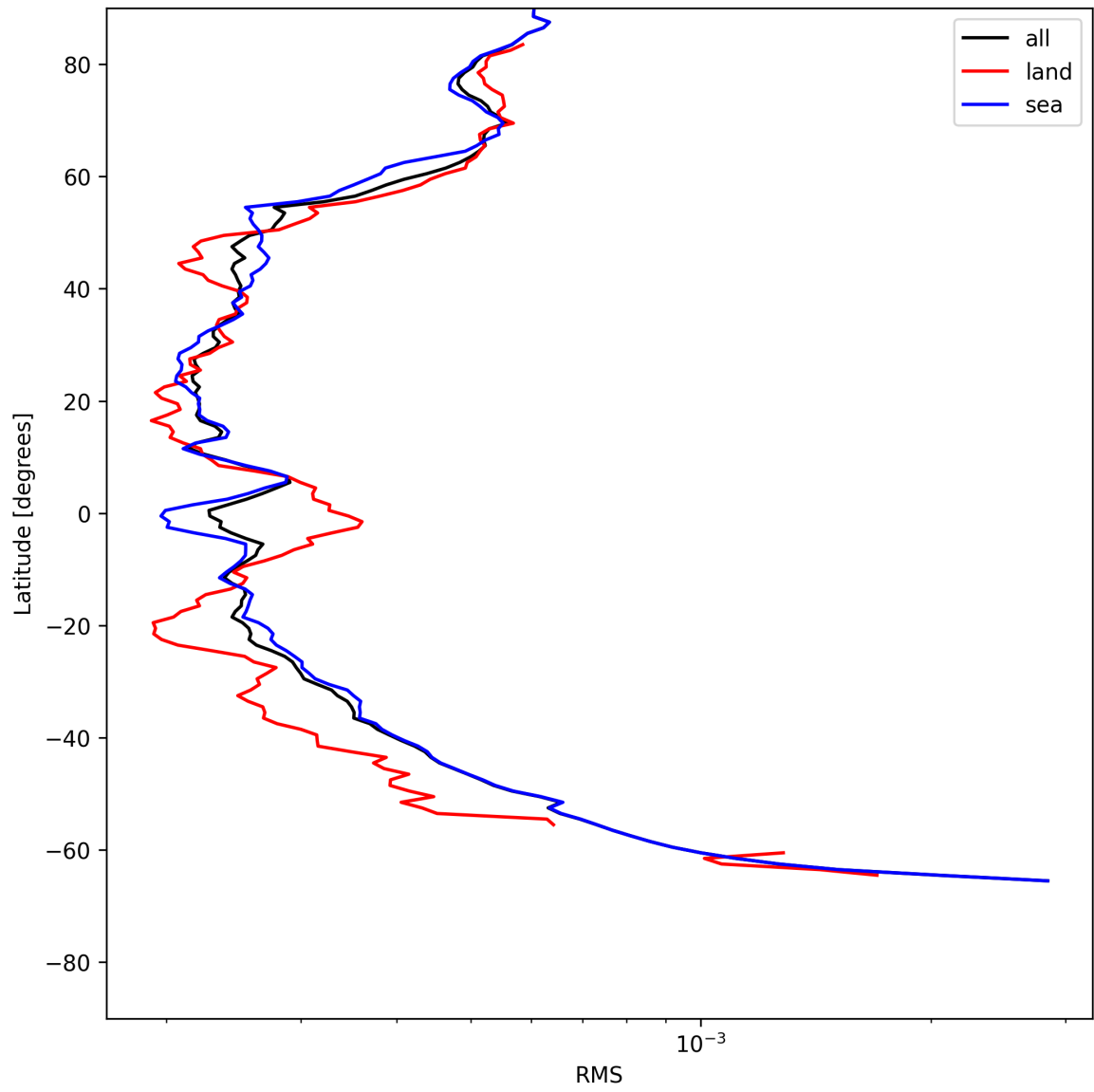
Figure 26: Zonal average of “RMS” for 2025-05-31 to 2025-06-01.
