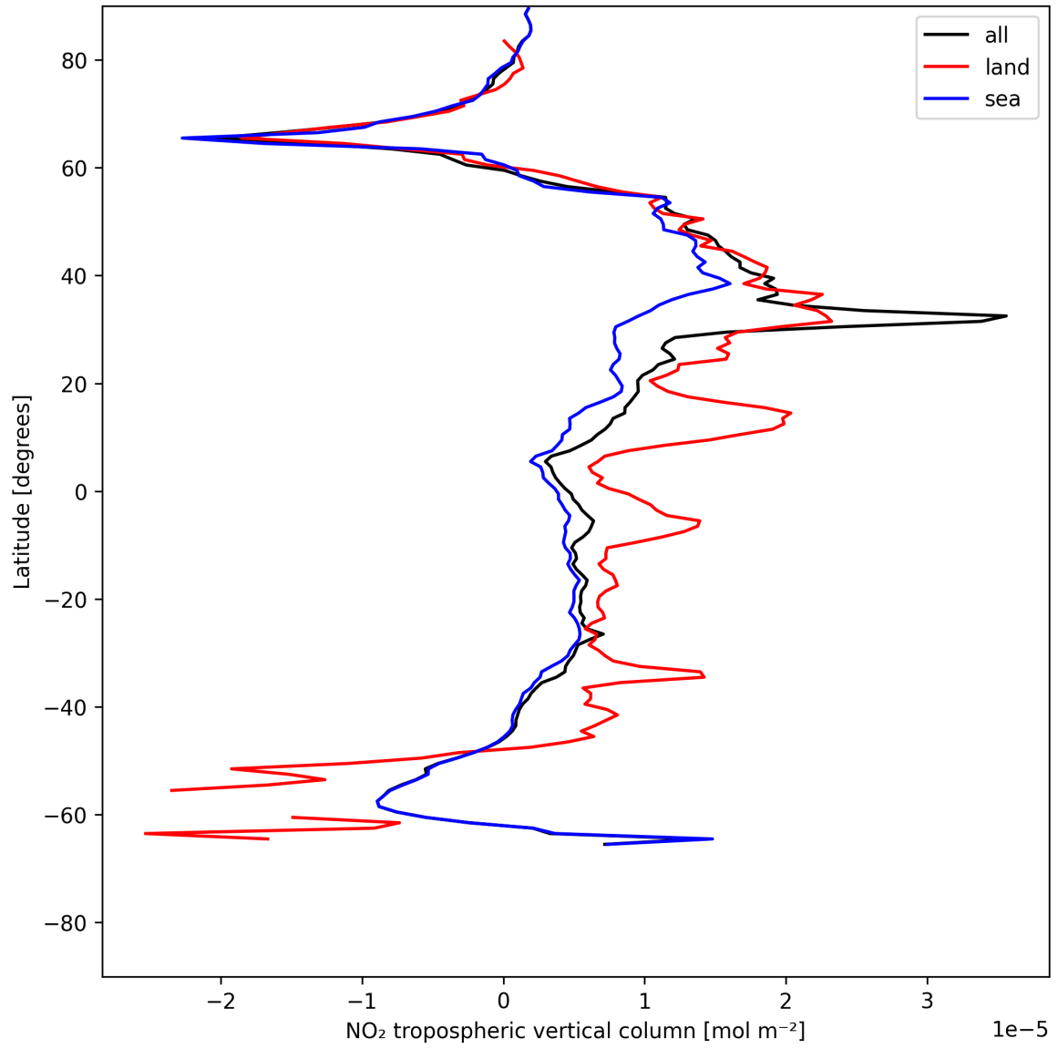
Figure 12: Zonal average of “NO 2 tropospheric vertical column” for 2025-05-31 to 2025-06-01.
