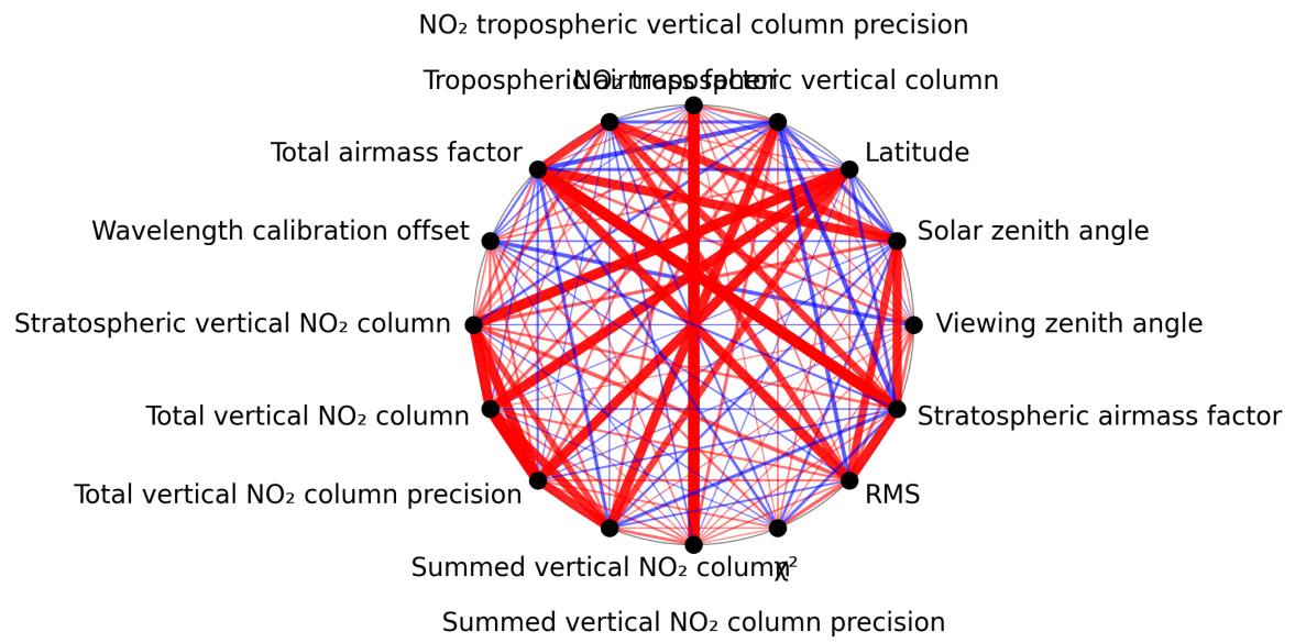
Figure 1: Map of correlation graph for 2025-05-31 to 2025-06-01.
