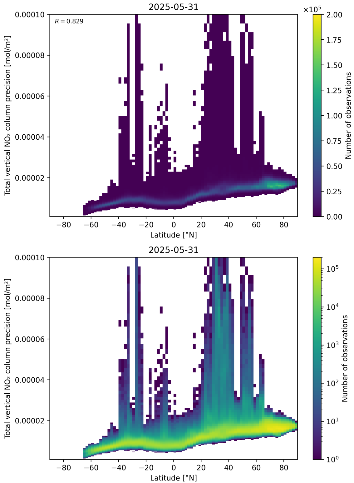
Figure 91: Scatter density plot of “Latitude” against “Total vertical NO 2 column precision” for 2025-05-31 to 2025-06-01.
