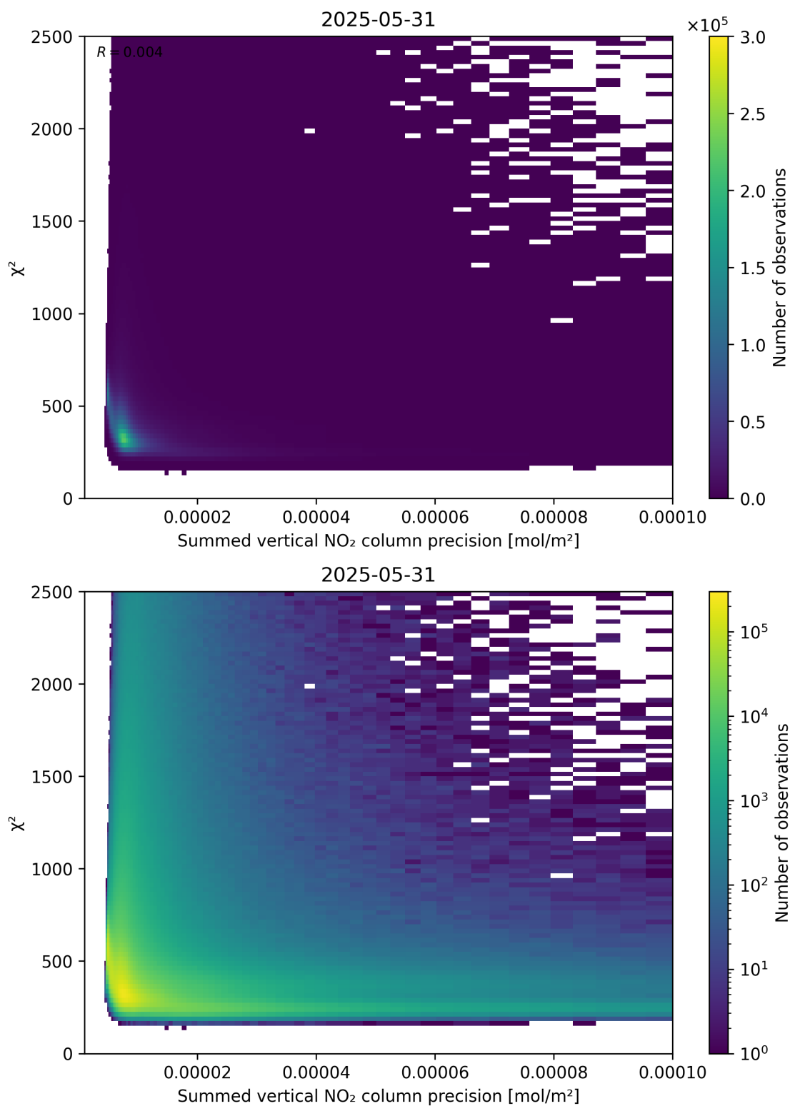
Figure 107: Scatter density plot of “Summed vertical NO 2 column precision” against “ \chi^2 ” for 2025-05-31 to 2025-06-01.
