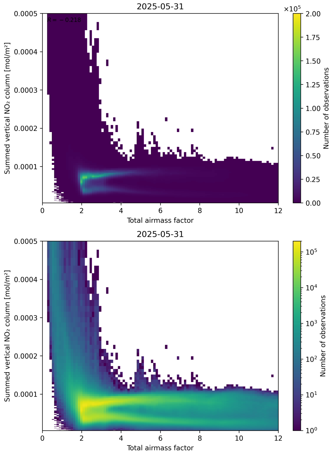
Figure 65: Scatter density plot of “Total airmass factor” against “Summed vertical NO 2 column” for 2025-05-31 to 2025-06-01.
