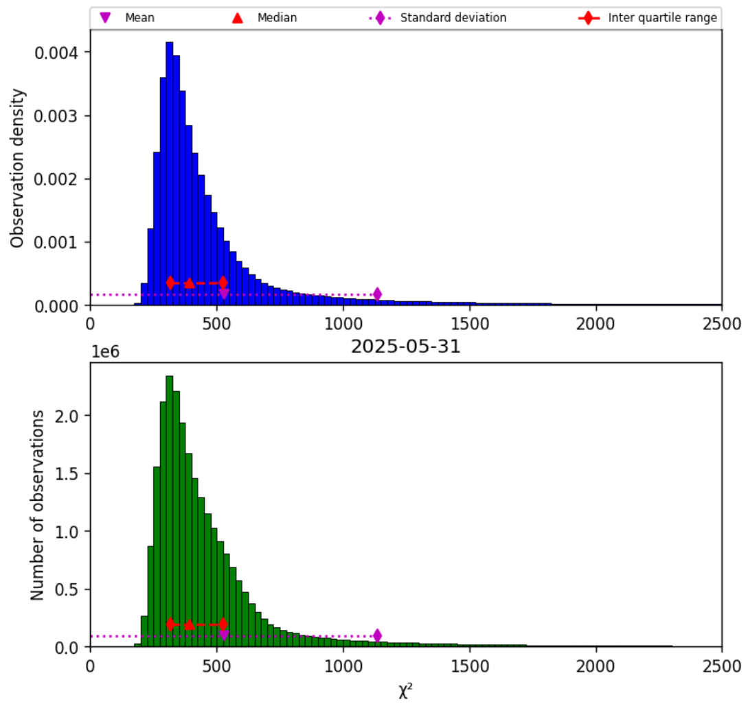
Figure 42: Histogram of “ \chi^2 ” for 2025-05-31 to 2025-06-01
