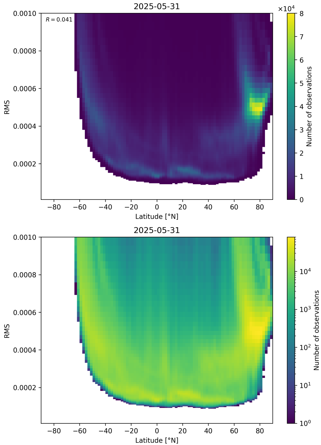
Figure 94: Scatter density plot of “Latitude” against “RMS” for 2025-05-31 to 2025-06-01.
