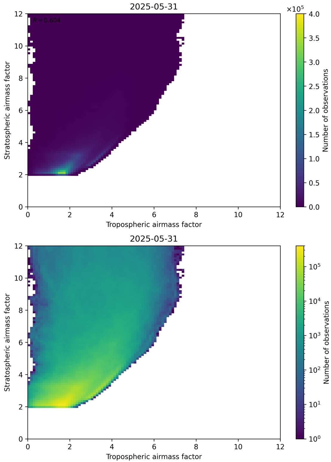
Figure 71: Scatter density plot of “Tropospheric airmass factor” against “Stratospheric airmass factor” for 2025-05-31 to 2025-06-01.
