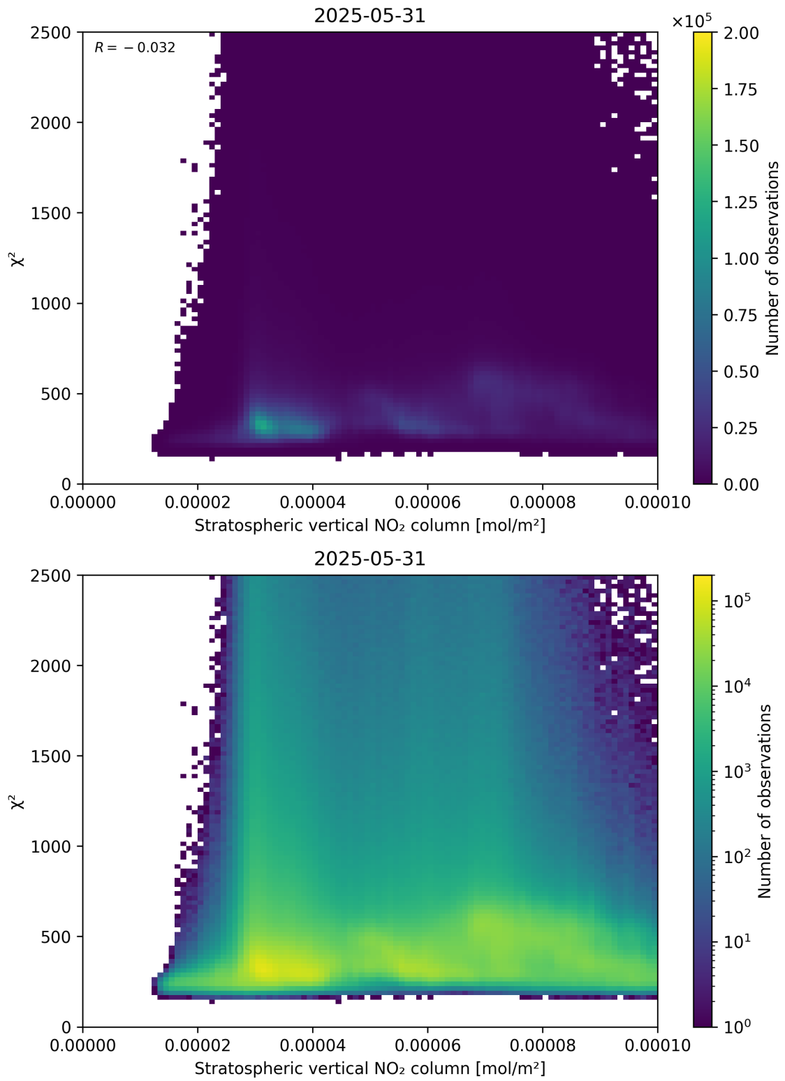
Figure 97: Scatter density plot of “Stratospheric vertical NO 2 column” against “ \chi^2 ” for 2025-05-31 to 2025-06-01.
