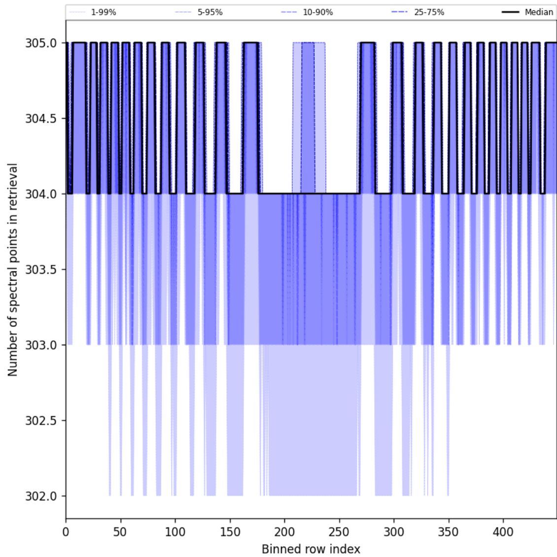
Figure 50: Along track statistics of “Number of spectral points in retrieval” for 2025-05-31 to 2025-06-01
