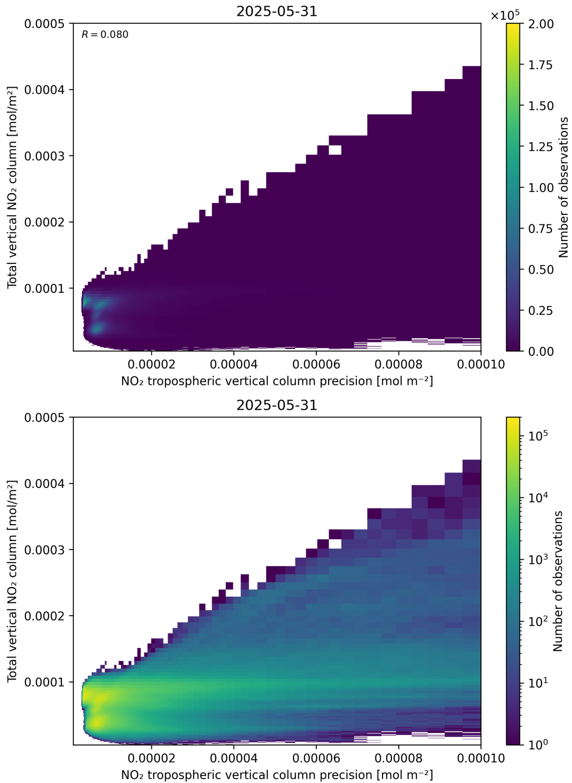
Figure 138: Scatter density plot of “NO 2 tropospheric vertical column precision” against “Total vertical NO 2 column” for 2025-05-31 to 2025-06-01.
