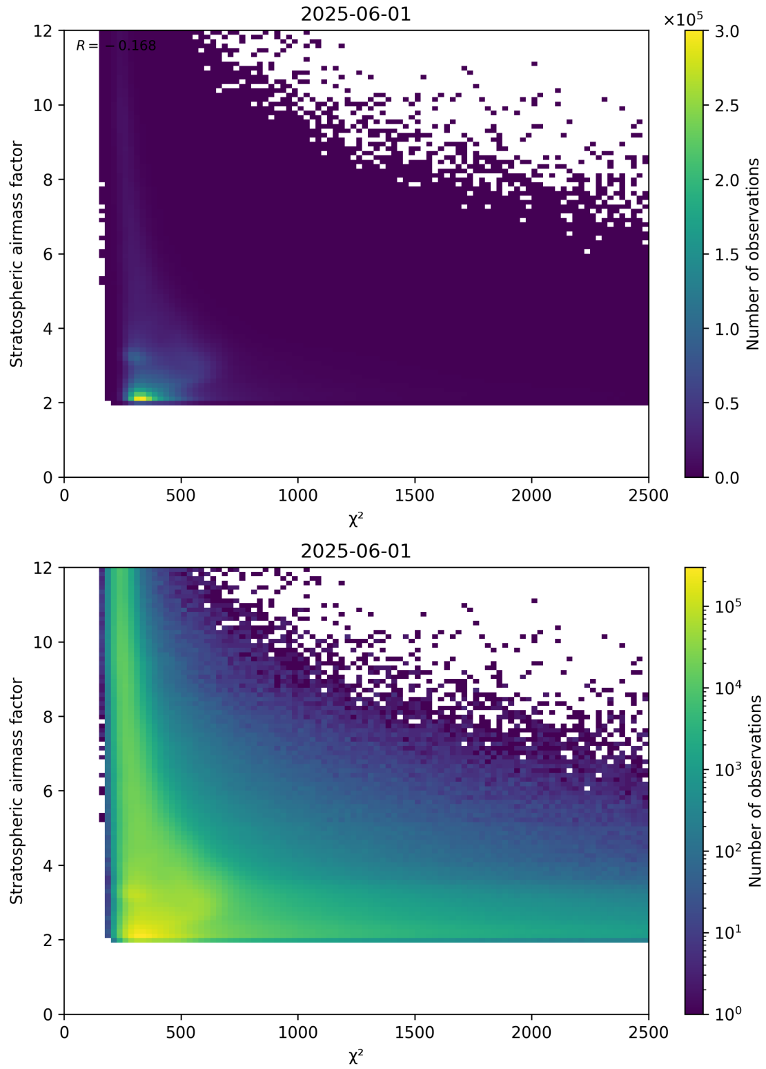
Figure 81: Scatter density plot of “ \chi^2 ” against “Stratospheric airmass factor” for 2025-06-01 to 2025-06-02.
