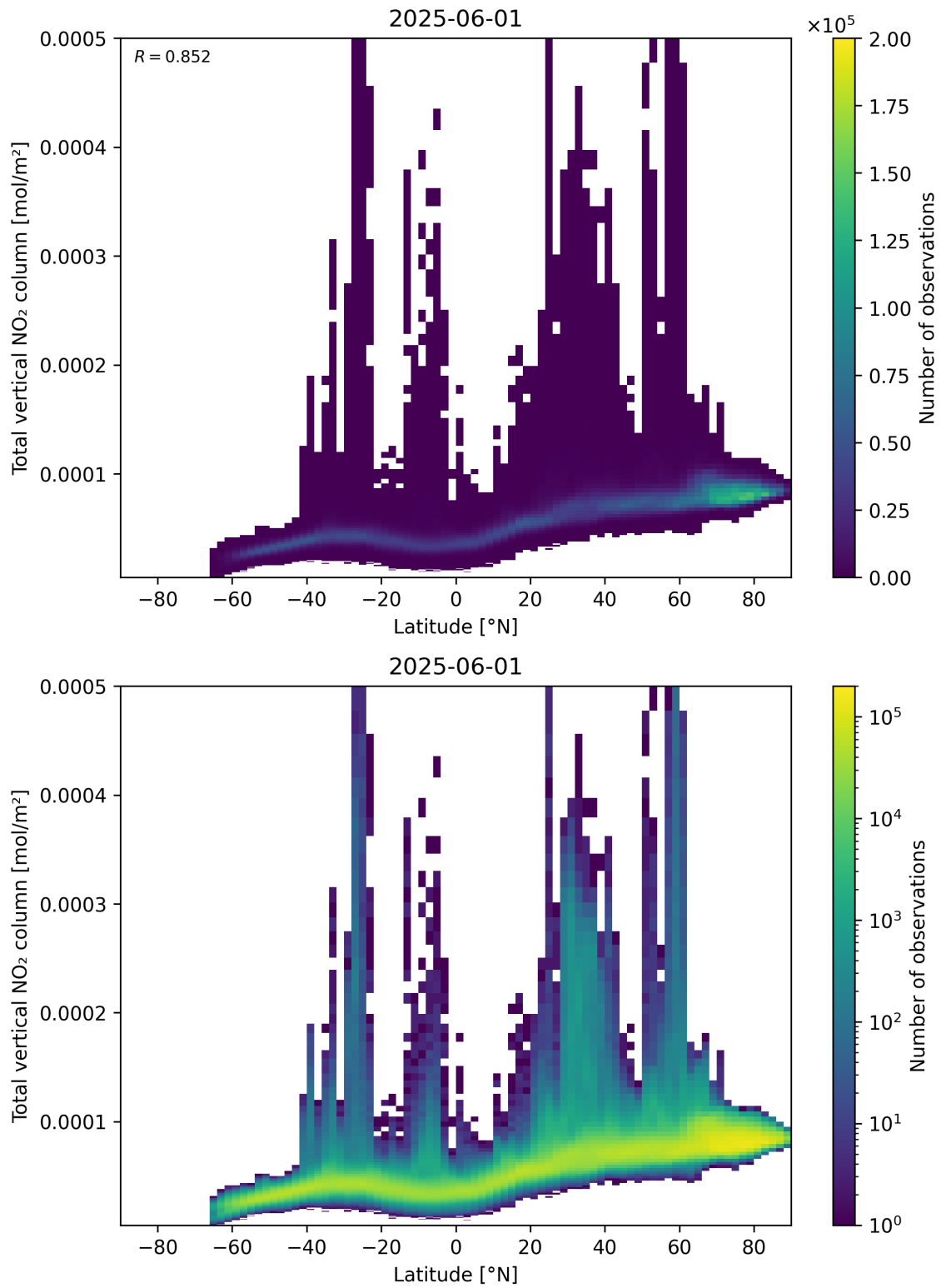
Figure 90: Scatter density plot of “Latitude” against “Total vertical NO 2 column” for 2025-06-01 to 2025-06-02.
