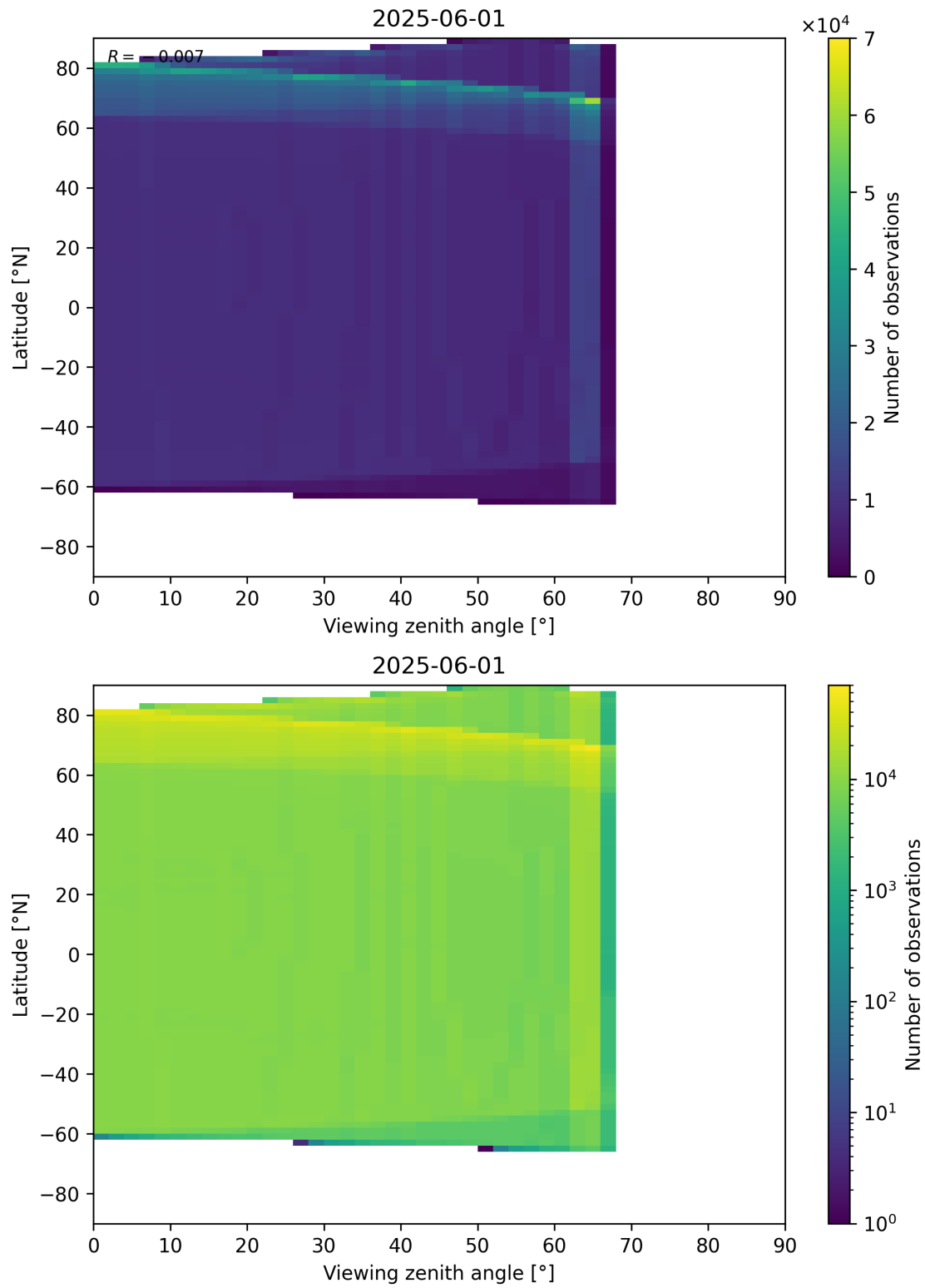
Figure 163: Scatter density plot of “Viewing zenith angle” against “Latitude” for 2025-06-01 to 2025-06-02.
