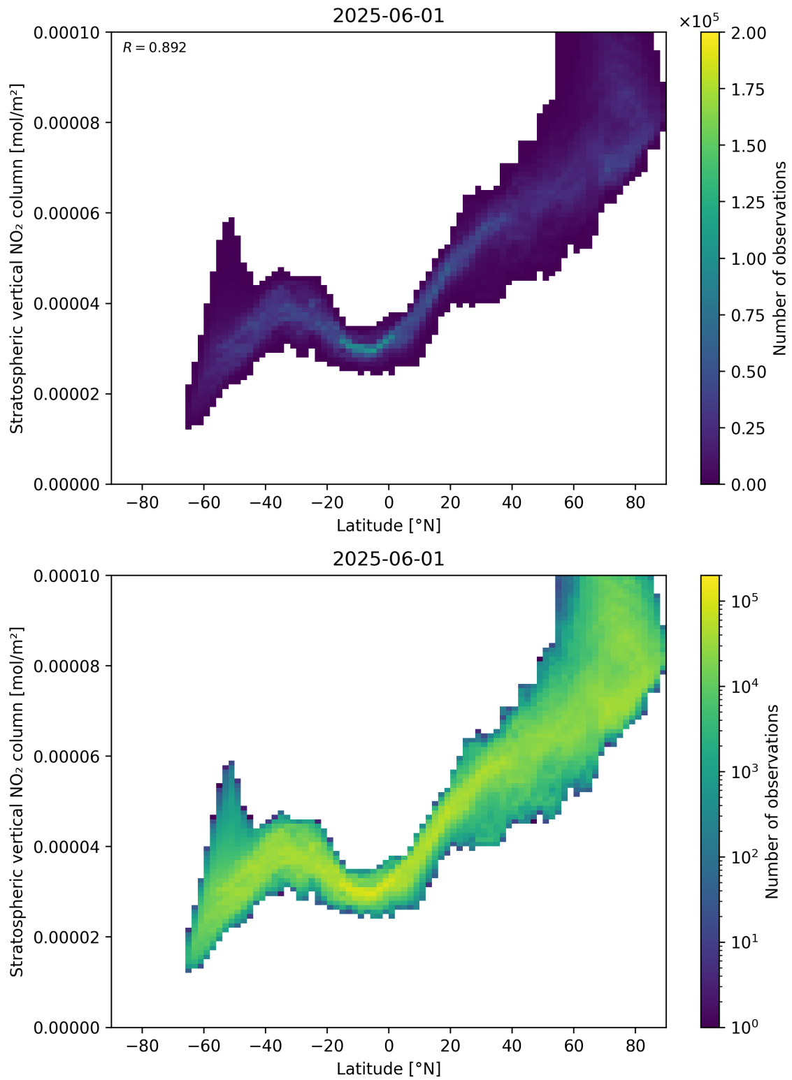
Figure 87: Scatter density plot of “Latitude” against “Stratospheric vertical NO 2 column” for 2025-06-01 to 2025-06-02.
