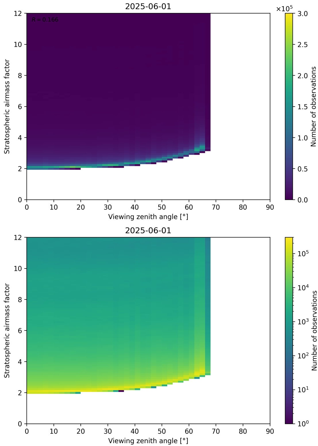
Figure 159: Scatter density plot of “Viewing zenith angle” against “Stratospheric airmass factor” for 2025-06-01 to 2025-06-02.
