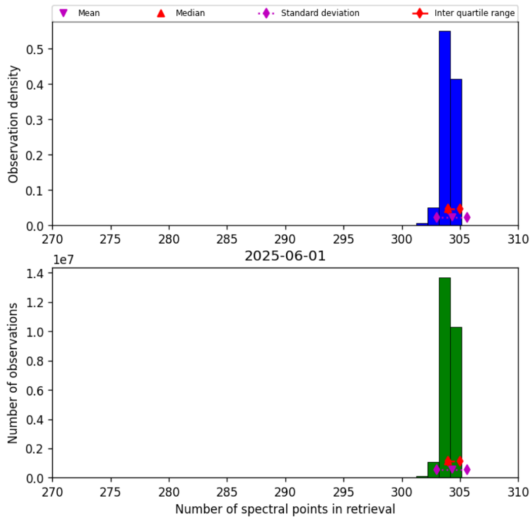
Figure 33: Histogram of “Number of spectral points in retrieval” for 2025-06-01 to 2025-06-02
