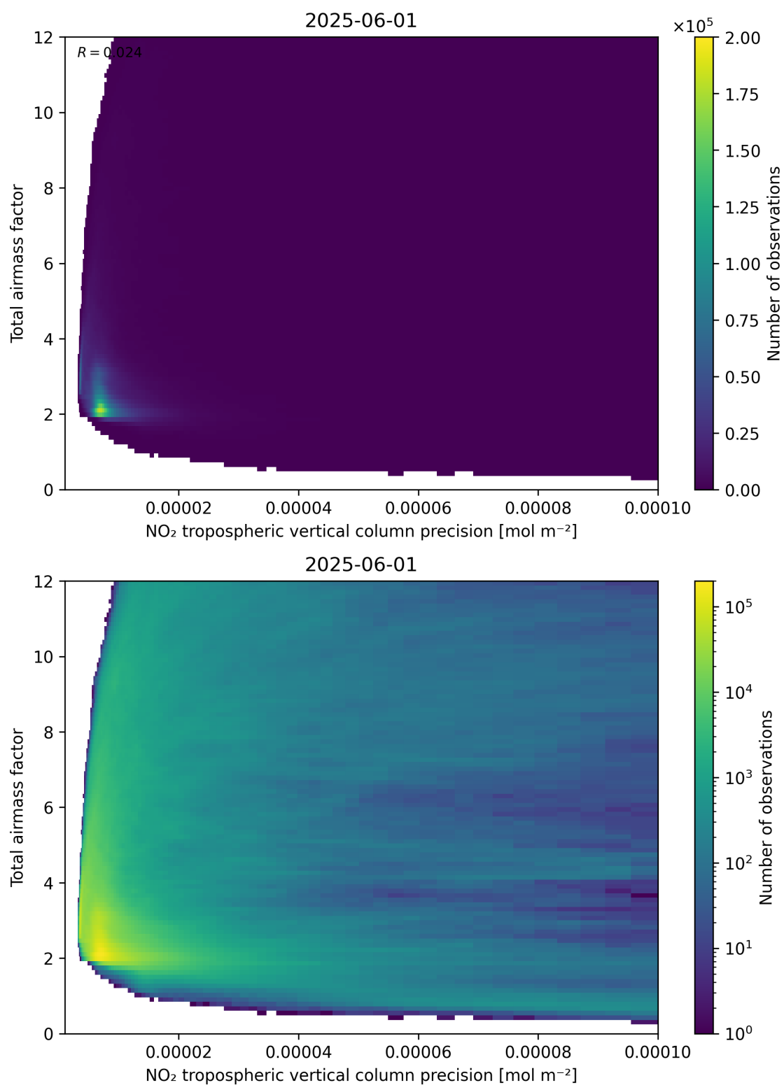
Figure 132: Scatter density plot of “NO 2 tropospheric vertical column precision” against “Total air mass factor” for 2025-06-01 to 2025-06-02.
