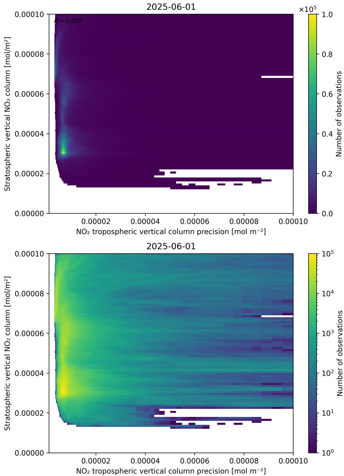
Figure 135: Scatter density plot of “NO 2 tropospheric vertical column precision” against “Stratospheric vertical NO 2 column” for 2025-06-01 to 2025-06-02.
