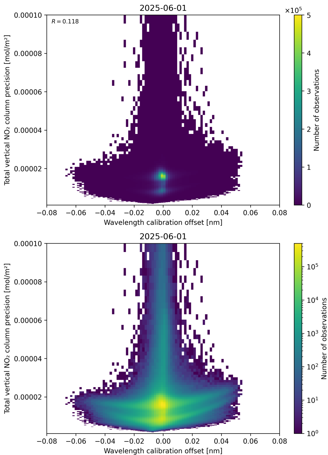
Figure 180: Scatter density plot of “Wavelength calibration offset” against “Total vertical NO 2 column precision” for 2025-06-01 to 2025-06-02.
