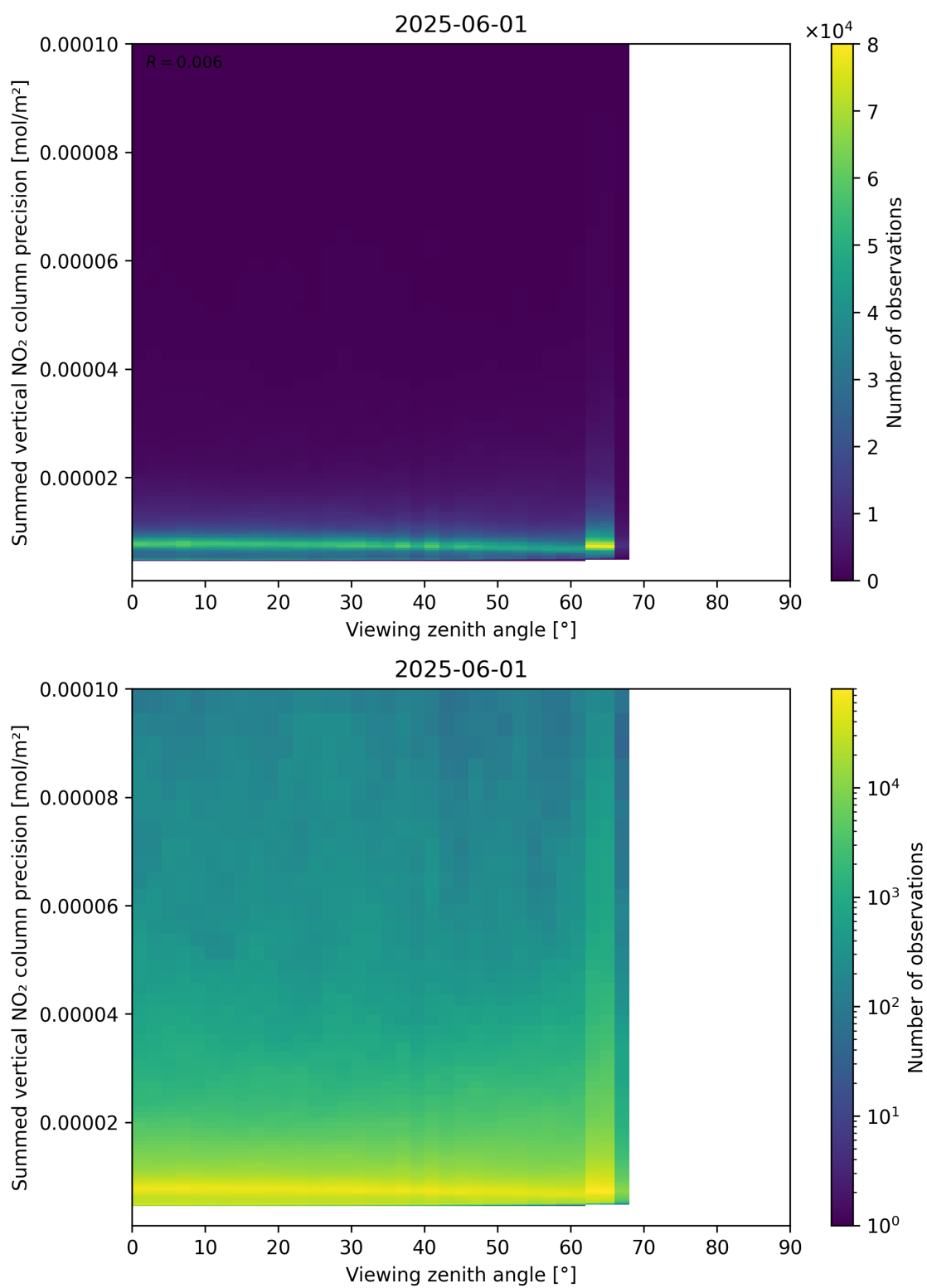
Figure 166: Scatter density plot of “Viewing zenith angle” against “Summed vertical NO 2 column precision” for 2025-06-01 to 2025-06-02.
