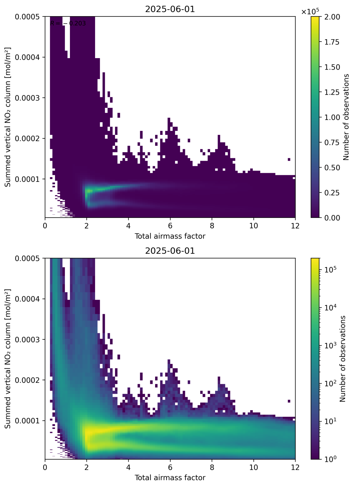
Figure 65: Scatter density plot of “Total airmass factor” against “Summed vertical NO 2 column” for 2025-06-01 to 2025-06-02.
