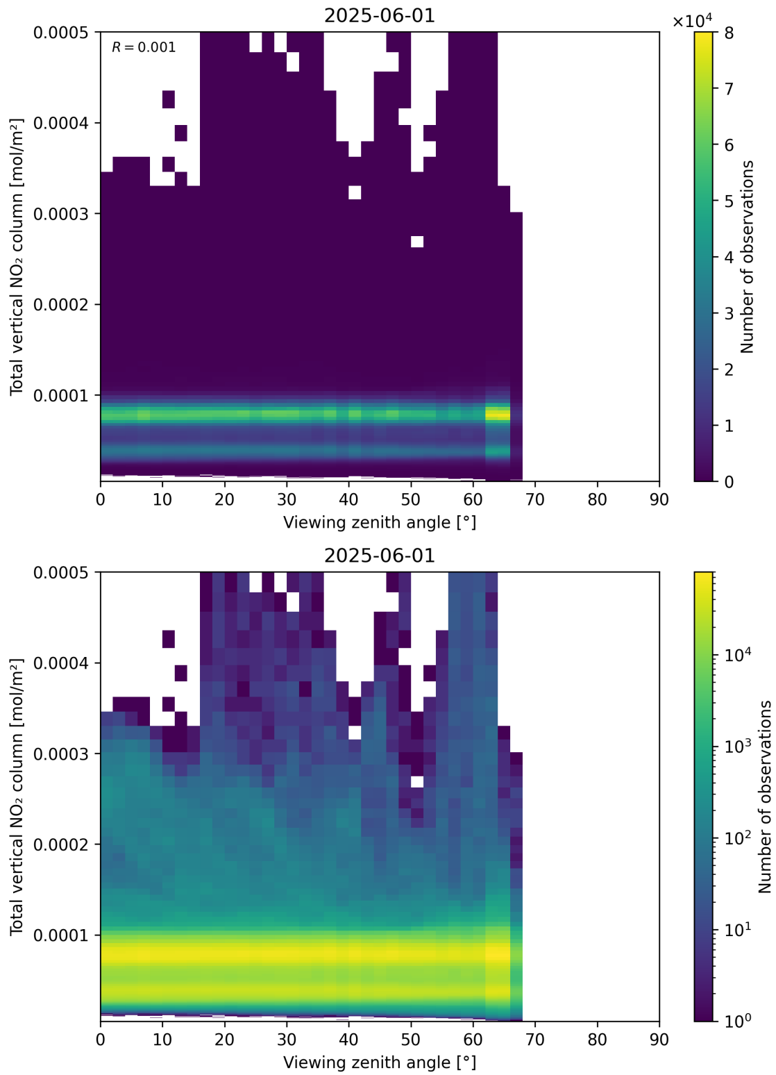
Figure 167: Scatter density plot of “Viewing zenith angle” against “Total vertical NO 2 column” for 2025-06-01 to 2025-06-02.
