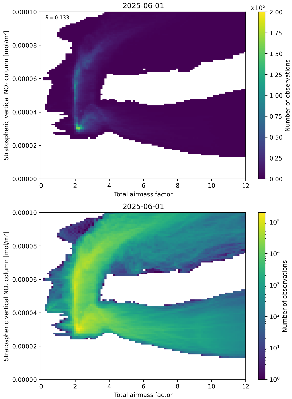
Figure 64: Scatter density plot of “Total airmass factor” against “Stratospheric vertical NO 2 column” for 2025-06-01 to 2025-06-02.
