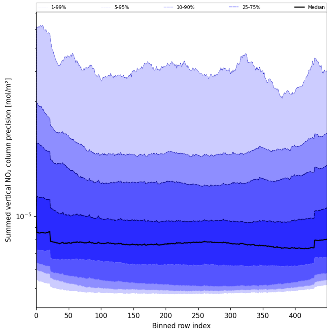
Figure 58: Along track statistics of “Summed vertical NO 2 column precision” for 2025-06-01 to 2025-06-02
