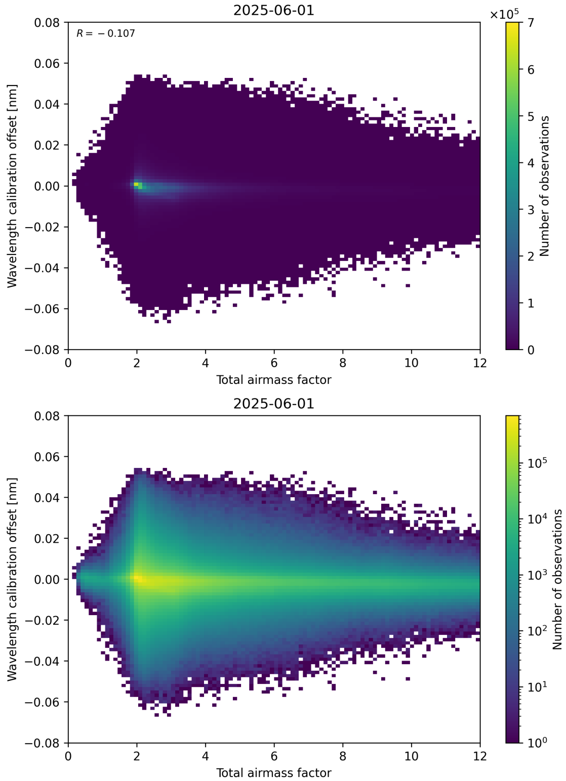
Figure 70: Scatter density plot of “Total airmass factor” against “Wavelength calibration offset” for 2025-06-01 to 2025-06-02.
