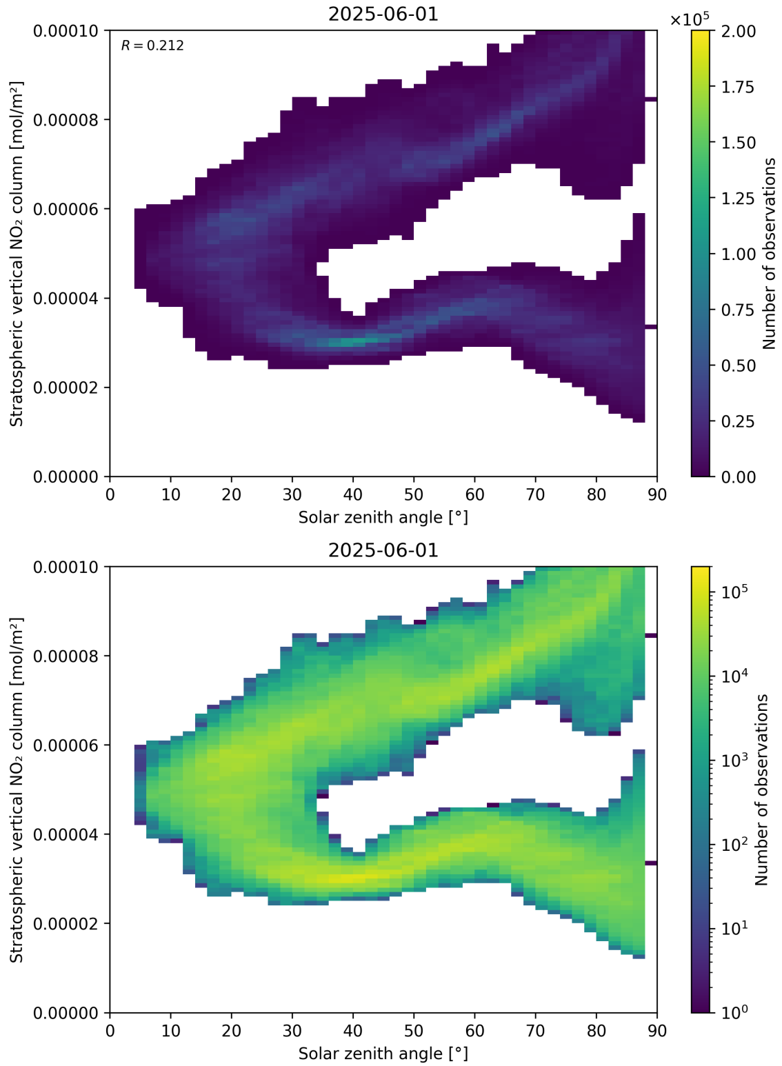
Figure 150: Scatter density plot of “Solar zenith angle” against “Stratospheric vertical NO 2 column” for 2025-06-01 to 2025-06-02.
