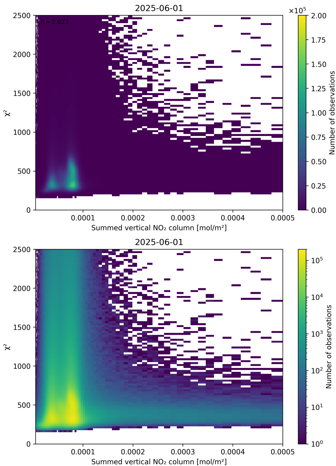
Figure 104: Scatter density plot of “Summed vertical NO 2 column” against “ \chi^2 ” for 2025-06-01 to 2025-06-02.
