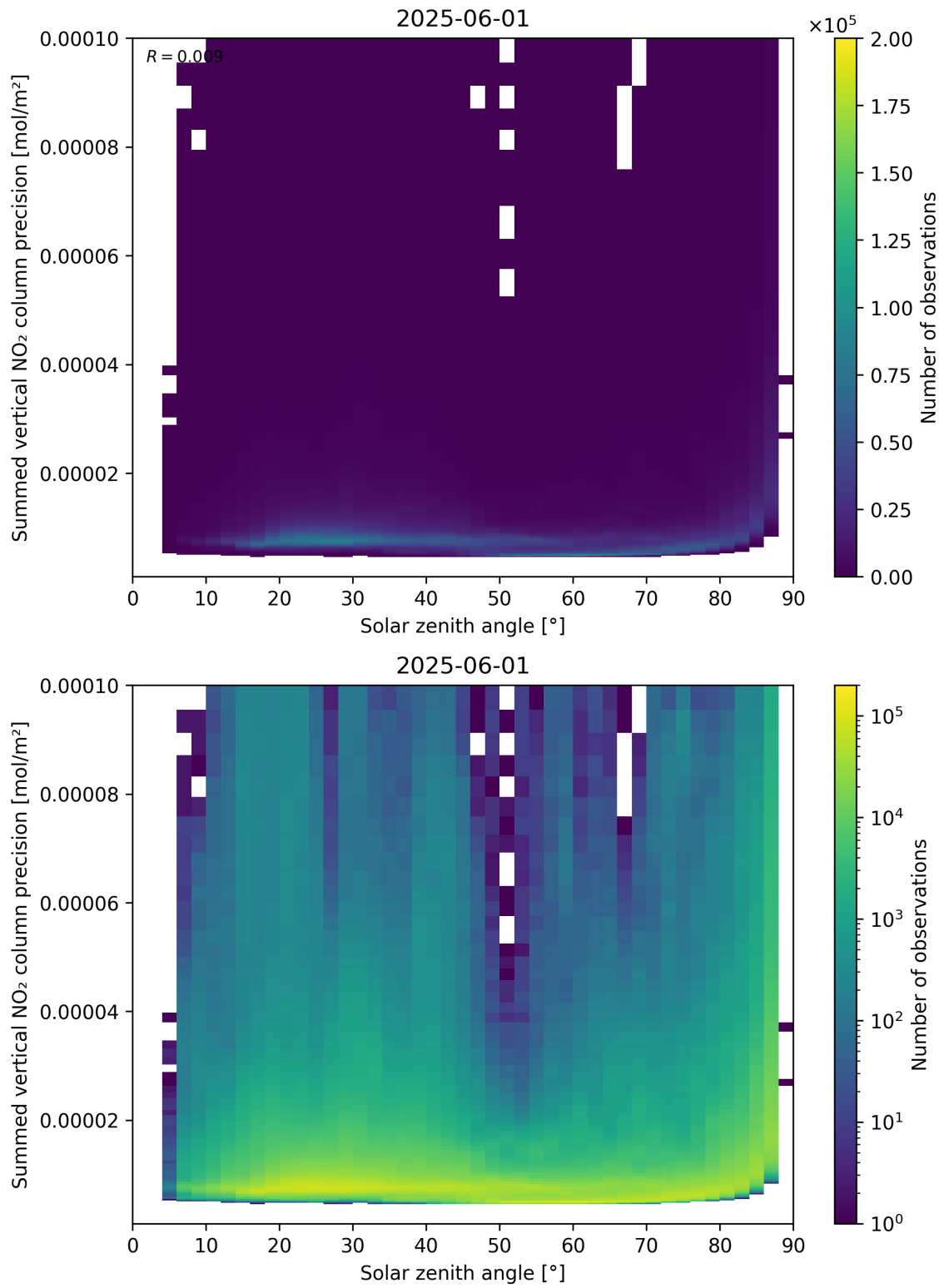
Figure 152: Scatter density plot of “Solar zenith angle” against “Summed vertical NO 2 column precision” for 2025-06-01 to 2025-06-02.
