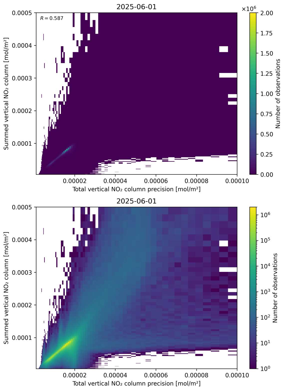
Figure 117: Scatter density plot of “Total vertical NO 2 column precision” against “Summed vertical NO 2 column” for 2025-06-01 to 2025-06-02.
