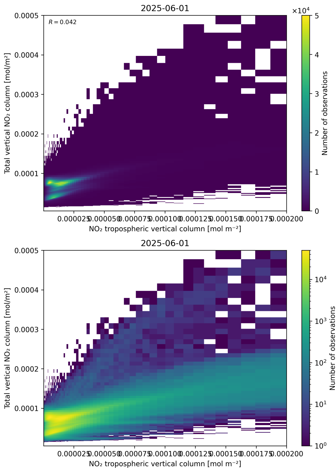
Figure 128: Scatter density plot of “NO 2 tropospheric vertical column” against “Total vertical NO 2 column” for 2025-06-01 to 2025-06-02.
