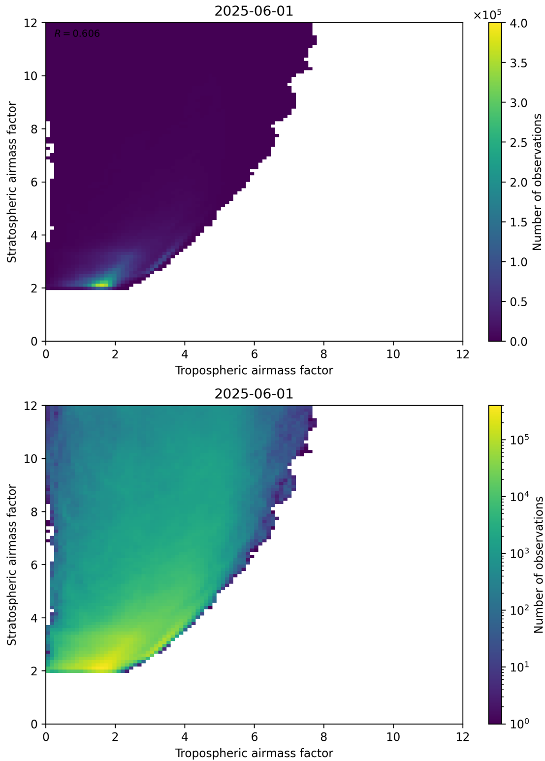
Figure 71: Scatter density plot of “Tropospheric airmass factor” against “Stratospheric airmass factor” for 2025-06-01 to 2025-06-02.
