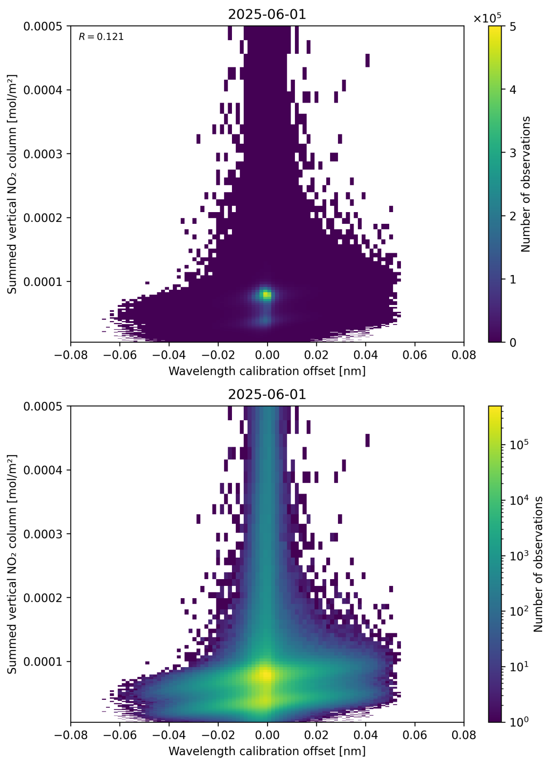
Figure 177: Scatter density plot of “Wavelength calibration offset” against “Summed vertical NO 2 column” for 2025-06-01 to 2025-06-02.
