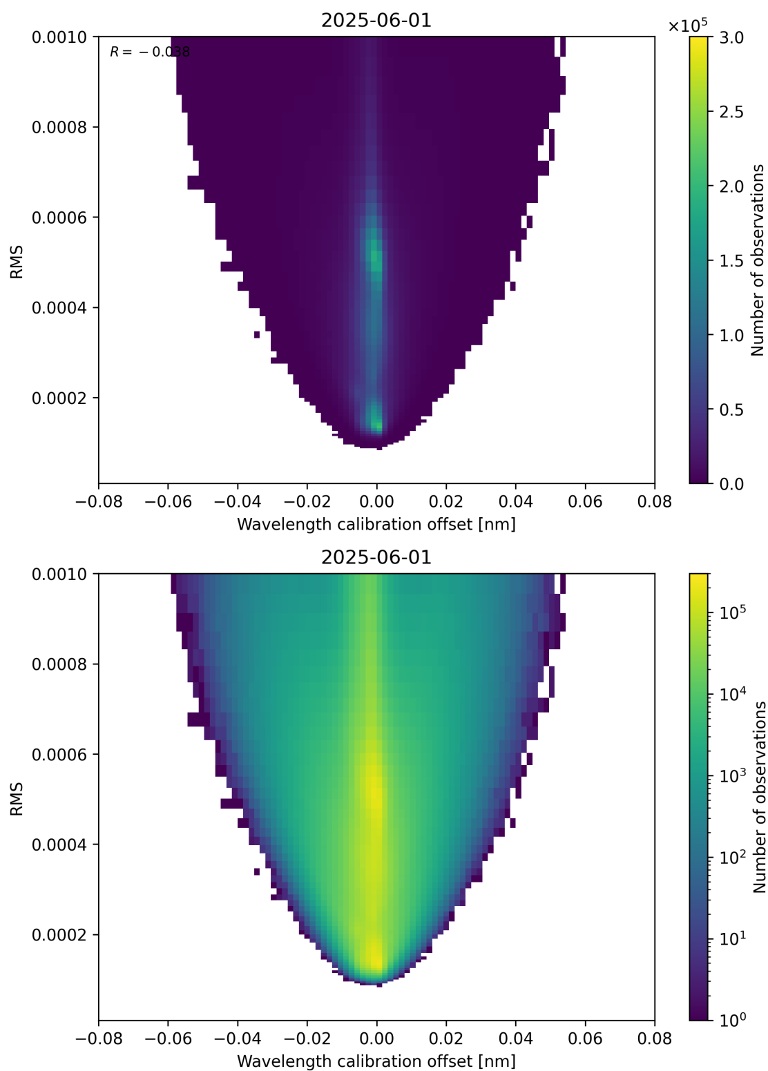
Figure 181: Scatter density plot of “Wavelength calibration offset” against “RMS” for 2025-06-01 to 2025-06-02.
