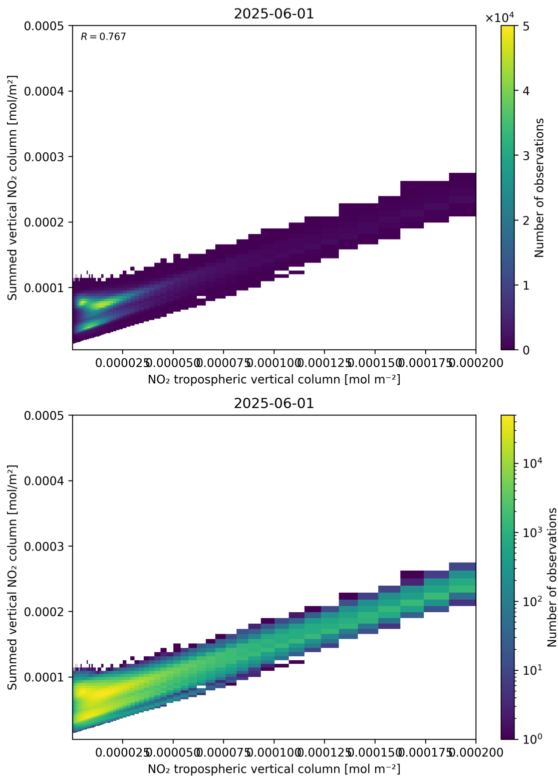
Figure 126: Scatter density plot of “NO 2 tropospheric vertical column” against “Summed vertical NO 2 column” for 2025-06-01 to 2025-06-02.
