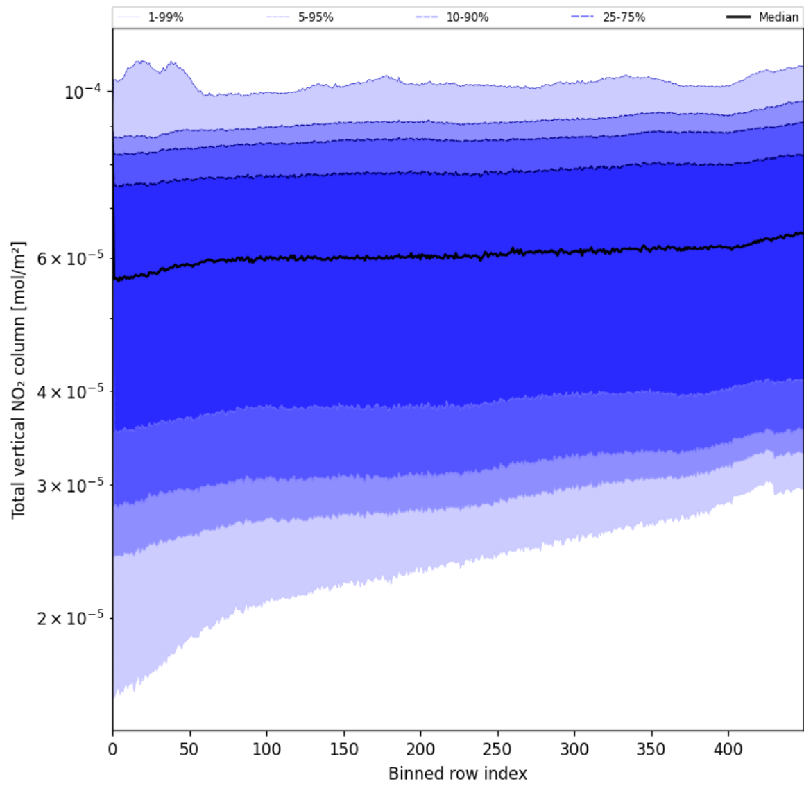
Figure 55: Along track statistics of “Total vertical NO 2 column” for 2025-06-01 to 2025-06-02
