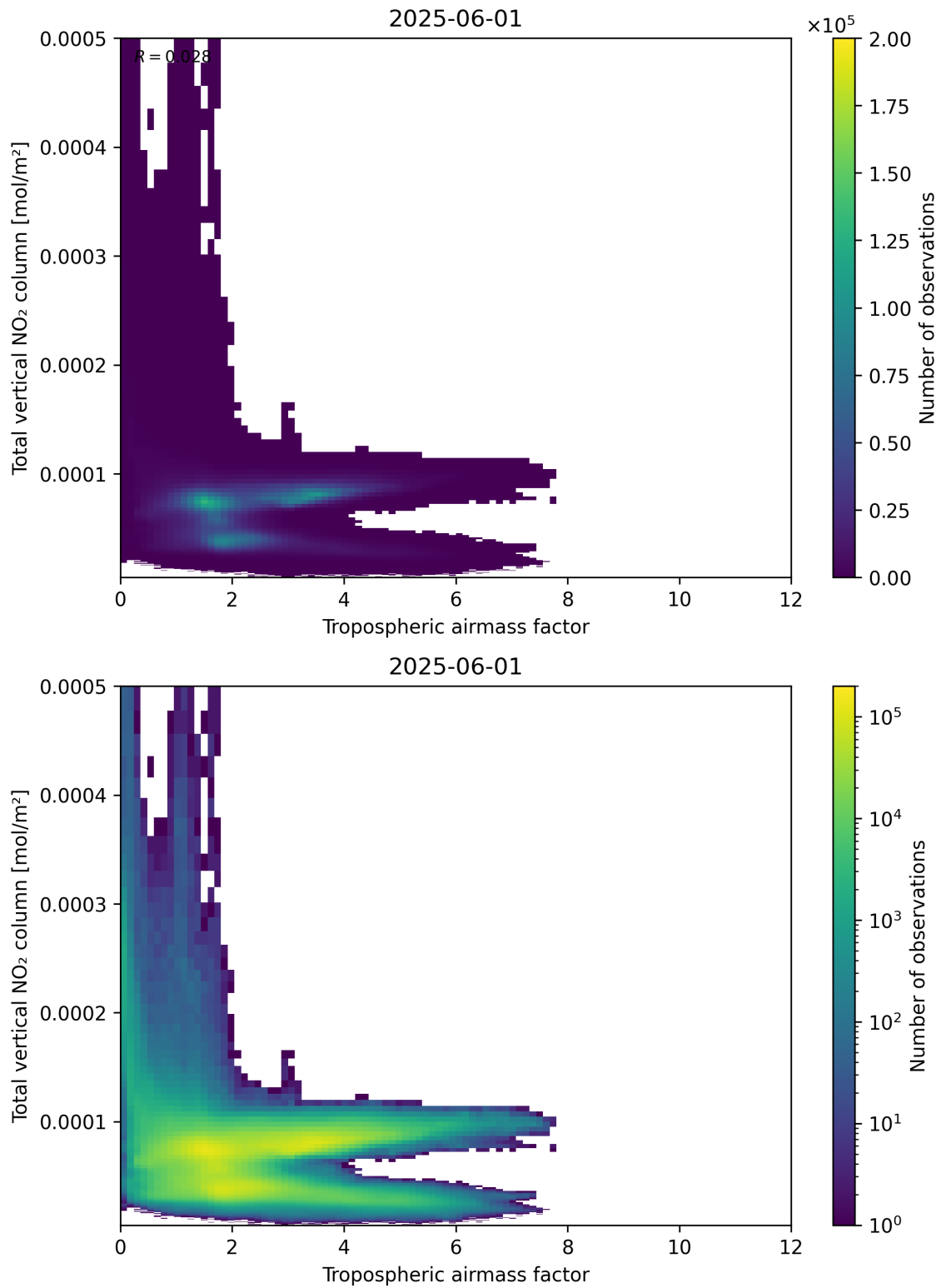
Figure 77: Scatter density plot of “Tropospheric airmass factor” against “Total vertical \text{NO}_2 column” for 2025-06-01 to 2025-06-02.
