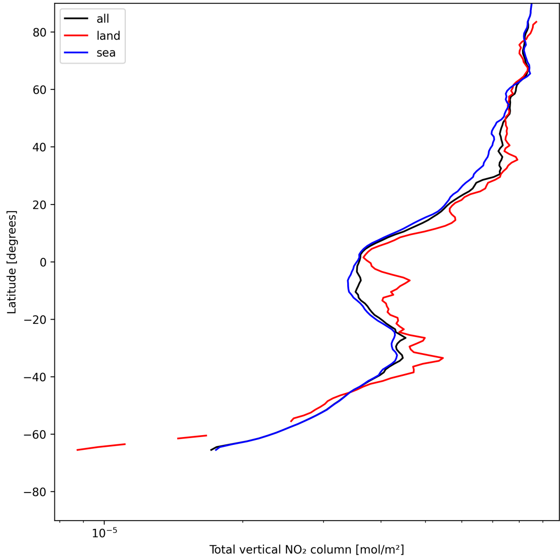
Figure 21: Zonal average of “Total vertical NO 2 column” for 2025-06-01 to 2025-06-02.
