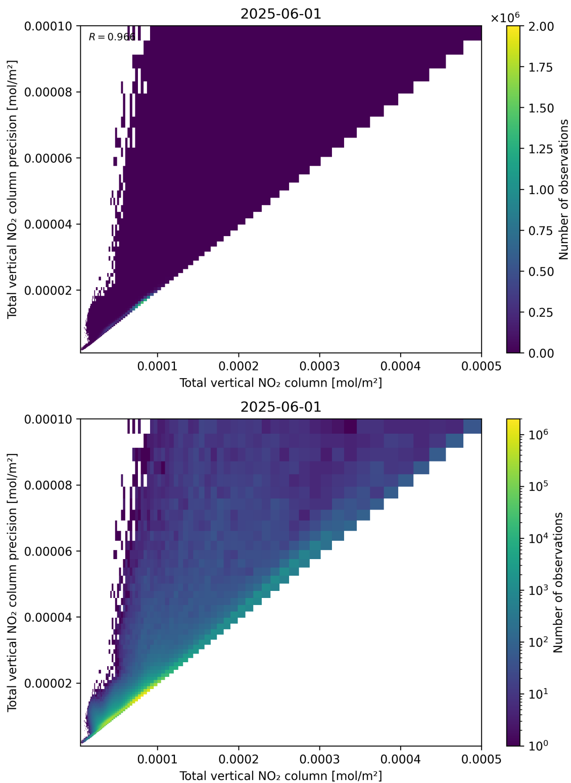
Figure 114: Scatter density plot of “Total vertical NO 2 column” against “Total vertical NO 2 column precision” for 2025-06-01 to 2025-06-02.
