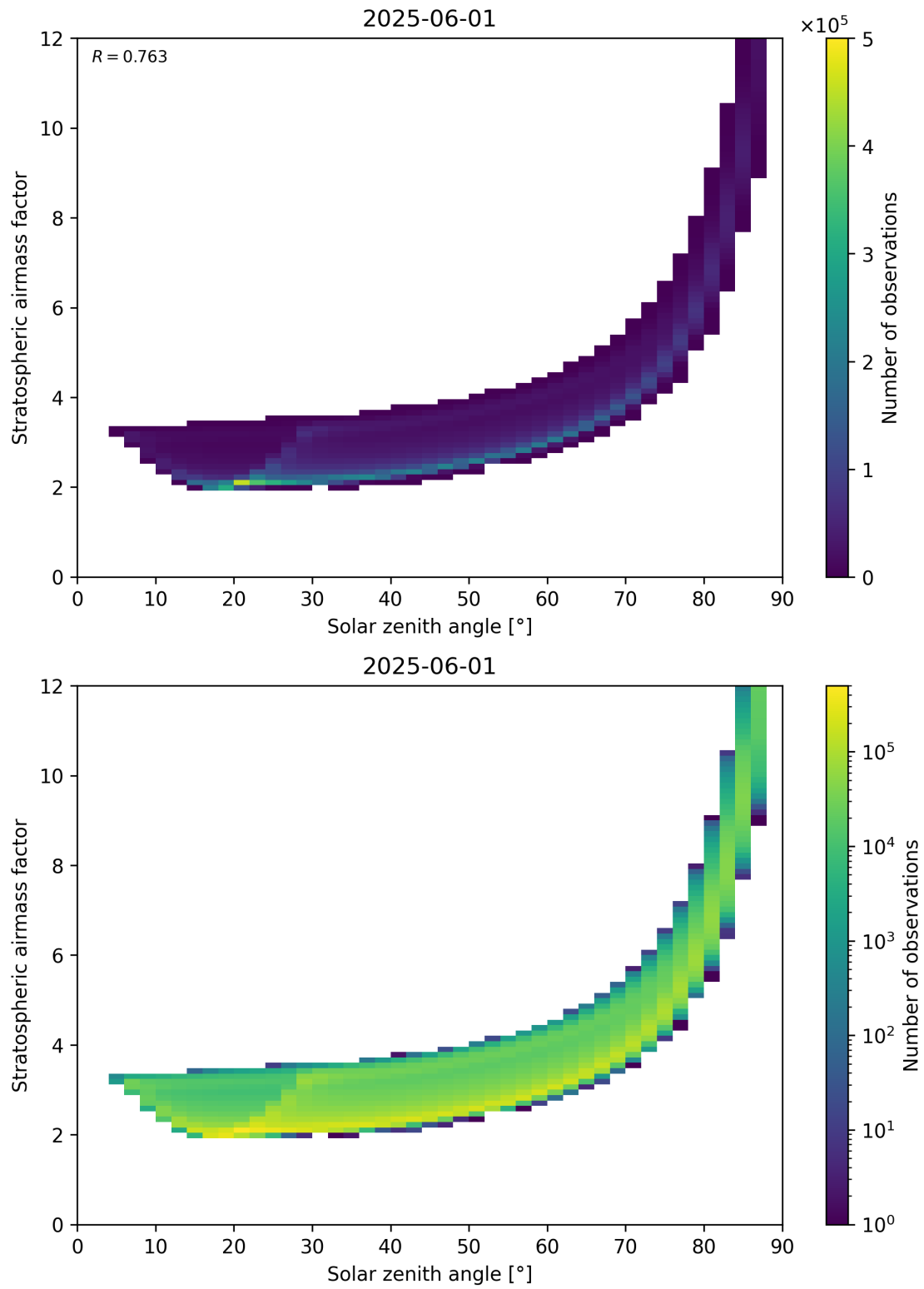
Figure 145: Scatter density plot of “Solar zenith angle” against “Stratospheric airmass factor” for 2025-06-01 to 2025-06-02.
