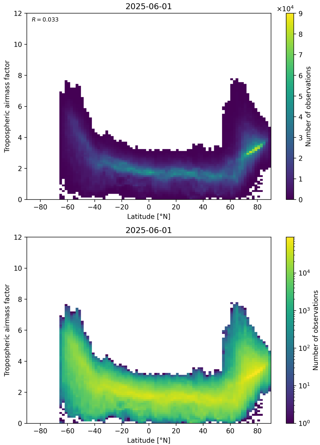
Figure 85: Scatter density plot of “Latitude” against “Tropospheric air mass factor” for 2025-06-01 to 2025-06-02.
