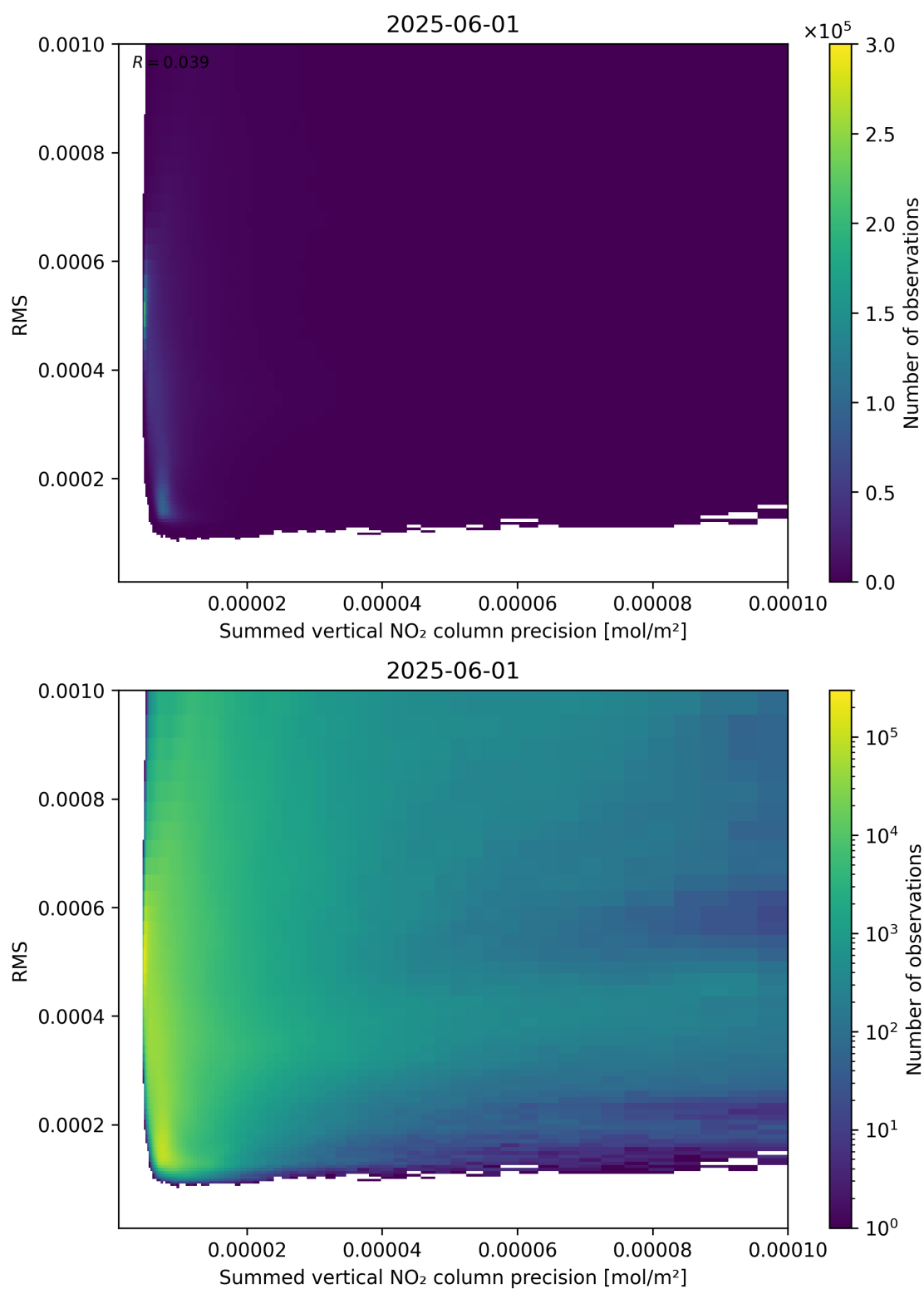
Figure 108: Scatter density plot of “Summed vertical NO 2 column precision” against “RMS” for 2025-06-01 to 2025-06-02.
