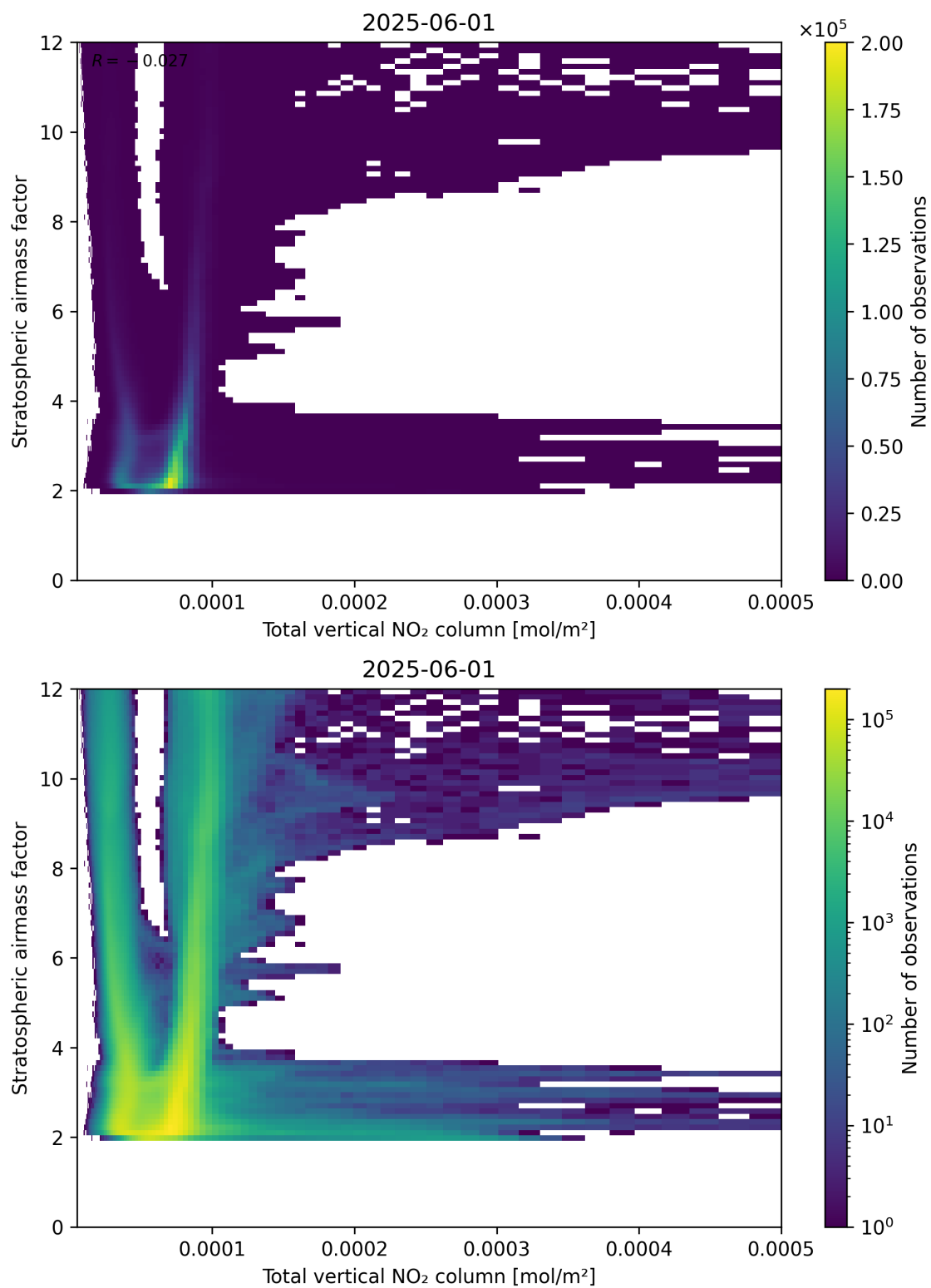
Figure 110: Scatter density plot of “Total vertical NO 2 column” against “Stratospheric airmass factor” for 2025-06-01 to 2025-06-02.
