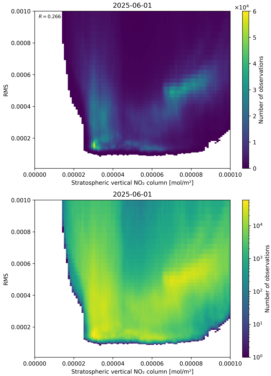
Figure 102: Scatter density plot of “Stratospheric vertical NO 2 column” against “RMS” for 2025-06-01 to 2025-06-02.
