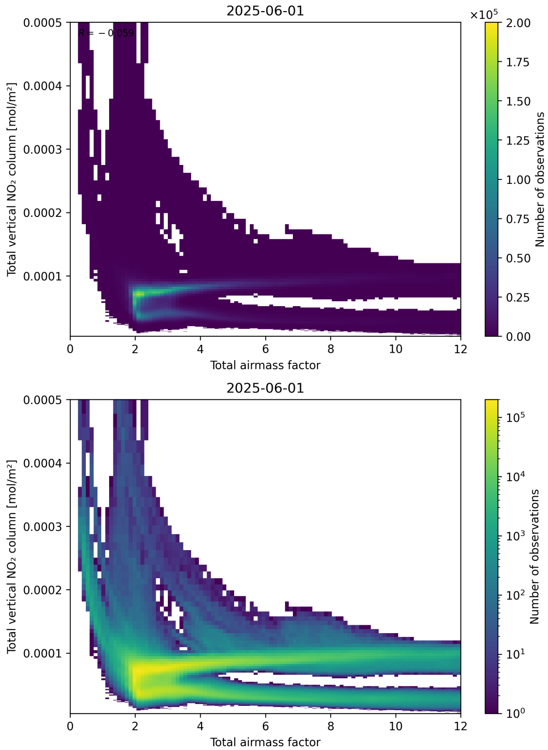
Figure 67: Scatter density plot of “Total airmass factor” against “Total vertical NO 2 column” for 2025-06-01 to 2025-06-02.
