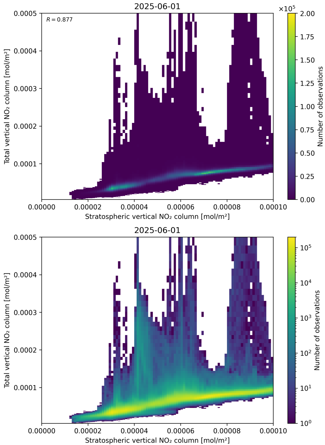
Figure 100: Scatter density plot of “Stratospheric vertical NO 2 column” against “Total vertical NO 2 column” for 2025-06-01 to 2025-06-02.
