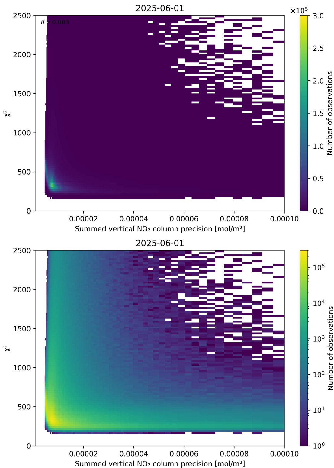
Figure 107: Scatter density plot of “Summed vertical NO 2 column precision” against “ \chi^2 ” for 2025-06-01 to 2025-06-02.
