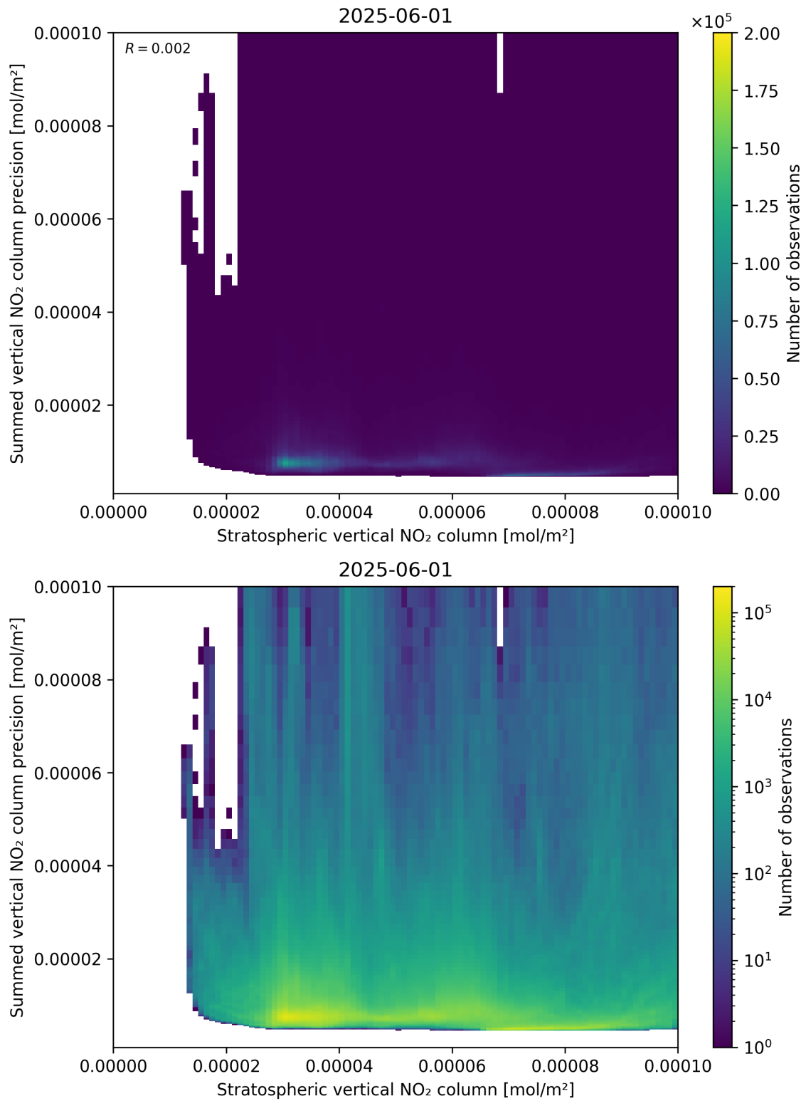
Figure 99: Scatter density plot of “Stratospheric vertical NO 2 column” against “Summed vertical NO 2 column precision” for 2025-06-01 to 2025-06-02.
