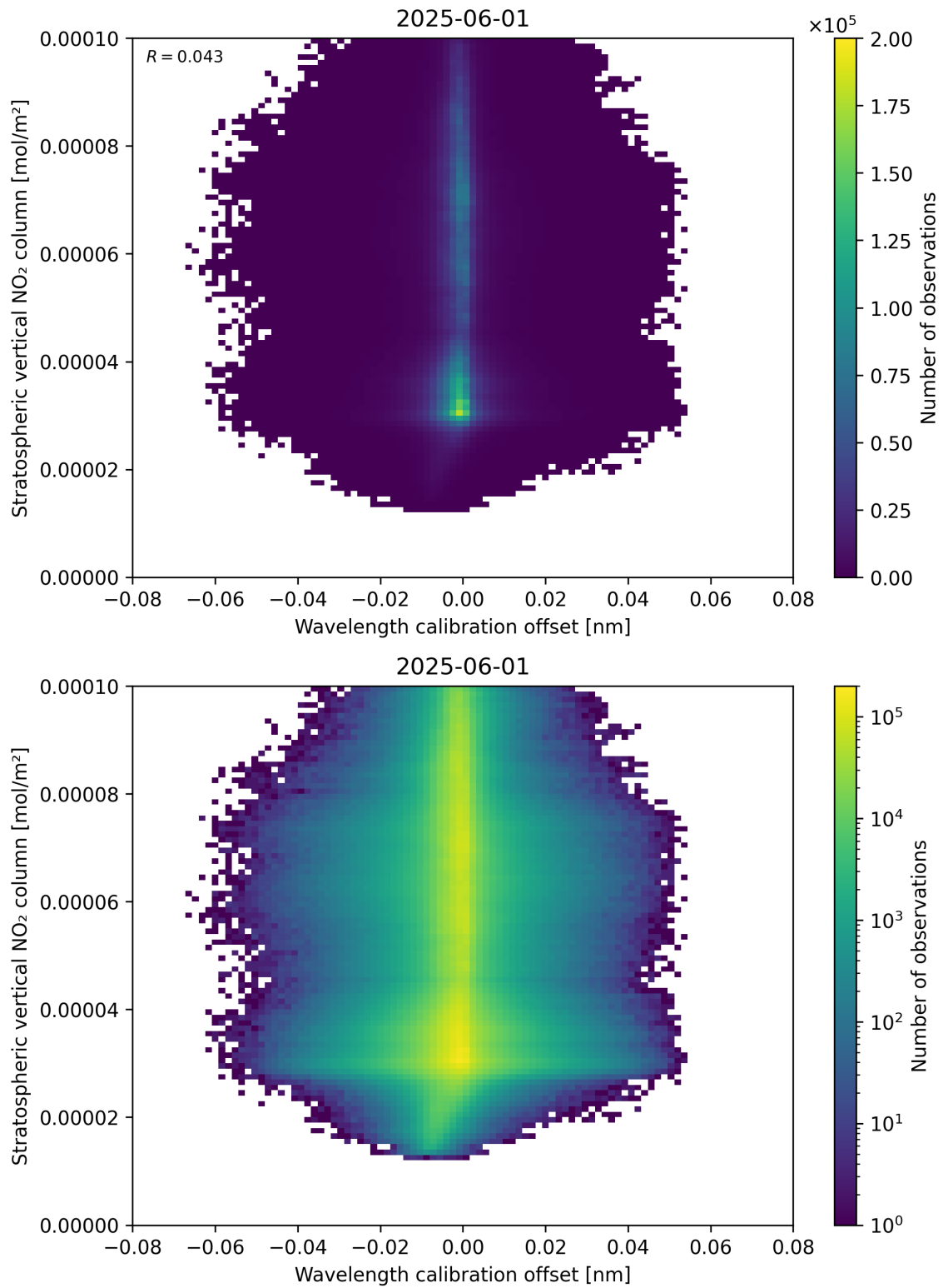
Figure 176: Scatter density plot of “Wavelength calibration offset” against “Stratospheric vertical NO 2 column” for 2025-06-01 to 2025-06-02.
