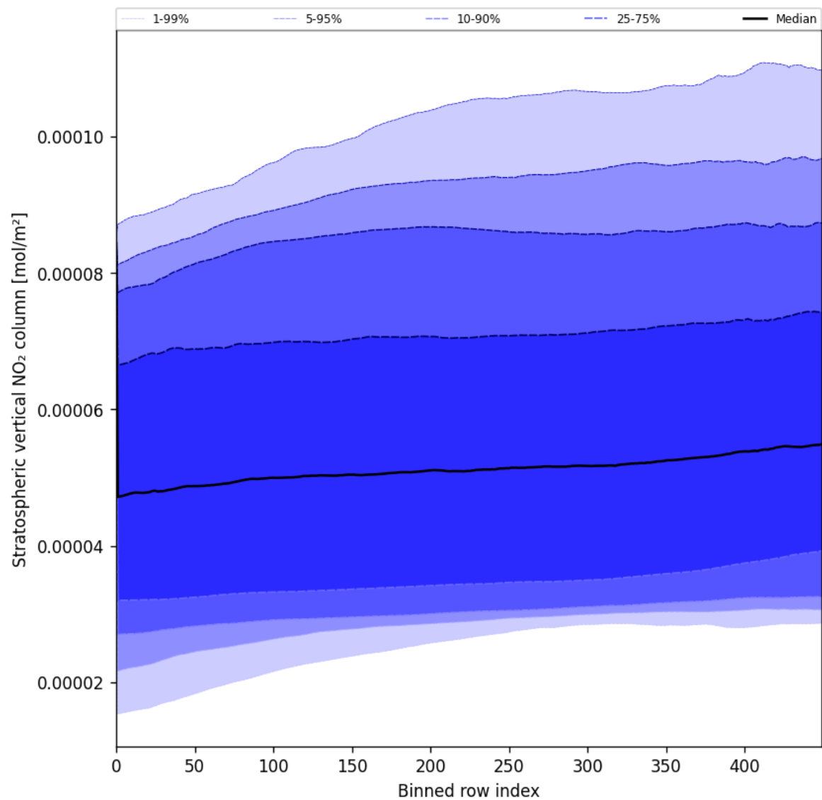
Figure 53: Along track statistics of “Stratospheric vertical NO 2 column” for 2025-06-01 to 2025-06-02
