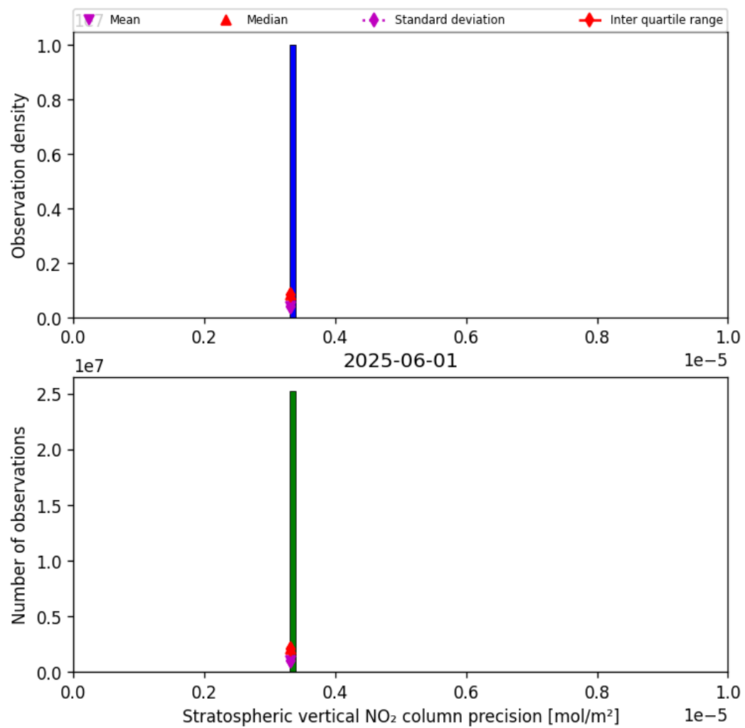
Figure 37: Histogram of “Stratospheric vertical NO 2 column precision” for 2025-06-01 to 2025-06-02
