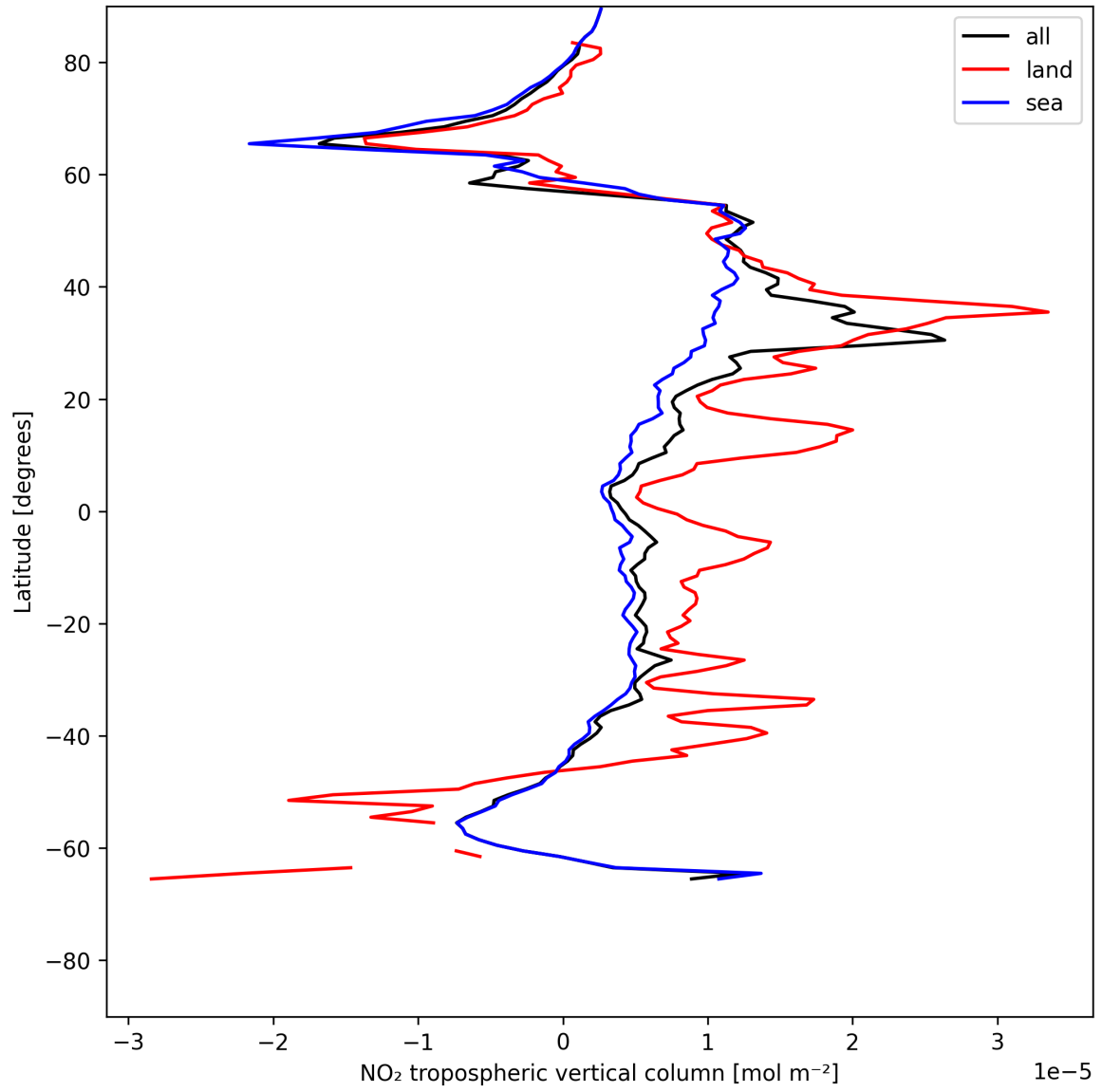
Figure 12: Zonal average of “NO 2 tropospheric vertical column” for 2025-06-01 to 2025-06-02.
