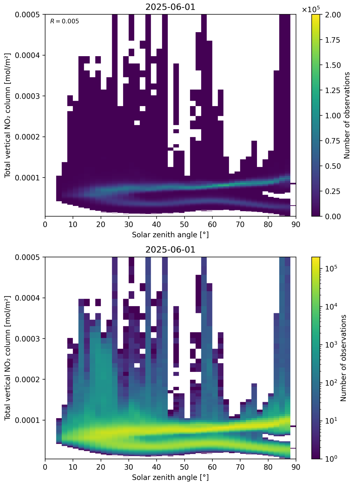
Figure 153: Scatter density plot of “Solar zenith angle” against “Total vertical NO 2 column” for 2025-06-01 to 2025-06-02.
