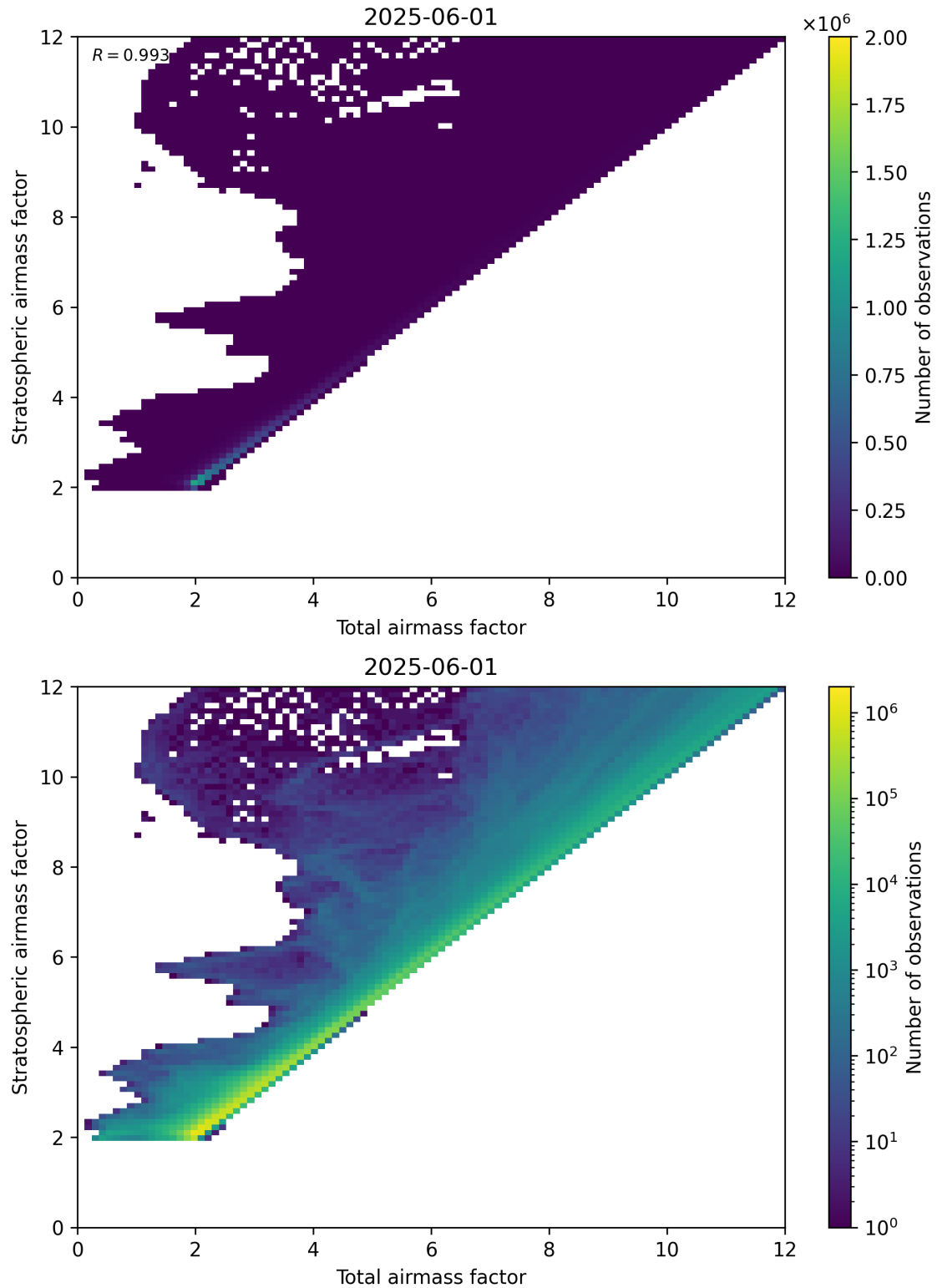
Figure 62: Scatter density plot of “Total airmass factor” against “Stratospheric airmass factor” for 2025-06-01 to 2025-06-02.
