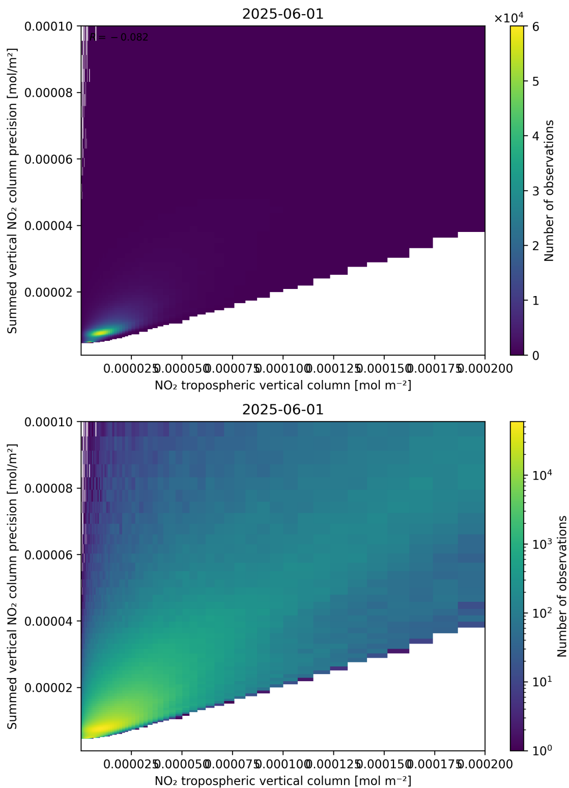
Figure 127: Scatter density plot of “NO 2 tropospheric vertical column” against “Summed vertical NO 2 column precision” for 2025-06-01 to 2025-06-02.
