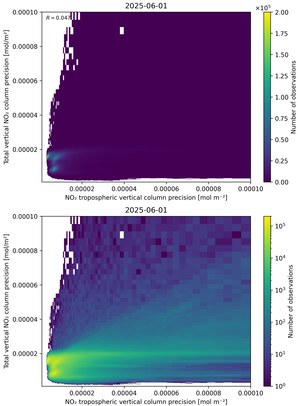
Figure 139: Scatter density plot of “NO 2 tropospheric vertical column precision” against “Total vertical NO 2 column precision” for 2025-06-01 to 2025-06-02.
