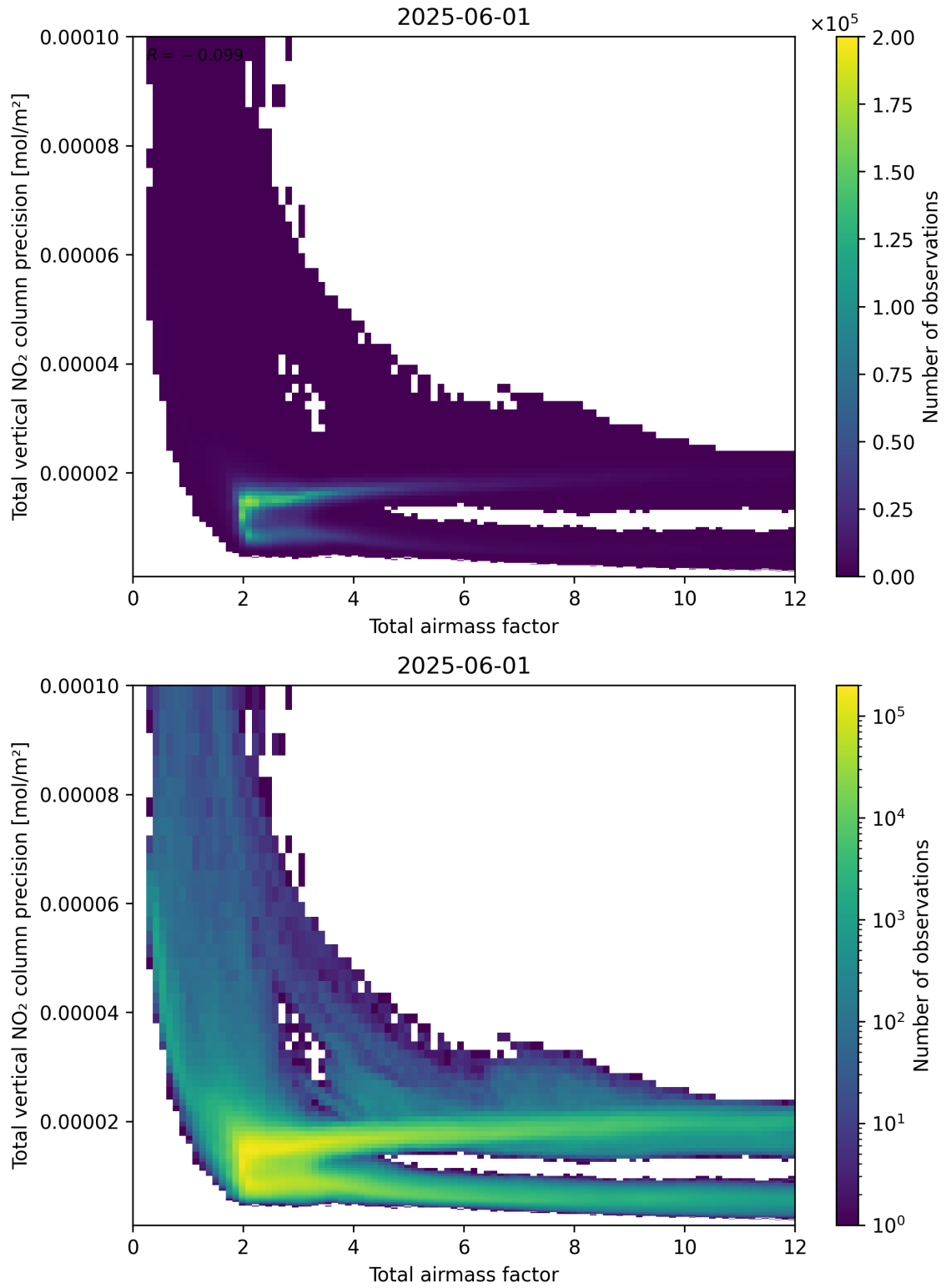
Figure 68: Scatter density plot of “Total airmass factor” against “Total vertical NO 2 column precision” for 2025-06-01 to 2025-06-02.
