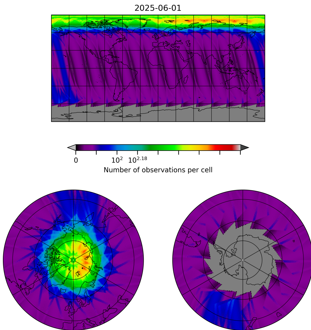
Figure 10: Map of the number of observations for 2025-06-01 to 2025-06-02
