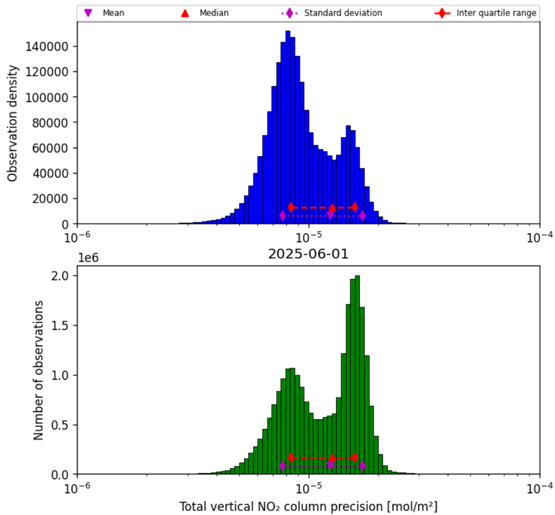
Figure 39: Histogram of “Total vertical NO 2 column precision” for 2025-06-01 to 2025-06-02
