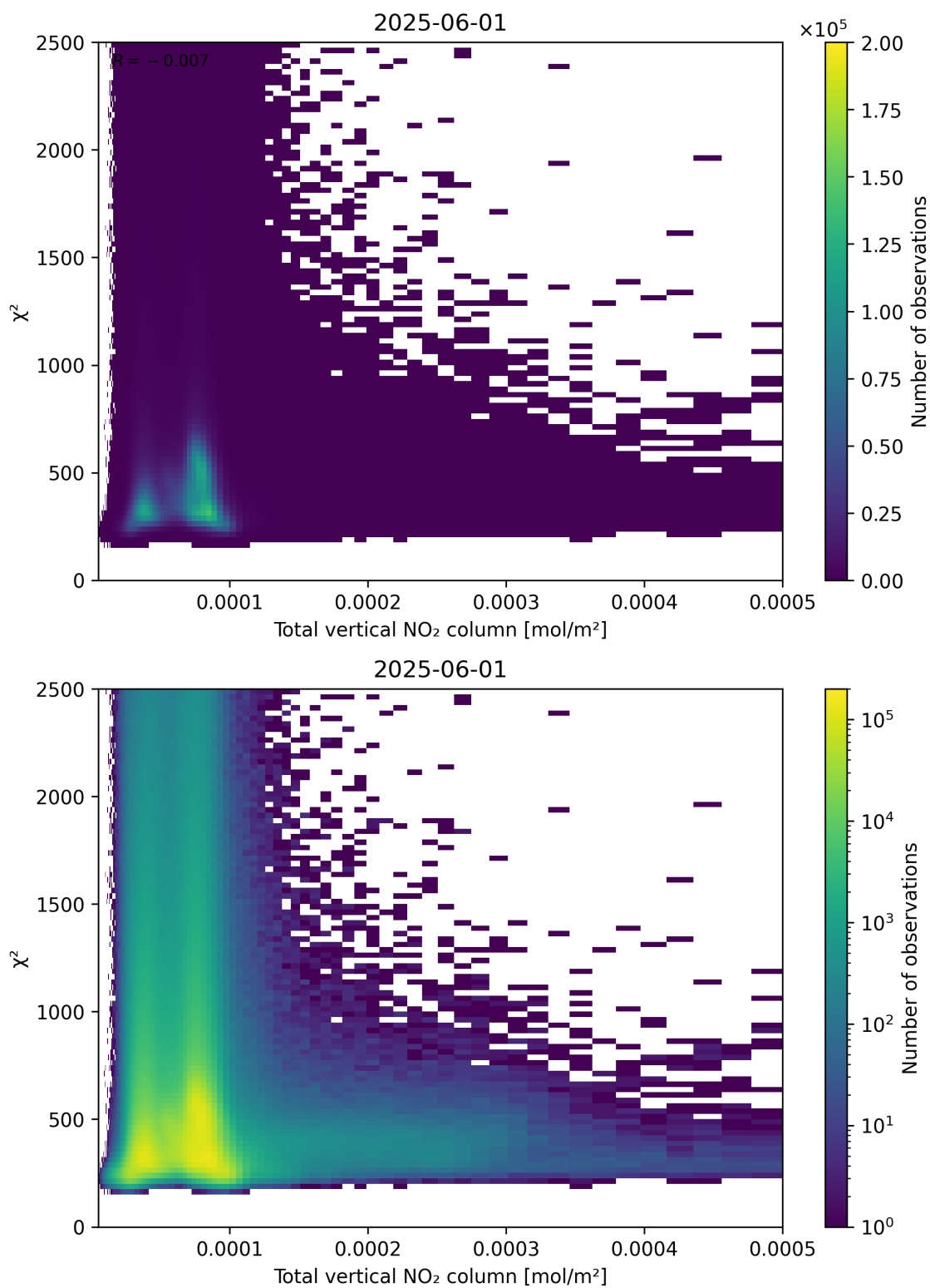
Figure 111: Scatter density plot of “Total vertical NO 2 column” against “ \chi^2 ” for 2025-06-01 to 2025-06-02.
