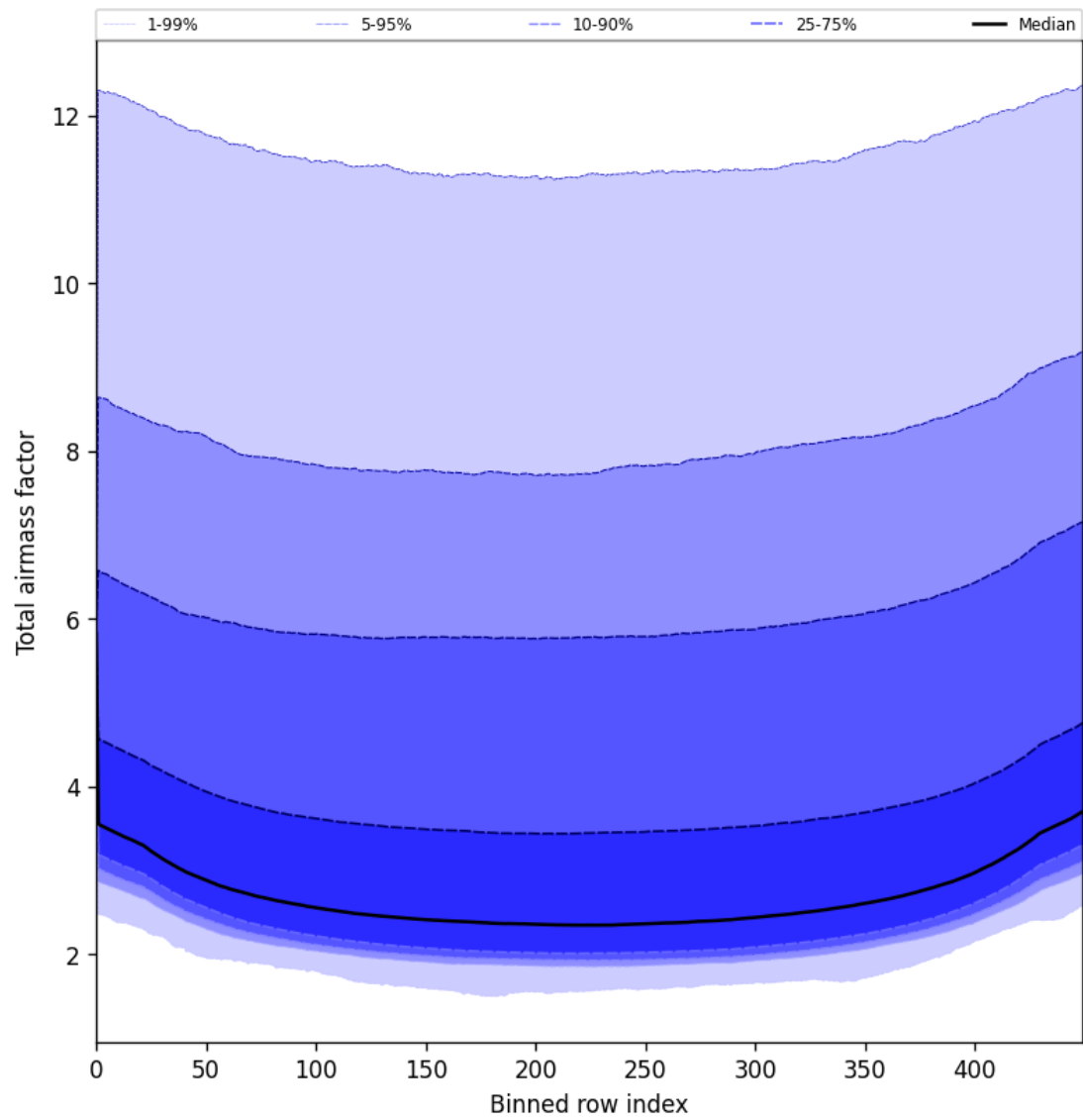
Figure 49: Along track statistics of “Total airmass factor” for 2025-06-01 to 2025-06-02
