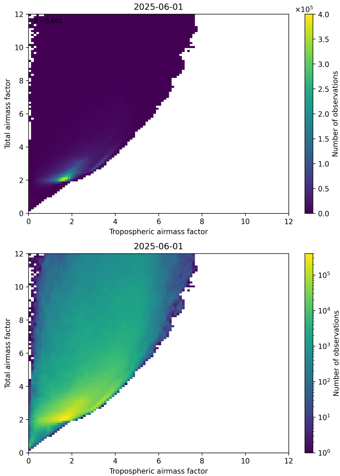
Figure 72: Scatter density plot of “Tropospheric airmass factor” against “Total airmass factor” for 2025-06-01 to 2025-06-02.
