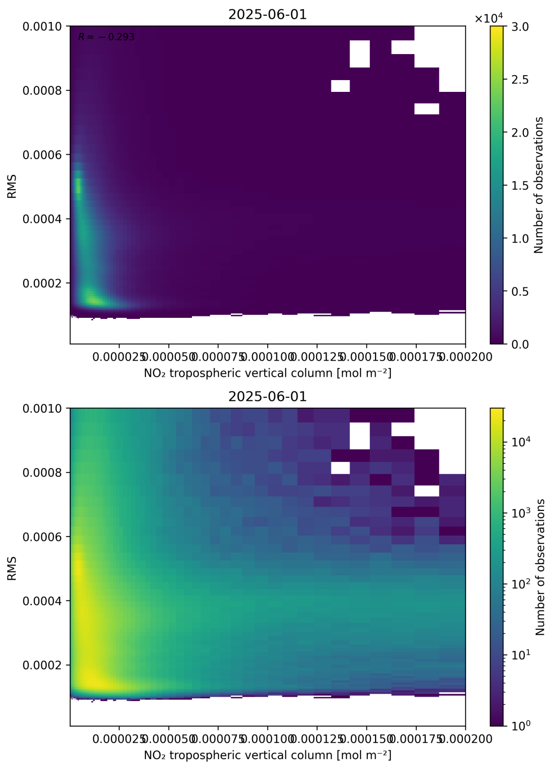
Figure 142: Scatter density plot of “NO 2 tropospheric vertical column” against “RMS” for 2025-06-01 to 2025-06-02.
