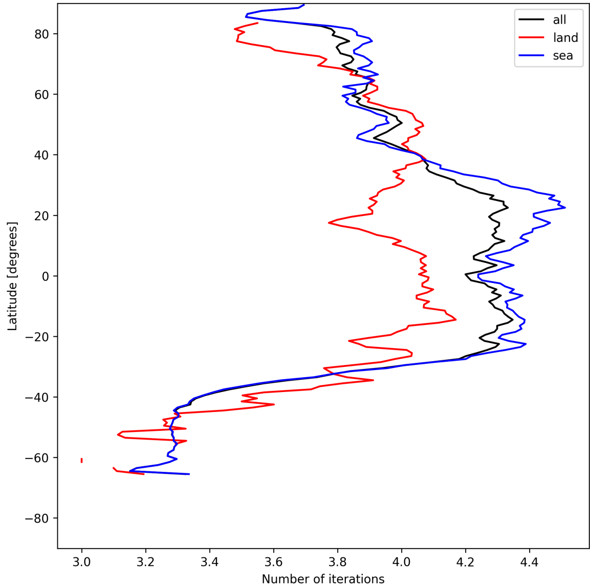
Figure 17: Zonal average of “Number of iterations” for 2025-06-01 to 2025-06-02.
