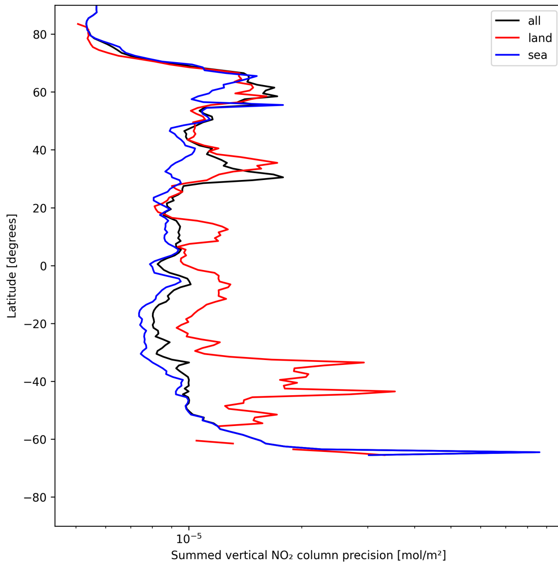
Figure 24: Zonal average of “Summed vertical NO 2 column precision” for 2025-06-01 to 2025-06-02.
