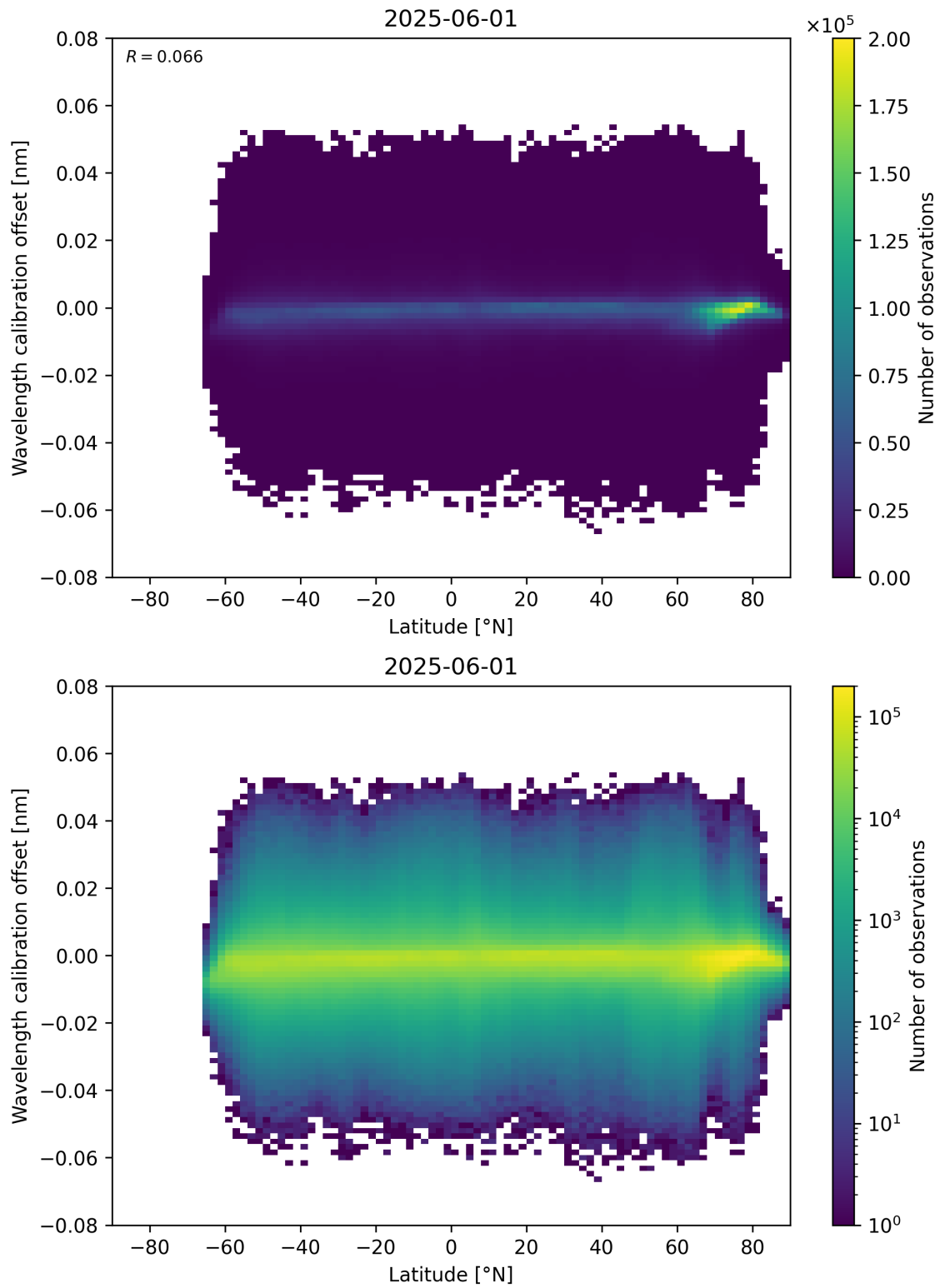
Figure 95: Scatter density plot of “Latitude” against “Wavelength calibration offset” for 2025-06-01 to 2025-06-02.
