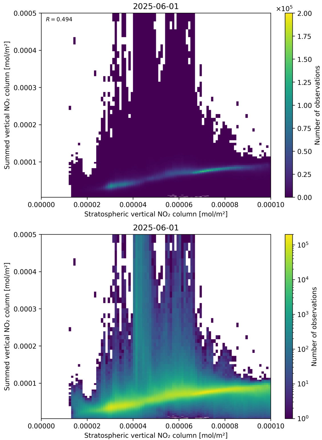
Figure 98: Scatter density plot of “Stratospheric vertical NO 2 column” against “Summed vertical NO 2 column” for 2025-06-01 to 2025-06-02.
