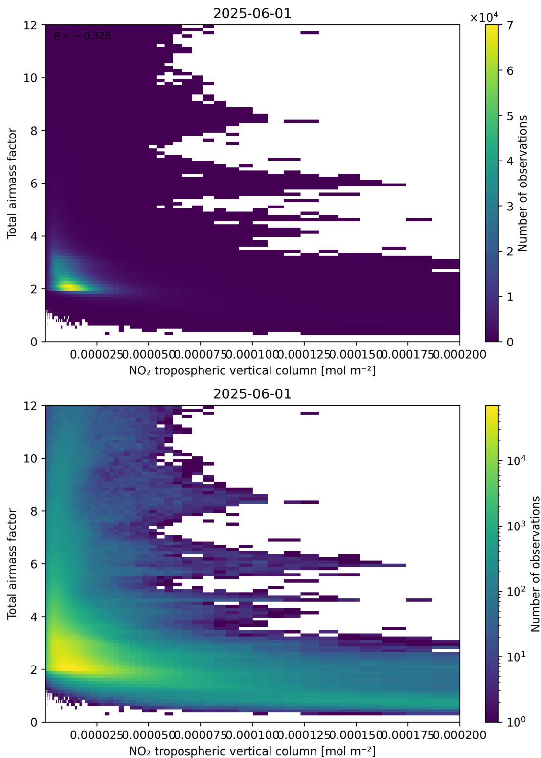
Figure 122: Scatter density plot of “NO 2 tropospheric vertical column” against “Total air mass factor” for 2025-06-01 to 2025-06-02.
