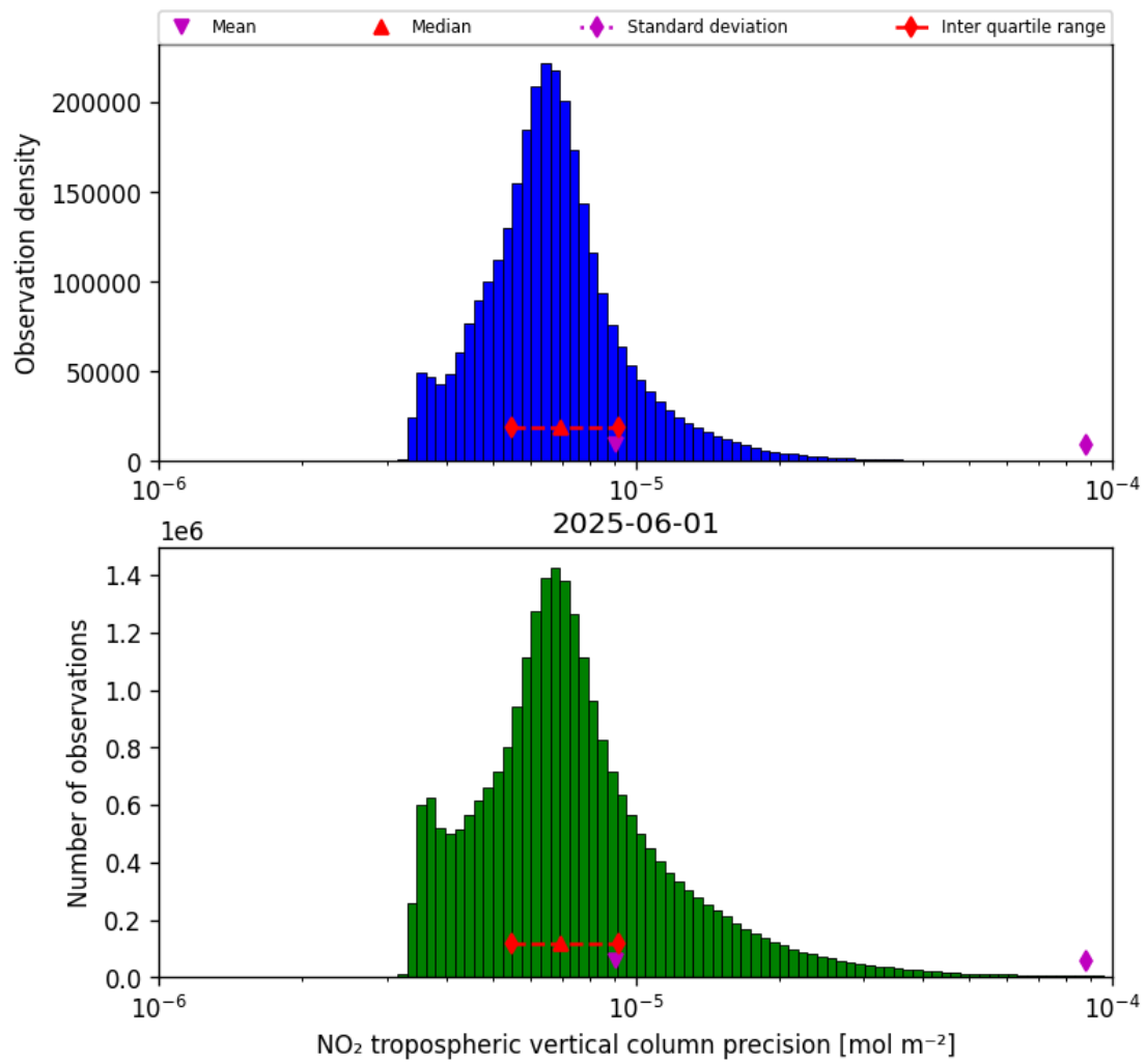
Figure 30: Histogram of “NO 2 tropospheric vertical column precision” for 2025-06-01 to 2025-06-02
