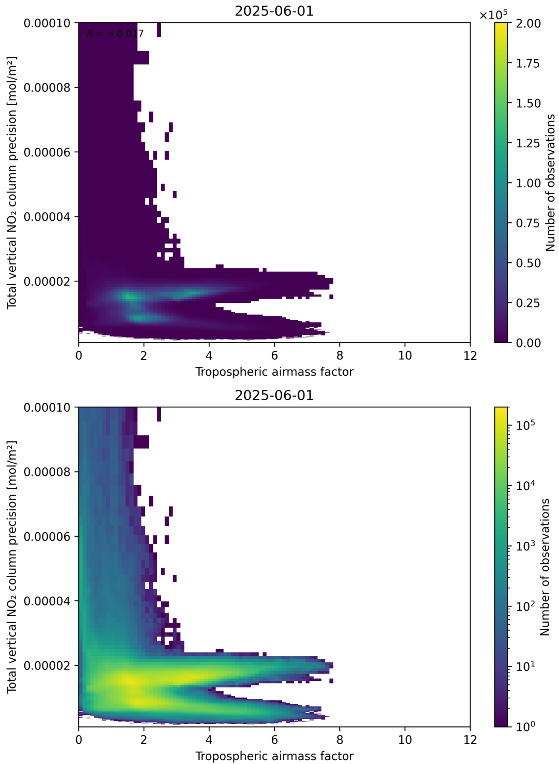
Figure 78: Scatter density plot of “Tropospheric air mass factor” against “Total vertical NO 2 column precision” for 2025-06-01 to 2025-06-02.
