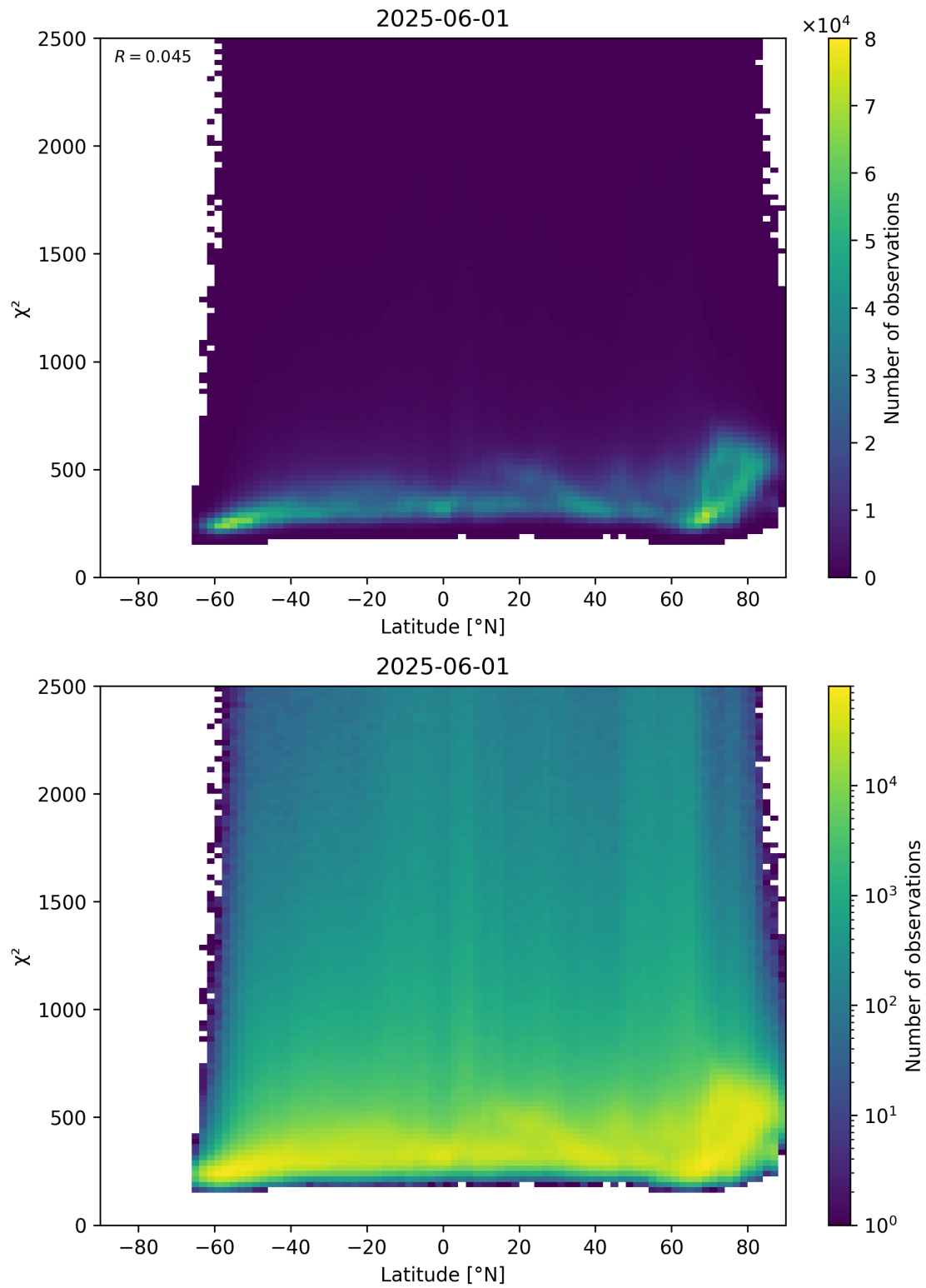
Figure 86: Scatter density plot of “Latitude” against “ \chi^2 ” for 2025-06-01 to 2025-06-02.
