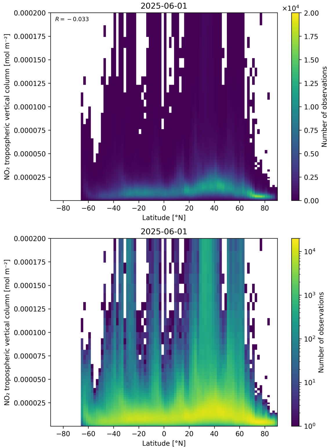
Figure 92: Scatter density plot of “Latitude” against “NO 2 tropospheric vertical column” for 2025-06-01 to 2025-06-02.
