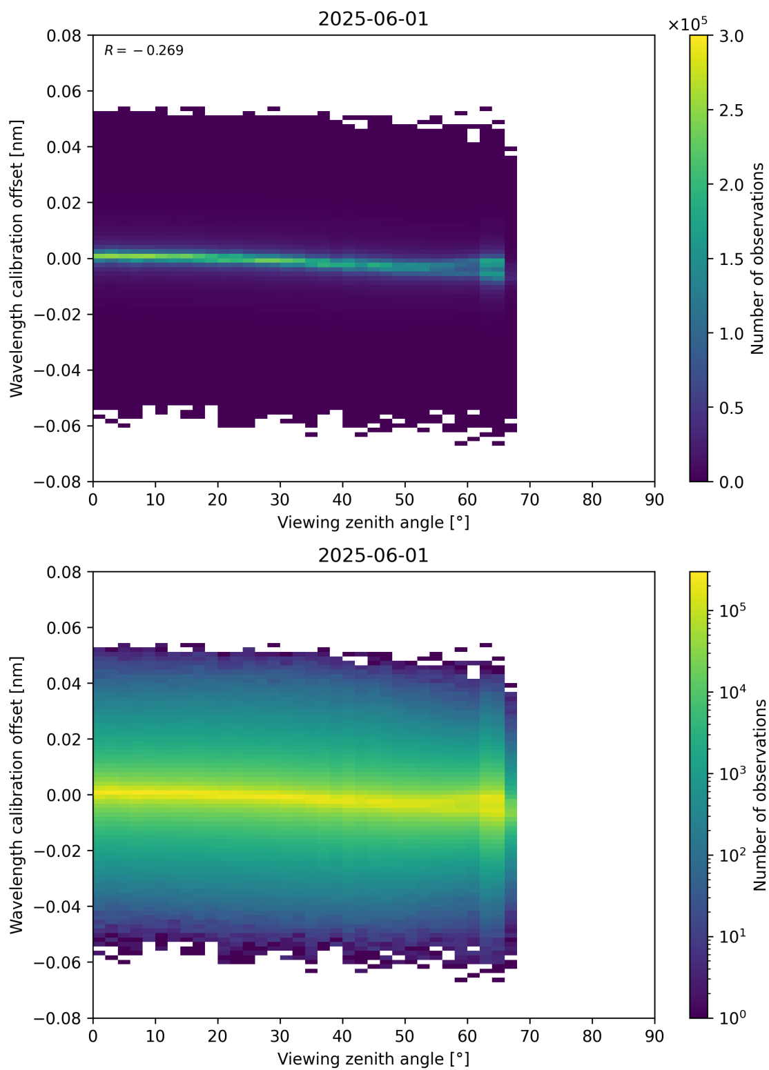
Figure 173: Scatter density plot of “Viewing zenith angle” against “Wavelength calibration offset” for 2025-06-01 to 2025-06-02.
