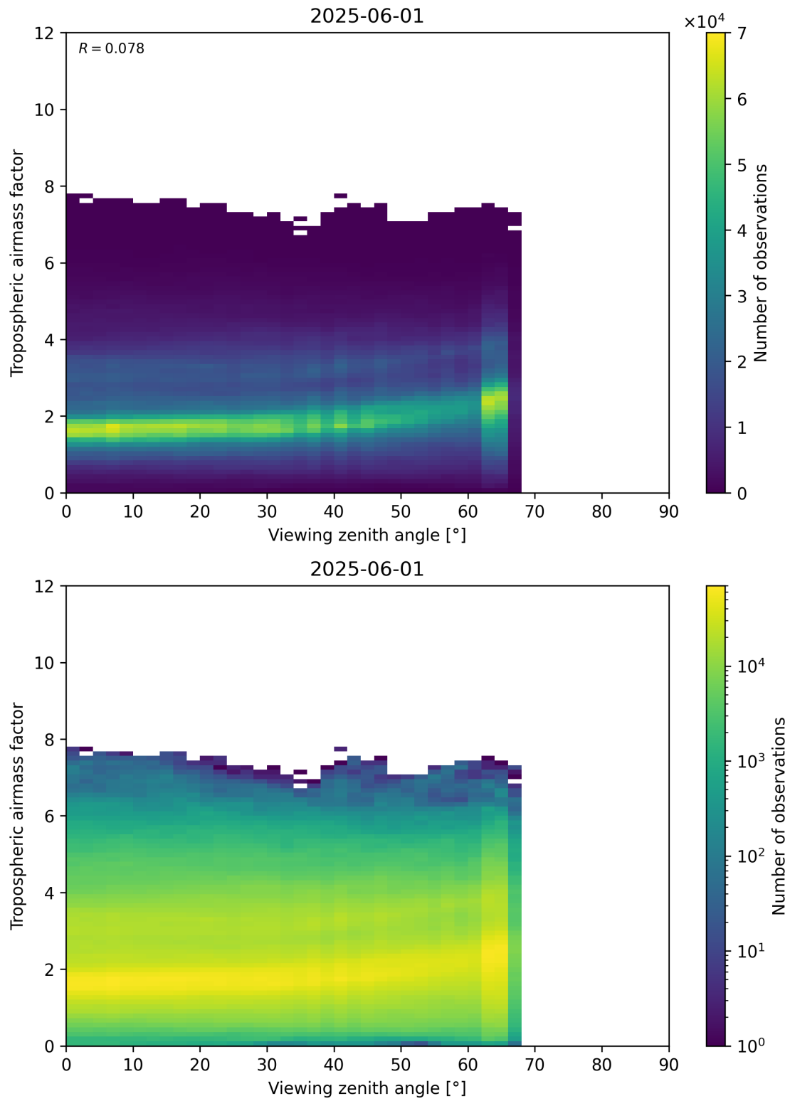
Figure 161: Scatter density plot of “Viewing zenith angle” against “Tropospheric airmass factor” for 2025-06-01 to 2025-06-02.
