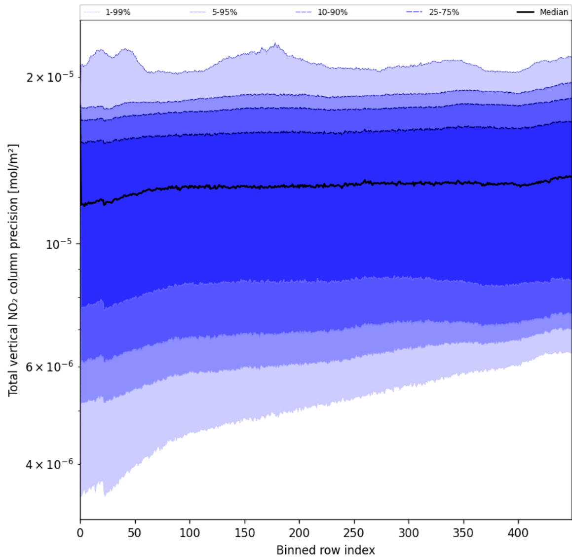
Figure 56: Along track statistics of “Total vertical NO 2 column precision” for 2025-06-01 to 2025-06-02
