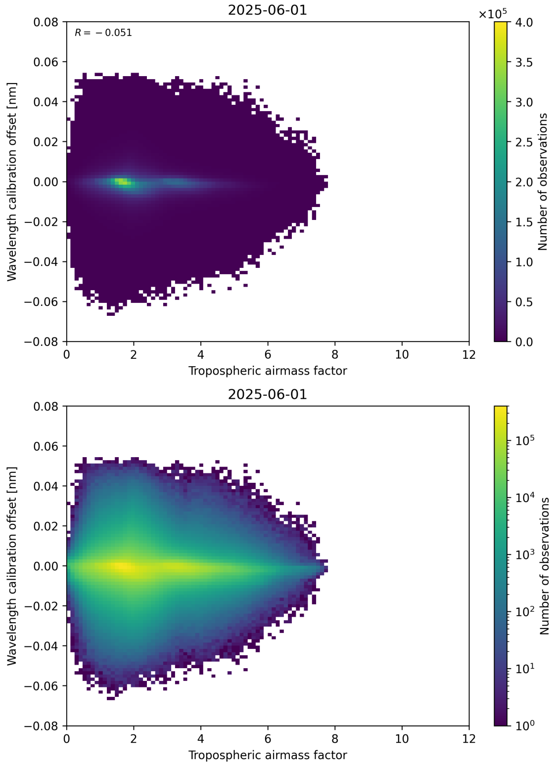
Figure 80: Scatter density plot of “Tropospheric airmass factor” against “Wavelength calibration offset” for 2025-06-01 to 2025-06-02.
