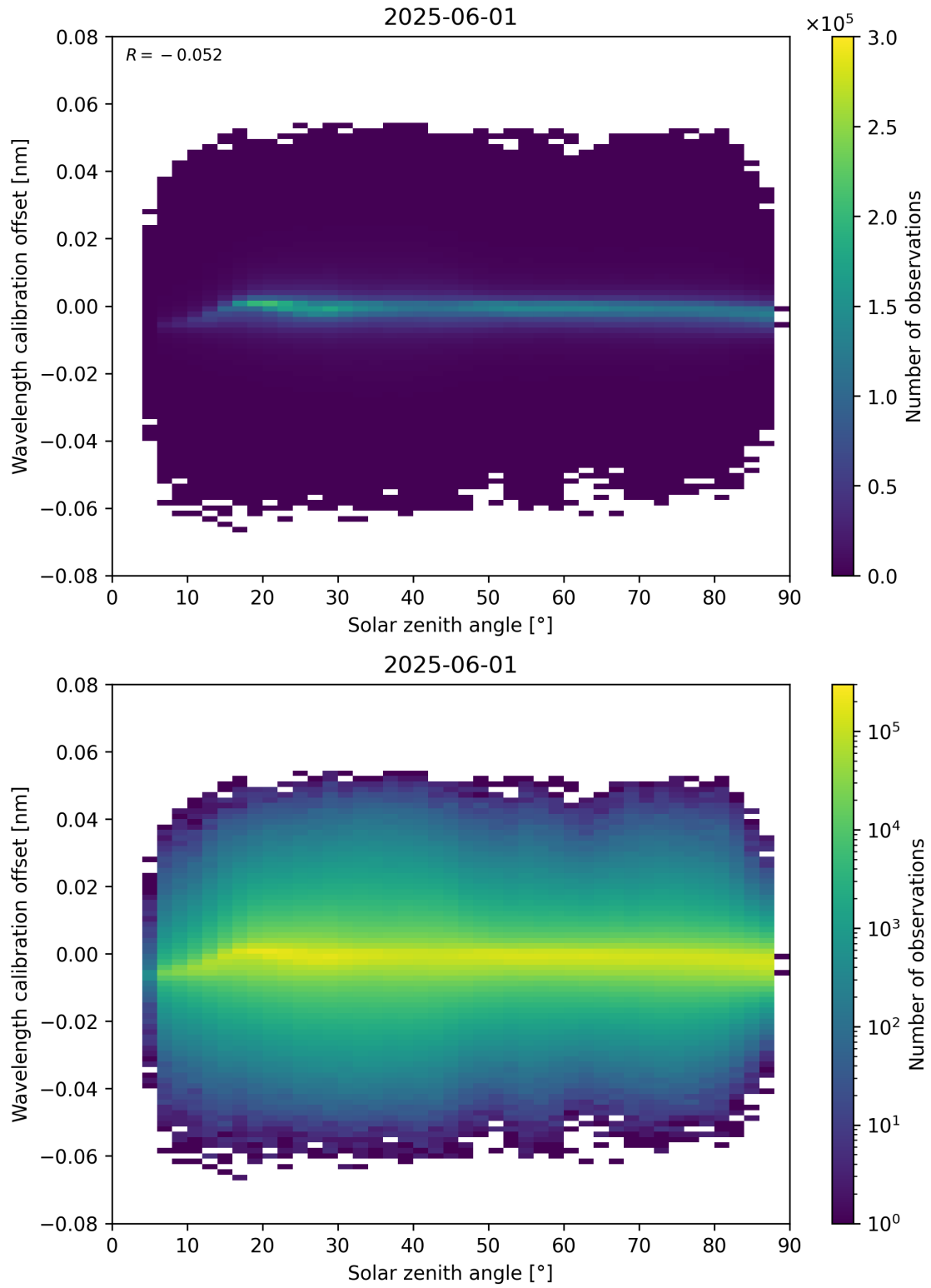
Figure 158: Scatter density plot of “Solar zenith angle” against “Wavelength calibration offset” for 2025-06-01 to 2025-06-02.
