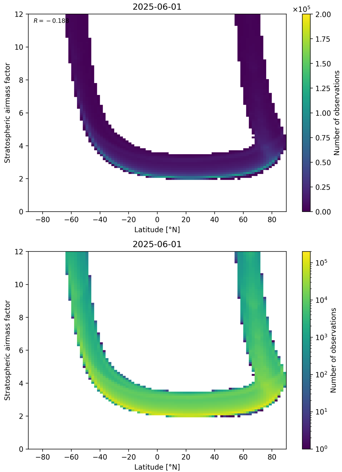
Figure 83: Scatter density plot of “Latitude” against “Stratospheric air mass factor” for 2025-06-01 to 2025-06-02.
