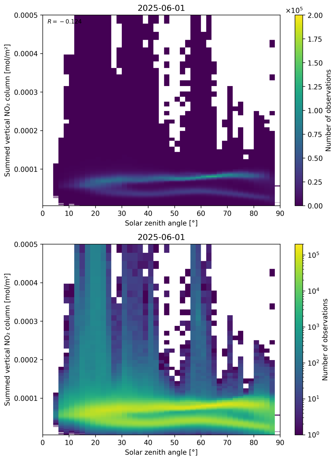
Figure 151: Scatter density plot of “Solar zenith angle” against “Summed vertical NO 2 column” for 2025-06-01 to 2025-06-02.
