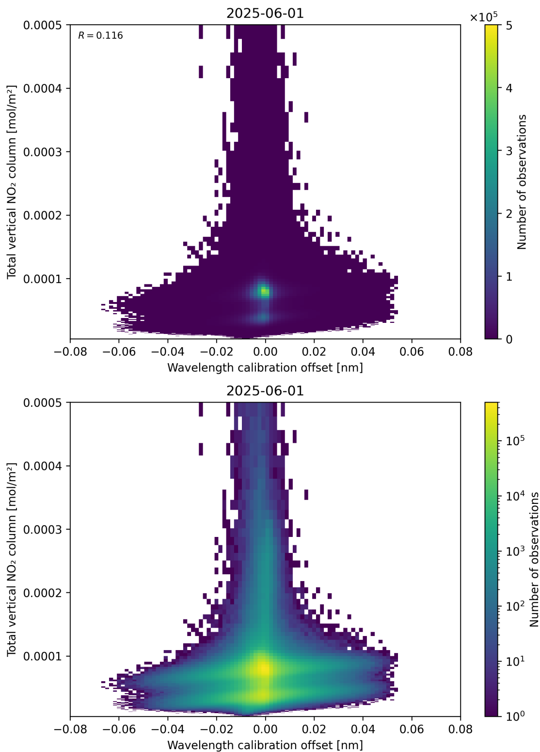
Figure 179: Scatter density plot of “Wavelength calibration offset” against “Total vertical NO 2 column” for 2025-06-01 to 2025-06-02.
