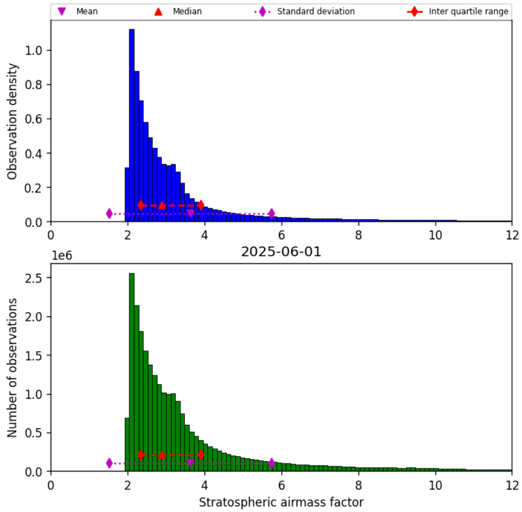
Figure 44: Histogram of “Stratospheric airmass factor” for 2025-06-01 to 2025-06-02
