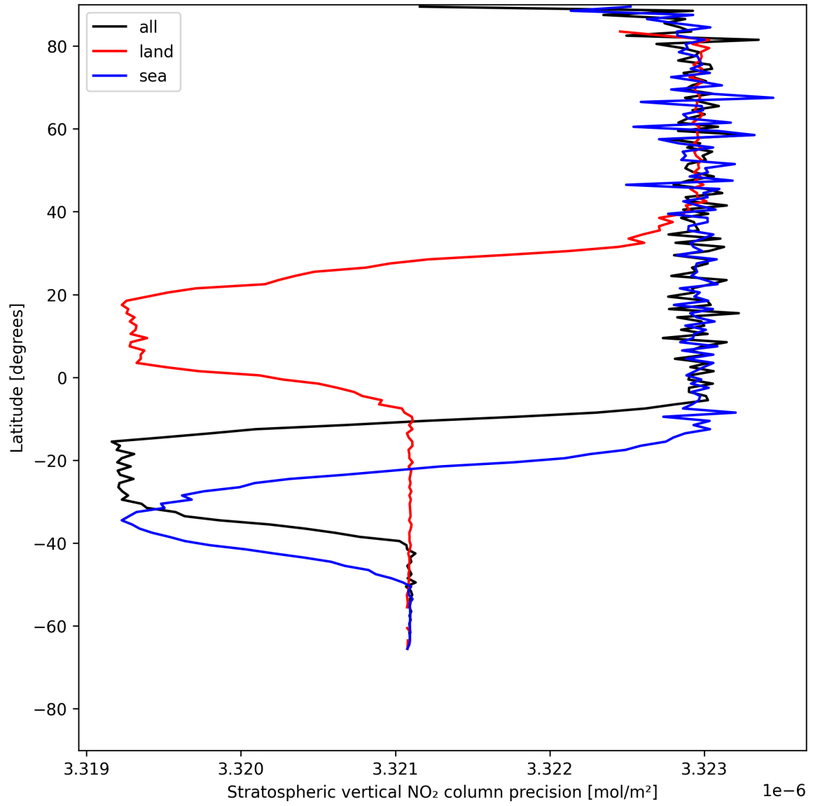
Figure 20: Zonal average of “Stratospheric vertical NO 2 column precision” for 2025-06-01 to 2025-06-02.
