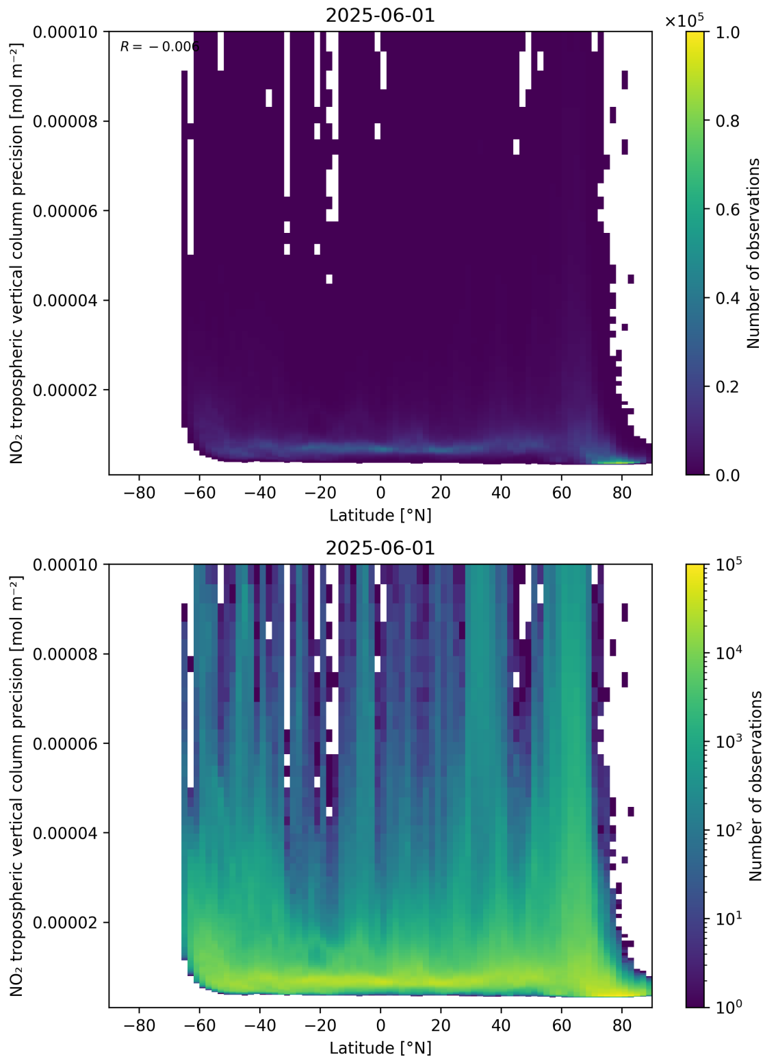
Figure 93: Scatter density plot of “Latitude” against “NO 2 tropospheric vertical column precision” for 2025-06-01 to 2025-06-02.
