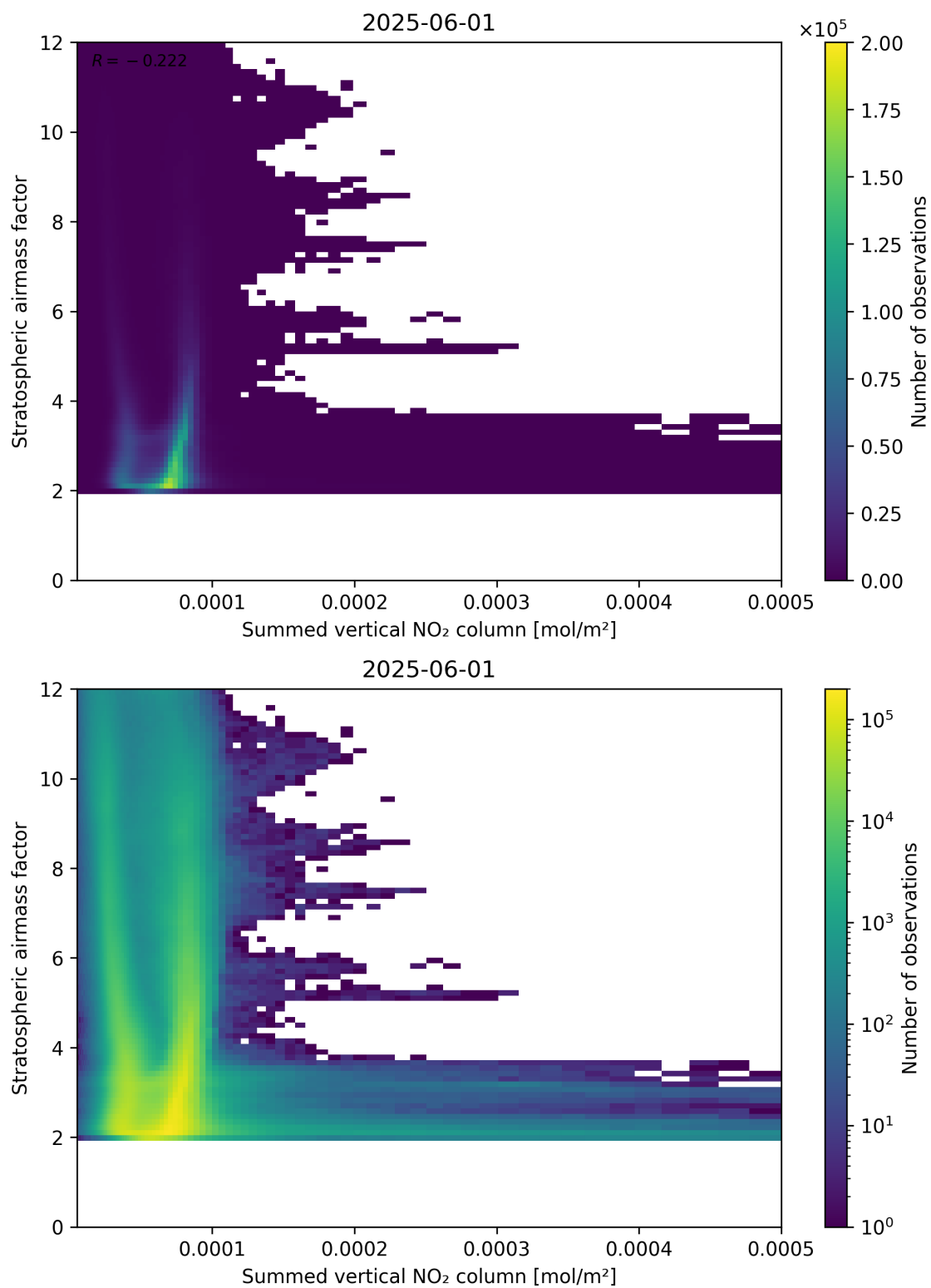
Figure 103: Scatter density plot of “Summed vertical NO 2 column” against “Stratospheric air mass factor” for 2025-06-01 to 2025-06-02.
