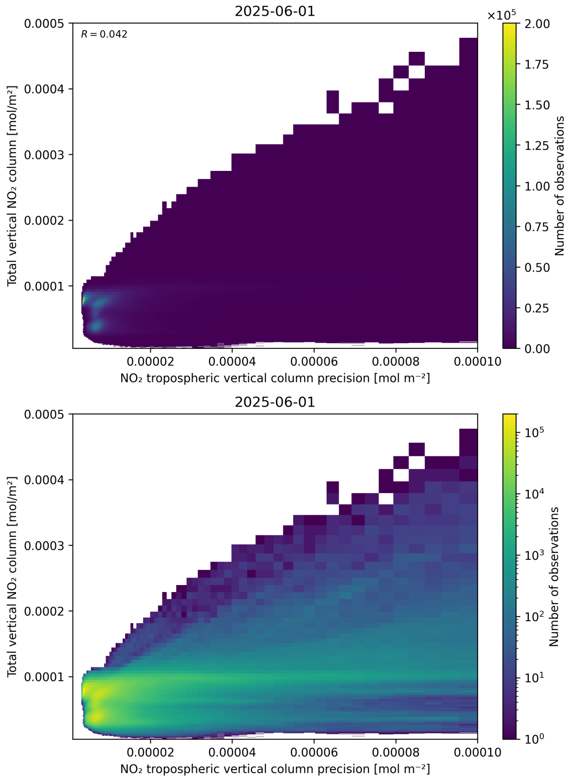
Figure 138: Scatter density plot of “NO 2 tropospheric vertical column precision” against “Total vertical NO 2 column” for 2025-06-01 to 2025-06-02.
