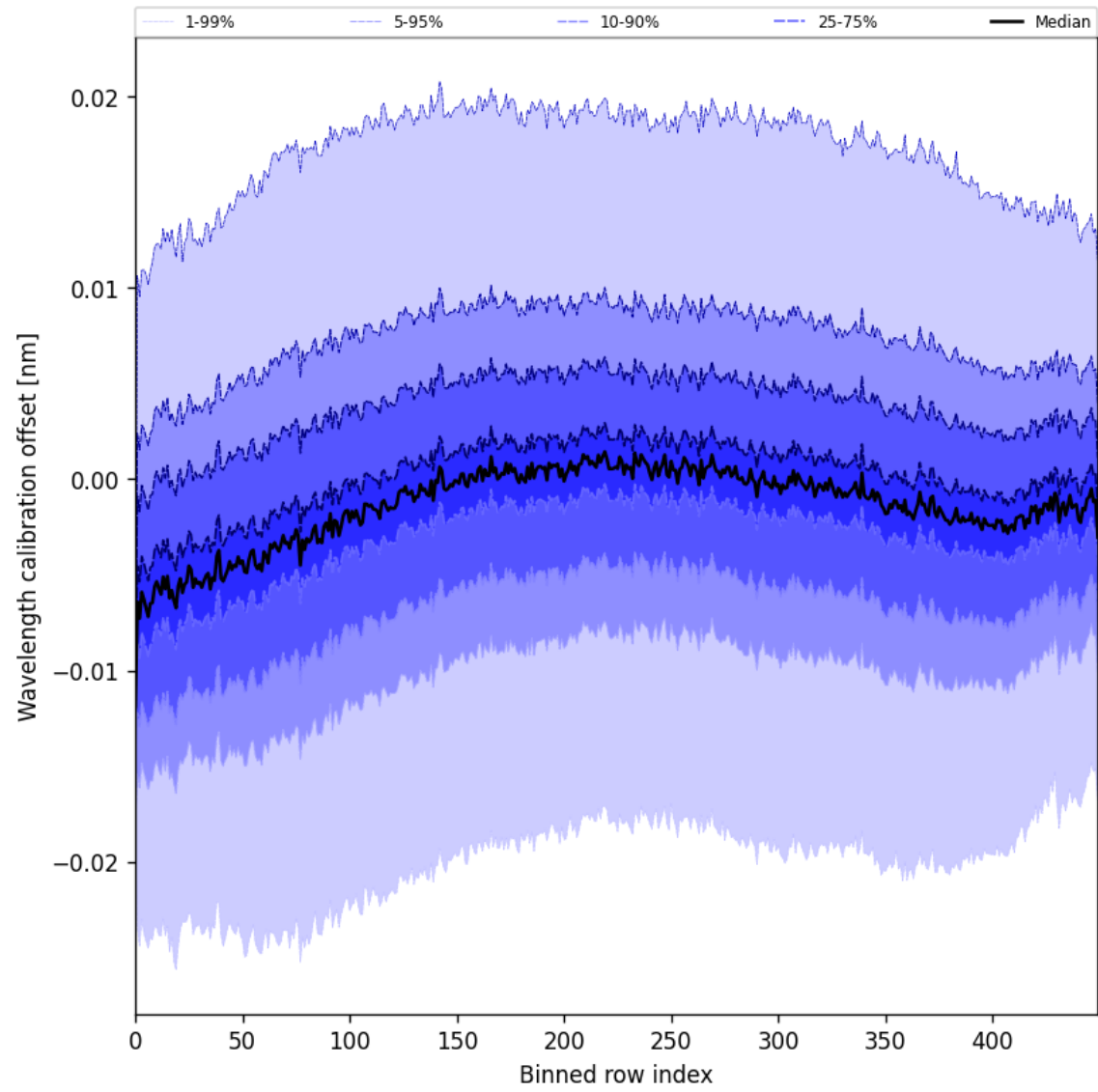
Figure 52: Along track statistics of “Wavelength calibration offset” for 2025-06-01 to 2025-06-02
