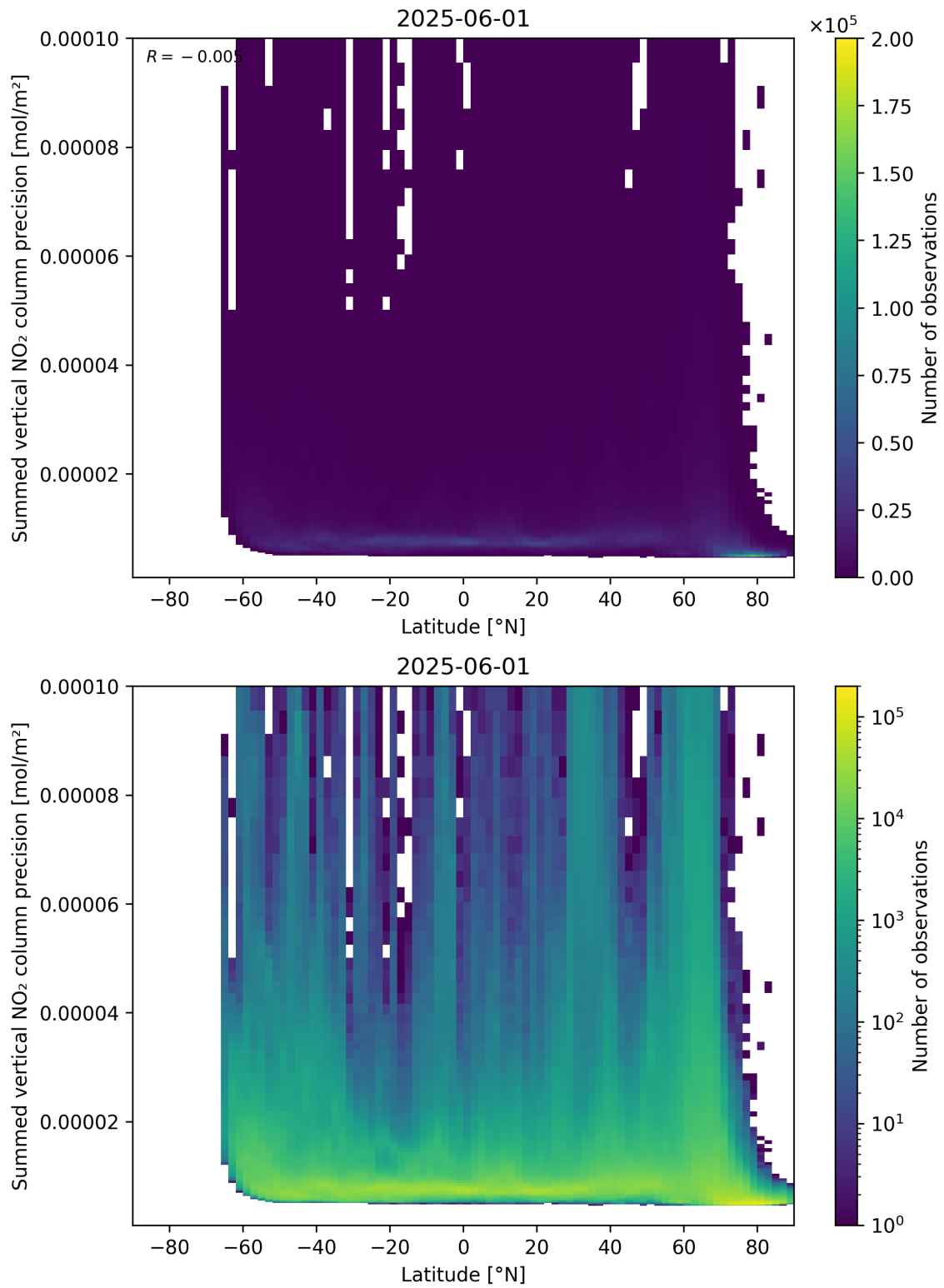
Figure 89: Scatter density plot of “Latitude” against “Summed vertical NO 2 column precision” for 2025-06-01 to 2025-06-02.
