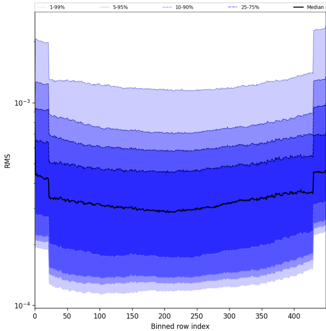
Figure 60: Along track statistics of “RMS” for 2025-06-01 to 2025-06-02
