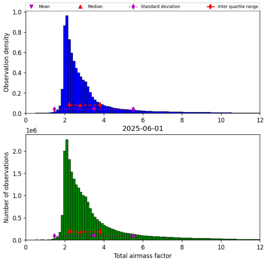
Figure 32: Histogram of “Total airmass factor” for 2025-06-01 to 2025-06-02
