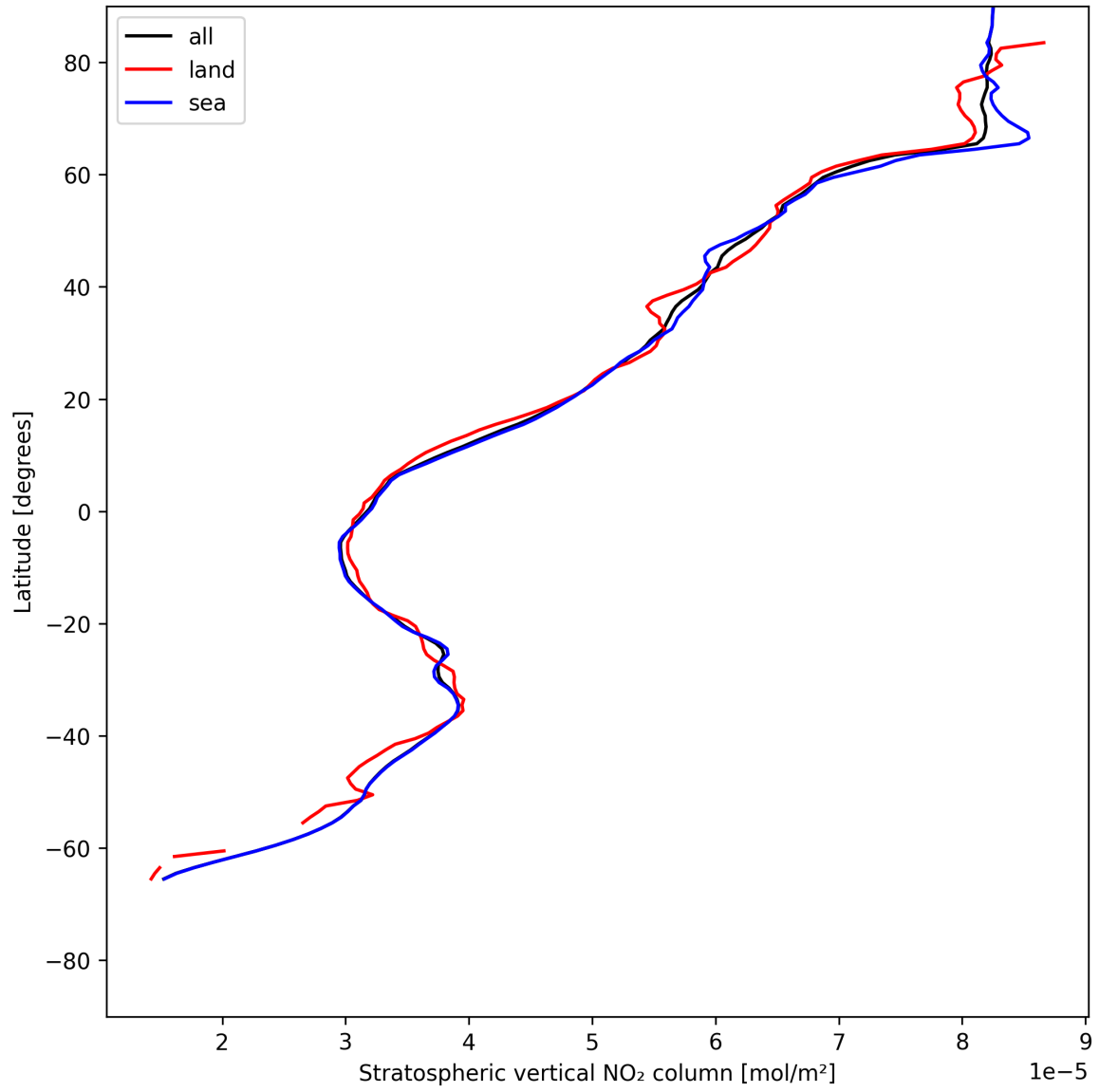
Figure 19: Zonal average of “Stratospheric vertical NO 2 column” for 2025-06-01 to 2025-06-02.
