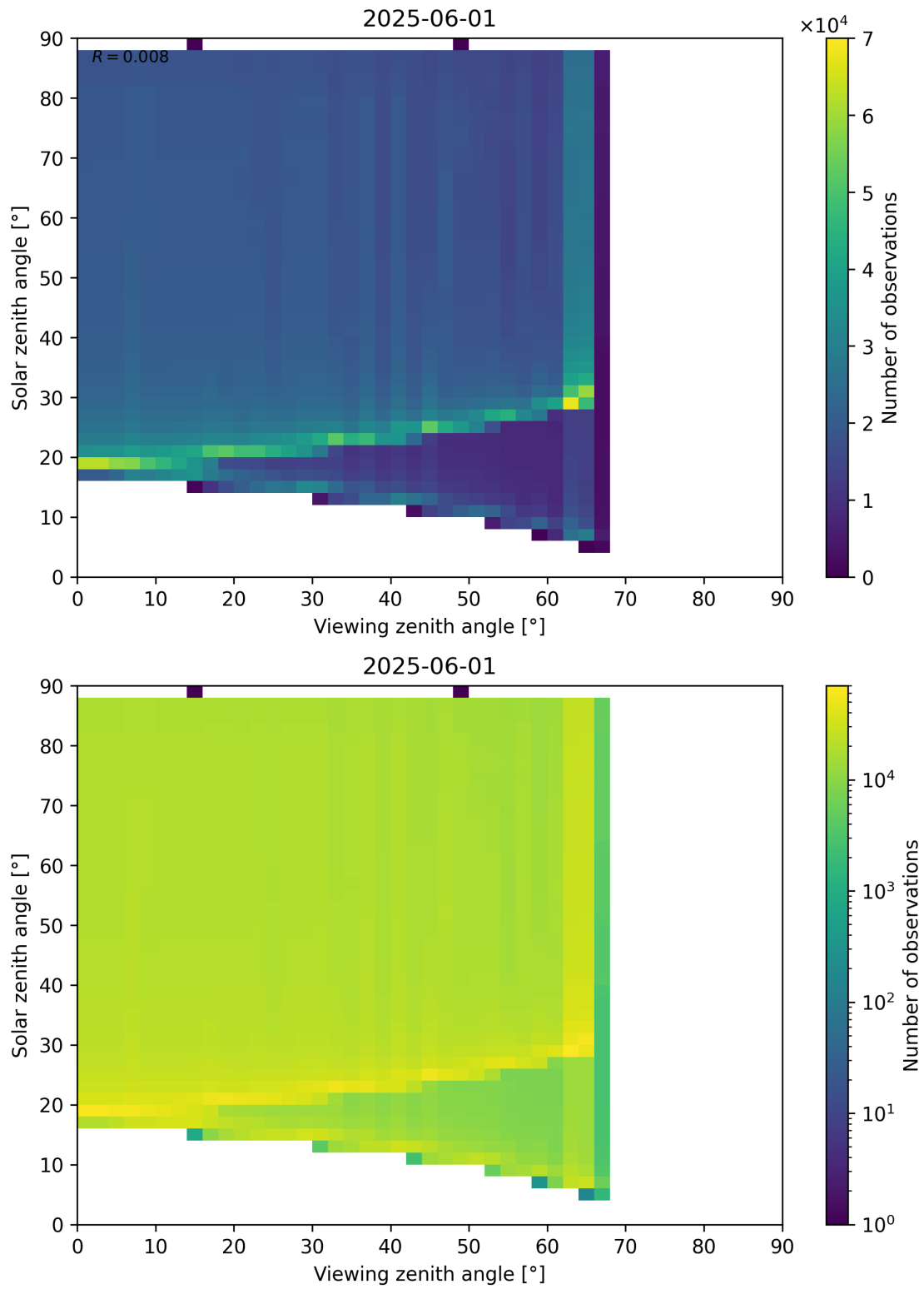
Figure 172: Scatter density plot of “Viewing zenith angle” against “Solar zenith angle” for 2025-06-01 to 2025-06-02.
