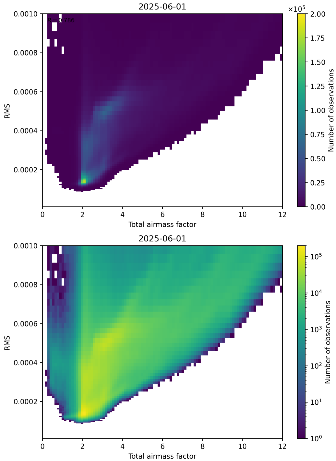
Figure 69: Scatter density plot of “Total airmass factor” against “RMS” for 2025-06-01 to 2025-06-02.
