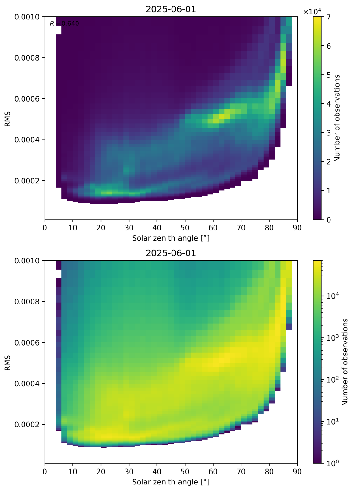
Figure 157: Scatter density plot of “Solar zenith angle” against “RMS” for 2025-06-01 to 2025-06-02.
