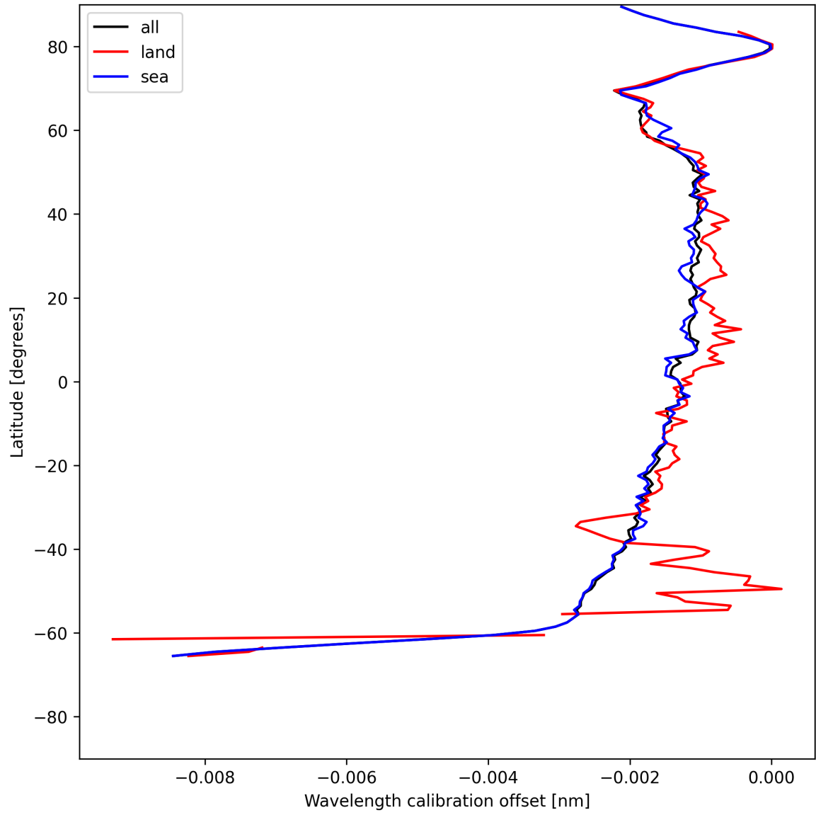
Figure 18: Zonal average of “Wavelength calibration offset” for 2025-06-01 to 2025-06-02.
