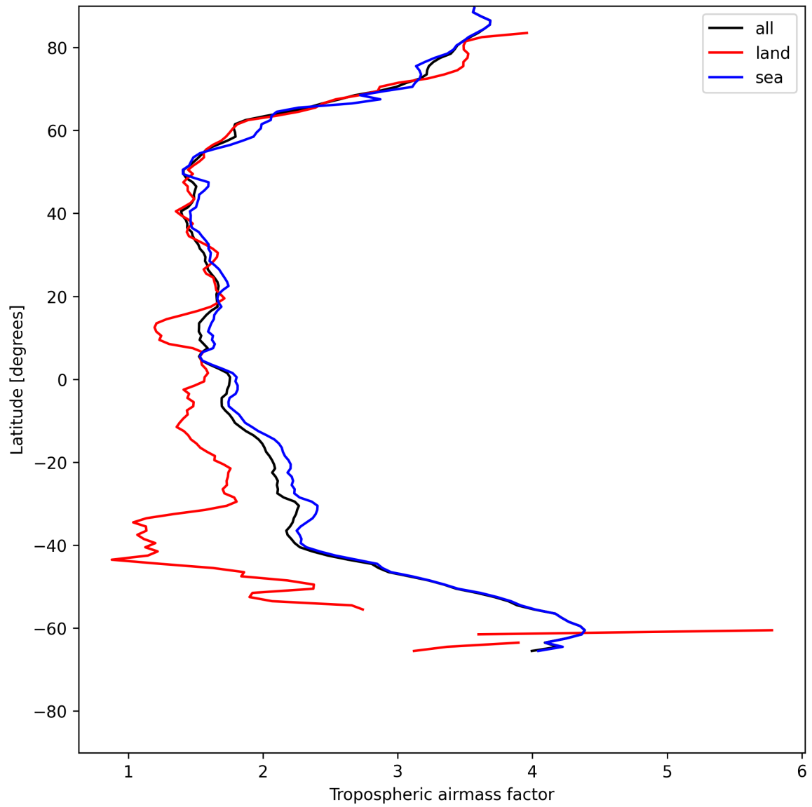
Figure 14: Zonal average of “Tropospheric airmass factor” for 2025-06-01 to 2025-06-02.
