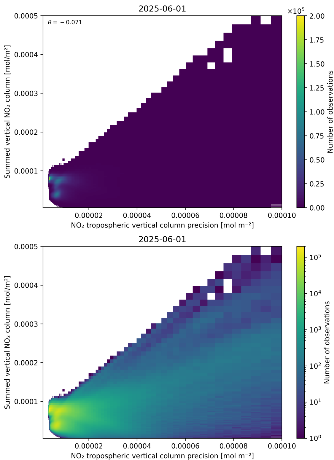
Figure 136: Scatter density plot of “NO 2 tropospheric vertical column precision” against “Summed vertical NO 2 column” for 2025-06-01 to 2025-06-02.
