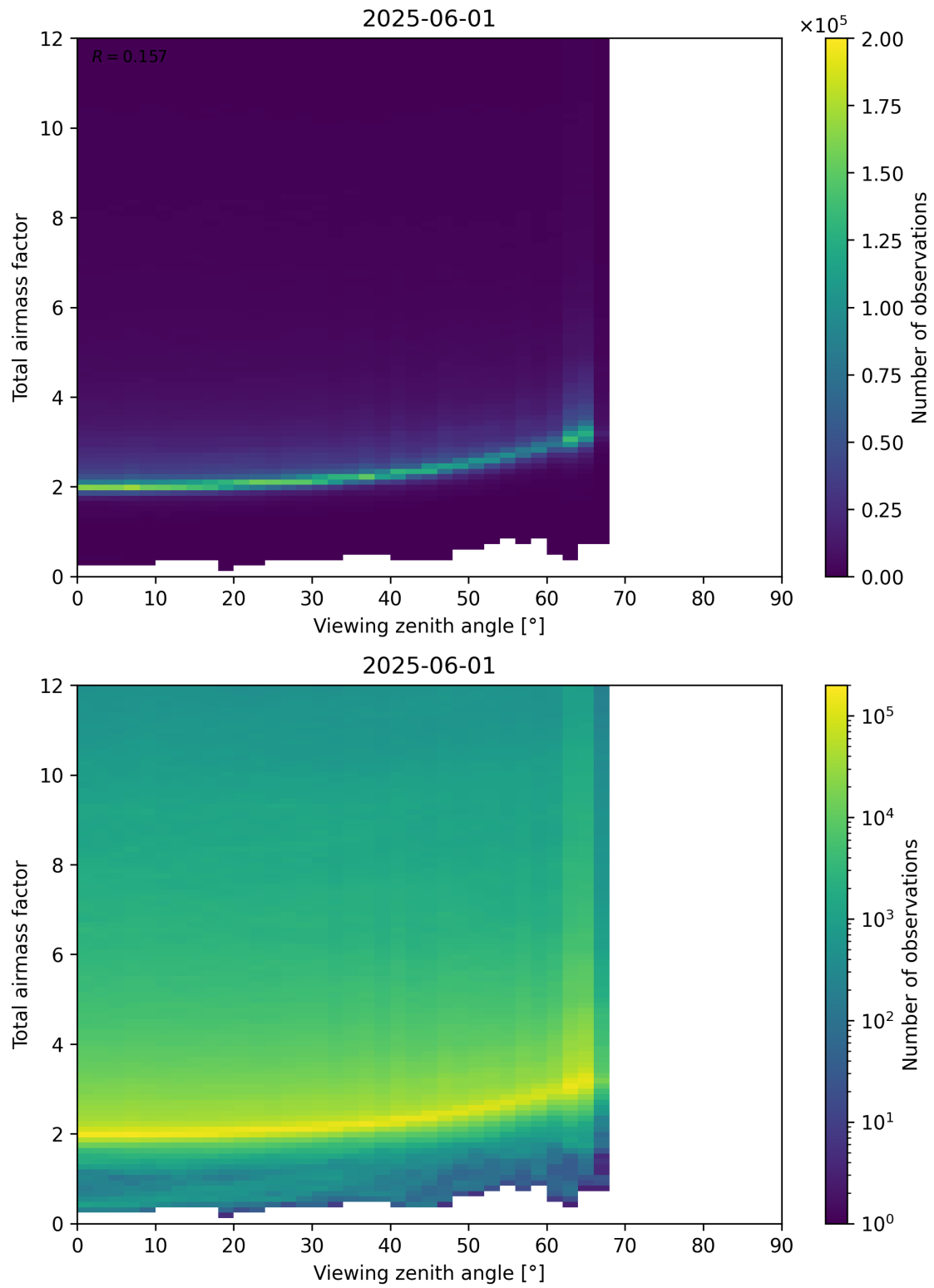
Figure 160: Scatter density plot of “Viewing zenith angle” against “Total airmass factor” for 2025-06-01 to 2025-06-02.
