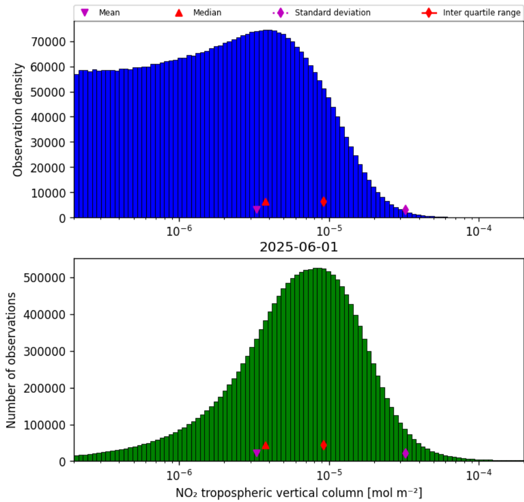
Figure 29: Histogram of “NO 2 tropospheric vertical column” for 2025-06-01 to 2025-06-02
