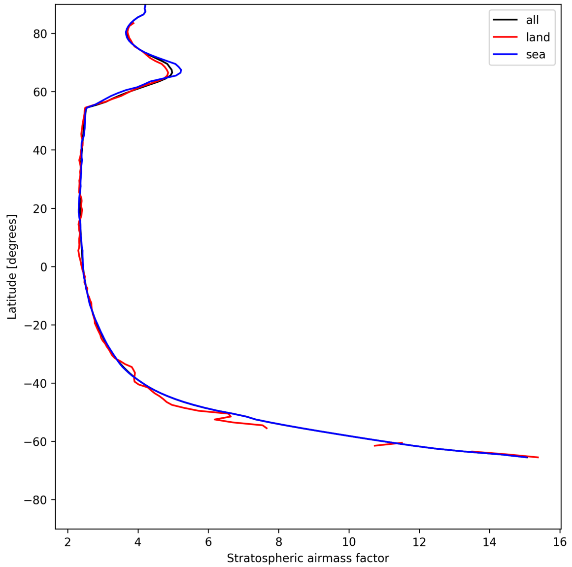
Figure 27: Zonal average of “Stratospheric airmass factor” for 2025-06-01 to 2025-06-02.
