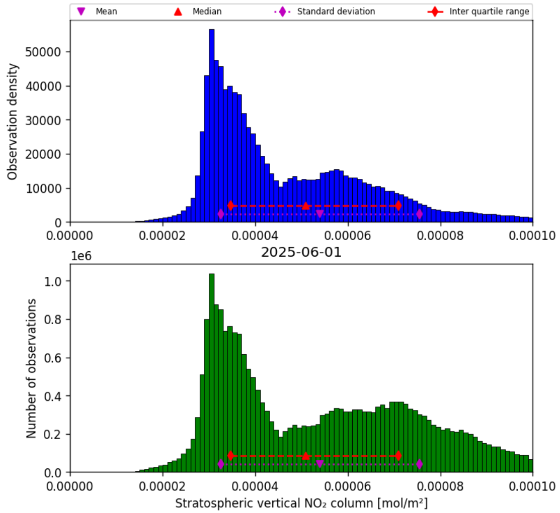
Figure 36: Histogram of “Stratospheric vertical NO 2 column” for 2025-06-01 to 2025-06-02
