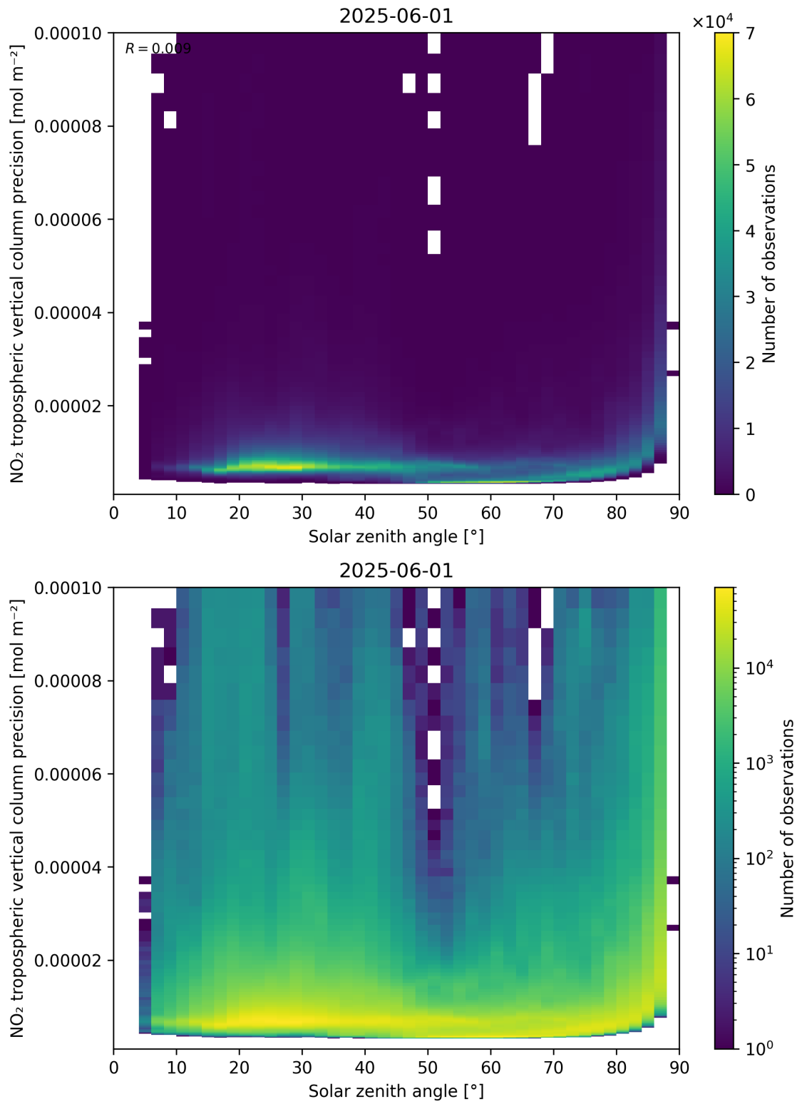
Figure 156: Scatter density plot of “Solar zenith angle” against “NO 2 tropospheric vertical column precision” for 2025-06-01 to 2025-06-02.
