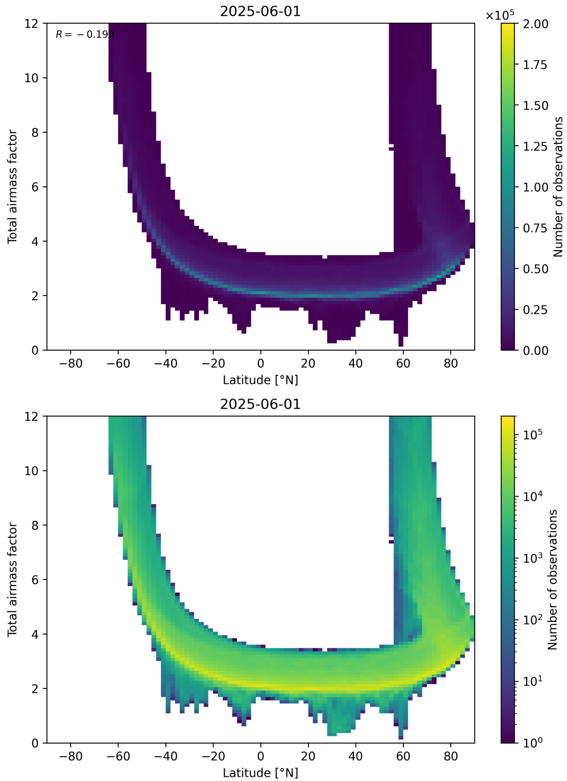
Figure 84: Scatter density plot of “Latitude” against “Total airmass factor” for 2025-06-01 to 2025-06-02.
