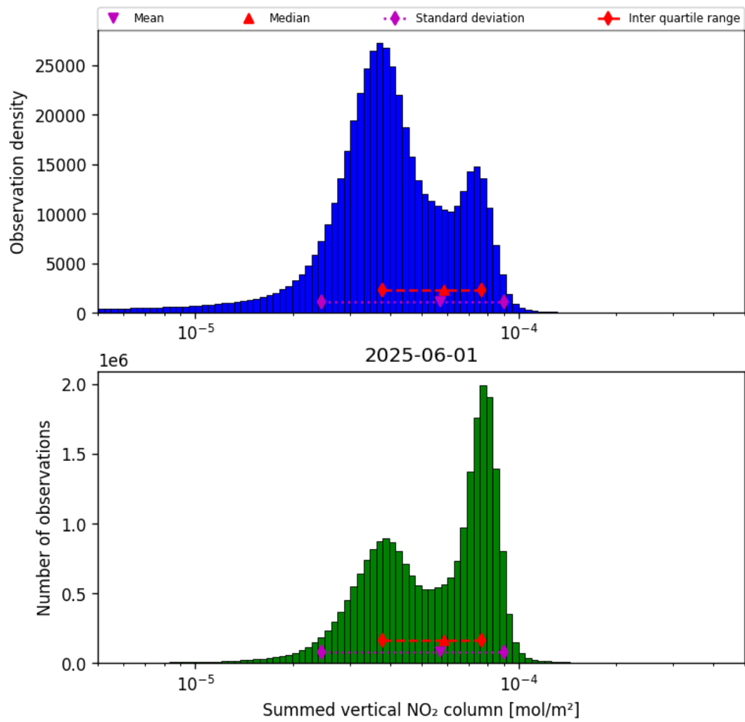
Figure 40: Histogram of “Summed vertical NO 2 column” for 2025-06-01 to 2025-06-02
