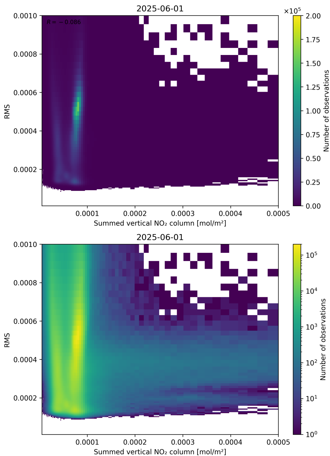
Figure 109: Scatter density plot of “Summed vertical NO 2 column” against “RMS” for 2025-06-01 to 2025-06-02.
