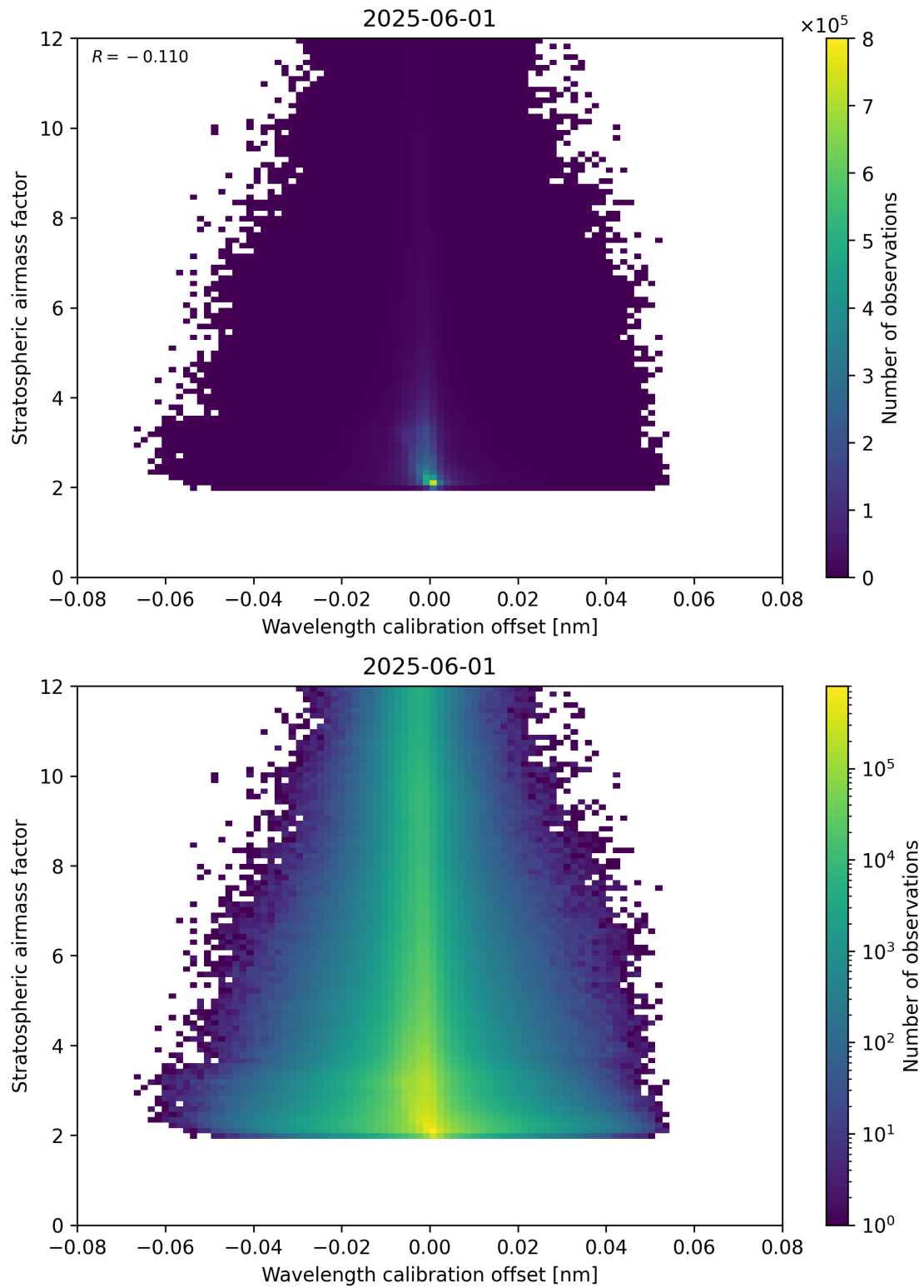
Figure 174: Scatter density plot of “Wavelength calibration offset” against “Stratospheric airmass factor” for 2025-06-01 to 2025-06-02.
