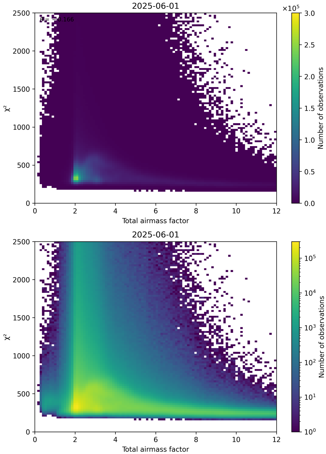
Figure 63: Scatter density plot of “Total airmass factor” against “ \chi^2 ” for 2025-06-01 to 2025-06-02.
