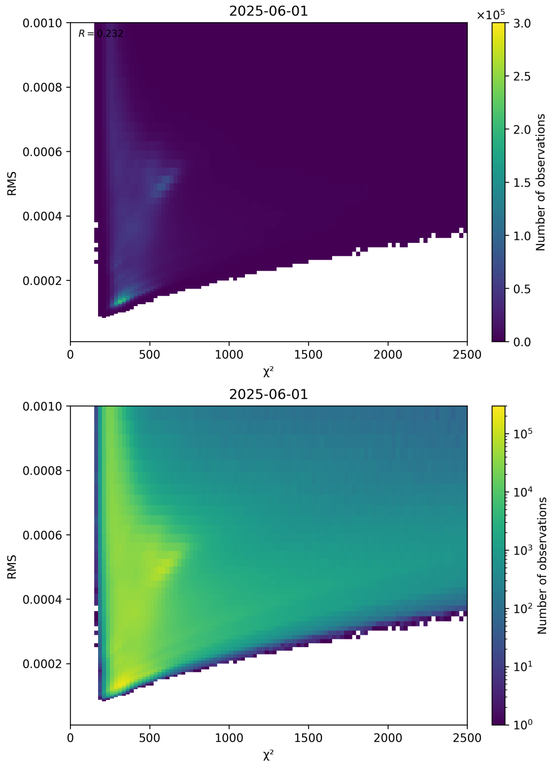
Figure 82: Scatter density plot of “ \chi^2 ” against “RMS” for 2025-06-01 to 2025-06-02.
