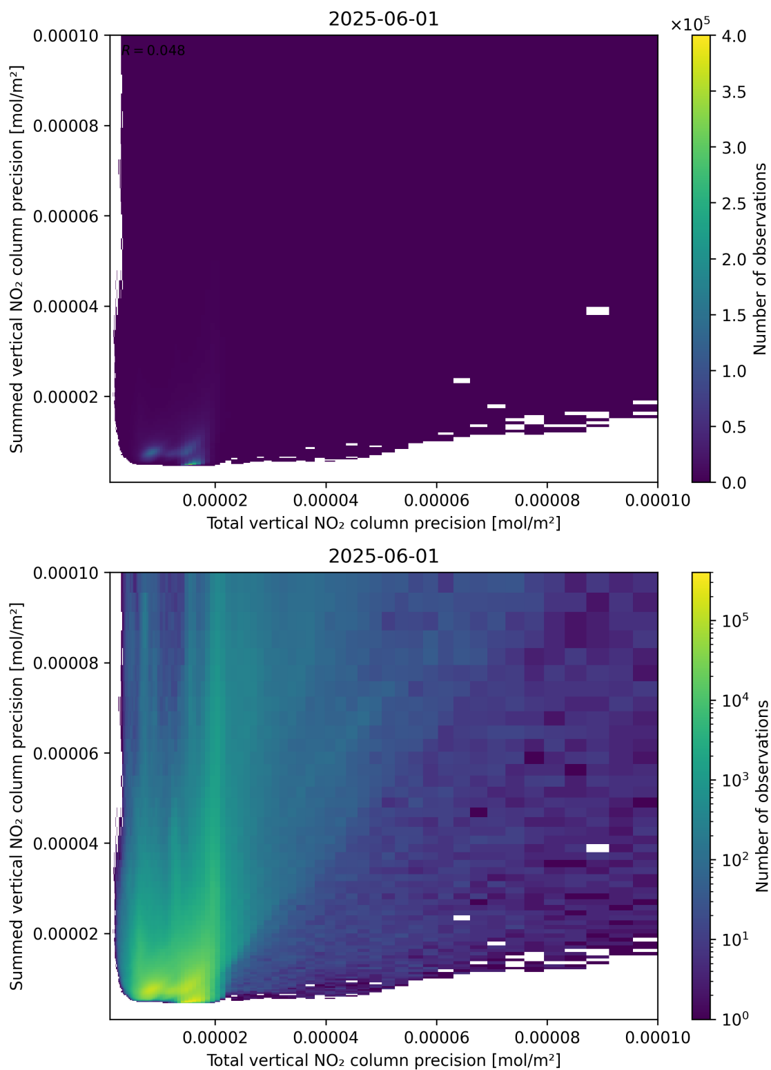
Figure 118: Scatter density plot of “Total vertical NO 2 column precision” against “Summed vertical NO 2 column precision” for 2025-06-01 to 2025-06-02.
