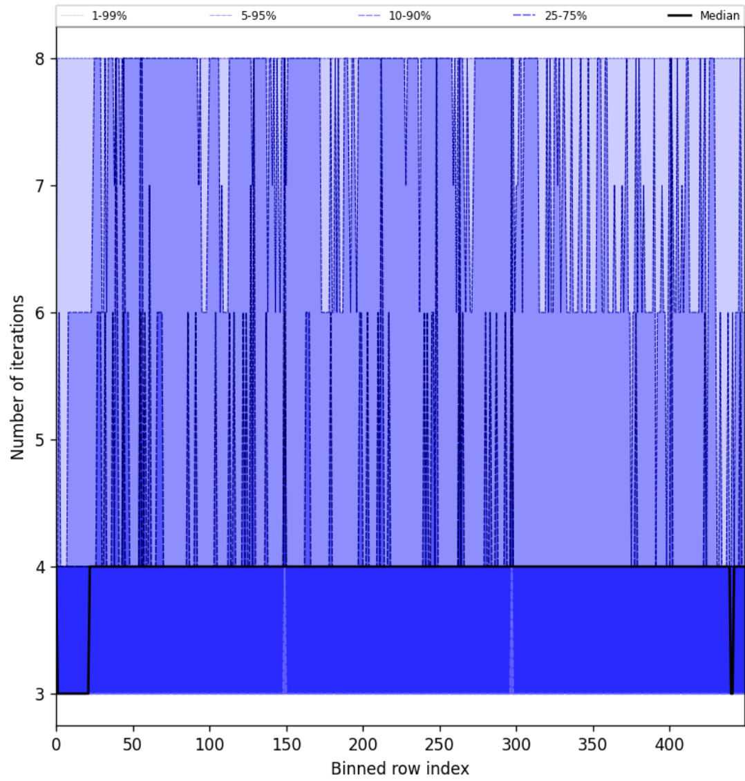
Figure 51: Along track statistics of “Number of iterations” for 2025-06-01 to 2025-06-02
