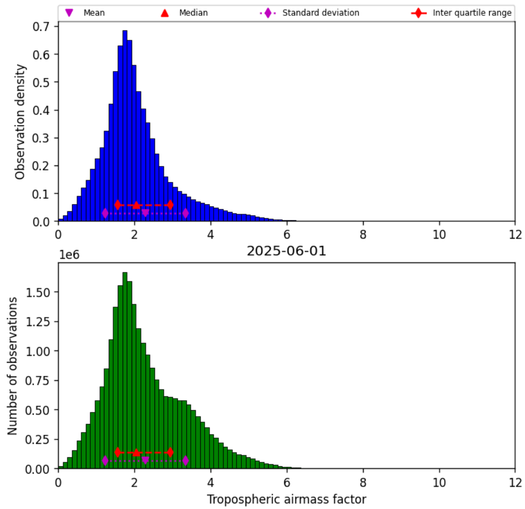
Figure 31: Histogram of “Tropospheric airmass factor” for 2025-06-01 to 2025-06-02
