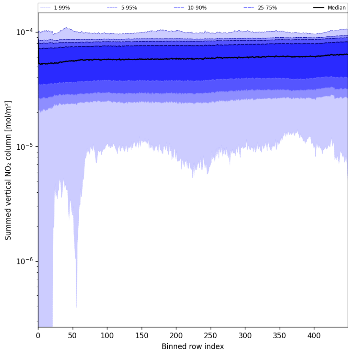
Figure 57: Along track statistics of “Summed vertical NO 2 column” for 2025-06-01 to 2025-06-02
