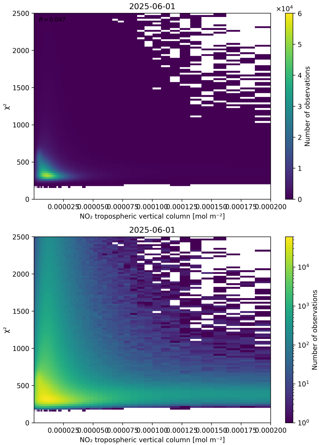
Figure 124: Scatter density plot of “NO 2 tropospheric vertical column” against “ \chi^2 ” for 2025-06-01 to 2025-06-02.
