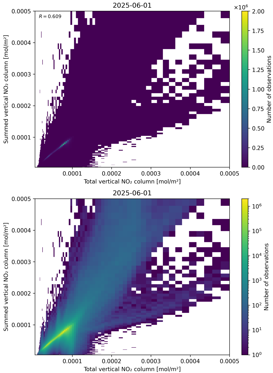
Figure 112: Scatter density plot of “Total vertical NO 2 column” against “Summed vertical NO 2 column” for 2025-06-01 to 2025-06-02.
