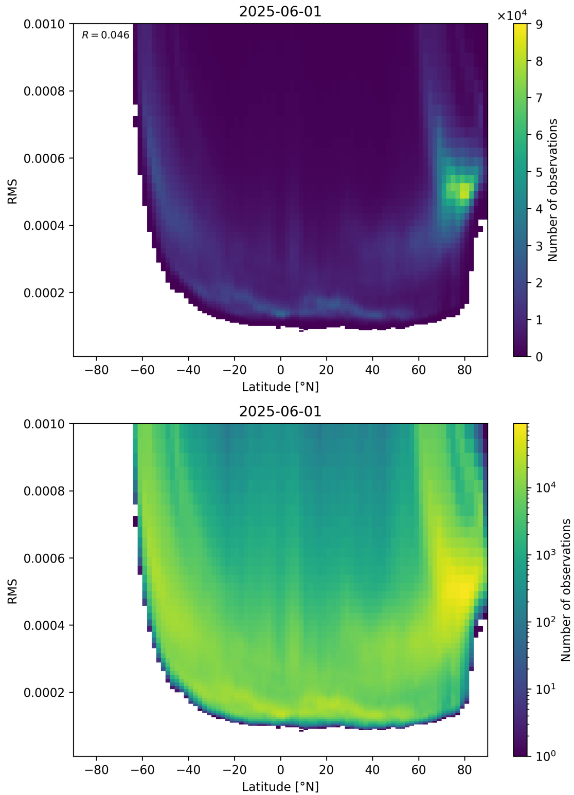
Figure 94: Scatter density plot of “Latitude” against “RMS” for 2025-06-01 to 2025-06-02.
