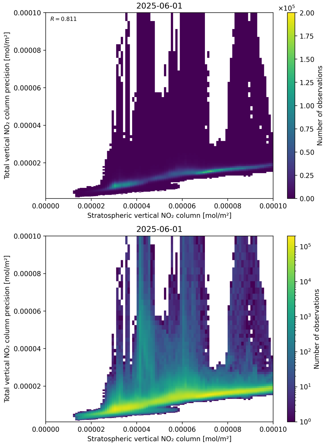
Figure 101: Scatter density plot of “Stratospheric vertical NO 2 column” against “Total vertical NO 2 column precision” for 2025-06-01 to 2025-06-02.
