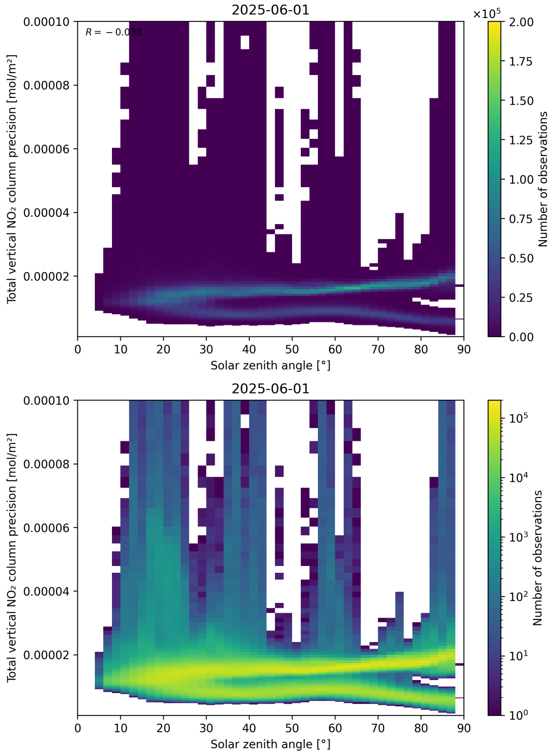
Figure 154: Scatter density plot of “Solar zenith angle” against “Total vertical NO 2 column precision” for 2025-06-01 to 2025-06-02.
