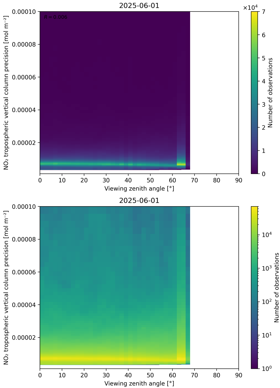
Figure 170: Scatter density plot of “Viewing zenith angle” against “NO 2 tropospheric vertical column precision” for 2025-06-01 to 2025-06-02.
