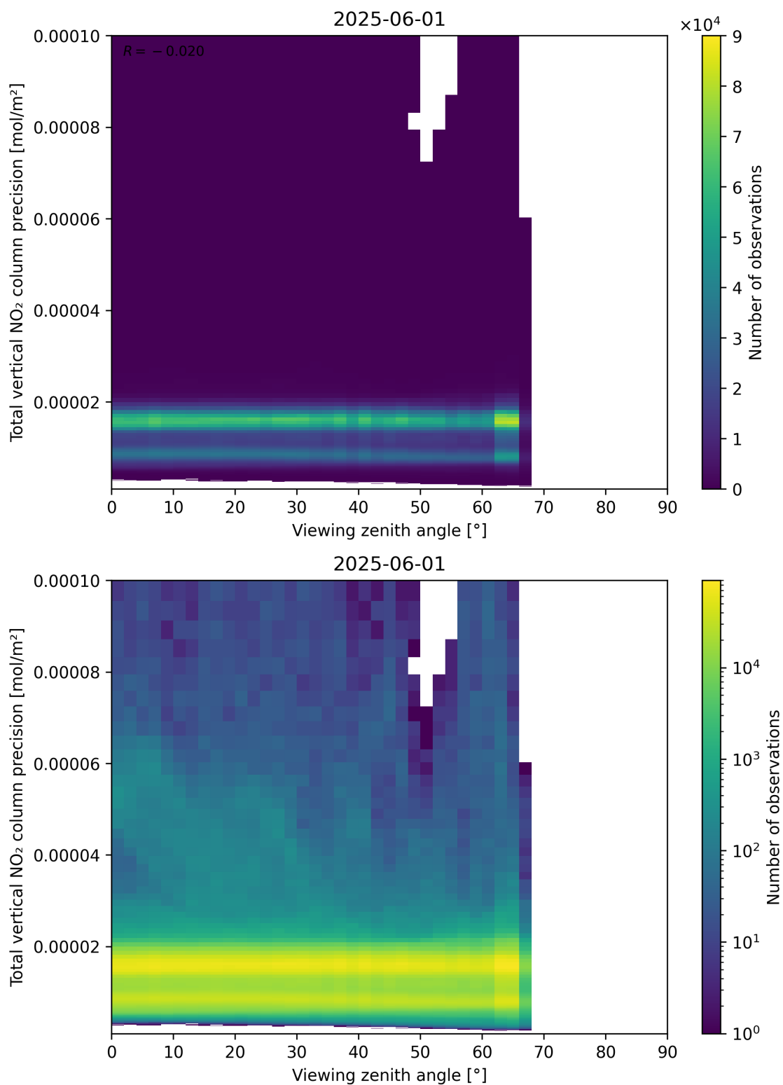
Figure 168: Scatter density plot of “Viewing zenith angle” against “Total vertical NO 2 column precision” for 2025-06-01 to 2025-06-02.
