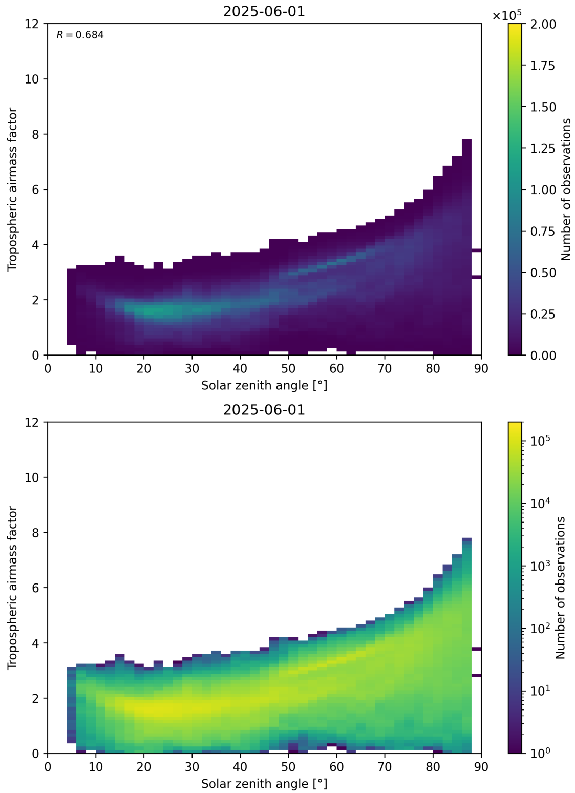
Figure 147: Scatter density plot of “Solar zenith angle” against “Tropospheric airmass factor” for 2025-06-01 to 2025-06-02.
