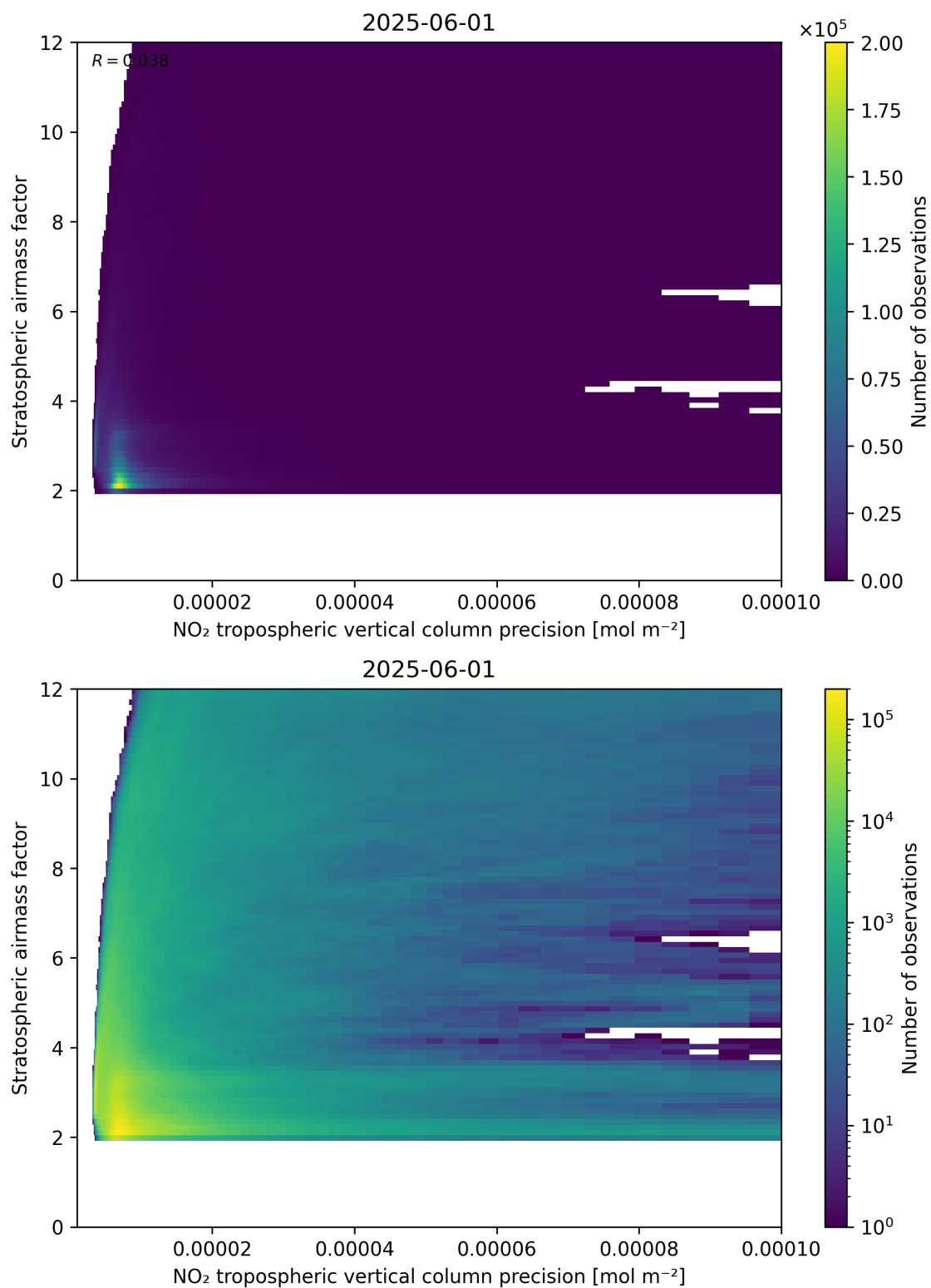
Figure 131: Scatter density plot of “NO 2 tropospheric vertical column precision” against “Stratospheric airmass factor” for 2025-06-01 to 2025-06-02.
