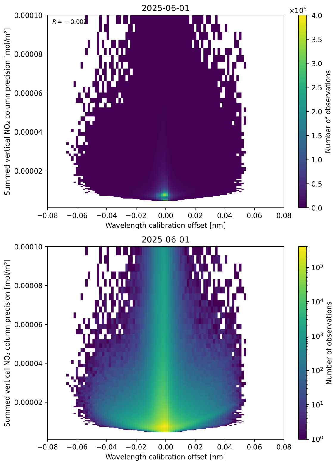
Figure 178: Scatter density plot of “Wavelength calibration offset” against “Summed vertical NO 2 column precision” for 2025-06-01 to 2025-06-02.
