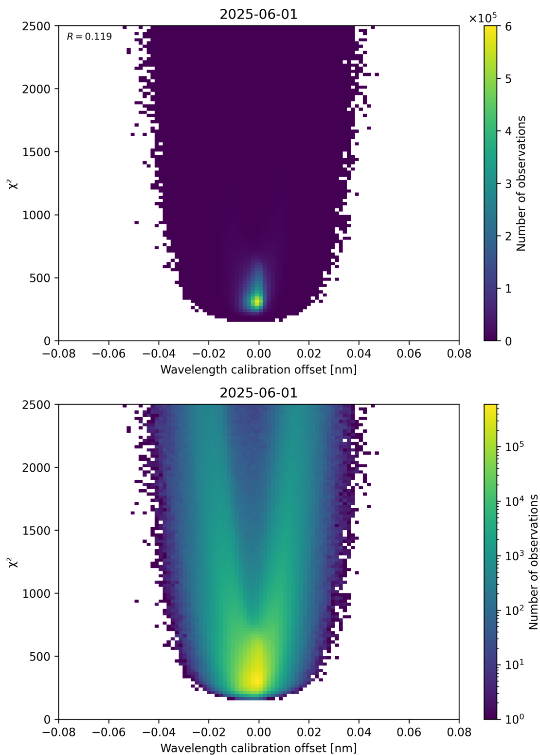
Figure 175: Scatter density plot of “Wavelength calibration offset” against “ \chi^2 ” for 2025-06-01 to 2025-06-02.
