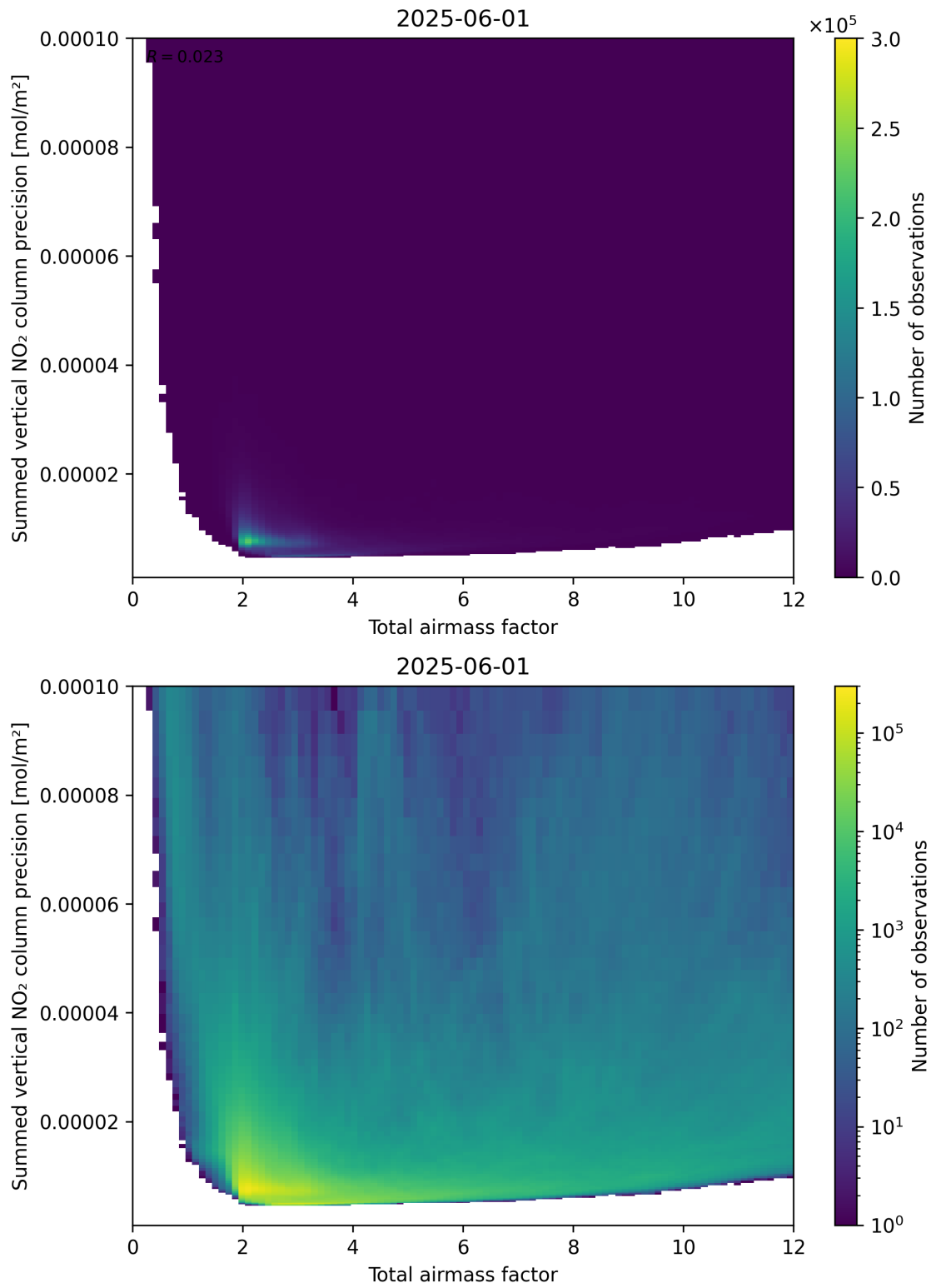
Figure 66: Scatter density plot of “Total airmass factor” against “Summed vertical NO 2 column precision” for 2025-06-01 to 2025-06-02.
