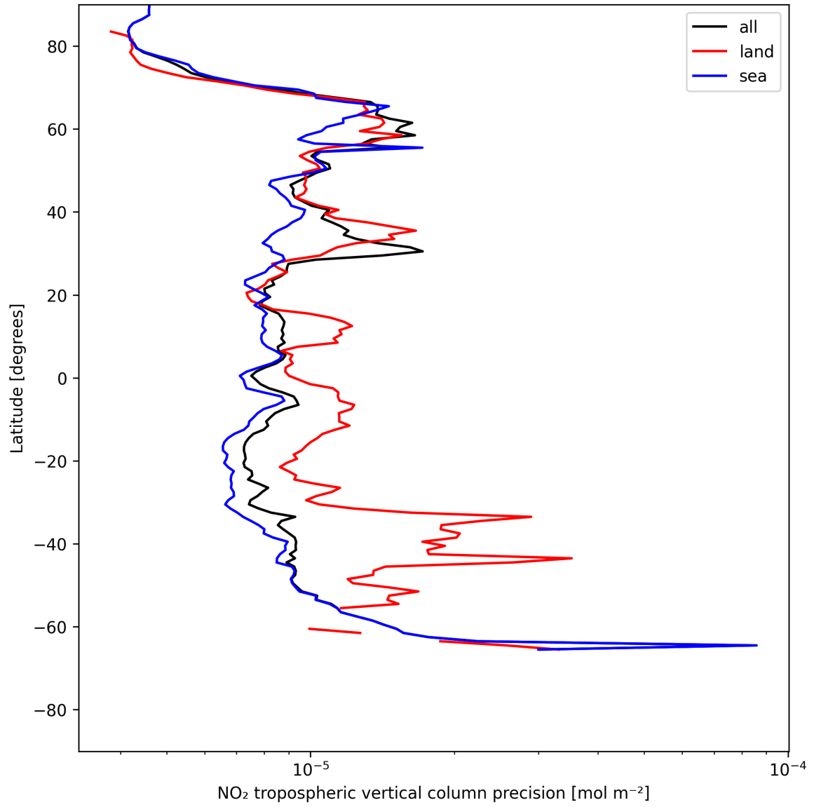
Figure 13: Zonal average of "NO 2 tropospheric vertical column precision" for 2025-06-01 to 2025-06-02.
