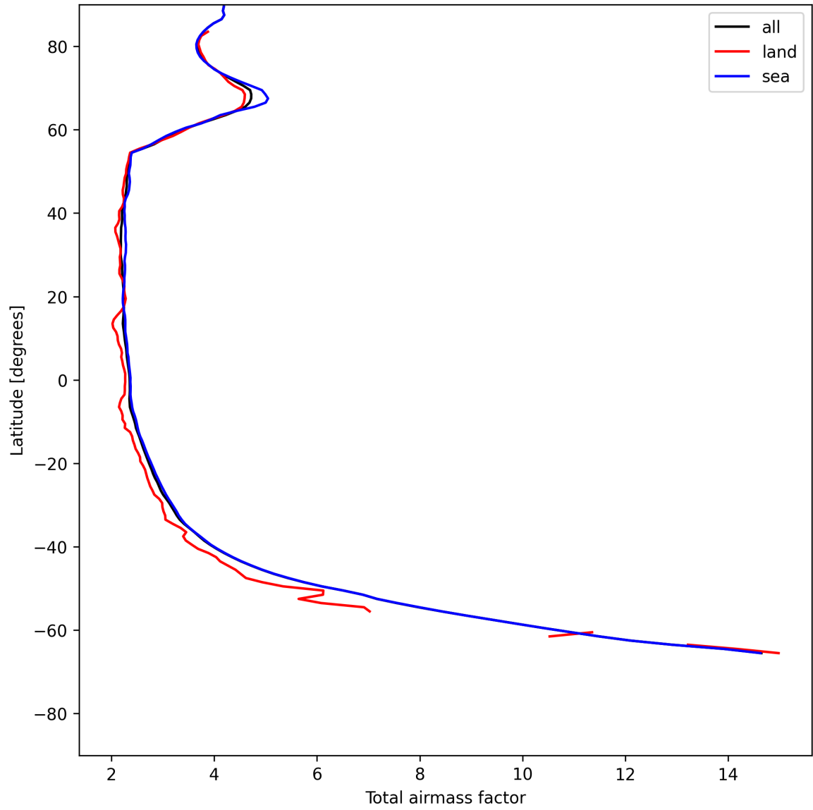
Figure 15: Zonal average of “Total airmass factor” for 2025-06-01 to 2025-06-02.
