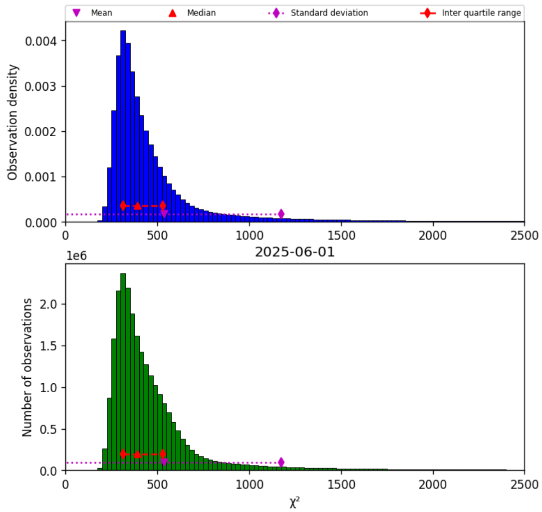
Figure 42: Histogram of " \chi^2 " for 2025-06-01 to 2025-06-02
