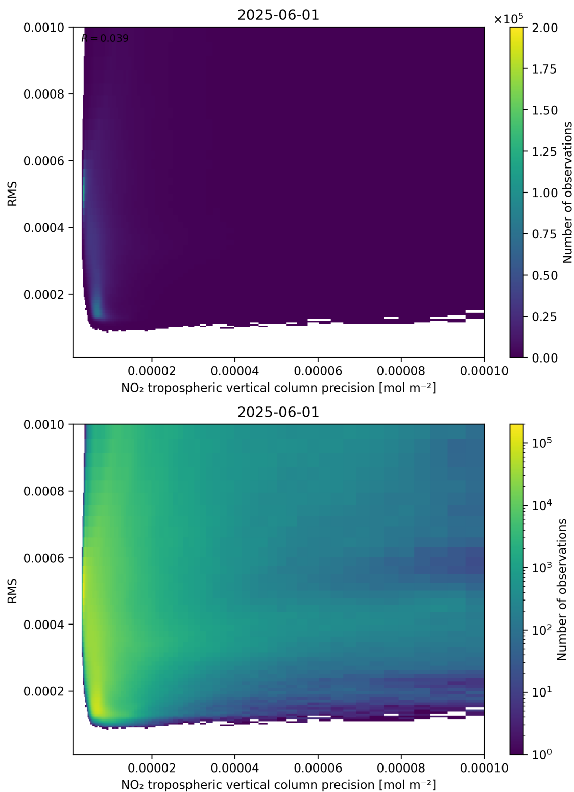
Figure 140: Scatter density plot of “NO 2 tropospheric vertical column precision” against “RMS” for 2025-06-01 to 2025-06-02.
