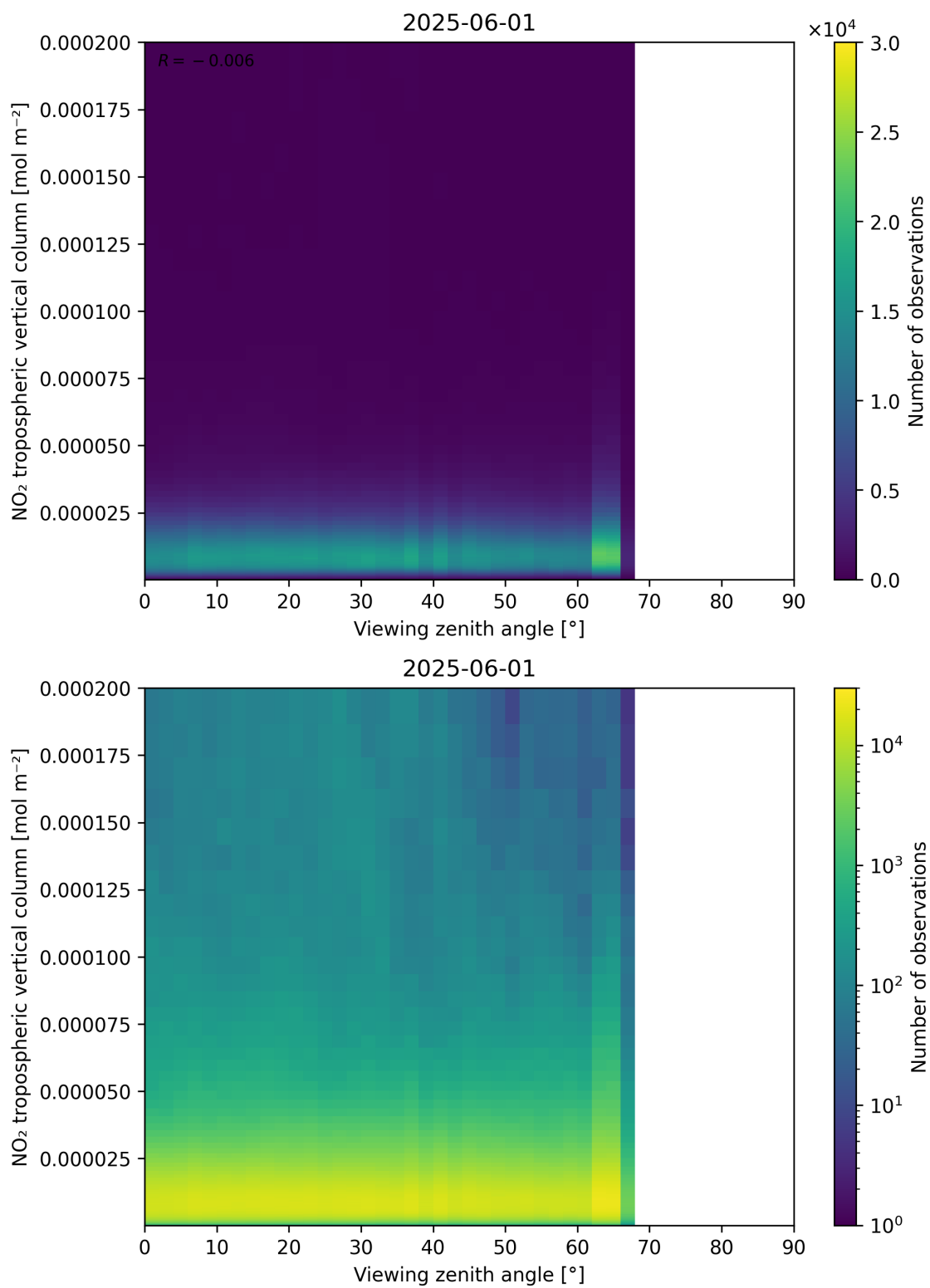
Figure 169: Scatter density plot of “Viewing zenith angle” against “NO 2 tropospheric vertical column” for 2025-06-01 to 2025-06-02.
