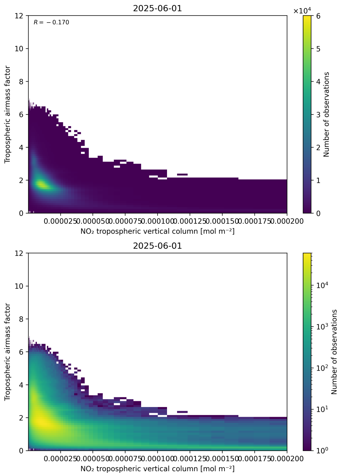
Figure 123: Scatter density plot of “NO 2 tropospheric vertical column” against “Tropospheric airmass factor” for 2025-06-01 to 2025-06-02.
