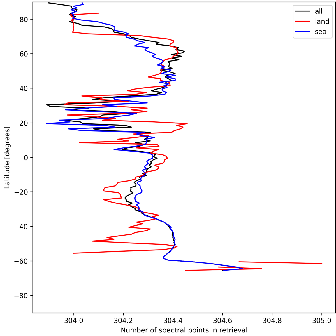
Figure 16: Zonal average of “Number of spectral points in retrieval” for 2025-06-01 to 2025-06-02.
