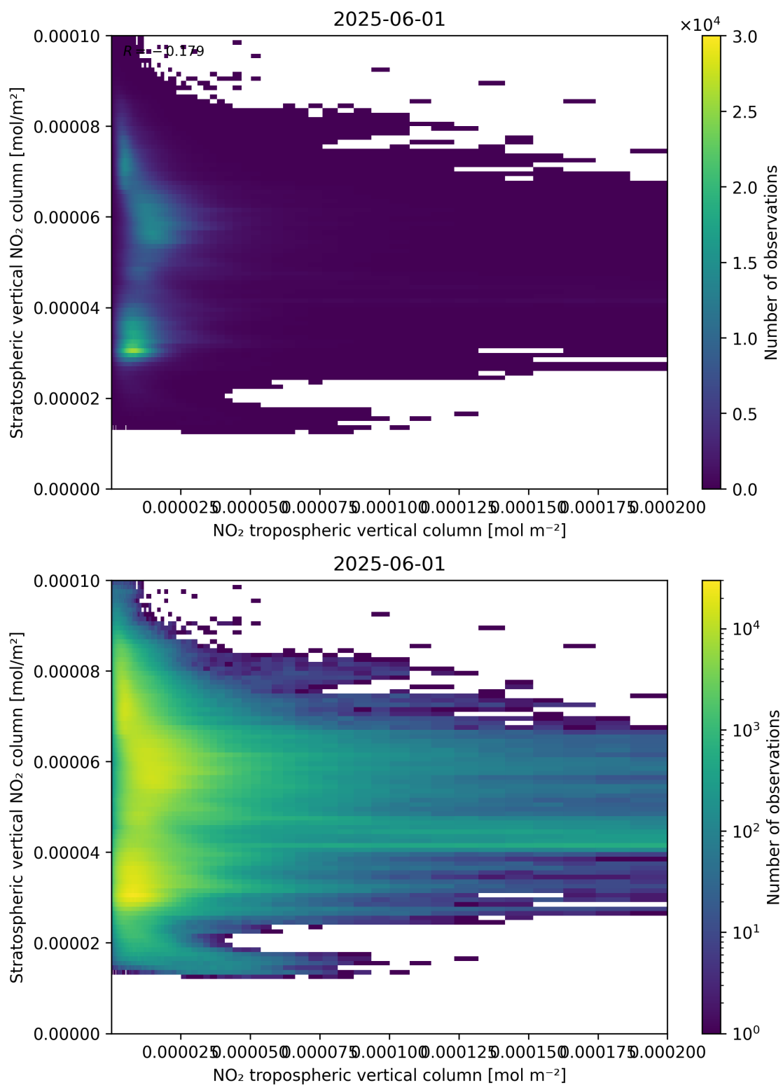
Figure 125: Scatter density plot of “NO 2 tropospheric vertical column” against “Stratospheric vertical NO 2 column” for 2025-06-01 to 2025-06-02.
