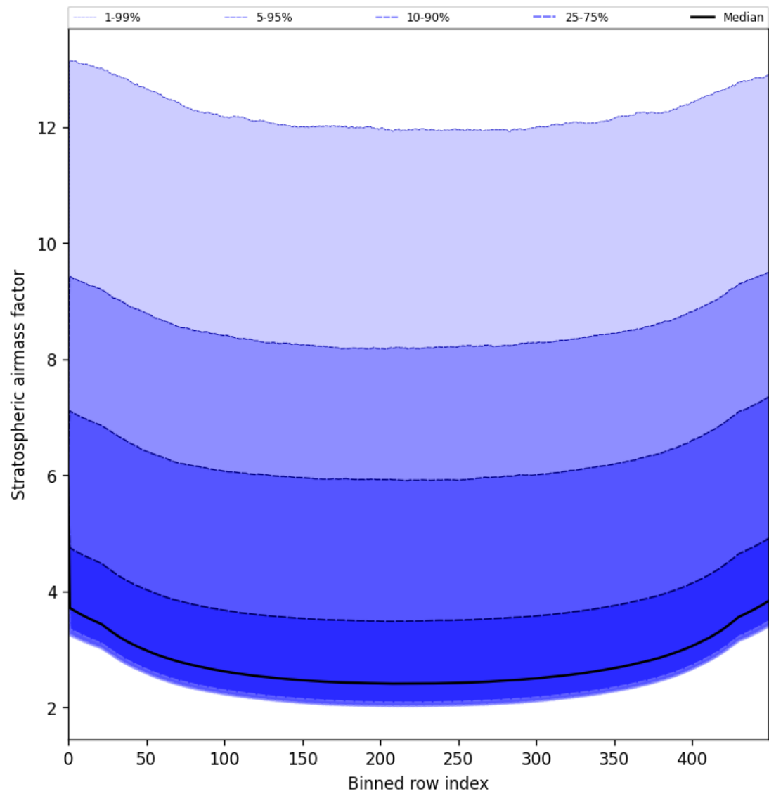
Figure 61: Along track statistics of “Stratospheric airmass factor” for 2025-06-01 to 2025-06-02
