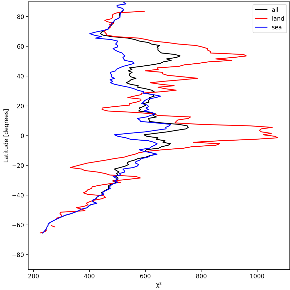
Figure 25: Zonal average of “ \chi^2 ” for 2025-06-01 to 2025-06-02.
