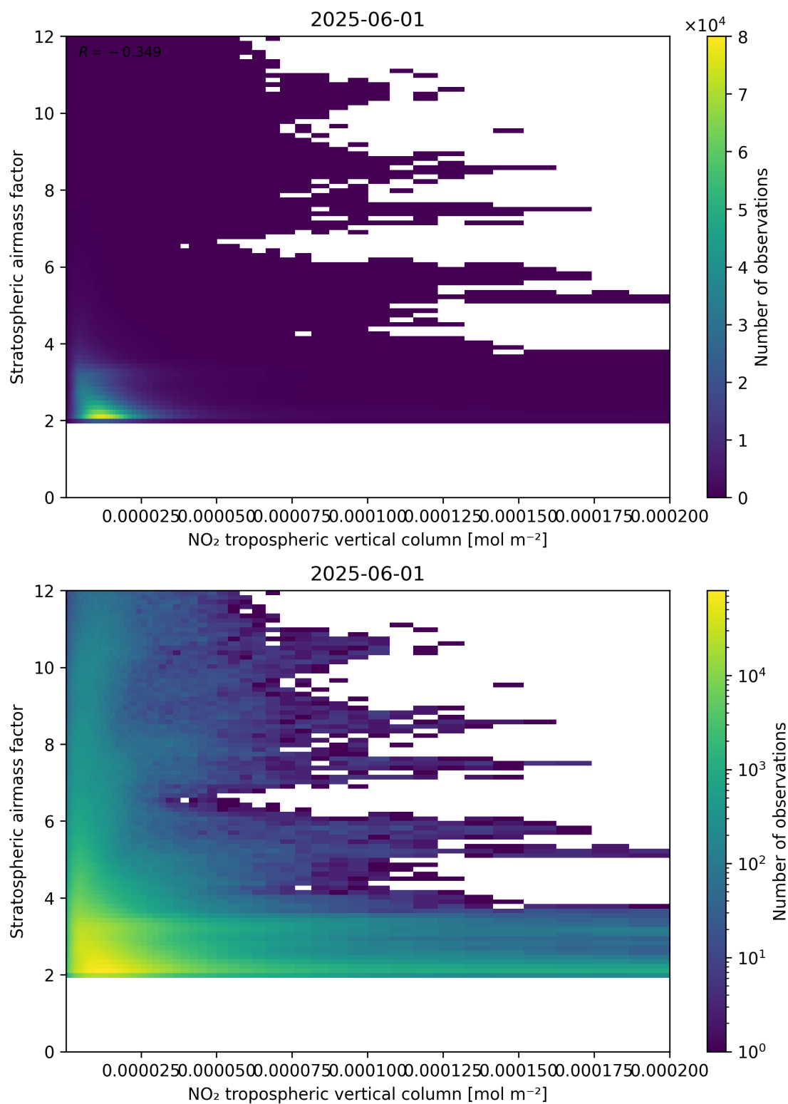
Figure 121: Scatter density plot of “NO 2 tropospheric vertical column” against “Stratospheric air mass factor” for 2025-06-01 to 2025-06-02.
