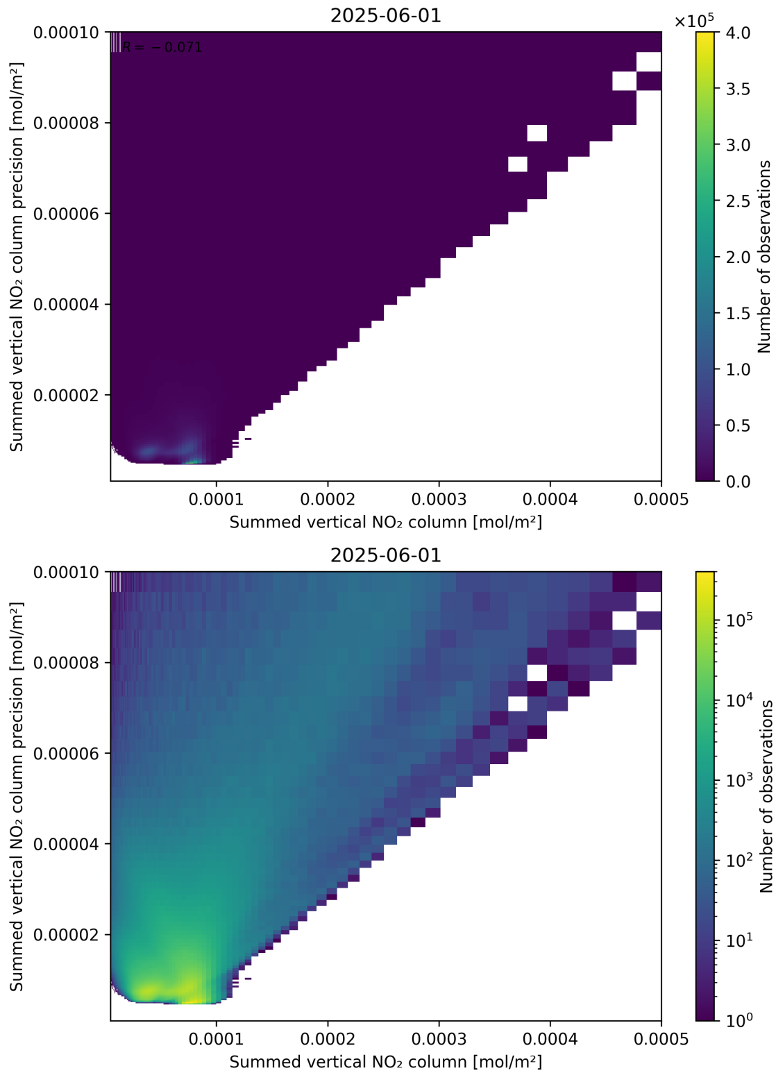
Figure 105: Scatter density plot of “Summed vertical NO 2 column” against “Summed vertical NO 2 column precision” for 2025-06-01 to 2025-06-02.
