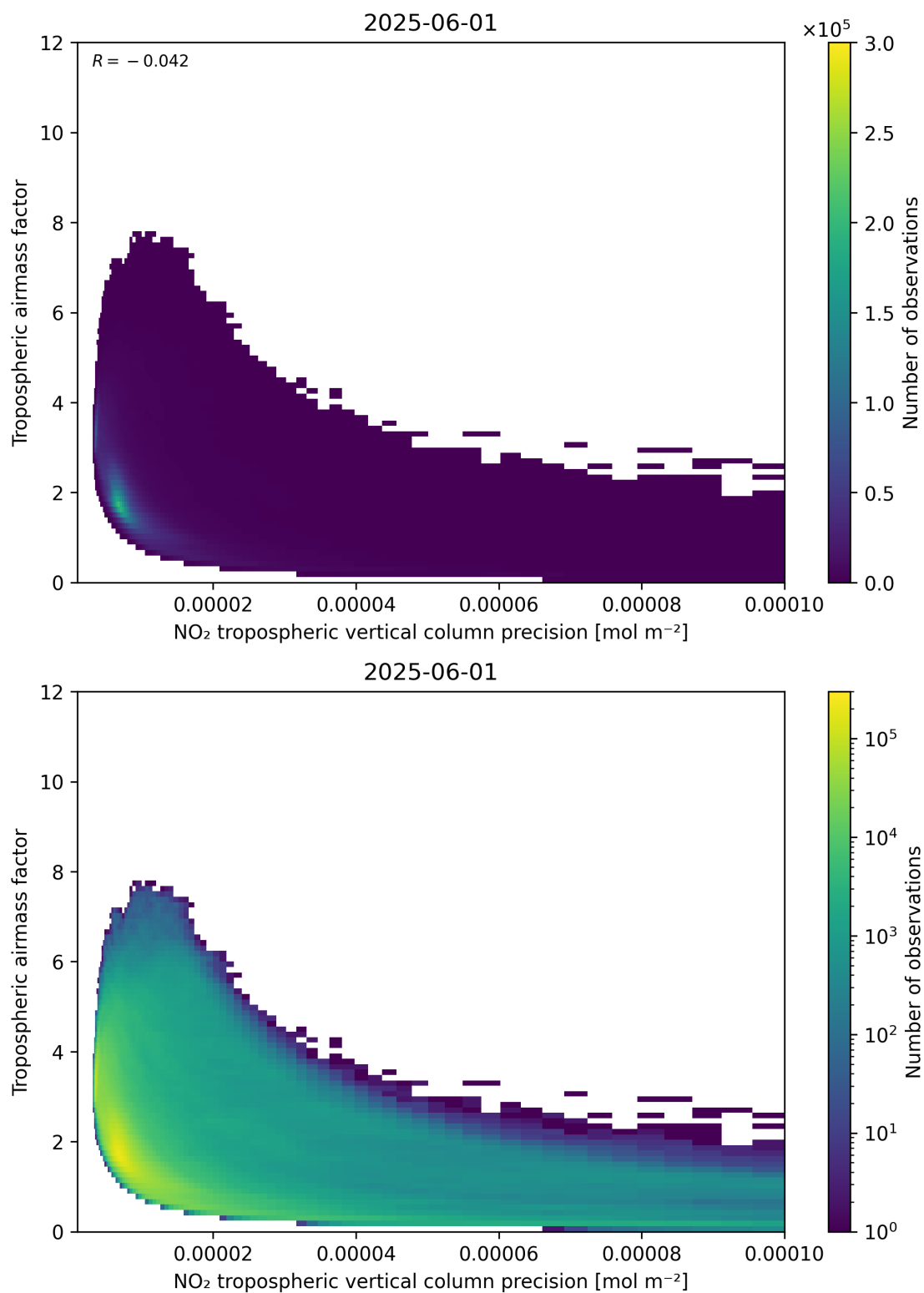
Figure 133: Scatter density plot of “NO 2 tropospheric vertical column precision” against “Tropospheric air mass factor” for 2025-06-01 to 2025-06-02.
