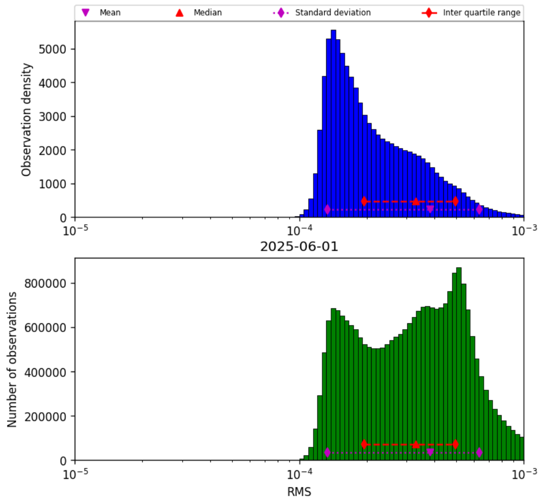
Figure 43: Histogram of “RMS” for 2025-06-01 to 2025-06-02
