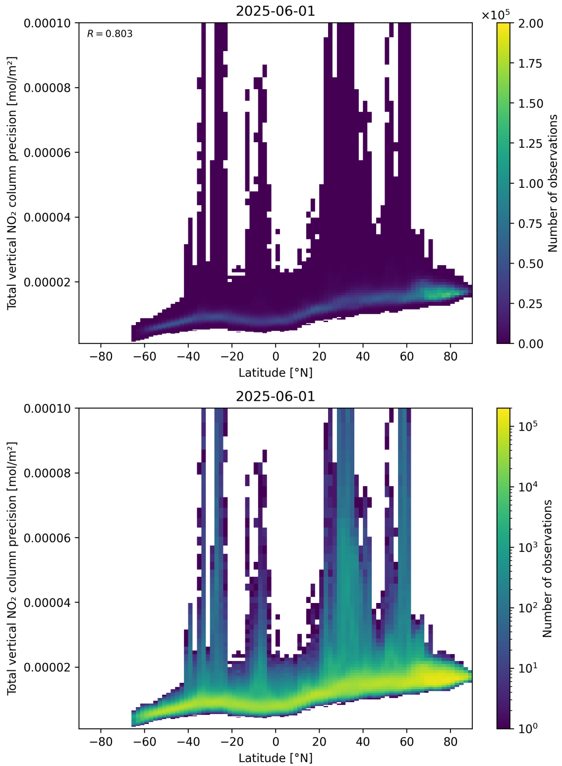
Figure 91: Scatter density plot of “Latitude” against “Total vertical NO 2 column precision” for 2025-06-01 to 2025-06-02.
