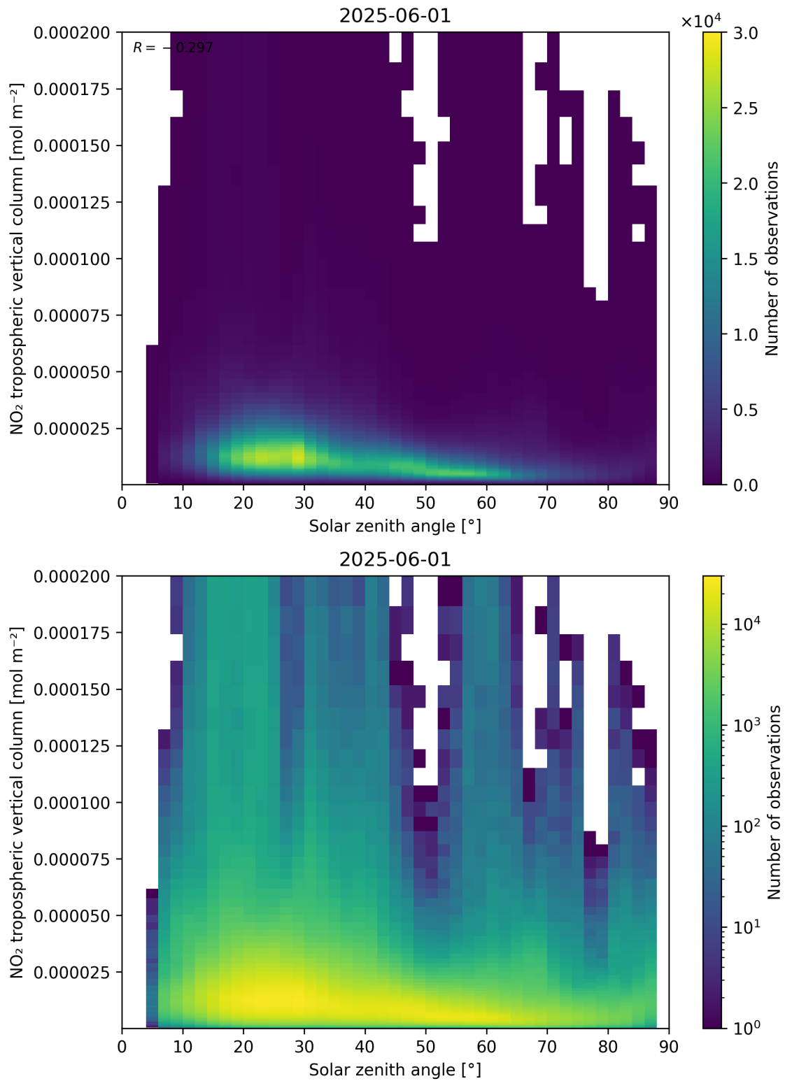
Figure 155: Scatter density plot of “Solar zenith angle” against “NO 2 tropospheric vertical column” for 2025-06-01 to 2025-06-02.
