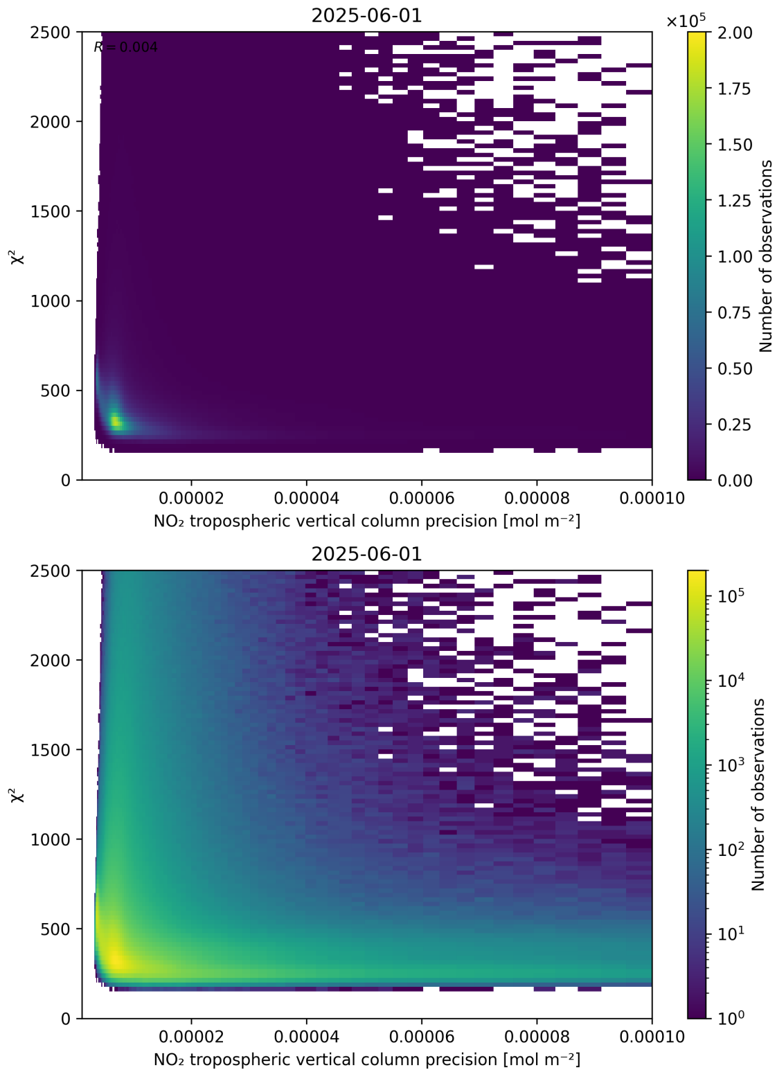
Figure 134: Scatter density plot of “NO 2 tropospheric vertical column precision” against “ \chi^2 ” for 2025-06-01 to 2025-06-02.
