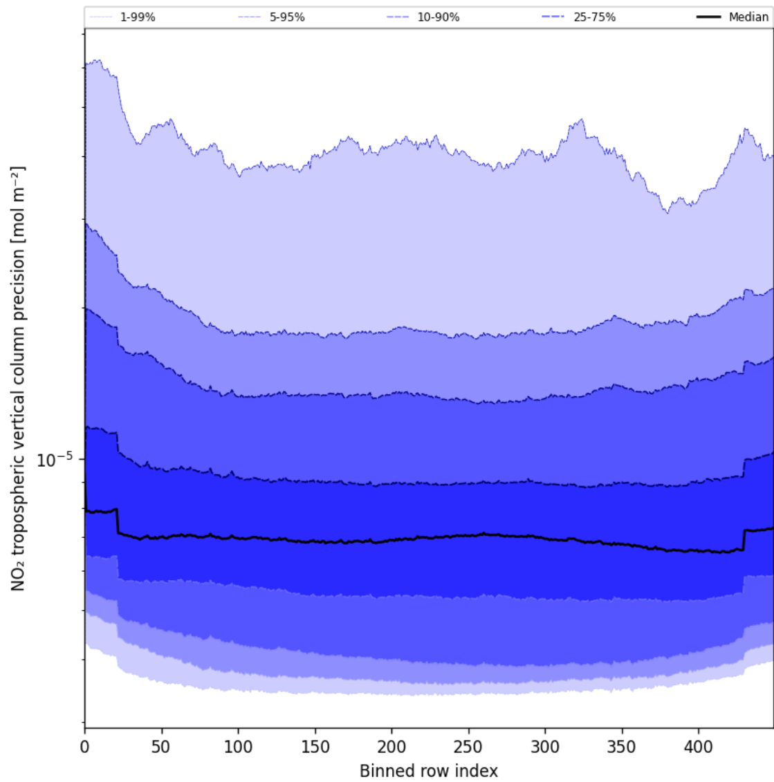
Figure 47: Along track statistics of “NO 2 tropospheric vertical column precision” for 2025-06-01 to 2025-06-02
