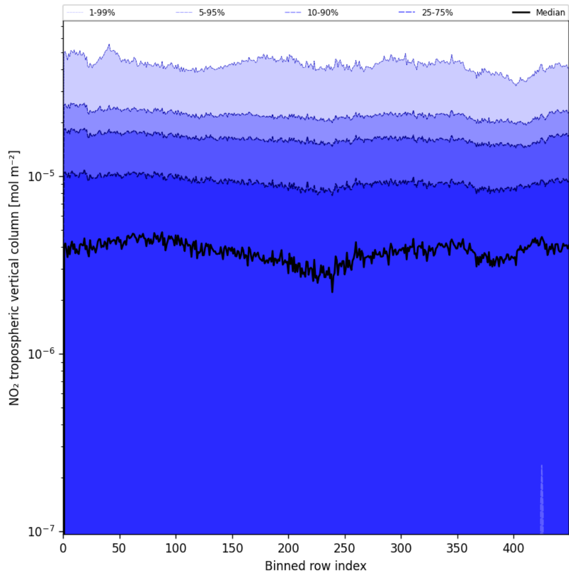
Figure 46: Along track statistics of “NO 2 tropospheric vertical column” for 2025-06-01 to 2025-06-02
