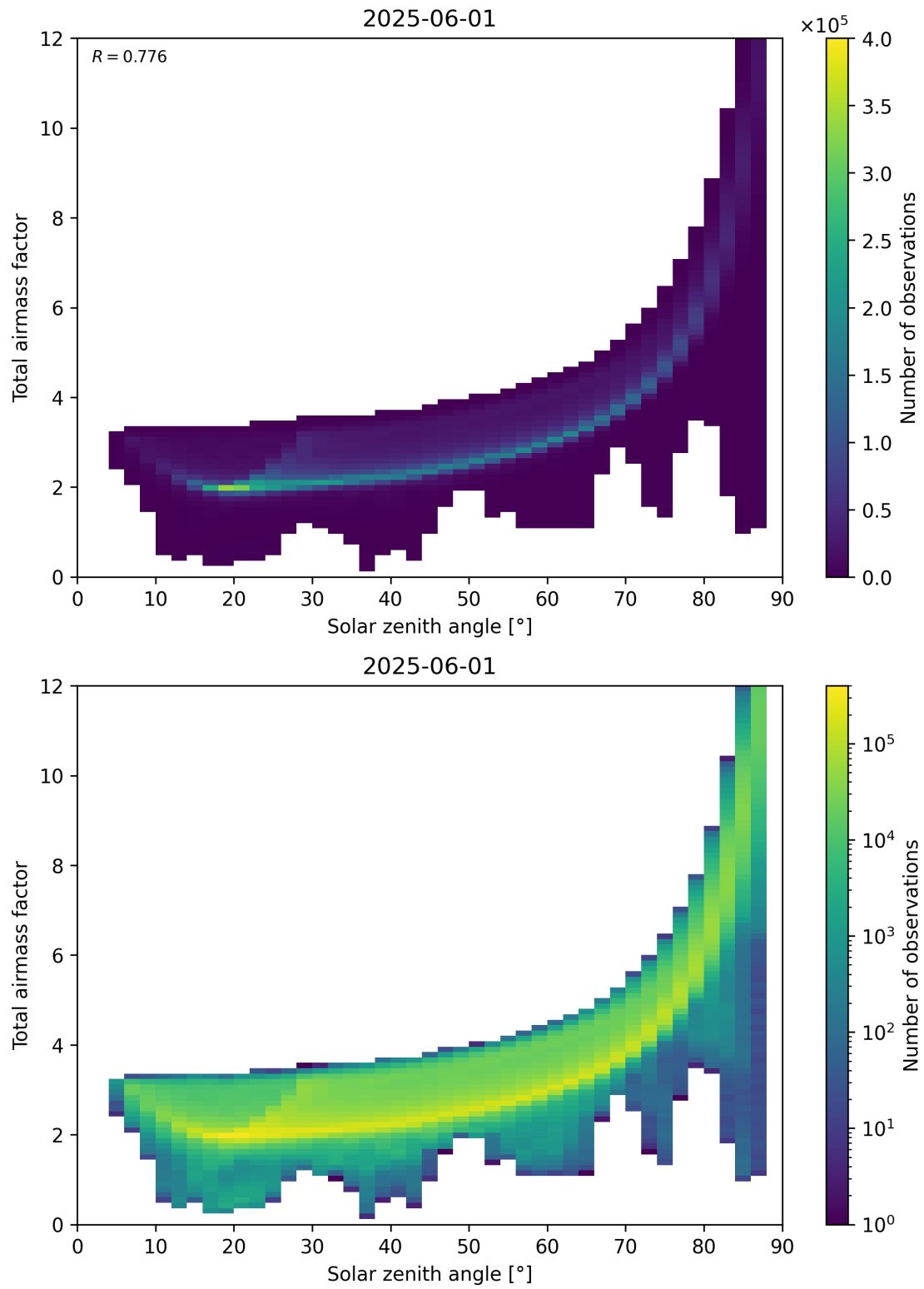
Figure 146: Scatter density plot of “Solar zenith angle” against “Total air mass factor” for 2025-06-01 to 2025-06-02.
