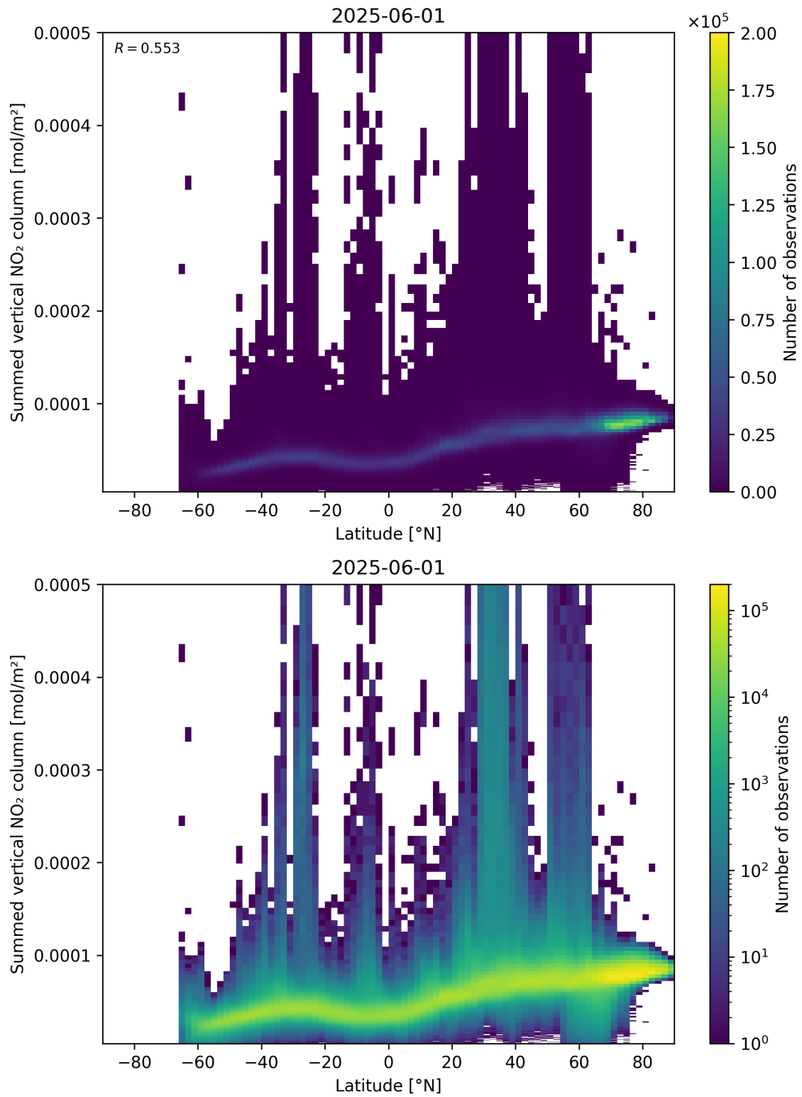
Figure 88: Scatter density plot of “Latitude” against “Summed vertical NO 2 column” for 2025-06-01 to 2025-06-02.
