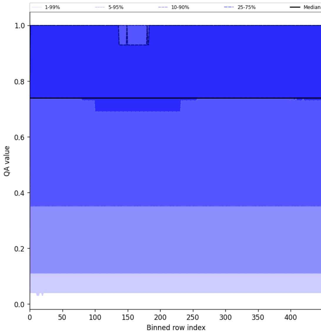
Figure 45: Along track statistics of “QA value” for 2025-06-01 to 2025-06-02
