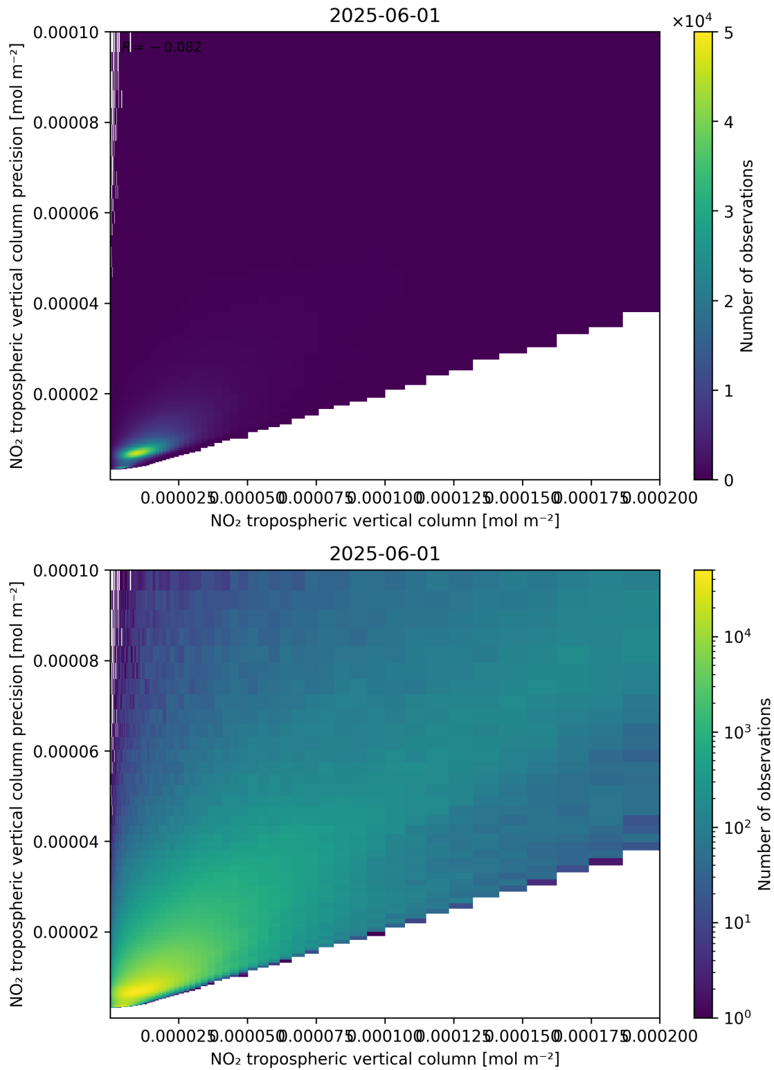
Figure 130: Scatter density plot of “NO 2 tropospheric vertical column” against “NO 2 tropospheric vertical column precision” for 2025-06-01 to 2025-06-02.
