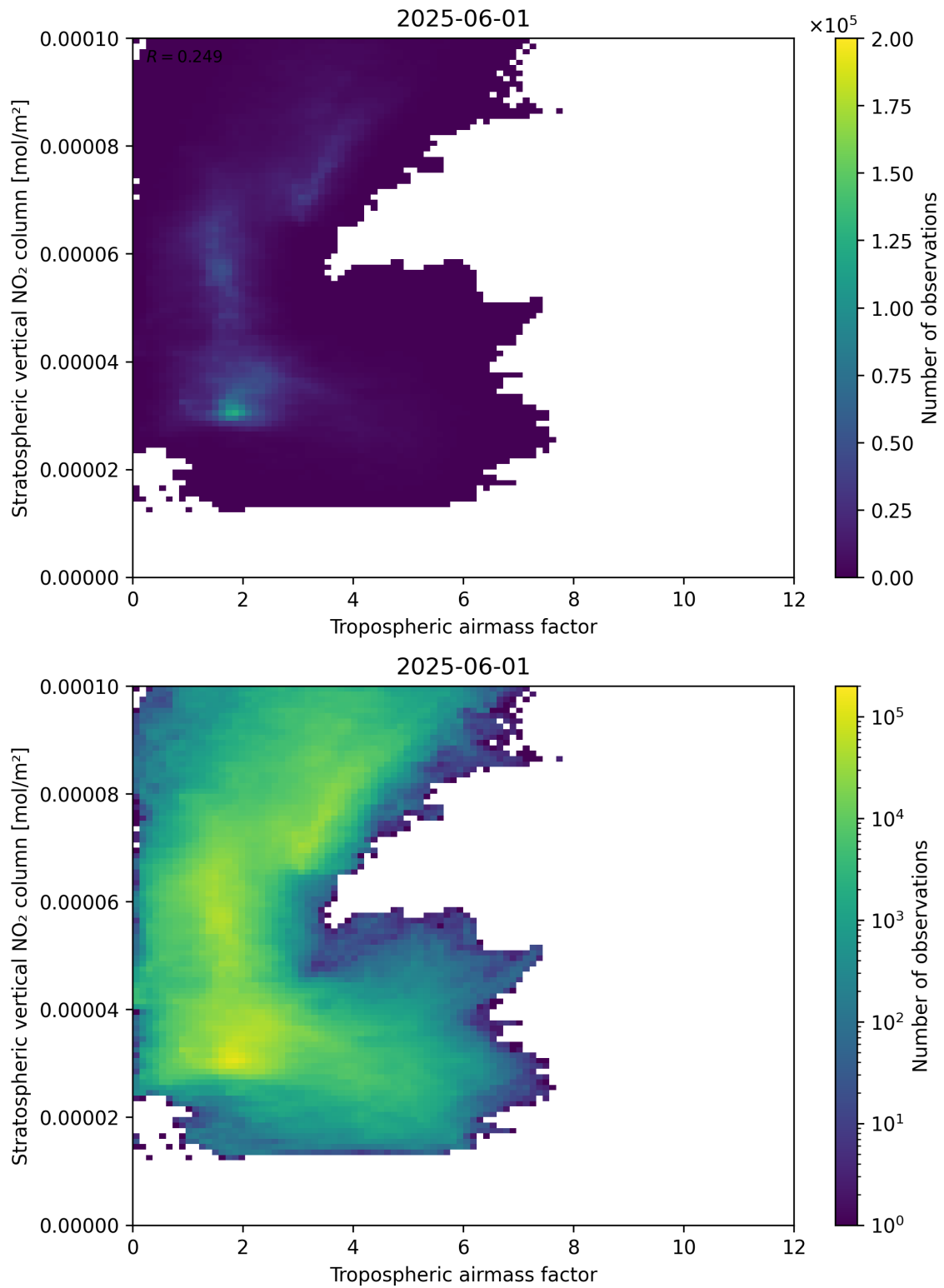
Figure 74: Scatter density plot of “Tropospheric air mass factor” against “Stratospheric vertical NO 2 column” for 2025-06-01 to 2025-06-02.
