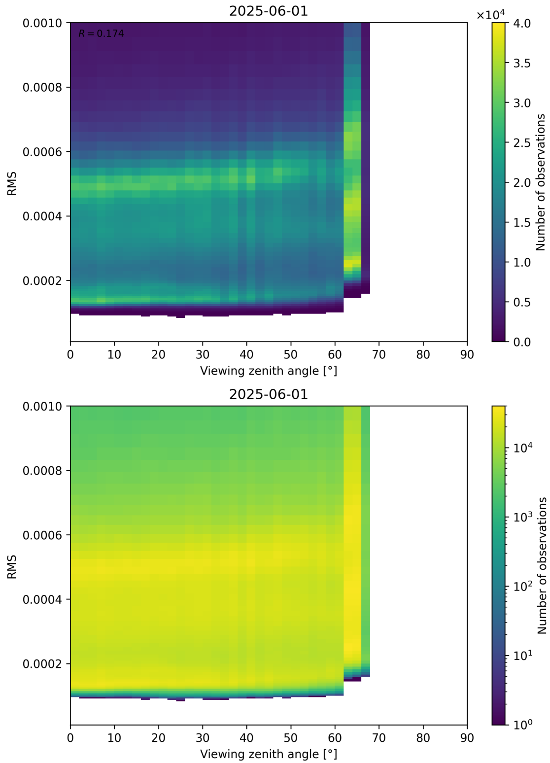
Figure 171: Scatter density plot of “Viewing zenith angle” against “RMS” for 2025-06-01 to 2025-06-02.
