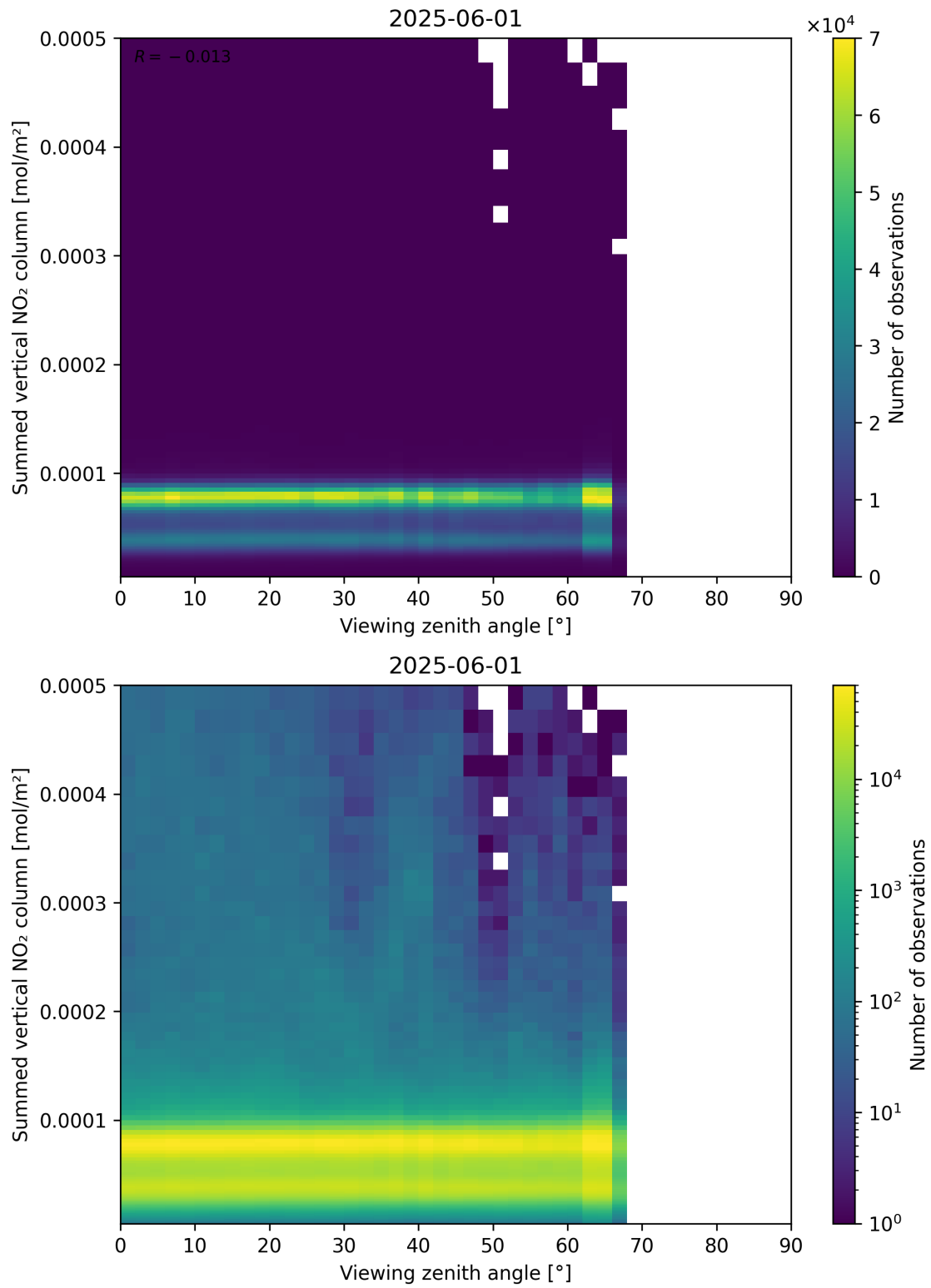
Figure 165: Scatter density plot of “Viewing zenith angle” against “Summed vertical NO 2 column” for 2025-06-01 to 2025-06-02.
