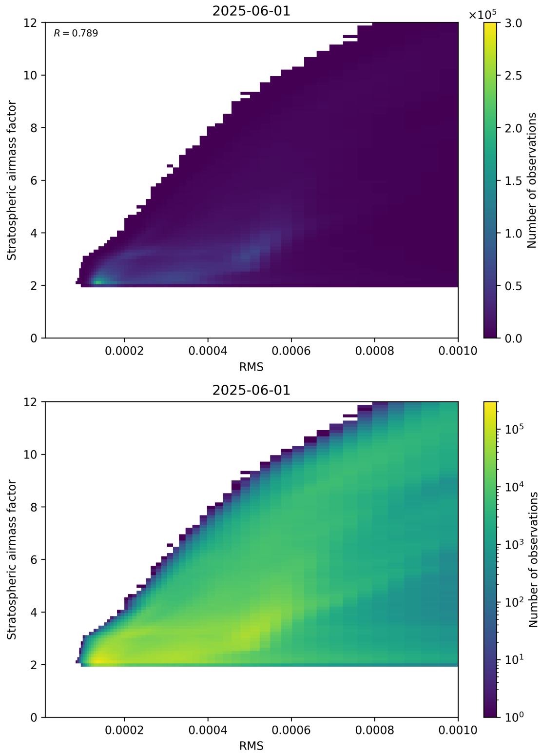
Figure 144: Scatter density plot of “RMS” against “Stratospheric airmass factor” for 2025-06-01 to 2025-06-02.
