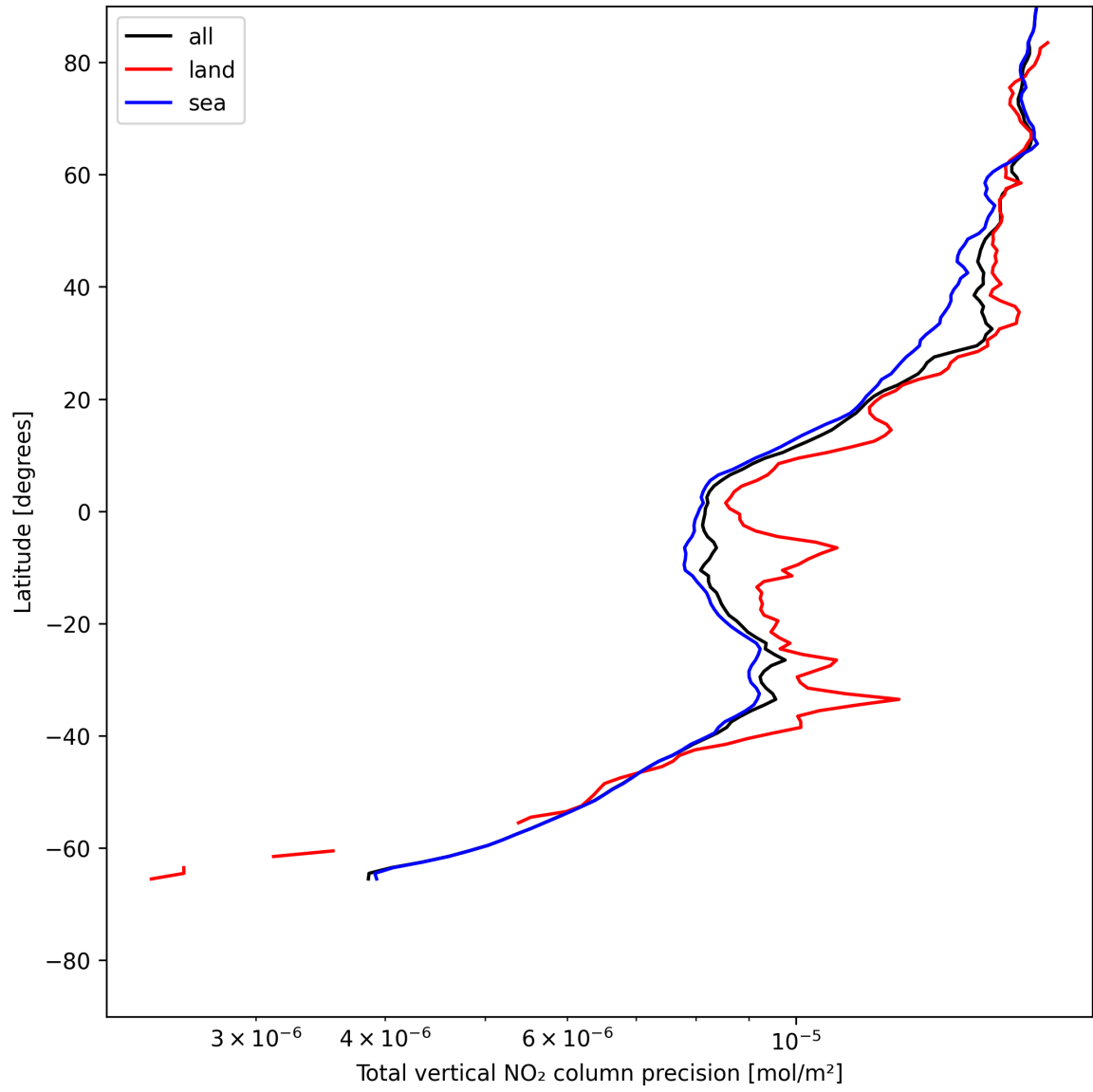
Figure 22: Zonal average of “Total vertical NO 2 column precision” for 2025-06-01 to 2025-06-02.
