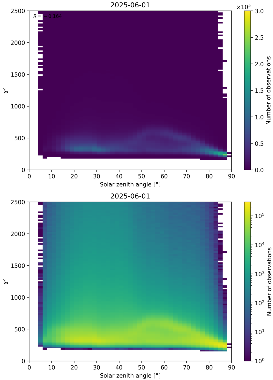
Figure 148: Scatter density plot of “Solar zenith angle” against “ \chi^2 ” for 2025-06-01 to 2025-06-02.
