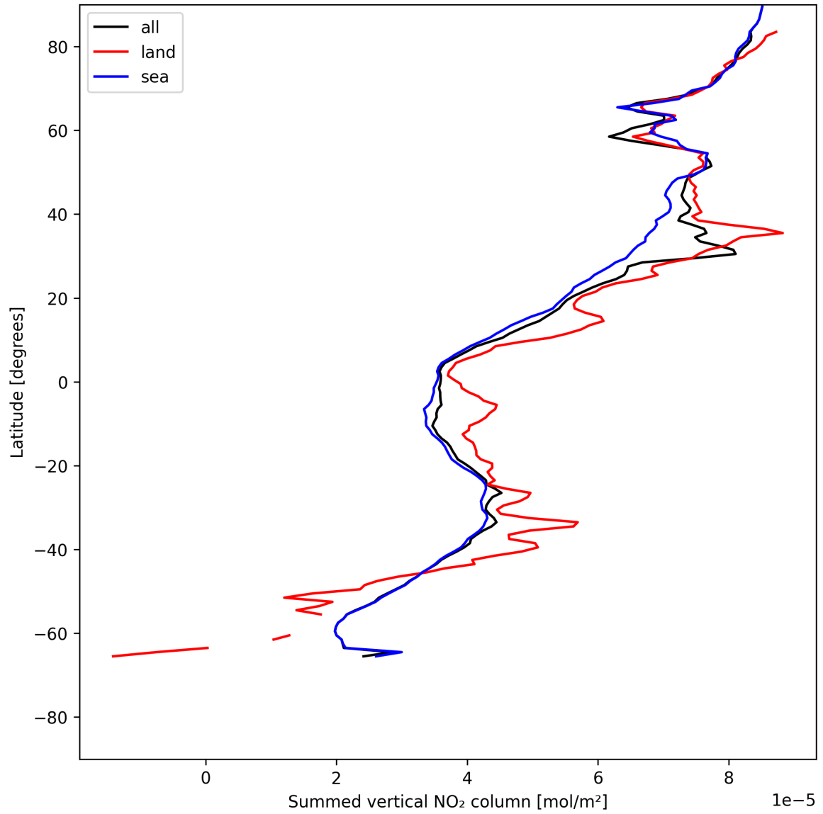
Figure 23: Zonal average of “Summed vertical NO 2 column” for 2025-06-01 to 2025-06-02.
