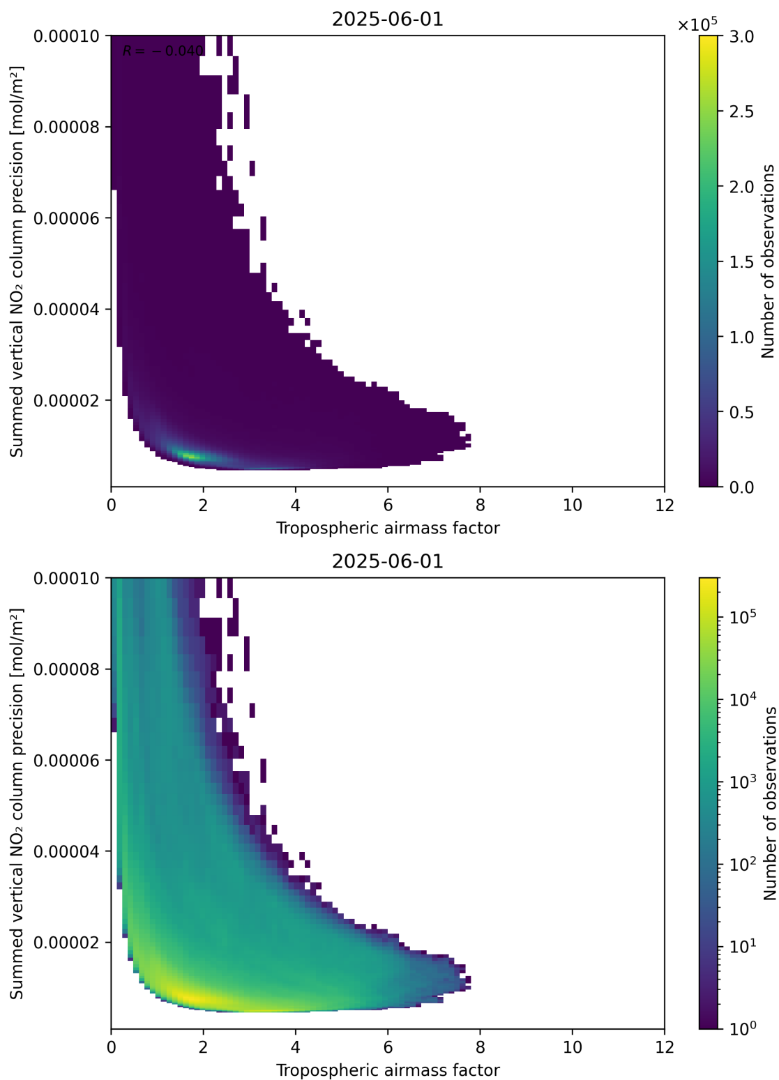
Figure 76: Scatter density plot of “Tropospheric air mass factor” against “Summed vertical NO 2 column precision” for 2025-06-01 to 2025-06-02.
