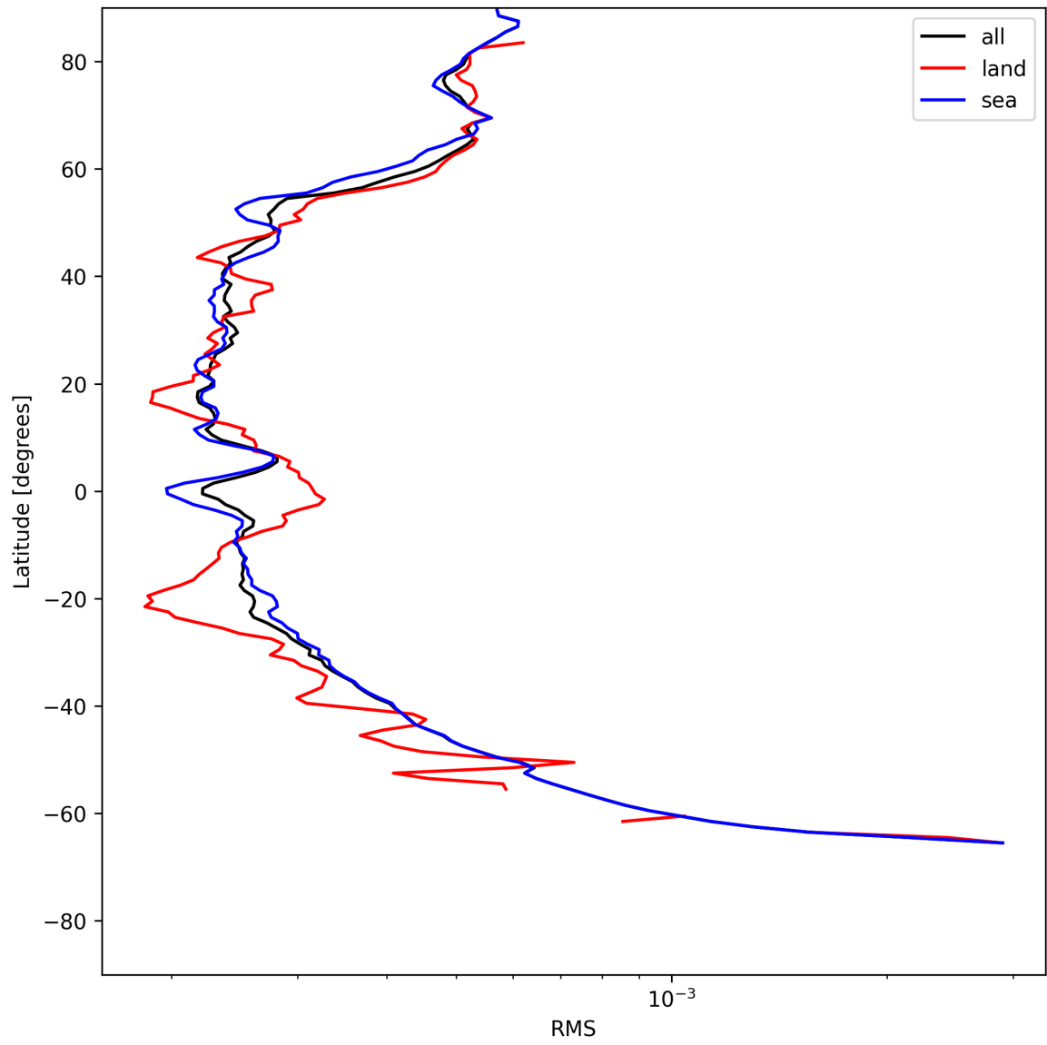
Figure 26: Zonal average of “RMS” for 2025-06-01 to 2025-06-02.
