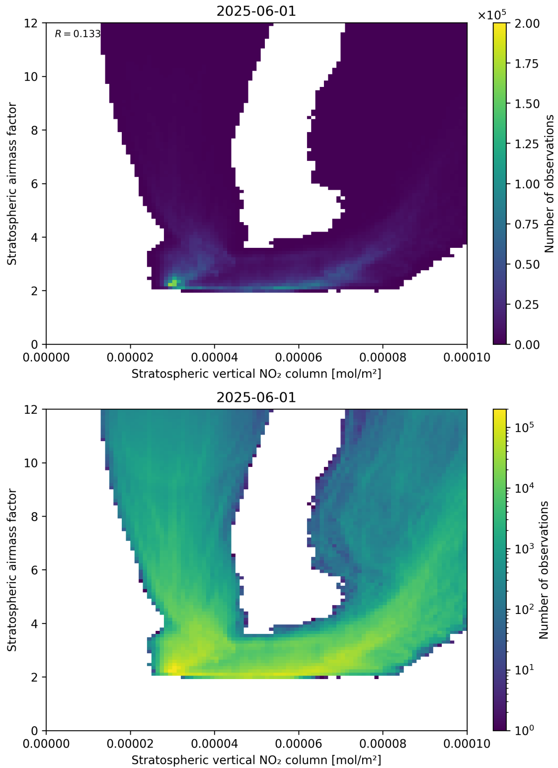
Figure 96: Scatter density plot of “Stratospheric vertical NO 2 column” against “Stratospheric airmass factor” for 2025-06-01 to 2025-06-02.
