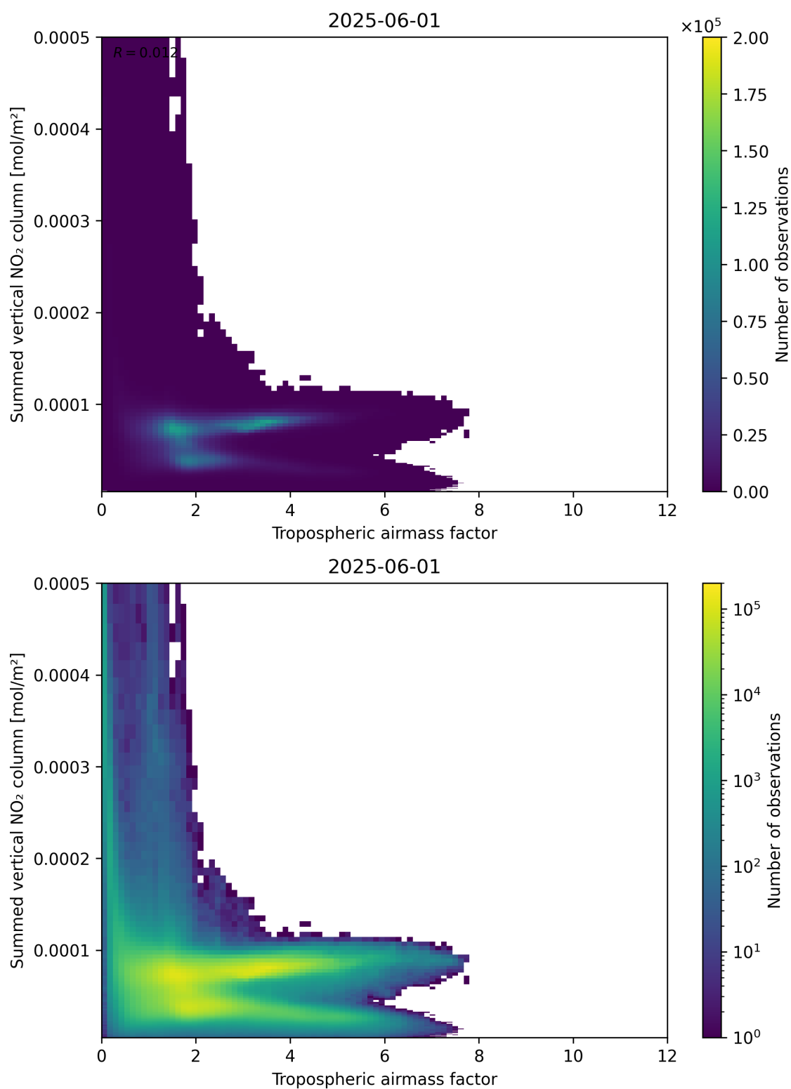
Figure 75: Scatter density plot of “Tropospheric air mass factor” against “Summed vertical NO 2 column” for 2025-06-01 to 2025-06-02.
