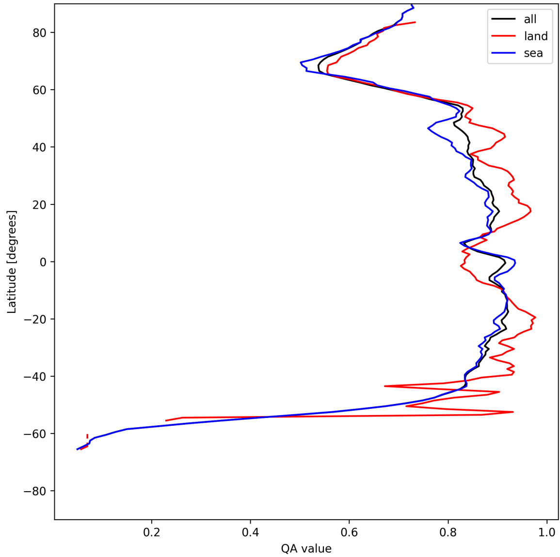
Figure 11: Zonal average of “QA value” for 2025-06-01 to 2025-06-02.
