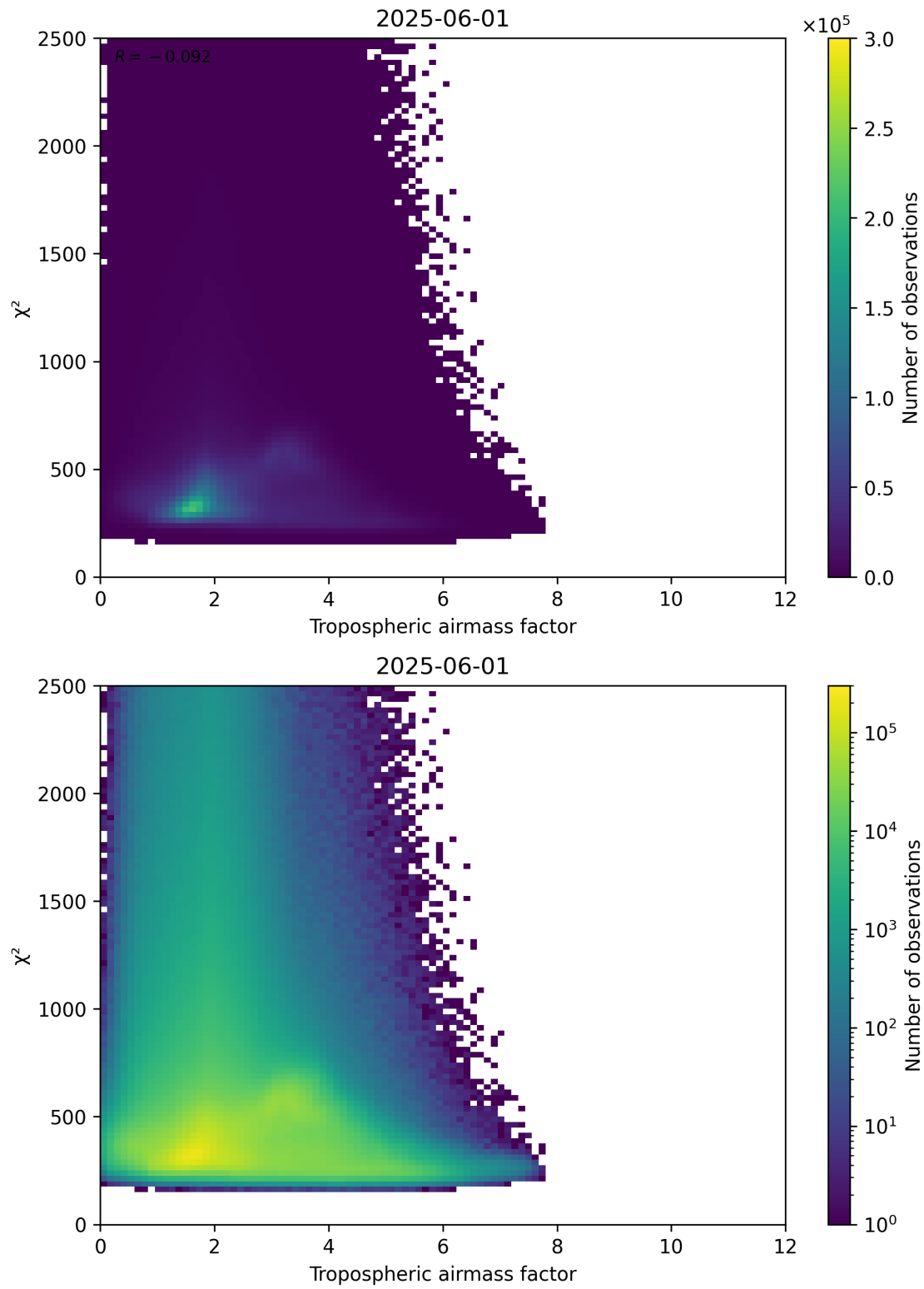
Figure 73: Scatter density plot of “Tropospheric airmass factor” against “ \chi^2 ” for 2025-06-01 to 2025-06-02.
