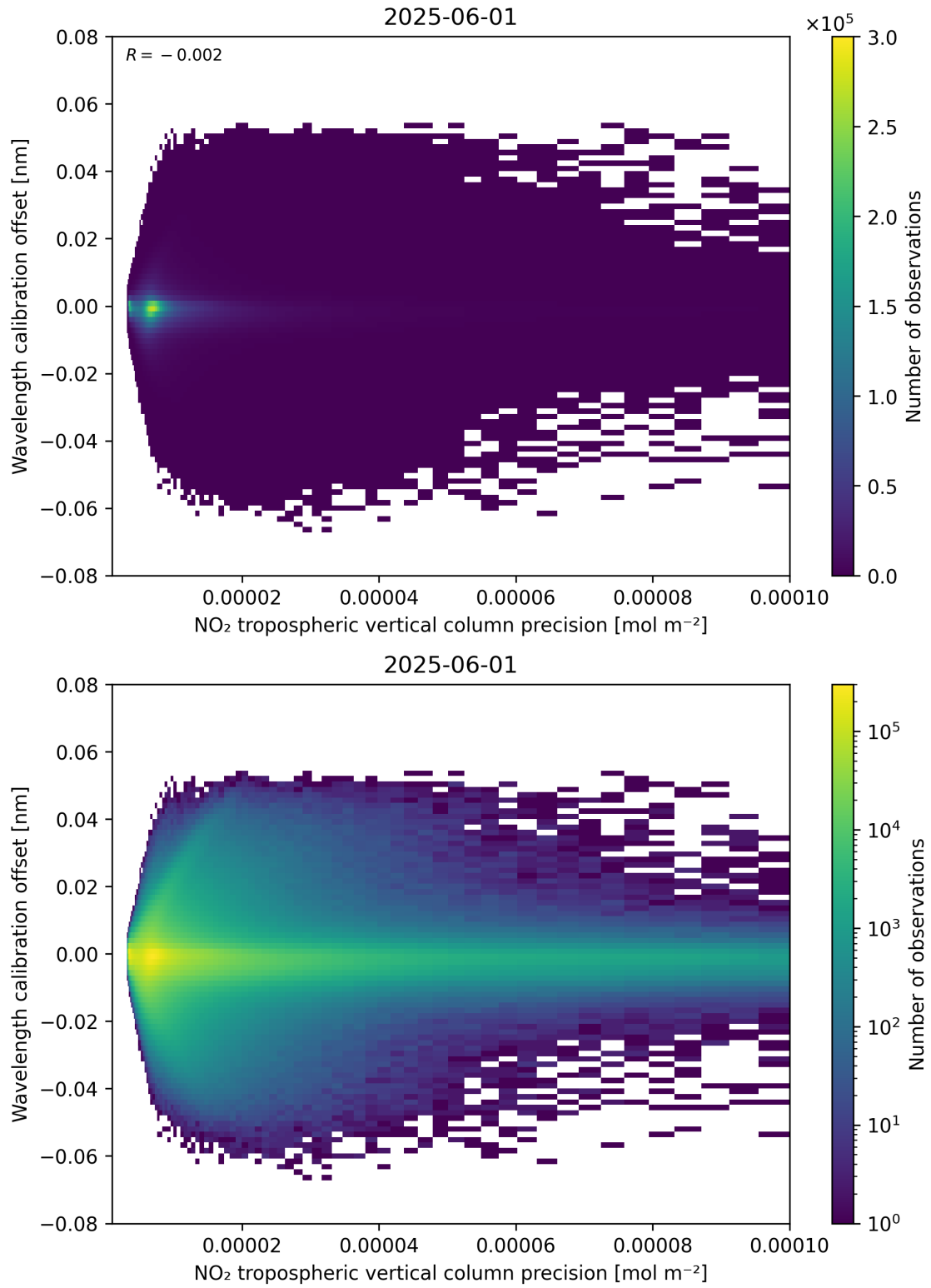
Figure 141: Scatter density plot of “NO 2 tropospheric vertical column precision” against “Wavelength calibration offset” for 2025-06-01 to 2025-06-02.
