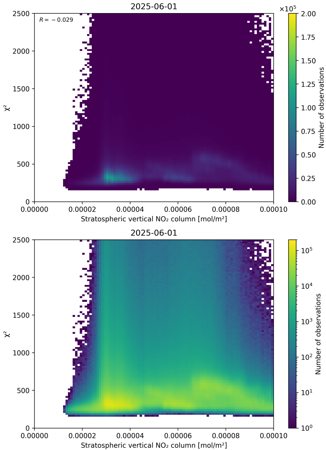
Figure 97: Scatter density plot of “Stratospheric vertical NO 2 column” against “ \chi^2 ” for 2025-06-01 to 2025-06-02.
