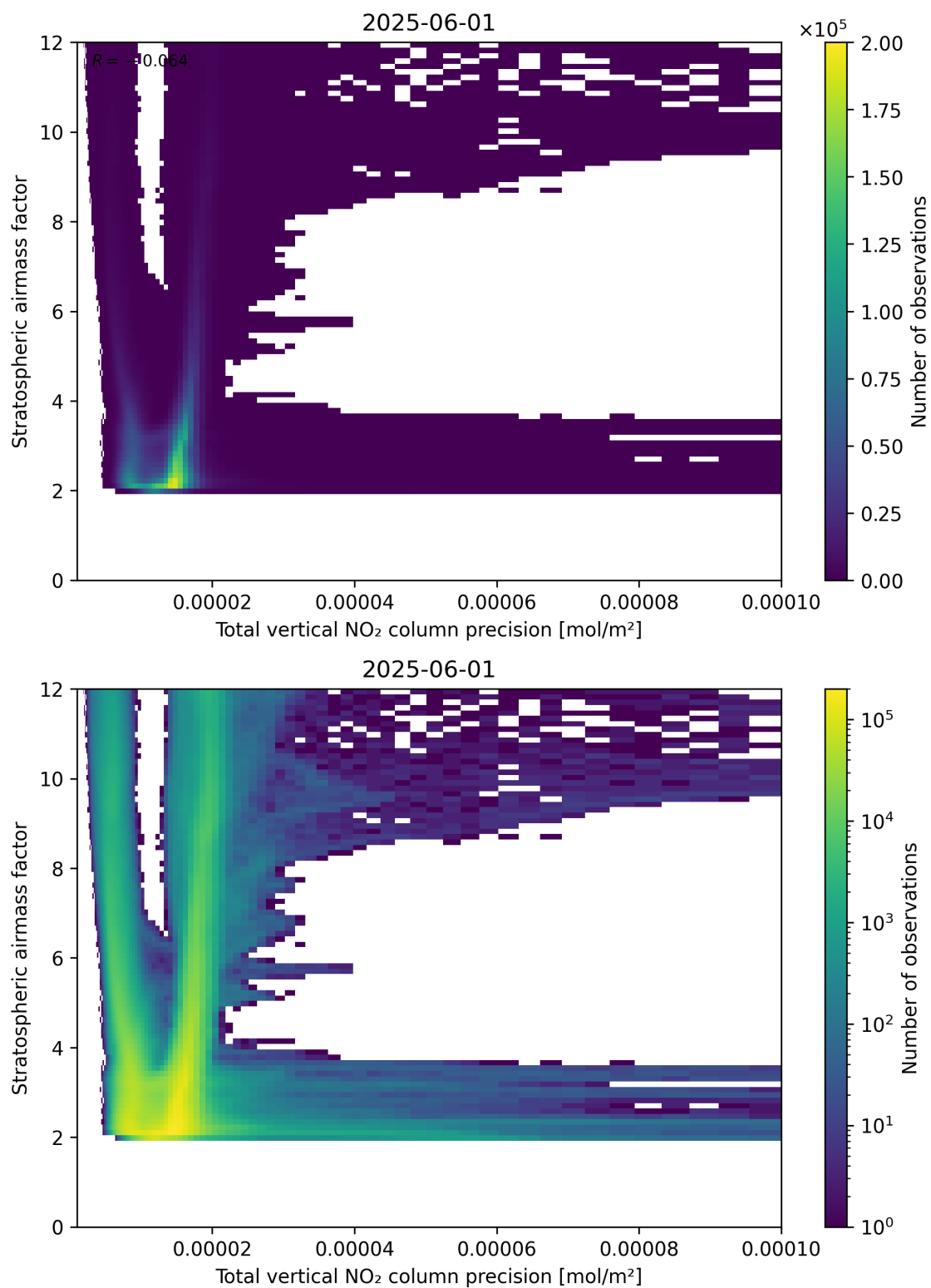
Figure 115: Scatter density plot of “Total vertical NO 2 column precision” against “Stratospheric air mass factor” for 2025-06-01 to 2025-06-02.
