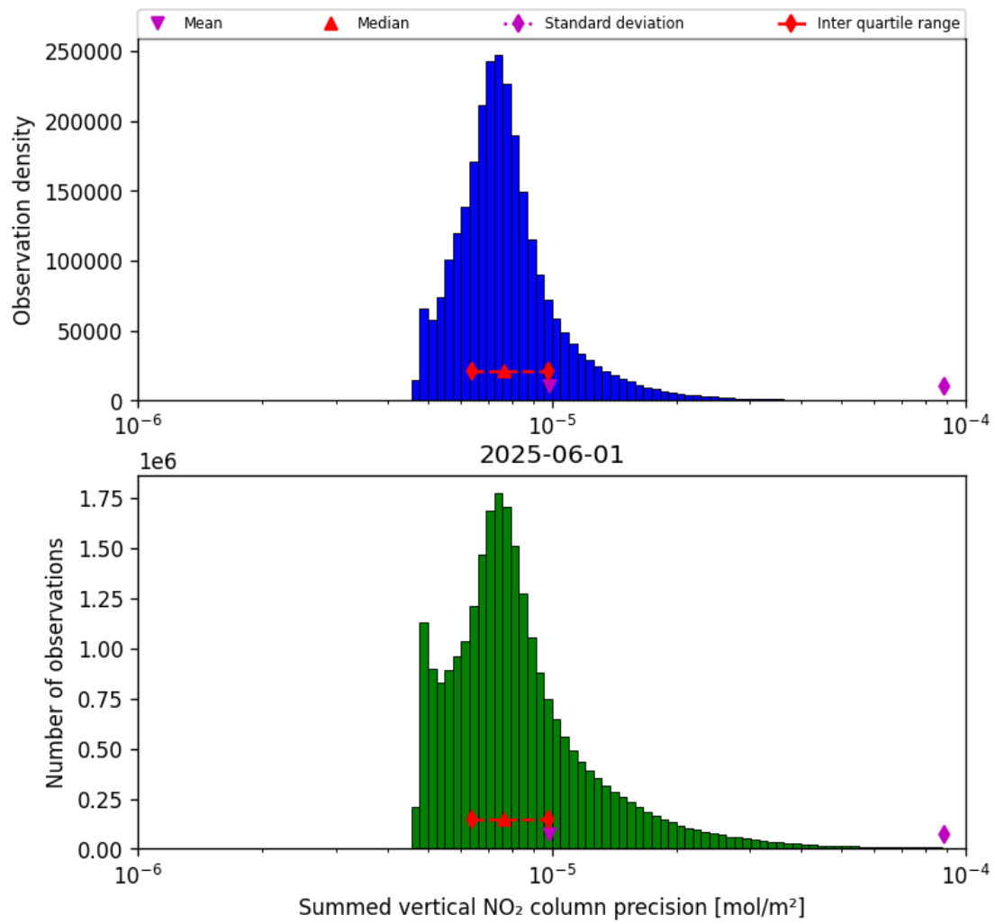
Figure 41: Histogram of "Summed vertical NO 2 column precision" for 2025-06-01 to 2025-06-02
