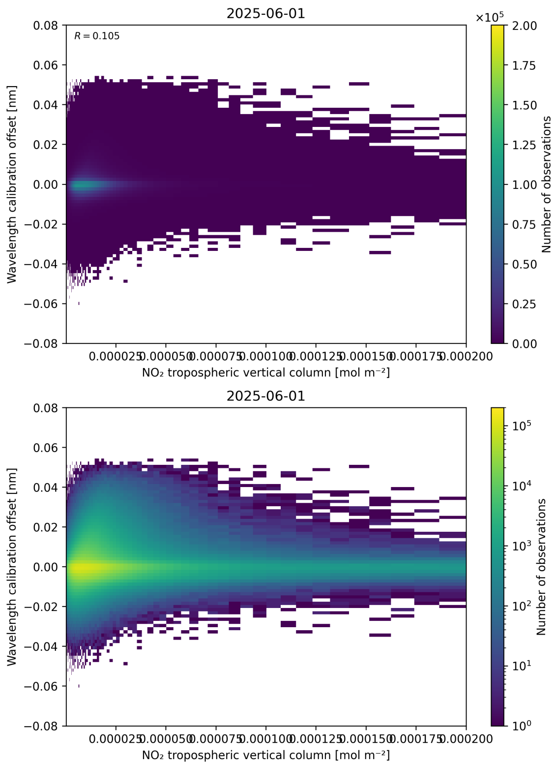
Figure 143: Scatter density plot of “NO 2 tropospheric vertical column” against “Wavelength calibration offset” for 2025-06-01 to 2025-06-02.
