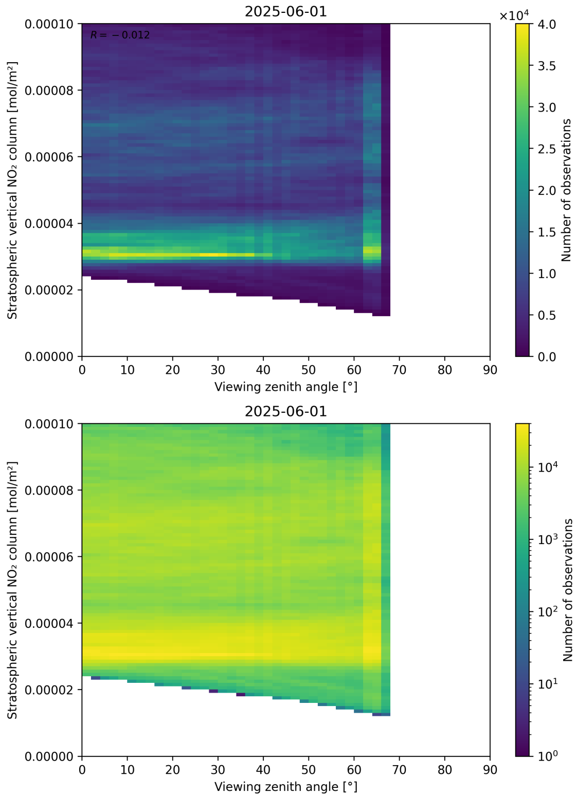
Figure 164: Scatter density plot of “Viewing zenith angle” against “Stratospheric vertical NO 2 column” for 2025-06-01 to 2025-06-02.
