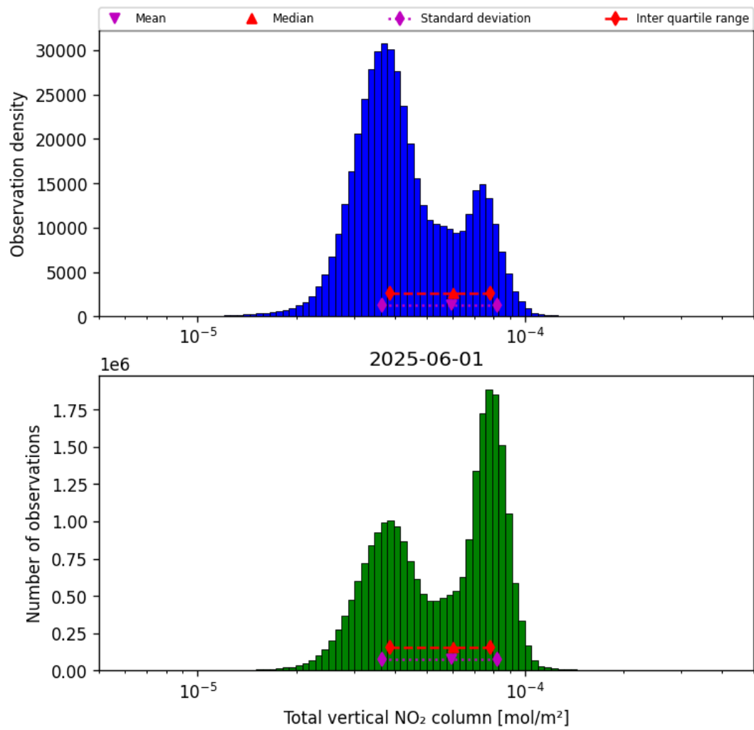
Figure 38: Histogram of “Total vertical NO 2 column” for 2025-06-01 to 2025-06-02
