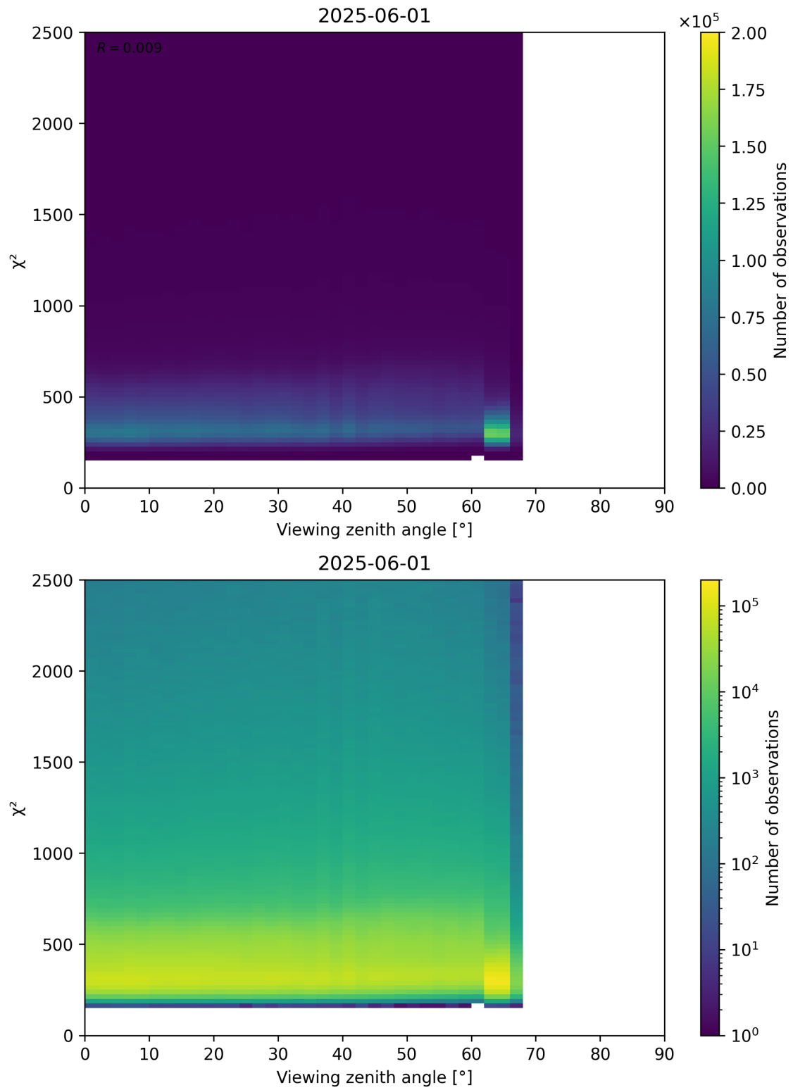
Figure 162: Scatter density plot of “Viewing zenith angle” against “ \chi^2 ” for 2025-06-01 to 2025-06-02.
