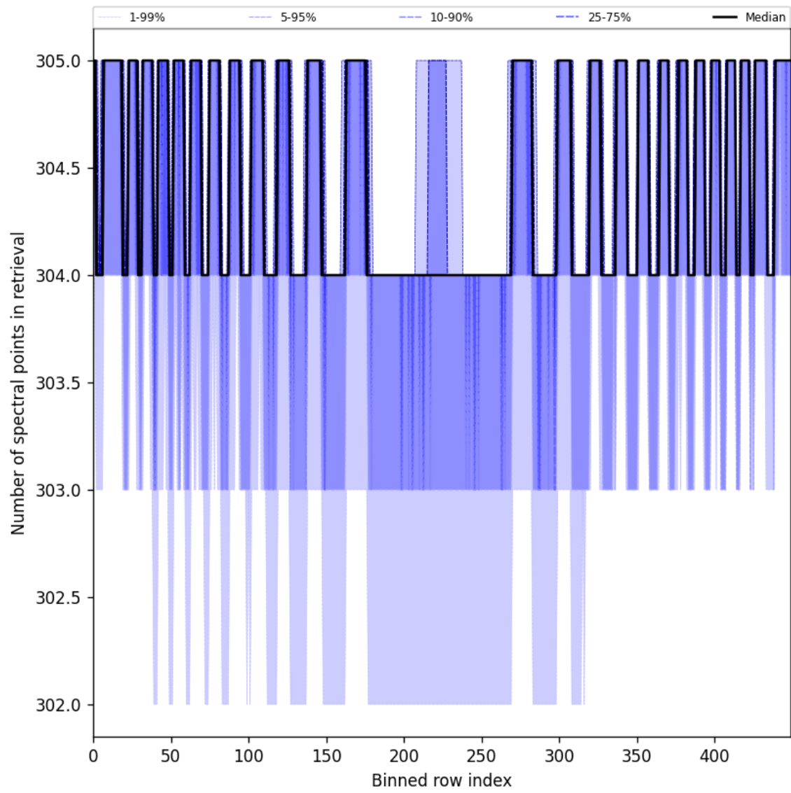
Figure 50: Along track statistics of “Number of spectral points in retrieval” for 2025-06-01 to 2025-06-02
