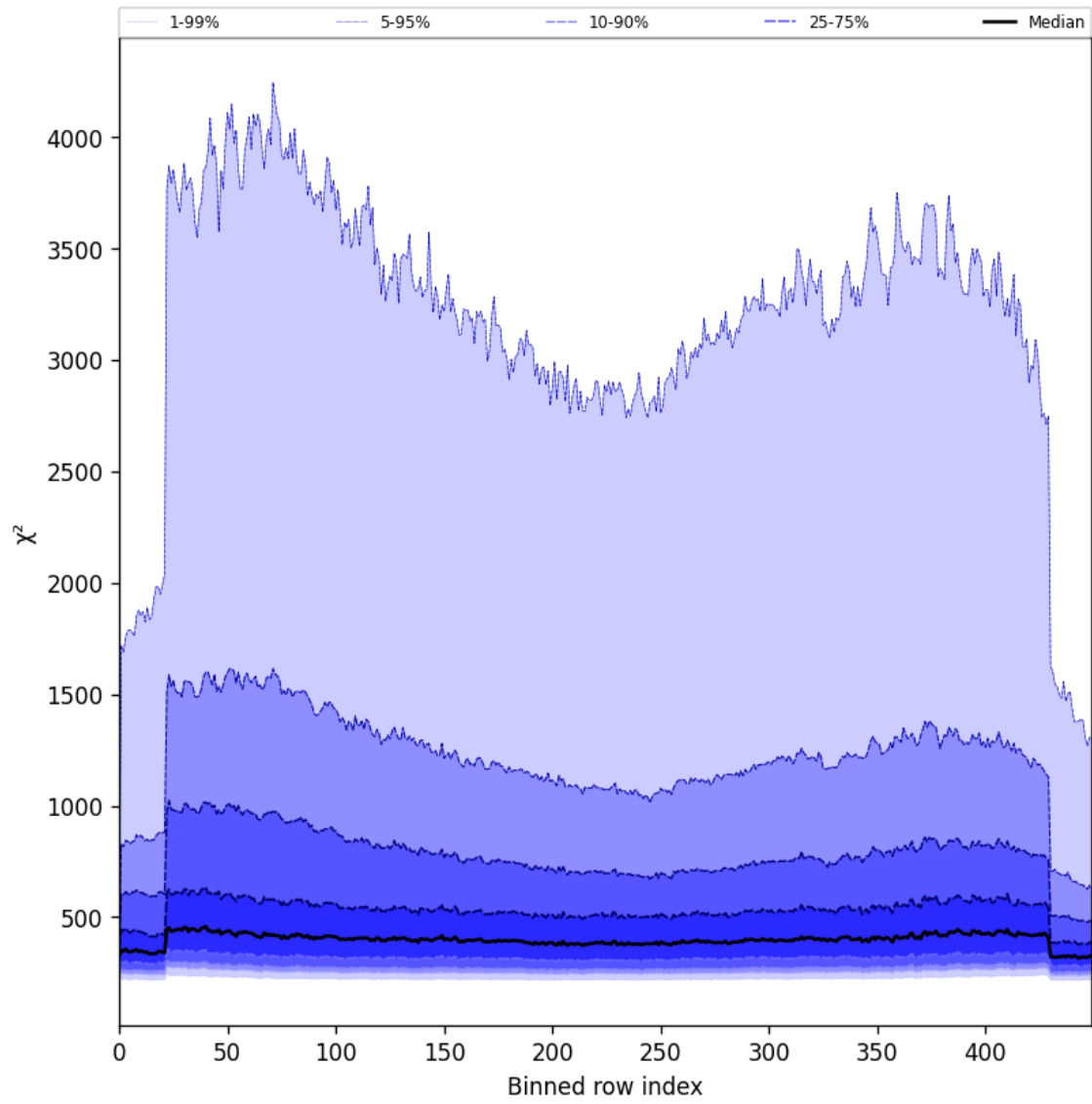
Figure 59: Along track statistics of “ \chi^2 ” for 2025-06-01 to 2025-06-02
