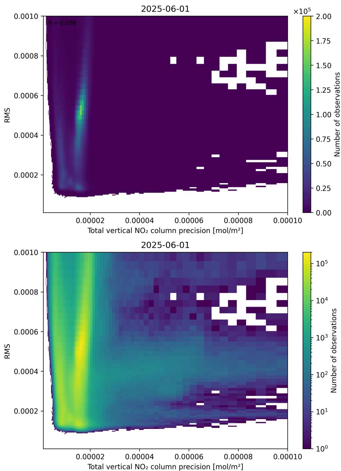
Figure 119: Scatter density plot of “Total vertical NO 2 column precision” against “RMS” for 2025-06-01 to 2025-06-02.
