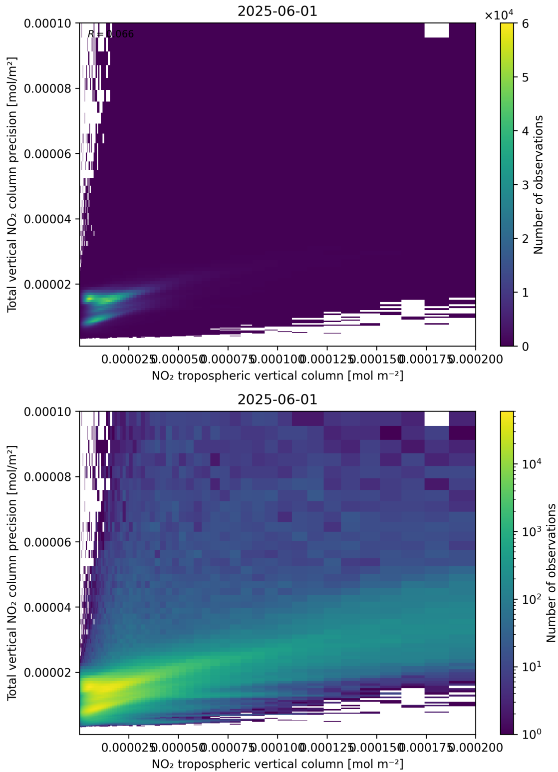
Figure 129: Scatter density plot of “NO 2 tropospheric vertical column” against “Total vertical NO 2 column precision” for 2025-06-01 to 2025-06-02.
