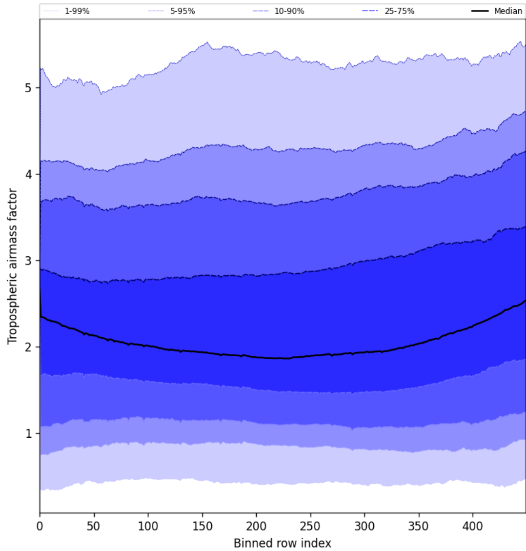
Figure 48: Along track statistics of “Tropospheric airmass factor” for 2025-06-01 to 2025-06-02
