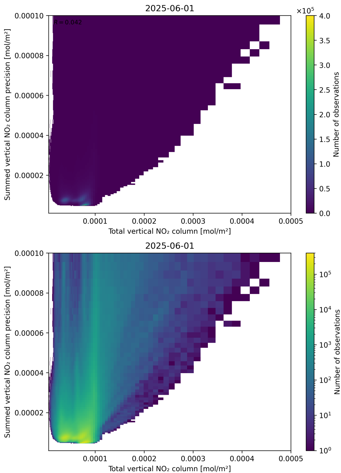
Figure 113: Scatter density plot of “Total vertical NO 2 column” against “Summed vertical NO 2 column precision” for 2025-06-01 to 2025-06-02.
