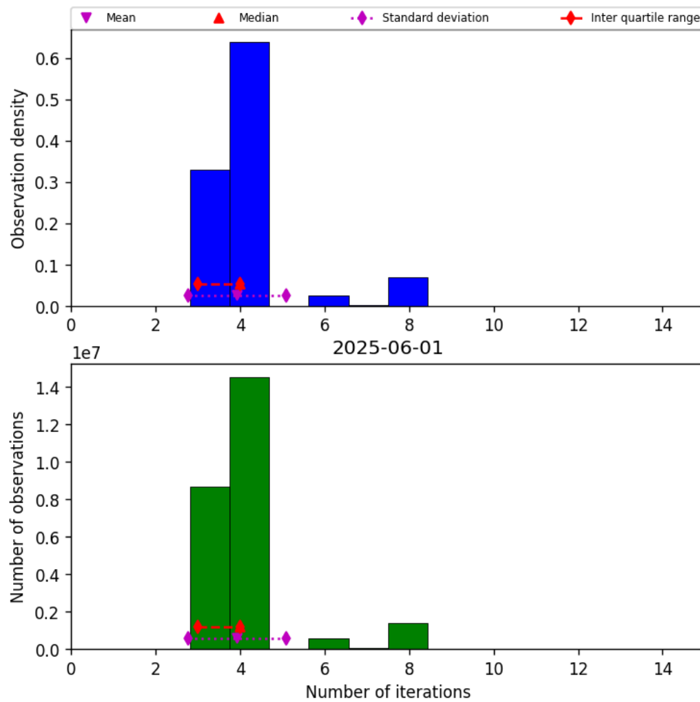
Figure 34: Histogram of “Number of iterations” for 2025-06-01 to 2025-06-02
