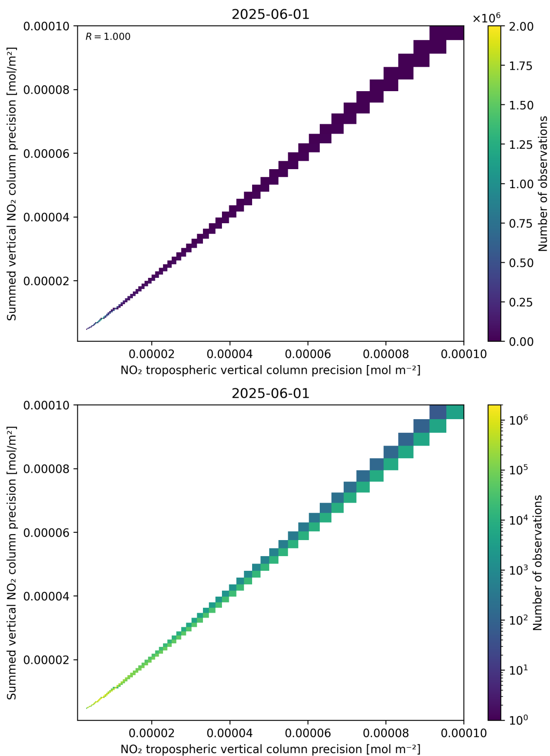
Figure 137: Scatter density plot of “NO 2 tropospheric vertical column precision” against “Summed vertical NO 2 column precision” for 2025-06-01 to 2025-06-02.
