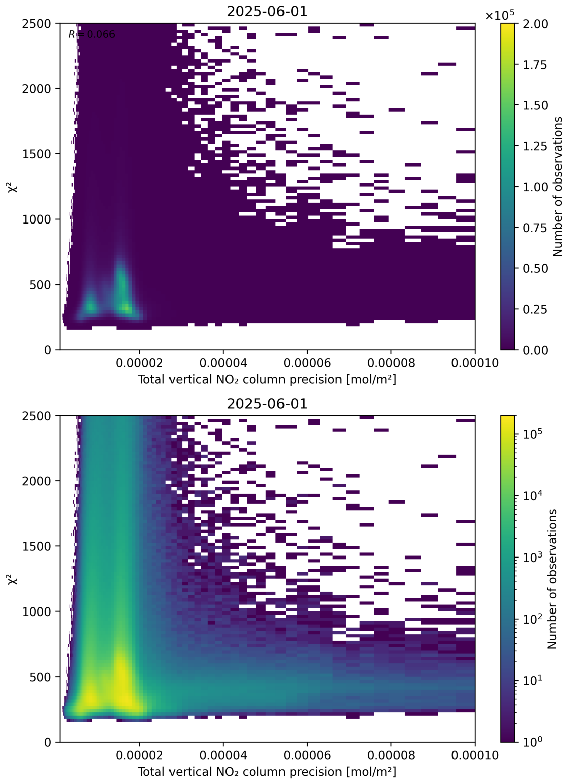
Figure 116: Scatter density plot of “Total vertical NO 2 column precision” against “ \chi^2 ” for 2025-06-01 to 2025-06-02.
