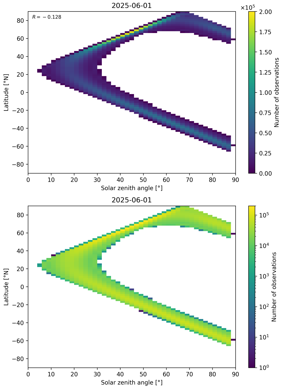
Figure 149: Scatter density plot of “Solar zenith angle” against “Latitude” for 2025-06-01 to 2025-06-02.
