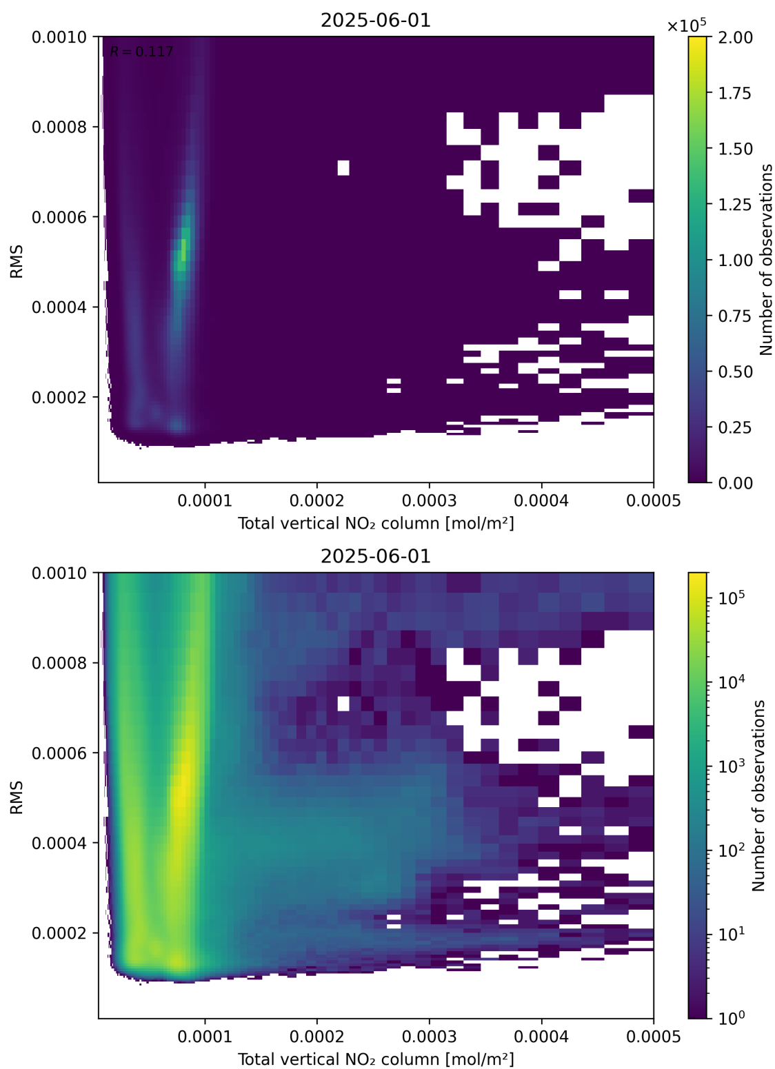
Figure 120: Scatter density plot of “Total vertical NO 2 column” against “RMS” for 2025-06-01 to 2025-06-02.
