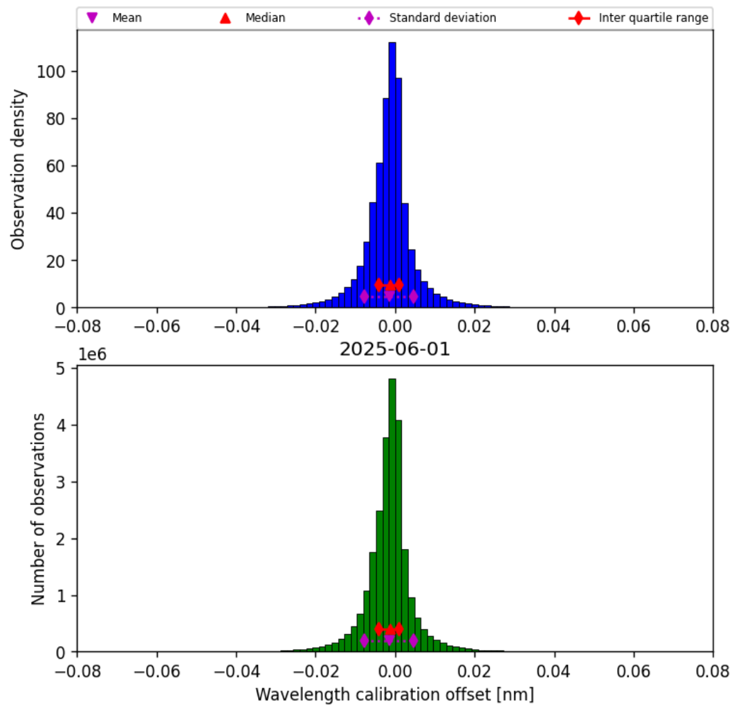
Figure 35: Histogram of “Wavelength calibration offset” for 2025-06-01 to 2025-06-02
