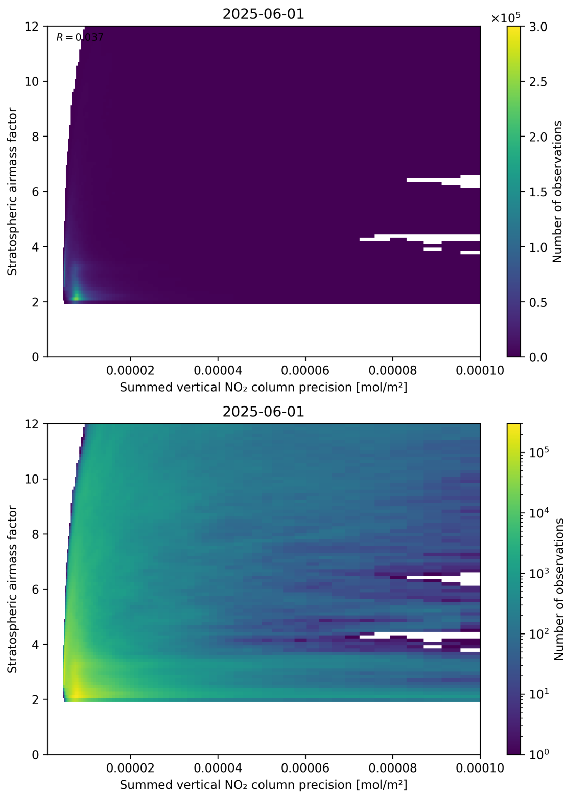
Figure 106: Scatter density plot of “Summed vertical NO 2 column precision” against “Stratospheric airmass factor” for 2025-06-01 to 2025-06-02.
