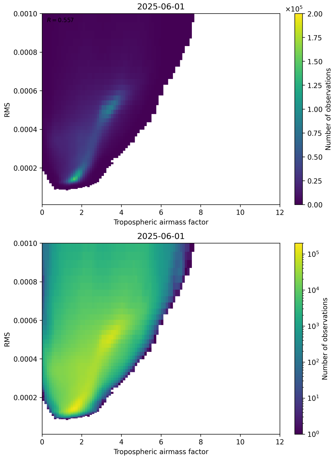
Figure 79: Scatter density plot of “Tropospheric airmass factor” against “RMS” for 2025-06-01 to 2025-06-02.
