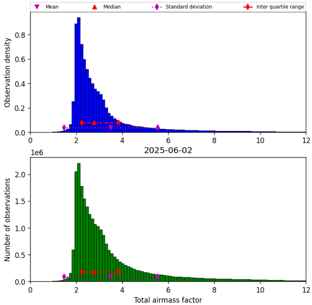
Figure 32: Histogram of “Total airmass factor” for 2025-06-01 to 2025-06-03
