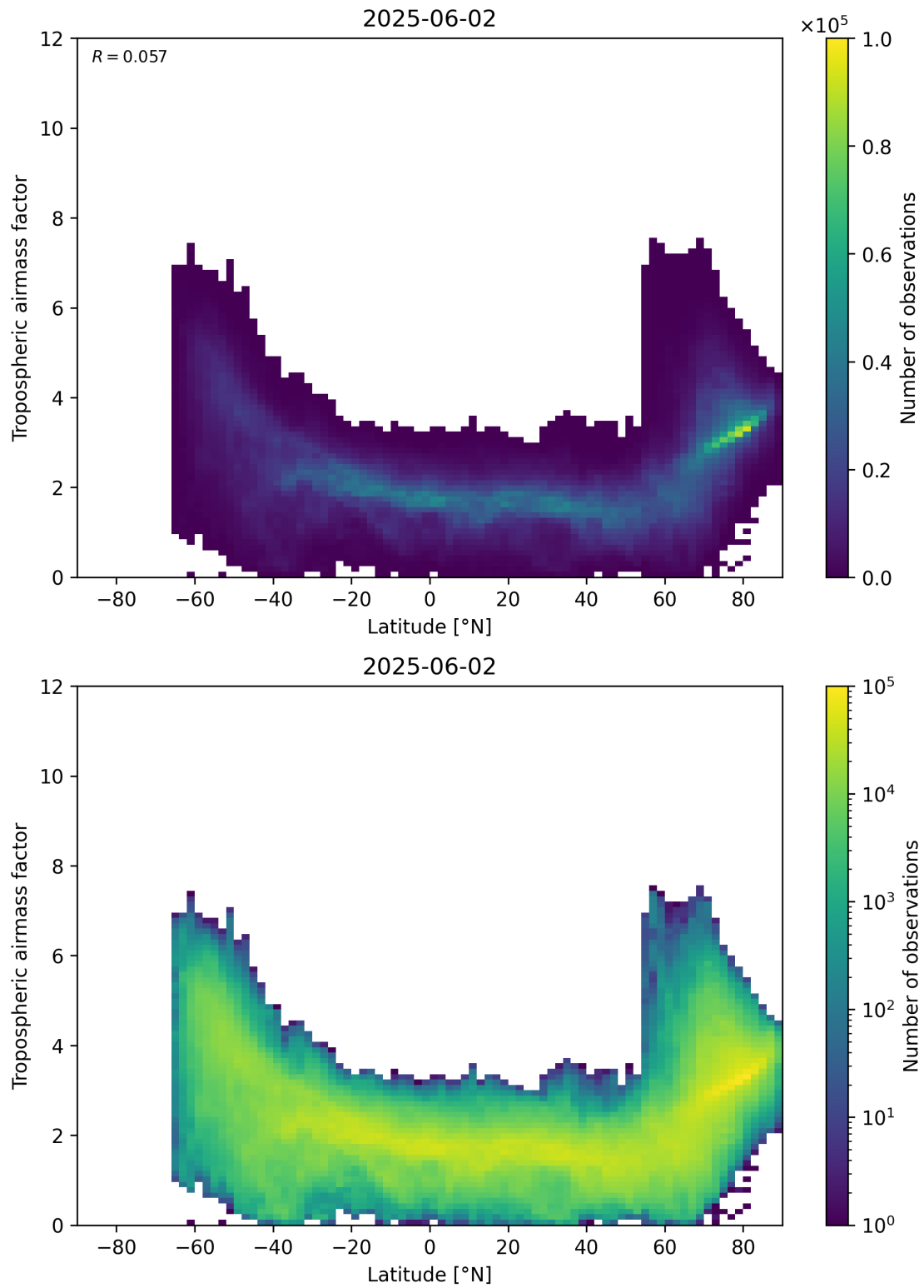
Figure 85: Scatter density plot of “Latitude” against “Tropospheric air mass factor” for 2025-06-01 to 2025-06-03.
