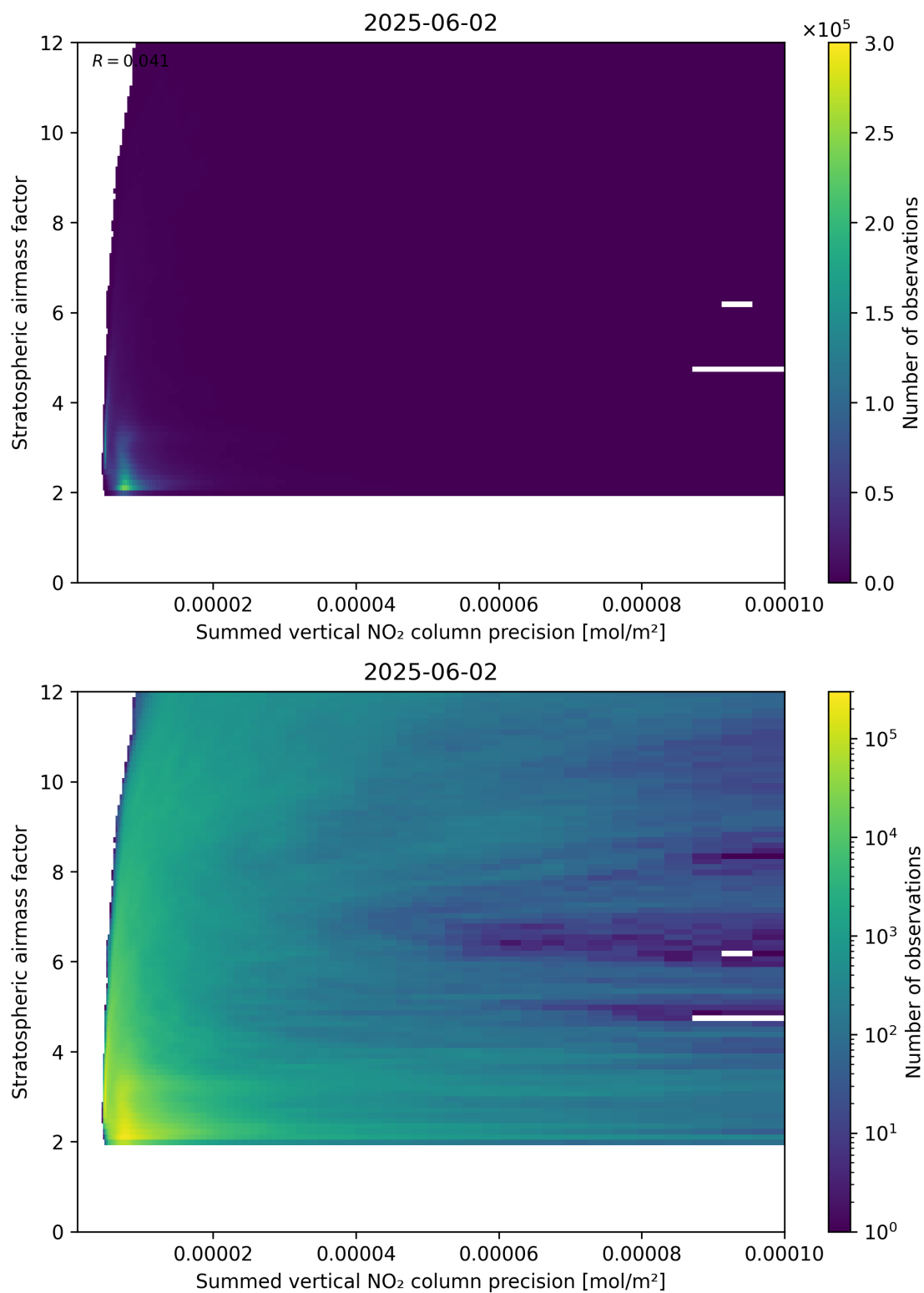
Figure 106: Scatter density plot of “Summed vertical NO 2 column precision” against “Stratospheric airmass factor” for 2025-06-01 to 2025-06-03.
