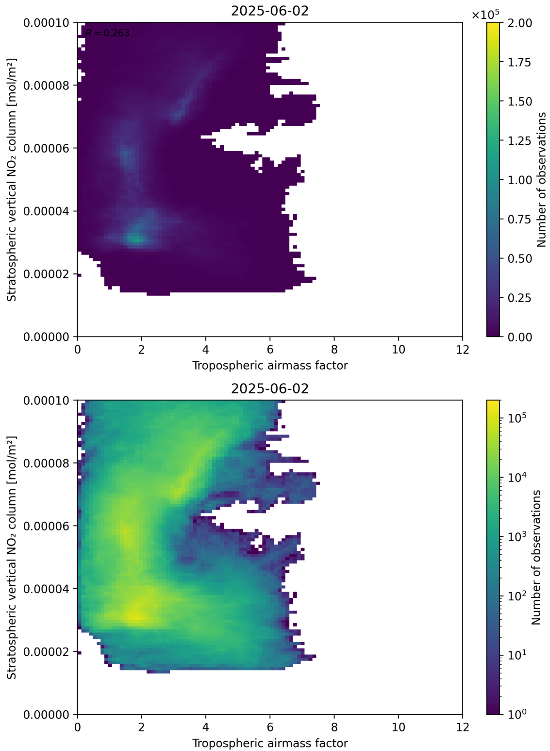
Figure 74: Scatter density plot of “Tropospheric air mass factor” against “Stratospheric vertical NO 2 column” for 2025-06-01 to 2025-06-03.
