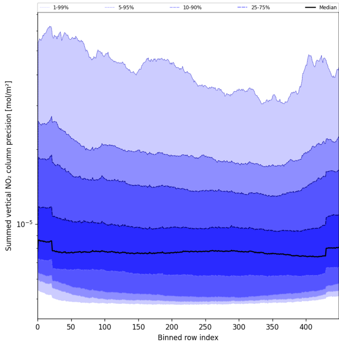
Figure 58: Along track statistics of “Summed vertical NO 2 column precision” for 2025-06-01 to 2025-06-03
