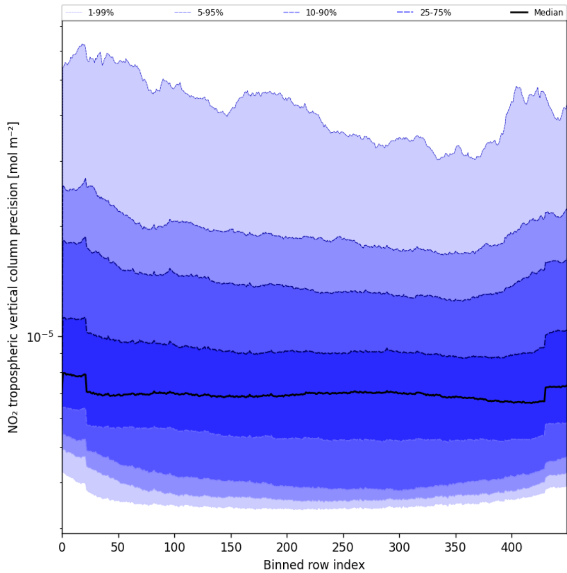
Figure 47: Along track statistics of “NO 2 tropospheric vertical column precision” for 2025-06-01 to 2025-06-03
