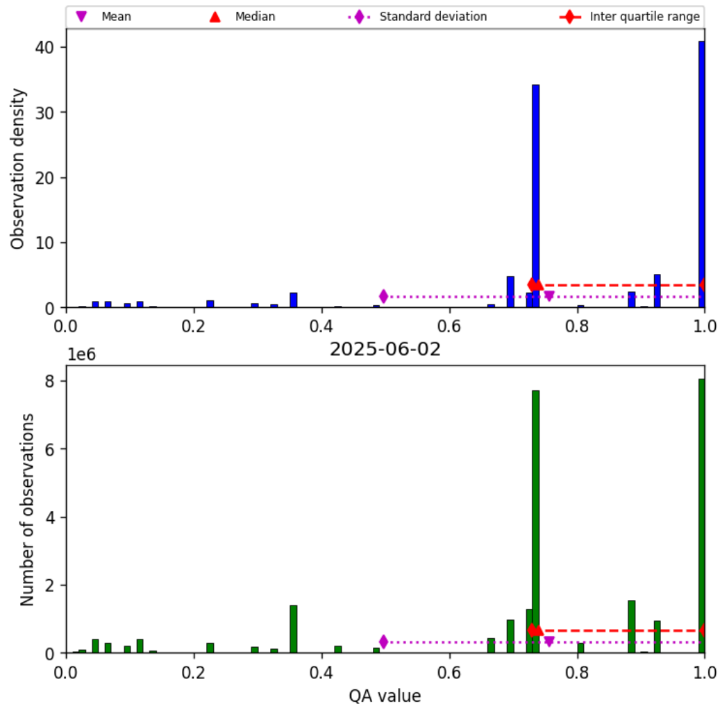
Figure 28: Histogram of “QA value” for 2025-06-01 to 2025-06-03
