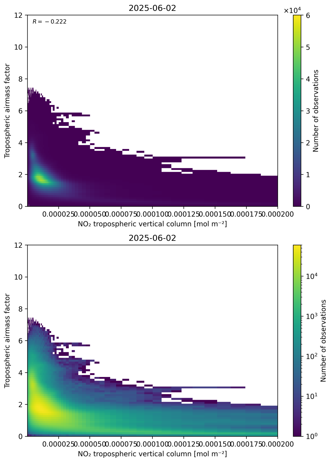
Figure 123: Scatter density plot of “NO 2 tropospheric vertical column” against “Tropospheric air mass factor” for 2025-06-01 to 2025-06-03.
