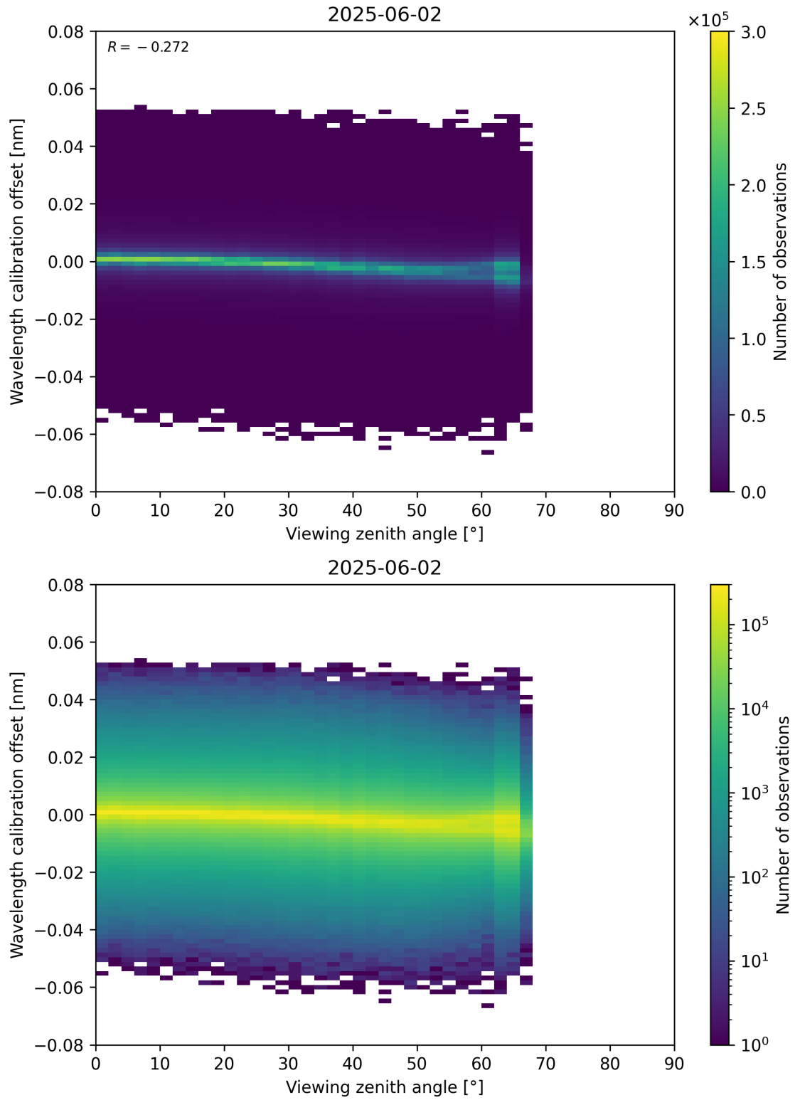
Figure 173: Scatter density plot of “Viewing zenith angle” against “Wavelength calibration offset” for 2025-06-01 to 2025-06-03.
