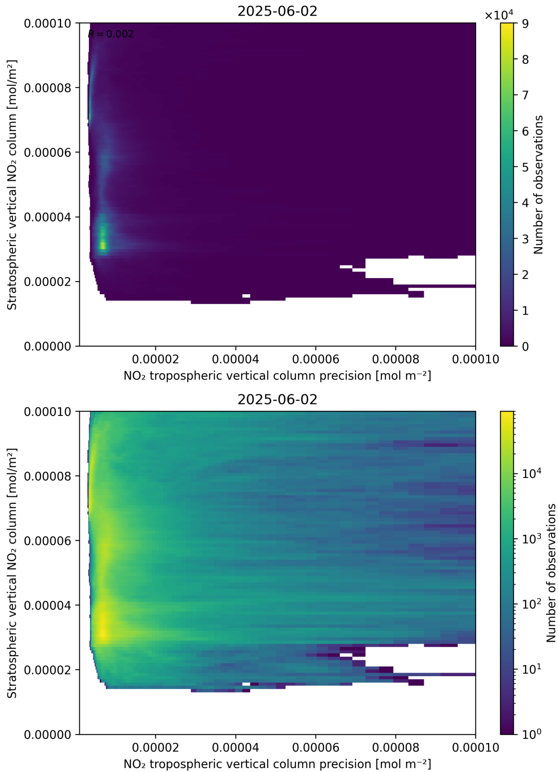
Figure 135: Scatter density plot of “NO 2 tropospheric vertical column precision” against “Stratospheric vertical NO 2 column” for 2025-06-01 to 2025-06-03.
