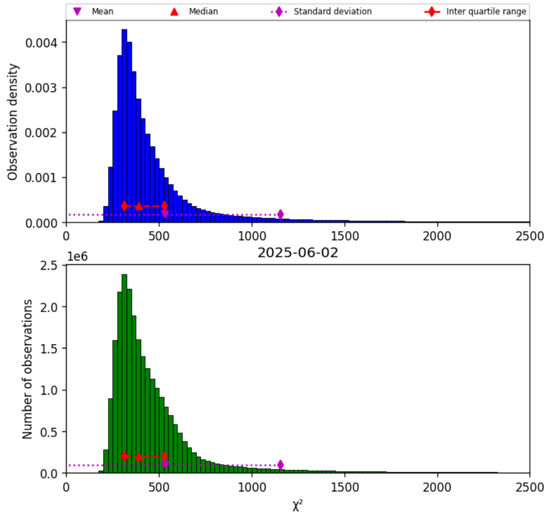
Figure 42: Histogram of " \chi^2 " for 2025-06-01 to 2025-06-03
