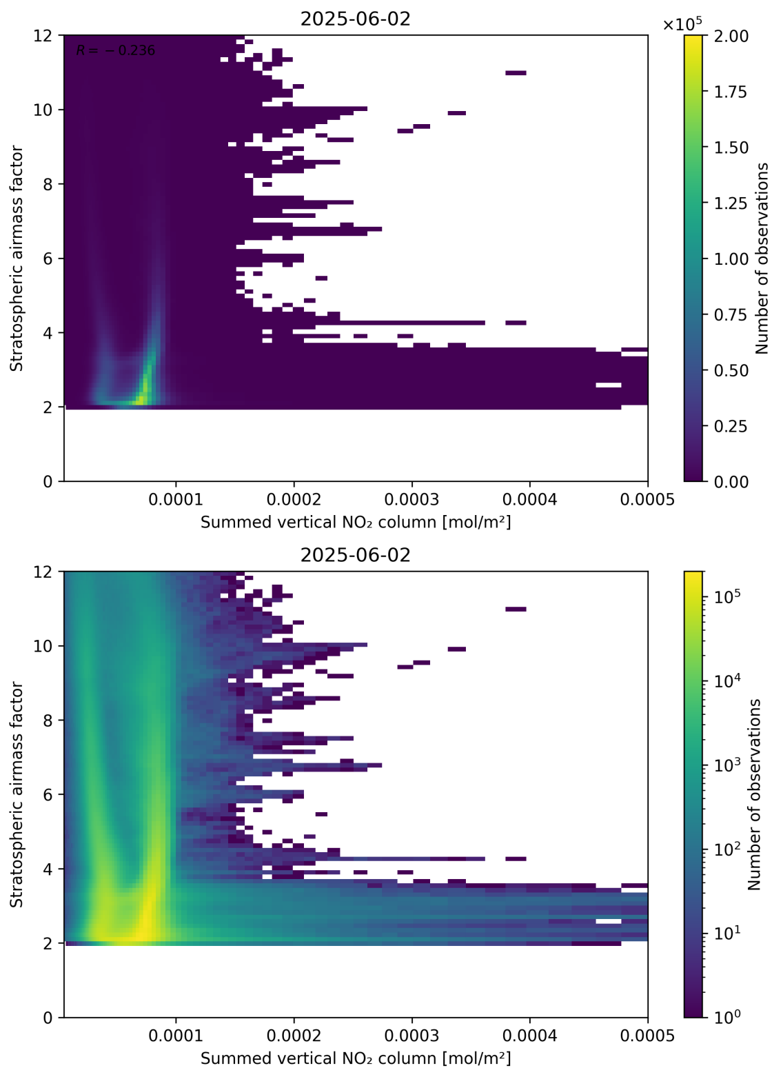
Figure 103: Scatter density plot of “Summed vertical NO 2 column” against “Stratospheric air mass factor” for 2025-06-01 to 2025-06-03.
