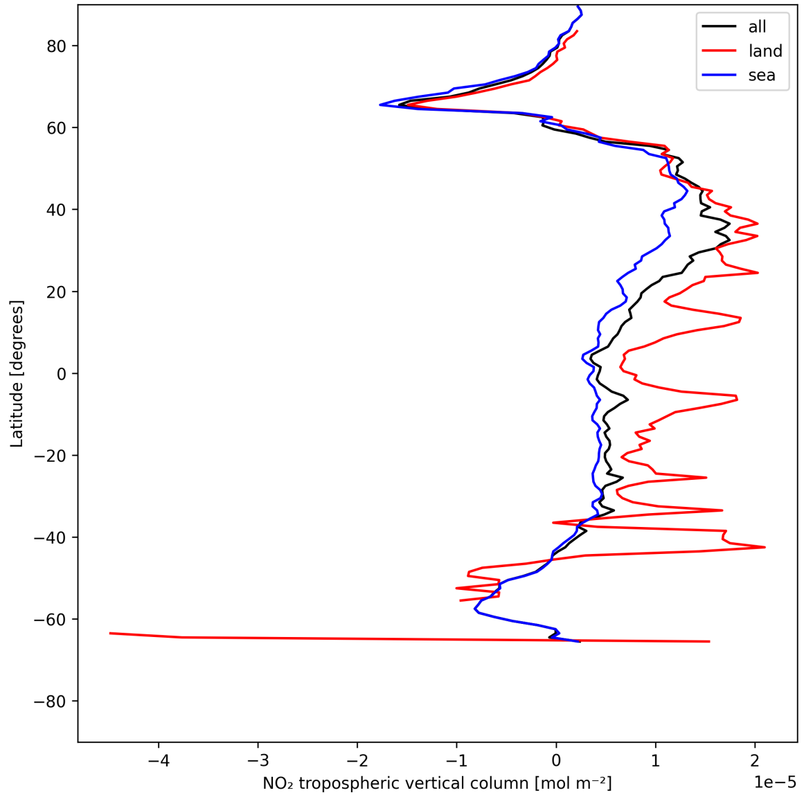
Figure 12: Zonal average of “NO 2 tropospheric vertical column” for 2025-06-01 to 2025-06-03.
