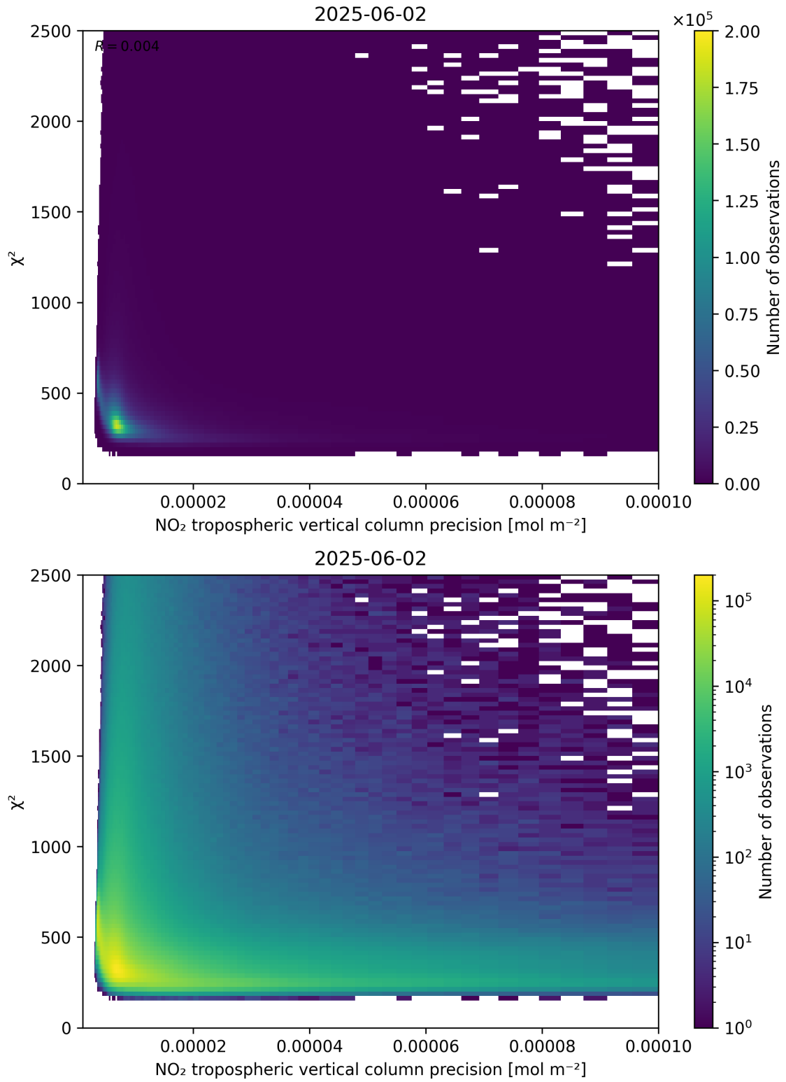
Figure 134: Scatter density plot of “NO 2 tropospheric vertical column precision” against “ \chi^2 ” for 2025-06-01 to 2025-06-03.
