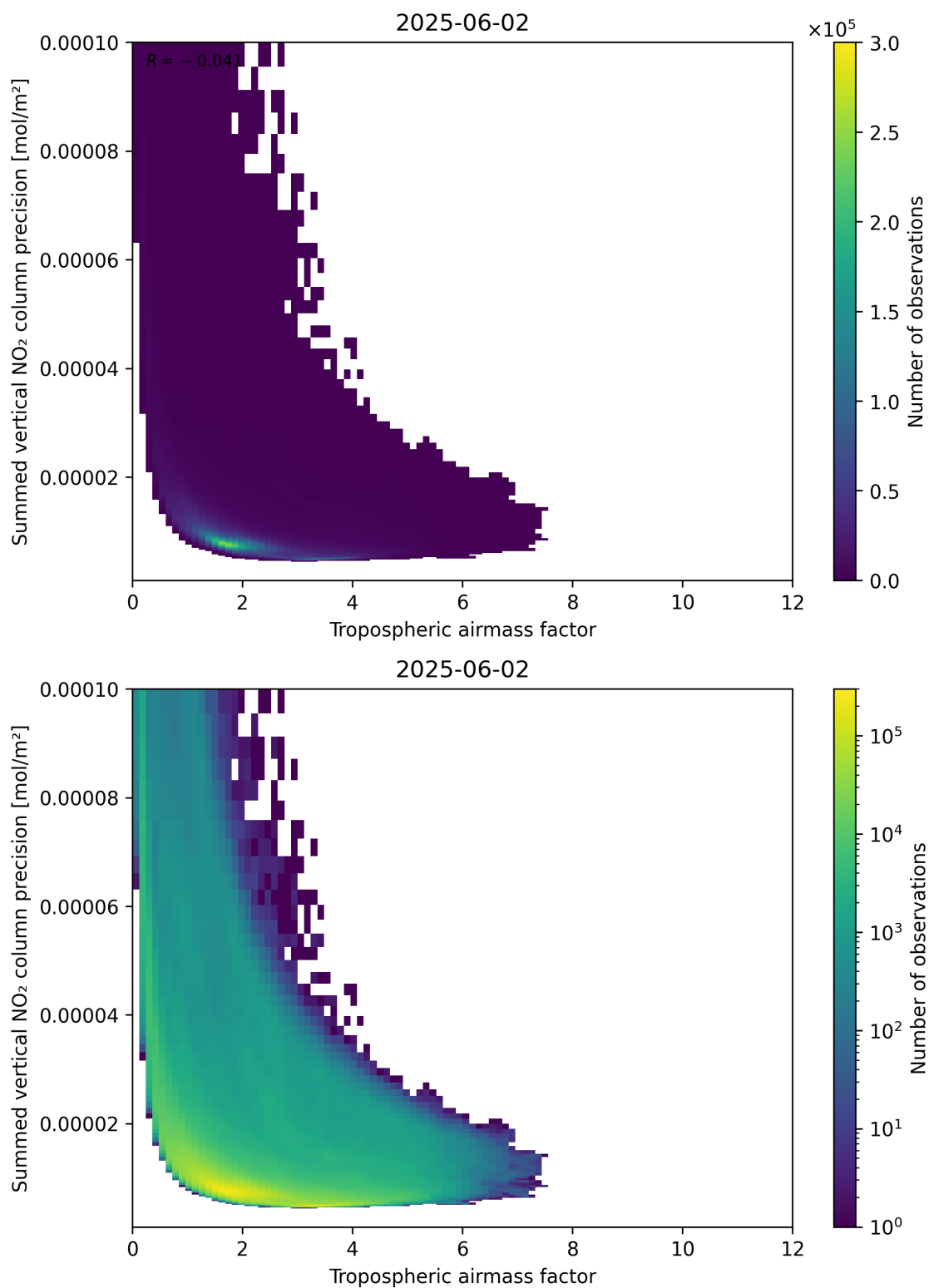
Figure 76: Scatter density plot of “Tropospheric air mass factor” against “Summed vertical NO 2 column precision” for 2025-06-01 to 2025-06-03.
