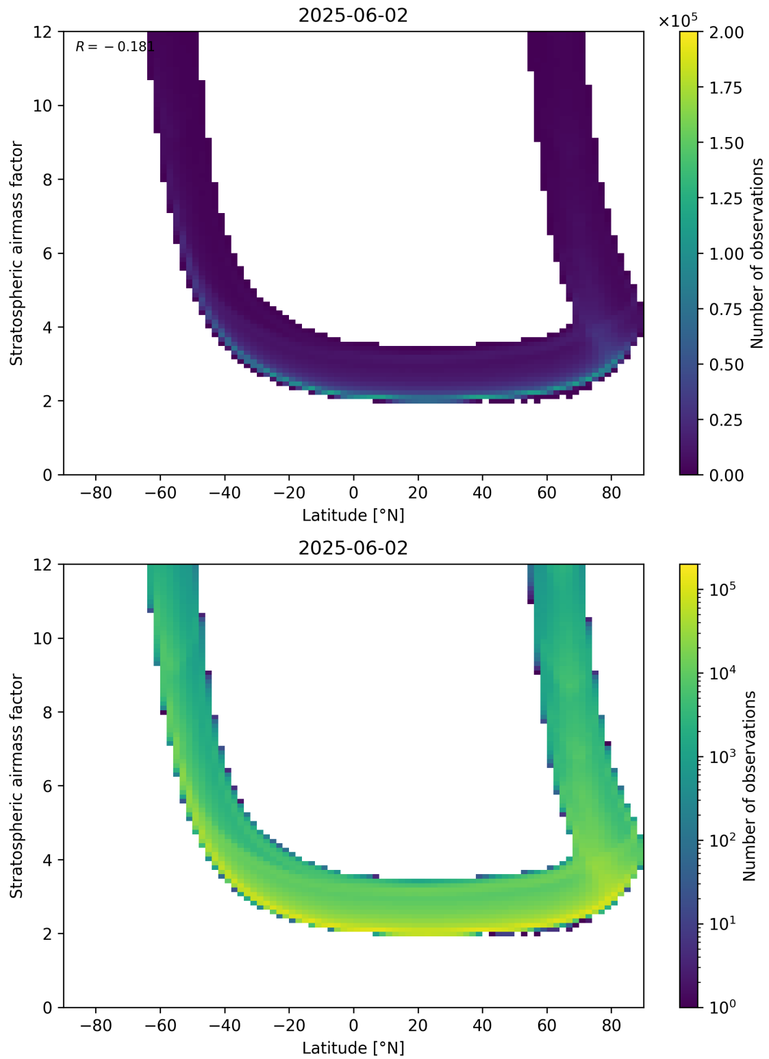
Figure 83: Scatter density plot of “Latitude” against “Stratospheric air mass factor” for 2025-06-01 to 2025-06-03.
