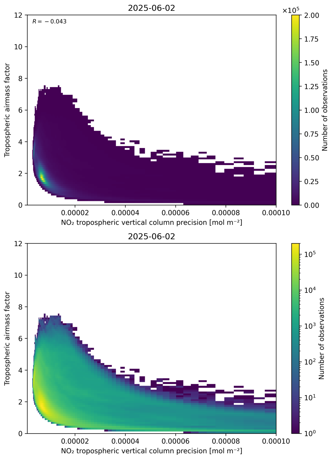
Figure 133: Scatter density plot of “NO 2 tropospheric vertical column precision” against “Tropospheric air mass factor” for 2025-06-01 to 2025-06-03.
