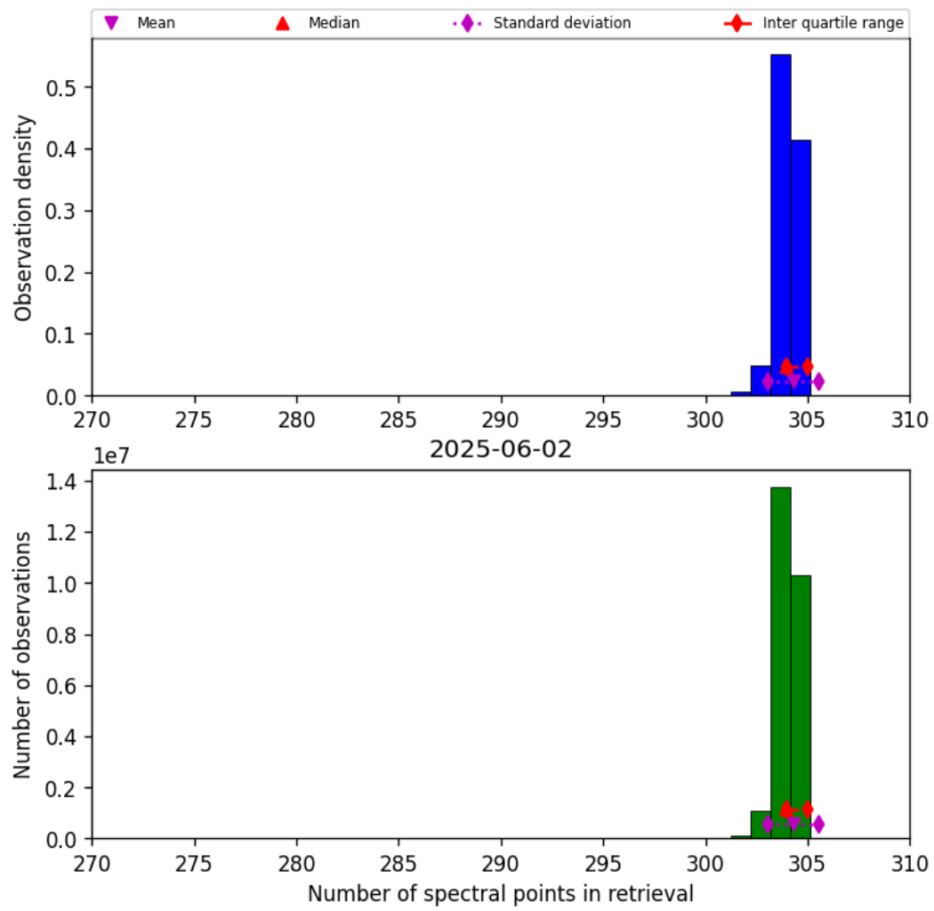
Figure 33: Histogram of “Number of spectral points in retrieval” for 2025-06-01 to 2025-06-03
