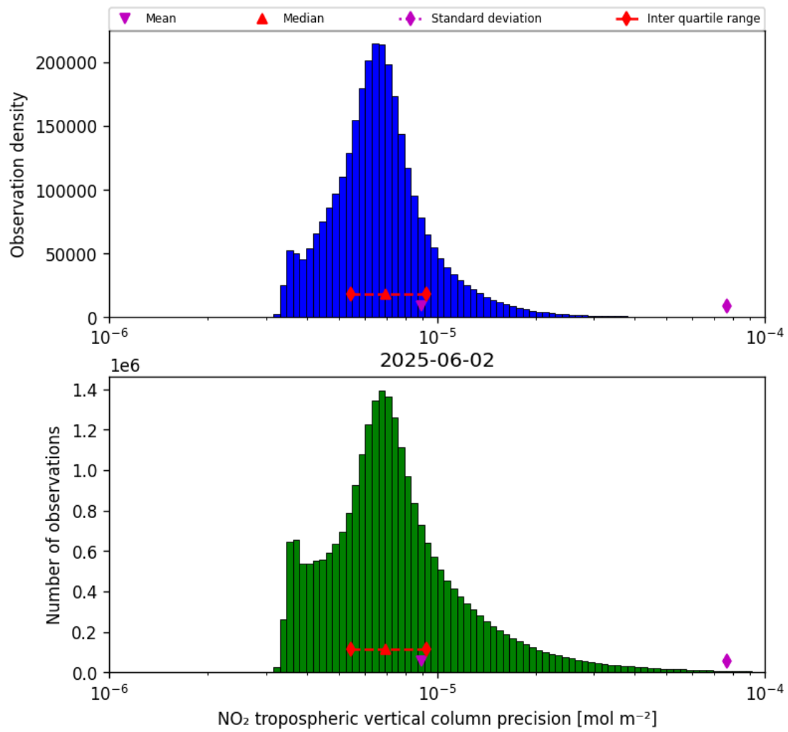
Figure 30: Histogram of “NO 2 tropospheric vertical column precision” for 2025-06-01 to 2025-06-03
