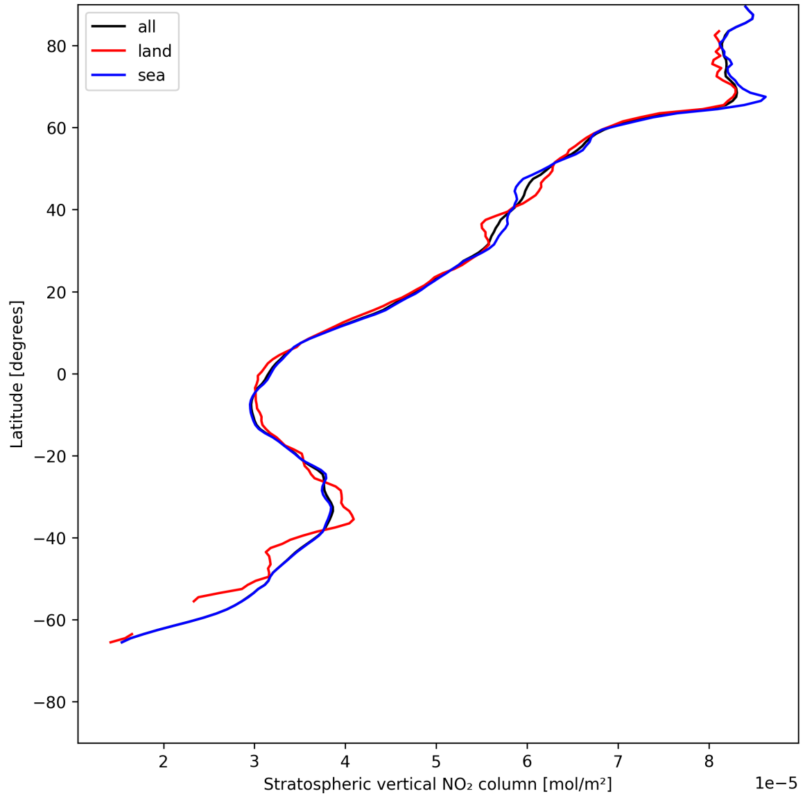
Figure 19: Zonal average of “Stratospheric vertical NO 2 column” for 2025-06-01 to 2025-06-03.
