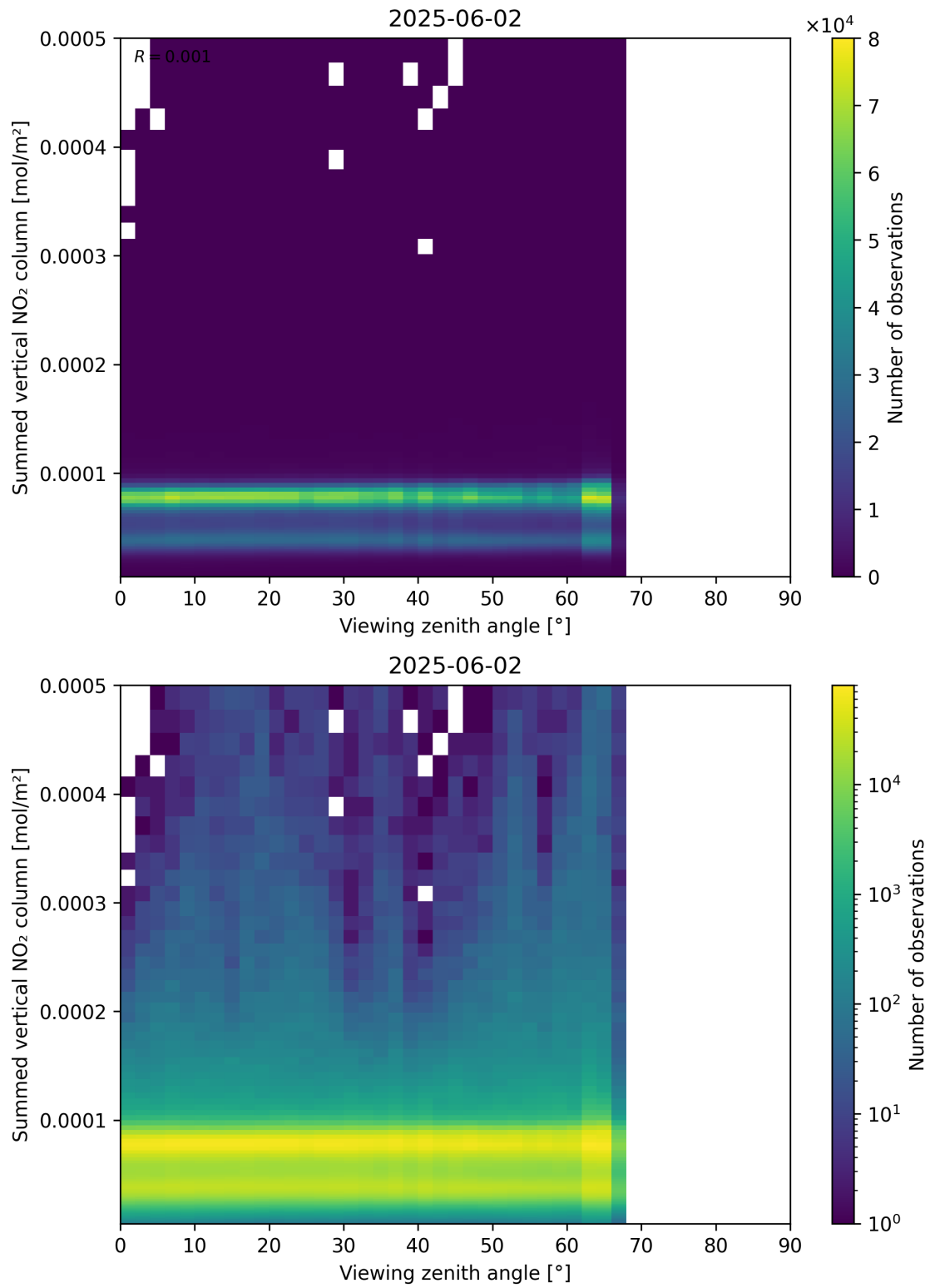
Figure 165: Scatter density plot of “Viewing zenith angle” against “Summed vertical NO 2 column” for 2025-06-01 to 2025-06-03.
