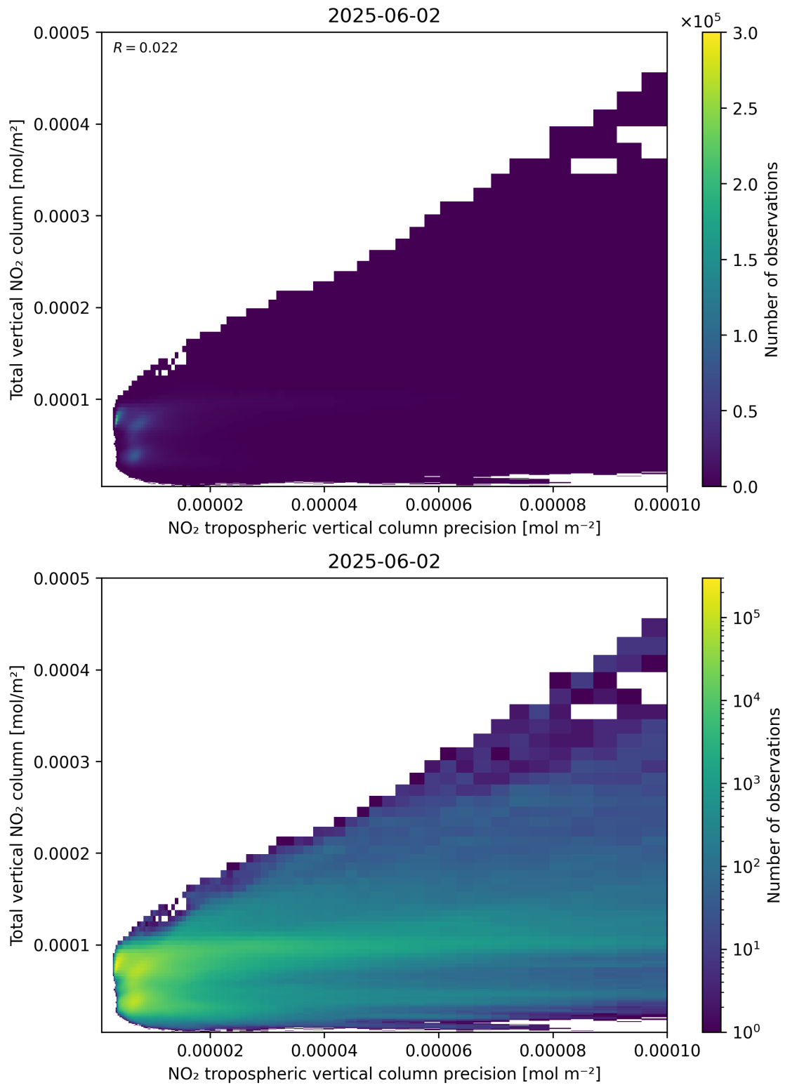
Figure 138: Scatter density plot of “NO 2 tropospheric vertical column precision” against “Total vertical NO 2 column” for 2025-06-01 to 2025-06-03.
