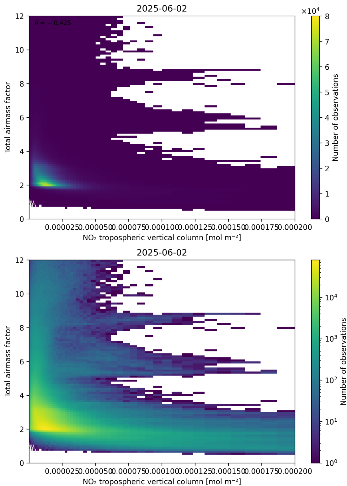
Figure 122: Scatter density plot of “NO 2 tropospheric vertical column” against “Total air mass factor” for 2025-06-01 to 2025-06-03.
