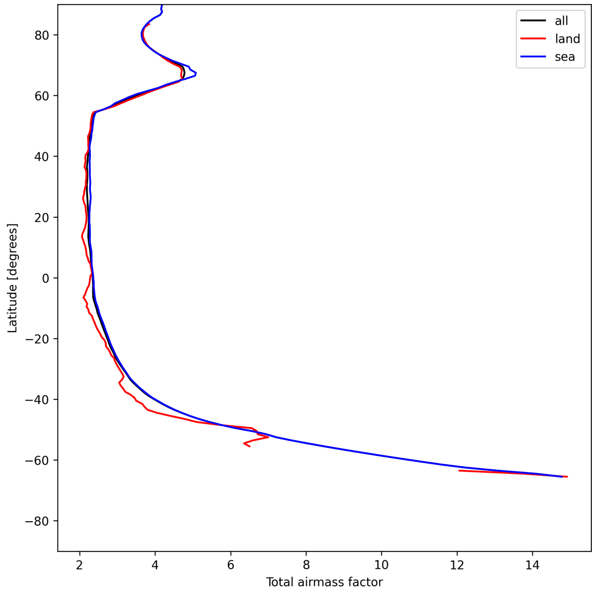
Figure 15: Zonal average of “Total airmass factor” for 2025-06-01 to 2025-06-03.
