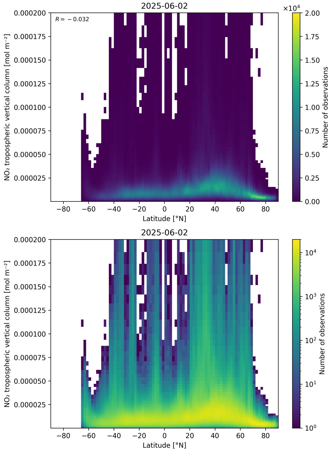
Figure 92: Scatter density plot of “Latitude” against “NO 2 tropospheric vertical column” for 2025-06-01 to 2025-06-03.
