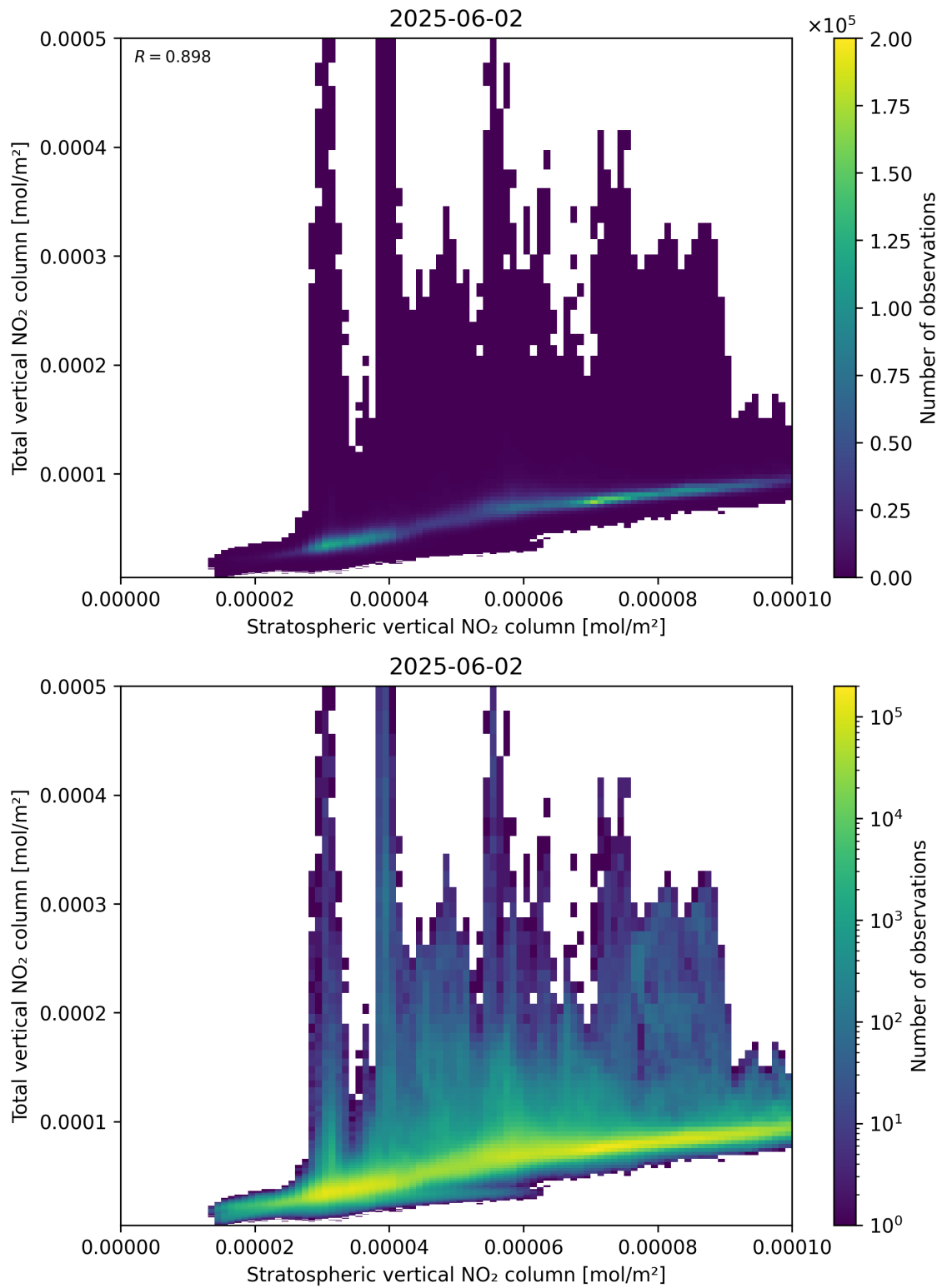
Figure 100: Scatter density plot of “Stratospheric vertical NO 2 column” against “Total vertical NO 2 column” for 2025-06-01 to 2025-06-03.
