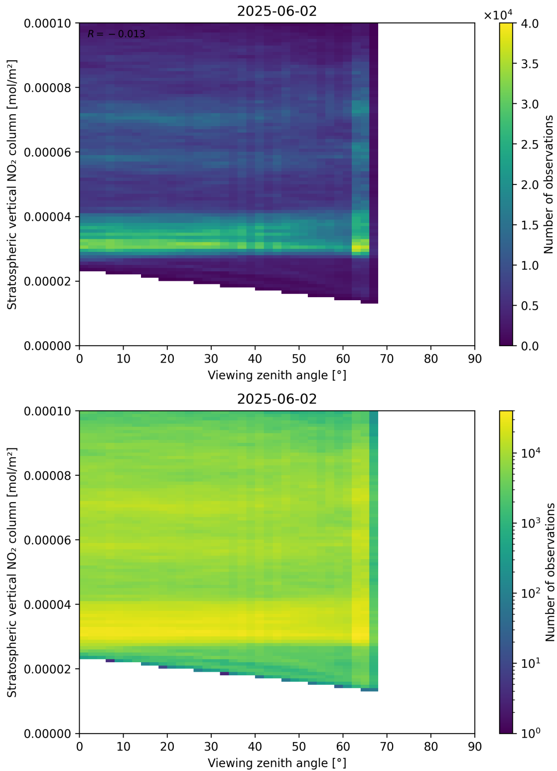
Figure 164: Scatter density plot of “Viewing zenith angle” against “Stratospheric vertical NO 2 column” for 2025-06-01 to 2025-06-03.
