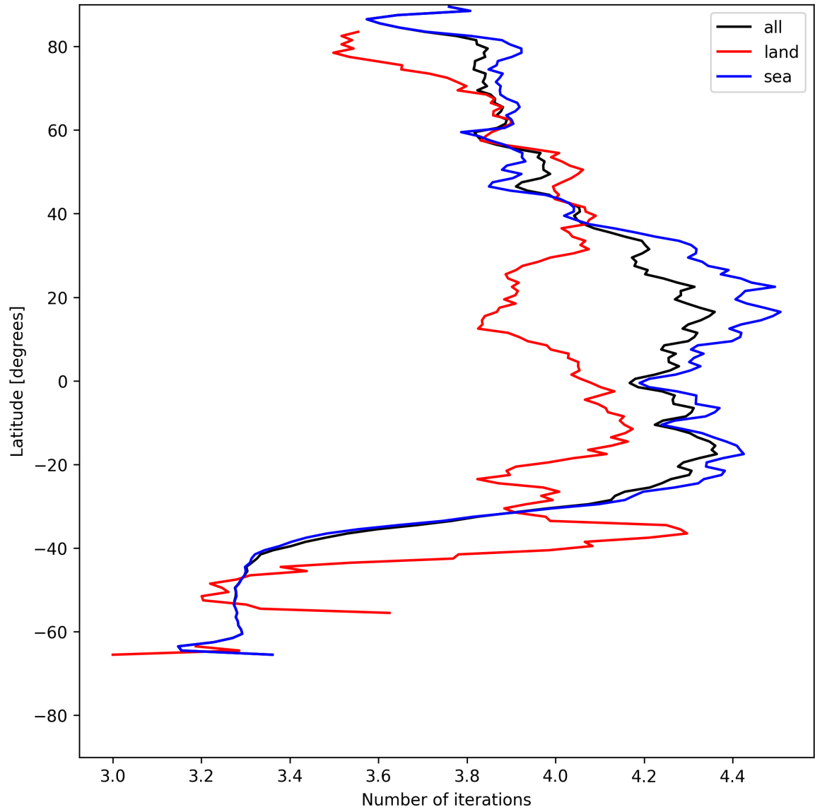
Figure 17: Zonal average of “Number of iterations” for 2025-06-01 to 2025-06-03.
