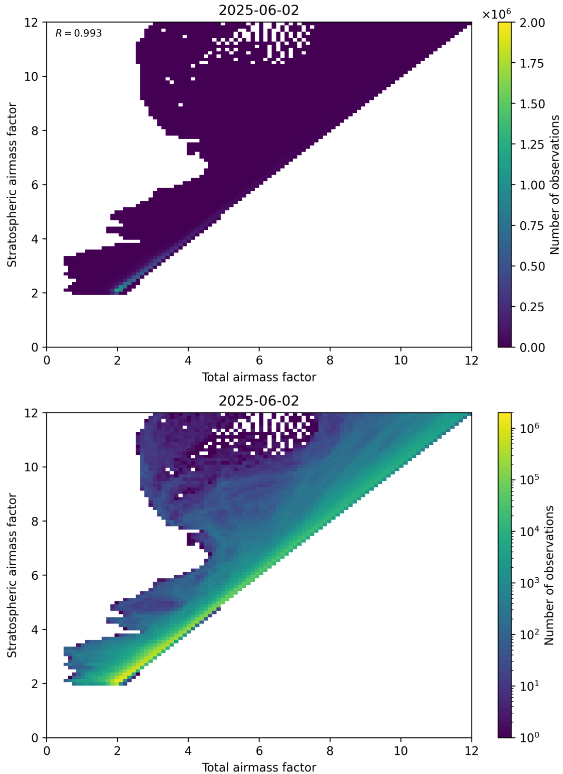
Figure 62: Scatter density plot of “Total airmass factor” against “Stratospheric airmass factor” for 2025-06-01 to 2025-06-03.
