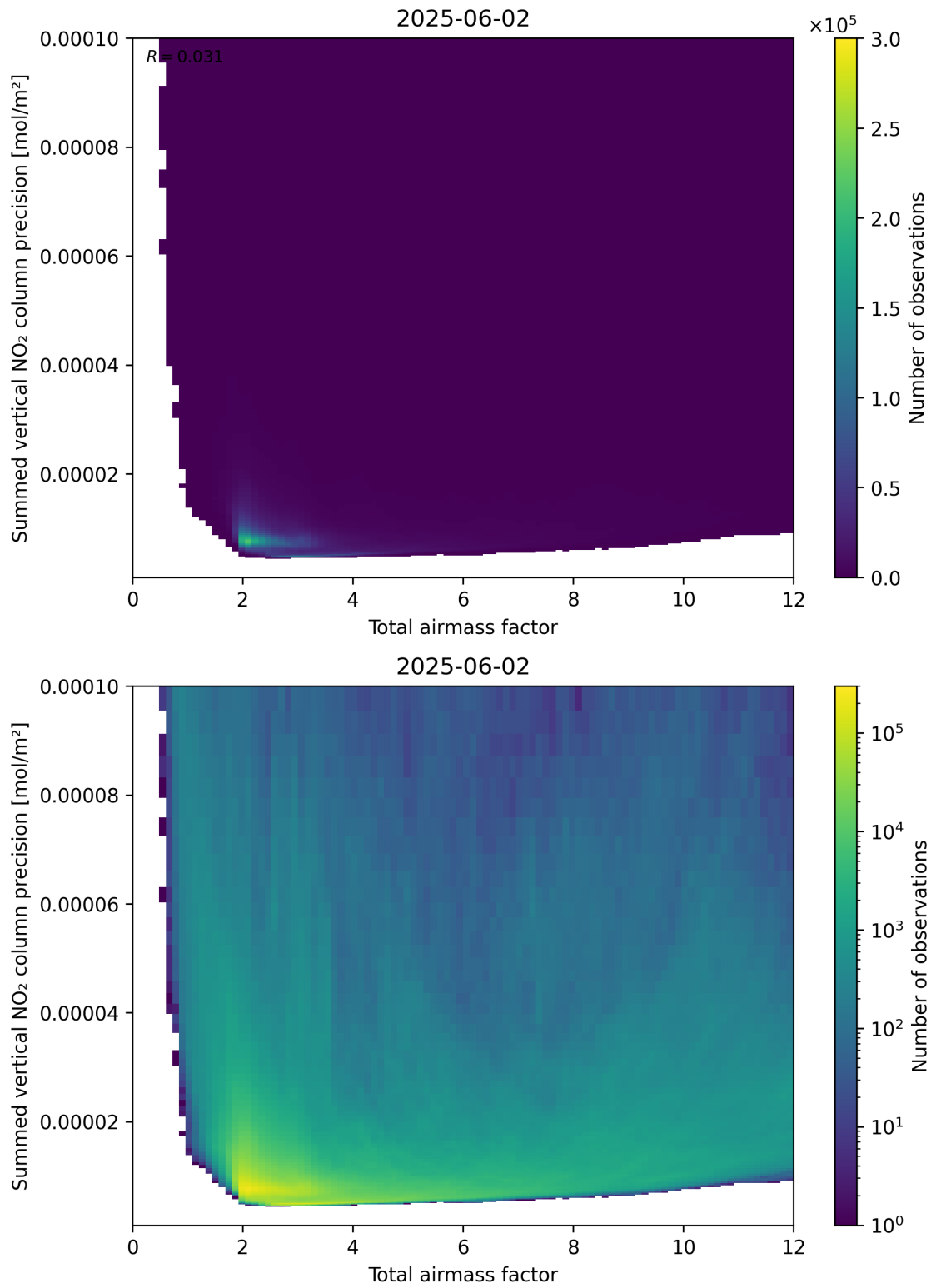
Figure 66: Scatter density plot of “Total airmass factor” against “Summed vertical NO 2 column precision” for 2025-06-01 to 2025-06-03.
