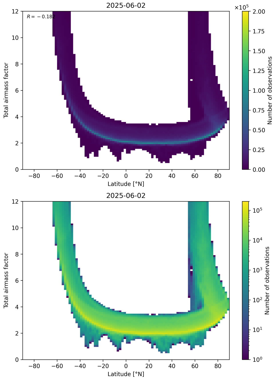
Figure 84: Scatter density plot of “Latitude” against “Total airmass factor” for 2025-06-01 to 2025-06-03.
