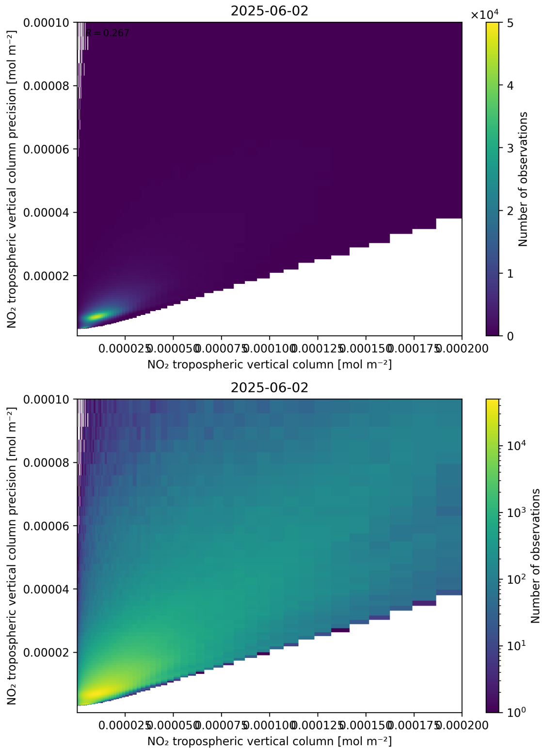
Figure 130: Scatter density plot of “NO 2 tropospheric vertical column” against “NO 2 tropospheric vertical column precision” for 2025-06-01 to 2025-06-03.
