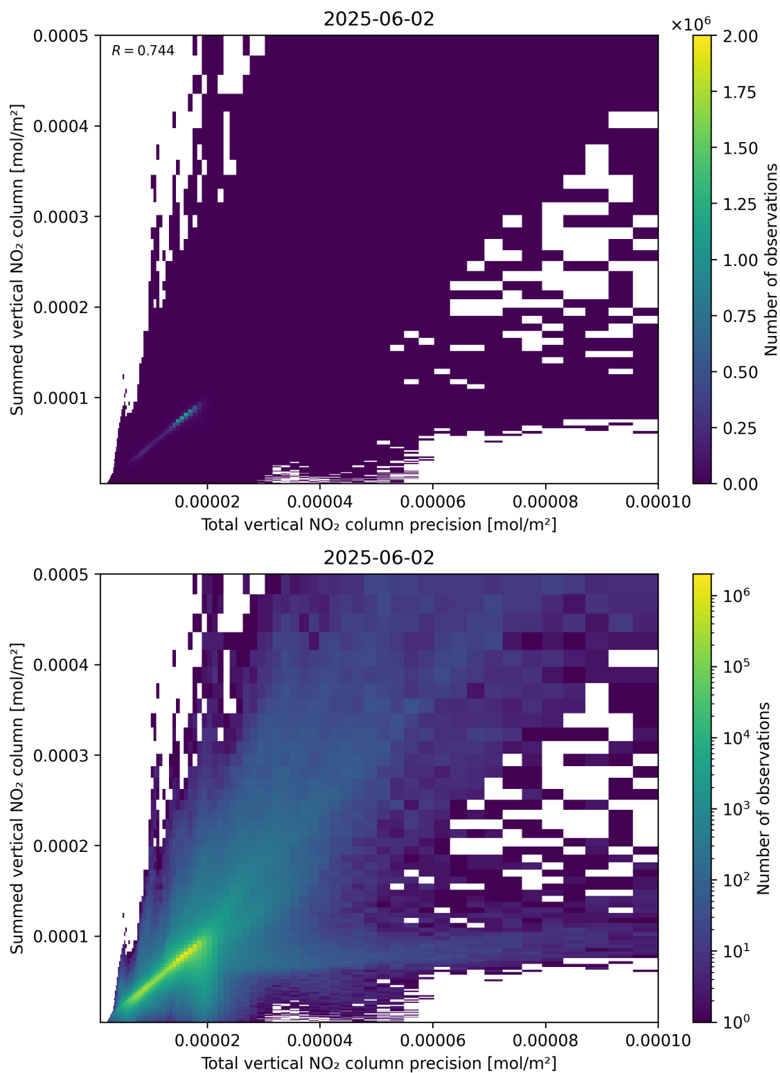
Figure 117: Scatter density plot of “Total vertical NO 2 column precision” against “Summed vertical NO 2 column” for 2025-06-01 to 2025-06-03.
