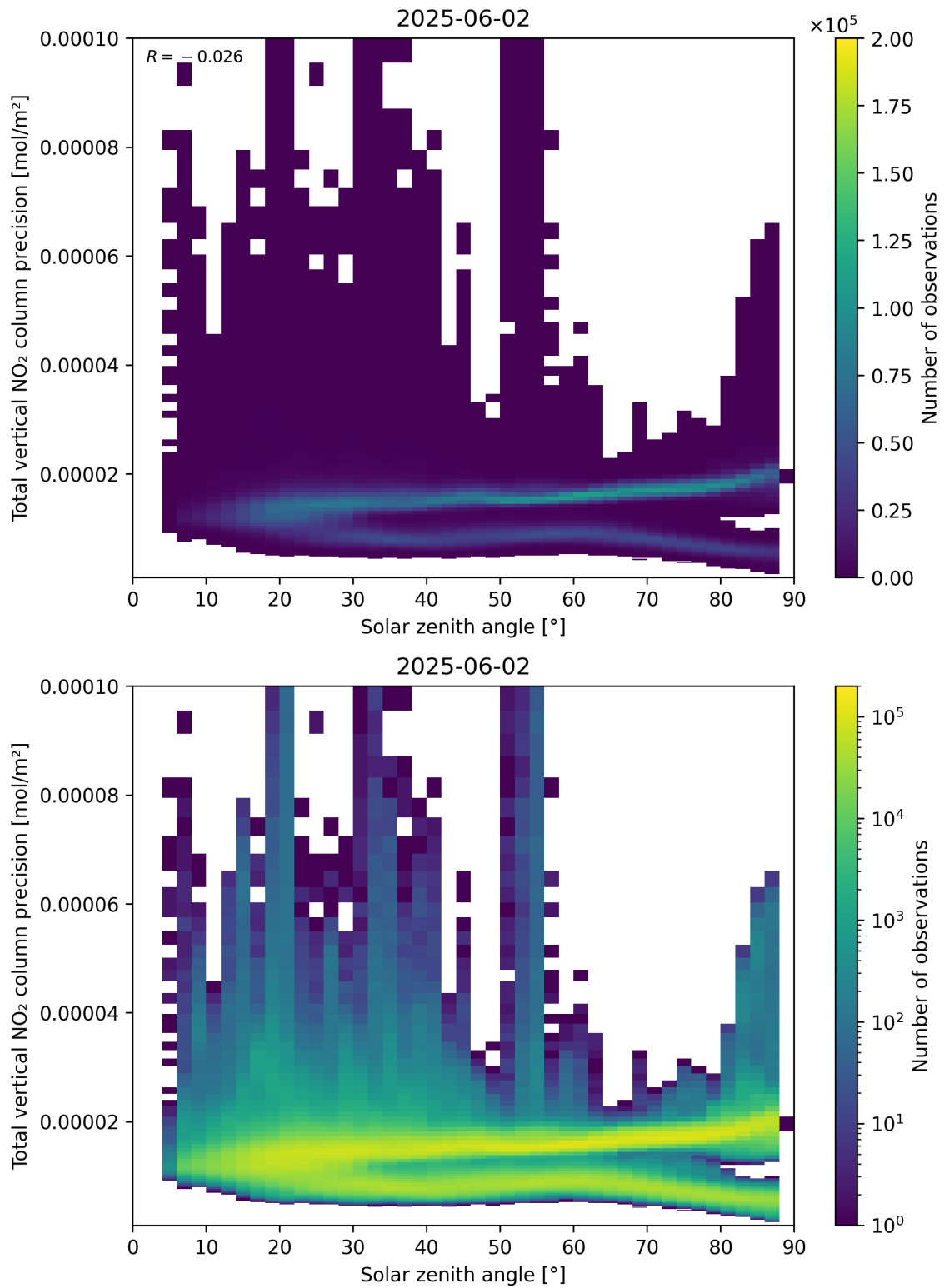
Figure 154: Scatter density plot of “Solar zenith angle” against “Total vertical NO 2 column precision” for 2025-06-01 to 2025-06-03.
