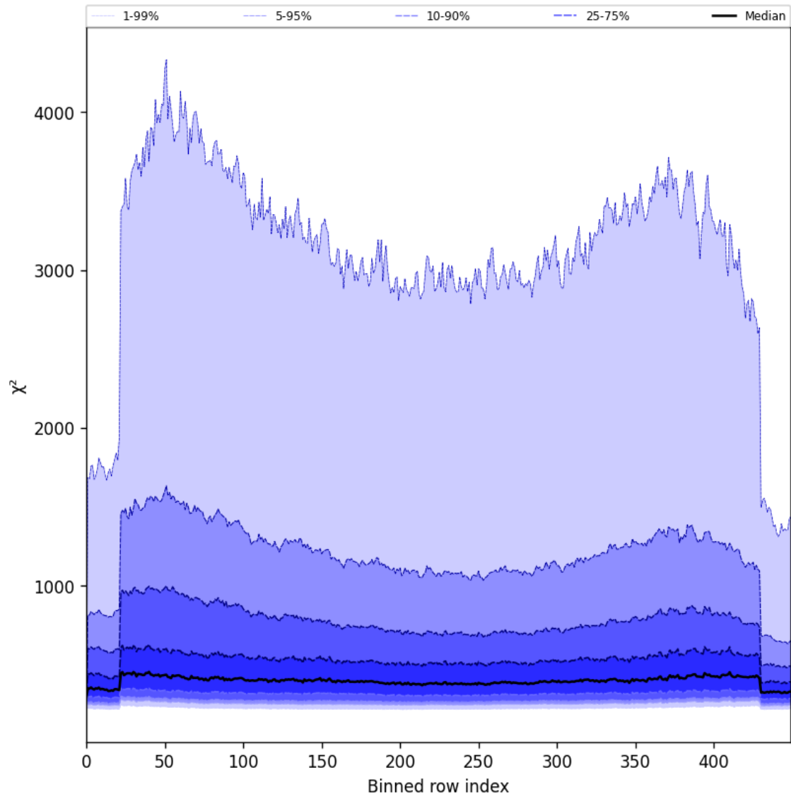
Figure 59: Along track statistics of “ \chi^2 ” for 2025-06-01 to 2025-06-03
