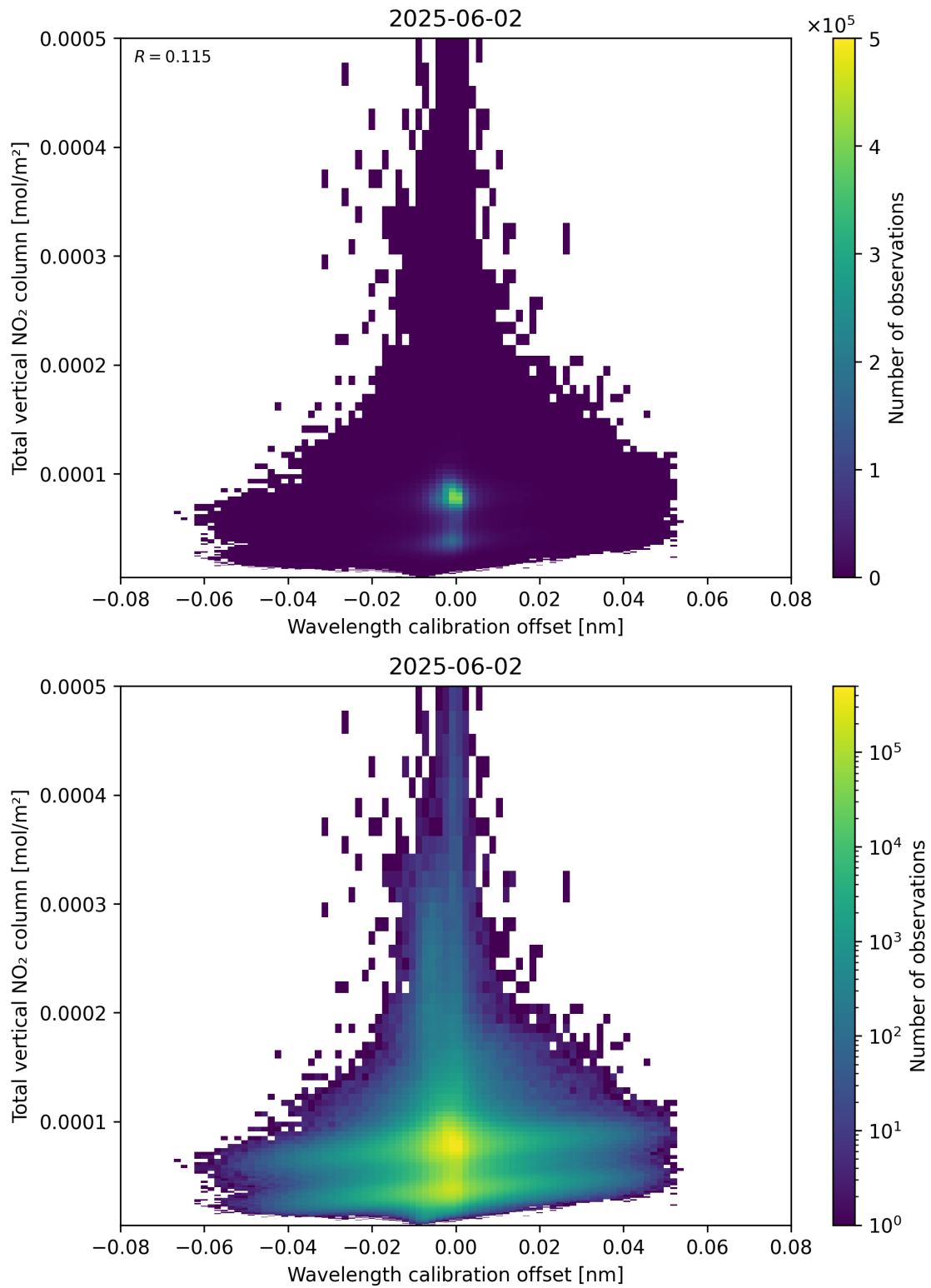
Figure 179: Scatter density plot of “Wavelength calibration offset” against “Total vertical NO 2 column” for 2025-06-01 to 2025-06-03.
