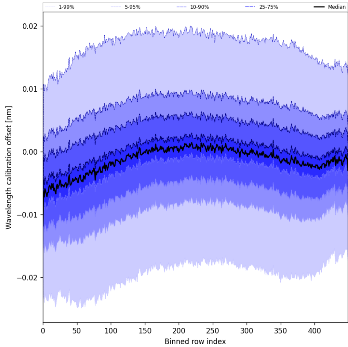
Figure 52: Along track statistics of “Wavelength calibration offset” for 2025-06-01 to 2025-06-03
