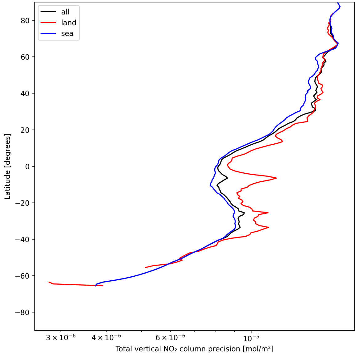
Figure 22: Zonal average of “Total vertical NO 2 column precision” for 2025-06-01 to 2025-06-03.
