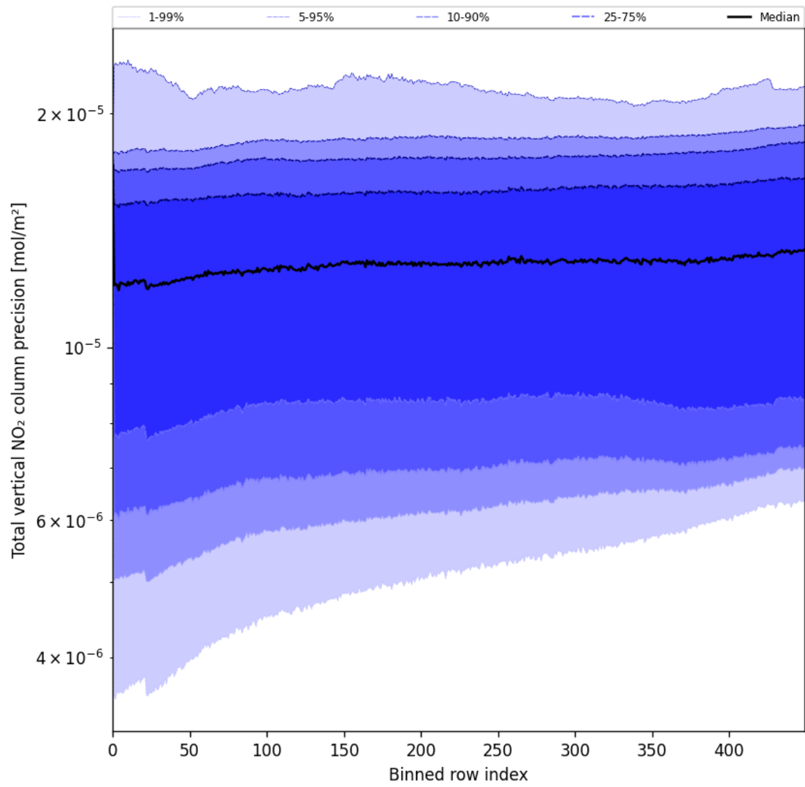
Figure 56: Along track statistics of “Total vertical NO 2 column precision” for 2025-06-01 to 2025-06-03
