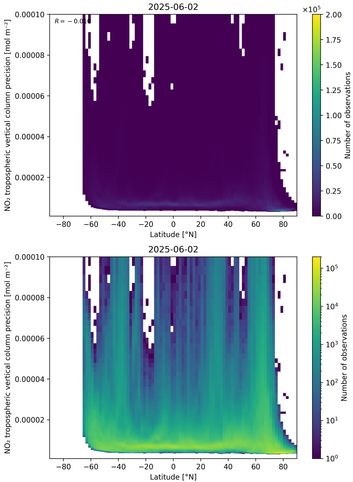
Figure 93: Scatter density plot of “Latitude” against “NO 2 tropospheric vertical column precision” for 2025-06-01 to 2025-06-03.
