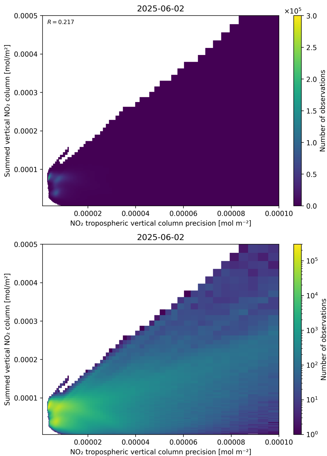
Figure 136: Scatter density plot of “NO 2 tropospheric vertical column precision” against “Summed vertical NO 2 column” for 2025-06-01 to 2025-06-03.
