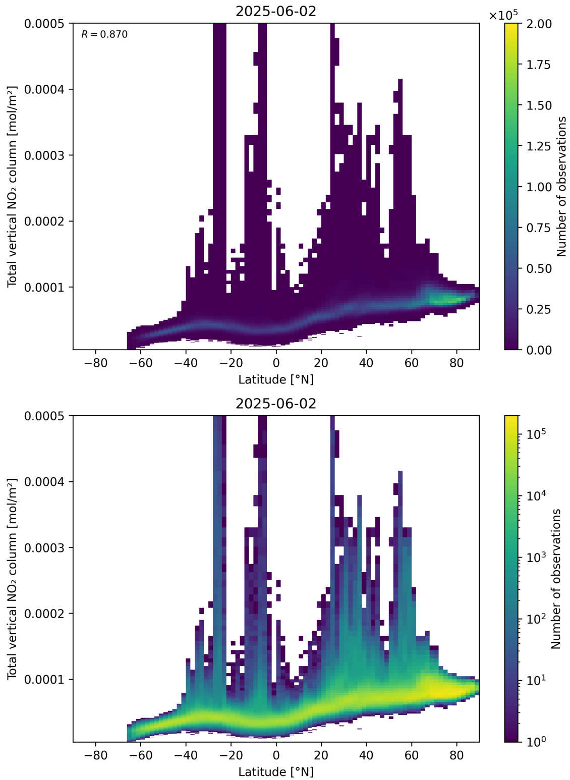
Figure 90: Scatter density plot of “Latitude” against “Total vertical NO 2 column” for 2025-06-01 to 2025-06-03.
