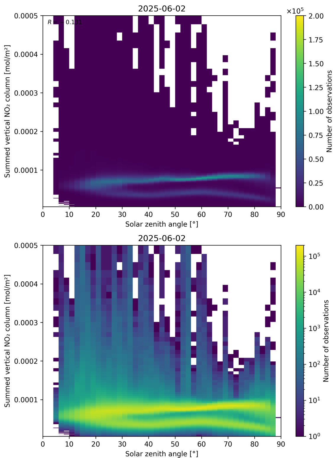
Figure 151: Scatter density plot of “Solar zenith angle” against “Summed vertical NO 2 column” for 2025-06-01 to 2025-06-03.
