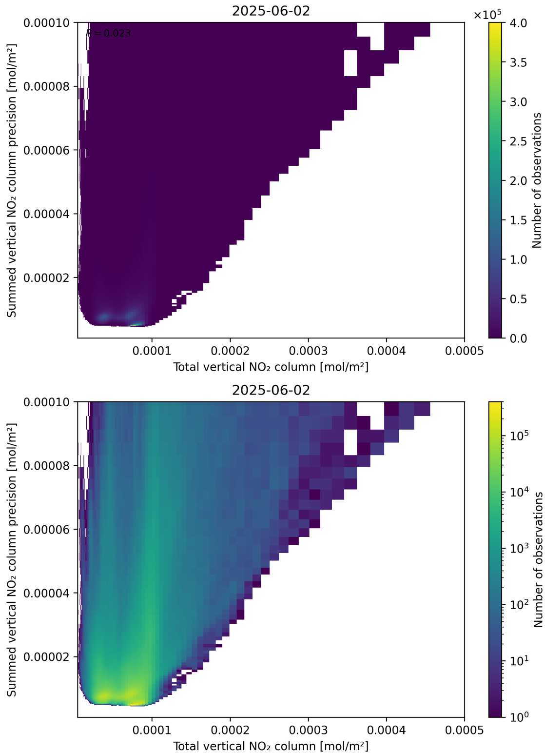
Figure 113: Scatter density plot of “Total vertical NO 2 column” against “Summed vertical NO 2 column precision” for 2025-06-01 to 2025-06-03.
