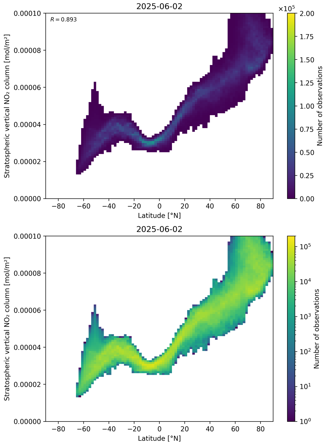
Figure 87: Scatter density plot of “Latitude” against “Stratospheric vertical \text{NO}_2 column” for 2025-06-01 to 2025-06-03.
