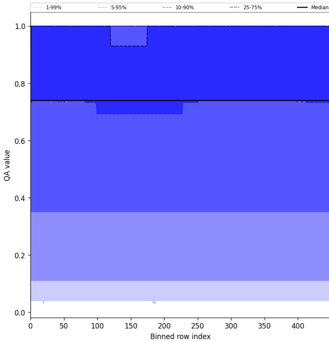
Figure 45: Along track statistics of “QA value” for 2025-06-01 to 2025-06-03
