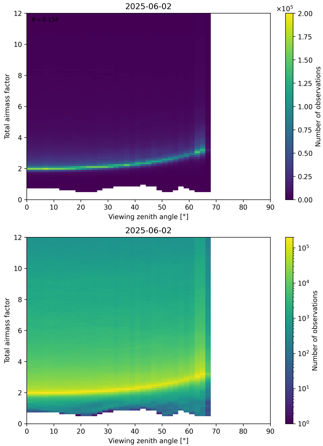
Figure 160: Scatter density plot of “Viewing zenith angle” against “Total airmass factor” for 2025-06-01 to 2025-06-03.
