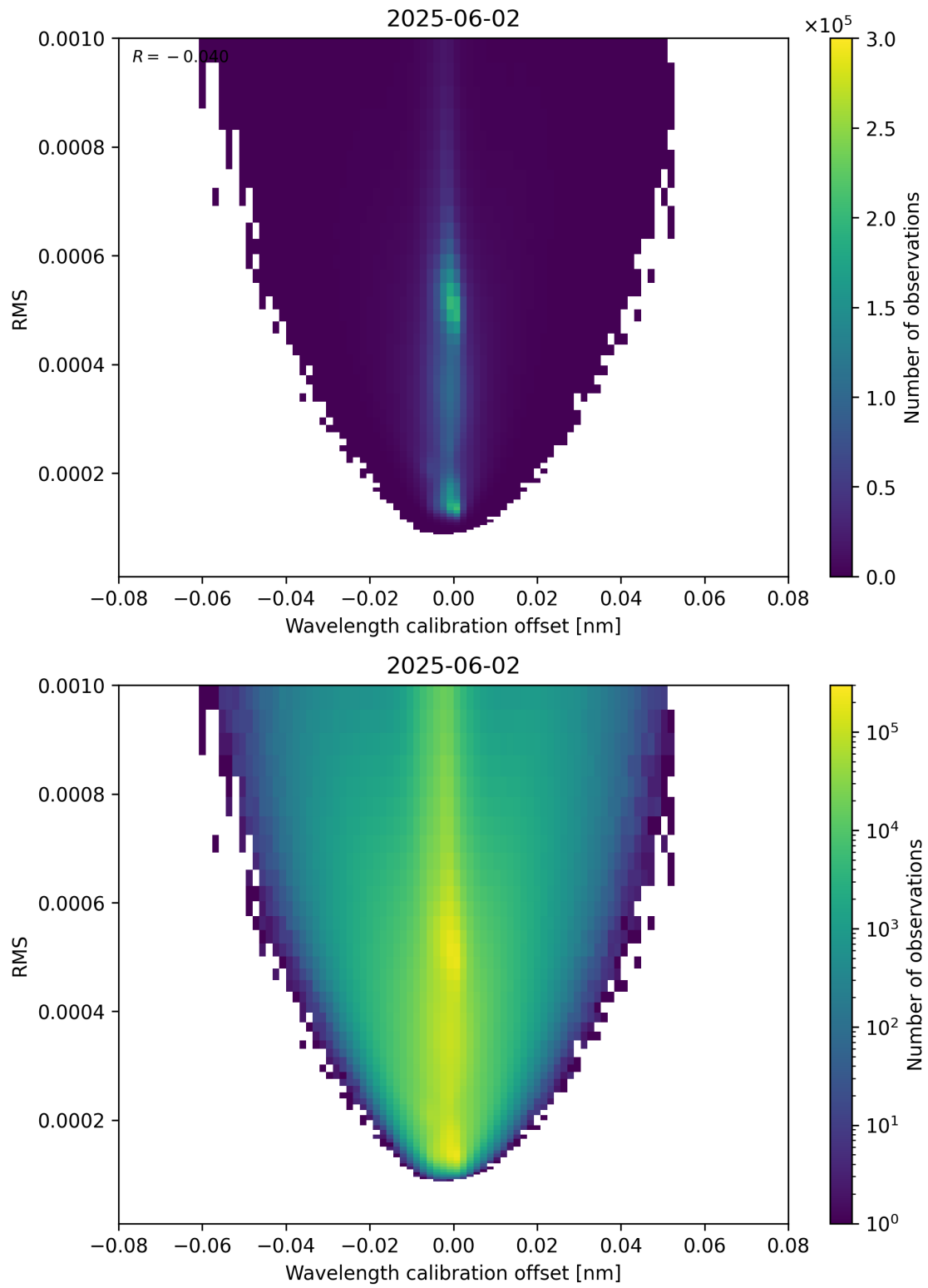
Figure 181: Scatter density plot of “Wavelength calibration offset” against “RMS” for 2025-06-01 to 2025-06-03.
