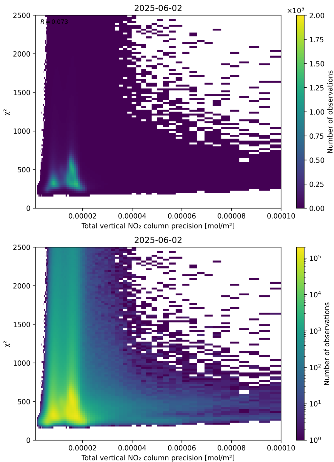
Figure 116: Scatter density plot of “Total vertical NO 2 column precision” against “ \chi^2 ” for 2025-06-01 to 2025-06-03.
