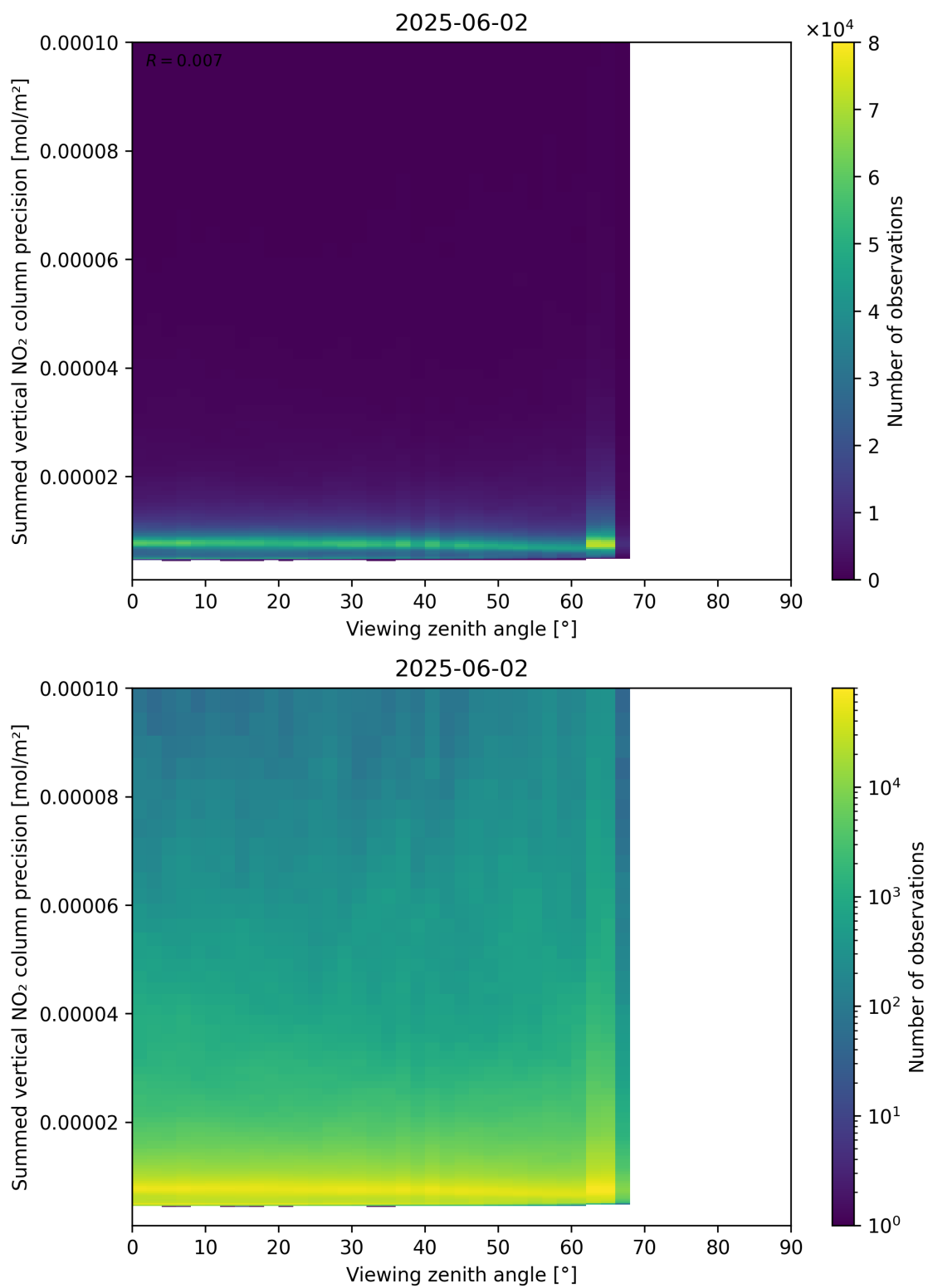
Figure 166: Scatter density plot of “Viewing zenith angle” against “Summed vertical NO 2 column precision” for 2025-06-01 to 2025-06-03.
