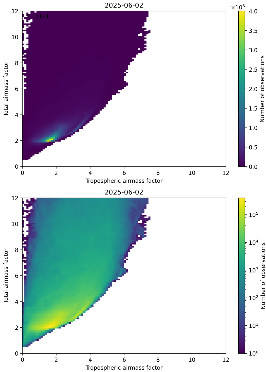
Figure 72: Scatter density plot of “Tropospheric airmass factor” against “Total airmass factor” for 2025-06-01 to 2025-06-03.
