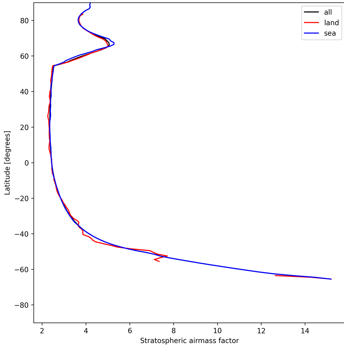
Figure 27: Zonal average of “Stratospheric air mass factor” for 2025-06-01 to 2025-06-03.
