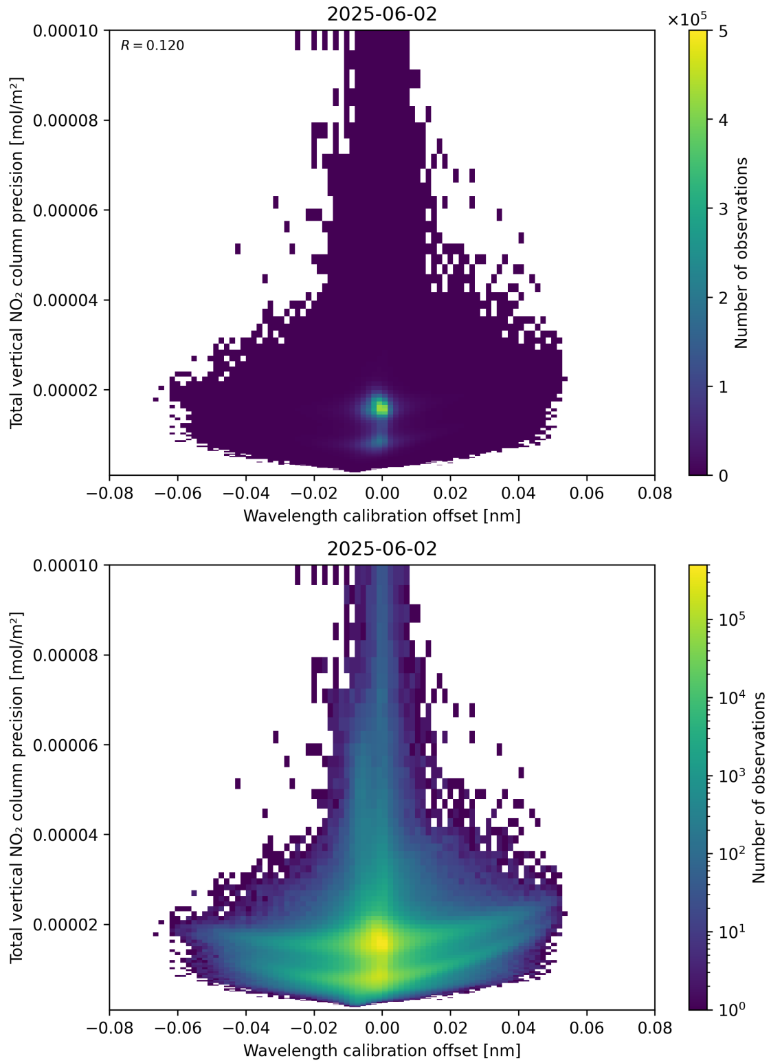
Figure 180: Scatter density plot of “Wavelength calibration offset” against “Total vertical NO 2 column precision” for 2025-06-01 to 2025-06-03.
