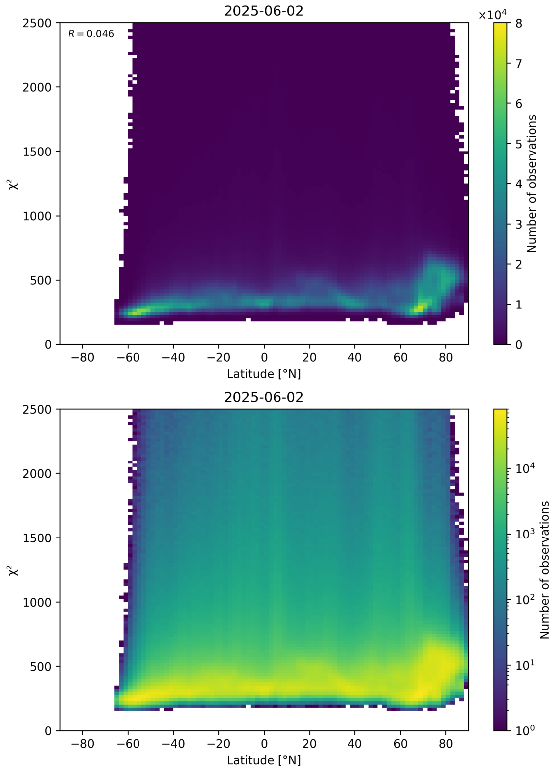
Figure 86: Scatter density plot of “Latitude” against “ \chi^2 ” for 2025-06-01 to 2025-06-03.
