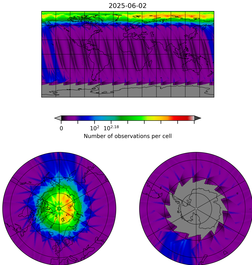
Figure 10: Map of the number of observations for 2025-06-01 to 2025-06-03
