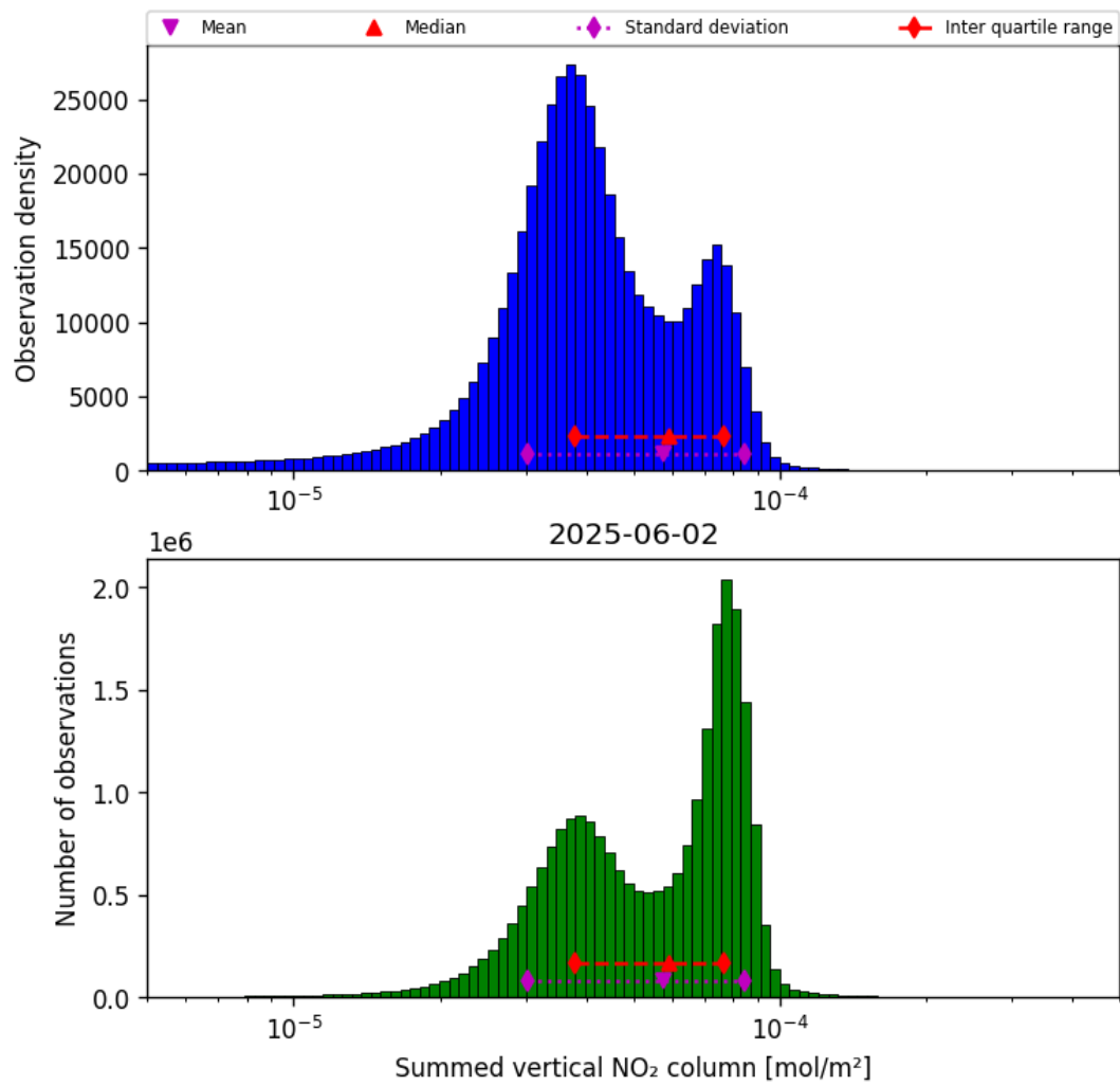
Figure 40: Histogram of “Summed vertical NO 2 column” for 2025-06-01 to 2025-06-03
