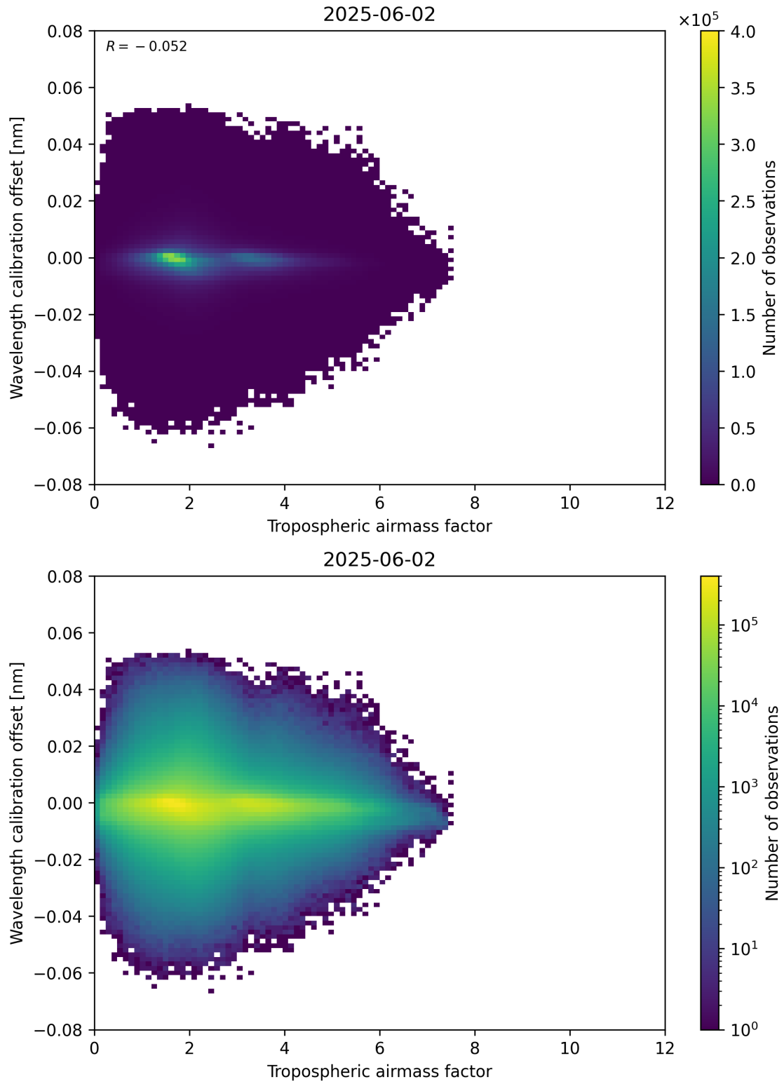
Figure 80: Scatter density plot of “Tropospheric airmass factor” against “Wavelength calibration offset” for 2025-06-01 to 2025-06-03.
