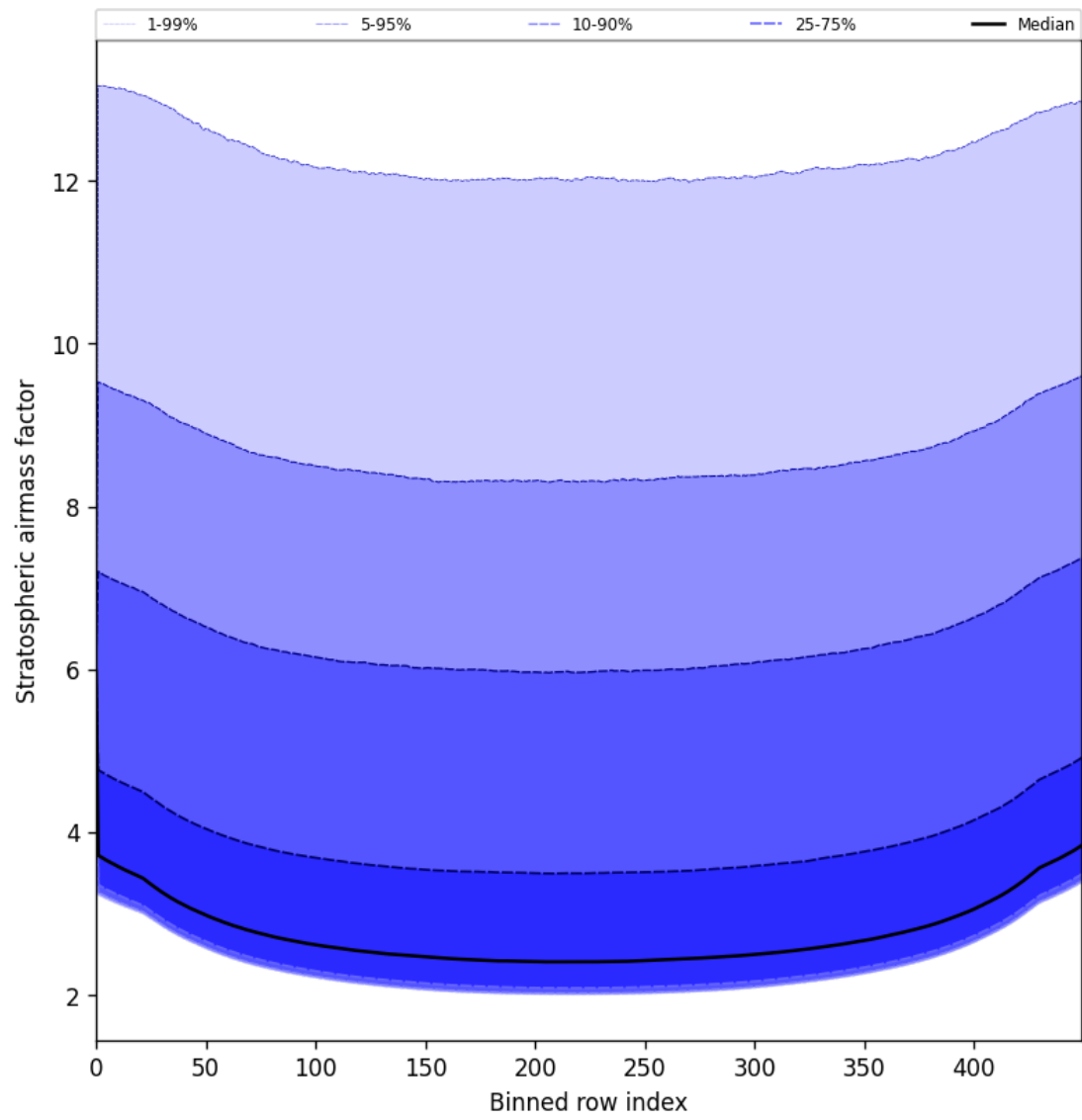
Figure 61: Along track statistics of “Stratospheric airmass factor” for 2025-06-01 to 2025-06-03
