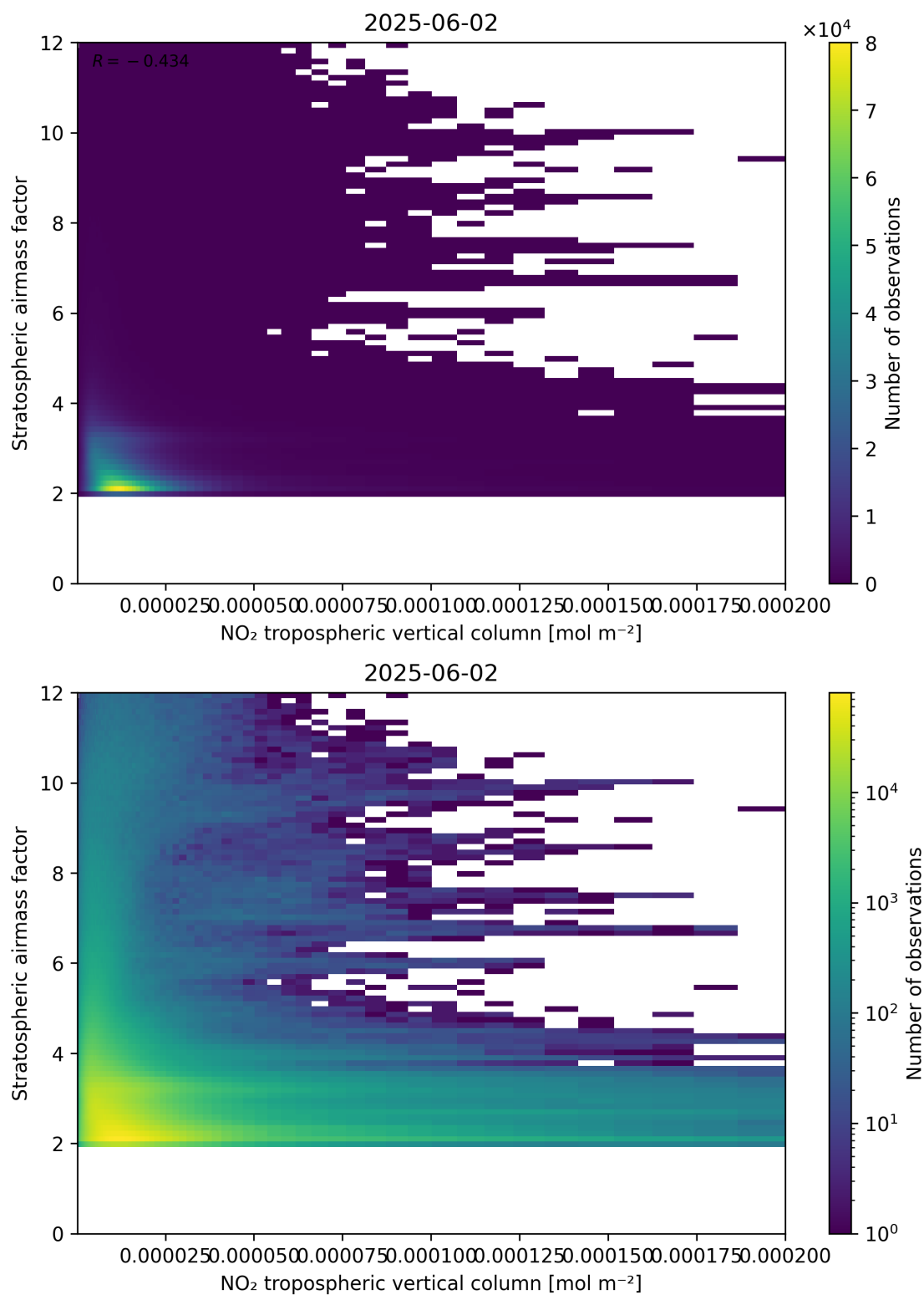
Figure 121: Scatter density plot of “NO 2 tropospheric vertical column” against “Stratospheric air mass factor” for 2025-06-01 to 2025-06-03.
