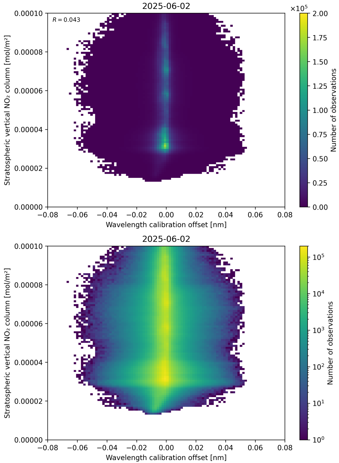
Figure 176: Scatter density plot of “Wavelength calibration offset” against “Stratospheric vertical NO 2 column” for 2025-06-01 to 2025-06-03.
