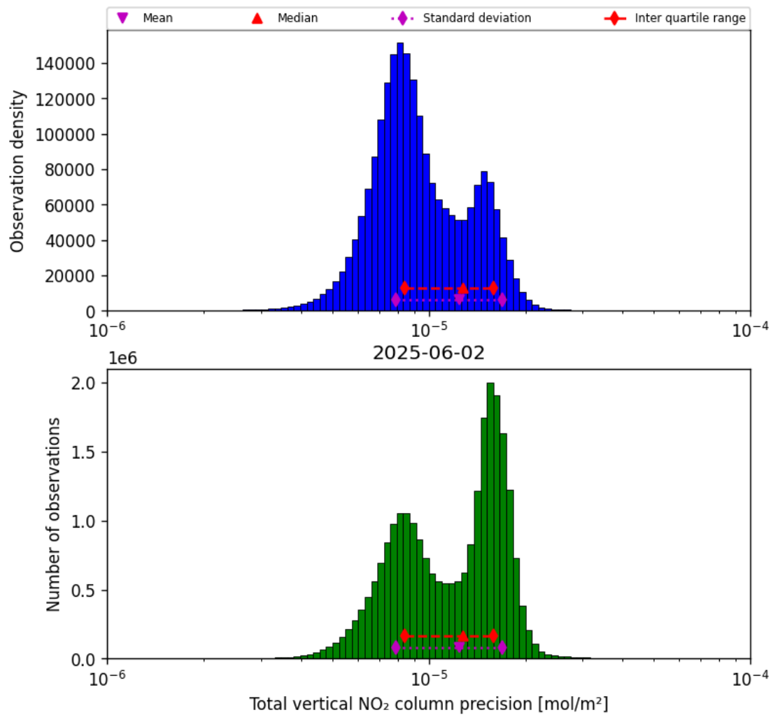
Figure 39: Histogram of “Total vertical NO 2 column precision” for 2025-06-01 to 2025-06-03
