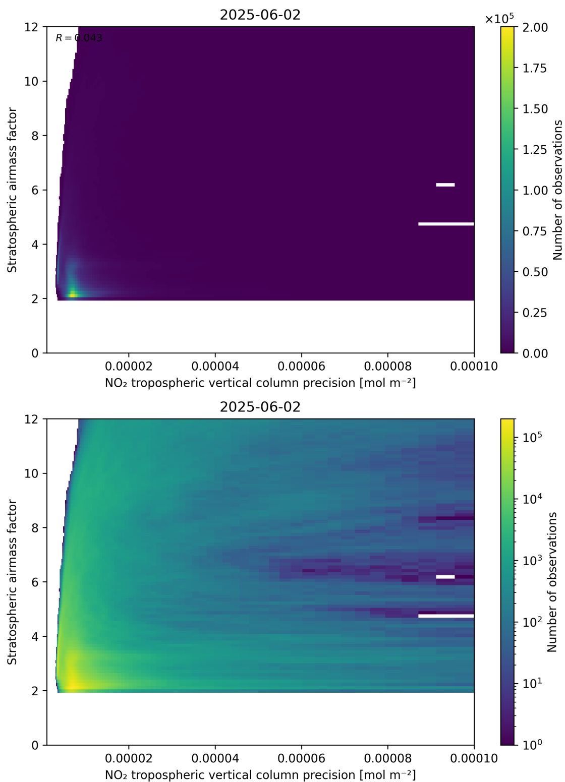
Figure 131: Scatter density plot of “NO 2 tropospheric vertical column precision” against “Stratospheric airmass factor” for 2025-06-01 to 2025-06-03.
