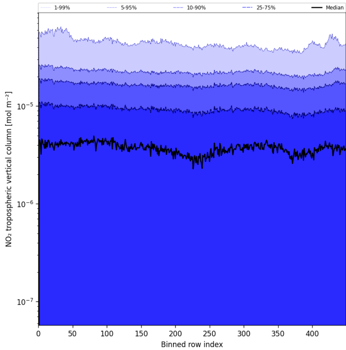
Figure 46: Along track statistics of “NO 2 tropospheric vertical column” for 2025-06-01 to 2025-06-03
