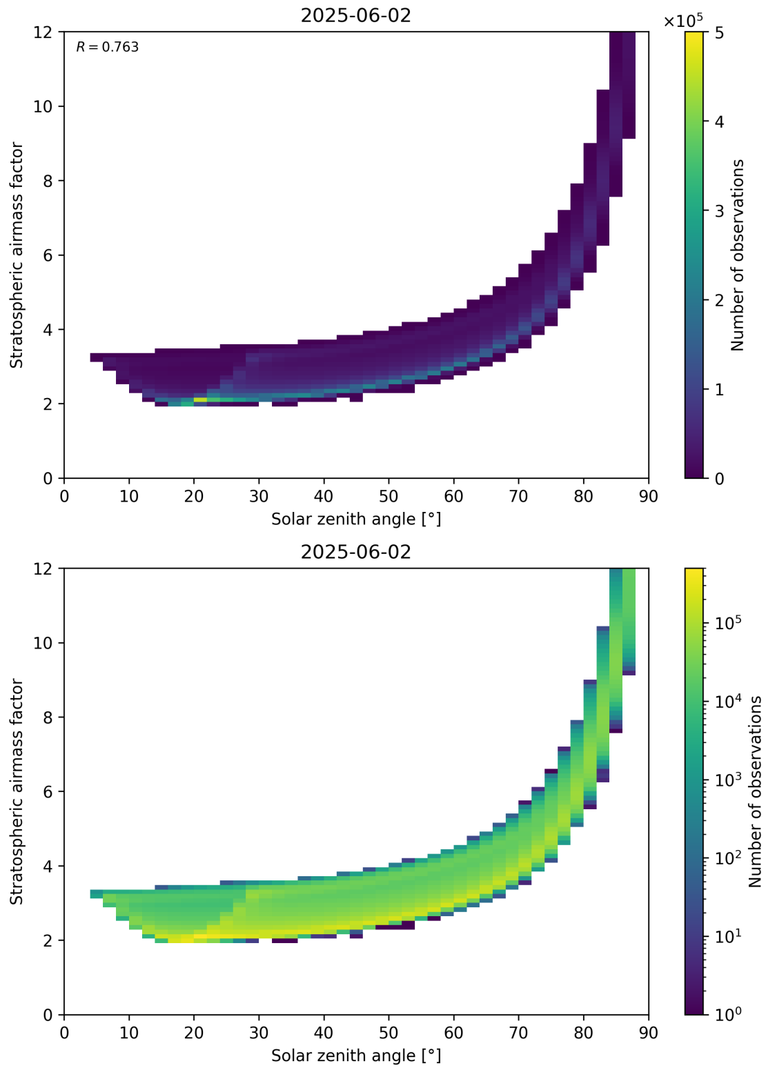
Figure 145: Scatter density plot of “Solar zenith angle” against “Stratospheric airmass factor” for 2025-06-01 to 2025-06-03.
