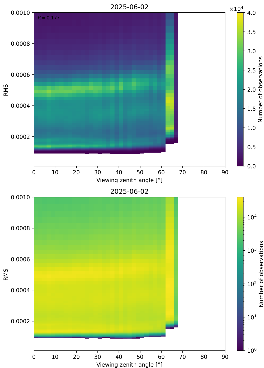
Figure 171: Scatter density plot of “Viewing zenith angle” against “RMS” for 2025-06-01 to 2025-06-03.
