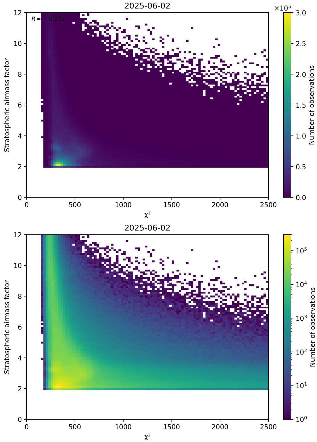
Figure 81: Scatter density plot of “ \chi^2 ” against “Stratospheric airmass factor” for 2025-06-01 to 2025-06-03.
