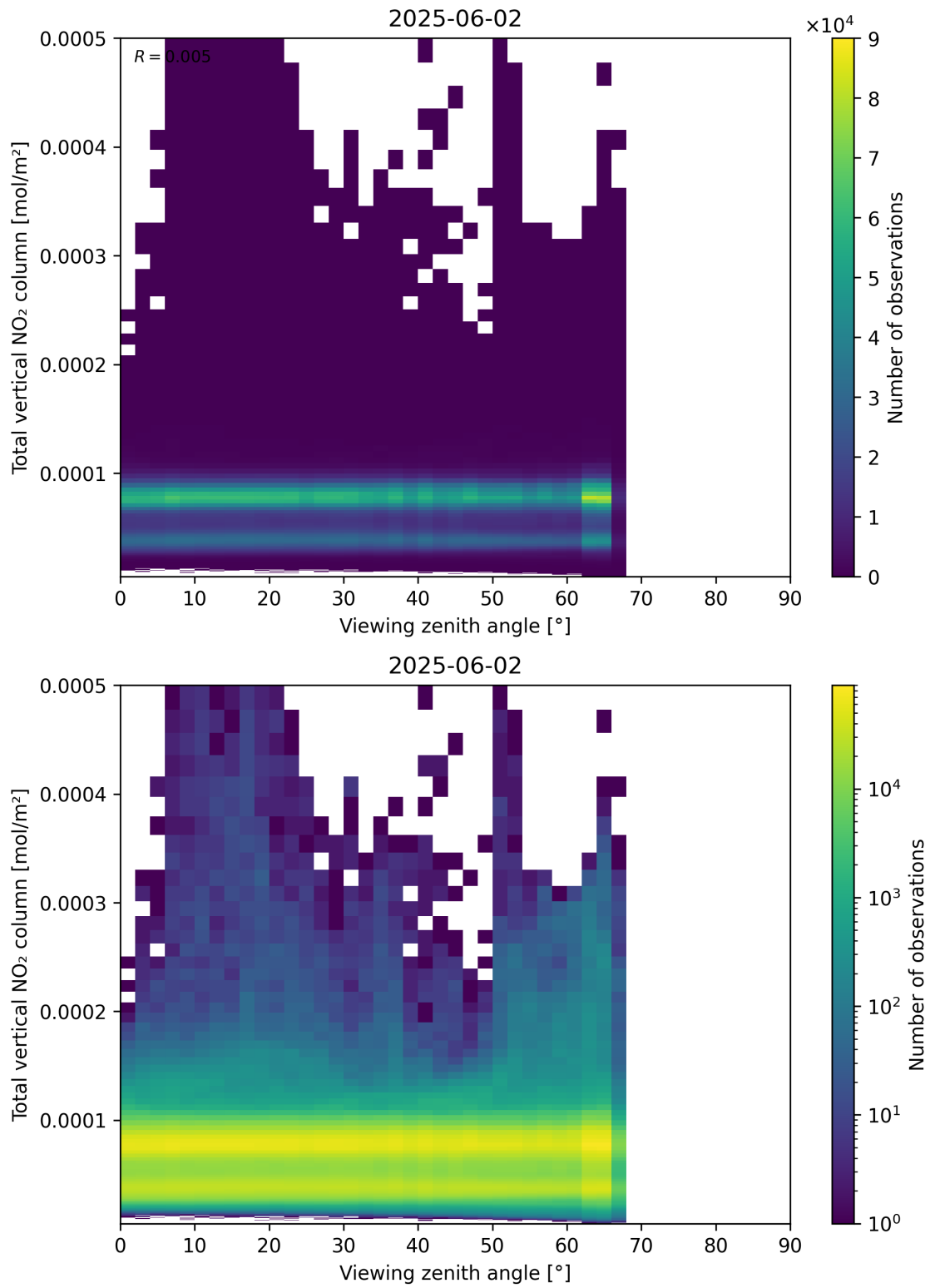
Figure 167: Scatter density plot of “Viewing zenith angle” against “Total vertical NO 2 column” for 2025-06-01 to 2025-06-03.
