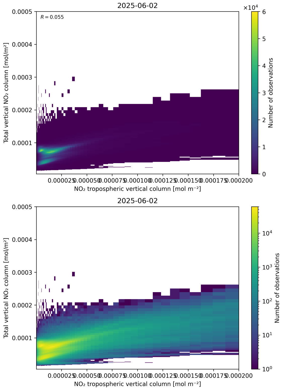
Figure 128: Scatter density plot of “NO 2 tropospheric vertical column” against “Total vertical NO 2 column” for 2025-06-01 to 2025-06-03.
