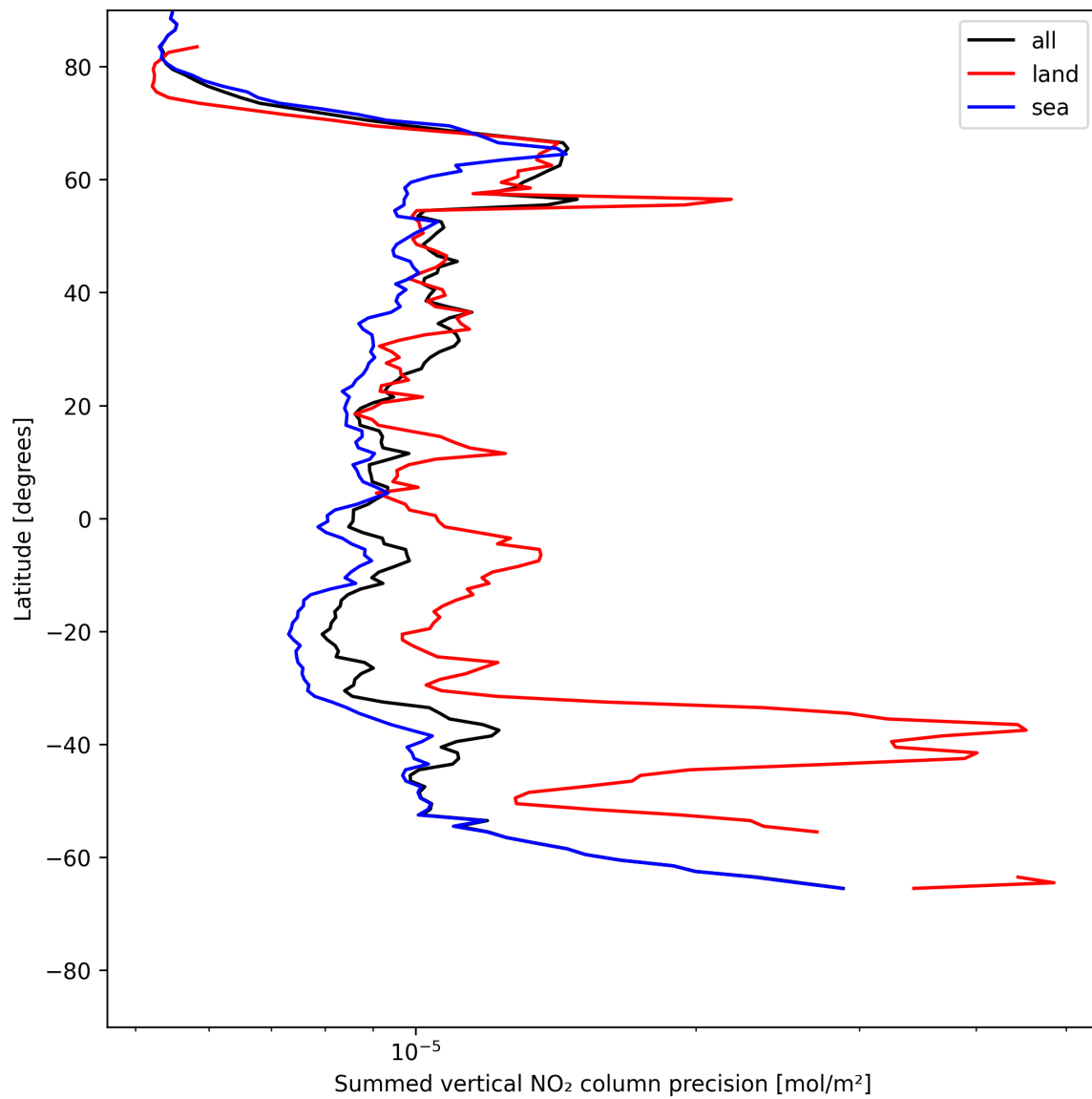
Figure 24: Zonal average of “Summed vertical NO 2 column precision” for 2025-06-01 to 2025-06-03.
