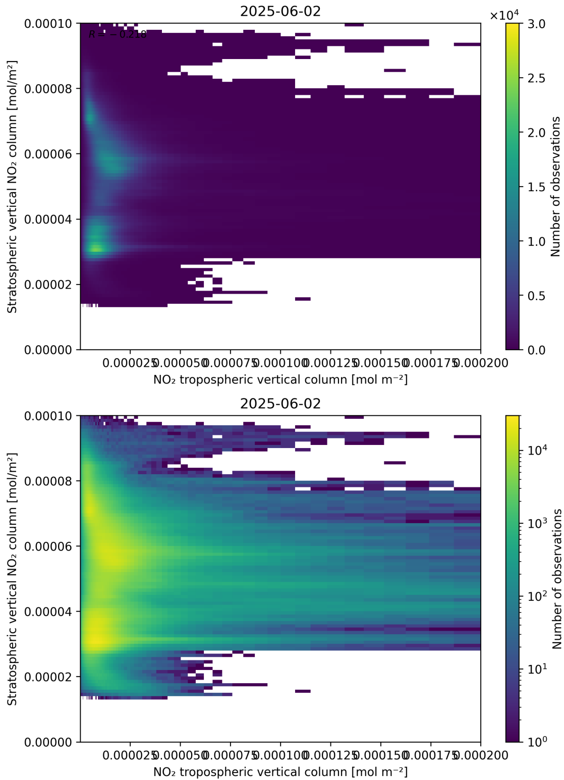
Figure 125: Scatter density plot of “NO 2 tropospheric vertical column” against “Stratospheric vertical NO 2 column” for 2025-06-01 to 2025-06-03.
