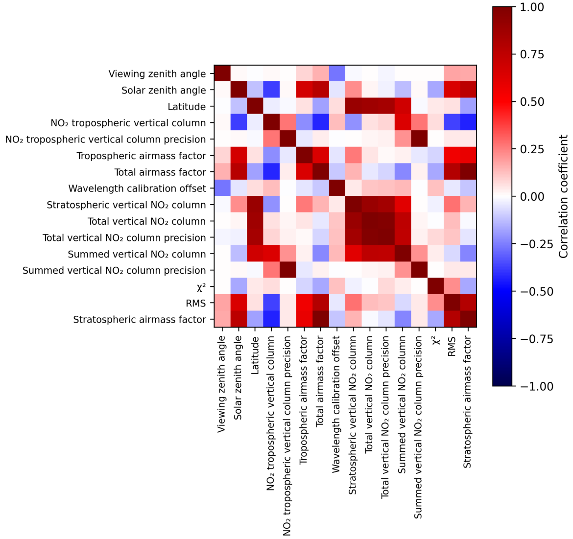
Figure 2: Map of correlation matrix for 2025-06-01 to 2025-06-03.
