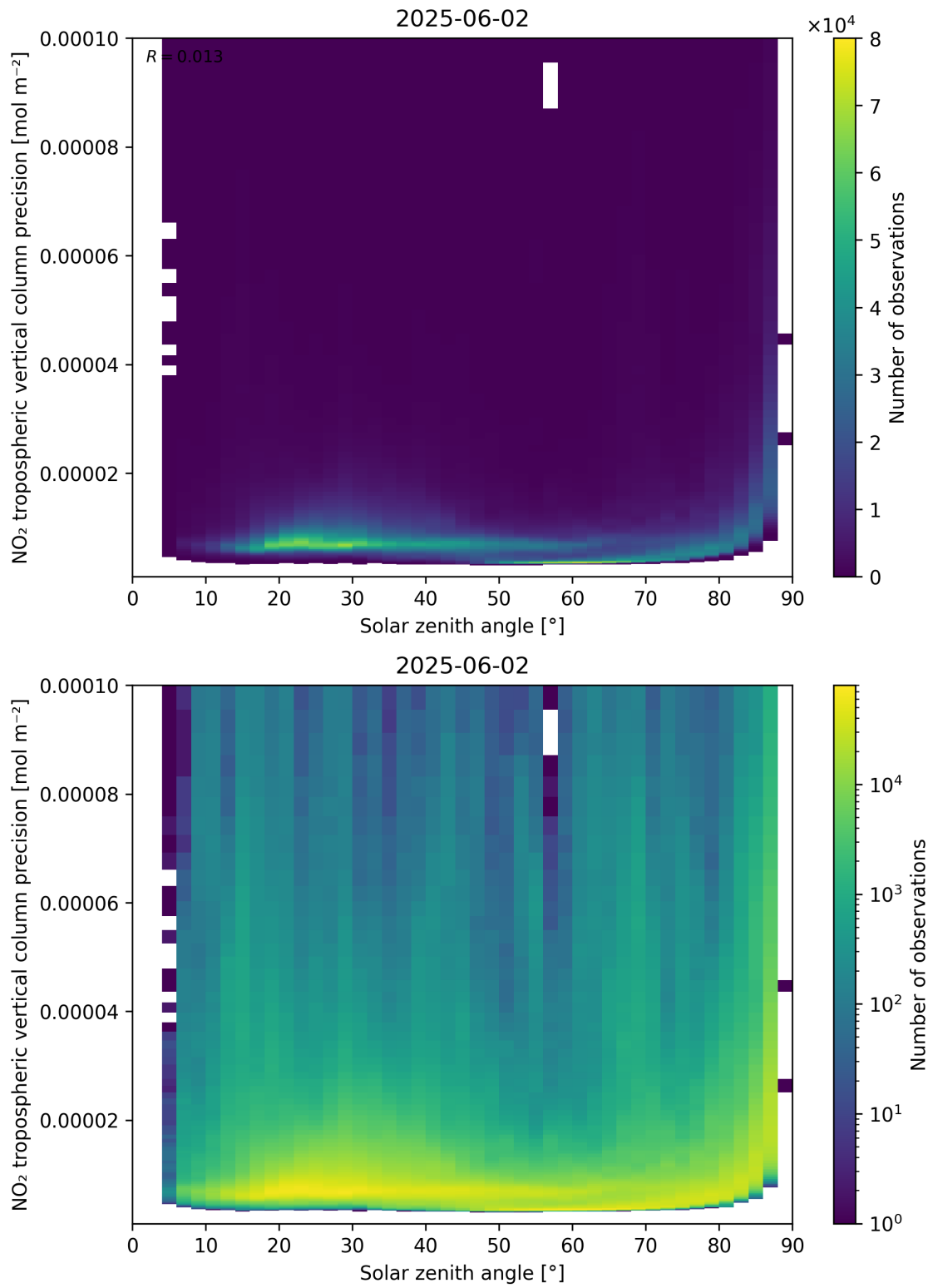
Figure 156: Scatter density plot of “Solar zenith angle” against “NO 2 tropospheric vertical column precision” for 2025-06-01 to 2025-06-03.
