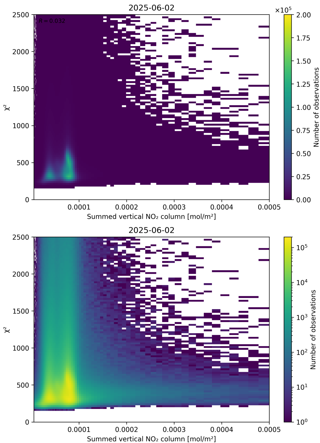
Figure 104: Scatter density plot of “Summed vertical NO 2 column” against “ \chi^2 ” for 2025-06-01 to 2025-06-03.
