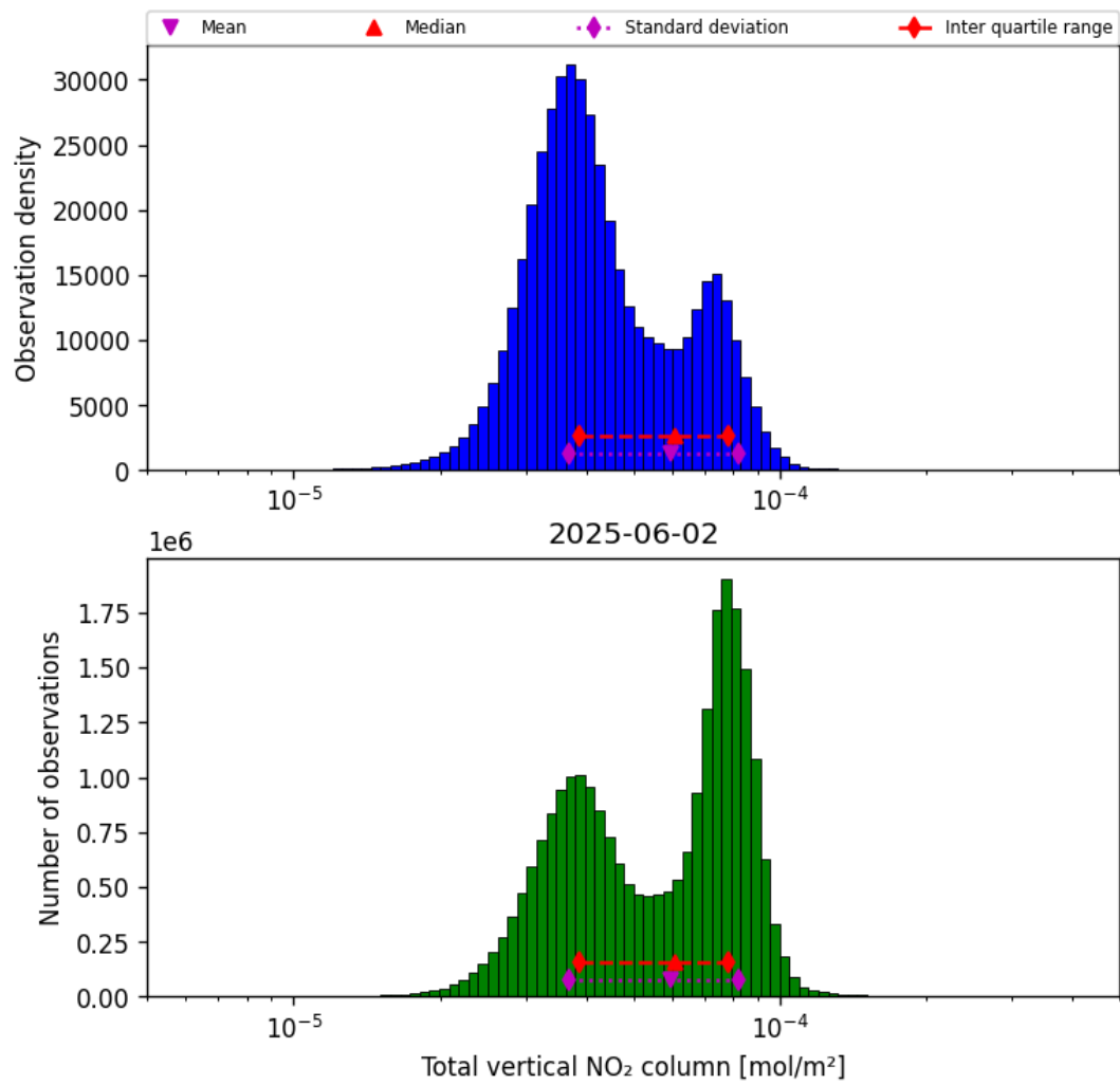
Figure 38: Histogram of “Total vertical NO 2 column” for 2025-06-01 to 2025-06-03
