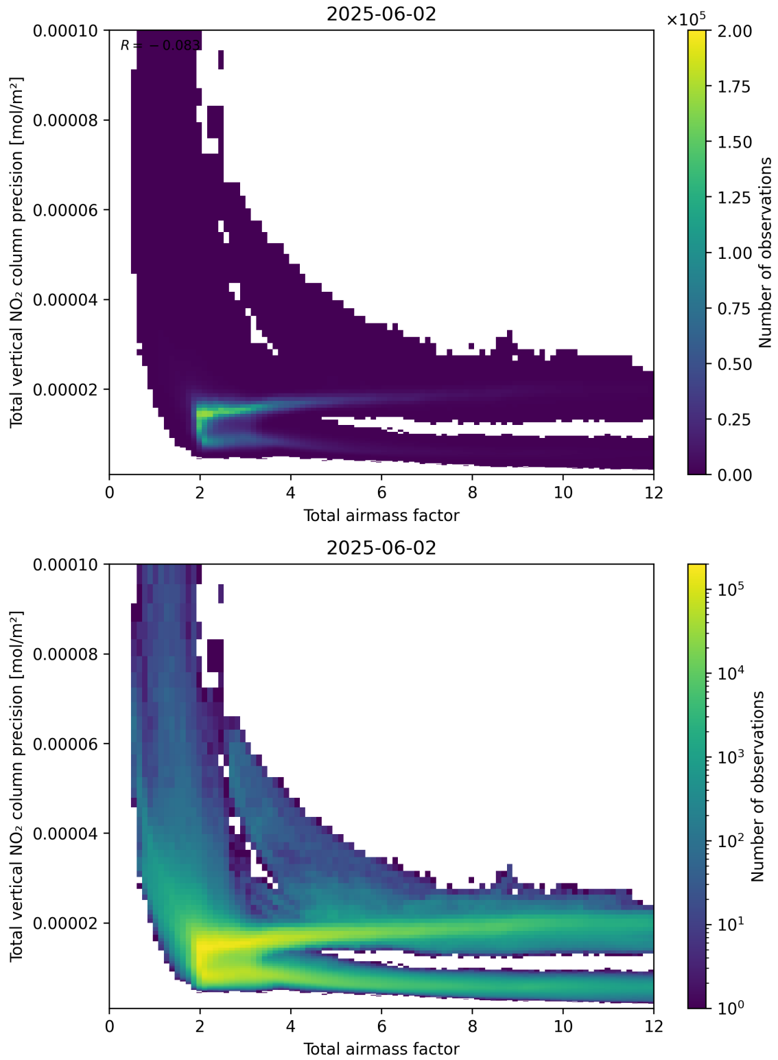
Figure 68: Scatter density plot of “Total airmass factor” against “Total vertical NO 2 column precision” for 2025-06-01 to 2025-06-03.
