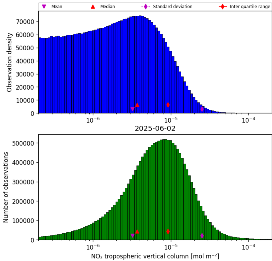
Figure 29: Histogram of “NO 2 tropospheric vertical column” for 2025-06-01 to 2025-06-03
