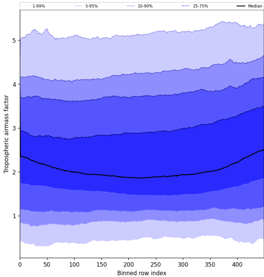
Figure 48: Along track statistics of “Tropospheric airmass factor” for 2025-06-01 to 2025-06-03
