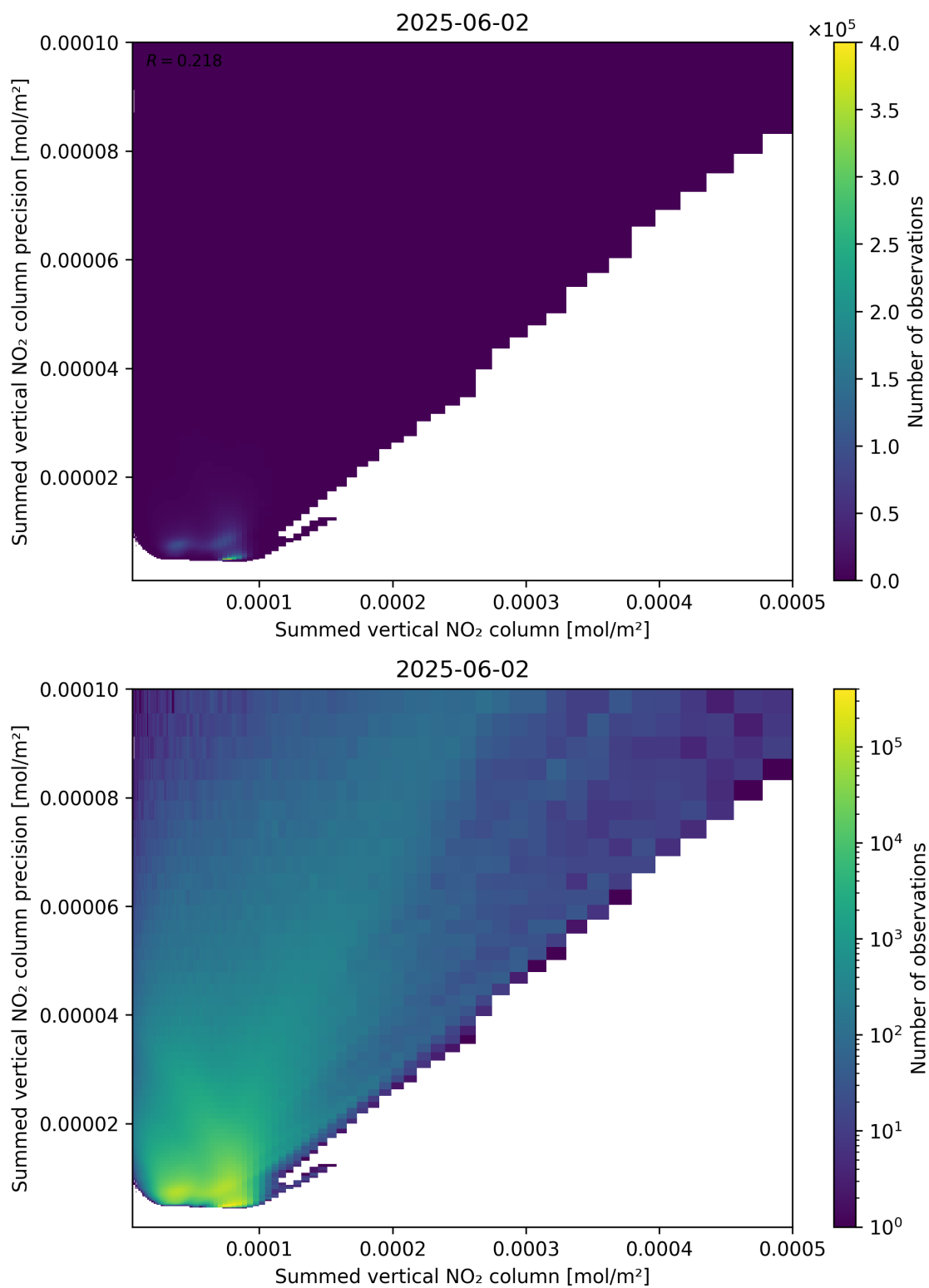
Figure 105: Scatter density plot of “Summed vertical NO 2 column” against “Summed vertical NO 2 column precision” for 2025-06-01 to 2025-06-03.
