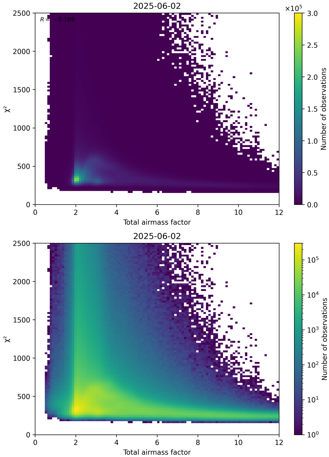
Figure 63: Scatter density plot of “Total airmass factor” against “ \chi^2 ” for 2025-06-01 to 2025-06-03.
