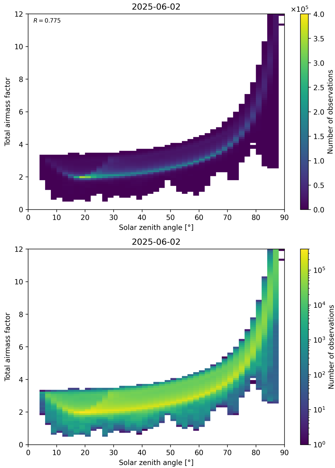
Figure 146: Scatter density plot of “Solar zenith angle” against “Total air mass factor” for 2025-06-01 to 2025-06-03.
