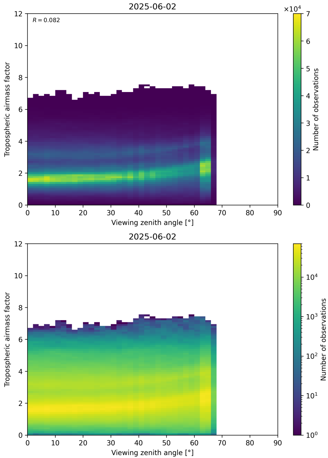
Figure 161: Scatter density plot of “Viewing zenith angle” against “Tropospheric airmass factor” for 2025-06-01 to 2025-06-03.
