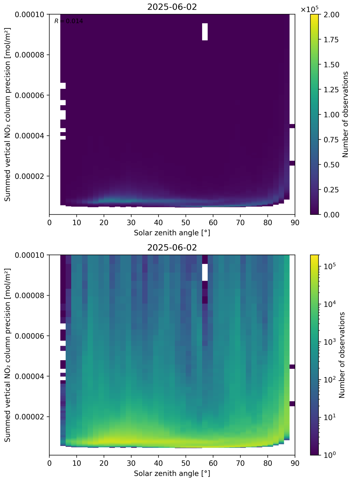
Figure 152: Scatter density plot of “Solar zenith angle” against “Summed vertical NO 2 column precision” for 2025-06-01 to 2025-06-03.
