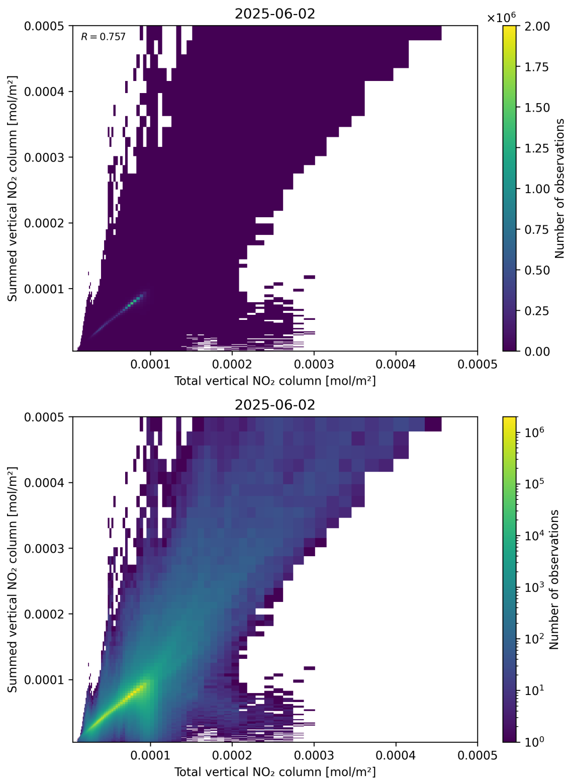
Figure 112: Scatter density plot of “Total vertical NO 2 column” against “Summed vertical NO 2 column” for 2025-06-01 to 2025-06-03.
