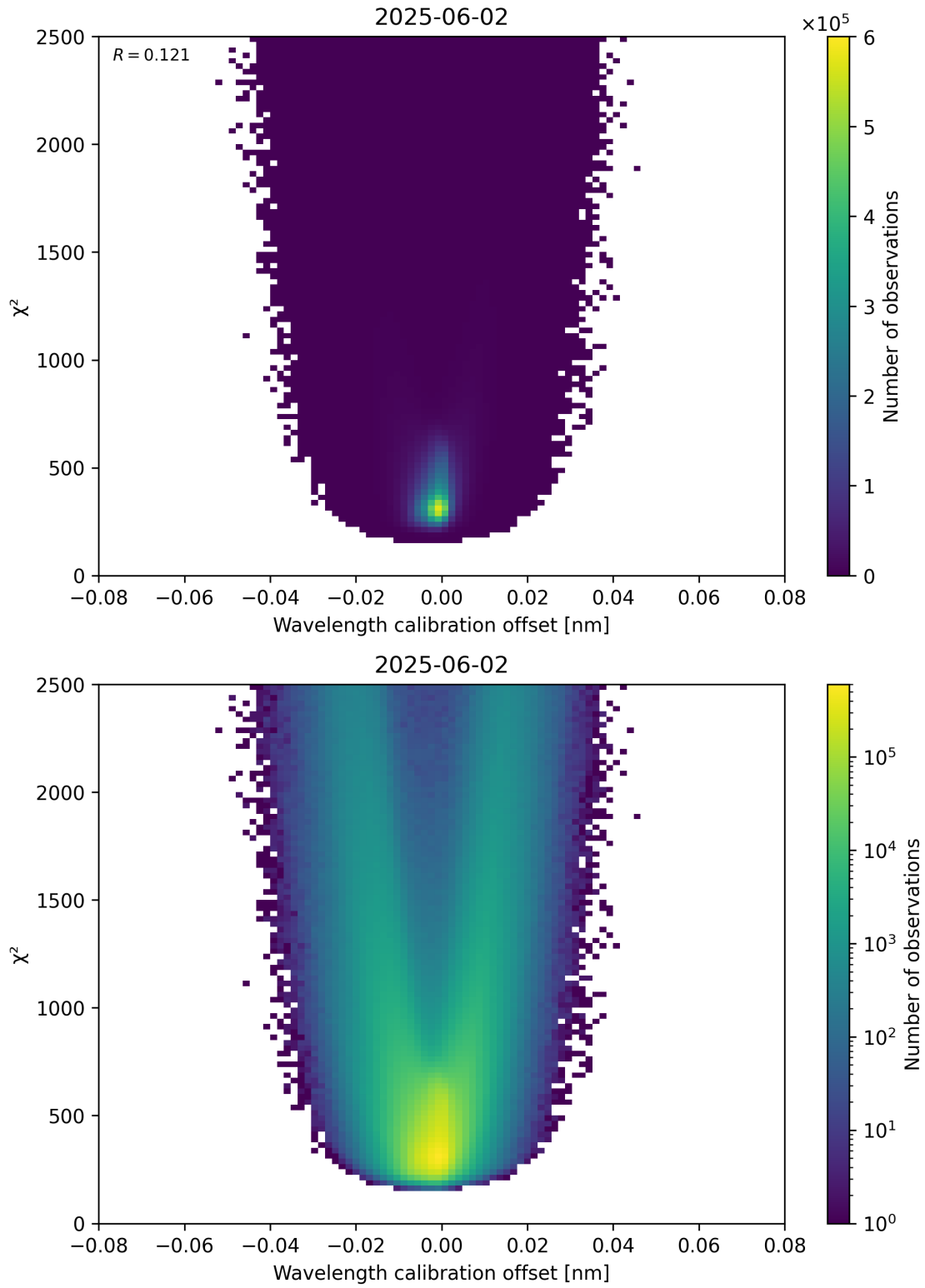
Figure 175: Scatter density plot of “Wavelength calibration offset” against “ \chi^2 ” for 2025-06-01 to 2025-06-03.
