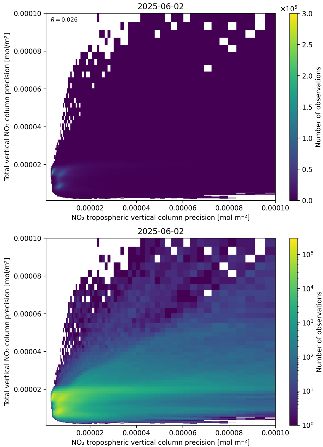
Figure 139: Scatter density plot of “NO 2 tropospheric vertical column precision” against “Total vertical NO 2 column precision” for 2025-06-01 to 2025-06-03.
