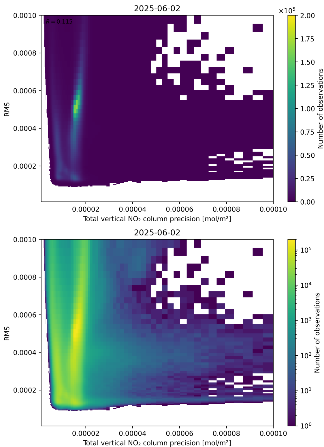
Figure 119: Scatter density plot of “Total vertical NO 2 column precision” against “RMS” for 2025-06-01 to 2025-06-03.
