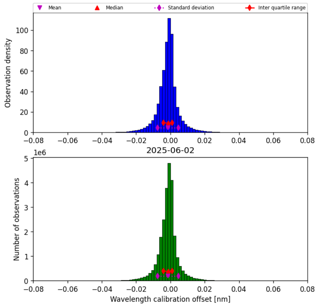
Figure 35: Histogram of “Wavelength calibration offset” for 2025-06-01 to 2025-06-03
