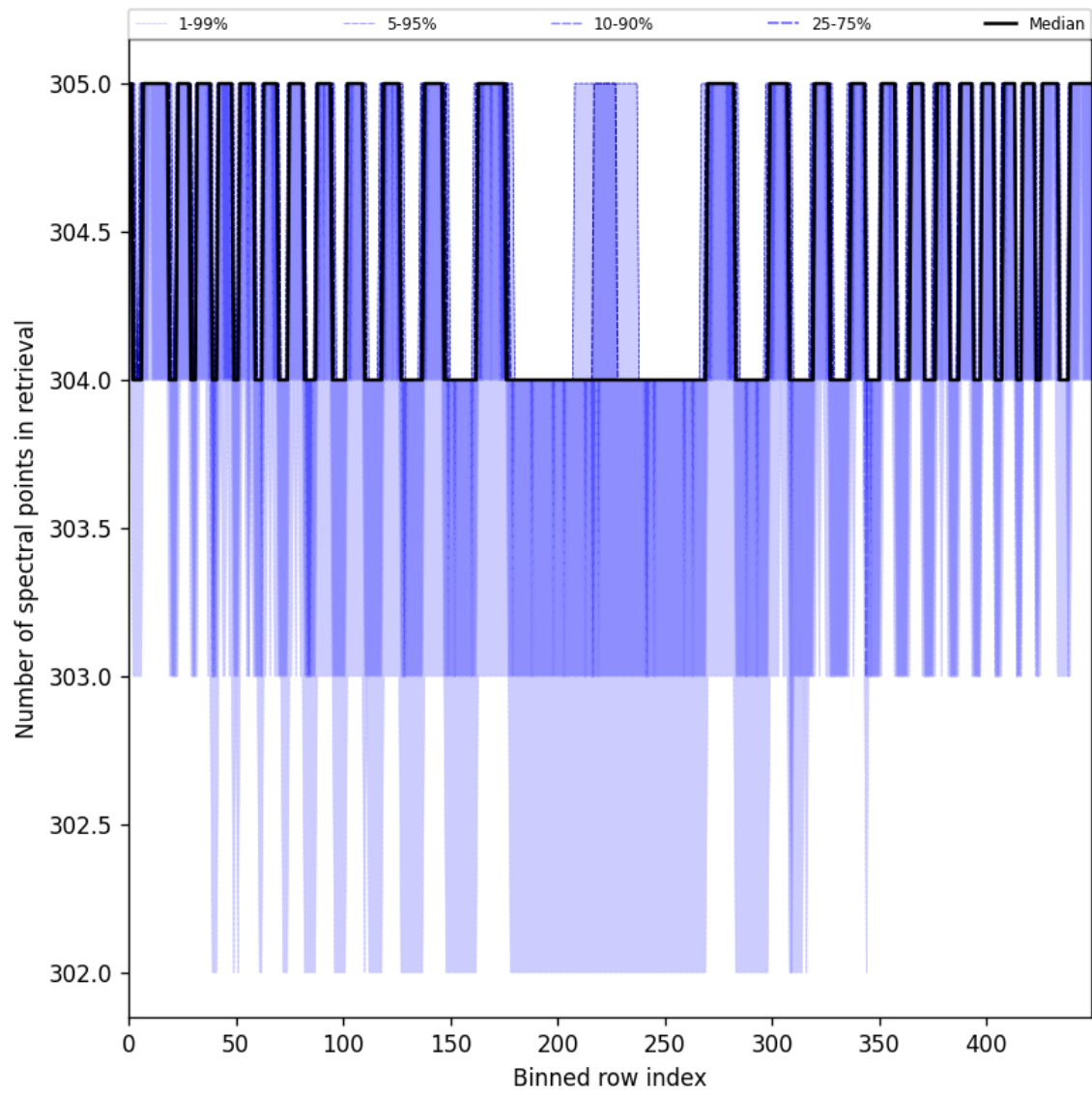
Figure 50: Along track statistics of “Number of spectral points in retrieval” for 2025-06-01 to 2025-06-03
