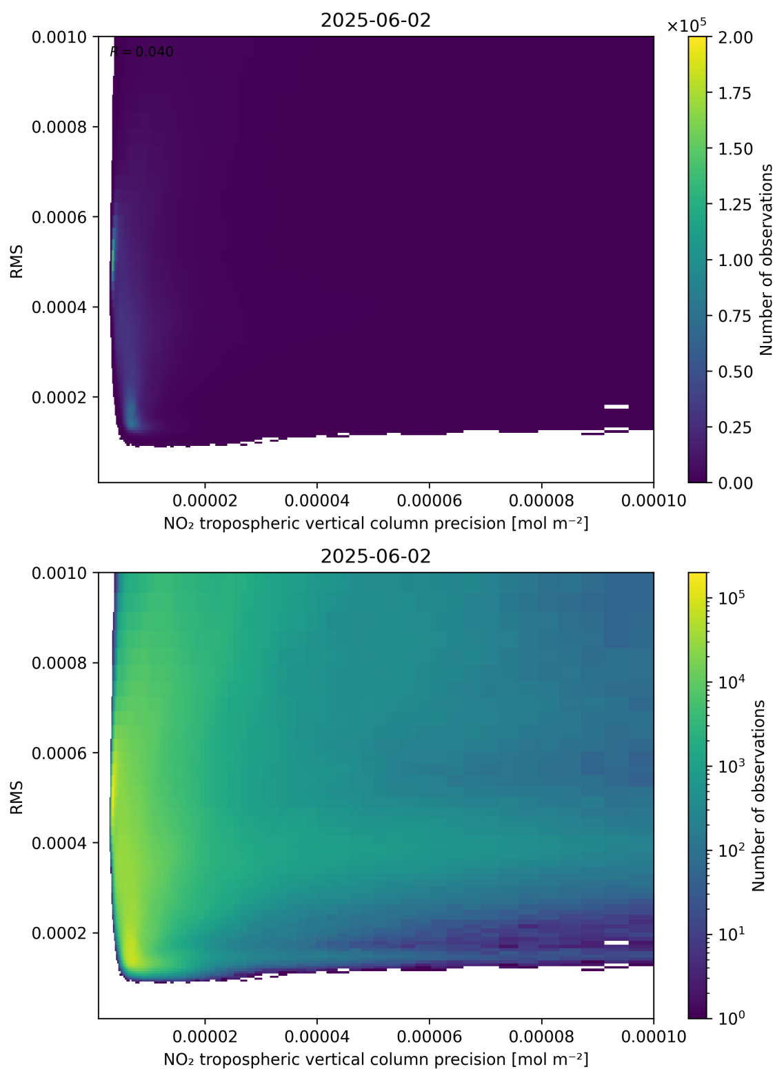
Figure 140: Scatter density plot of “NO 2 tropospheric vertical column precision” against “RMS” for 2025-06-01 to 2025-06-03.
