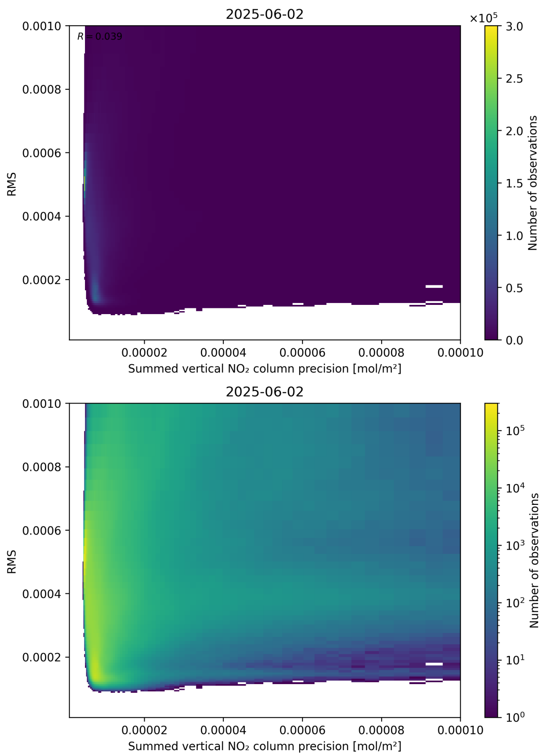
Figure 108: Scatter density plot of “Summed vertical NO 2 column precision” against “RMS” for 2025-06-01 to 2025-06-03.
