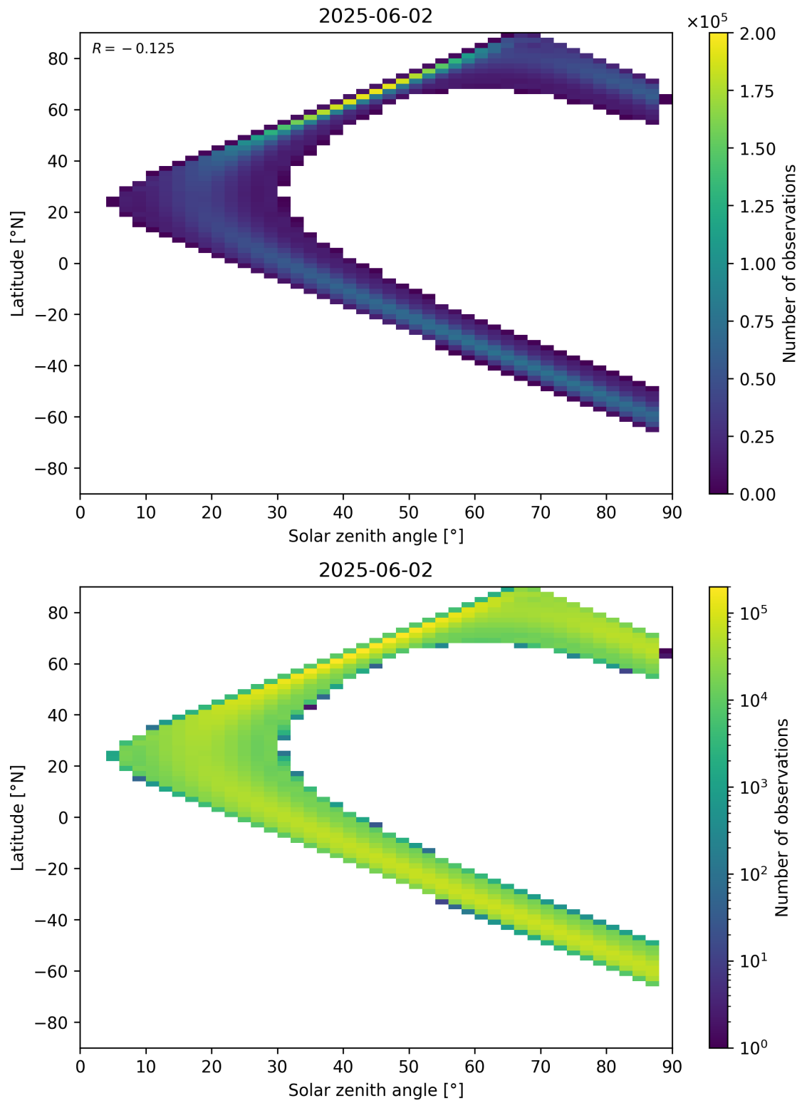
Figure 149: Scatter density plot of “Solar zenith angle” against “Latitude” for 2025-06-01 to 2025-06-03.
