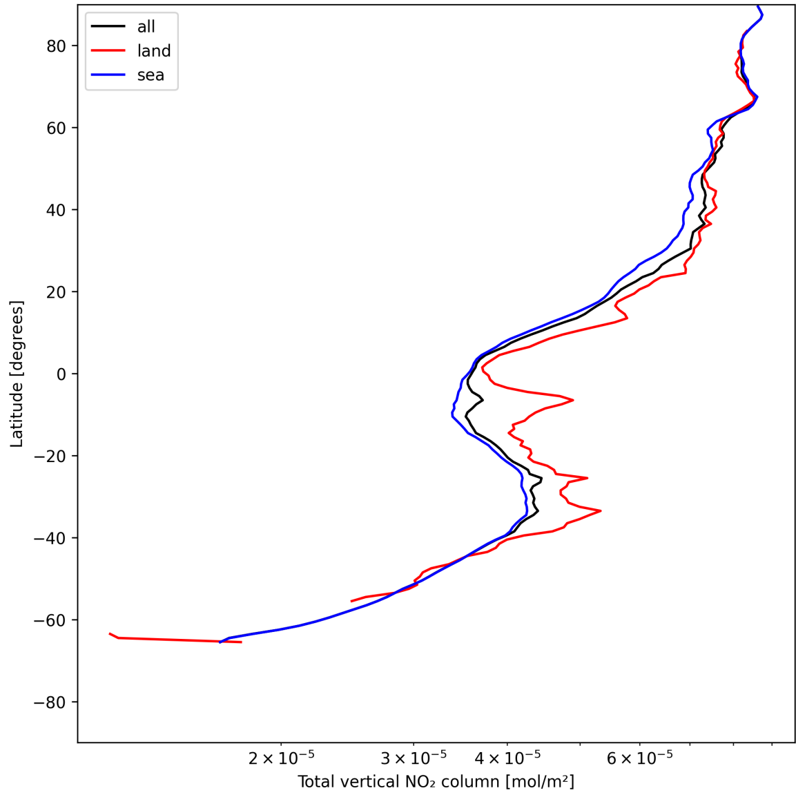
Figure 21: Zonal average of “Total vertical NO 2 column” for 2025-06-01 to 2025-06-03.
