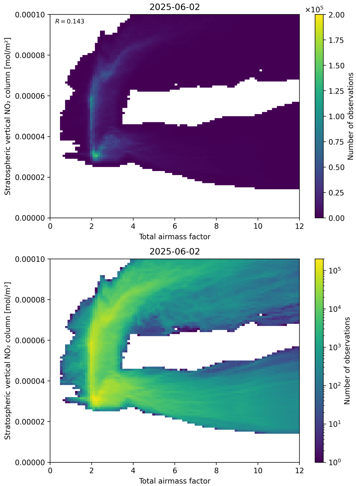
Figure 64: Scatter density plot of “Total airmass factor” against “Stratospheric vertical NO 2 column” for 2025-06-01 to 2025-06-03.
