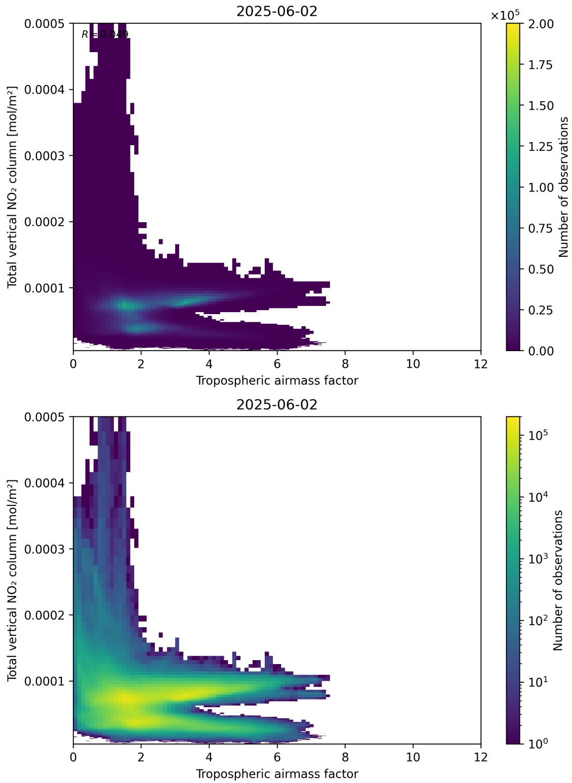
Figure 77: Scatter density plot of “Tropospheric airmass factor” against “Total vertical NO 2 column” for 2025-06-01 to 2025-06-03.
