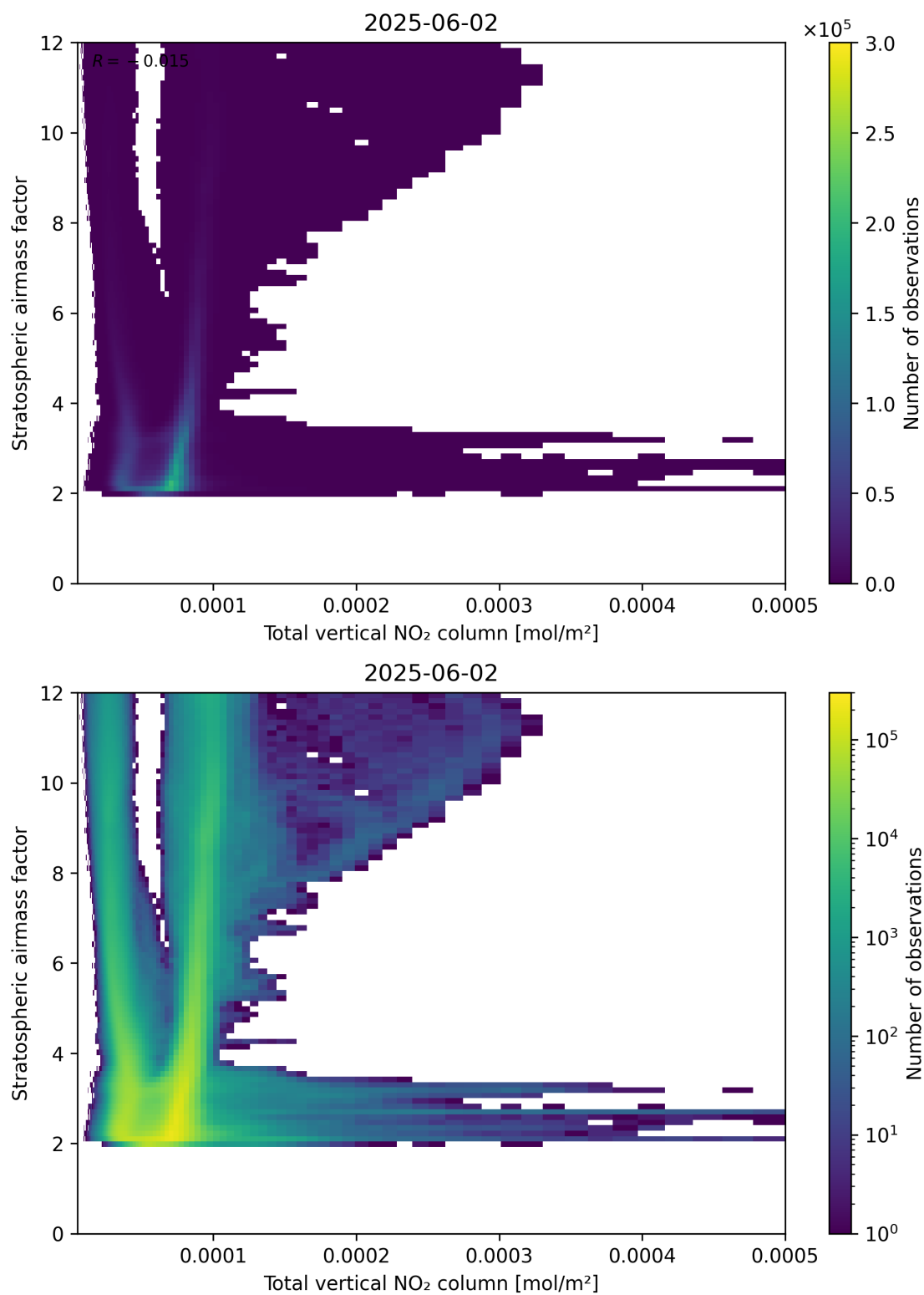
Figure 110: Scatter density plot of “Total vertical NO 2 column” against “Stratospheric airmass factor” for 2025-06-01 to 2025-06-03.
