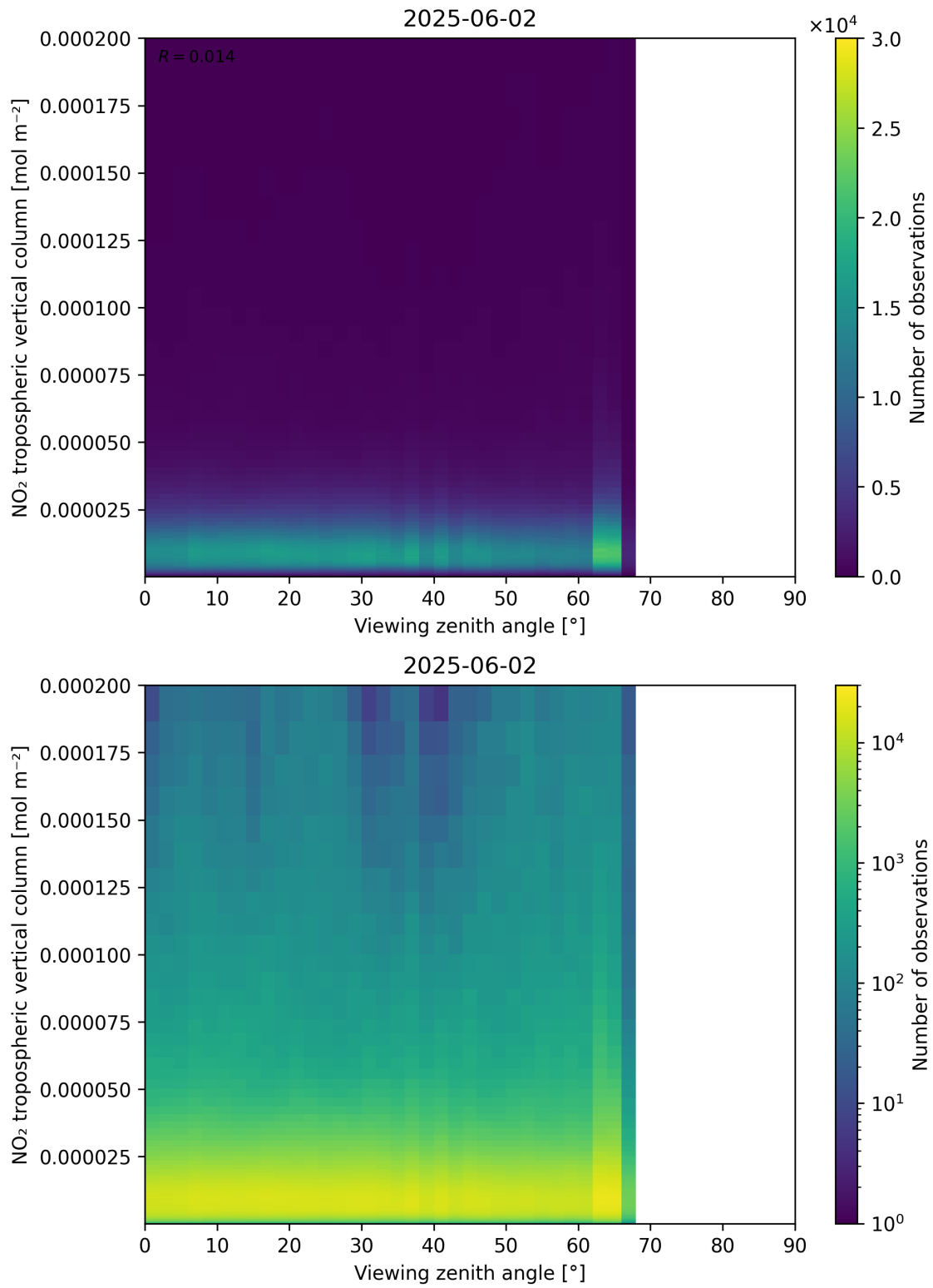
Figure 169: Scatter density plot of “Viewing zenith angle” against “NO 2 tropospheric vertical column” for 2025-06-01 to 2025-06-03.
