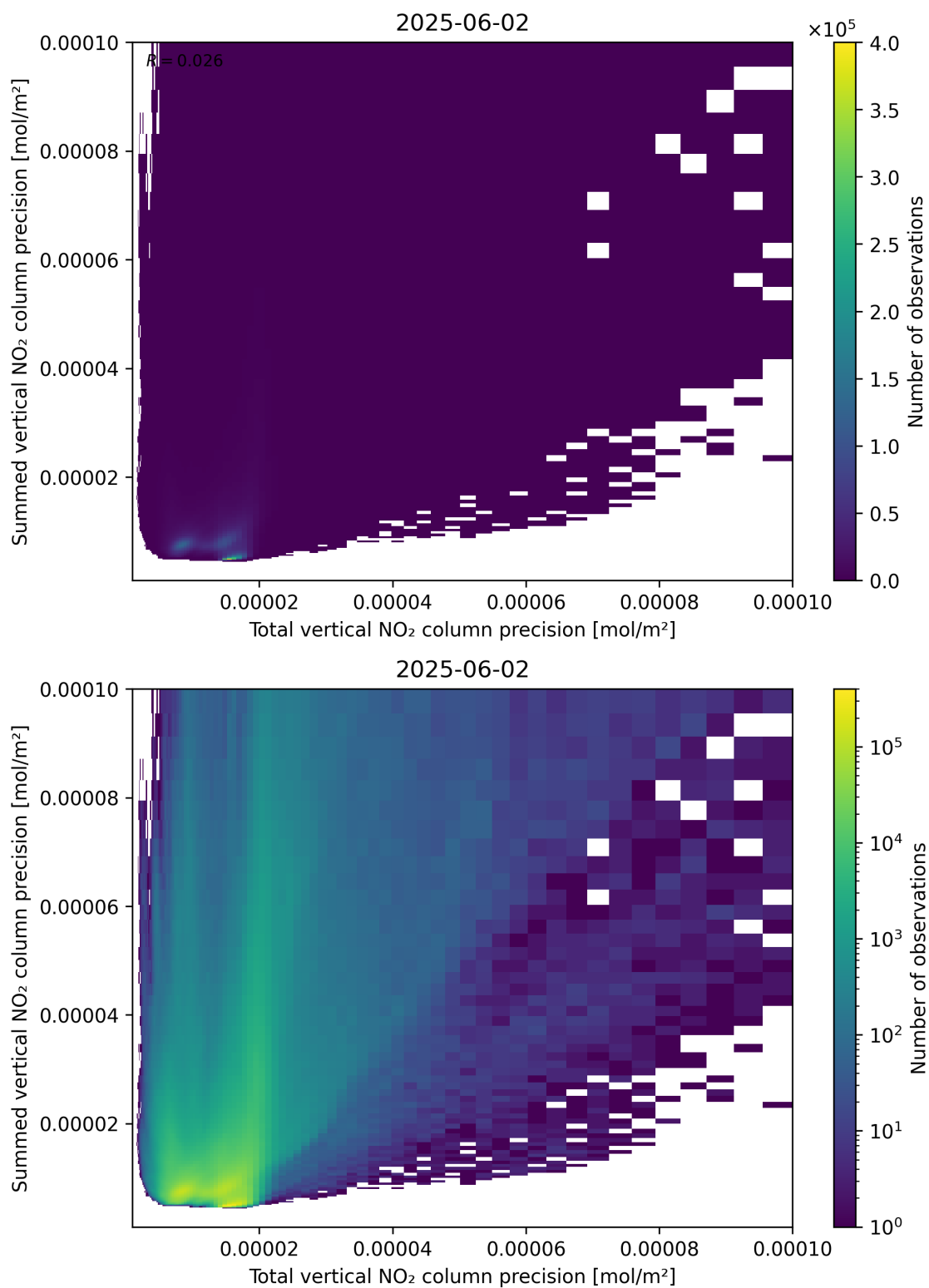
Figure 118: Scatter density plot of “Total vertical NO 2 column precision” against “Summed vertical NO 2 column precision” for 2025-06-01 to 2025-06-03.
