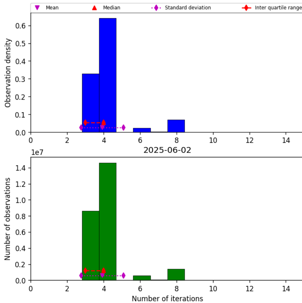
Figure 34: Histogram of “Number of iterations” for 2025-06-01 to 2025-06-03
