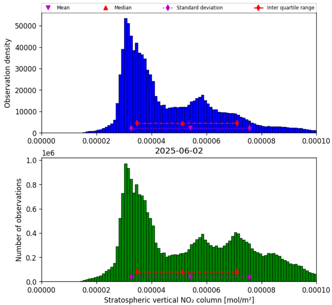
Figure 36: Histogram of “Stratospheric vertical NO 2 column” for 2025-06-01 to 2025-06-03
