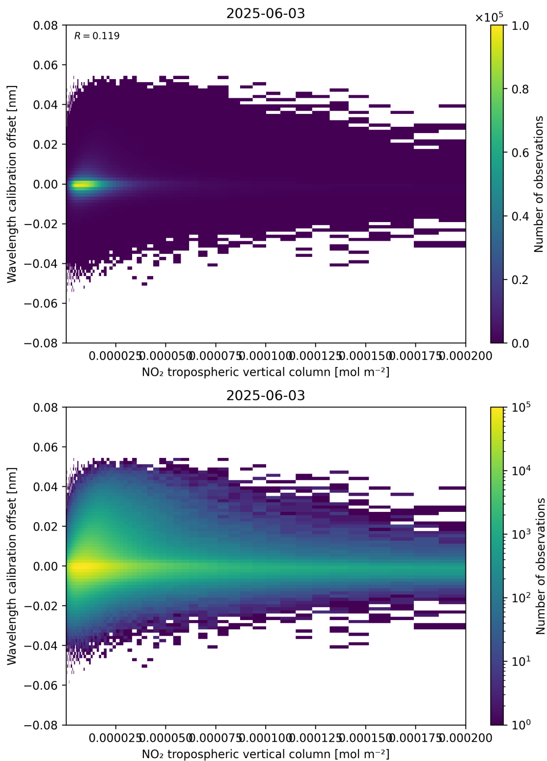
Figure 143: Scatter density plot of “NO 2 tropospheric vertical column” against “Wavelength calibration offset” for 2025-06-02 to 2025-06-04.
