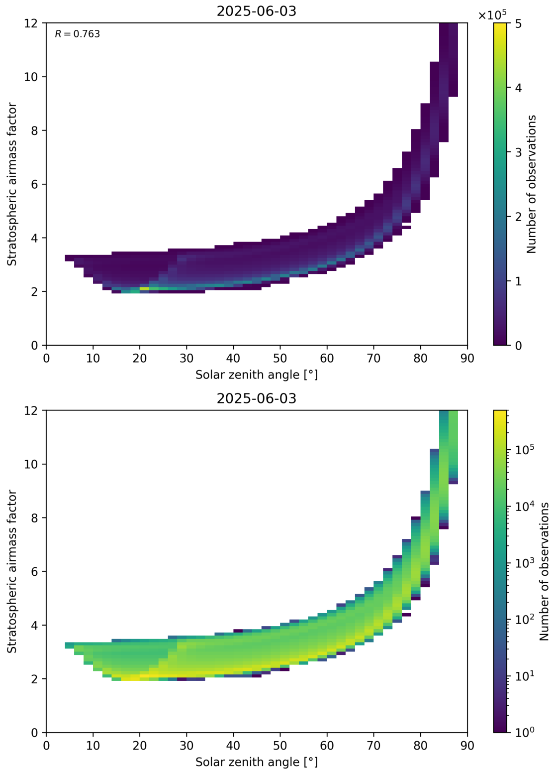
Figure 145: Scatter density plot of “Solar zenith angle” against “Stratospheric airmass factor” for 2025-06-02 to 2025-06-04.
