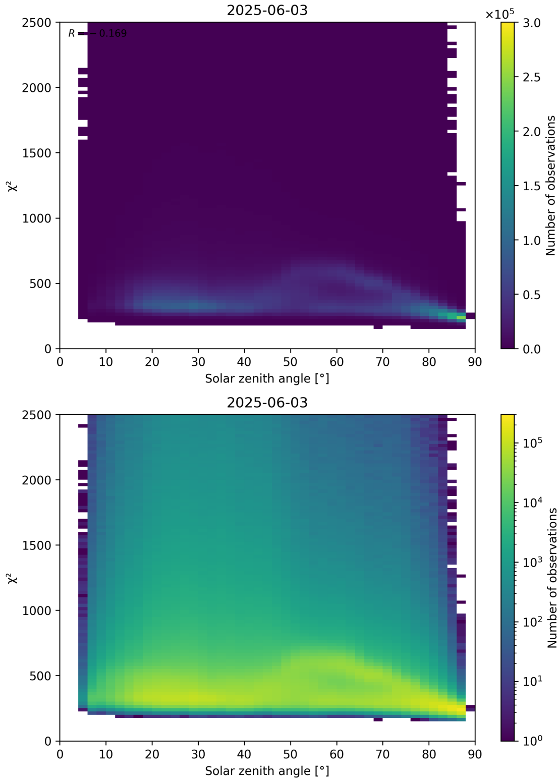
Figure 148: Scatter density plot of “Solar zenith angle” against “ \chi^2 ” for 2025-06-02 to 2025-06-04.
