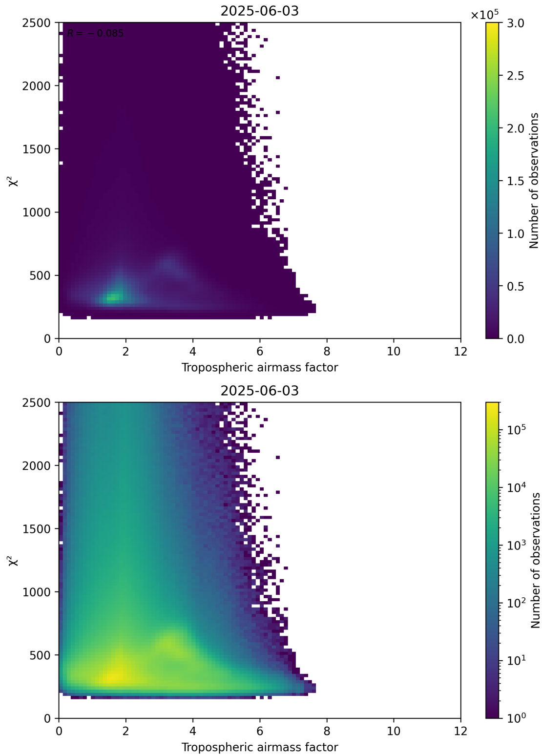
Figure 73: Scatter density plot of “Tropospheric airmass factor” against “ \chi^2 ” for 2025-06-02 to 2025-06-04.
