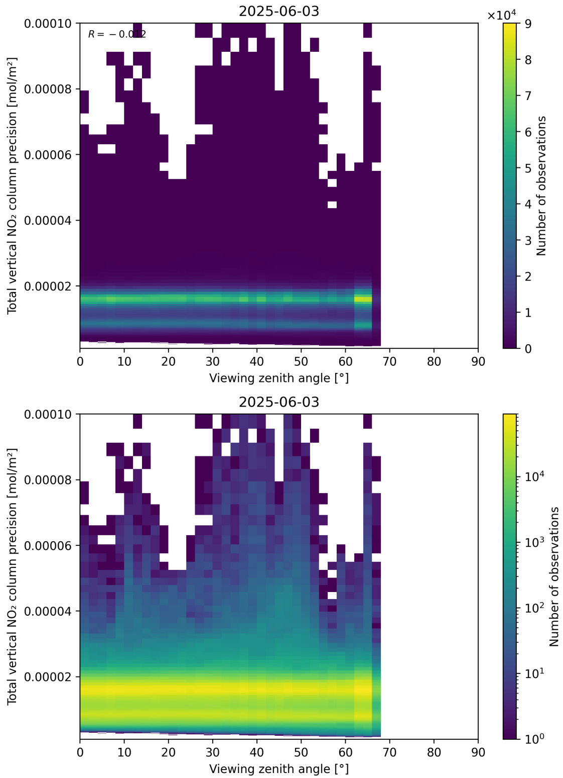
Figure 168: Scatter density plot of “Viewing zenith angle” against “Total vertical NO 2 column precision” for 2025-06-02 to 2025-06-04.
