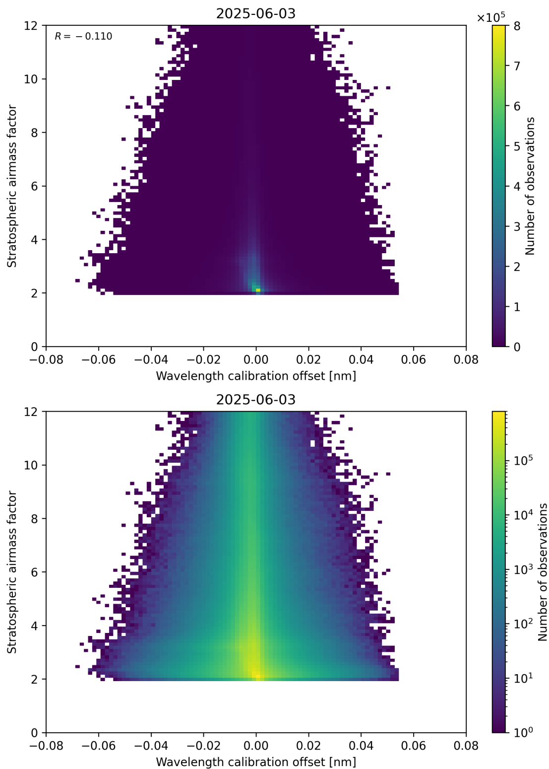
Figure 174: Scatter density plot of “Wavelength calibration offset” against “Stratospheric airmass factor” for 2025-06-02 to 2025-06-04.
