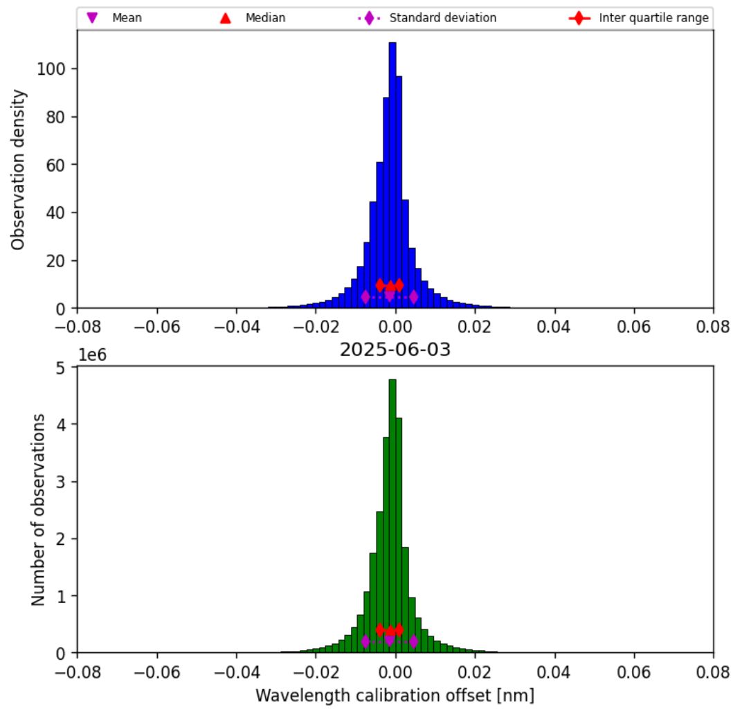
Figure 35: Histogram of “Wavelength calibration offset” for 2025-06-02 to 2025-06-04
