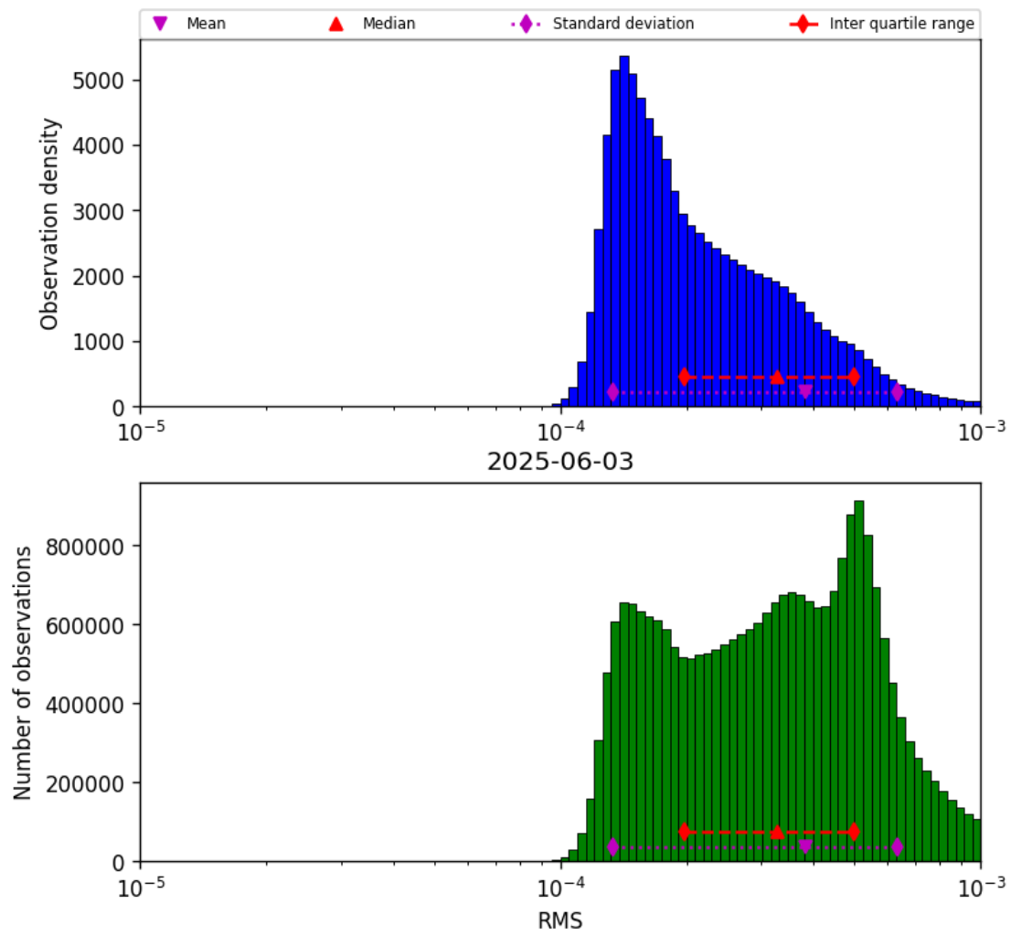
Figure 43: Histogram of “RMS” for 2025-06-02 to 2025-06-04
