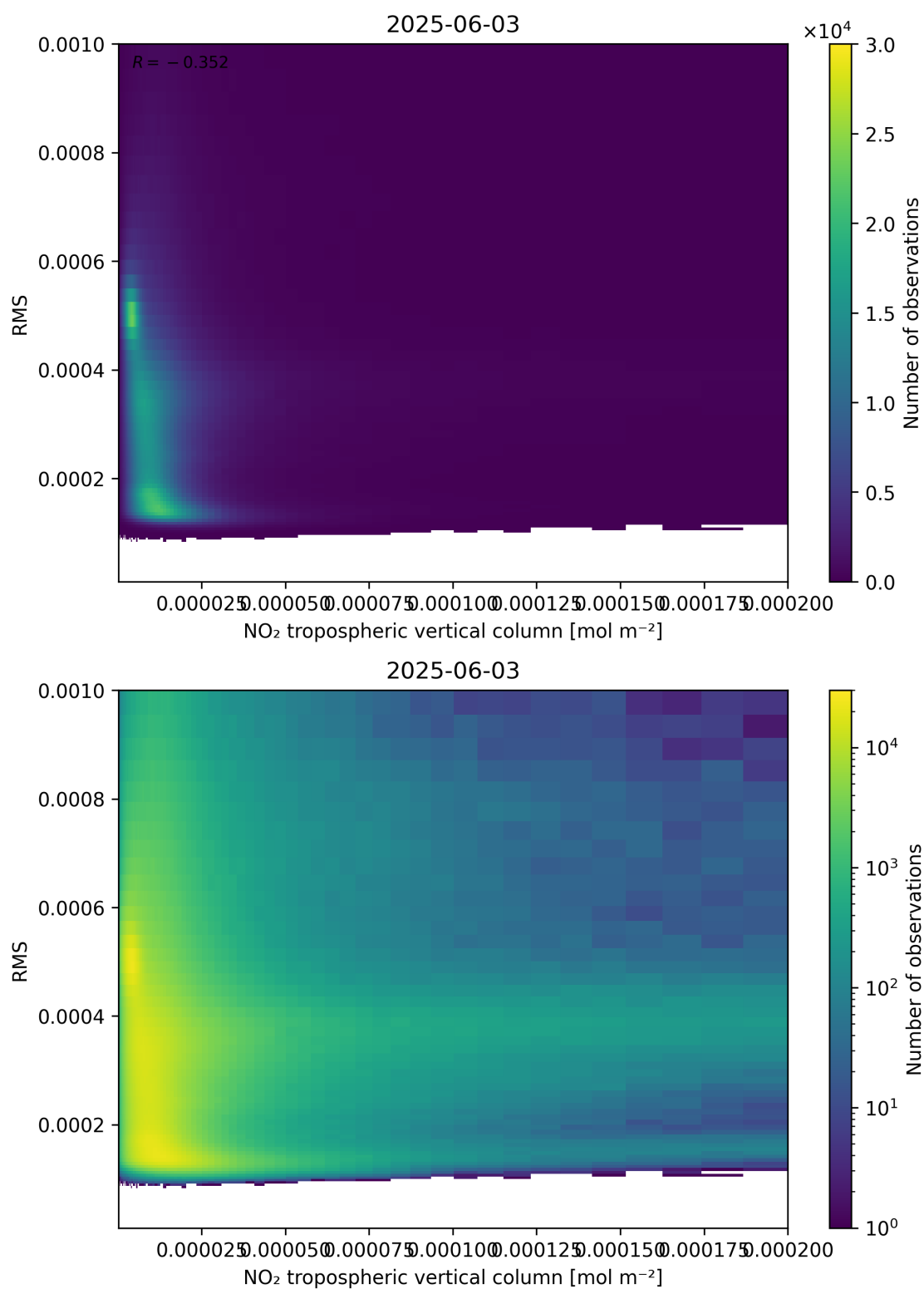
Figure 142: Scatter density plot of “NO 2 tropospheric vertical column” against “RMS” for 2025-06-02 to 2025-06-04.
