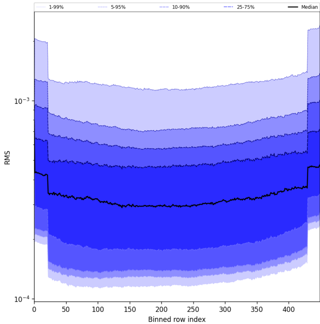
Figure 60: Along track statistics of “RMS” for 2025-06-02 to 2025-06-04
