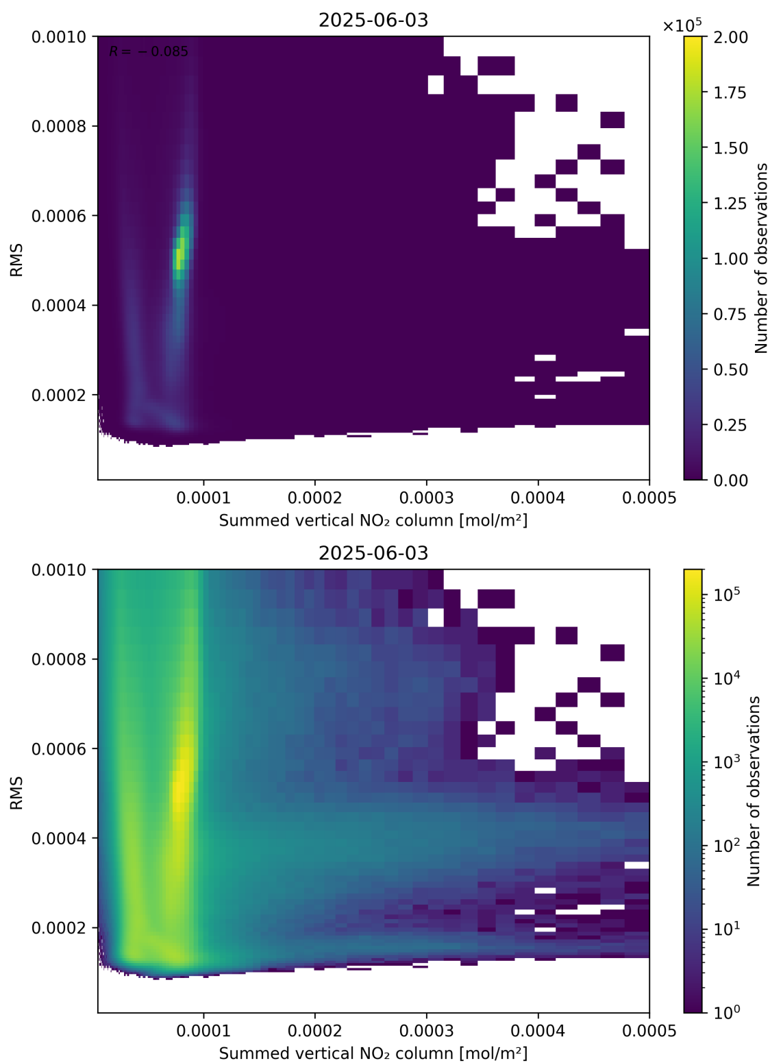
Figure 109: Scatter density plot of “Summed vertical NO 2 column” against “RMS” for 2025-06-02 to 2025-06-04.
