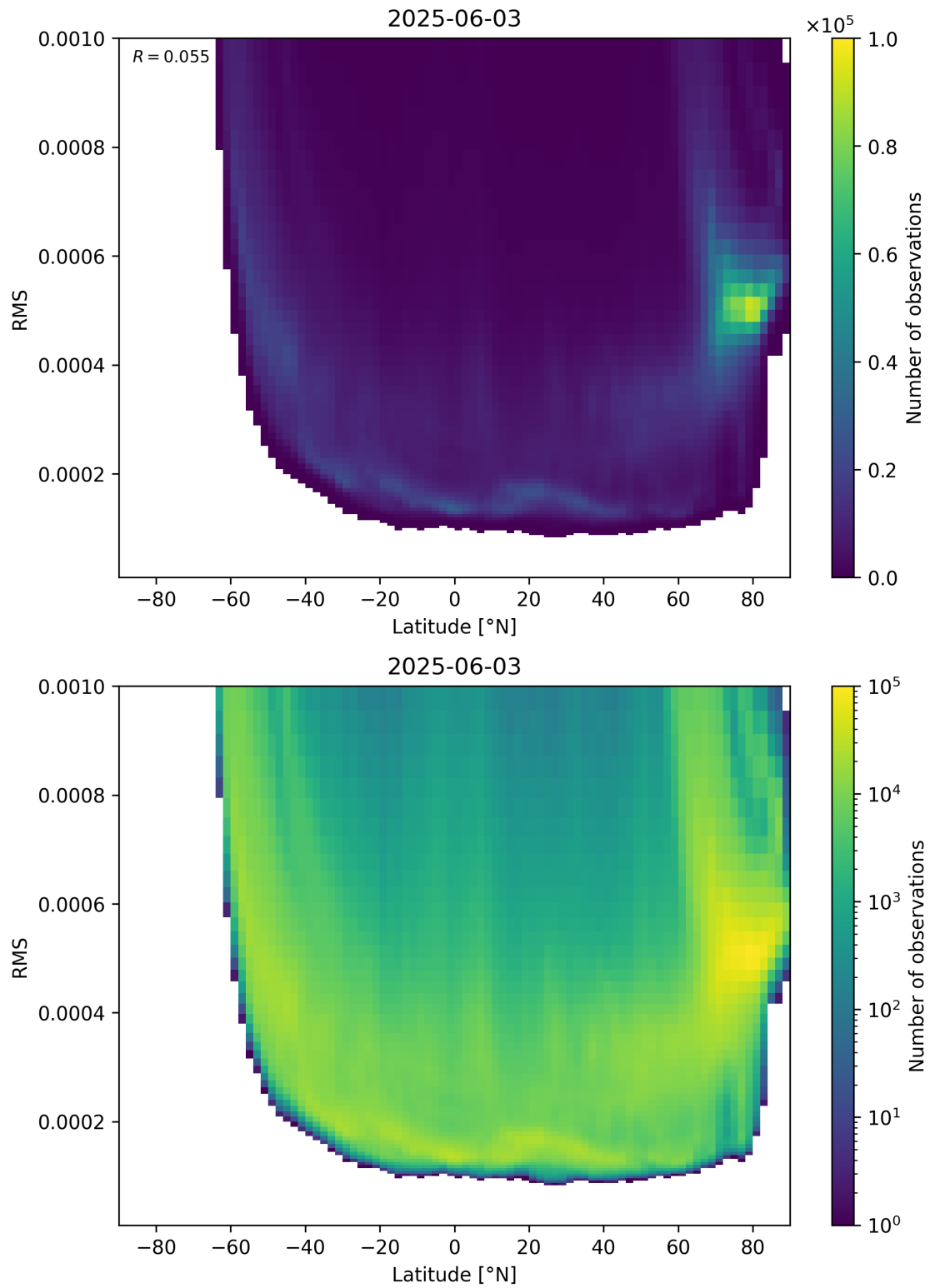
Figure 94: Scatter density plot of “Latitude” against “RMS” for 2025-06-02 to 2025-06-04.
