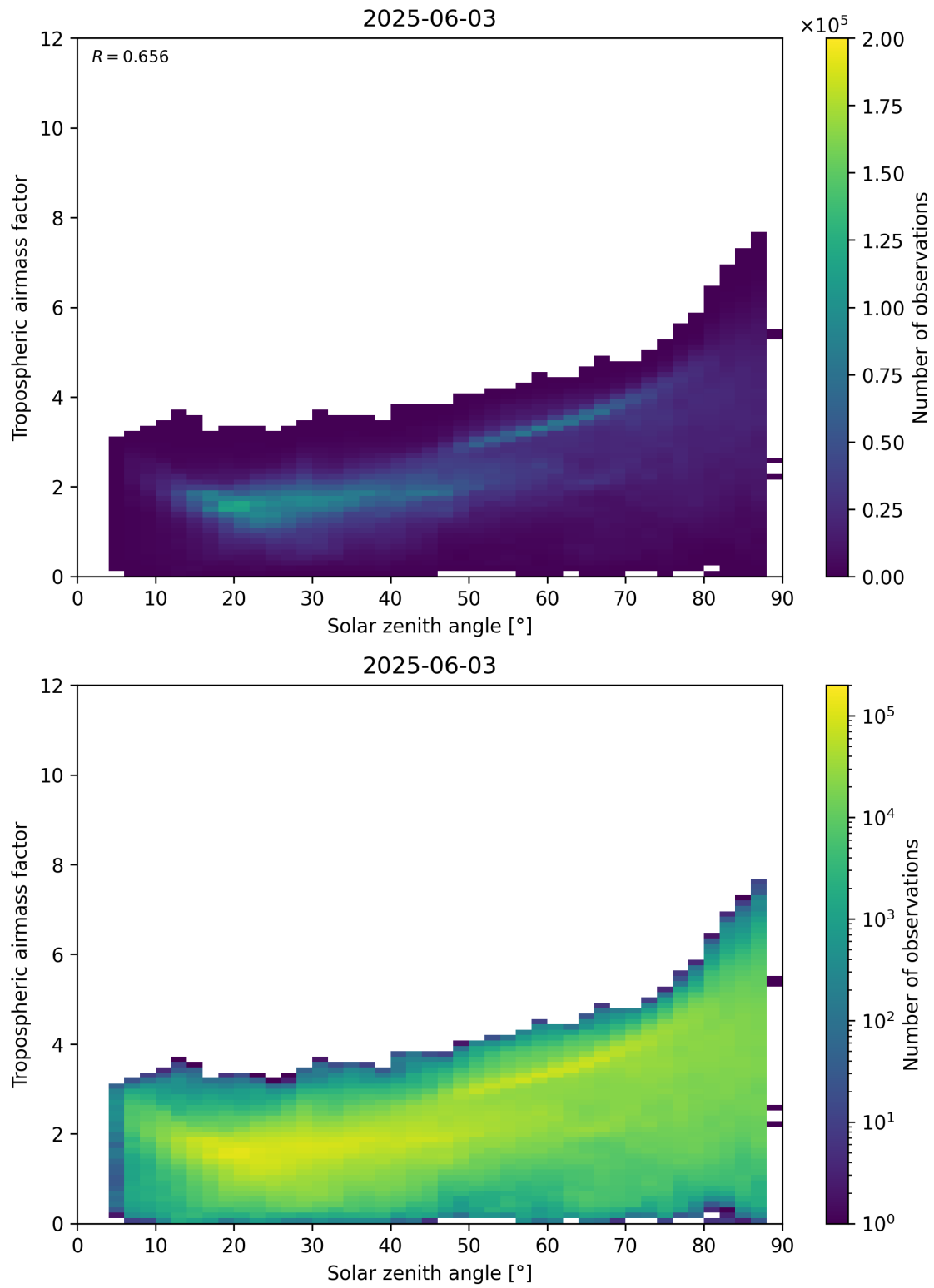
Figure 147: Scatter density plot of “Solar zenith angle” against “Tropospheric airmass factor” for 2025-06-02 to 2025-06-04.
