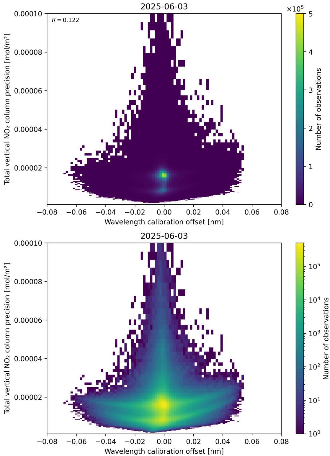
Figure 180: Scatter density plot of “Wavelength calibration offset” against “Total vertical NO 2 column precision” for 2025-06-02 to 2025-06-04.
