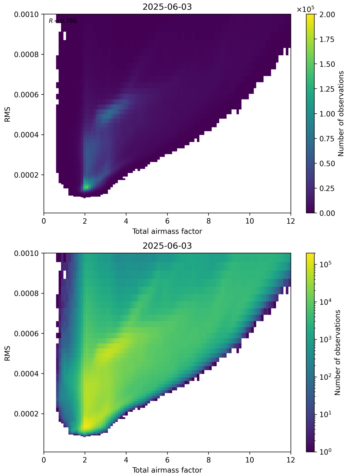
Figure 69: Scatter density plot of “Total airmass factor” against “RMS” for 2025-06-02 to 2025-06-04.
