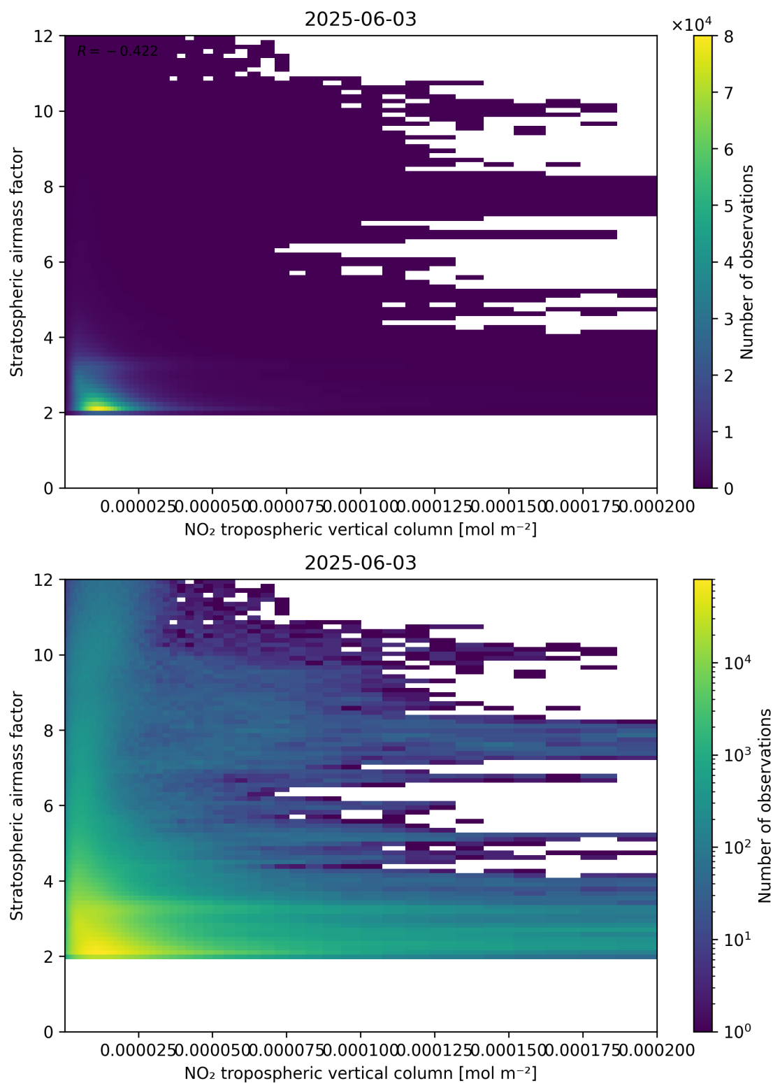
Figure 121: Scatter density plot of “NO 2 tropospheric vertical column” against “Stratospheric air mass factor” for 2025-06-02 to 2025-06-04.
