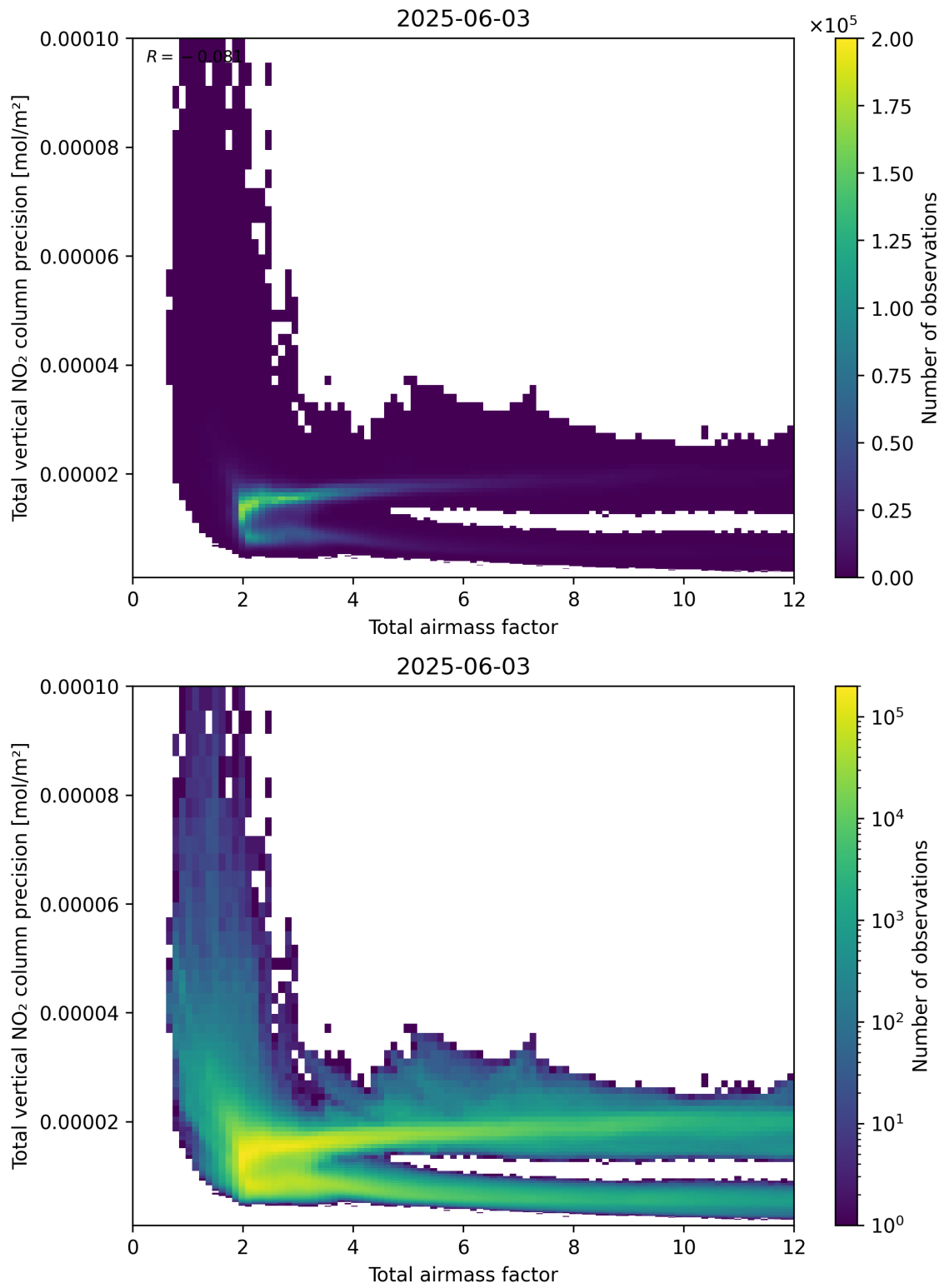
Figure 68: Scatter density plot of “Total airmass factor” against “Total vertical NO 2 column precision” for 2025-06-02 to 2025-06-04.
