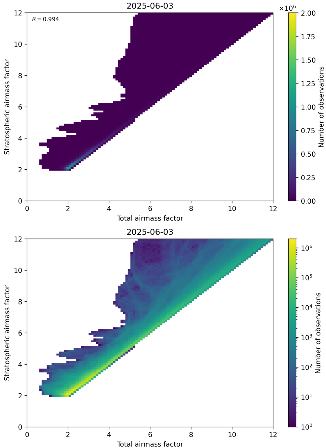
Figure 62: Scatter density plot of “Total airmass factor” against “Stratospheric airmass factor” for 2025-06-02 to 2025-06-04.
