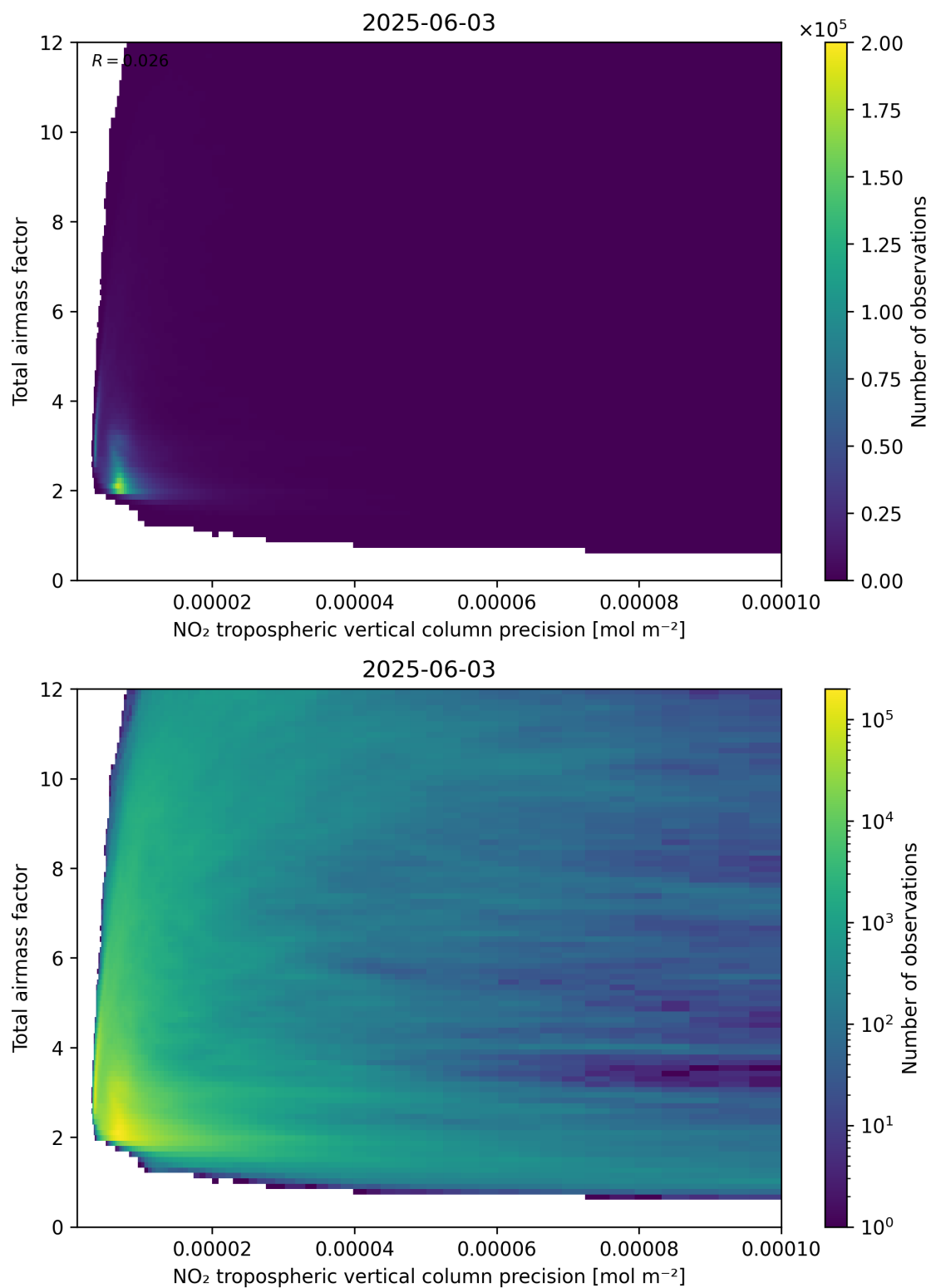
Figure 132: Scatter density plot of “NO 2 tropospheric vertical column precision” against “Total air mass factor” for 2025-06-02 to 2025-06-04.
