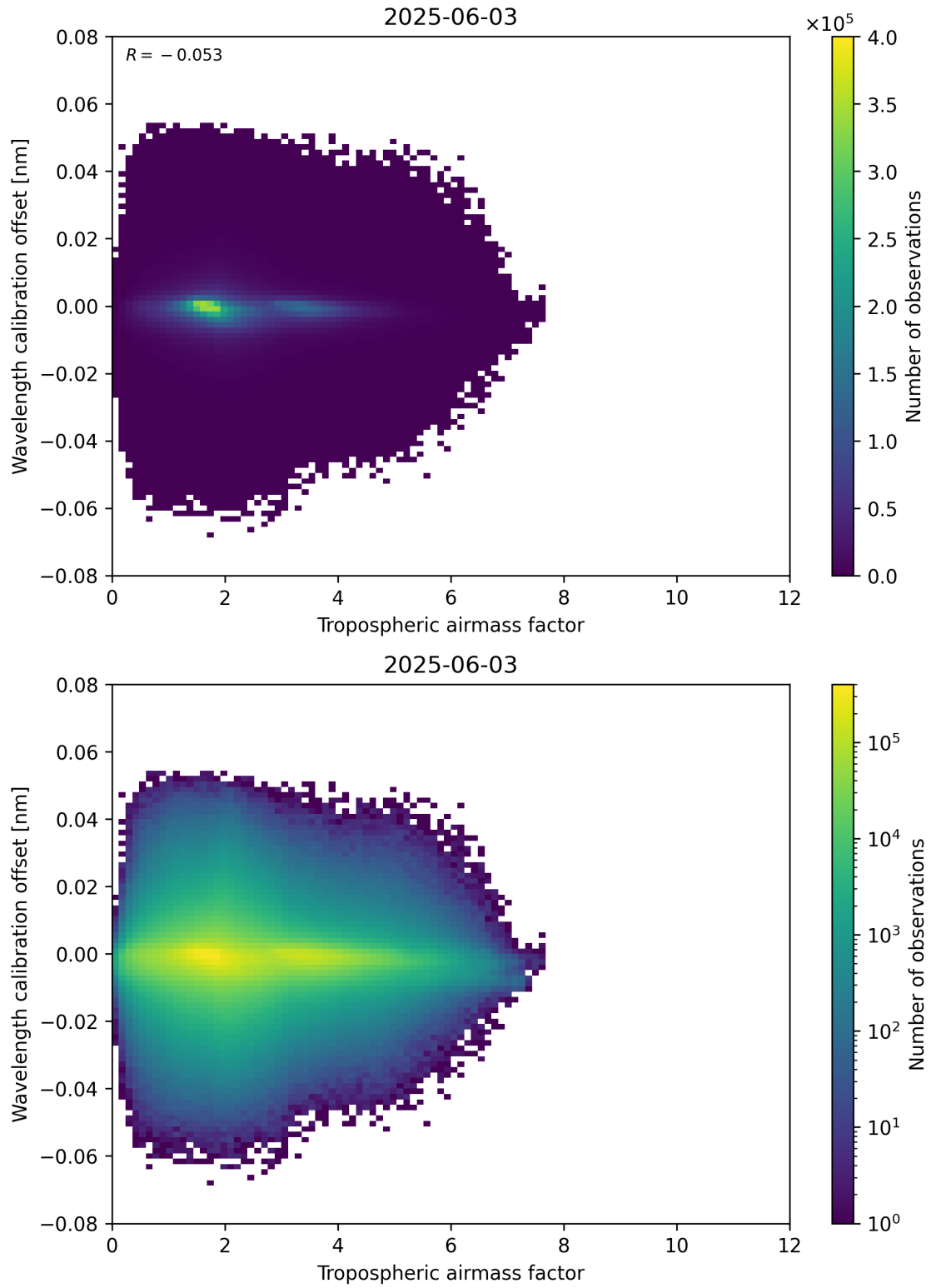
Figure 80: Scatter density plot of “Tropospheric airmass factor” against “Wavelength calibration offset” for 2025-06-02 to 2025-06-04.
