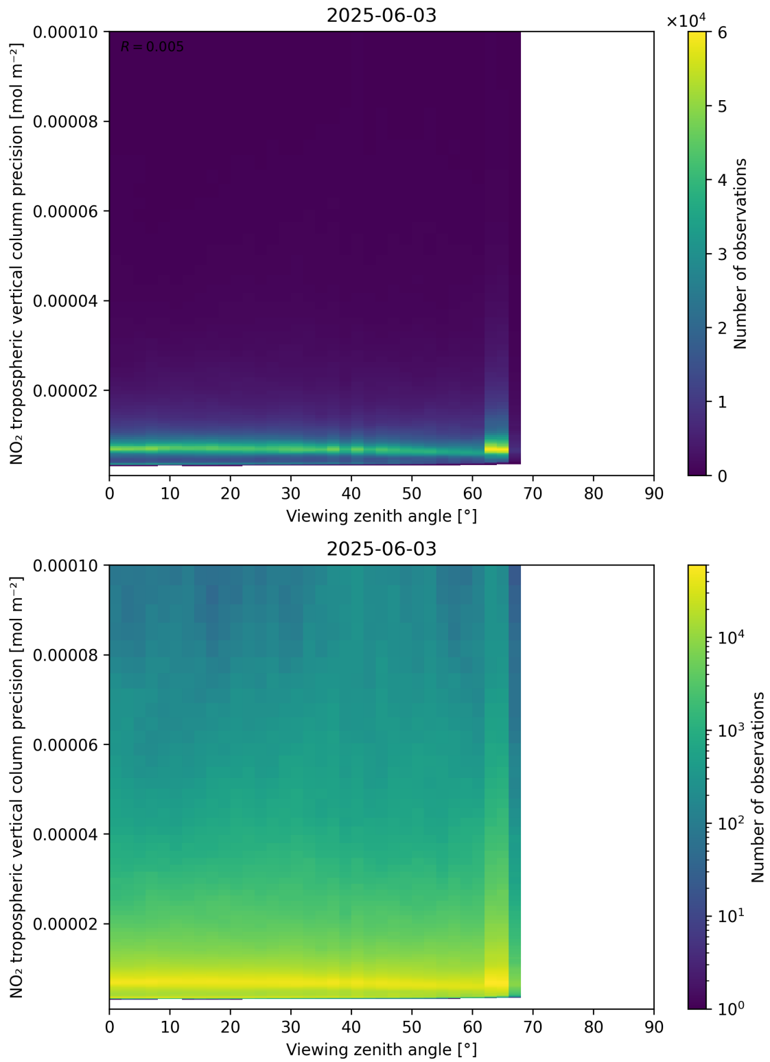
Figure 170: Scatter density plot of “Viewing zenith angle” against “NO 2 tropospheric vertical column precision” for 2025-06-02 to 2025-06-04.
