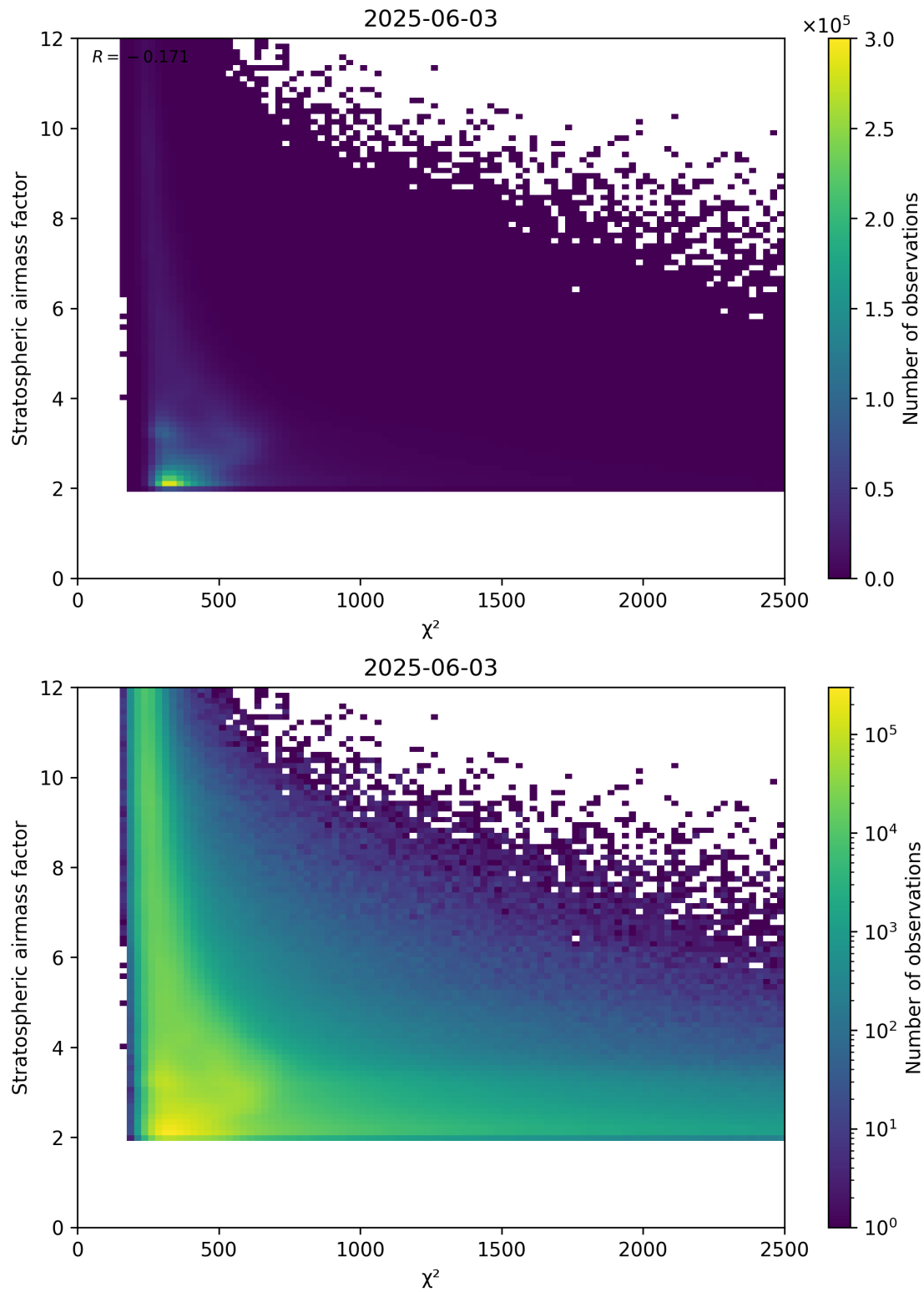
Figure 81: Scatter density plot of “ \chi^2 ” against “Stratospheric airmass factor” for 2025-06-02 to 2025-06-04.
