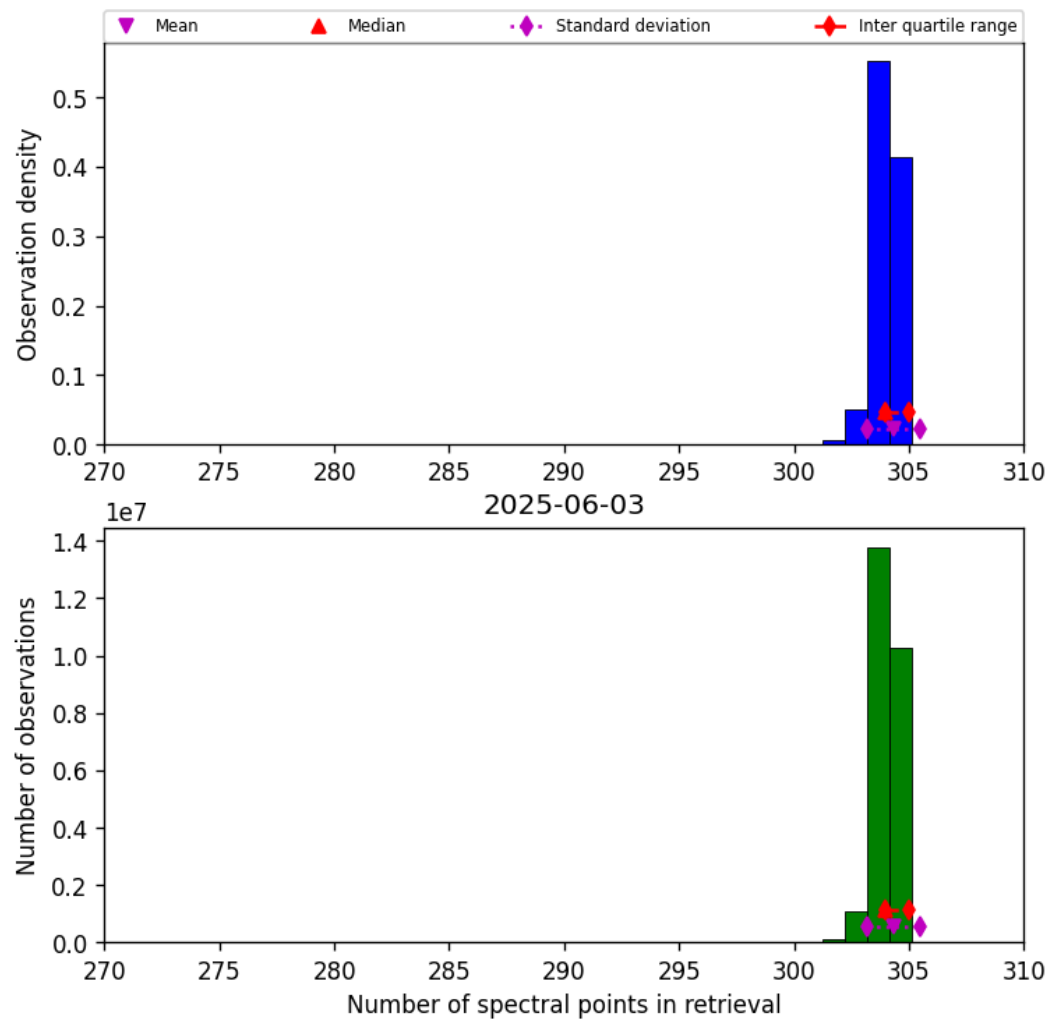
Figure 33: Histogram of “Number of spectral points in retrieval” for 2025-06-02 to 2025-06-04
