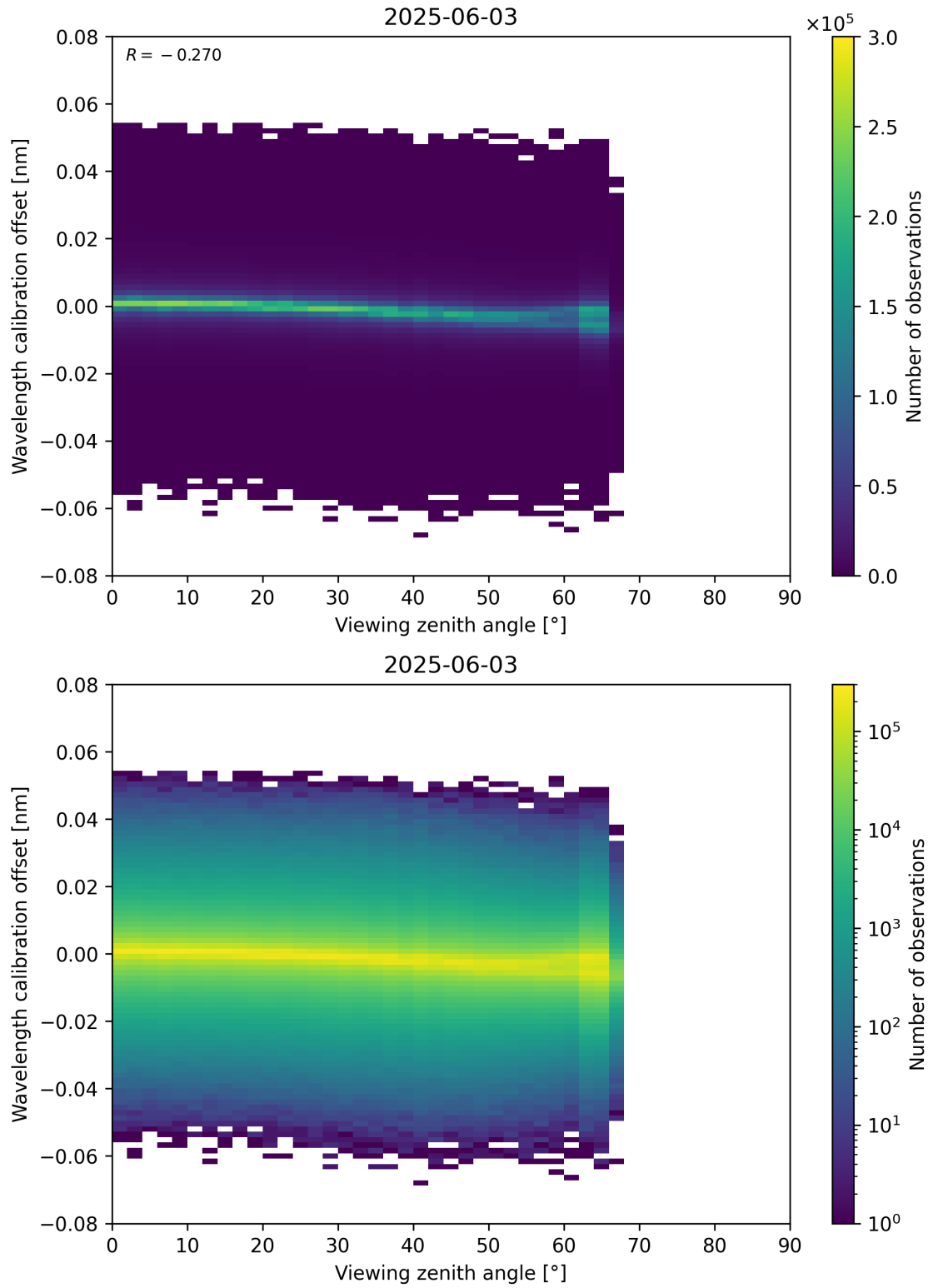
Figure 173: Scatter density plot of “Viewing zenith angle” against “Wavelength calibration offset” for 2025-06-02 to 2025-06-04.
