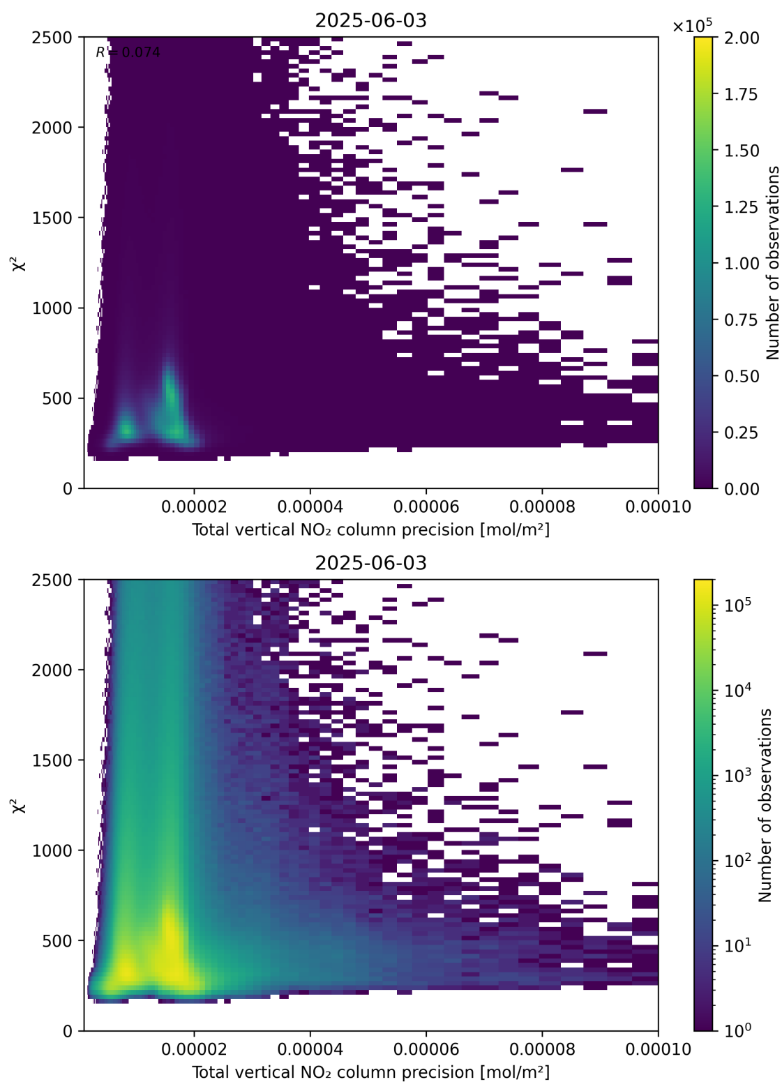
Figure 116: Scatter density plot of “Total vertical NO 2 column precision” against “ \chi^2 ” for 2025-06-02 to 2025-06-04.
