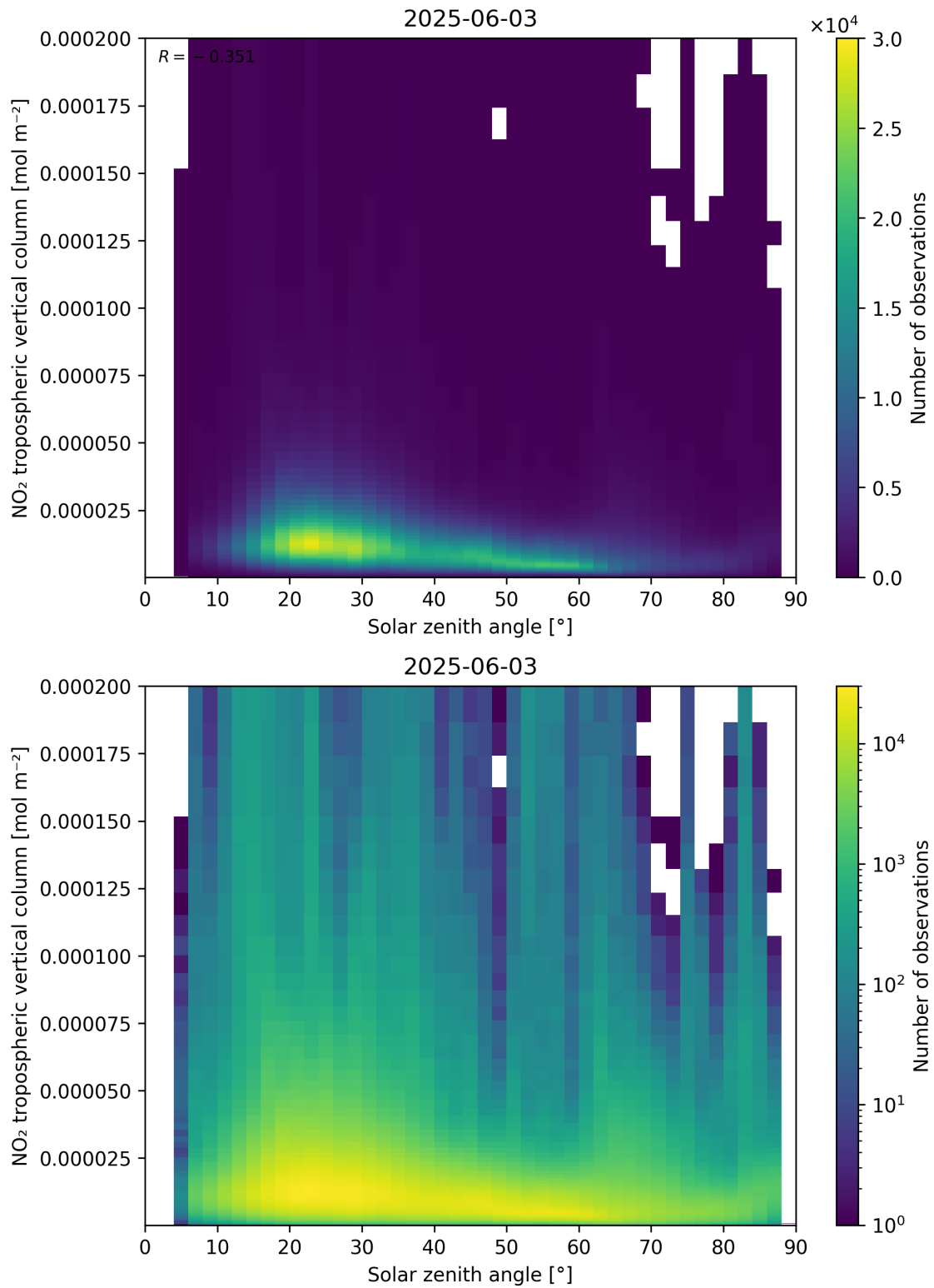
Figure 155: Scatter density plot of “Solar zenith angle” against “NO 2 tropospheric vertical column” for 2025-06-02 to 2025-06-04.
