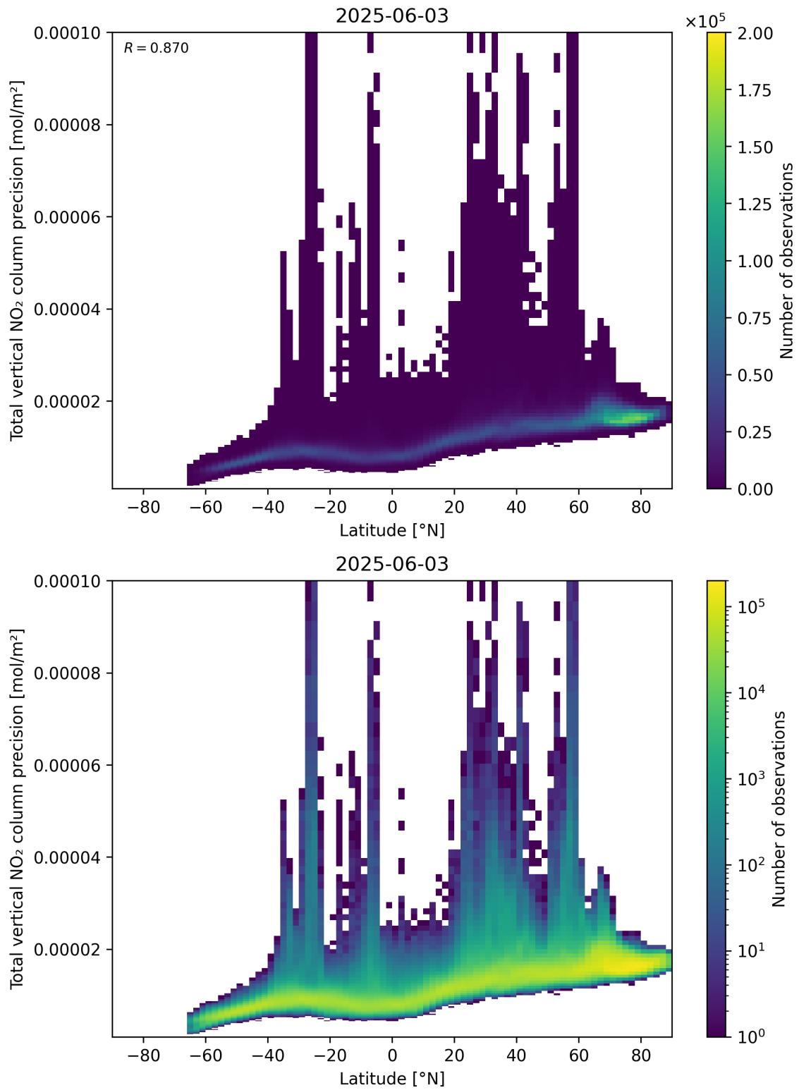
Figure 91: Scatter density plot of “Latitude” against “Total vertical NO 2 column precision” for 2025-06-02 to 2025-06-04.
