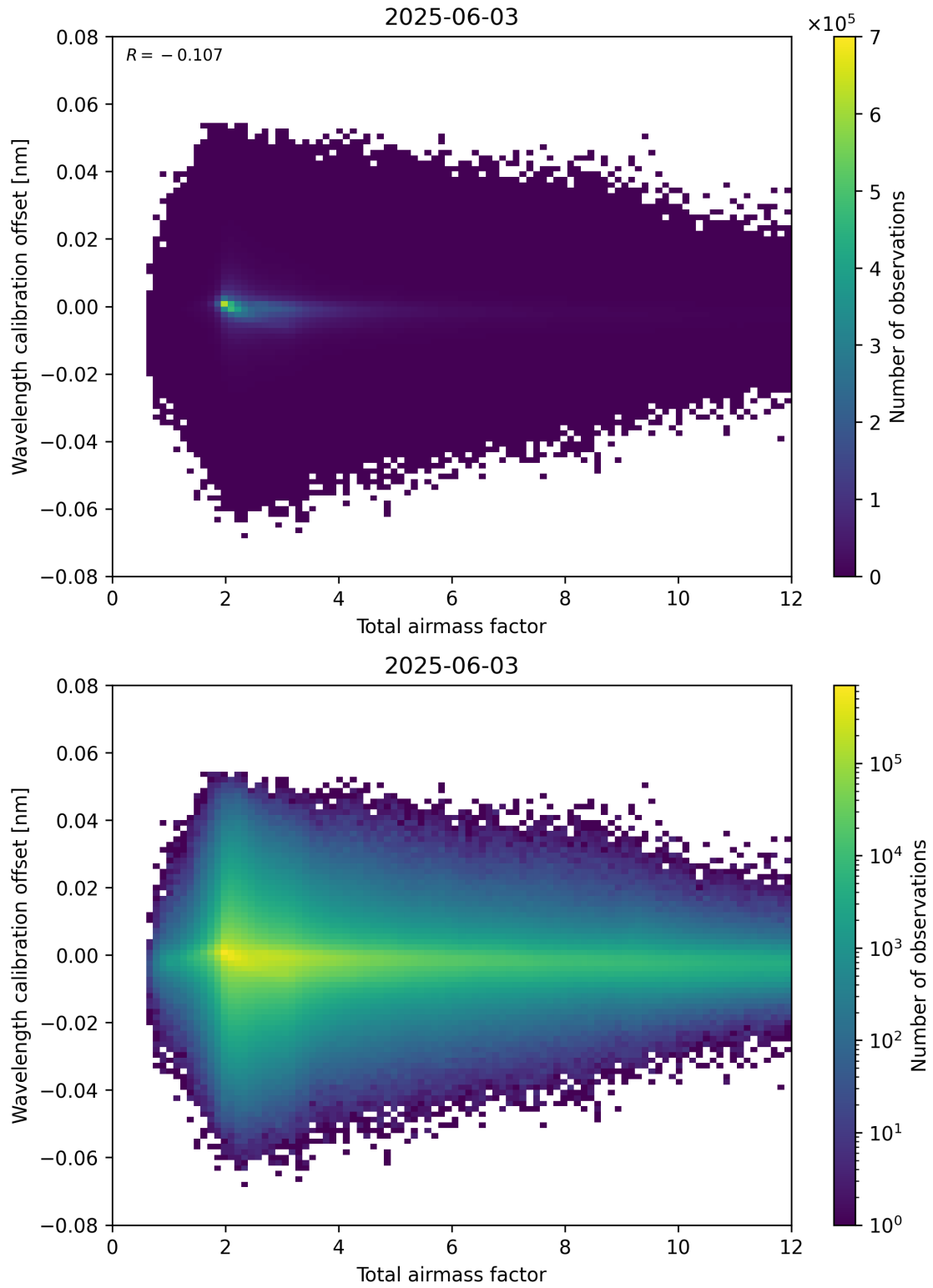
Figure 70: Scatter density plot of “Total airmass factor” against “Wavelength calibration offset” for 2025-06-02 to 2025-06-04.
