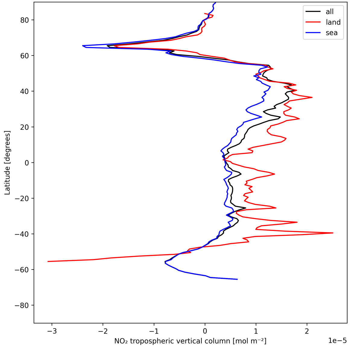
Figure 12: Zonal average of “NO 2 tropospheric vertical column” for 2025-06-02 to 2025-06-04.
