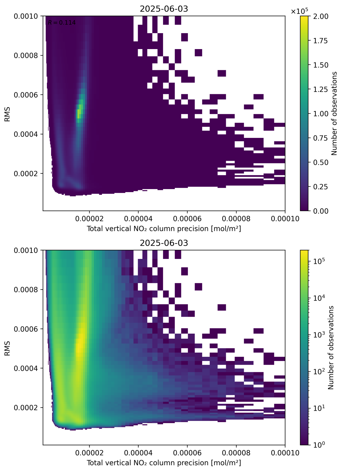
Figure 119: Scatter density plot of “Total vertical NO 2 column precision” against “RMS” for 2025-06-02 to 2025-06-04.
