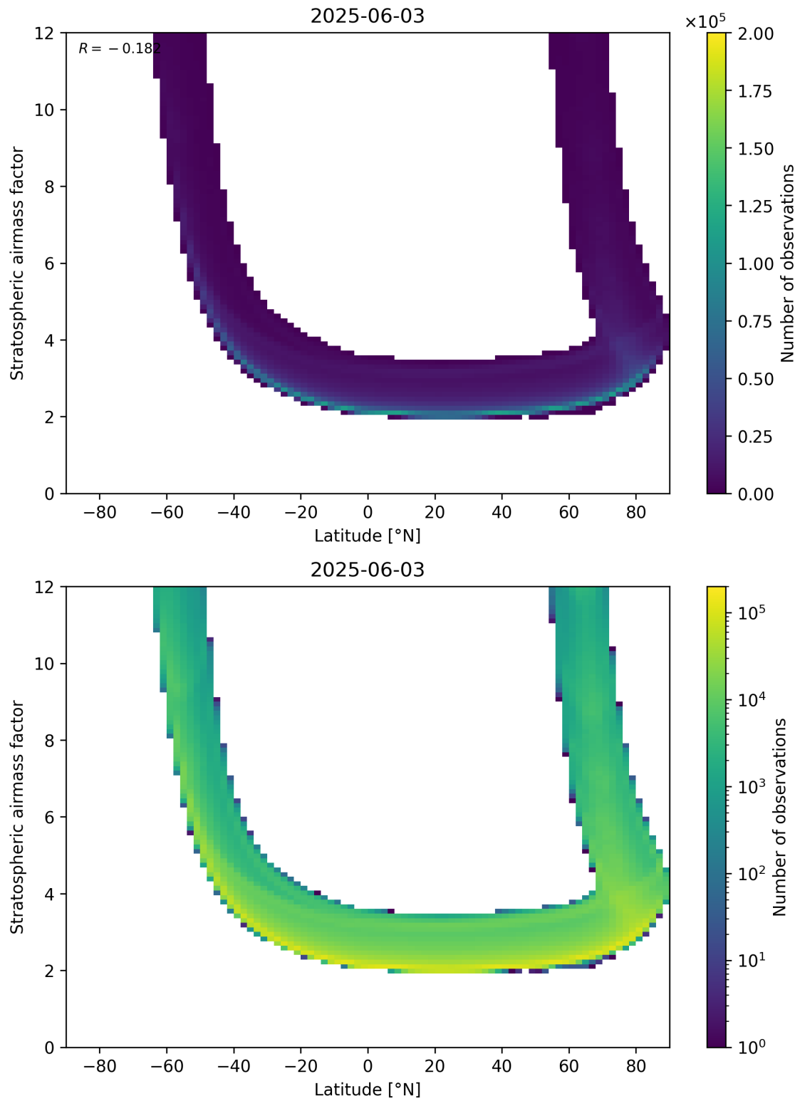
Figure 83: Scatter density plot of “Latitude” against “Stratospheric air mass factor” for 2025-06-02 to 2025-06-04.
