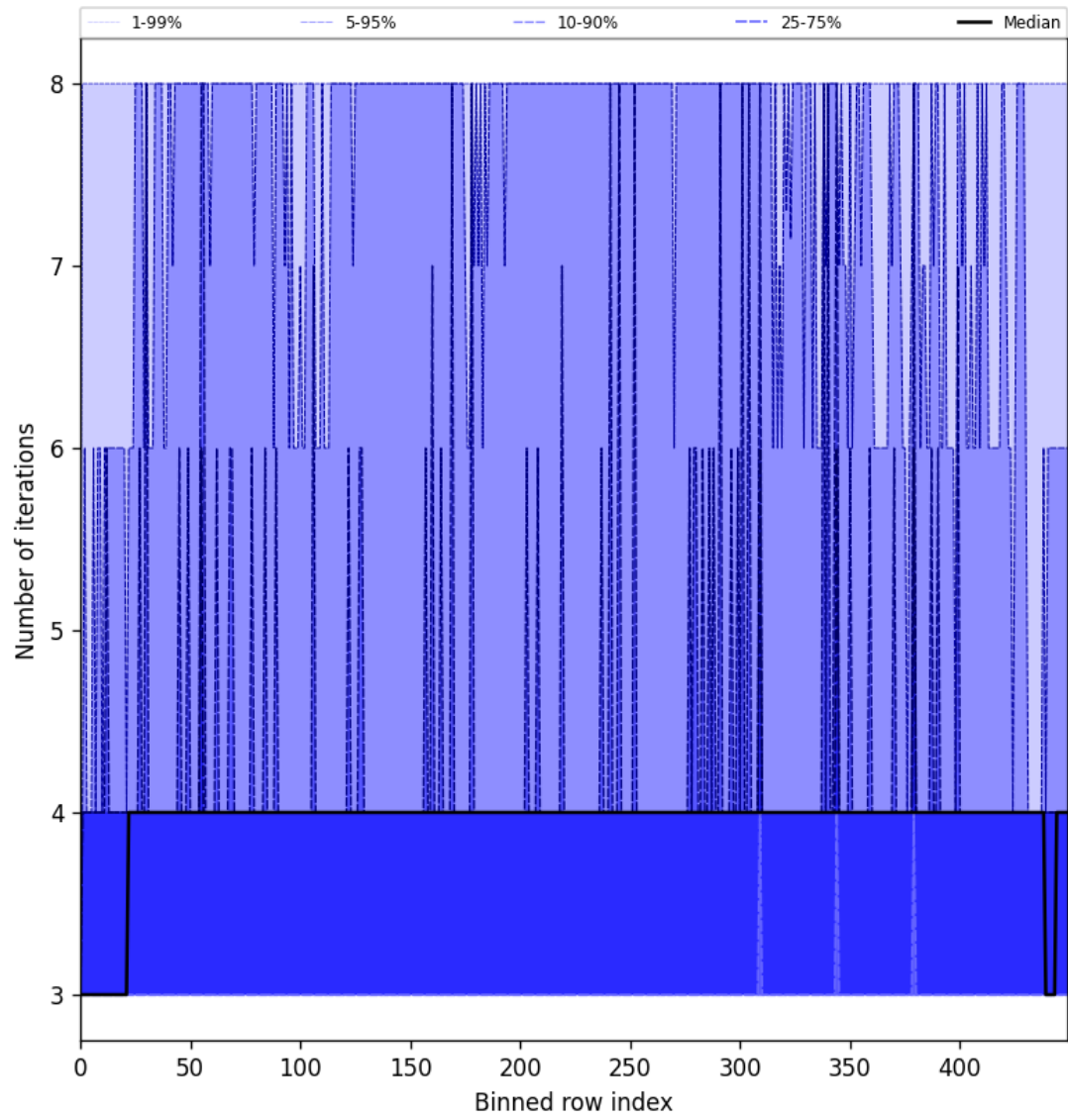
Figure 51: Along track statistics of “Number of iterations” for 2025-06-02 to 2025-06-04
