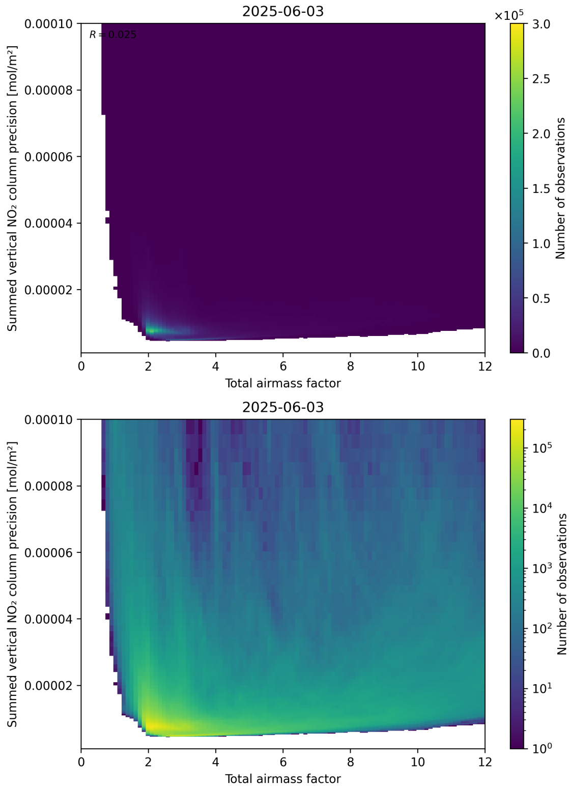
Figure 66: Scatter density plot of “Total airmass factor” against “Summed vertical NO 2 column precision” for 2025-06-02 to 2025-06-04.
