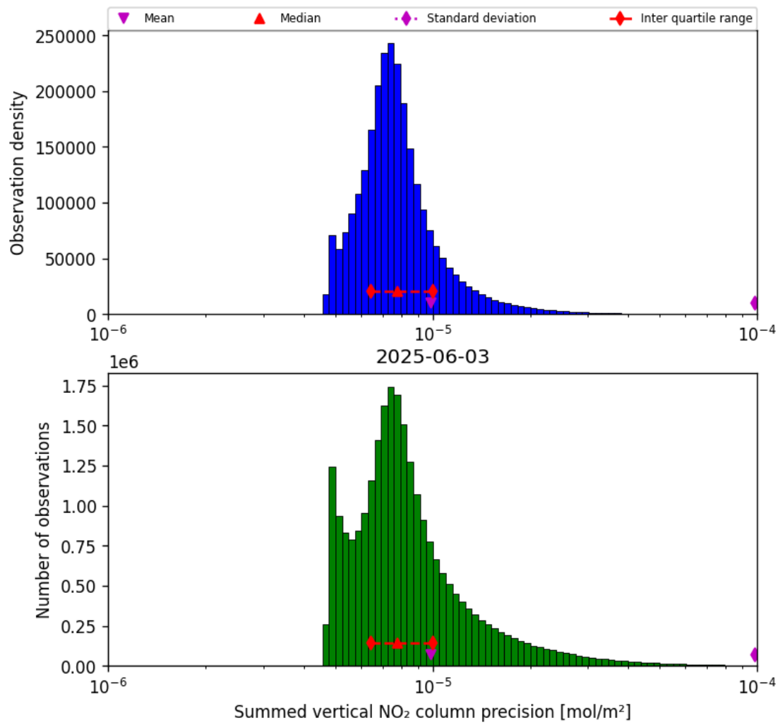
Figure 41: Histogram of “Summed vertical NO 2 column precision” for 2025-06-02 to 2025-06-04
