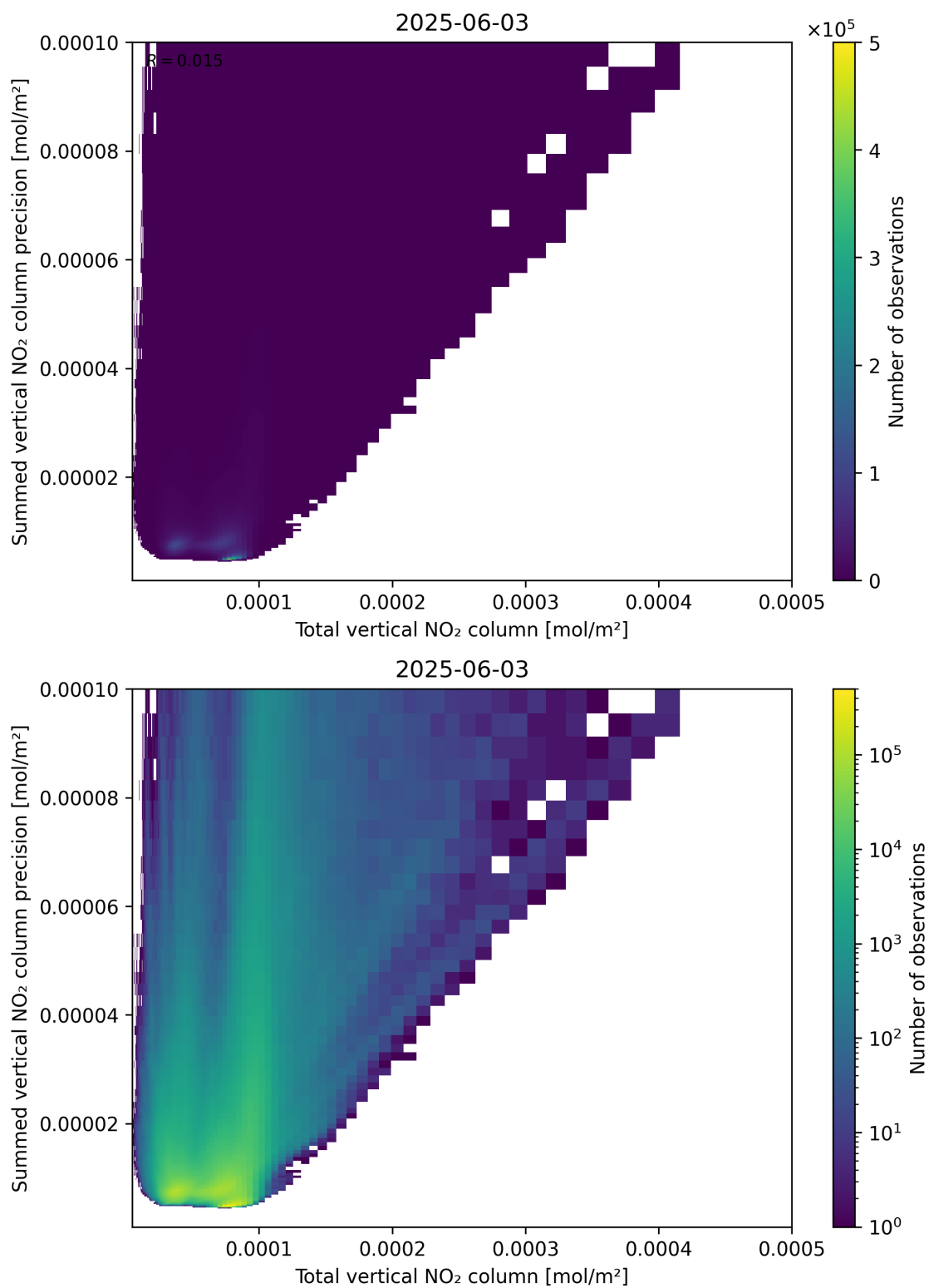
Figure 113: Scatter density plot of “Total vertical NO 2 column” against “Summed vertical NO 2 column precision” for 2025-06-02 to 2025-06-04.
