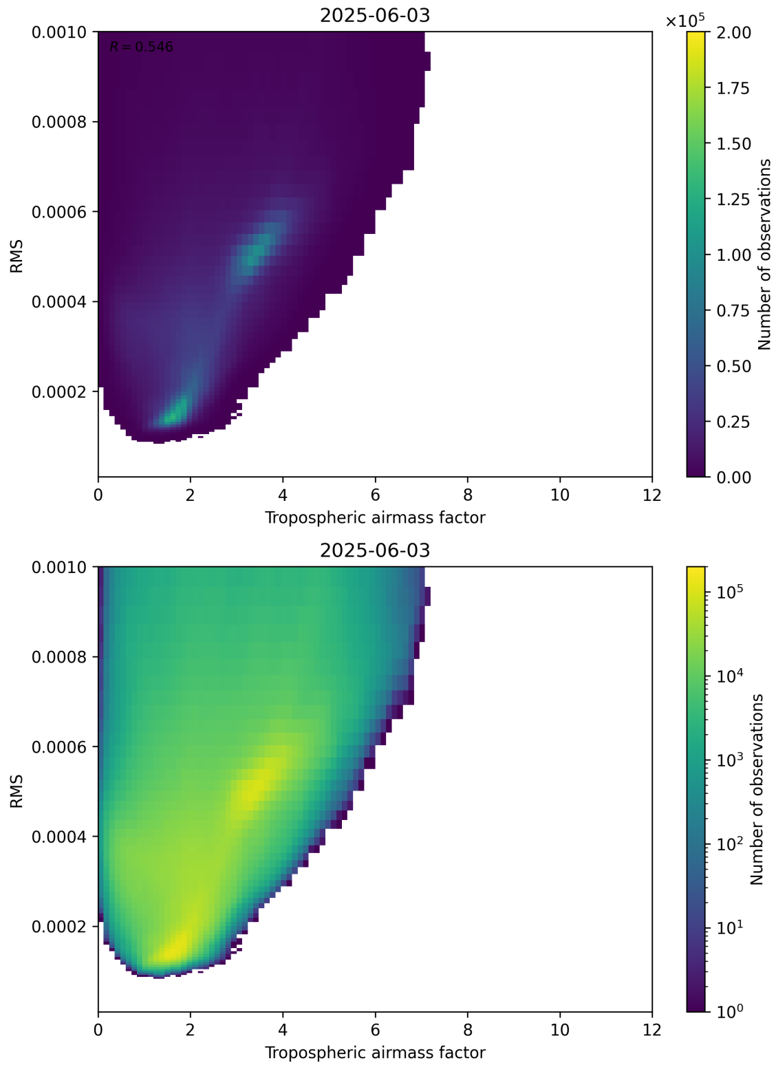
Figure 79: Scatter density plot of “Tropospheric airmass factor” against “RMS” for 2025-06-02 to 2025-06-04.
