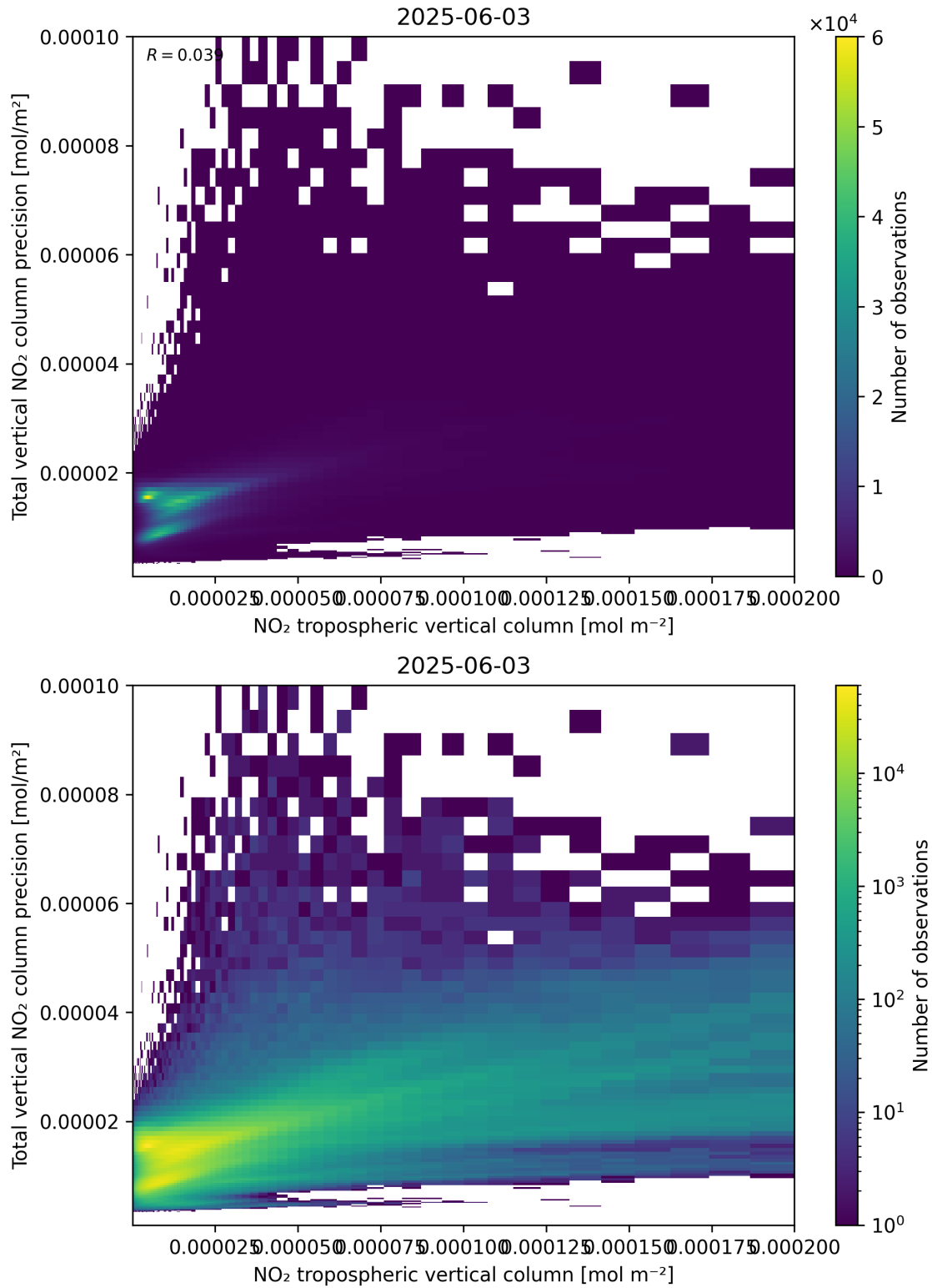
Figure 129: Scatter density plot of “NO 2 tropospheric vertical column” against “Total vertical NO 2 column precision” for 2025-06-02 to 2025-06-04.
