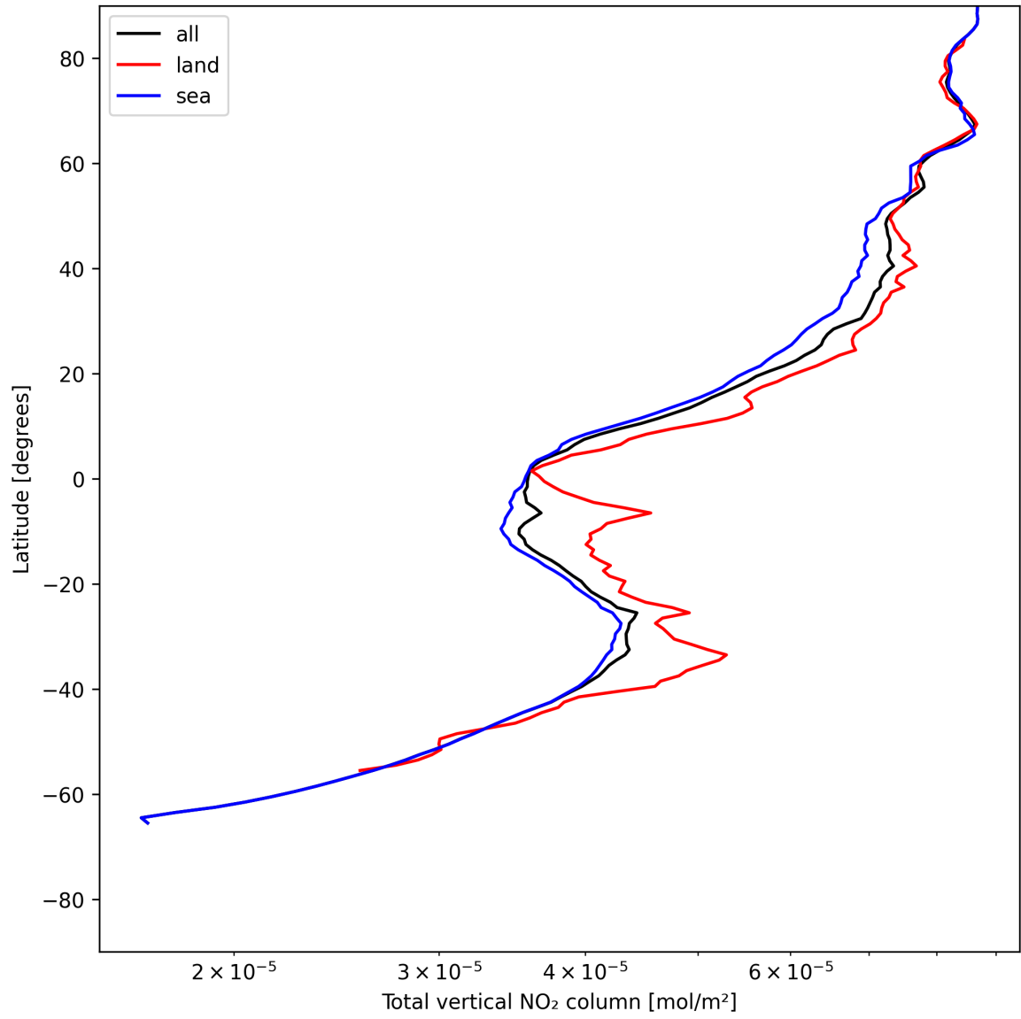
Figure 21: Zonal average of “Total vertical NO 2 column” for 2025-06-02 to 2025-06-04.
