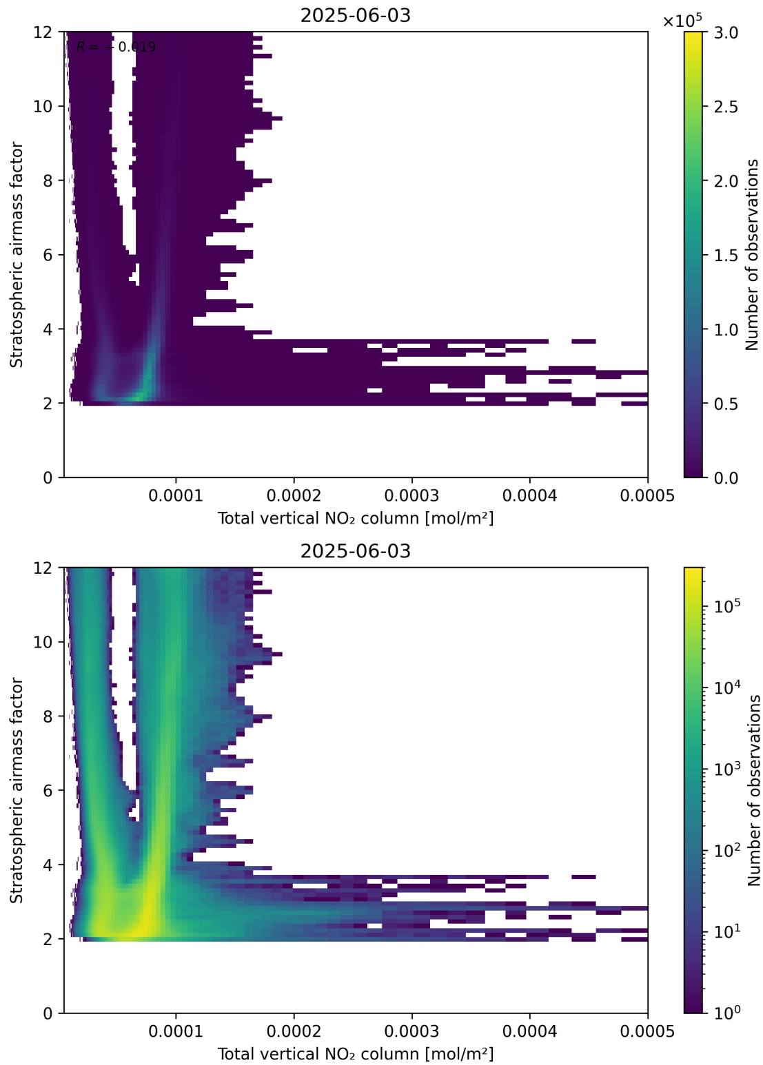
Figure 110: Scatter density plot of “Total vertical NO 2 column” against “Stratospheric airmass factor” for 2025-06-02 to 2025-06-04.
