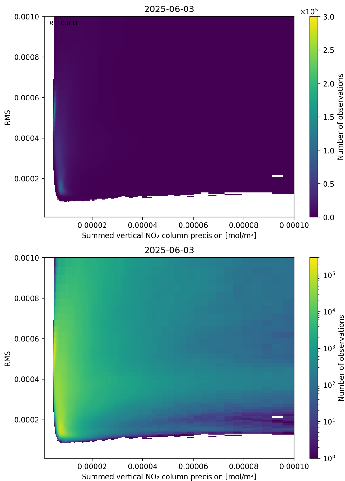
Figure 108: Scatter density plot of “Summed vertical NO 2 column precision” against “RMS” for 2025-06-02 to 2025-06-04.
