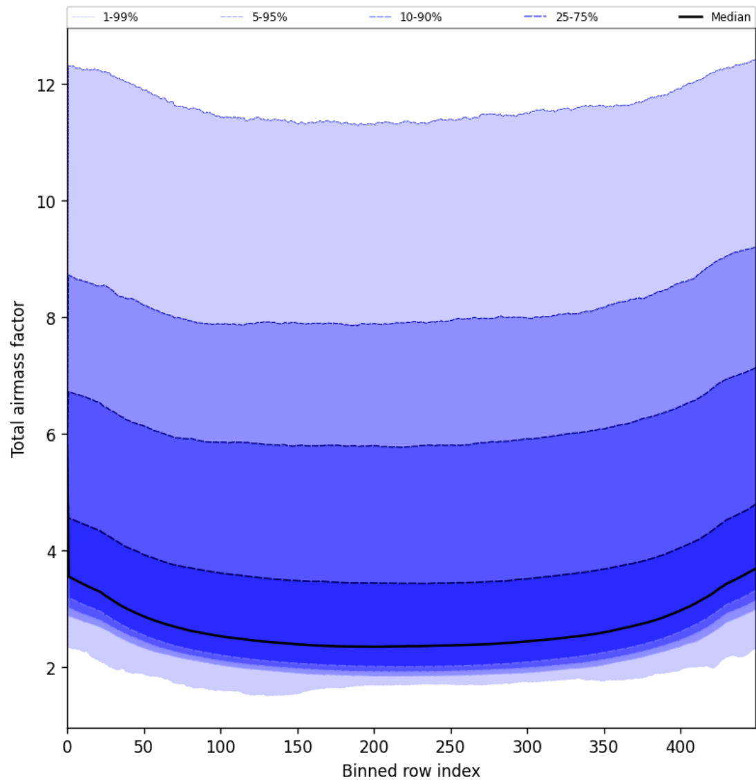
Figure 49: Along track statistics of “Total airmass factor” for 2025-06-02 to 2025-06-04
