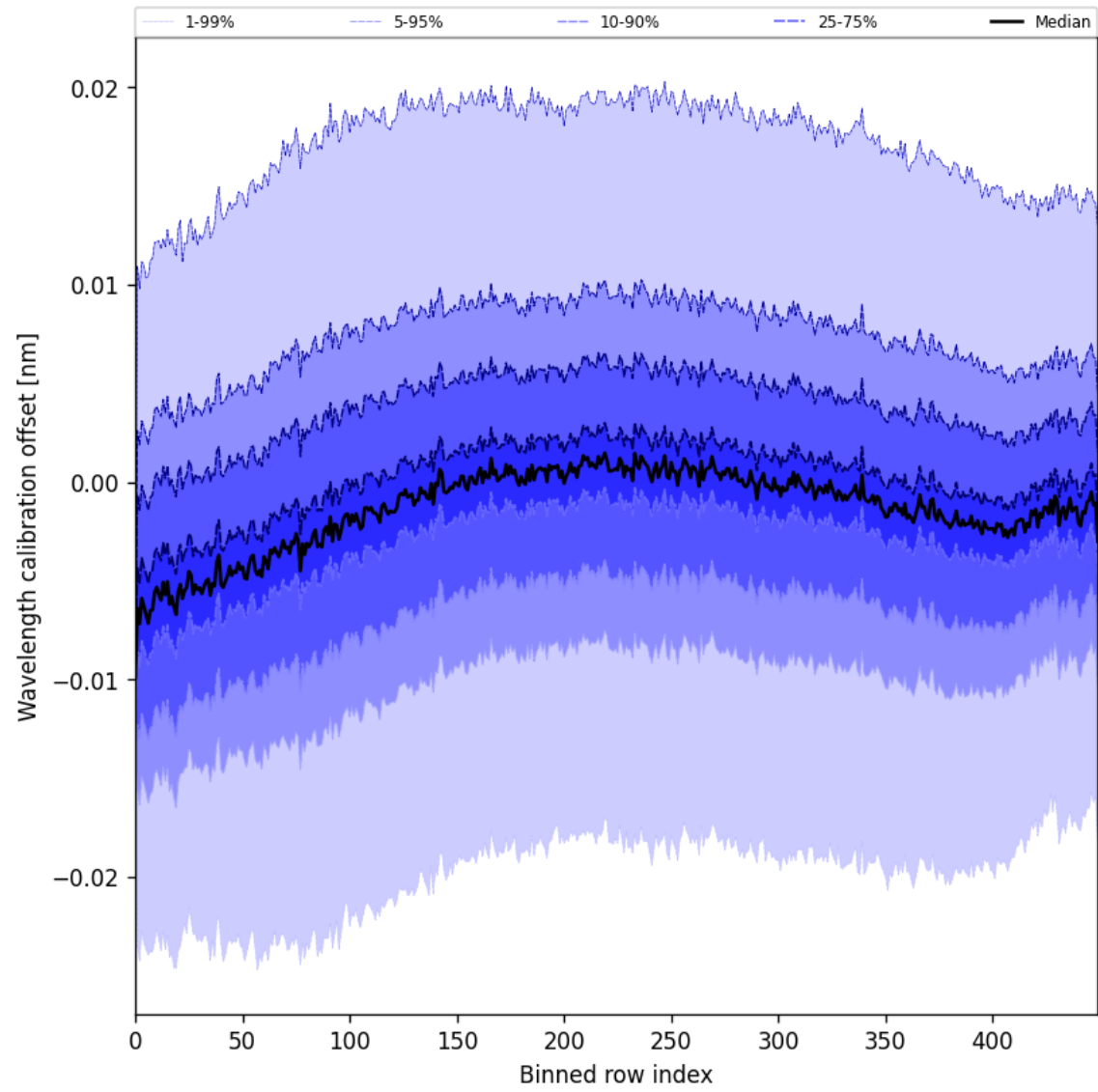
Figure 52: Along track statistics of “Wavelength calibration offset” for 2025-06-02 to 2025-06-04
