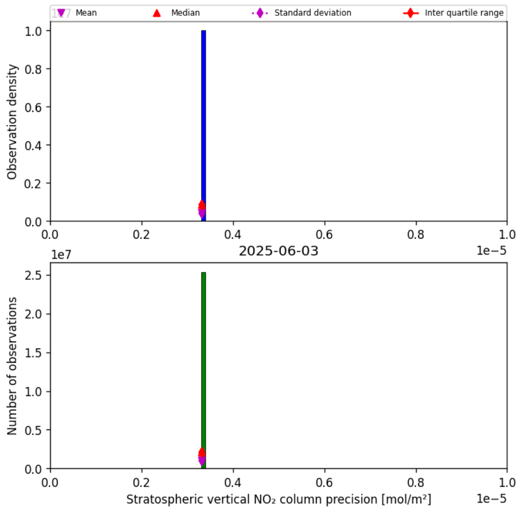
Figure 37: Histogram of “Stratospheric vertical NO 2 column precision” for 2025-06-02 to 2025-06-04
