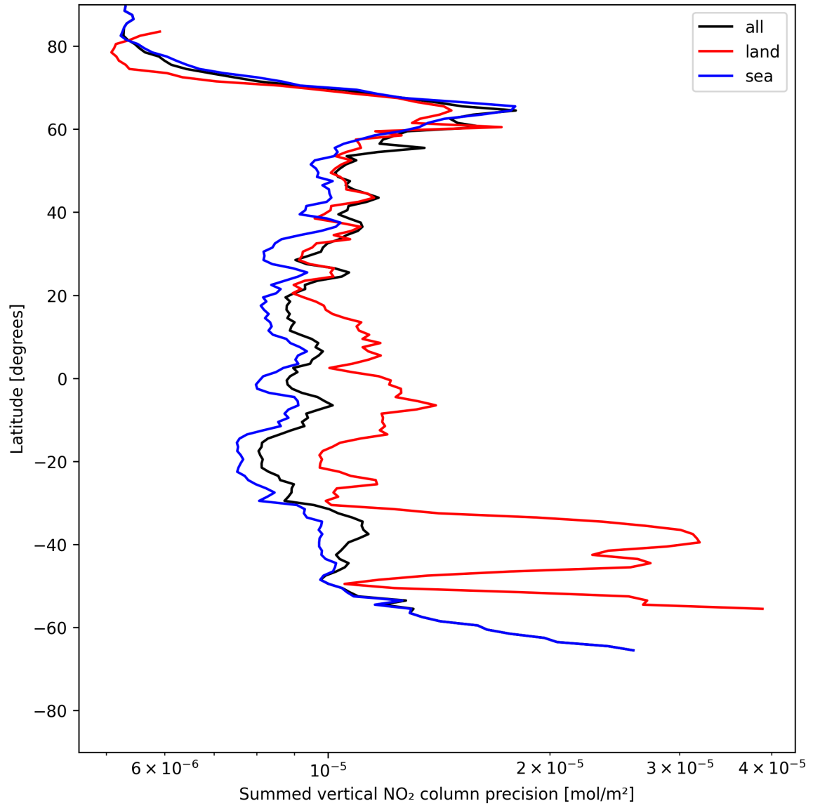
Figure 24: Zonal average of “Summed vertical NO 2 column precision” for 2025-06-02 to 2025-06-04.
