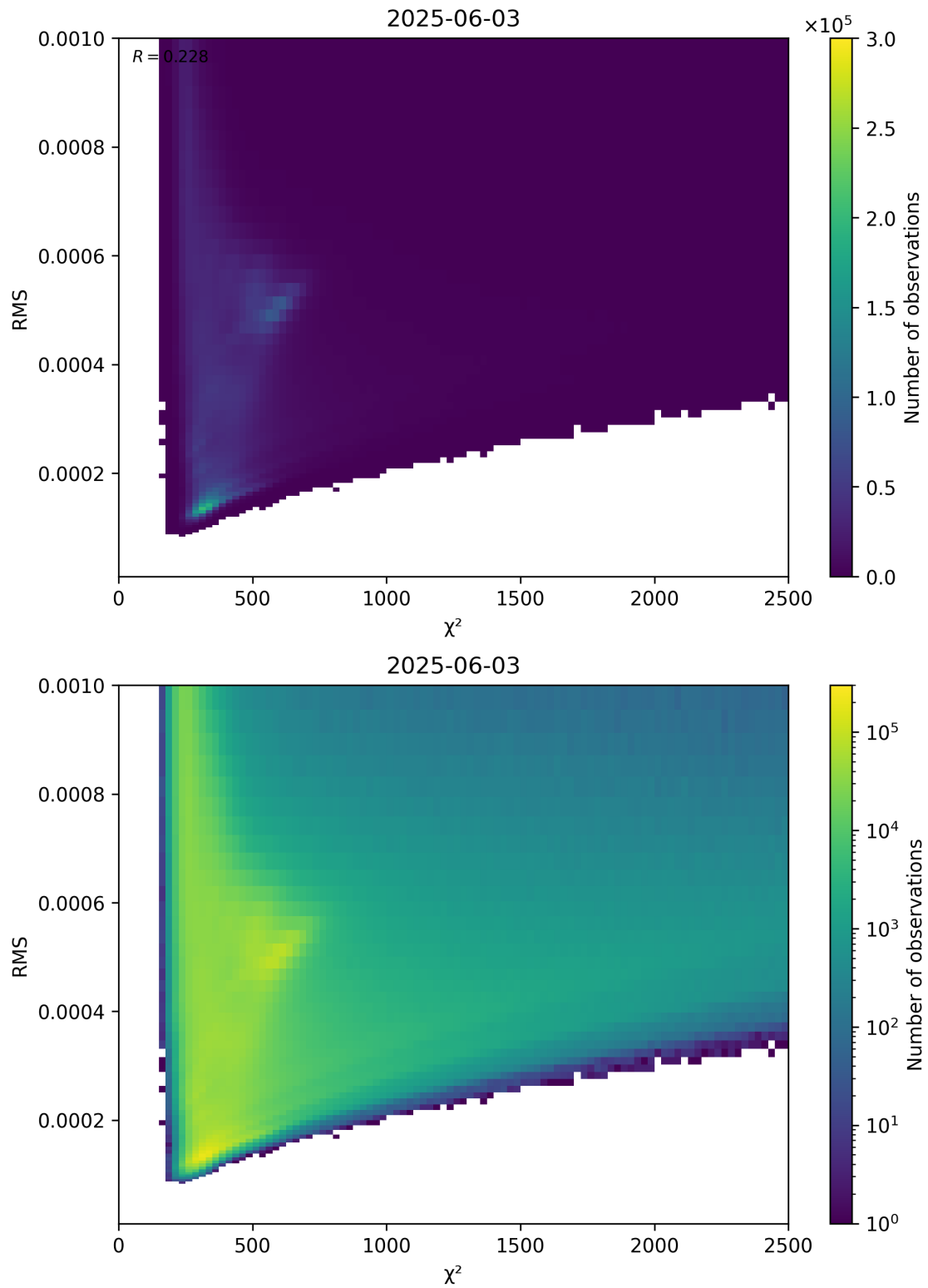
Figure 82: Scatter density plot of “ \chi^2 ” against “RMS” for 2025-06-02 to 2025-06-04.
