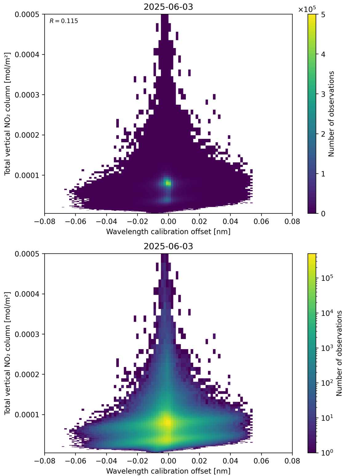
Figure 179: Scatter density plot of “Wavelength calibration offset” against “Total vertical NO 2 column” for 2025-06-02 to 2025-06-04.
