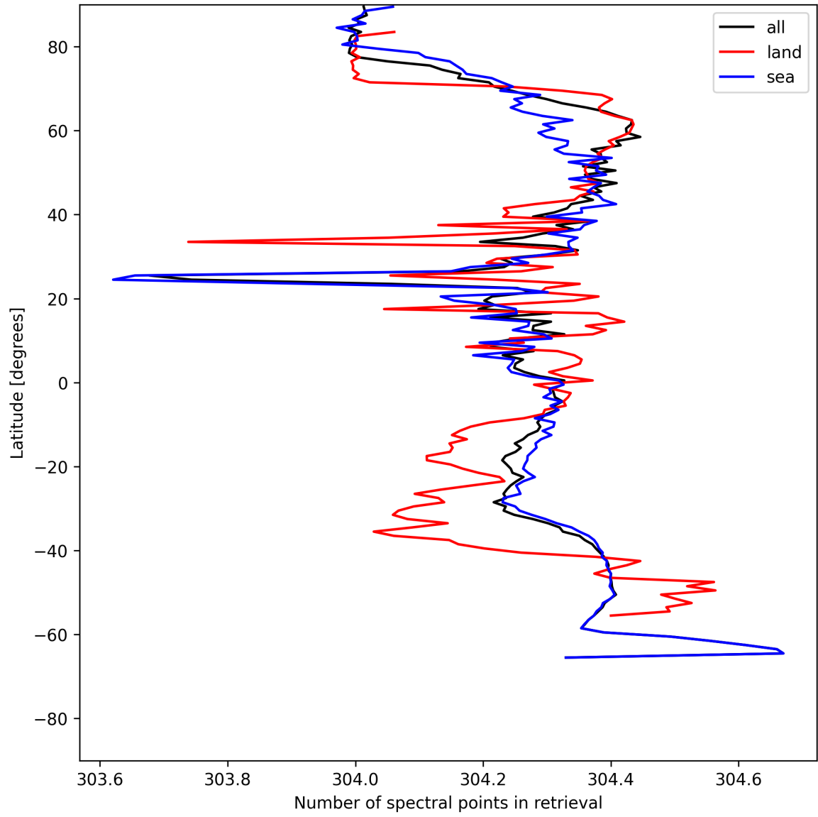
Figure 16: Zonal average of “Number of spectral points in retrieval” for 2025-06-02 to 2025-06-04.
