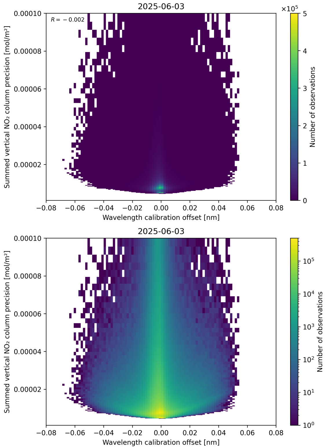
Figure 178: Scatter density plot of “Wavelength calibration offset” against “Summed vertical NO 2 column precision” for 2025-06-02 to 2025-06-04.
