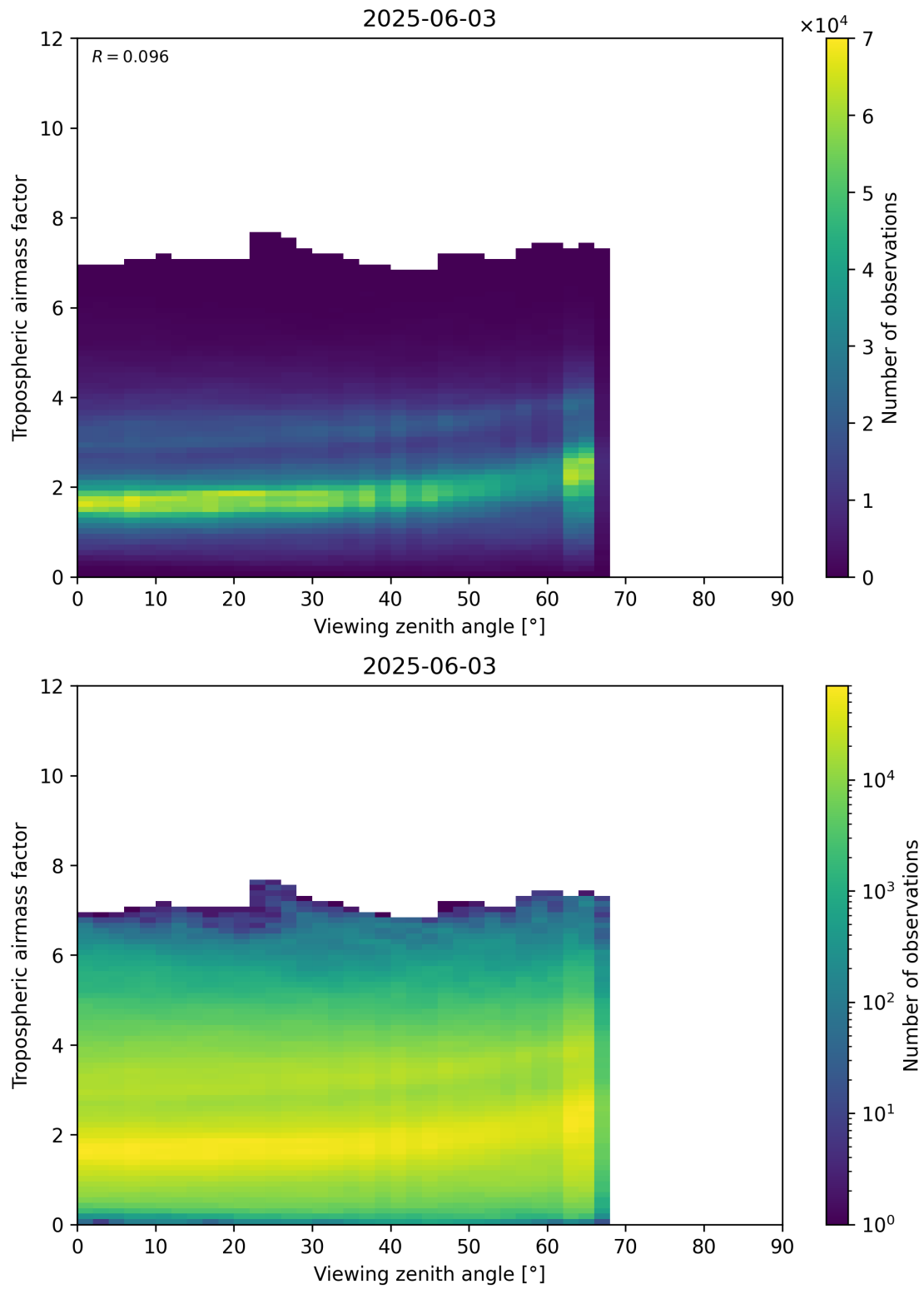
Figure 161: Scatter density plot of “Viewing zenith angle” against “Tropospheric airmass factor” for 2025-06-02 to 2025-06-04.
