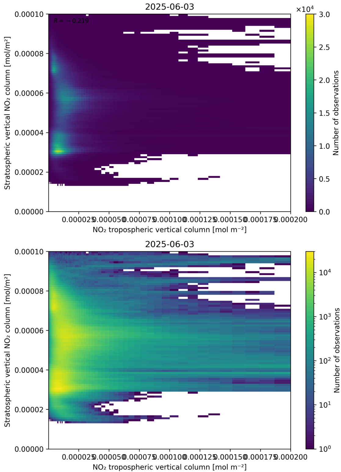
Figure 125: Scatter density plot of “NO 2 tropospheric vertical column” against “Stratospheric vertical NO 2 column” for 2025-06-02 to 2025-06-04.
