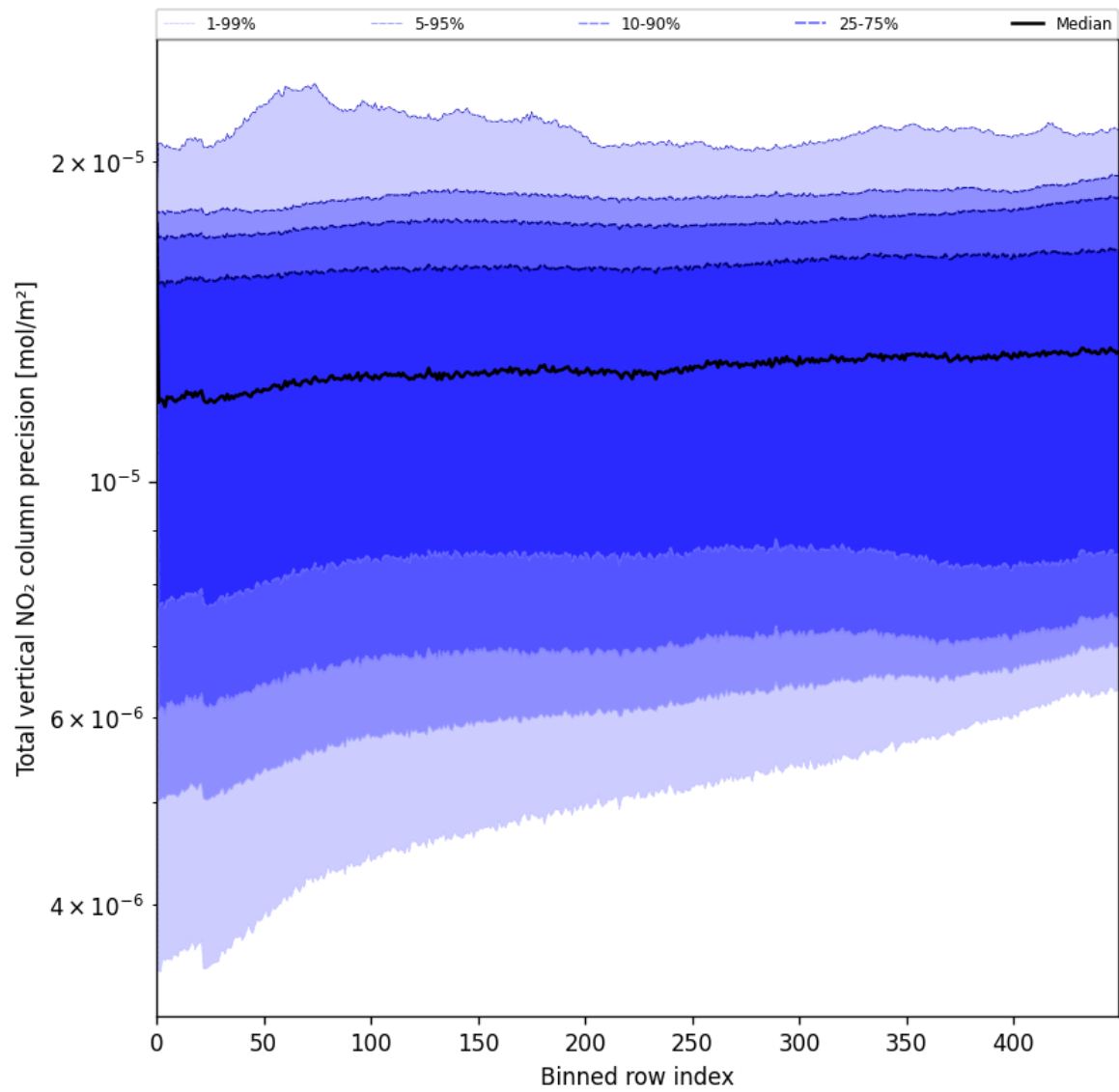
Figure 56: Along track statistics of "Total vertical NO 2 column precision" for 2025-06-02 to 2025-06-04
