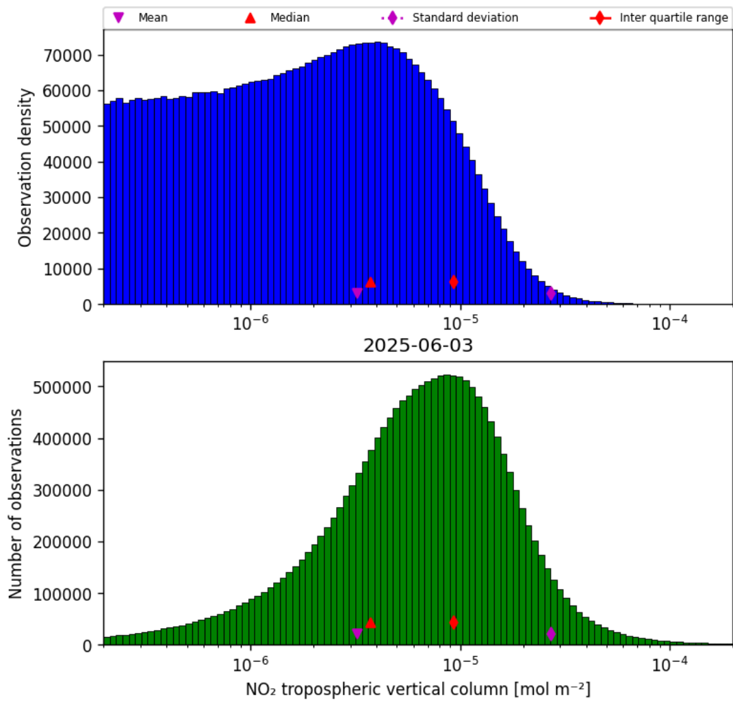
Figure 29: Histogram of “NO 2 tropospheric vertical column” for 2025-06-02 to 2025-06-04
