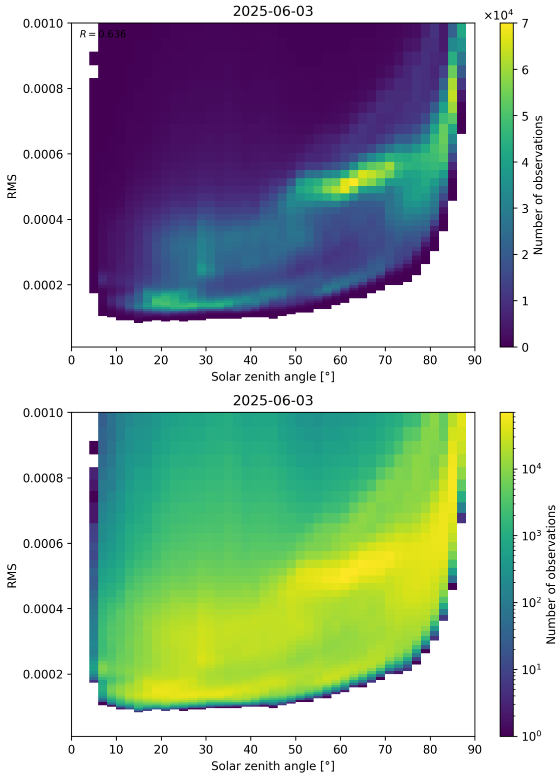
Figure 157: Scatter density plot of “Solar zenith angle” against “RMS” for 2025-06-02 to 2025-06-04.
