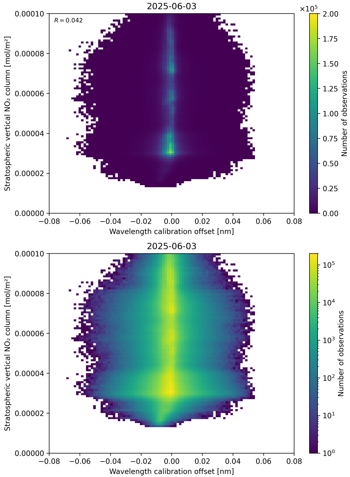
Figure 176: Scatter density plot of “Wavelength calibration offset” against “Stratospheric vertical NO 2 column” for 2025-06-02 to 2025-06-04.
