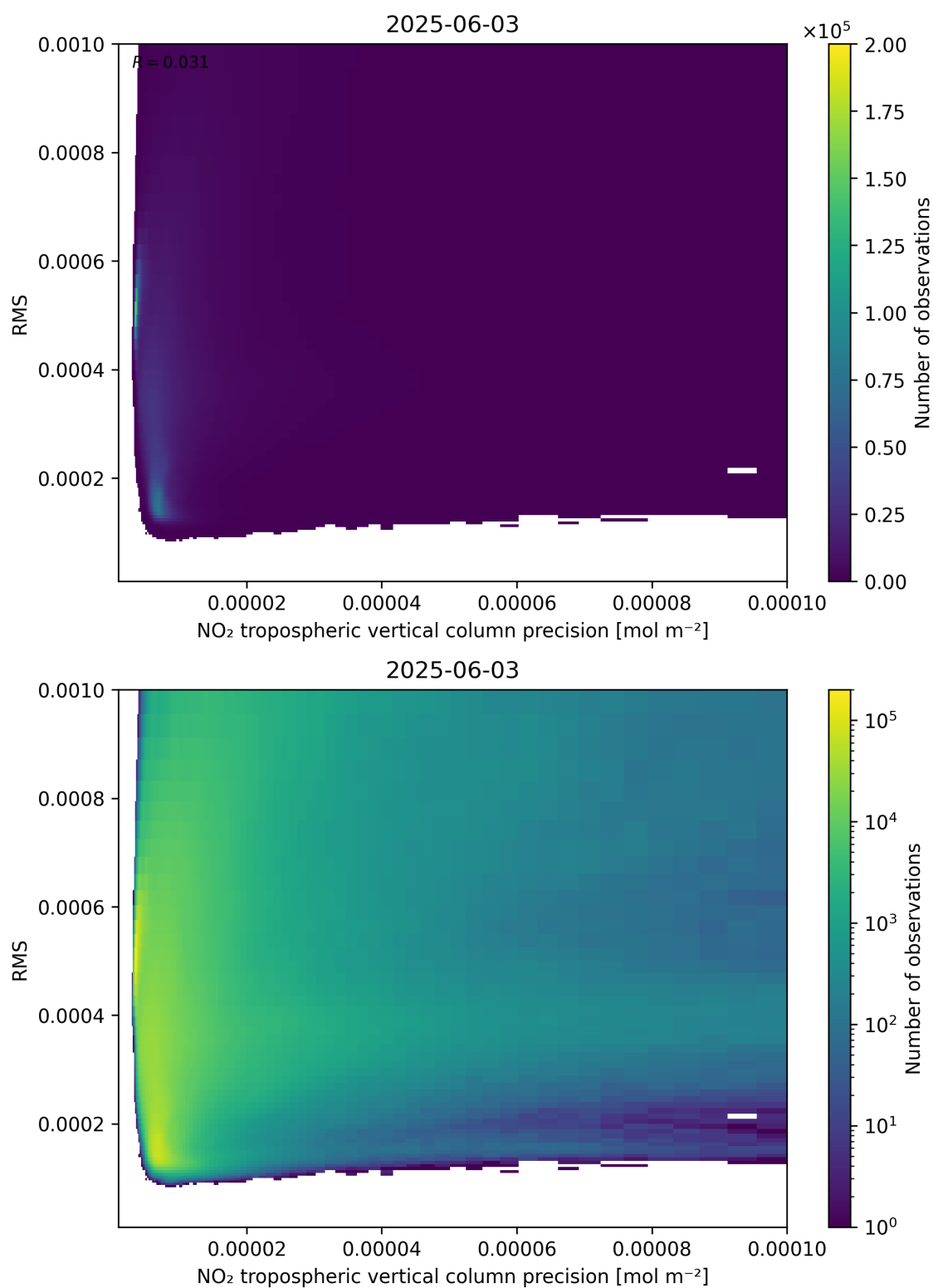
Figure 140: Scatter density plot of “NO 2 tropospheric vertical column precision” against “RMS” for 2025-06-02 to 2025-06-04.
