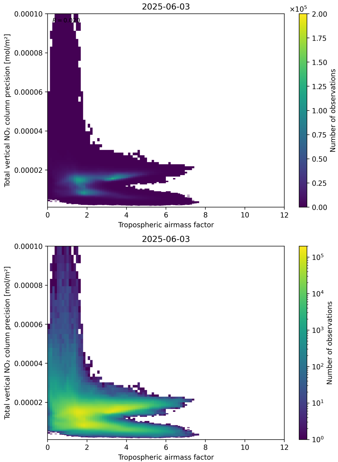
Figure 78: Scatter density plot of “Tropospheric air mass factor” against “Total vertical NO 2 column precision” for 2025-06-02 to 2025-06-04.
