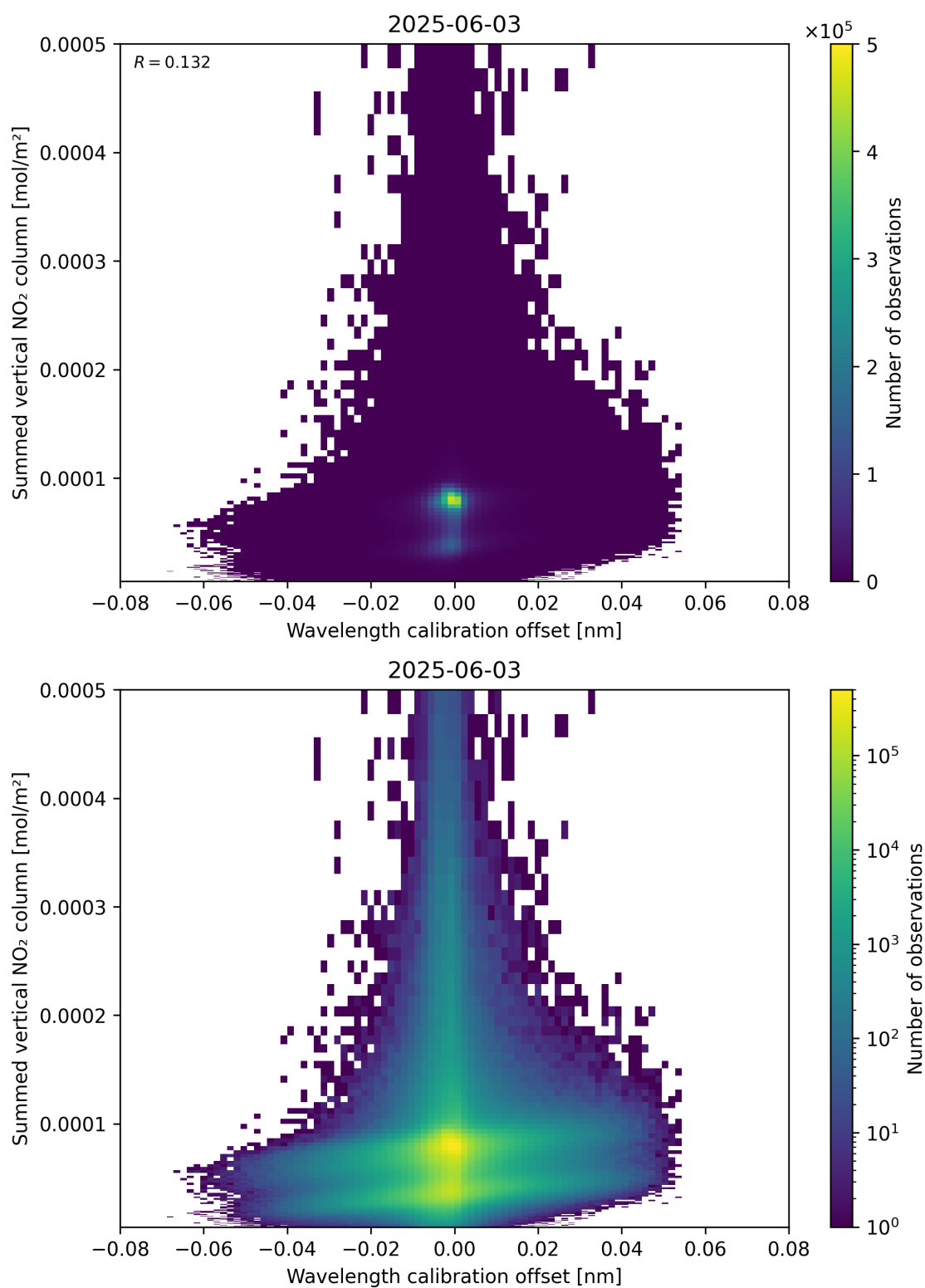
Figure 177: Scatter density plot of “Wavelength calibration offset” against “Summed vertical NO 2 column” for 2025-06-02 to 2025-06-04.
