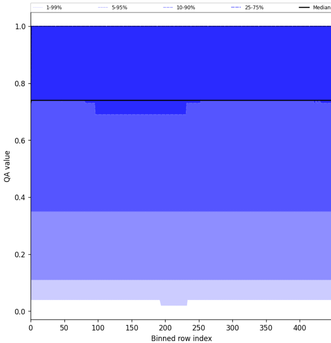
Figure 45: Along track statistics of “QA value” for 2025-06-02 to 2025-06-04
