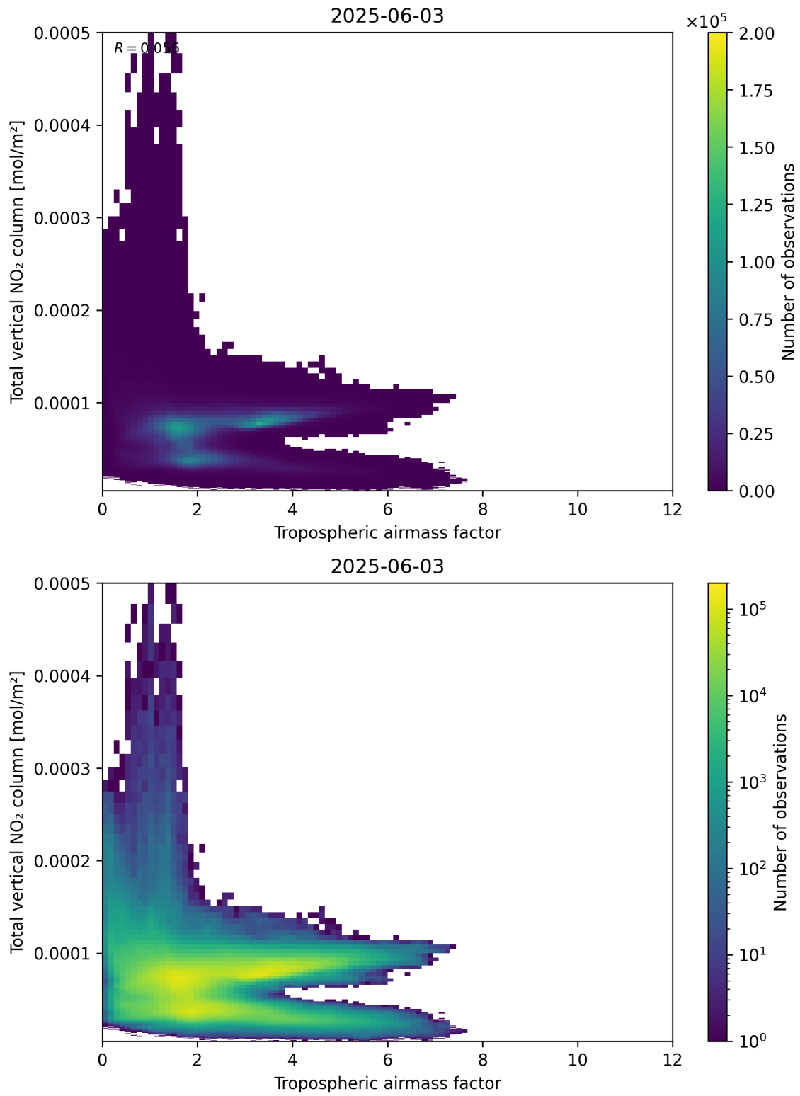
Figure 77: Scatter density plot of “Tropospheric airmass factor” against “Total vertical NO 2 column” for 2025-06-02 to 2025-06-04.
