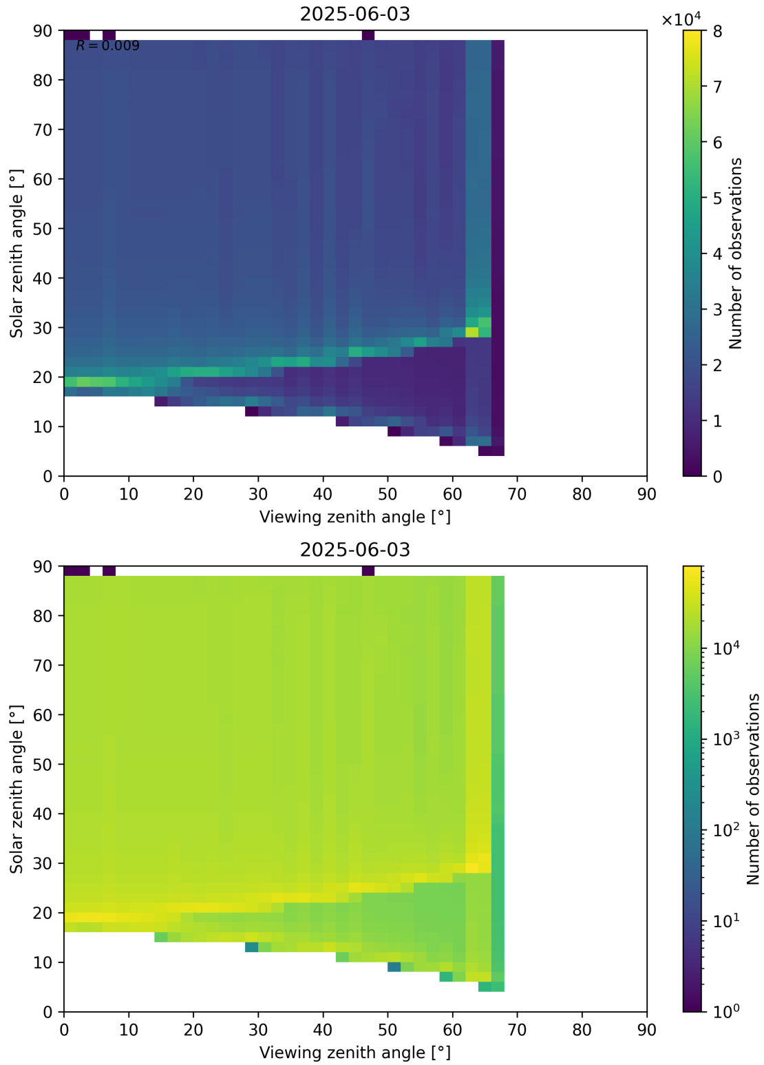
Figure 172: Scatter density plot of “Viewing zenith angle” against “Solar zenith angle” for 2025-06-02 to 2025-06-04.
