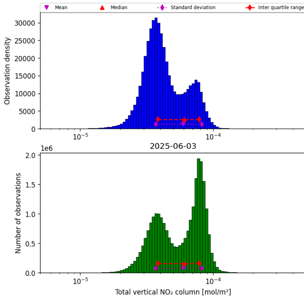
Figure 38: Histogram of “Total vertical NO 2 column” for 2025-06-02 to 2025-06-04
