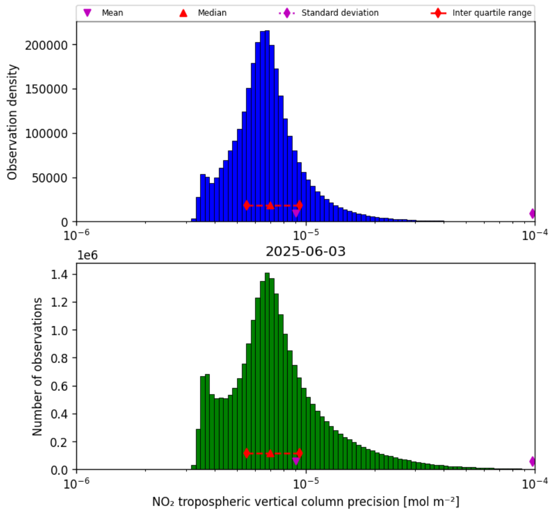
Figure 30: Histogram of “NO 2 tropospheric vertical column precision” for 2025-06-02 to 2025-06-04
