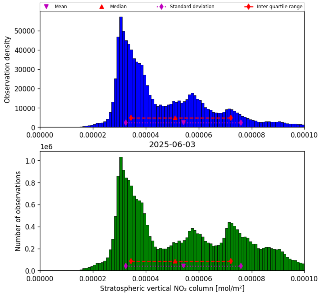
Figure 36: Histogram of “Stratospheric vertical NO 2 column” for 2025-06-02 to 2025-06-04
