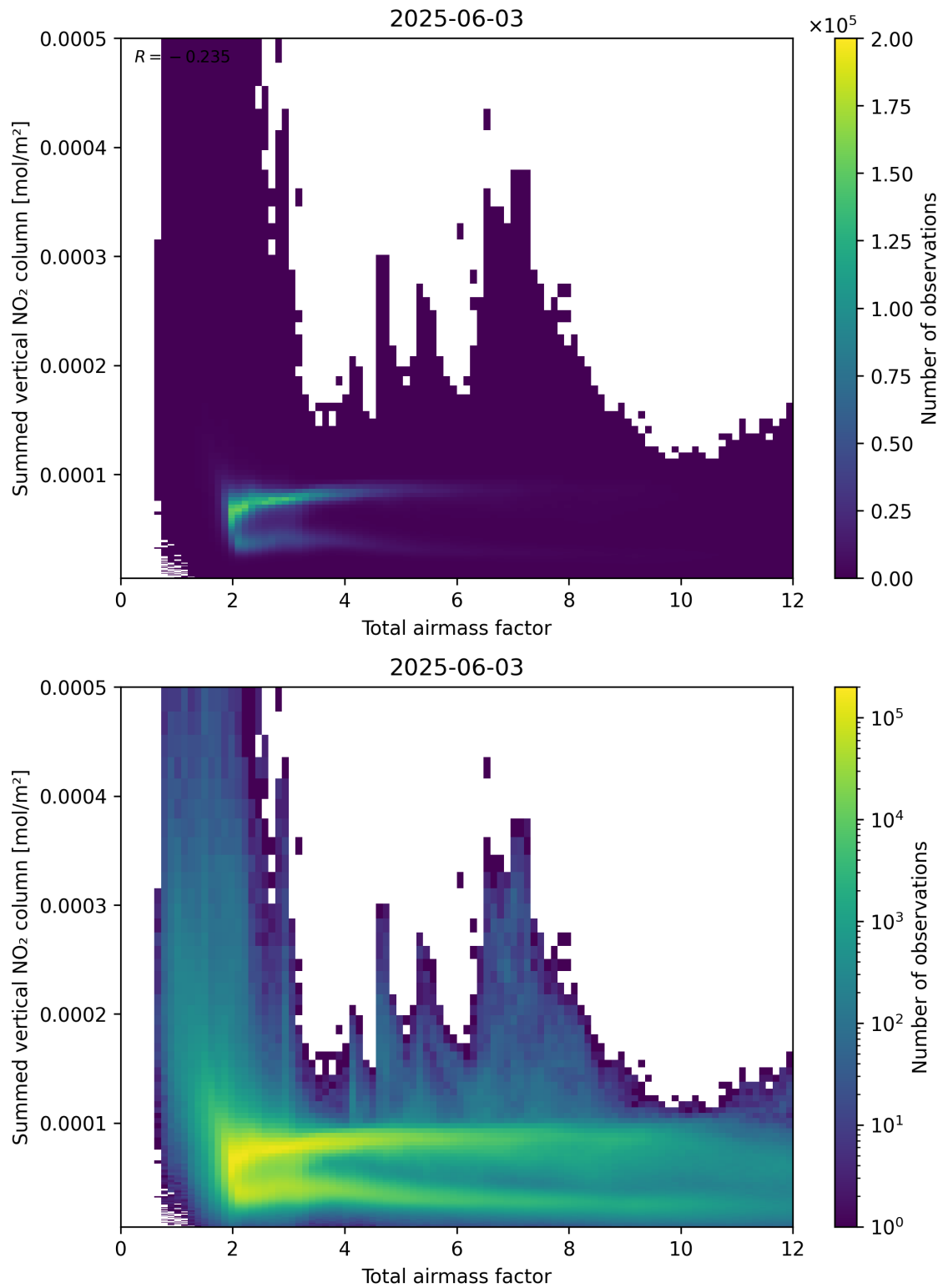
Figure 65: Scatter density plot of “Total airmass factor” against “Summed vertical NO 2 column” for 2025-06-02 to 2025-06-04.
