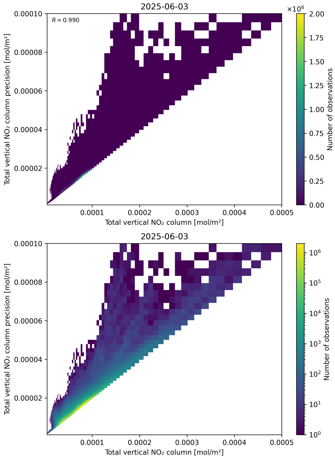
Figure 114: Scatter density plot of “Total vertical NO 2 column” against “Total vertical NO 2 column precision” for 2025-06-02 to 2025-06-04.
