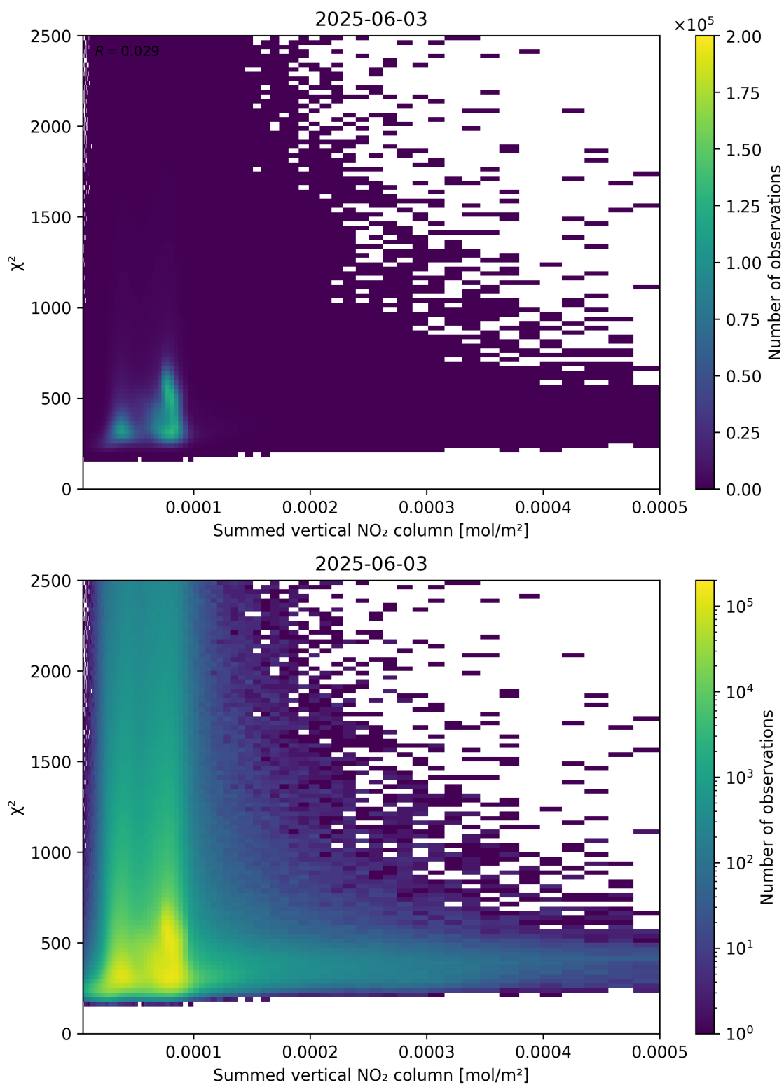
Figure 104: Scatter density plot of “Summed vertical NO 2 column” against “ \chi^2 ” for 2025-06-02 to 2025-06-04.
