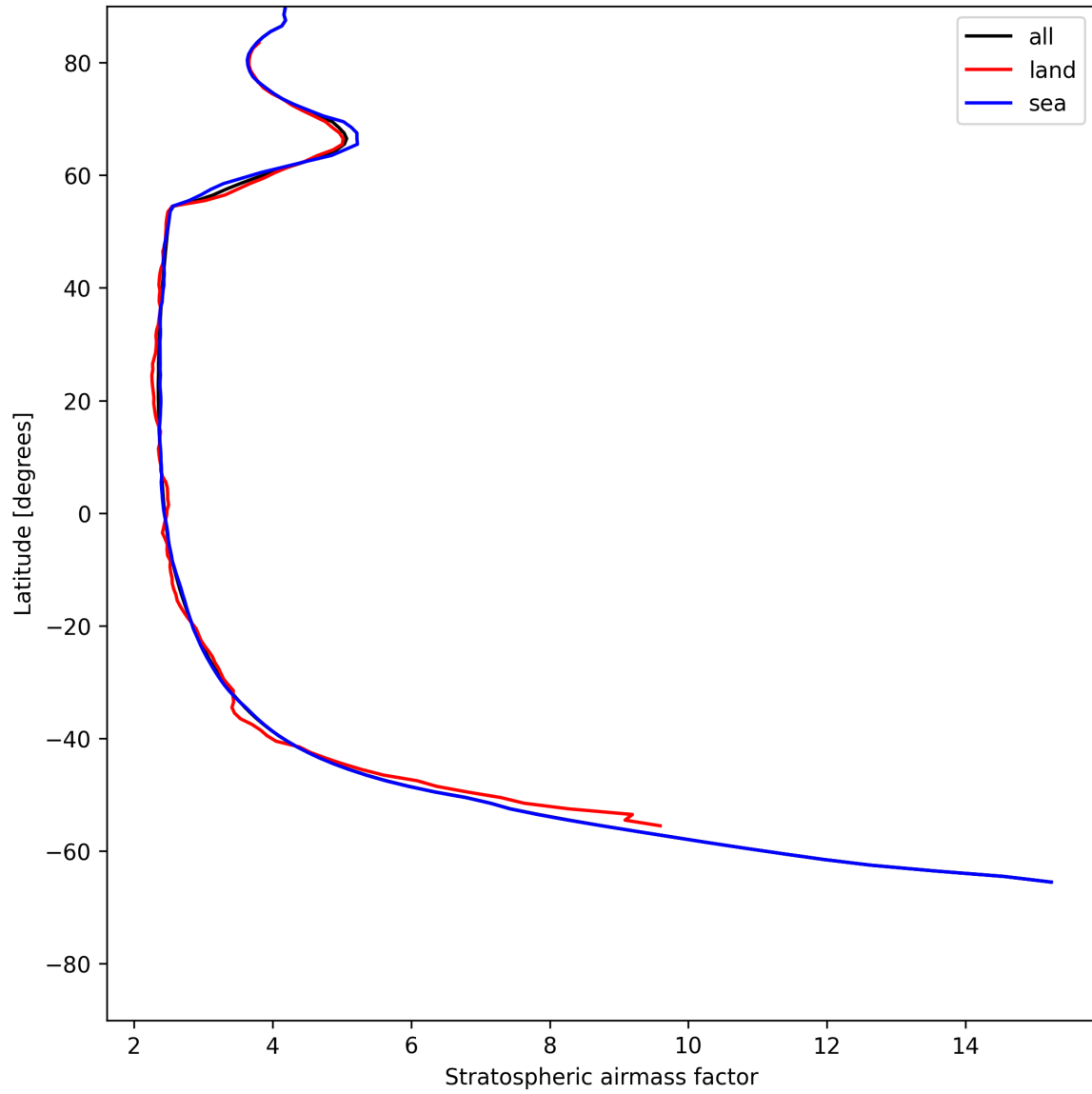
Figure 27: Zonal average of “Stratospheric airmass factor” for 2025-06-02 to 2025-06-04.
