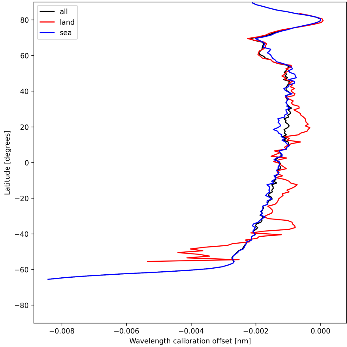
Figure 18: Zonal average of “Wavelength calibration offset” for 2025-06-02 to 2025-06-04.
