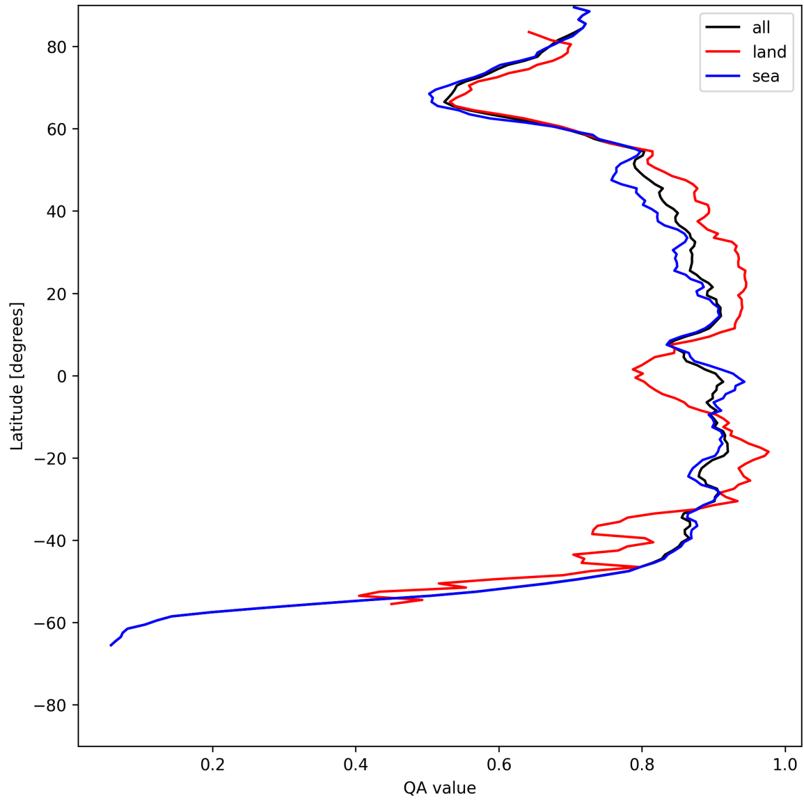
Figure 11: Zonal average of “QA value” for 2025-06-02 to 2025-06-04.
