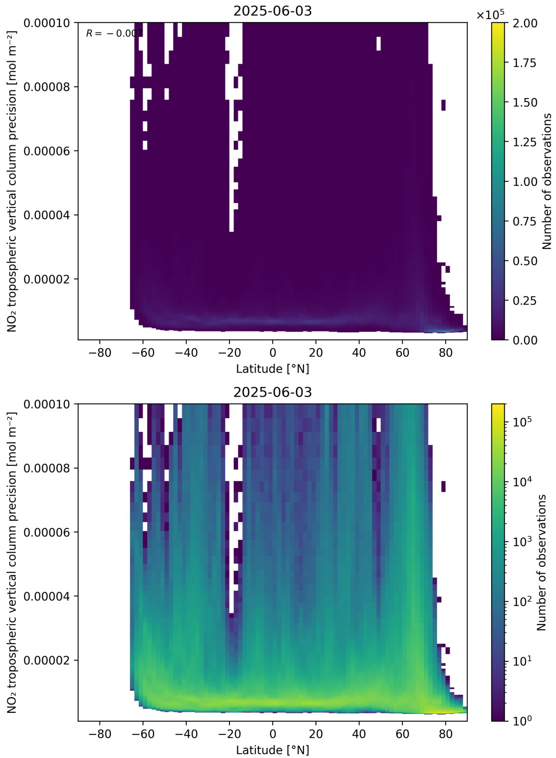
Figure 93: Scatter density plot of “Latitude” against “NO 2 tropospheric vertical column precision” for 2025-06-02 to 2025-06-04.
