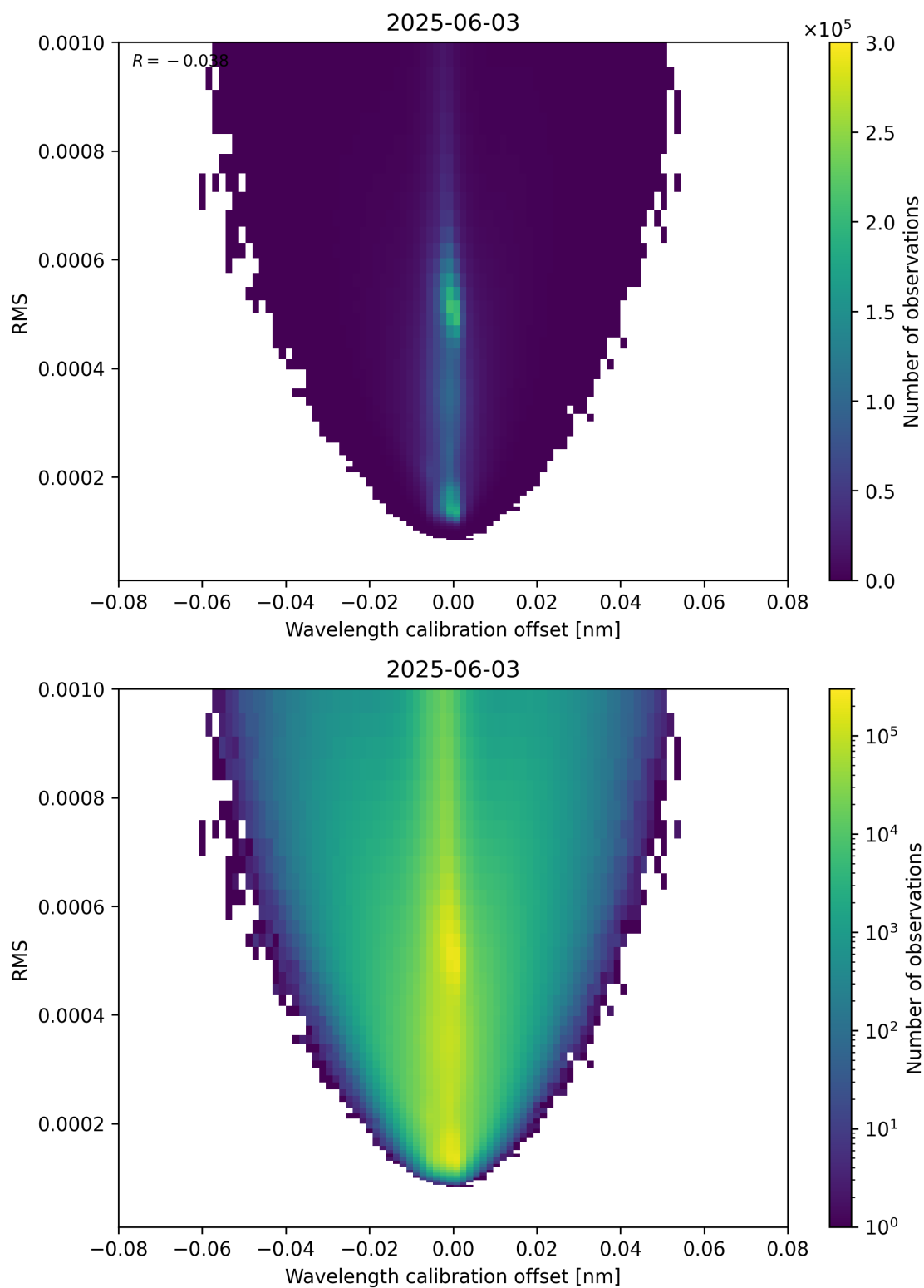
Figure 181: Scatter density plot of “Wavelength calibration offset” against “RMS” for 2025-06-02 to 2025-06-04.
