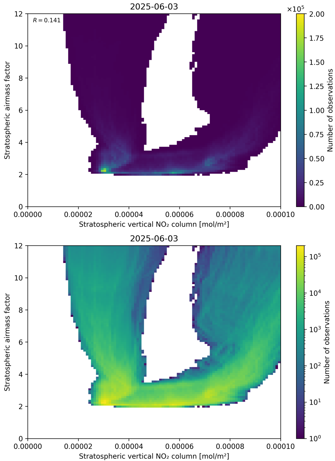
Figure 96: Scatter density plot of “Stratospheric vertical NO 2 column” against “Stratospheric airmass factor” for 2025-06-02 to 2025-06-04.
