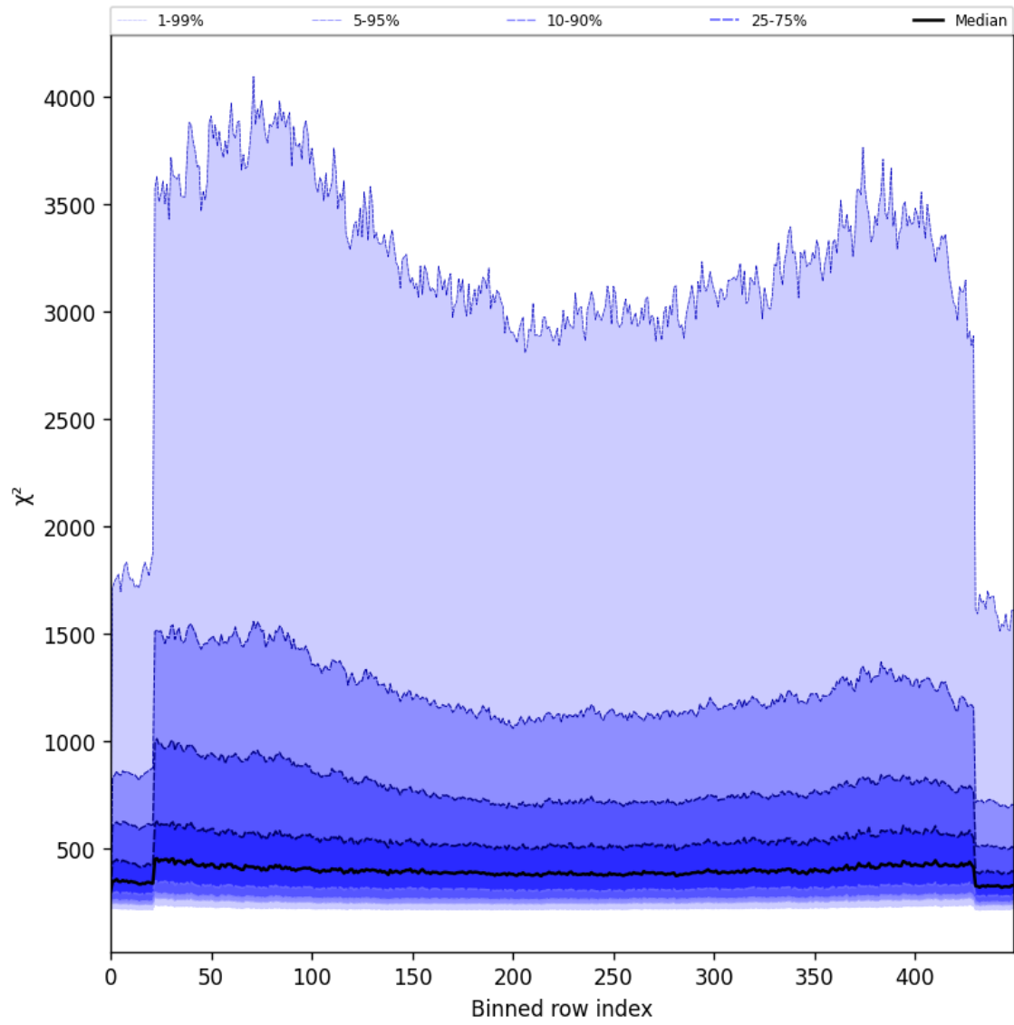
Figure 59: Along track statistics of “ \chi^2 ” for 2025-06-02 to 2025-06-04
