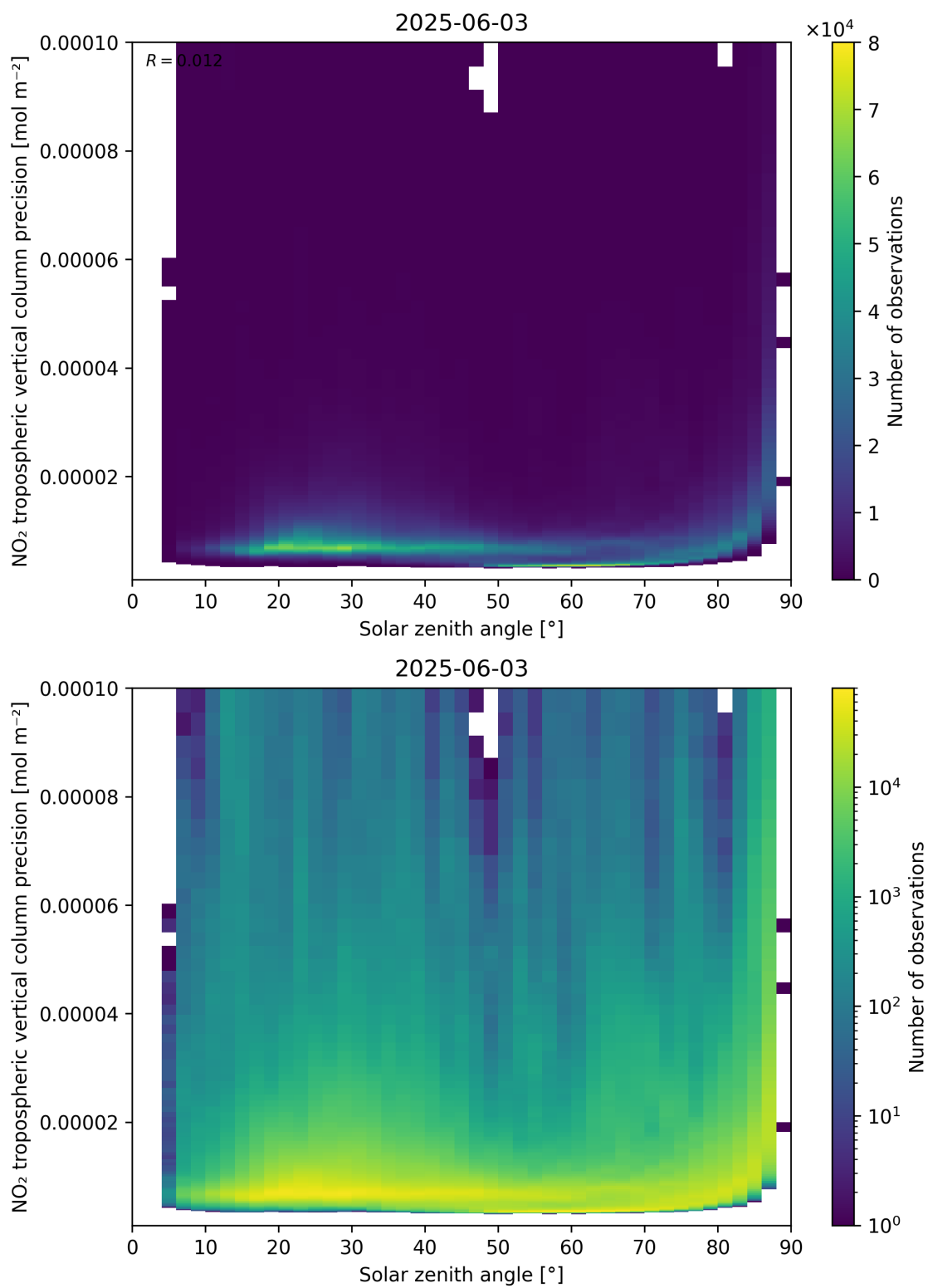
Figure 156: Scatter density plot of “Solar zenith angle” against “NO 2 tropospheric vertical column precision” for 2025-06-02 to 2025-06-04.
