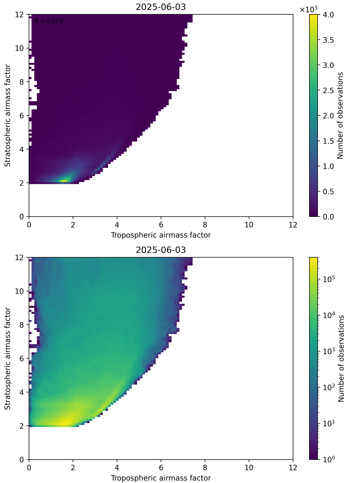
Figure 71: Scatter density plot of “Tropospheric airmass factor” against “Stratospheric airmass factor” for 2025-06-02 to 2025-06-04.
