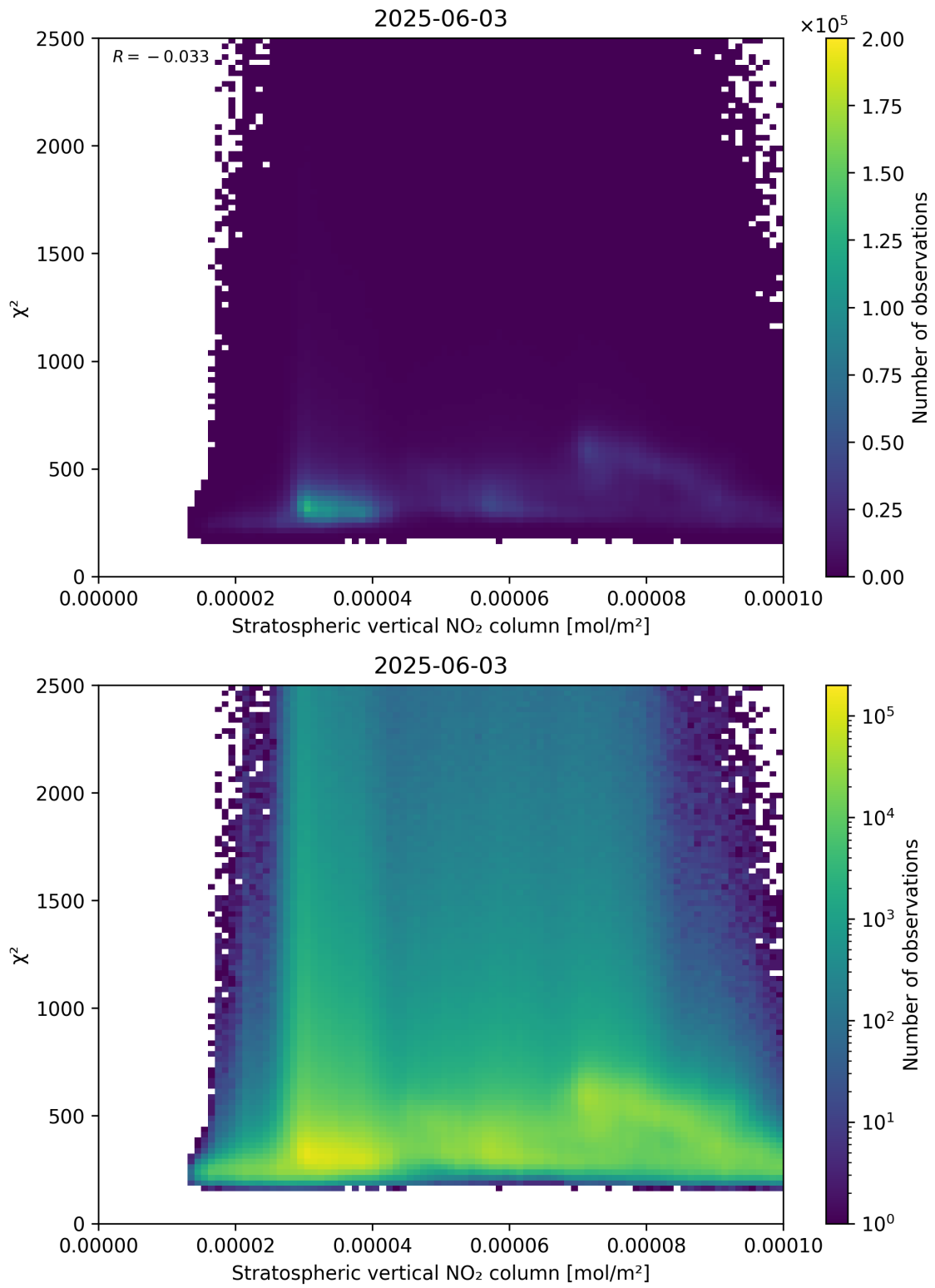
Figure 97: Scatter density plot of “Stratospheric vertical NO 2 column” against “ \chi^2 ” for 2025-06-02 to 2025-06-04.
