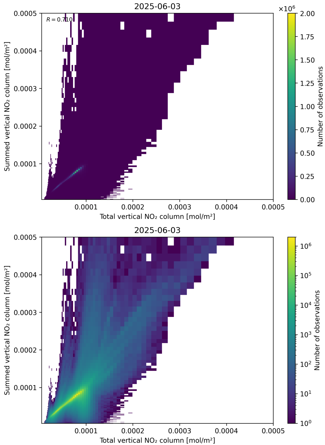
Figure 112: Scatter density plot of “Total vertical NO 2 column” against “Summed vertical NO 2 column” for 2025-06-02 to 2025-06-04.
