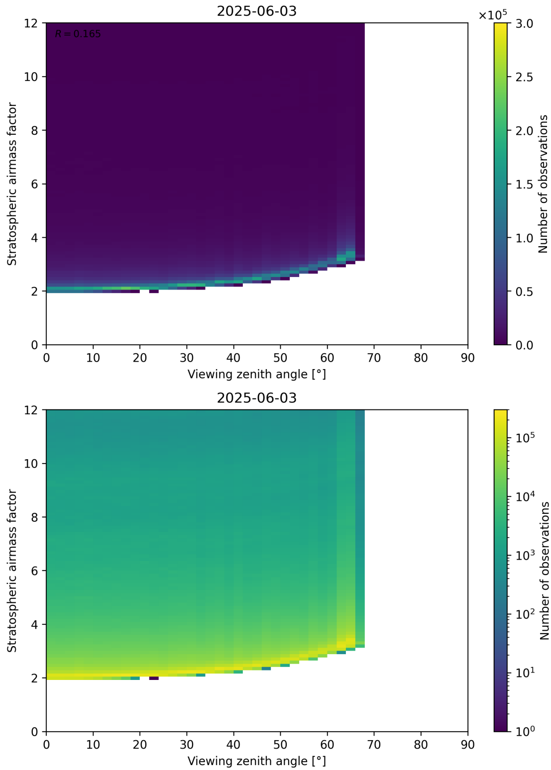
Figure 159: Scatter density plot of “Viewing zenith angle” against “Stratospheric airmass factor” for 2025-06-02 to 2025-06-04.
