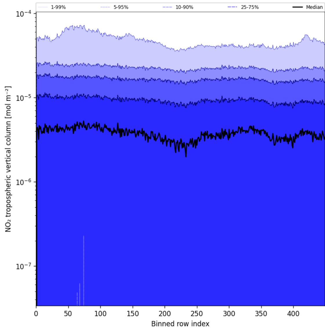
Figure 46: Along track statistics of "NO 2 tropospheric vertical column" for 2025-06-02 to 2025-06-04
