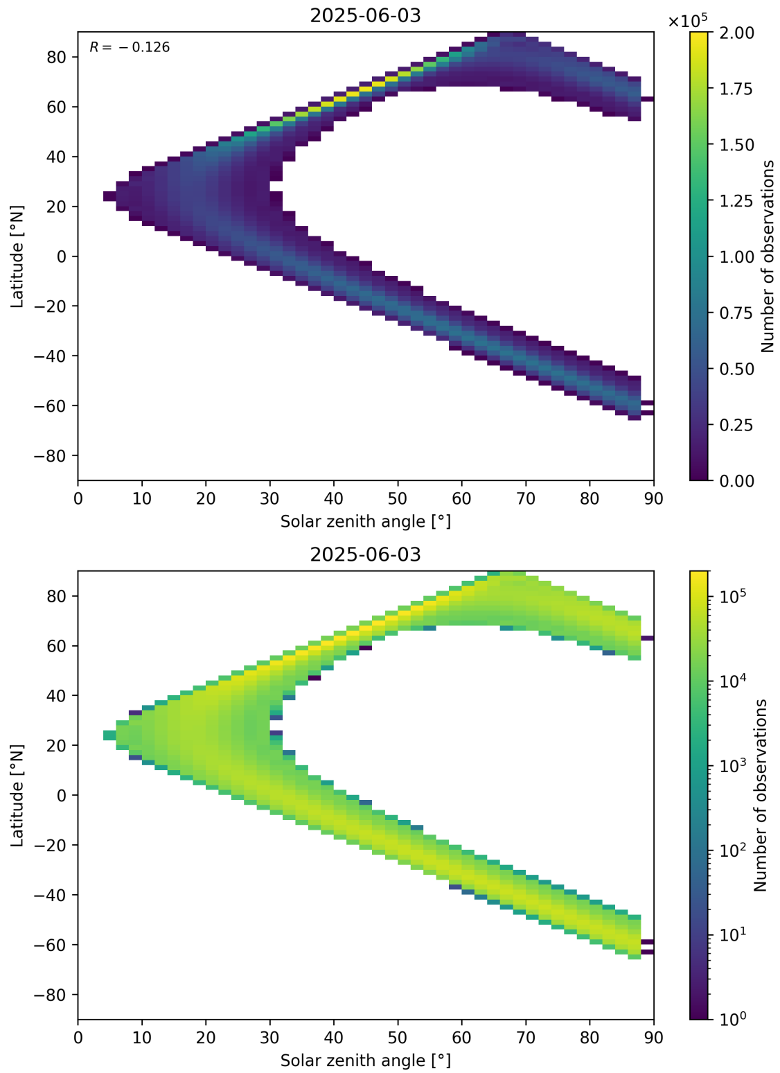
Figure 149: Scatter density plot of “Solar zenith angle” against “Latitude” for 2025-06-02 to 2025-06-04.
