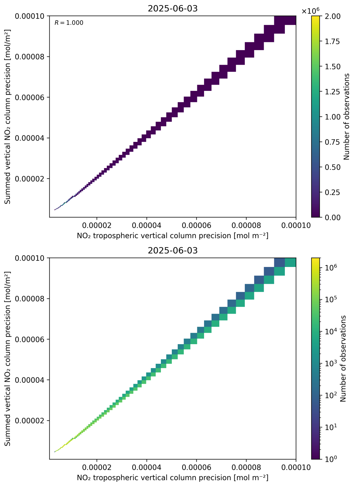
Figure 137: Scatter density plot of “NO 2 tropospheric vertical column precision” against “Summed vertical NO 2 column precision” for 2025-06-02 to 2025-06-04.
