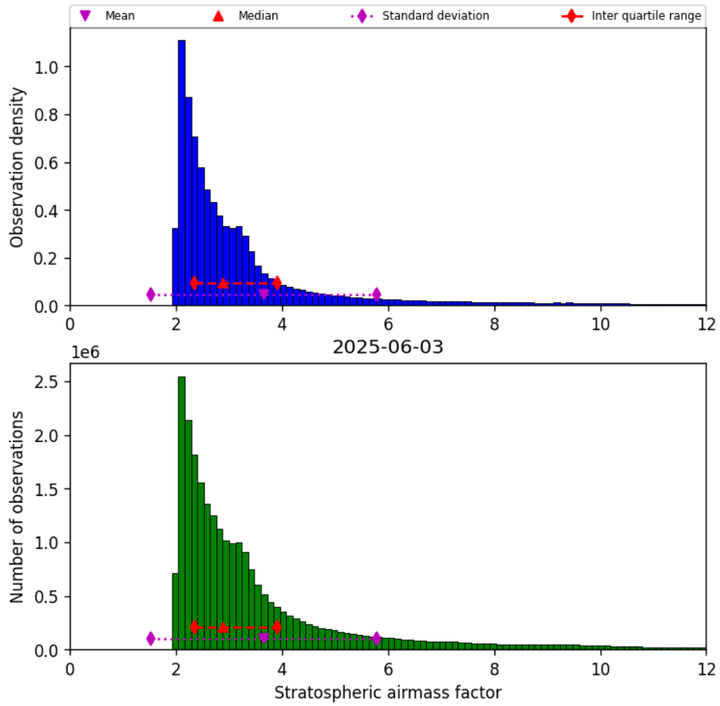
Figure 44: Histogram of “Stratospheric airmass factor” for 2025-06-02 to 2025-06-04
