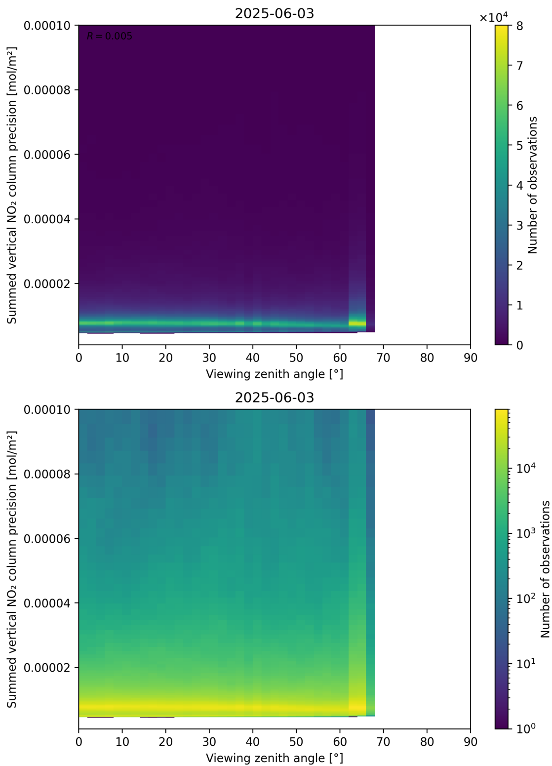
Figure 166: Scatter density plot of “Viewing zenith angle” against “Summed vertical NO 2 column precision” for 2025-06-02 to 2025-06-04.
