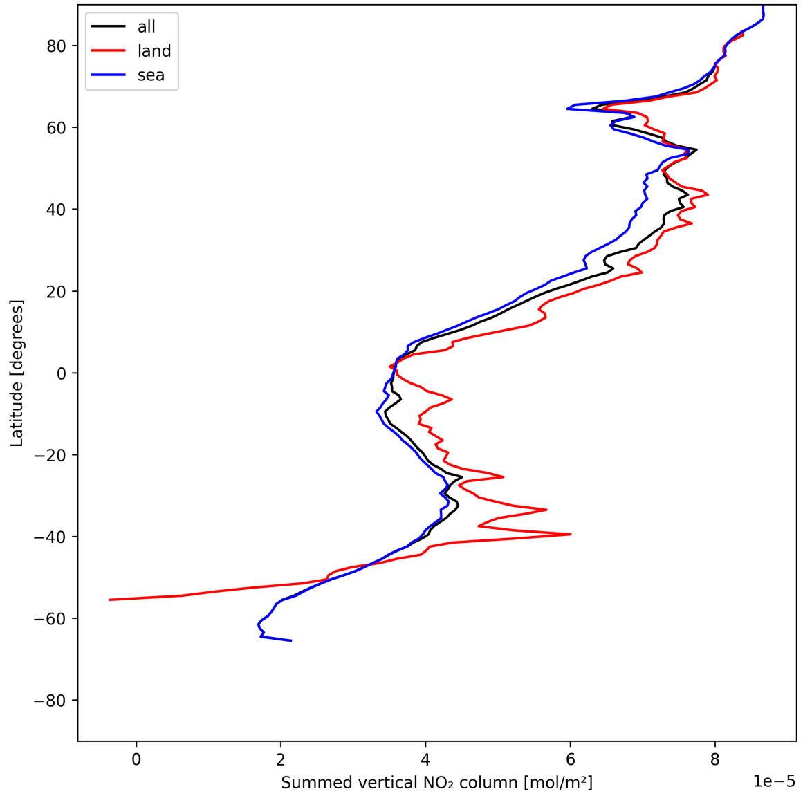
Figure 23: Zonal average of “Summed vertical NO 2 column” for 2025-06-02 to 2025-06-04.
