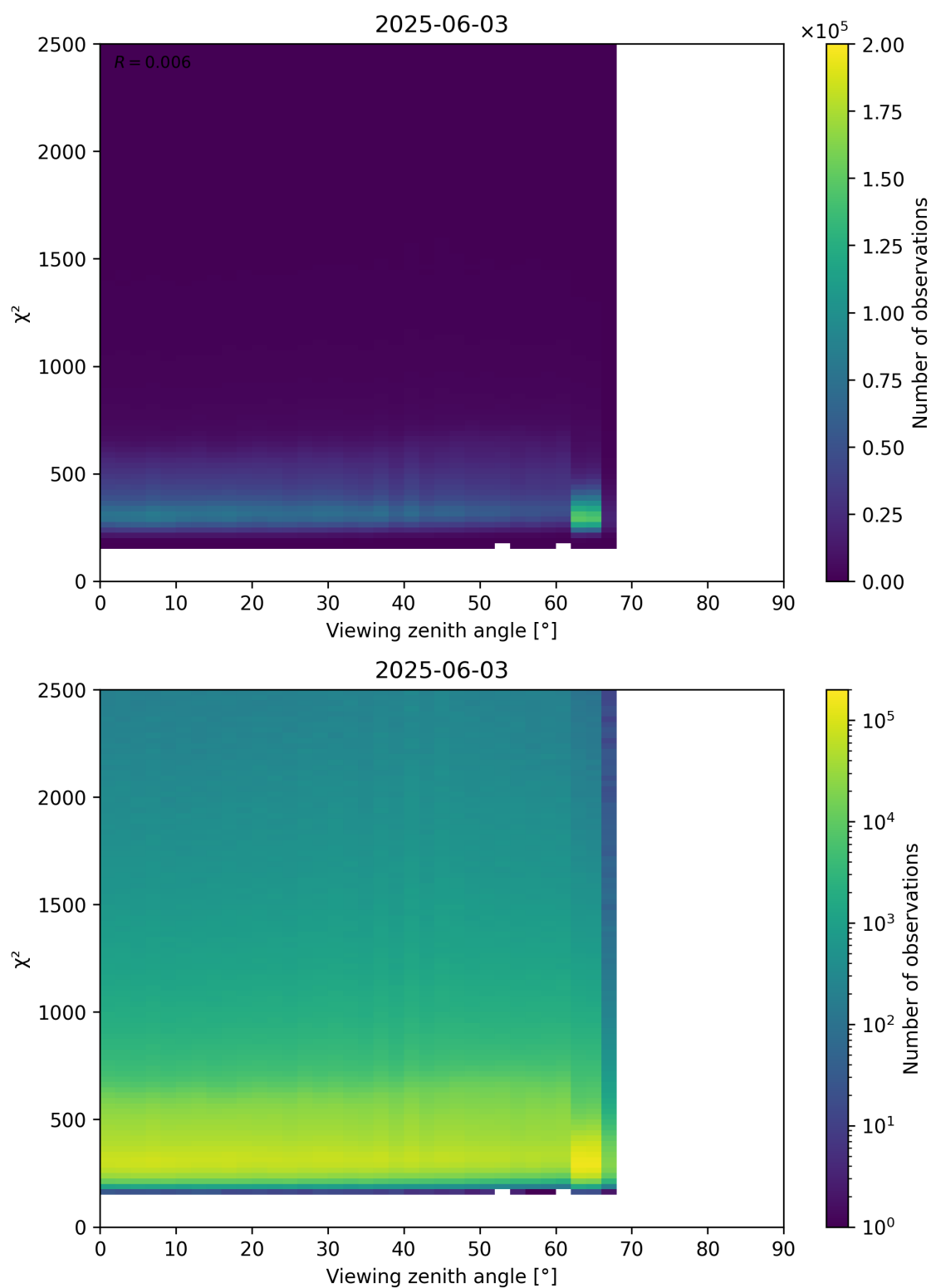
Figure 162: Scatter density plot of “Viewing zenith angle” against “ \chi^2 ” for 2025-06-02 to 2025-06-04.
