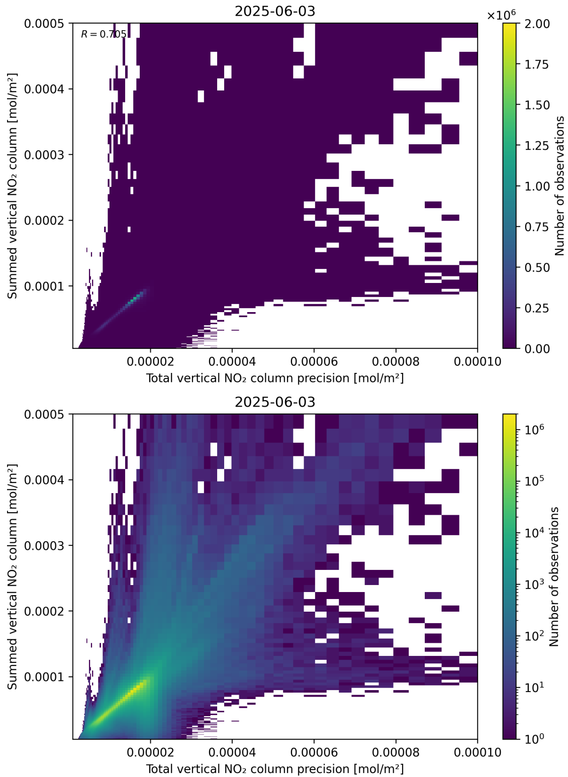
Figure 117: Scatter density plot of “Total vertical NO 2 column precision” against “Summed vertical NO 2 column” for 2025-06-02 to 2025-06-04.
