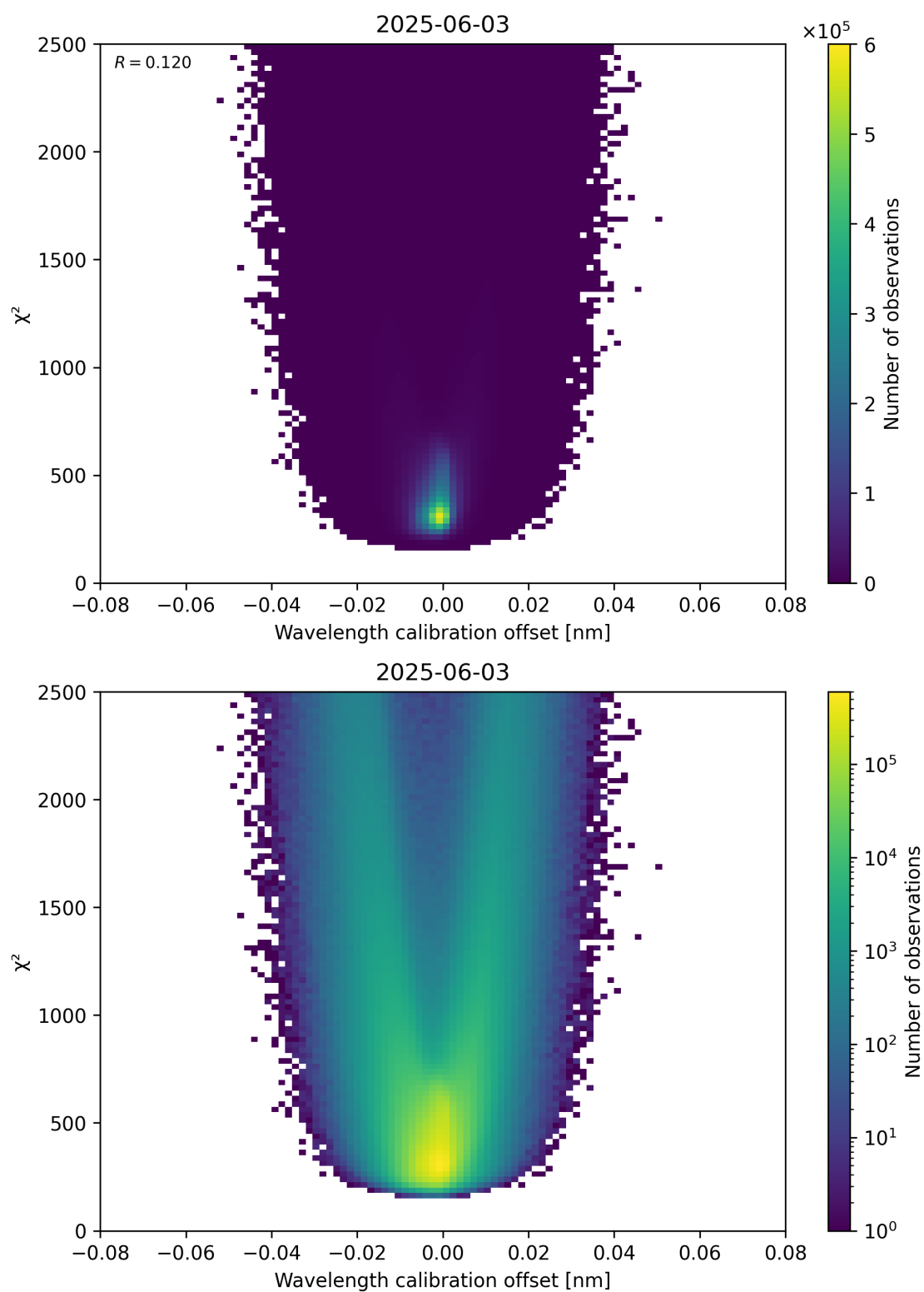
Figure 175: Scatter density plot of “Wavelength calibration offset” against “ \chi^2 ” for 2025-06-02 to 2025-06-04.
