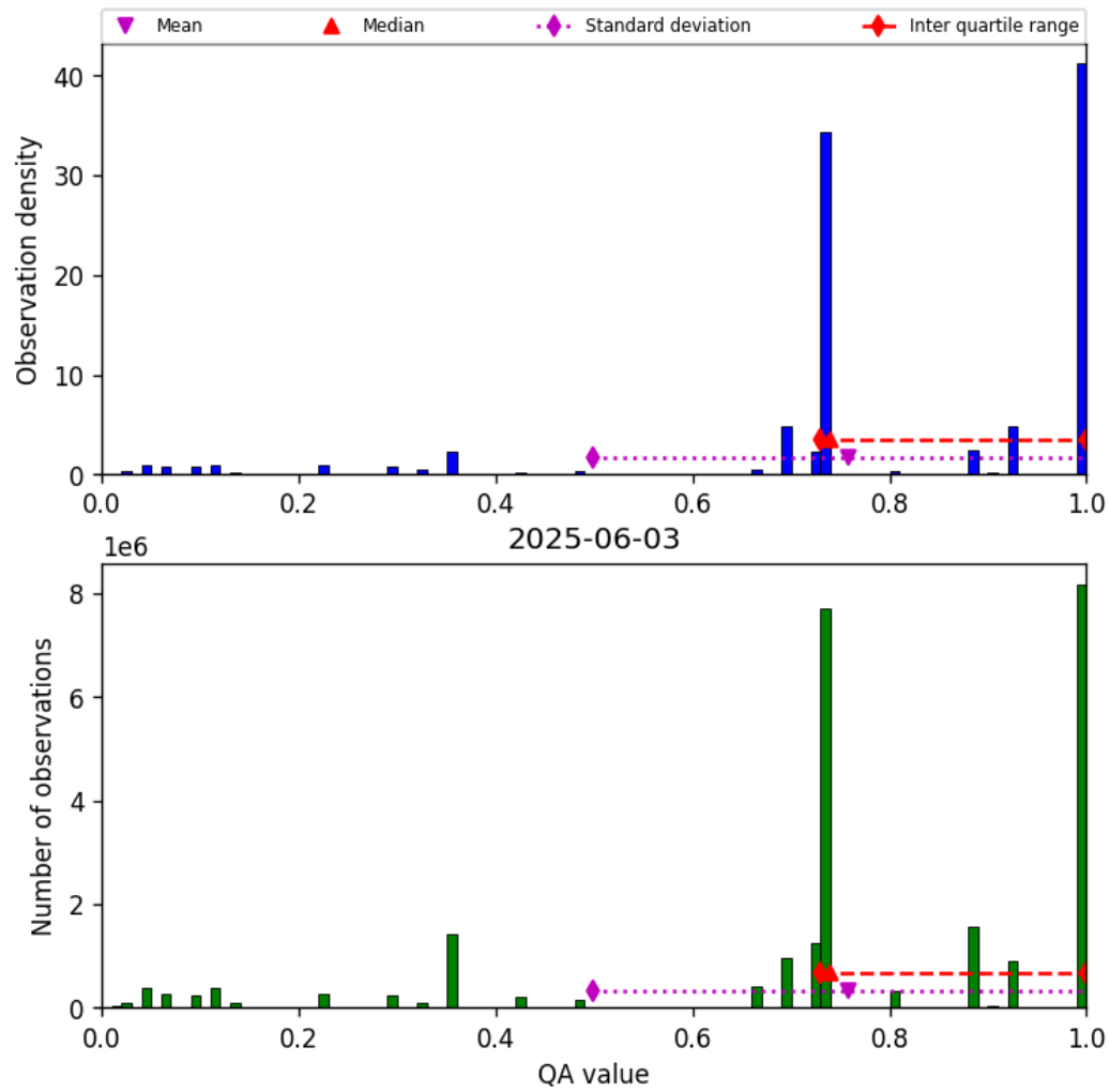
Figure 28: Histogram of “QA value” for 2025-06-02 to 2025-06-04
