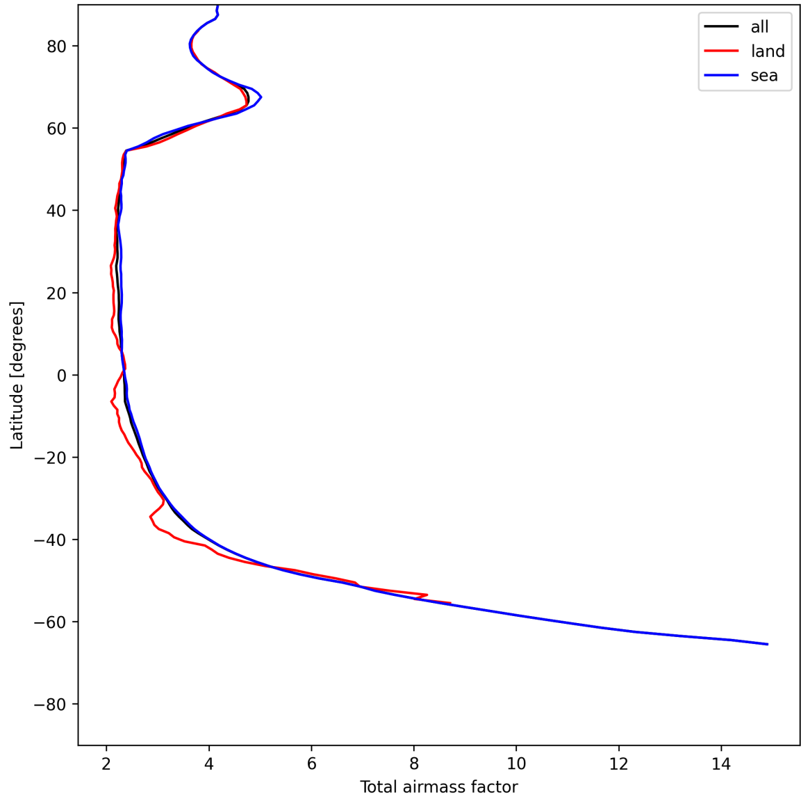
Figure 15: Zonal average of “Total airmass factor” for 2025-06-02 to 2025-06-04.
