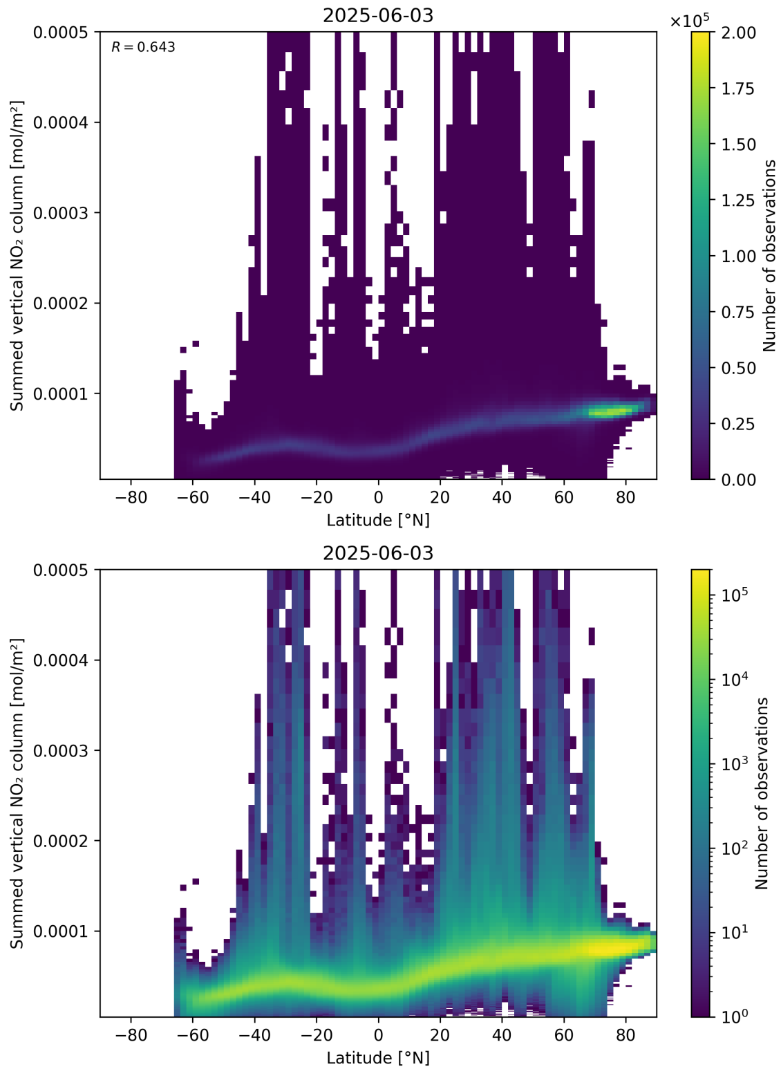
Figure 88: Scatter density plot of “Latitude” against “Summed vertical NO 2 column” for 2025-06-02 to 2025-06-04.
