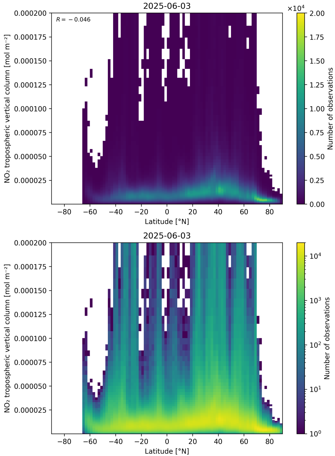
Figure 92: Scatter density plot of “Latitude” against “NO 2 tropospheric vertical column” for 2025-06-02 to 2025-06-04.
