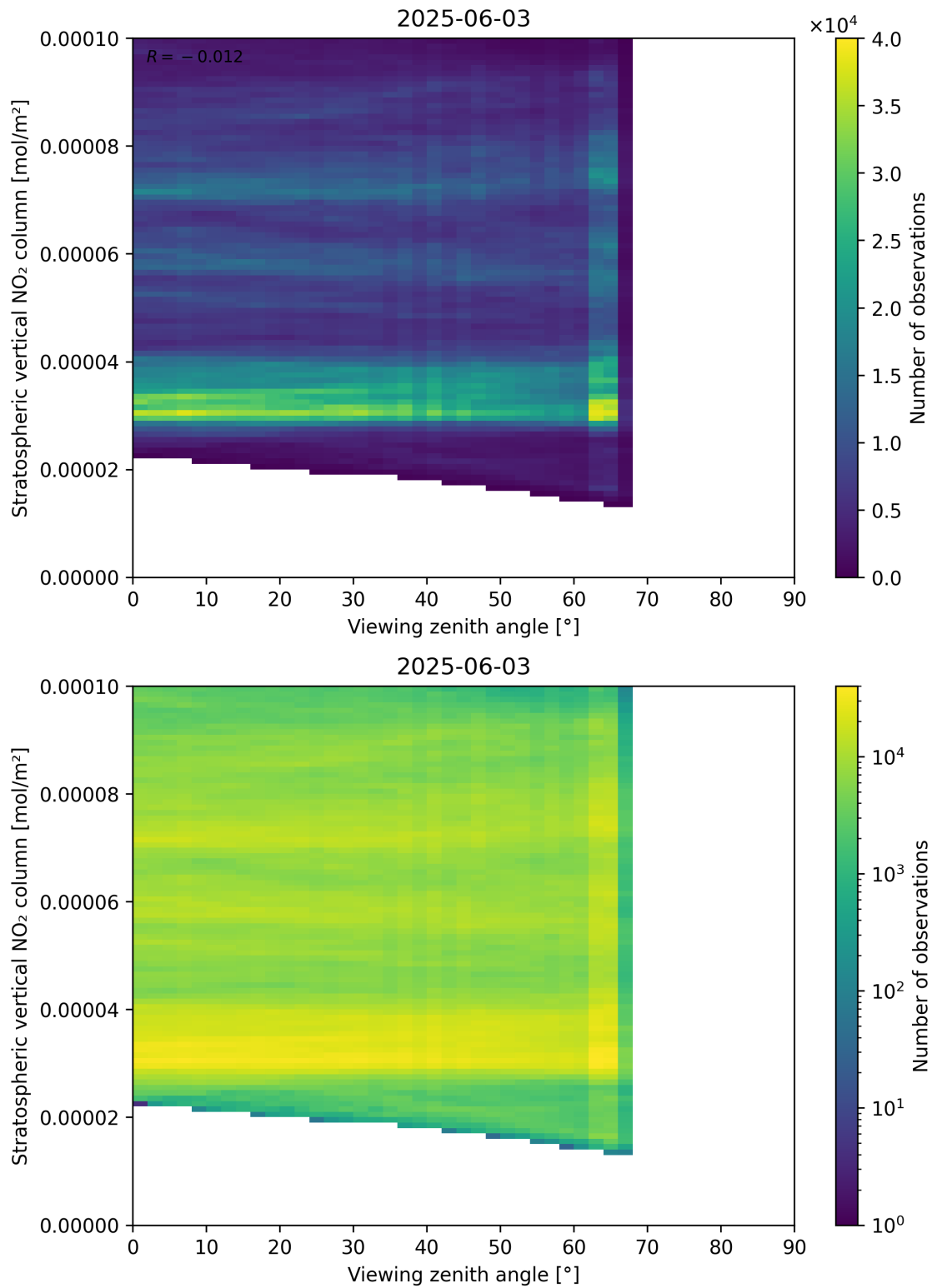
Figure 164: Scatter density plot of “Viewing zenith angle” against “Stratospheric vertical NO 2 column” for 2025-06-02 to 2025-06-04.
