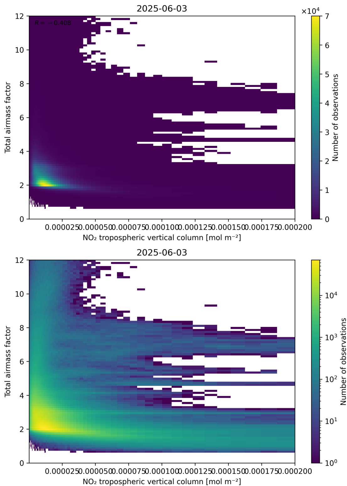
Figure 122: Scatter density plot of “NO 2 tropospheric vertical column” against “Total air mass factor” for 2025-06-02 to 2025-06-04.
