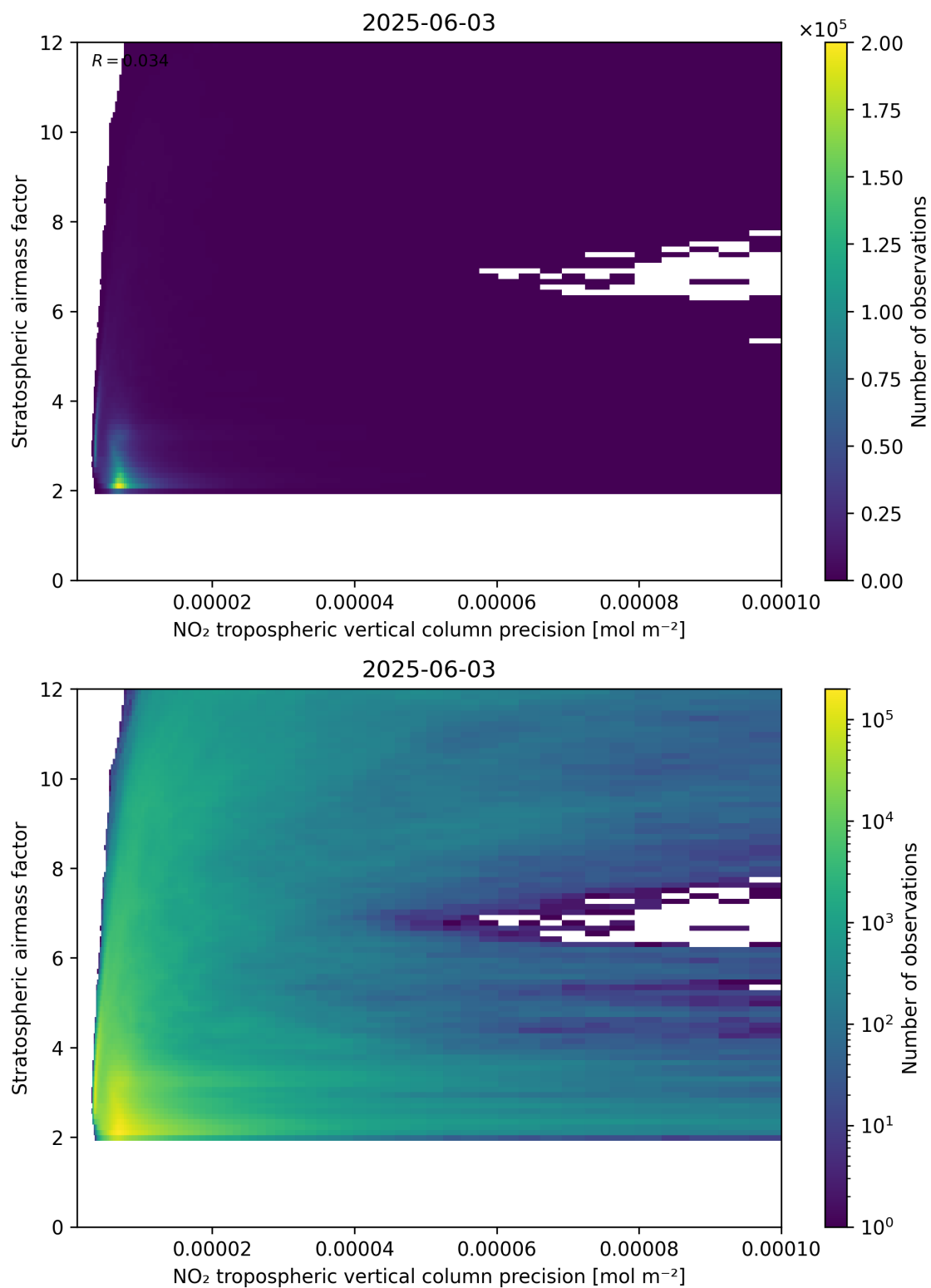
Figure 131: Scatter density plot of “NO 2 tropospheric vertical column precision” against “Stratospheric airmass factor” for 2025-06-02 to 2025-06-04.
