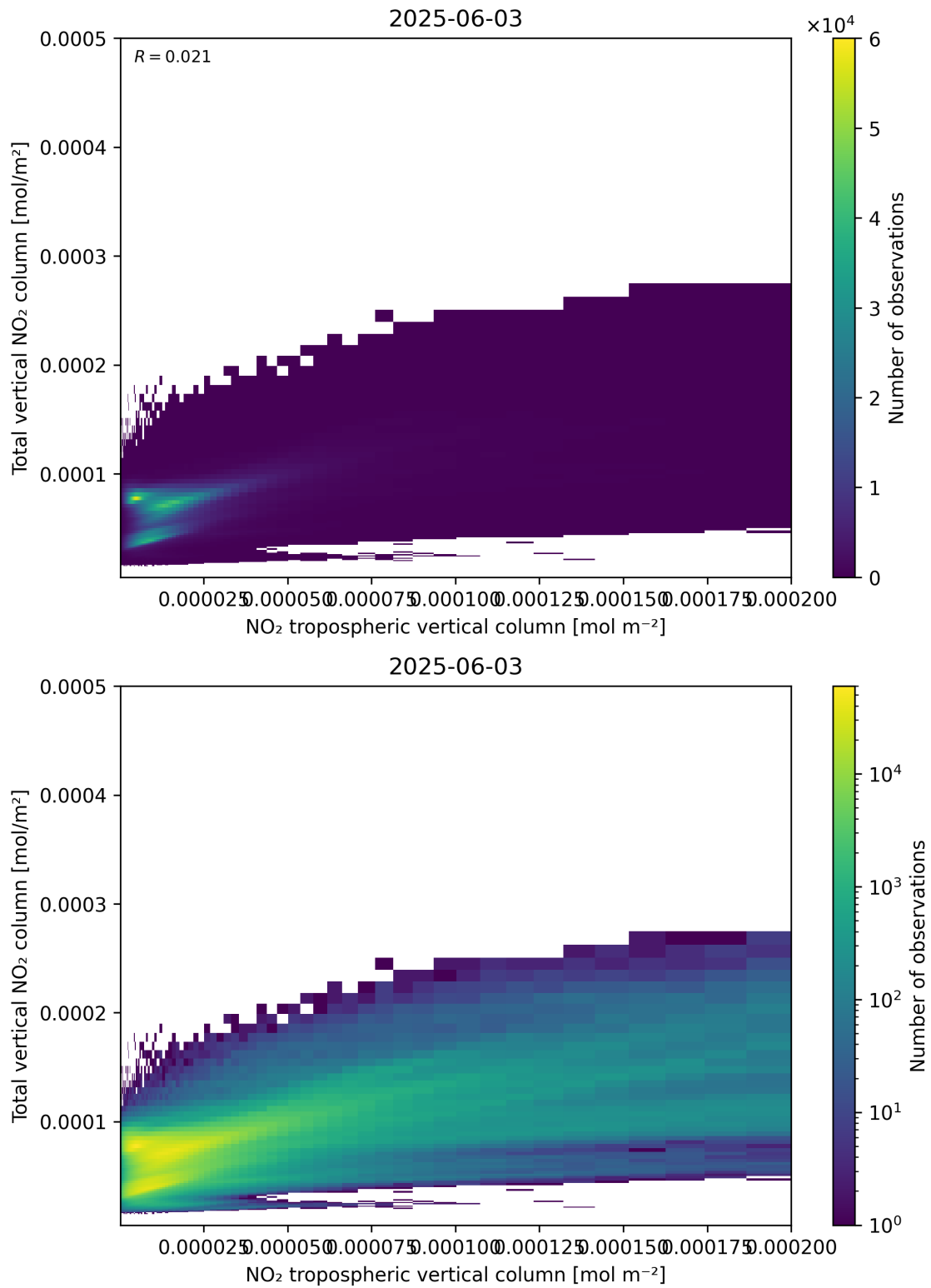
Figure 128: Scatter density plot of “NO 2 tropospheric vertical column” against “Total vertical NO 2 column” for 2025-06-02 to 2025-06-04.
