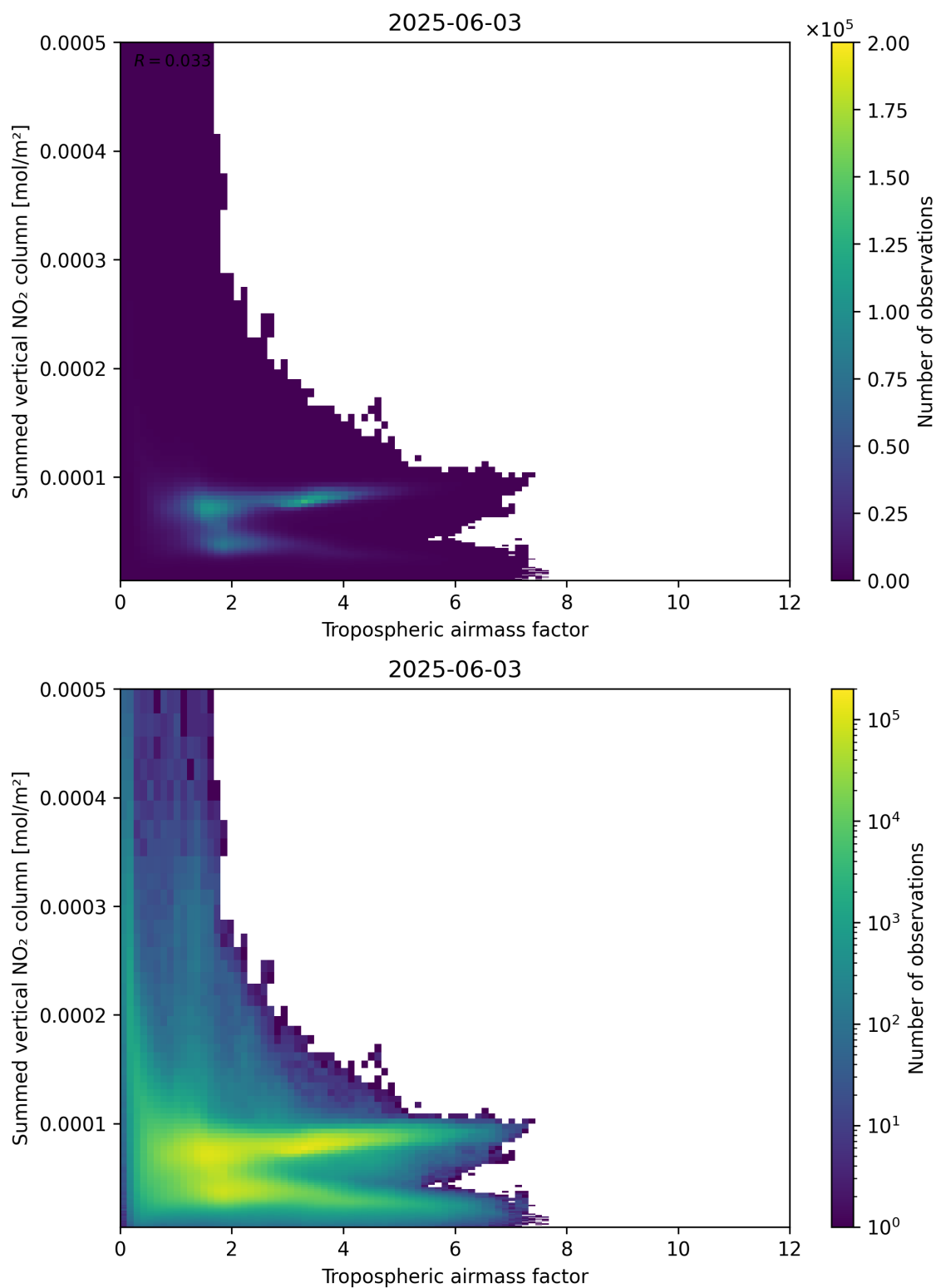
Figure 75: Scatter density plot of “Tropospheric airmass factor” against “Summed vertical NO 2 column” for 2025-06-02 to 2025-06-04.
