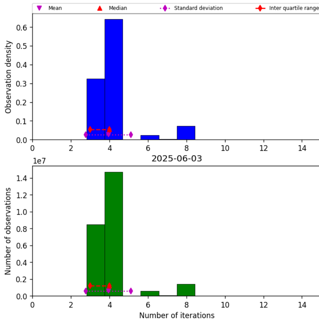
Figure 34: Histogram of “Number of iterations” for 2025-06-02 to 2025-06-04
