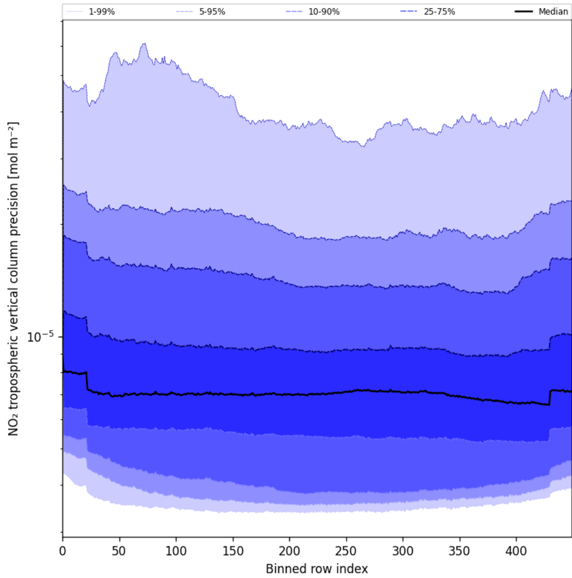
Figure 47: Along track statistics of “NO 2 tropospheric vertical column precision” for 2025-06-02 to 2025-06-04
