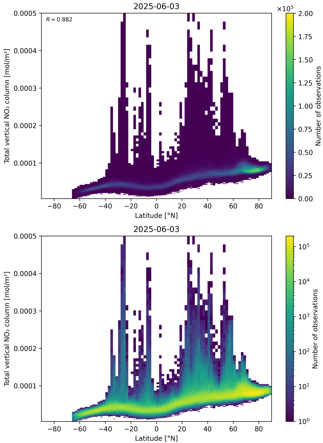
Figure 90: Scatter density plot of “Latitude” against “Total vertical NO 2 column” for 2025-06-02 to 2025-06-04.
