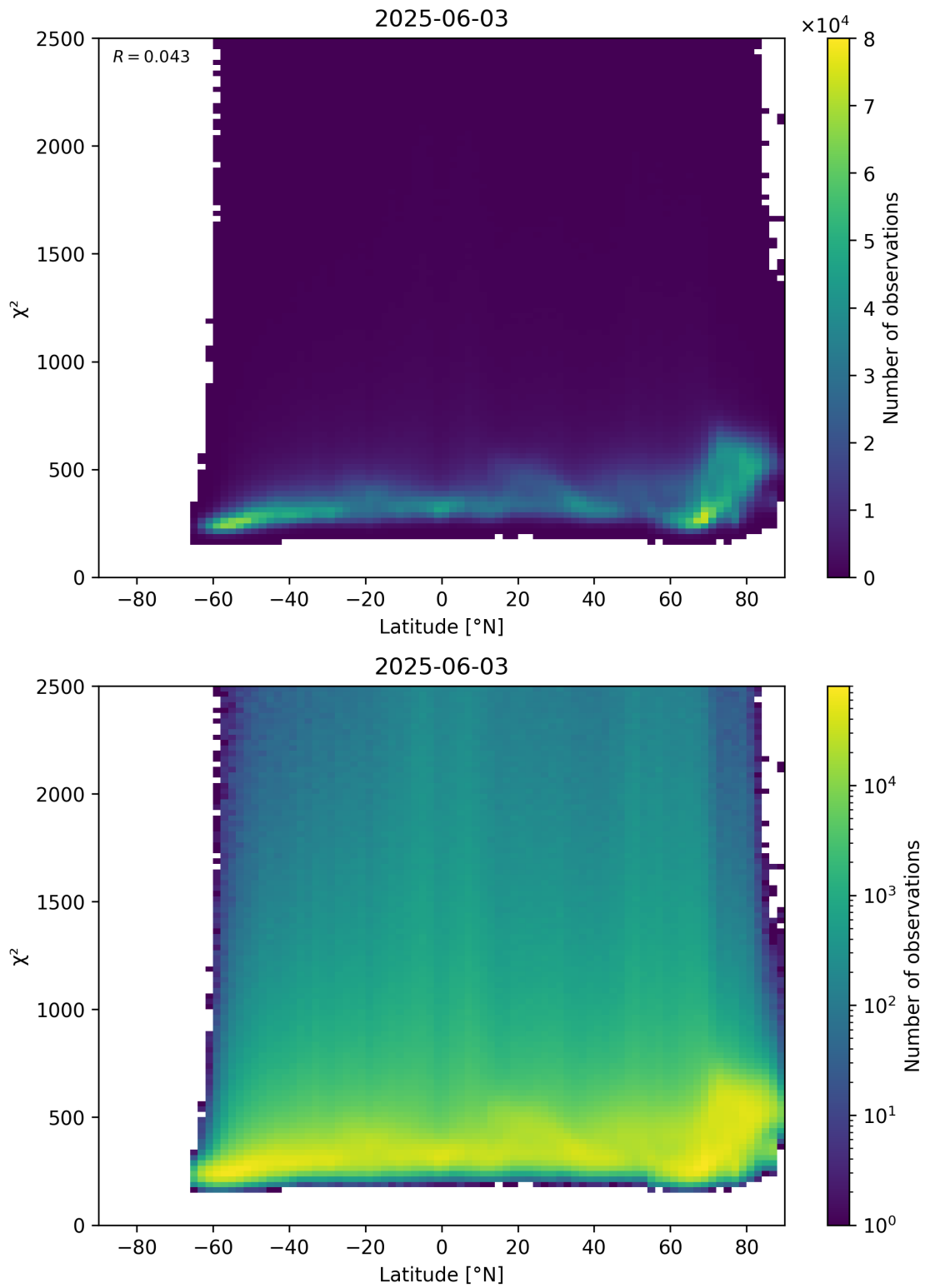
Figure 86: Scatter density plot of “Latitude” against “ \chi^2 ” for 2025-06-02 to 2025-06-04.
