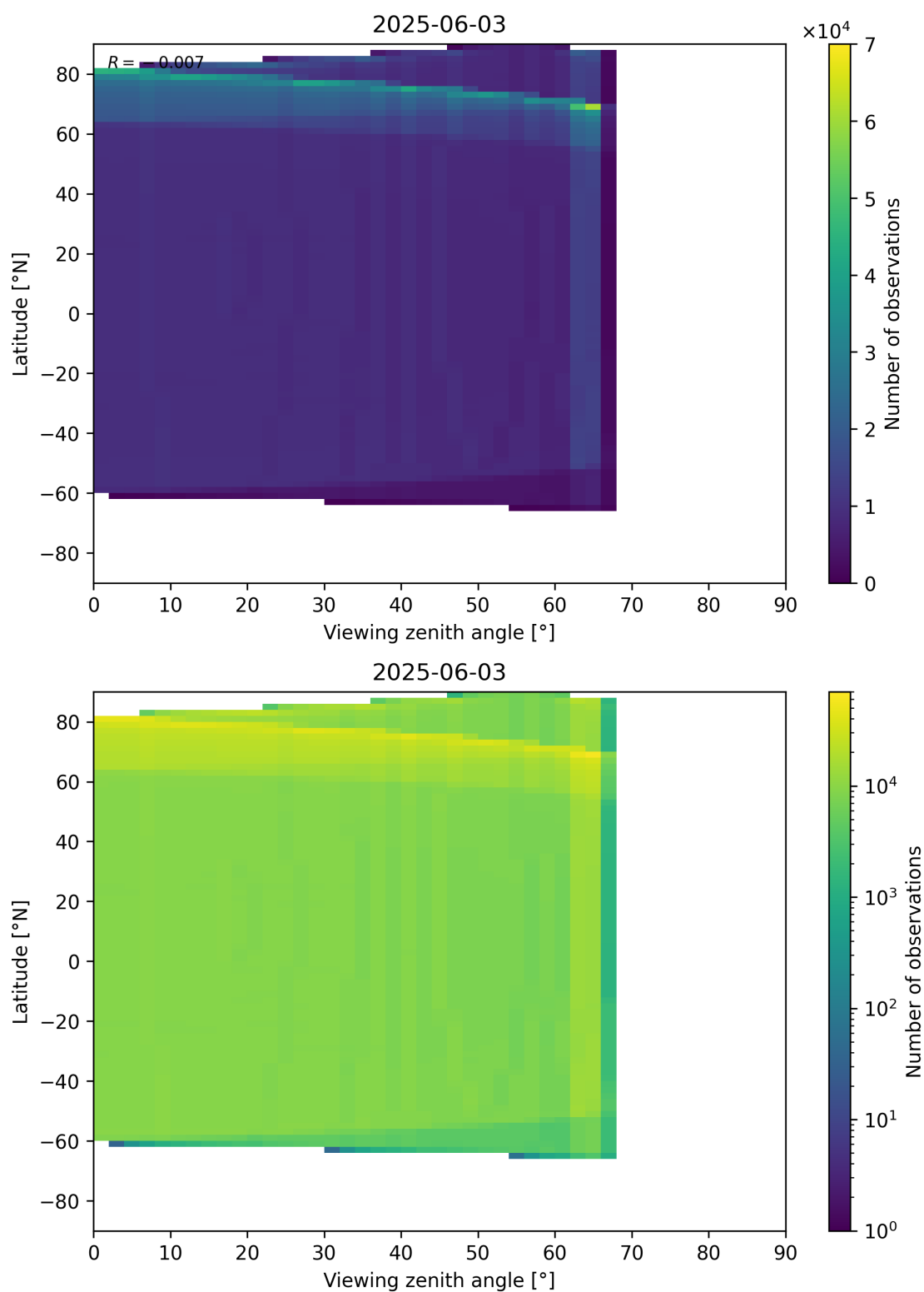
Figure 163: Scatter density plot of “Viewing zenith angle” against “Latitude” for 2025-06-02 to 2025-06-04.
