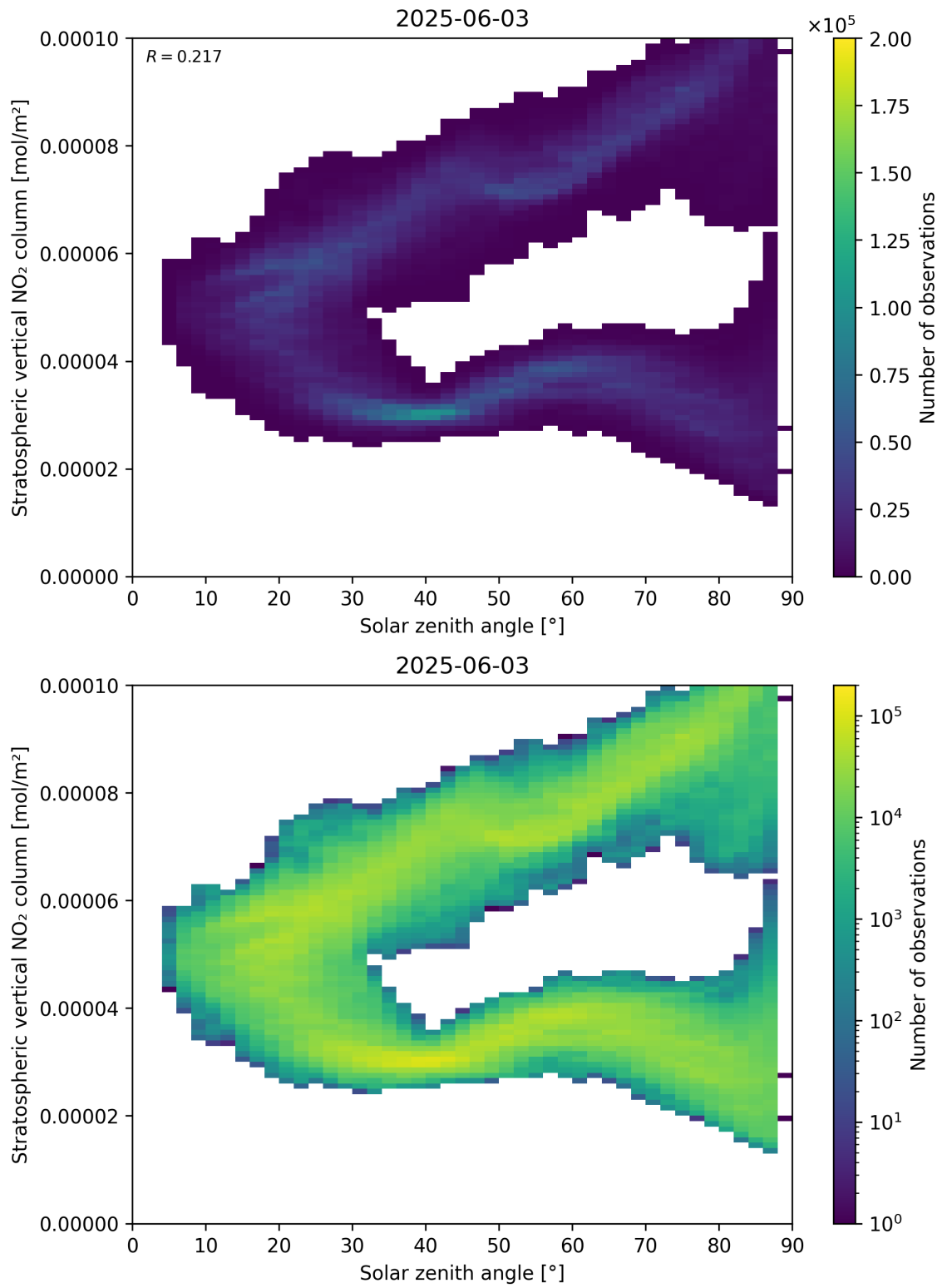
Figure 150: Scatter density plot of “Solar zenith angle” against “Stratospheric vertical NO 2 column” for 2025-06-02 to 2025-06-04.
