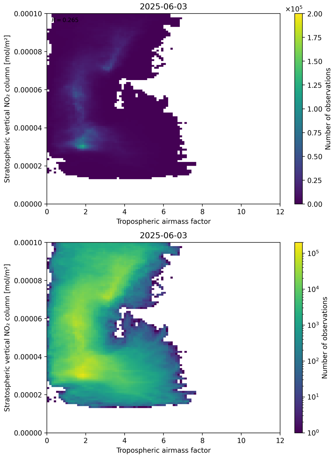
Figure 74: Scatter density plot of “Tropospheric airmass factor” against “Stratospheric vertical NO 2 column” for 2025-06-02 to 2025-06-04.
