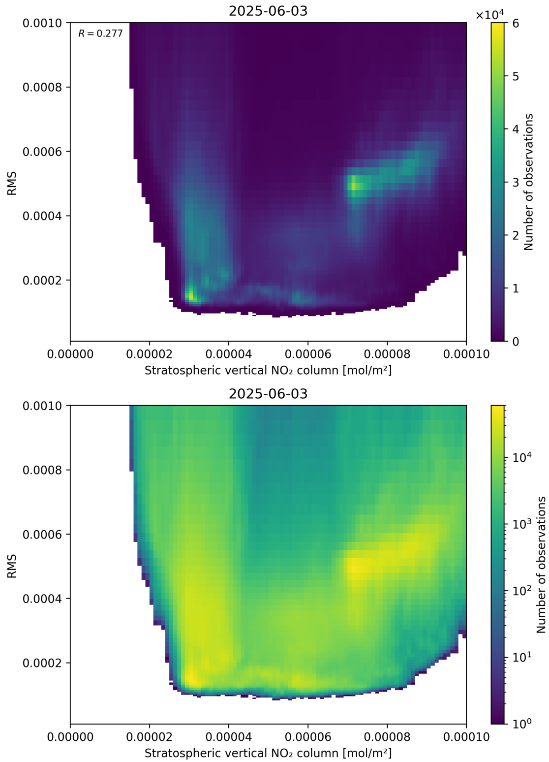
Figure 102: Scatter density plot of “Stratospheric vertical NO 2 column” against “RMS” for 2025-06-02 to 2025-06-04.
