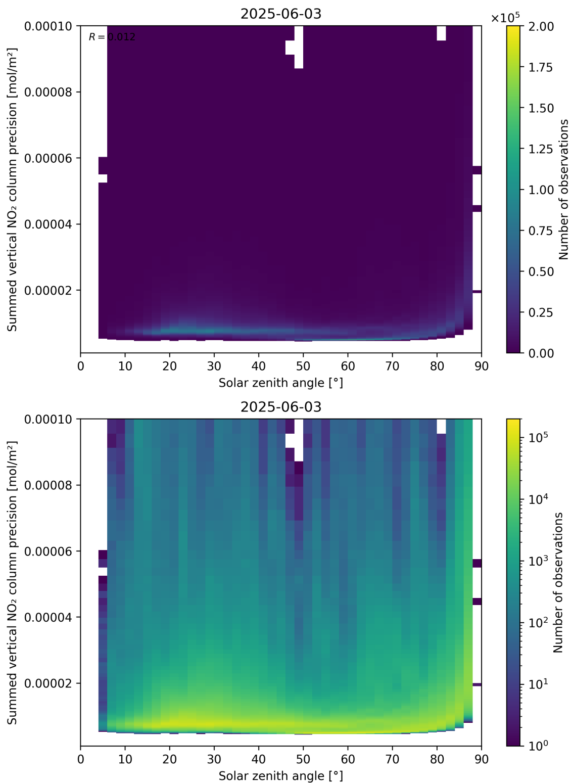
Figure 152: Scatter density plot of “Solar zenith angle” against “Summed vertical NO 2 column precision” for 2025-06-02 to 2025-06-04.
