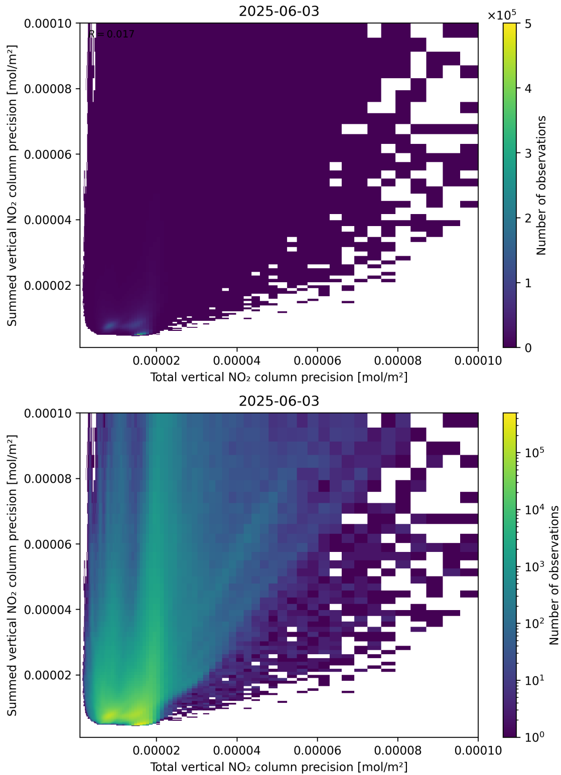
Figure 118: Scatter density plot of “Total vertical NO 2 column precision” against “Summed vertical NO 2 column precision” for 2025-06-02 to 2025-06-04.
