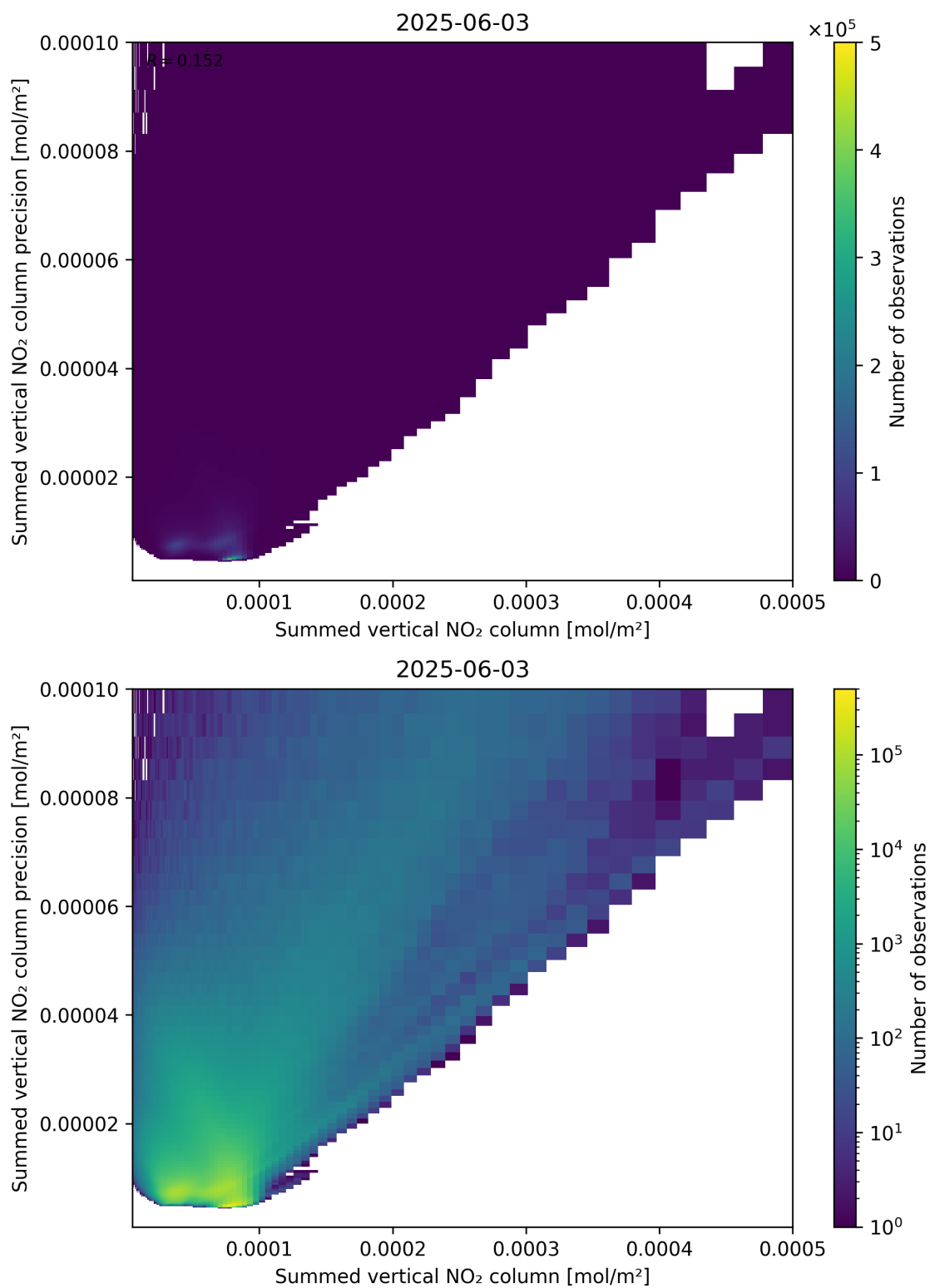
Figure 105: Scatter density plot of “Summed vertical NO 2 column” against “Summed vertical NO 2 column precision” for 2025-06-02 to 2025-06-04.
