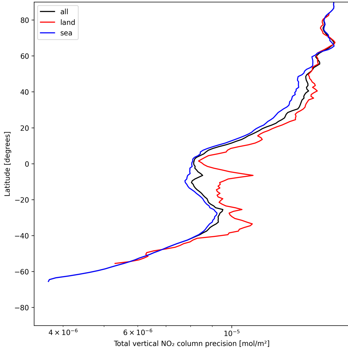
Figure 22: Zonal average of “Total vertical NO 2 column precision” for 2025-06-02 to 2025-06-04.
