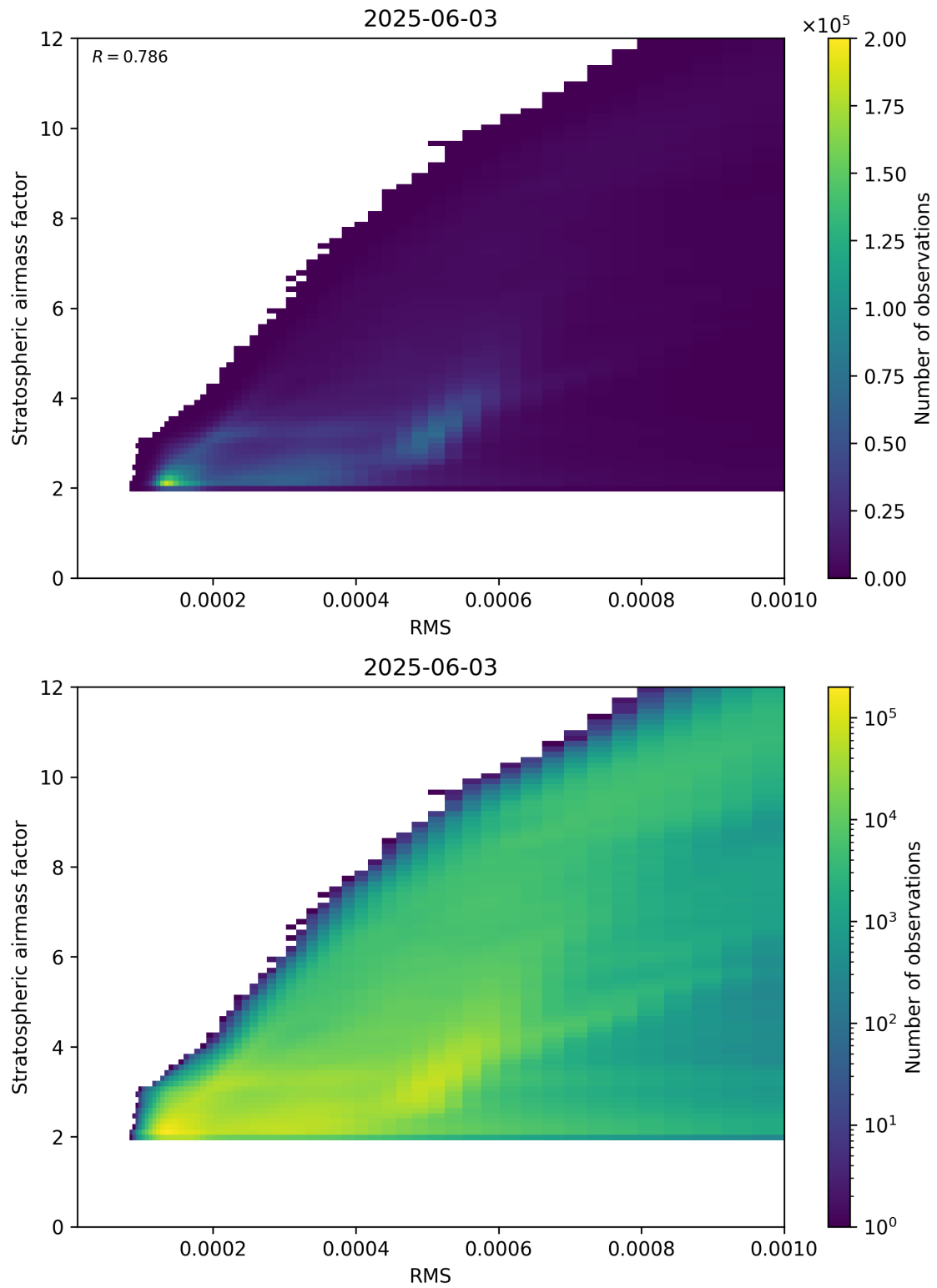
Figure 144: Scatter density plot of “RMS” against “Stratospheric airmass factor” for 2025-06-02 to 2025-06-04.
