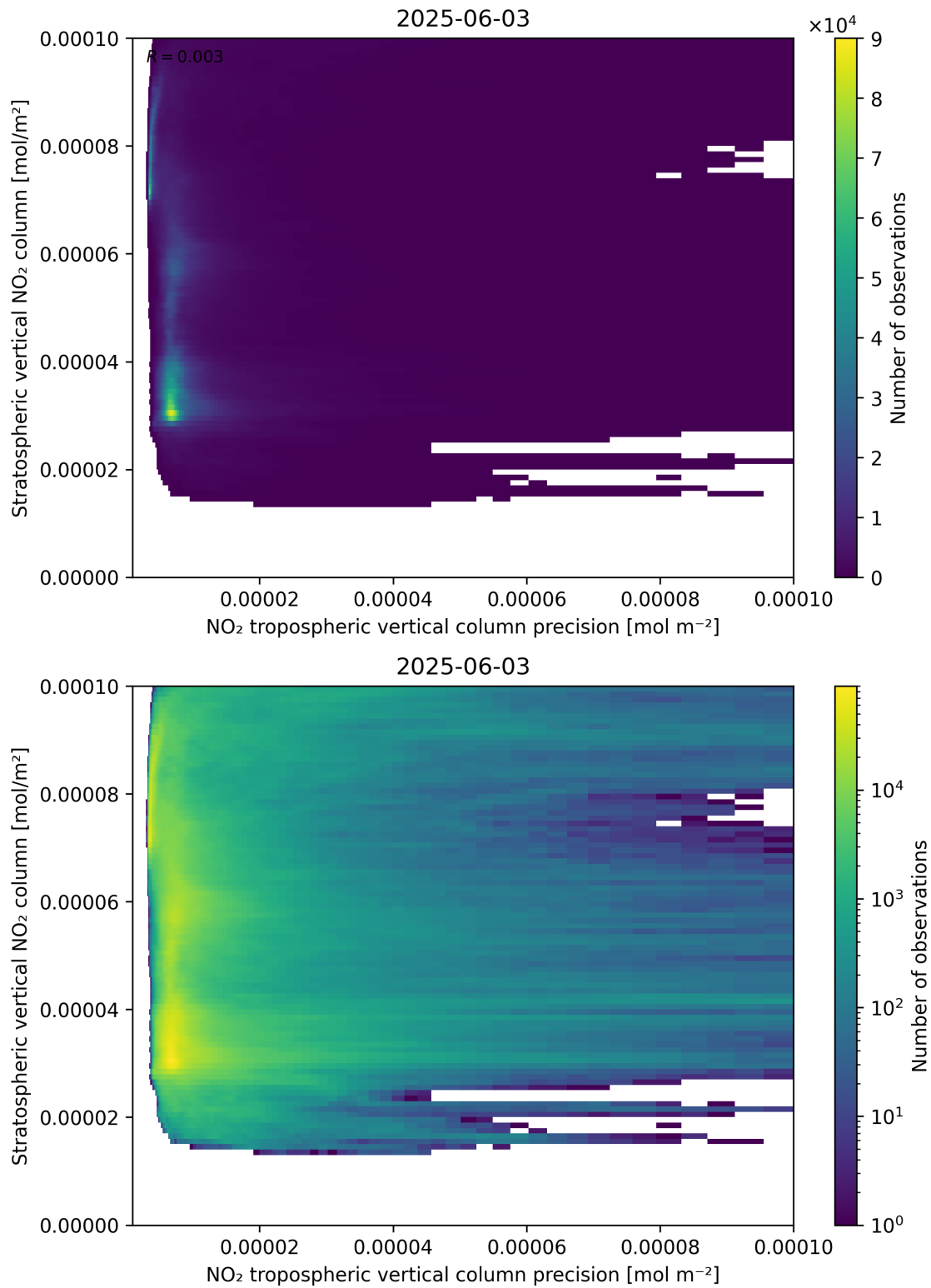
Figure 135: Scatter density plot of “NO 2 tropospheric vertical column precision” against “Stratospheric vertical NO 2 column” for 2025-06-02 to 2025-06-04.
