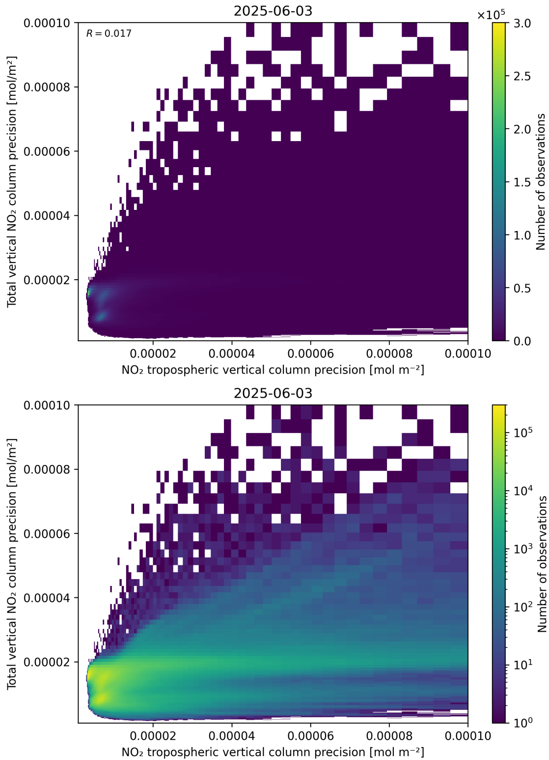
Figure 139: Scatter density plot of “NO 2 tropospheric vertical column precision” against “Total vertical NO 2 column precision” for 2025-06-02 to 2025-06-04.
