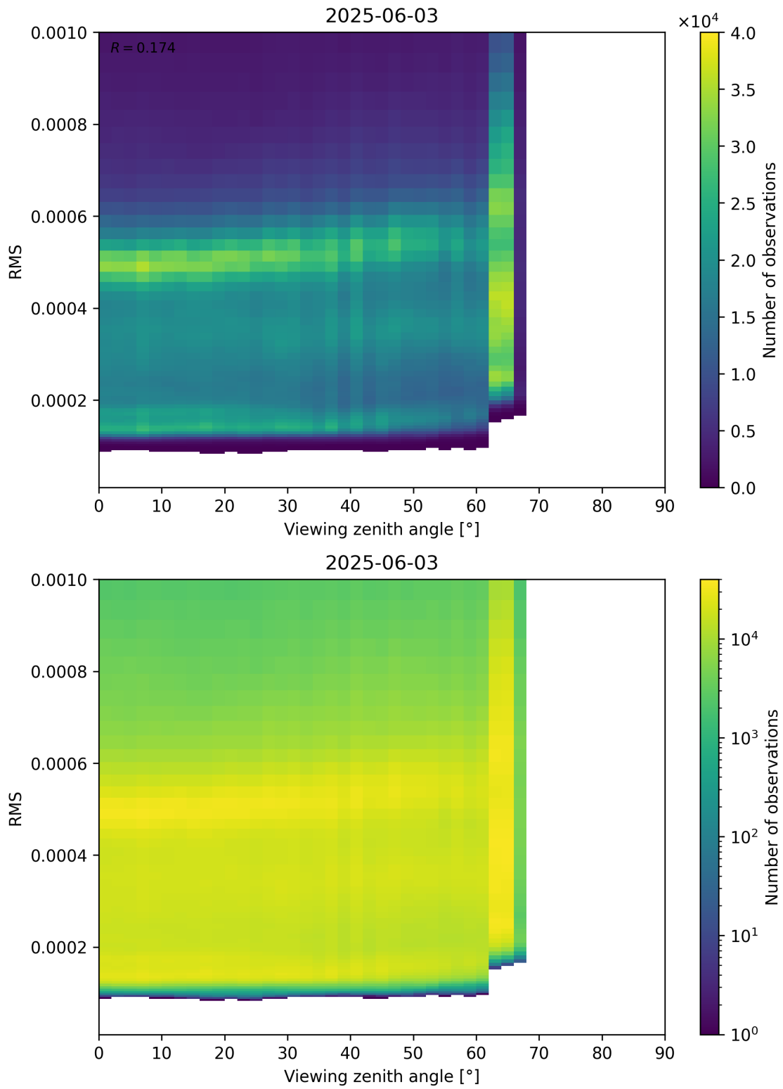
Figure 171: Scatter density plot of “Viewing zenith angle” against “RMS” for 2025-06-02 to 2025-06-04.
