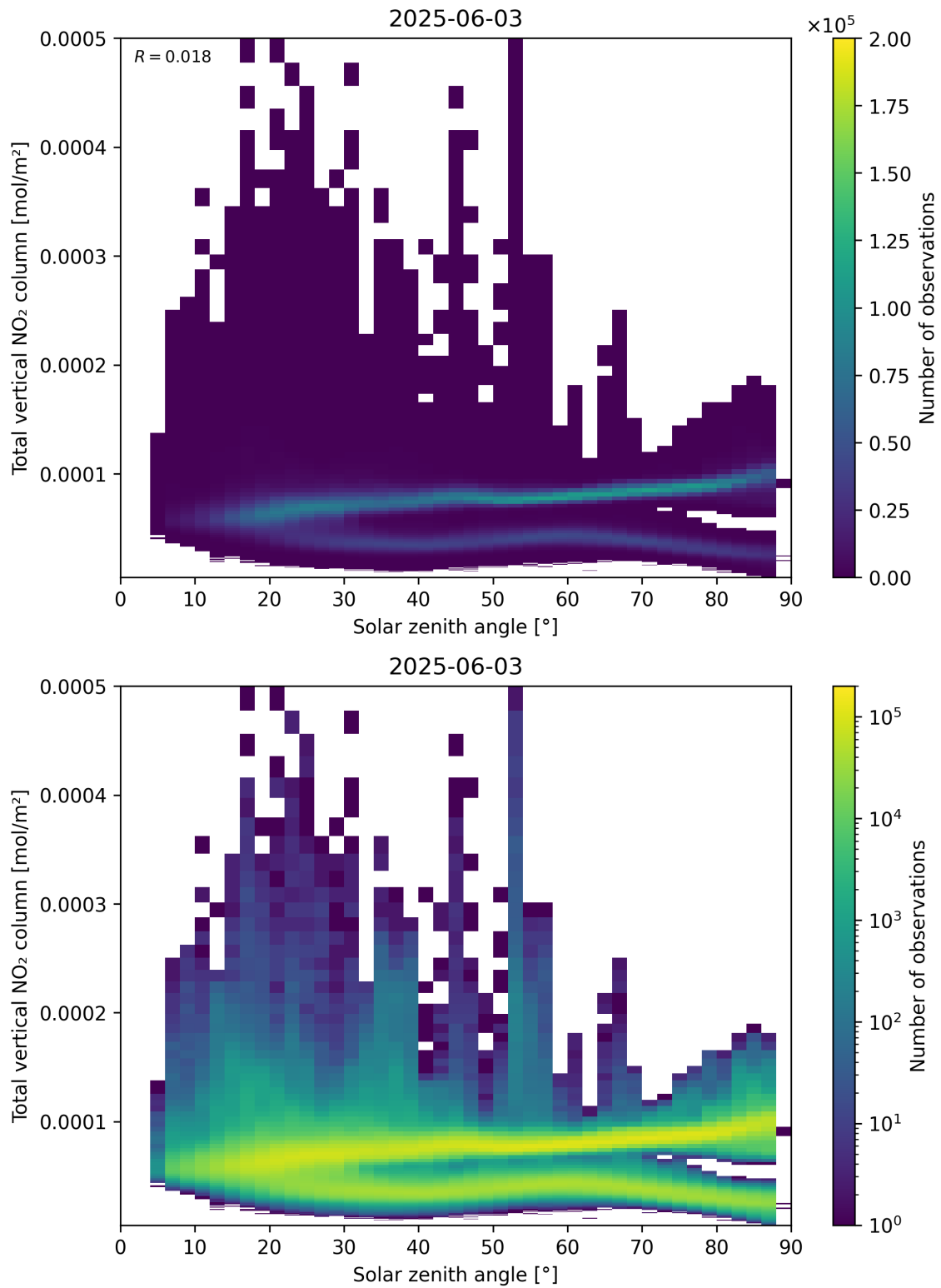
Figure 153: Scatter density plot of “Solar zenith angle” against “Total vertical NO 2 column” for 2025-06-02 to 2025-06-04.
