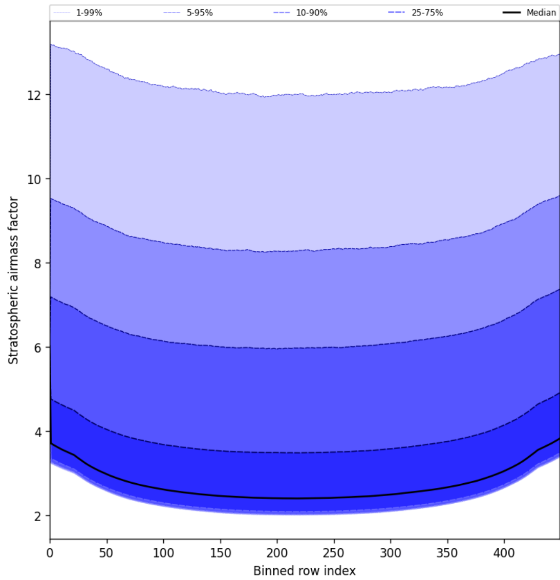
Figure 61: Along track statistics of “Stratospheric airmass factor” for 2025-06-02 to 2025-06-04
