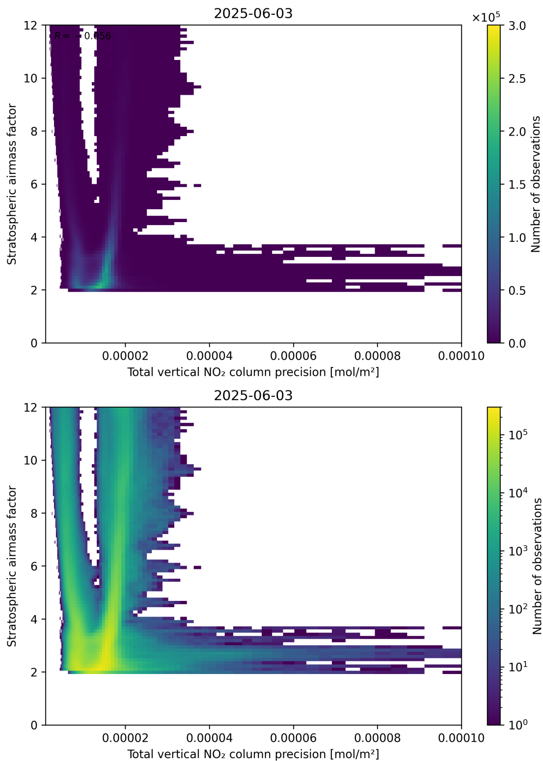
Figure 115: Scatter density plot of “Total vertical NO 2 column precision” against “Stratospheric air mass factor” for 2025-06-02 to 2025-06-04.
