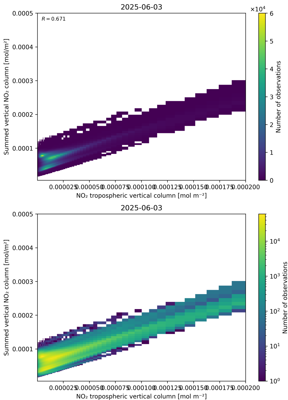
Figure 126: Scatter density plot of “NO 2 tropospheric vertical column” against “Summed vertical NO 2 column” for 2025-06-02 to 2025-06-04.
