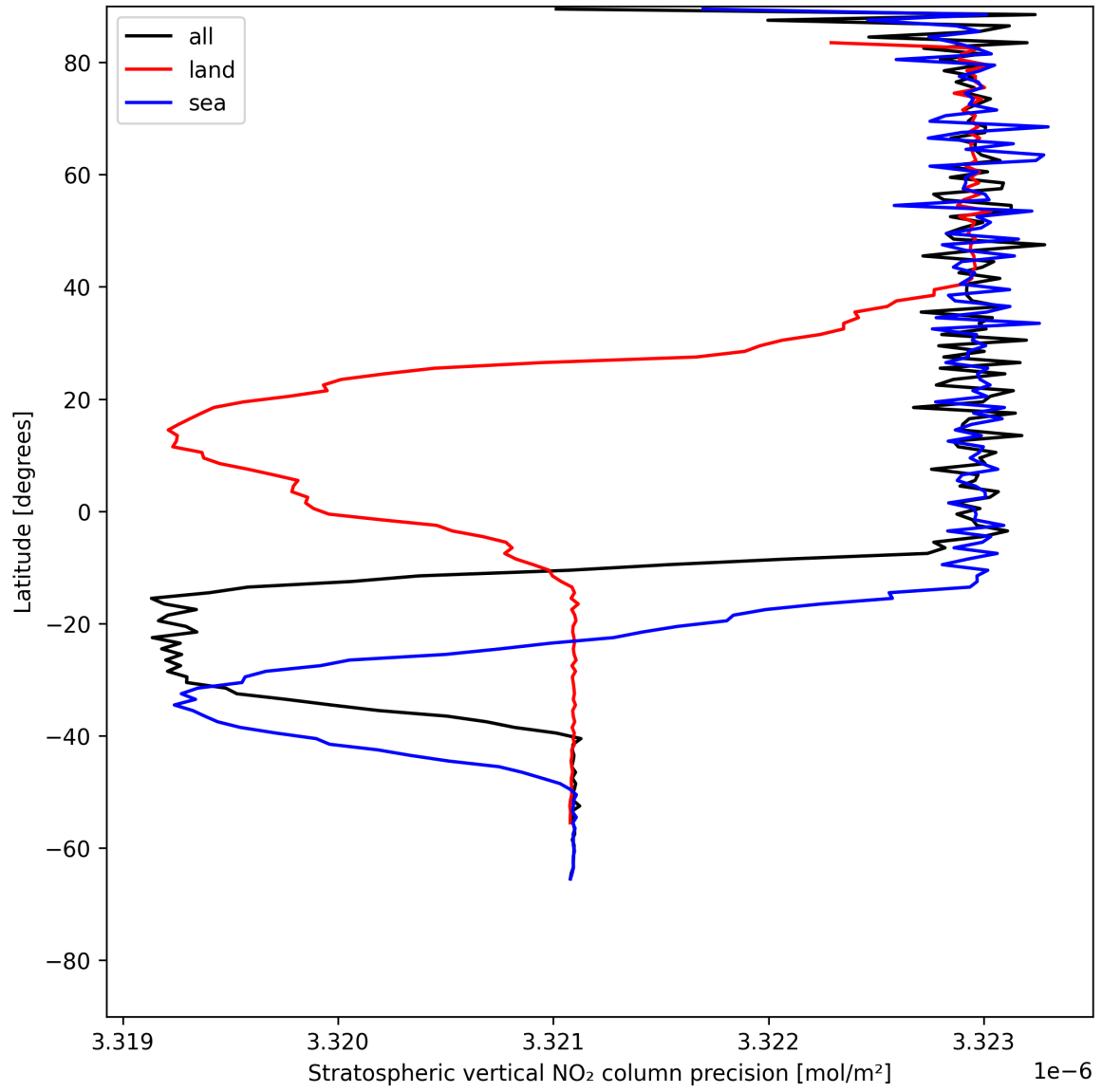
Figure 20: Zonal average of “Stratospheric vertical NO 2 column precision” for 2025-06-02 to 2025-06-04.
