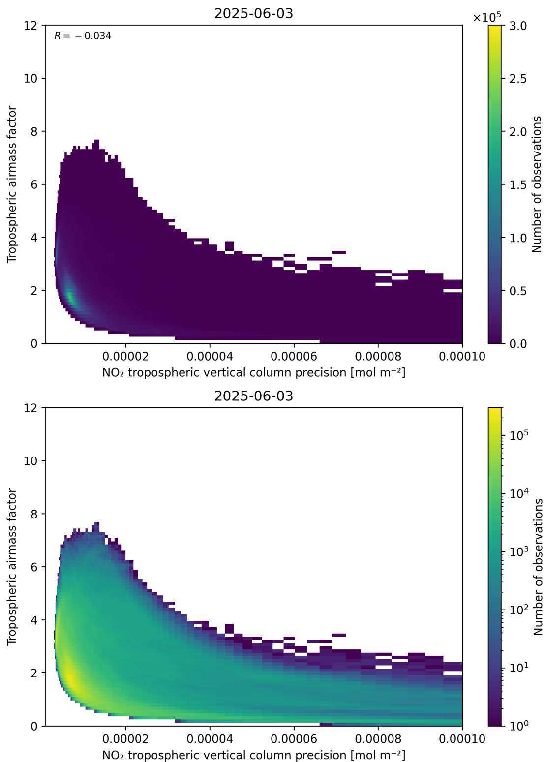
Figure 133: Scatter density plot of “NO 2 tropospheric vertical column precision” against “Tropospheric air mass factor” for 2025-06-02 to 2025-06-04.
