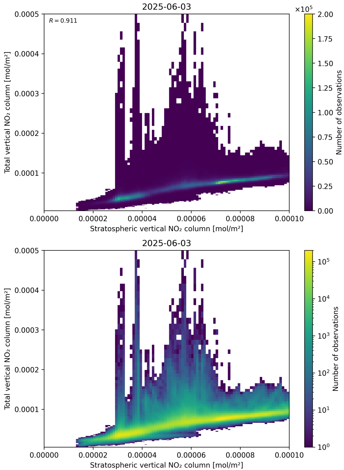
Figure 100: Scatter density plot of “Stratospheric vertical NO 2 column” against “Total vertical NO 2 column” for 2025-06-02 to 2025-06-04.
