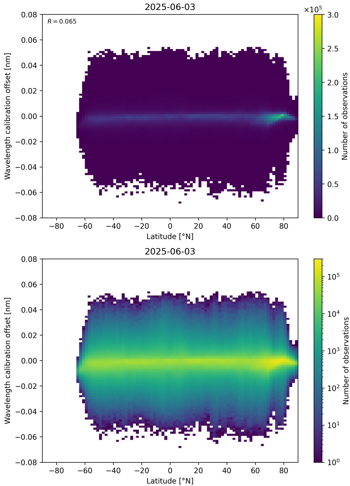
Figure 95: Scatter density plot of “Latitude” against “Wavelength calibration offset” for 2025-06-02 to 2025-06-04.
