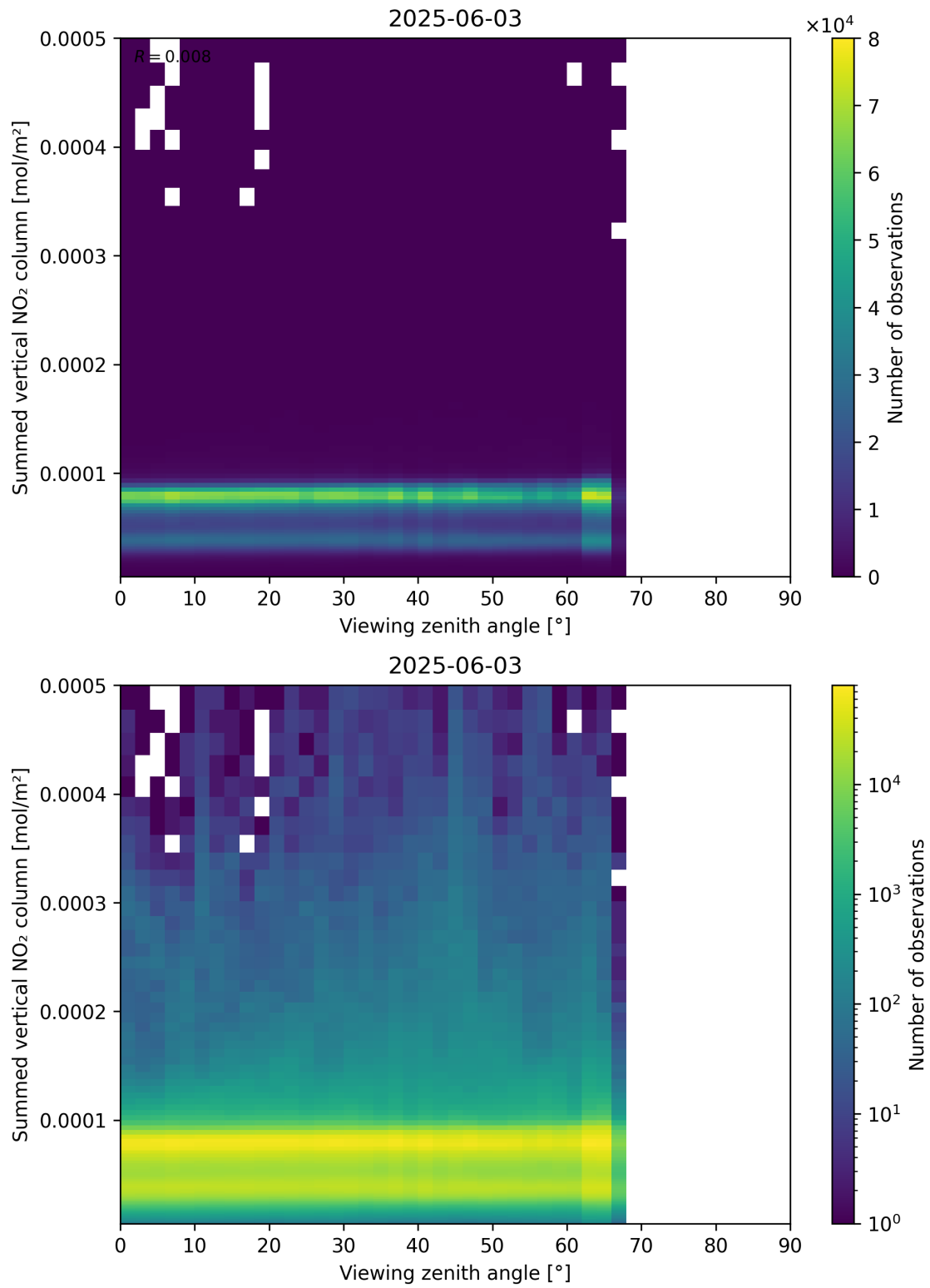
Figure 165: Scatter density plot of “Viewing zenith angle” against “Summed vertical NO 2 column” for 2025-06-02 to 2025-06-04.
