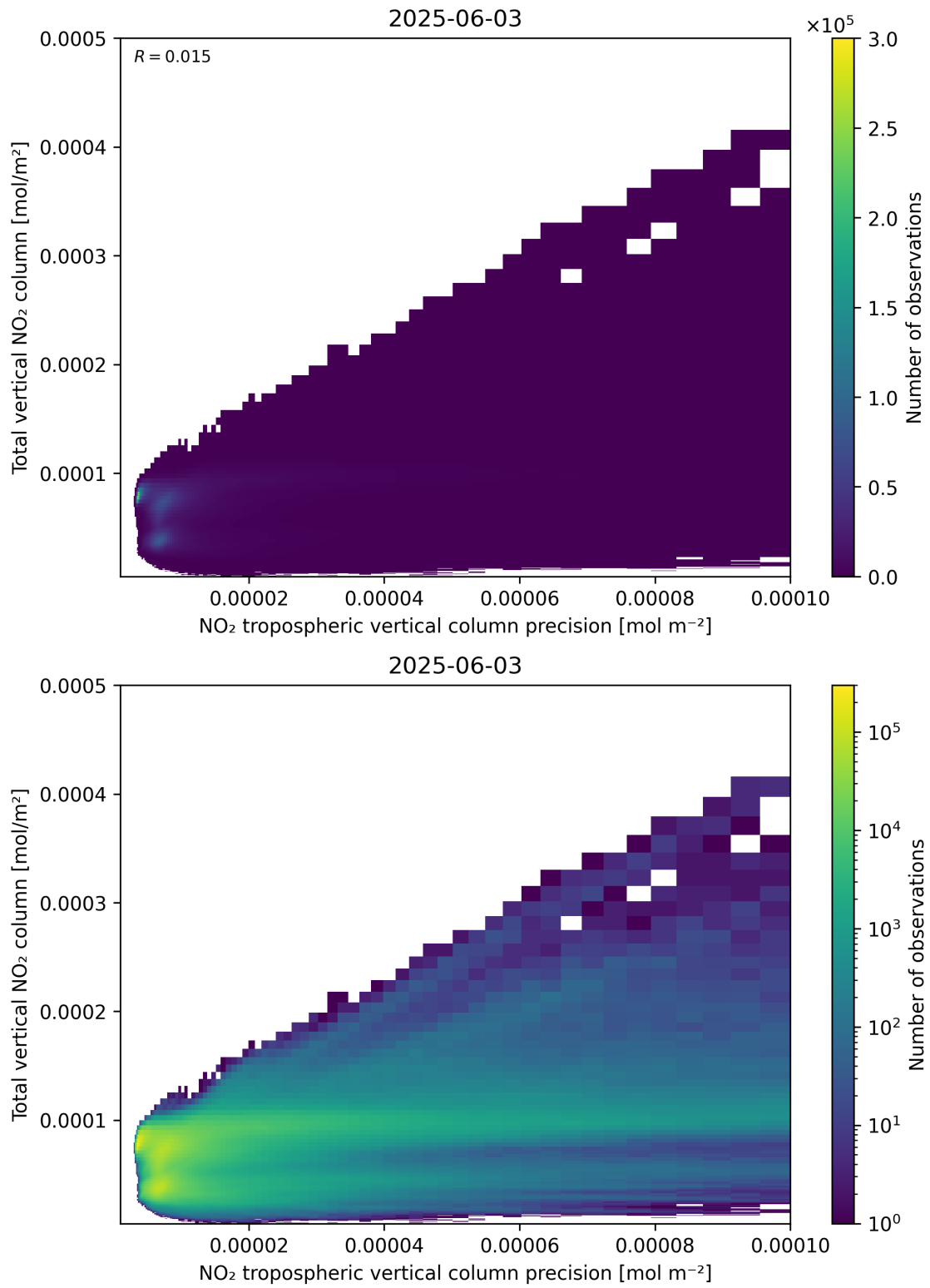
Figure 138: Scatter density plot of “NO 2 tropospheric vertical column precision” against “Total vertical NO 2 column” for 2025-06-02 to 2025-06-04.
