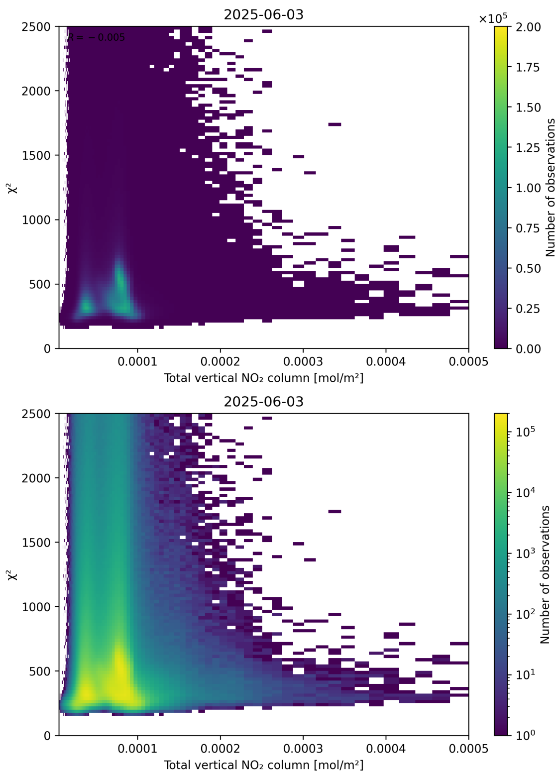
Figure 111: Scatter density plot of “Total vertical NO 2 column” against “ \chi^2 ” for 2025-06-02 to 2025-06-04.
