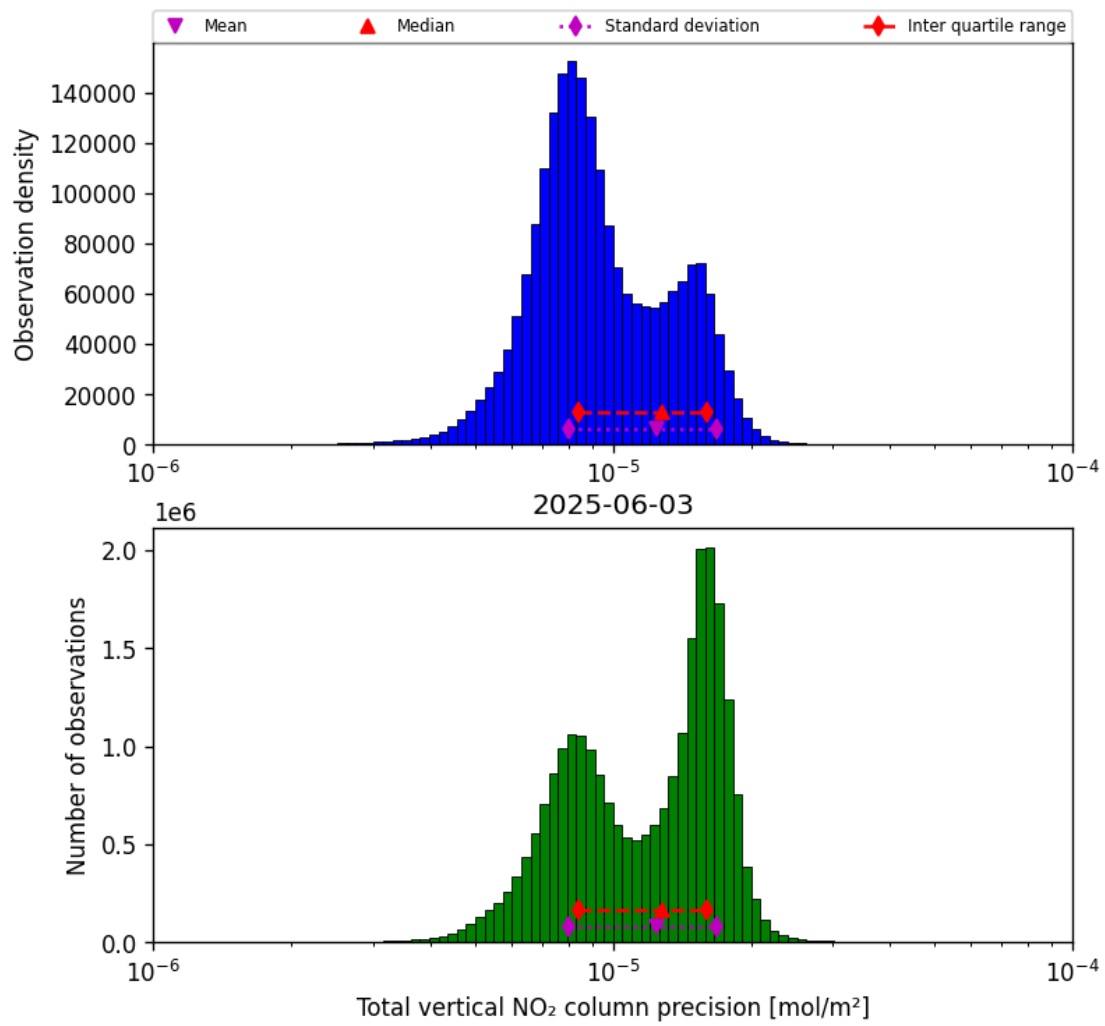
Figure 39: Histogram of “Total vertical NO 2 column precision” for 2025-06-02 to 2025-06-04
