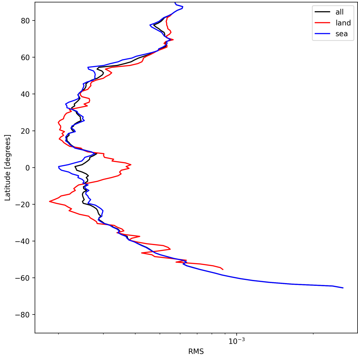
Figure 26: Zonal average of “RMS” for 2025-06-02 to 2025-06-04.
