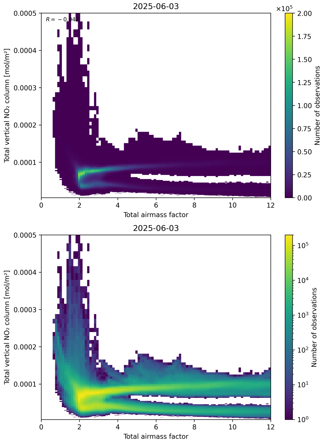
Figure 67: Scatter density plot of “Total airmass factor” against “Total vertical NO 2 column” for 2025-06-02 to 2025-06-04.
