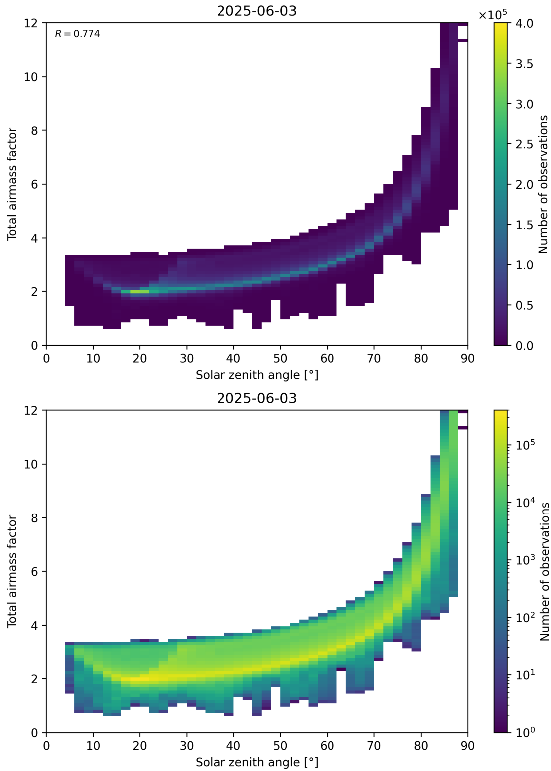
Figure 146: Scatter density plot of “Solar zenith angle” against “Total air mass factor” for 2025-06-02 to 2025-06-04.
