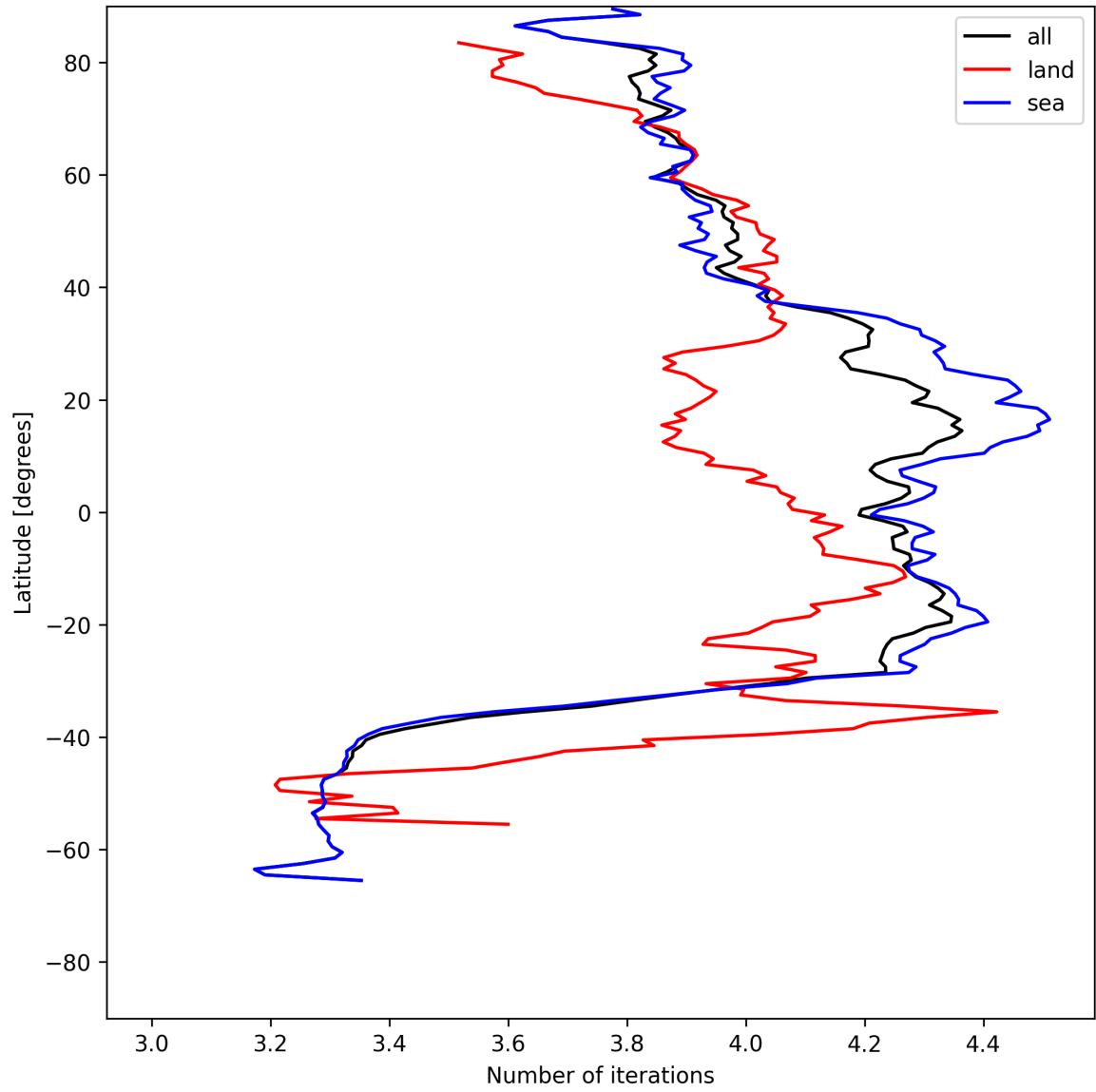
Figure 17: Zonal average of “Number of iterations” for 2025-06-02 to 2025-06-04.
