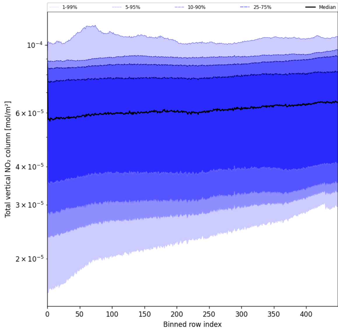
Figure 55: Along track statistics of “Total vertical NO 2 column” for 2025-06-02 to 2025-06-04
