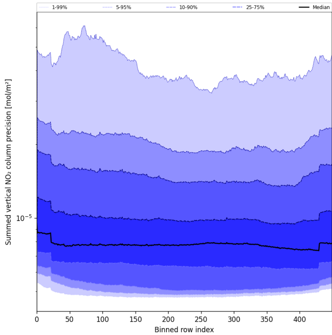
Figure 58: Along track statistics of “Summed vertical NO 2 column precision” for 2025-06-02 to 2025-06-04
