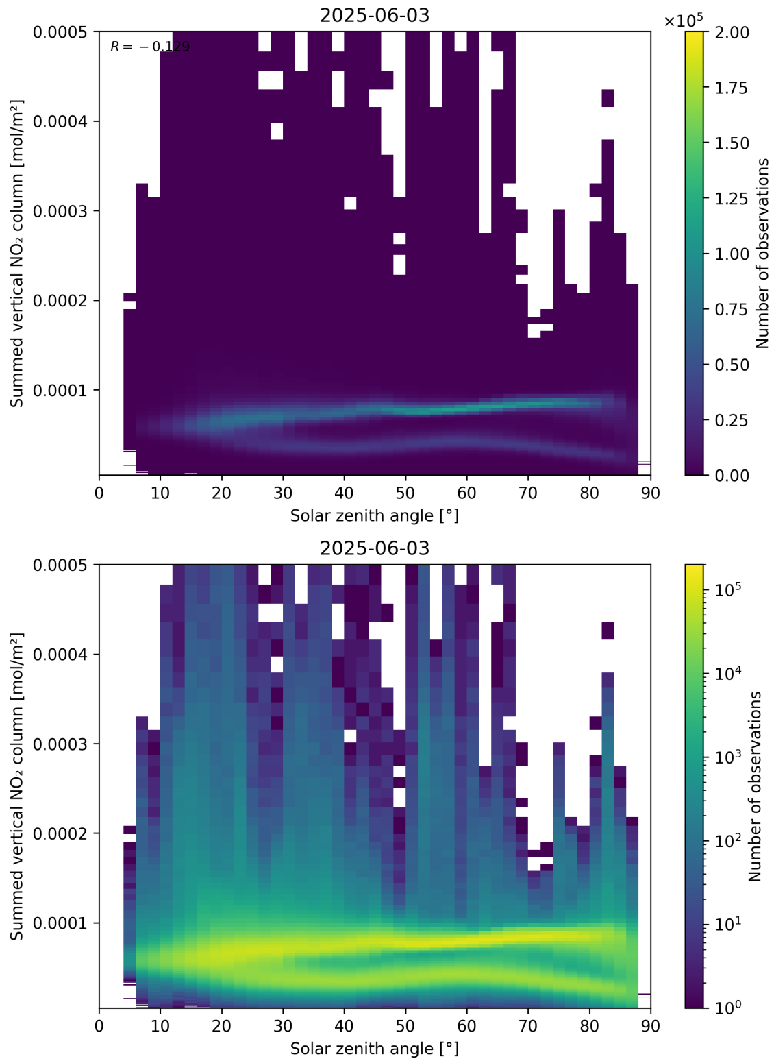
Figure 151: Scatter density plot of “Solar zenith angle” against “Summed vertical NO 2 column” for 2025-06-02 to 2025-06-04.
