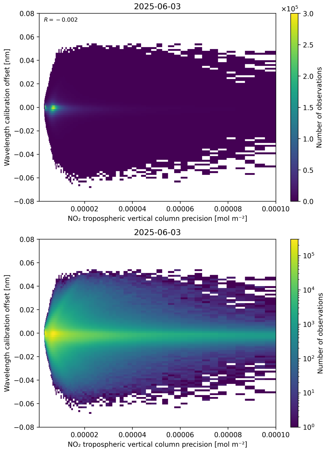
Figure 141: Scatter density plot of “NO 2 tropospheric vertical column precision” against “Wavelength calibration offset” for 2025-06-02 to 2025-06-04.
