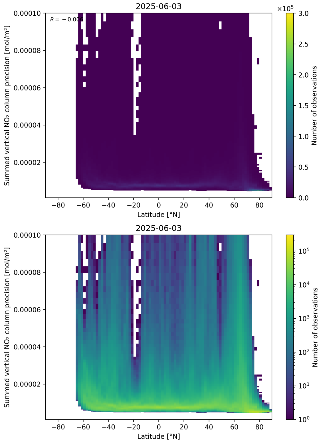
Figure 89: Scatter density plot of “Latitude” against “Summed vertical NO 2 column precision” for 2025-06-02 to 2025-06-04.
