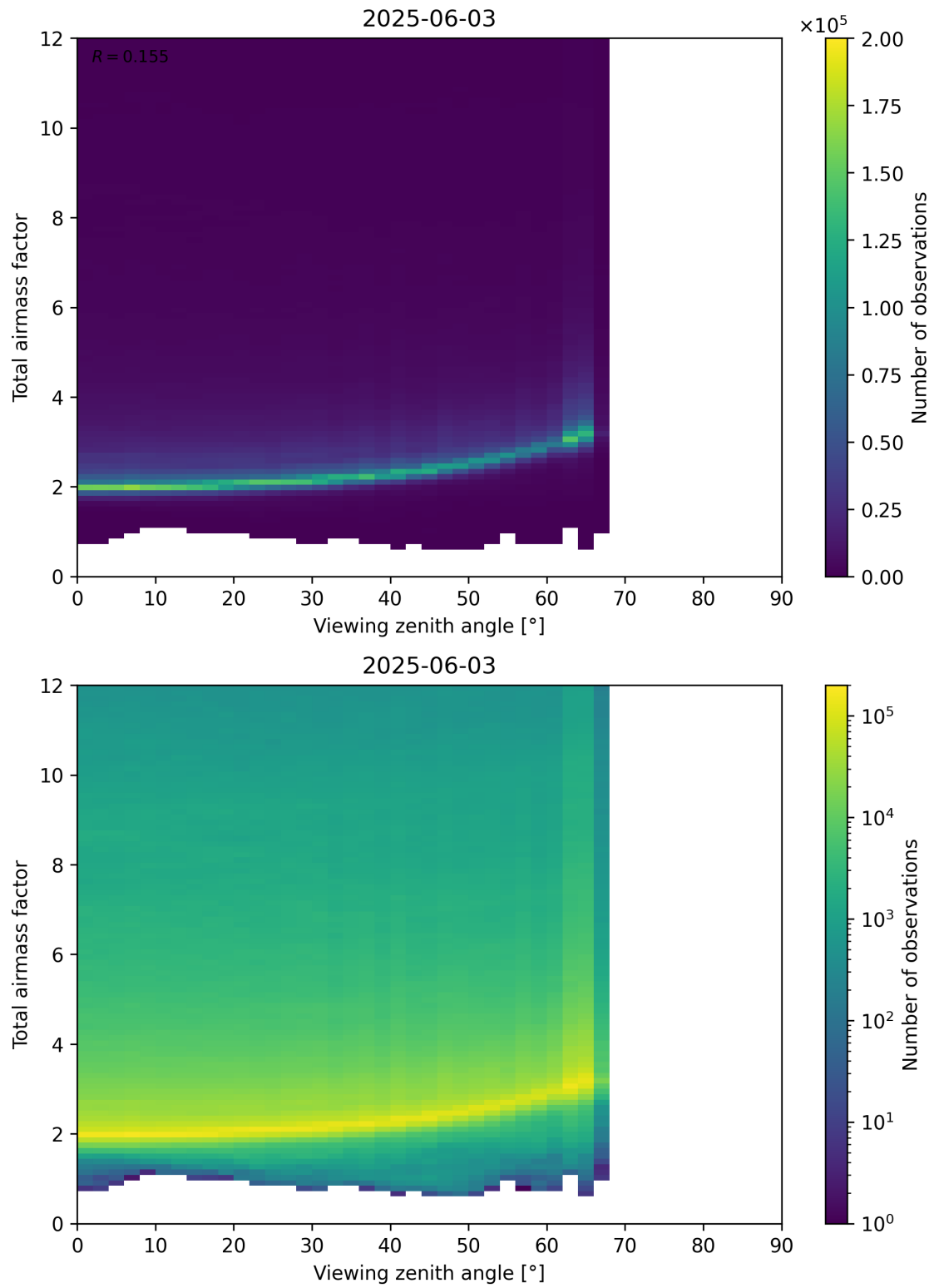
Figure 160: Scatter density plot of “Viewing zenith angle” against “Total airmass factor” for 2025-06-02 to 2025-06-04.
