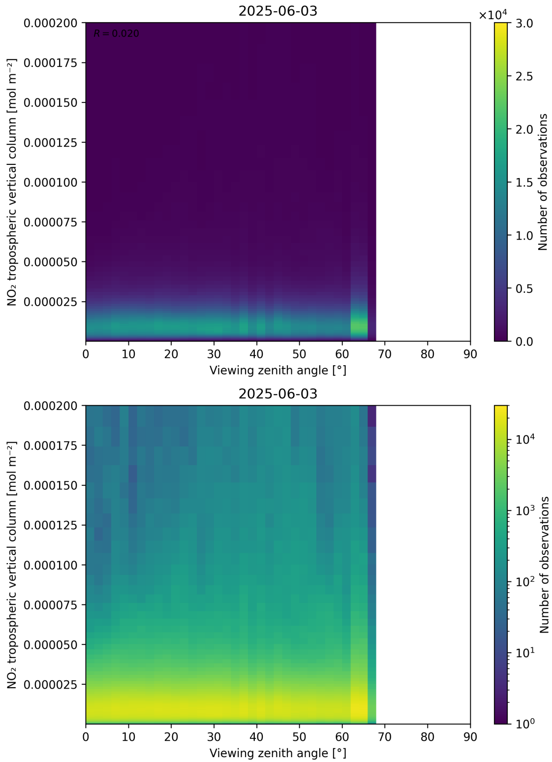
Figure 169: Scatter density plot of “Viewing zenith angle” against “NO 2 tropospheric vertical column” for 2025-06-02 to 2025-06-04.
