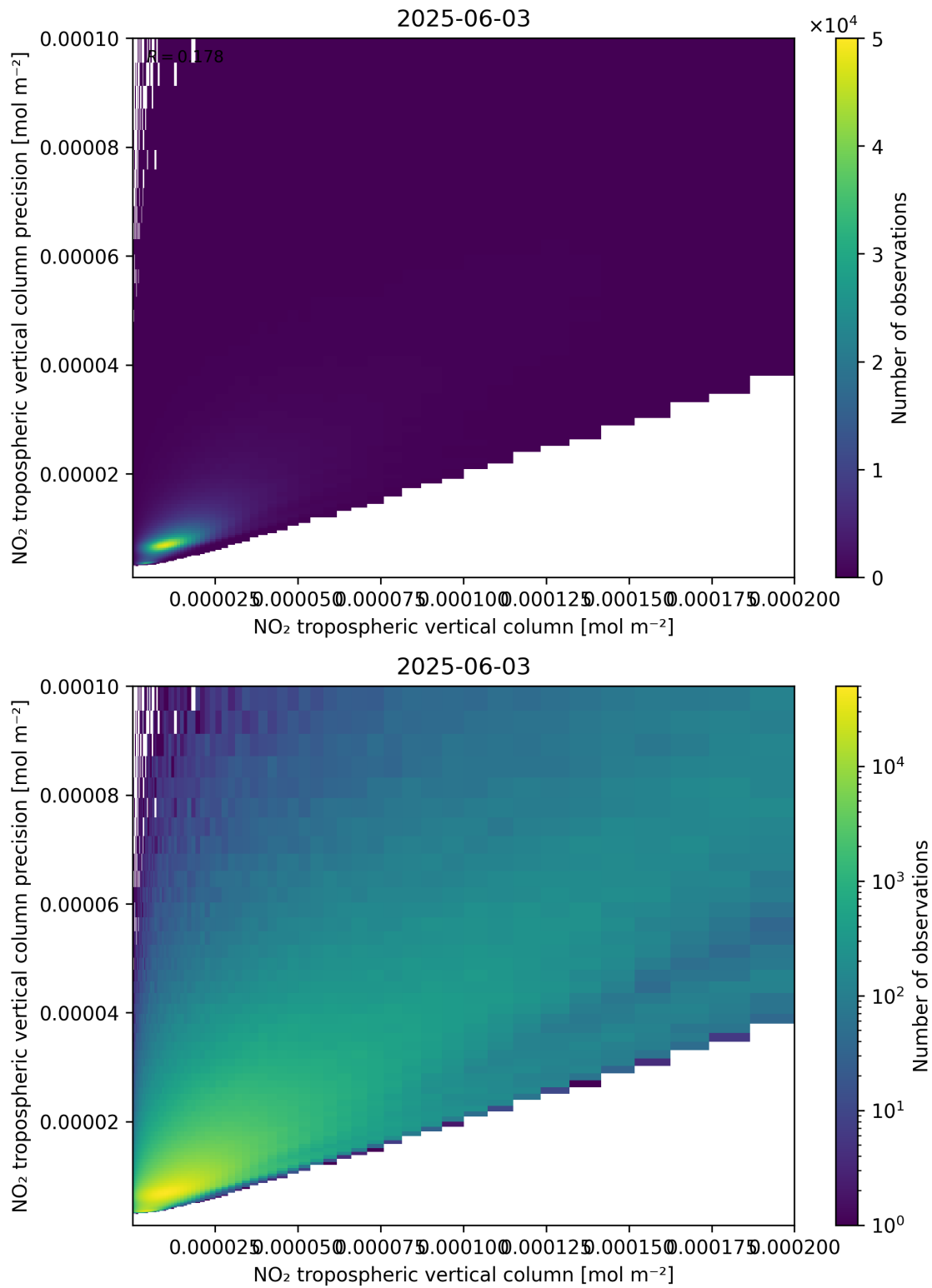
Figure 130: Scatter density plot of “NO 2 tropospheric vertical column” against “NO 2 tropospheric vertical column precision” for 2025-06-02 to 2025-06-04.
