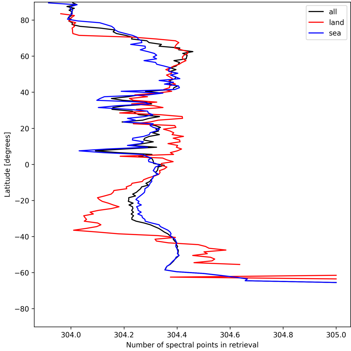
Figure 16: Zonal average of “Number of spectral points in retrieval” for 2025-06-03 to 2025-06-05.
