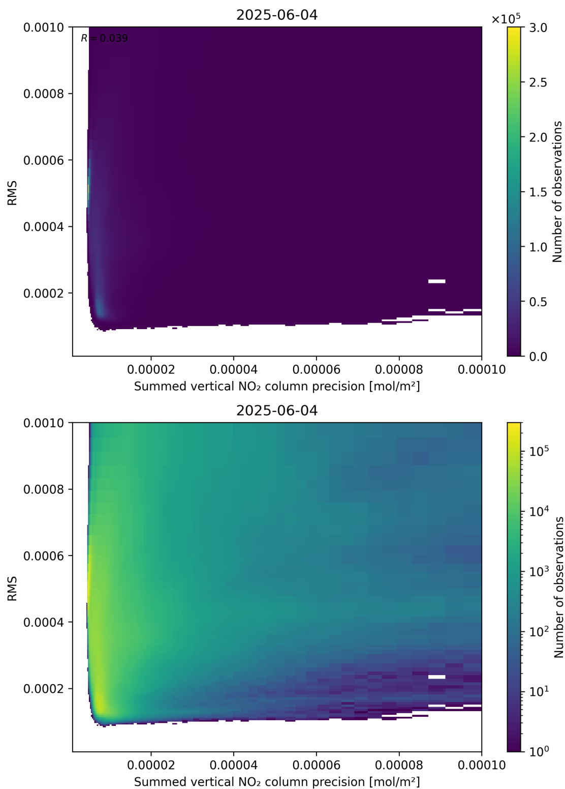
Figure 108: Scatter density plot of “Summed vertical NO 2 column precision” against “RMS” for 2025-06-03 to 2025-06-05.
