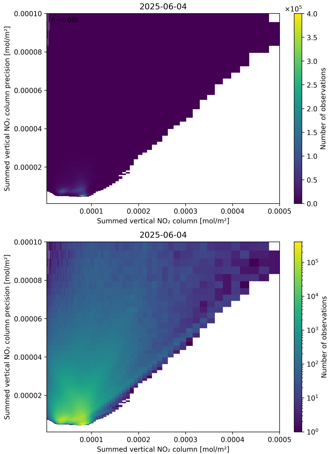
Figure 105: Scatter density plot of “Summed vertical NO 2 column” against “Summed vertical NO 2 column precision” for 2025-06-03 to 2025-06-05.
