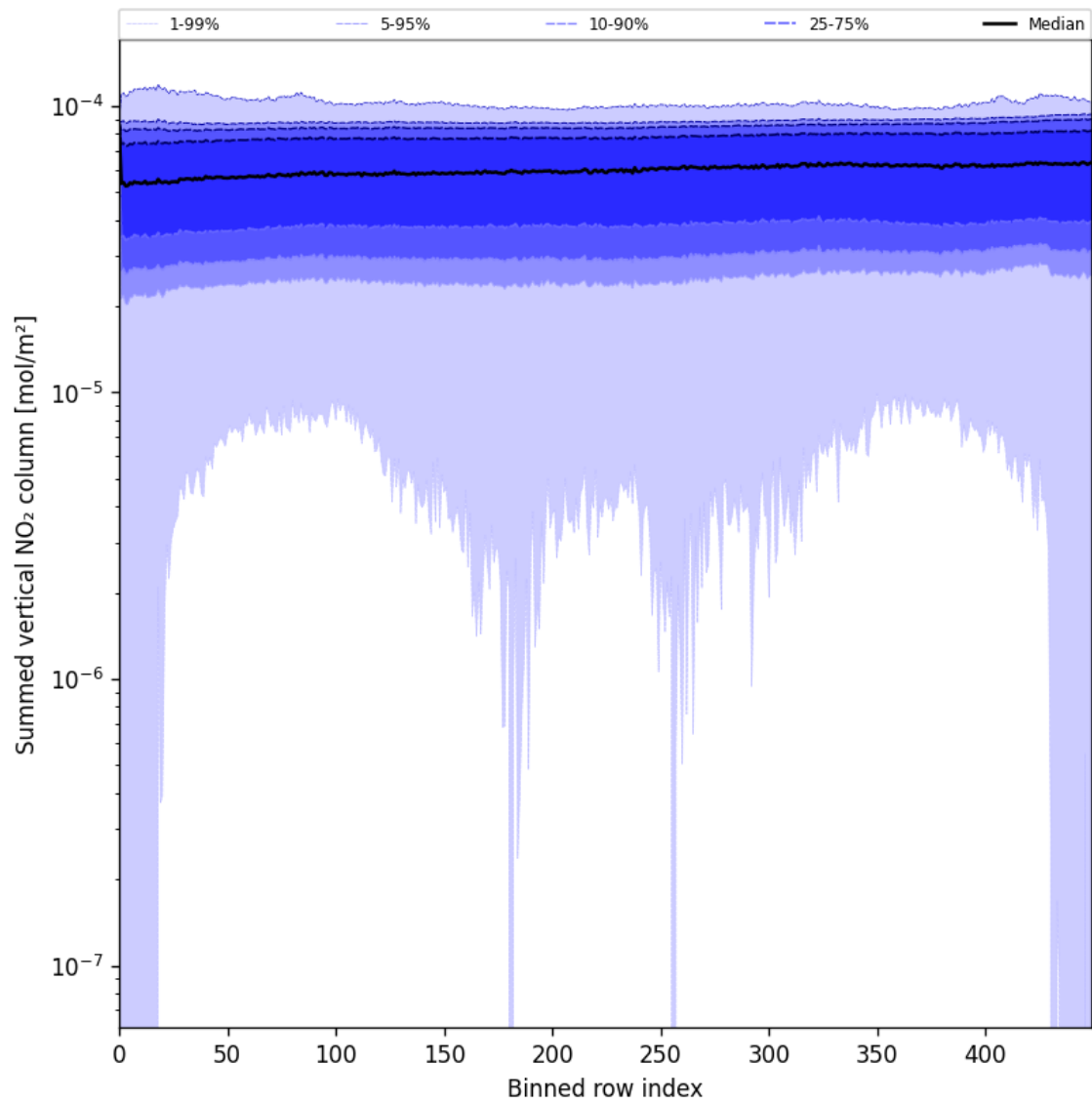
Figure 57: Along track statistics of “Summed vertical NO 2 column” for 2025-06-03 to 2025-06-05
