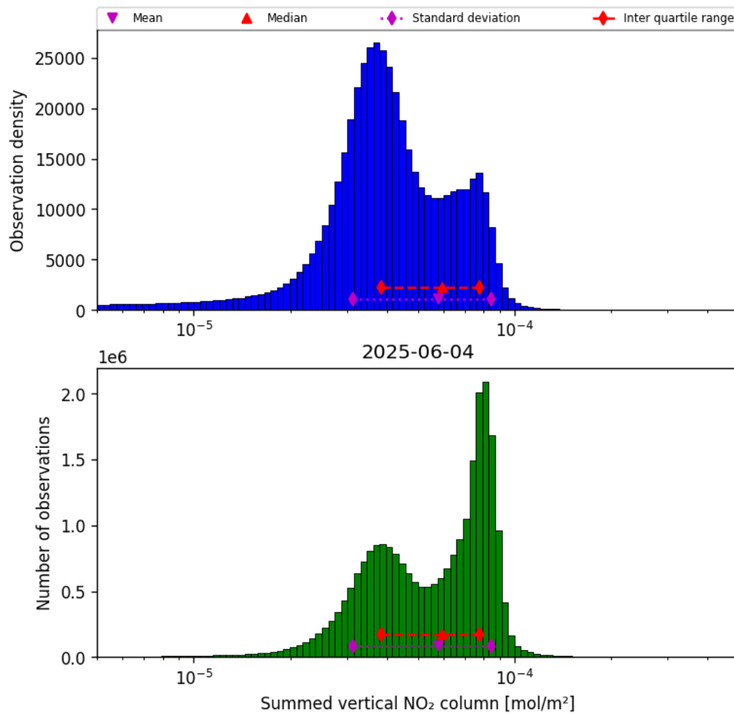
Figure 40: Histogram of “Summed vertical NO 2 column” for 2025-06-03 to 2025-06-05
