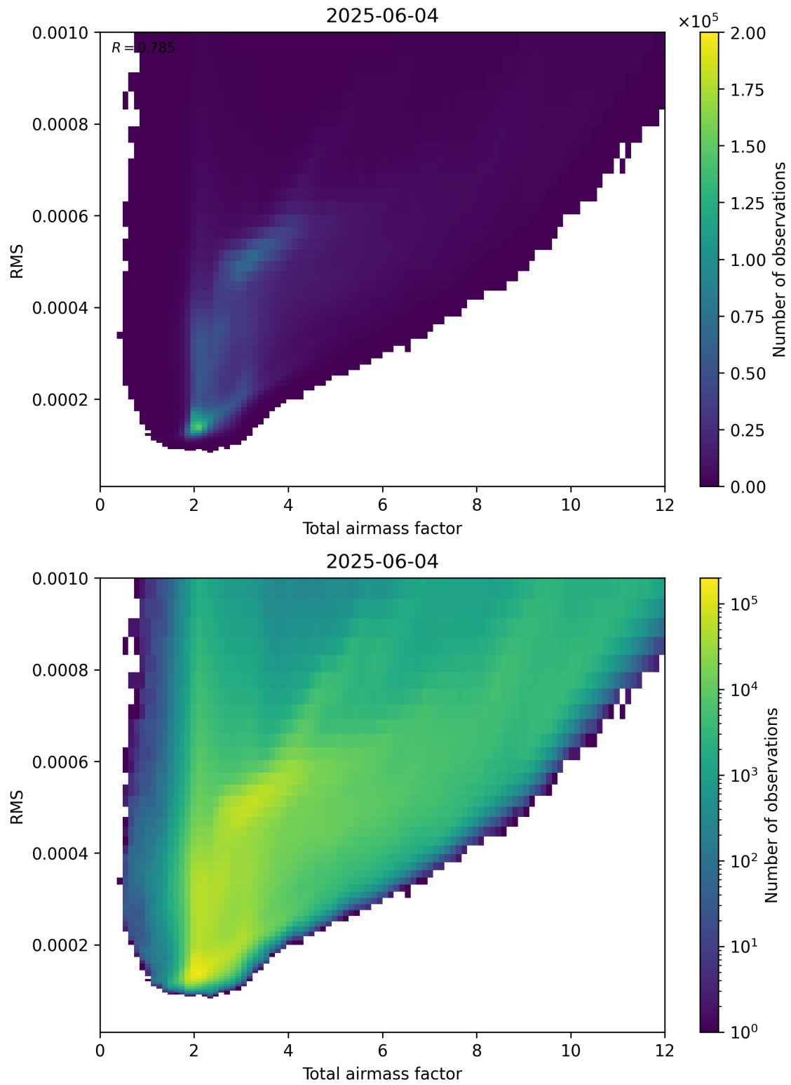
Figure 69: Scatter density plot of “Total airmass factor” against “RMS” for 2025-06-03 to 2025-06-05.
