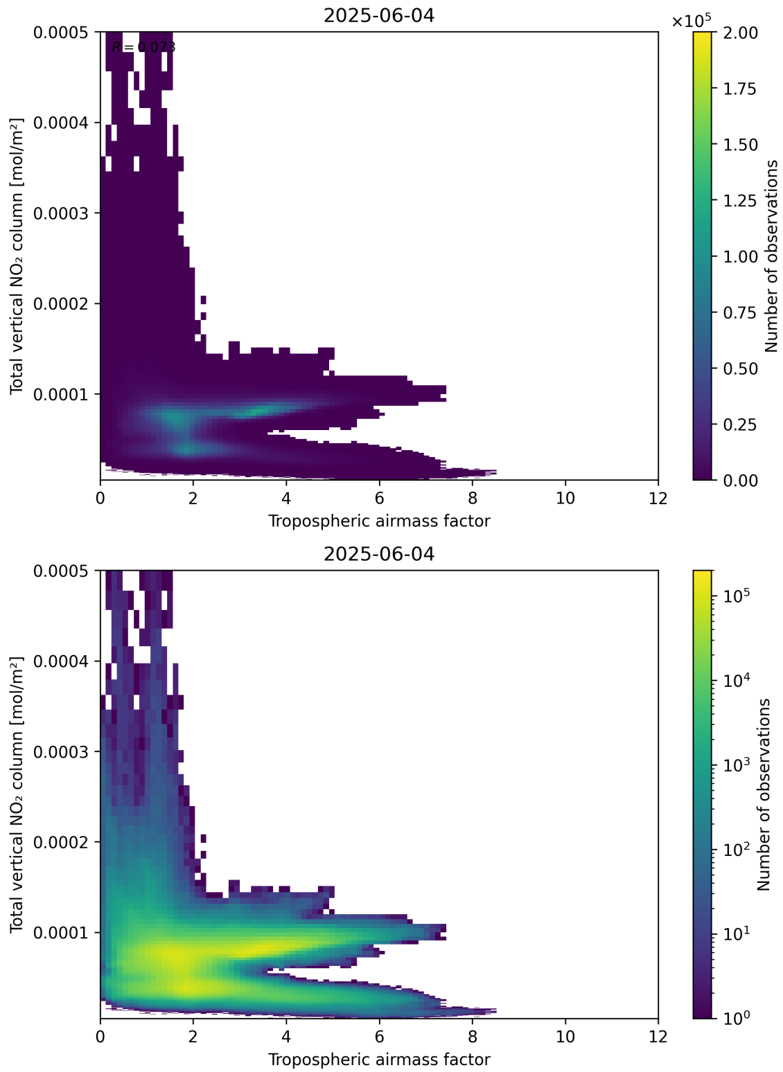
Figure 77: Scatter density plot of “Tropospheric airmass factor” against “Total vertical NO 2 column” for 2025-06-03 to 2025-06-05.
