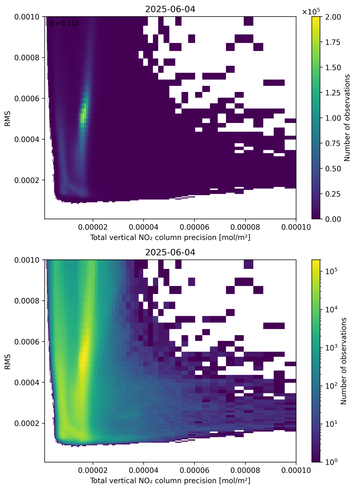
Figure 119: Scatter density plot of “Total vertical NO 2 column precision” against “RMS” for 2025-06-03 to 2025-06-05.
