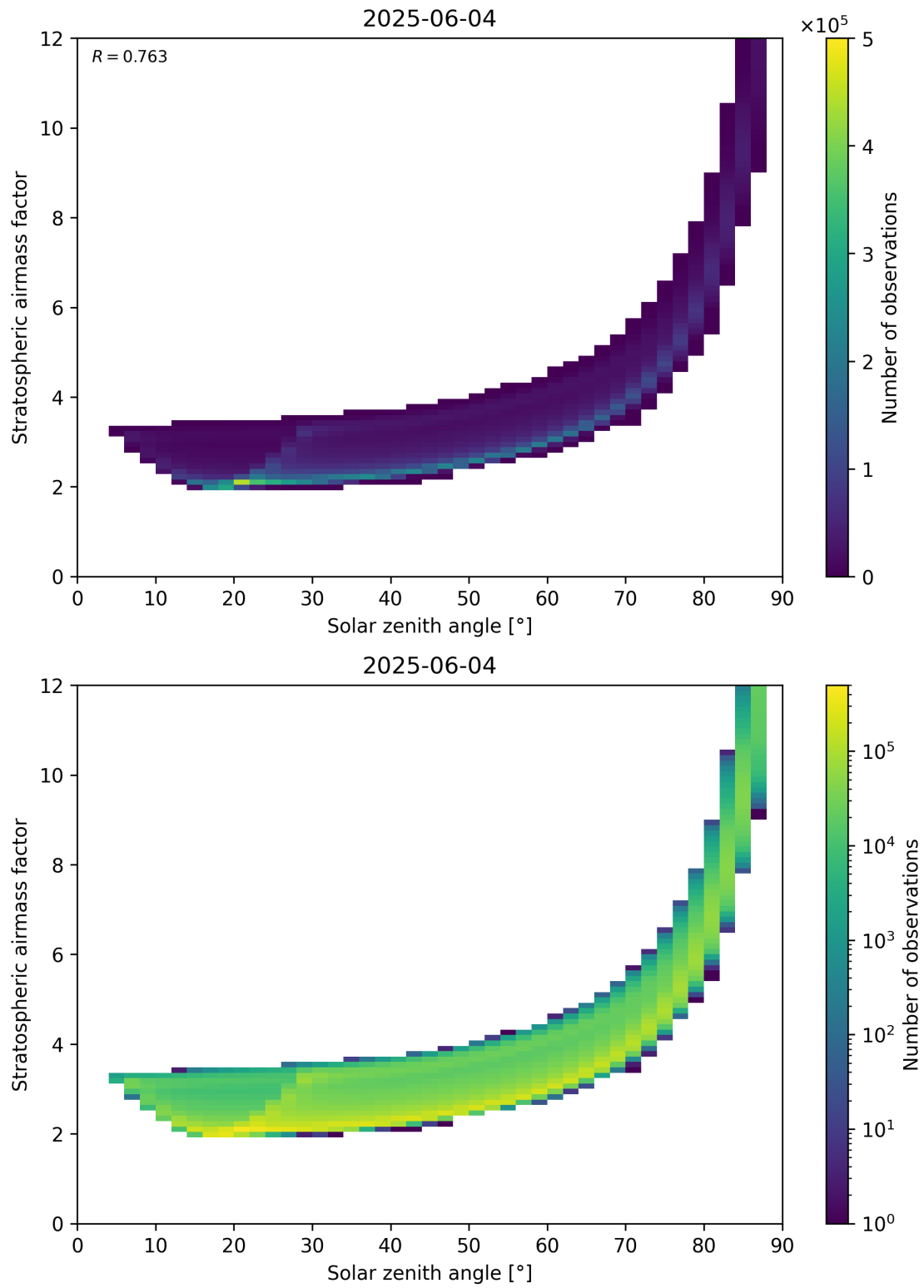
Figure 145: Scatter density plot of “Solar zenith angle” against “Stratospheric airmass factor” for 2025-06-03 to 2025-06-05.
