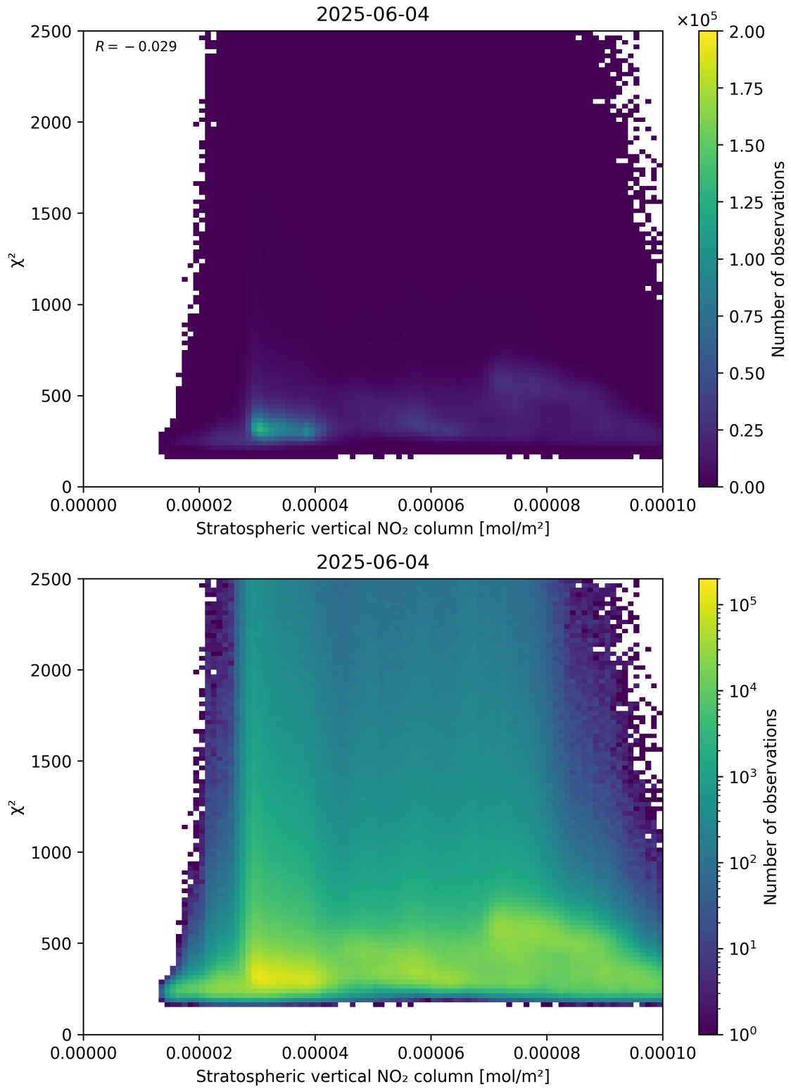
Figure 97: Scatter density plot of “Stratospheric vertical NO 2 column” against “ \chi^2 ” for 2025-06-03 to 2025-06-05.
