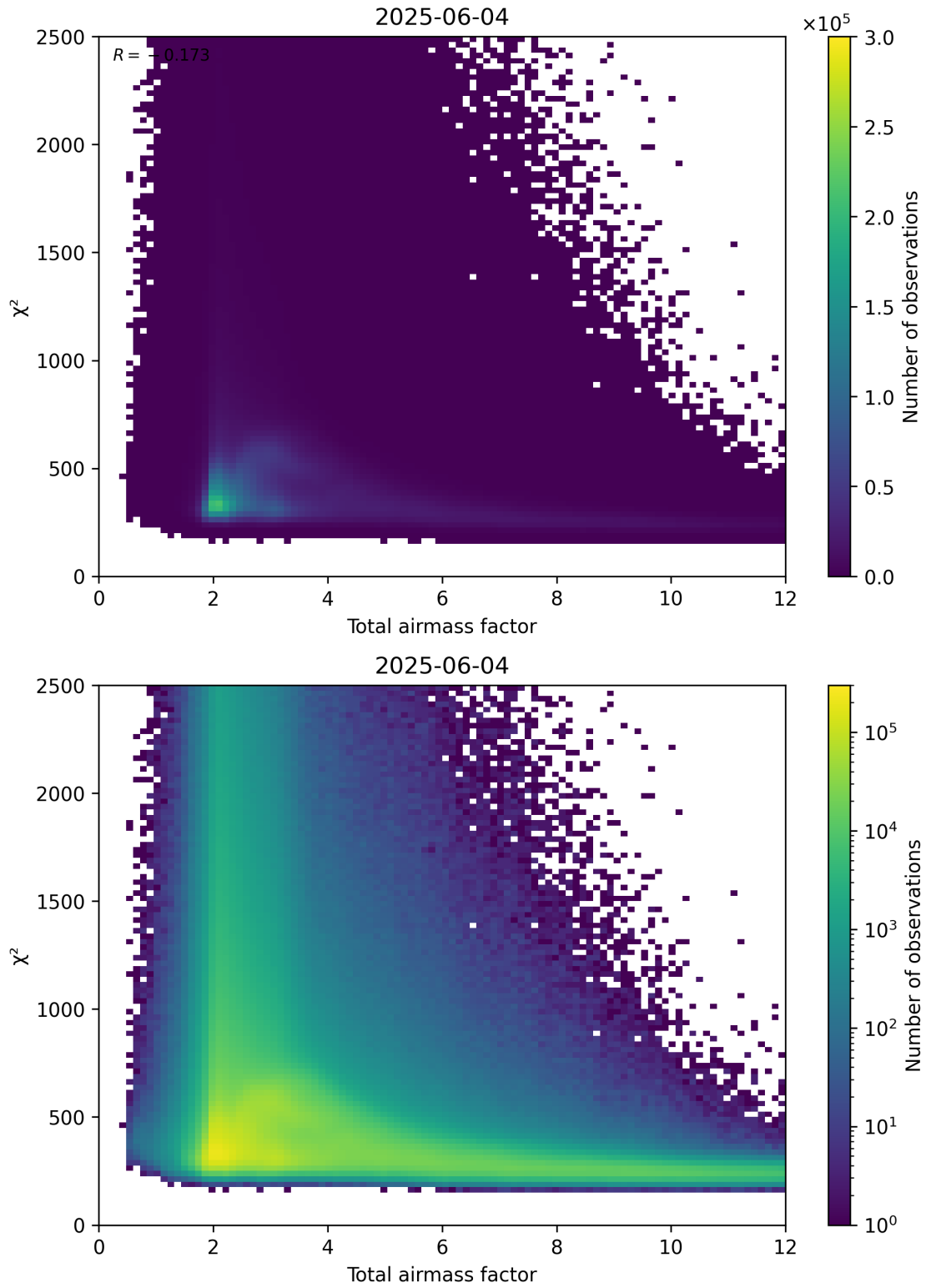
Figure 63: Scatter density plot of “Total airmass factor” against “ \chi^2 ” for 2025-06-03 to 2025-06-05.
