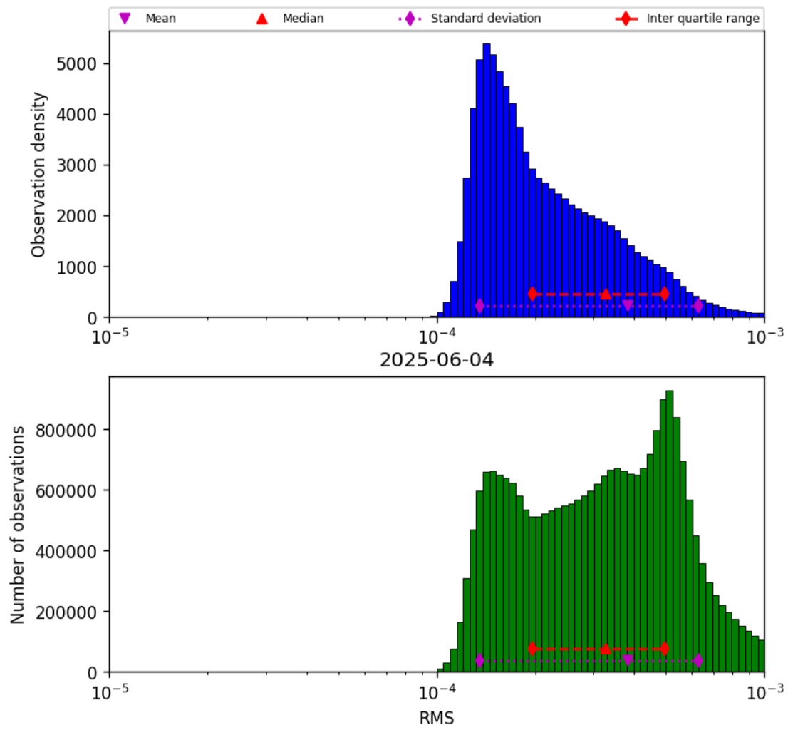
Figure 43: Histogram of “RMS” for 2025-06-03 to 2025-06-05
