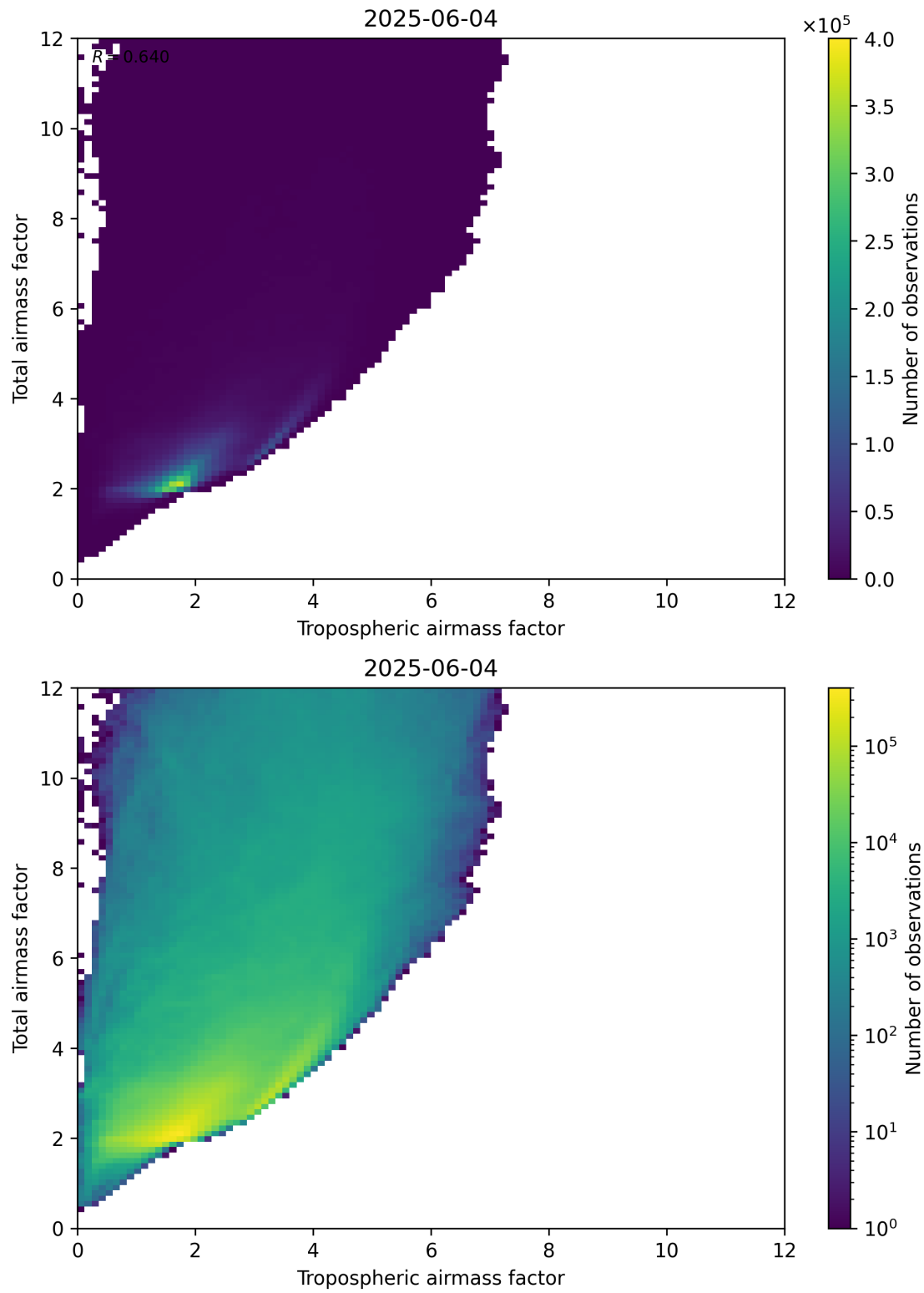
Figure 72: Scatter density plot of “Tropospheric airmass factor” against “Total airmass factor” for 2025-06-03 to 2025-06-05.
