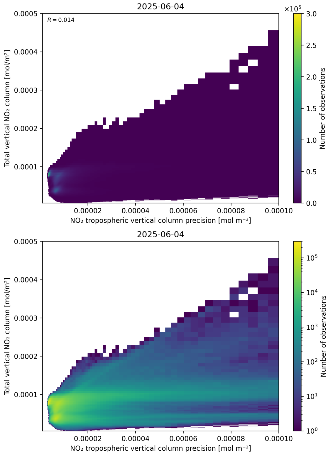
Figure 138: Scatter density plot of “NO 2 tropospheric vertical column precision” against “Total vertical NO 2 column” for 2025-06-03 to 2025-06-05.
