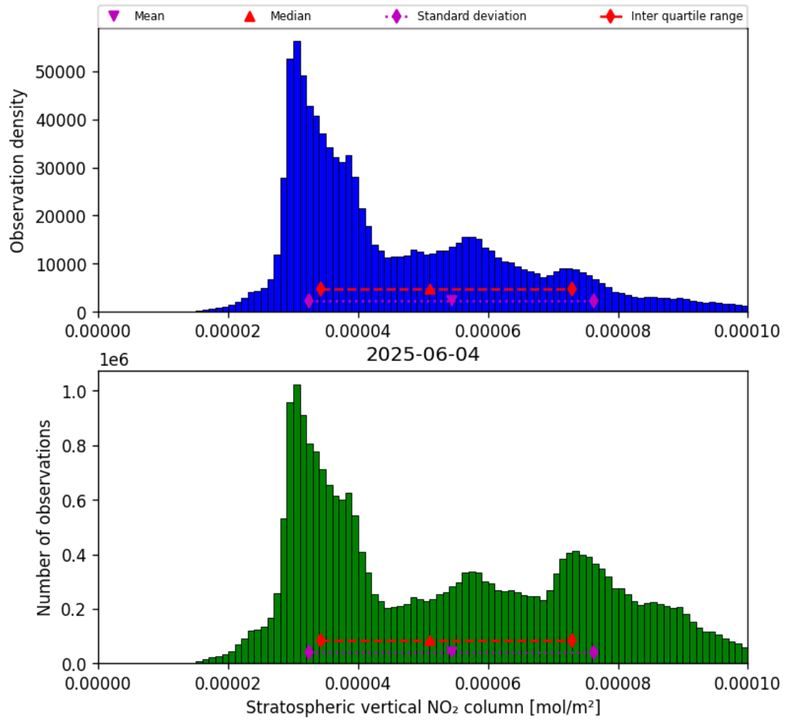
Figure 36: Histogram of “Stratospheric vertical NO 2 column” for 2025-06-03 to 2025-06-05
