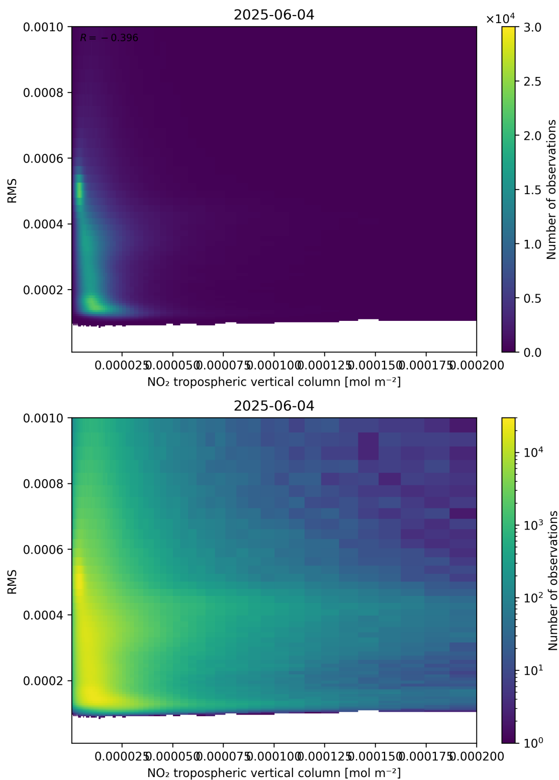
Figure 142: Scatter density plot of “NO 2 tropospheric vertical column” against “RMS” for 2025-06-03 to 2025-06-05.
