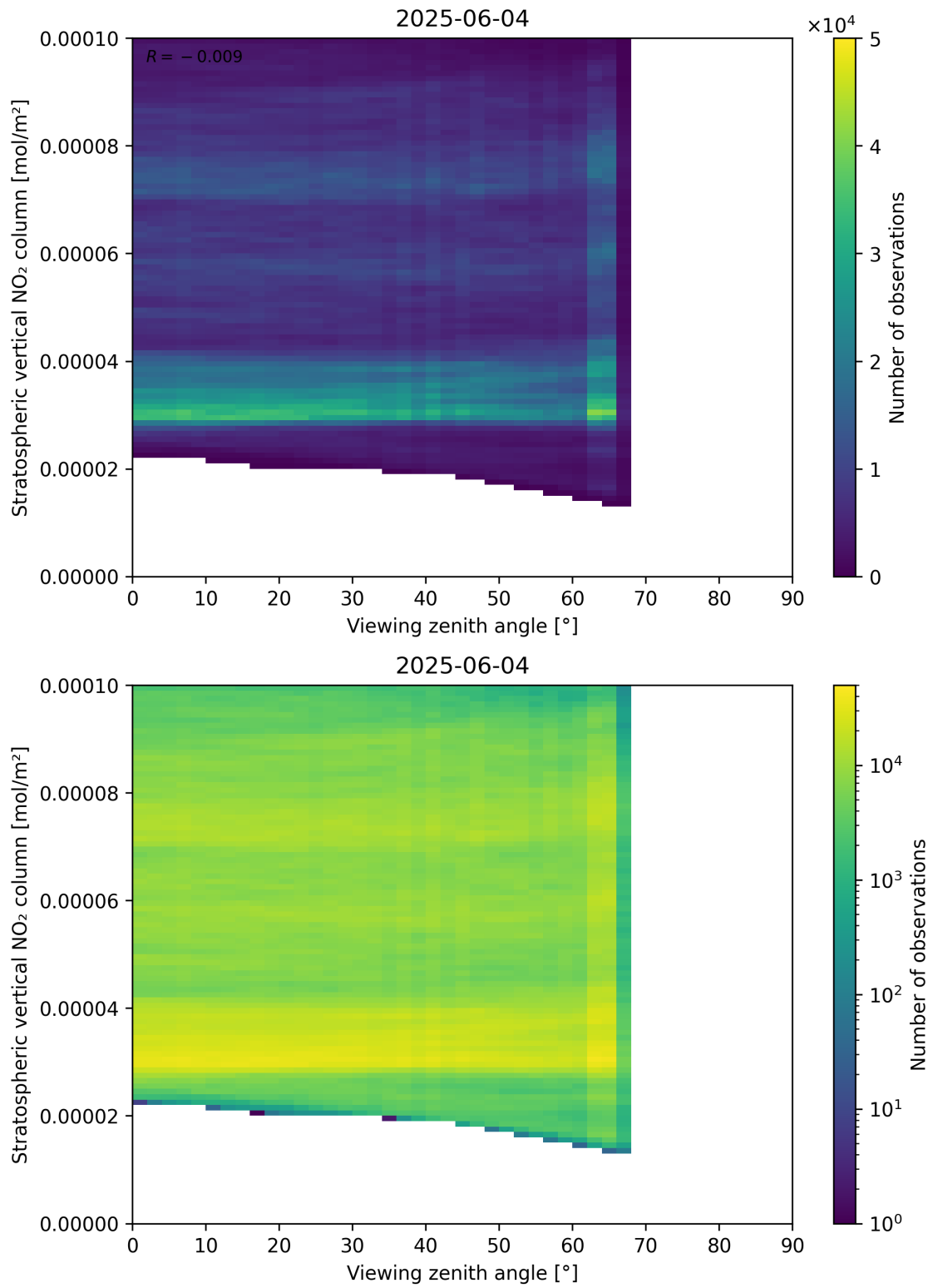
Figure 164: Scatter density plot of “Viewing zenith angle” against “Stratospheric vertical NO 2 column” for 2025-06-03 to 2025-06-05.
