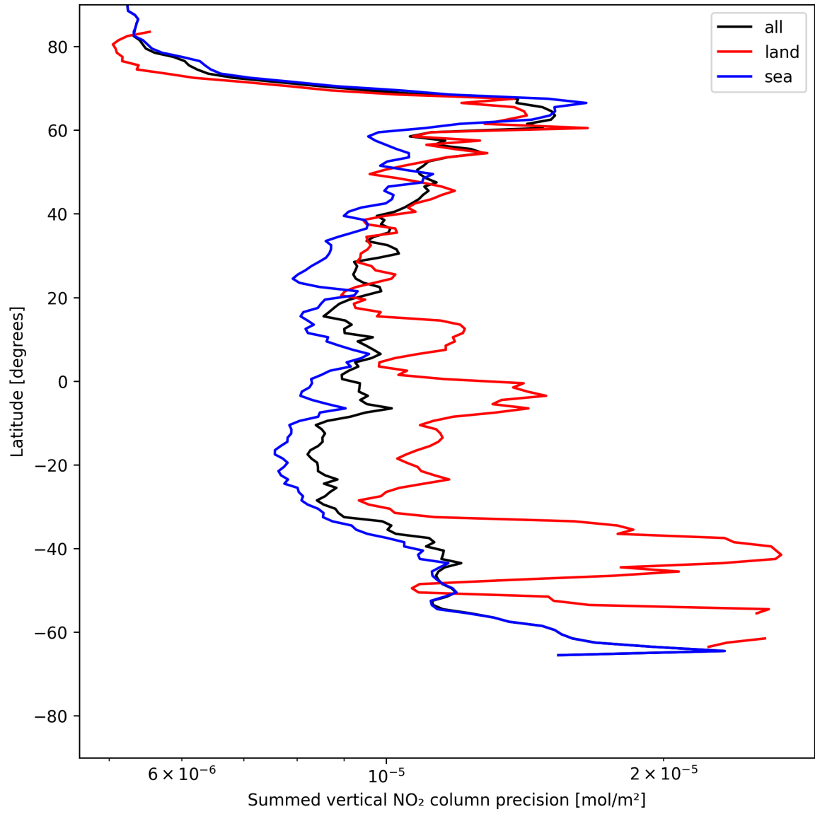
Figure 24: Zonal average of “Summed vertical NO 2 column precision” for 2025-06-03 to 2025-06-05.
