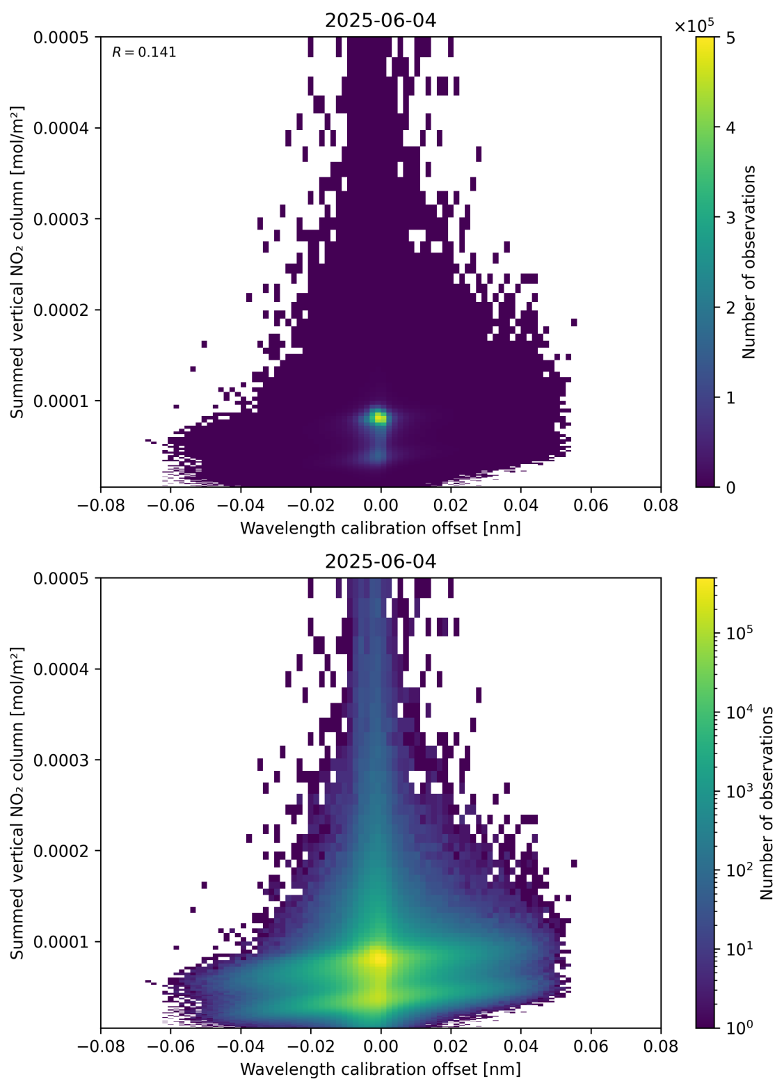
Figure 177: Scatter density plot of “Wavelength calibration offset” against “Summed vertical NO 2 column” for 2025-06-03 to 2025-06-05.
