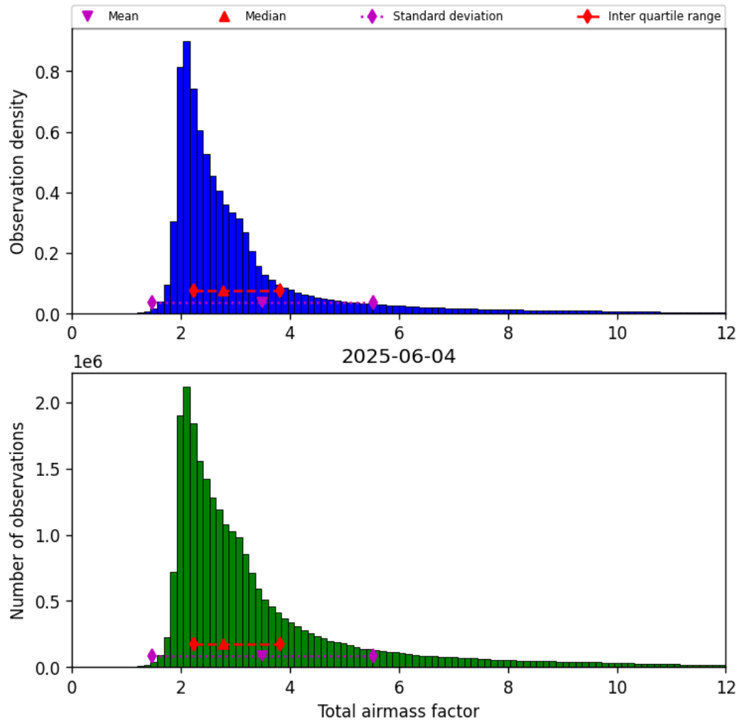
Figure 32: Histogram of “Total airmass factor” for 2025-06-03 to 2025-06-05
