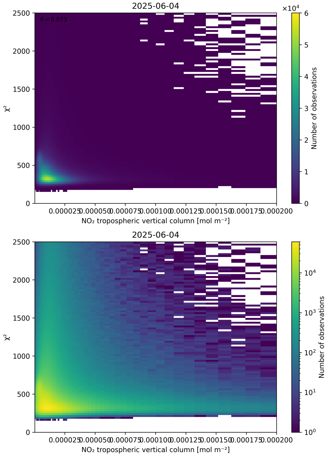
Figure 124: Scatter density plot of “NO 2 tropospheric vertical column” against “ \chi^2 ” for 2025-06-03 to 2025-06-05.
