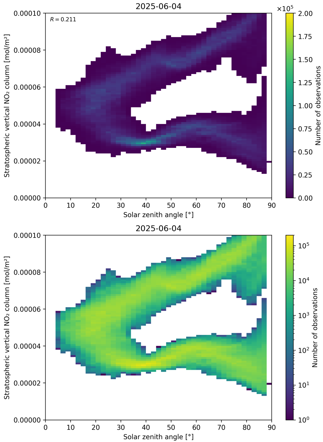
Figure 150: Scatter density plot of “Solar zenith angle” against “Stratospheric vertical NO 2 column” for 2025-06-03 to 2025-06-05.
