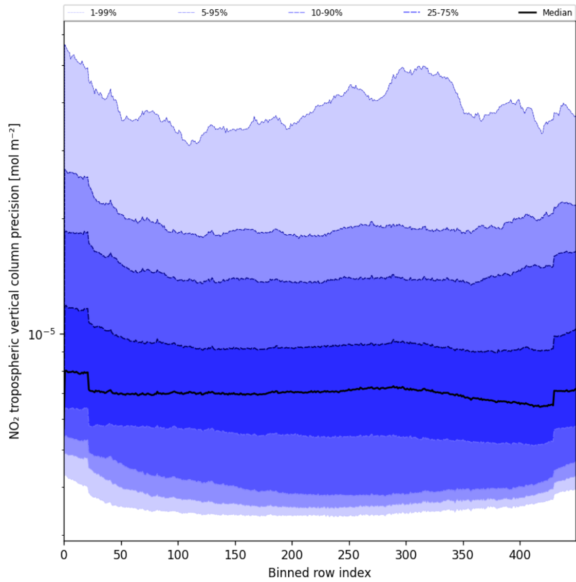
Figure 47: Along track statistics of “NO 2 tropospheric vertical column precision” for 2025-06-03 to 2025-06-05
