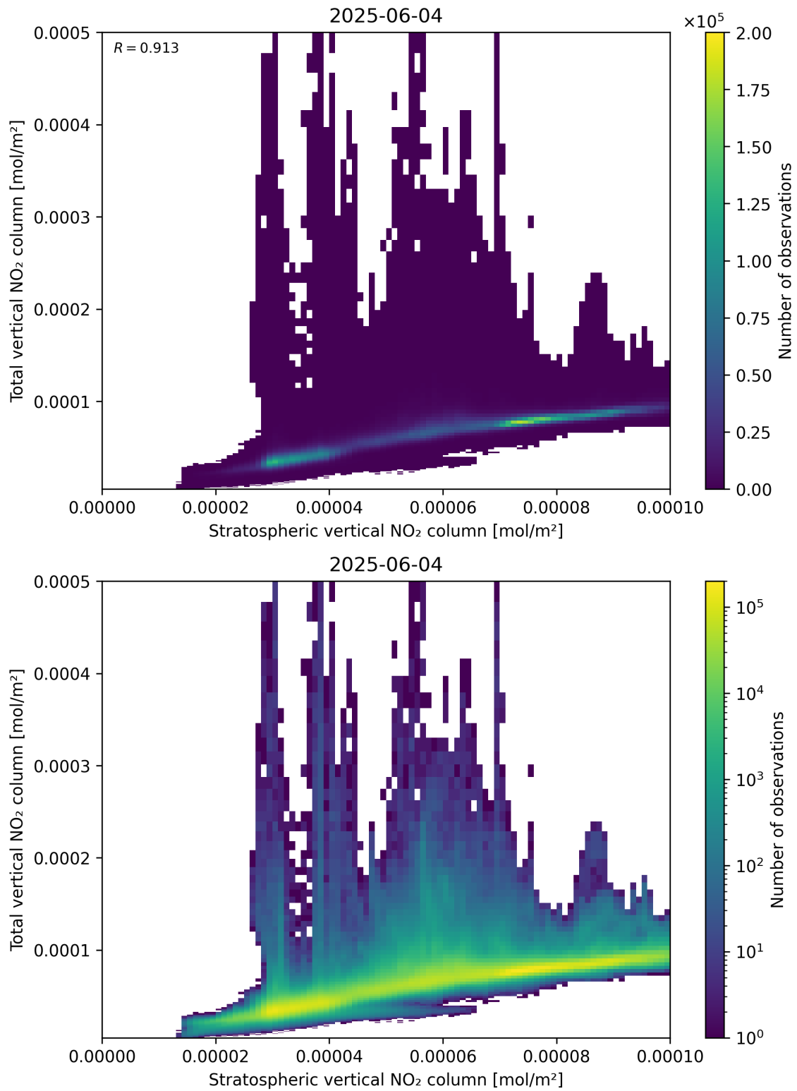
Figure 100: Scatter density plot of “Stratospheric vertical NO 2 column” against “Total vertical NO 2 column” for 2025-06-03 to 2025-06-05.
