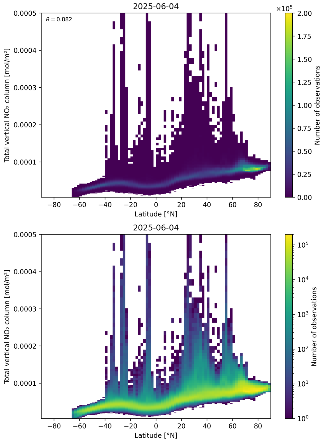
Figure 90: Scatter density plot of “Latitude” against “Total vertical NO 2 column” for 2025-06-03 to 2025-06-05.
