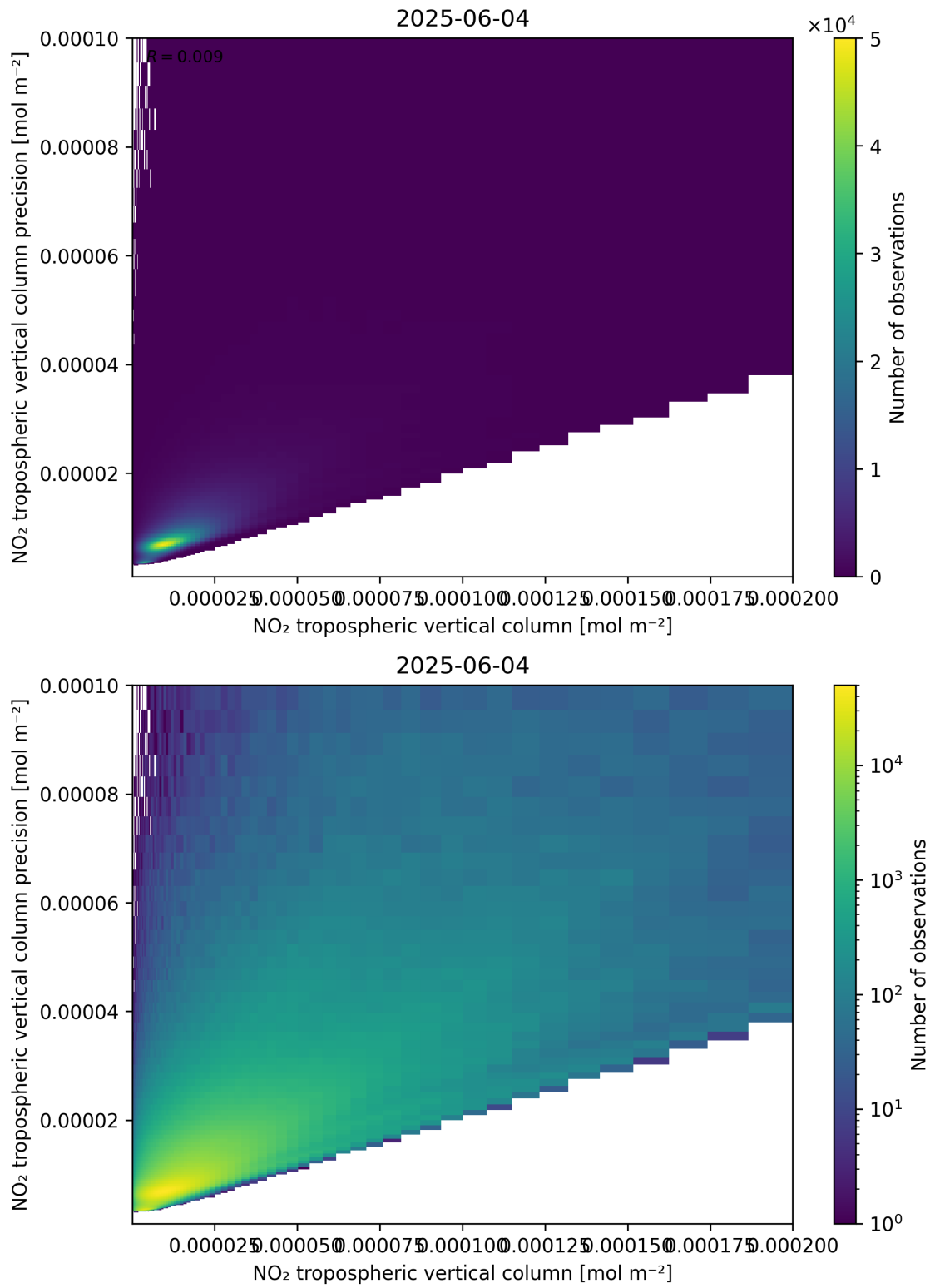
Figure 130: Scatter density plot of “NO 2 tropospheric vertical column” against “NO 2 tropospheric vertical column precision” for 2025-06-03 to 2025-06-05.
