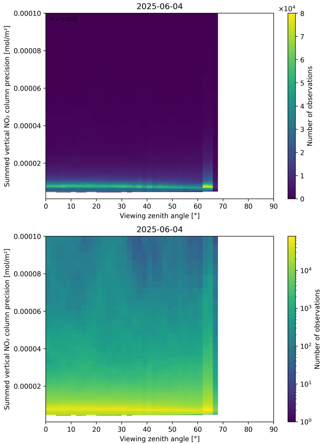
Figure 166: Scatter density plot of “Viewing zenith angle” against “Summed vertical NO 2 column precision” for 2025-06-03 to 2025-06-05.
