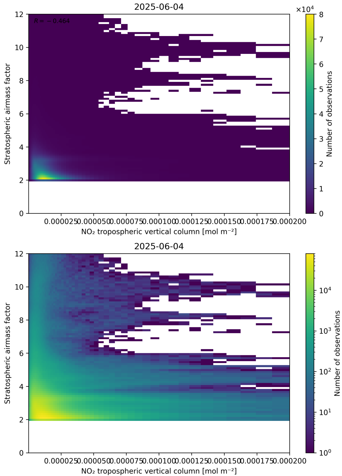
Figure 121: Scatter density plot of “NO 2 tropospheric vertical column” against “Stratospheric air mass factor” for 2025-06-03 to 2025-06-05.
