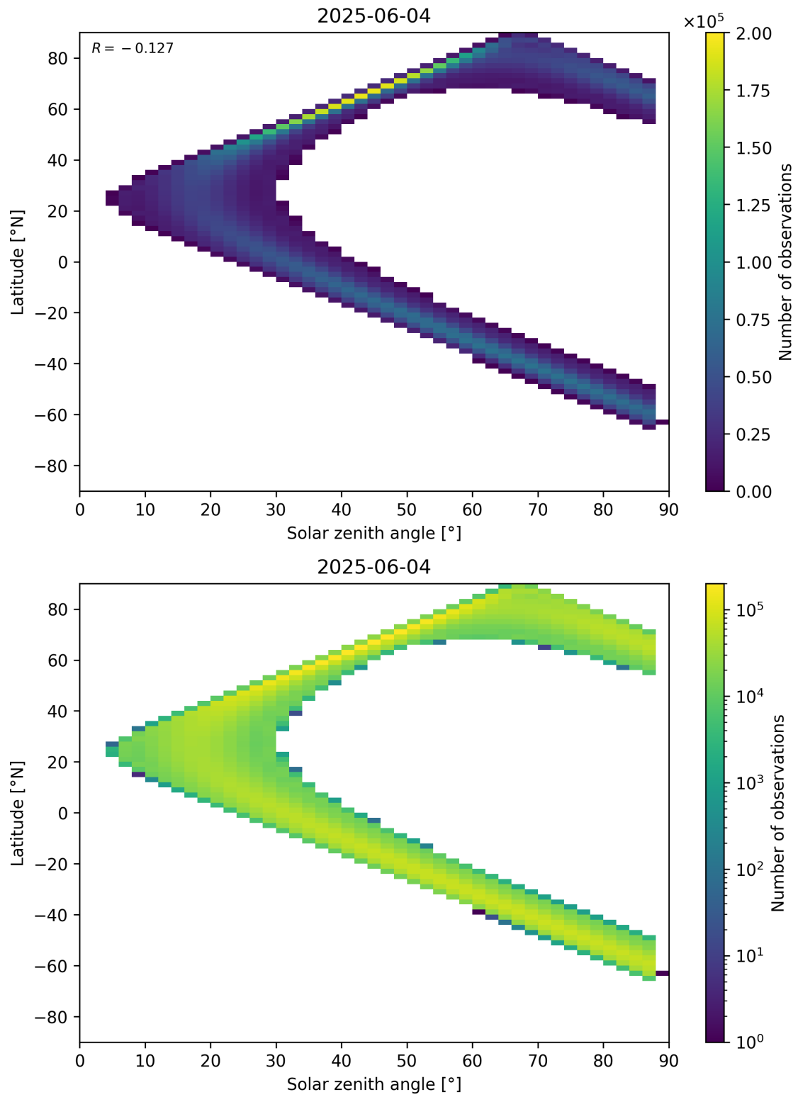
Figure 149: Scatter density plot of “Solar zenith angle” against “Latitude” for 2025-06-03 to 2025-06-05.
