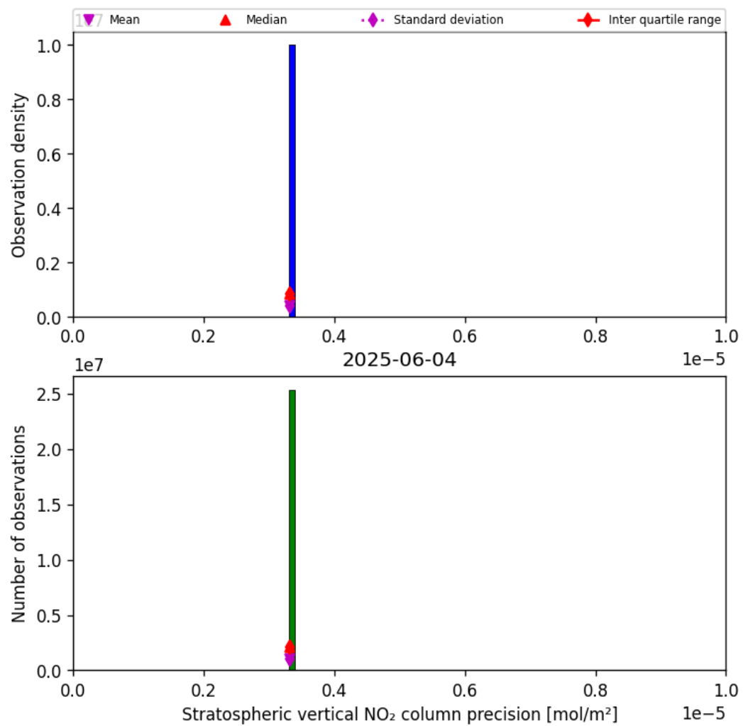
Figure 37: Histogram of “Stratospheric vertical NO 2 column precision” for 2025-06-03 to 2025-06-05
