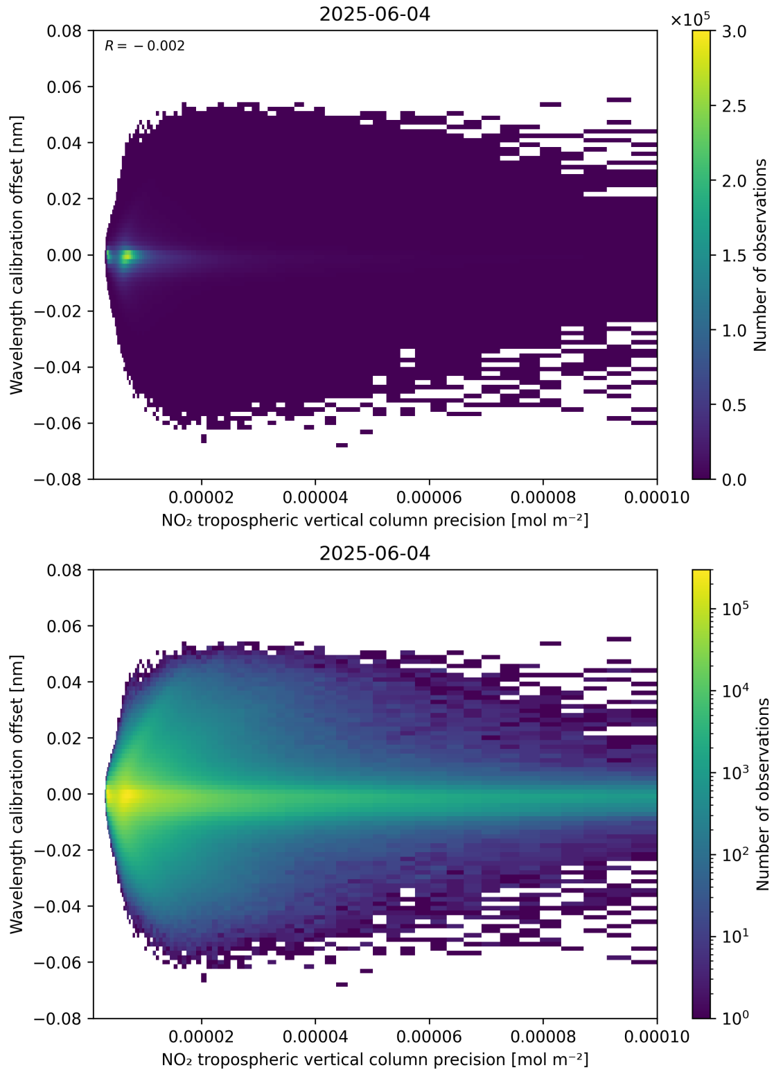
Figure 141: Scatter density plot of “NO 2 tropospheric vertical column precision” against “Wavelength calibration offset” for 2025-06-03 to 2025-06-05.
