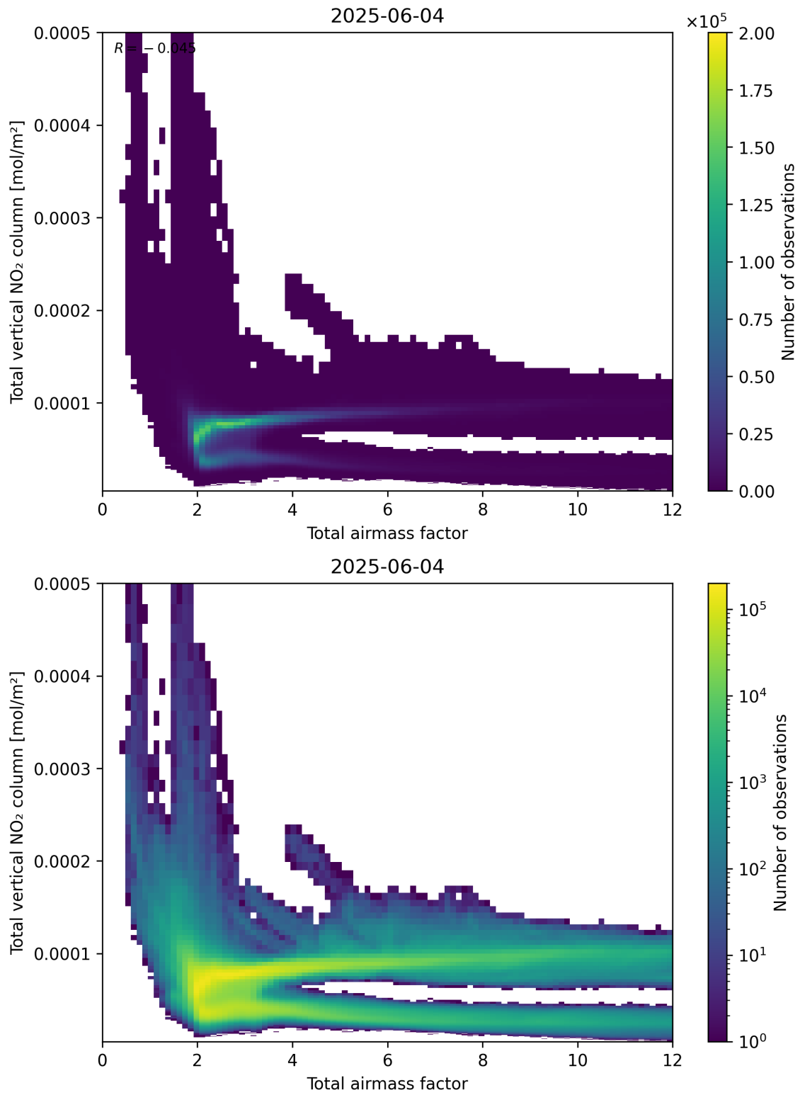
Figure 67: Scatter density plot of “Total airmass factor” against “Total vertical NO 2 column” for 2025-06-03 to 2025-06-05.
