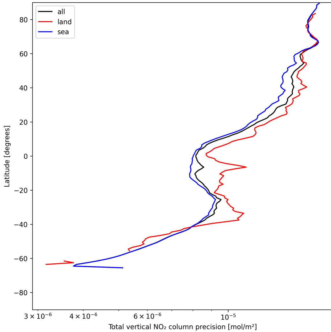
Figure 22: Zonal average of “Total vertical NO 2 column precision” for 2025-06-03 to 2025-06-05.
