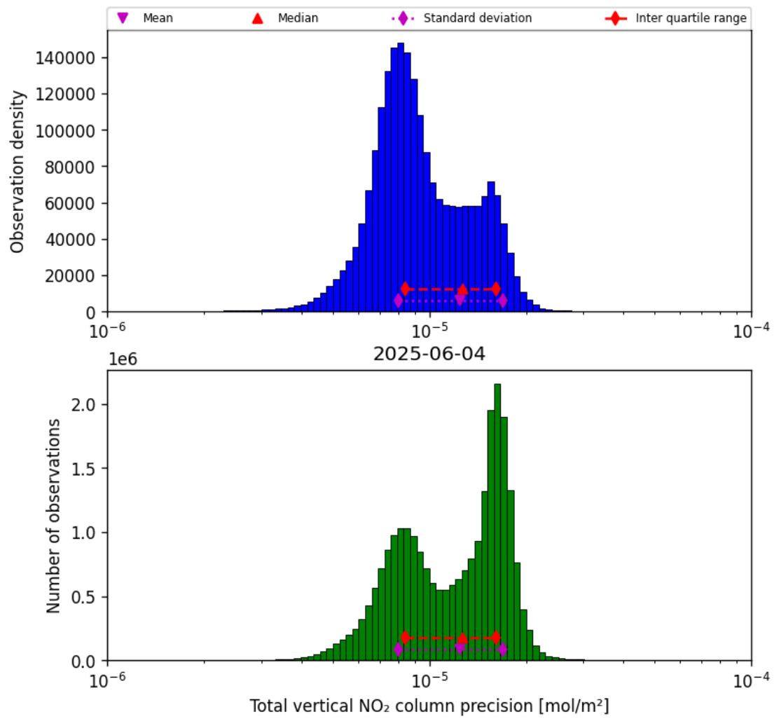
Figure 39: Histogram of “Total vertical NO 2 column precision” for 2025-06-03 to 2025-06-05
