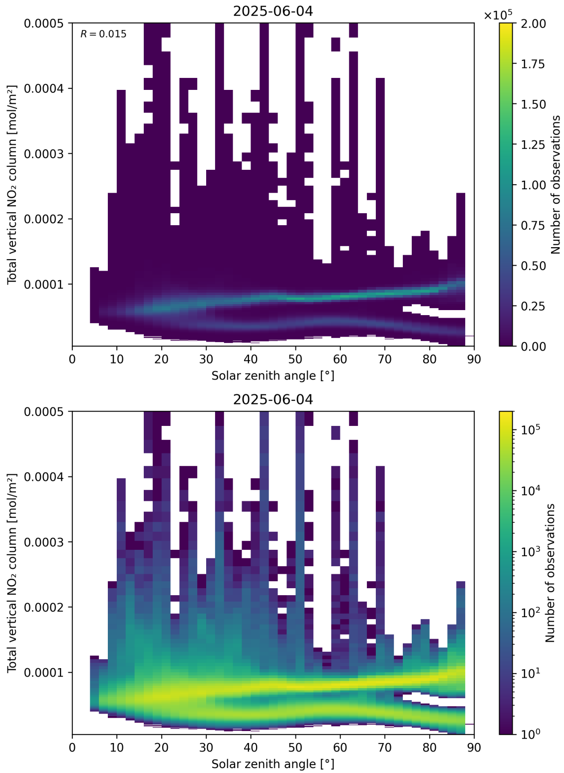
Figure 153: Scatter density plot of “Solar zenith angle” against “Total vertical NO 2 column” for 2025-06-03 to 2025-06-05.
