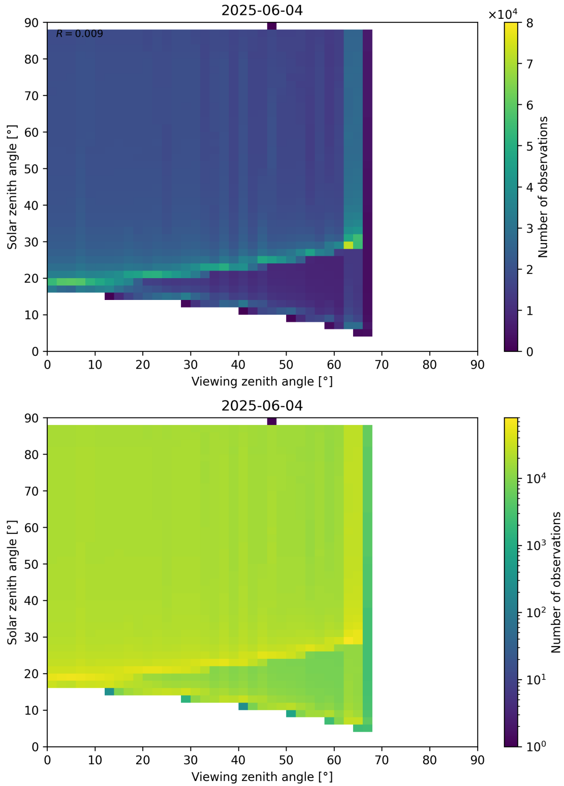
Figure 172: Scatter density plot of “Viewing zenith angle” against “Solar zenith angle” for 2025-06-03 to 2025-06-05.
