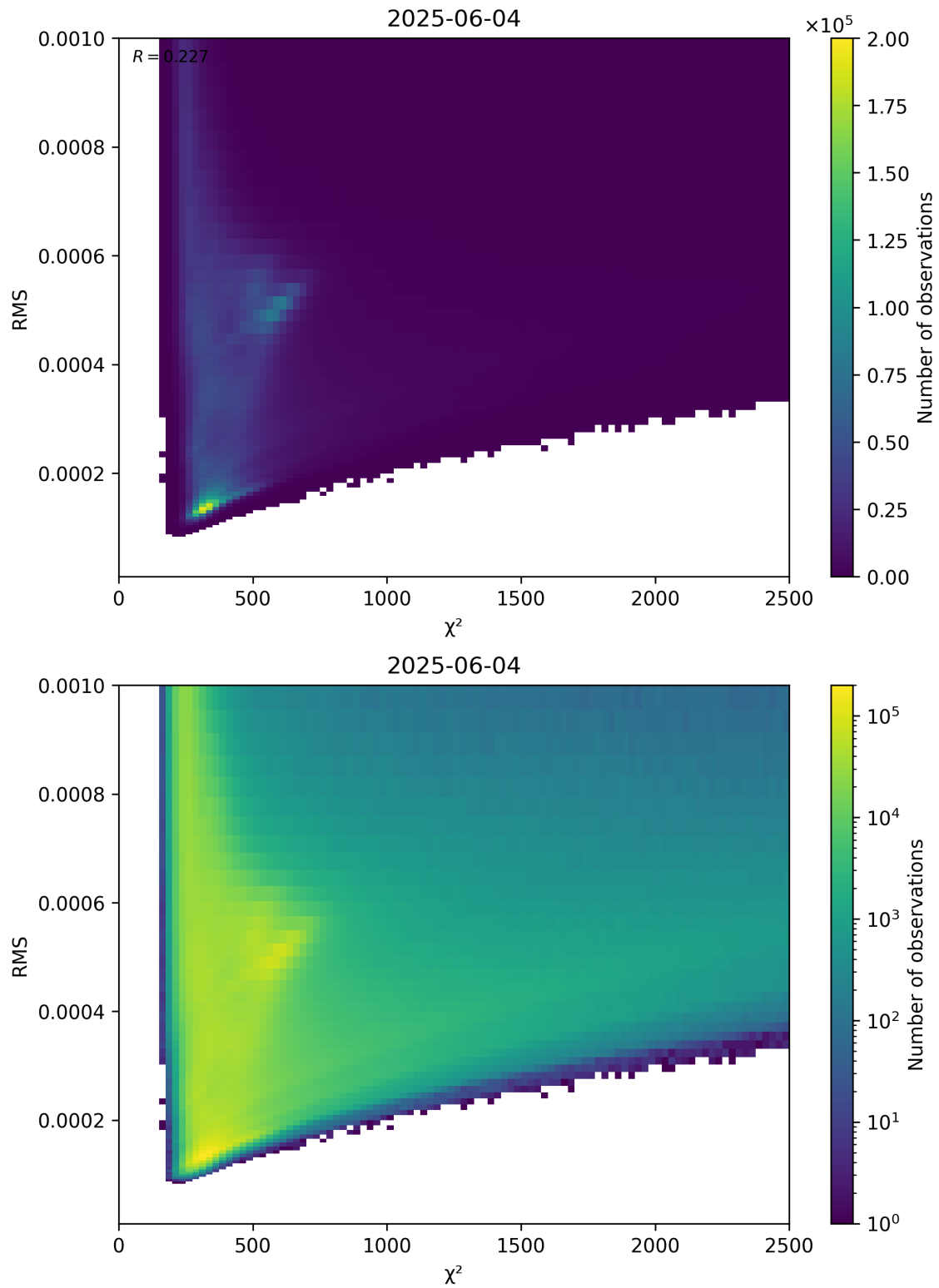
Figure 82: Scatter density plot of “ \chi^2 ” against “RMS” for 2025-06-03 to 2025-06-05.
