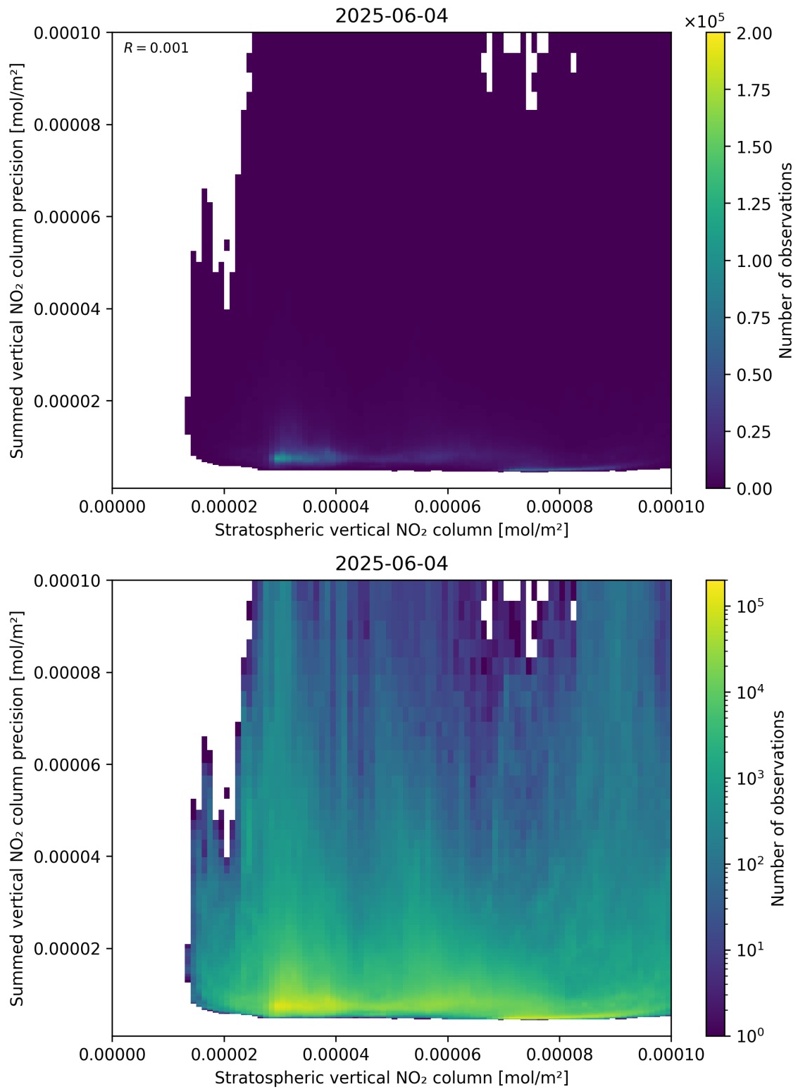
Figure 99: Scatter density plot of “Stratospheric vertical NO 2 column” against “Summed vertical NO 2 column precision” for 2025-06-03 to 2025-06-05.
