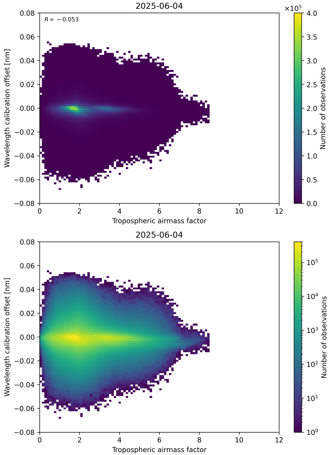
Figure 80: Scatter density plot of “Tropospheric airmass factor” against “Wavelength calibration offset” for 2025-06-03 to 2025-06-05.
