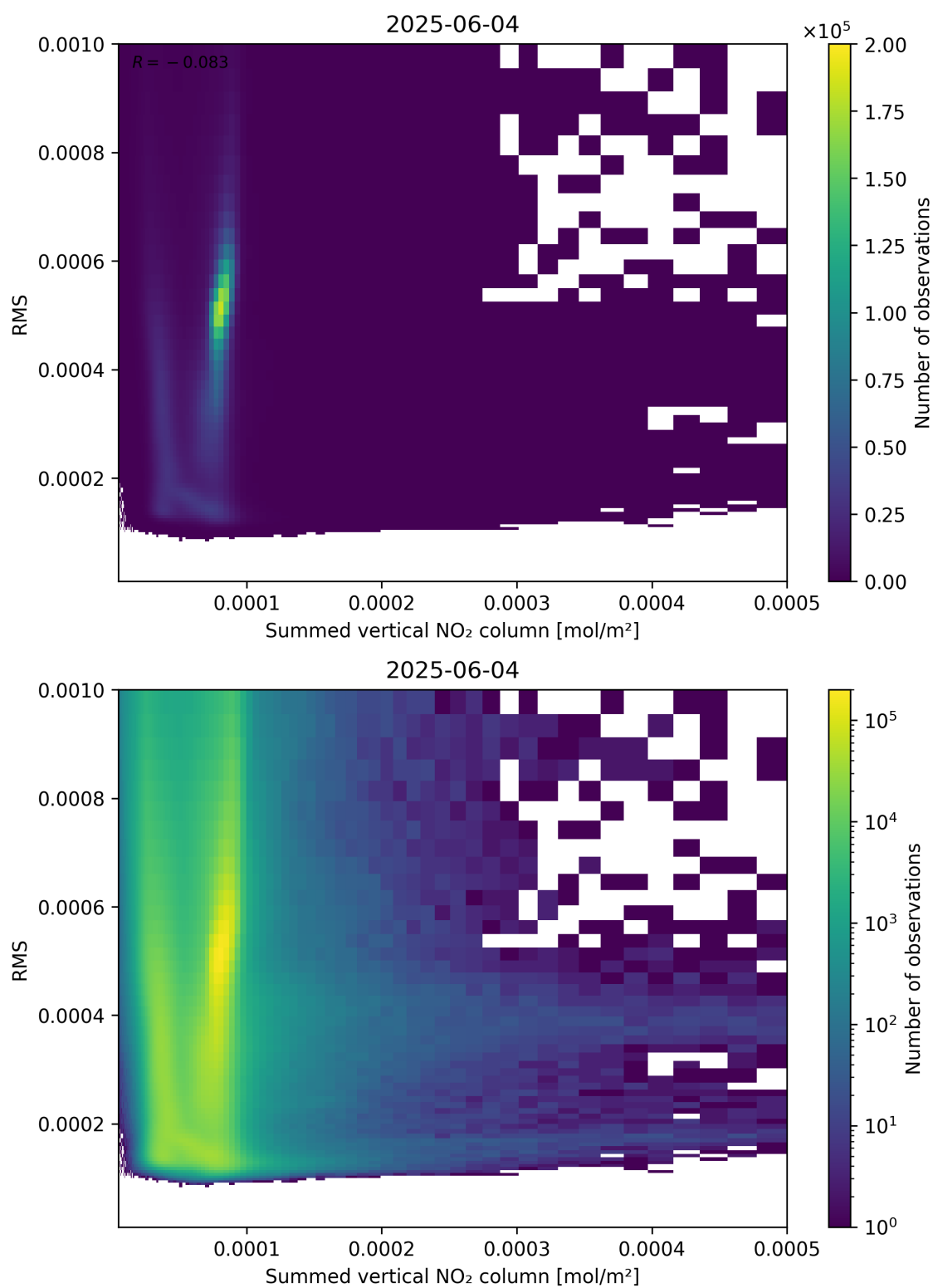
Figure 109: Scatter density plot of “Summed vertical NO 2 column” against “RMS” for 2025-06-03 to 2025-06-05.
