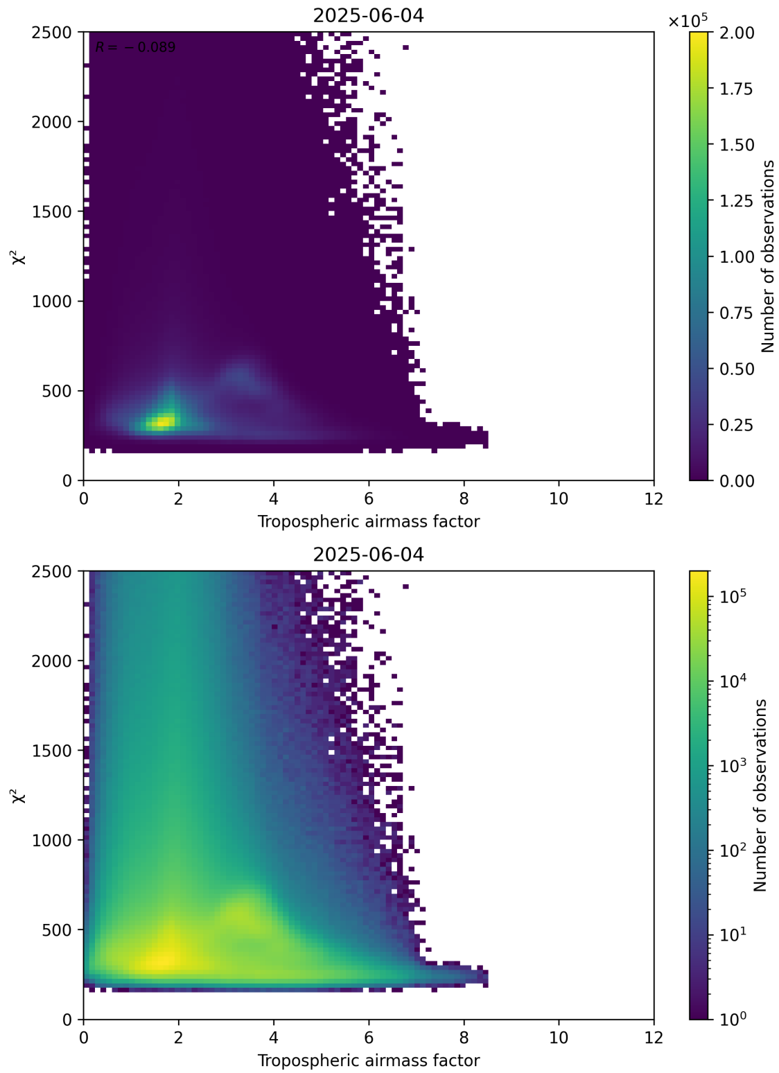
Figure 73: Scatter density plot of “Tropospheric airmass factor” against “ \chi^2 ” for 2025-06-03 to 2025-06-05.
