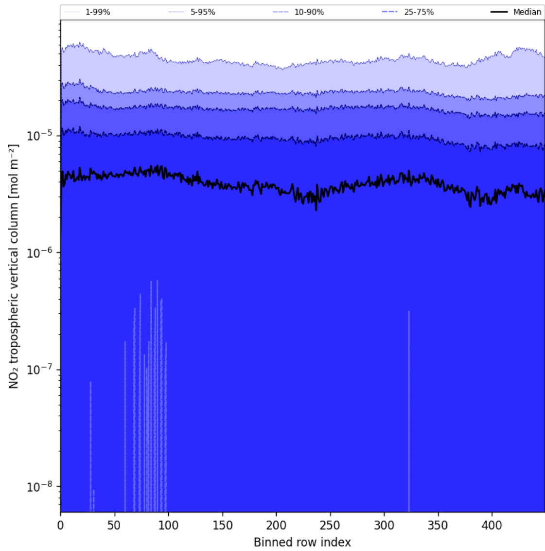
Figure 46: Along track statistics of “NO 2 tropospheric vertical column” for 2025-06-03 to 2025-06-05
