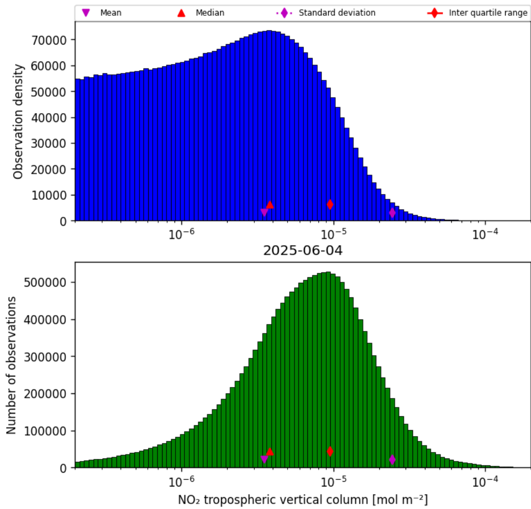
Figure 29: Histogram of “NO 2 tropospheric vertical column” for 2025-06-03 to 2025-06-05
