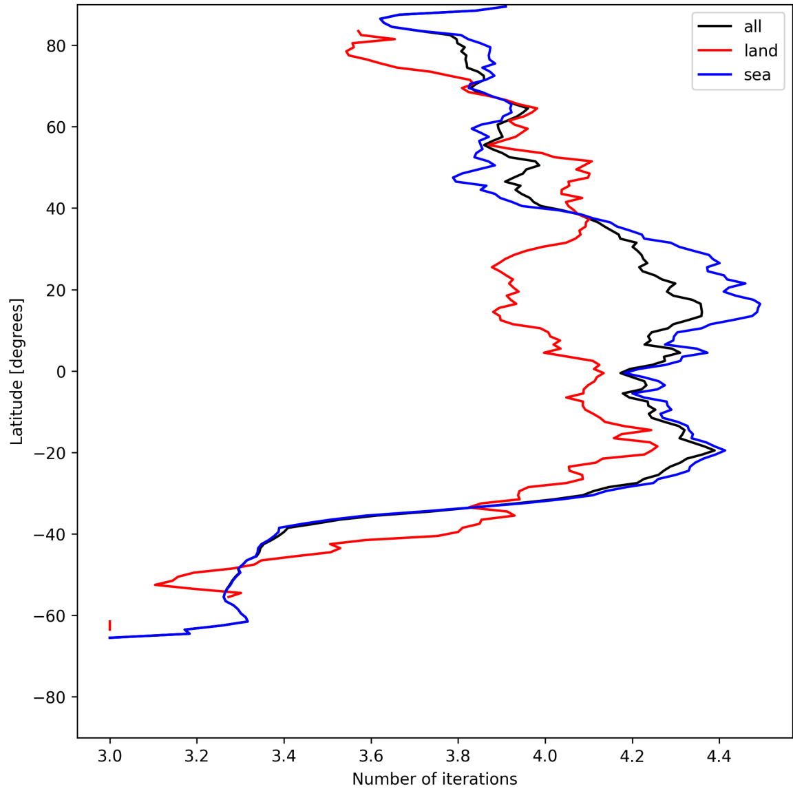
Figure 17: Zonal average of “Number of iterations” for 2025-06-03 to 2025-06-05.
