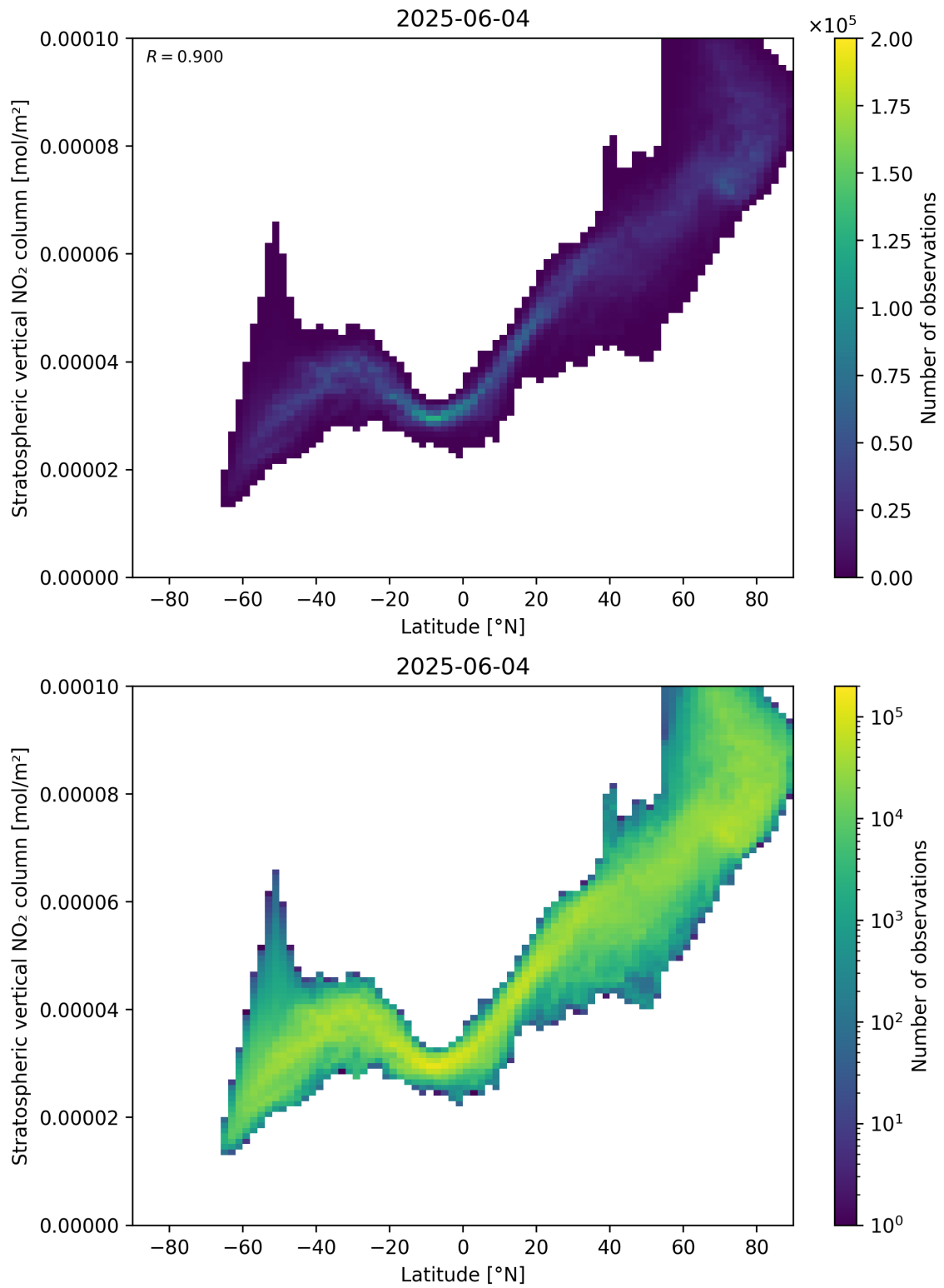
Figure 87: Scatter density plot of “Latitude” against “Stratospheric vertical \text{NO}_2 column” for 2025-06-03 to 2025-06-05.
