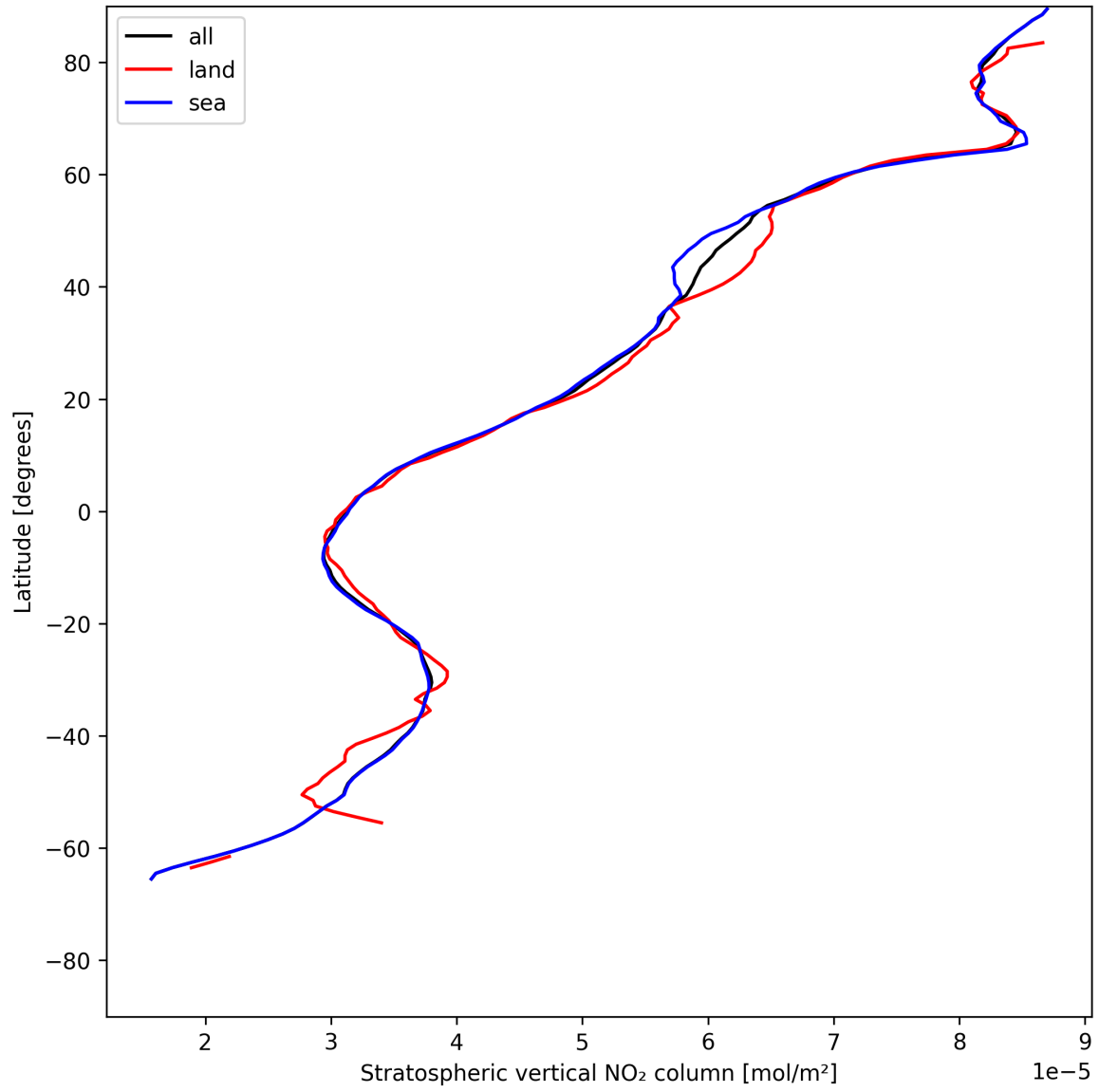
Figure 19: Zonal average of “Stratospheric vertical NO 2 column” for 2025-06-03 to 2025-06-05.
