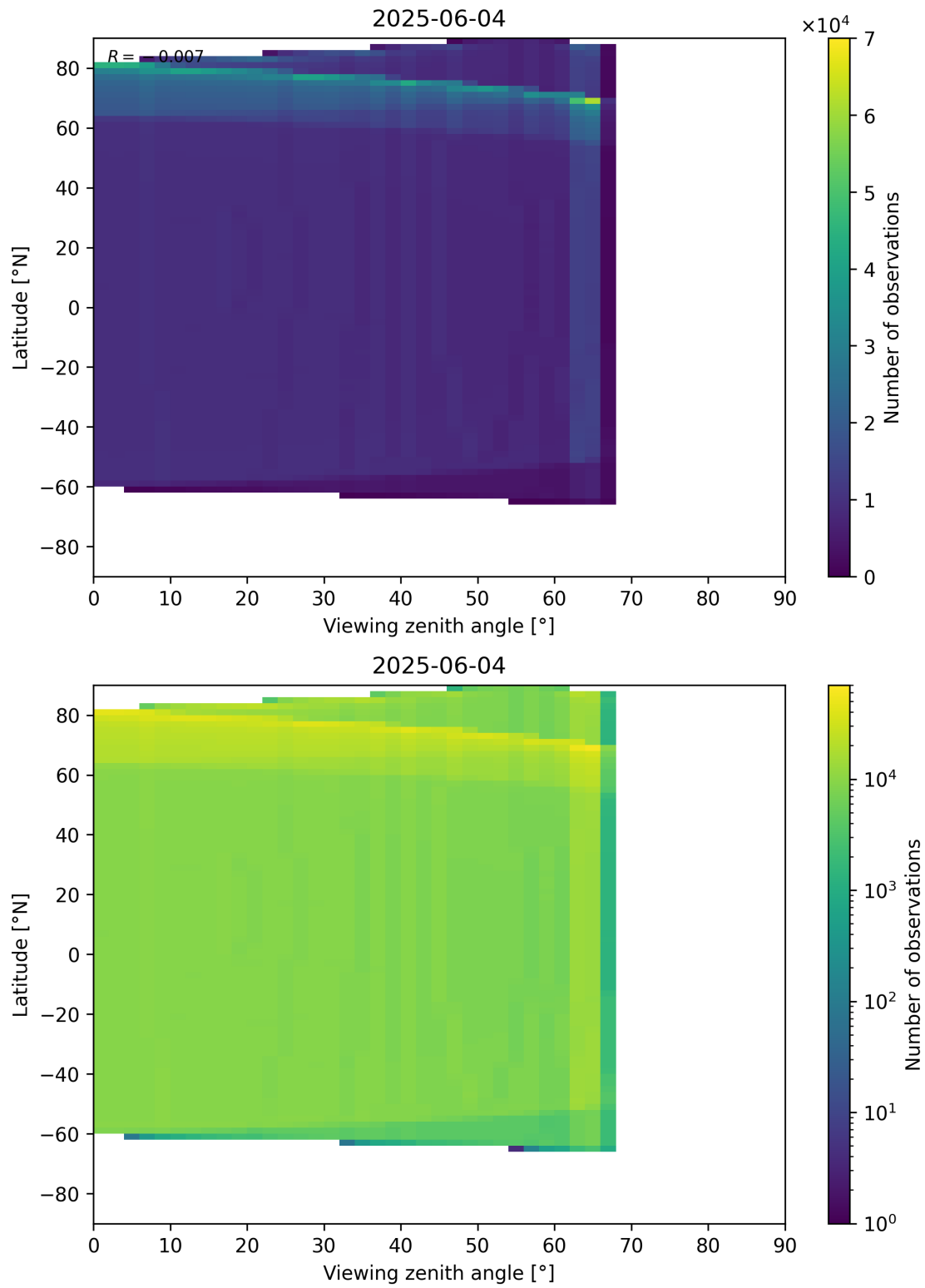
Figure 163: Scatter density plot of “Viewing zenith angle” against “Latitude” for 2025-06-03 to 2025-06-05.
