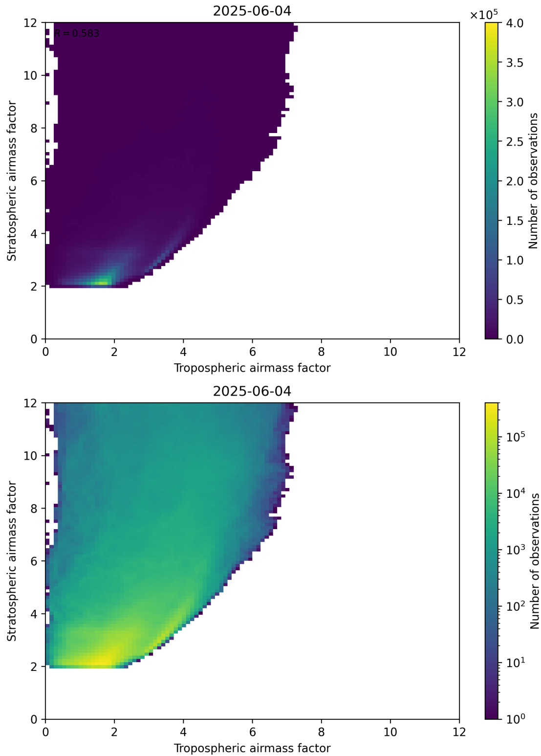
Figure 71: Scatter density plot of “Tropospheric airmass factor” against “Stratospheric airmass factor” for 2025-06-03 to 2025-06-05.
