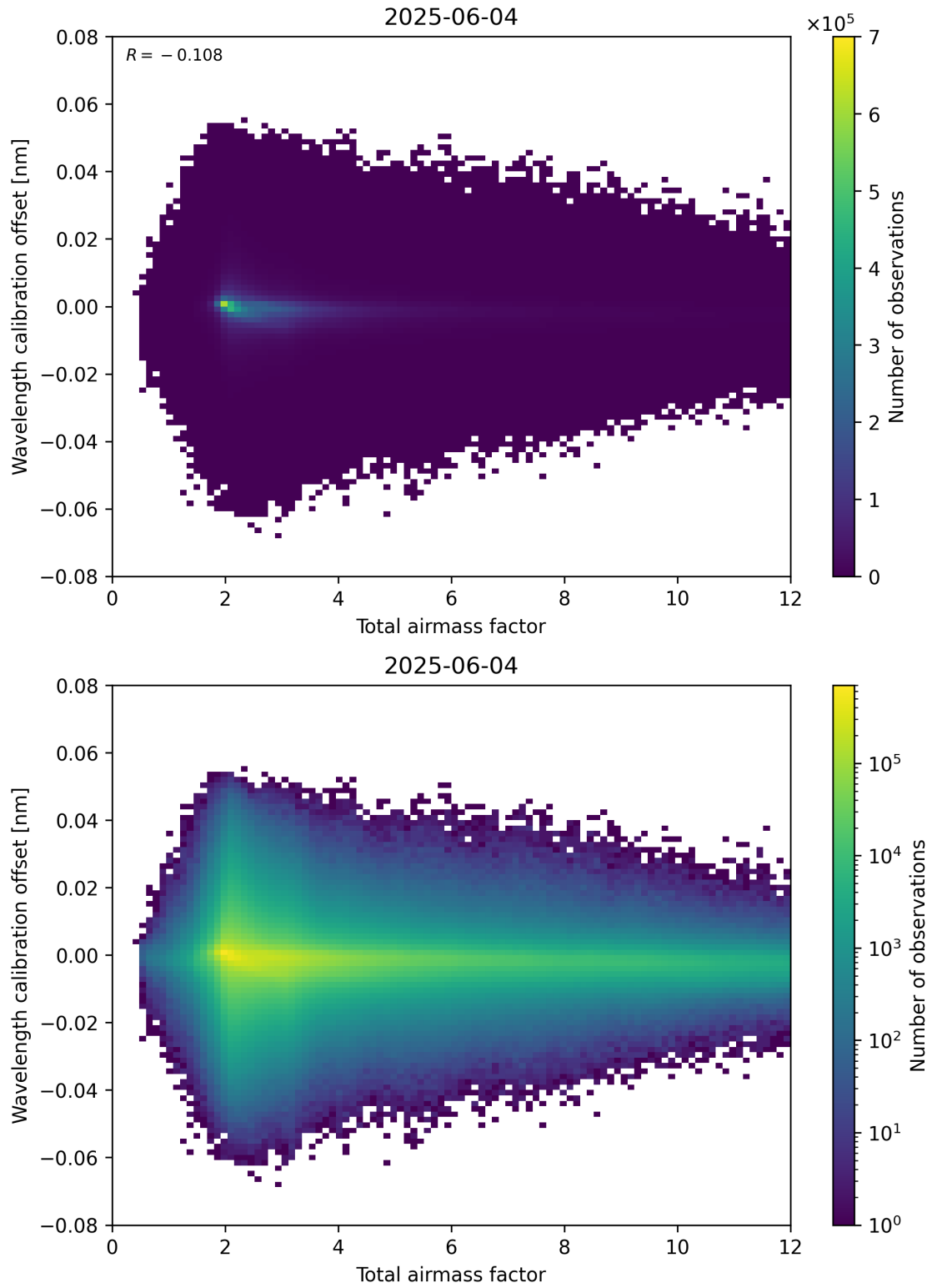
Figure 70: Scatter density plot of “Total airmass factor” against “Wavelength calibration offset” for 2025-06-03 to 2025-06-05.
