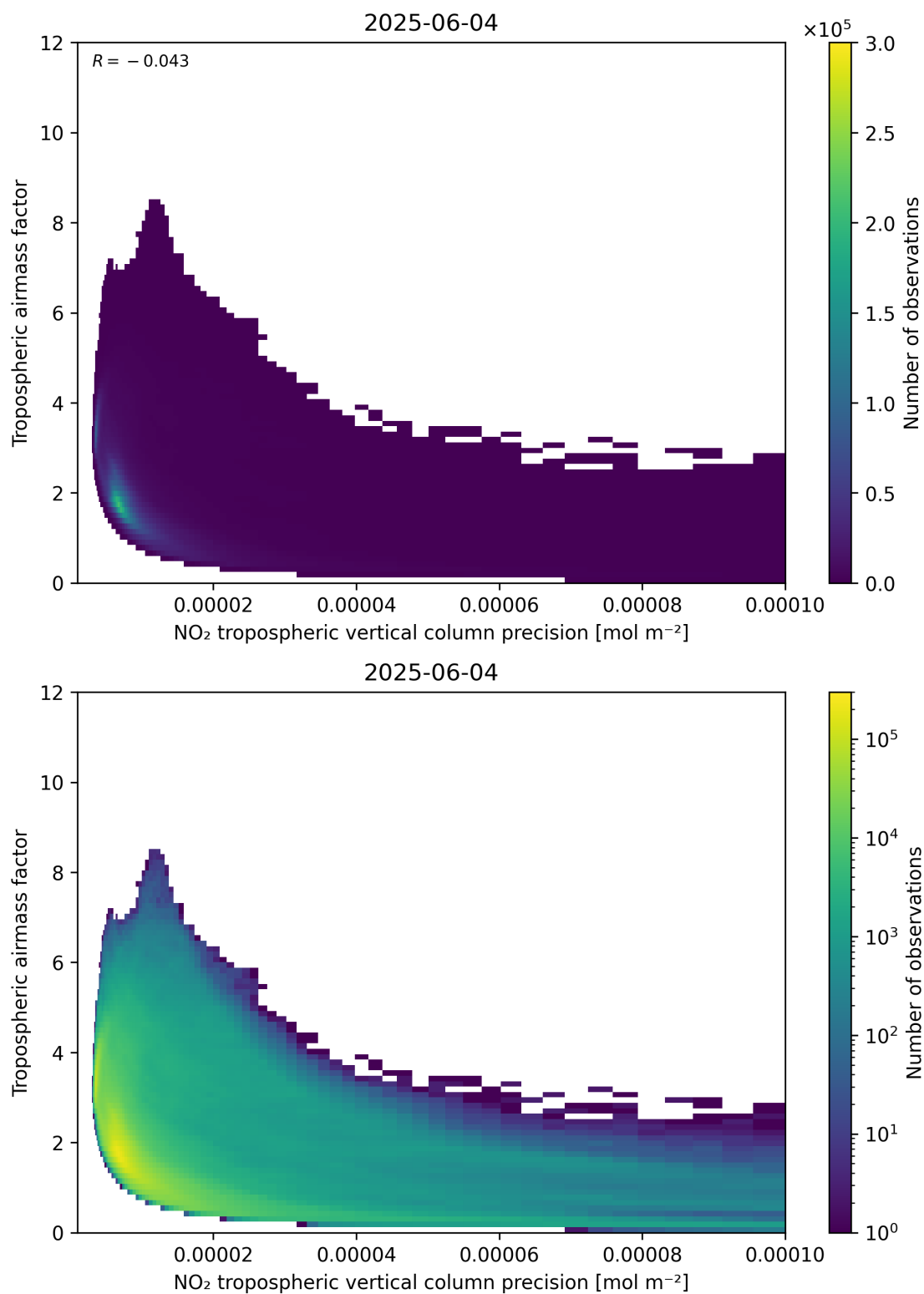
Figure 133: Scatter density plot of “NO 2 tropospheric vertical column precision” against “Tropospheric air mass factor” for 2025-06-03 to 2025-06-05.
