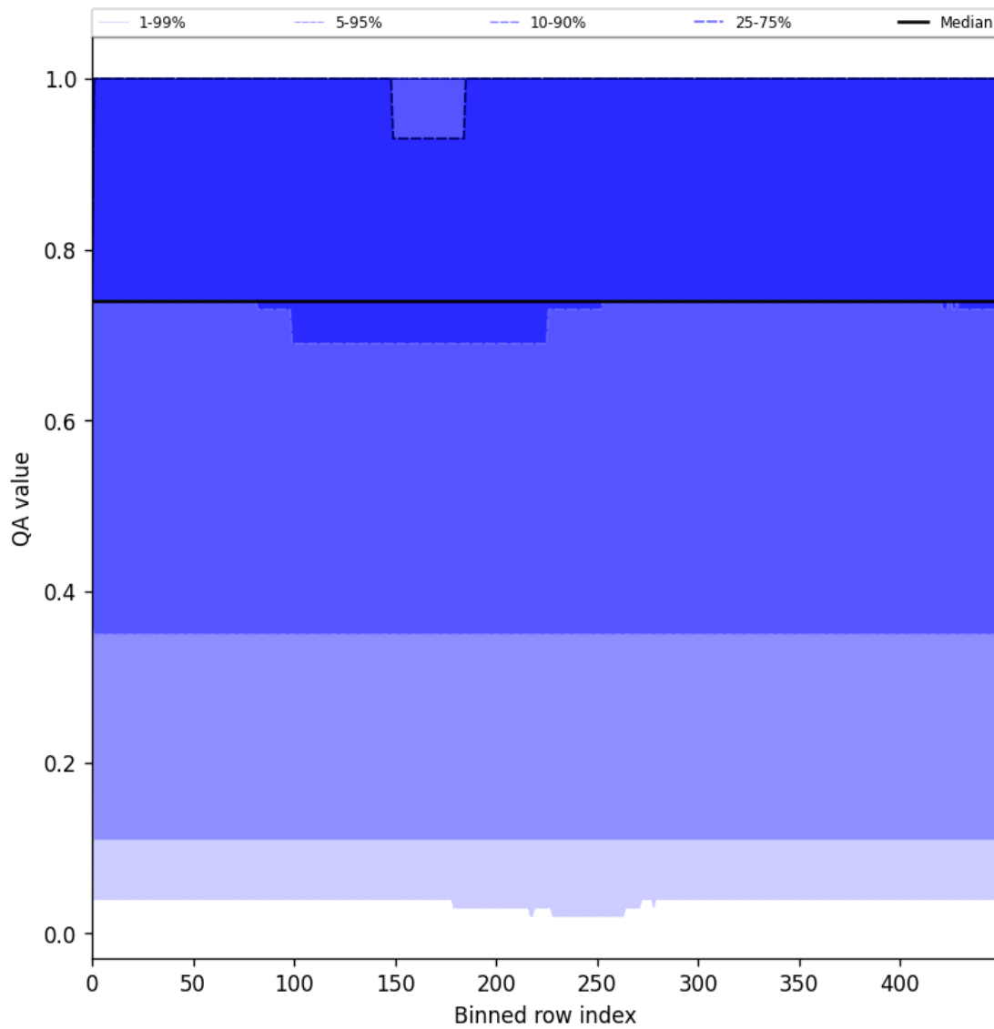
Figure 45: Along track statistics of “QA value” for 2025-06-03 to 2025-06-05
