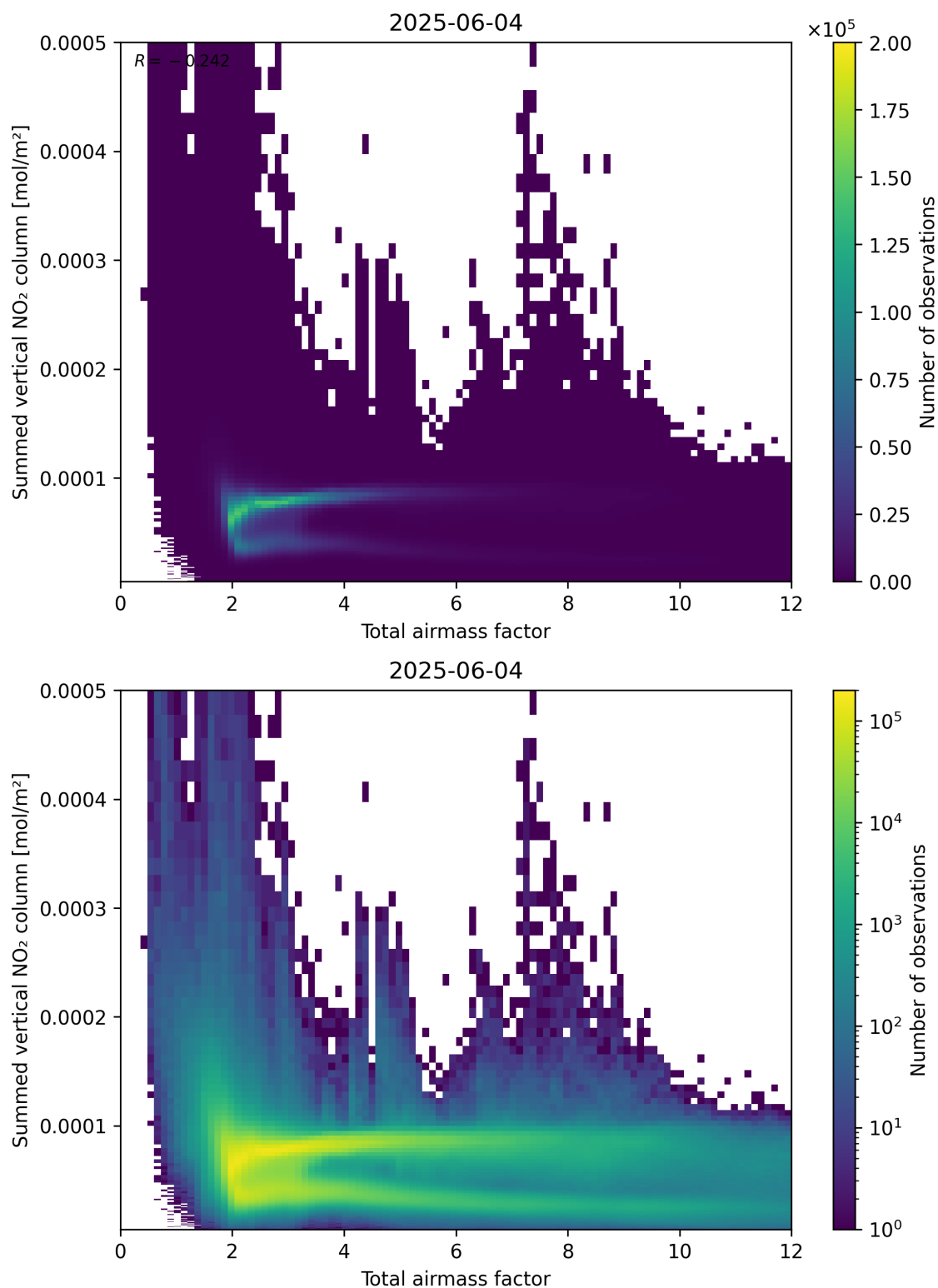
Figure 65: Scatter density plot of “Total airmass factor” against “Summed vertical NO 2 column” for 2025-06-03 to 2025-06-05.
