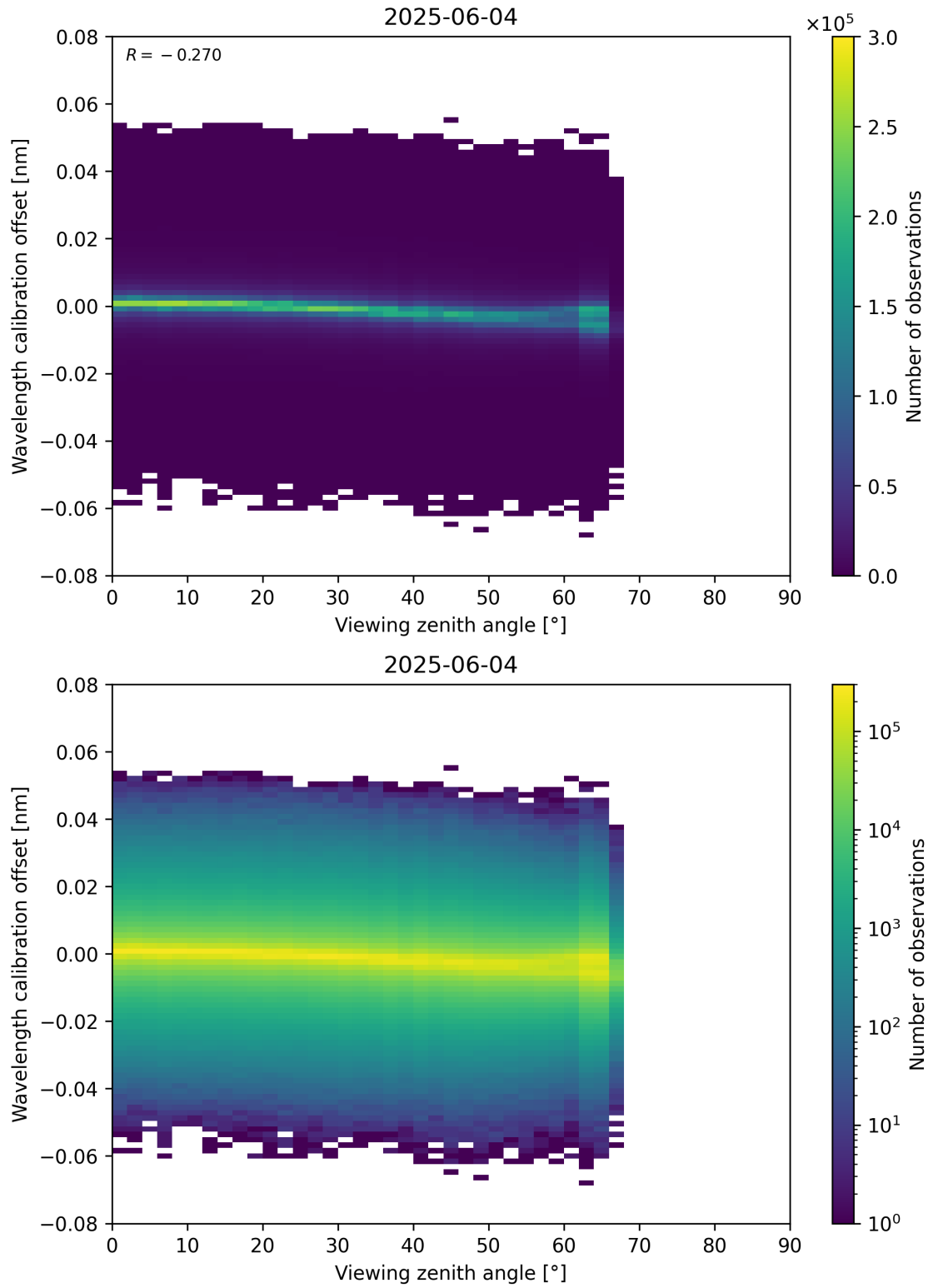
Figure 173: Scatter density plot of “Viewing zenith angle” against “Wavelength calibration offset” for 2025-06-03 to 2025-06-05.
