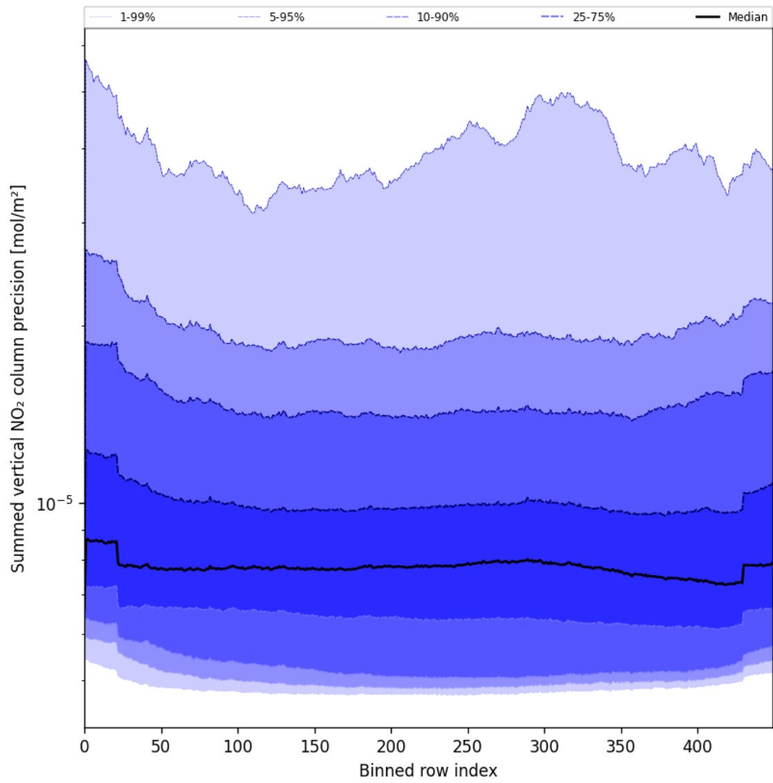
Figure 58: Along track statistics of “Summed vertical NO 2 column precision” for 2025-06-03 to 2025-06-05
