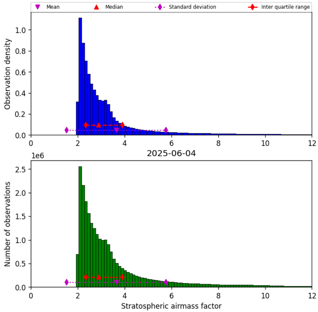
Figure 44: Histogram of “Stratospheric airmass factor” for 2025-06-03 to 2025-06-05
