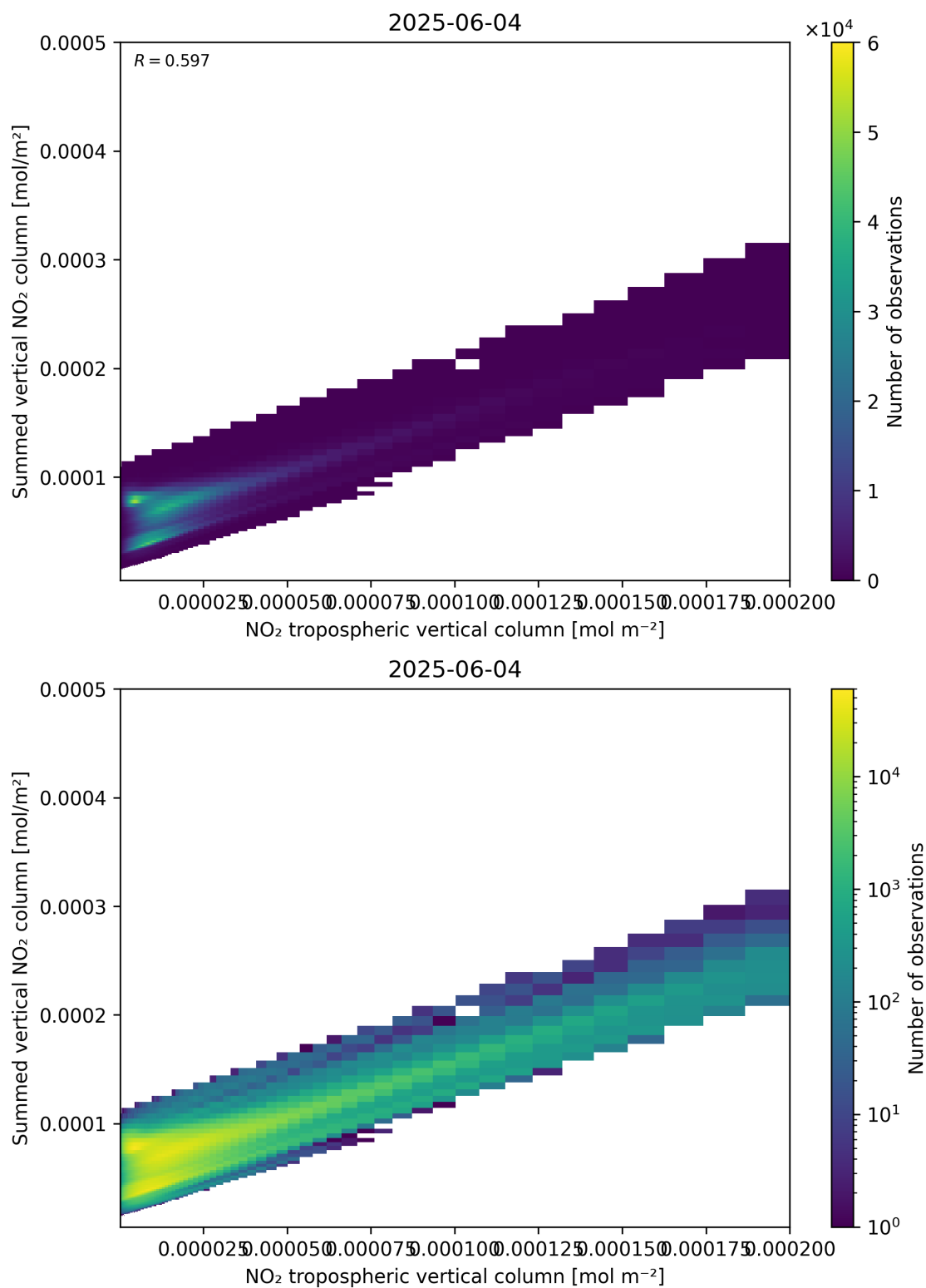
Figure 126: Scatter density plot of “NO 2 tropospheric vertical column” against “Summed vertical NO 2 column” for 2025-06-03 to 2025-06-05.
