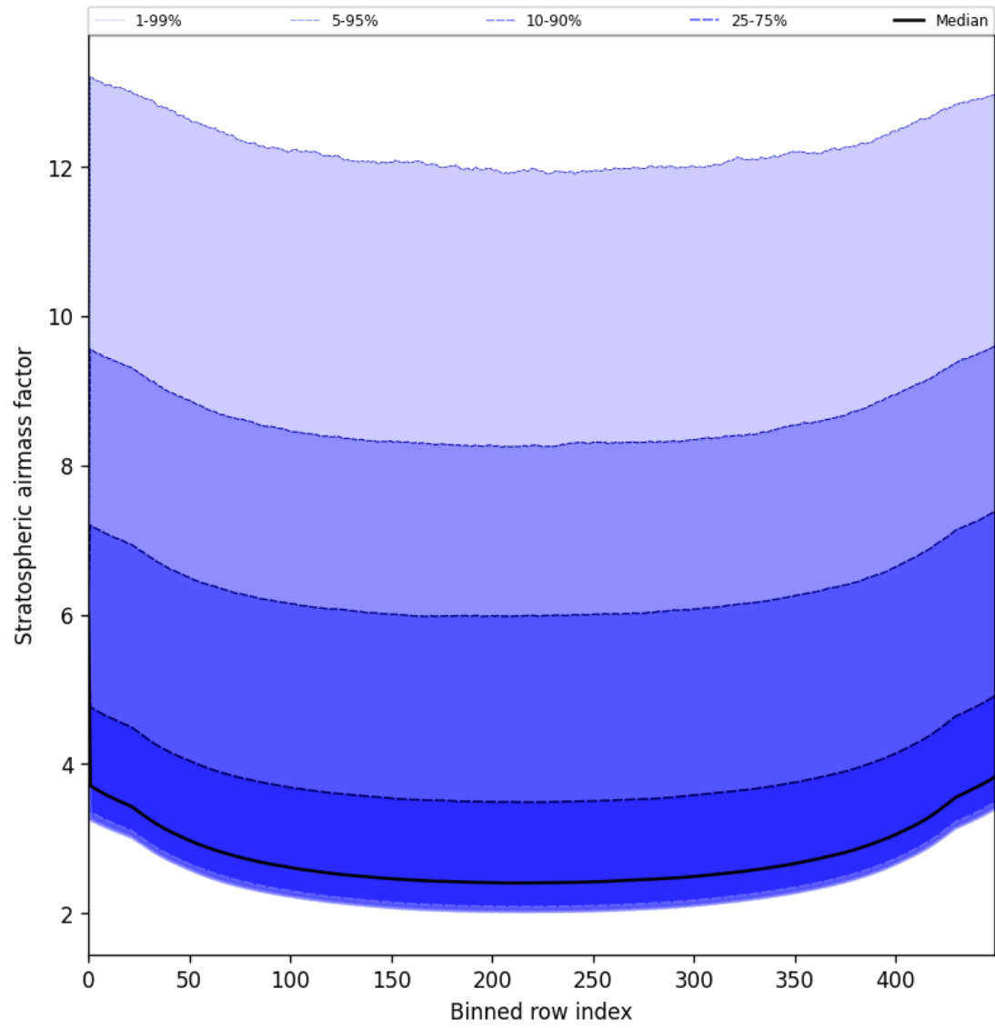
Figure 61: Along track statistics of “Stratospheric airmass factor” for 2025-06-03 to 2025-06-05
