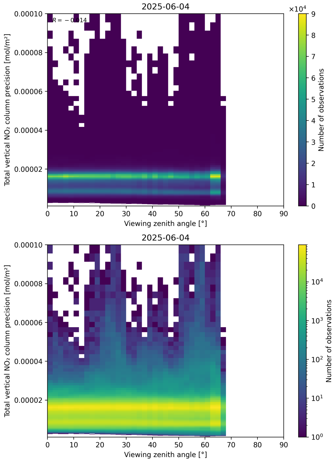
Figure 168: Scatter density plot of “Viewing zenith angle” against “Total vertical NO 2 column precision” for 2025-06-03 to 2025-06-05.
