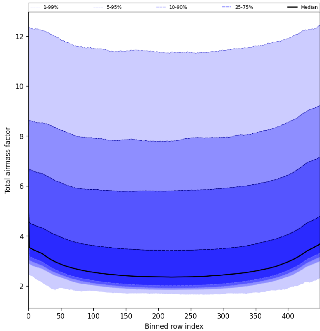
Figure 49: Along track statistics of “Total airmass factor” for 2025-06-03 to 2025-06-05
