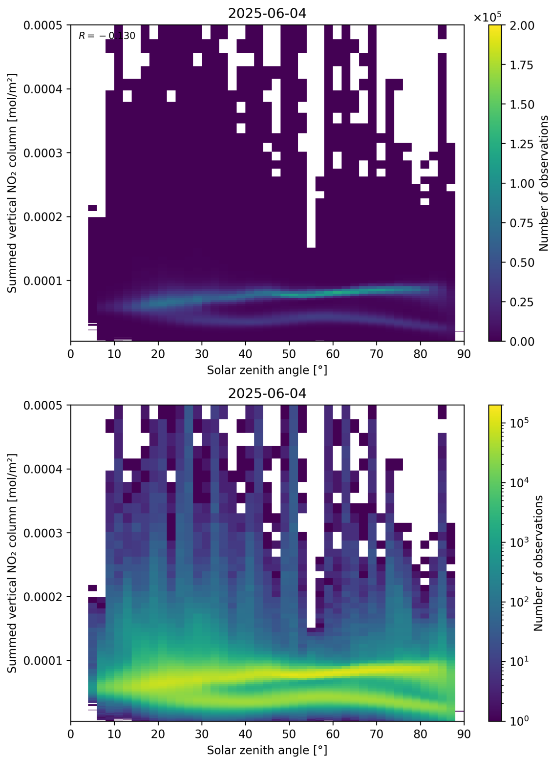
Figure 151: Scatter density plot of “Solar zenith angle” against “Summed vertical NO 2 column” for 2025-06-03 to 2025-06-05.
