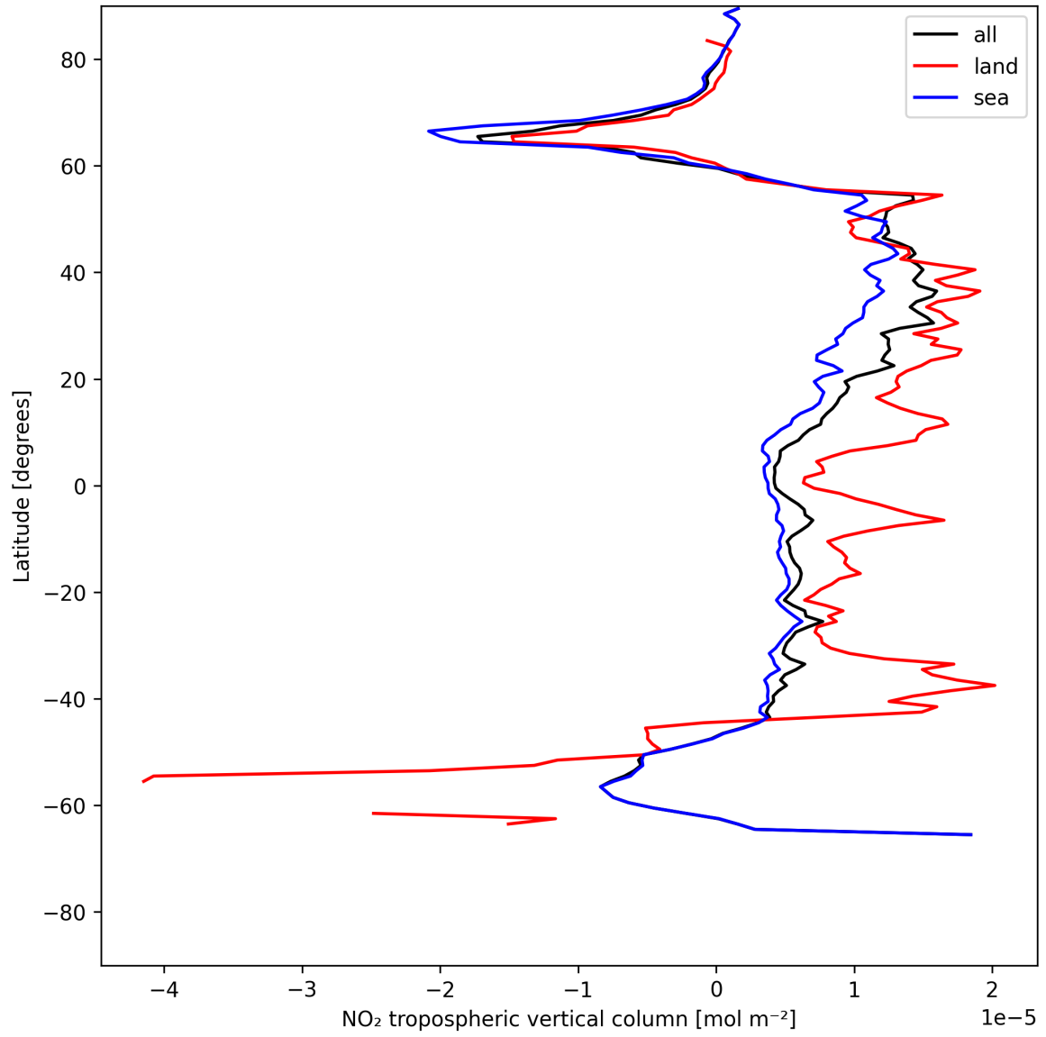
Figure 12: Zonal average of “NO 2 tropospheric vertical column” for 2025-06-03 to 2025-06-05.
