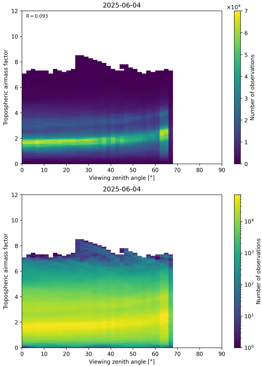
Figure 161: Scatter density plot of “Viewing zenith angle” against “Tropospheric airmass factor” for 2025-06-03 to 2025-06-05.
