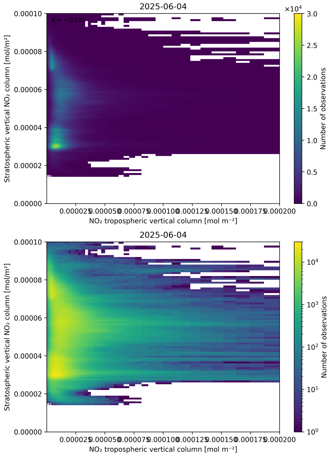
Figure 125: Scatter density plot of “NO 2 tropospheric vertical column” against “Stratospheric vertical NO 2 column” for 2025-06-03 to 2025-06-05.
