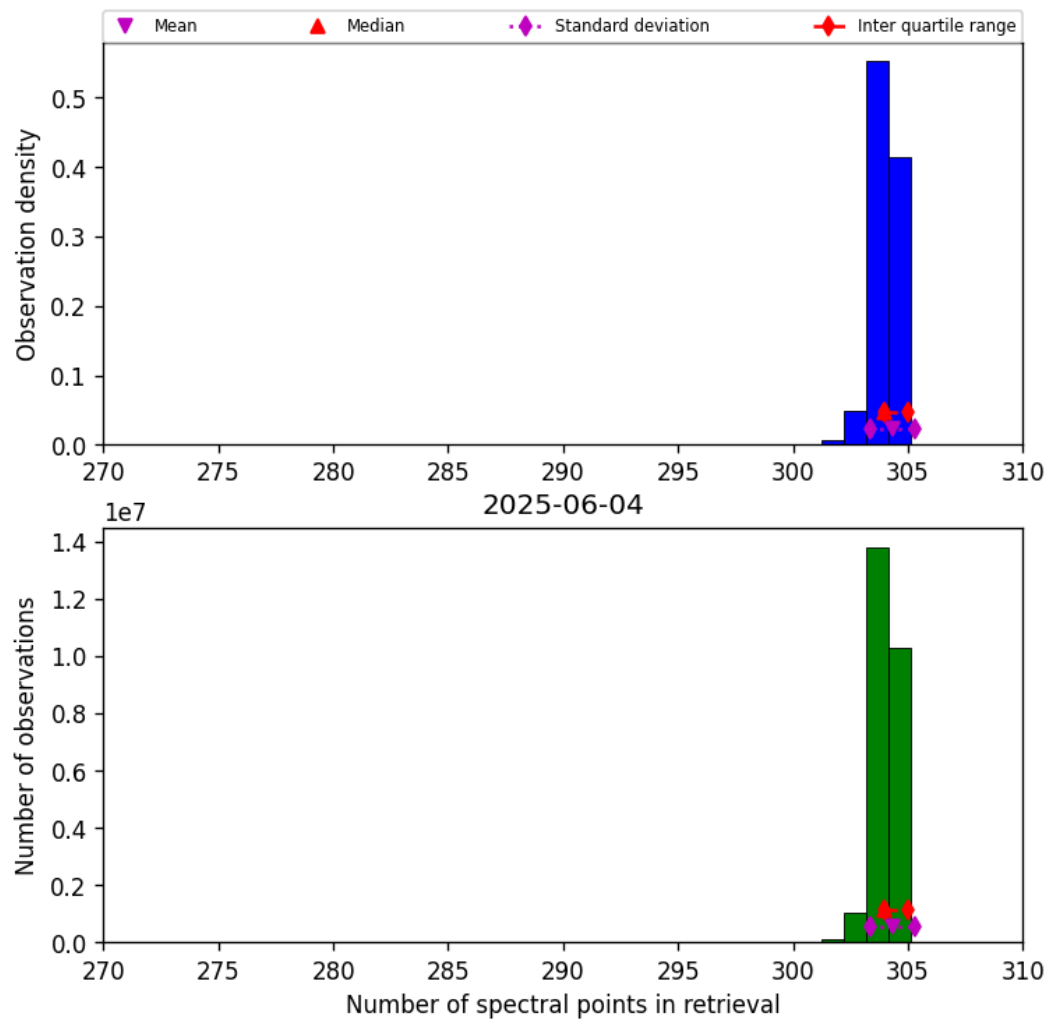
Figure 33: Histogram of “Number of spectral points in retrieval” for 2025-06-03 to 2025-06-05
