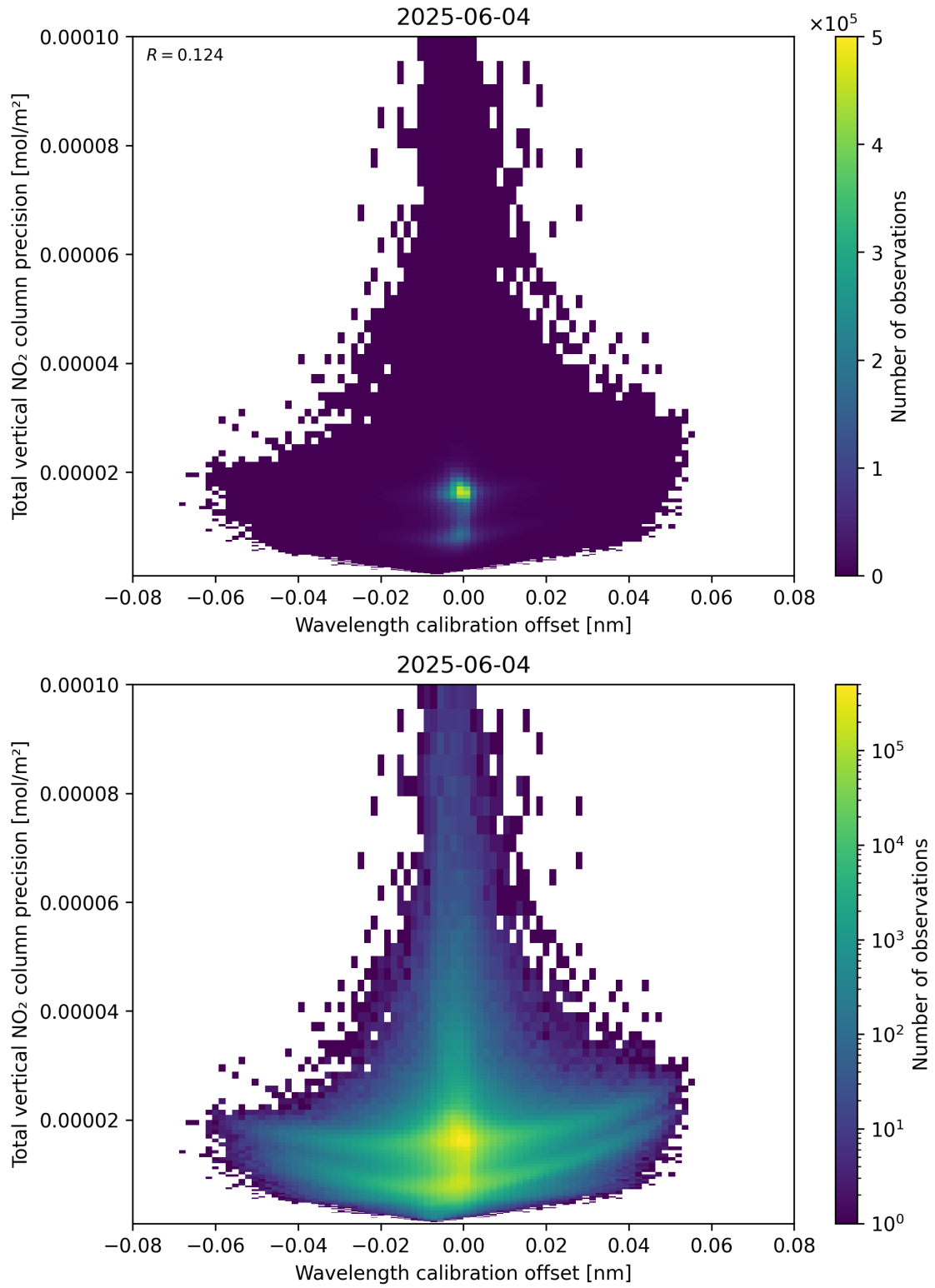
Figure 180: Scatter density plot of “Wavelength calibration offset” against “Total vertical NO 2 column precision” for 2025-06-03 to 2025-06-05.
