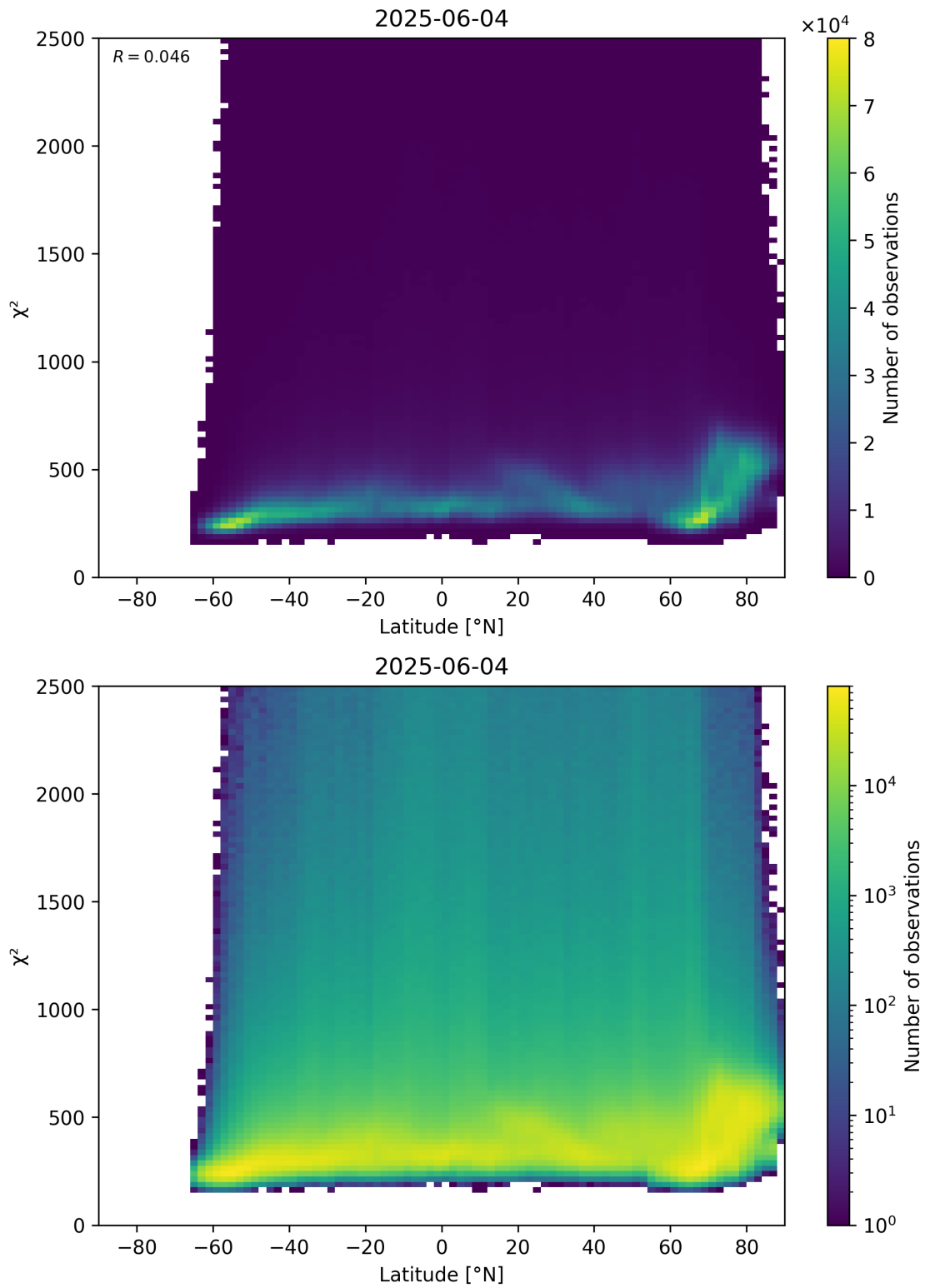
Figure 86: Scatter density plot of “Latitude” against “ \chi^2 ” for 2025-06-03 to 2025-06-05.
