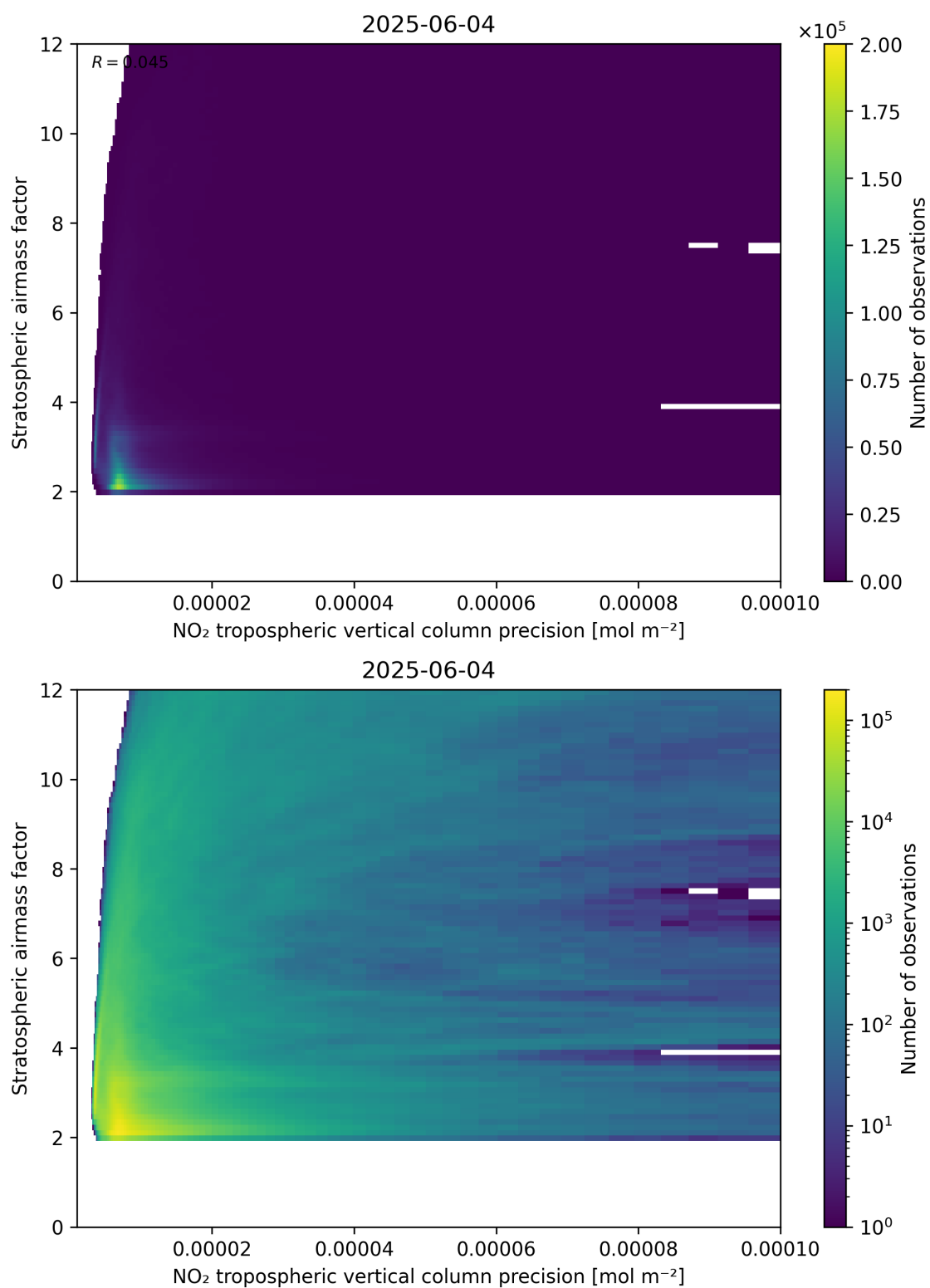
Figure 131: Scatter density plot of “NO 2 tropospheric vertical column precision” against “Stratospheric airmass factor” for 2025-06-03 to 2025-06-05.
