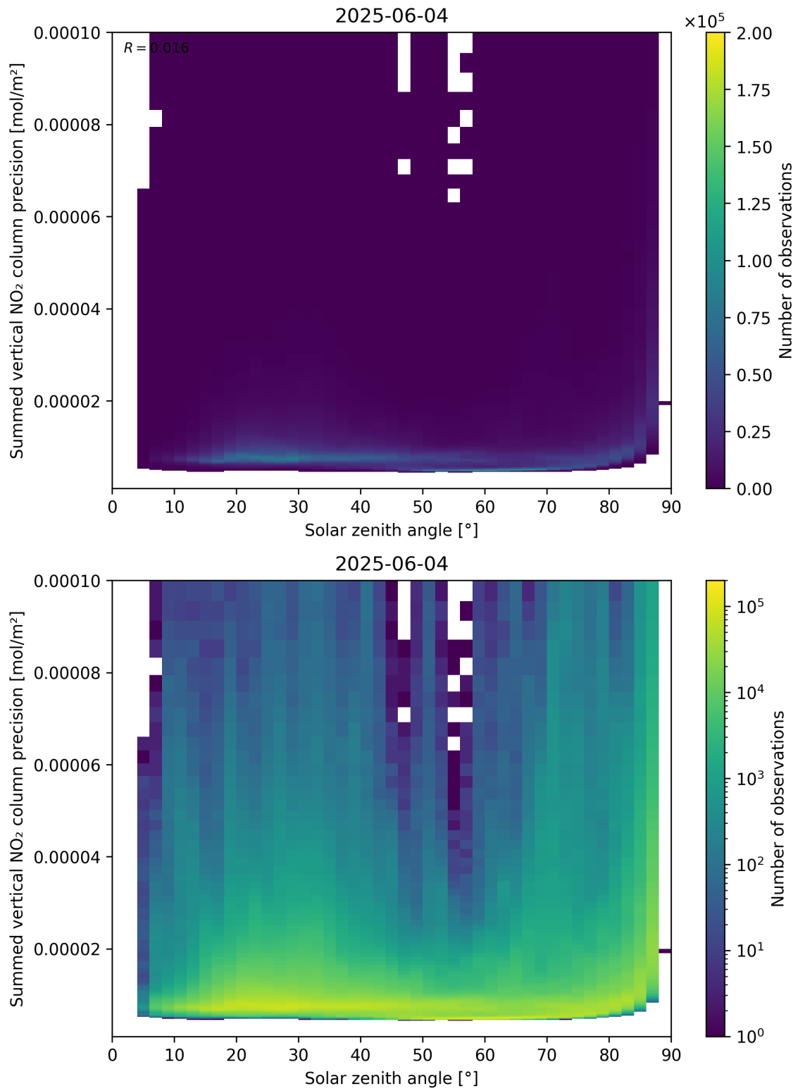
Figure 152: Scatter density plot of “Solar zenith angle” against “Summed vertical NO 2 column precision” for 2025-06-03 to 2025-06-05.
