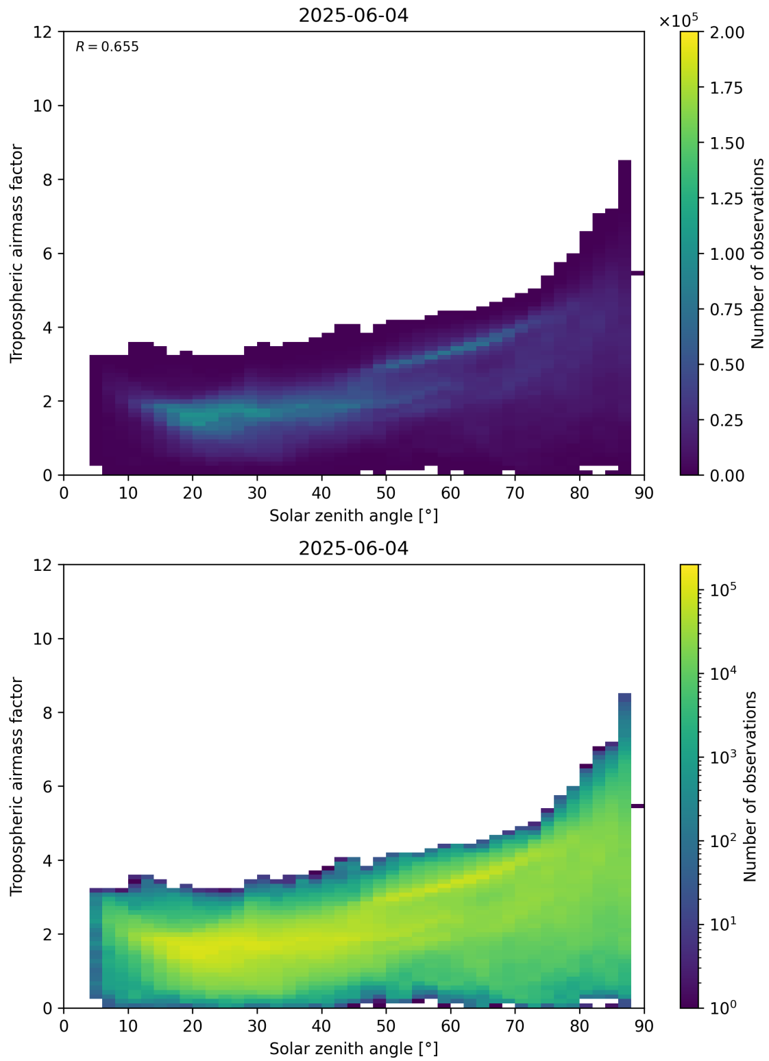
Figure 147: Scatter density plot of “Solar zenith angle” against “Tropospheric airmass factor” for 2025-06-03 to 2025-06-05.
