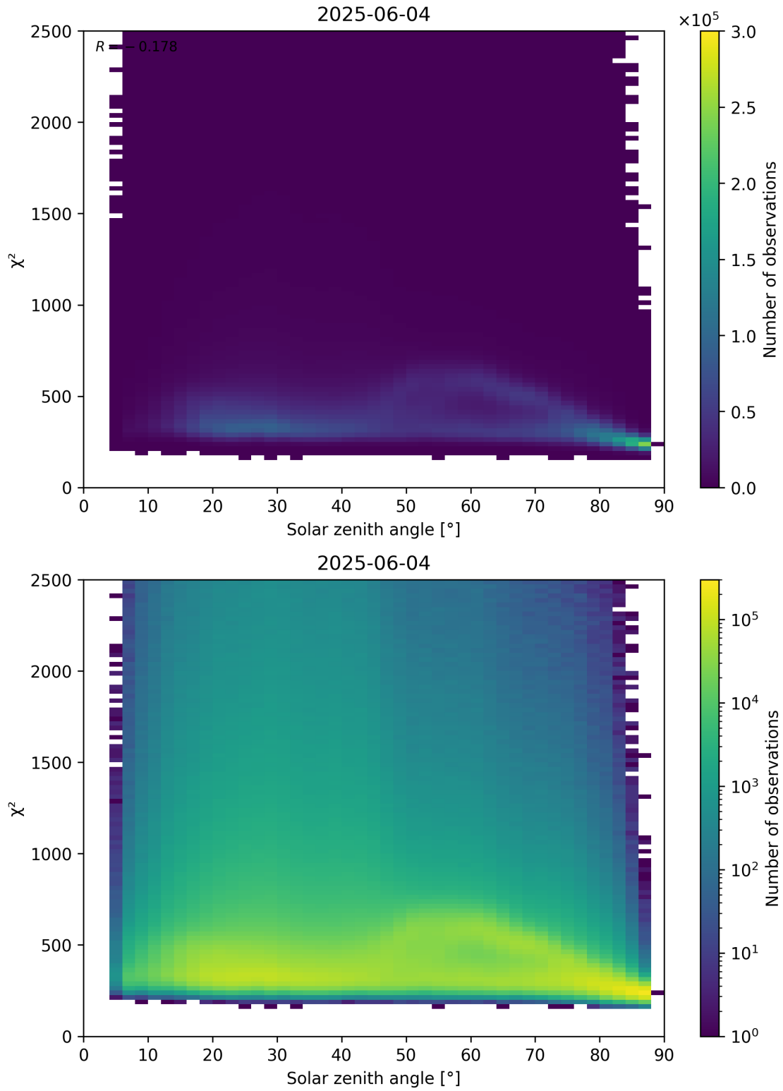
Figure 148: Scatter density plot of “Solar zenith angle” against “ \chi^2 ” for 2025-06-03 to 2025-06-05.
