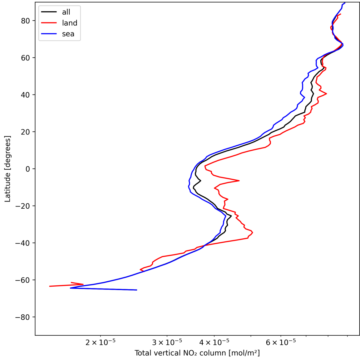
Figure 21: Zonal average of “Total vertical NO 2 column” for 2025-06-03 to 2025-06-05.
