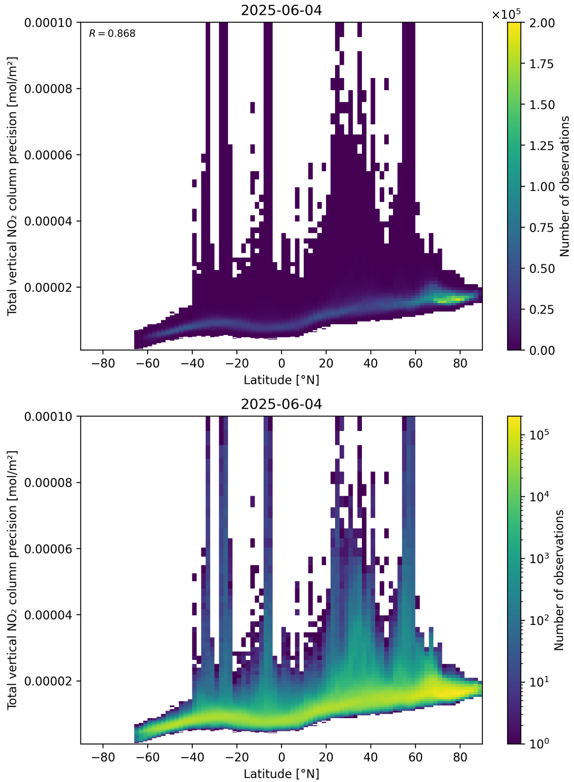
Figure 91: Scatter density plot of “Latitude” against “Total vertical NO 2 column precision” for 2025-06-03 to 2025-06-05.
