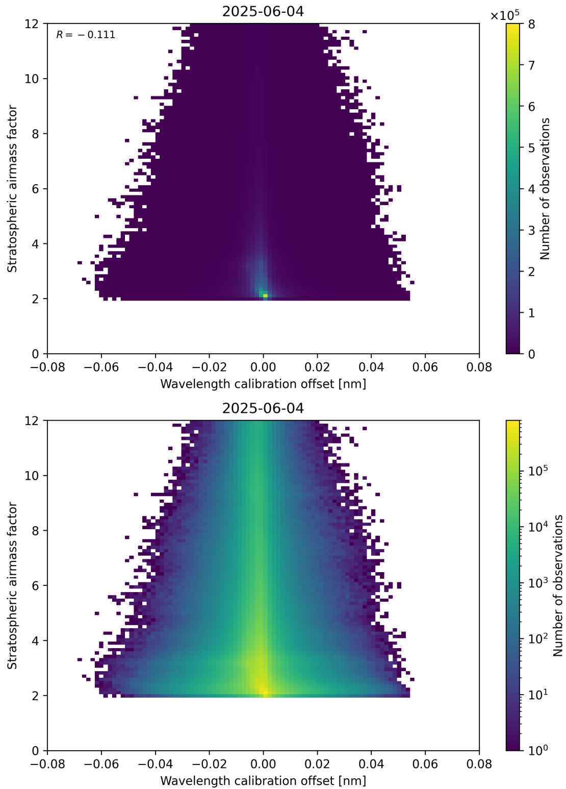
Figure 174: Scatter density plot of “Wavelength calibration offset” against “Stratospheric airmass factor” for 2025-06-03 to 2025-06-05.
