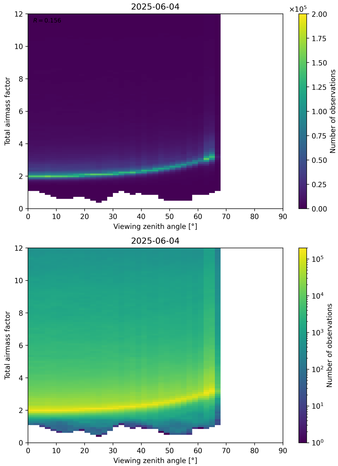
Figure 160: Scatter density plot of “Viewing zenith angle” against “Total airmass factor” for 2025-06-03 to 2025-06-05.
