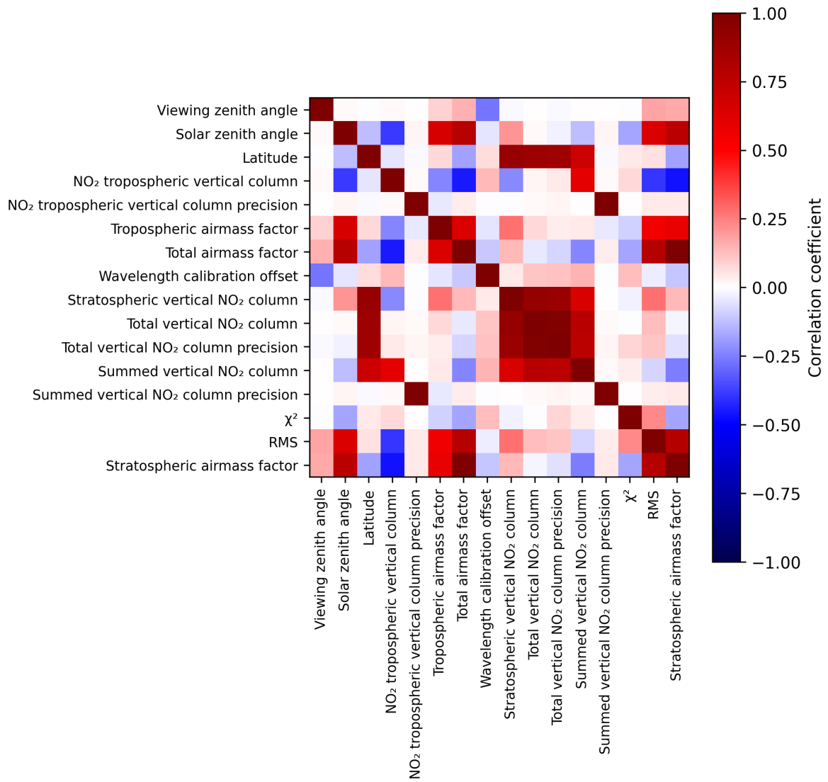
Figure 2: Map of correlation matrix for 2025-06-03 to 2025-06-05.
