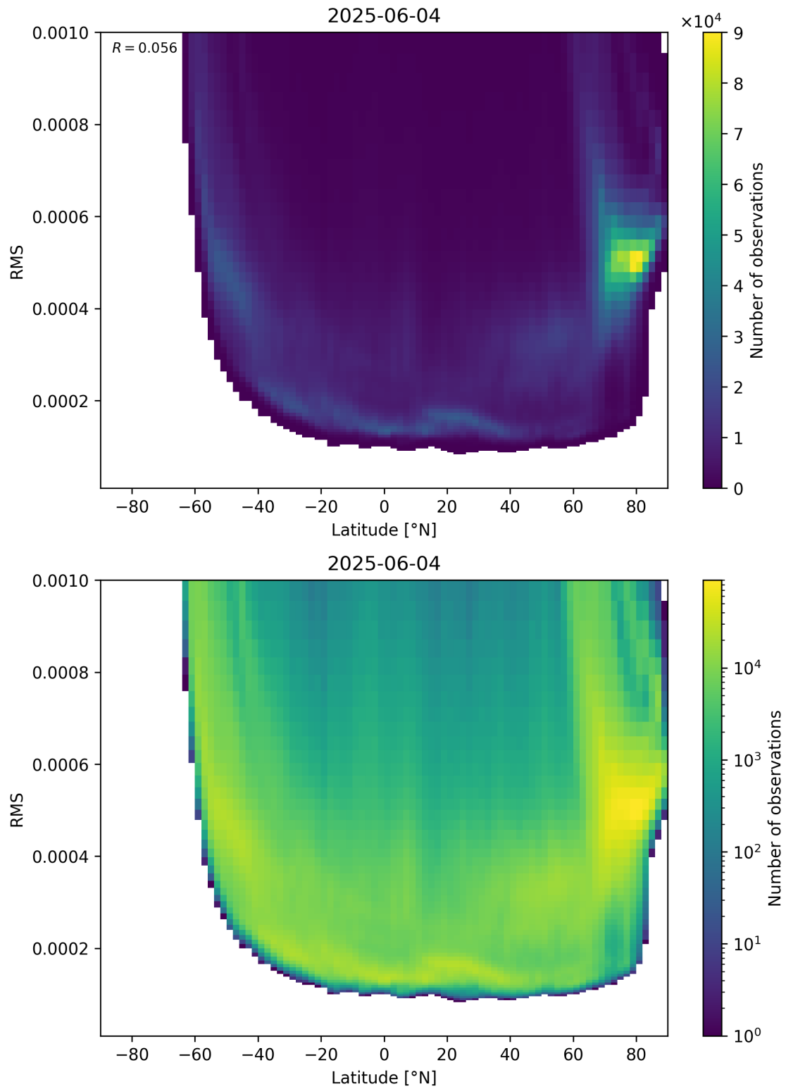
Figure 94: Scatter density plot of “Latitude” against “RMS” for 2025-06-03 to 2025-06-05.
