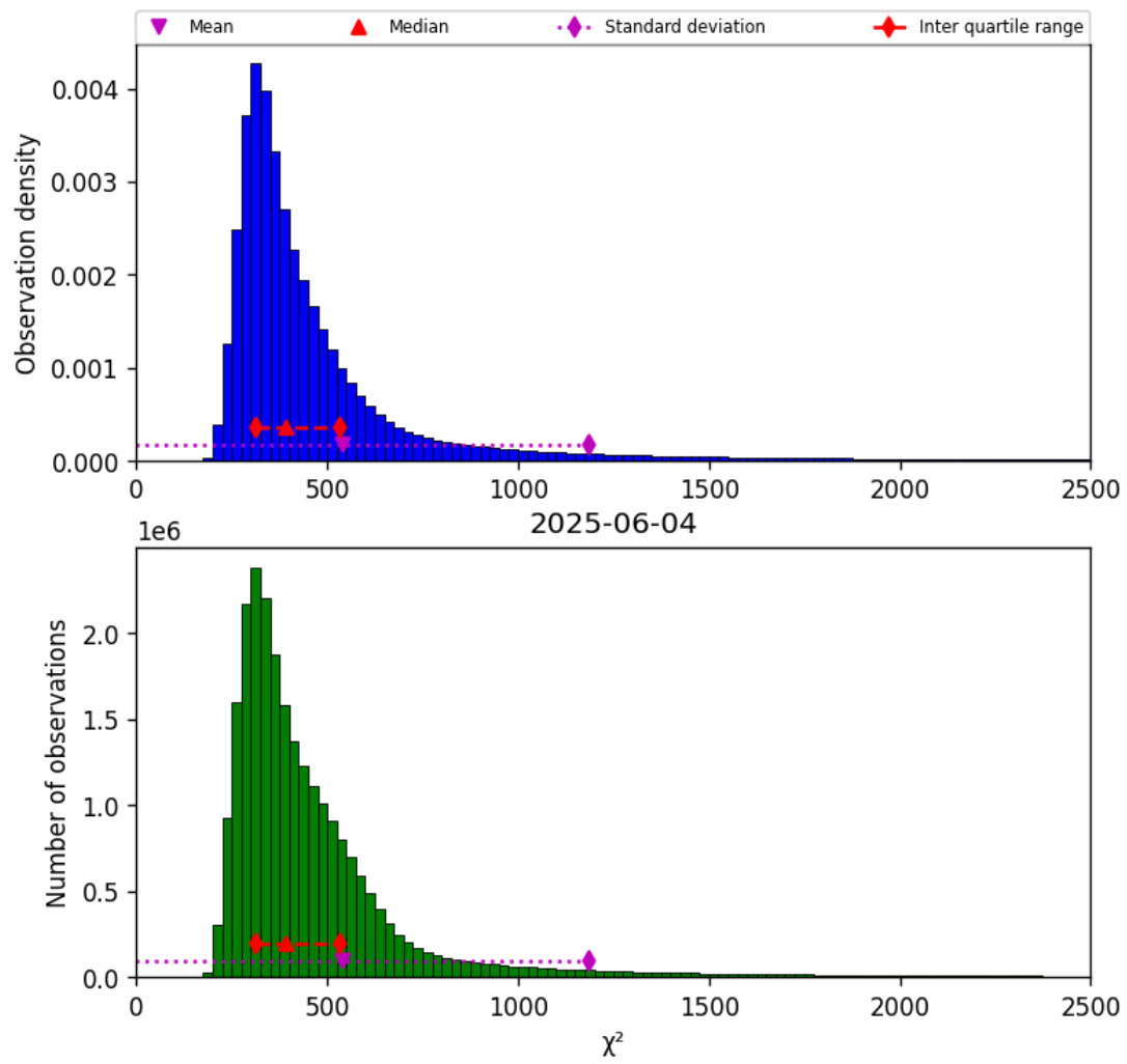
Figure 42: Histogram of “ \chi^2 ” for 2025-06-03 to 2025-06-05
