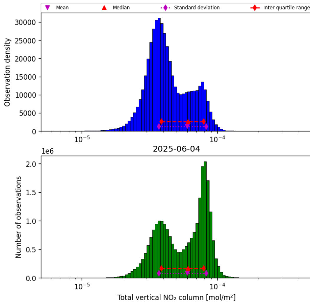
Figure 38: Histogram of “Total vertical NO 2 column” for 2025-06-03 to 2025-06-05
