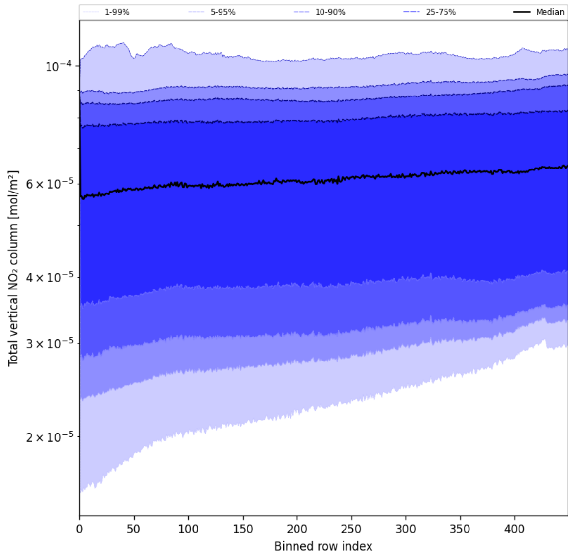
Figure 55: Along track statistics of “Total vertical NO 2 column” for 2025-06-03 to 2025-06-05
