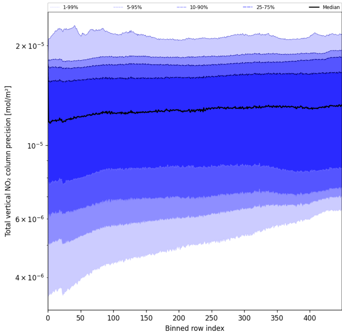
Figure 56: Along track statistics of "Total vertical NO 2 column precision" for 2025-06-03 to 2025-06-05
