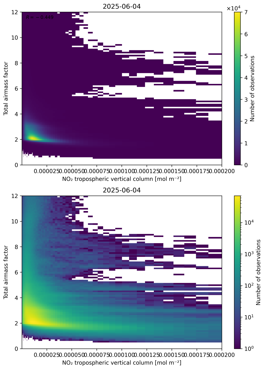
Figure 122: Scatter density plot of “NO 2 tropospheric vertical column” against “Total air mass factor” for 2025-06-03 to 2025-06-05.
