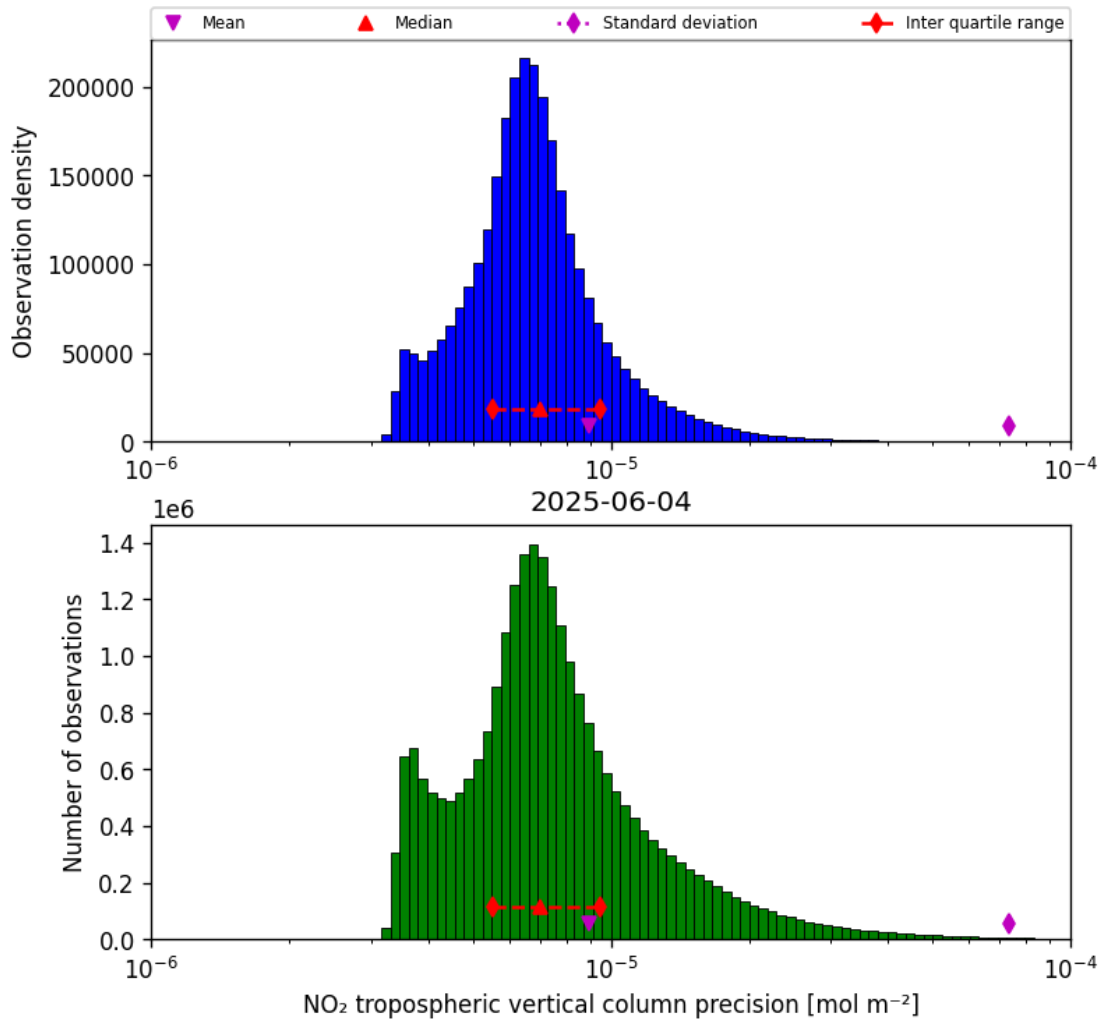
Figure 30: Histogram of “NO 2 tropospheric vertical column precision” for 2025-06-03 to 2025-06-05
