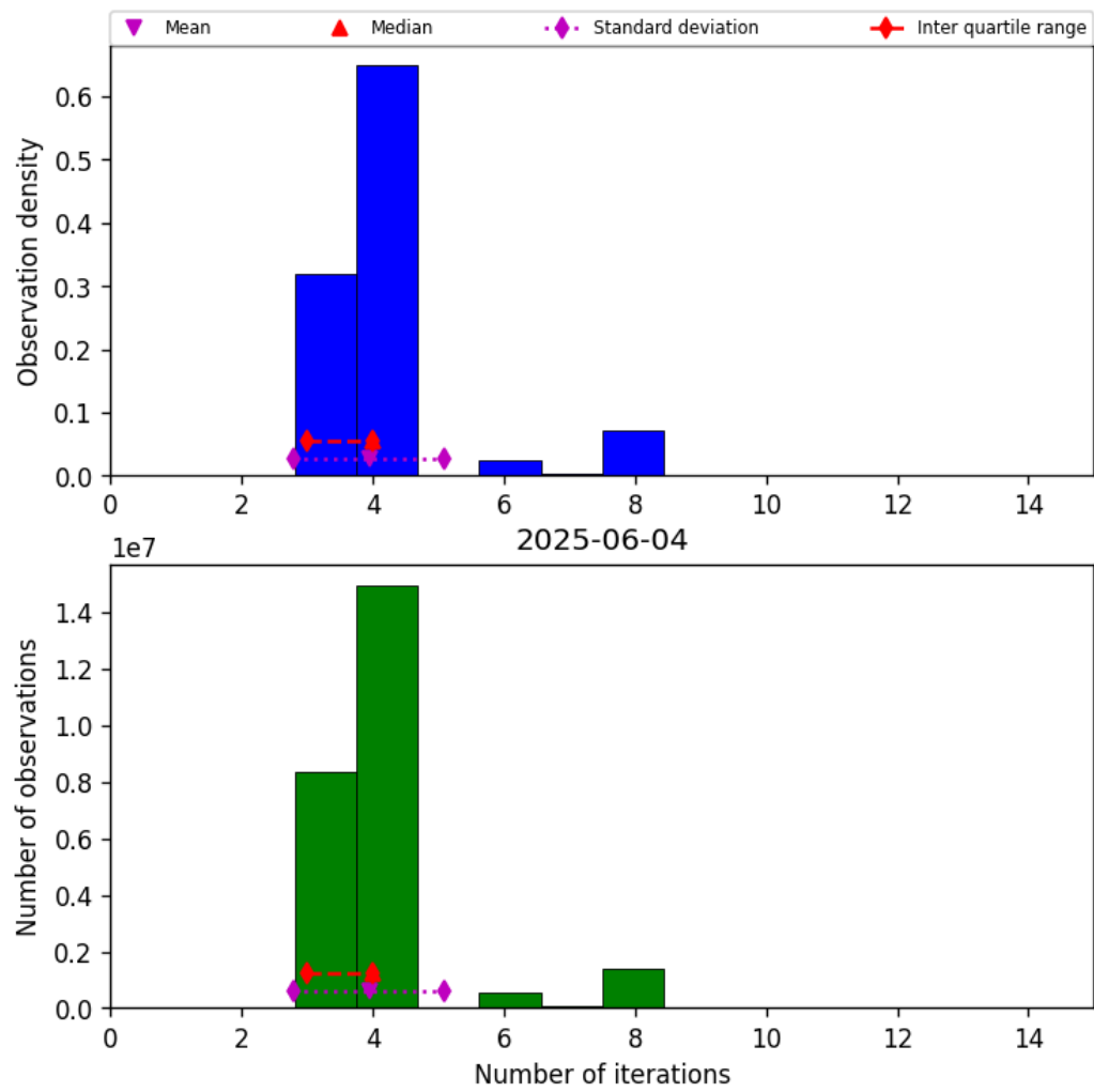
Figure 34: Histogram of “Number of iterations” for 2025-06-03 to 2025-06-05
