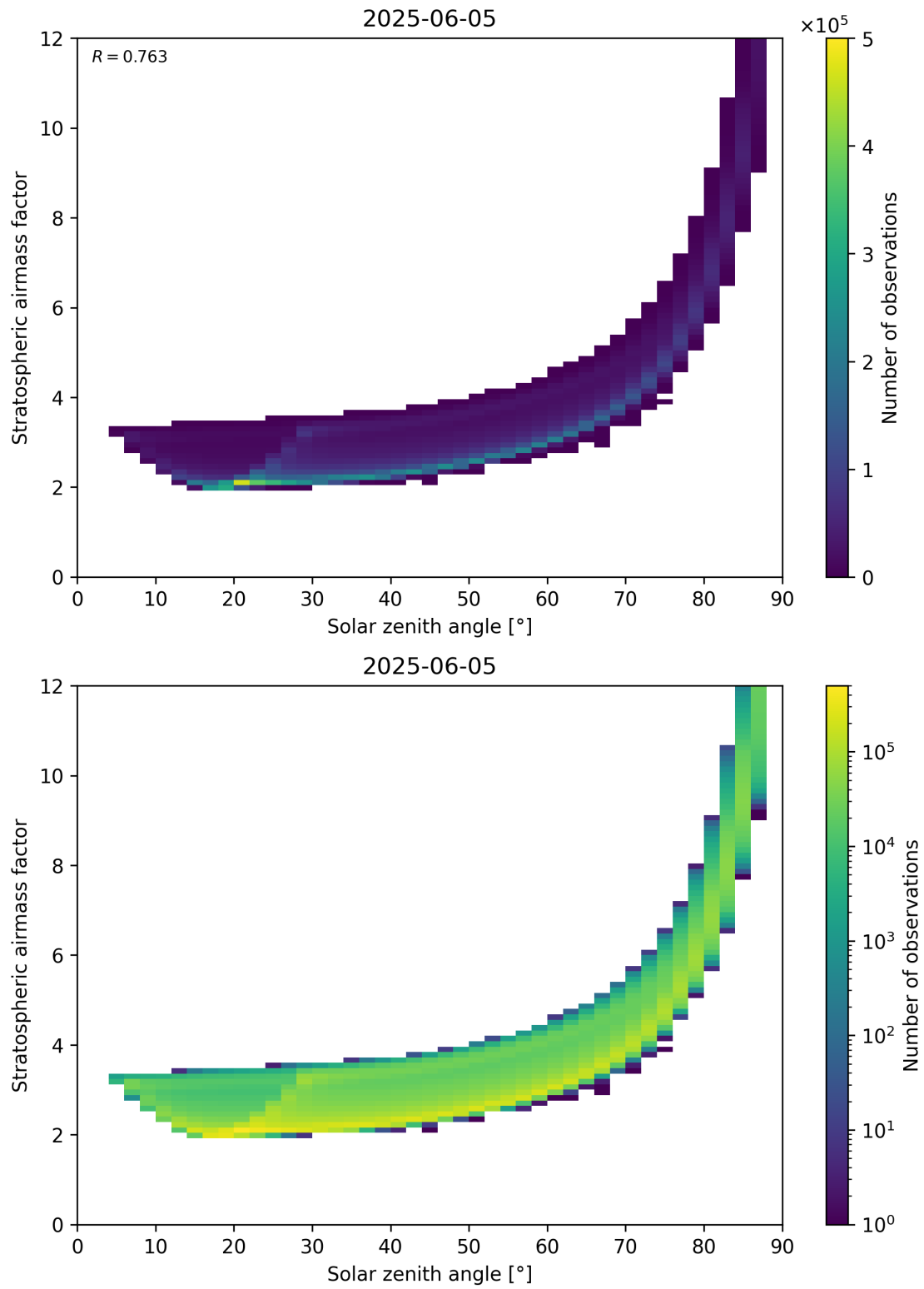
Figure 145: Scatter density plot of “Solar zenith angle” against “Stratospheric airmass factor” for 2025-06-04 to 2025-06-06.
