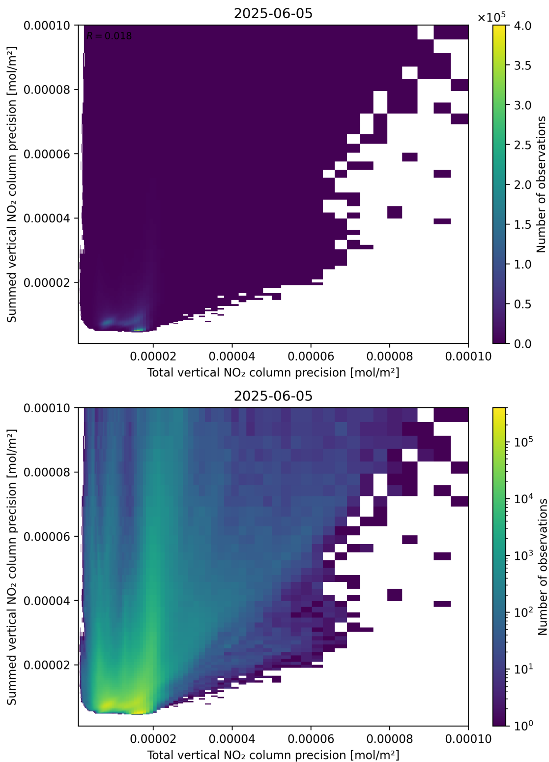
Figure 118: Scatter density plot of “Total vertical NO 2 column precision” against “Summed vertical NO 2 column precision” for 2025-06-04 to 2025-06-06.
