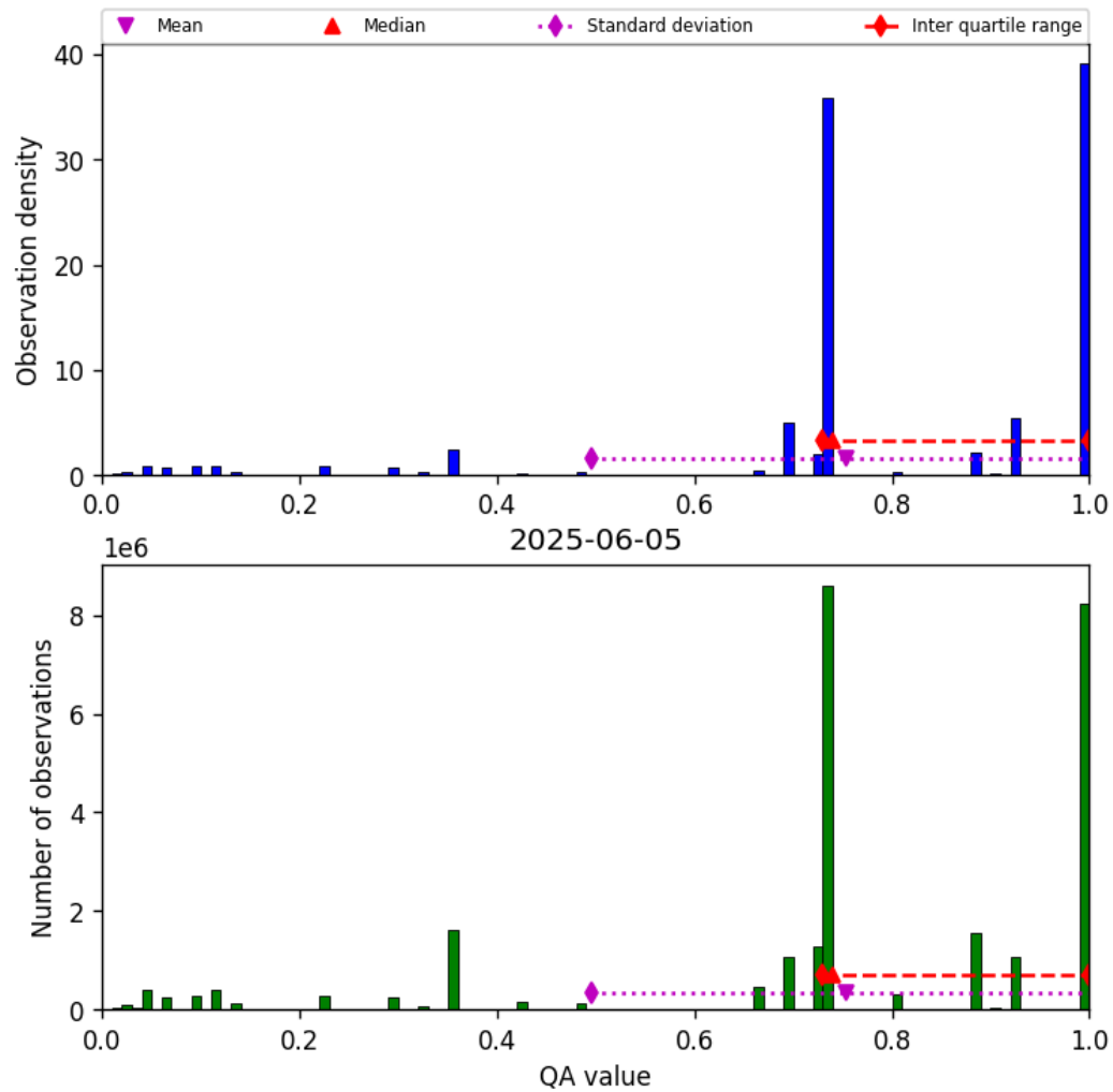
Figure 28: Histogram of “QA value” for 2025-06-04 to 2025-06-06
