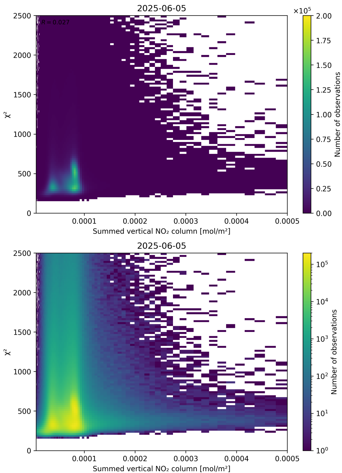
Figure 104: Scatter density plot of “Summed vertical NO 2 column” against “ \chi^2 ” for 2025-06-04 to 2025-06-06.
