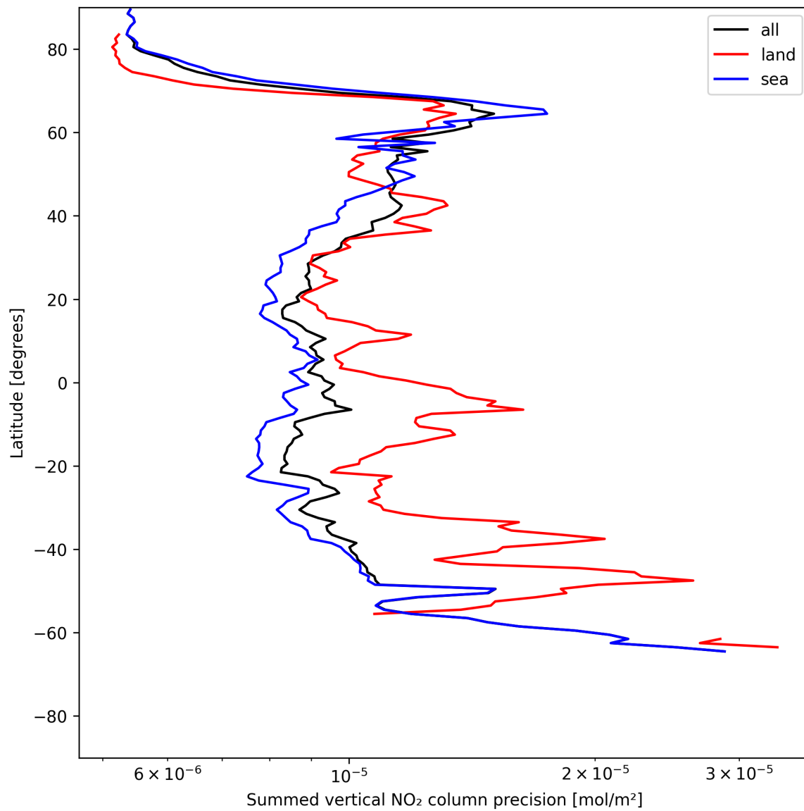
Figure 24: Zonal average of “Summed vertical NO 2 column precision” for 2025-06-04 to 2025-06-06.
