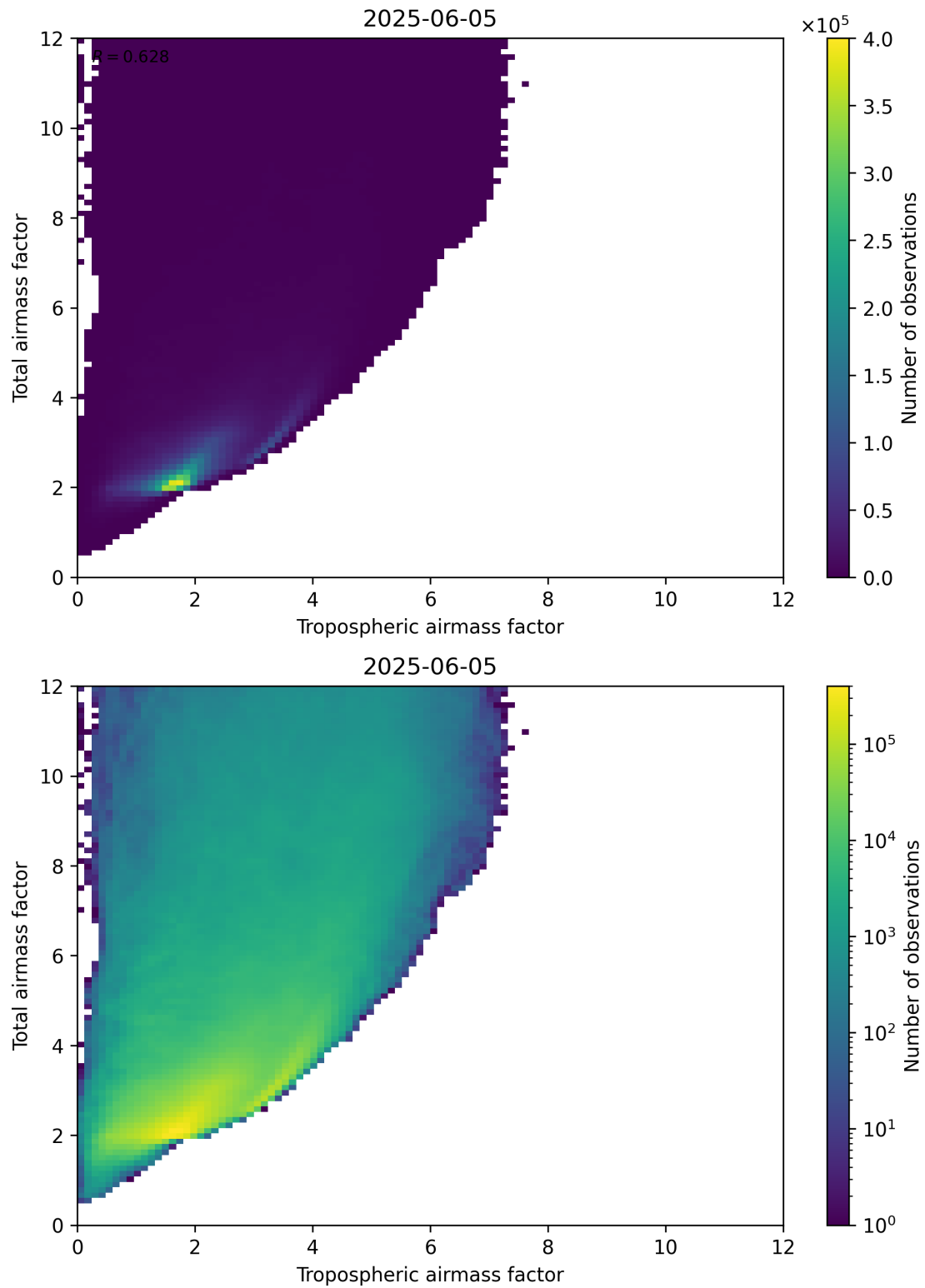
Figure 72: Scatter density plot of “Tropospheric airmass factor” against “Total airmass factor” for 2025-06-04 to 2025-06-06.
