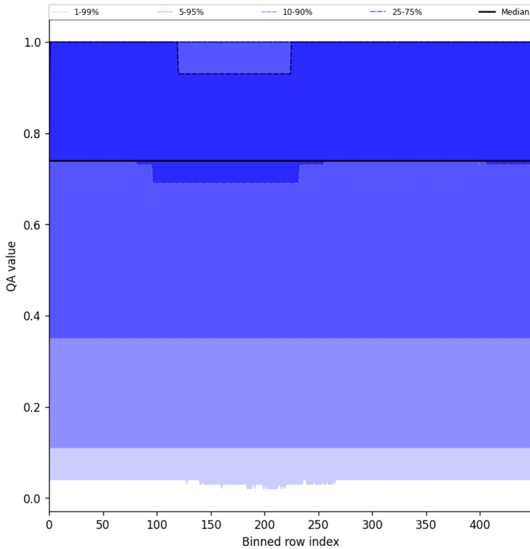
Figure 45: Along track statistics of “QA value” for 2025-06-04 to 2025-06-06
