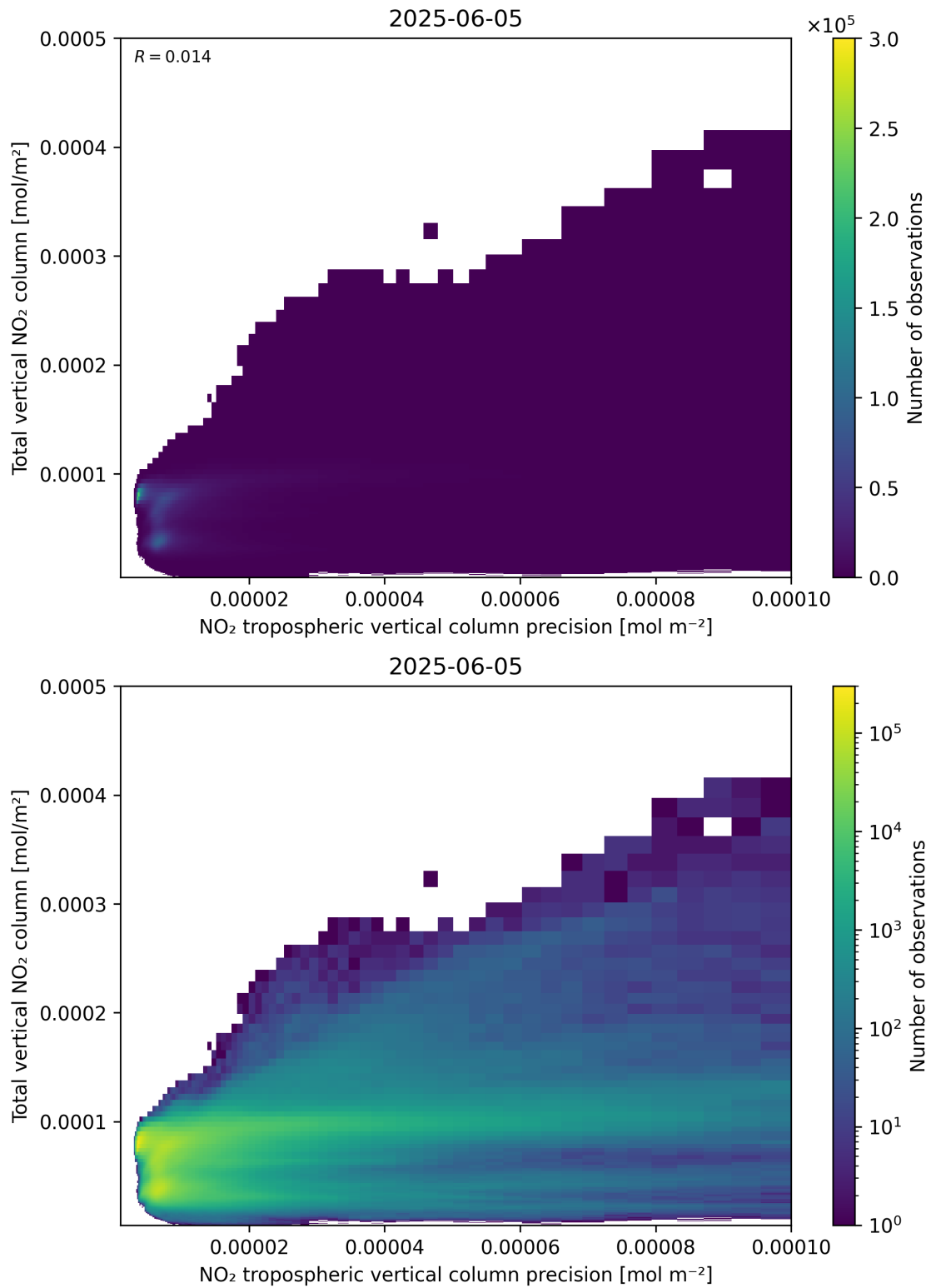
Figure 138: Scatter density plot of “NO 2 tropospheric vertical column precision” against “Total vertical NO 2 column” for 2025-06-04 to 2025-06-06.
