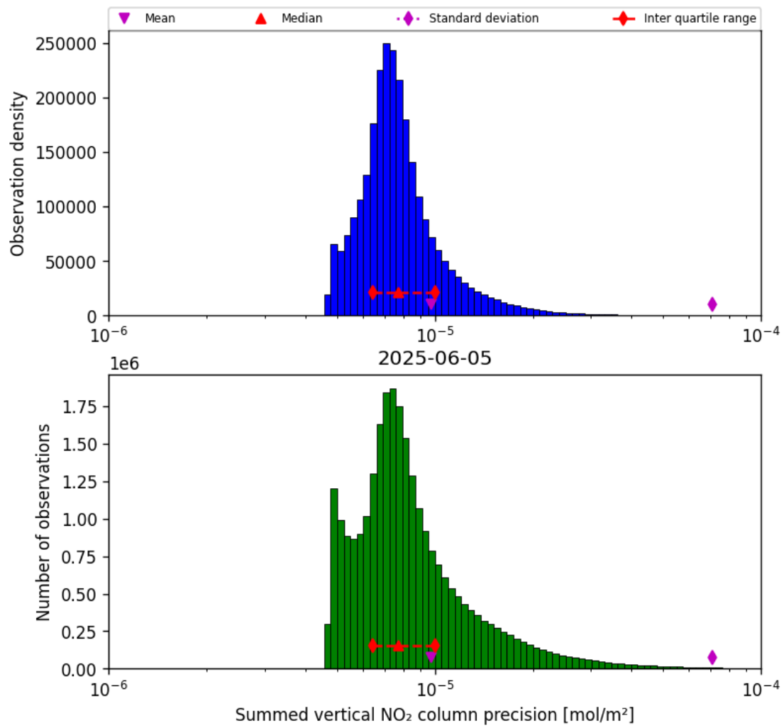
Figure 41: Histogram of “Summed vertical NO 2 column precision” for 2025-06-04 to 2025-06-06
