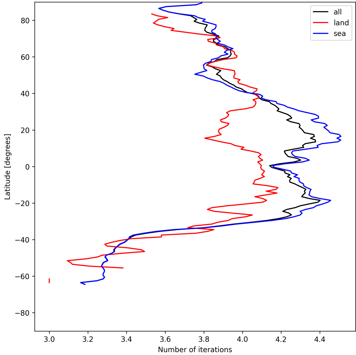
Figure 17: Zonal average of “Number of iterations” for 2025-06-04 to 2025-06-06.
