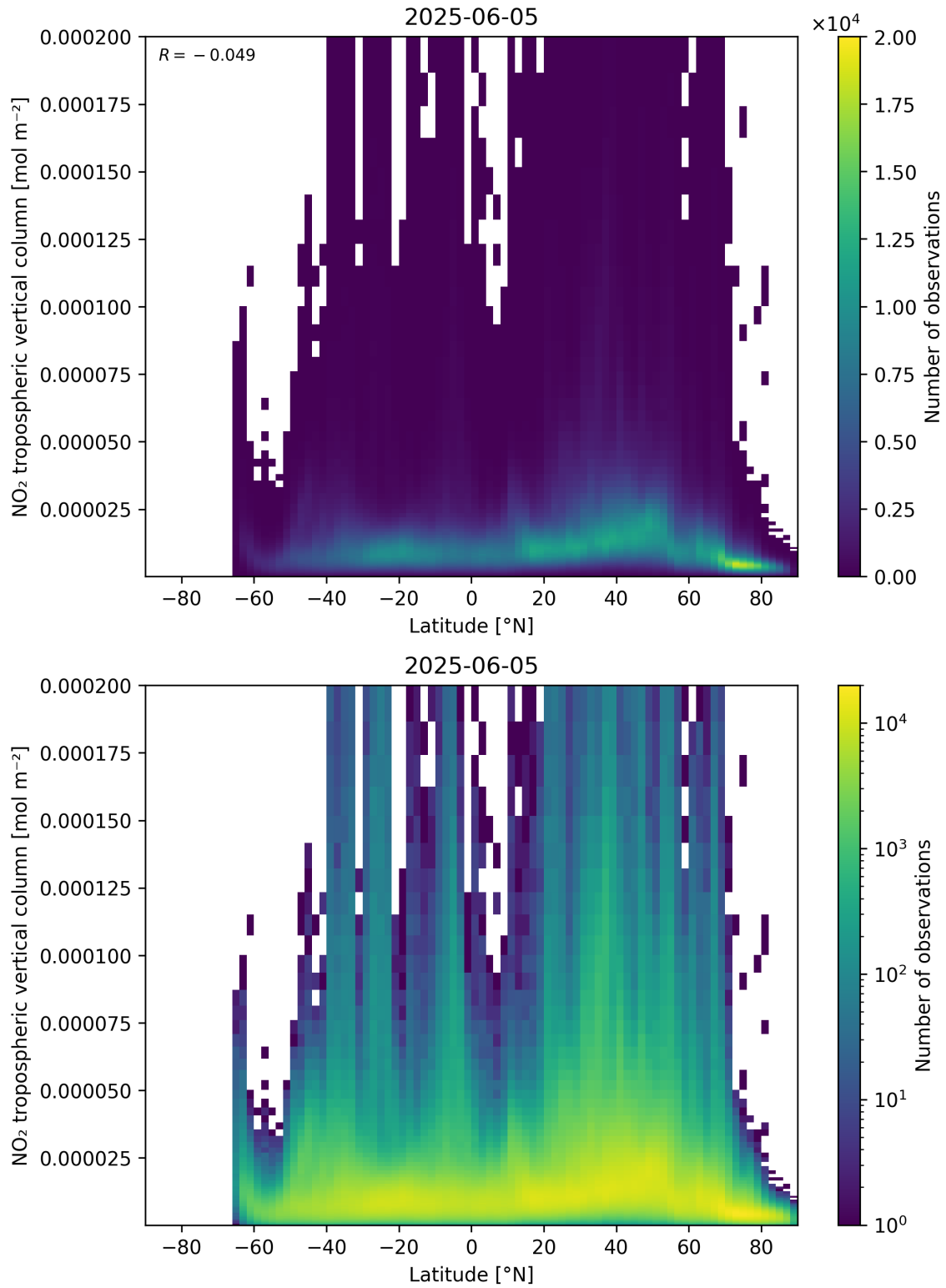
Figure 92: Scatter density plot of “Latitude” against “NO 2 tropospheric vertical column” for 2025-06-04 to 2025-06-06.
