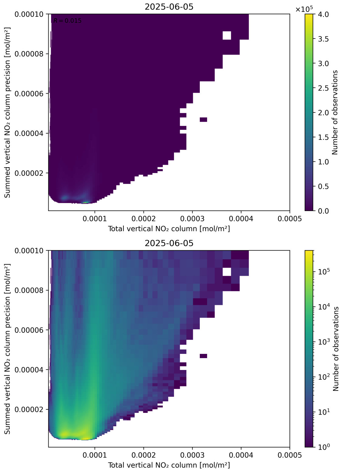
Figure 113: Scatter density plot of “Total vertical NO 2 column” against “Summed vertical NO 2 column precision” for 2025-06-04 to 2025-06-06.
