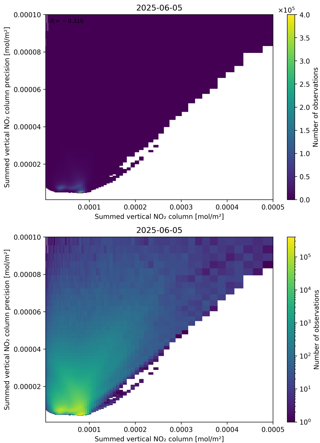
Figure 105: Scatter density plot of “Summed vertical NO 2 column” against “Summed vertical NO 2 column precision” for 2025-06-04 to 2025-06-06.
