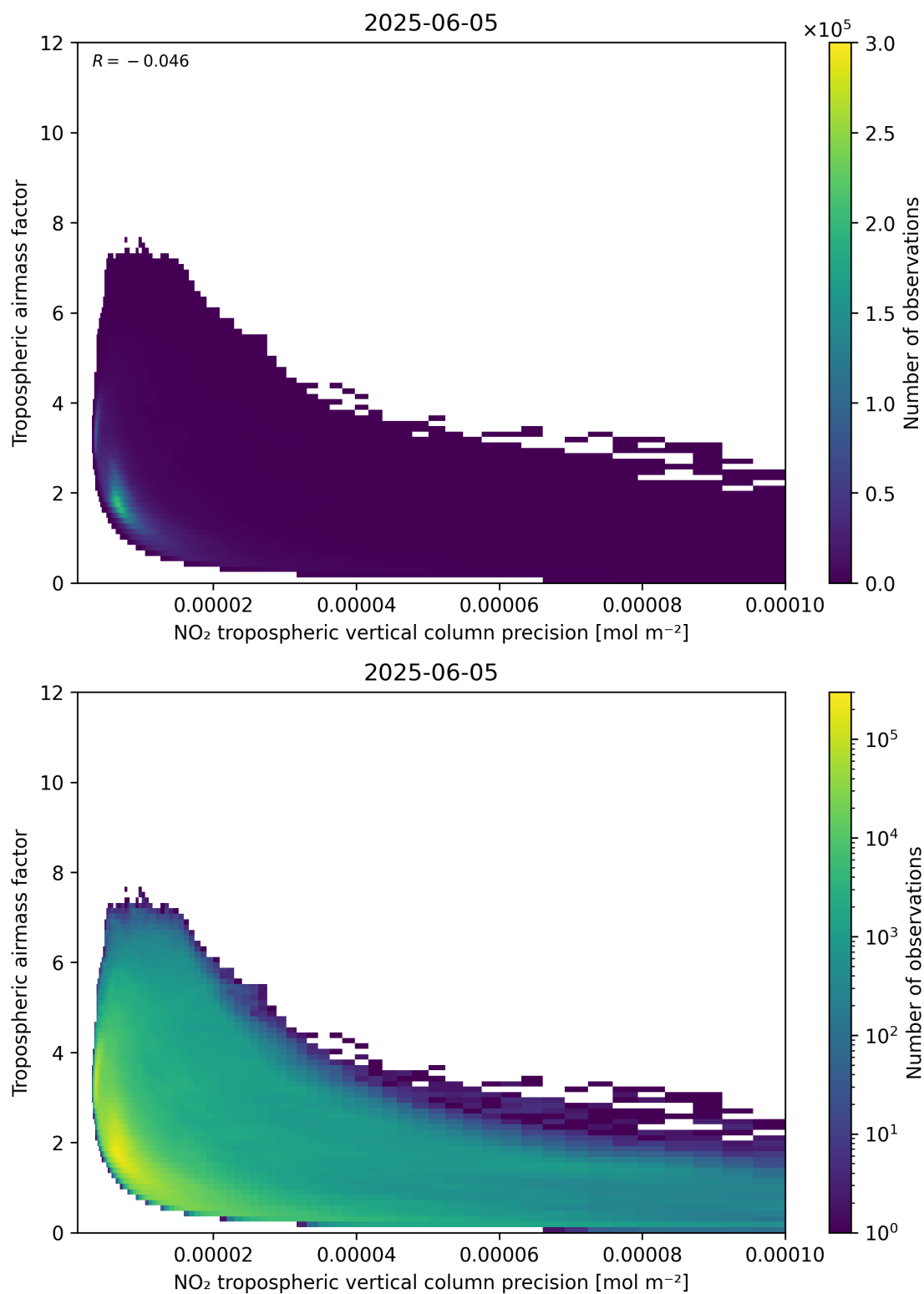
Figure 133: Scatter density plot of “NO 2 tropospheric vertical column precision” against “Tropospheric air mass factor” for 2025-06-04 to 2025-06-06.
