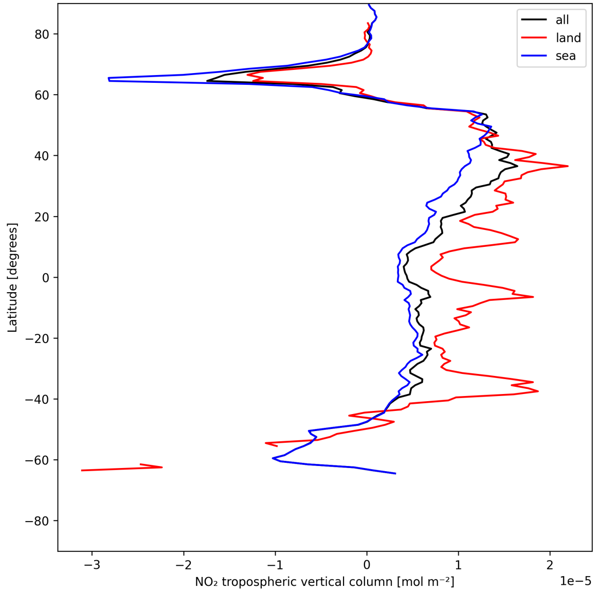
Figure 12: Zonal average of “NO 2 tropospheric vertical column” for 2025-06-04 to 2025-06-06.
