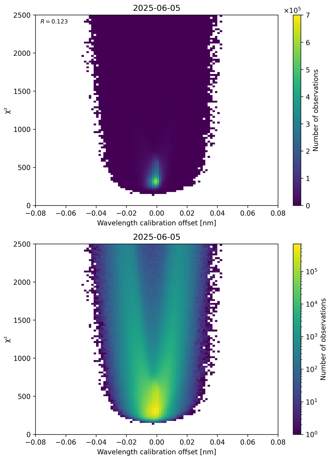
Figure 175: Scatter density plot of “Wavelength calibration offset” against “ \chi^2 ” for 2025-06-04 to 2025-06-06.
