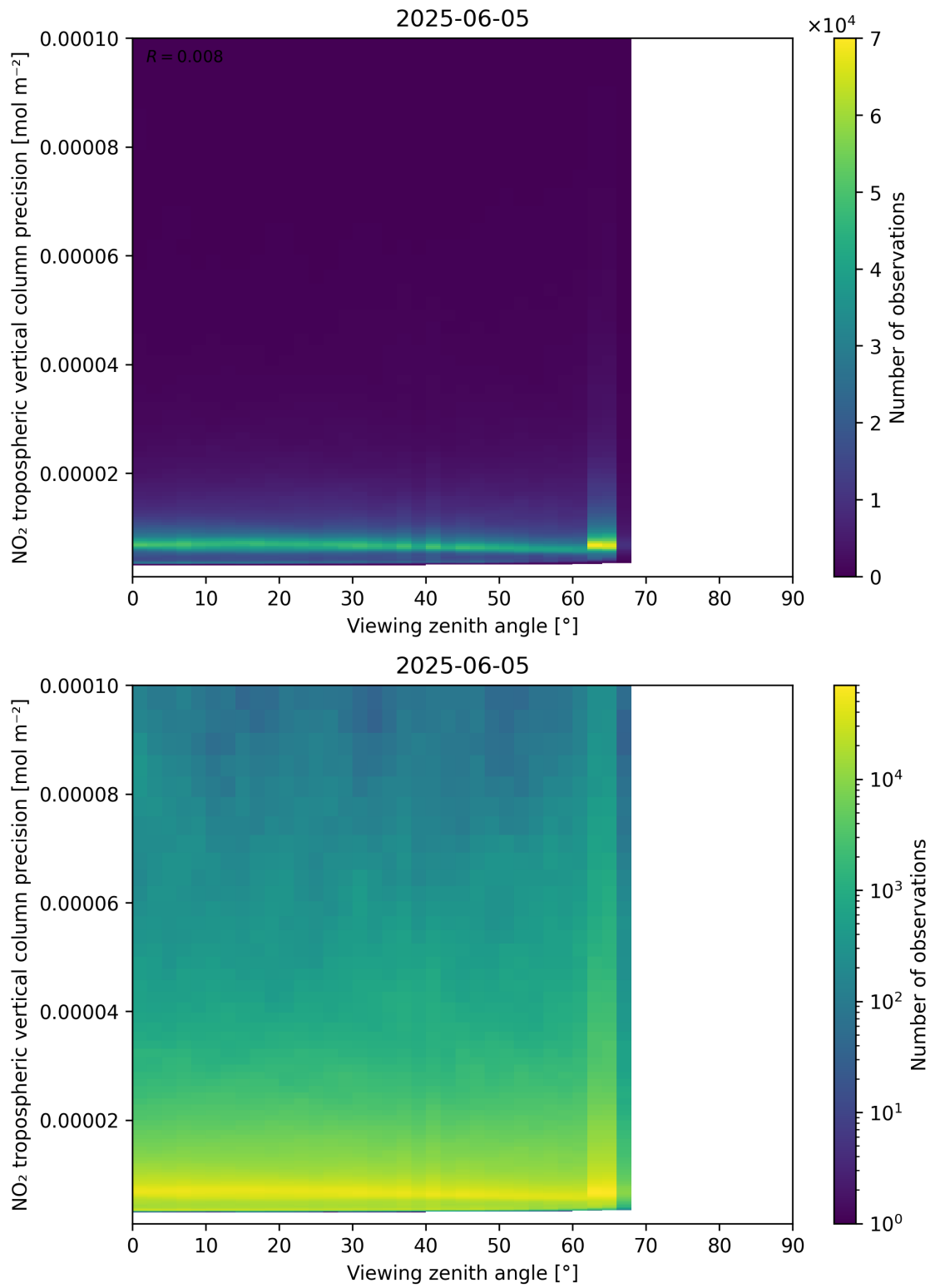
Figure 170: Scatter density plot of “Viewing zenith angle” against “NO 2 tropospheric vertical column precision” for 2025-06-04 to 2025-06-06.
