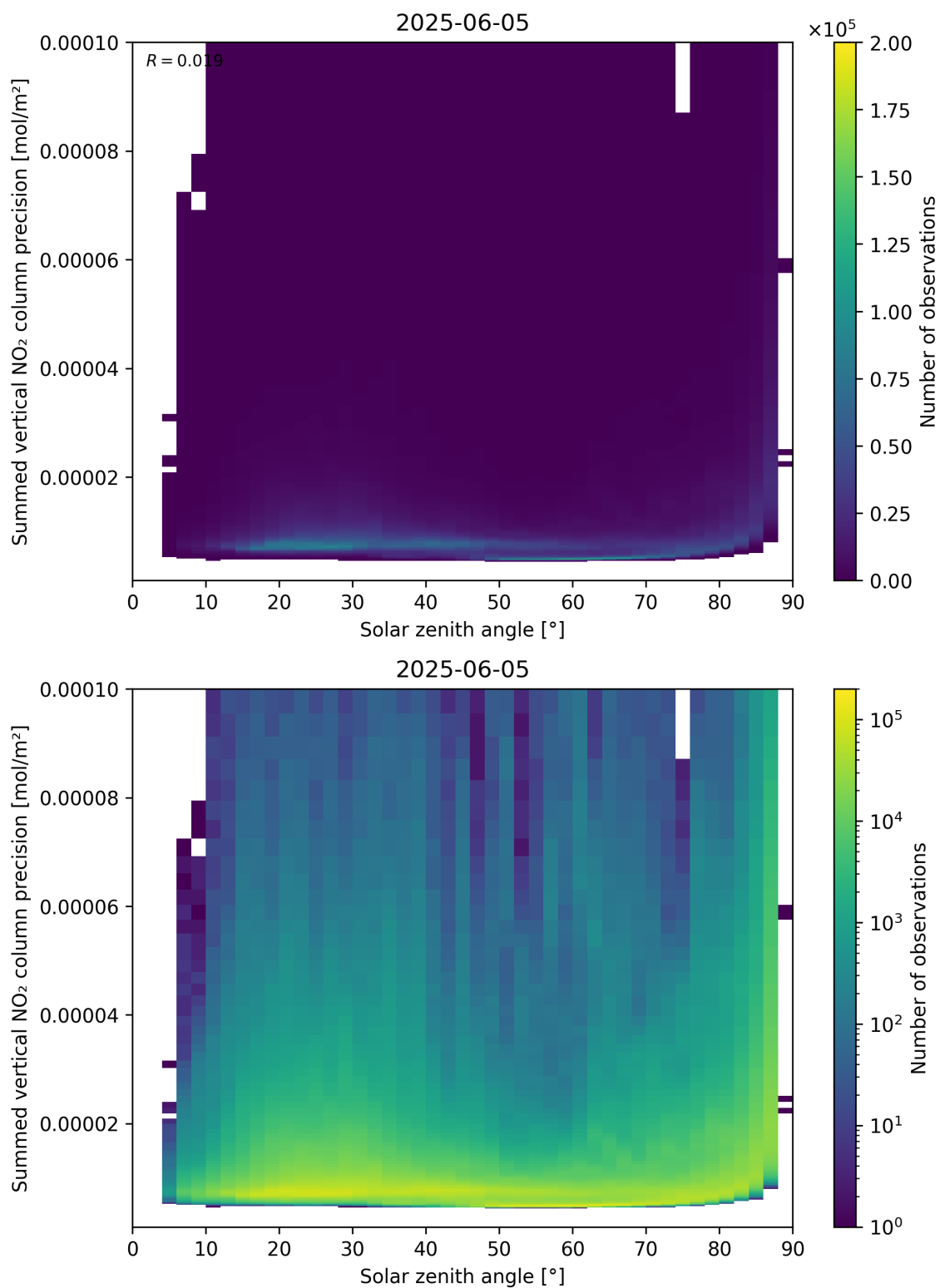
Figure 152: Scatter density plot of “Solar zenith angle” against “Summed vertical NO 2 column precision” for 2025-06-04 to 2025-06-06.
