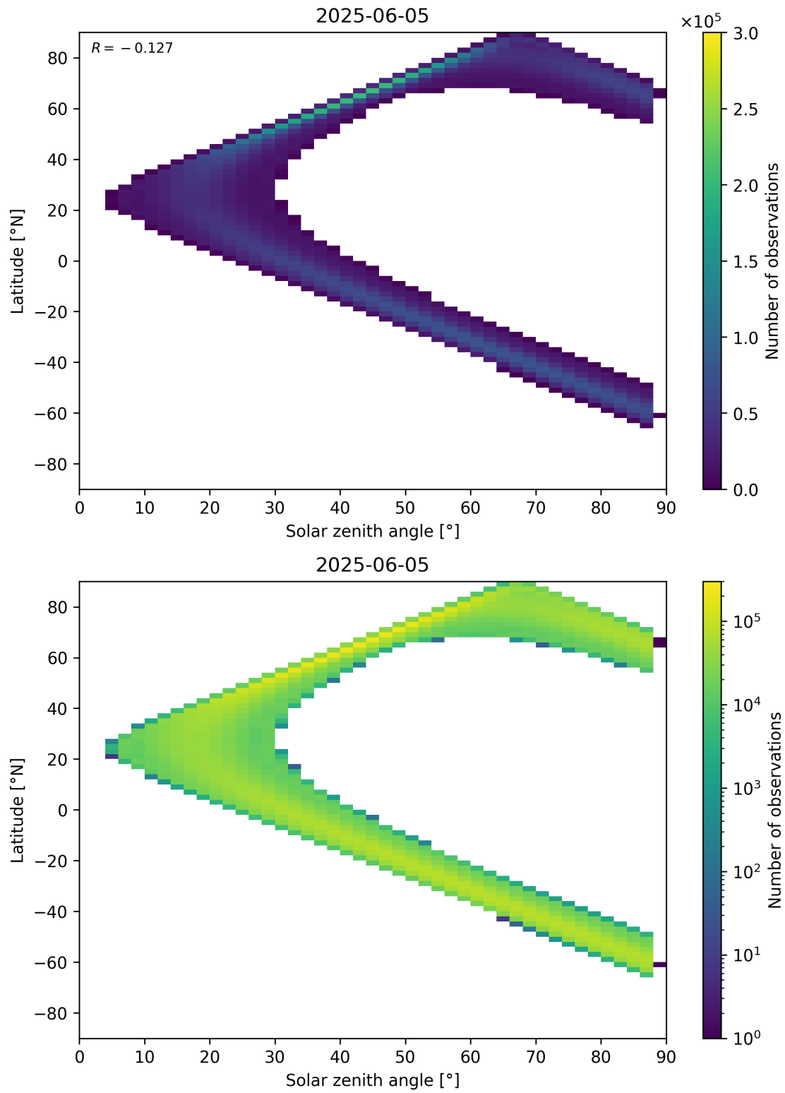
Figure 149: Scatter density plot of “Solar zenith angle” against “Latitude” for 2025-06-04 to 2025-06-06.
