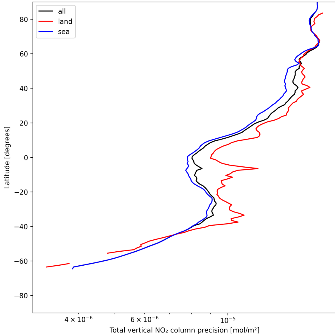
Figure 22: Zonal average of “Total vertical NO 2 column precision” for 2025-06-04 to 2025-06-06.
