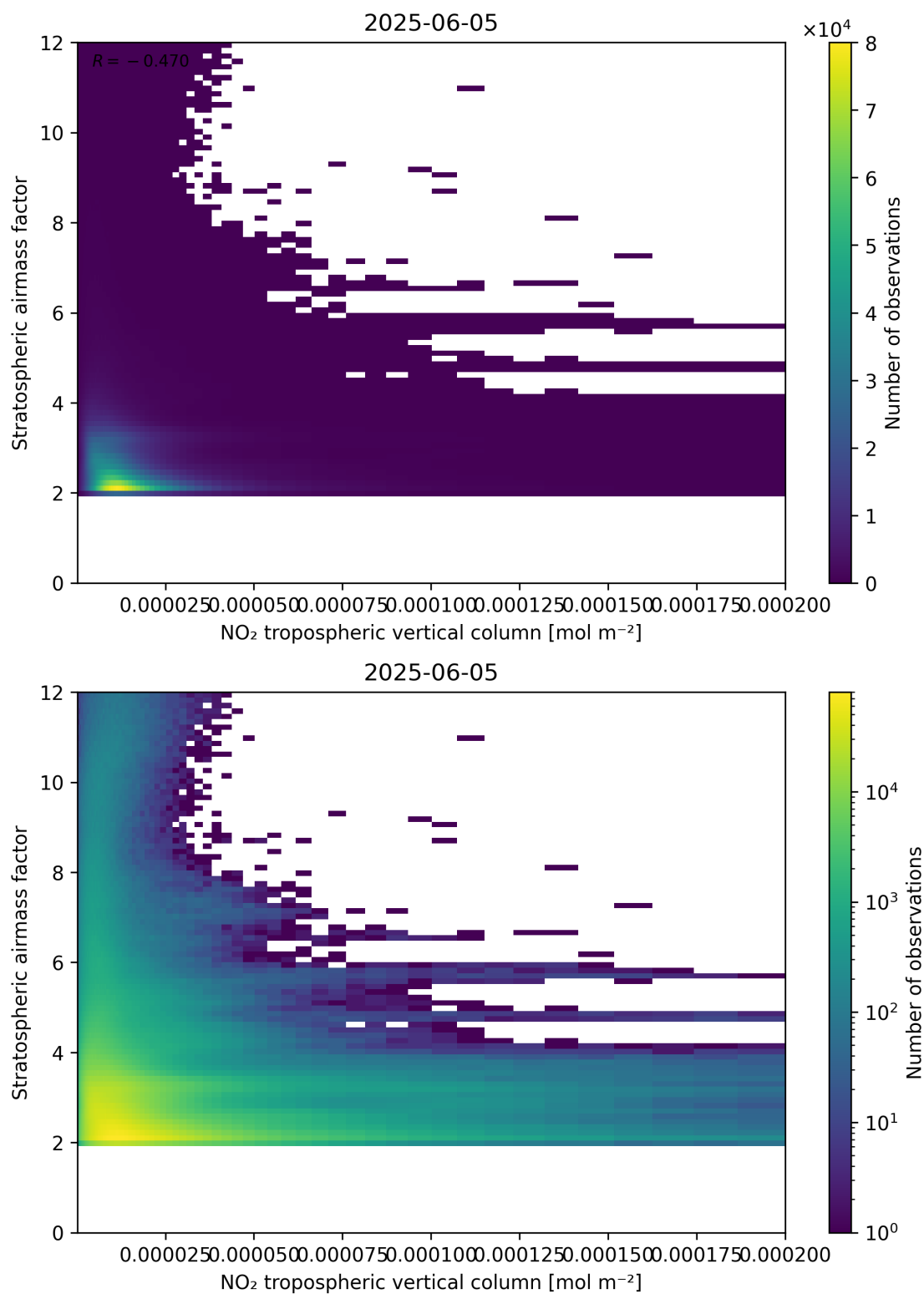
Figure 121: Scatter density plot of “NO 2 tropospheric vertical column” against “Stratospheric air mass factor” for 2025-06-04 to 2025-06-06.
