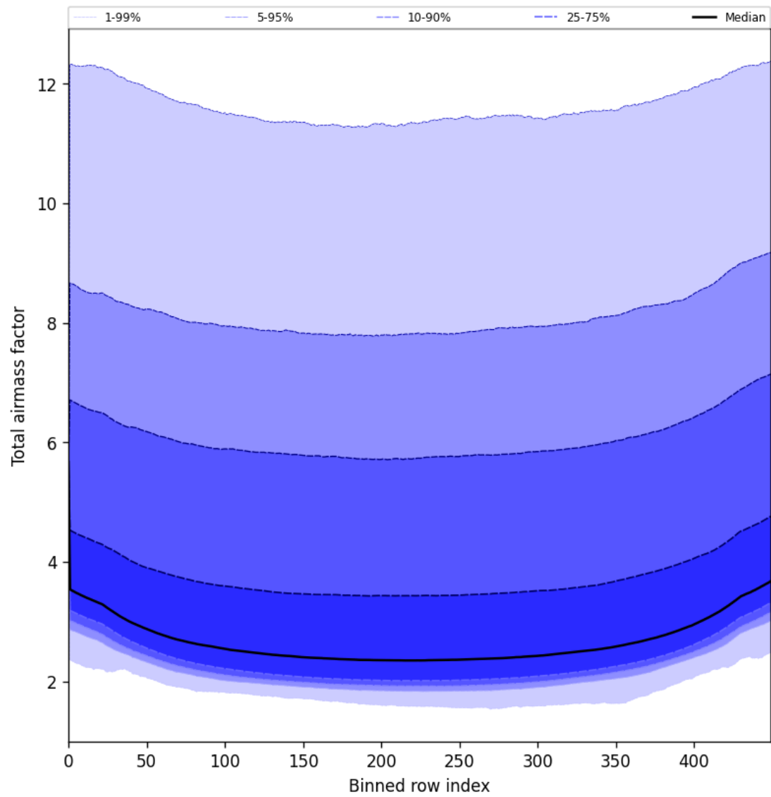
Figure 49: Along track statistics of “Total airmass factor” for 2025-06-04 to 2025-06-06
