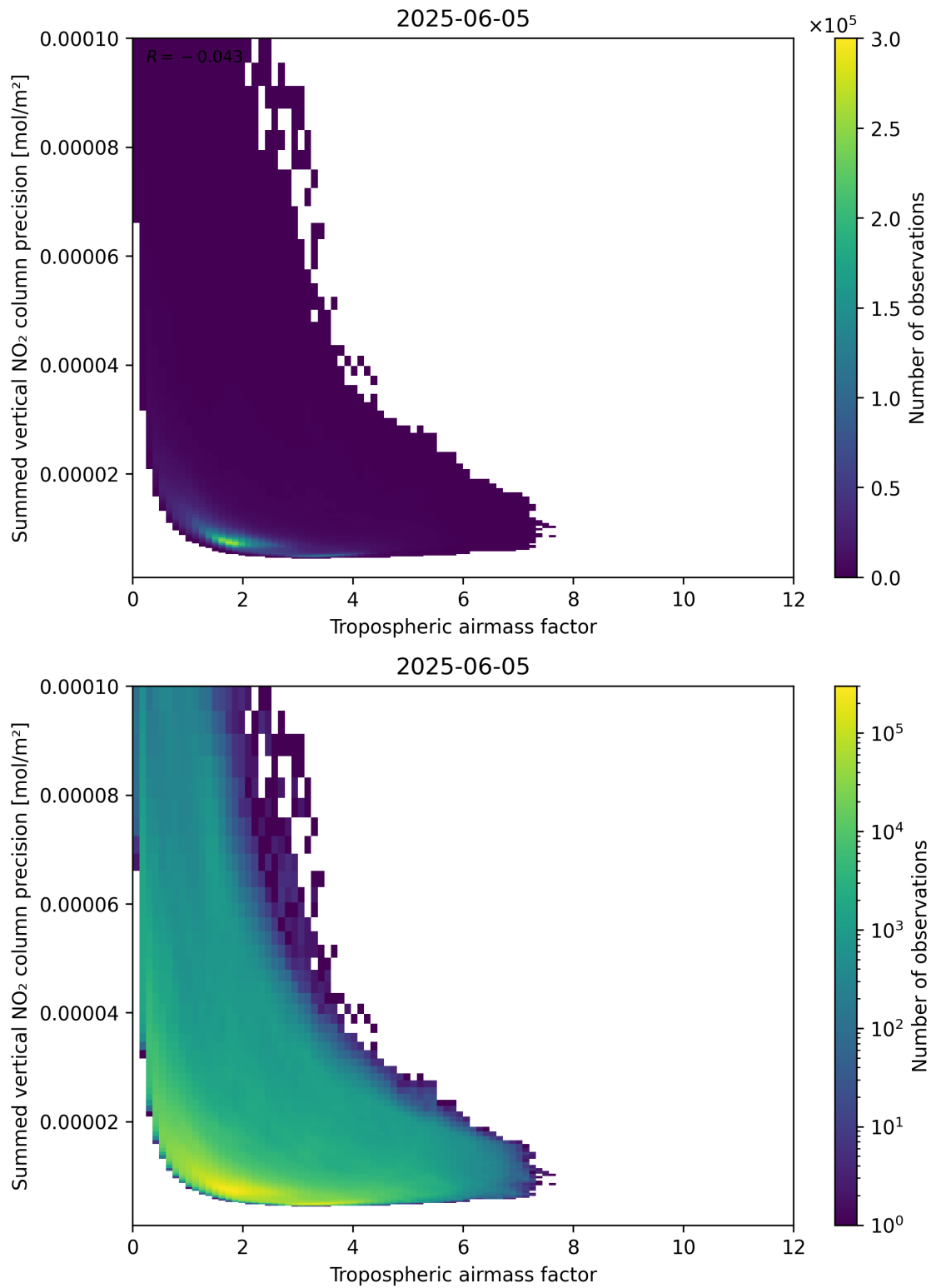
Figure 76: Scatter density plot of “Tropospheric air mass factor” against “Summed vertical NO 2 column precision” for 2025-06-04 to 2025-06-06.
