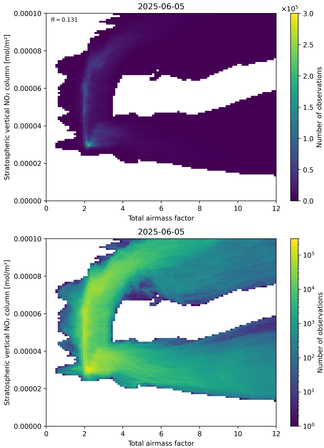
Figure 64: Scatter density plot of “Total airmass factor” against “Stratospheric vertical NO 2 column” for 2025-06-04 to 2025-06-06.
