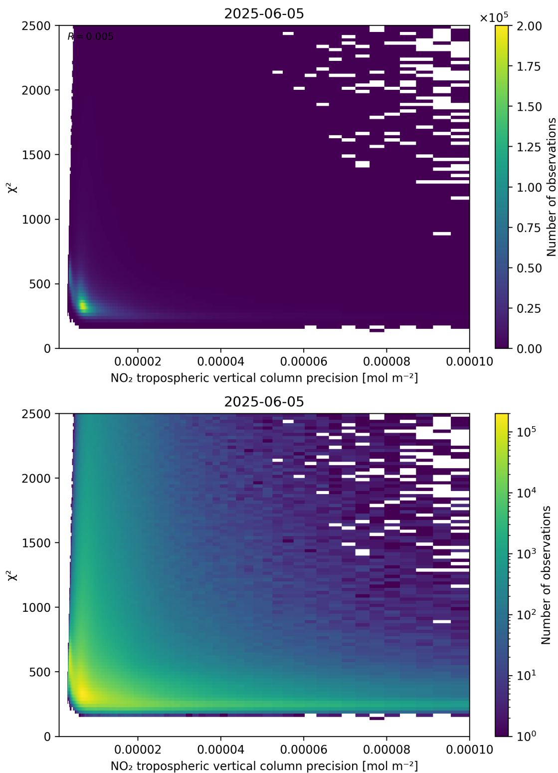
Figure 134: Scatter density plot of “NO 2 tropospheric vertical column precision” against “ \chi^2 ” for 2025-06-04 to 2025-06-06.
