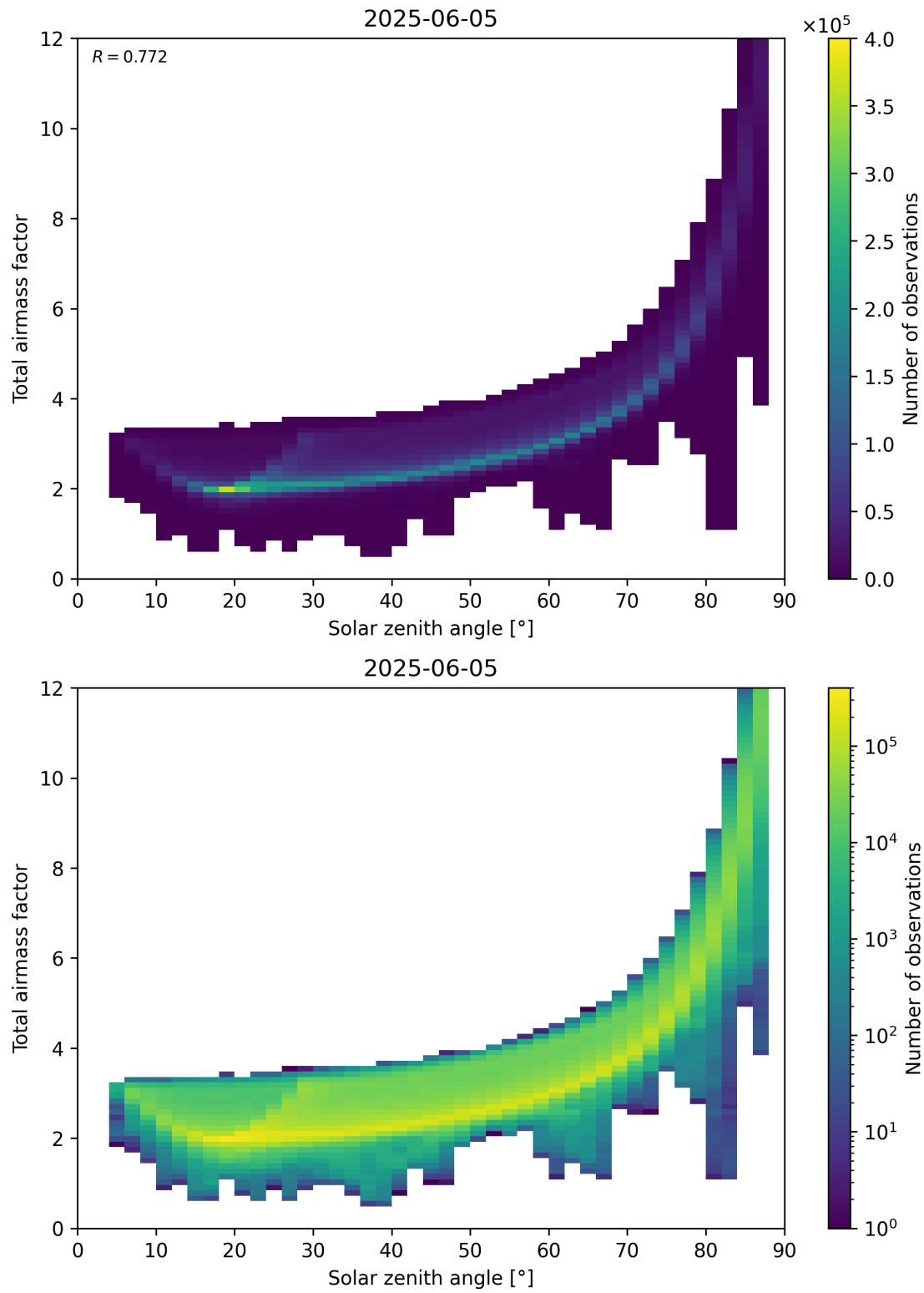
Figure 146: Scatter density plot of “Solar zenith angle” against “Total air mass factor” for 2025-06-04 to 2025-06-06.
