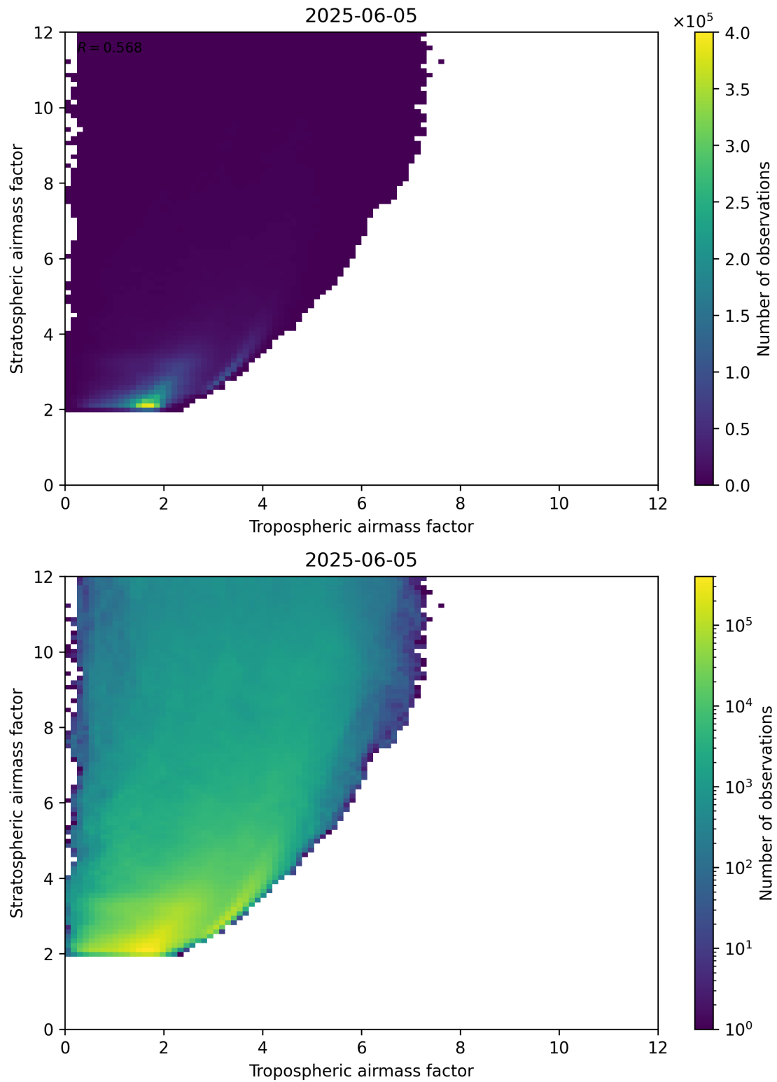
Figure 71: Scatter density plot of “Tropospheric airmass factor” against “Stratospheric airmass factor” for 2025-06-04 to 2025-06-06.
