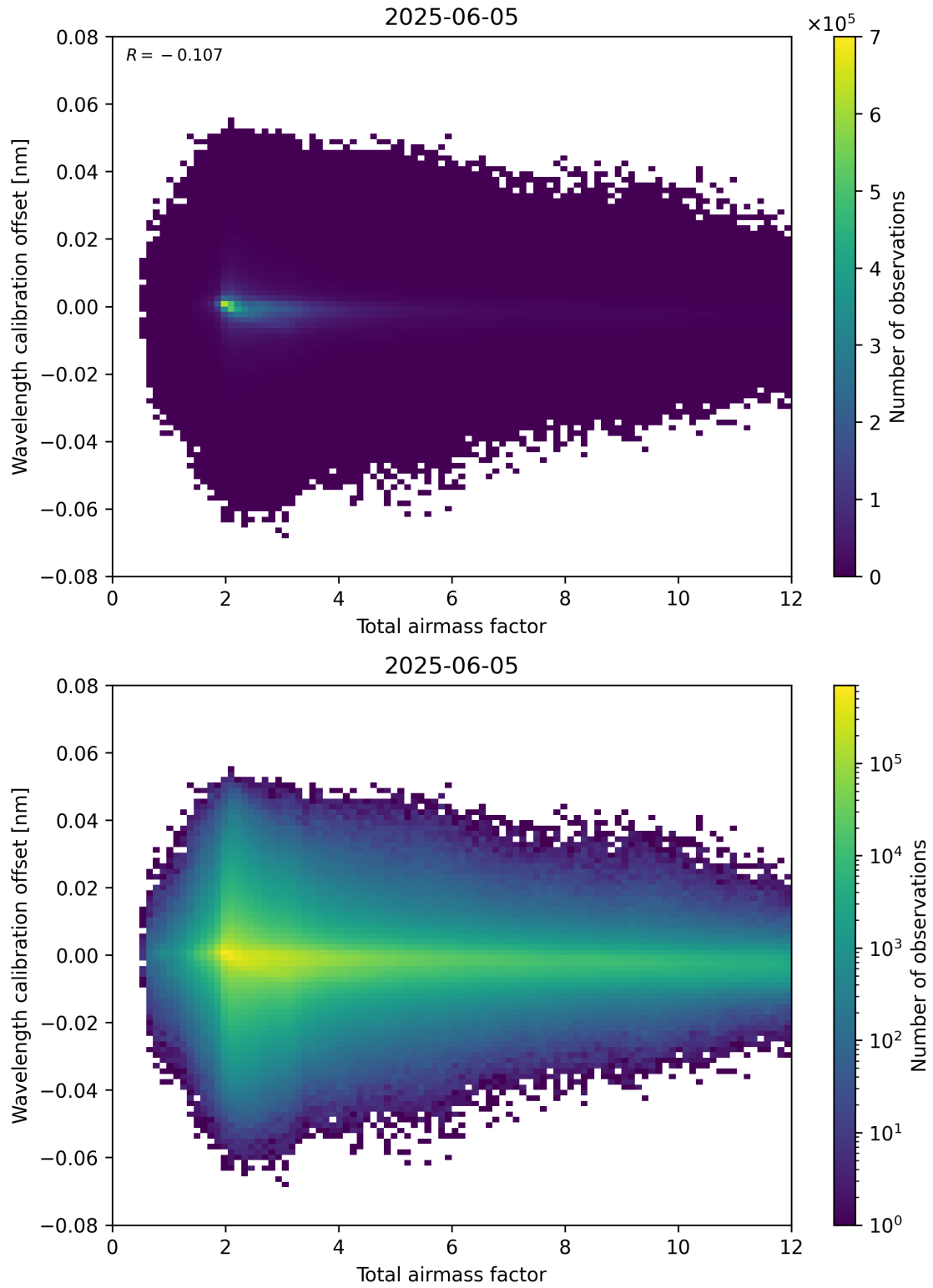
Figure 70: Scatter density plot of “Total airmass factor” against “Wavelength calibration offset” for 2025-06-04 to 2025-06-06.
