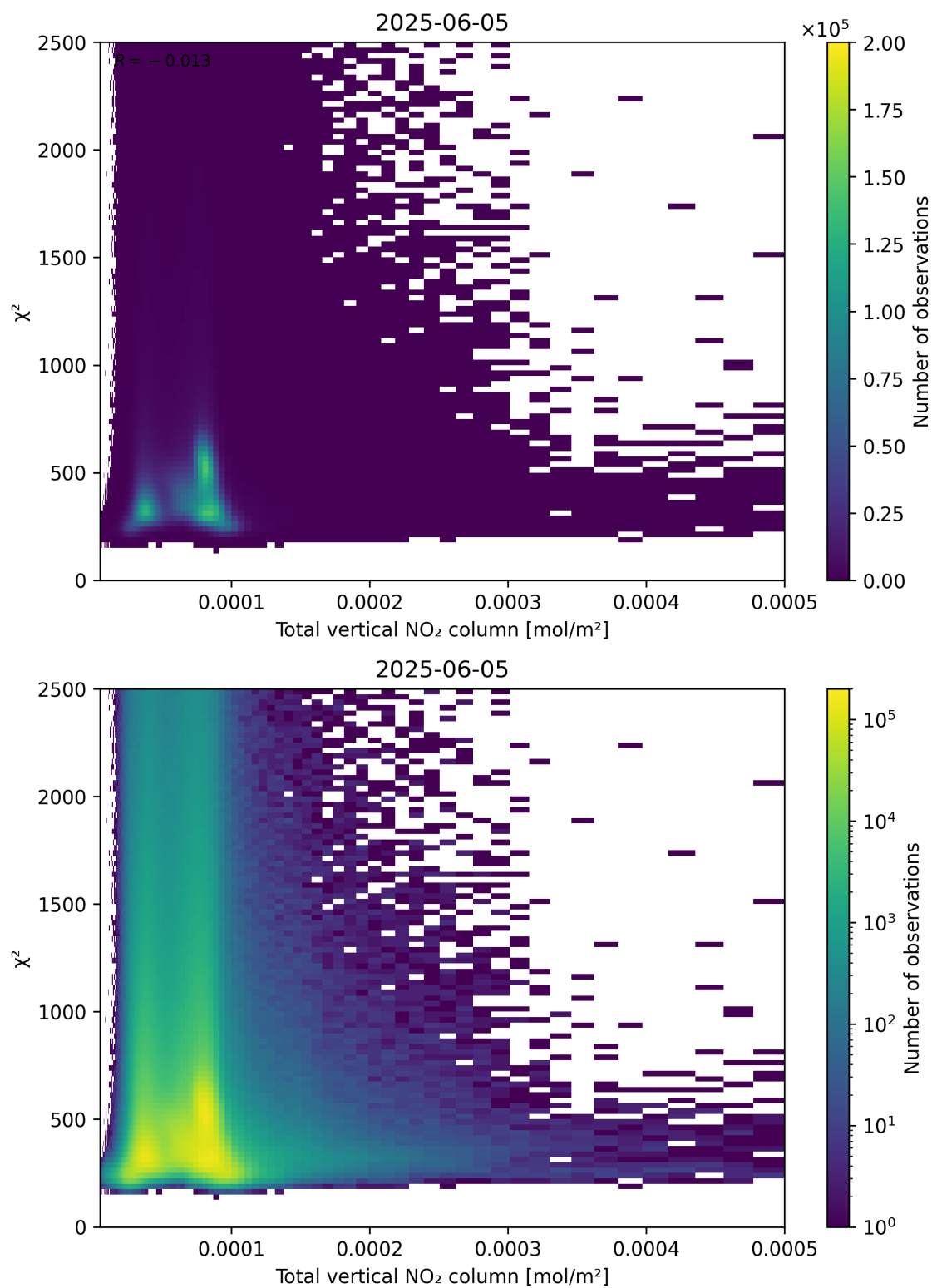
Figure 111: Scatter density plot of “Total vertical NO 2 column” against “ \chi^2 ” for 2025-06-04 to 2025-06-06.
