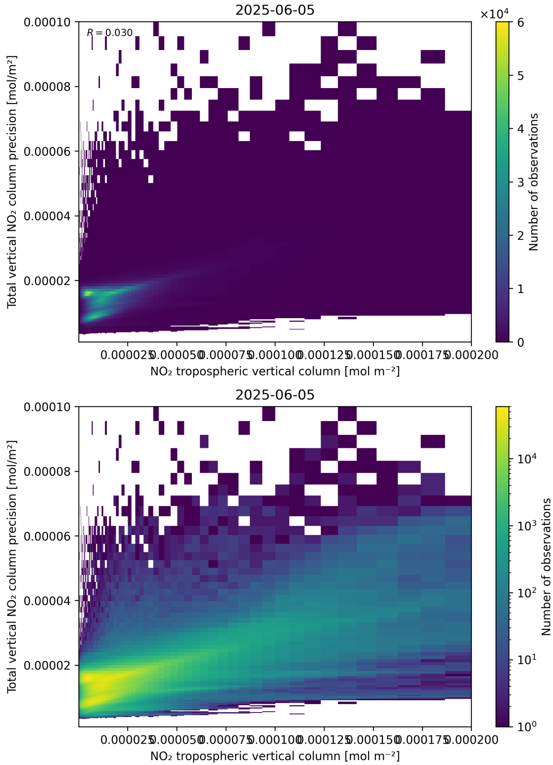
Figure 129: Scatter density plot of “NO 2 tropospheric vertical column” against “Total vertical NO 2 column precision” for 2025-06-04 to 2025-06-06.
