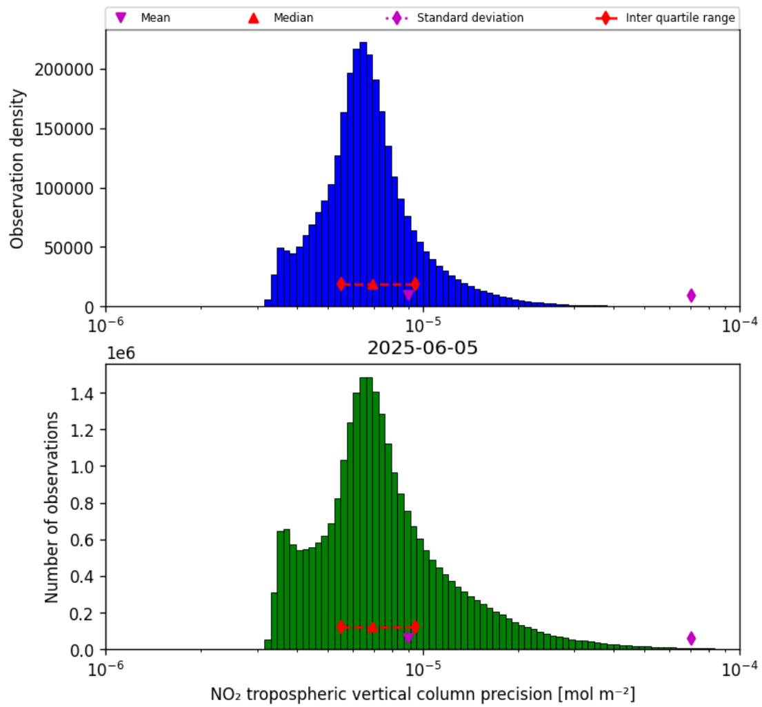
Figure 30: Histogram of “NO 2 tropospheric vertical column precision” for 2025-06-04 to 2025-06-06
