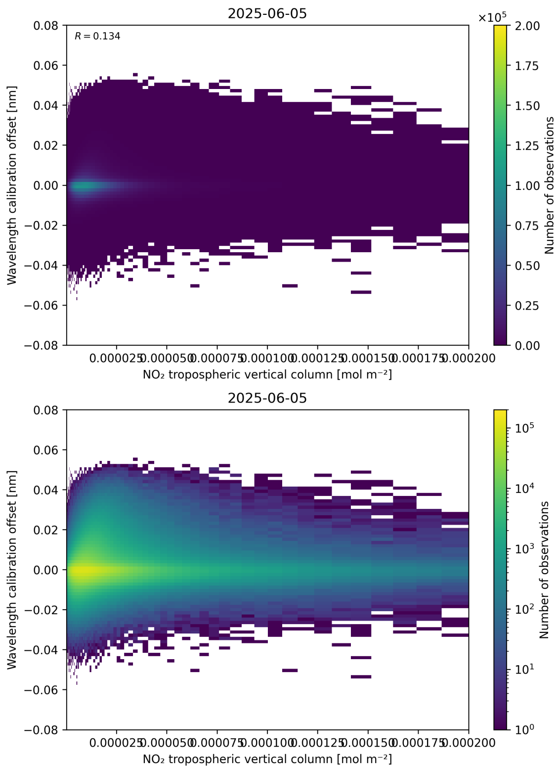
Figure 143: Scatter density plot of “NO 2 tropospheric vertical column” against “Wavelength calibration offset” for 2025-06-04 to 2025-06-06.
