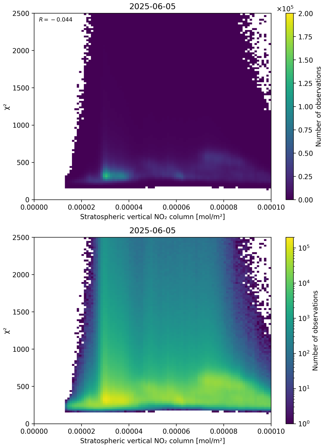
Figure 97: Scatter density plot of “Stratospheric vertical NO 2 column” against “ \chi^2 ” for 2025-06-04 to 2025-06-06.
