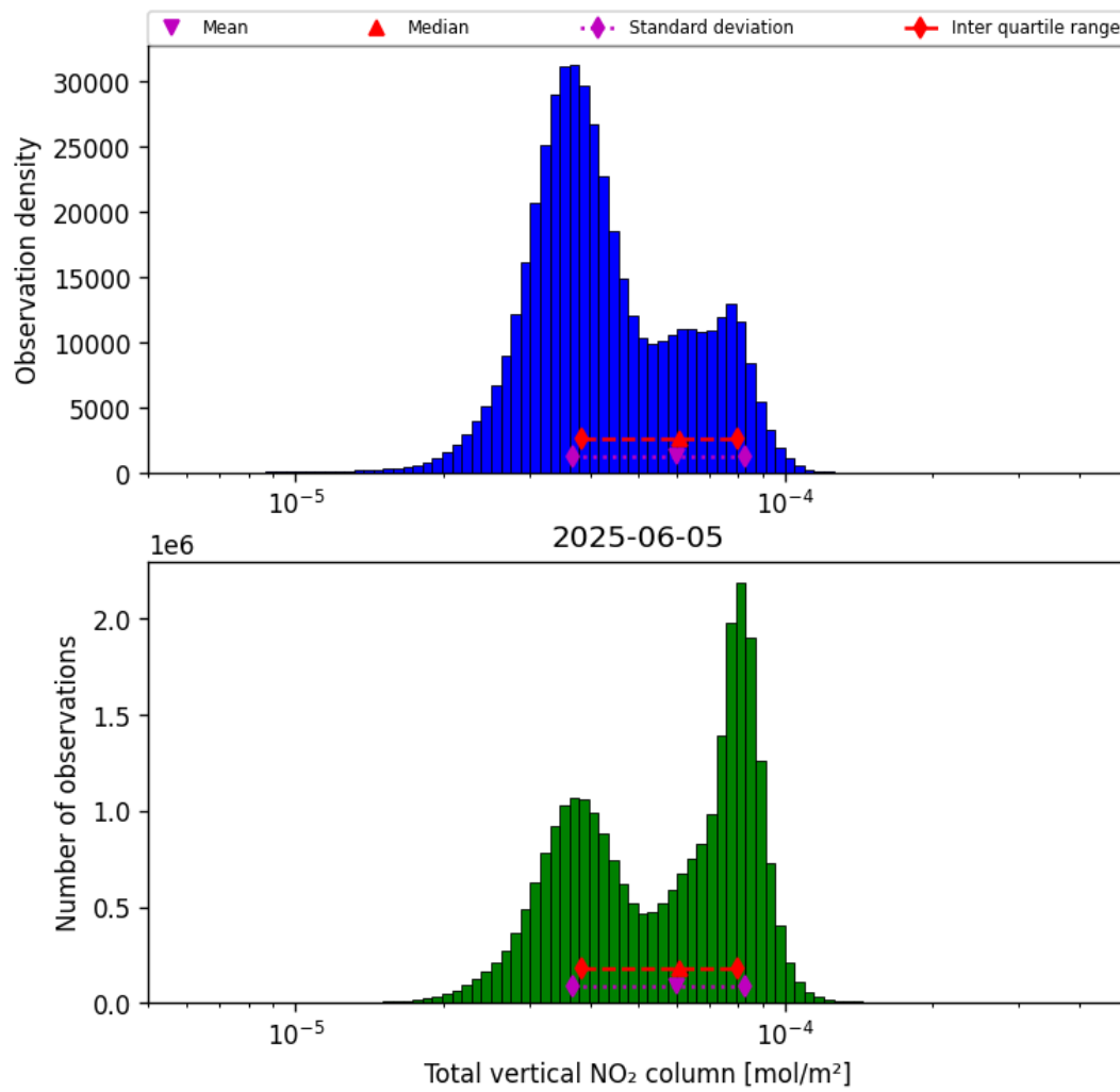
Figure 38: Histogram of “Total vertical NO 2 column” for 2025-06-04 to 2025-06-06
