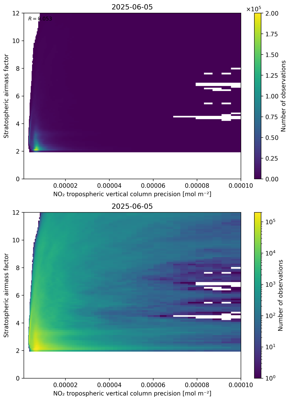
Figure 131: Scatter density plot of “NO 2 tropospheric vertical column precision” against “Stratospheric airmass factor” for 2025-06-04 to 2025-06-06.
