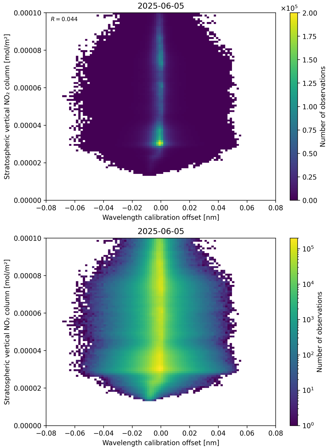
Figure 176: Scatter density plot of “Wavelength calibration offset” against “Stratospheric vertical NO 2 column” for 2025-06-04 to 2025-06-06.
