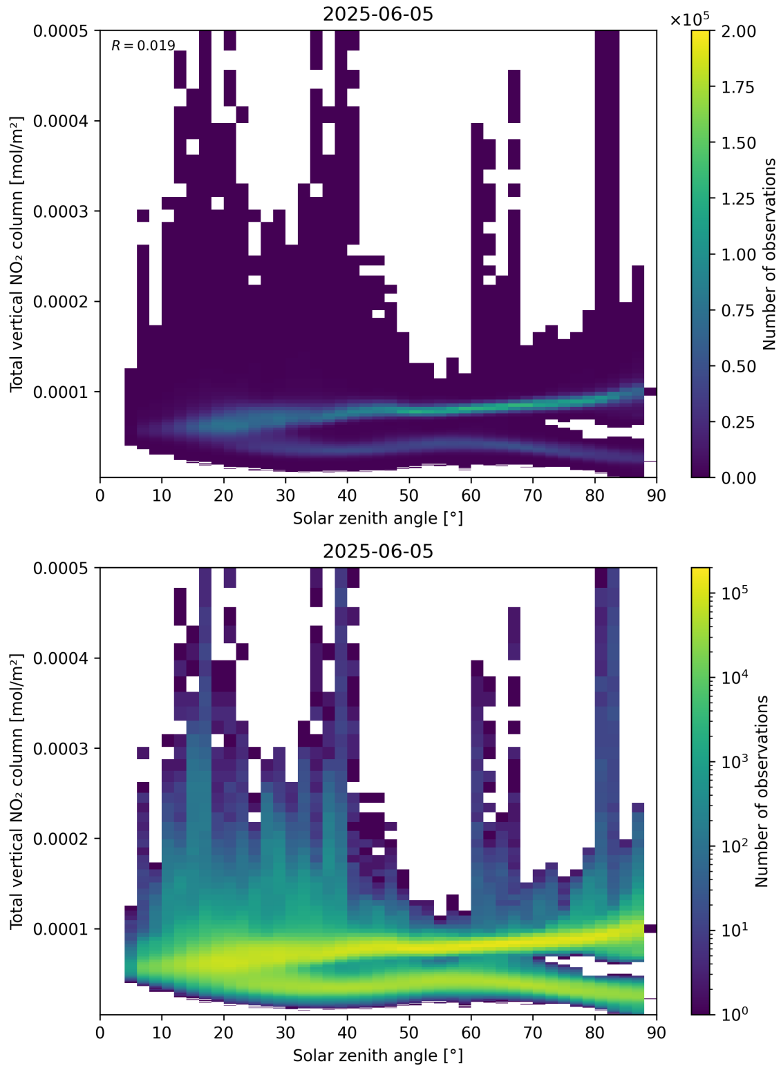
Figure 153: Scatter density plot of “Solar zenith angle” against “Total vertical NO 2 column” for 2025-06-04 to 2025-06-06.
