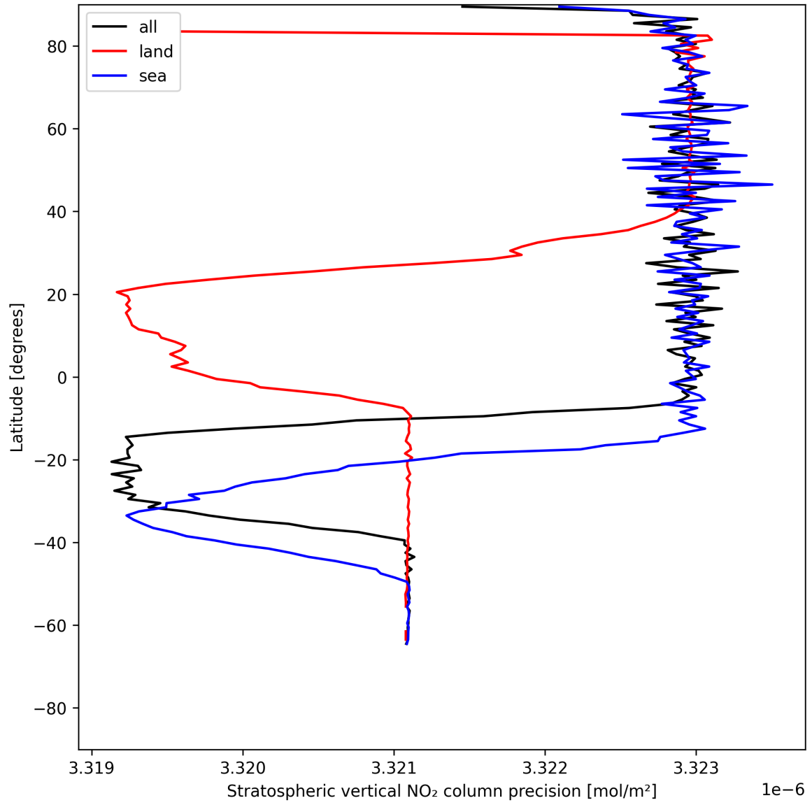
Figure 20: Zonal average of “Stratospheric vertical NO 2 column precision” for 2025-06-04 to 2025-06-06.
