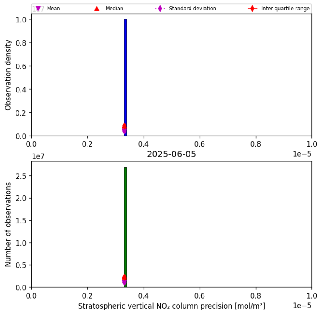
Figure 37: Histogram of “Stratospheric vertical NO 2 column precision” for 2025-06-04 to 2025-06-06
