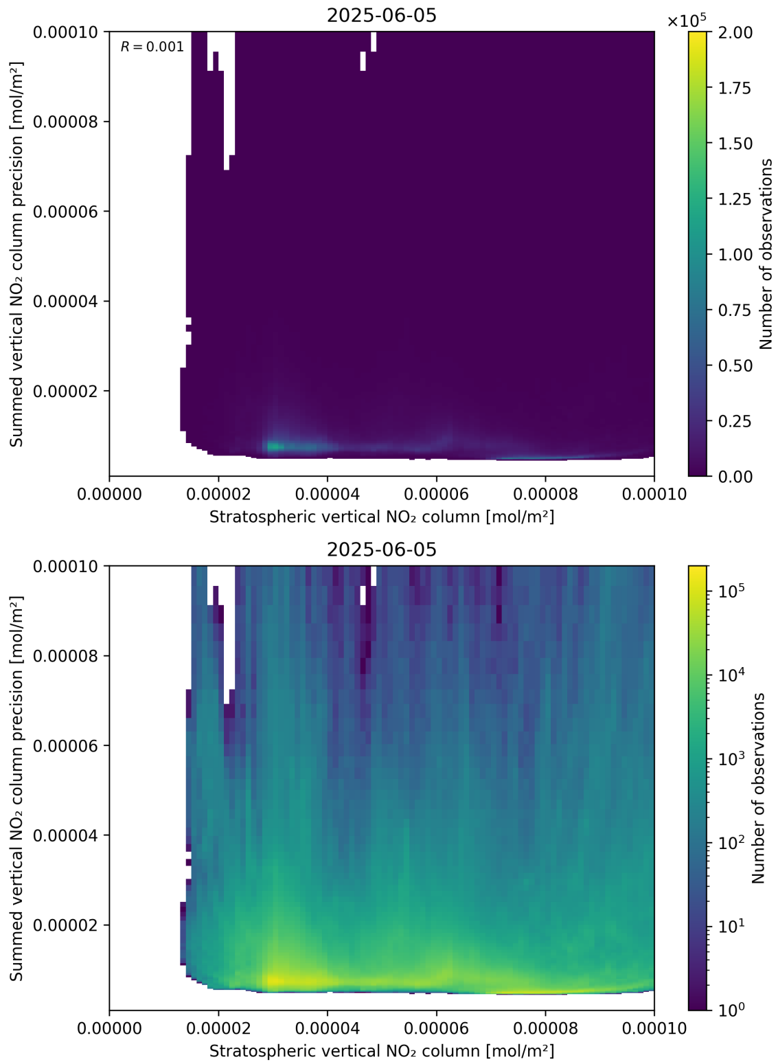
Figure 99: Scatter density plot of “Stratospheric vertical NO 2 column” against “Summed vertical NO 2 column precision” for 2025-06-04 to 2025-06-06.
