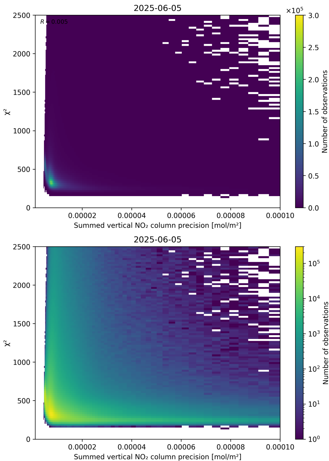
Figure 107: Scatter density plot of “Summed vertical NO 2 column precision” against “ \chi^2 ” for 2025-06-04 to 2025-06-06.
