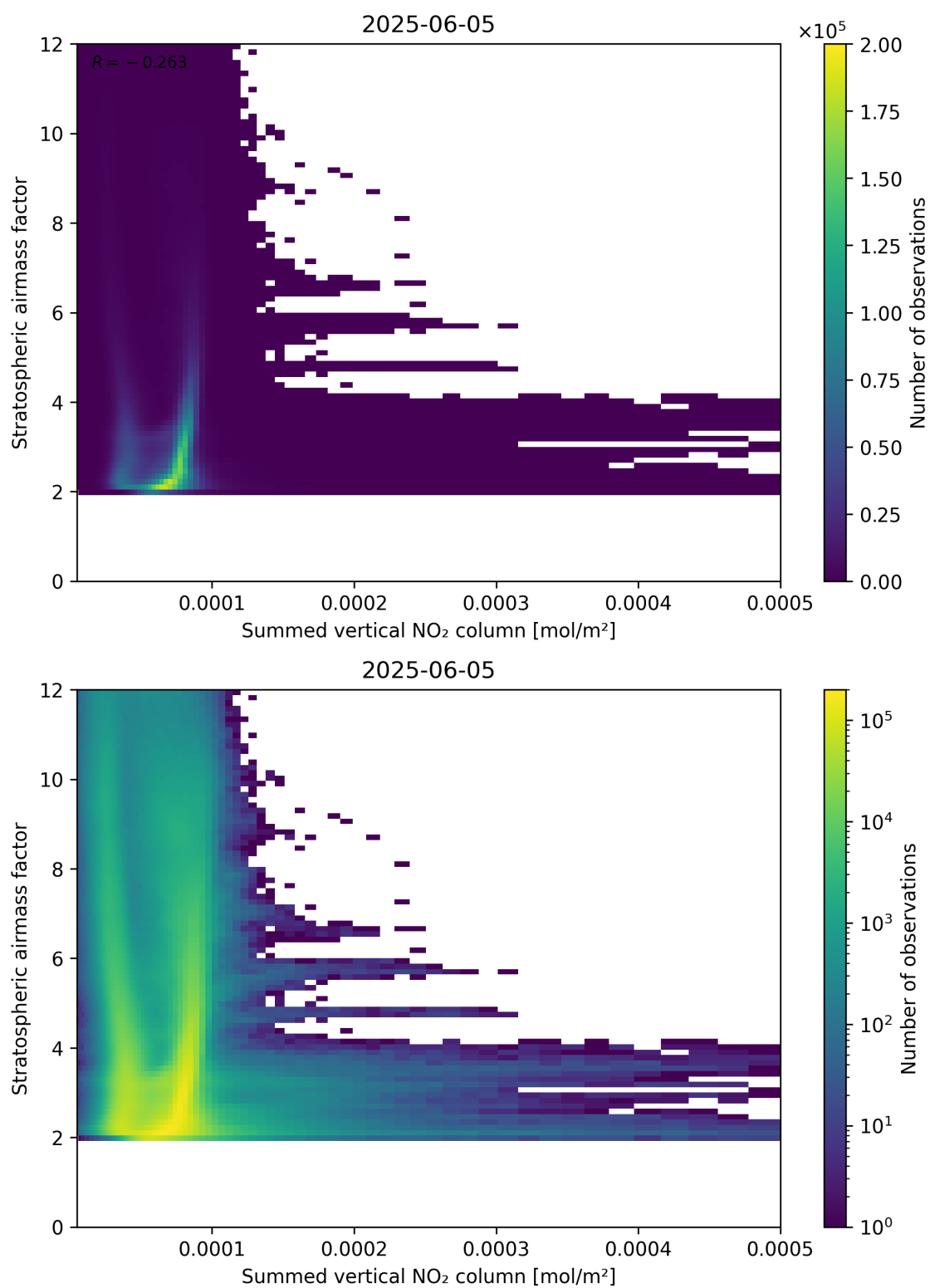
Figure 103: Scatter density plot of “Summed vertical NO 2 column” against “Stratospheric airmass factor” for 2025-06-04 to 2025-06-06.
