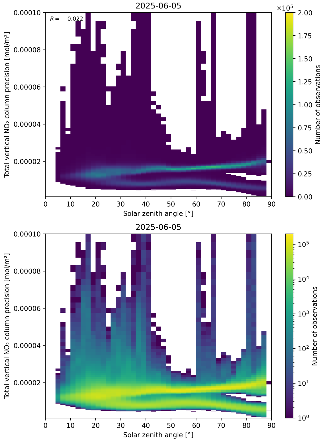
Figure 154: Scatter density plot of “Solar zenith angle” against “Total vertical NO 2 column precision” for 2025-06-04 to 2025-06-06.
