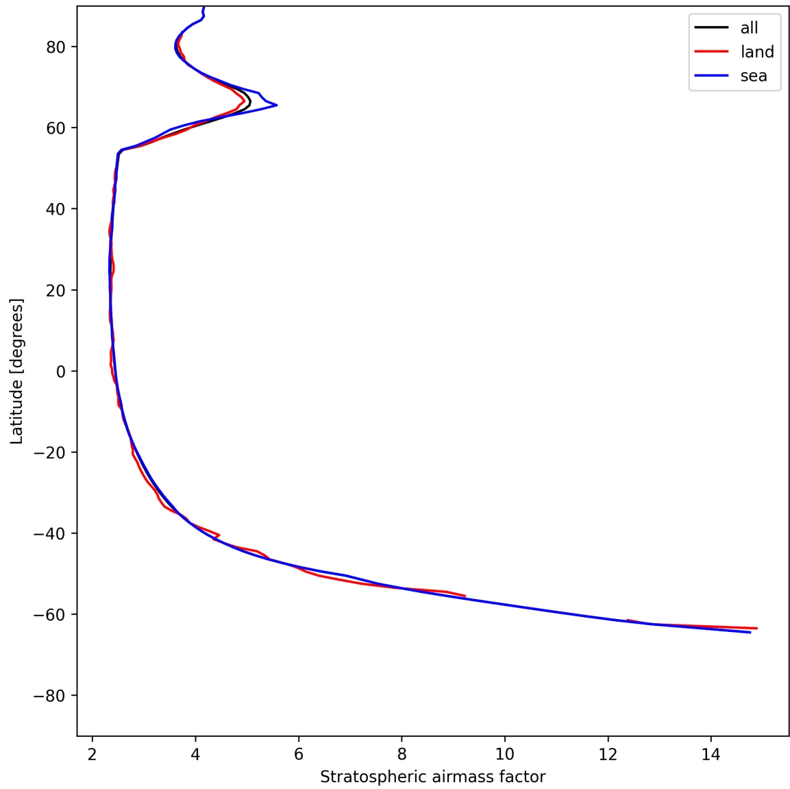
Figure 27: Zonal average of “Stratospheric air mass factor” for 2025-06-04 to 2025-06-06.
