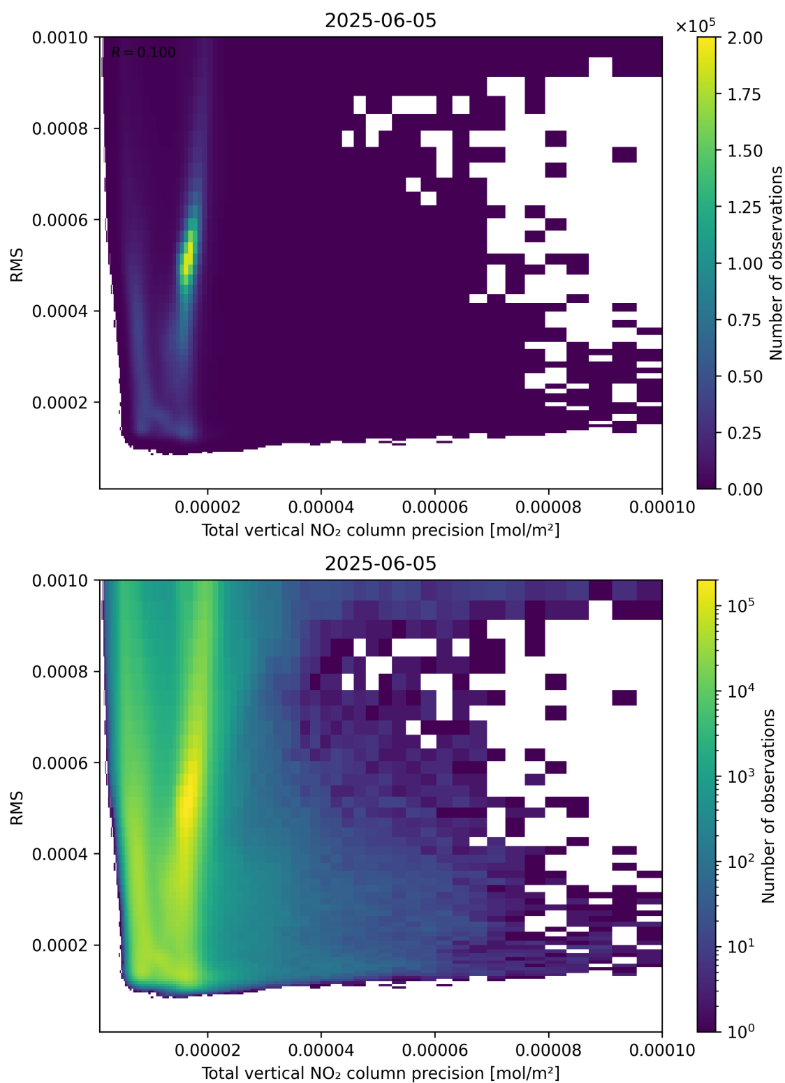
Figure 119: Scatter density plot of “Total vertical NO 2 column precision” against “RMS” for 2025-06-04 to 2025-06-06.
