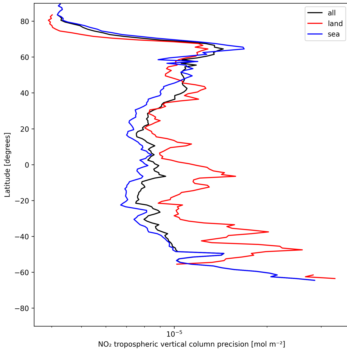
Figure 13: Zonal average of “NO 2 tropospheric vertical column precision” for 2025-06-04 to 2025-06-06.
