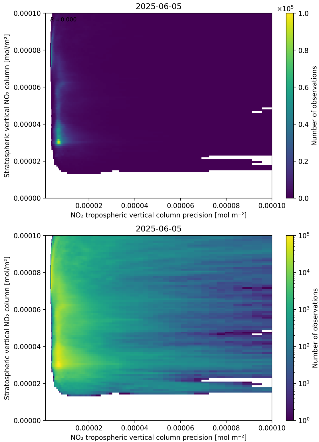
Figure 135: Scatter density plot of “NO 2 tropospheric vertical column precision” against “Stratospheric vertical NO 2 column” for 2025-06-04 to 2025-06-06.
