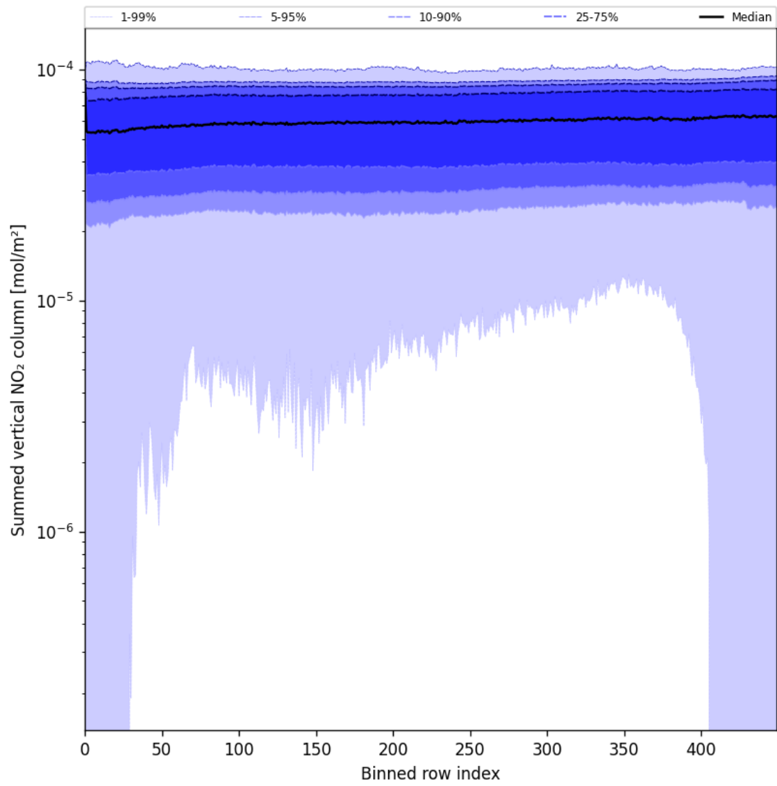
Figure 57: Along track statistics of “Summed vertical NO 2 column” for 2025-06-04 to 2025-06-06
