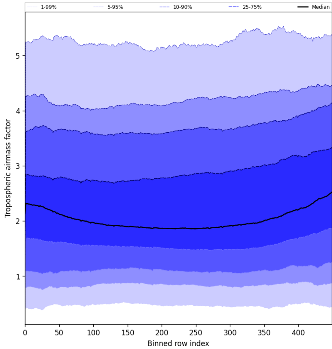
Figure 48: Along track statistics of “Tropospheric air mass factor” for 2025-06-04 to 2025-06-06
