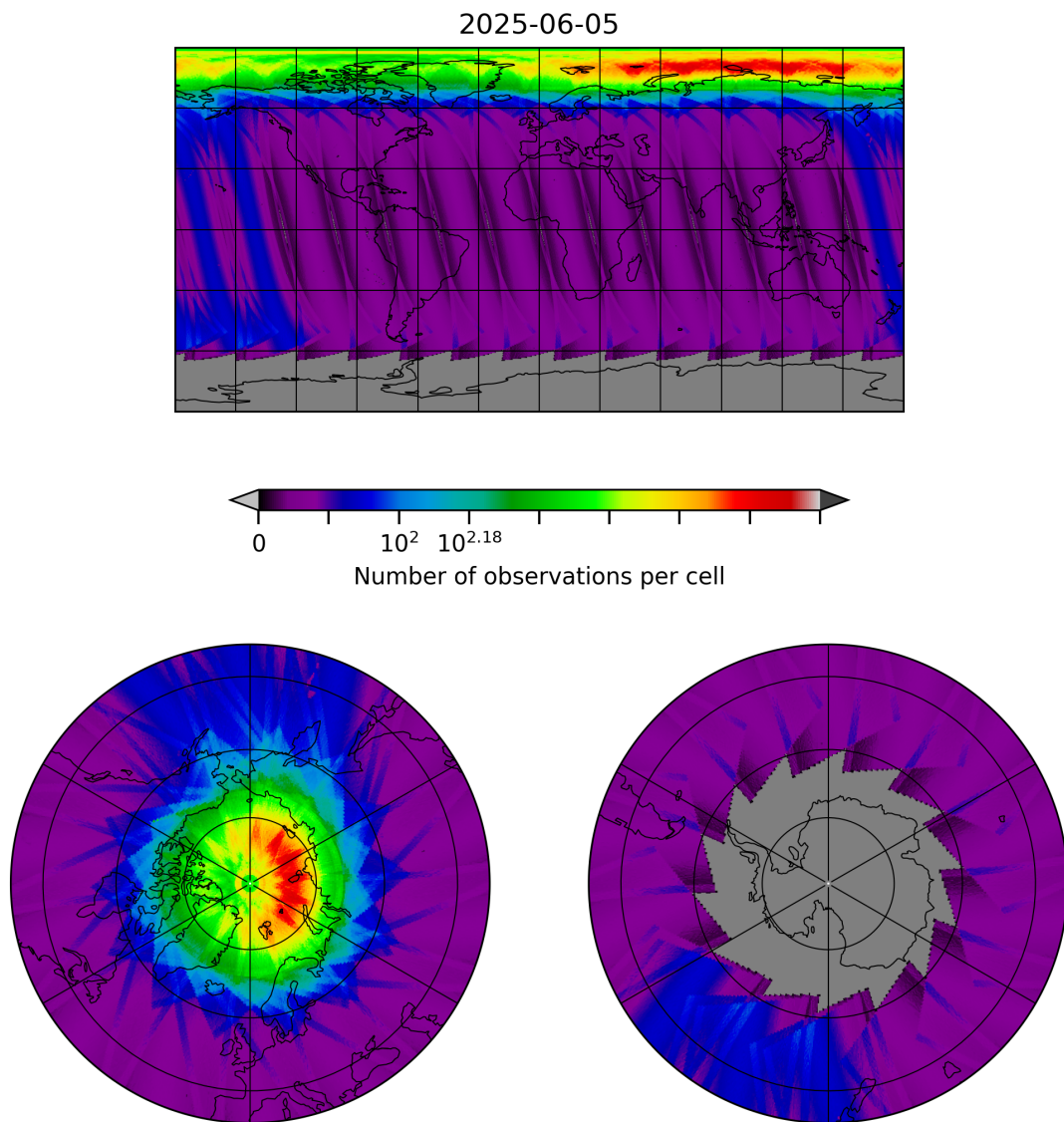
Figure 10: Map of the number of observations for 2025-06-04 to 2025-06-06
