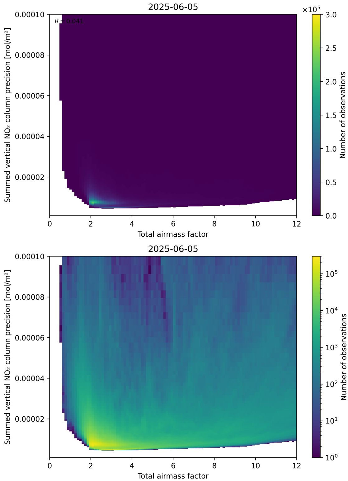
Figure 66: Scatter density plot of “Total airmass factor” against “Summed vertical NO 2 column precision” for 2025-06-04 to 2025-06-06.
