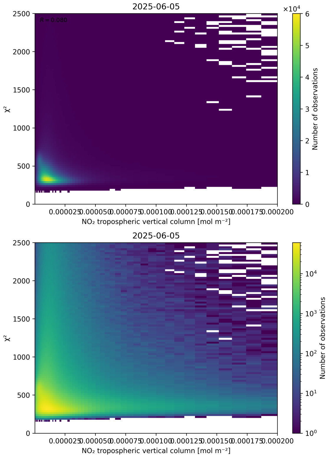
Figure 124: Scatter density plot of “NO 2 tropospheric vertical column” against “ \chi^2 ” for 2025-06-04 to 2025-06-06.
