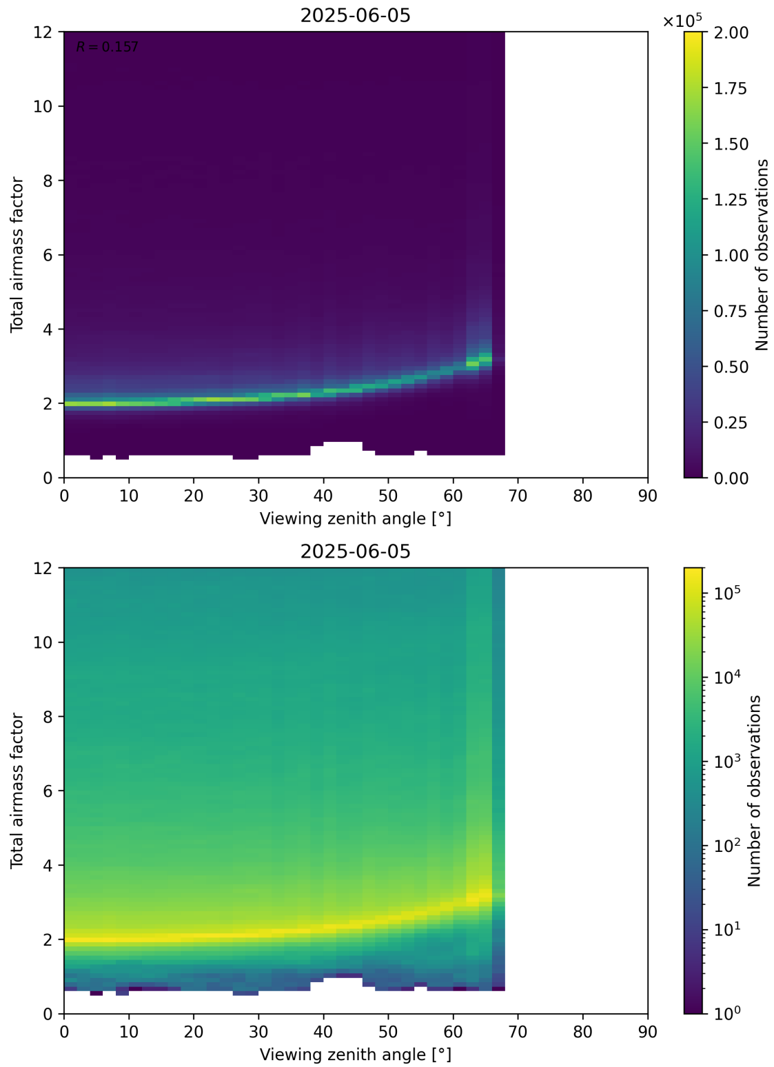
Figure 160: Scatter density plot of “Viewing zenith angle” against “Total airmass factor” for 2025-06-04 to 2025-06-06.
