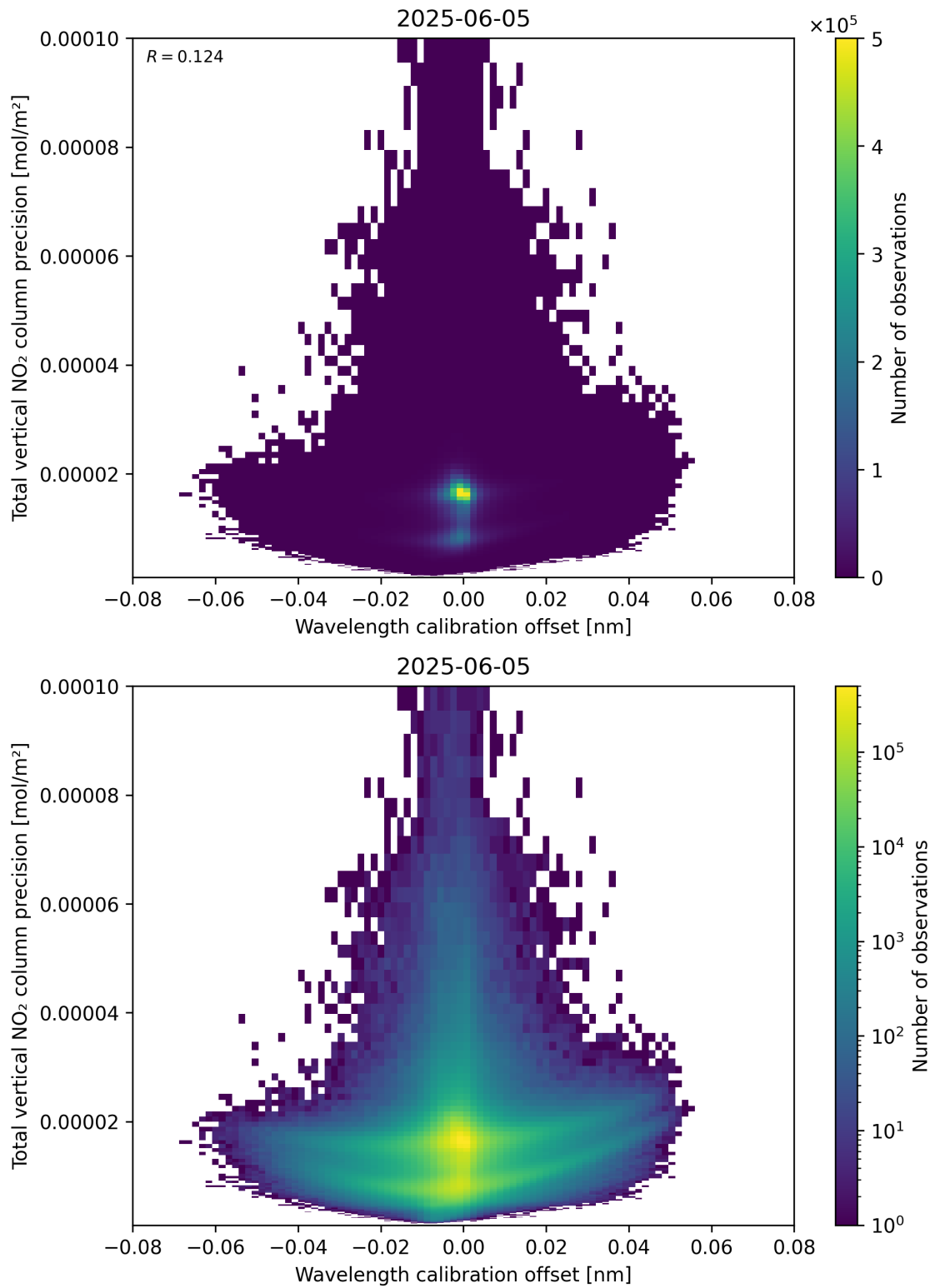
Figure 180: Scatter density plot of “Wavelength calibration offset” against “Total vertical NO 2 column precision” for 2025-06-04 to 2025-06-06.
