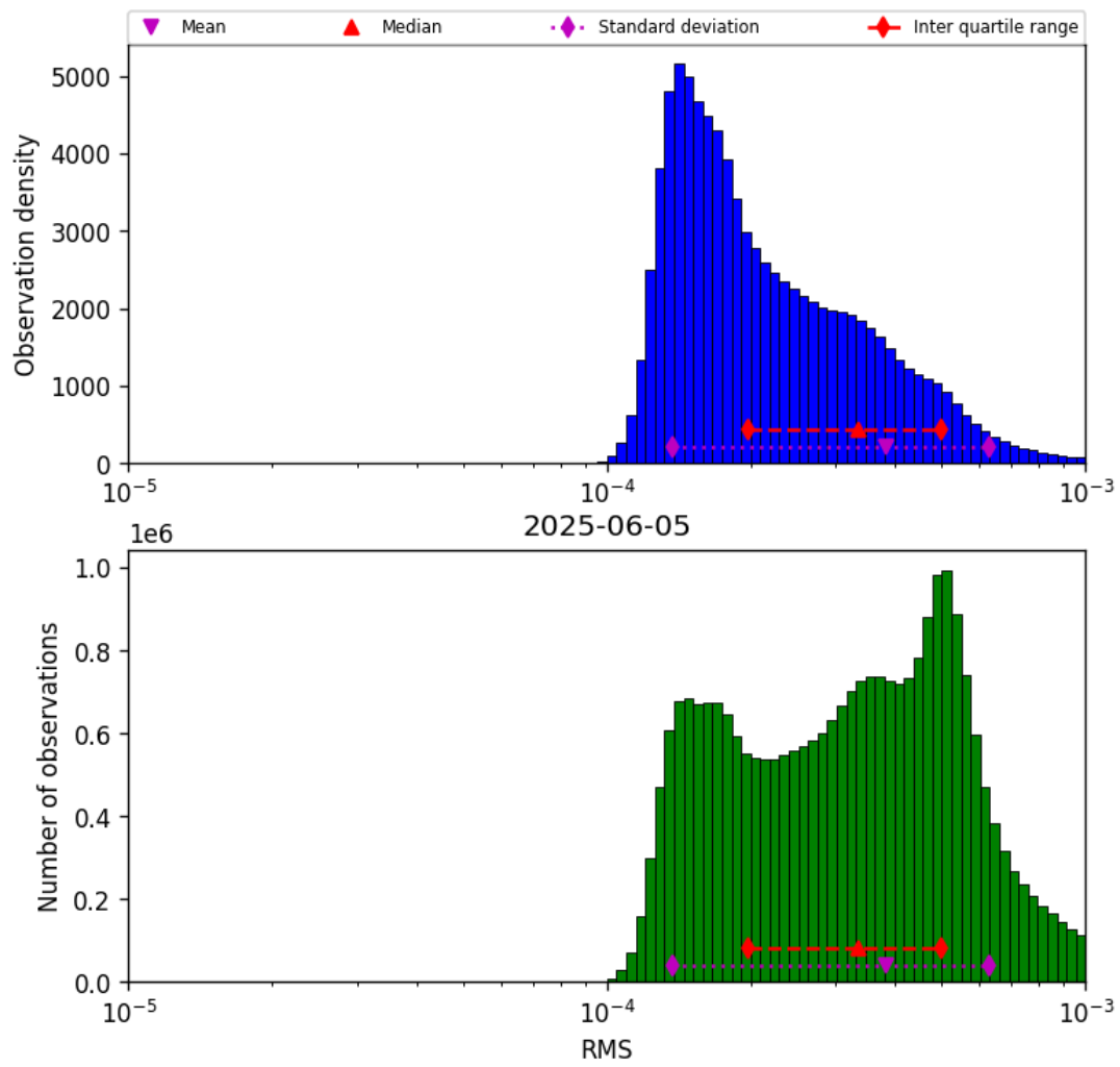
Figure 43: Histogram of “RMS” for 2025-06-04 to 2025-06-06
