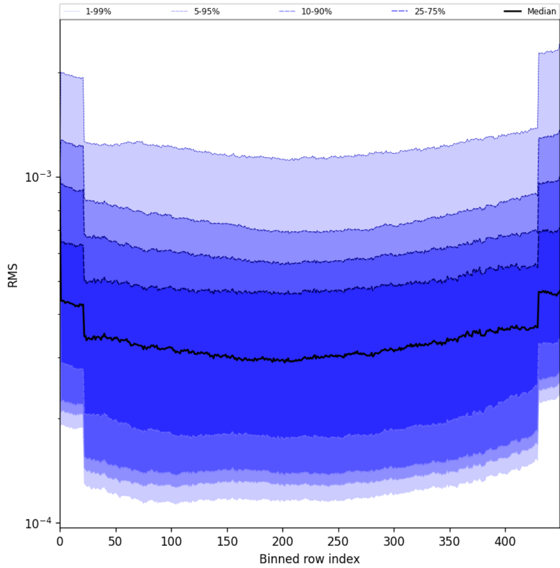
Figure 60: Along track statistics of “RMS” for 2025-06-04 to 2025-06-06
