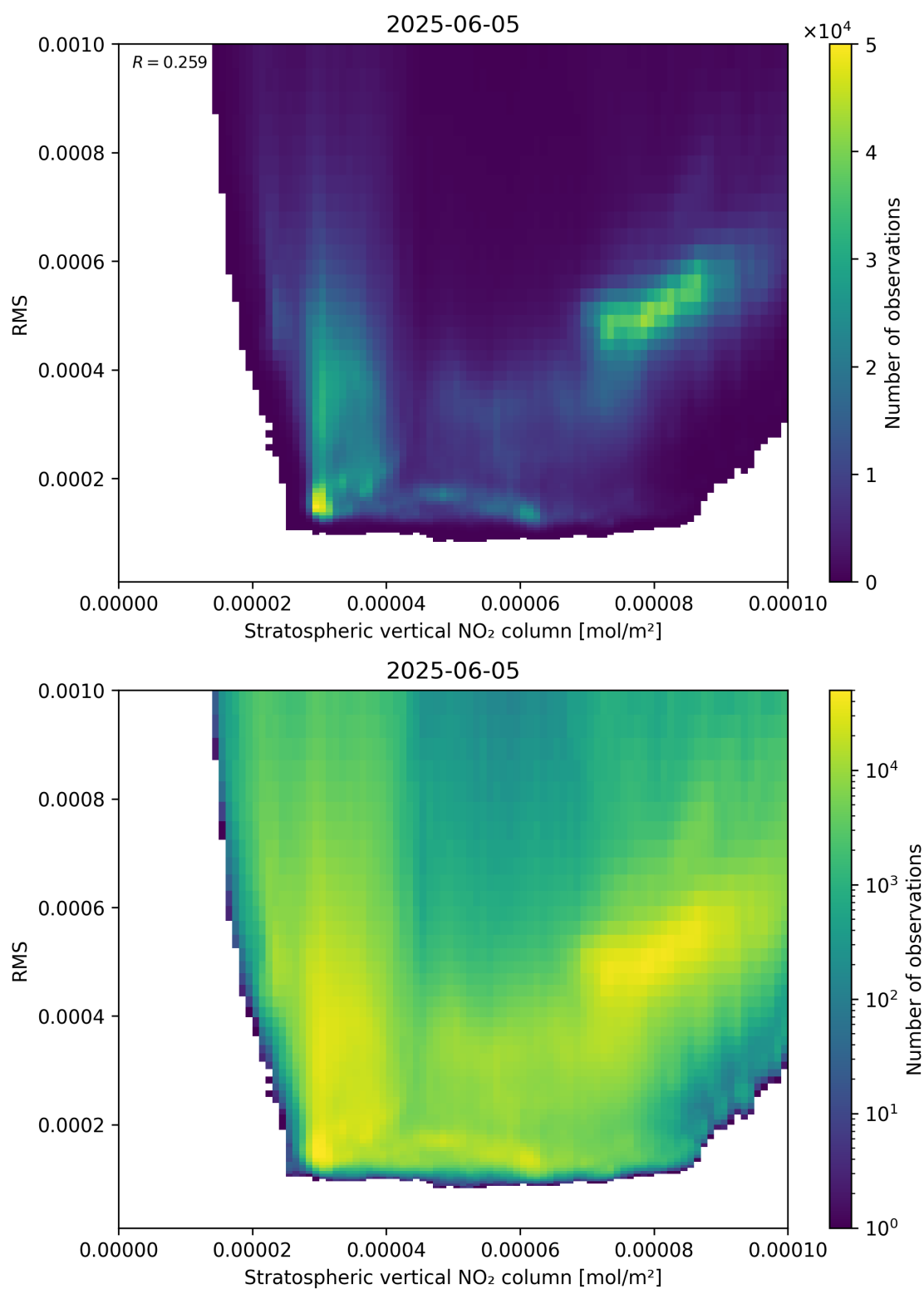
Figure 102: Scatter density plot of “Stratospheric vertical NO 2 column” against “RMS” for 2025-06-04 to 2025-06-06.
