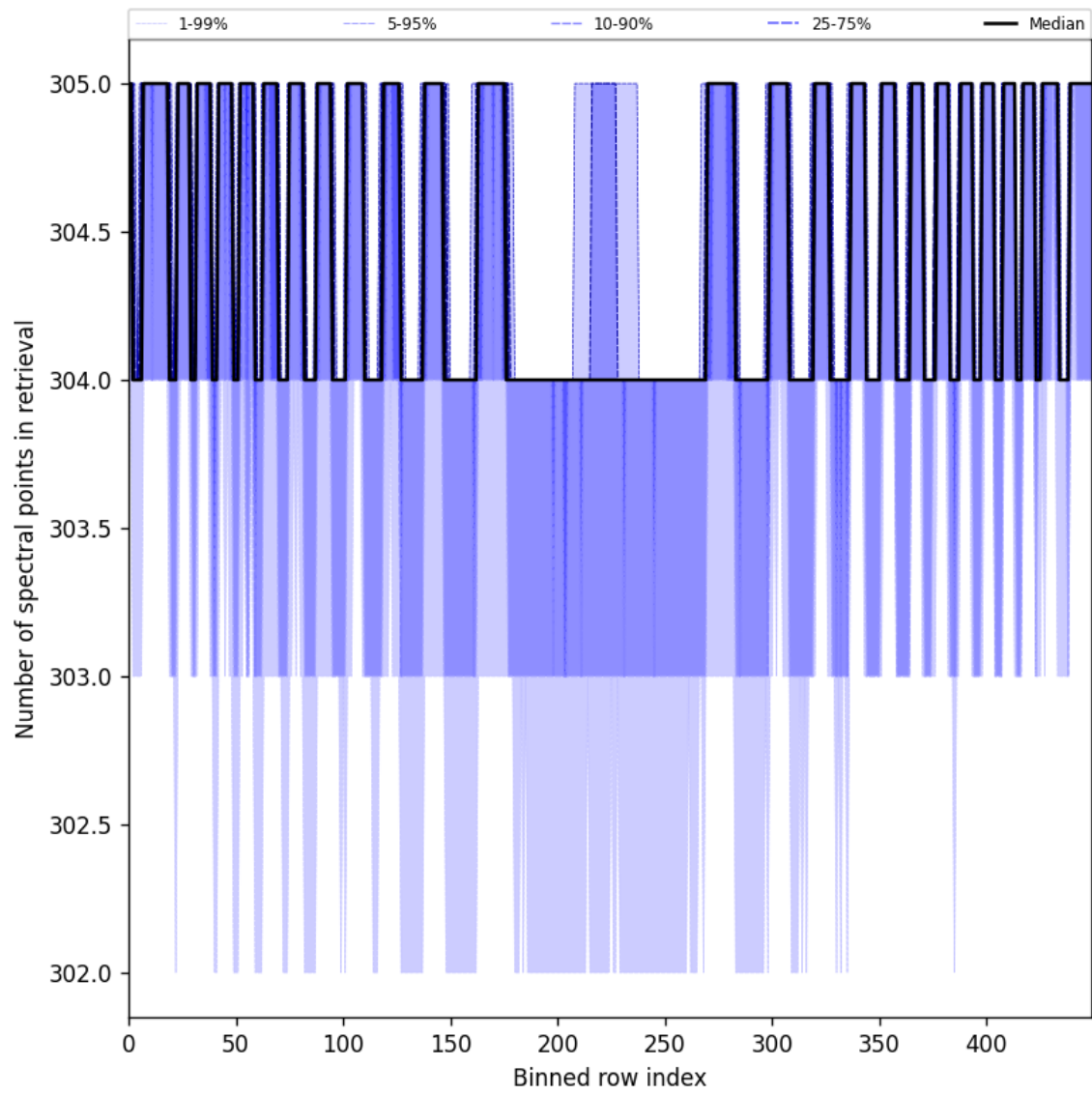
Figure 50: Along track statistics of “Number of spectral points in retrieval” for 2025-06-04 to 2025-06-06
