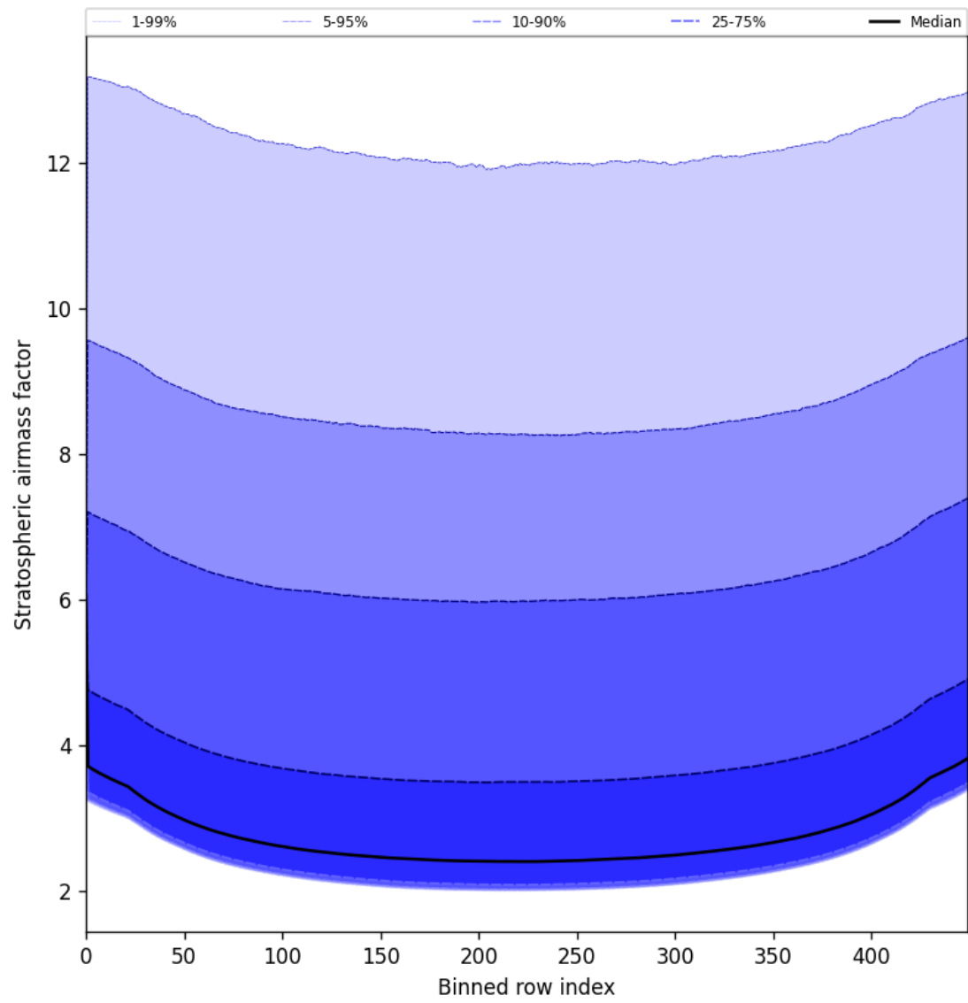
Figure 61: Along track statistics of “Stratospheric airmass factor” for 2025-06-04 to 2025-06-06
