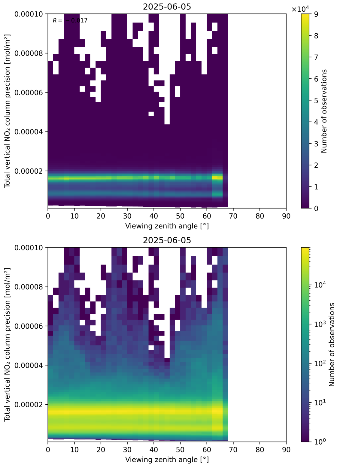
Figure 168: Scatter density plot of “Viewing zenith angle” against “Total vertical NO 2 column precision” for 2025-06-04 to 2025-06-06.
