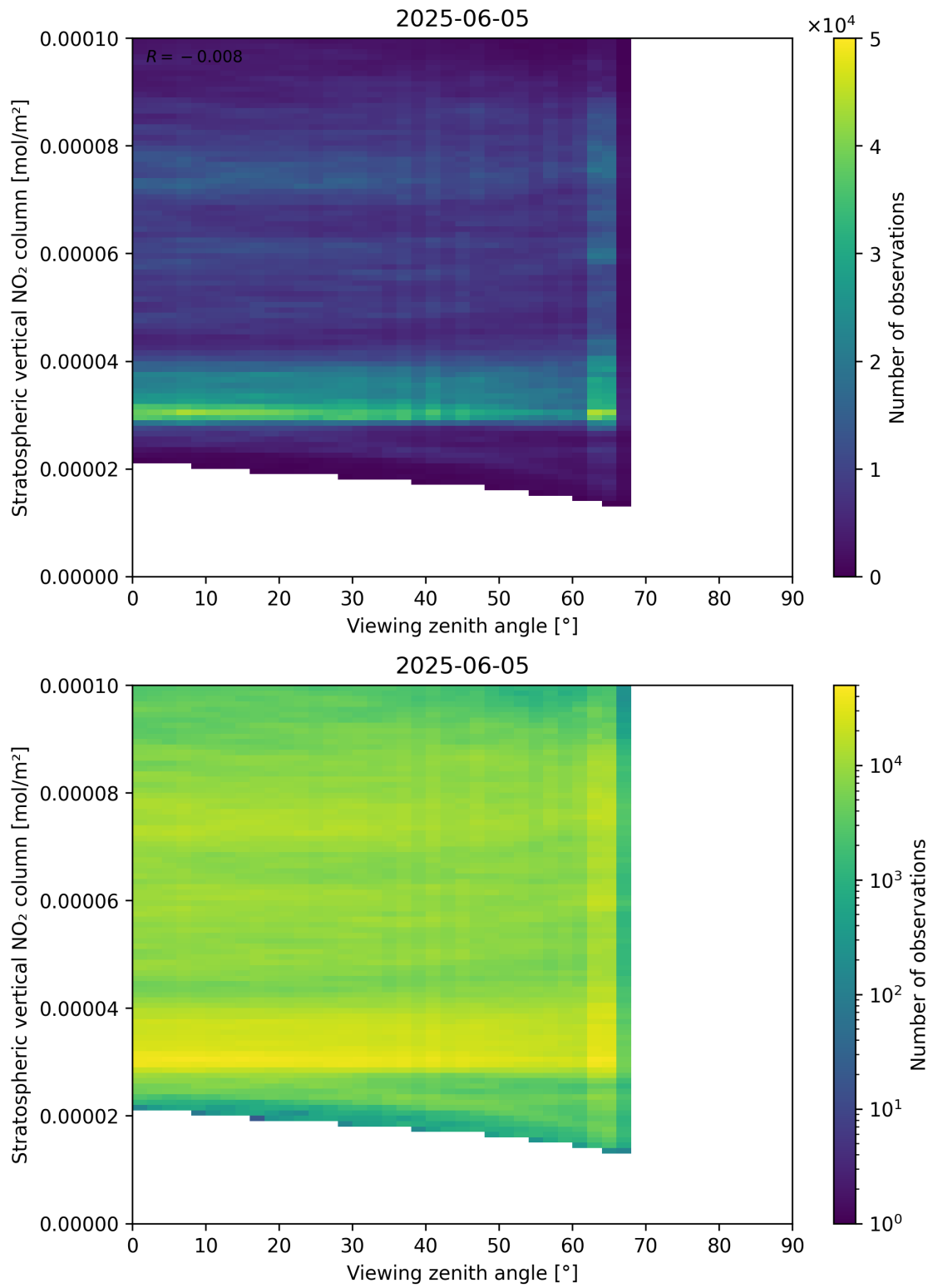
Figure 164: Scatter density plot of “Viewing zenith angle” against “Stratospheric vertical NO 2 column” for 2025-06-04 to 2025-06-06.
