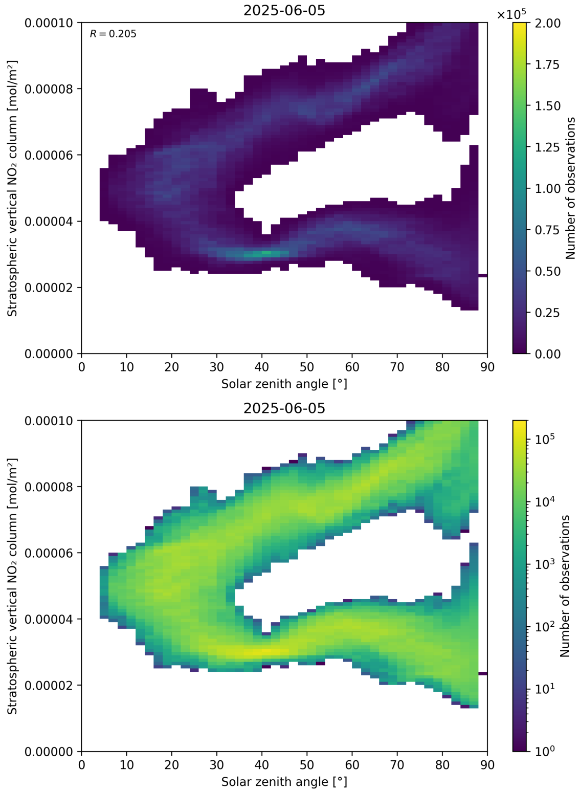
Figure 150: Scatter density plot of “Solar zenith angle” against “Stratospheric vertical NO 2 column” for 2025-06-04 to 2025-06-06.
