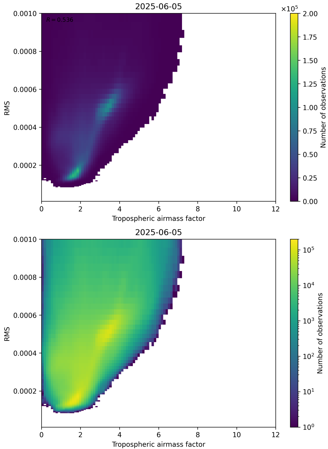
Figure 79: Scatter density plot of “Tropospheric airmass factor” against “RMS” for 2025-06-04 to 2025-06-06.
