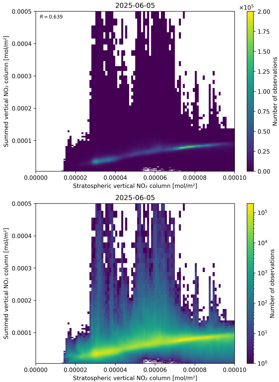
Figure 98: Scatter density plot of “Stratospheric vertical NO 2 column” against “Summed vertical NO 2 column” for 2025-06-04 to 2025-06-06.
