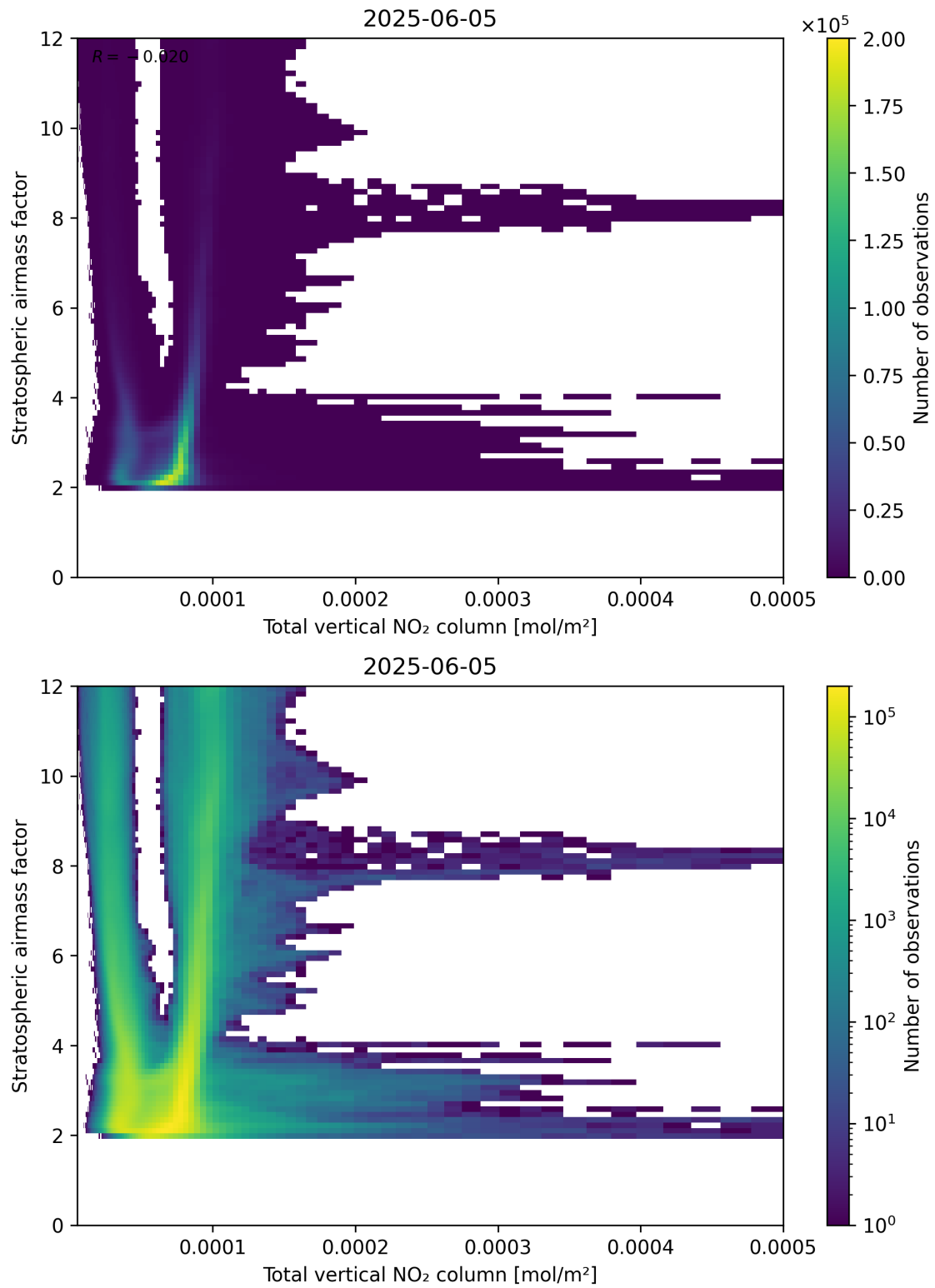
Figure 110: Scatter density plot of “Total vertical NO 2 column” against “Stratospheric airmass factor” for 2025-06-04 to 2025-06-06.
