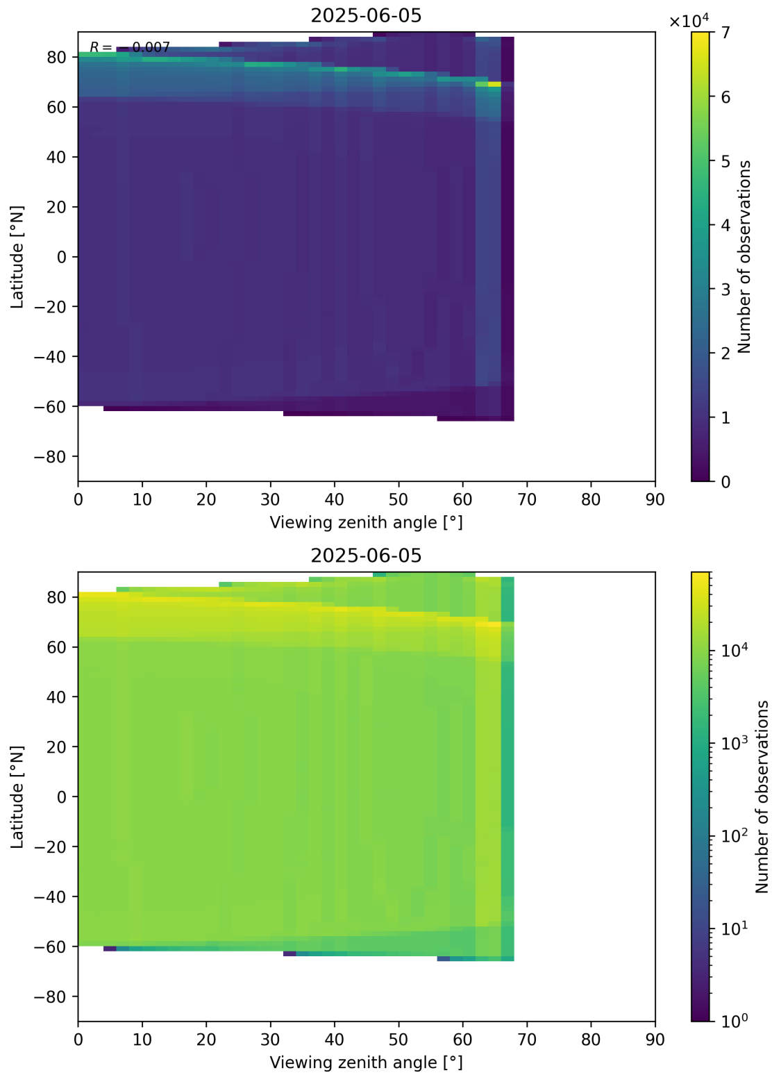
Figure 163: Scatter density plot of “Viewing zenith angle” against “Latitude” for 2025-06-04 to 2025-06-06.
