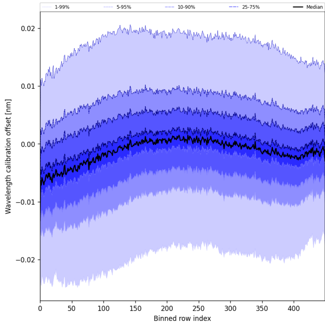
Figure 52: Along track statistics of “Wavelength calibration offset” for 2025-06-04 to 2025-06-06
