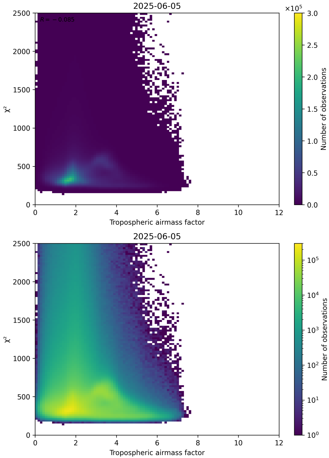
Figure 73: Scatter density plot of “Tropospheric airmass factor” against “ \chi^2 ” for 2025-06-04 to 2025-06-06.
