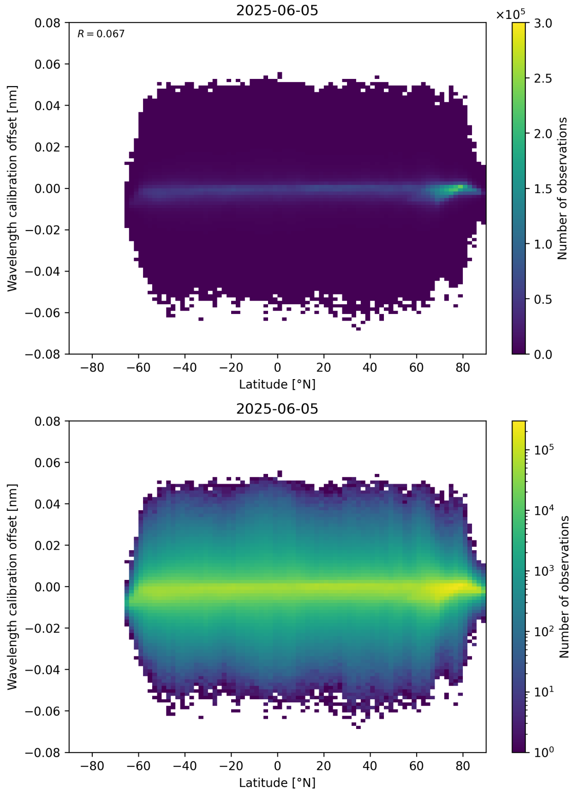
Figure 95: Scatter density plot of “Latitude” against “Wavelength calibration offset” for 2025-06-04 to 2025-06-06.
