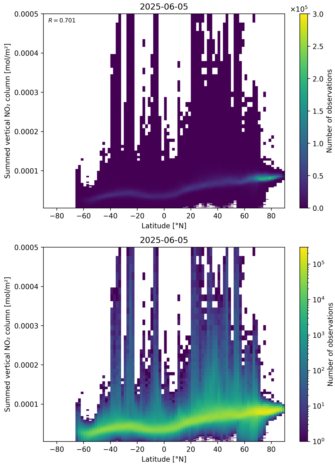
Figure 88: Scatter density plot of “Latitude” against “Summed vertical NO 2 column” for 2025-06-04 to 2025-06-06.
