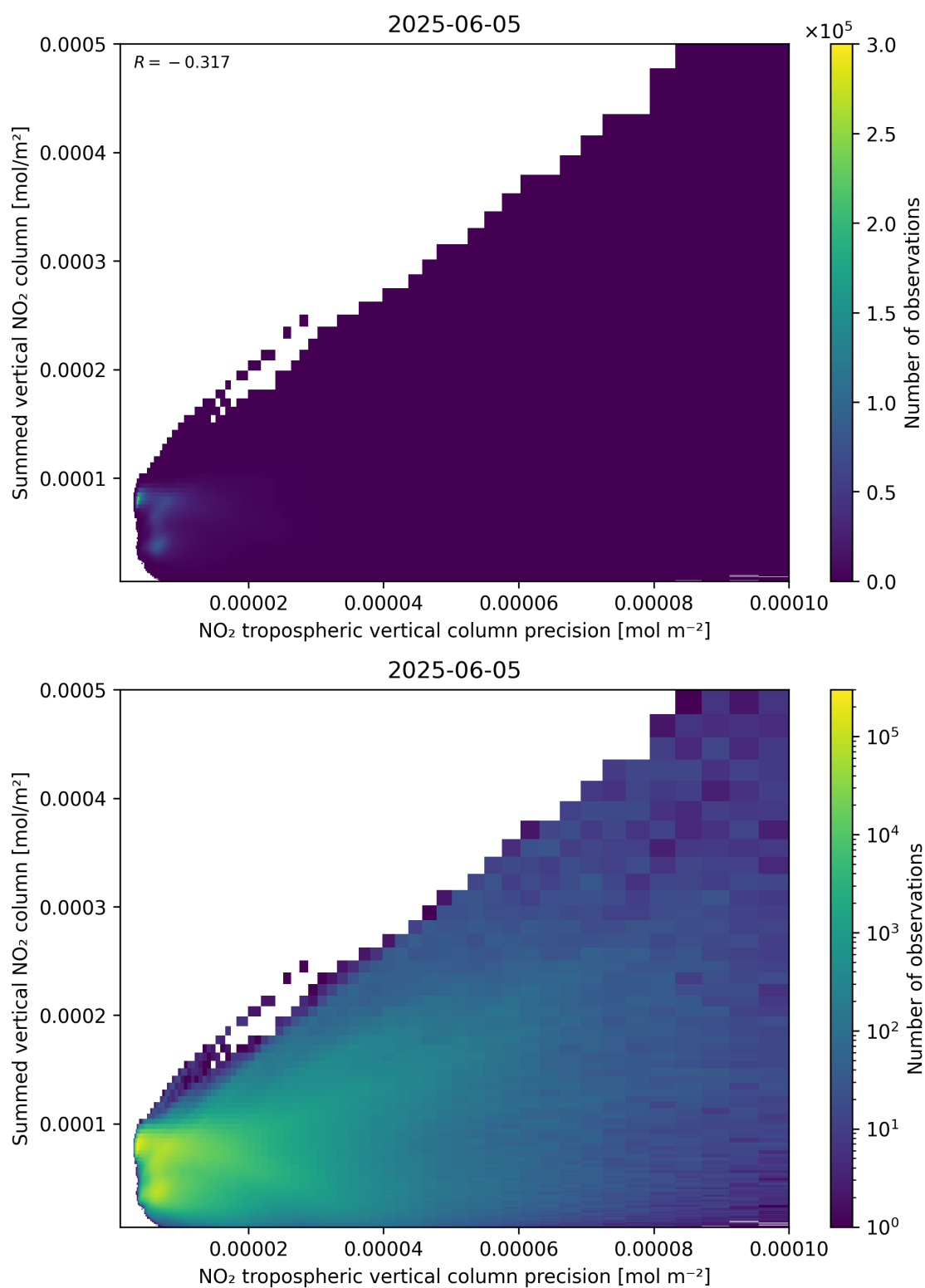
Figure 136: Scatter density plot of “NO 2 tropospheric vertical column precision” against “Summed vertical NO 2 column” for 2025-06-04 to 2025-06-06.
