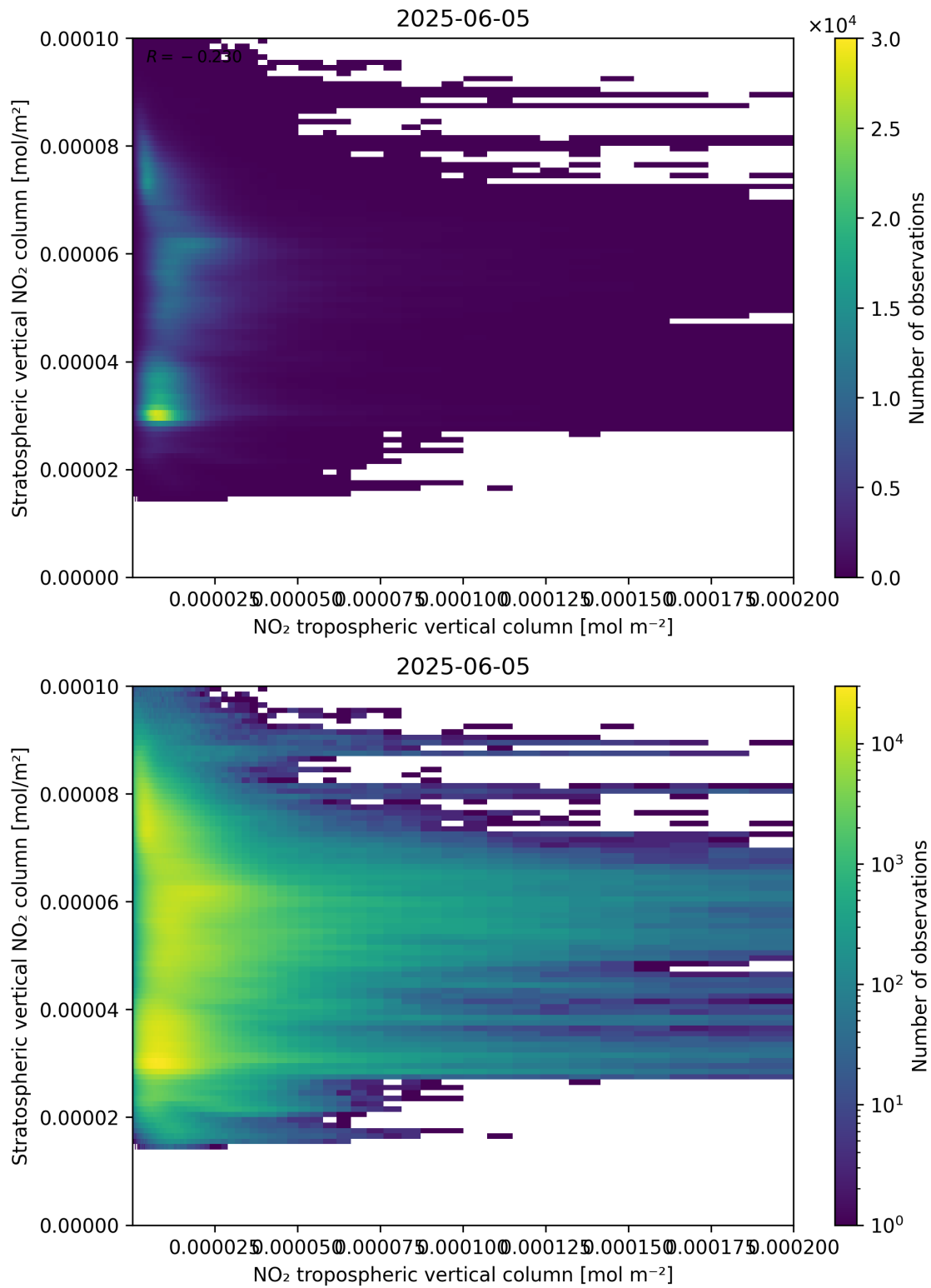
Figure 125: Scatter density plot of “NO 2 tropospheric vertical column” against “Stratospheric vertical NO 2 column” for 2025-06-04 to 2025-06-06.
