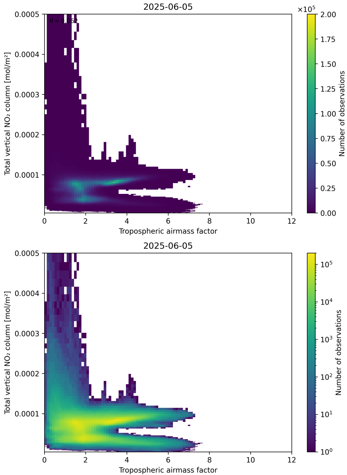
Figure 77: Scatter density plot of “Tropospheric airmass factor” against “Total vertical NO 2 column” for 2025-06-04 to 2025-06-06.
