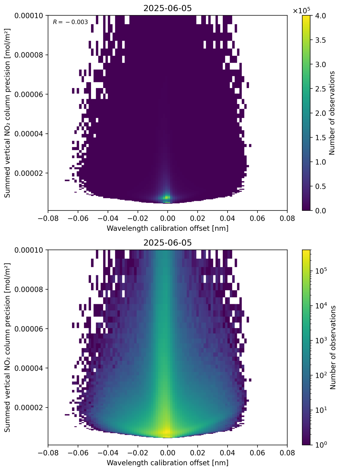
Figure 178: Scatter density plot of “Wavelength calibration offset” against “Summed vertical NO 2 column precision” for 2025-06-04 to 2025-06-06.
