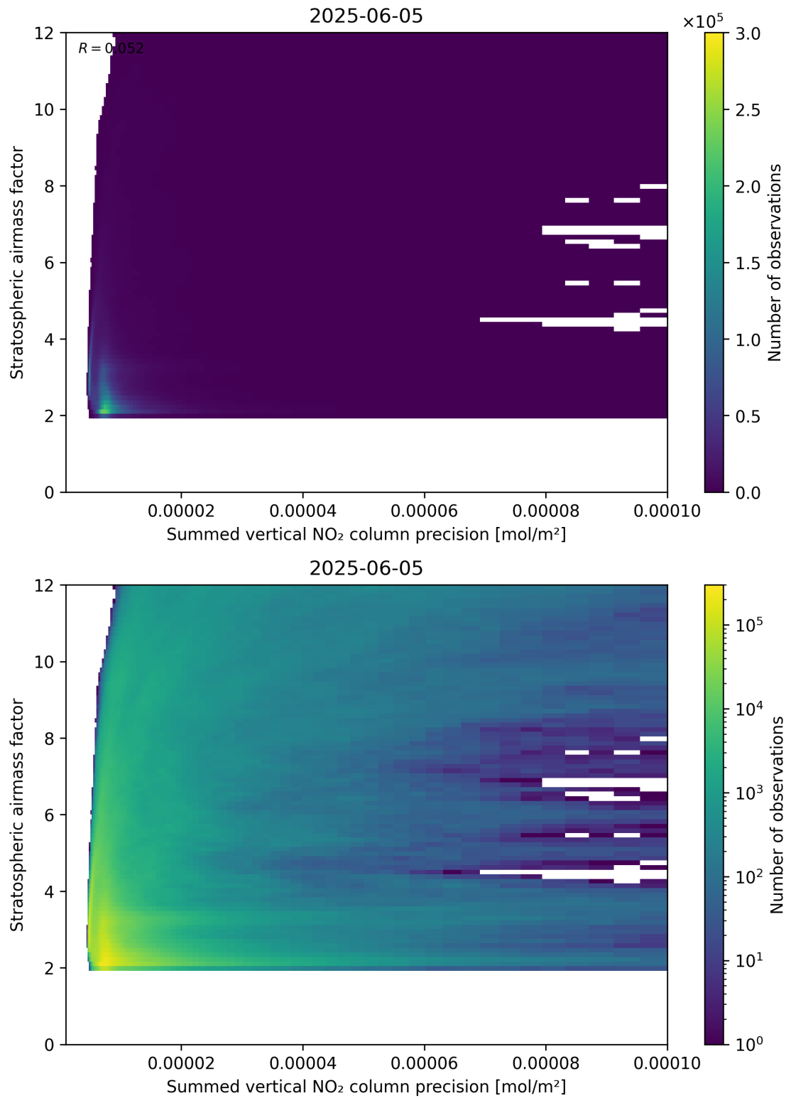
Figure 106: Scatter density plot of “Summed vertical NO 2 column precision” against “Stratospheric airmass factor” for 2025-06-04 to 2025-06-06.
