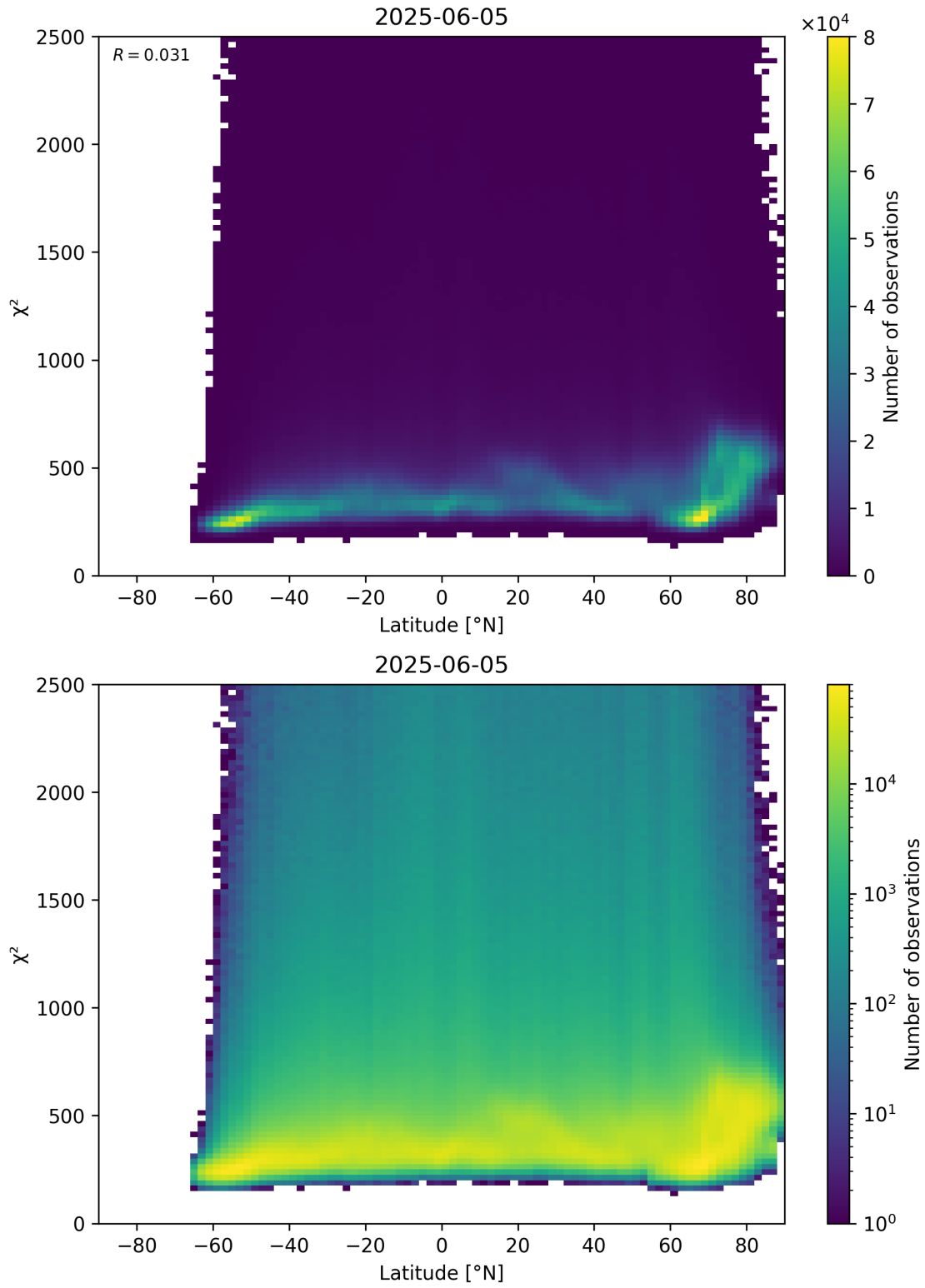
Figure 86: Scatter density plot of “Latitude” against “ \chi^2 ” for 2025-06-04 to 2025-06-06.
