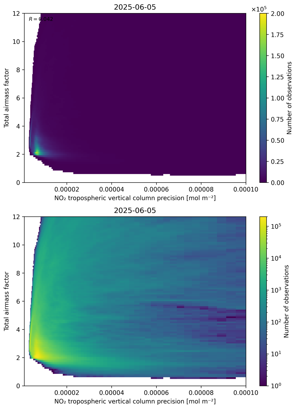
Figure 132: Scatter density plot of “NO 2 tropospheric vertical column precision” against “Total air mass factor” for 2025-06-04 to 2025-06-06.
