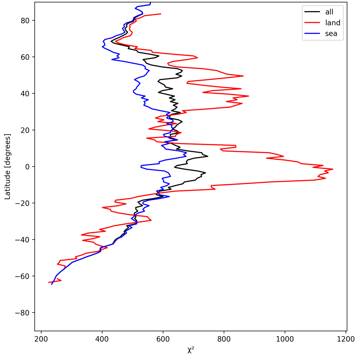
Figure 25: Zonal average of “ \chi^2 ” for 2025-06-04 to 2025-06-06.
