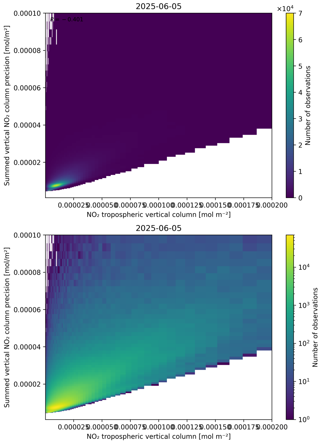
Figure 127: Scatter density plot of “NO 2 tropospheric vertical column” against “Summed vertical NO 2 column precision” for 2025-06-04 to 2025-06-06.
