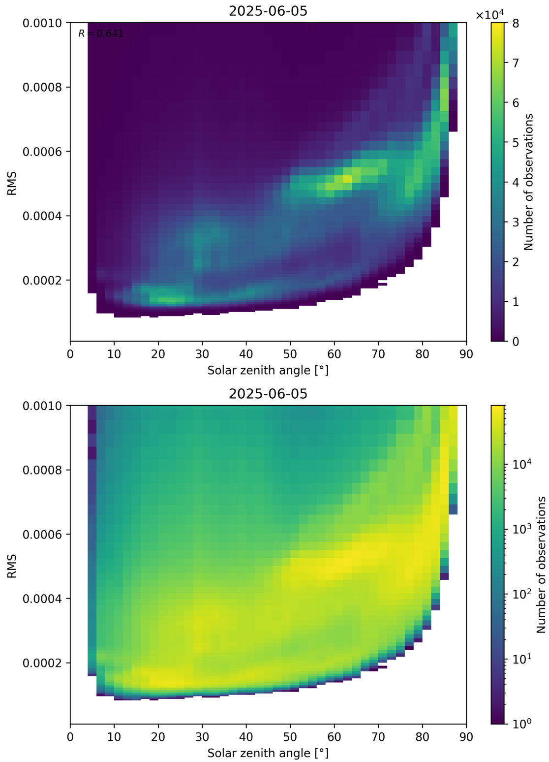
Figure 157: Scatter density plot of “Solar zenith angle” against “RMS” for 2025-06-04 to 2025-06-06.
