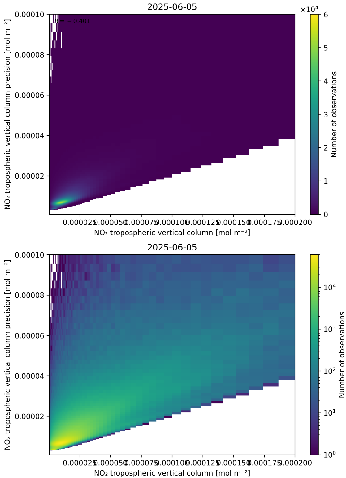
Figure 130: Scatter density plot of “NO 2 tropospheric vertical column” against “NO 2 tropospheric vertical column precision” for 2025-06-04 to 2025-06-06.
