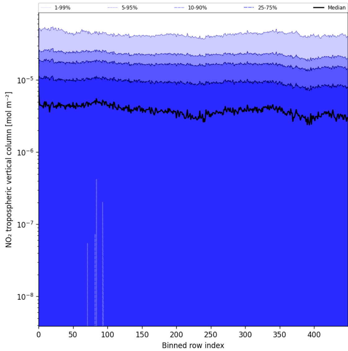
Figure 46: Along track statistics of “NO 2 tropospheric vertical column” for 2025-06-04 to 2025-06-06
