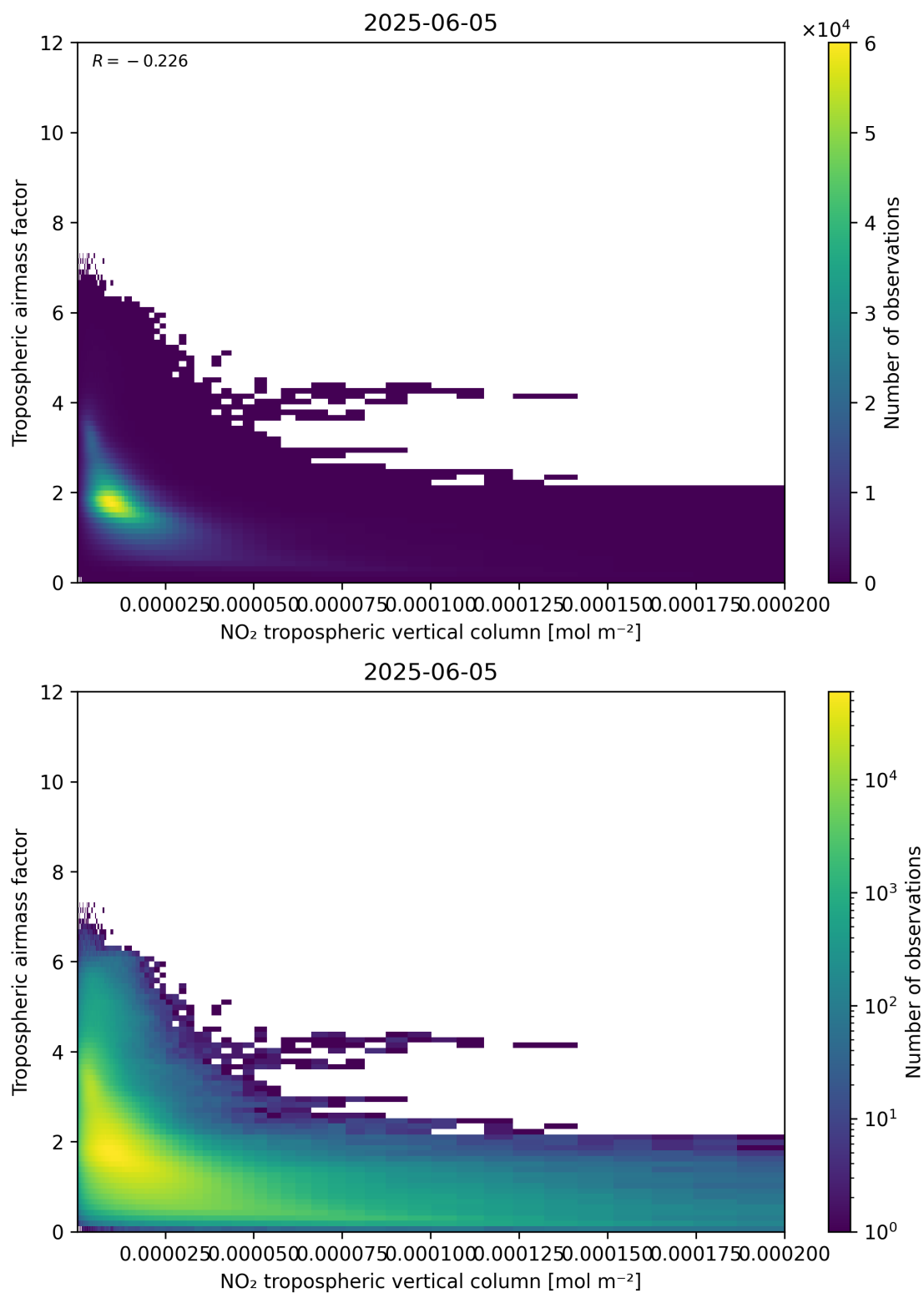
Figure 123: Scatter density plot of “NO 2 tropospheric vertical column” against “Tropospheric air mass factor” for 2025-06-04 to 2025-06-06.
