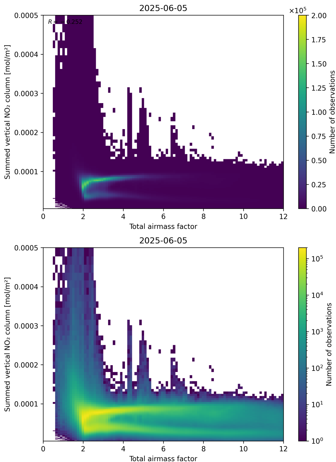
Figure 65: Scatter density plot of “Total airmass factor” against “Summed vertical NO 2 column” for 2025-06-04 to 2025-06-06.
