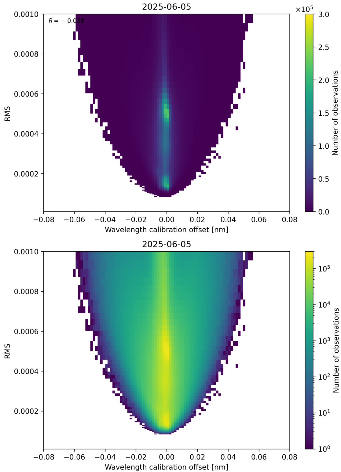
Figure 181: Scatter density plot of “Wavelength calibration offset” against “RMS” for 2025-06-04 to 2025-06-06.
