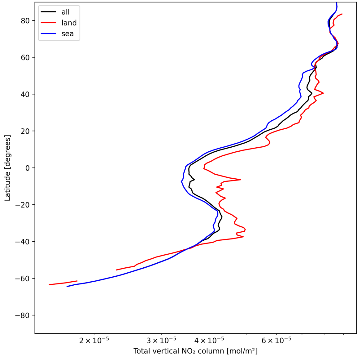
Figure 21: Zonal average of “Total vertical NO 2 column” for 2025-06-04 to 2025-06-06.
