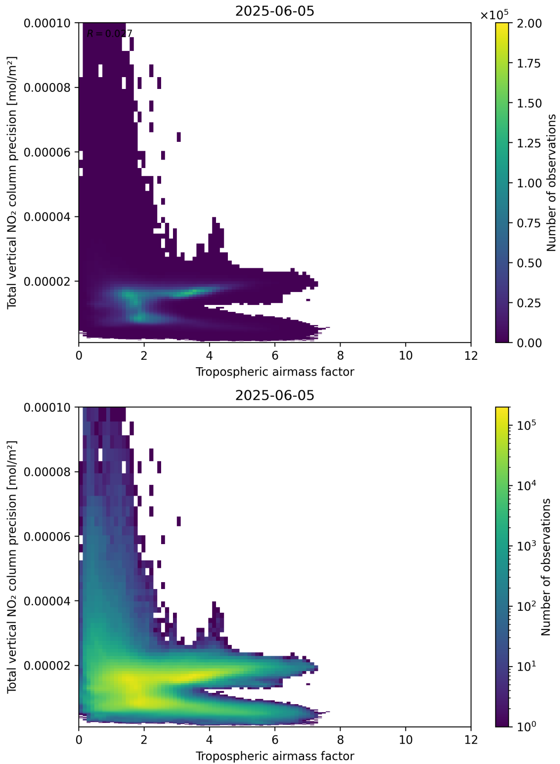
Figure 78: Scatter density plot of “Tropospheric airmass factor” against “Total vertical NO 2 column precision” for 2025-06-04 to 2025-06-06.
