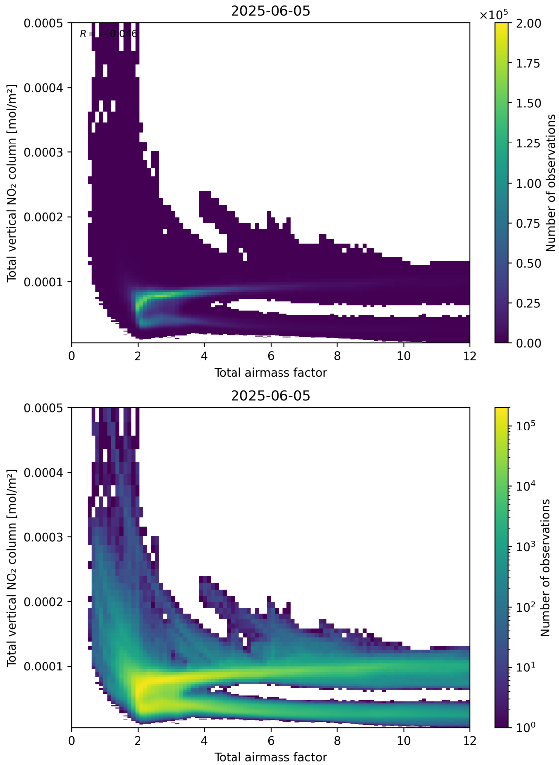
Figure 67: Scatter density plot of “Total airmass factor” against “Total vertical NO 2 column” for 2025-06-04 to 2025-06-06.
