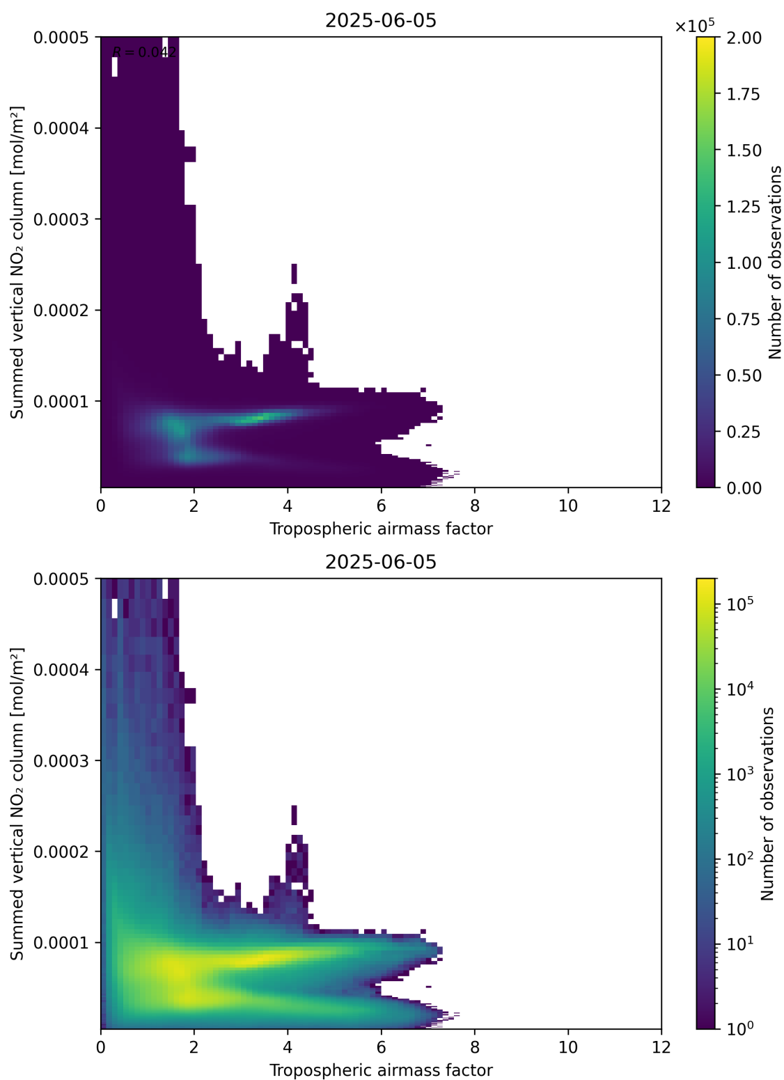
Figure 75: Scatter density plot of “Tropospheric airmass factor” against “Summed vertical NO 2 column” for 2025-06-04 to 2025-06-06.
