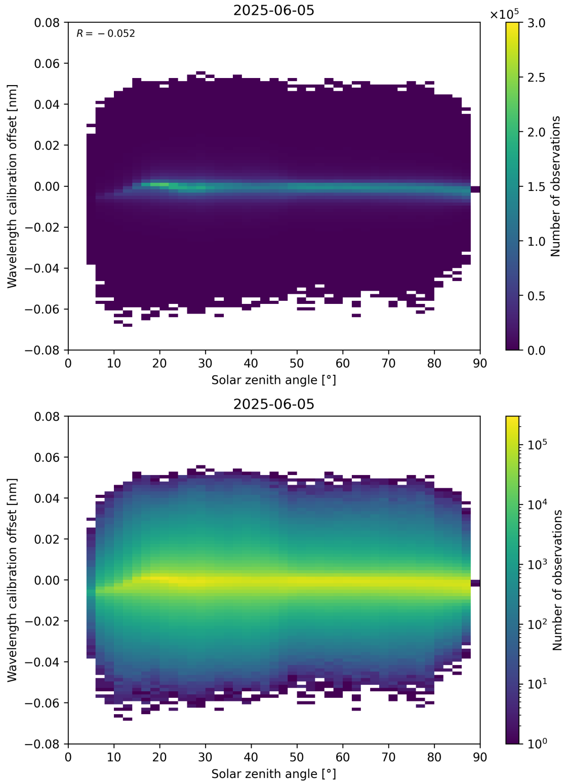
Figure 158: Scatter density plot of “Solar zenith angle” against “Wavelength calibration offset” for 2025-06-04 to 2025-06-06.
