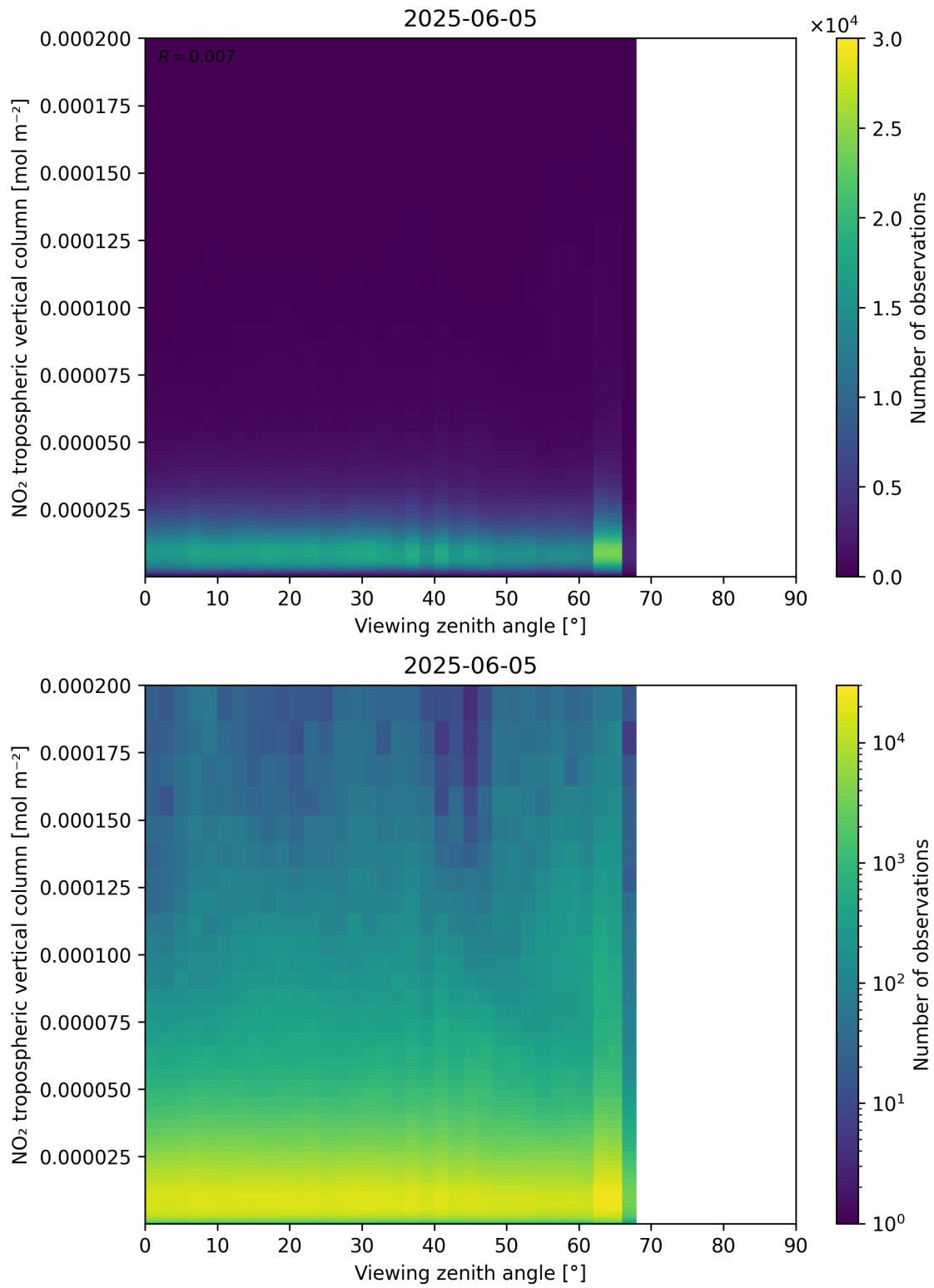
Figure 169: Scatter density plot of “Viewing zenith angle” against “NO 2 tropospheric vertical column” for 2025-06-04 to 2025-06-06.
