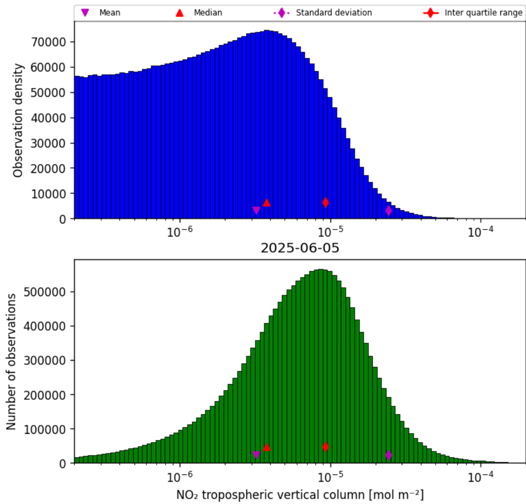
Figure 29: Histogram of “NO 2 tropospheric vertical column” for 2025-06-04 to 2025-06-06
