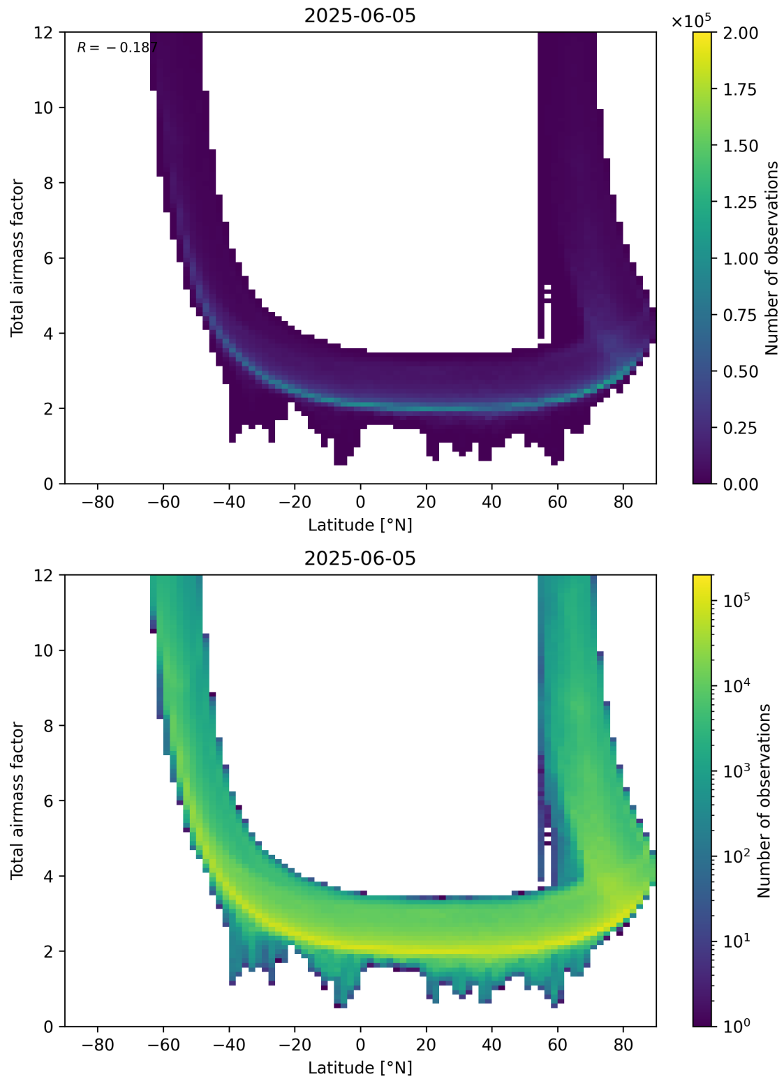
Figure 84: Scatter density plot of “Latitude” against “Total airmass factor” for 2025-06-04 to 2025-06-06.
