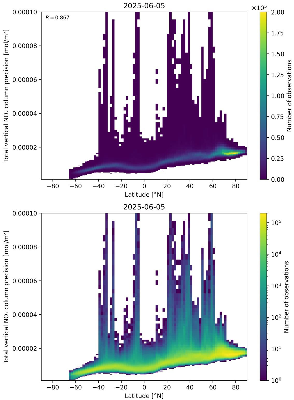
Figure 91: Scatter density plot of “Latitude” against “Total vertical NO 2 column precision” for 2025-06-04 to 2025-06-06.
