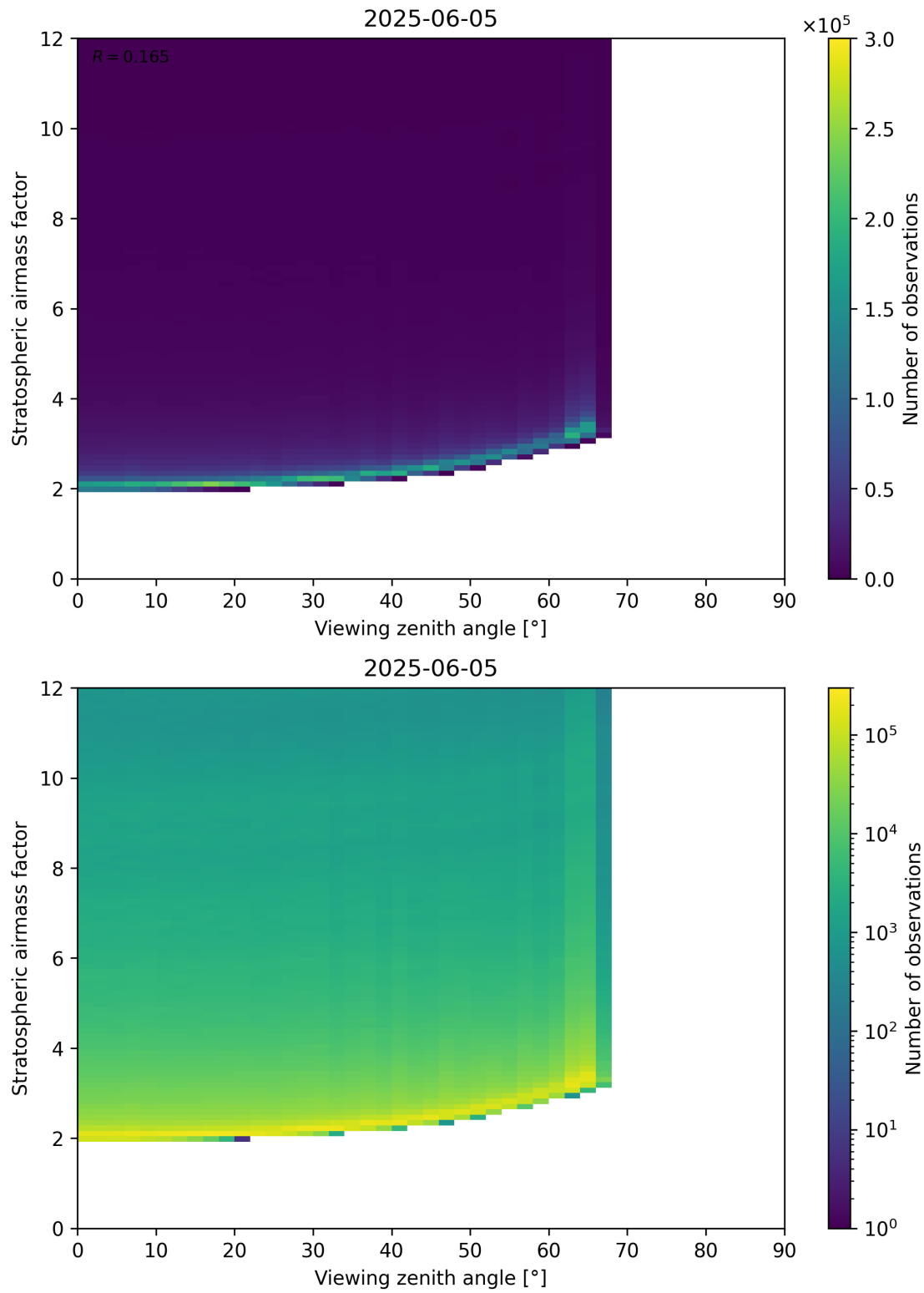
Figure 159: Scatter density plot of “Viewing zenith angle” against “Stratospheric airmass factor” for 2025-06-04 to 2025-06-06.
