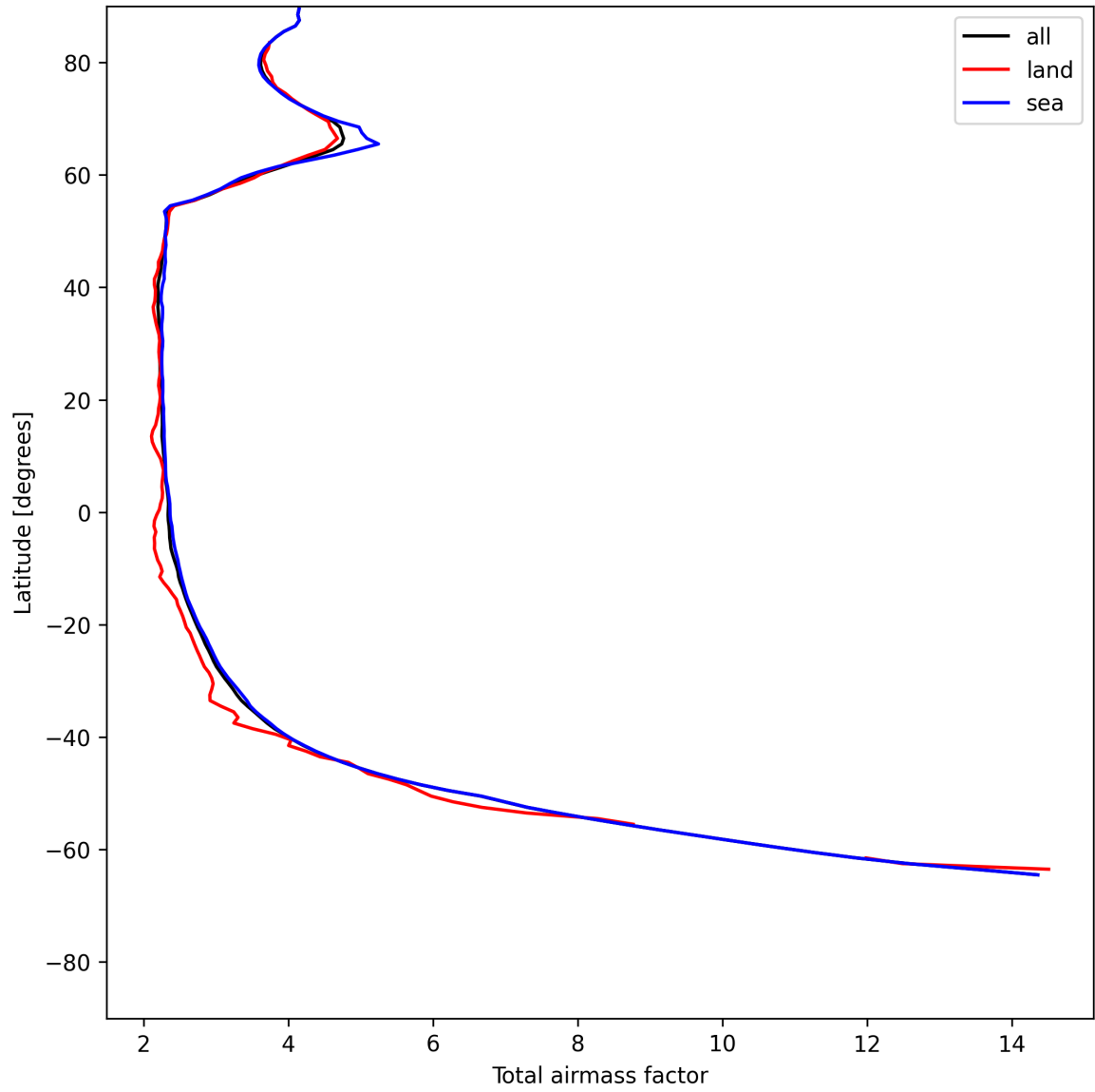
Figure 15: Zonal average of “Total airmass factor” for 2025-06-04 to 2025-06-06.
