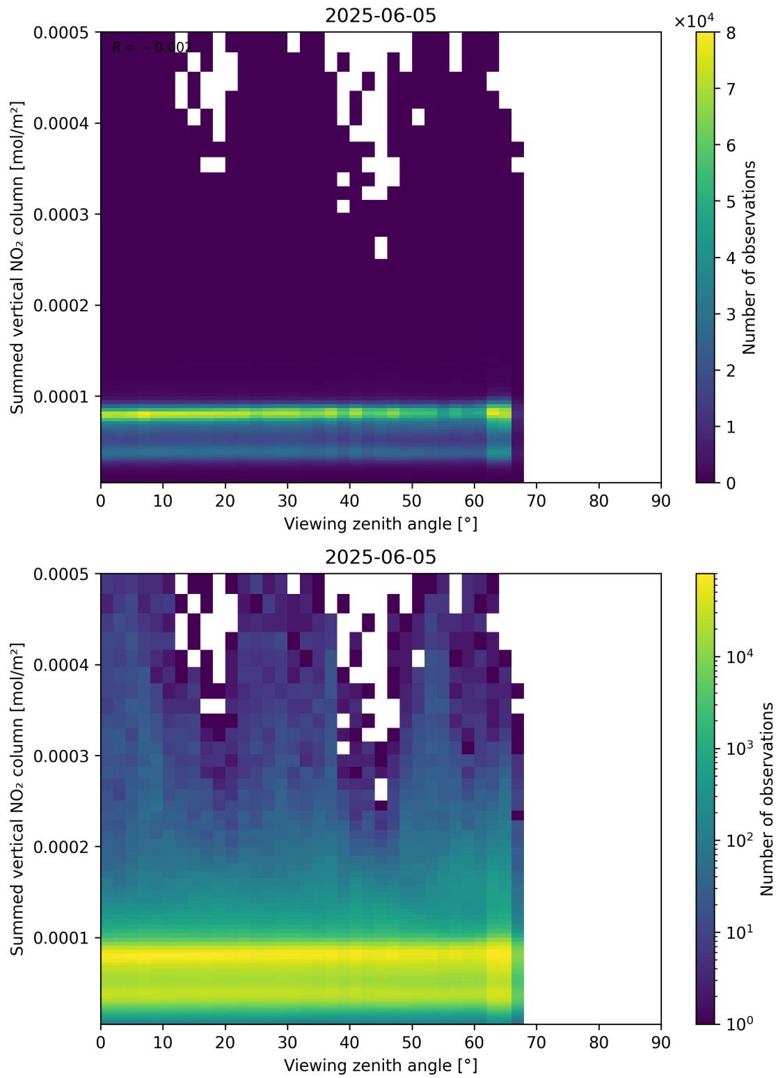
Figure 165: Scatter density plot of “Viewing zenith angle” against “Summed vertical NO 2 column” for 2025-06-04 to 2025-06-06.
