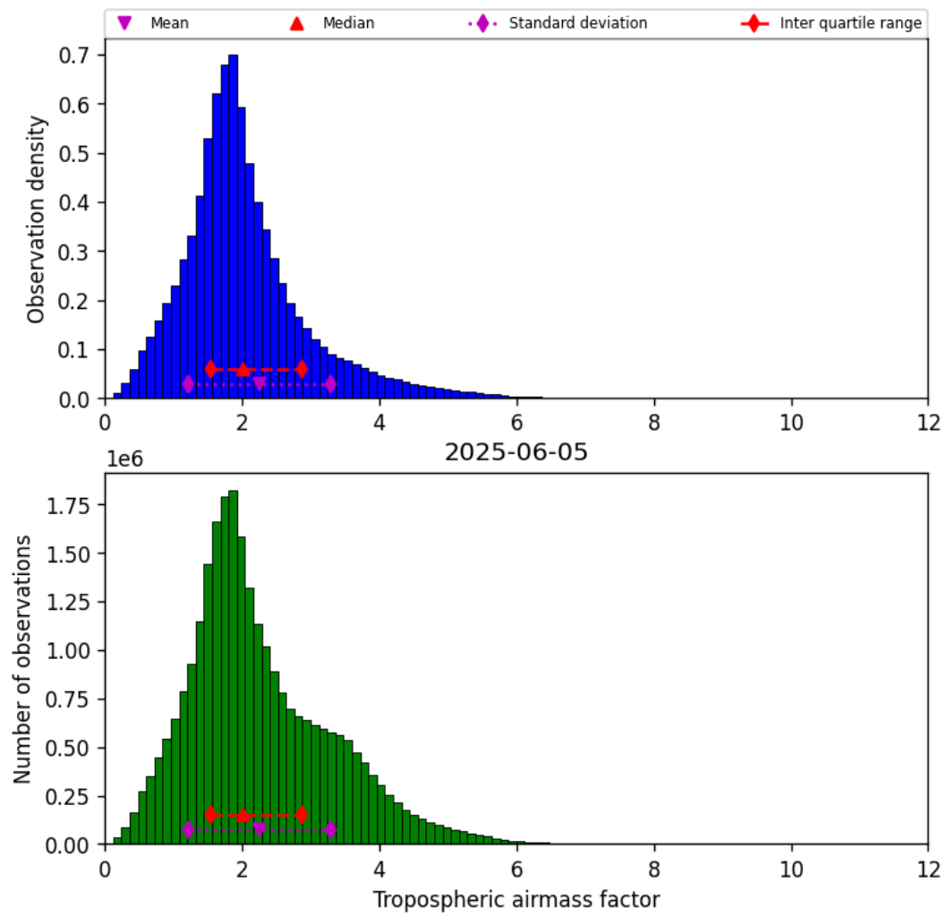
Figure 31: Histogram of “Tropospheric airmass factor” for 2025-06-04 to 2025-06-06
