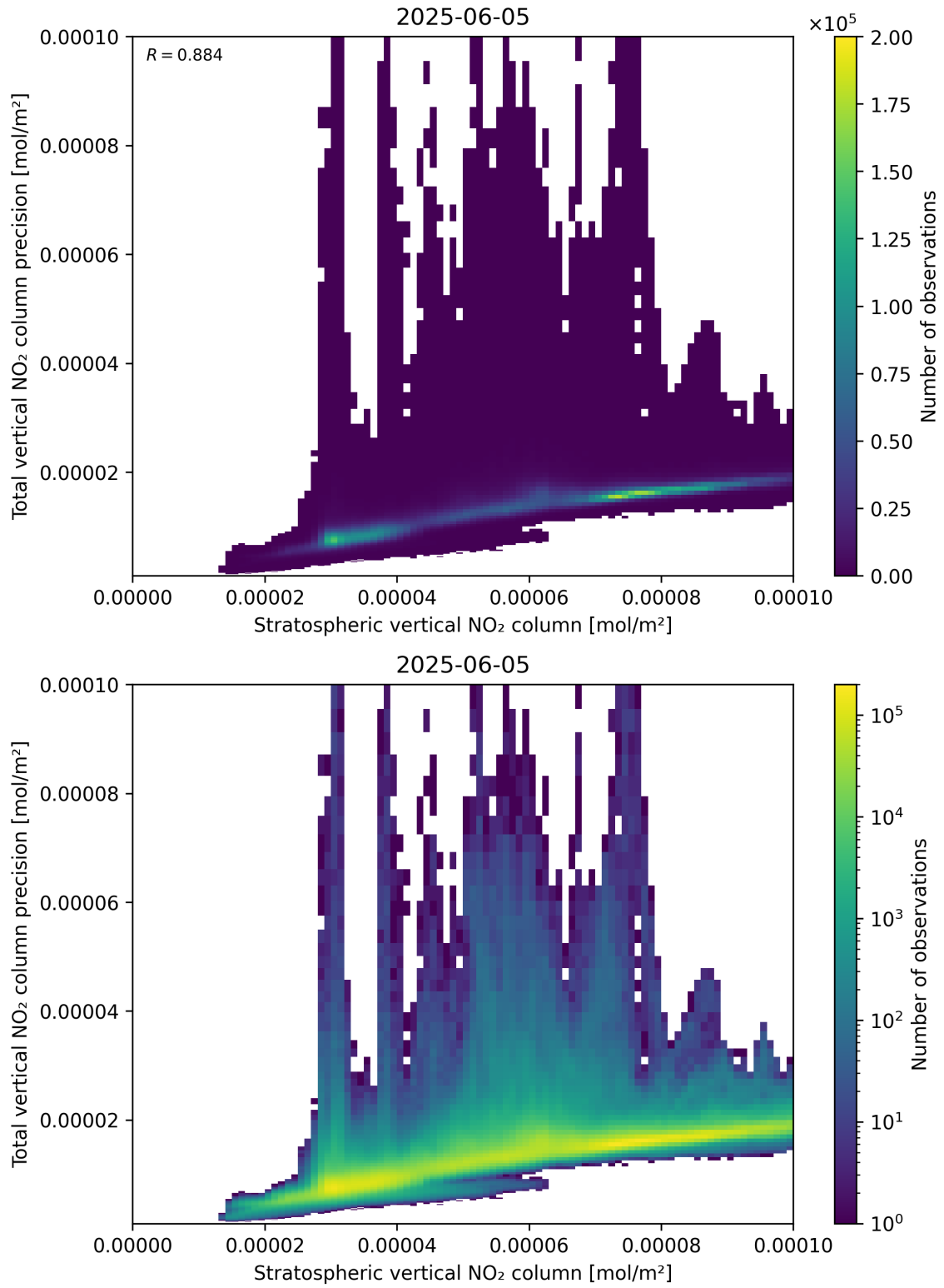
Figure 101: Scatter density plot of “Stratospheric vertical NO 2 column” against “Total vertical NO 2 column precision” for 2025-06-04 to 2025-06-06.
