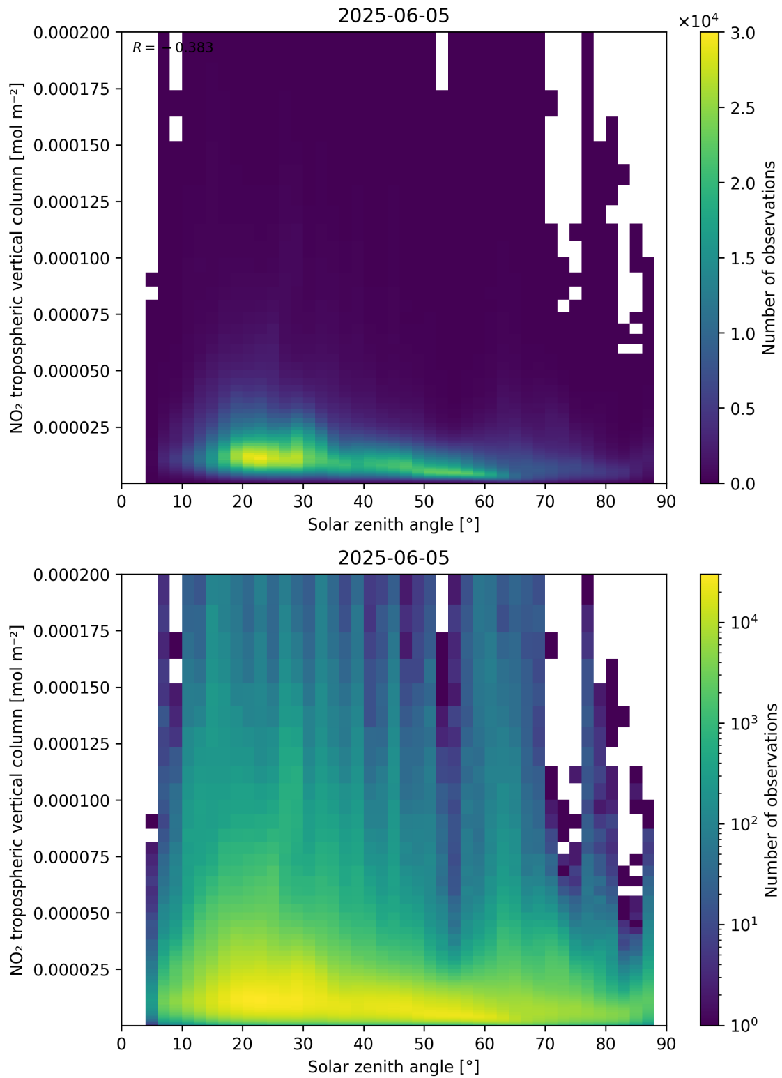
Figure 155: Scatter density plot of “Solar zenith angle” against “NO 2 tropospheric vertical column” for 2025-06-04 to 2025-06-06.
