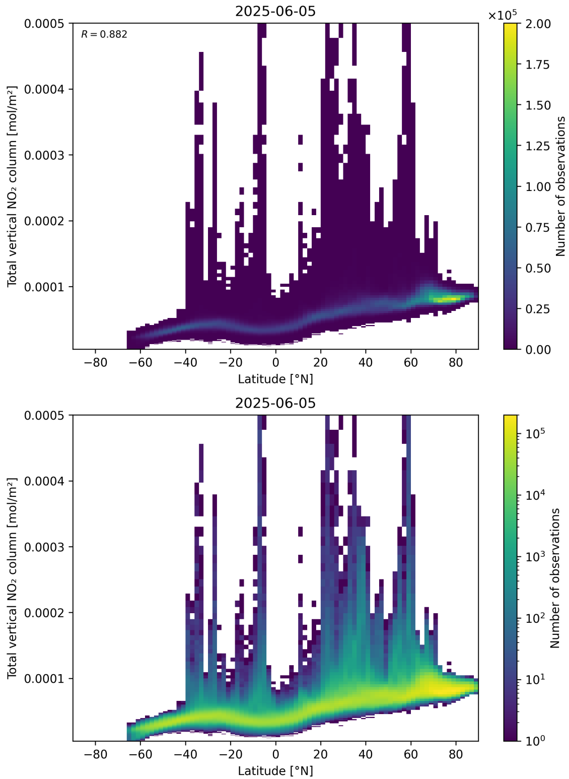
Figure 90: Scatter density plot of “Latitude” against “Total vertical NO 2 column” for 2025-06-04 to 2025-06-06.
