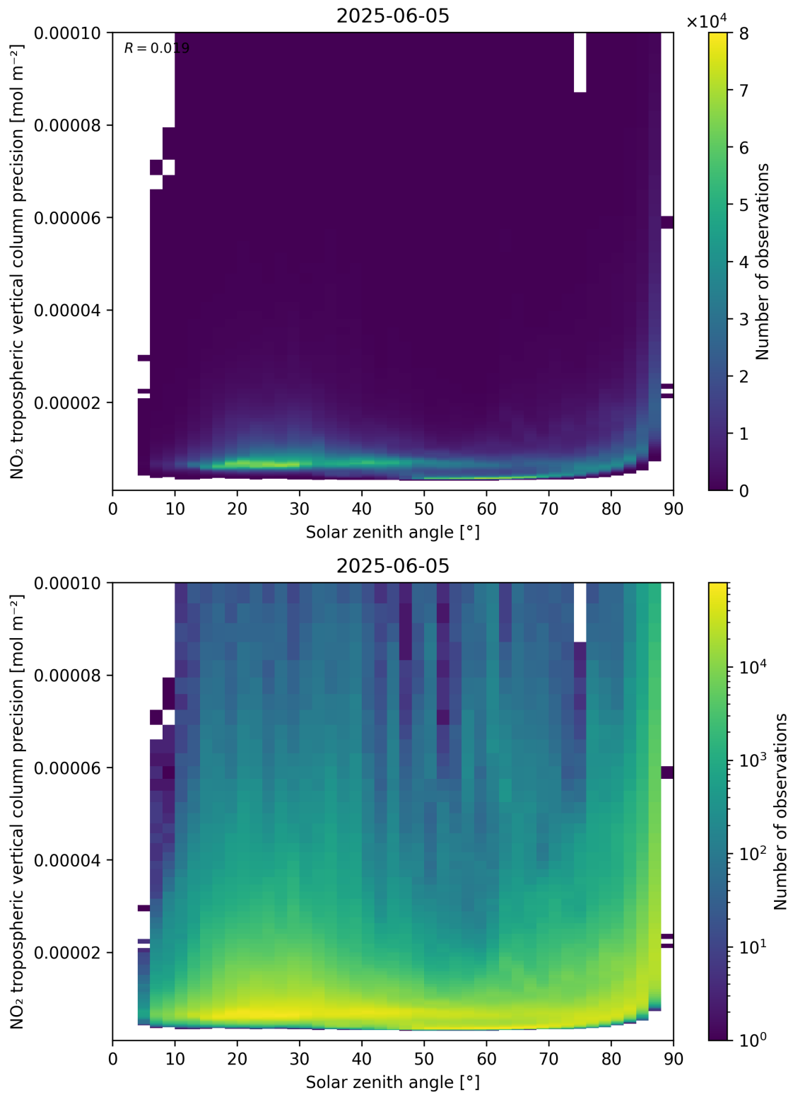
Figure 156: Scatter density plot of “Solar zenith angle” against “NO 2 tropospheric vertical column precision” for 2025-06-04 to 2025-06-06.
