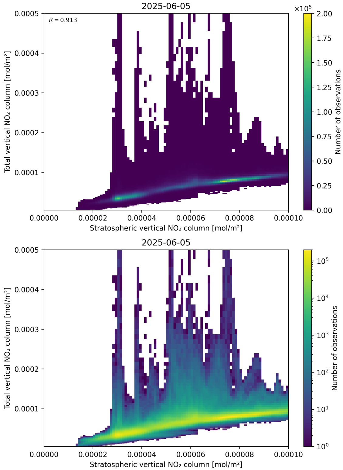
Figure 100: Scatter density plot of “Stratospheric vertical NO 2 column” against “Total vertical NO 2 column” for 2025-06-04 to 2025-06-06.
