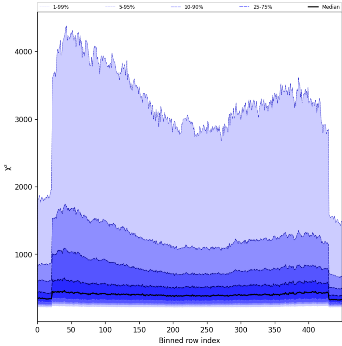
Figure 59: Along track statistics of “ \chi^2 ” for 2025-06-04 to 2025-06-06
