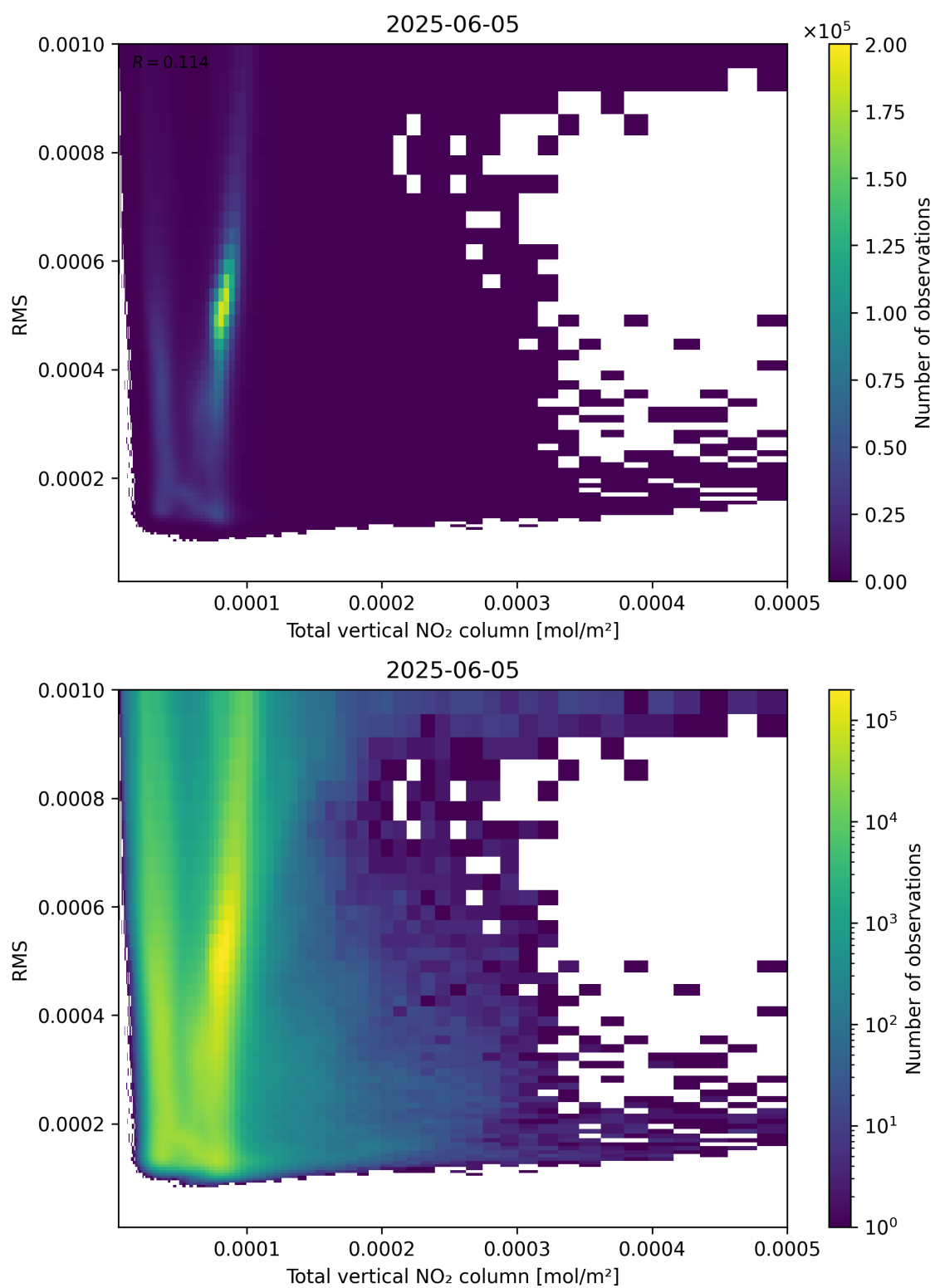
Figure 120: Scatter density plot of “Total vertical NO 2 column” against “RMS” for 2025-06-04 to 2025-06-06.
