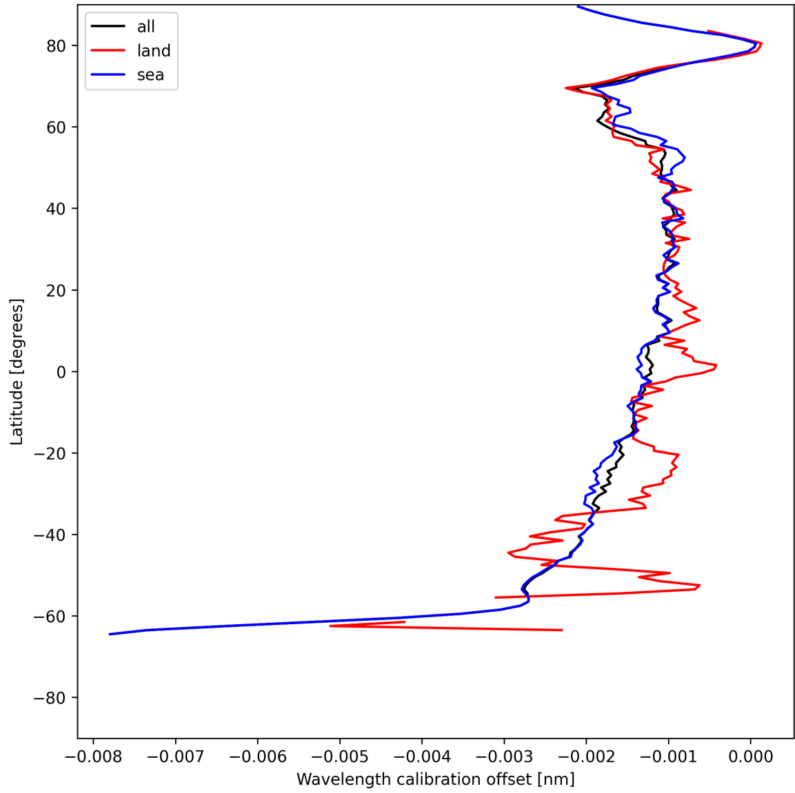
Figure 18: Zonal average of “Wavelength calibration offset” for 2025-06-04 to 2025-06-06.
