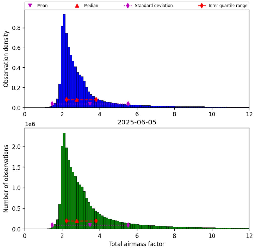
Figure 32: Histogram of “Total airmass factor” for 2025-06-04 to 2025-06-06
