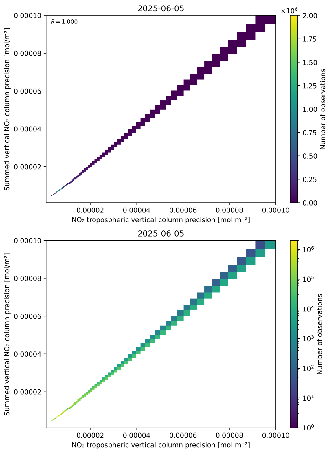
Figure 137: Scatter density plot of “NO 2 tropospheric vertical column precision” against “Summed vertical NO 2 column precision” for 2025-06-04 to 2025-06-06.
