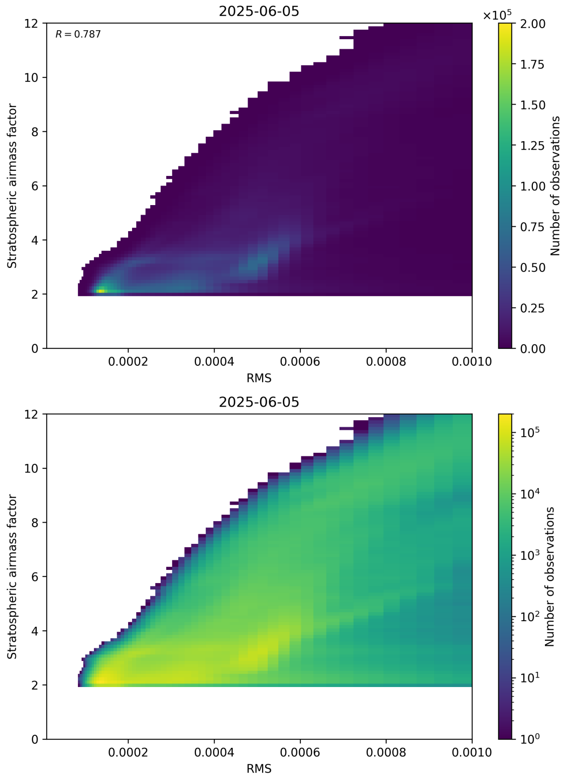
Figure 144: Scatter density plot of “RMS” against “Stratospheric airmass factor” for 2025-06-04 to 2025-06-06.
