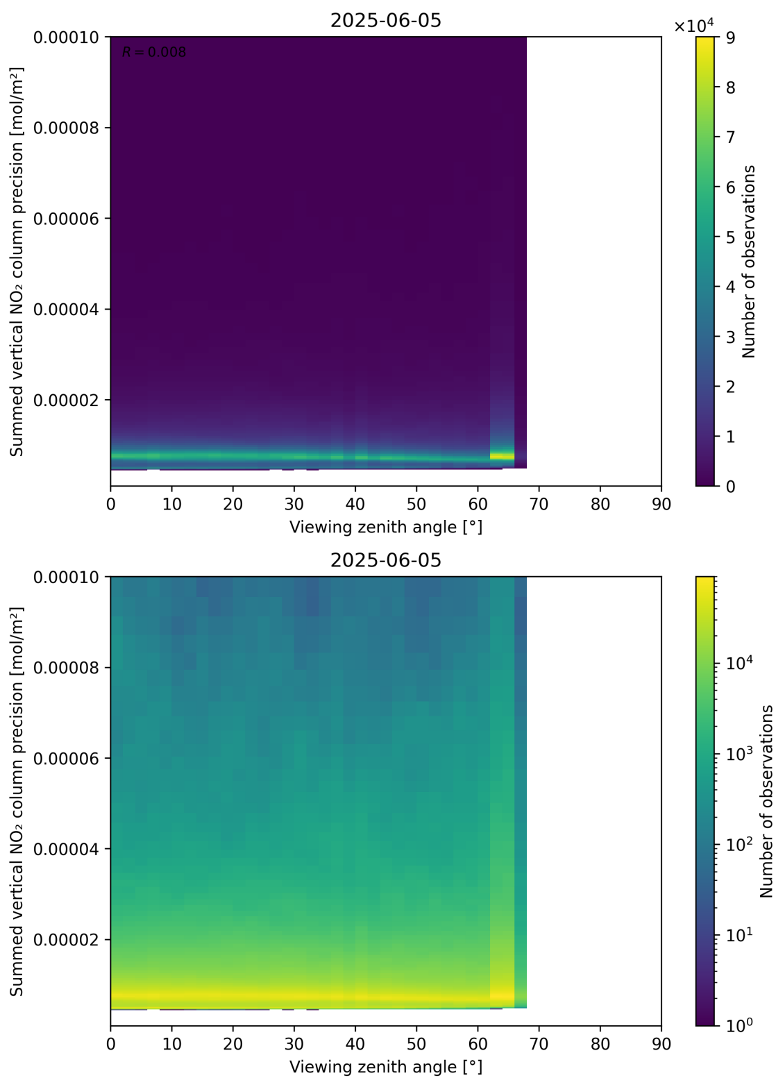
Figure 166: Scatter density plot of “Viewing zenith angle” against “Summed vertical NO 2 column precision” for 2025-06-04 to 2025-06-06.
