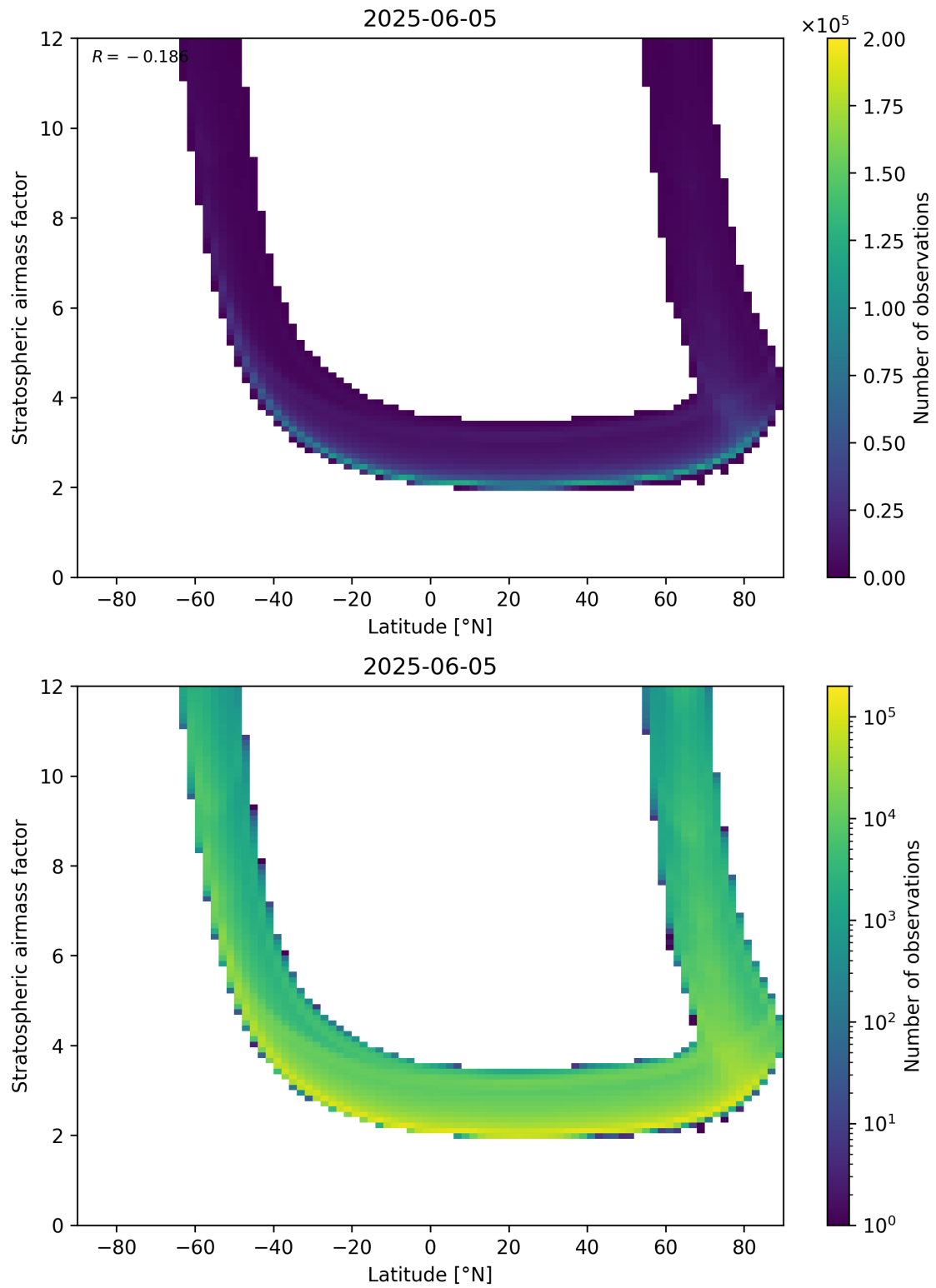
Figure 83: Scatter density plot of “Latitude” against “Stratospheric air mass factor” for 2025-06-04 to 2025-06-06.
