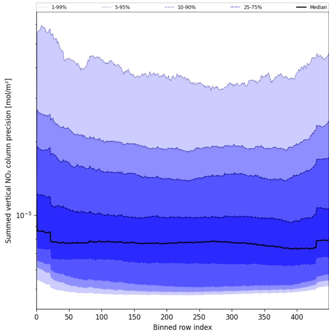
Figure 58: Along track statistics of “Summed vertical NO 2 column precision” for 2025-06-04 to 2025-06-06
