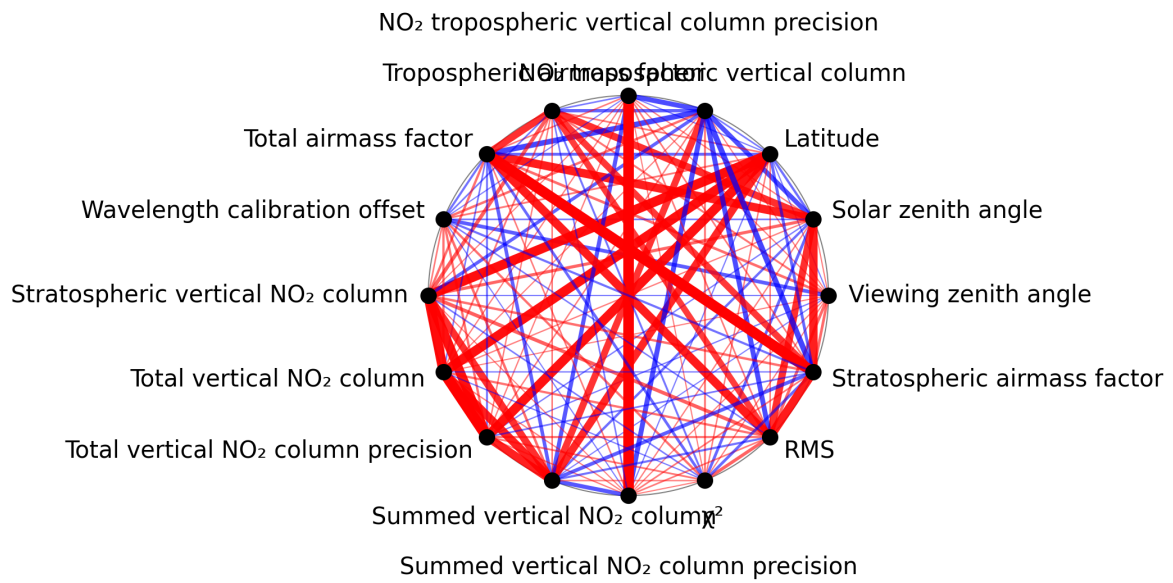
Figure 1: Map of correlation graph for 2025-06-04 to 2025-06-06.
