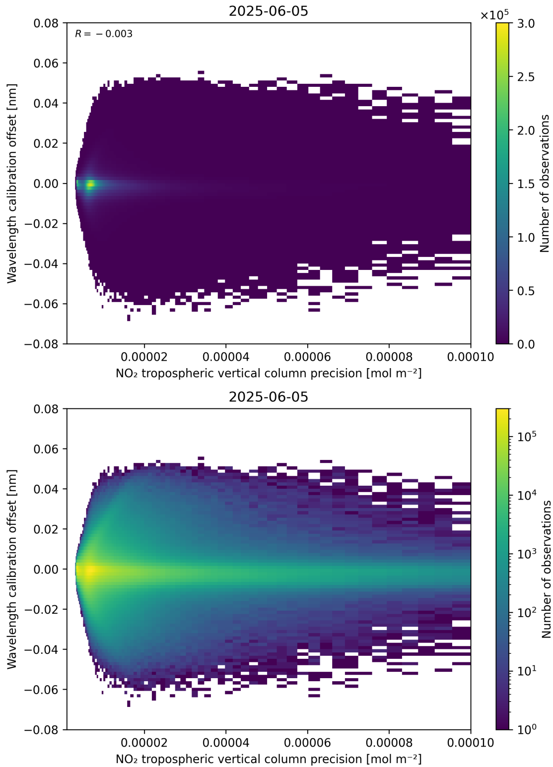
Figure 141: Scatter density plot of “NO 2 tropospheric vertical column precision” against “Wavelength calibration offset” for 2025-06-04 to 2025-06-06.
