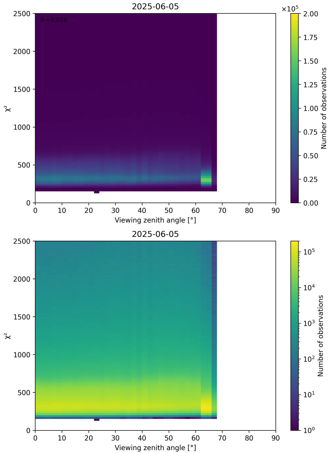
Figure 162: Scatter density plot of “Viewing zenith angle” against “ \chi^2 ” for 2025-06-04 to 2025-06-06.
