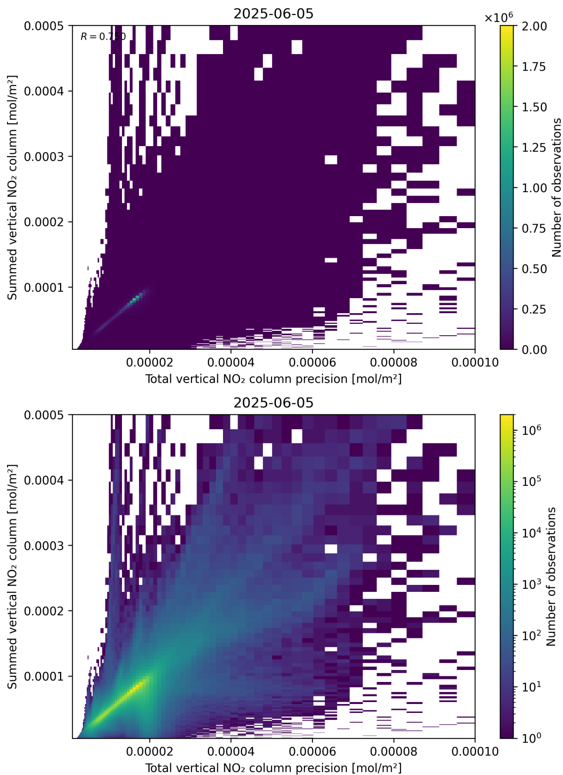
Figure 117: Scatter density plot of “Total vertical NO 2 column precision” against “Summed vertical NO 2 column” for 2025-06-04 to 2025-06-06.
