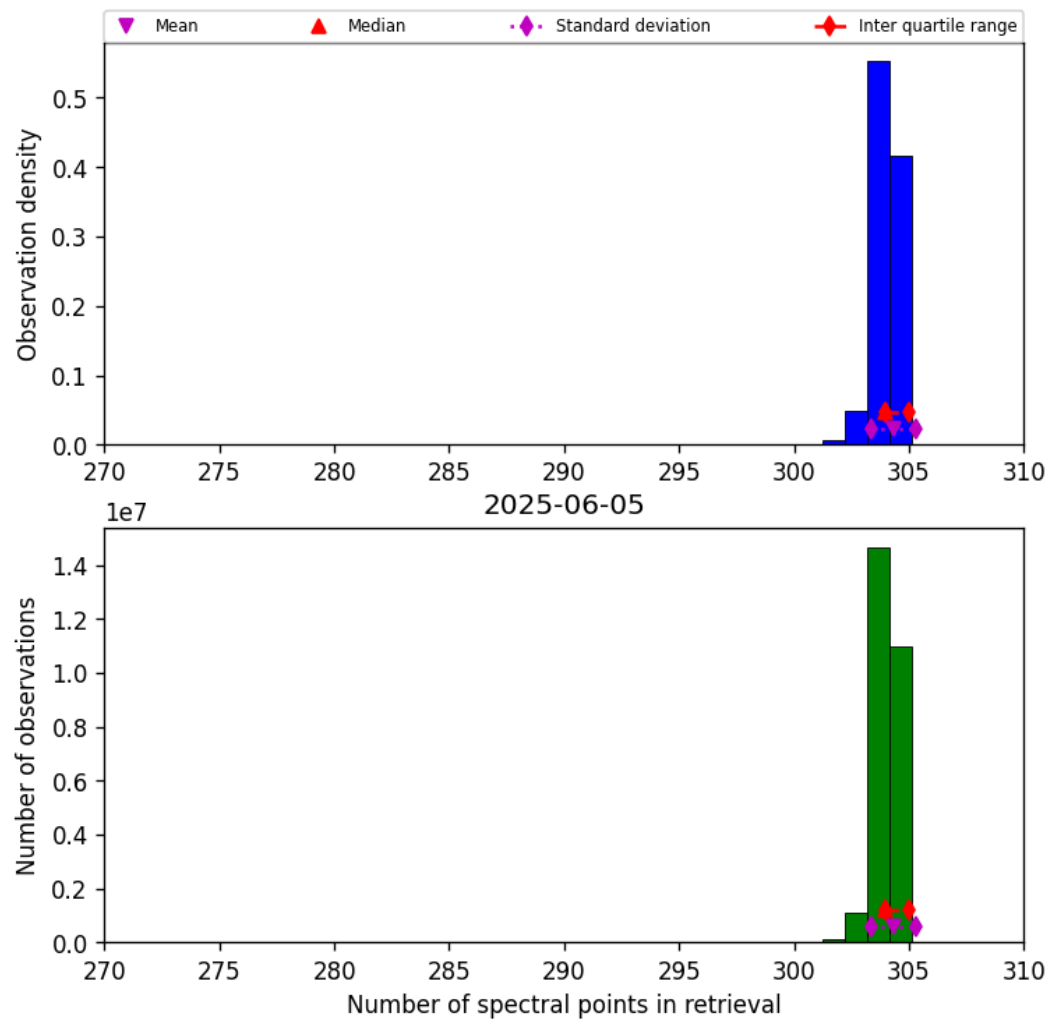
Figure 33: Histogram of “Number of spectral points in retrieval” for 2025-06-04 to 2025-06-06
