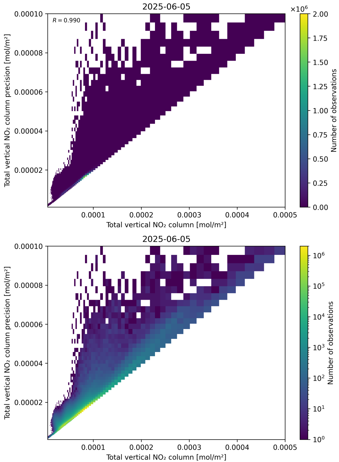
Figure 114: Scatter density plot of “Total vertical NO 2 column” against “Total vertical NO 2 column precision” for 2025-06-04 to 2025-06-06.
