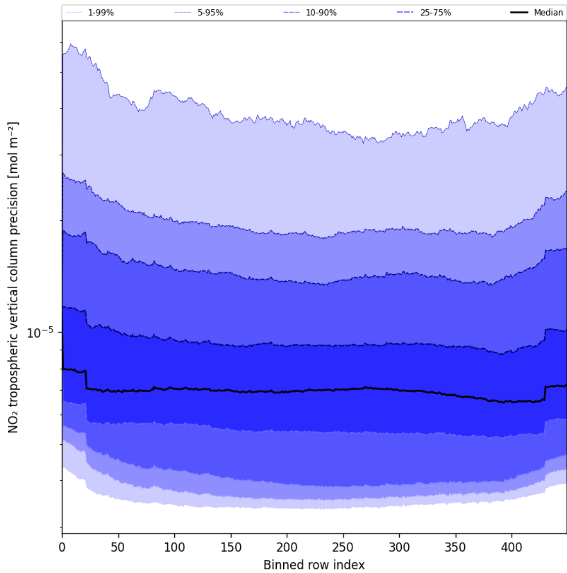
Figure 47: Along track statistics of “NO 2 tropospheric vertical column precision” for 2025-06-04 to 2025-06-06
