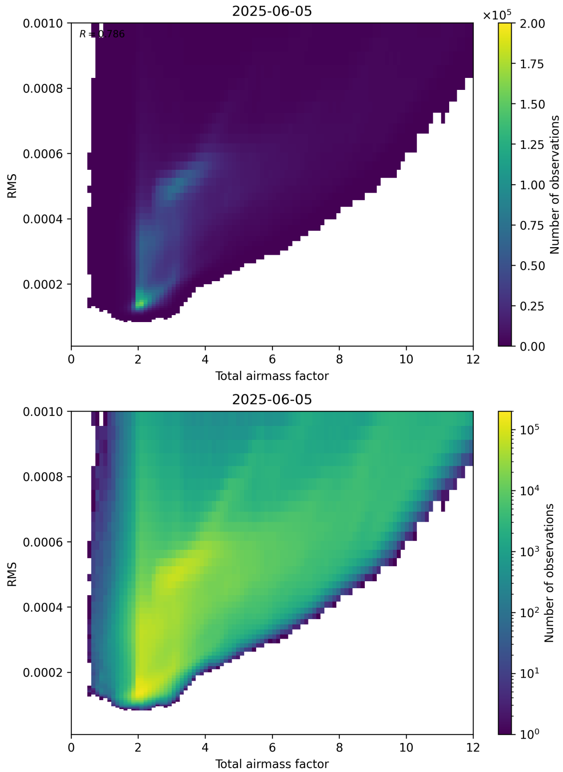
Figure 69: Scatter density plot of “Total airmass factor” against “RMS” for 2025-06-04 to 2025-06-06.
