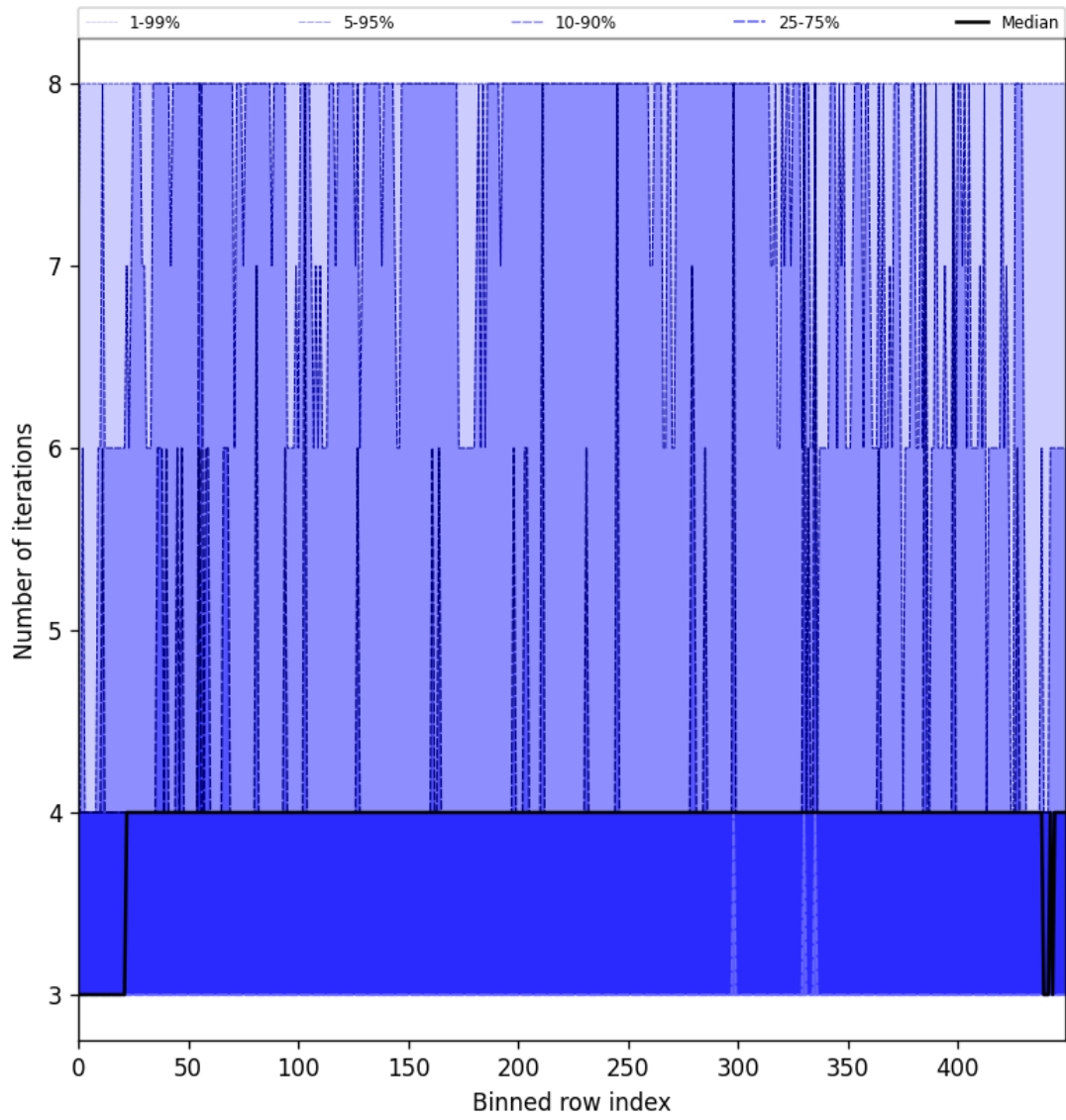
Figure 51: Along track statistics of “Number of iterations” for 2025-06-04 to 2025-06-06
