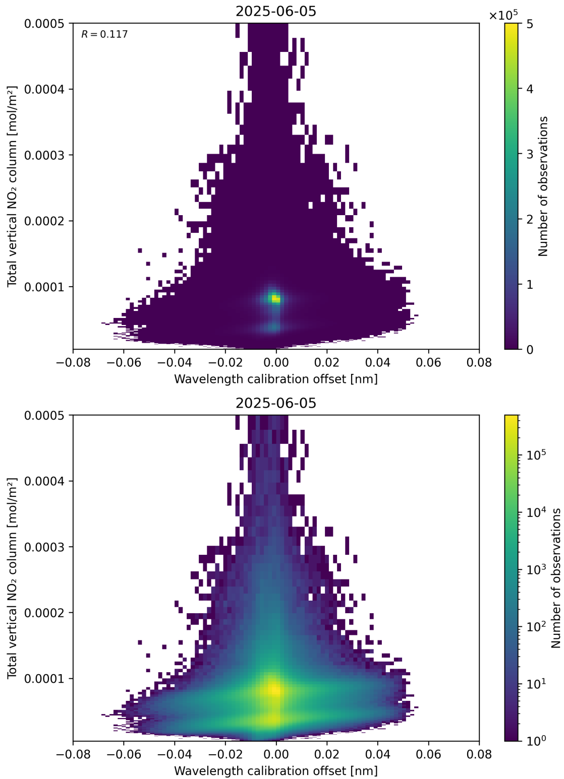
Figure 179: Scatter density plot of “Wavelength calibration offset” against “Total vertical NO 2 column” for 2025-06-04 to 2025-06-06.
