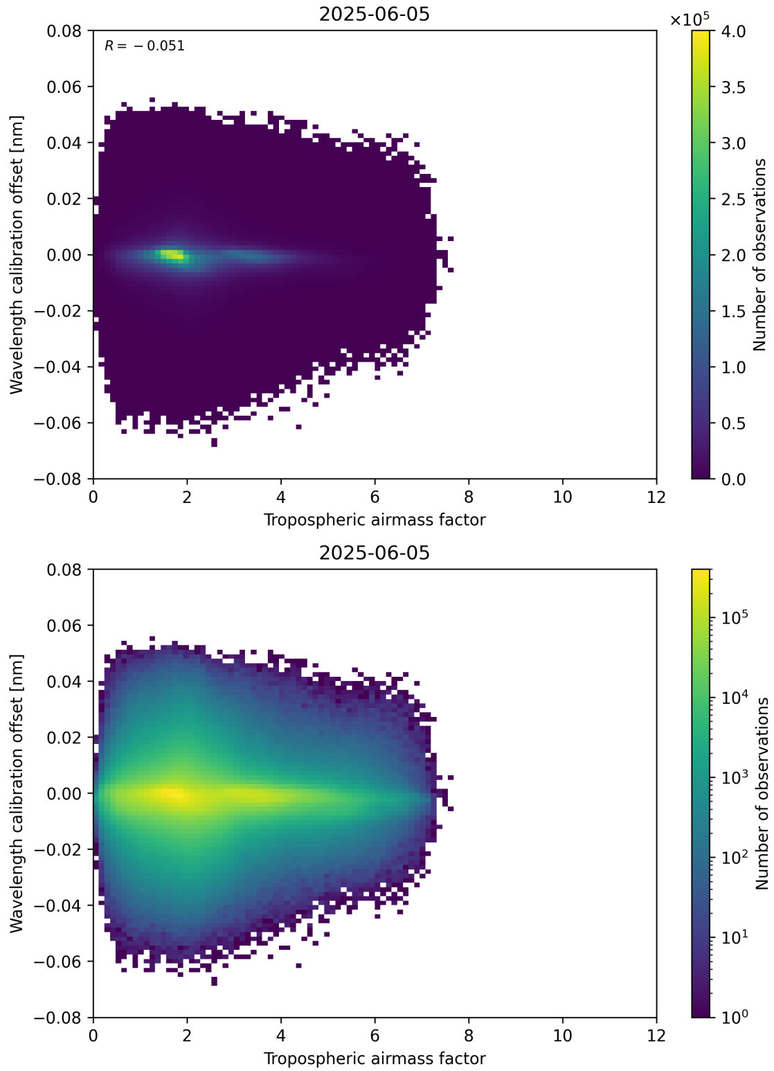
Figure 80: Scatter density plot of “Tropospheric airmass factor” against “Wavelength calibration offset” for 2025-06-04 to 2025-06-06.
