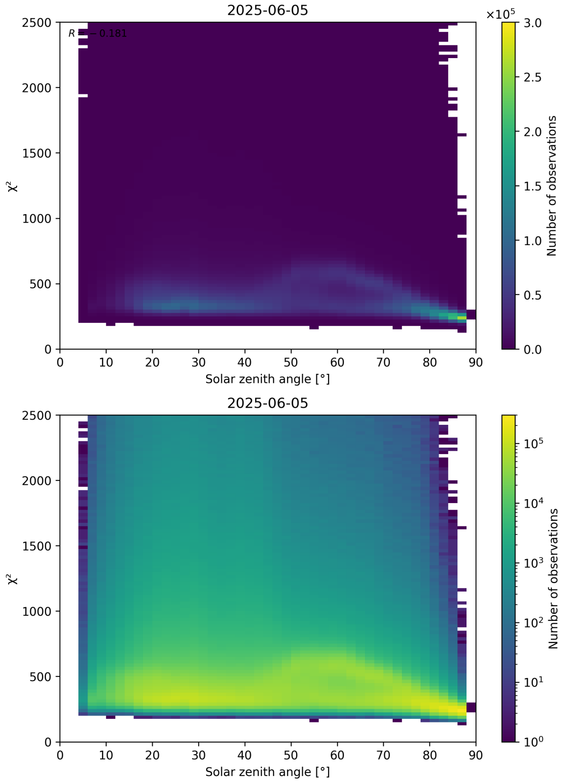
Figure 148: Scatter density plot of “Solar zenith angle” against “ \chi^2 ” for 2025-06-04 to 2025-06-06.
