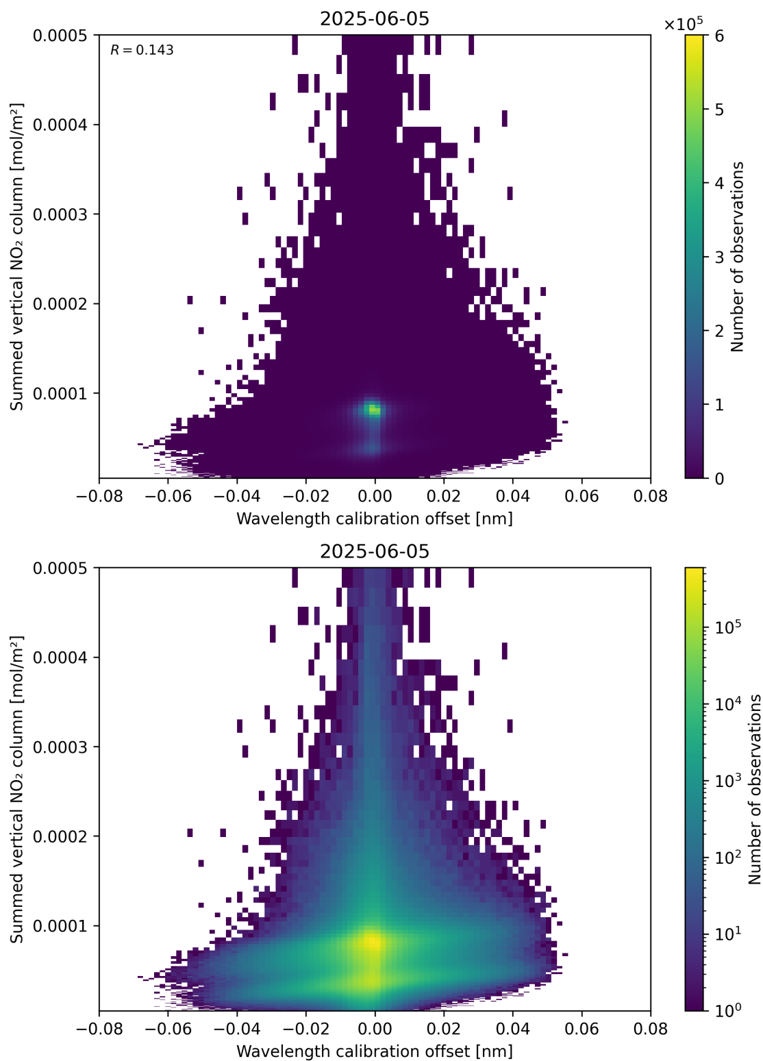
Figure 177: Scatter density plot of “Wavelength calibration offset” against “Summed vertical NO 2 column” for 2025-06-04 to 2025-06-06.
