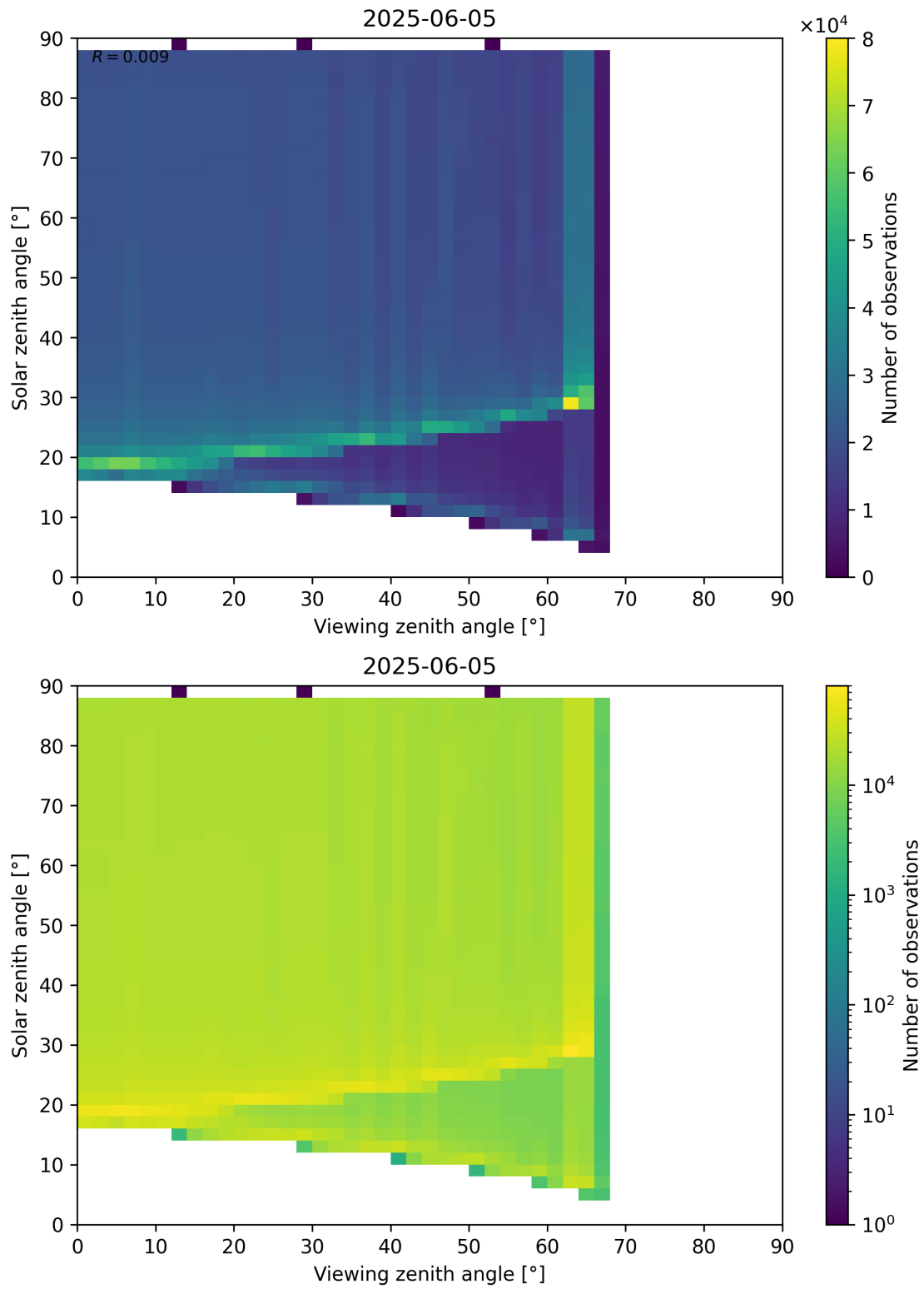
Figure 172: Scatter density plot of “Viewing zenith angle” against “Solar zenith angle” for 2025-06-04 to 2025-06-06.
