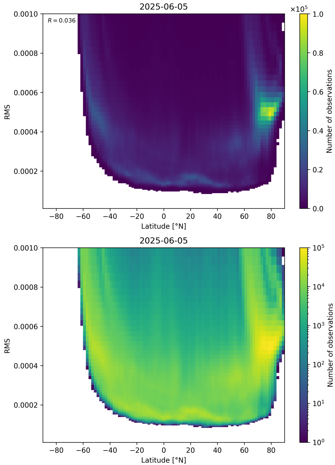
Figure 94: Scatter density plot of “Latitude” against “RMS” for 2025-06-04 to 2025-06-06.
