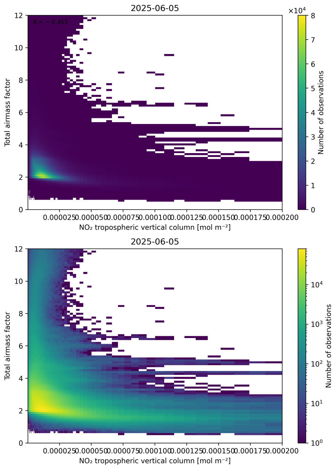
Figure 122: Scatter density plot of “NO 2 tropospheric vertical column” against “Total air mass factor” for 2025-06-04 to 2025-06-06.
