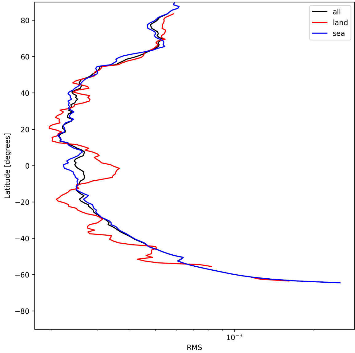
Figure 26: Zonal average of “RMS” for 2025-06-04 to 2025-06-06.
