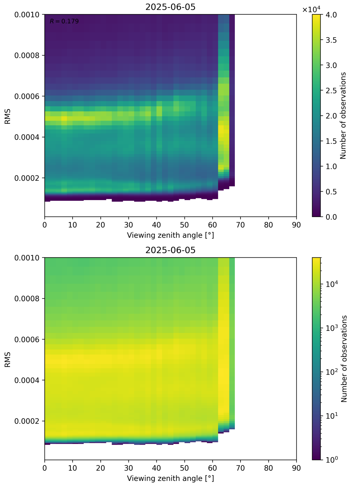
Figure 171: Scatter density plot of “Viewing zenith angle” against “RMS” for 2025-06-04 to 2025-06-06.
