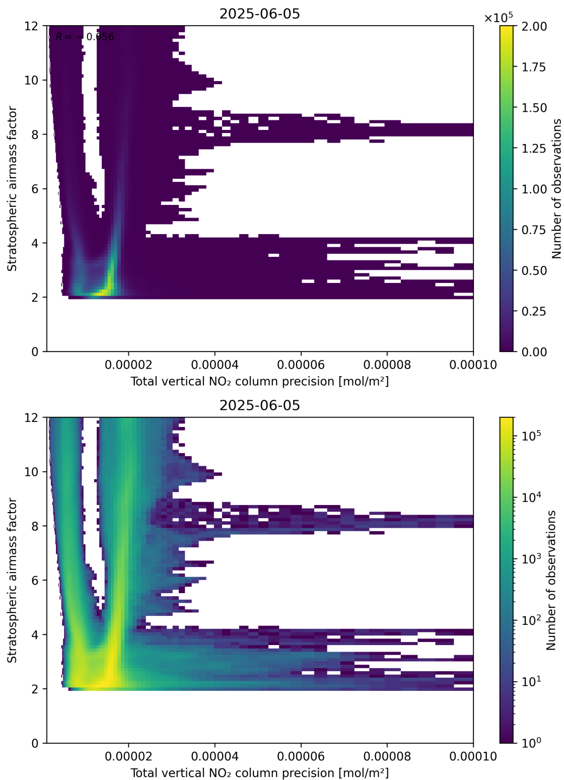
Figure 115: Scatter density plot of “Total vertical NO 2 column precision” against “Stratospheric air mass factor” for 2025-06-04 to 2025-06-06.
