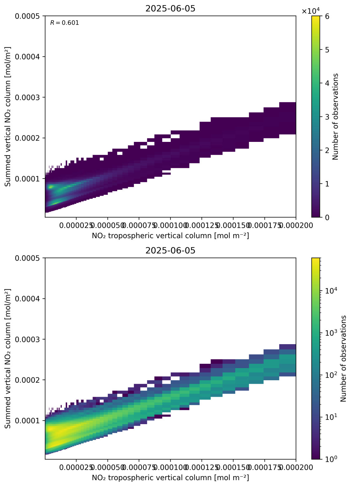
Figure 126: Scatter density plot of “NO 2 tropospheric vertical column” against “Summed vertical NO 2 column” for 2025-06-04 to 2025-06-06.
