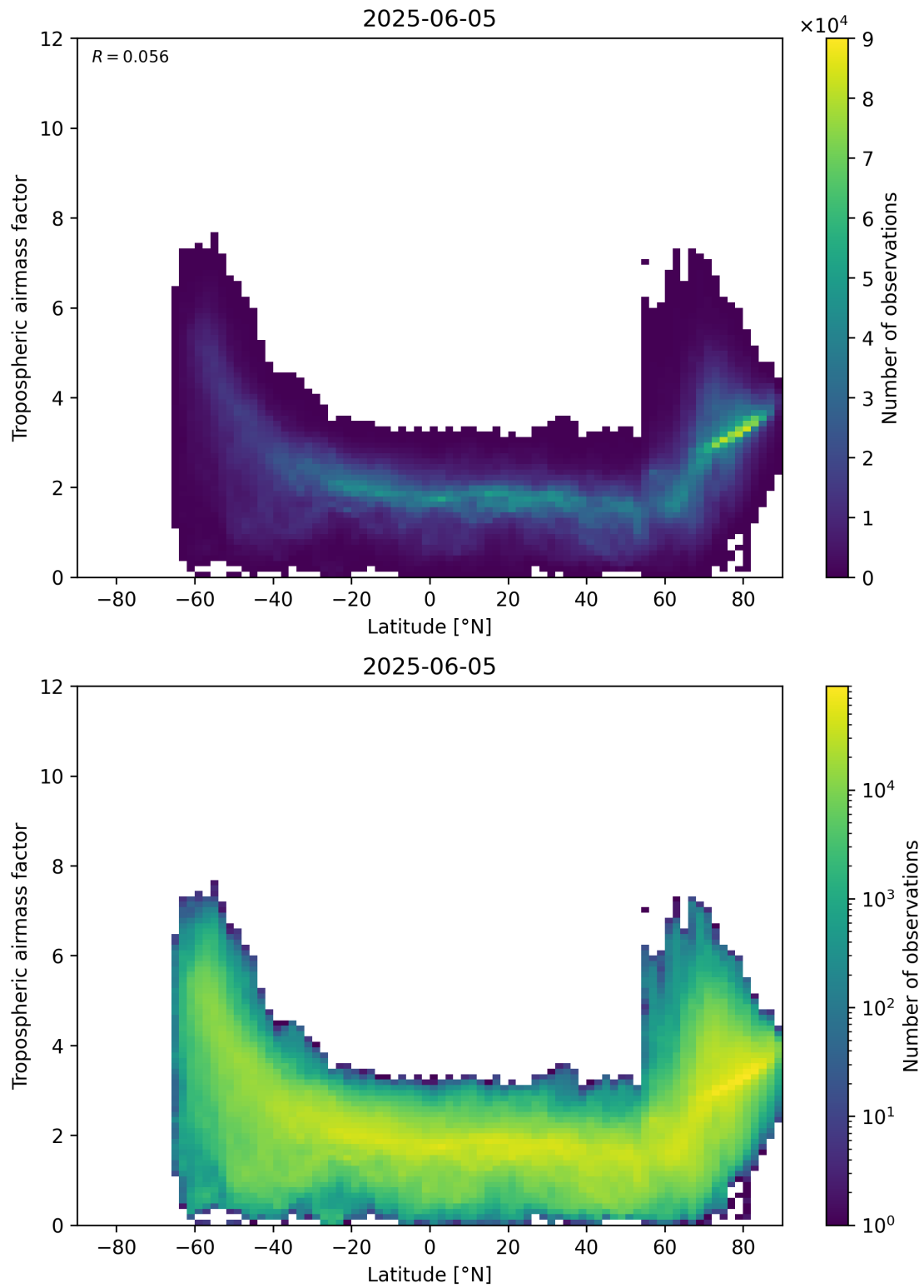
Figure 85: Scatter density plot of “Latitude” against “Tropospheric airmass factor” for 2025-06-04 to 2025-06-06.
