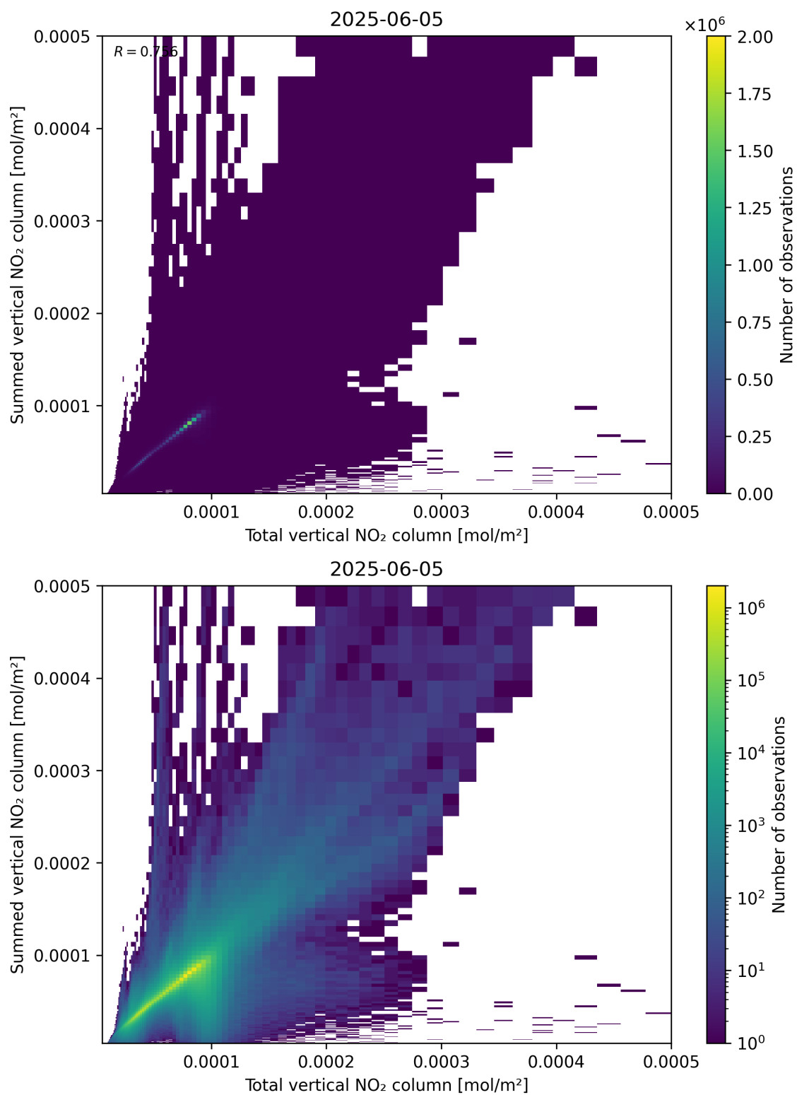
Figure 112: Scatter density plot of “Total vertical NO 2 column” against “Summed vertical NO 2 column” for 2025-06-04 to 2025-06-06.
