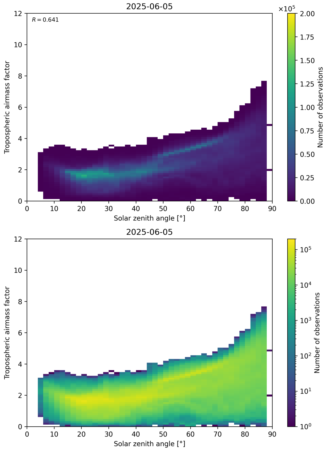
Figure 147: Scatter density plot of “Solar zenith angle” against “Tropospheric airmass factor” for 2025-06-04 to 2025-06-06.
