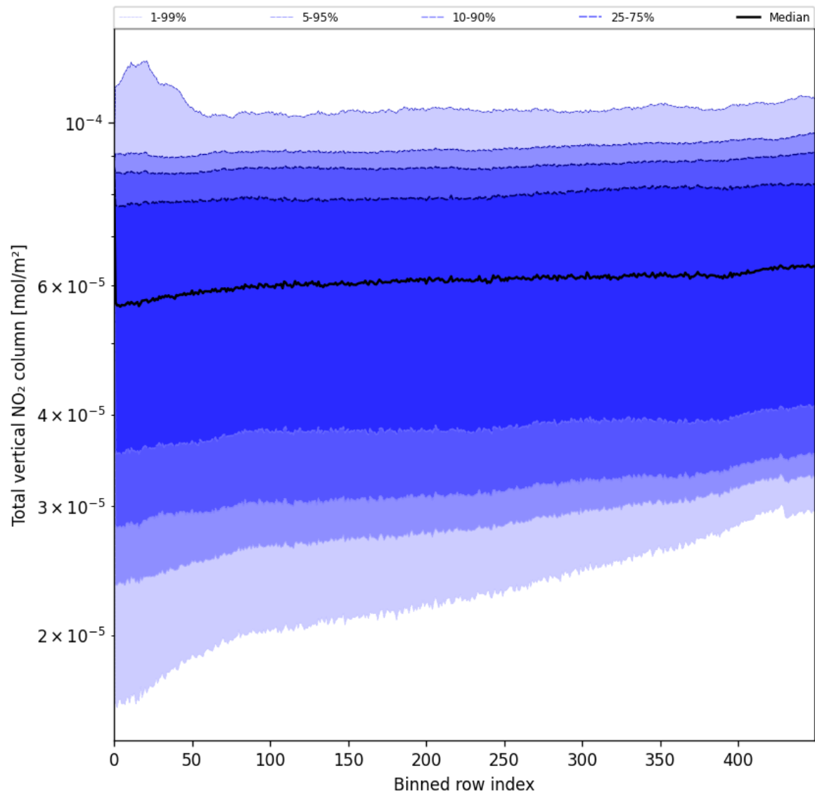
Figure 55: Along track statistics of “Total vertical NO 2 column” for 2025-06-04 to 2025-06-06
