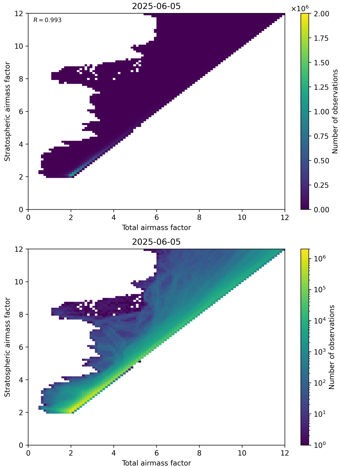
Figure 62: Scatter density plot of “Total airmass factor” against “Stratospheric airmass factor” for 2025-06-04 to 2025-06-06.
