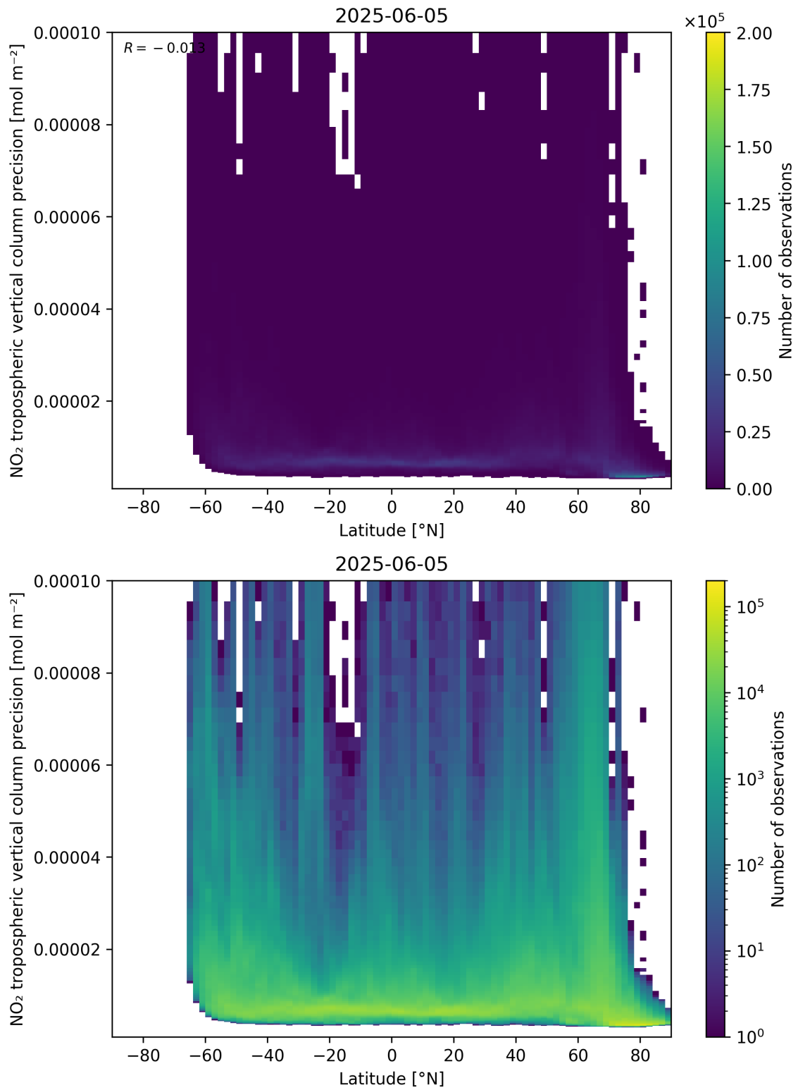
Figure 93: Scatter density plot of “Latitude” against “NO 2 tropospheric vertical column precision” for 2025-06-04 to 2025-06-06.
