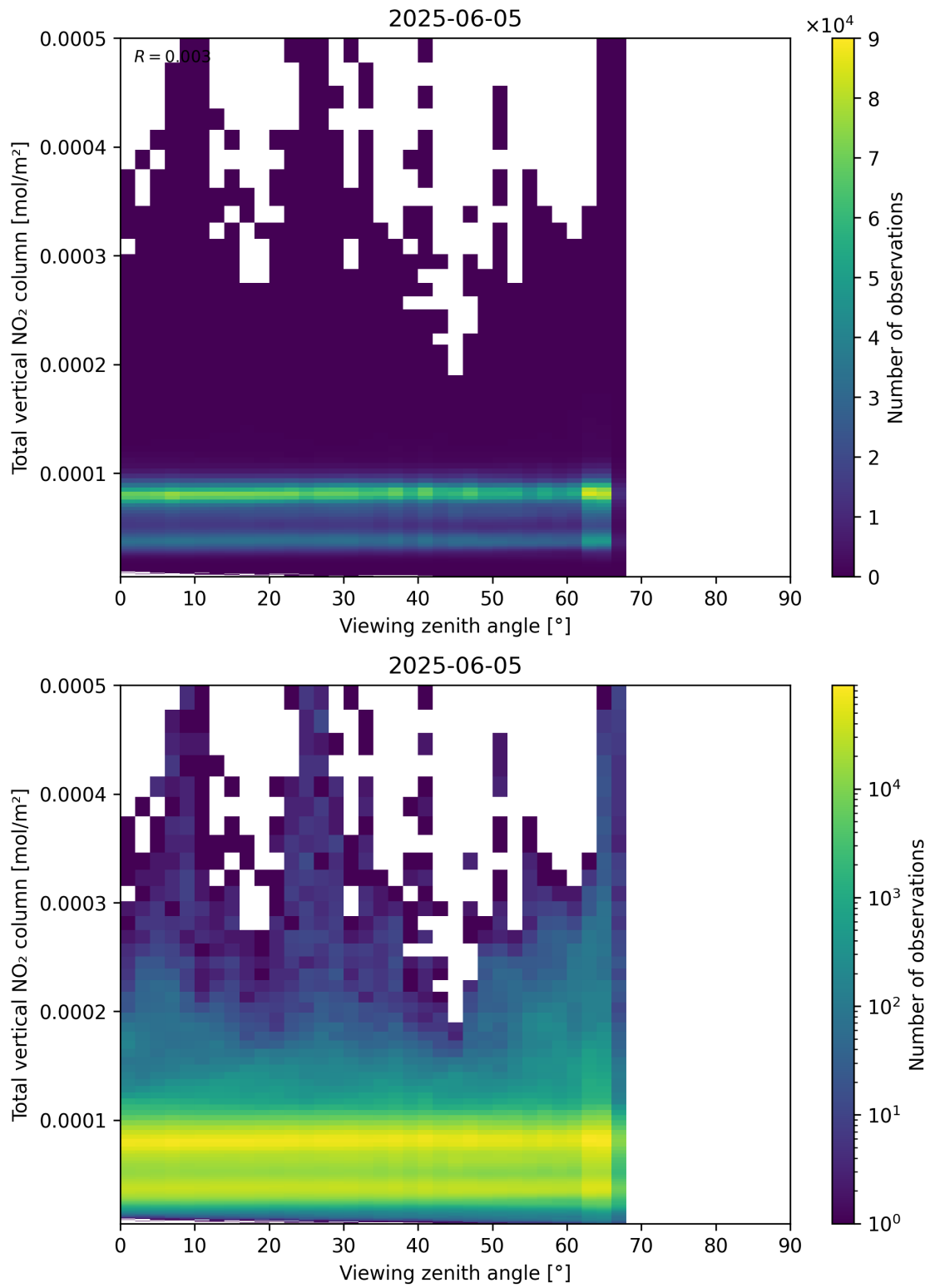
Figure 167: Scatter density plot of “Viewing zenith angle” against “Total vertical NO 2 column” for 2025-06-04 to 2025-06-06.
