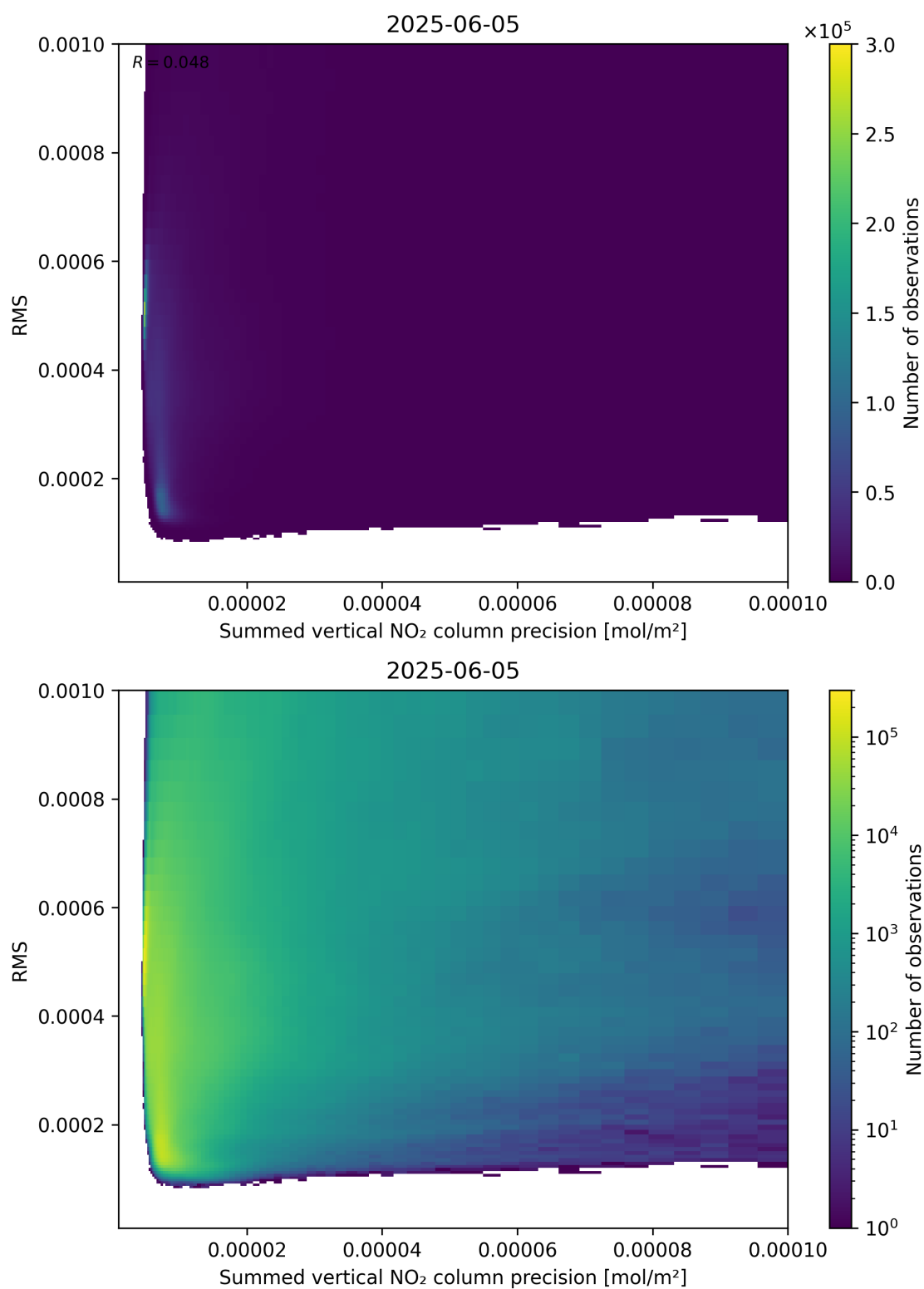
Figure 108: Scatter density plot of “Summed vertical NO 2 column precision” against “RMS” for 2025-06-04 to 2025-06-06.
