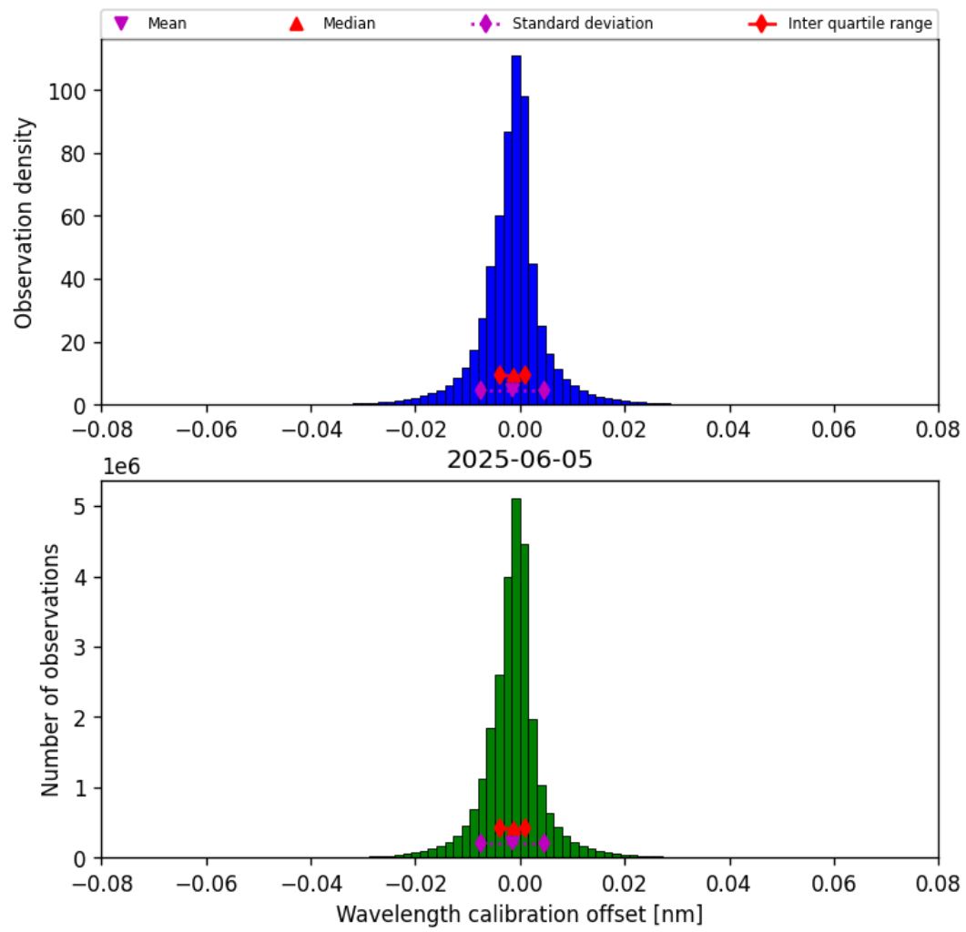
Figure 35: Histogram of “Wavelength calibration offset” for 2025-06-04 to 2025-06-06
