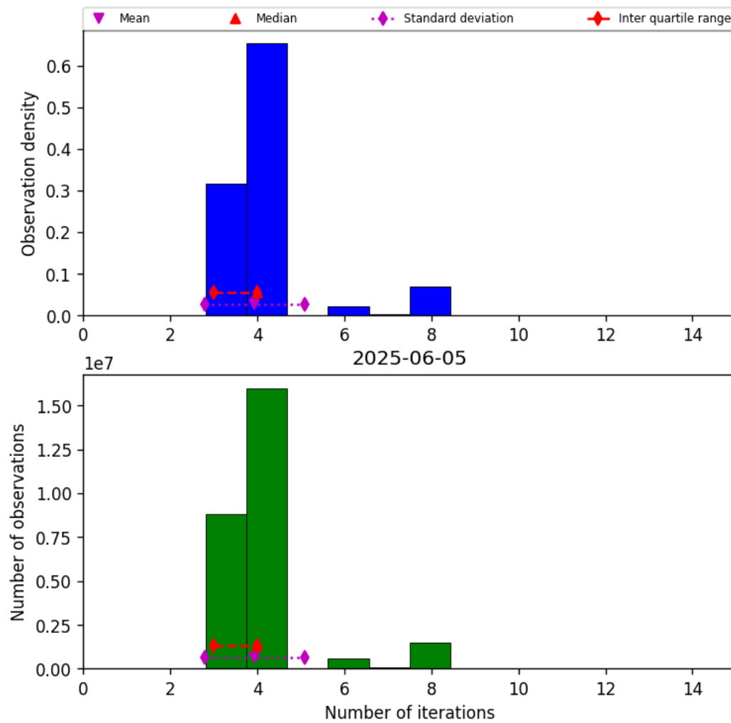
Figure 34: Histogram of “Number of iterations” for 2025-06-04 to 2025-06-06
