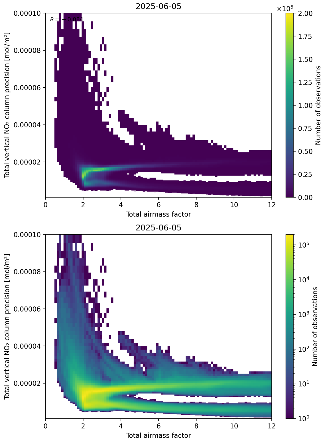
Figure 68: Scatter density plot of “Total airmass factor” against “Total vertical NO 2 column precision” for 2025-06-04 to 2025-06-06.
