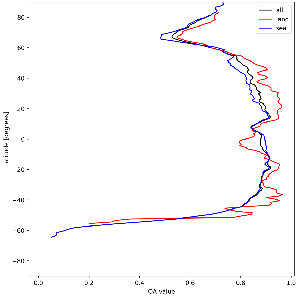
Figure 11: Zonal average of “QA value” for 2025-06-04 to 2025-06-06.
