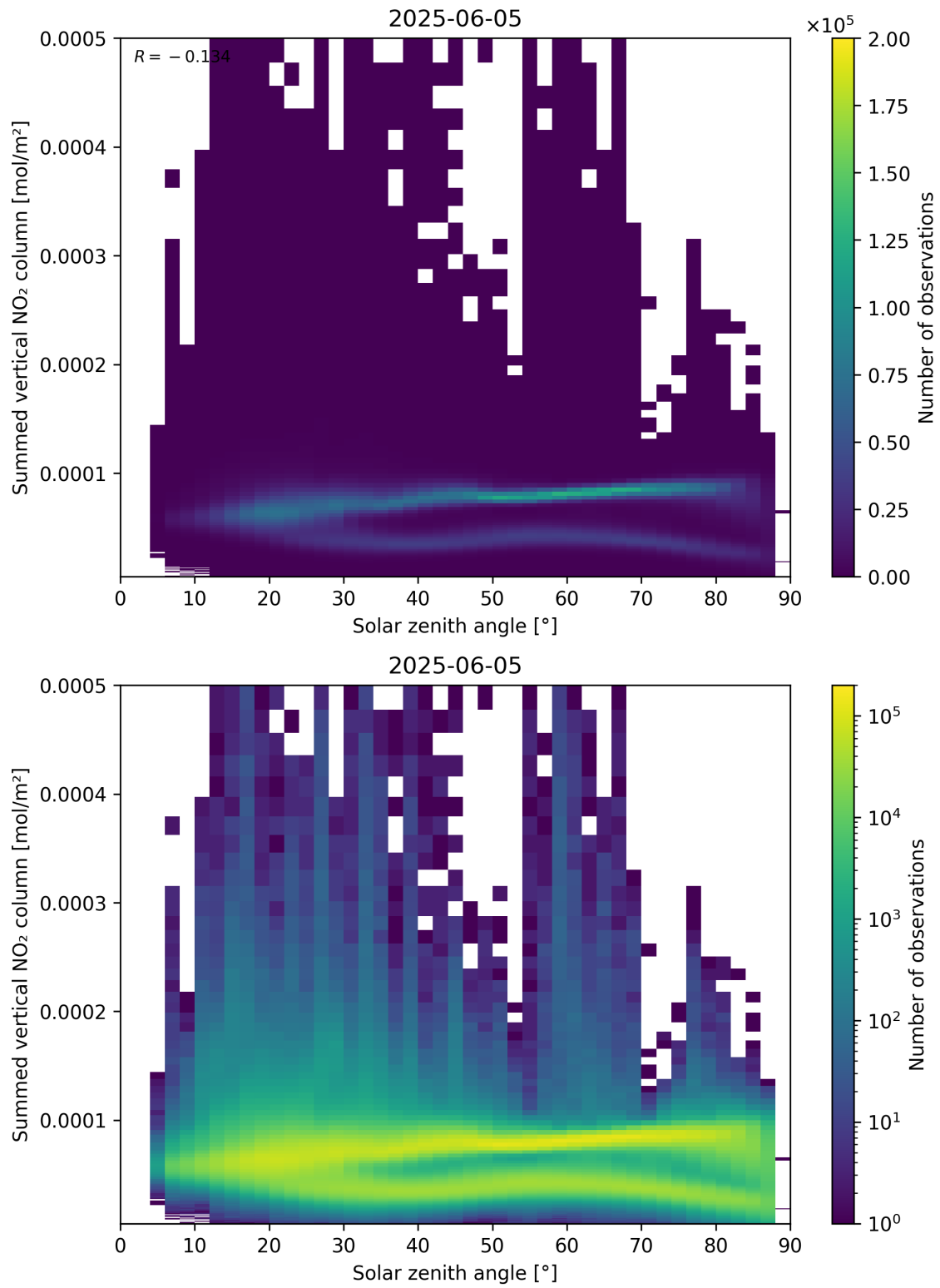
Figure 151: Scatter density plot of “Solar zenith angle” against “Summed vertical NO 2 column” for 2025-06-04 to 2025-06-06.
