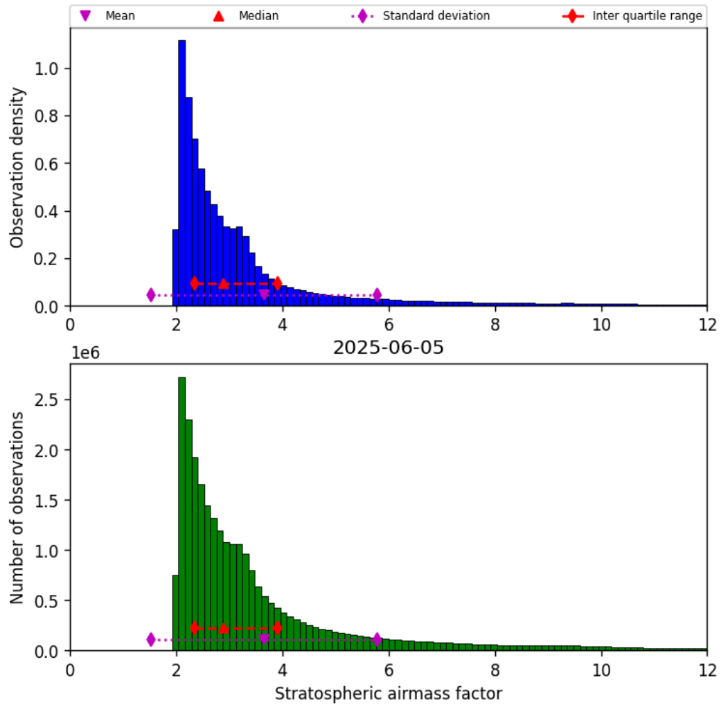
Figure 44: Histogram of “Stratospheric airmass factor” for 2025-06-04 to 2025-06-06
