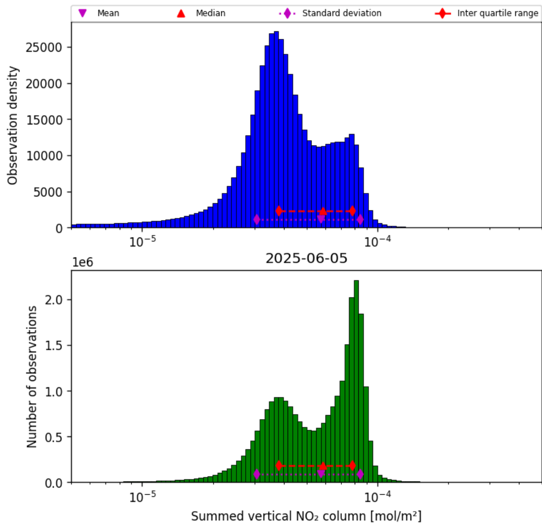
Figure 40: Histogram of “Summed vertical NO 2 column” for 2025-06-04 to 2025-06-06
