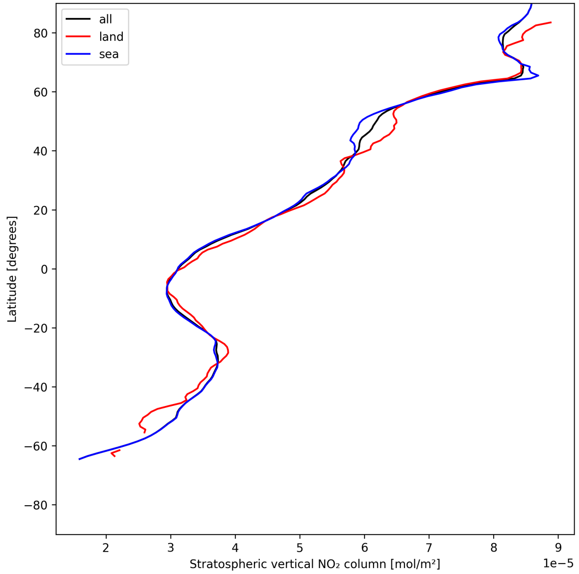
Figure 19: Zonal average of “Stratospheric vertical NO 2 column” for 2025-06-04 to 2025-06-06.
