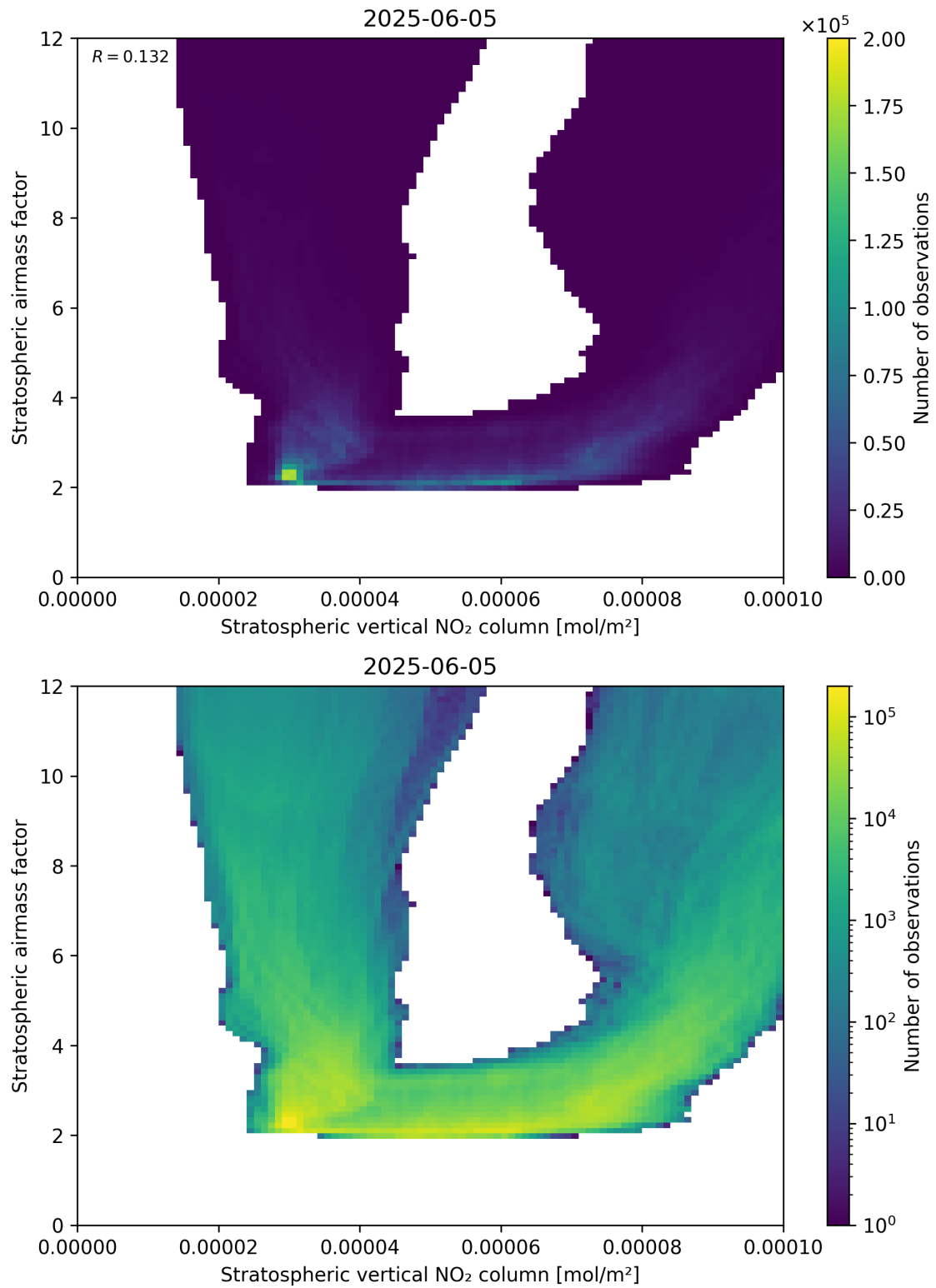
Figure 96: Scatter density plot of “Stratospheric vertical NO 2 column” against “Stratospheric airmass factor” for 2025-06-04 to 2025-06-06.
