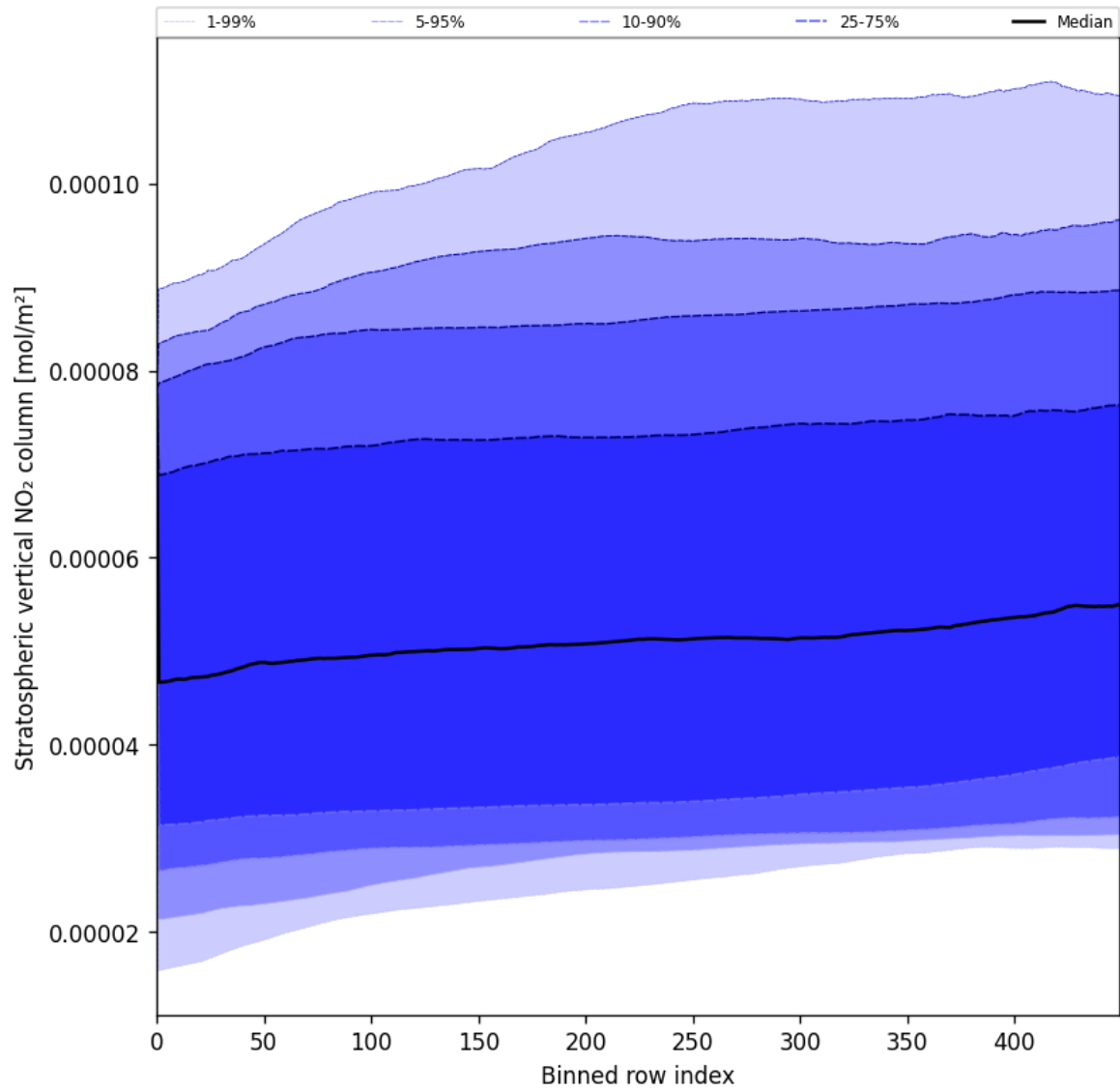
Figure 53: Along track statistics of “Stratospheric vertical NO 2 column” for 2025-06-04 to 2025-06-06
