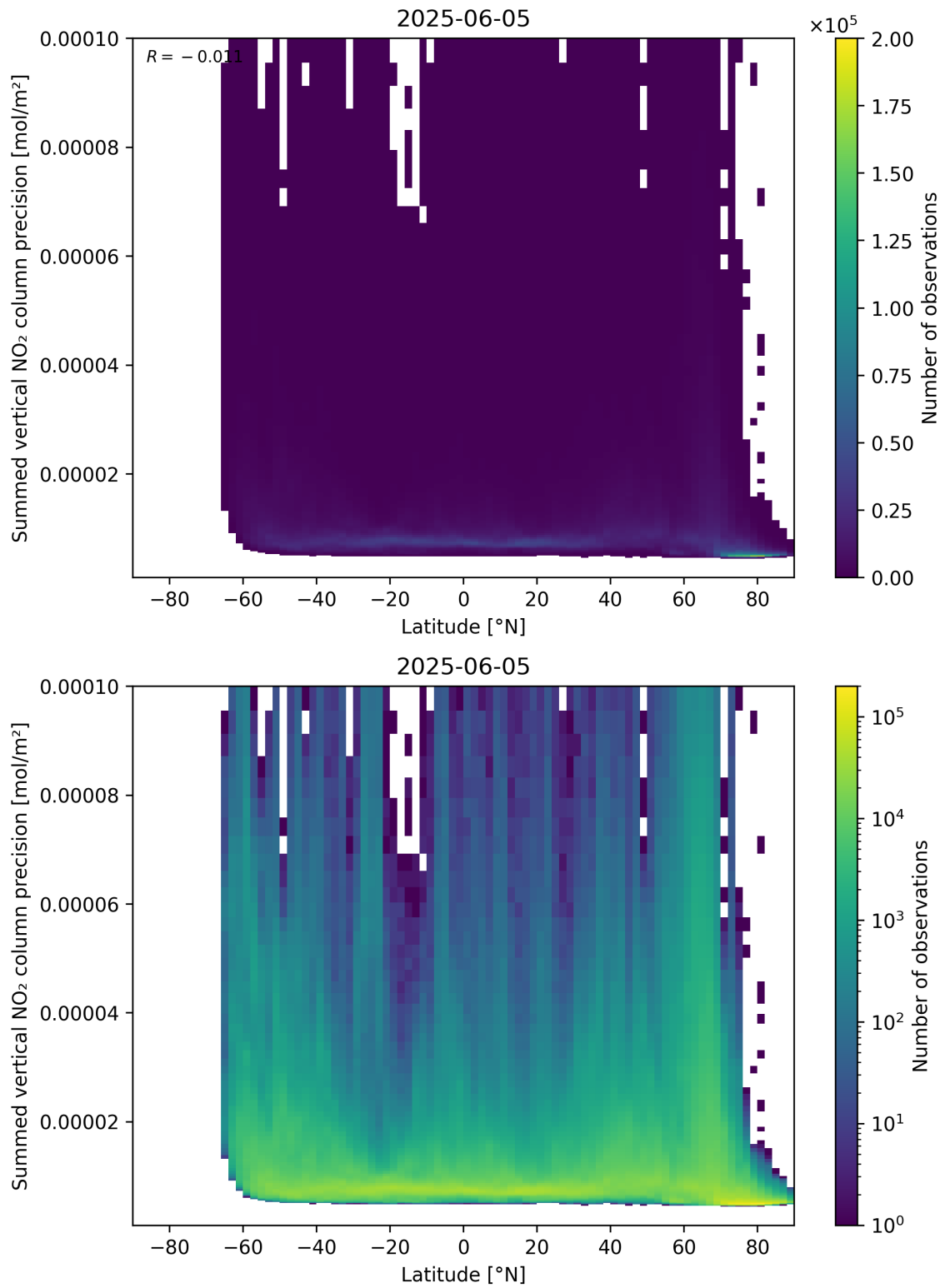
Figure 89: Scatter density plot of “Latitude” against “Summed vertical NO 2 column precision” for 2025-06-04 to 2025-06-06.
