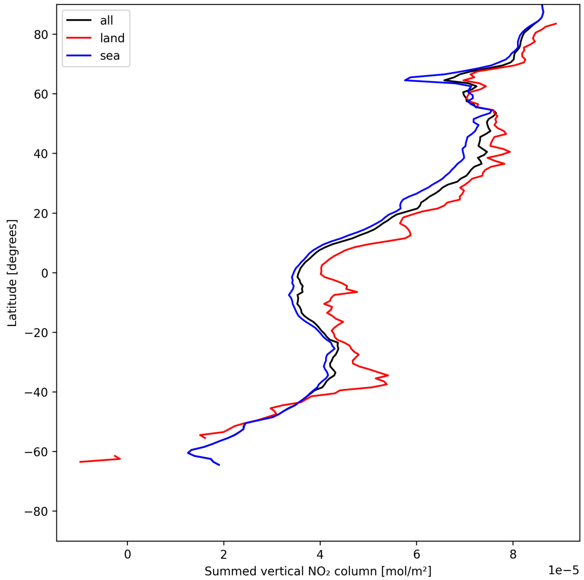
Figure 23: Zonal average of “Summed vertical NO 2 column” for 2025-06-04 to 2025-06-06.
