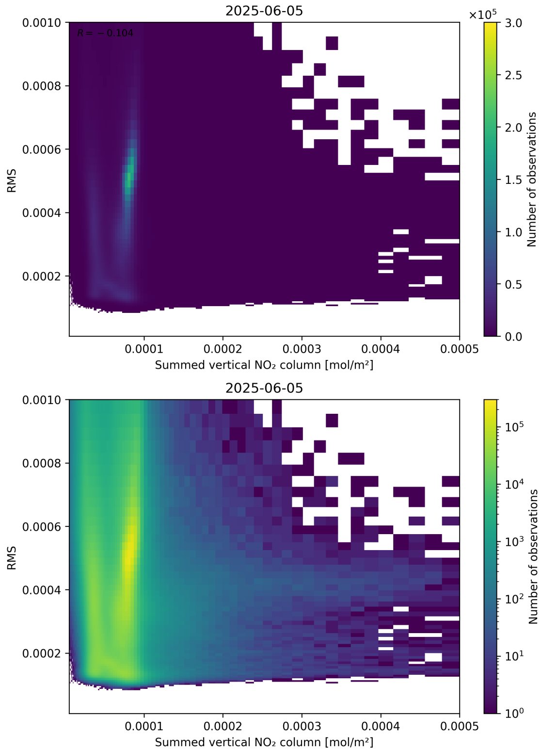
Figure 109: Scatter density plot of “Summed vertical NO 2 column” against “RMS” for 2025-06-04 to 2025-06-06.
