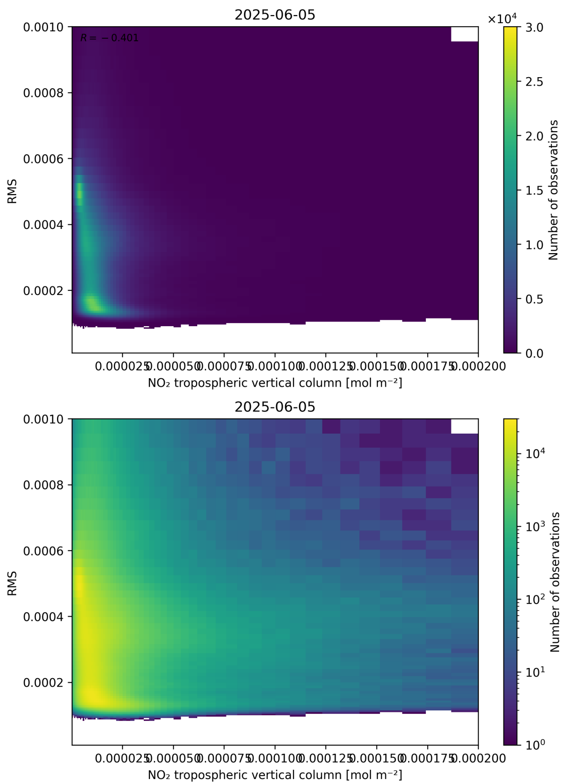
Figure 142: Scatter density plot of “NO 2 tropospheric vertical column” against “RMS” for 2025-06-04 to 2025-06-06.
