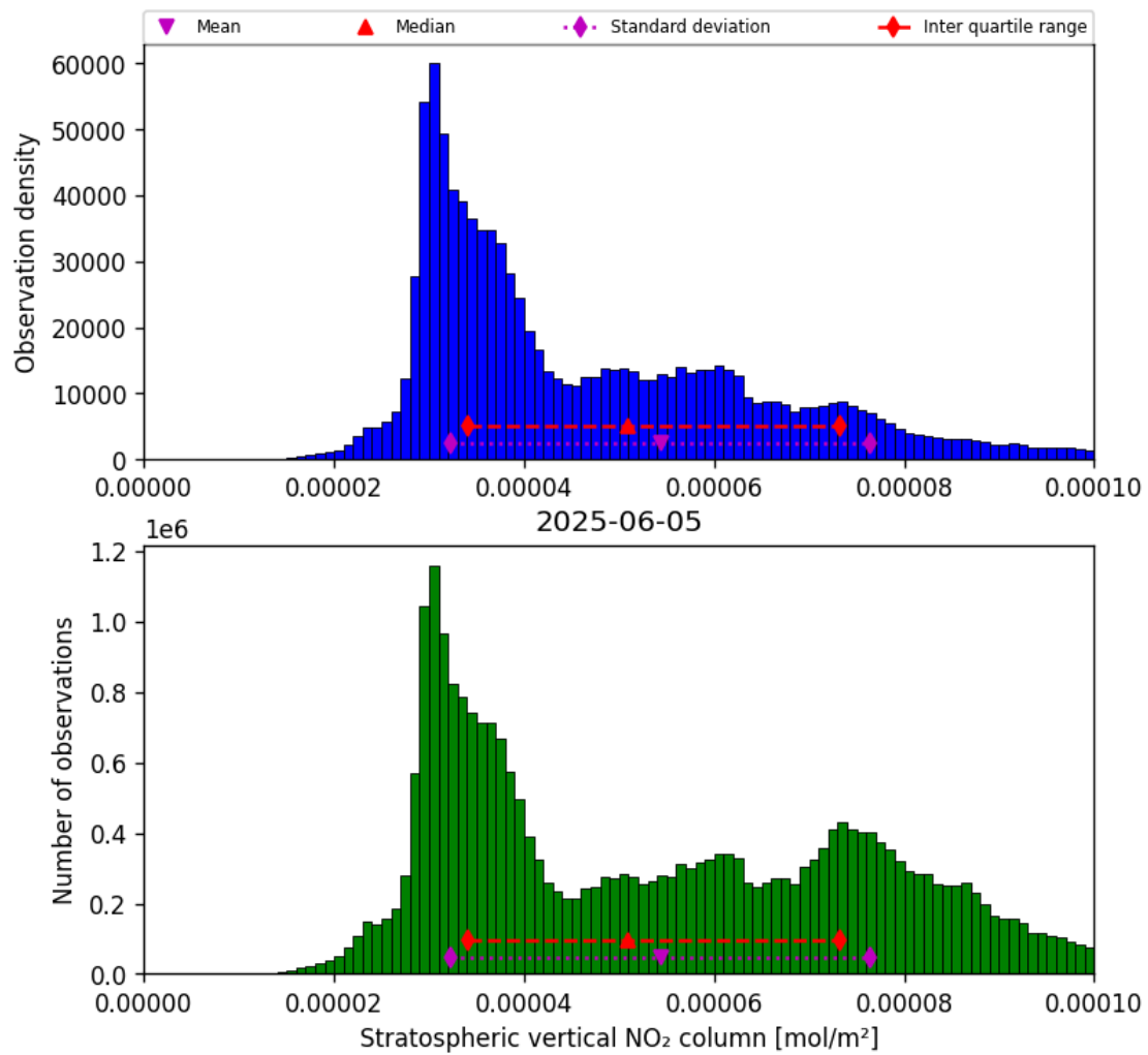
Figure 36: Histogram of “Stratospheric vertical NO 2 column” for 2025-06-04 to 2025-06-06
