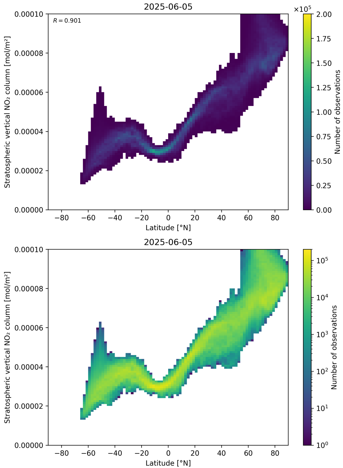
Figure 87: Scatter density plot of “Latitude” against “Stratospheric vertical \text{NO}_2 column” for 2025-06-04 to 2025-06-06.
