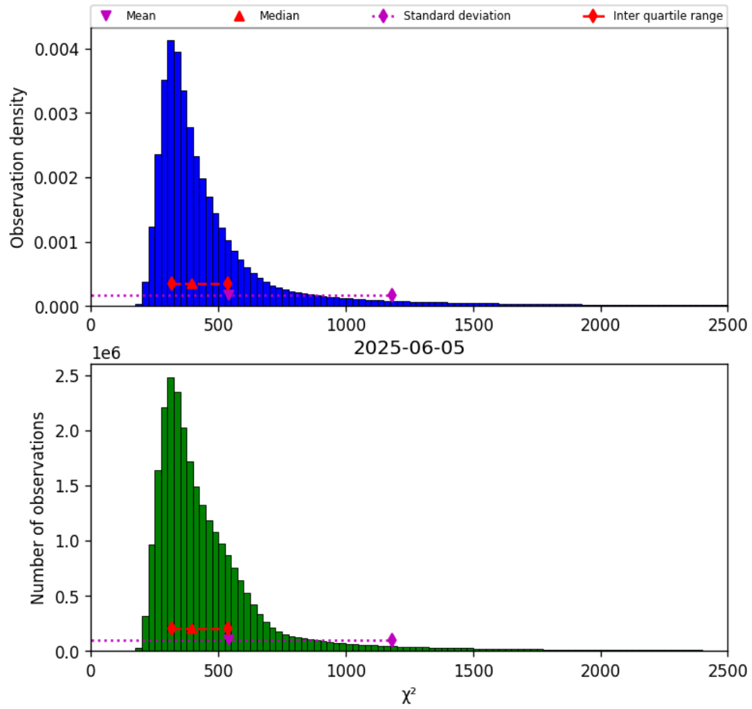
Figure 42: Histogram of “ \chi^2 ” for 2025-06-04 to 2025-06-06
