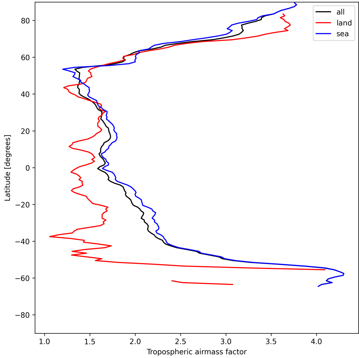
Figure 14: Zonal average of “Tropospheric airmass factor” for 2025-06-04 to 2025-06-06.
