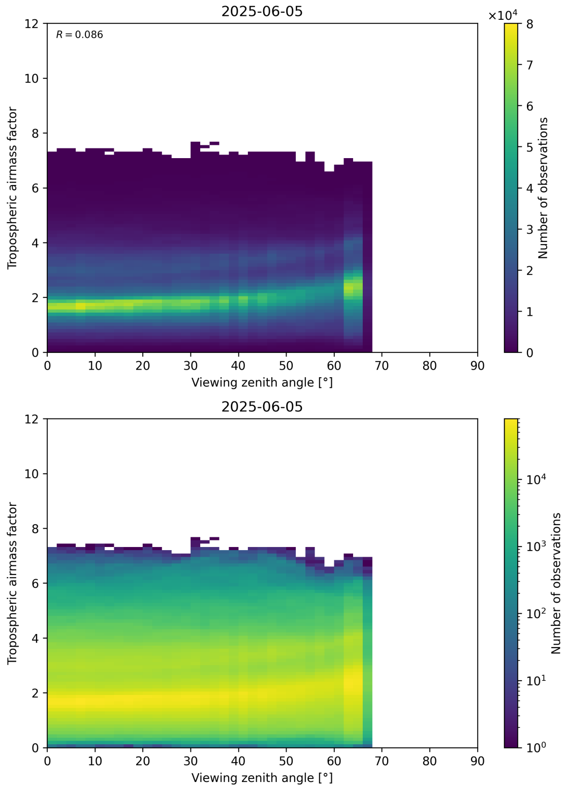
Figure 161: Scatter density plot of “Viewing zenith angle” against “Tropospheric airmass factor” for 2025-06-04 to 2025-06-06.
