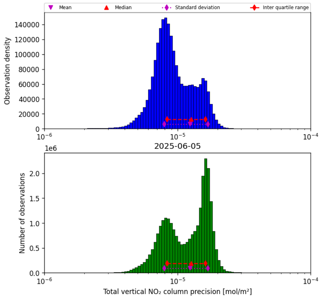
Figure 39: Histogram of “Total vertical NO 2 column precision” for 2025-06-04 to 2025-06-06
