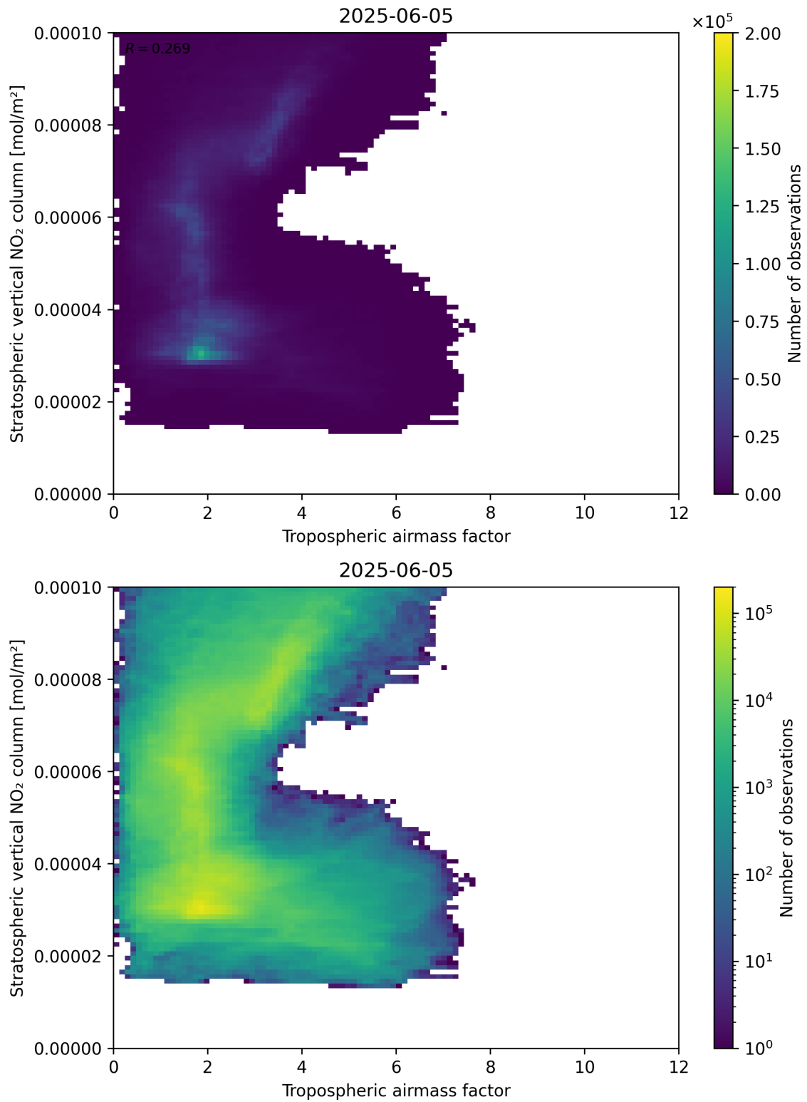
Figure 74: Scatter density plot of “Tropospheric air mass factor” against “Stratospheric vertical NO 2 column” for 2025-06-04 to 2025-06-06.
