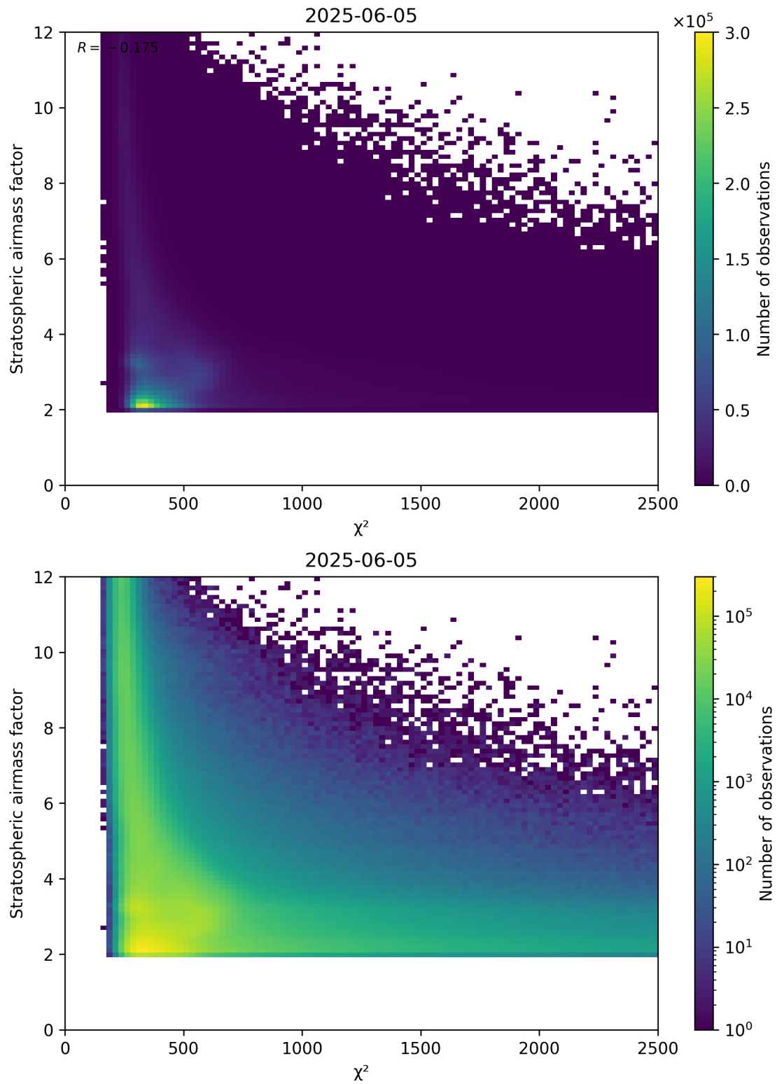
Figure 81: Scatter density plot of “ \chi^2 ” against “Stratospheric airmass factor” for 2025-06-04 to 2025-06-06.
