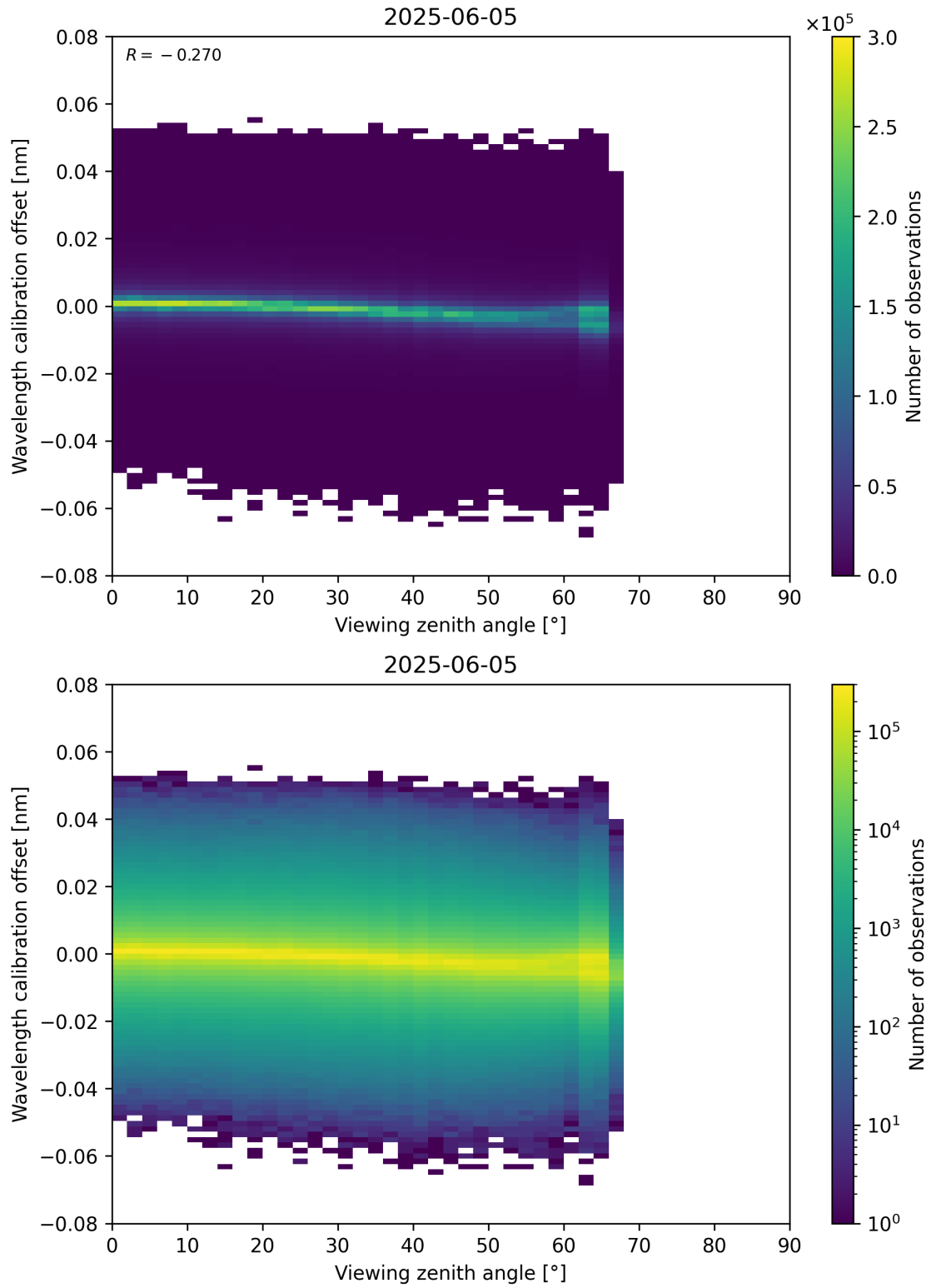
Figure 173: Scatter density plot of “Viewing zenith angle” against “Wavelength calibration offset” for 2025-06-04 to 2025-06-06.
