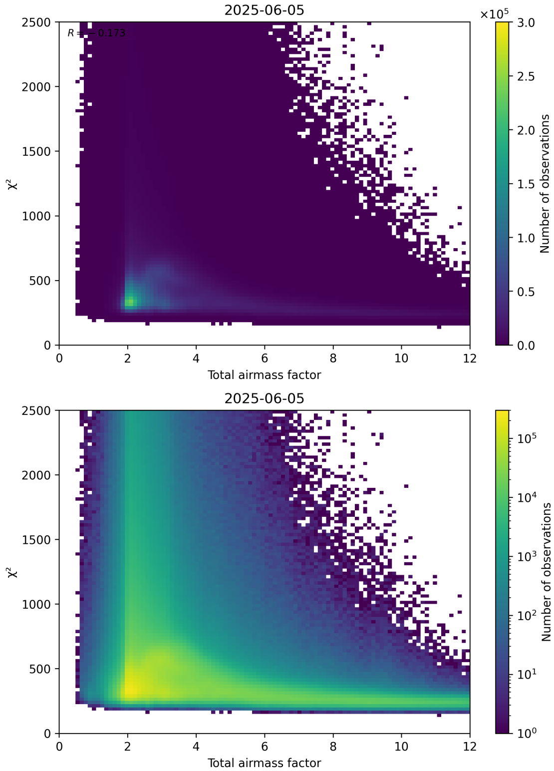
Figure 63: Scatter density plot of “Total airmass factor” against “ \chi^2 ” for 2025-06-04 to 2025-06-06.
