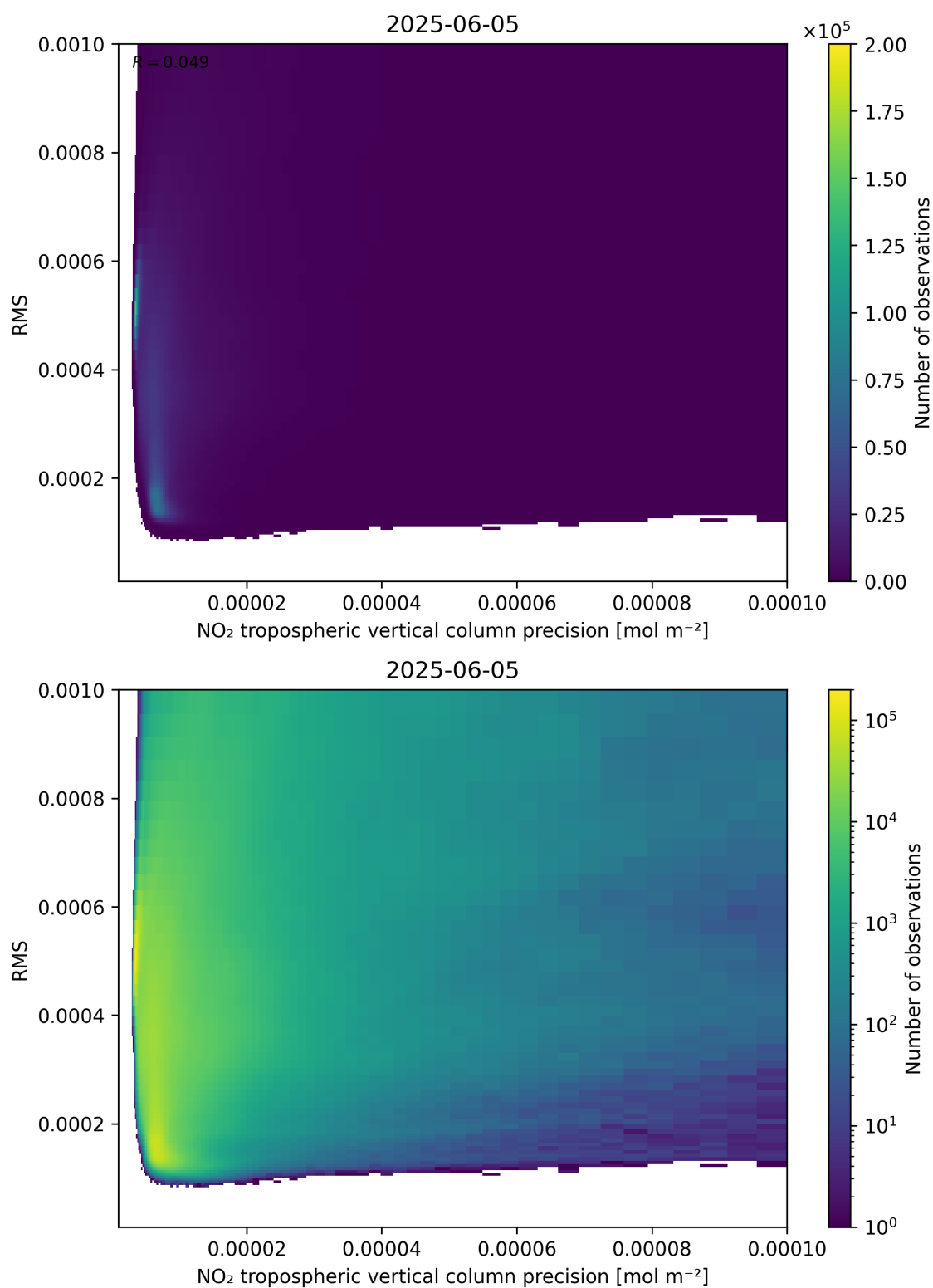
Figure 140: Scatter density plot of “NO 2 tropospheric vertical column precision” against “RMS” for 2025-06-04 to 2025-06-06.
