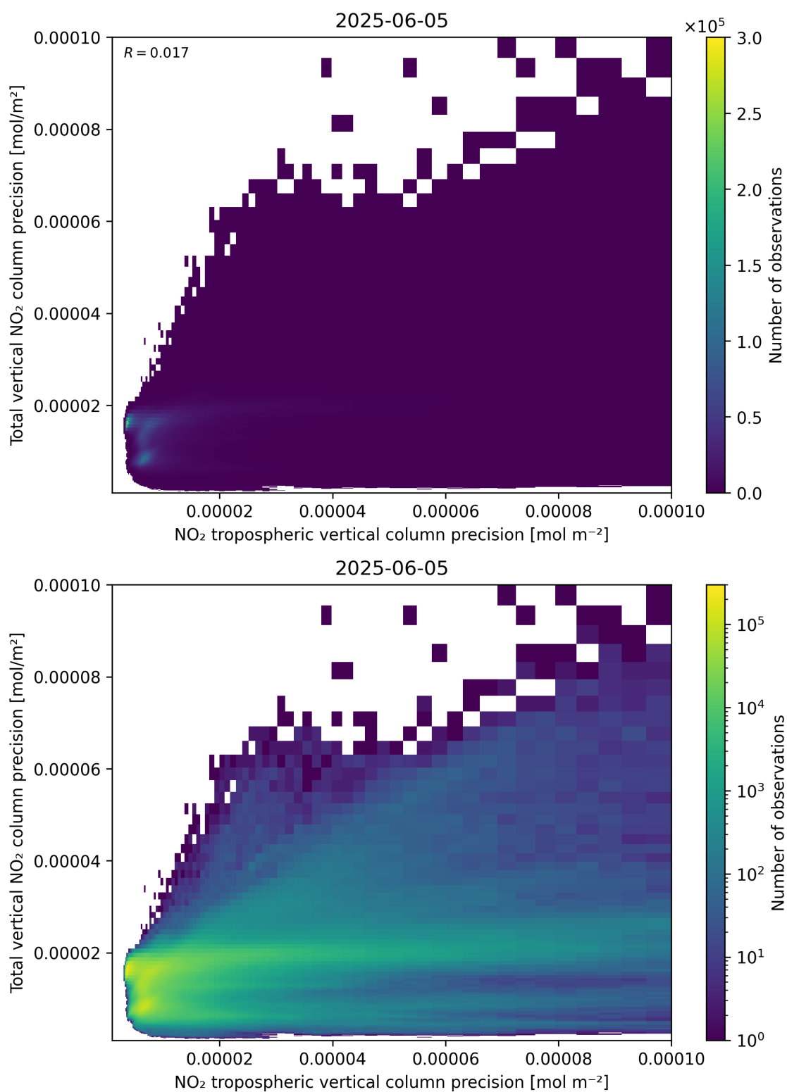
Figure 139: Scatter density plot of “NO 2 tropospheric vertical column precision” against “Total vertical NO 2 column precision” for 2025-06-04 to 2025-06-06.
