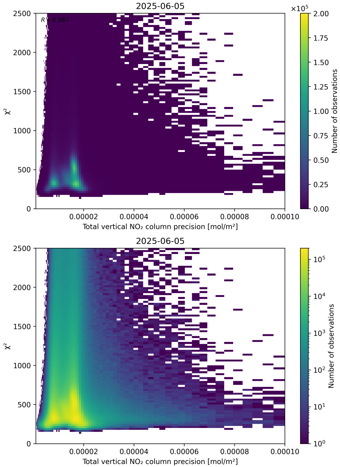
Figure 116: Scatter density plot of “Total vertical NO 2 column precision” against “ \chi^2 ” for 2025-06-04 to 2025-06-06.
