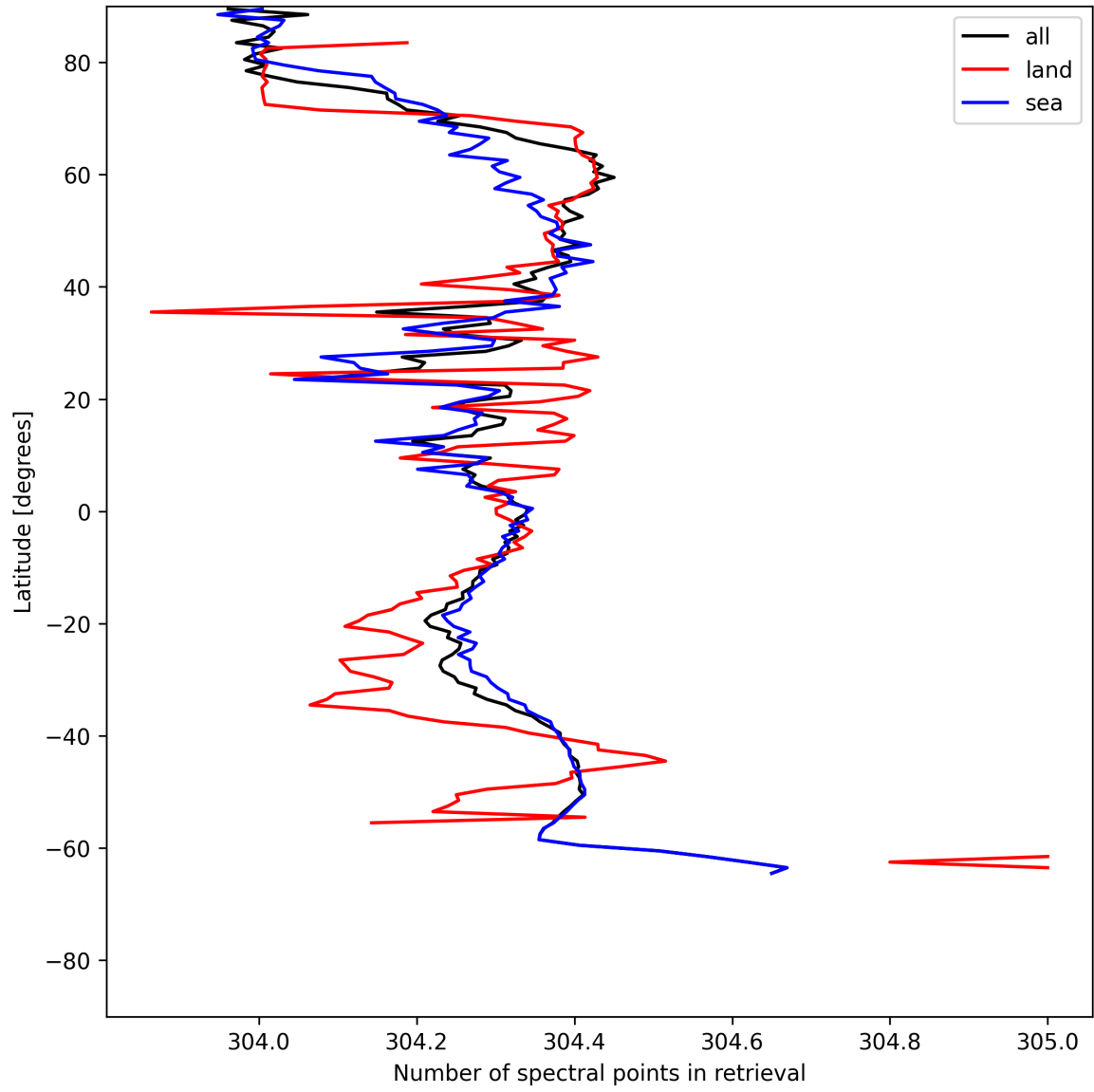
Figure 16: Zonal average of “Number of spectral points in retrieval” for 2025-06-04 to 2025-06-06.
