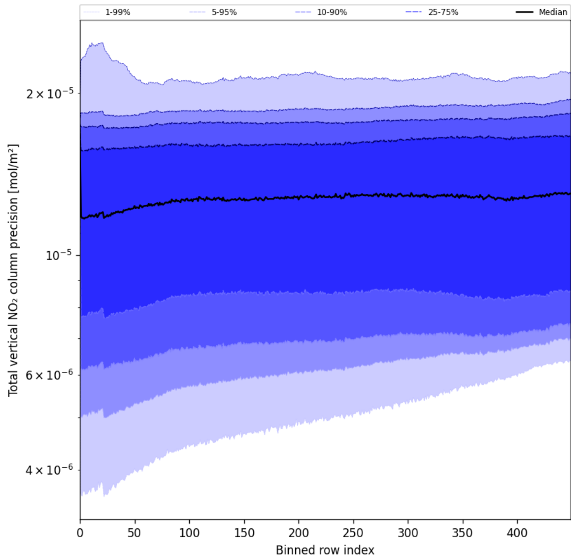
Figure 56: Along track statistics of “Total vertical NO 2 column precision” for 2025-06-04 to 2025-06-06
