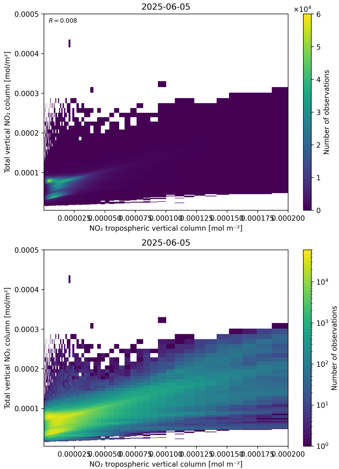
Figure 128: Scatter density plot of “NO 2 tropospheric vertical column” against “Total vertical NO 2 column” for 2025-06-04 to 2025-06-06.
