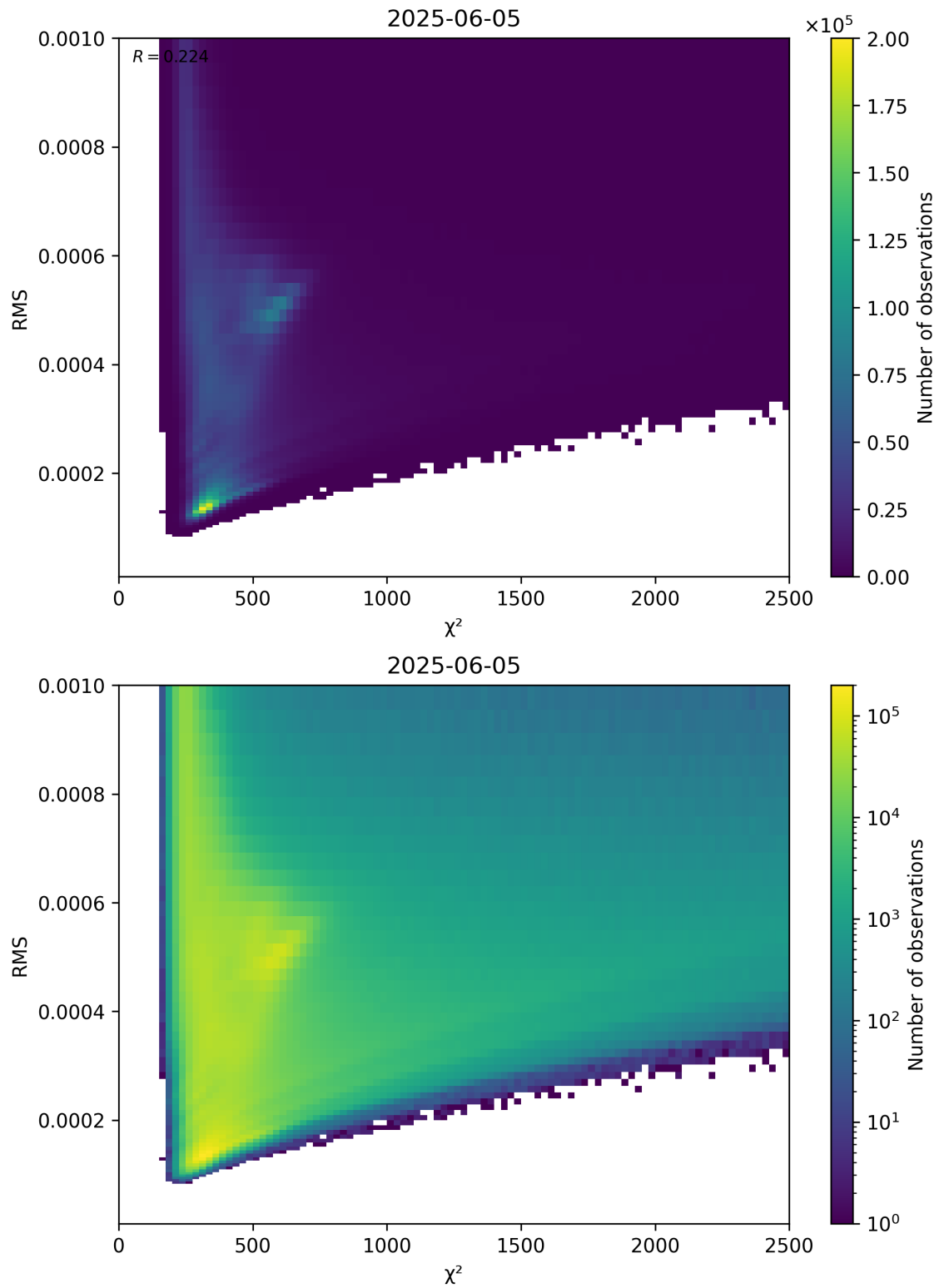
Figure 82: Scatter density plot of “ \chi^2 ” against “RMS” for 2025-06-04 to 2025-06-06.
