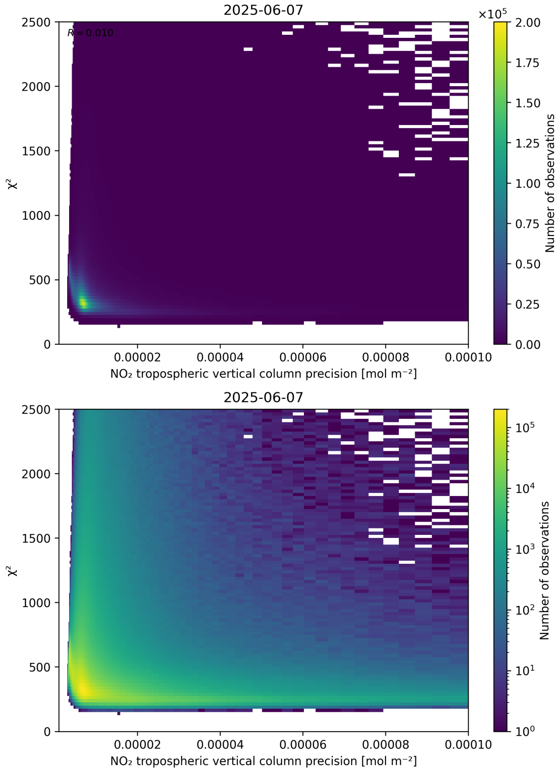
Figure 134: Scatter density plot of “NO 2 tropospheric vertical column precision” against “ \chi^2 ” for 2025-06-06 to 2025-06-08.
