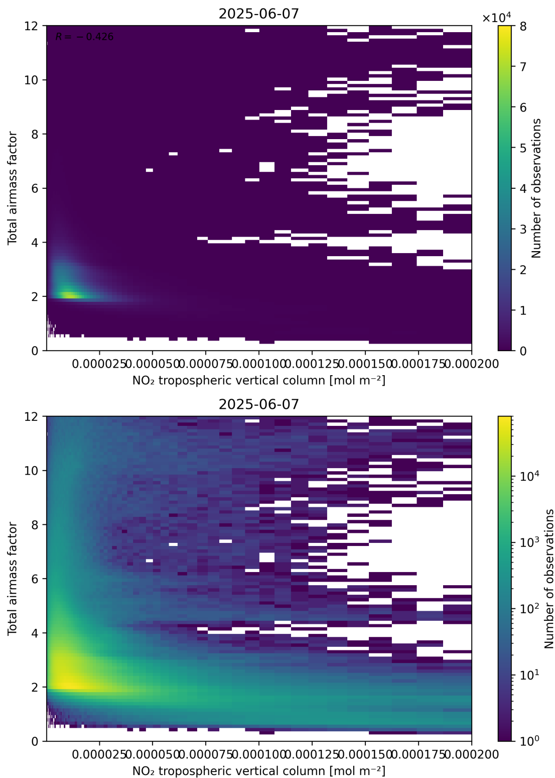
Figure 122: Scatter density plot of “NO 2 tropospheric vertical column” against “Total air mass factor” for 2025-06-06 to 2025-06-08.
