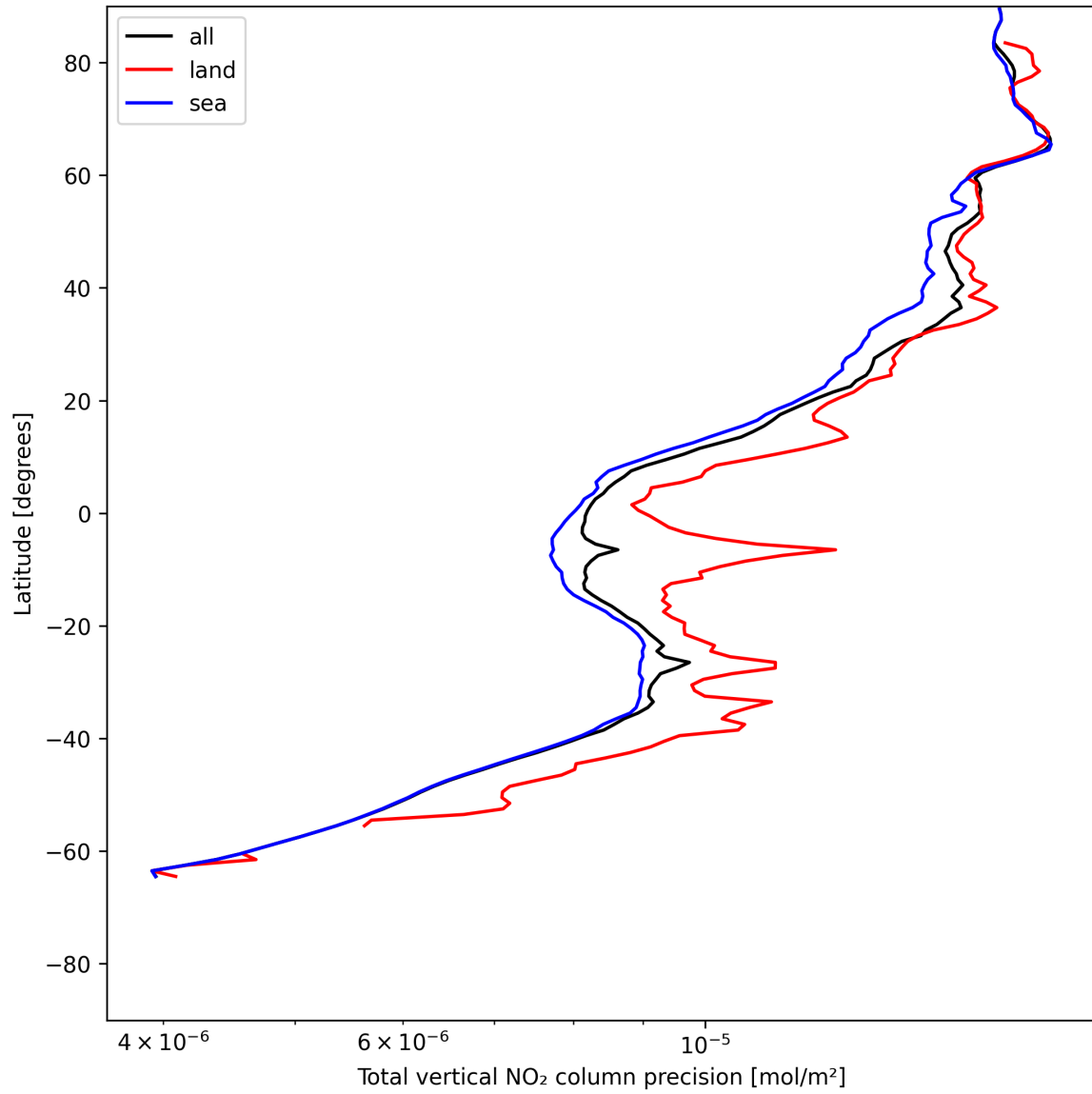
Figure 22: Zonal average of “Total vertical NO 2 column precision” for 2025-06-06 to 2025-06-08.
