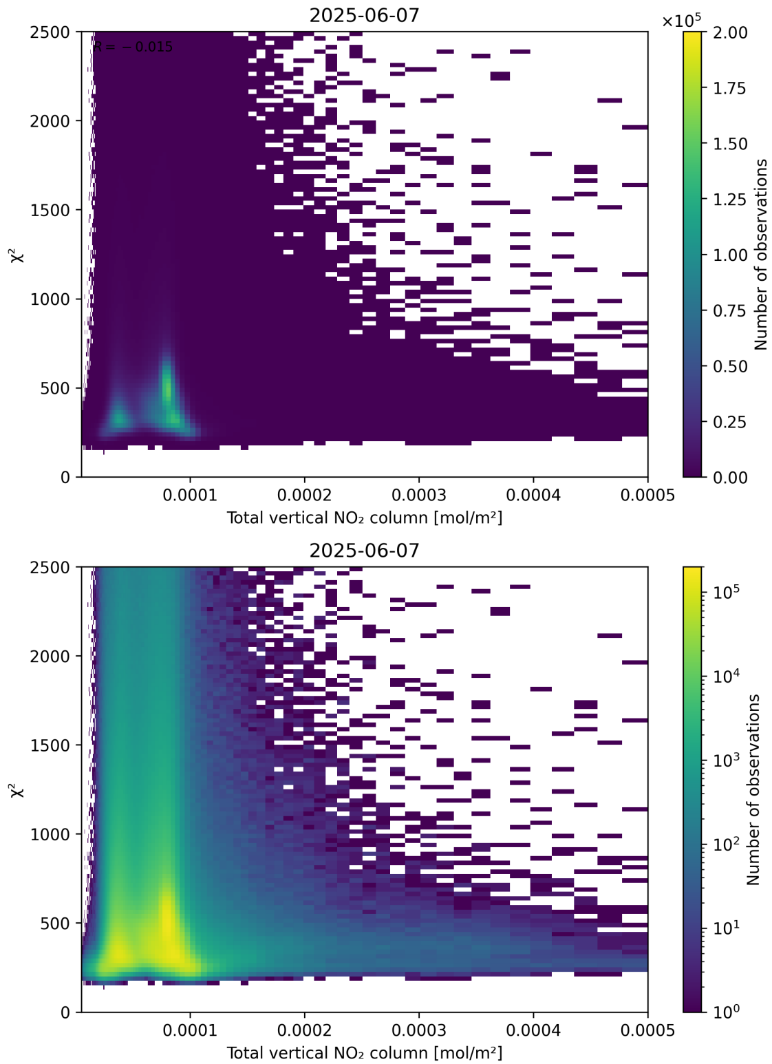
Figure 111: Scatter density plot of “Total vertical NO 2 column” against “ \chi^2 ” for 2025-06-06 to 2025-06-08.
