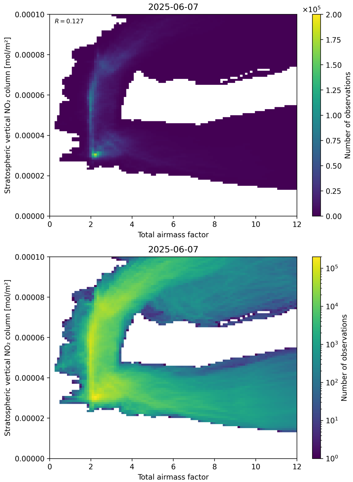
Figure 64: Scatter density plot of “Total airmass factor” against “Stratospheric vertical NO 2 column” for 2025-06-06 to 2025-06-08.
