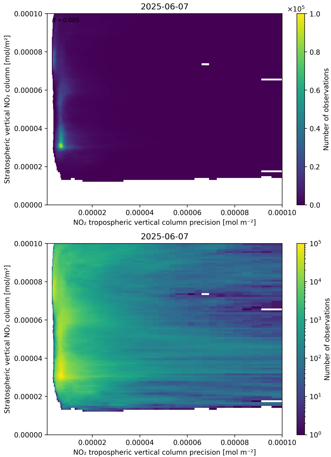
Figure 135: Scatter density plot of “NO 2 tropospheric vertical column precision” against “Stratospheric vertical NO 2 column” for 2025-06-06 to 2025-06-08.
