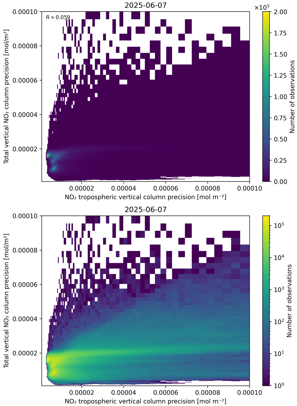
Figure 139: Scatter density plot of “NO 2 tropospheric vertical column precision” against “Total vertical NO 2 column precision” for 2025-06-06 to 2025-06-08.
