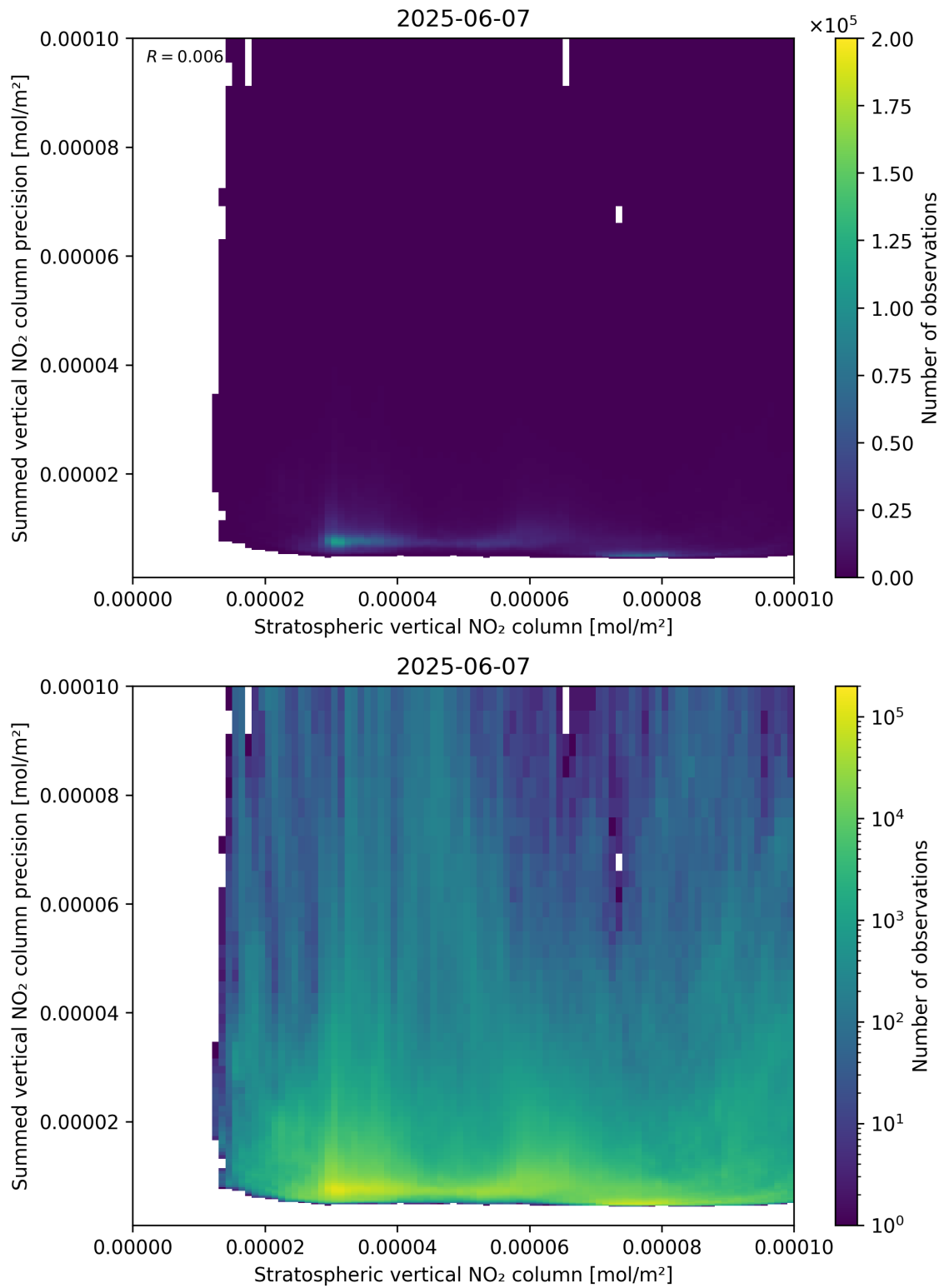
Figure 99: Scatter density plot of “Stratospheric vertical NO 2 column” against “Summed vertical NO 2 column precision” for 2025-06-06 to 2025-06-08.
