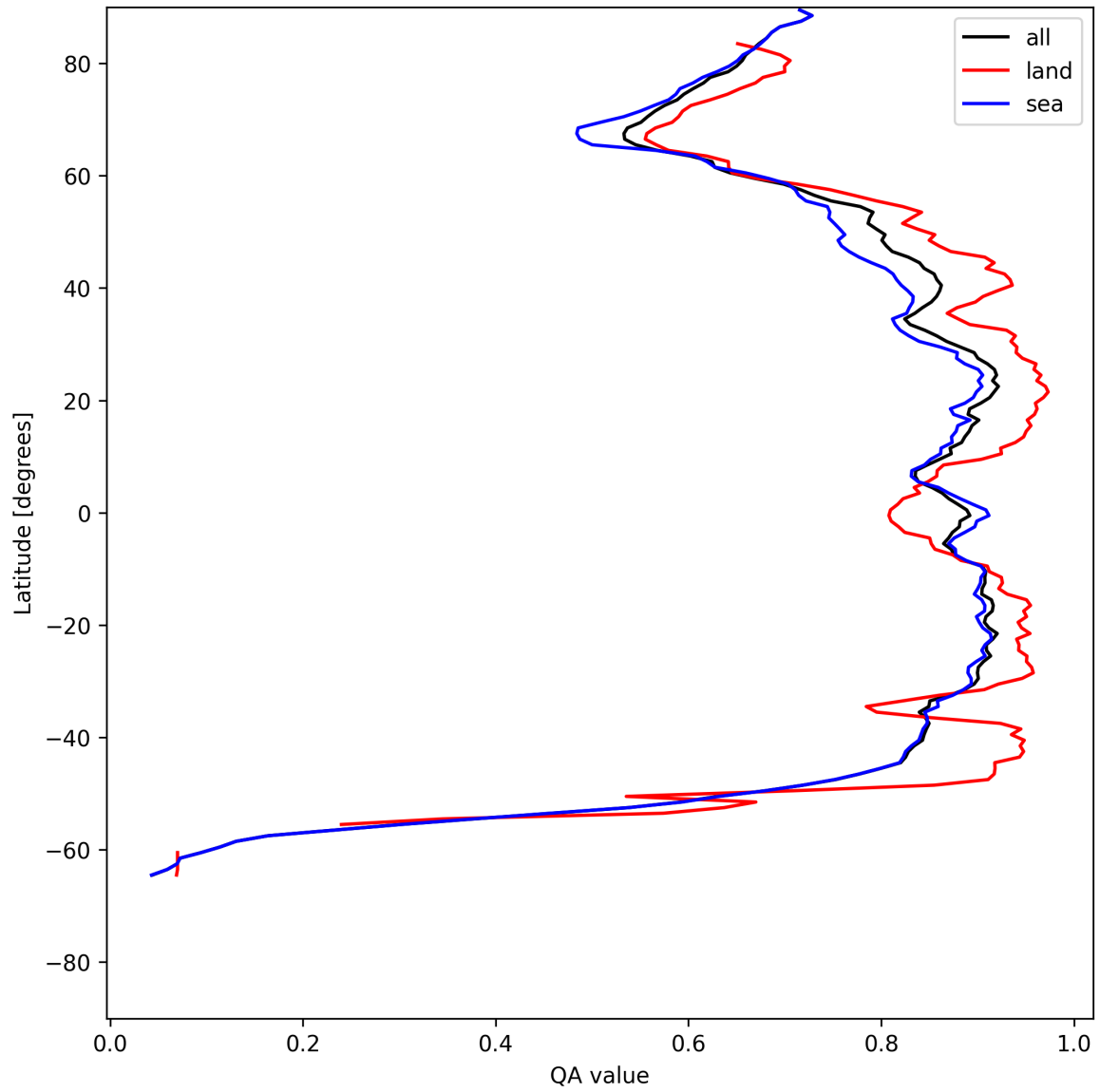
Figure 11: Zonal average of “QA value” for 2025-06-06 to 2025-06-08.
