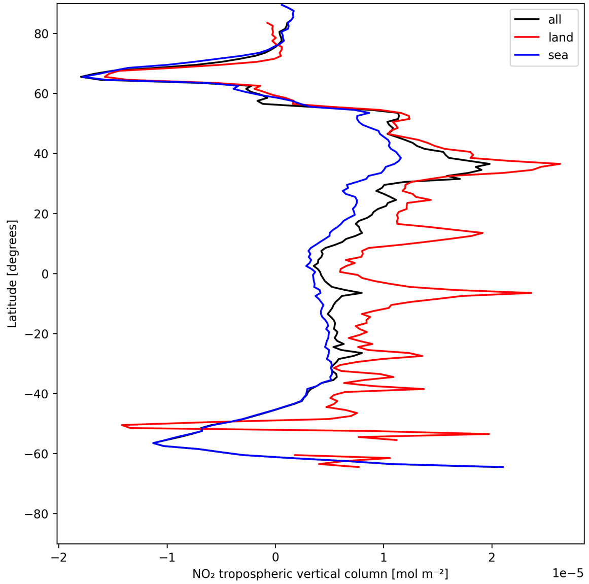
Figure 12: Zonal average of “NO 2 tropospheric vertical column” for 2025-06-06 to 2025-06-08.
