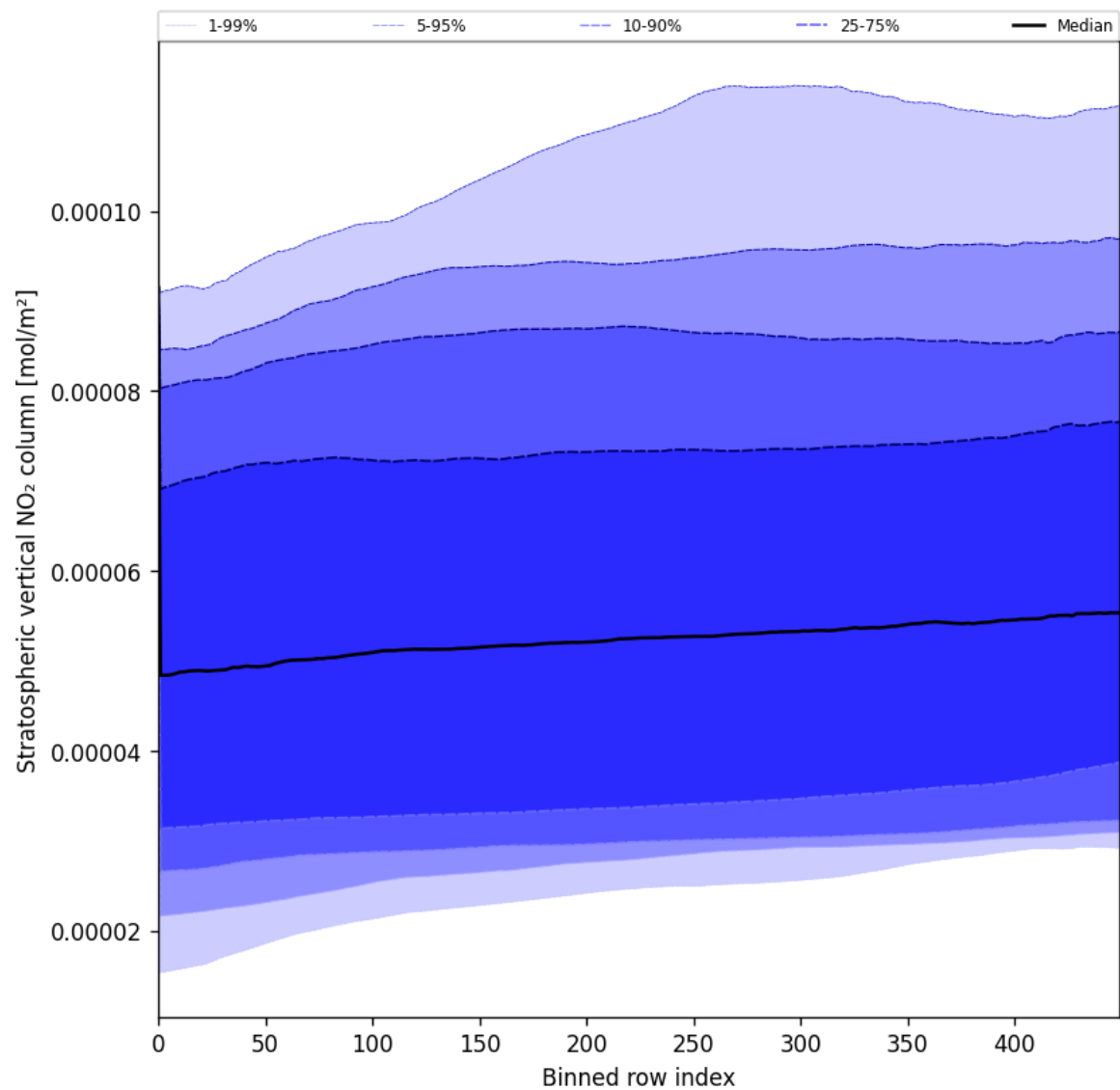
Figure 53: Along track statistics of “Stratospheric vertical NO 2 column” for 2025-06-06 to 2025-06-08
