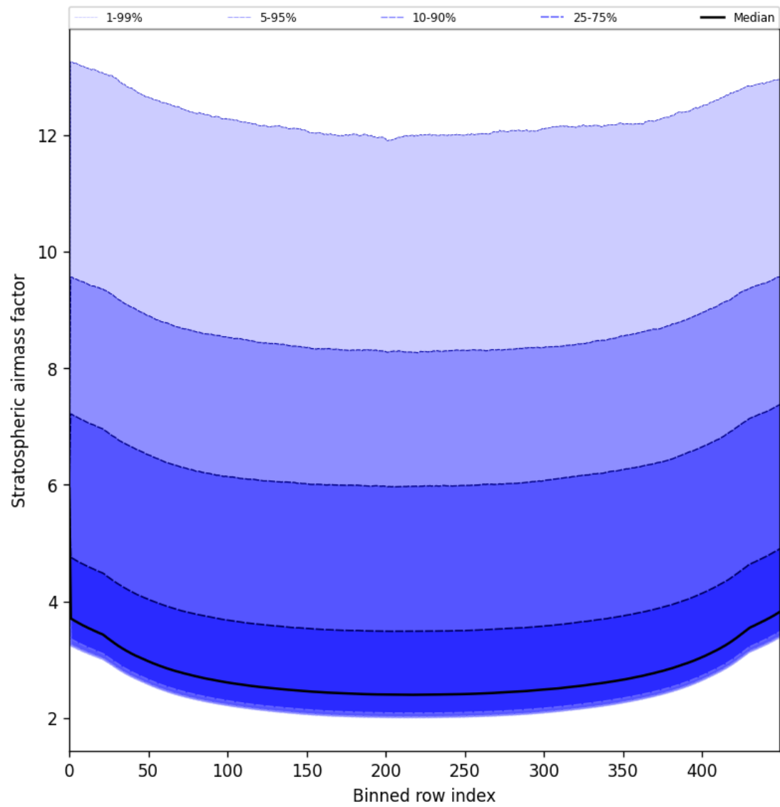
Figure 61: Along track statistics of “Stratospheric airmass factor” for 2025-06-06 to 2025-06-08
