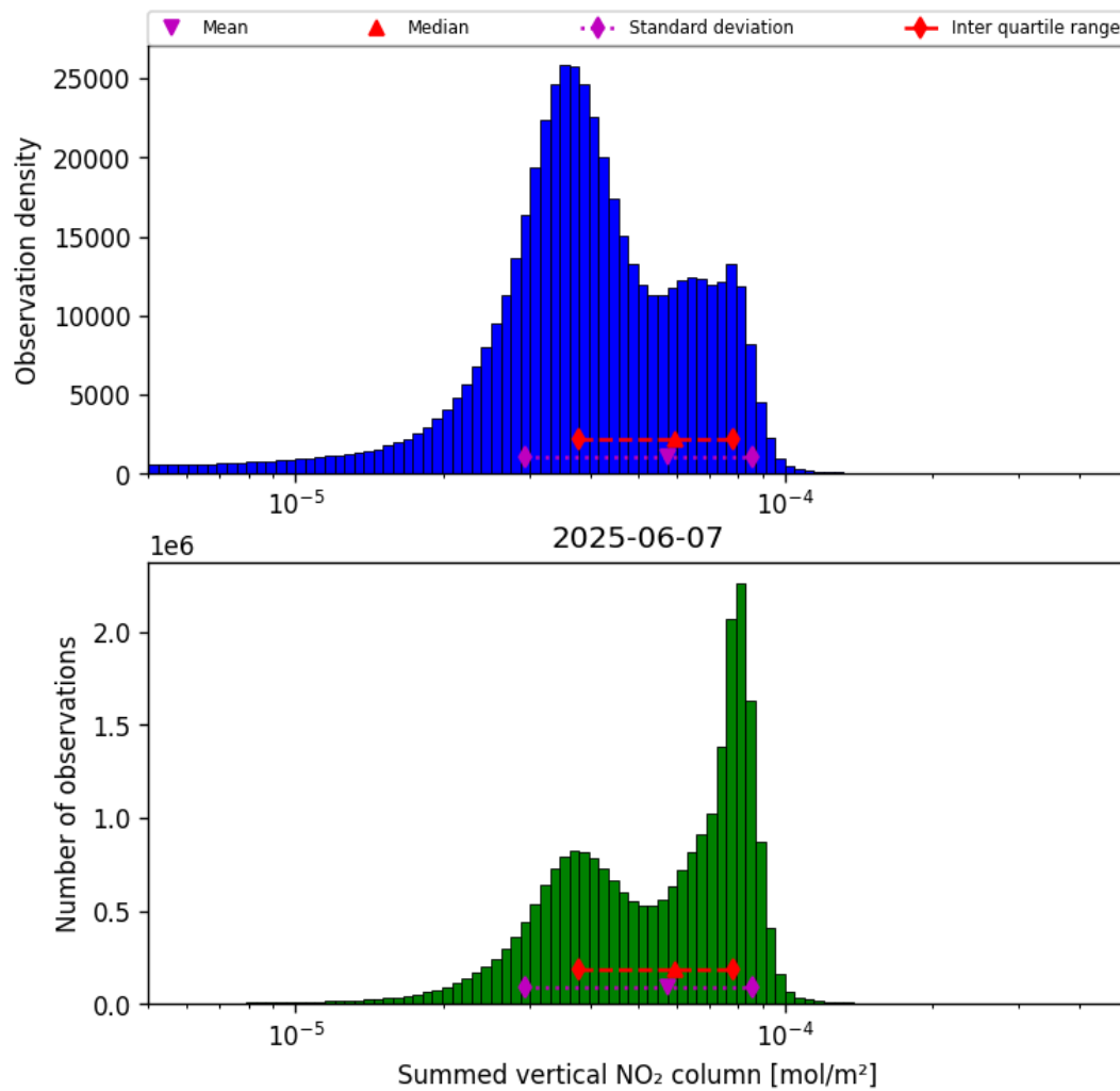
Figure 40: Histogram of “Summed vertical NO 2 column” for 2025-06-06 to 2025-06-08
