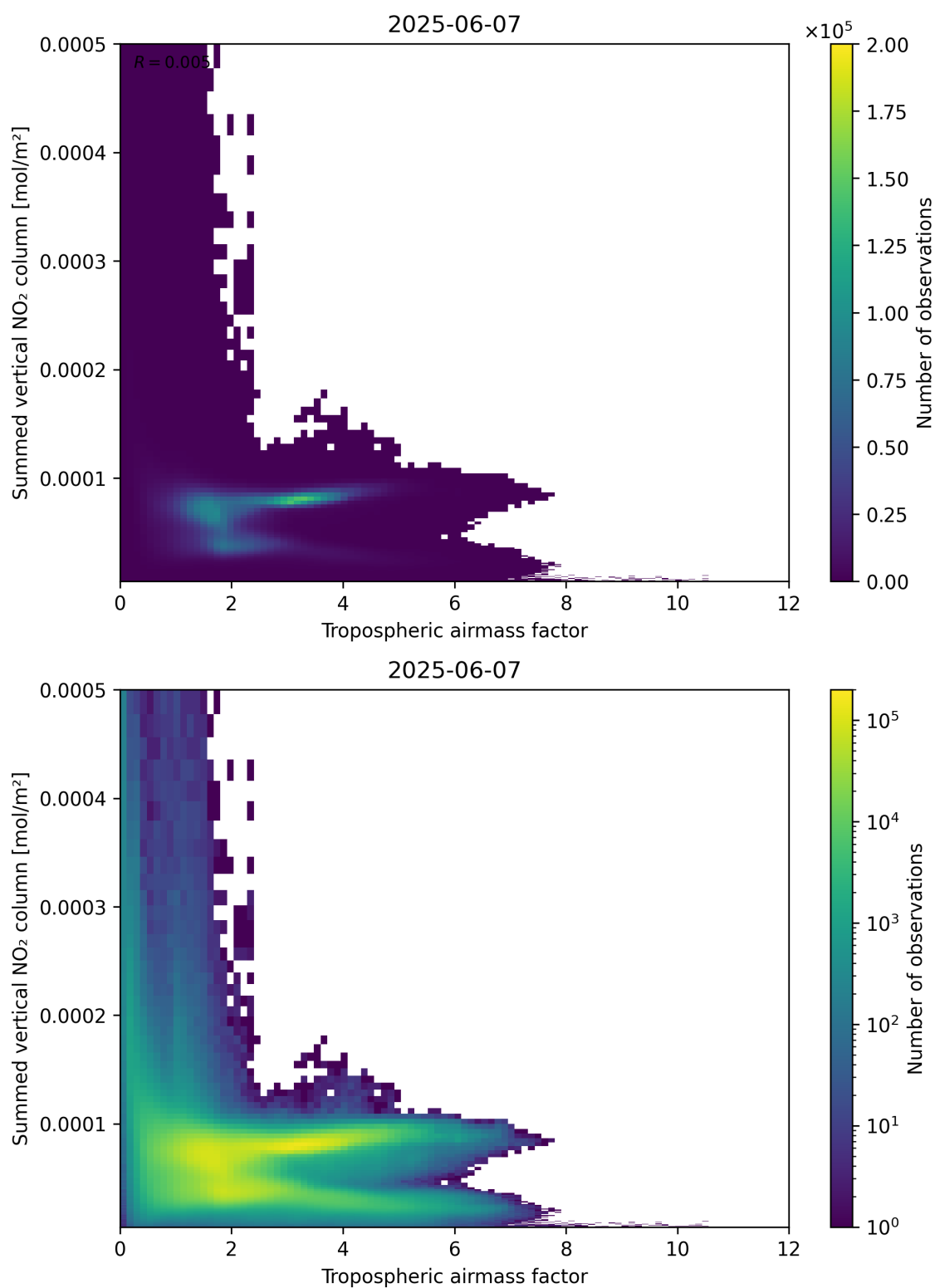
Figure 75: Scatter density plot of “Tropospheric airmass factor” against “Summed vertical NO 2 column” for 2025-06-06 to 2025-06-08.
