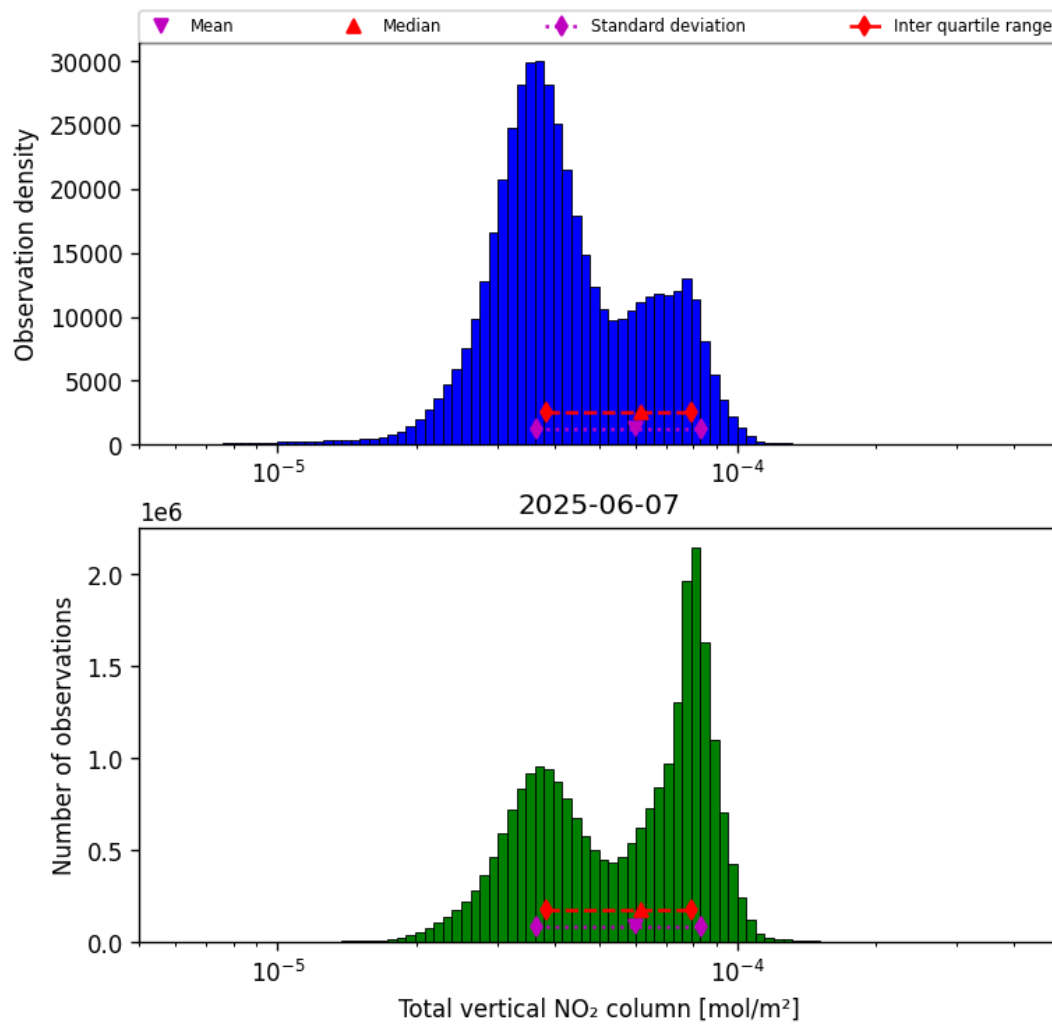
Figure 38: Histogram of “Total vertical NO 2 column” for 2025-06-06 to 2025-06-08
