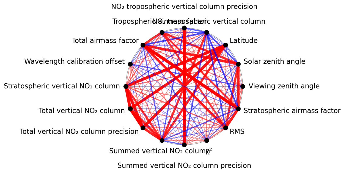
Figure 1: Map of correlation graph for 2025-06-06 to 2025-06-08.
