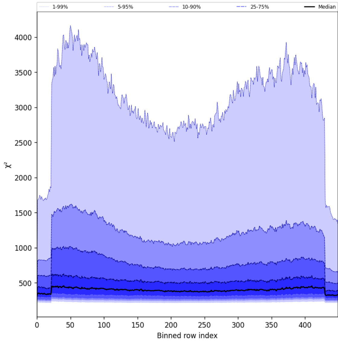
Figure 59: Along track statistics of “ \chi^2 ” for 2025-06-06 to 2025-06-08
