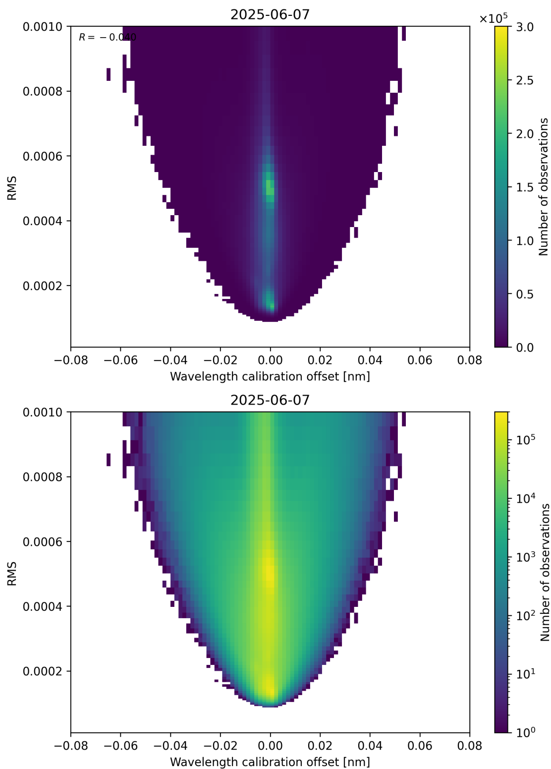
Figure 181: Scatter density plot of “Wavelength calibration offset” against “RMS” for 2025-06-06 to 2025-06-08.
