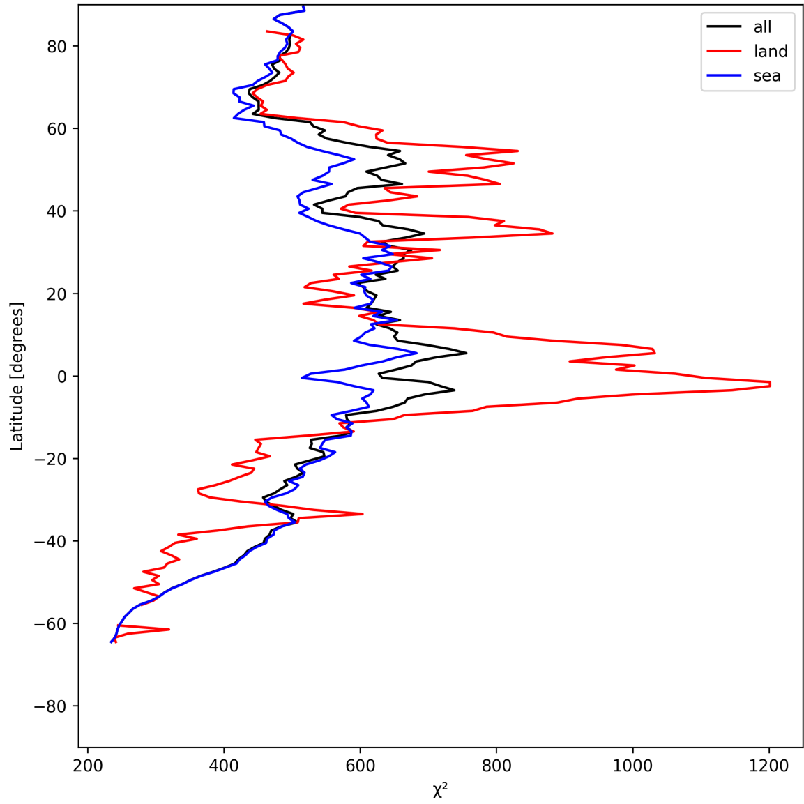
Figure 25: Zonal average of “ \chi^2 ” for 2025-06-06 to 2025-06-08.
