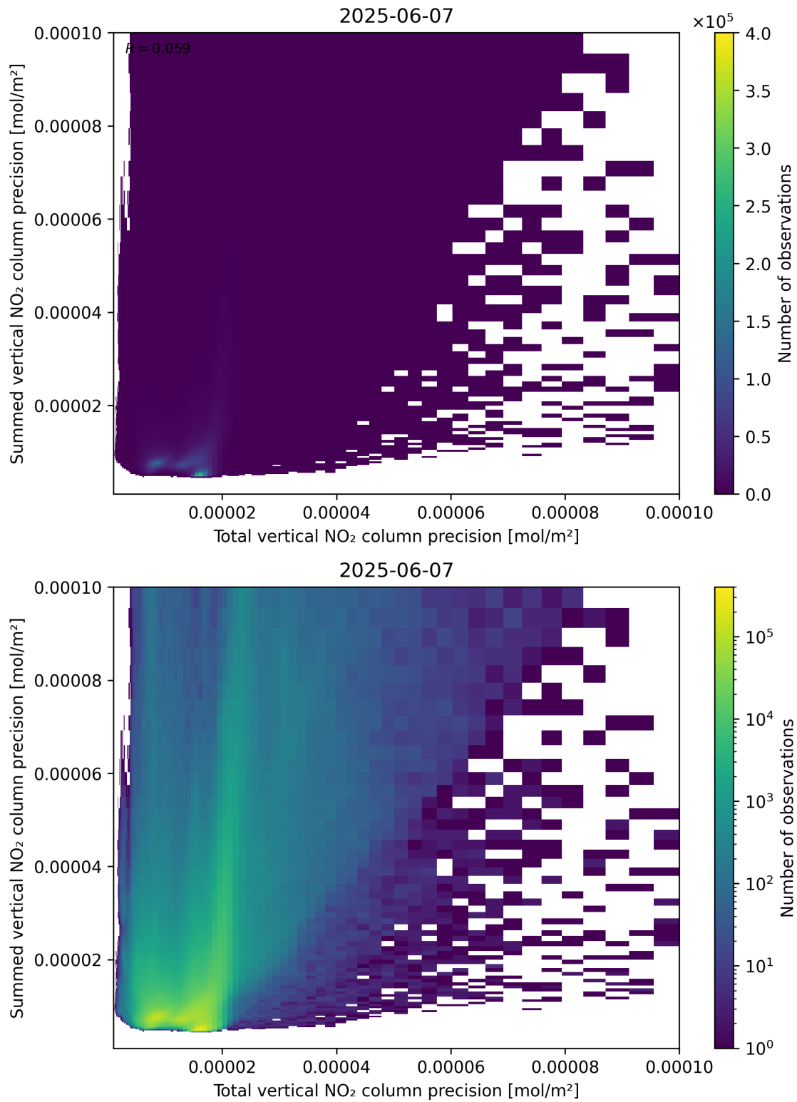
Figure 118: Scatter density plot of “Total vertical NO 2 column precision” against “Summed vertical NO 2 column precision” for 2025-06-06 to 2025-06-08.
