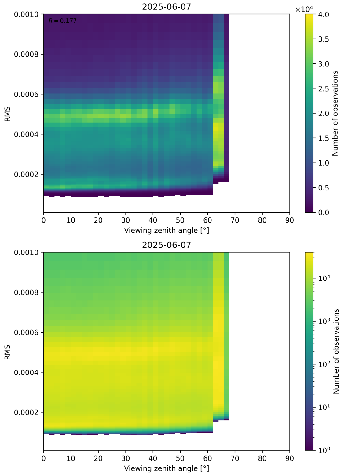
Figure 171: Scatter density plot of “Viewing zenith angle” against “RMS” for 2025-06-06 to 2025-06-08.
