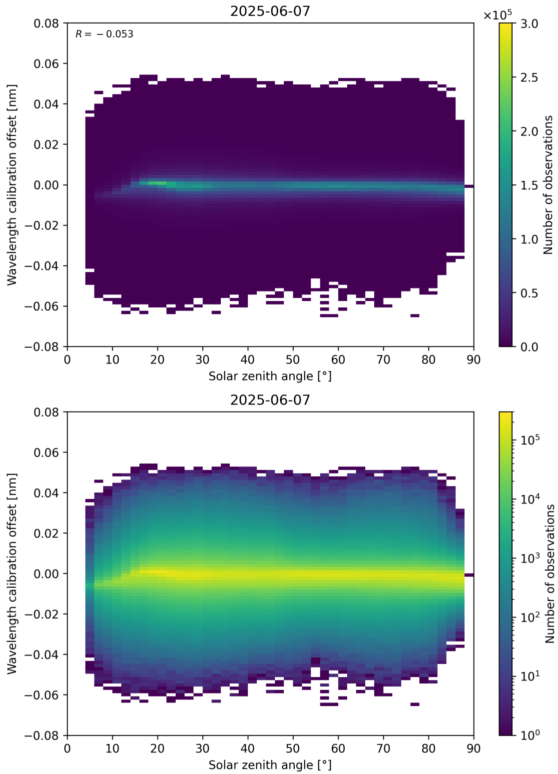
Figure 158: Scatter density plot of “Solar zenith angle” against “Wavelength calibration offset” for 2025-06-06 to 2025-06-08.
