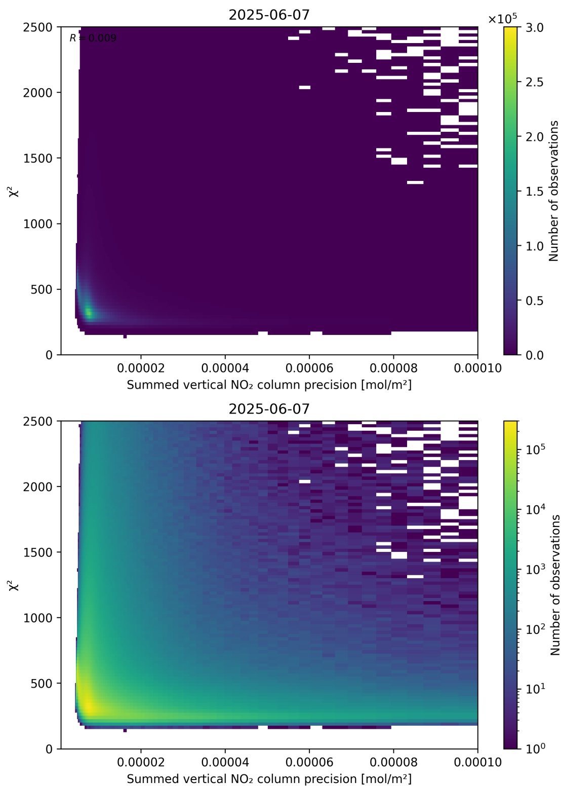
Figure 107: Scatter density plot of “Summed vertical NO 2 column precision” against “ \chi^2 ” for 2025-06-06 to 2025-06-08.
