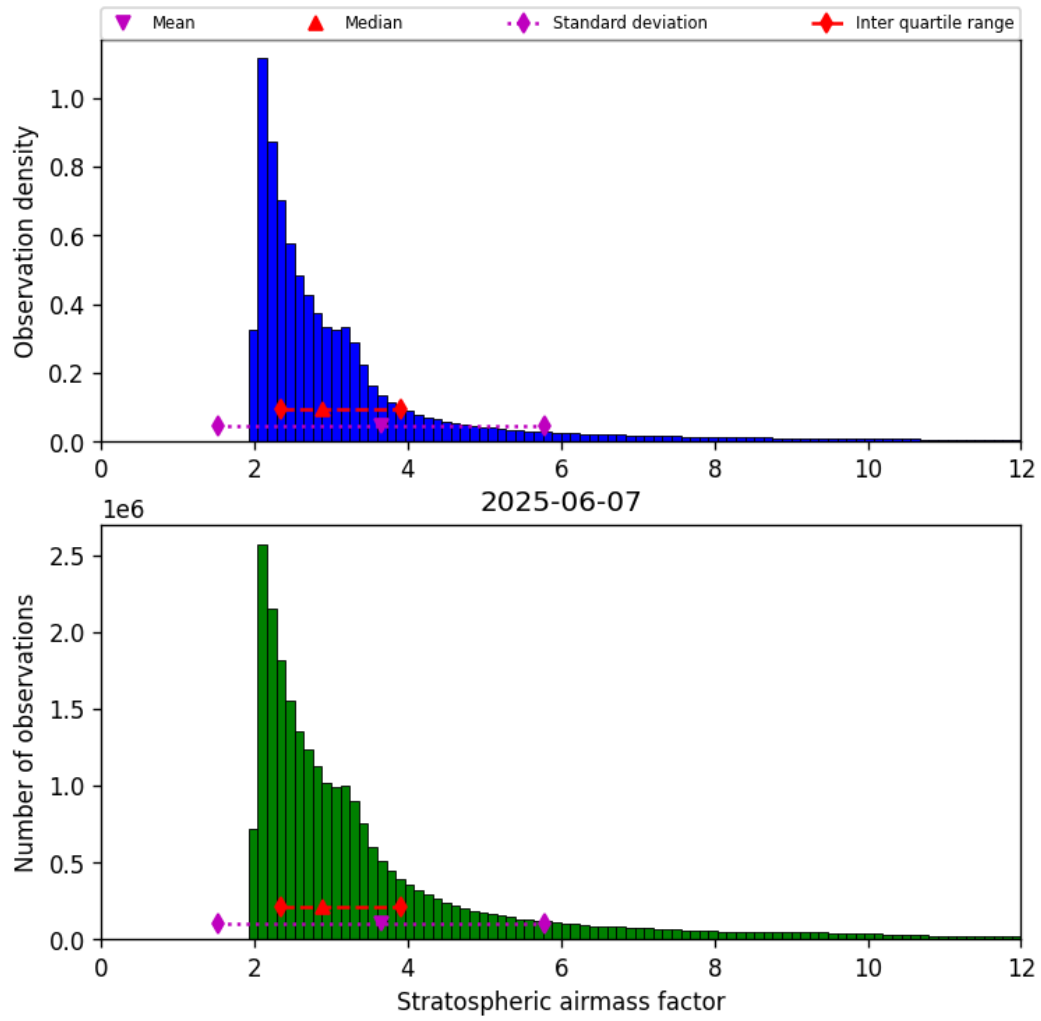
Figure 44: Histogram of “Stratospheric airmass factor” for 2025-06-06 to 2025-06-08
