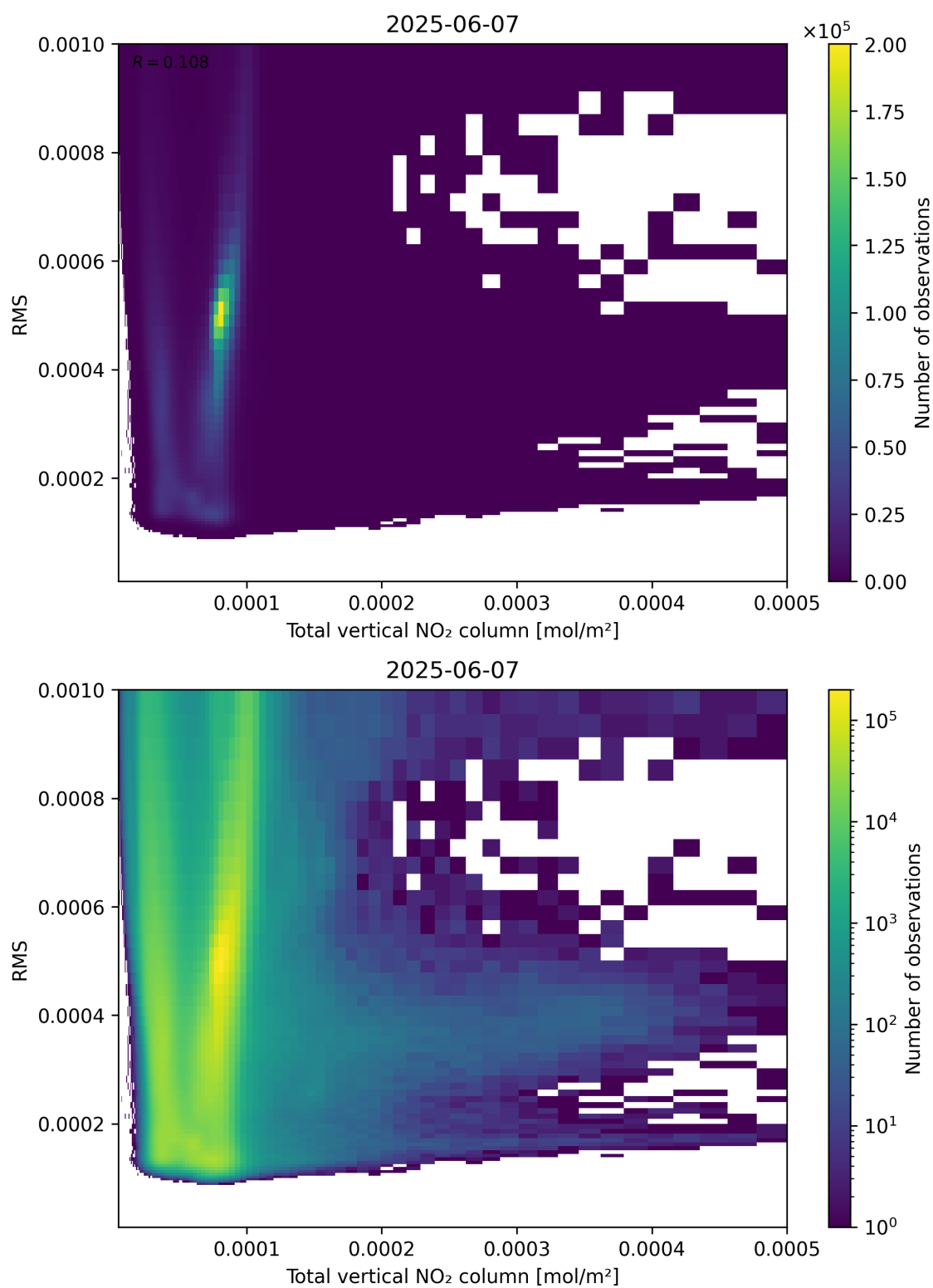
Figure 120: Scatter density plot of “Total vertical NO 2 column” against “RMS” for 2025-06-06 to 2025-06-08.
