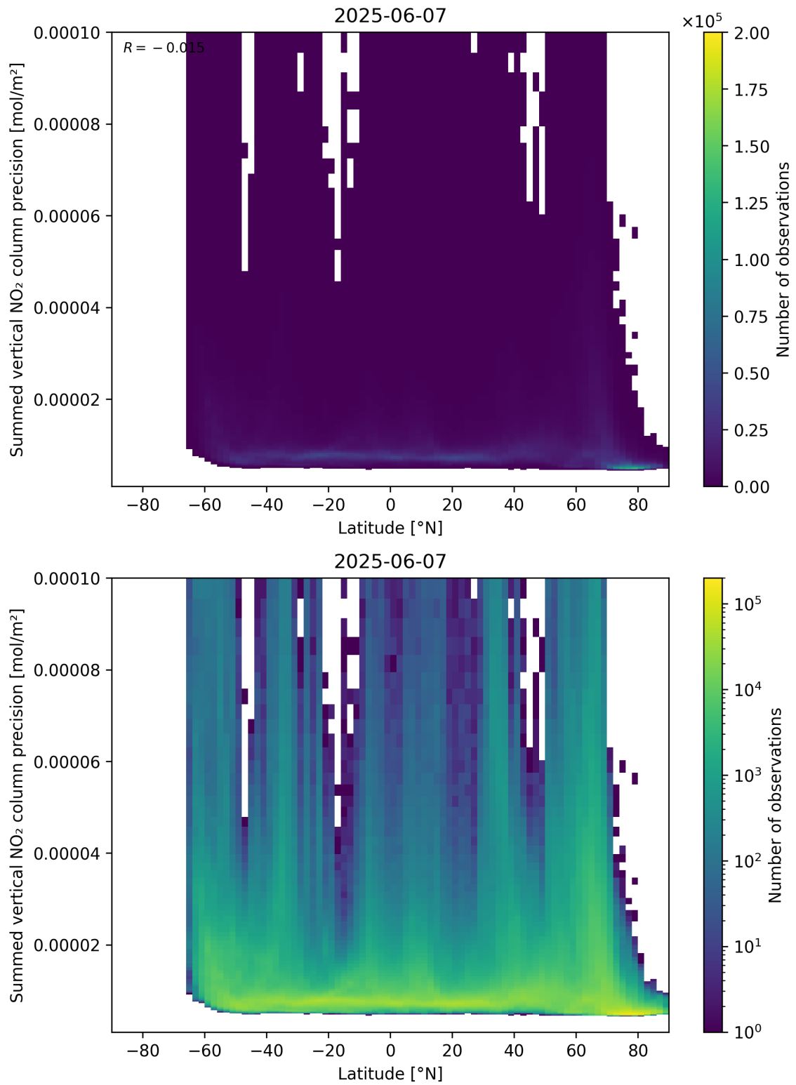
Figure 89: Scatter density plot of “Latitude” against “Summed vertical NO 2 column precision” for 2025-06-06 to 2025-06-08.
