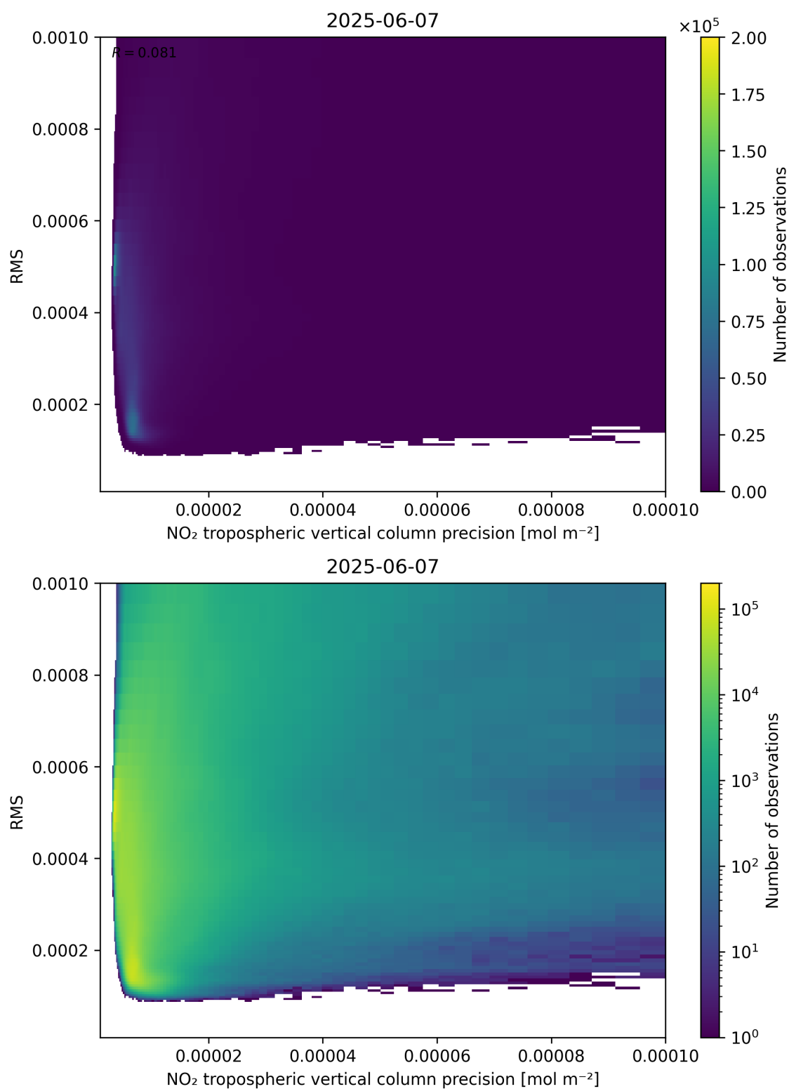
Figure 140: Scatter density plot of “NO 2 tropospheric vertical column precision” against “RMS” for 2025-06-06 to 2025-06-08.
