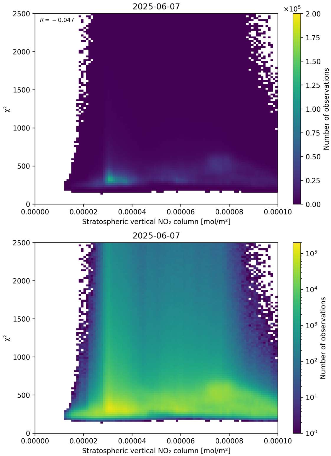
Figure 97: Scatter density plot of “Stratospheric vertical NO 2 column” against “ \chi^2 ” for 2025-06-06 to 2025-06-08.
