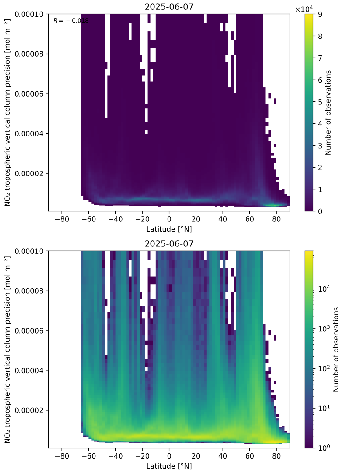
Figure 93: Scatter density plot of “Latitude” against “NO 2 tropospheric vertical column precision” for 2025-06-06 to 2025-06-08.
