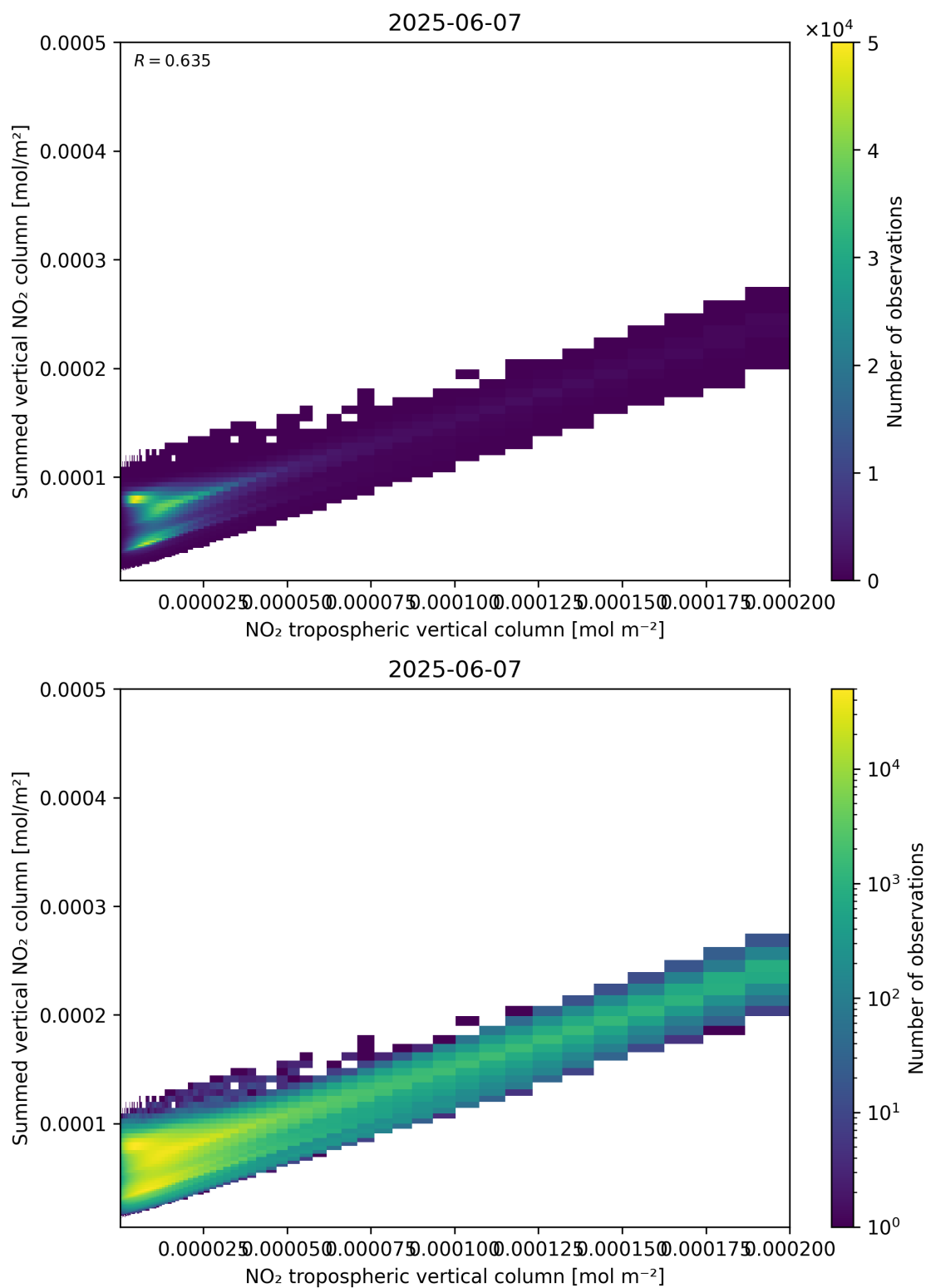
Figure 126: Scatter density plot of “NO 2 tropospheric vertical column” against “Summed vertical NO 2 column” for 2025-06-06 to 2025-06-08.
