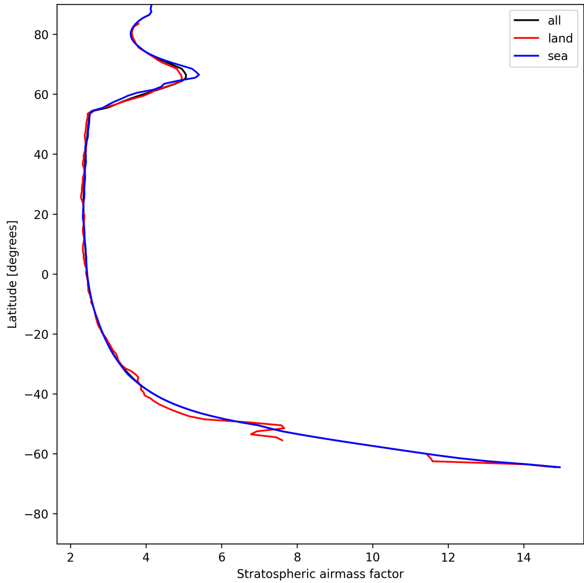
Figure 27: Zonal average of “Stratospheric air mass factor” for 2025-06-06 to 2025-06-08.
