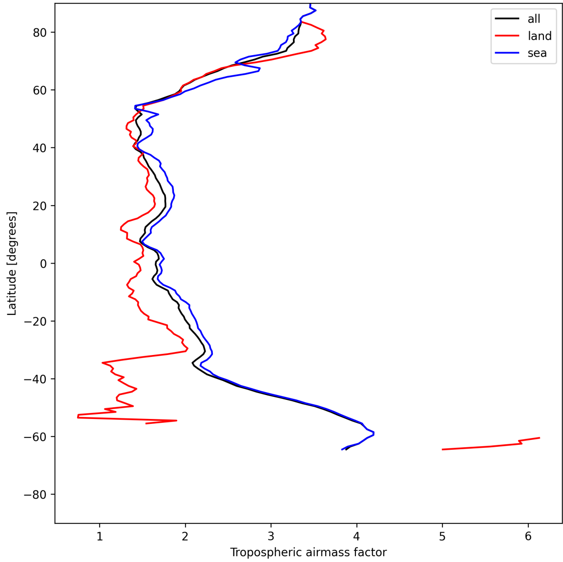
Figure 14: Zonal average of “Tropospheric air mass factor” for 2025-06-06 to 2025-06-08.
