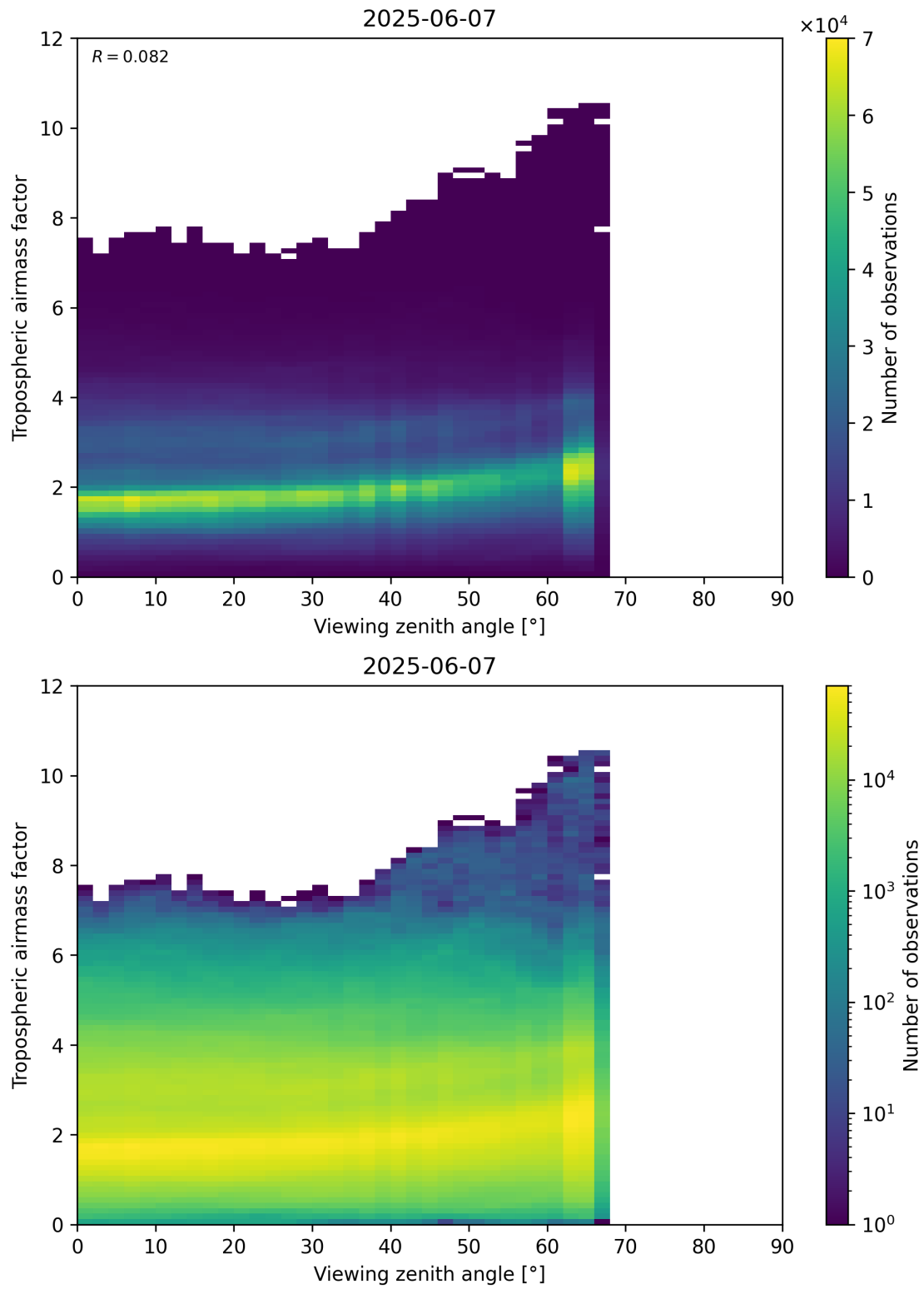
Figure 161: Scatter density plot of “Viewing zenith angle” against “Tropospheric airmass factor” for 2025-06-06 to 2025-06-08.
