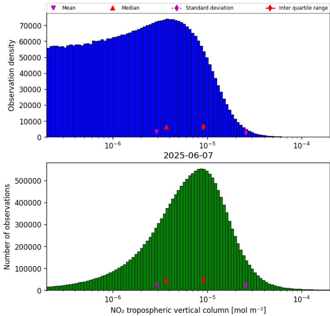
Figure 29: Histogram of “NO 2 tropospheric vertical column” for 2025-06-06 to 2025-06-08
