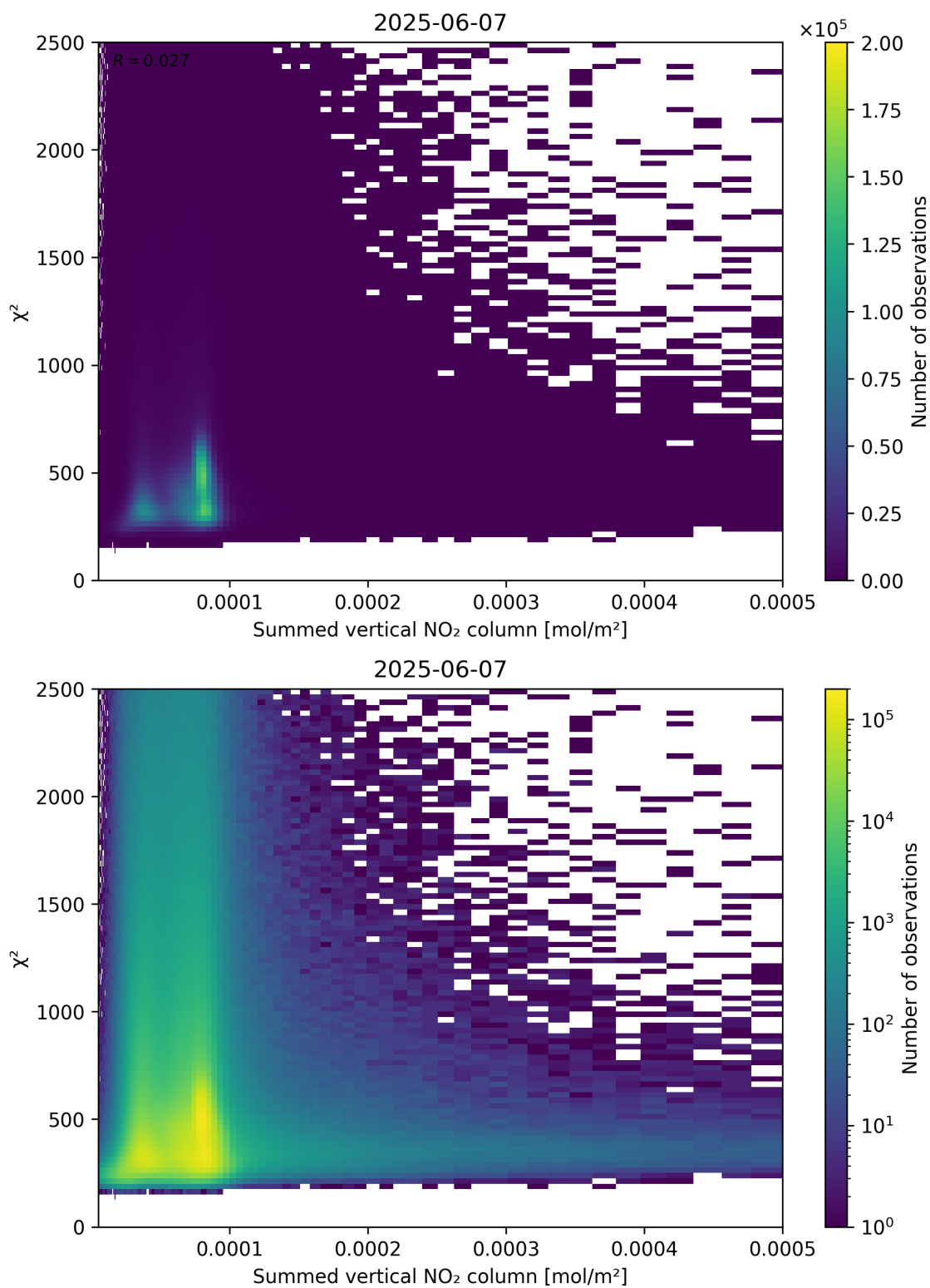
Figure 104: Scatter density plot of “Summed vertical NO 2 column” against “ \chi^2 ” for 2025-06-06 to 2025-06-08.
