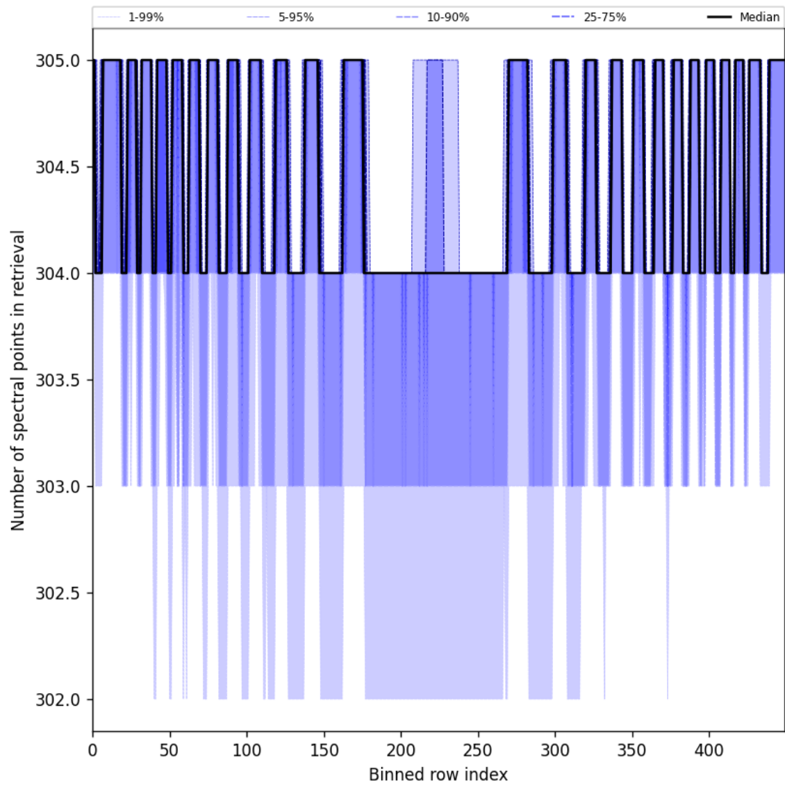
Figure 50: Along track statistics of “Number of spectral points in retrieval” for 2025-06-06 to 2025-06-08
