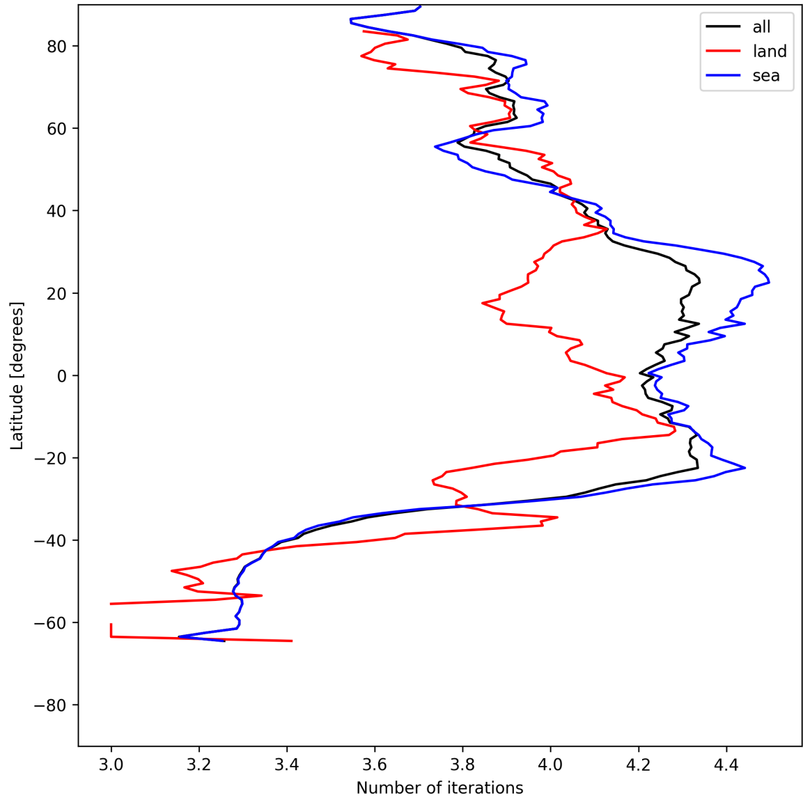
Figure 17: Zonal average of “Number of iterations” for 2025-06-06 to 2025-06-08.
