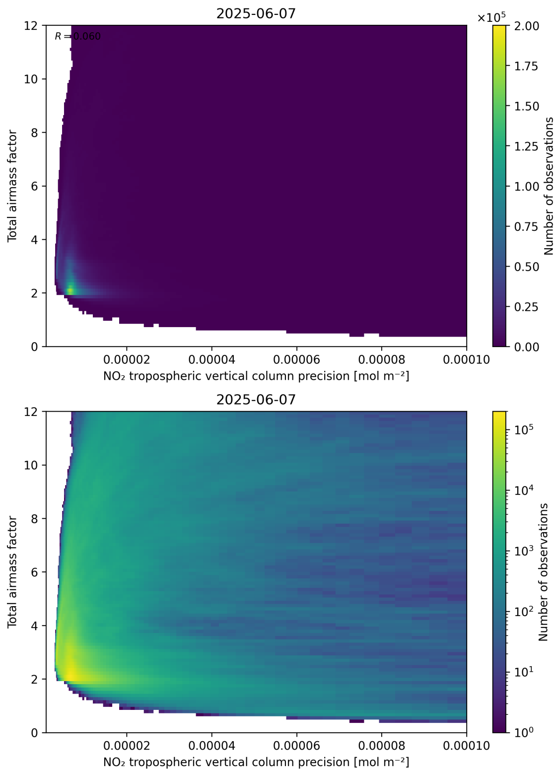
Figure 132: Scatter density plot of “NO 2 tropospheric vertical column precision” against “Total air mass factor” for 2025-06-06 to 2025-06-08.
