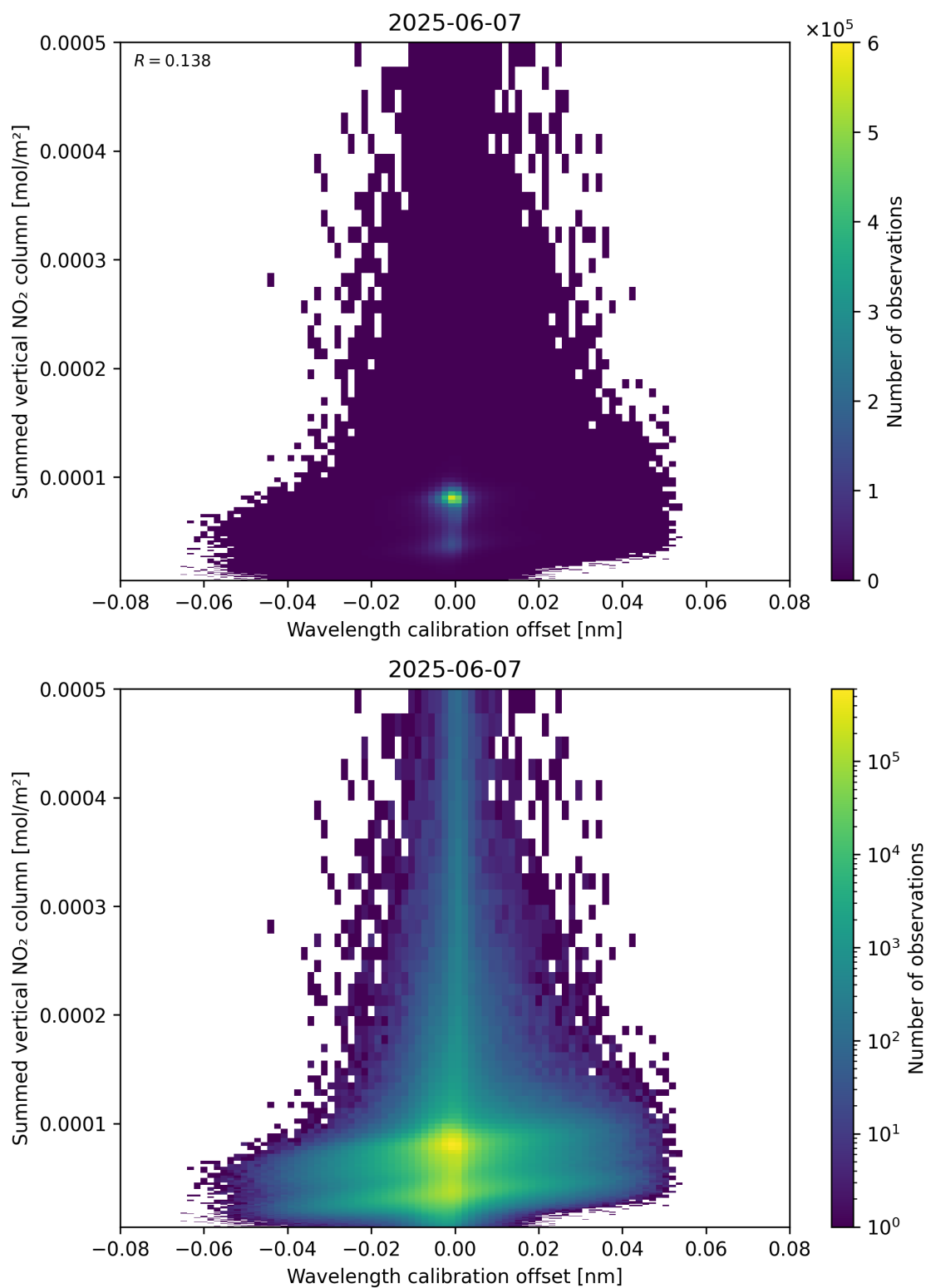
Figure 177: Scatter density plot of “Wavelength calibration offset” against “Summed vertical NO 2 column” for 2025-06-06 to 2025-06-08.
