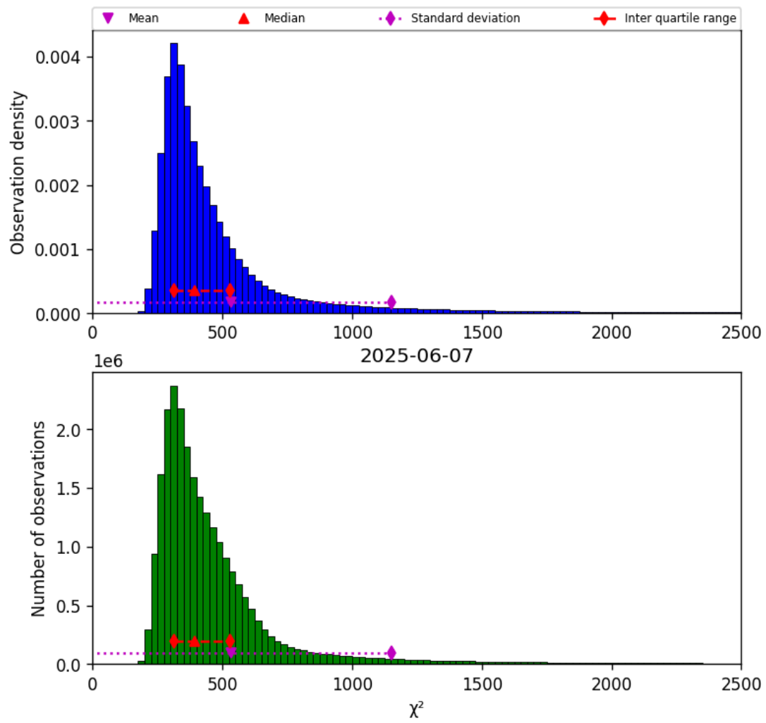
Figure 42: Histogram of “ \chi^2 ” for 2025-06-06 to 2025-06-08
