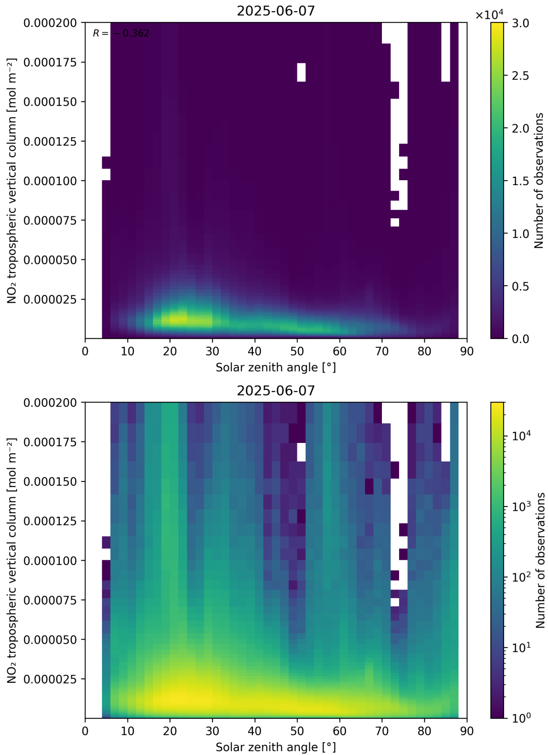
Figure 155: Scatter density plot of “Solar zenith angle” against “NO 2 tropospheric vertical column” for 2025-06-06 to 2025-06-08.
