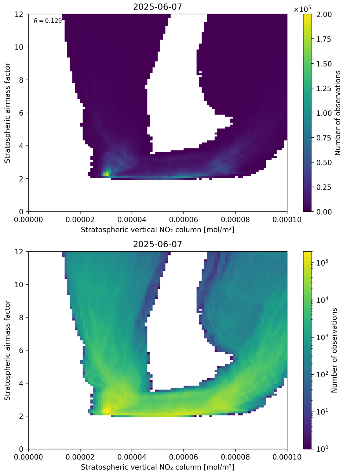
Figure 96: Scatter density plot of “Stratospheric vertical NO 2 column” against “Stratospheric airmass factor” for 2025-06-06 to 2025-06-08.
