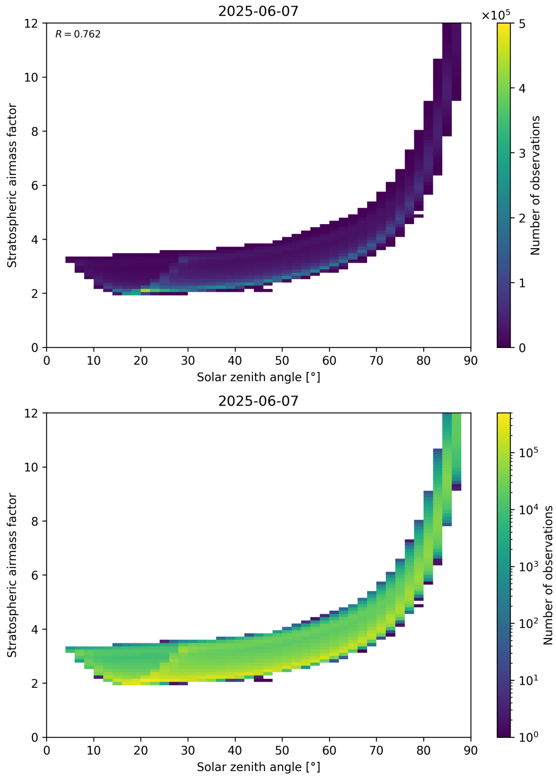
Figure 145: Scatter density plot of “Solar zenith angle” against “Stratospheric airmass factor” for 2025-06-06 to 2025-06-08.
