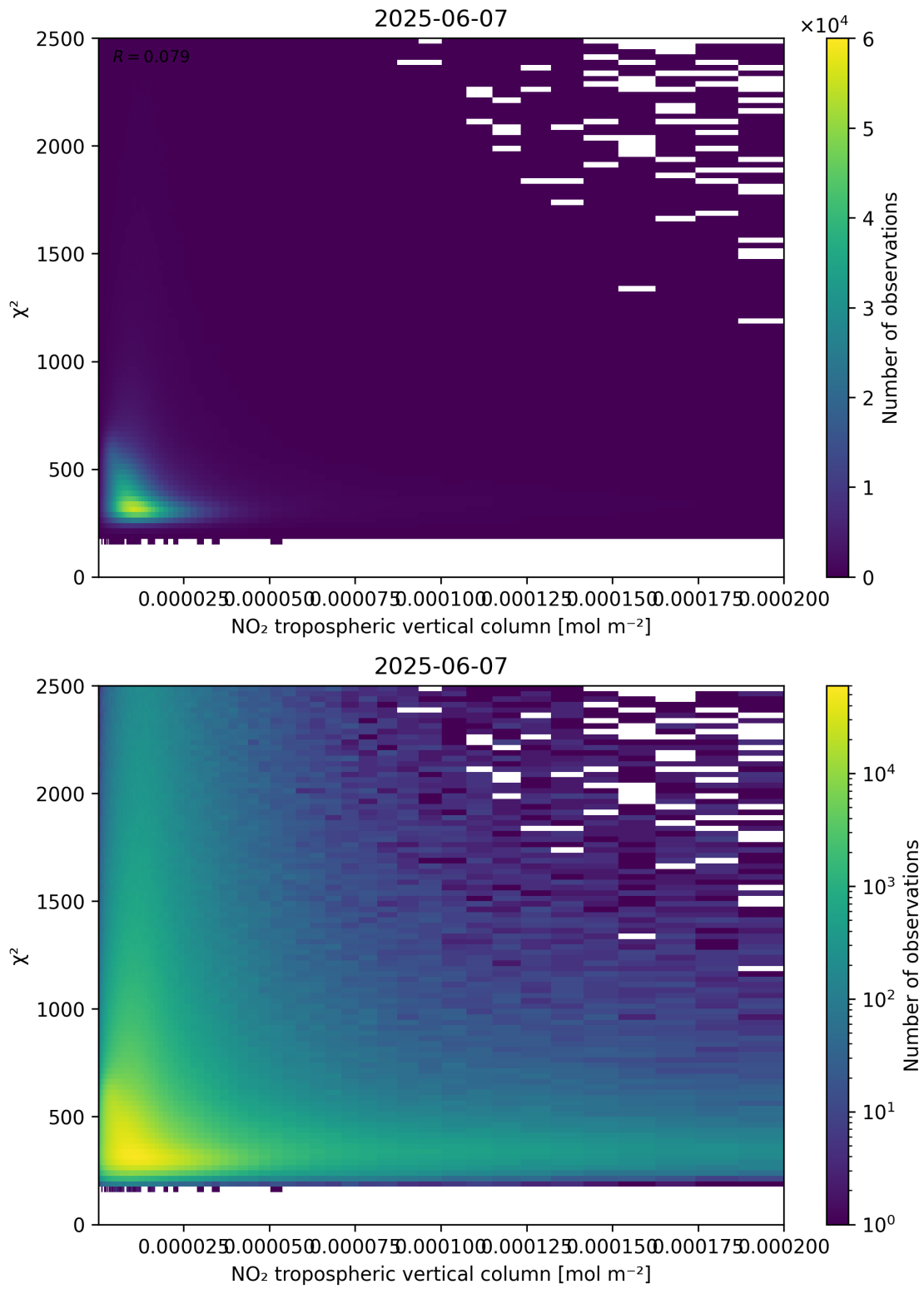
Figure 124: Scatter density plot of “NO 2 tropospheric vertical column” against “ \chi^2 ” for 2025-06-06 to 2025-06-08.
