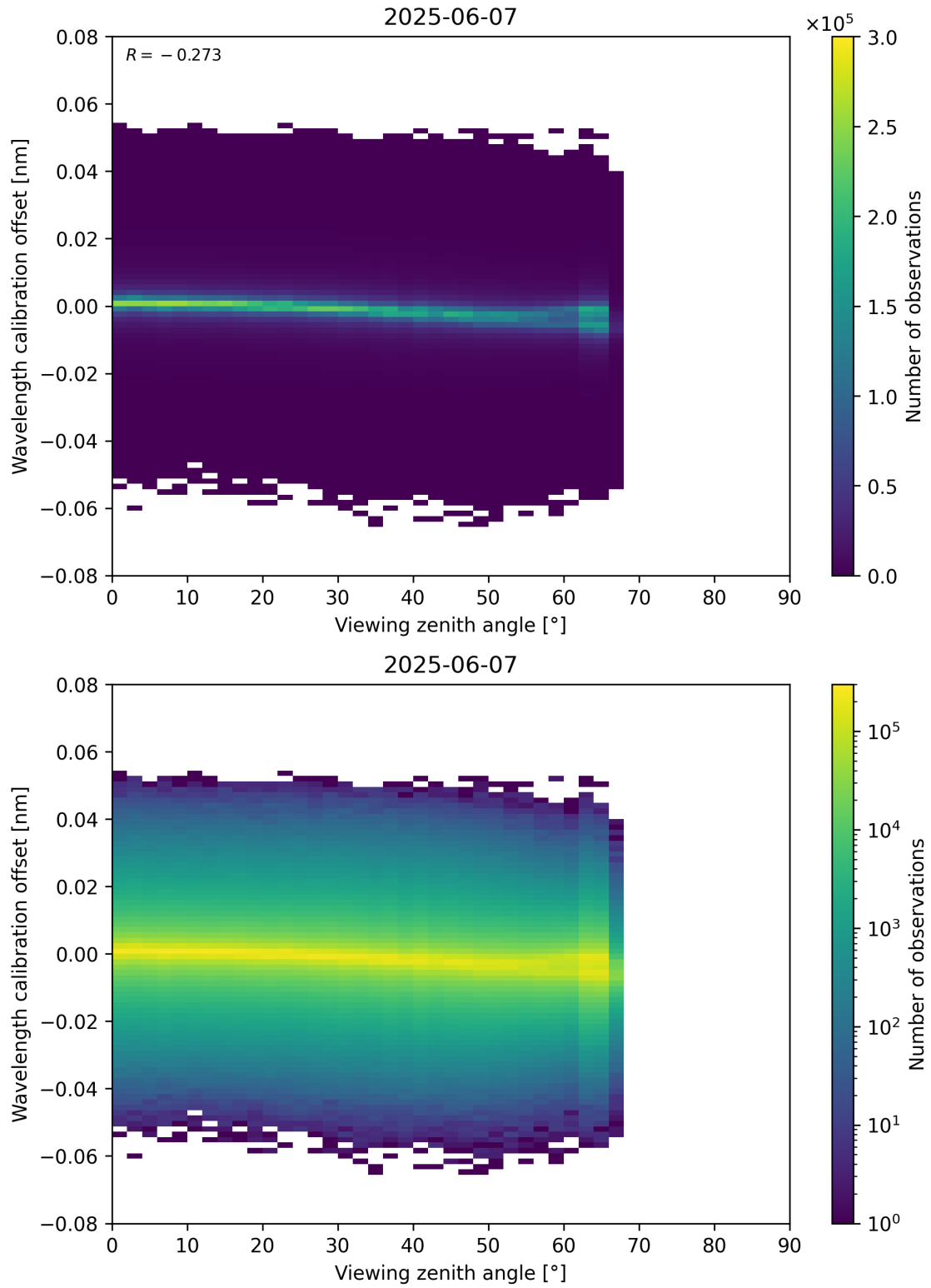
Figure 173: Scatter density plot of “Viewing zenith angle” against “Wavelength calibration offset” for 2025-06-06 to 2025-06-08.
