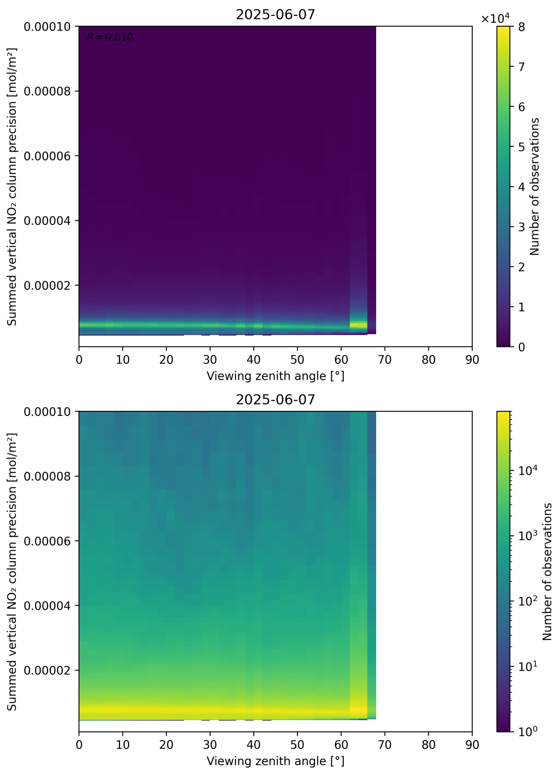
Figure 166: Scatter density plot of “Viewing zenith angle” against “Summed vertical NO 2 column precision” for 2025-06-06 to 2025-06-08.
