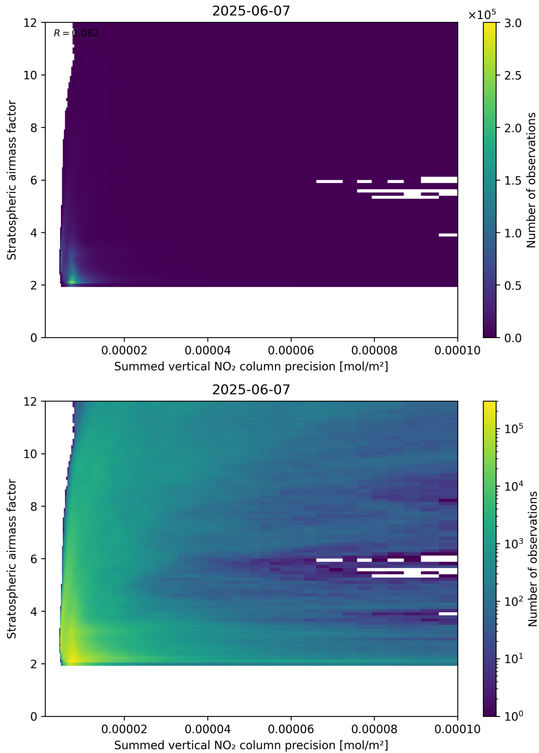
Figure 106: Scatter density plot of “Summed vertical NO 2 column precision” against “Stratospheric airmass factor” for 2025-06-06 to 2025-06-08.
