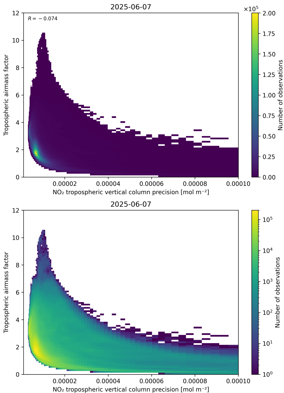
Figure 133: Scatter density plot of “NO 2 tropospheric vertical column precision” against “Tropospheric air mass factor” for 2025-06-06 to 2025-06-08.
