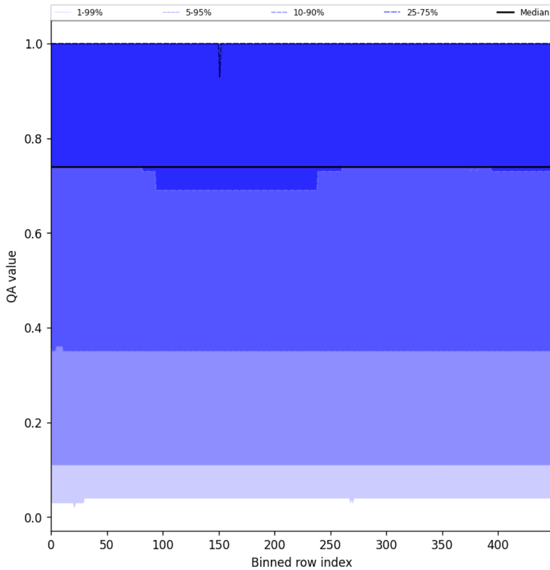
Figure 45: Along track statistics of “QA value” for 2025-06-06 to 2025-06-08
