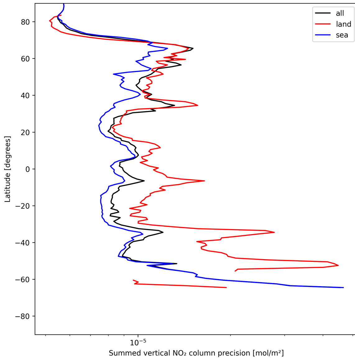
Figure 24: Zonal average of “Summed vertical NO 2 column precision” for 2025-06-06 to 2025-06-08.
