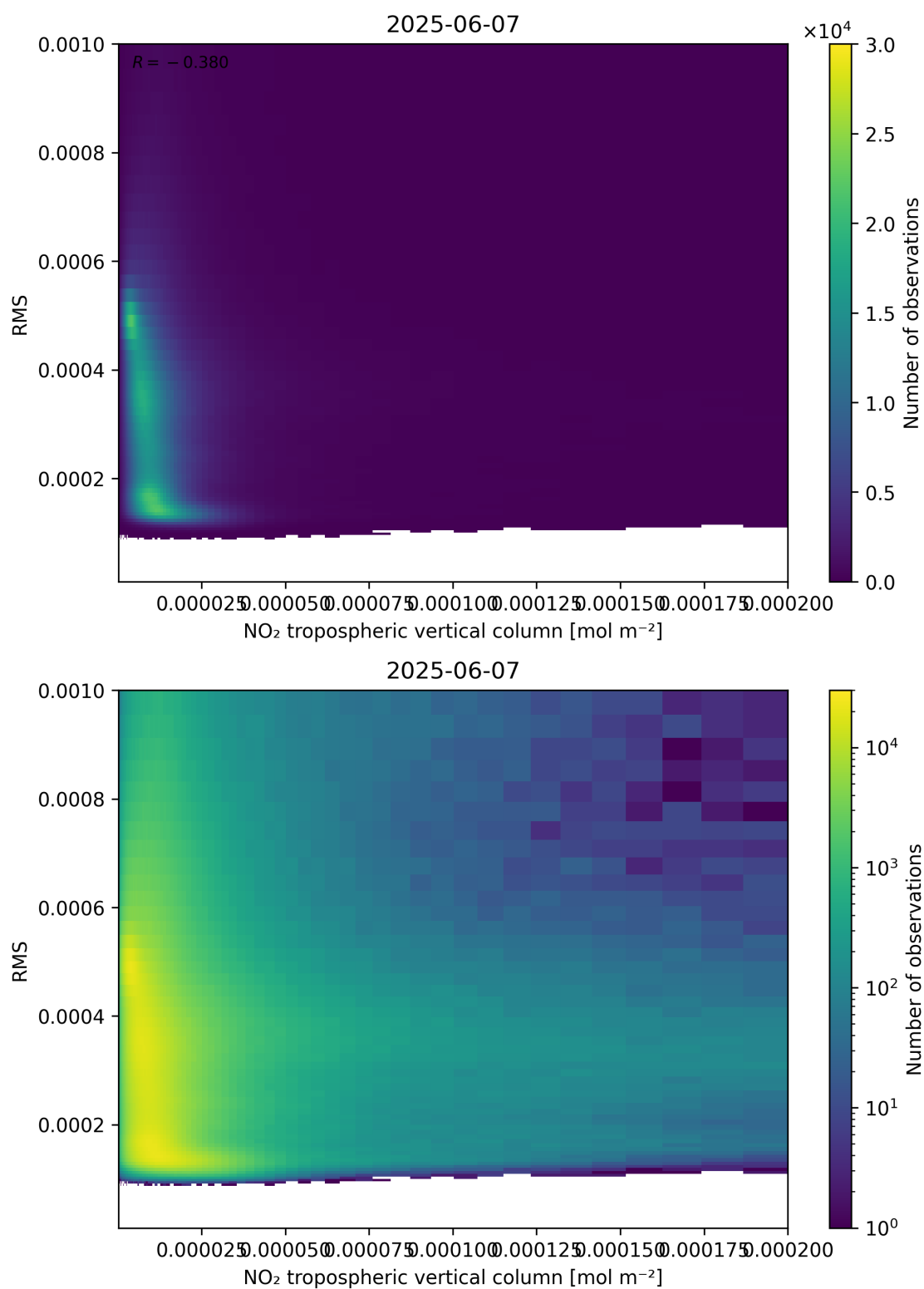
Figure 142: Scatter density plot of “NO 2 tropospheric vertical column” against “RMS” for 2025-06-06 to 2025-06-08.
