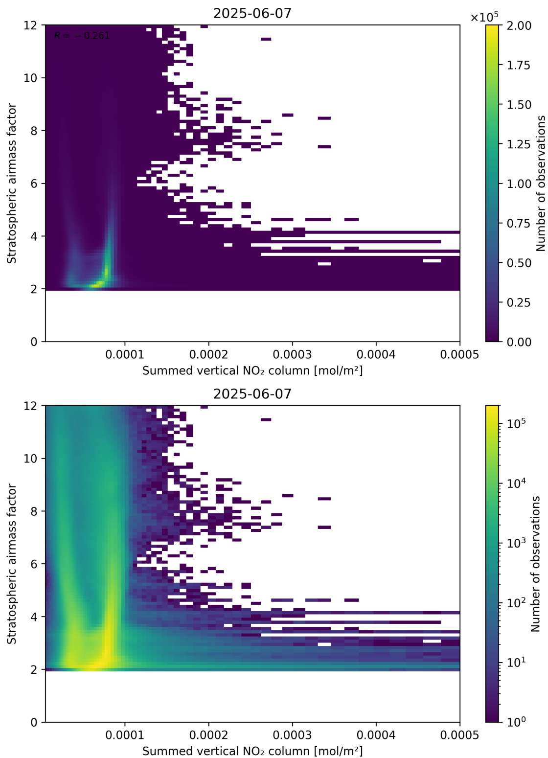
Figure 103: Scatter density plot of “Summed vertical NO 2 column” against “Stratospheric airmass factor” for 2025-06-06 to 2025-06-08.
