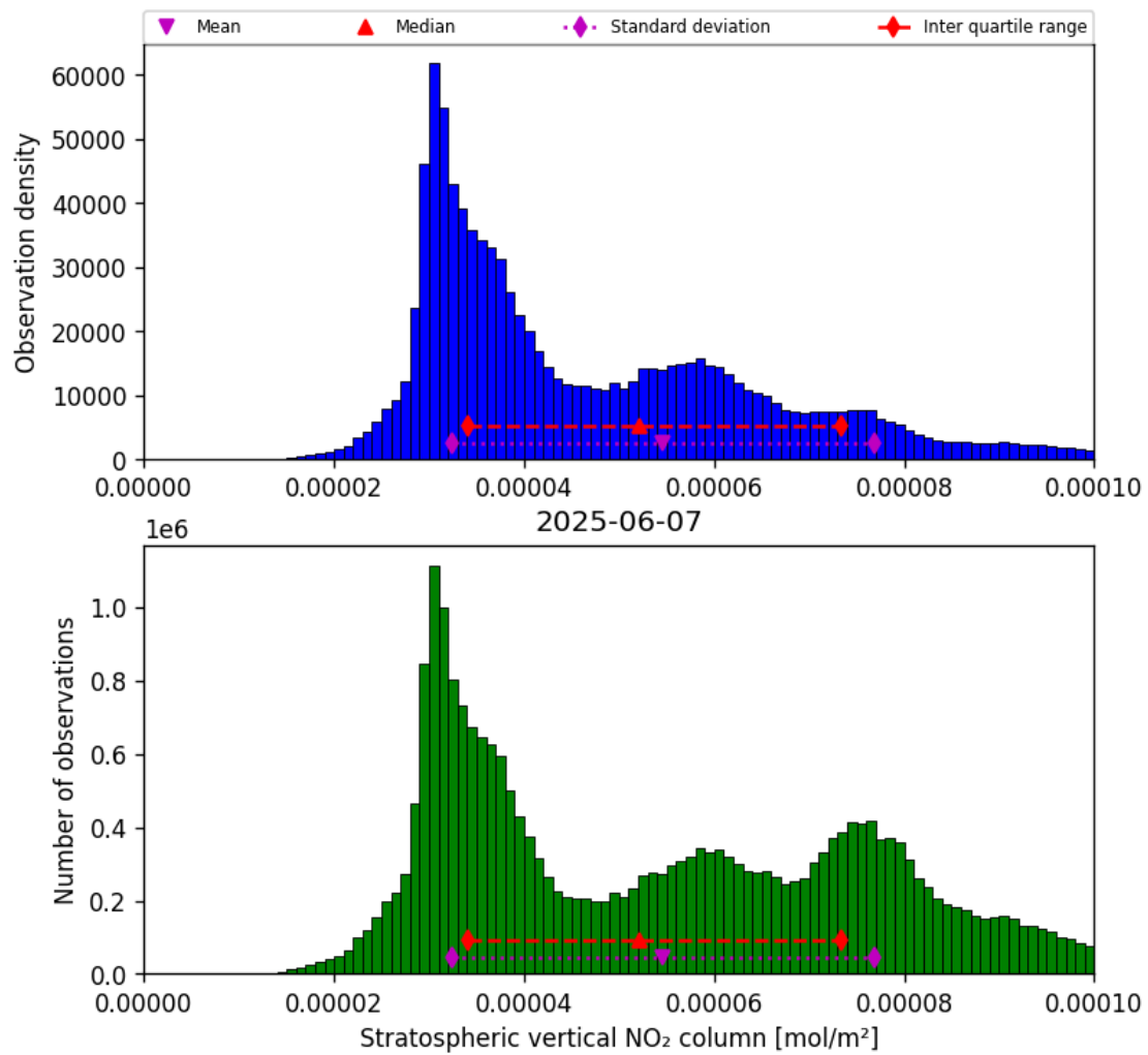
Figure 36: Histogram of “Stratospheric vertical NO 2 column” for 2025-06-06 to 2025-06-08
