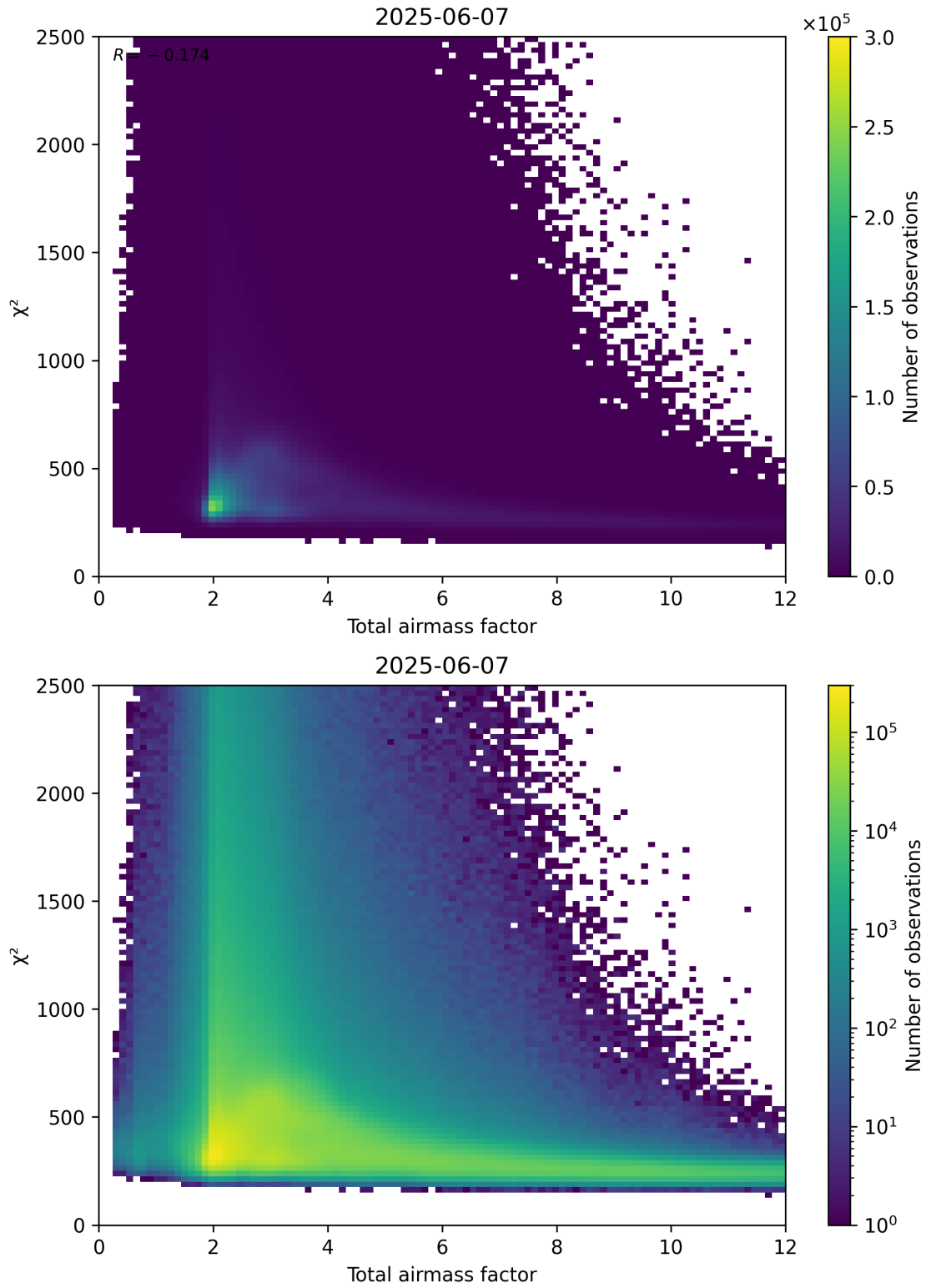
Figure 63: Scatter density plot of “Total airmass factor” against “ \chi^2 ” for 2025-06-06 to 2025-06-08.
