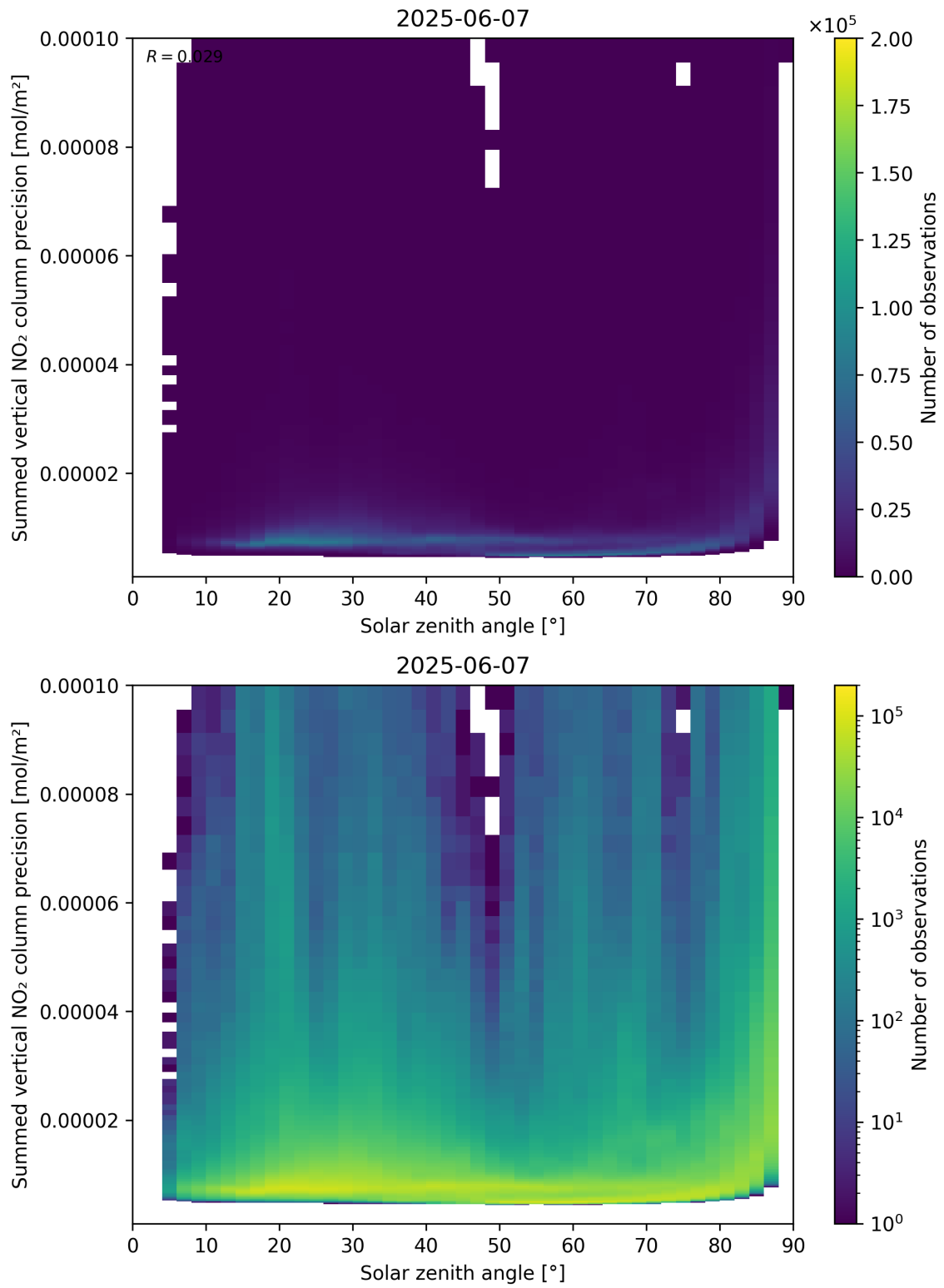
Figure 152: Scatter density plot of “Solar zenith angle” against “Summed vertical NO 2 column precision” for 2025-06-06 to 2025-06-08.
