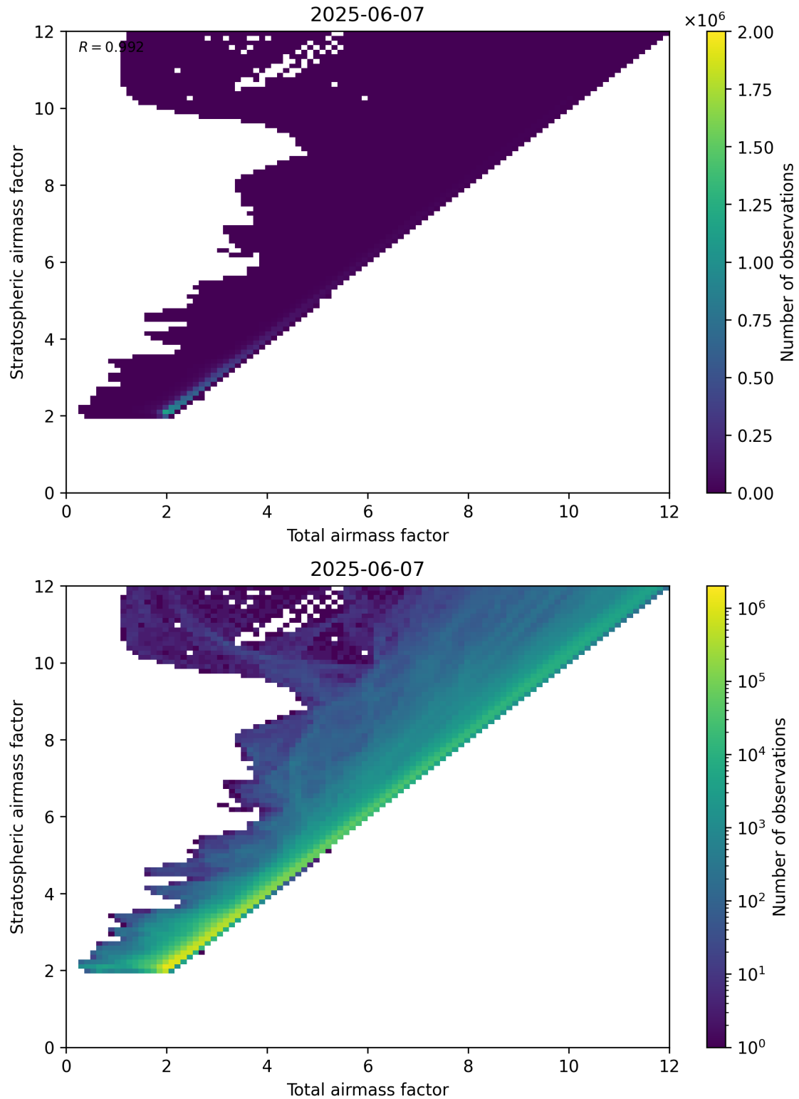
Figure 62: Scatter density plot of “Total airmass factor” against “Stratospheric airmass factor” for 2025-06-06 to 2025-06-08.
