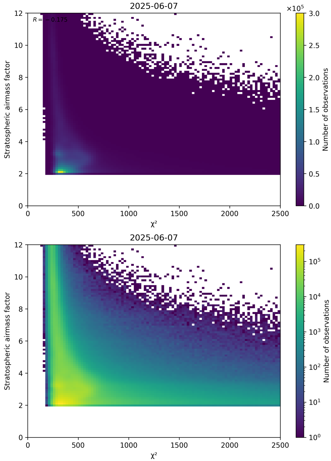
Figure 81: Scatter density plot of “ \chi^2 ” against “Stratospheric airmass factor” for 2025-06-06 to 2025-06-08.
