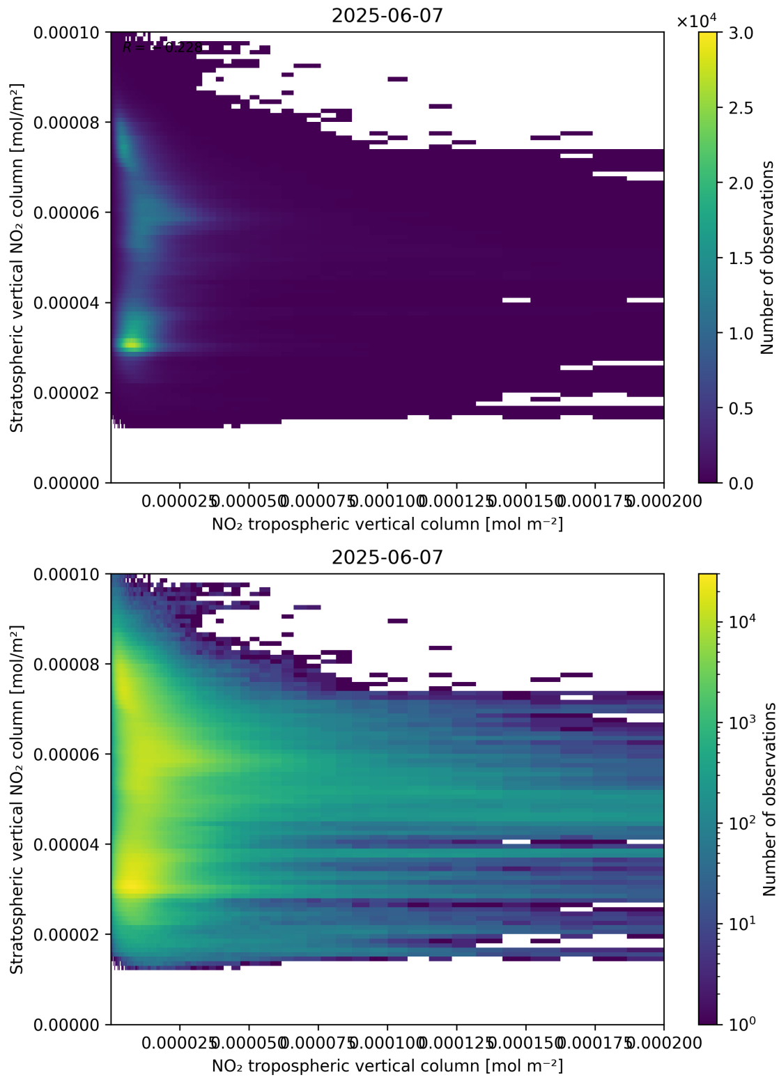
Figure 125: Scatter density plot of “NO 2 tropospheric vertical column” against “Stratospheric vertical NO 2 column” for 2025-06-06 to 2025-06-08.
