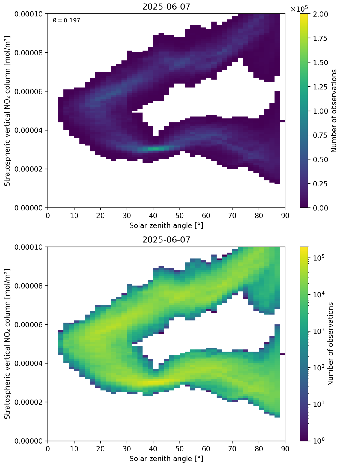
Figure 150: Scatter density plot of “Solar zenith angle” against “Stratospheric vertical NO 2 column” for 2025-06-06 to 2025-06-08.
