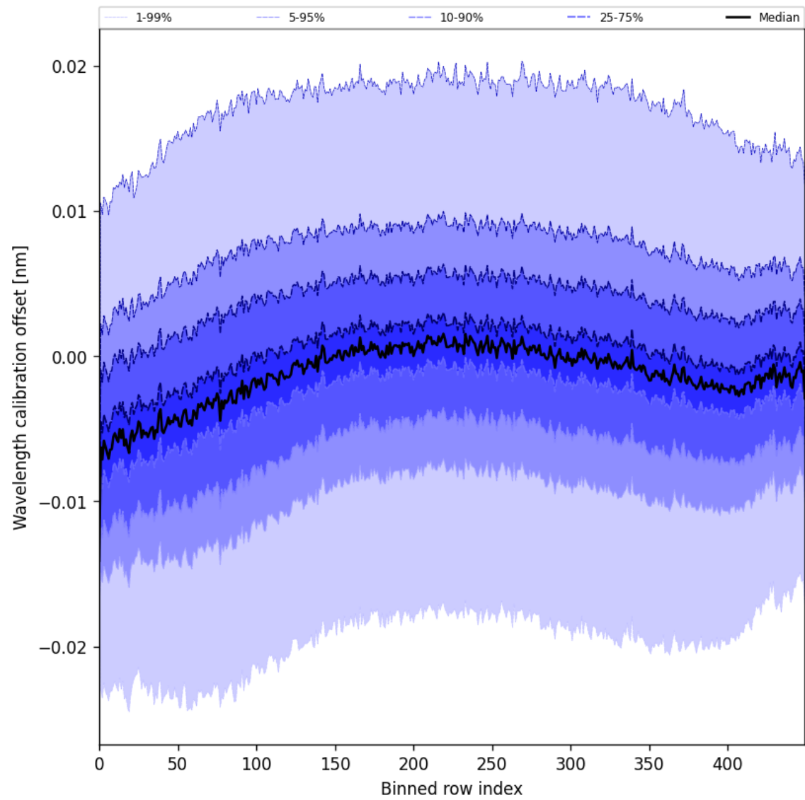
Figure 52: Along track statistics of “Wavelength calibration offset” for 2025-06-06 to 2025-06-08
