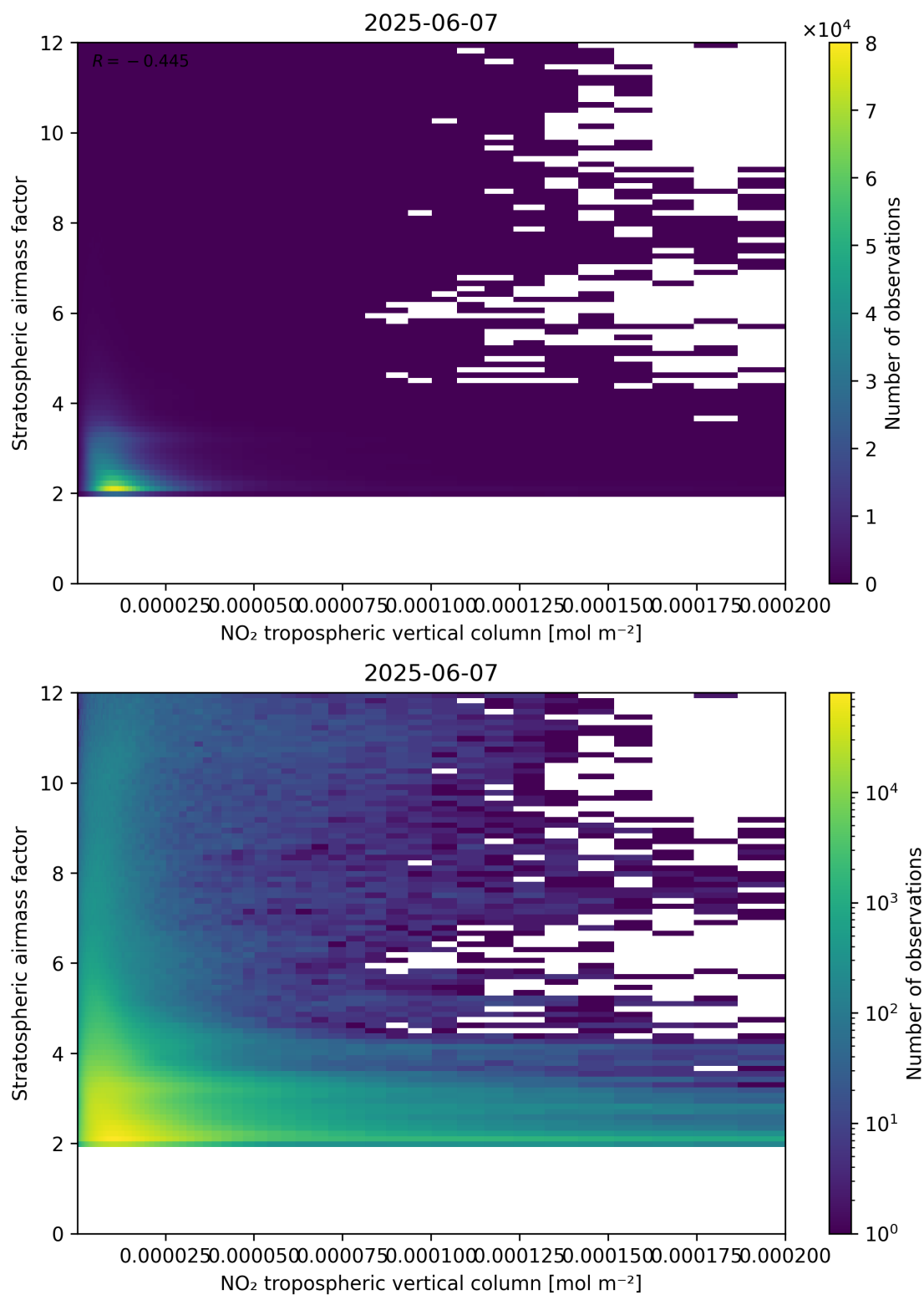
Figure 121: Scatter density plot of “NO 2 tropospheric vertical column” against “Stratospheric air mass factor” for 2025-06-06 to 2025-06-08.
