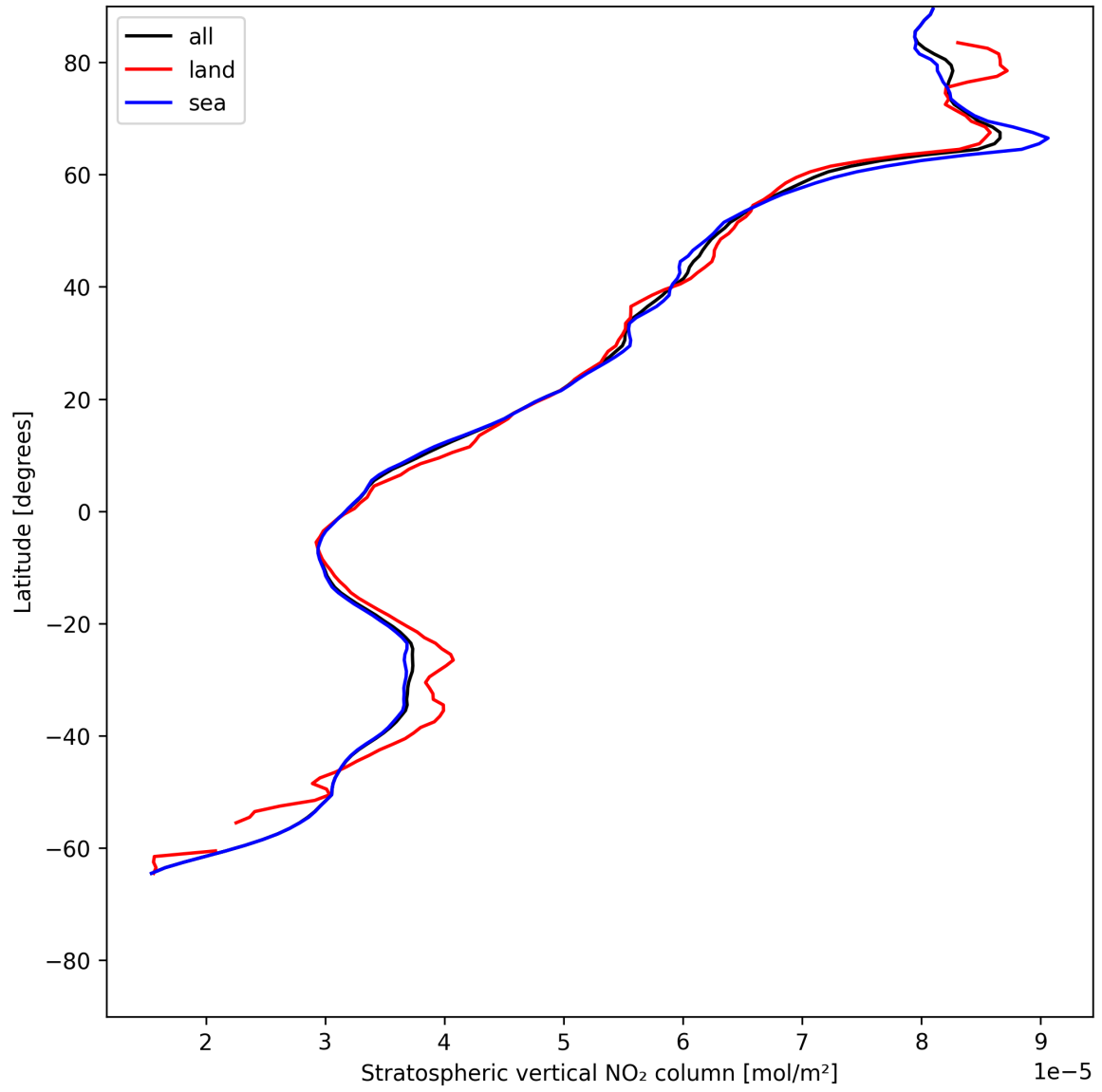
Figure 19: Zonal average of “Stratospheric vertical NO 2 column” for 2025-06-06 to 2025-06-08.
