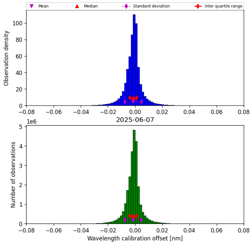
Figure 35: Histogram of “Wavelength calibration offset” for 2025-06-06 to 2025-06-08
