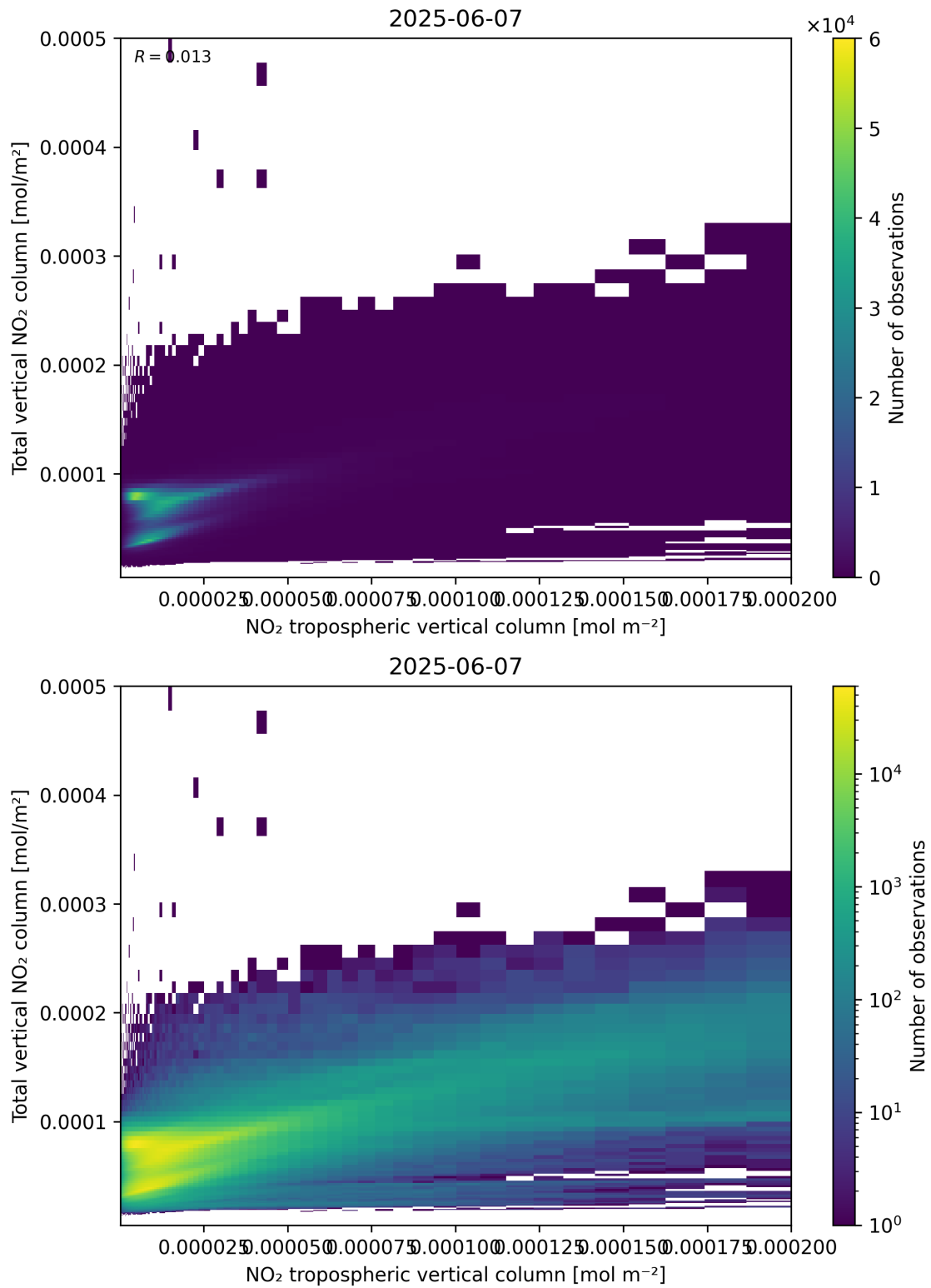
Figure 128: Scatter density plot of “NO 2 tropospheric vertical column” against “Total vertical NO 2 column” for 2025-06-06 to 2025-06-08.
