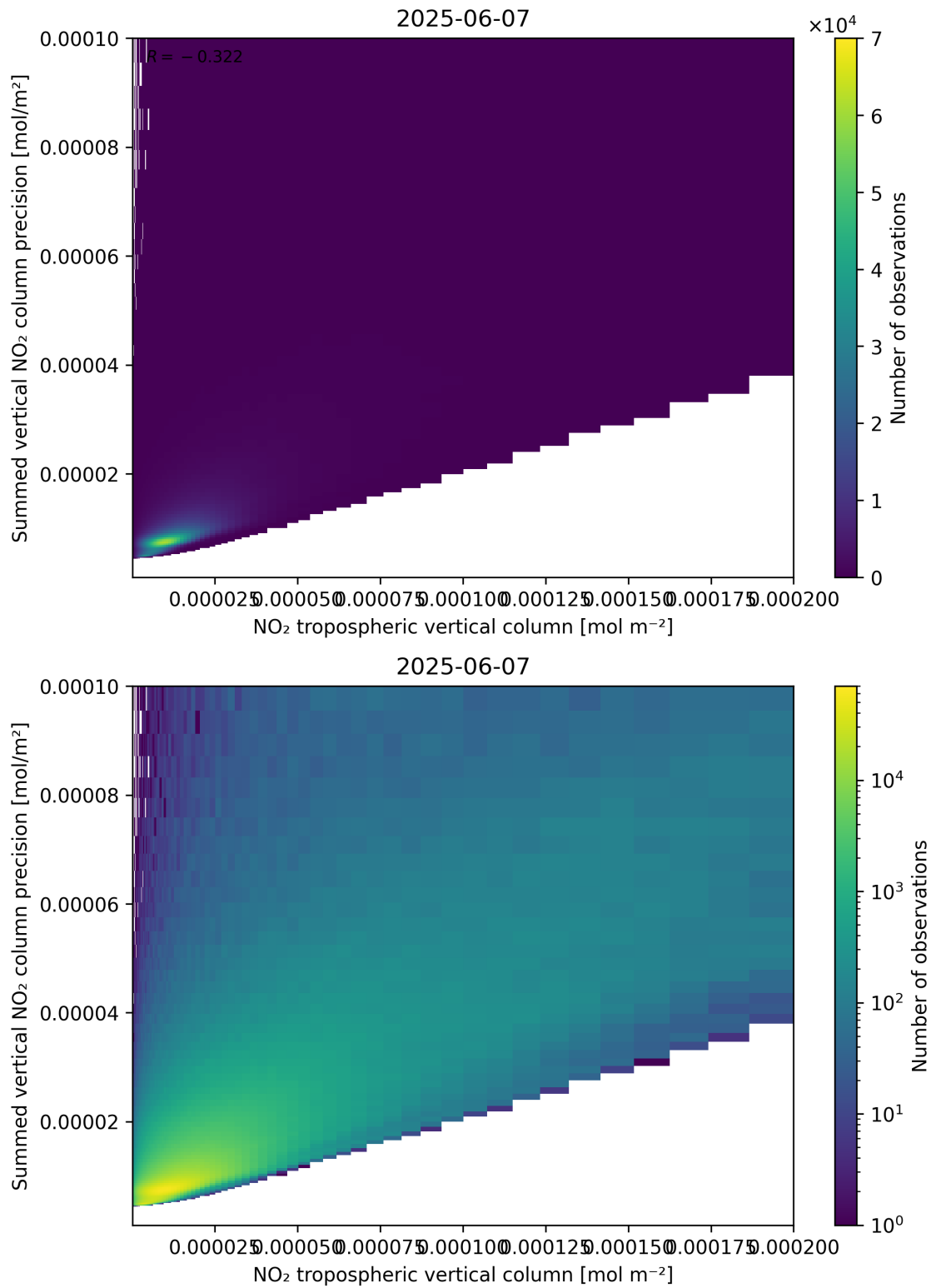
Figure 127: Scatter density plot of “NO 2 tropospheric vertical column” against “Summed vertical NO 2 column precision” for 2025-06-06 to 2025-06-08.
