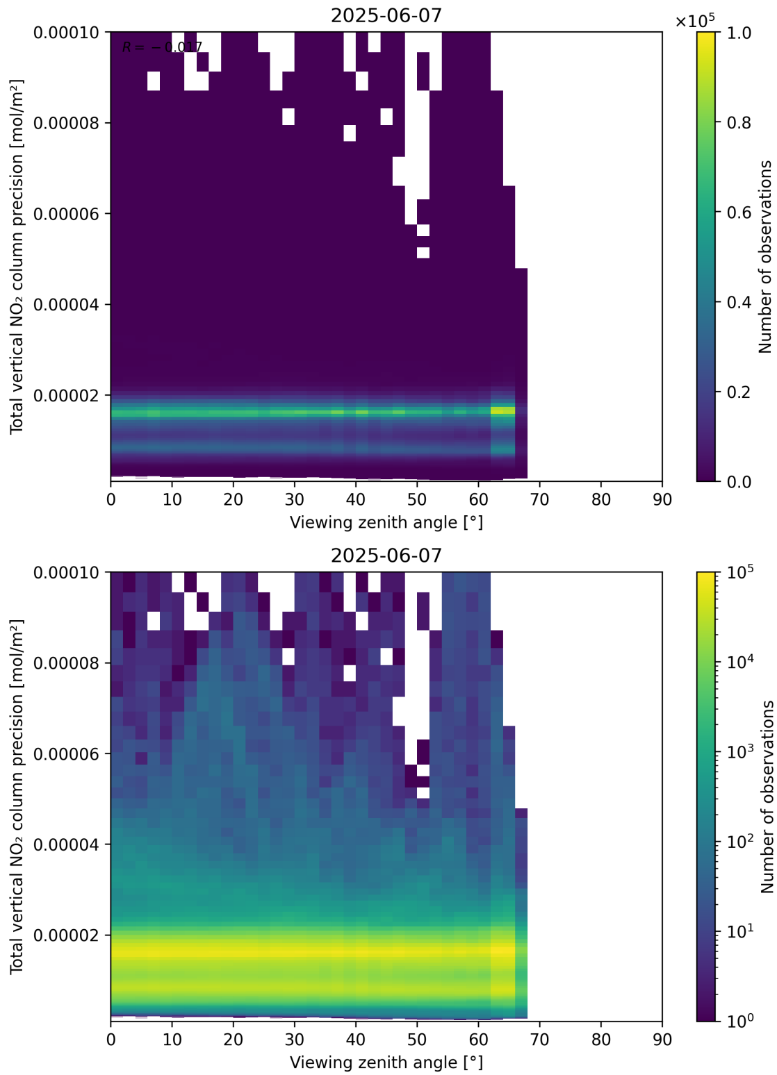
Figure 168: Scatter density plot of “Viewing zenith angle” against “Total vertical NO 2 column precision” for 2025-06-06 to 2025-06-08.
