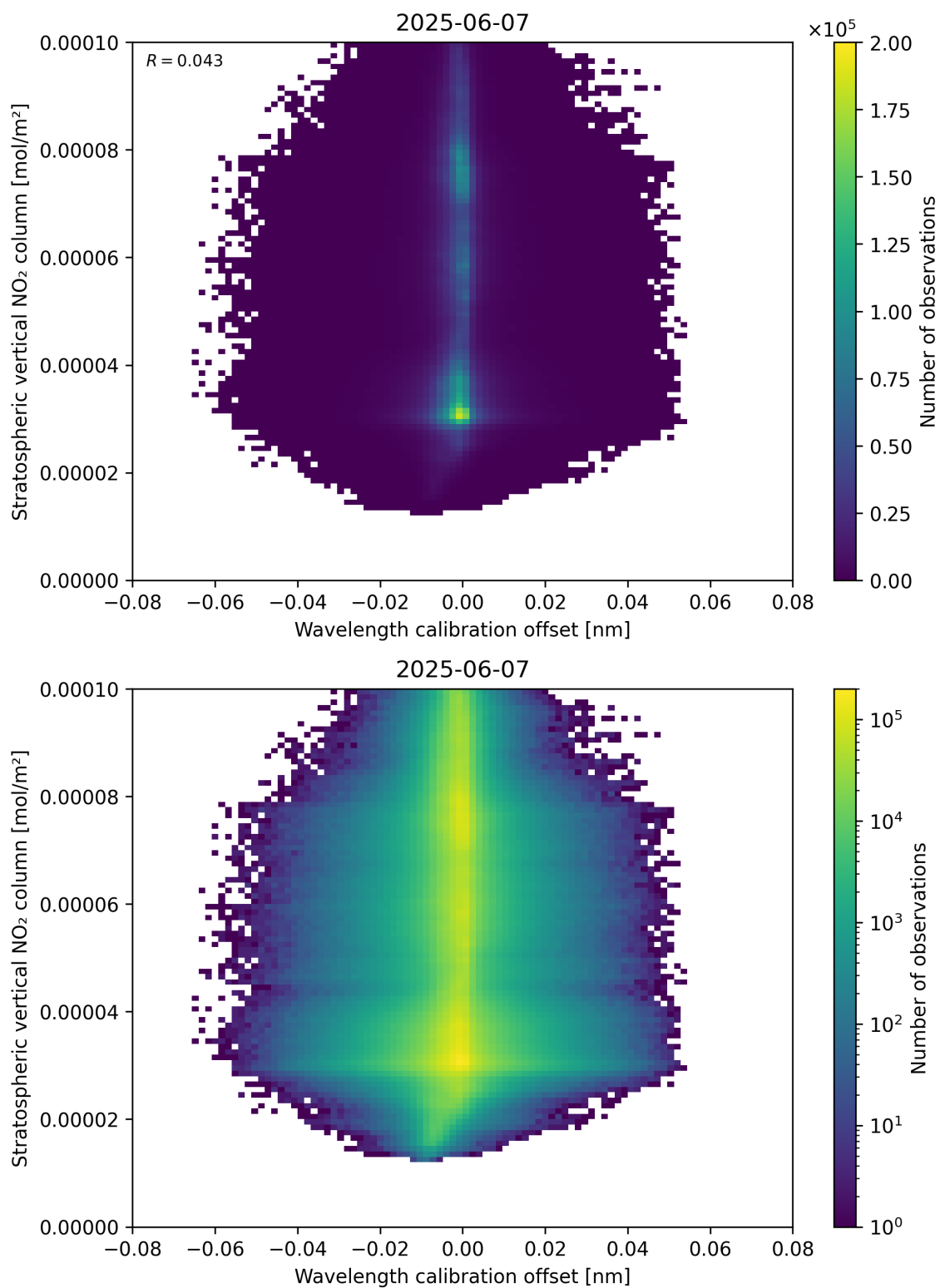
Figure 176: Scatter density plot of “Wavelength calibration offset” against “Stratospheric vertical NO 2 column” for 2025-06-06 to 2025-06-08.
