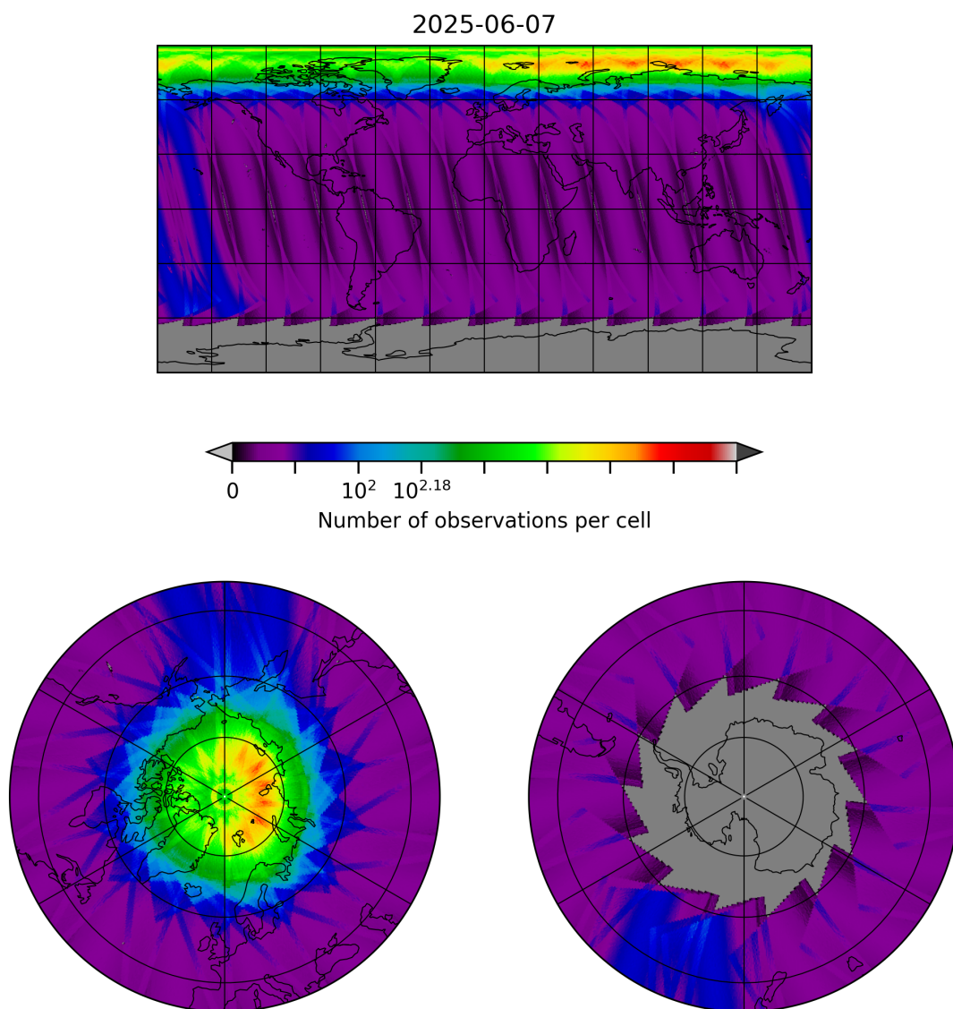
Figure 10: Map of the number of observations for 2025-06-06 to 2025-06-08
