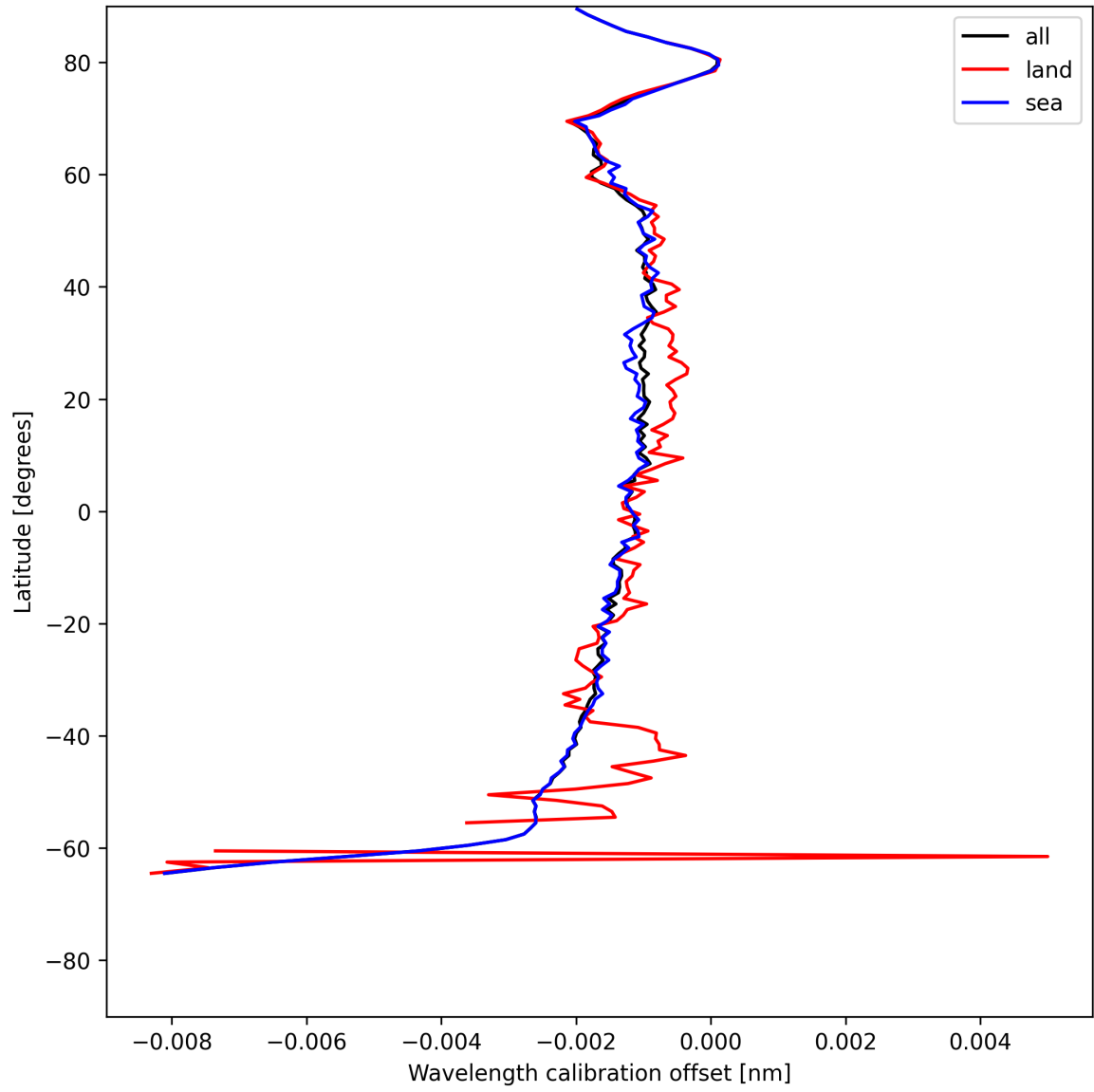
Figure 18: Zonal average of “Wavelength calibration offset” for 2025-06-06 to 2025-06-08.
