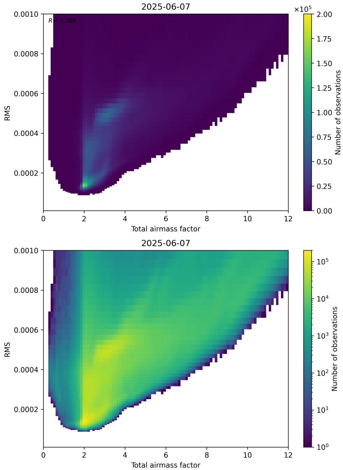
Figure 69: Scatter density plot of “Total airmass factor” against “RMS” for 2025-06-06 to 2025-06-08.
