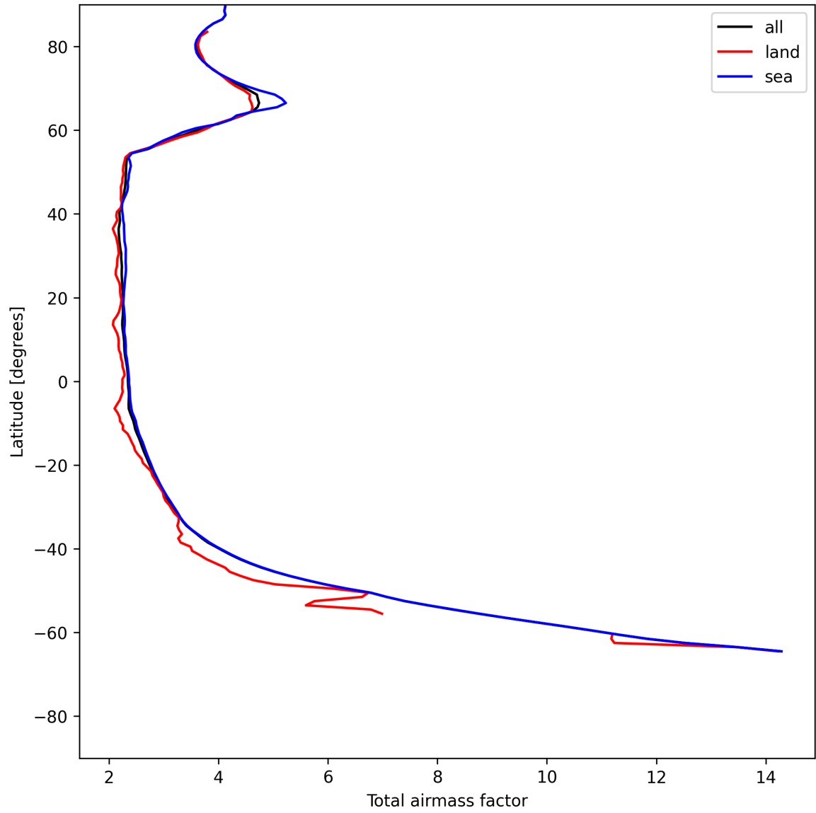
Figure 15: Zonal average of “Total airmass factor” for 2025-06-06 to 2025-06-08.
