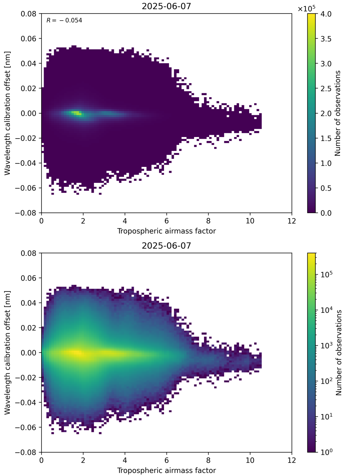
Figure 80: Scatter density plot of “Tropospheric airmass factor” against “Wavelength calibration offset” for 2025-06-06 to 2025-06-08.
