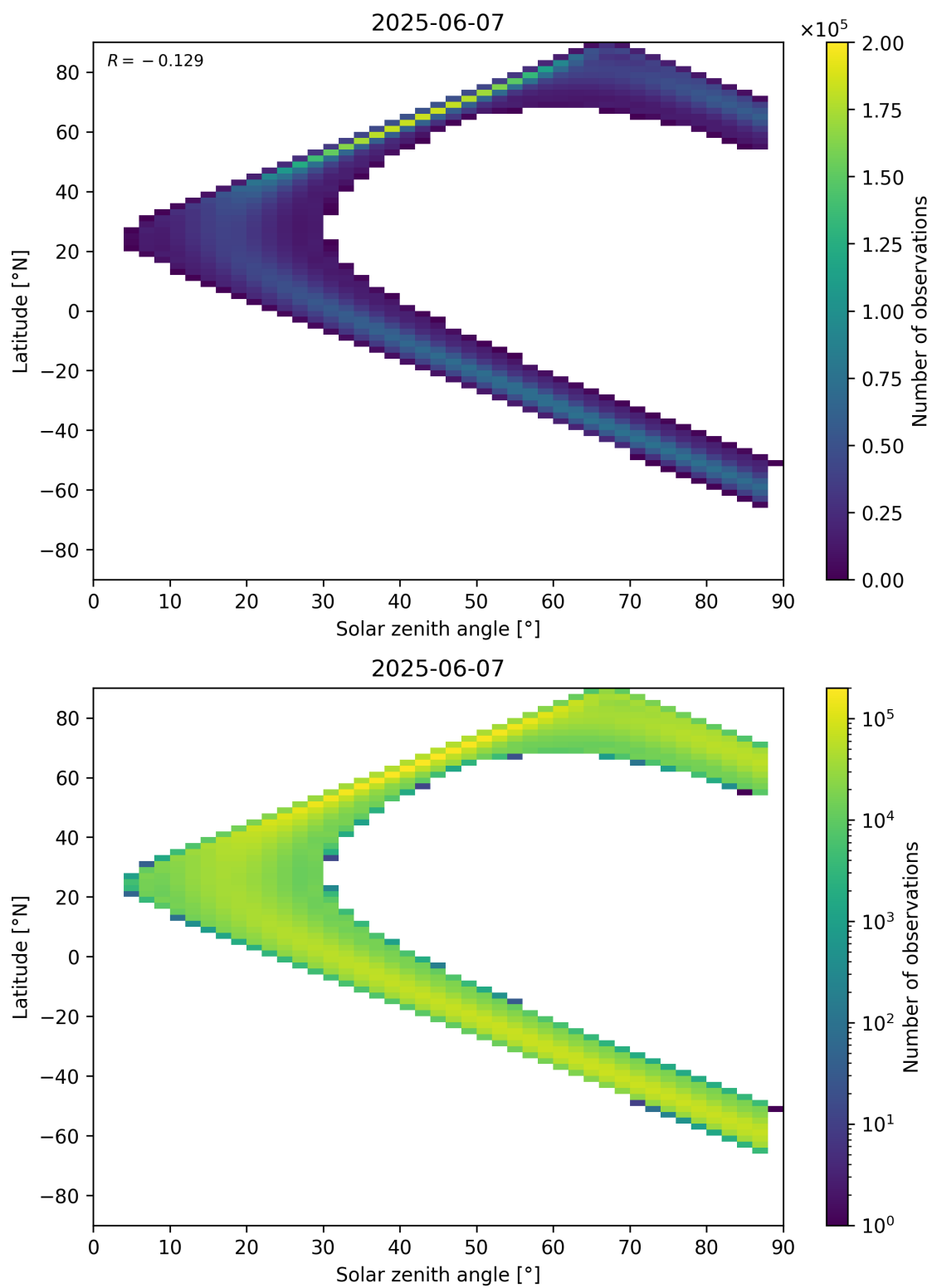
Figure 149: Scatter density plot of “Solar zenith angle” against “Latitude” for 2025-06-06 to 2025-06-08.
