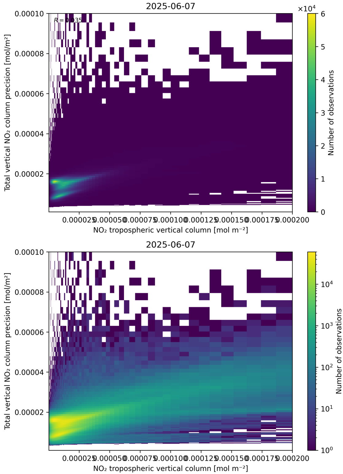
Figure 129: Scatter density plot of “NO 2 tropospheric vertical column” against “Total vertical NO 2 column precision” for 2025-06-06 to 2025-06-08.
