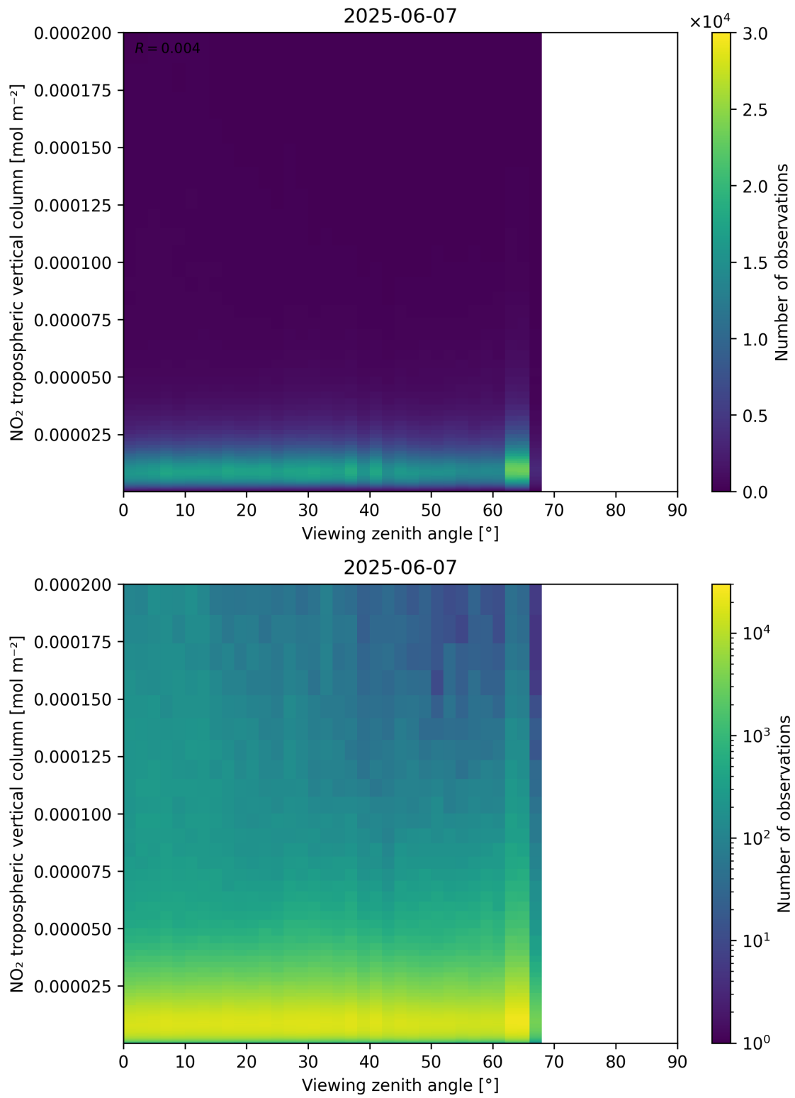
Figure 169: Scatter density plot of “Viewing zenith angle” against “NO 2 tropospheric vertical column” for 2025-06-06 to 2025-06-08.
