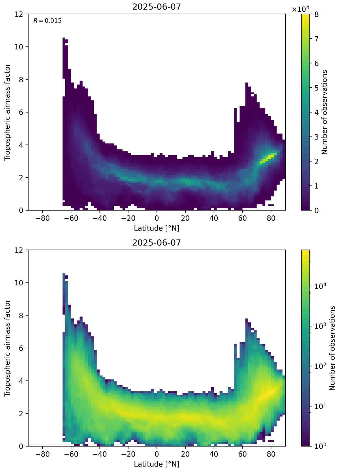
Figure 85: Scatter density plot of “Latitude” against “Tropospheric airmass factor” for 2025-06-06 to 2025-06-08.
