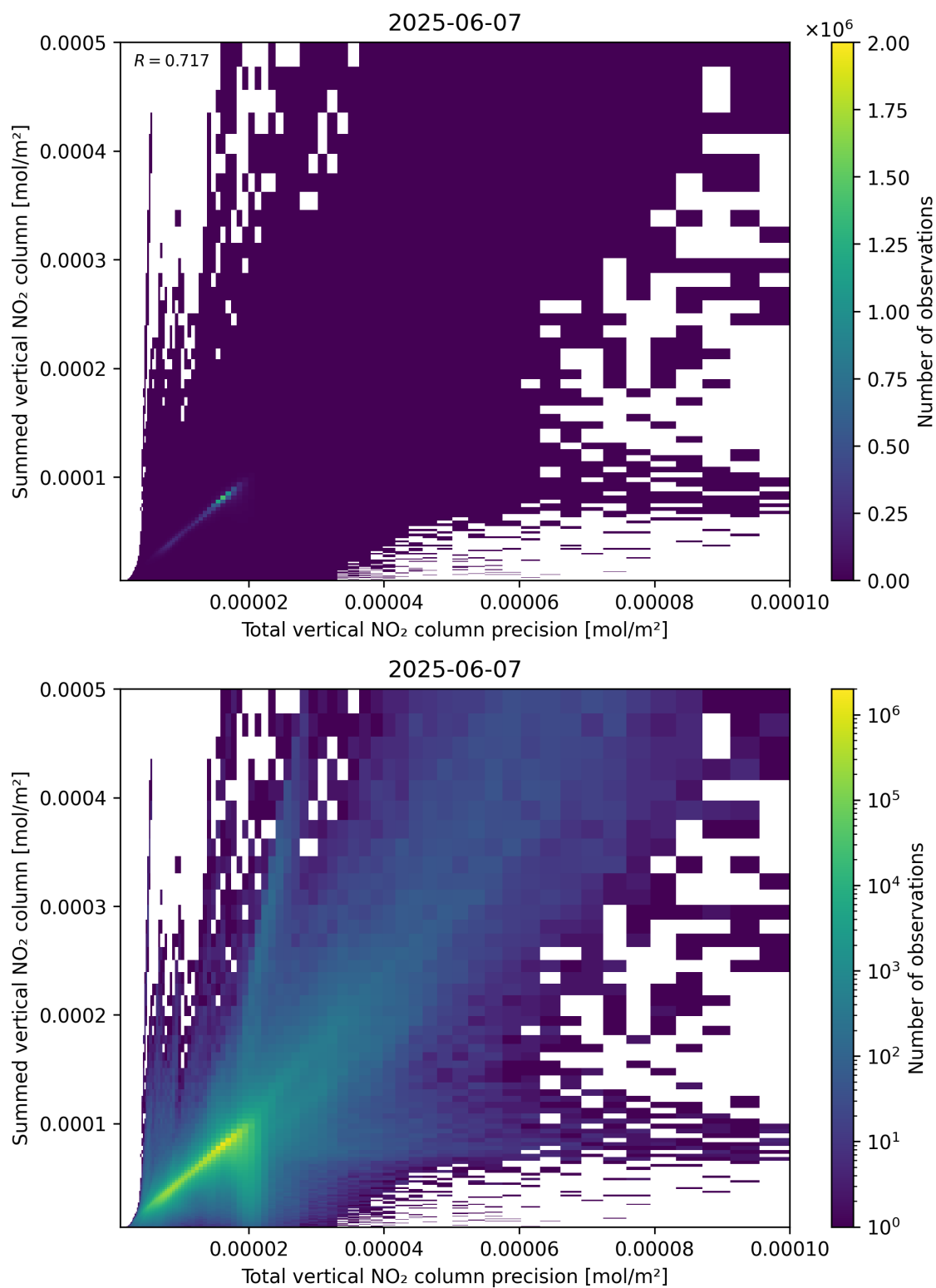
Figure 117: Scatter density plot of “Total vertical NO 2 column precision” against “Summed vertical NO 2 column” for 2025-06-06 to 2025-06-08.
