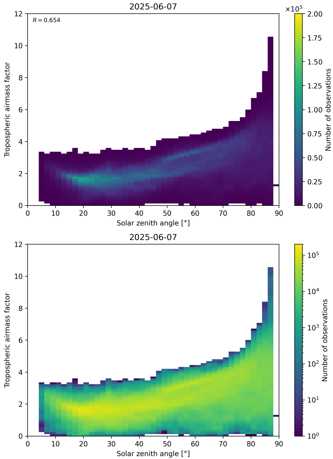
Figure 147: Scatter density plot of “Solar zenith angle” against “Tropospheric airmass factor” for 2025-06-06 to 2025-06-08.
