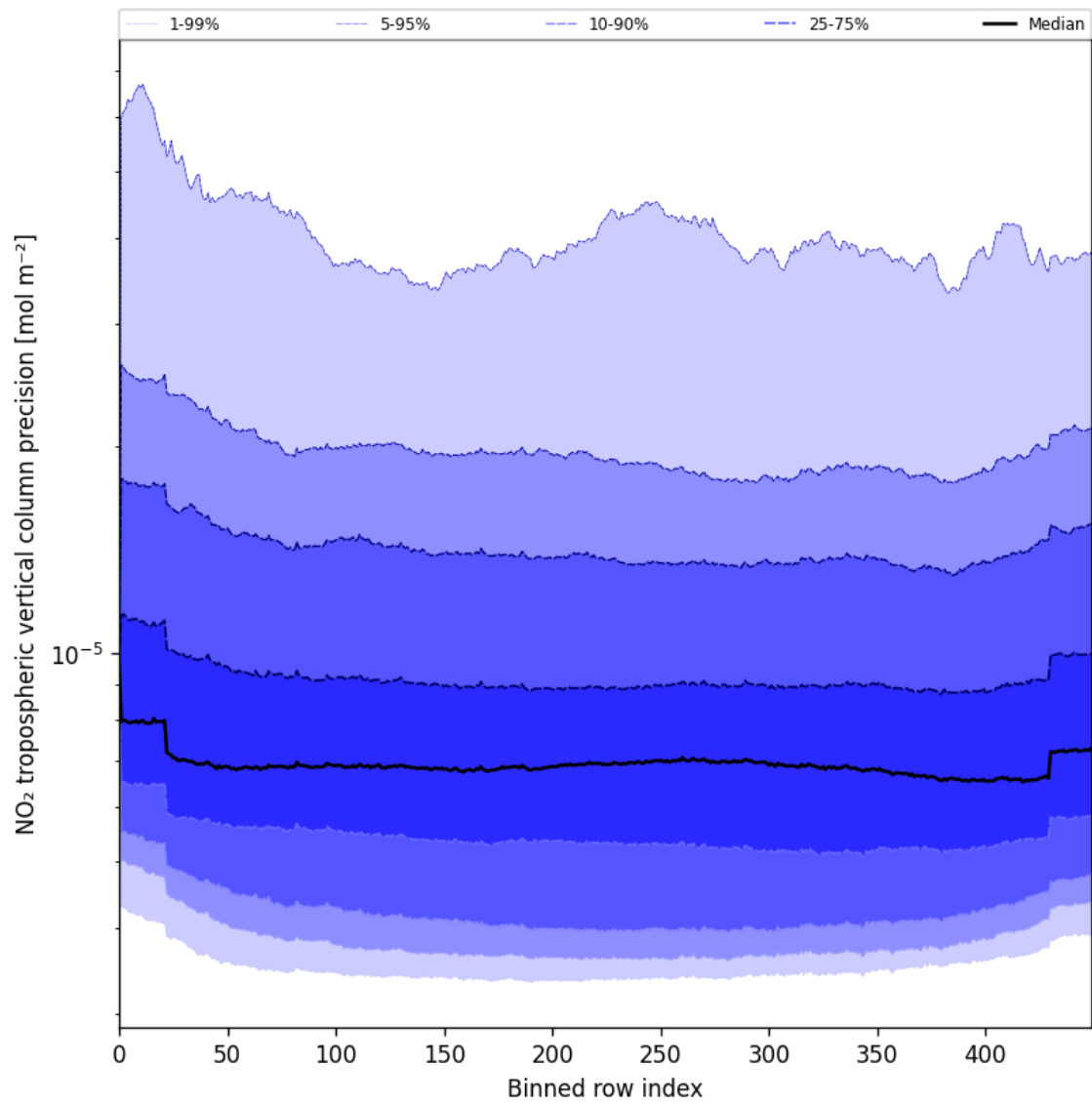
Figure 47: Along track statistics of “NO 2 tropospheric vertical column precision” for 2025-06-06 to 2025-06-08
