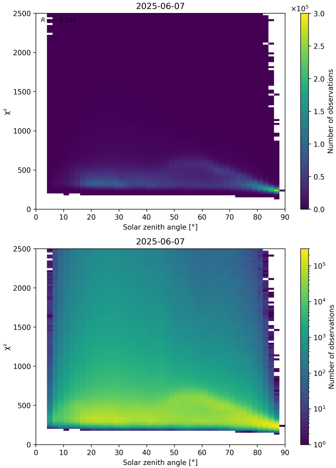
Figure 148: Scatter density plot of “Solar zenith angle” against “ \chi^2 ” for 2025-06-06 to 2025-06-08.
