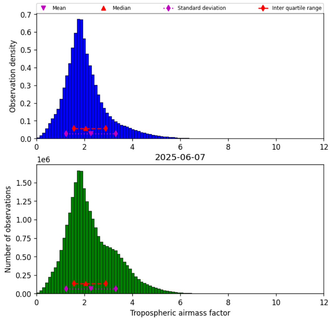
Figure 31: Histogram of “Tropospheric airmass factor” for 2025-06-06 to 2025-06-08
