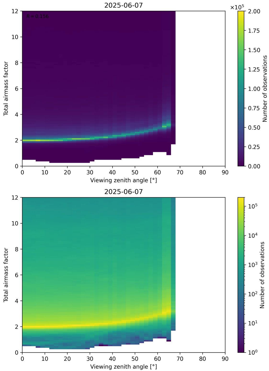
Figure 160: Scatter density plot of “Viewing zenith angle” against “Total airmass factor” for 2025-06-06 to 2025-06-08.
