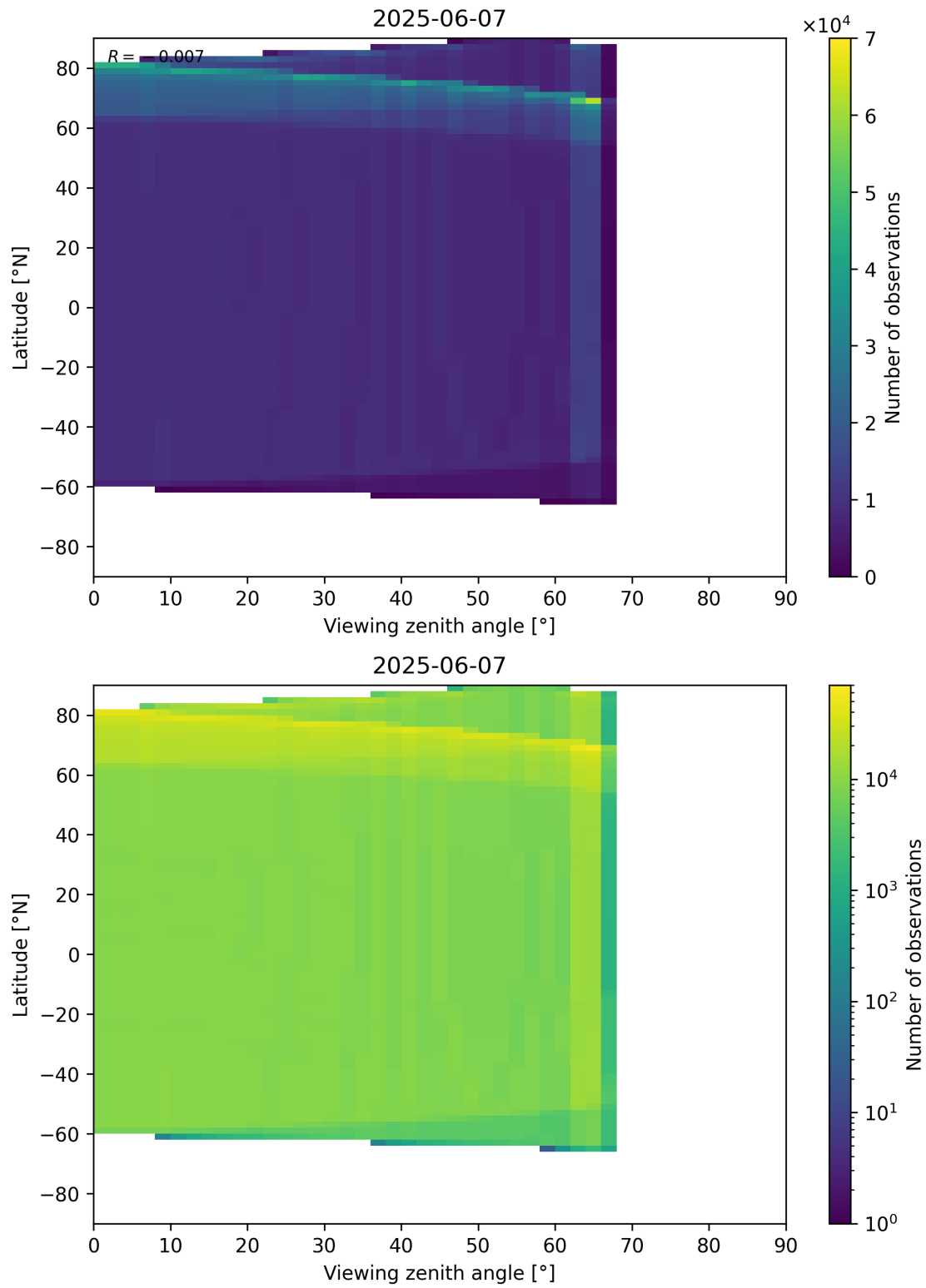
Figure 163: Scatter density plot of “Viewing zenith angle” against “Latitude” for 2025-06-06 to 2025-06-08.
