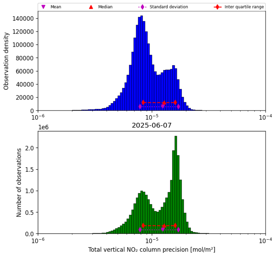
Figure 39: Histogram of “Total vertical NO 2 column precision” for 2025-06-06 to 2025-06-08
