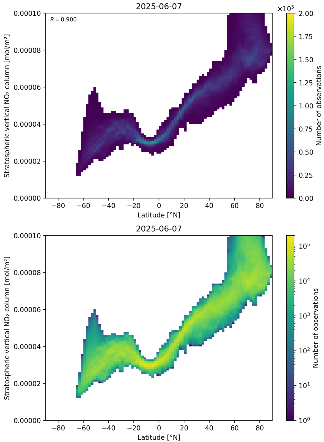
Figure 87: Scatter density plot of “Latitude” against “Stratospheric vertical NO 2 column” for 2025-06-06 to 2025-06-08.
