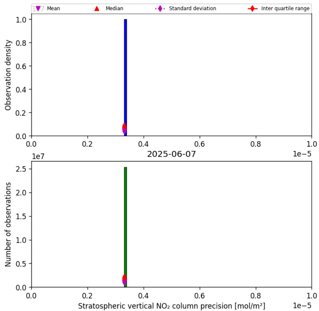
Figure 37: Histogram of “Stratospheric vertical NO 2 column precision” for 2025-06-06 to 2025-06-08
