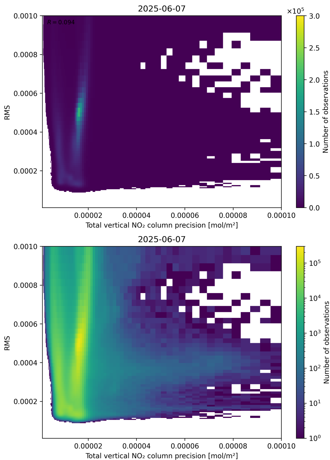
Figure 119: Scatter density plot of “Total vertical NO 2 column precision” against “RMS” for 2025-06-06 to 2025-06-08.
