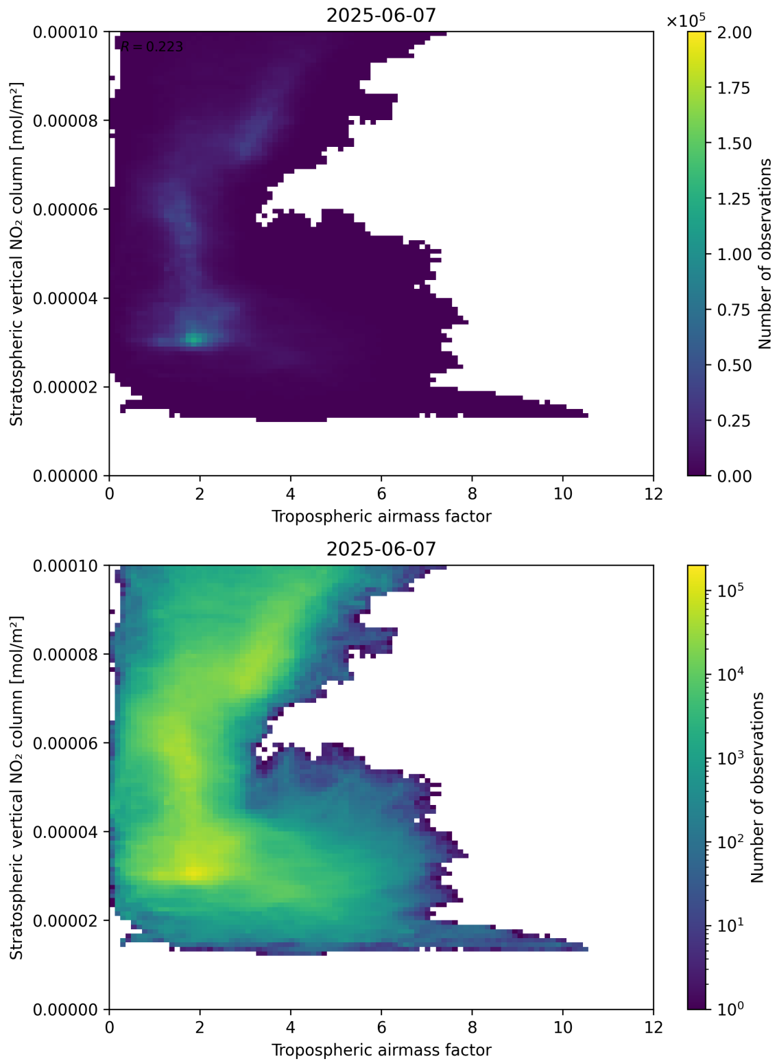
Figure 74: Scatter density plot of “Tropospheric air mass factor” against “Stratospheric vertical NO 2 column” for 2025-06-06 to 2025-06-08.
