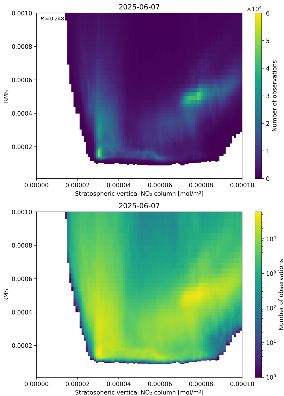
Figure 102: Scatter density plot of “Stratospheric vertical NO 2 column” against “RMS” for 2025-06-06 to 2025-06-08.
