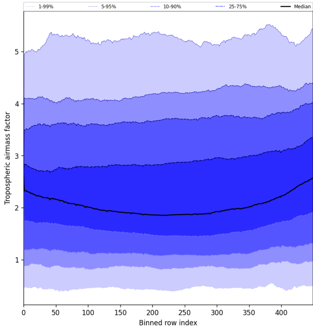
Figure 48: Along track statistics of “Tropospheric airmass factor” for 2025-06-06 to 2025-06-08
