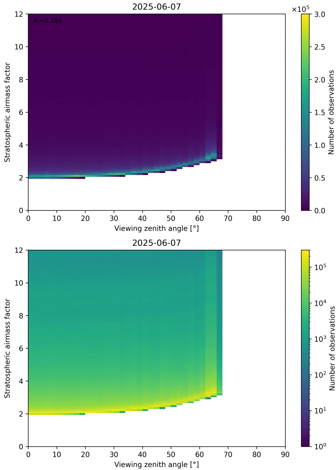
Figure 159: Scatter density plot of “Viewing zenith angle” against “Stratospheric airmass factor” for 2025-06-06 to 2025-06-08.
