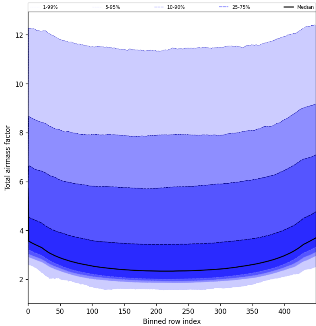
Figure 49: Along track statistics of “Total airmass factor” for 2025-06-06 to 2025-06-08
