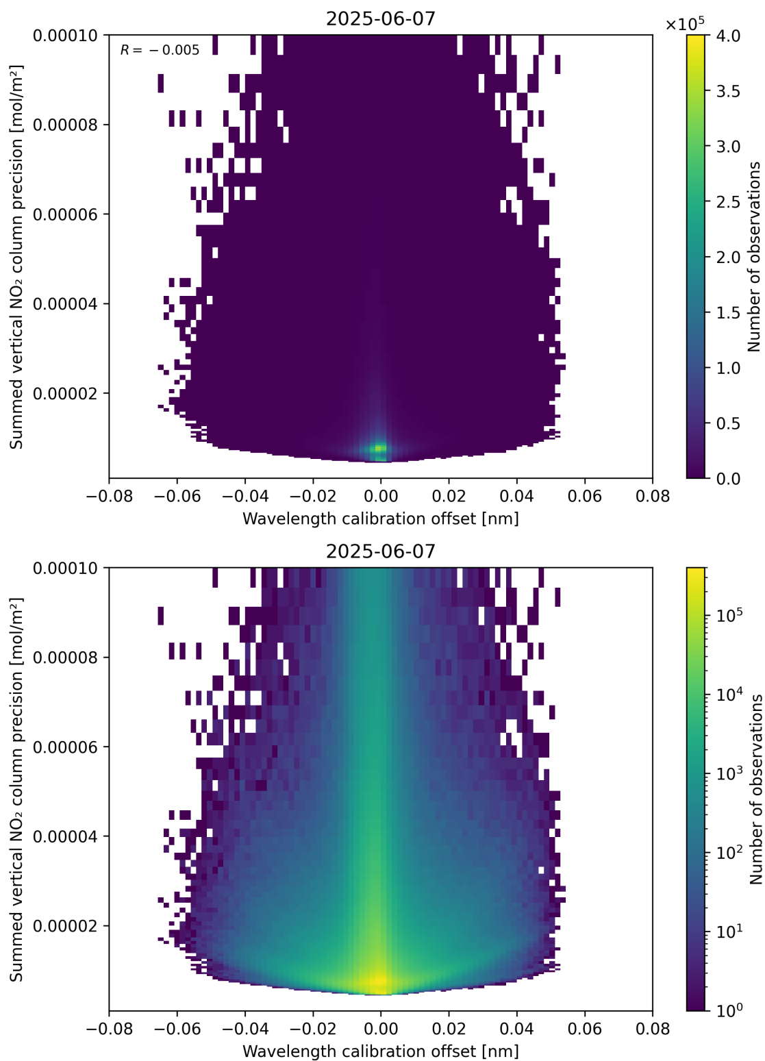
Figure 178: Scatter density plot of “Wavelength calibration offset” against “Summed vertical NO 2 column precision” for 2025-06-06 to 2025-06-08.
