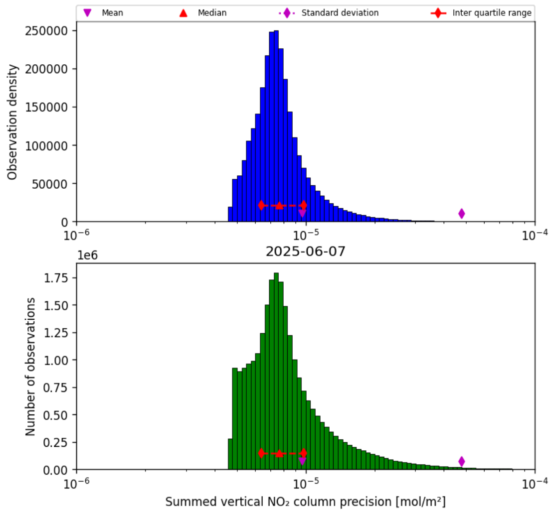
Figure 41: Histogram of “Summed vertical NO 2 column precision” for 2025-06-06 to 2025-06-08
