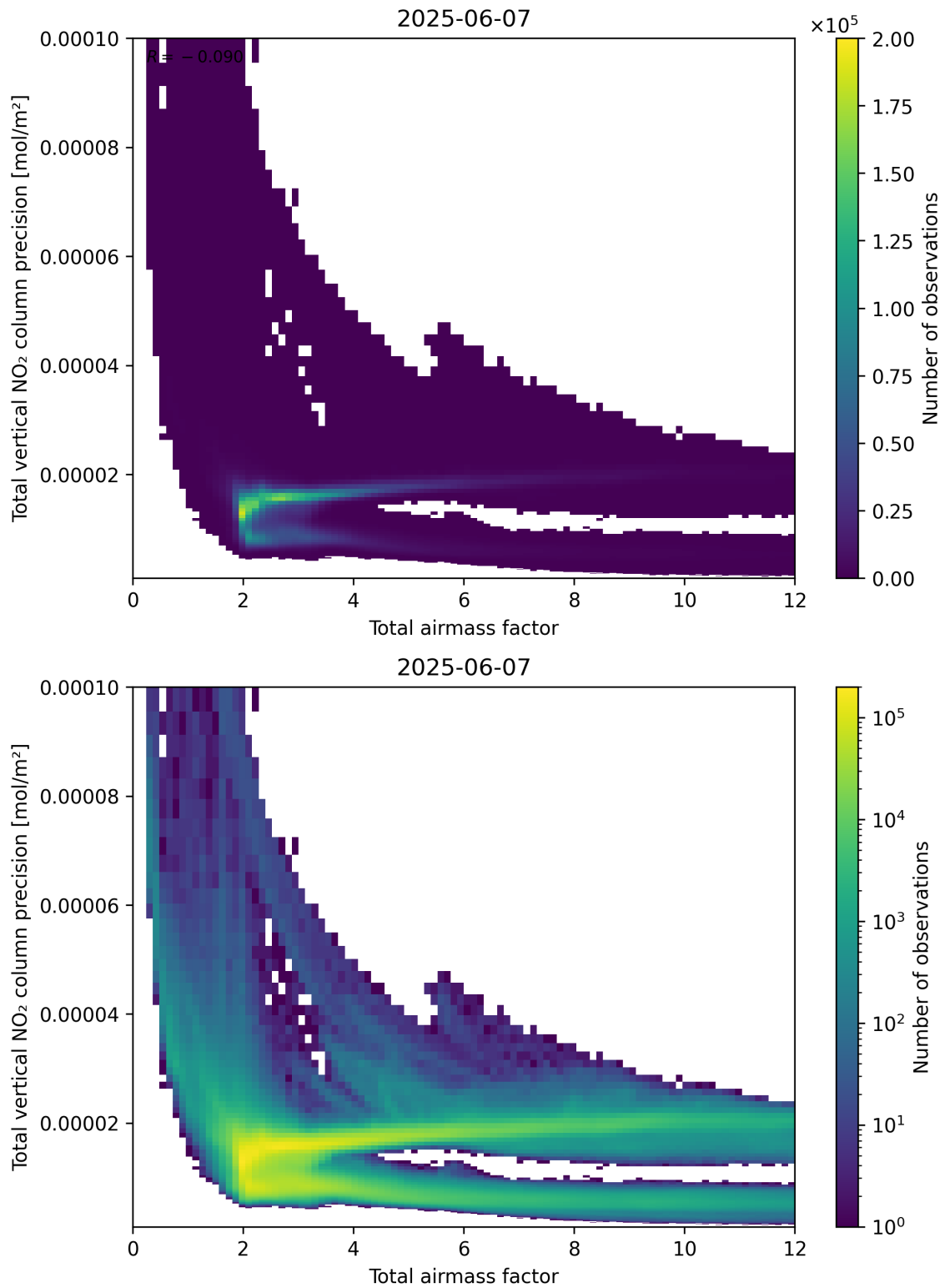
Figure 68: Scatter density plot of “Total airmass factor” against “Total vertical NO 2 column precision” for 2025-06-06 to 2025-06-08.
