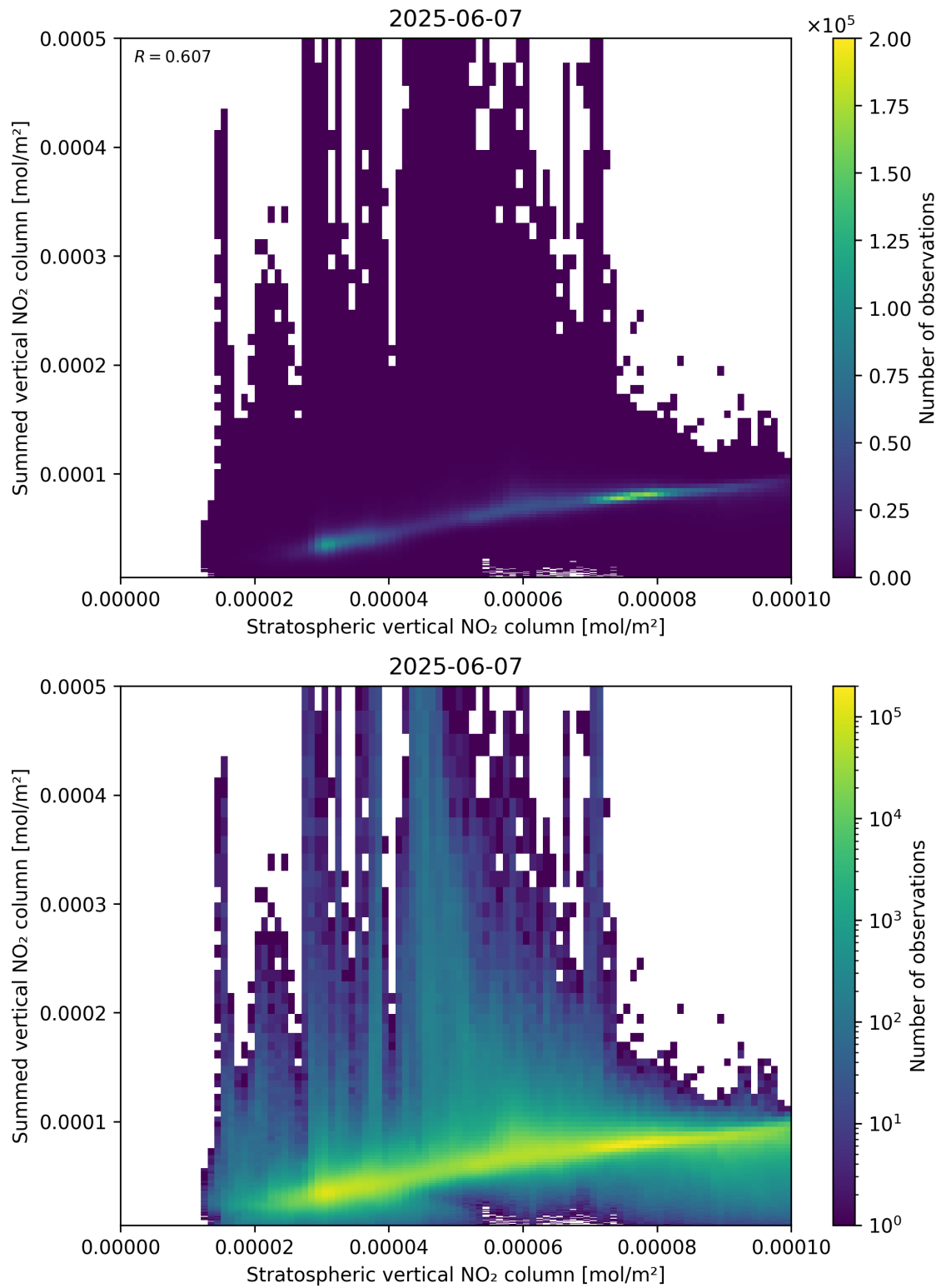
Figure 98: Scatter density plot of “Stratospheric vertical NO 2 column” against “Summed vertical NO 2 column” for 2025-06-06 to 2025-06-08.
