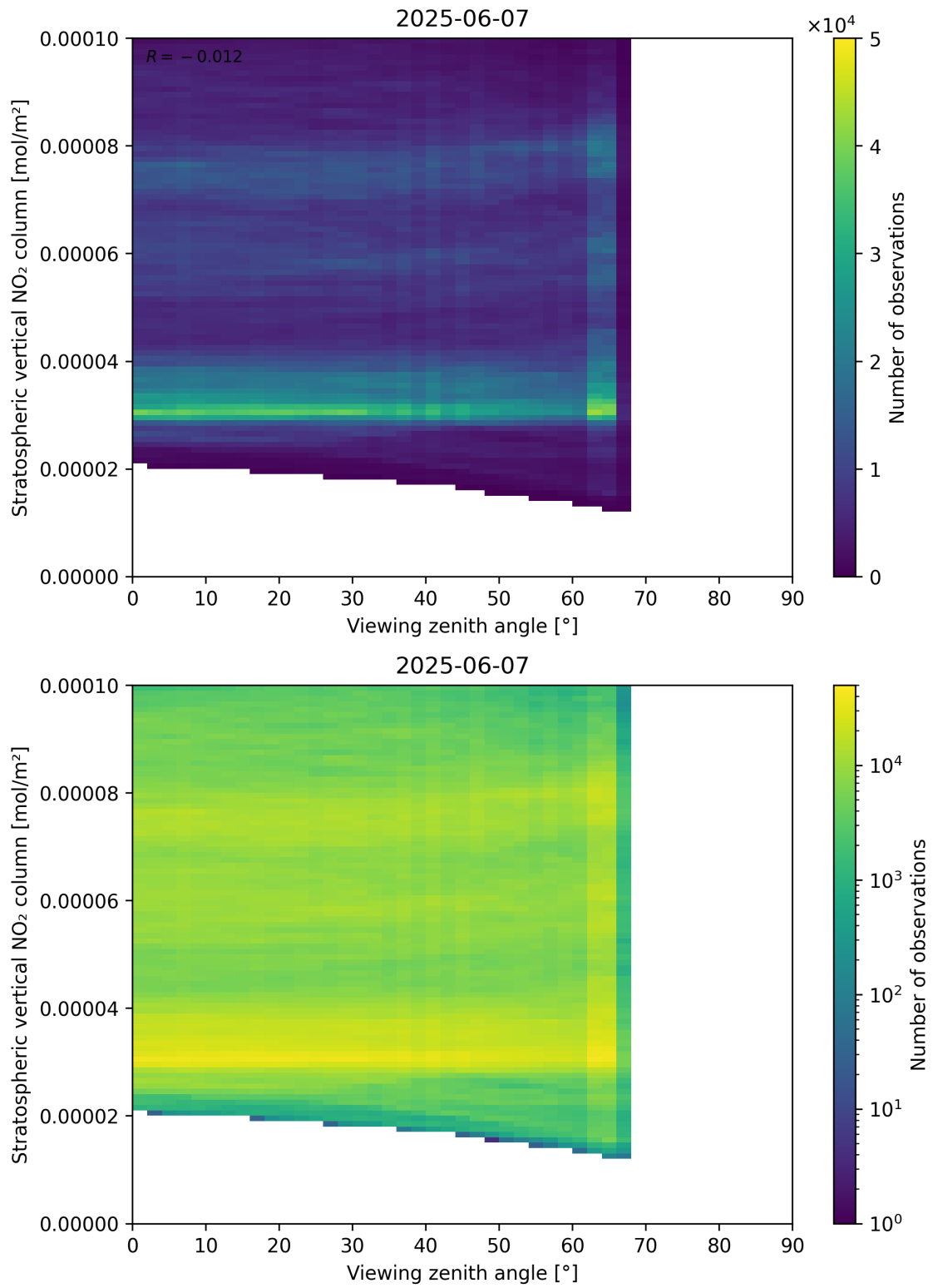
Figure 164: Scatter density plot of “Viewing zenith angle” against “Stratospheric vertical NO 2 column” for 2025-06-06 to 2025-06-08.
