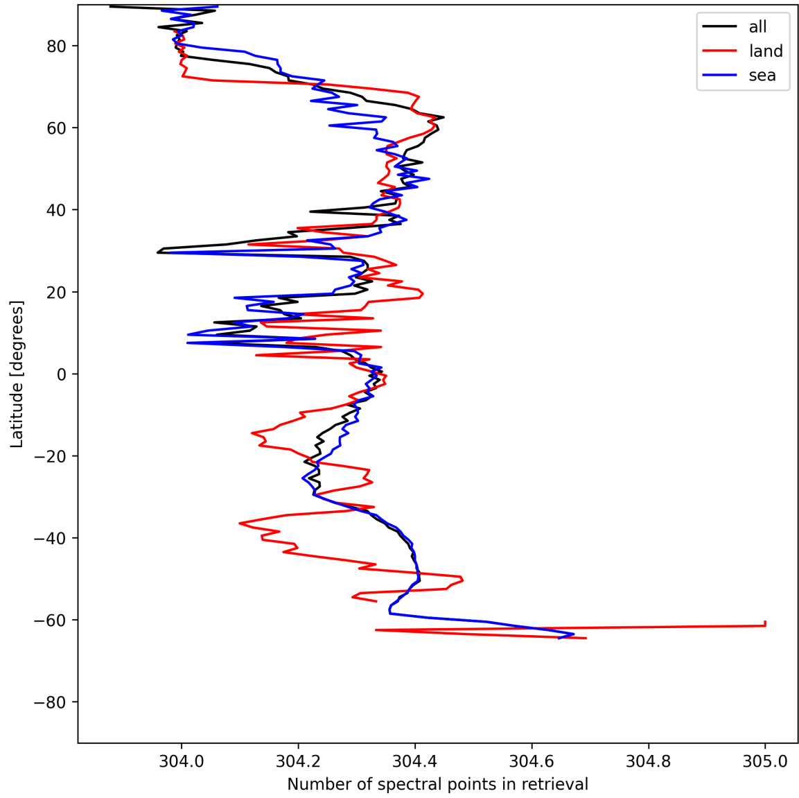
Figure 16: Zonal average of “Number of spectral points in retrieval” for 2025-06-06 to 2025-06-08.
