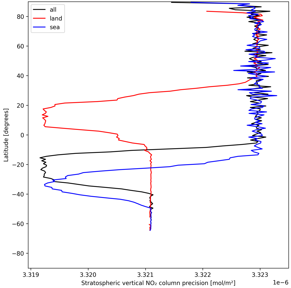
Figure 20: Zonal average of “Stratospheric vertical NO 2 column precision” for 2025-06-06 to 2025-06-08.
