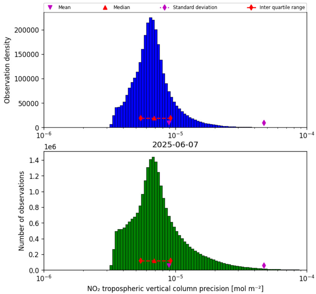
Figure 30: Histogram of “NO 2 tropospheric vertical column precision” for 2025-06-06 to 2025-06-08
