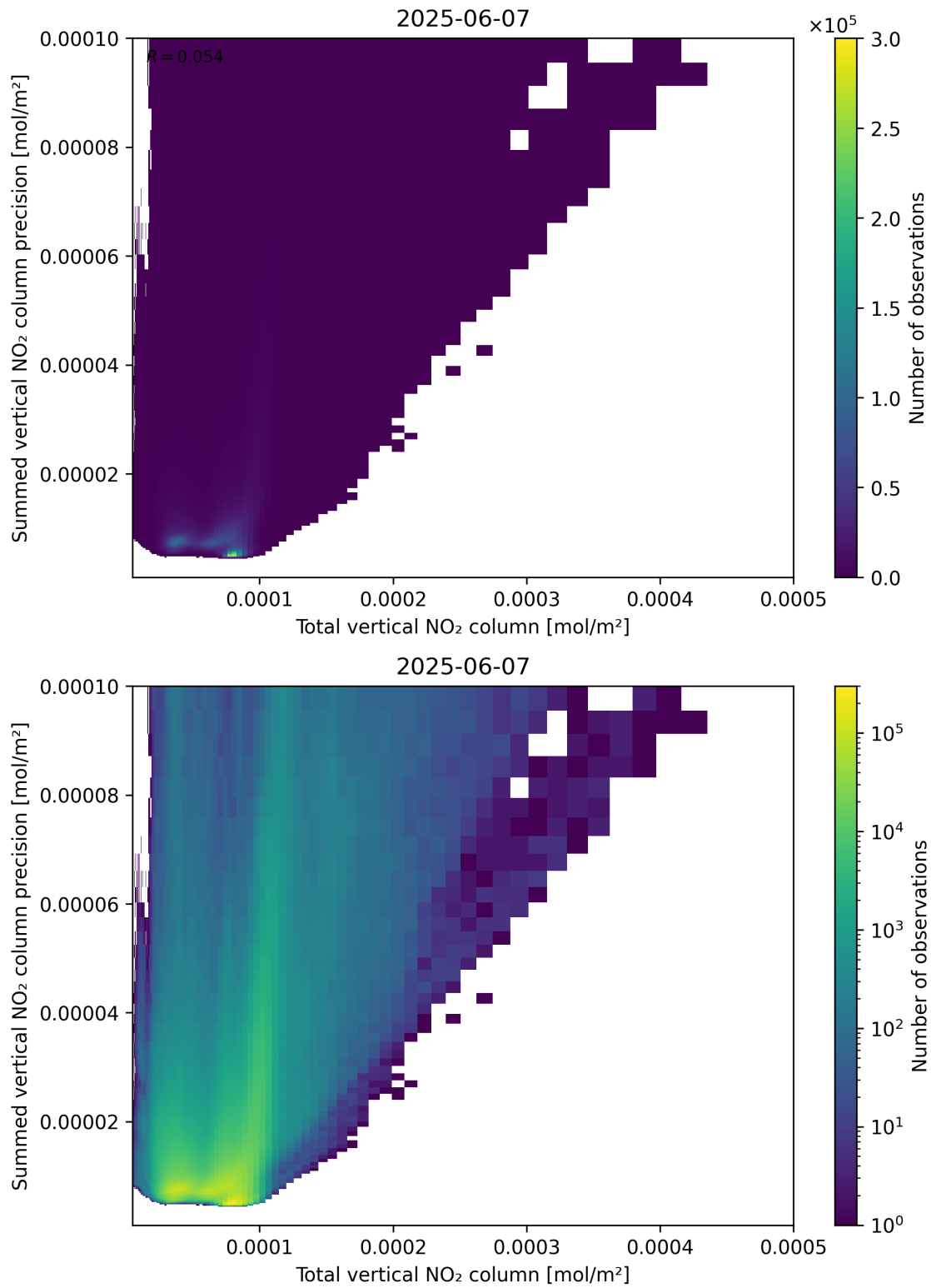
Figure 113: Scatter density plot of “Total vertical NO 2 column” against “Summed vertical NO 2 column precision” for 2025-06-06 to 2025-06-08.
