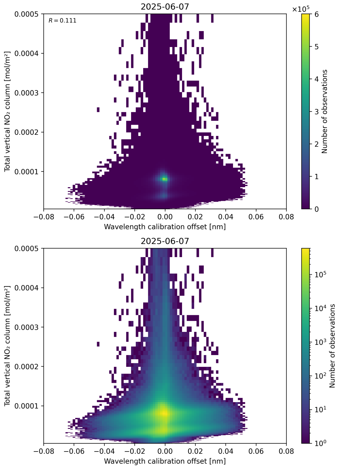
Figure 179: Scatter density plot of “Wavelength calibration offset” against “Total vertical NO 2 column” for 2025-06-06 to 2025-06-08.
