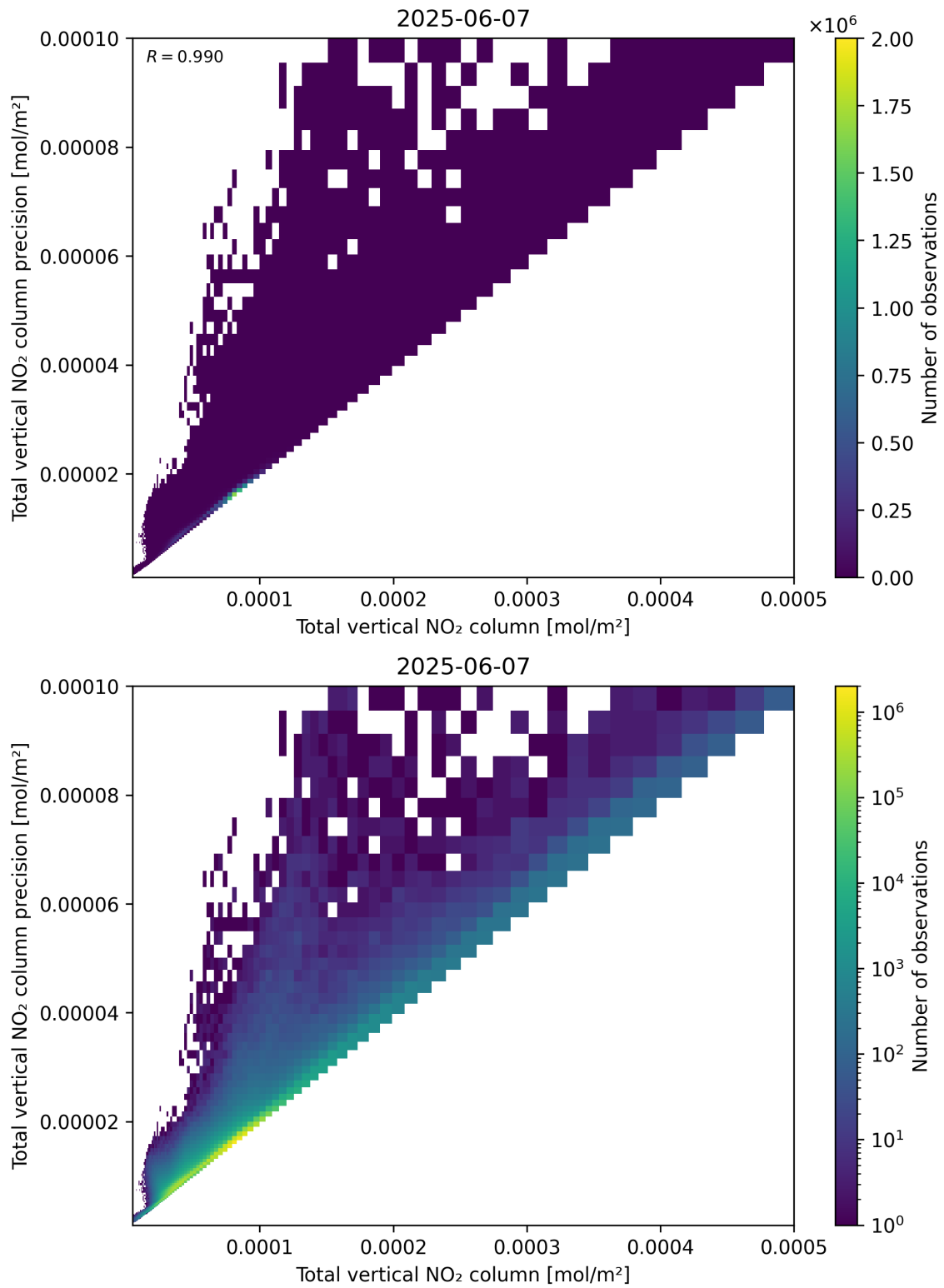
Figure 114: Scatter density plot of “Total vertical NO 2 column” against “Total vertical NO 2 column precision” for 2025-06-06 to 2025-06-08.
