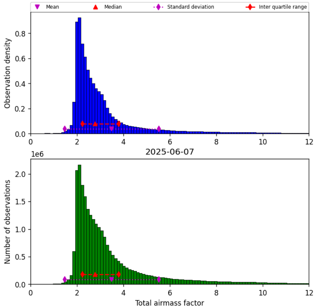
Figure 32: Histogram of “Total airmass factor” for 2025-06-06 to 2025-06-08
