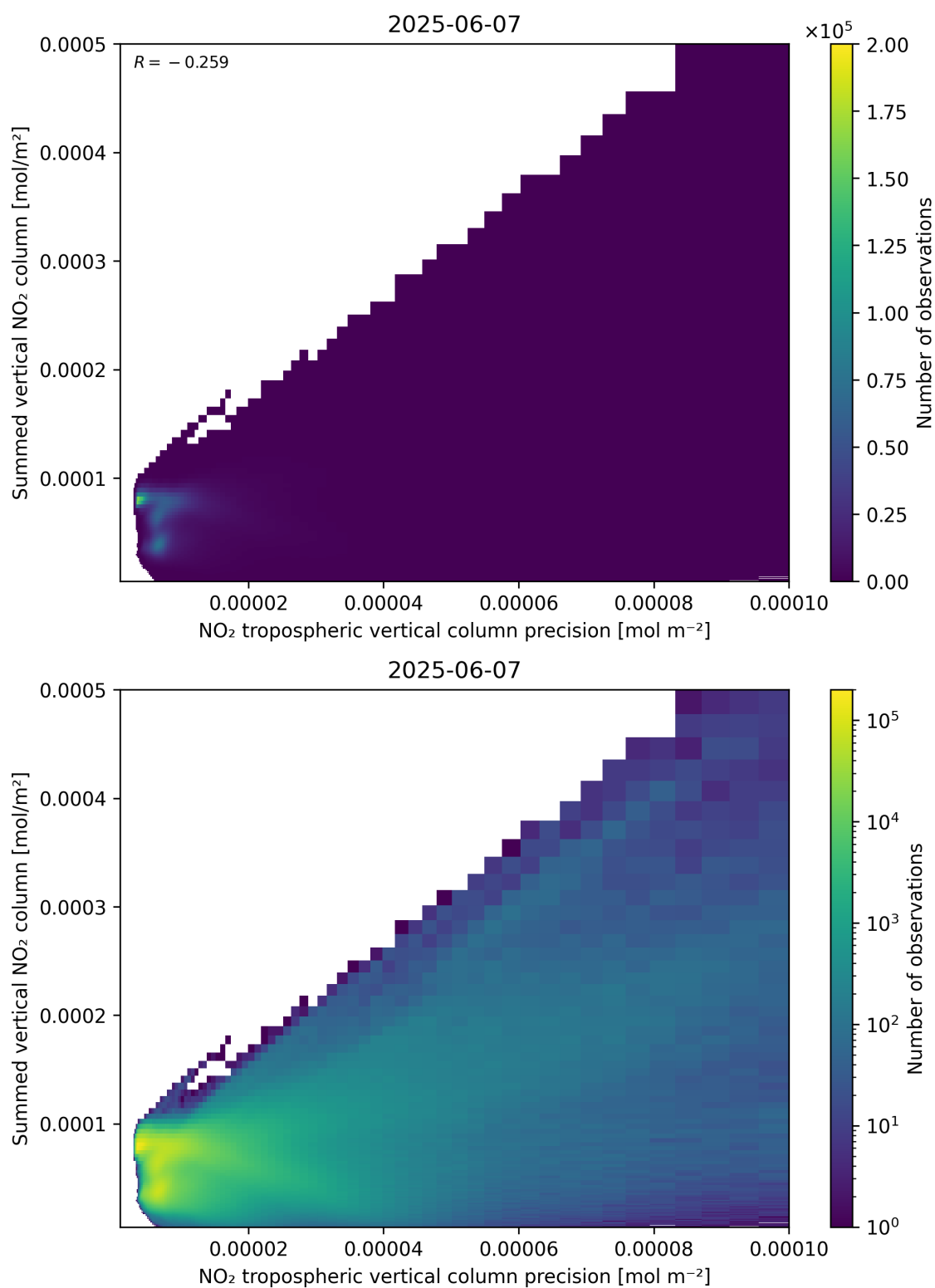
Figure 136: Scatter density plot of “NO 2 tropospheric vertical column precision” against “Summed vertical NO 2 column” for 2025-06-06 to 2025-06-08.
