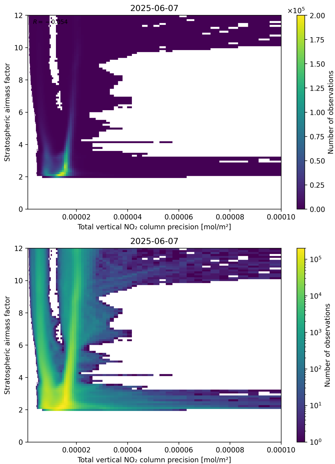
Figure 115: Scatter density plot of “Total vertical NO 2 column precision” against “Stratospheric air mass factor” for 2025-06-06 to 2025-06-08.
