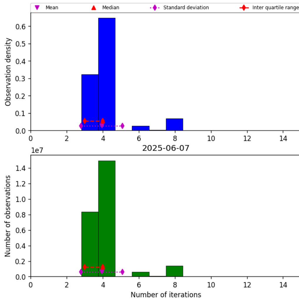
Figure 34: Histogram of “Number of iterations” for 2025-06-06 to 2025-06-08
