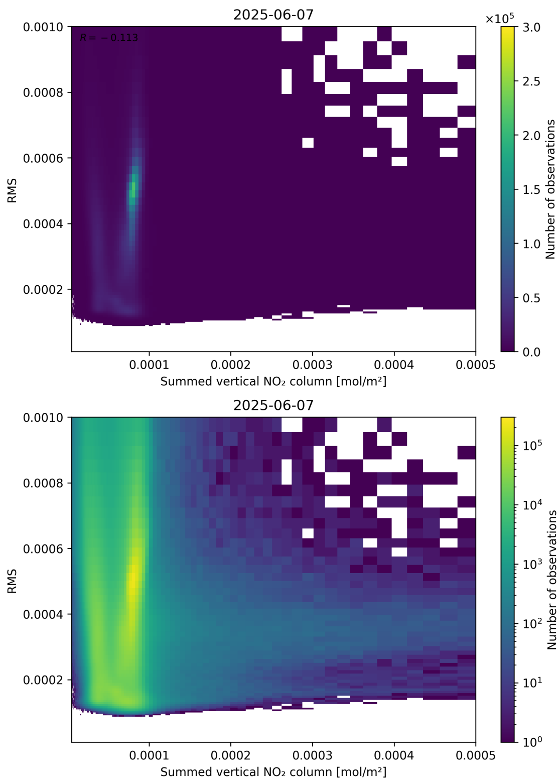
Figure 109: Scatter density plot of “Summed vertical NO 2 column” against “RMS” for 2025-06-06 to 2025-06-08.
