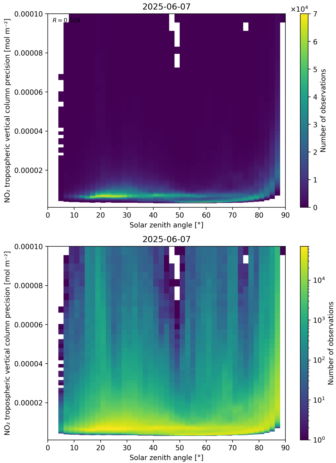
Figure 156: Scatter density plot of “Solar zenith angle” against “NO 2 tropospheric vertical column precision” for 2025-06-06 to 2025-06-08.
