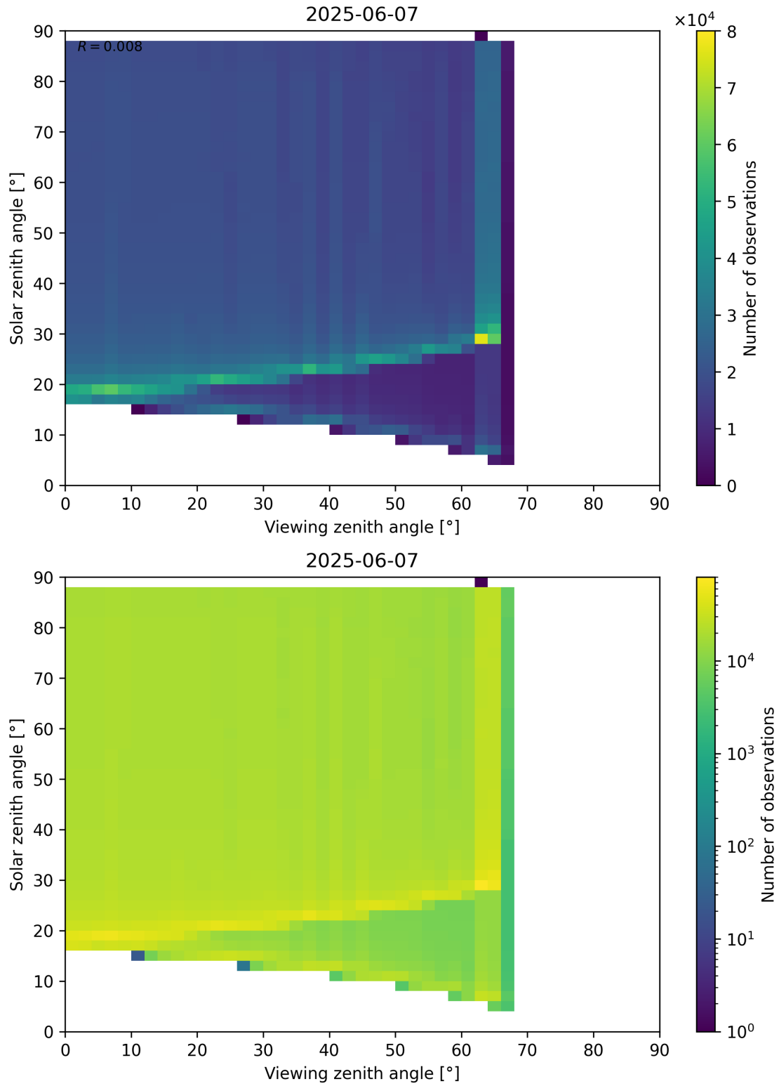
Figure 172: Scatter density plot of “Viewing zenith angle” against “Solar zenith angle” for 2025-06-06 to 2025-06-08.
