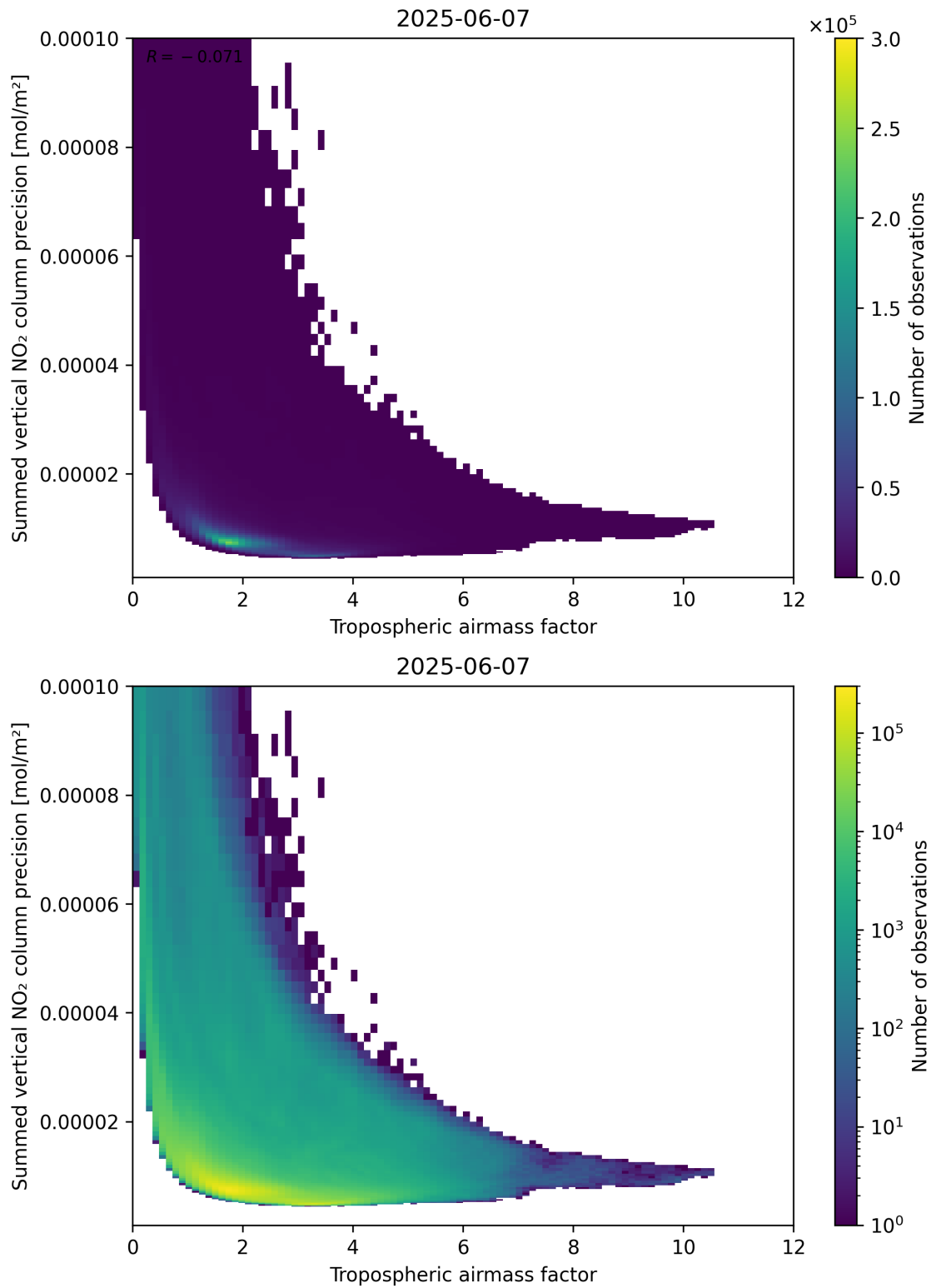
Figure 76: Scatter density plot of “Tropospheric air mass factor” against “Summed vertical NO 2 column precision” for 2025-06-06 to 2025-06-08.
