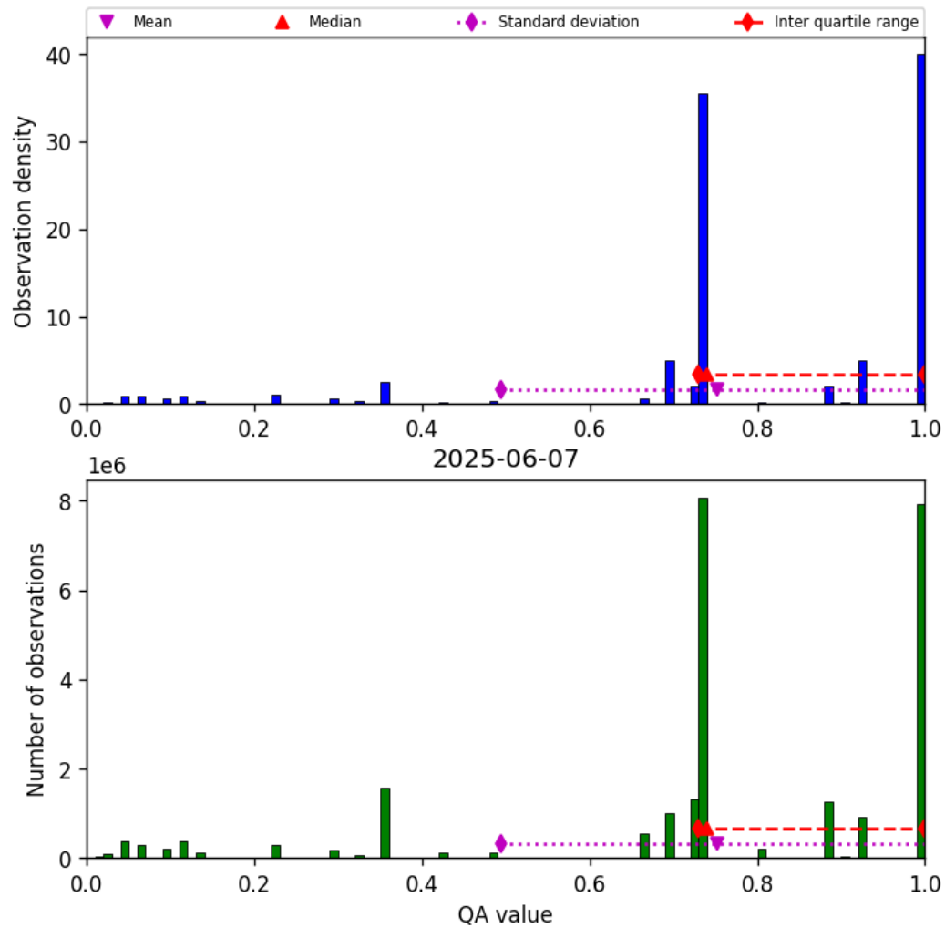
Figure 28: Histogram of “QA value” for 2025-06-06 to 2025-06-08
