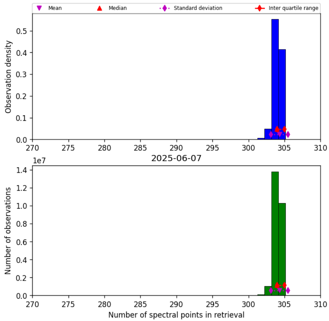
Figure 33: Histogram of “Number of spectral points in retrieval” for 2025-06-06 to 2025-06-08
