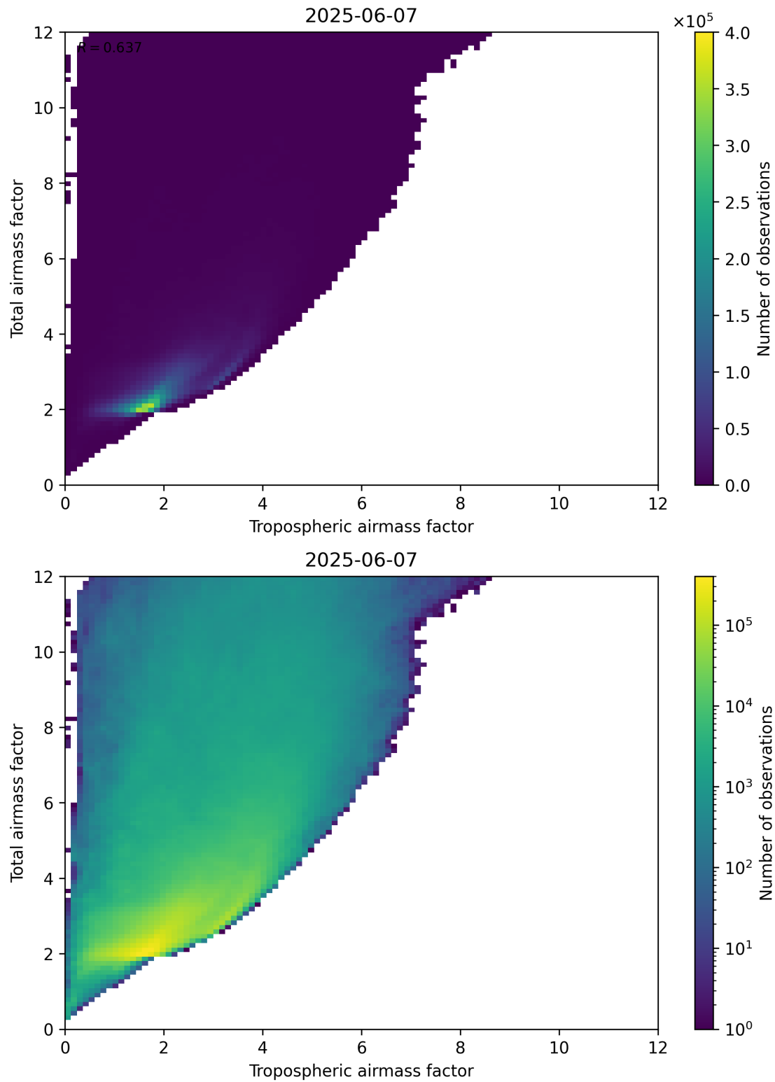
Figure 72: Scatter density plot of “Tropospheric airmass factor” against “Total airmass factor” for 2025-06-06 to 2025-06-08.
