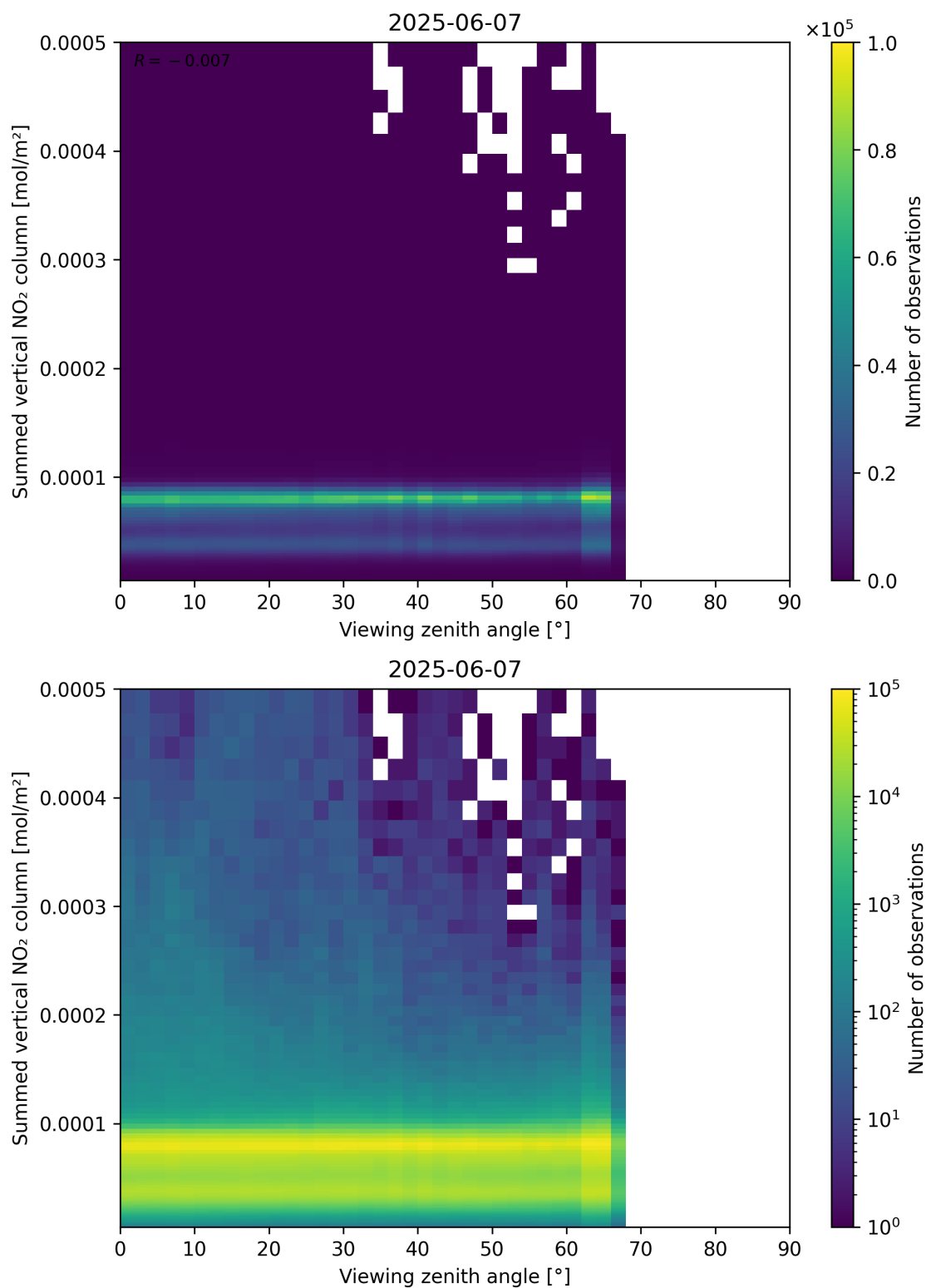
Figure 165: Scatter density plot of “Viewing zenith angle” against “Summed vertical NO 2 column” for 2025-06-06 to 2025-06-08.
