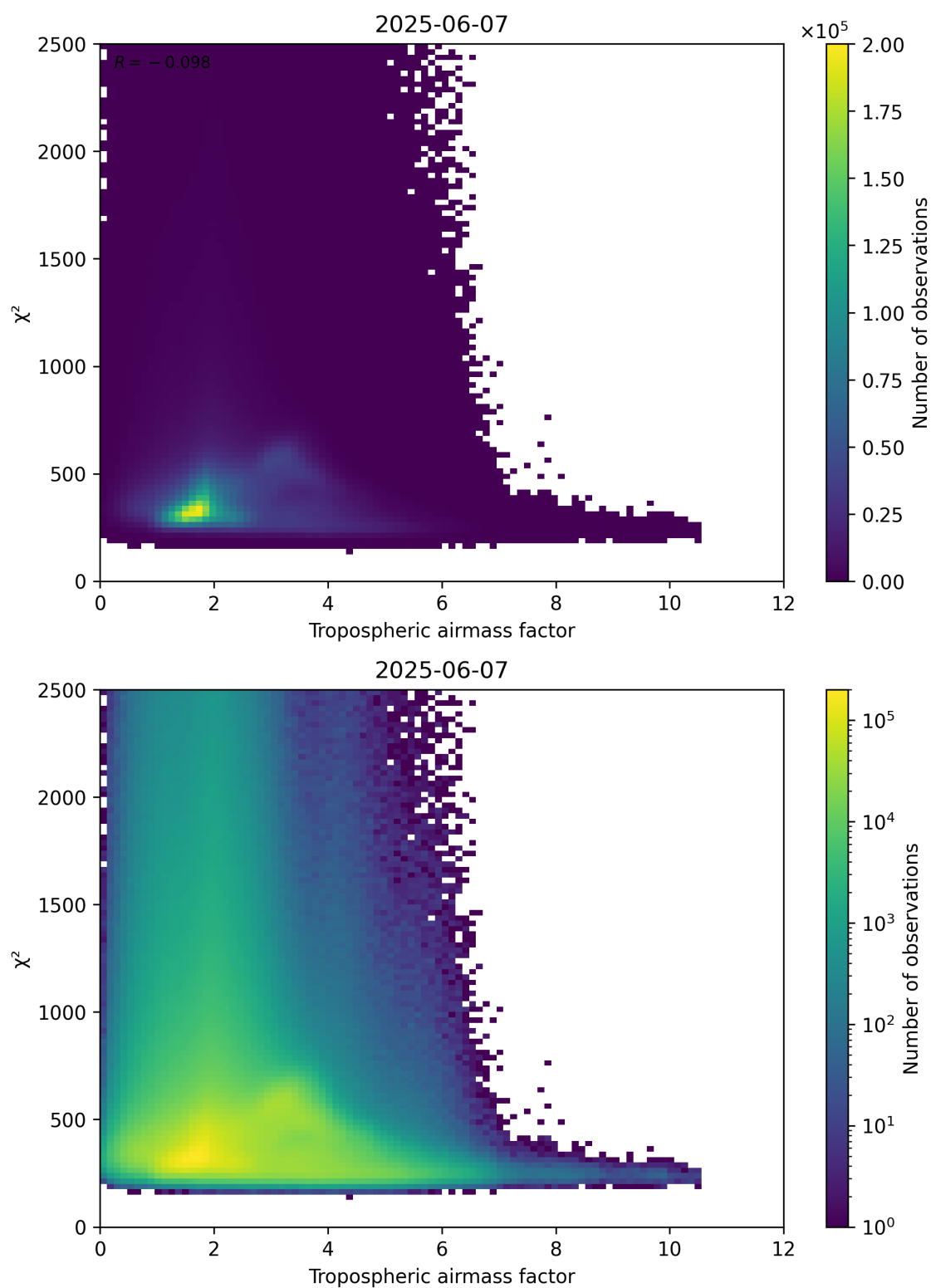
Figure 73: Scatter density plot of “Tropospheric airmass factor” against “ \chi^2 ” for 2025-06-06 to 2025-06-08.
