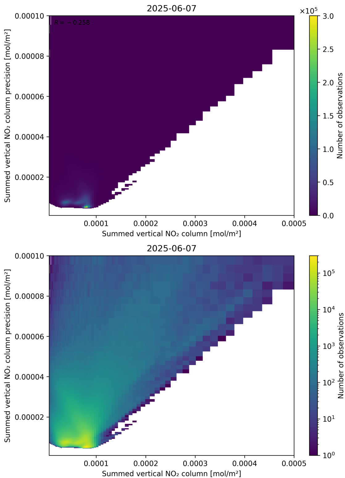
Figure 105: Scatter density plot of “Summed vertical NO 2 column” against “Summed vertical NO 2 column precision” for 2025-06-06 to 2025-06-08.
