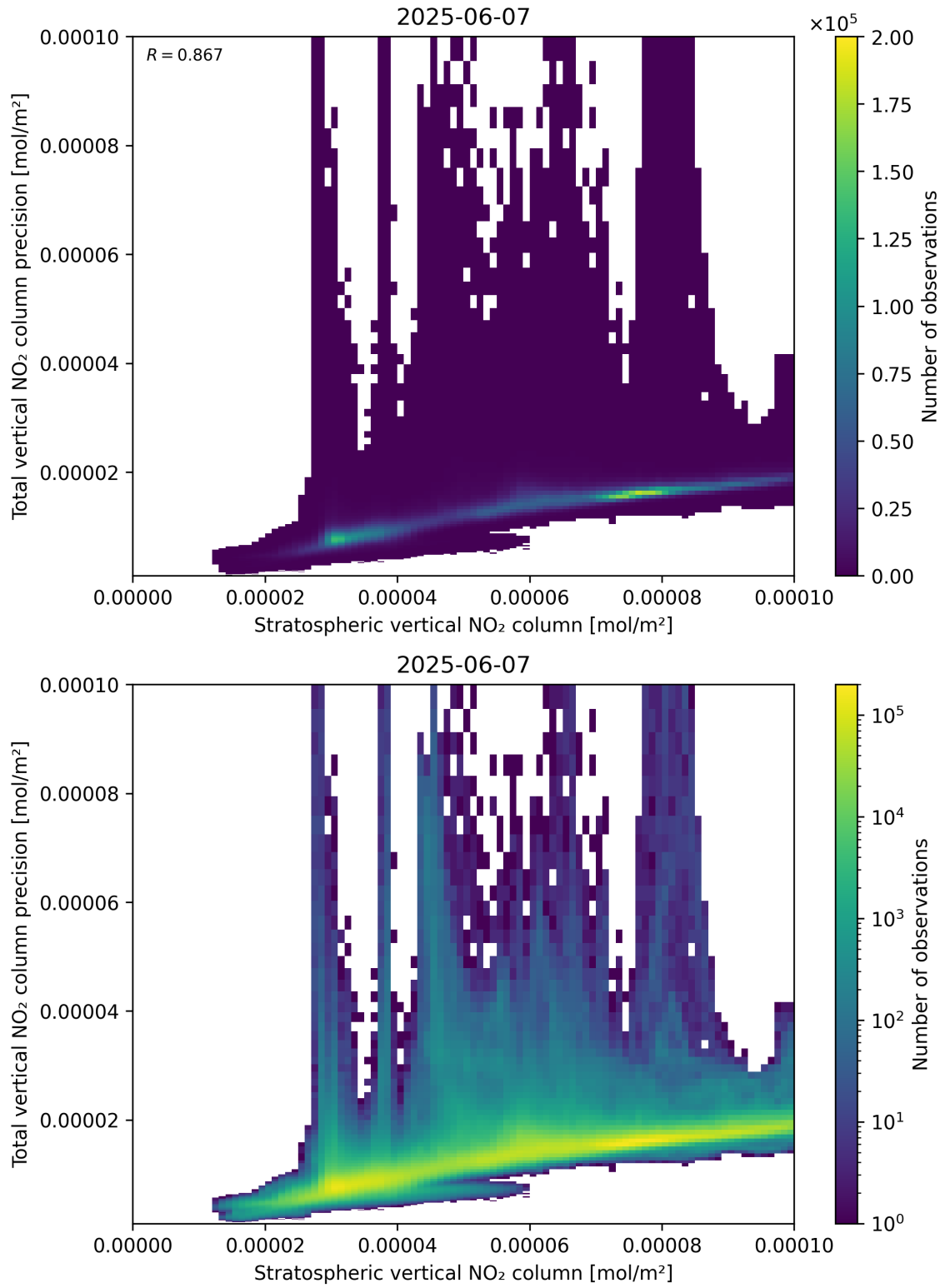
Figure 101: Scatter density plot of “Stratospheric vertical NO 2 column” against “Total vertical NO 2 column precision” for 2025-06-06 to 2025-06-08.
