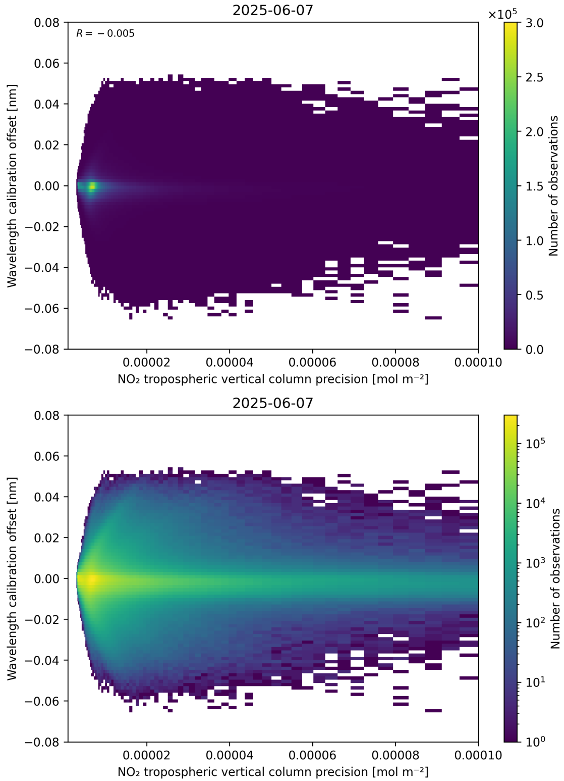
Figure 141: Scatter density plot of “NO 2 tropospheric vertical column precision” against “Wavelength calibration offset” for 2025-06-06 to 2025-06-08.
