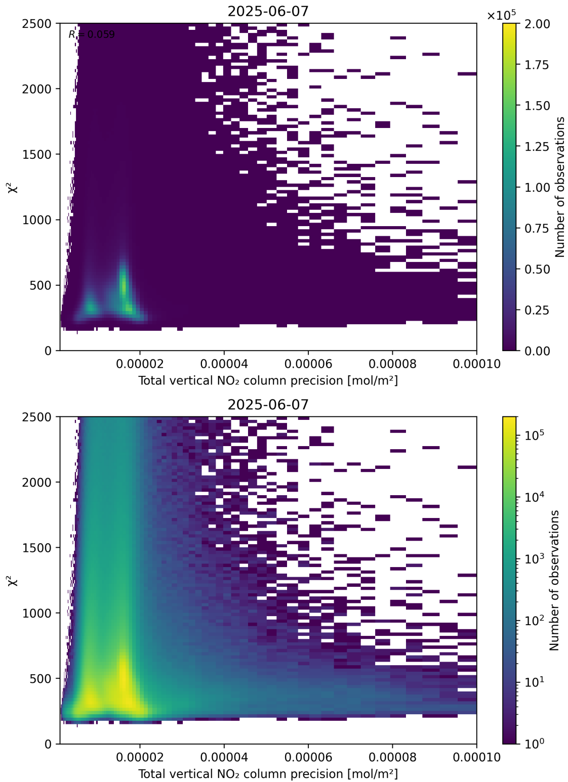
Figure 116: Scatter density plot of “Total vertical NO 2 column precision” against “ \chi^2 ” for 2025-06-06 to 2025-06-08.
