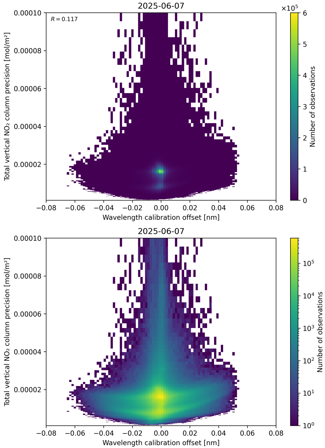
Figure 180: Scatter density plot of “Wavelength calibration offset” against “Total vertical NO 2 column precision” for 2025-06-06 to 2025-06-08.
