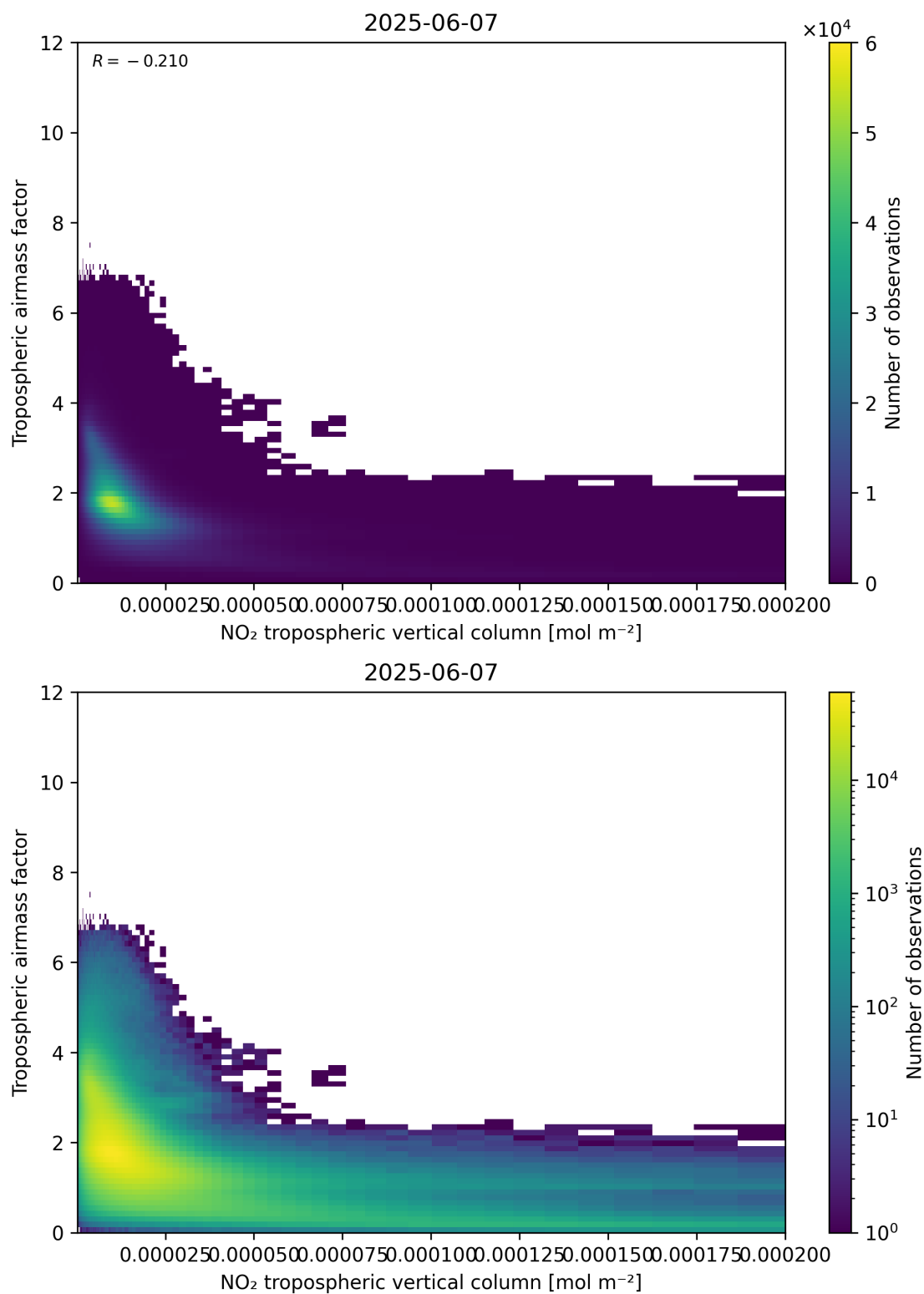
Figure 123: Scatter density plot of “NO 2 tropospheric vertical column” against “Tropospheric air mass factor” for 2025-06-06 to 2025-06-08.
