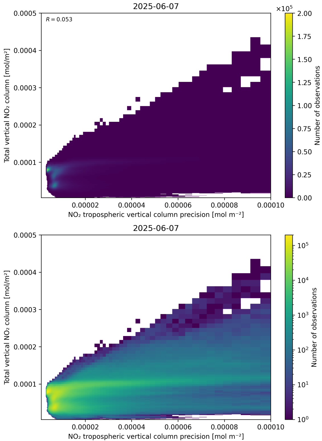
Figure 138: Scatter density plot of “NO 2 tropospheric vertical column precision” against “Total vertical NO 2 column” for 2025-06-06 to 2025-06-08.
