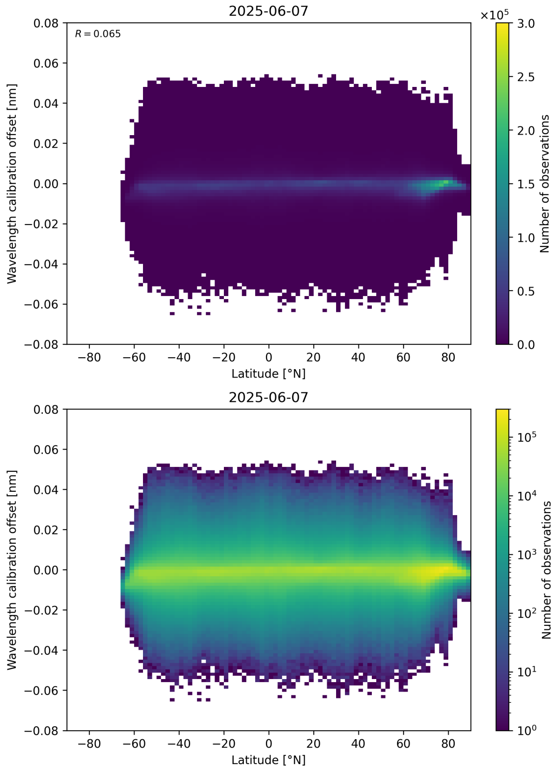
Figure 95: Scatter density plot of “Latitude” against “Wavelength calibration offset” for 2025-06-06 to 2025-06-08.
