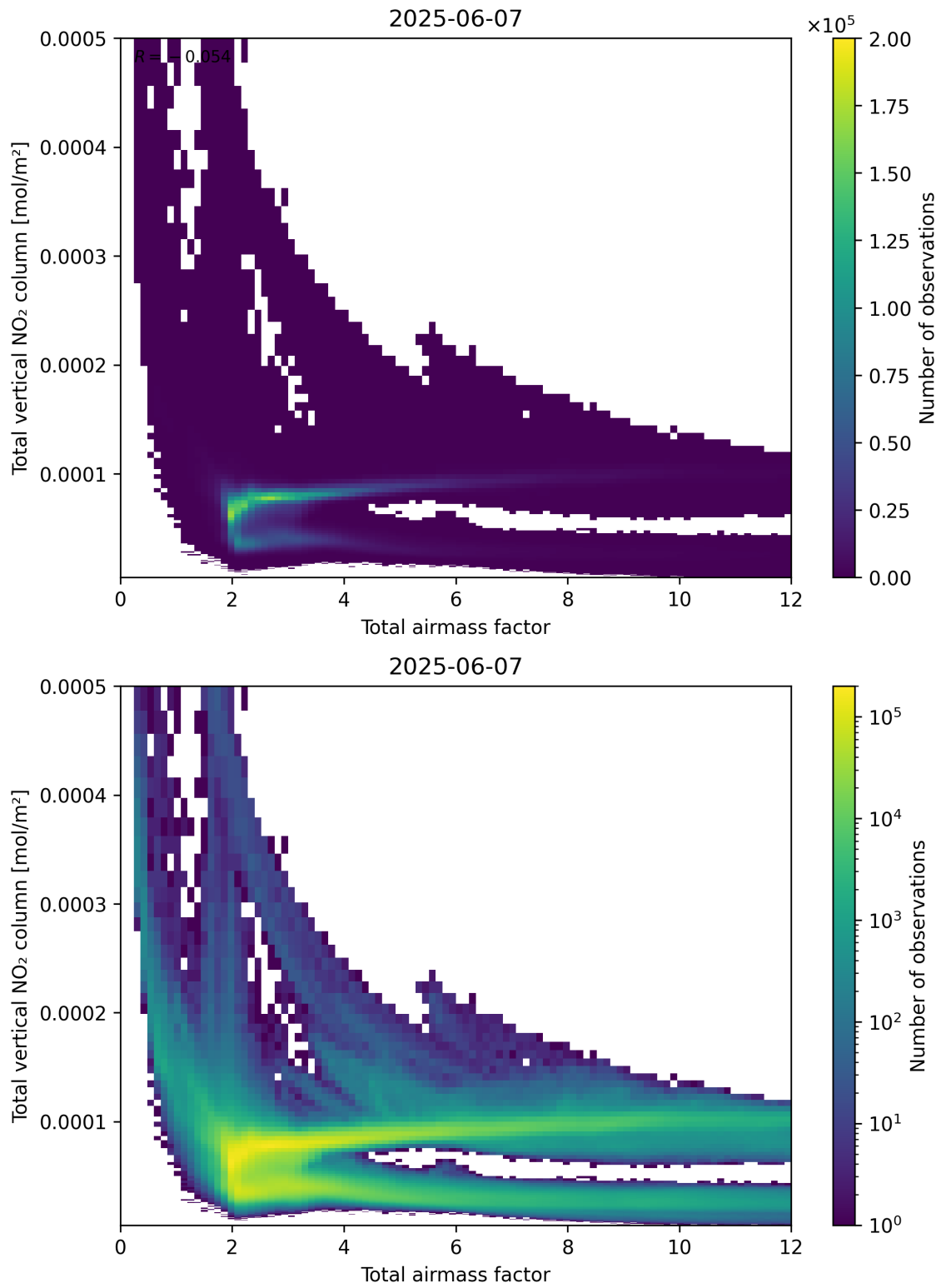
Figure 67: Scatter density plot of “Total airmass factor” against “Total vertical NO 2 column” for 2025-06-06 to 2025-06-08.
