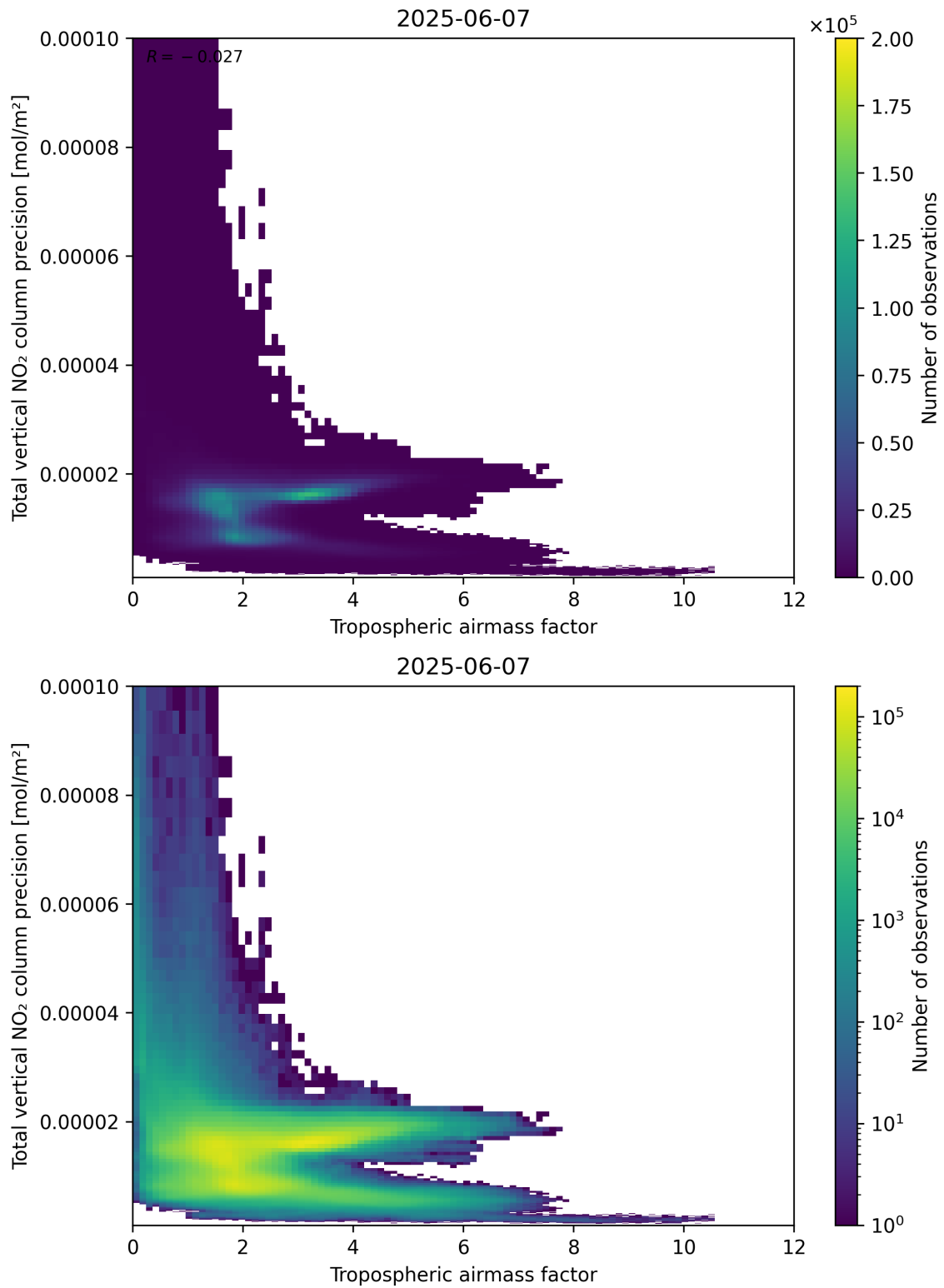
Figure 78: Scatter density plot of “Tropospheric air mass factor” against “Total vertical NO 2 column precision” for 2025-06-06 to 2025-06-08.
