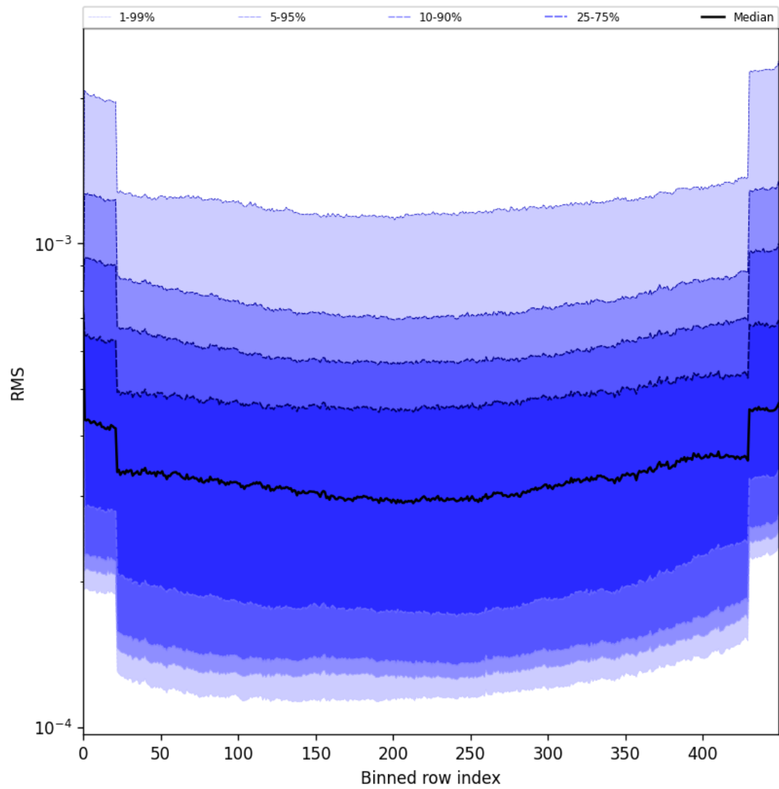
Figure 60: Along track statistics of “RMS” for 2025-06-06 to 2025-06-08
