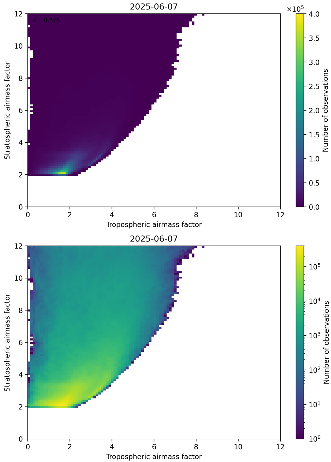
Figure 71: Scatter density plot of “Tropospheric airmass factor” against “Stratospheric airmass factor” for 2025-06-06 to 2025-06-08.
