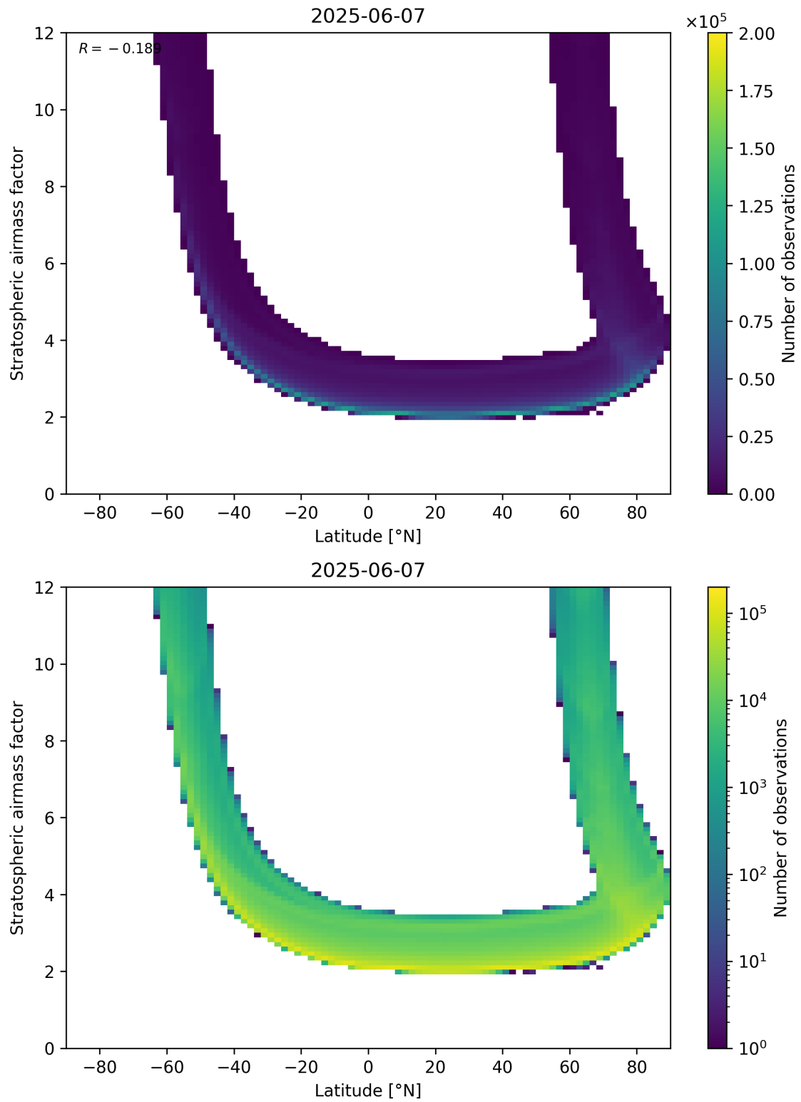
Figure 83: Scatter density plot of “Latitude” against “Stratospheric air mass factor” for 2025-06-06 to 2025-06-08.
