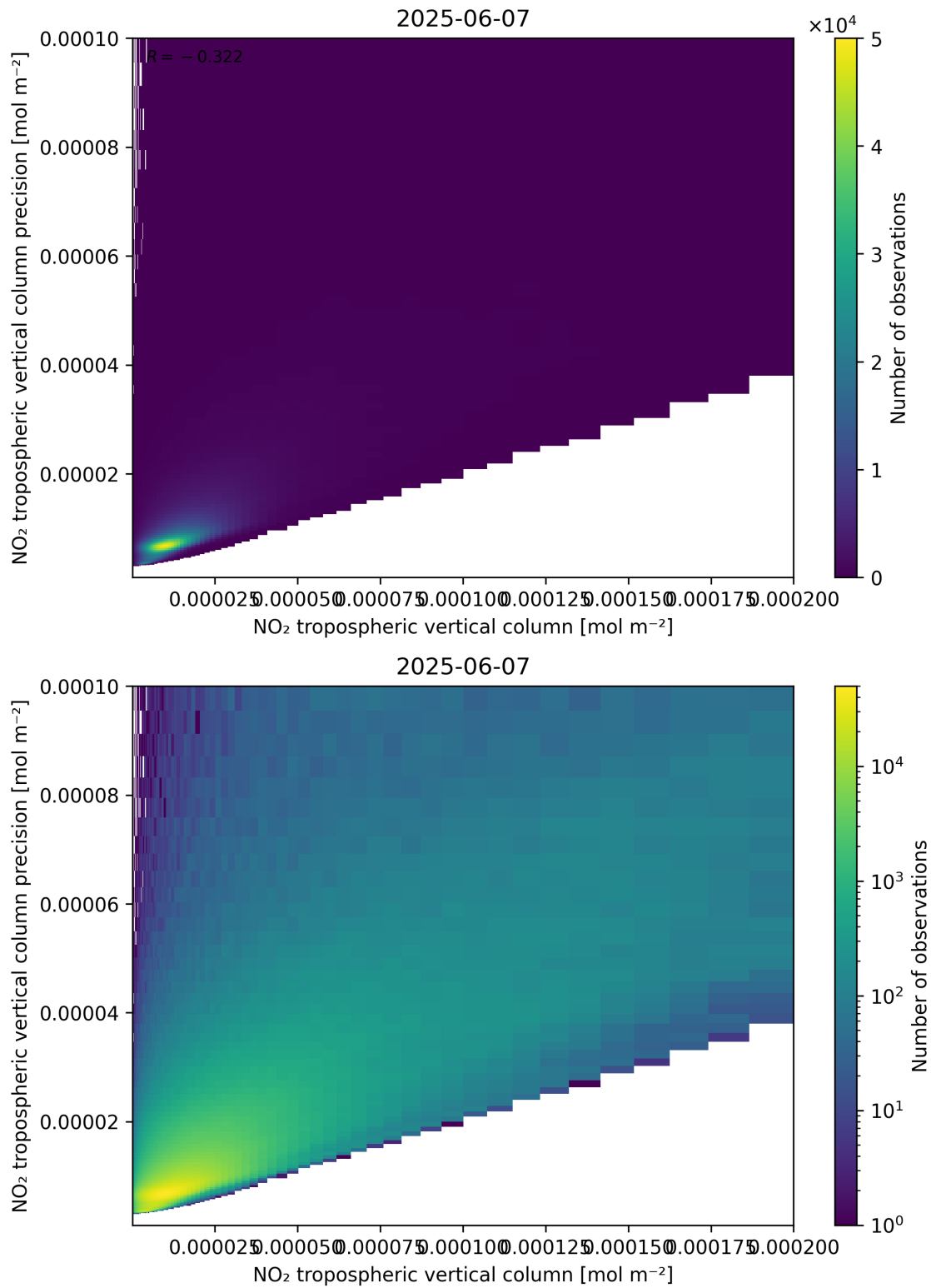
Figure 130: Scatter density plot of “NO 2 tropospheric vertical column” against “NO 2 tropospheric vertical column precision” for 2025-06-06 to 2025-06-08.
