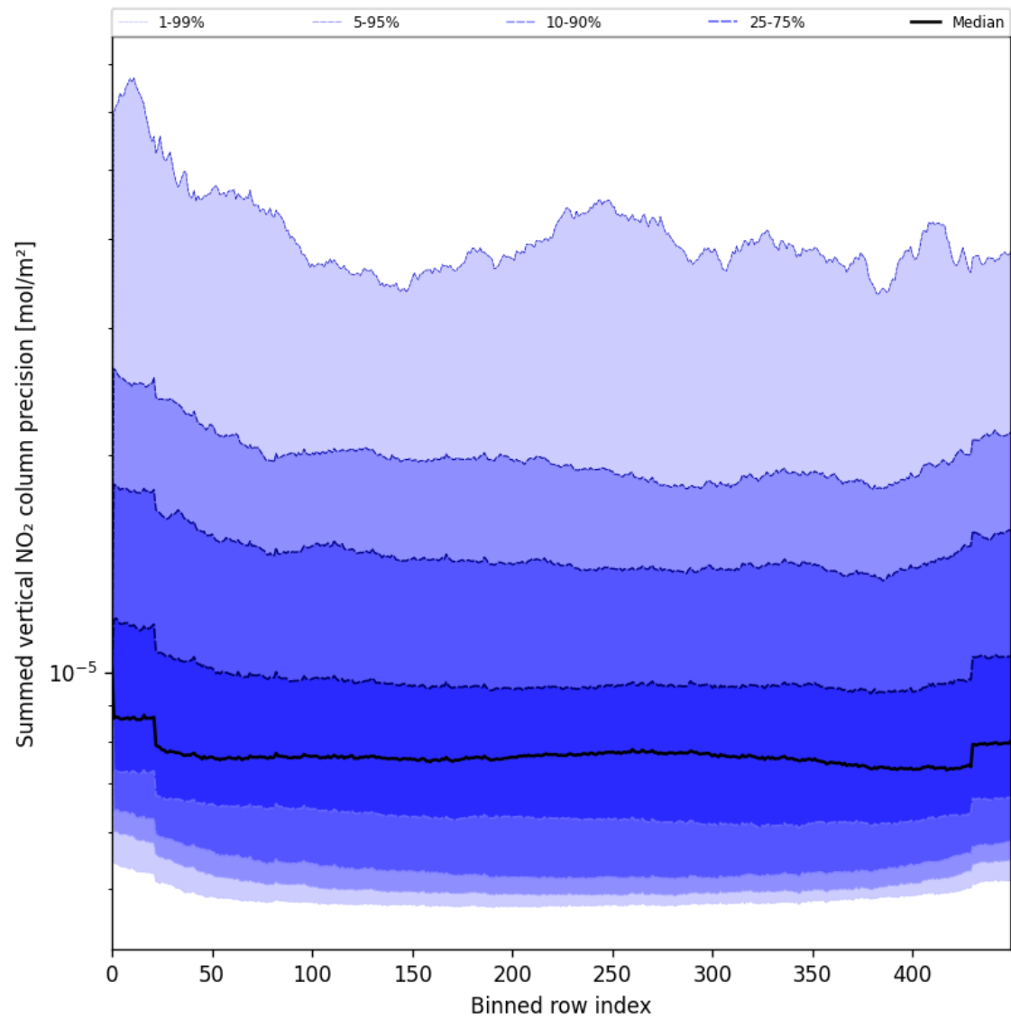
Figure 58: Along track statistics of “Summed vertical NO 2 column precision” for 2025-06-06 to 2025-06-08
