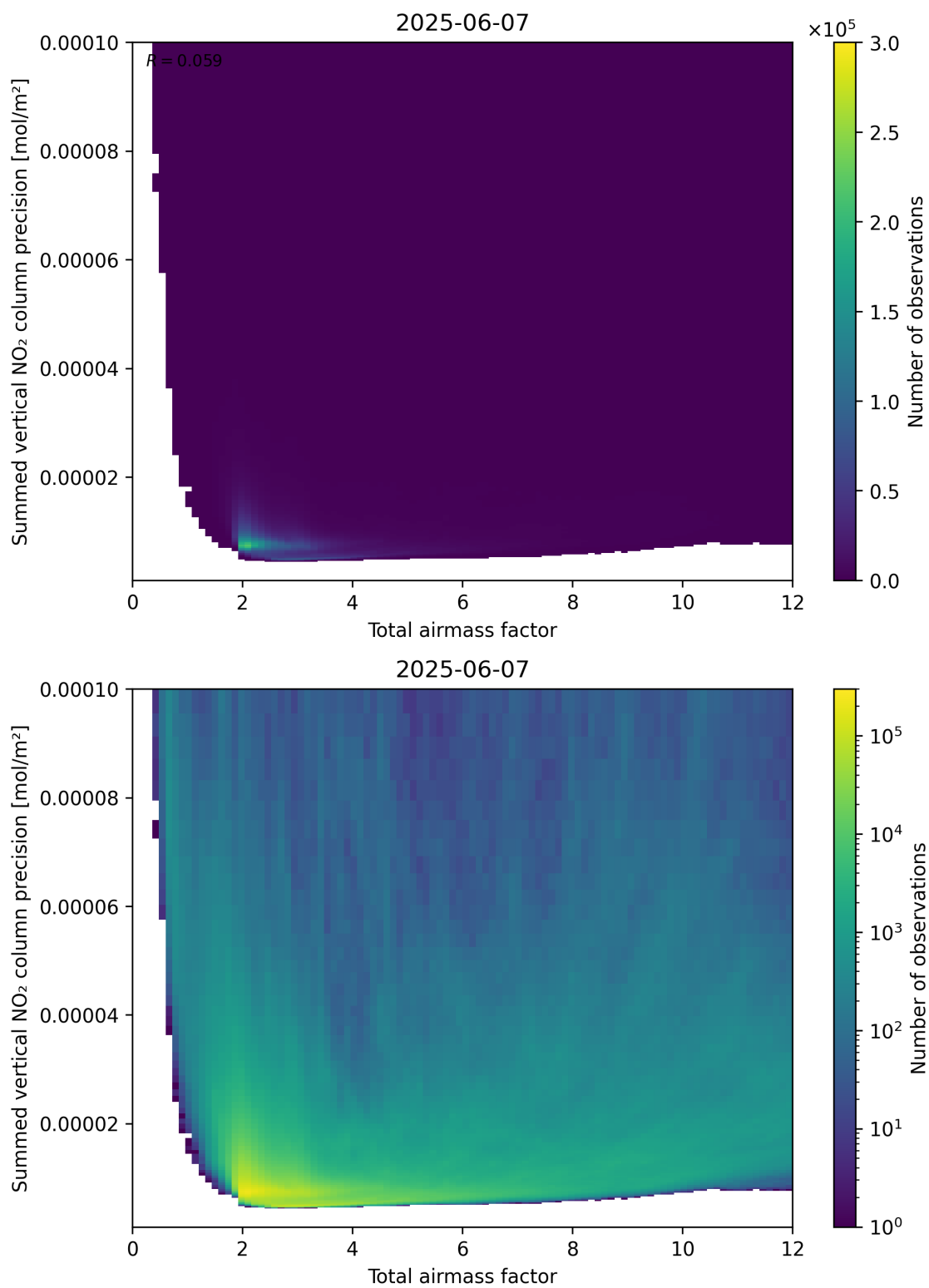
Figure 66: Scatter density plot of “Total airmass factor” against “Summed vertical NO 2 column precision” for 2025-06-06 to 2025-06-08.
