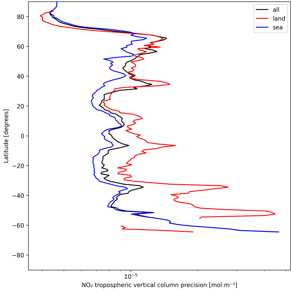
Figure 13: Zonal average of “NO 2 tropospheric vertical column precision” for 2025-06-06 to 2025-06-08.
