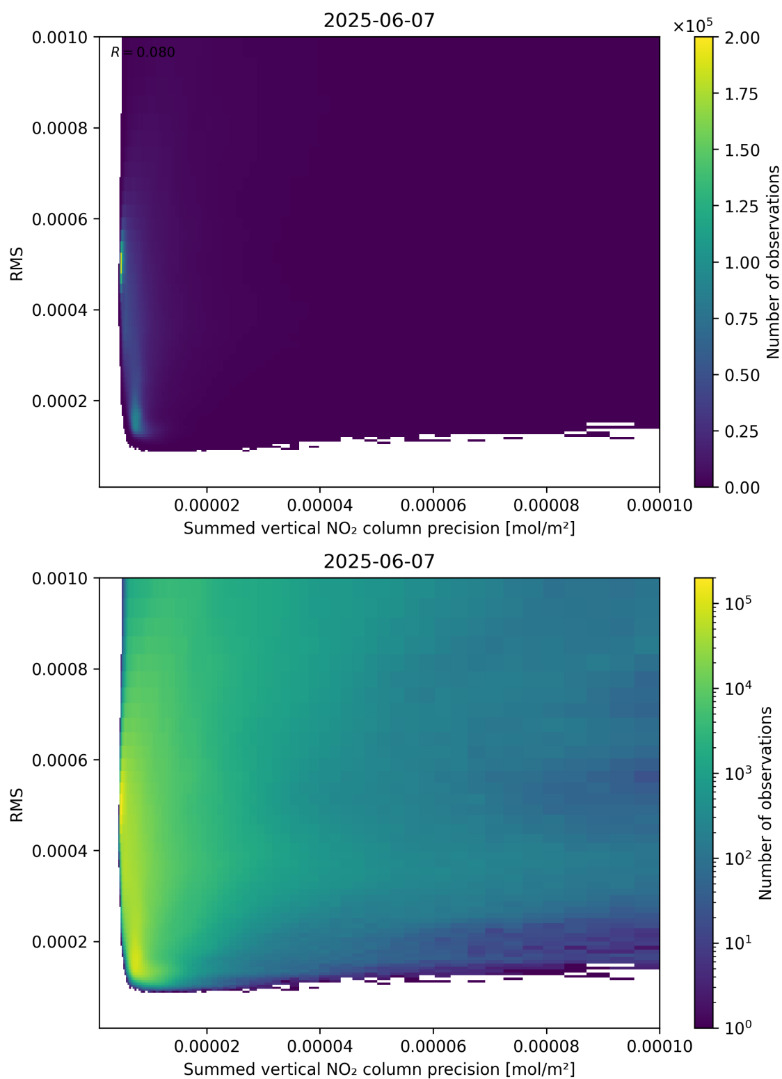
Figure 108: Scatter density plot of “Summed vertical NO 2 column precision” against “RMS” for 2025-06-06 to 2025-06-08.
