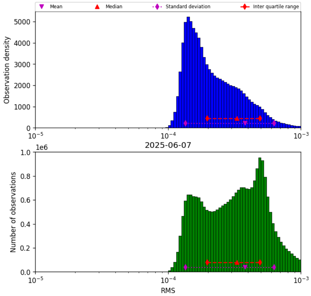
Figure 43: Histogram of “RMS” for 2025-06-06 to 2025-06-08
