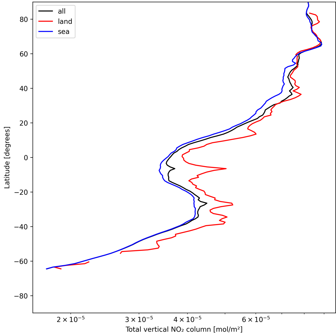
Figure 21: Zonal average of “Total vertical NO 2 column” for 2025-06-06 to 2025-06-08.
