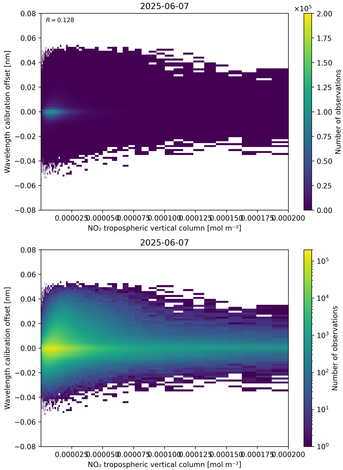
Figure 143: Scatter density plot of “NO 2 tropospheric vertical column” against “Wavelength calibration offset” for 2025-06-06 to 2025-06-08.
