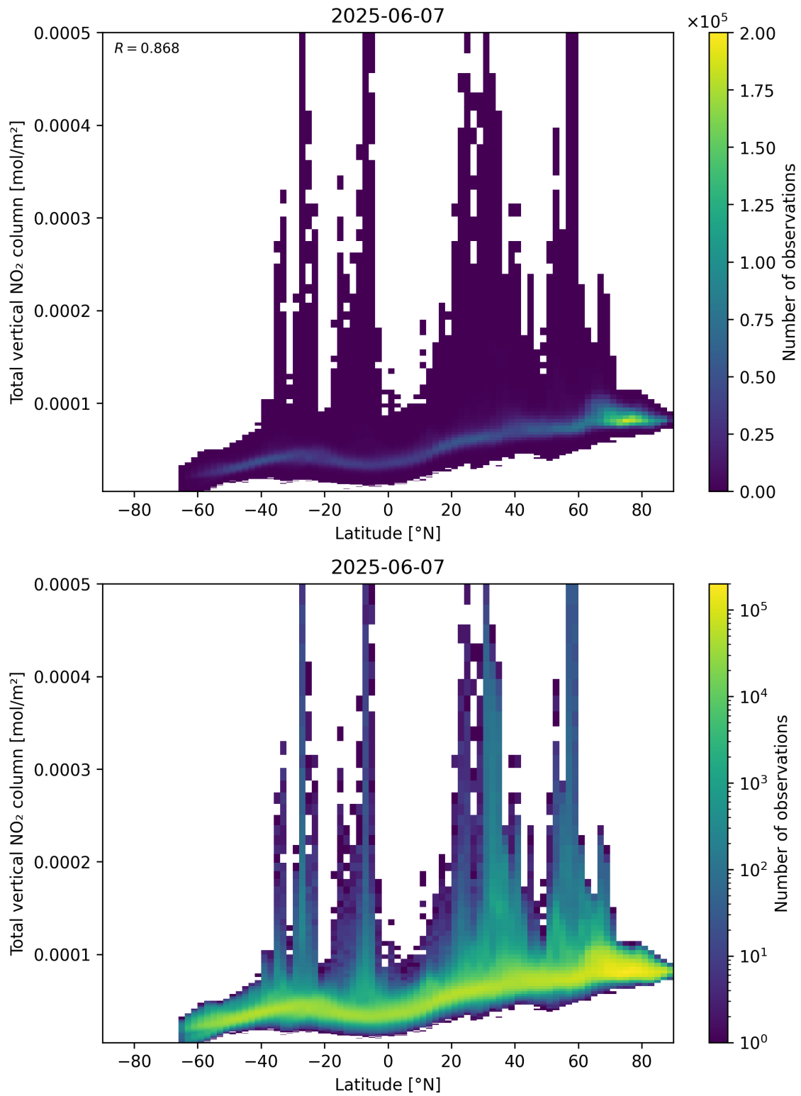
Figure 90: Scatter density plot of “Latitude” against “Total vertical NO 2 column” for 2025-06-06 to 2025-06-08.
