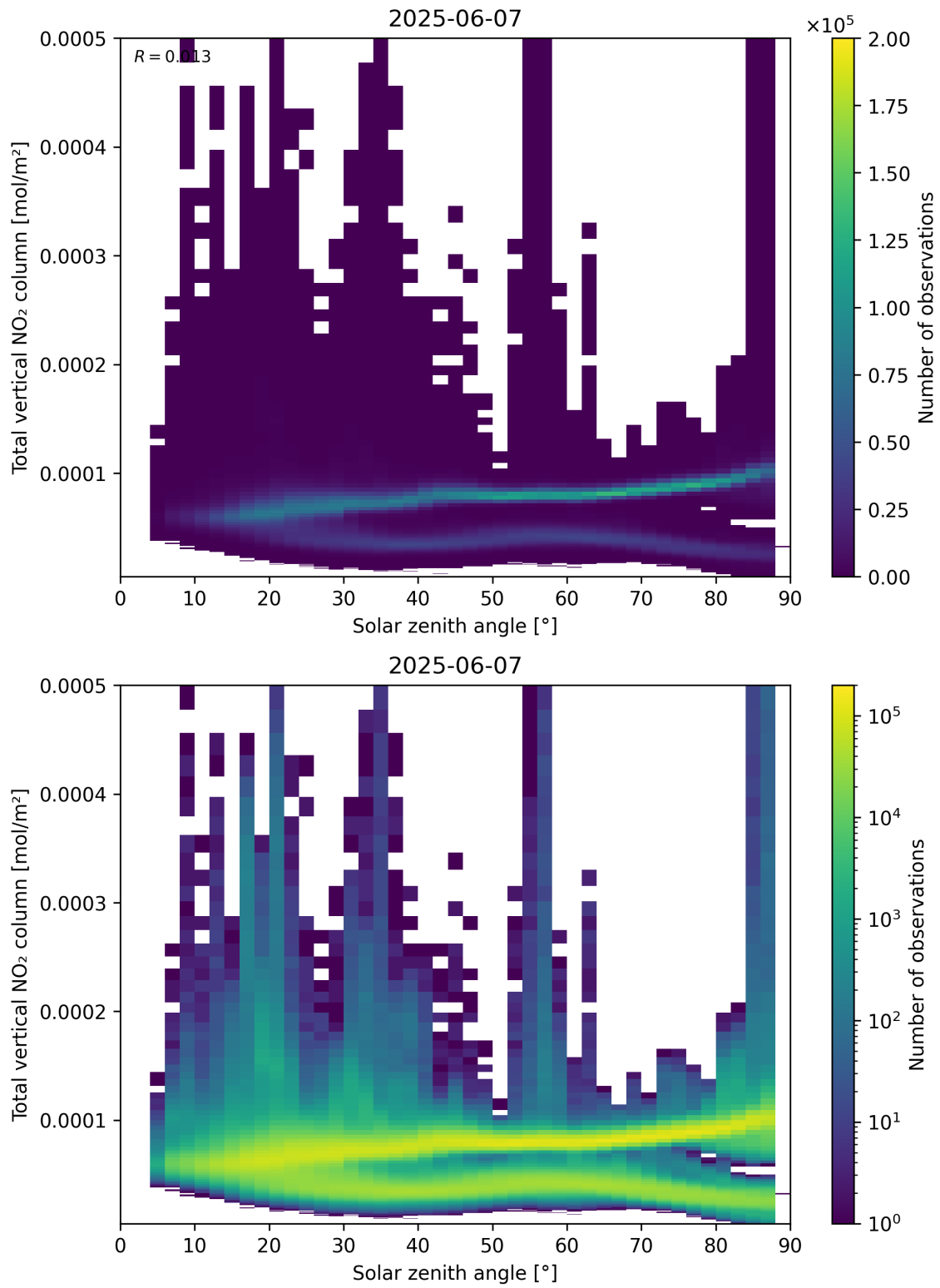
Figure 153: Scatter density plot of “Solar zenith angle” against “Total vertical NO 2 column” for 2025-06-06 to 2025-06-08.
