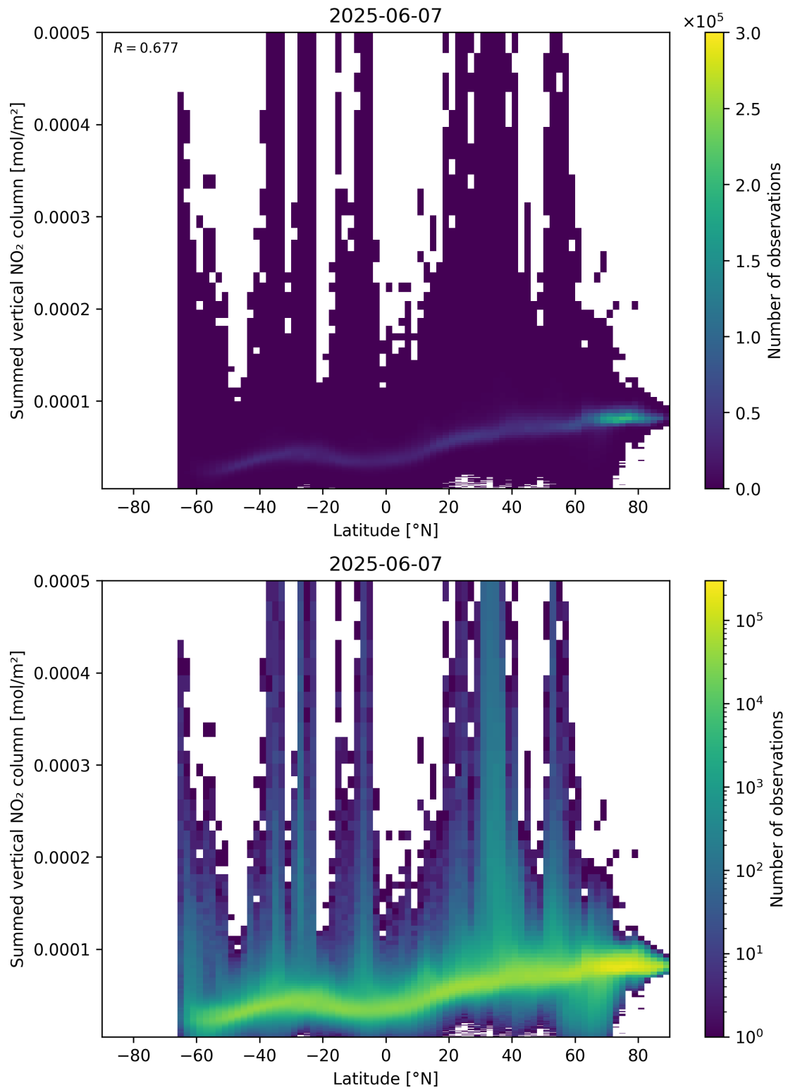
Figure 88: Scatter density plot of “Latitude” against “Summed vertical NO 2 column” for 2025-06-06 to 2025-06-08.
