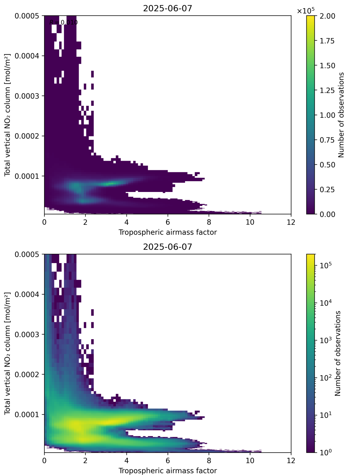
Figure 77: Scatter density plot of “Tropospheric airmass factor” against “Total vertical NO 2 column” for 2025-06-06 to 2025-06-08.
