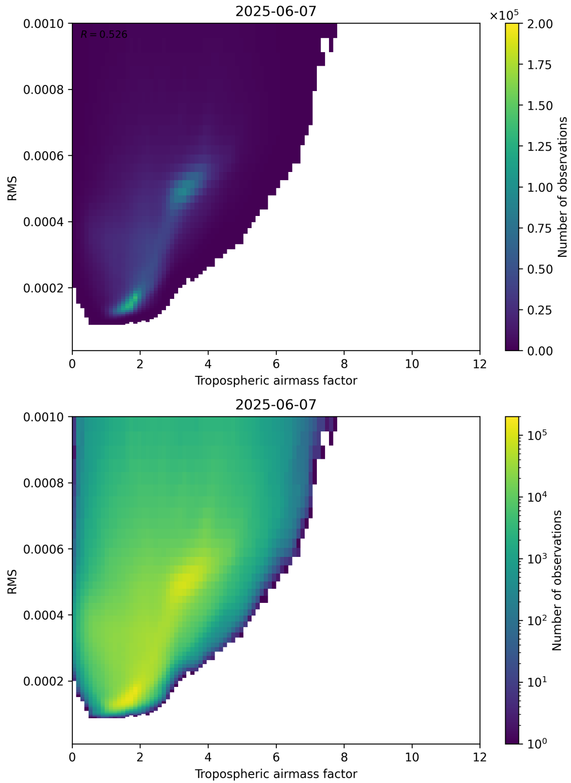
Figure 79: Scatter density plot of “Tropospheric airmass factor” against “RMS” for 2025-06-06 to 2025-06-08.
