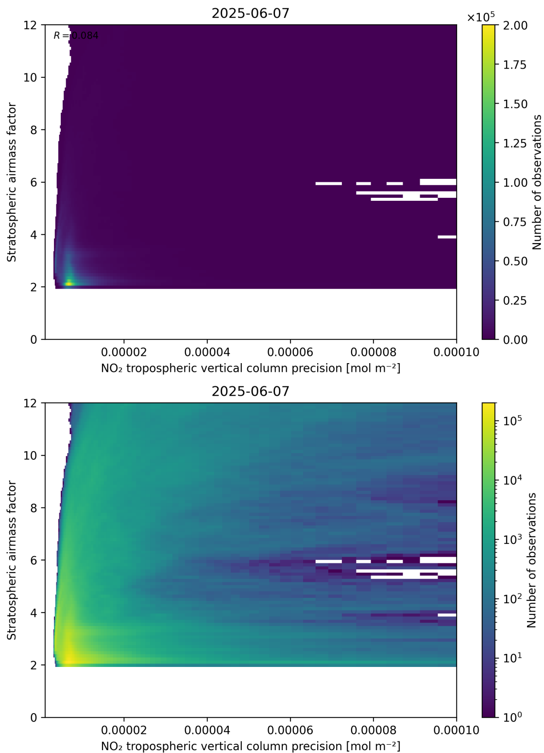
Figure 131: Scatter density plot of “NO 2 tropospheric vertical column precision” against “Stratospheric airmass factor” for 2025-06-06 to 2025-06-08.
