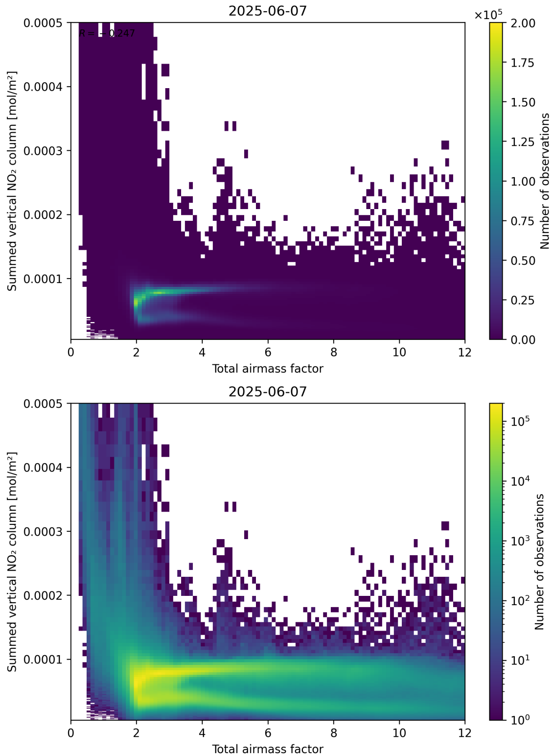
Figure 65: Scatter density plot of “Total airmass factor” against “Summed vertical NO 2 column” for 2025-06-06 to 2025-06-08.
