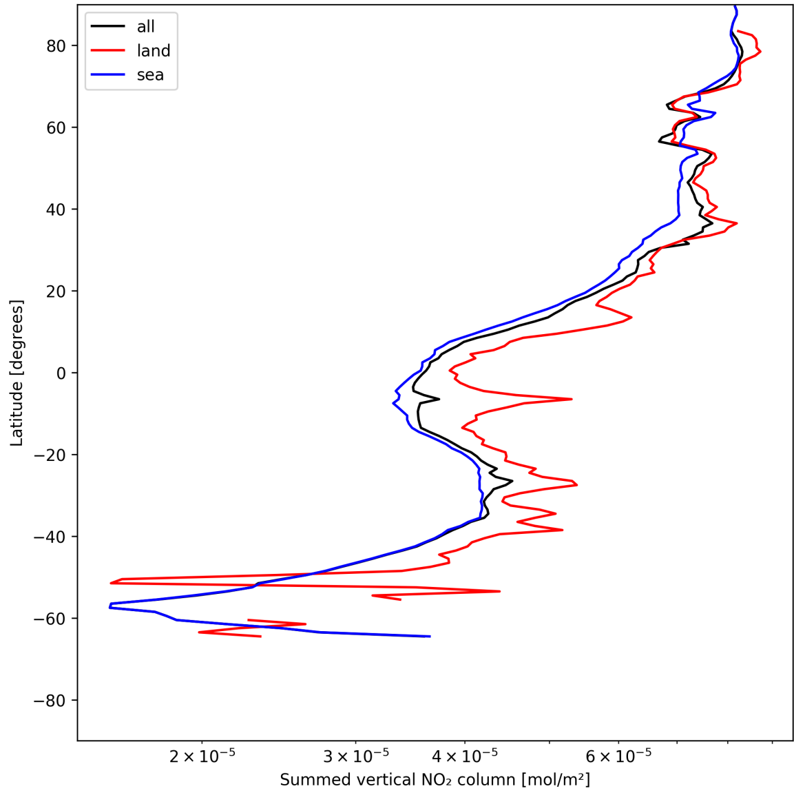
Figure 23: Zonal average of “Summed vertical NO 2 column” for 2025-06-06 to 2025-06-08.
