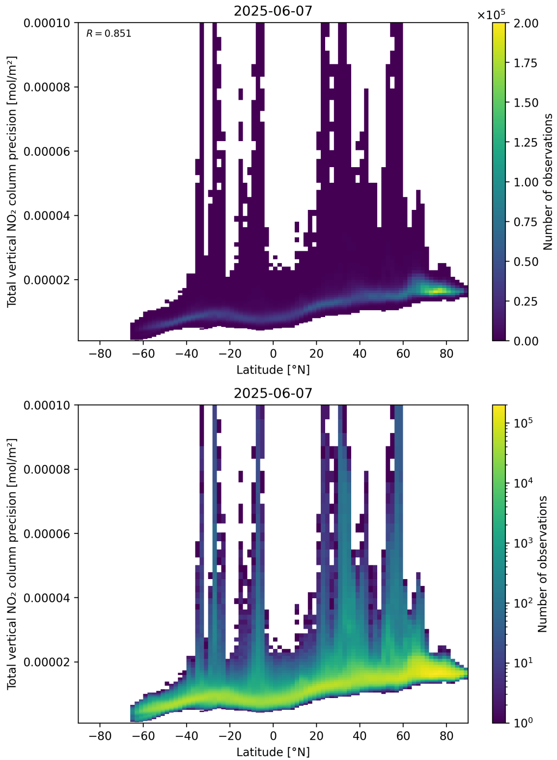
Figure 91: Scatter density plot of “Latitude” against “Total vertical NO 2 column precision” for 2025-06-06 to 2025-06-08.
