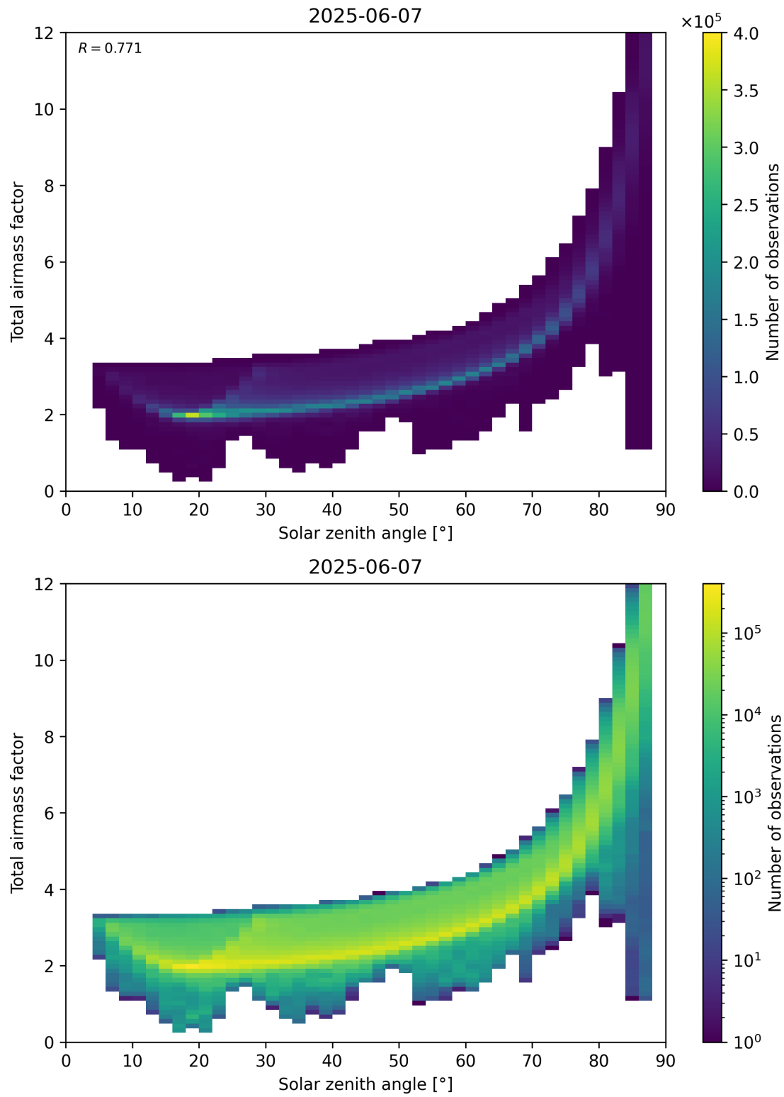
Figure 146: Scatter density plot of “Solar zenith angle” against “Total air mass factor” for 2025-06-06 to 2025-06-08.
