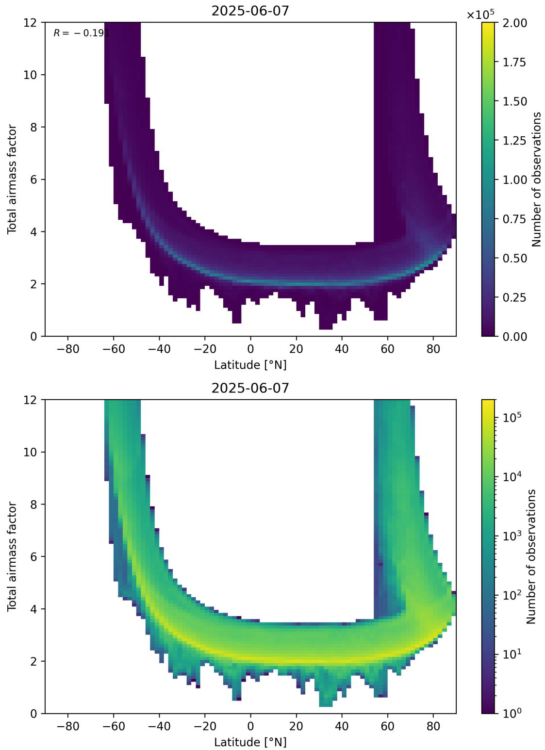
Figure 84: Scatter density plot of “Latitude” against “Total airmass factor” for 2025-06-06 to 2025-06-08.
