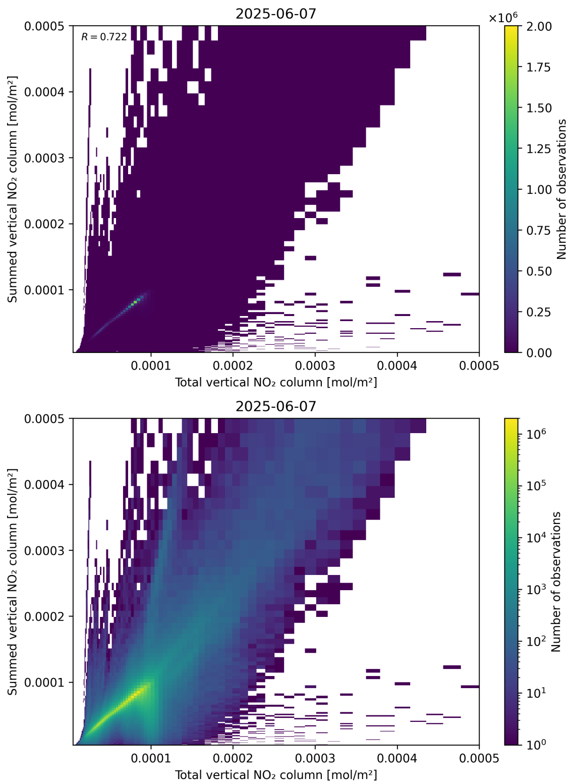
Figure 112: Scatter density plot of “Total vertical NO 2 column” against “Summed vertical NO 2 column” for 2025-06-06 to 2025-06-08.
