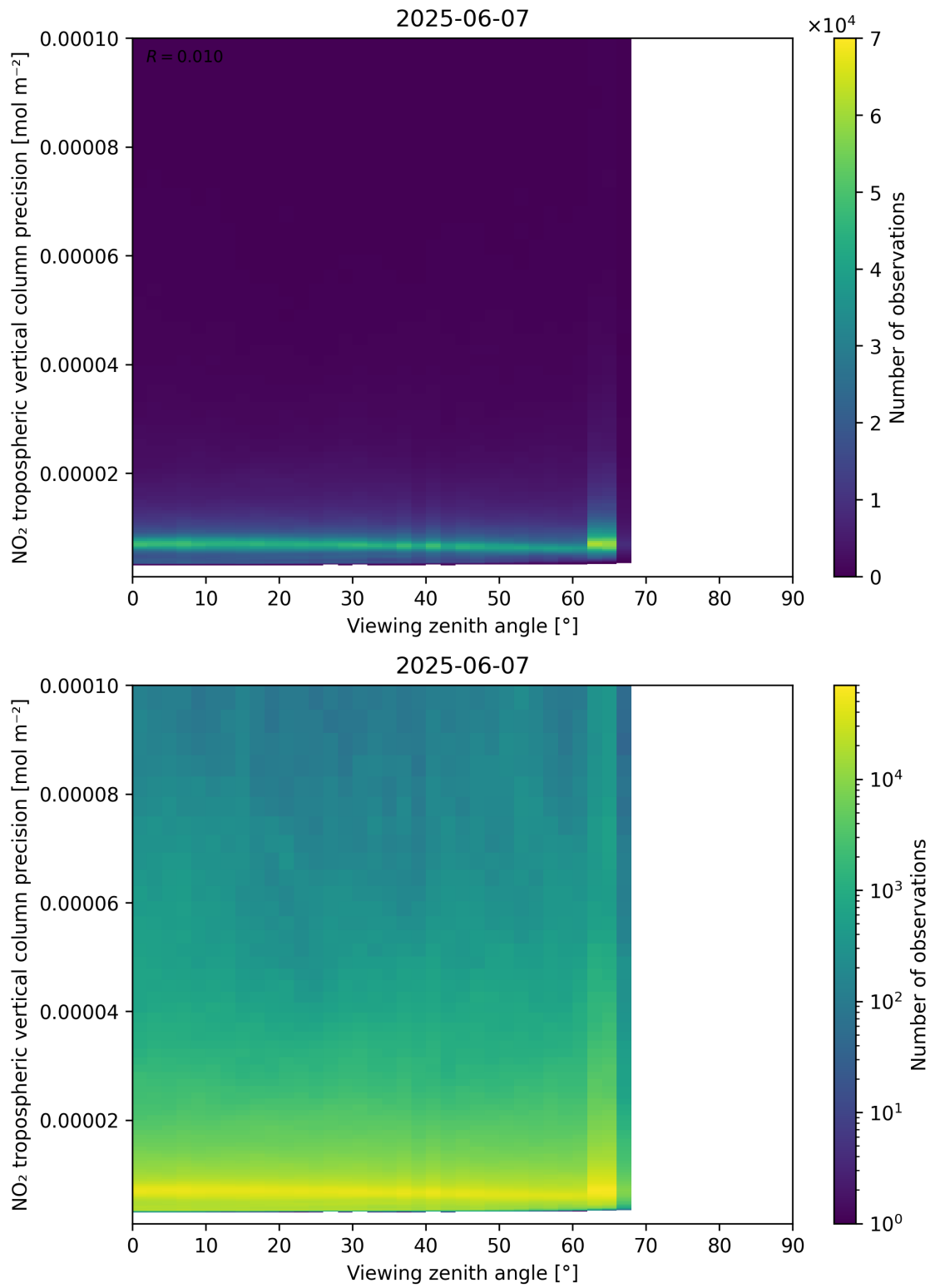
Figure 170: Scatter density plot of “Viewing zenith angle” against “NO 2 tropospheric vertical column precision” for 2025-06-06 to 2025-06-08.
