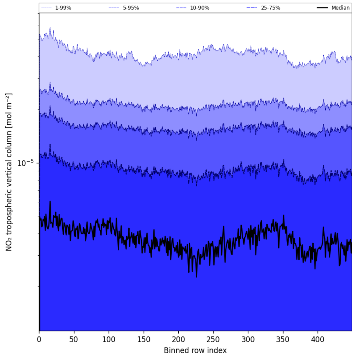
Figure 46: Along track statistics of “NO 2 tropospheric vertical column” for 2025-06-06 to 2025-06-08
