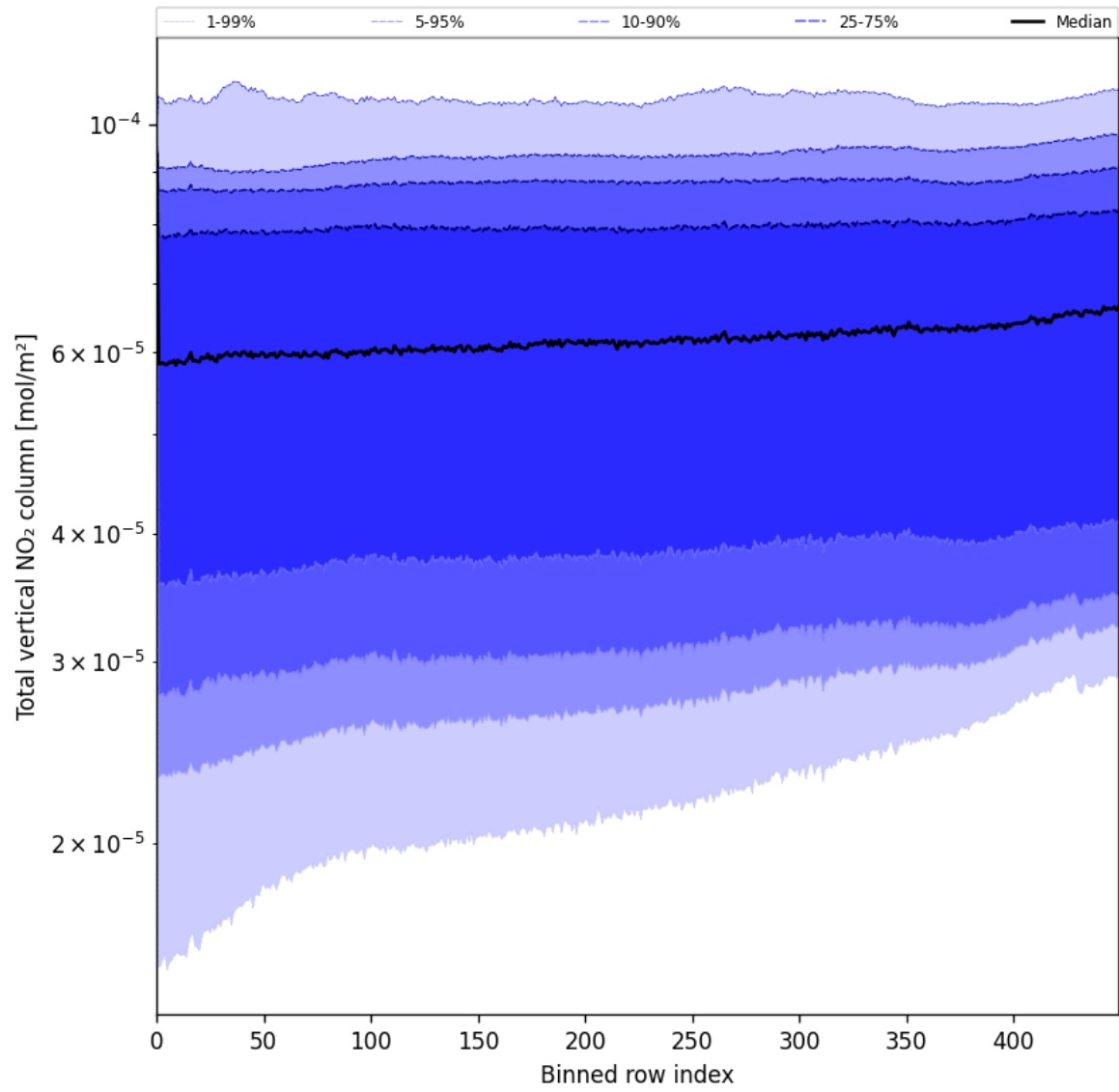
Figure 55: Along track statistics of “Total vertical NO 2 column” for 2025-06-06 to 2025-06-08
