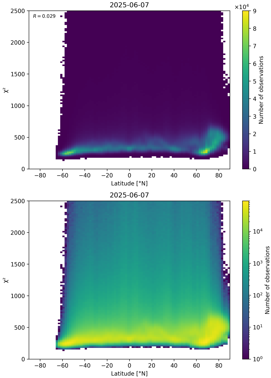
Figure 86: Scatter density plot of “Latitude” against “ \chi^2 ” for 2025-06-06 to 2025-06-08.
