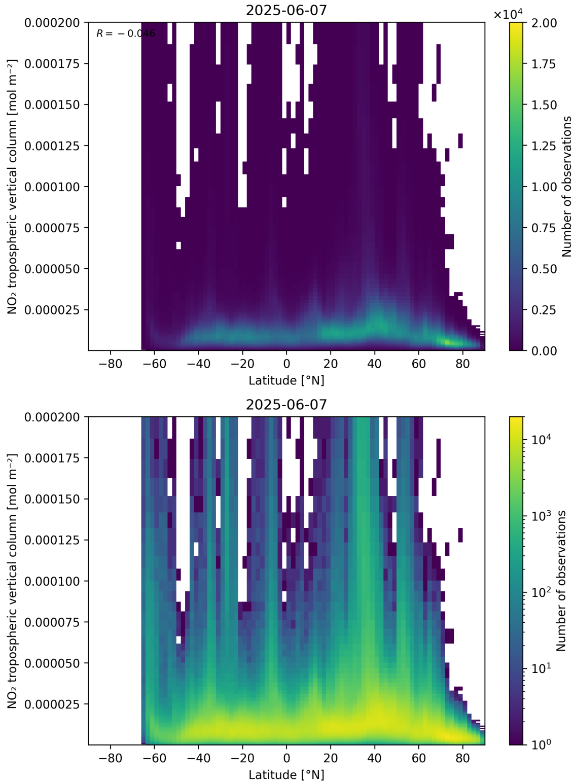
Figure 92: Scatter density plot of “Latitude” against “NO 2 tropospheric vertical column” for 2025-06-06 to 2025-06-08.
