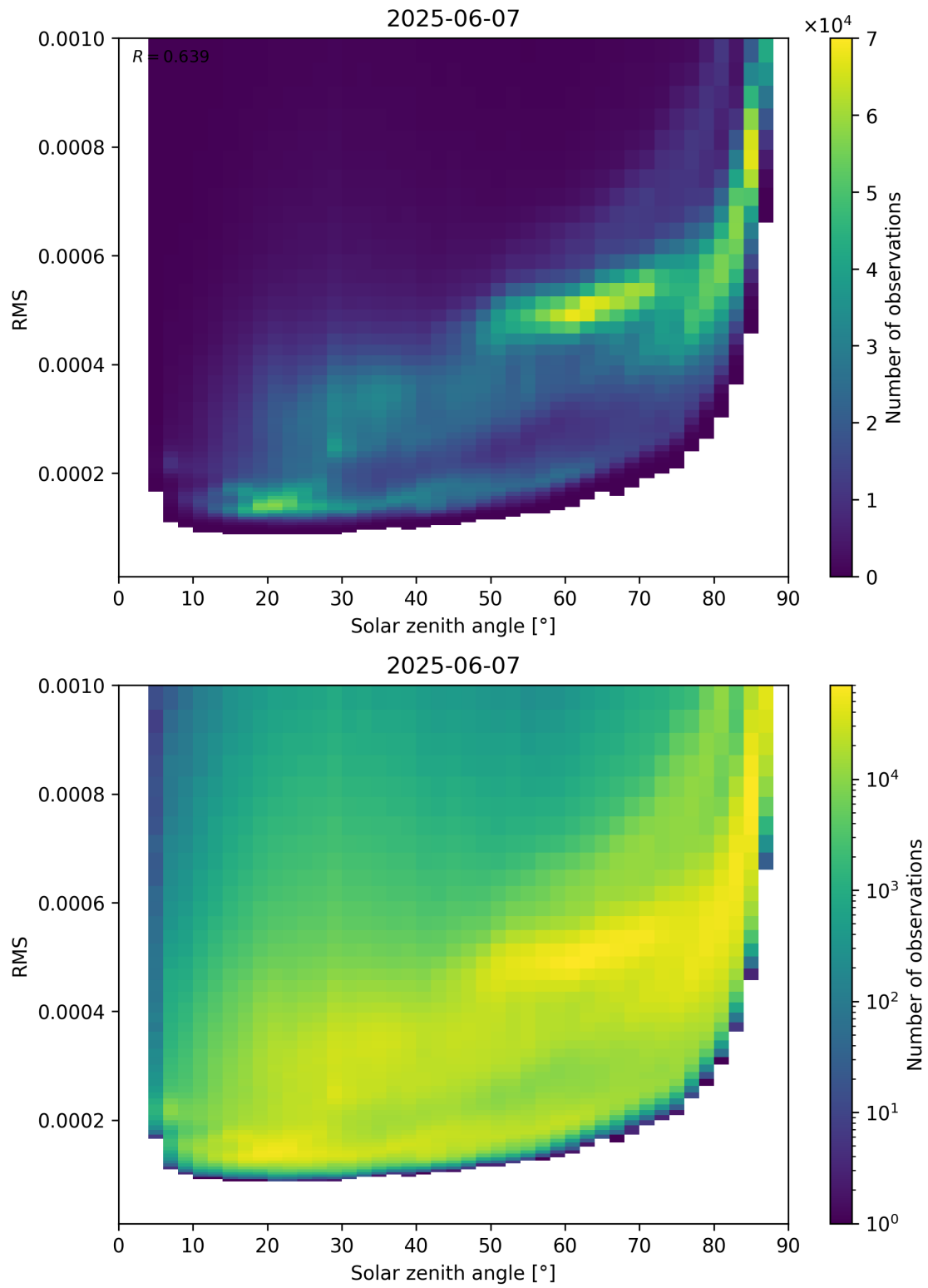
Figure 157: Scatter density plot of “Solar zenith angle” against “RMS” for 2025-06-06 to 2025-06-08.
