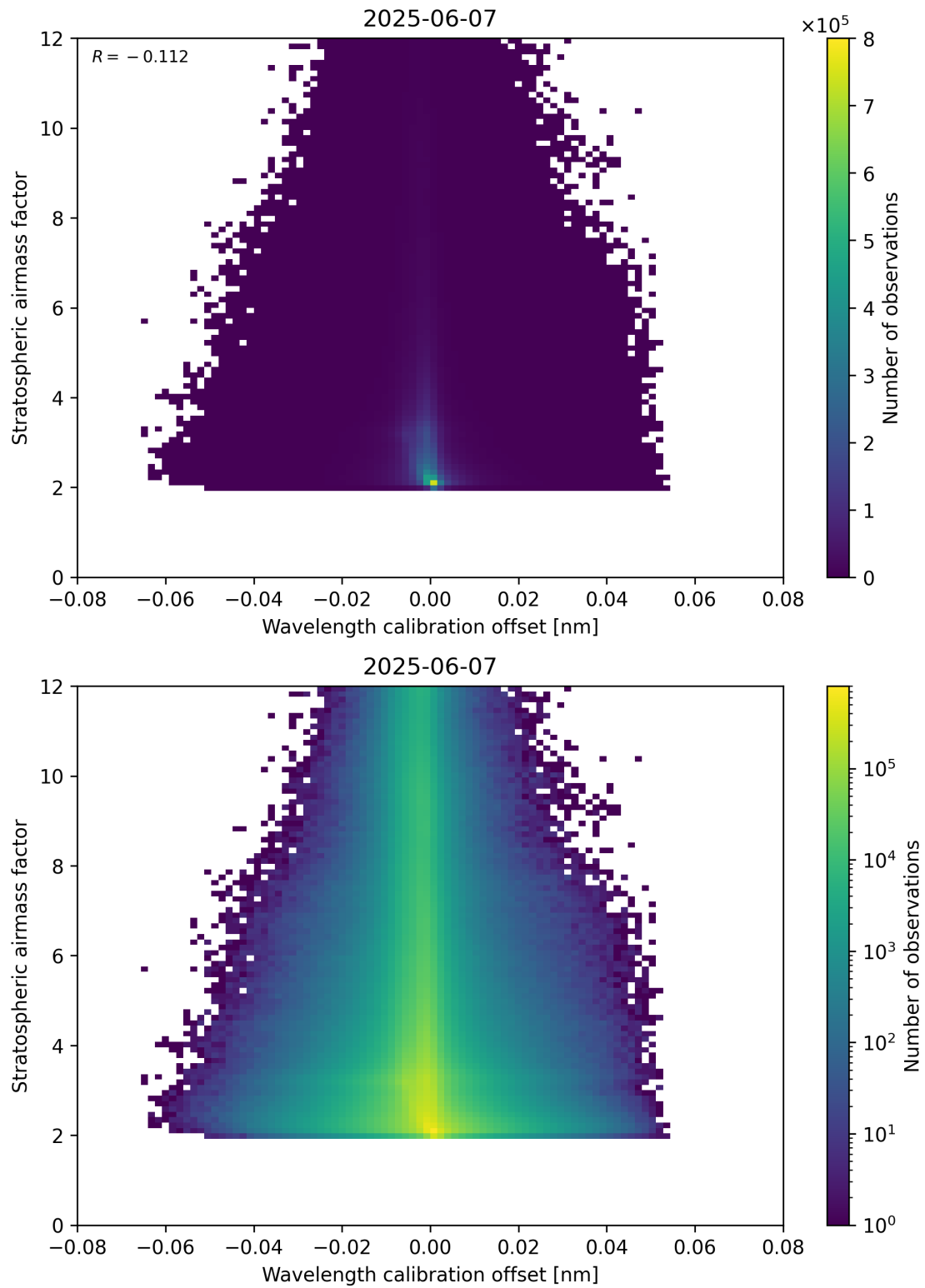
Figure 174: Scatter density plot of “Wavelength calibration offset” against “Stratospheric air mass factor” for 2025-06-06 to 2025-06-08.
