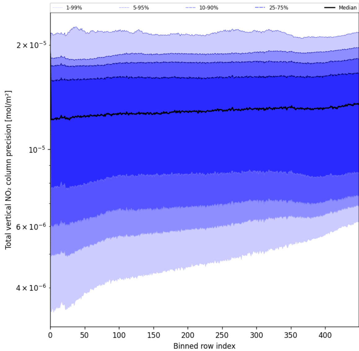
Figure 56: Along track statistics of “Total vertical NO 2 column precision” for 2025-06-06 to 2025-06-08
