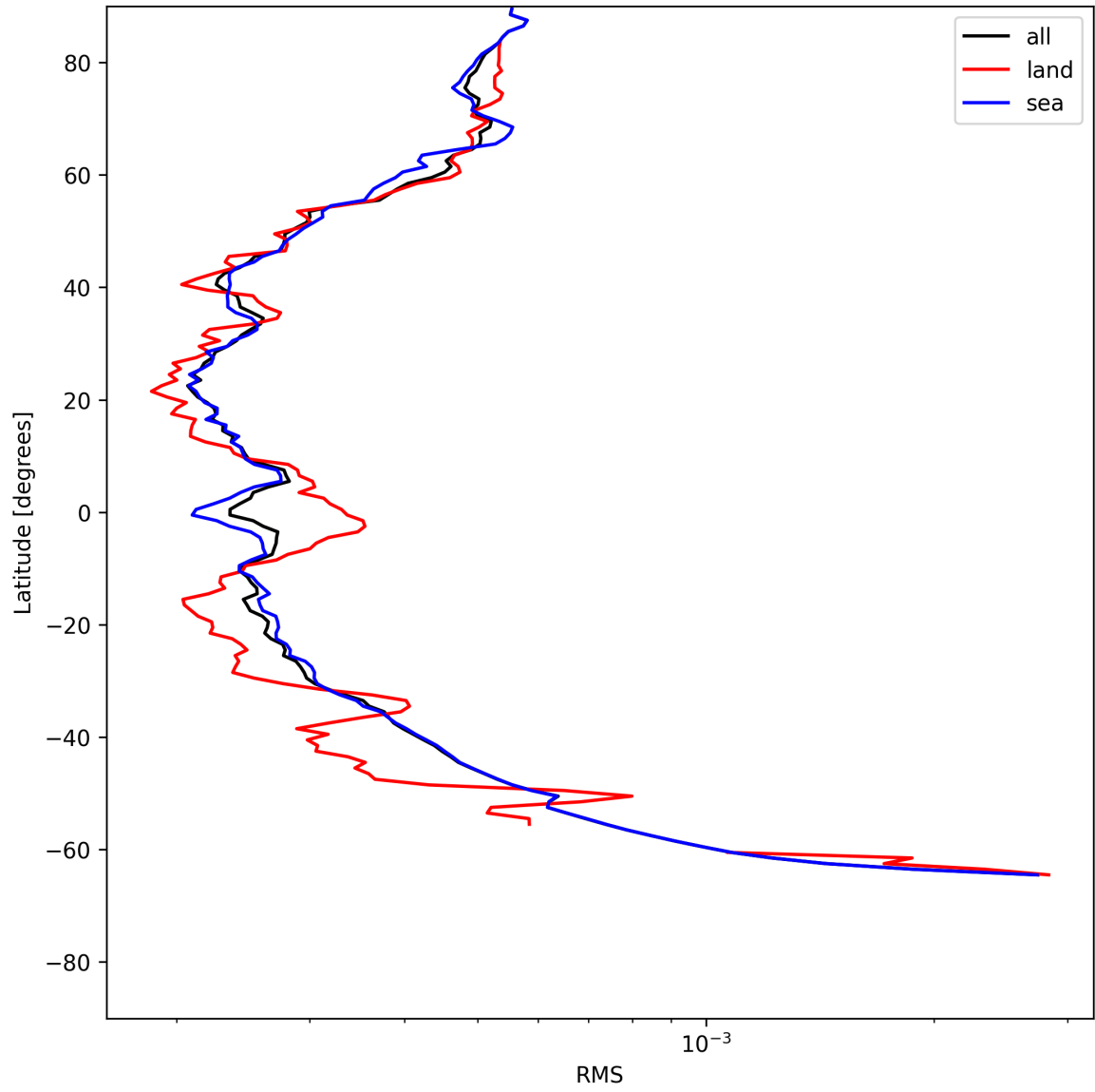
Figure 26: Zonal average of “RMS” for 2025-06-06 to 2025-06-08.
