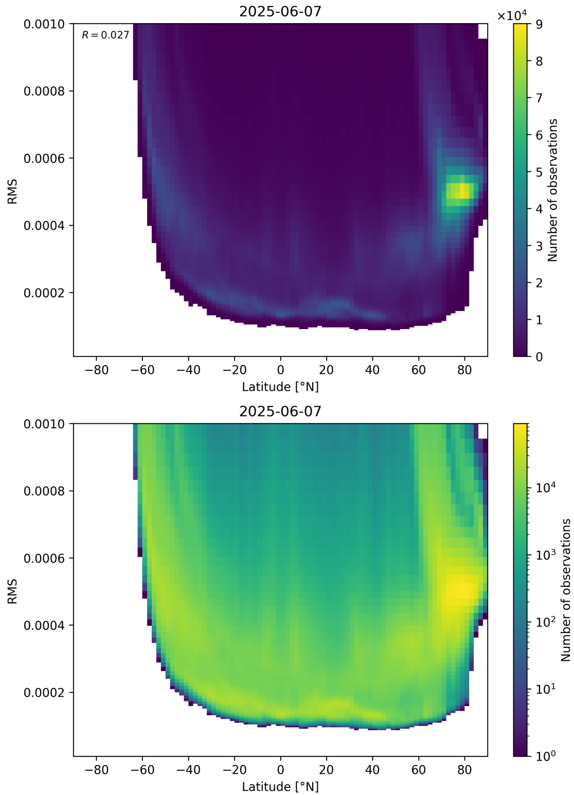
Figure 94: Scatter density plot of “Latitude” against “RMS” for 2025-06-06 to 2025-06-08.
