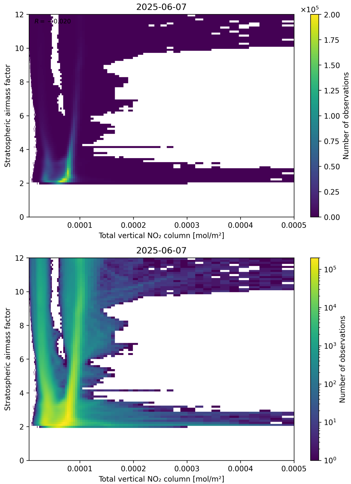
Figure 110: Scatter density plot of “Total vertical NO 2 column” against “Stratospheric airmass factor” for 2025-06-06 to 2025-06-08.
