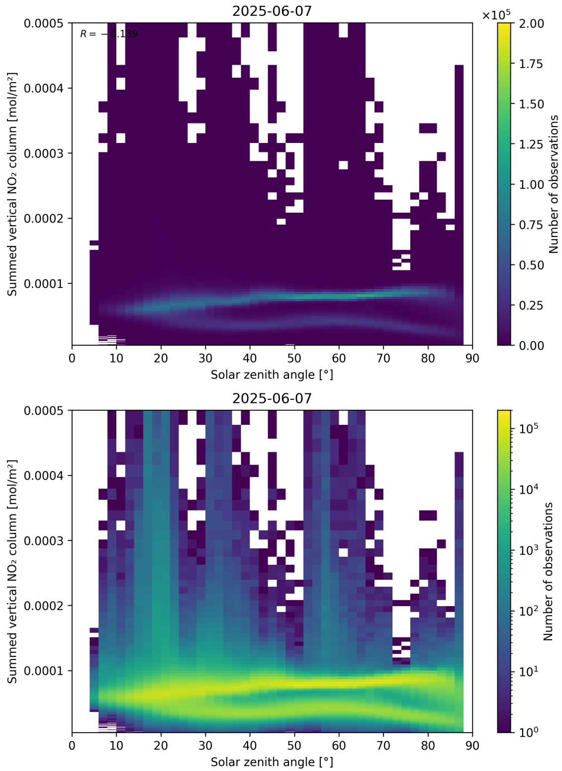
Figure 151: Scatter density plot of “Solar zenith angle” against “Summed vertical NO 2 column” for 2025-06-06 to 2025-06-08.
