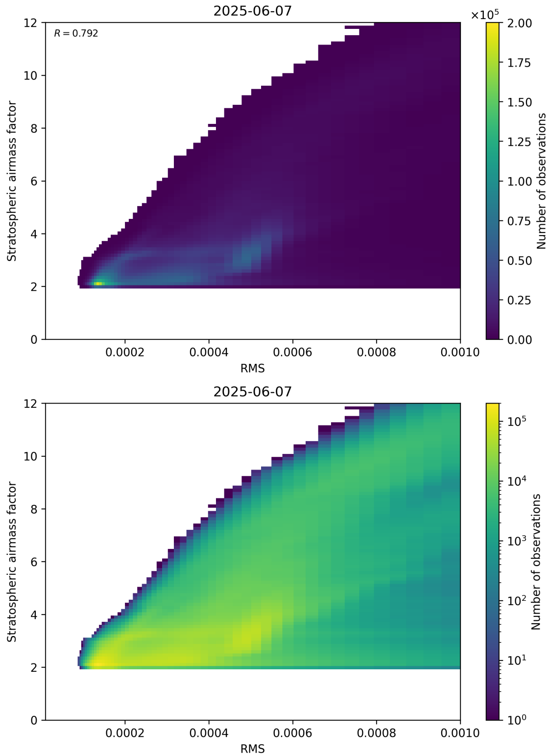
Figure 144: Scatter density plot of “RMS” against “Stratospheric airmass factor” for 2025-06-06 to 2025-06-08.
