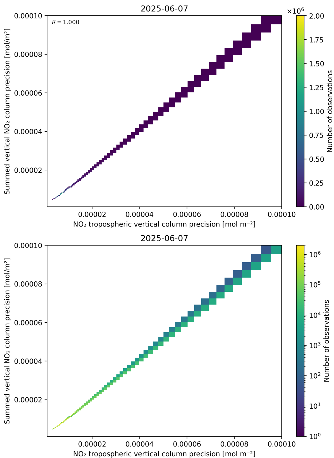
Figure 137: Scatter density plot of “NO 2 tropospheric vertical column precision” against “Summed vertical NO 2 column precision” for 2025-06-06 to 2025-06-08.
