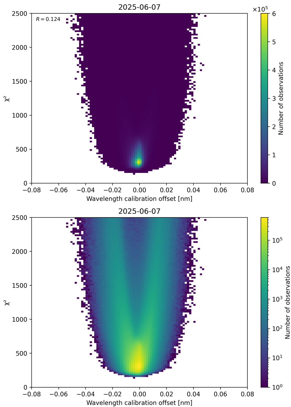
Figure 175: Scatter density plot of “Wavelength calibration offset” against “ \chi^2 ” for 2025-06-06 to 2025-06-08.
