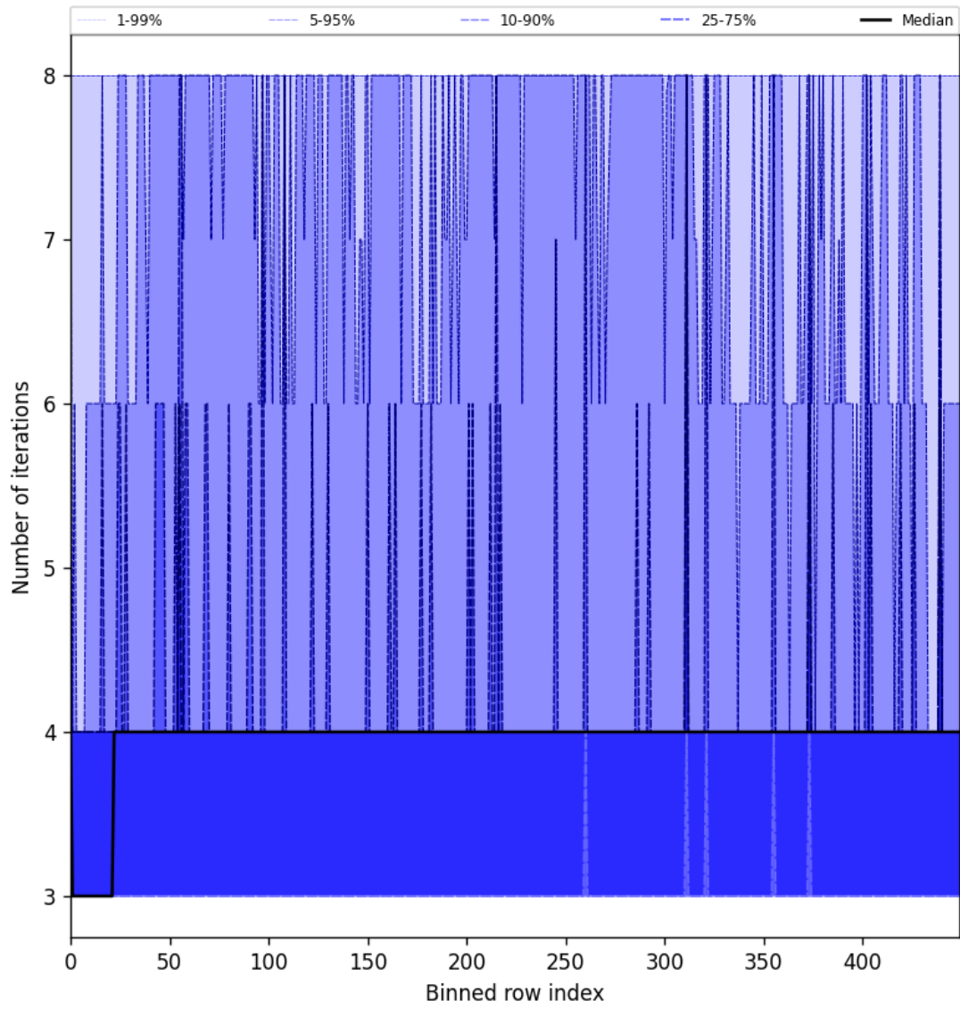
Figure 51: Along track statistics of “Number of iterations” for 2025-06-06 to 2025-06-08
