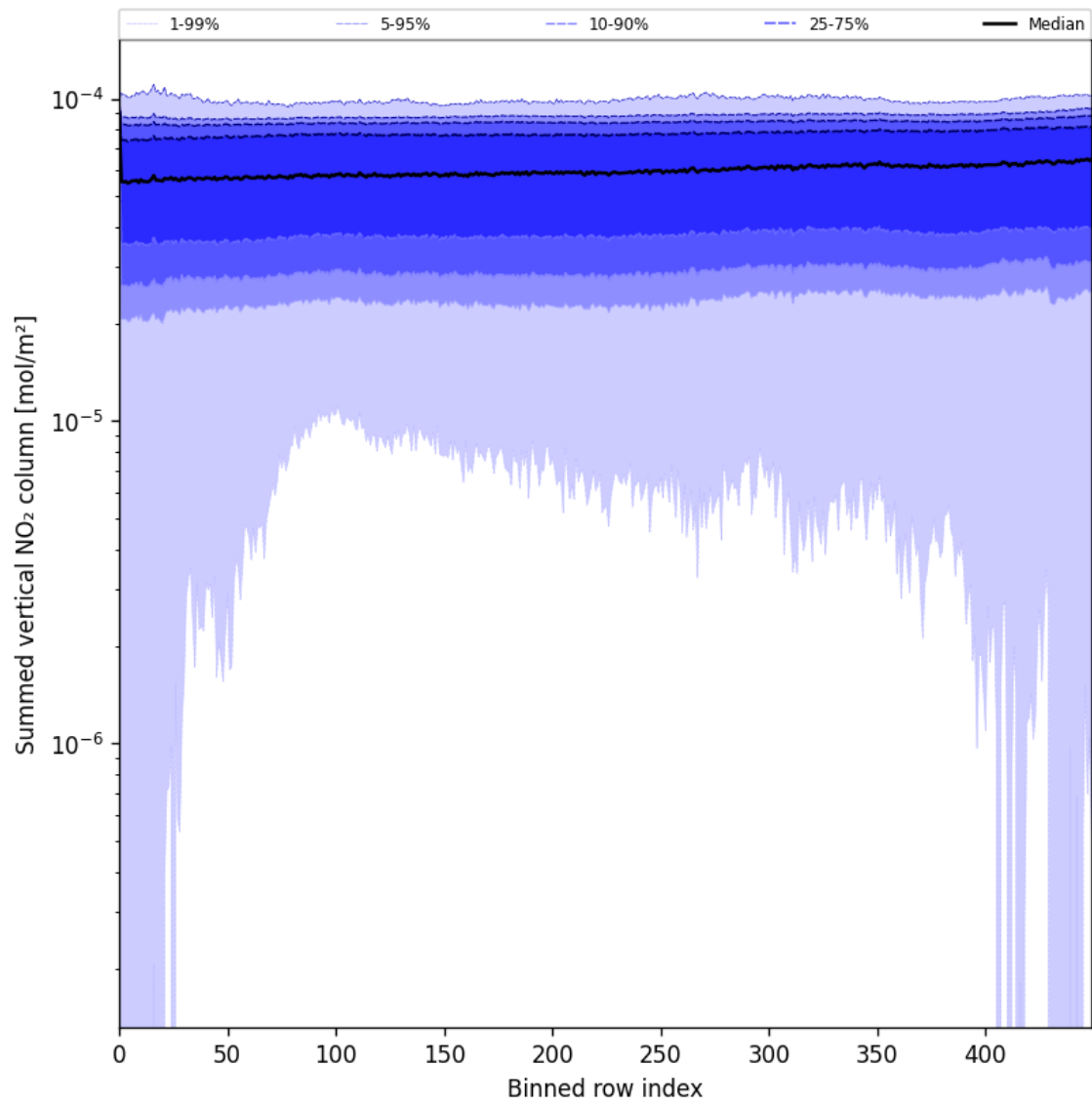
Figure 57: Along track statistics of “Summed vertical NO 2 column” for 2025-06-06 to 2025-06-08
