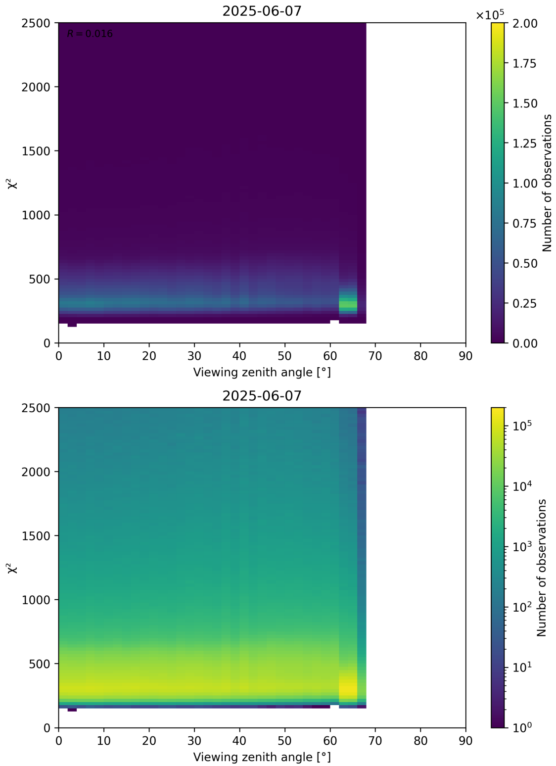
Figure 162: Scatter density plot of “Viewing zenith angle” against “ \chi^2 ” for 2025-06-06 to 2025-06-08.
