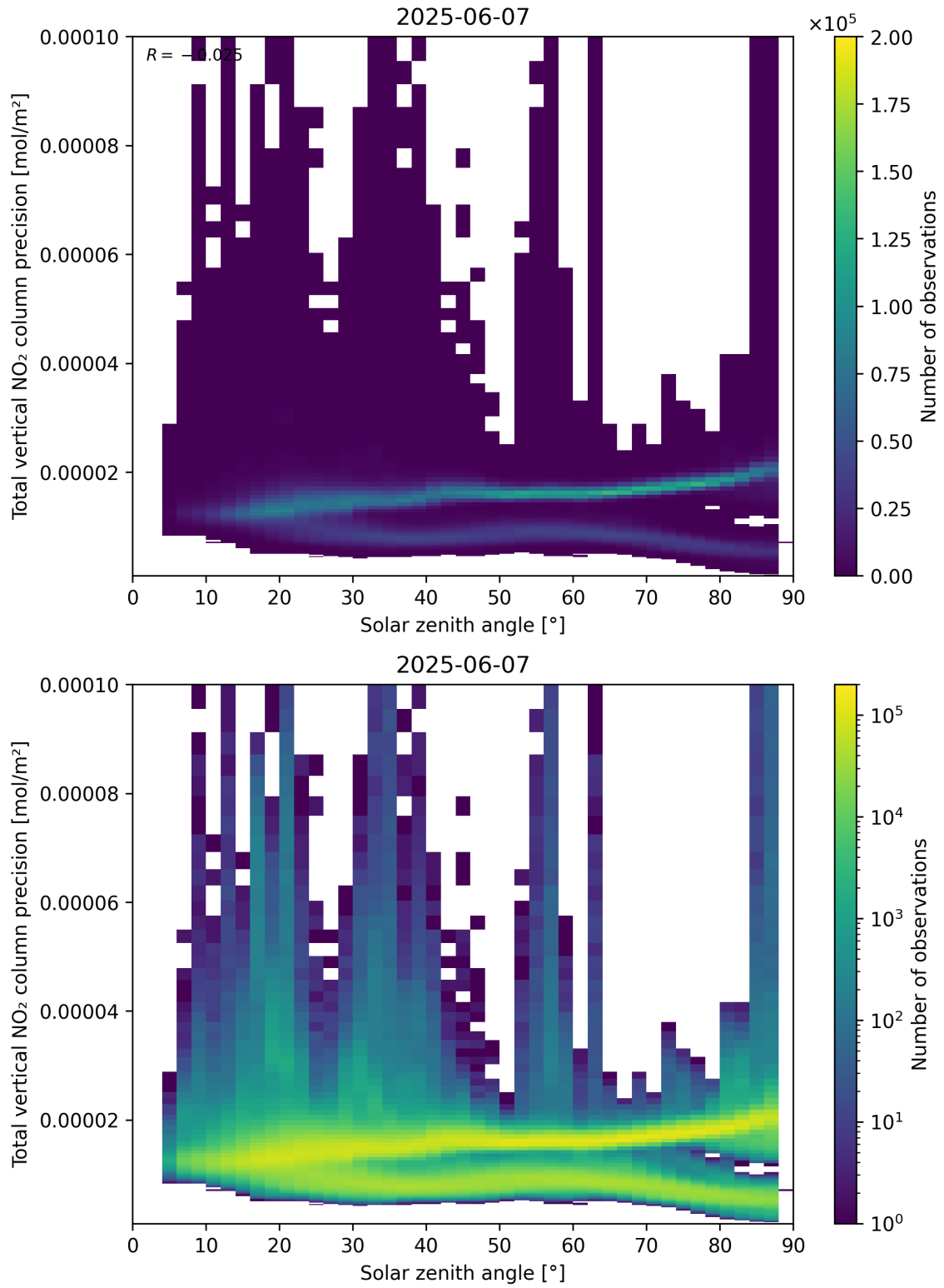
Figure 154: Scatter density plot of “Solar zenith angle” against “Total vertical NO 2 column precision” for 2025-06-06 to 2025-06-08.
