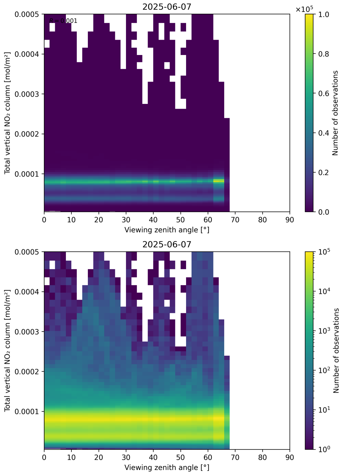
Figure 167: Scatter density plot of “Viewing zenith angle” against “Total vertical NO 2 column” for 2025-06-06 to 2025-06-08.
