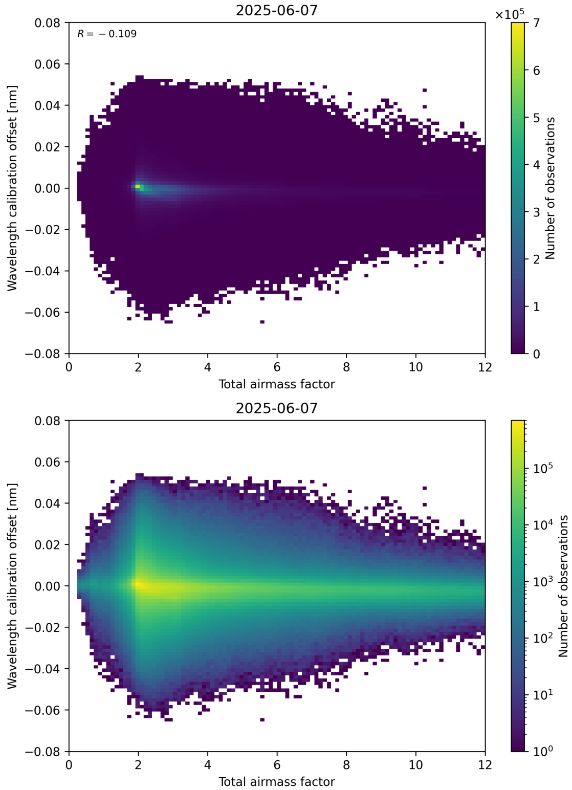
Figure 70: Scatter density plot of “Total airmass factor” against “Wavelength calibration offset” for 2025-06-06 to 2025-06-08.
