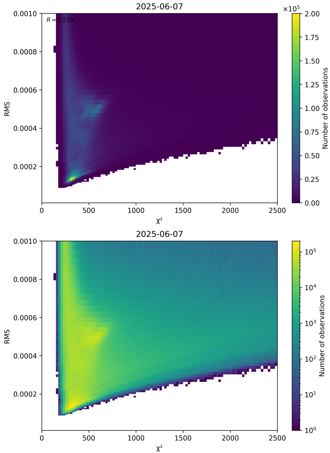
Figure 82: Scatter density plot of “ \chi^2 ” against “RMS” for 2025-06-06 to 2025-06-08.
