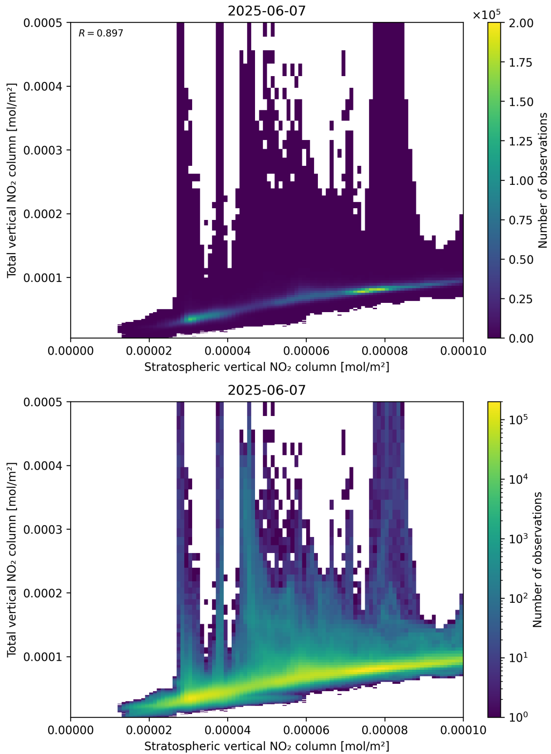
Figure 100: Scatter density plot of “Stratospheric vertical NO 2 column” against “Total vertical NO 2 column” for 2025-06-06 to 2025-06-08.
