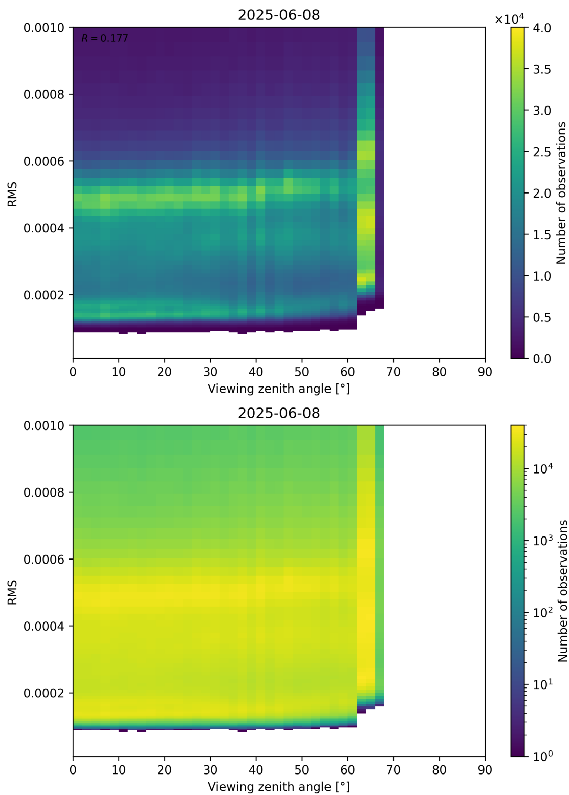
Figure 171: Scatter density plot of “Viewing zenith angle” against “RMS” for 2025-06-07 to 2025-06-09.
