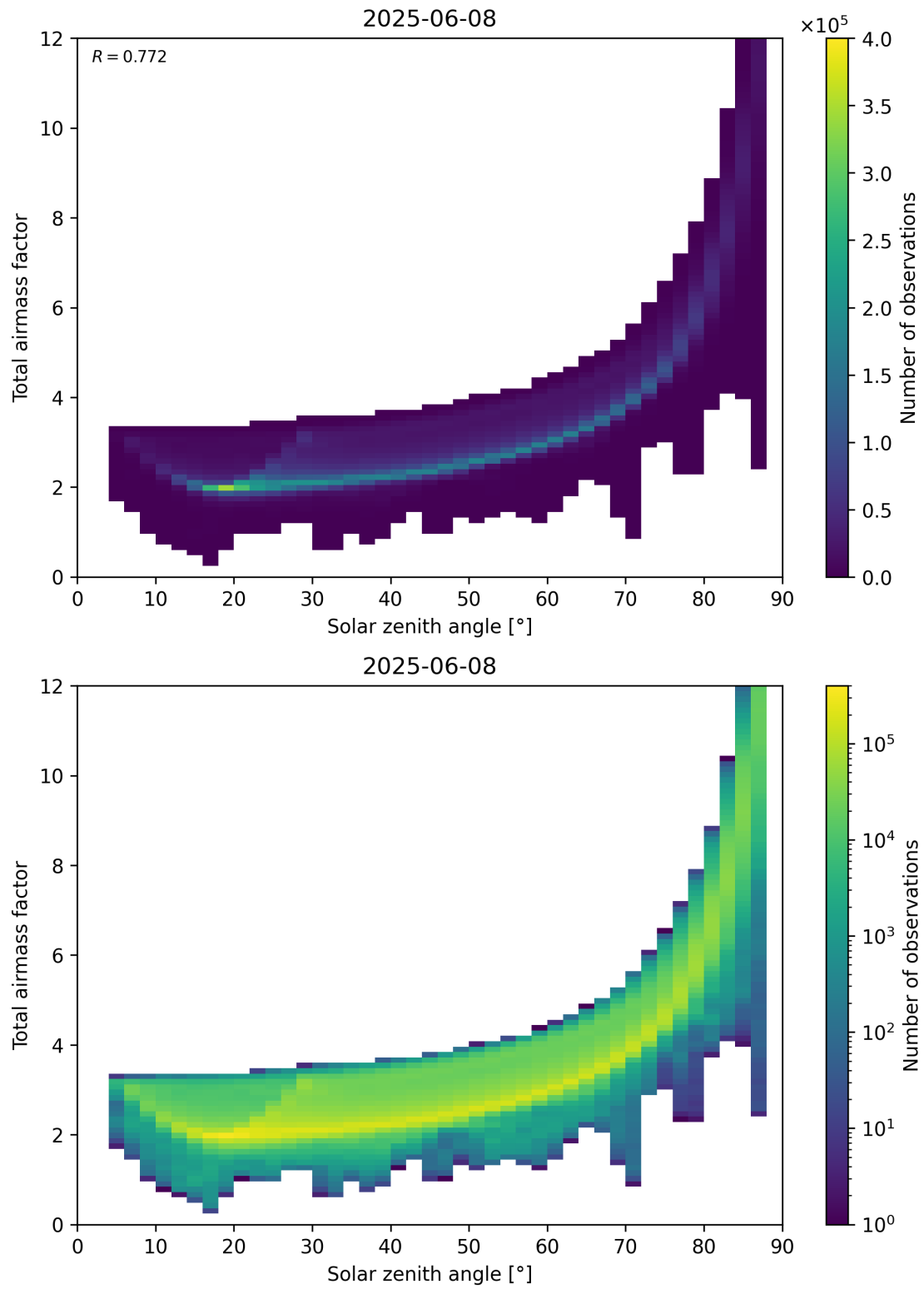
Figure 146: Scatter density plot of “Solar zenith angle” against “Total air mass factor” for 2025-06-07 to 2025-06-09.
