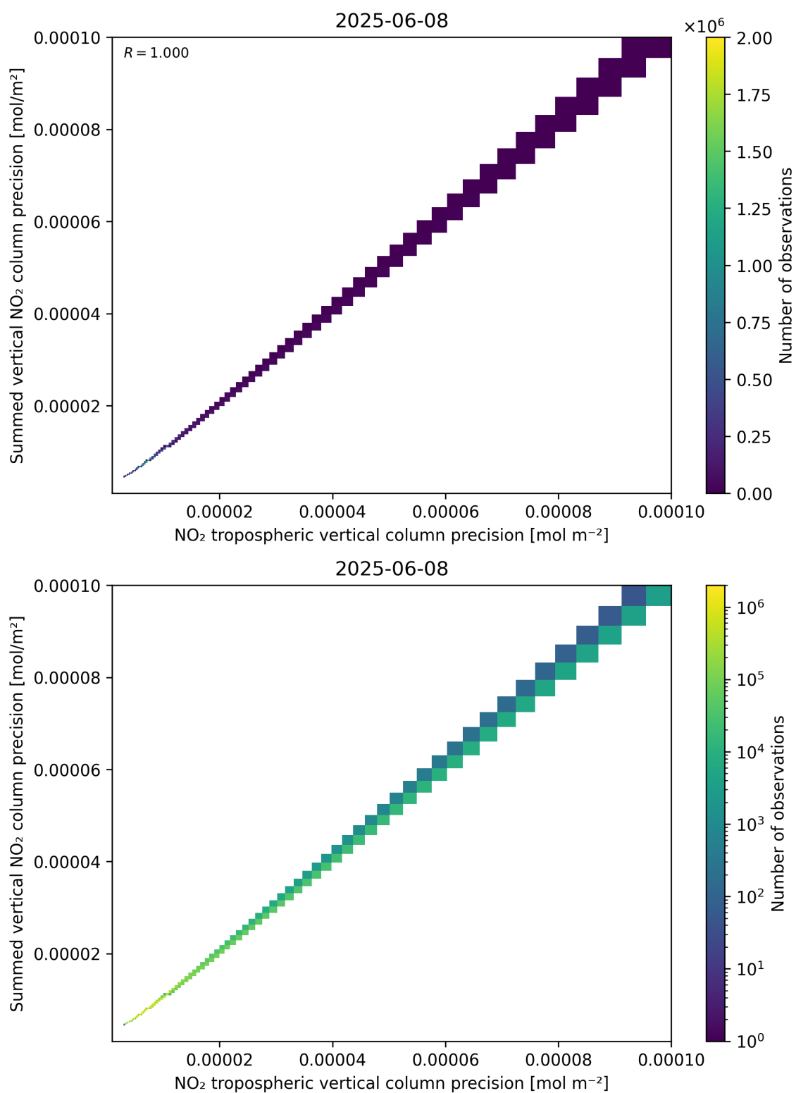
Figure 137: Scatter density plot of “NO 2 tropospheric vertical column precision” against “Summed vertical NO 2 column precision” for 2025-06-07 to 2025-06-09.
