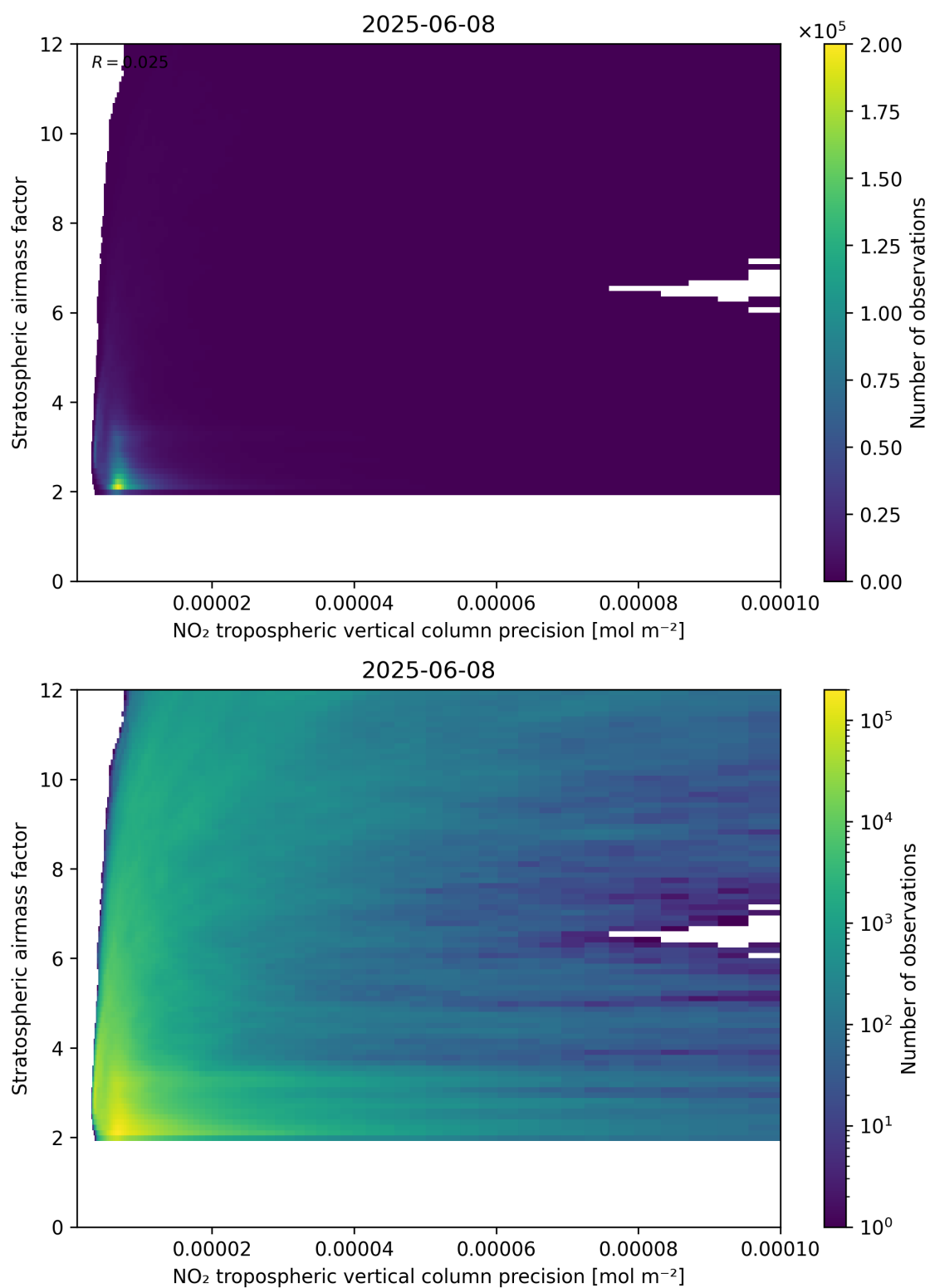
Figure 131: Scatter density plot of “NO 2 tropospheric vertical column precision” against “Stratospheric airmass factor” for 2025-06-07 to 2025-06-09.
