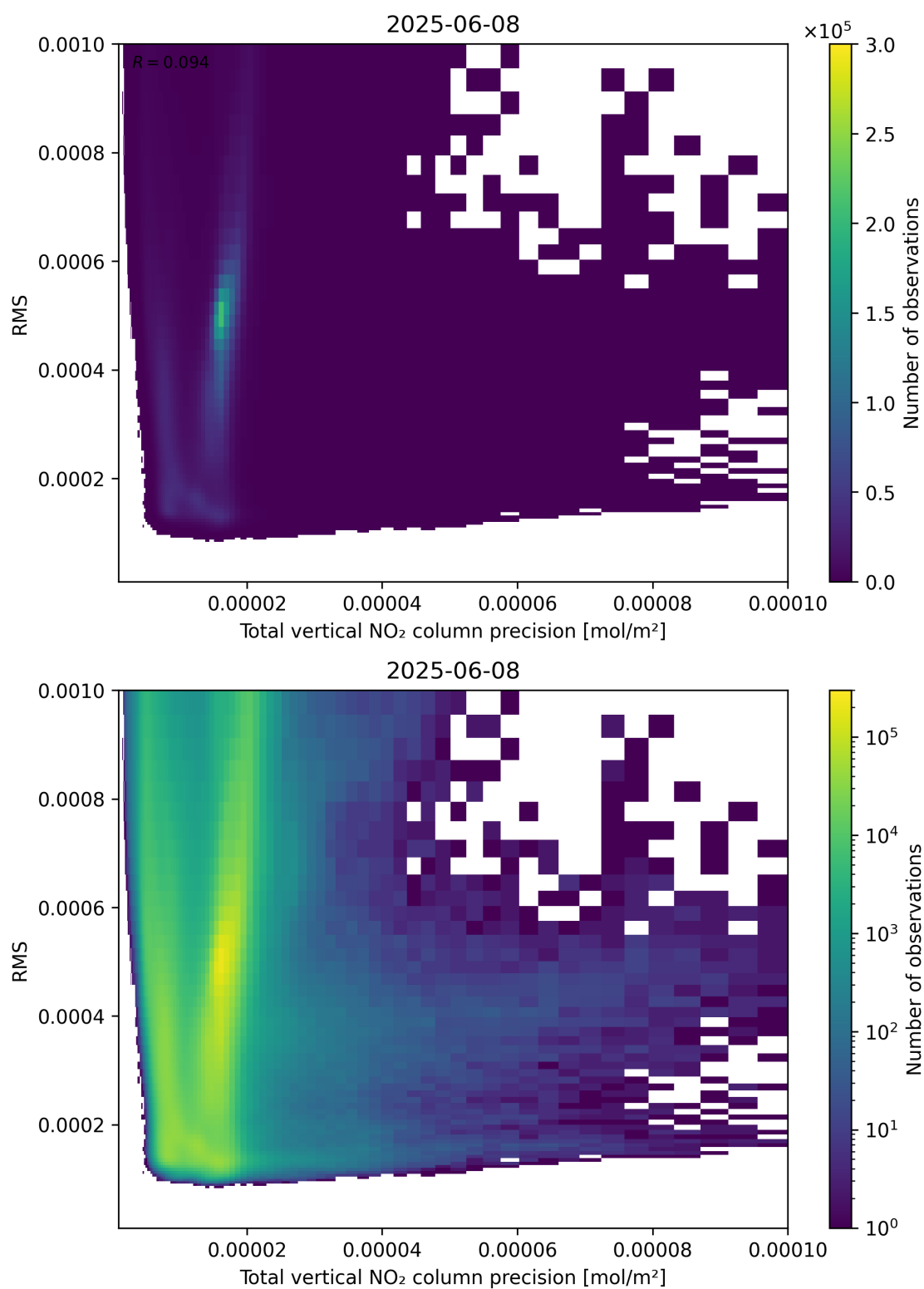
Figure 119: Scatter density plot of “Total vertical NO 2 column precision” against “RMS” for 2025-06-07 to 2025-06-09.
