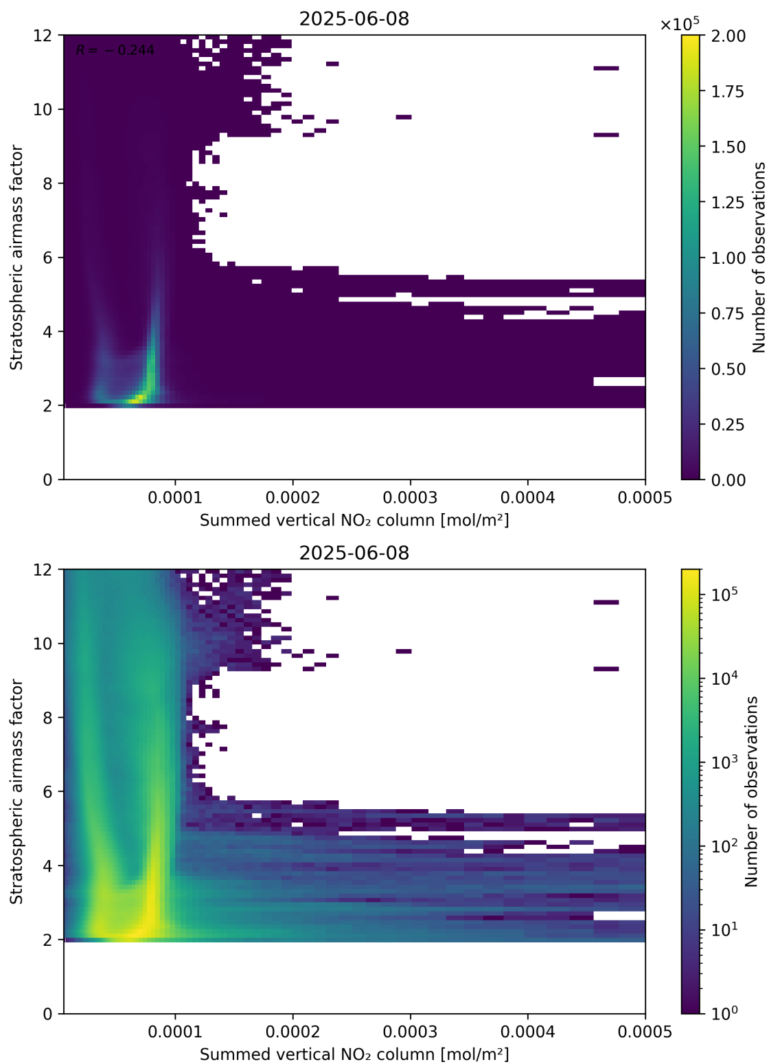
Figure 103: Scatter density plot of “Summed vertical NO 2 column” against “Stratospheric air mass factor” for 2025-06-07 to 2025-06-09.
