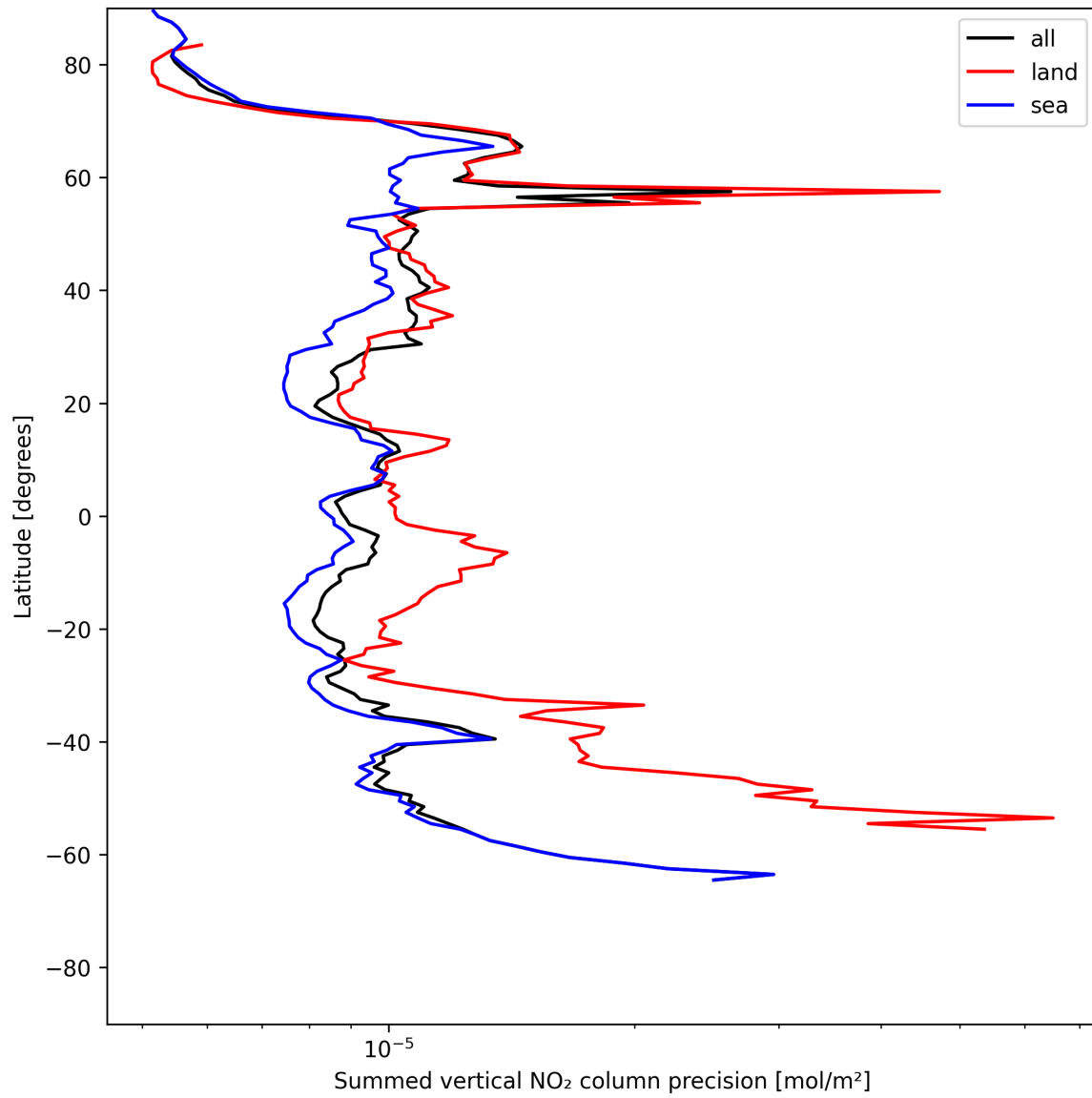
Figure 24: Zonal average of “Summed vertical NO 2 column precision” for 2025-06-07 to 2025-06-09.
