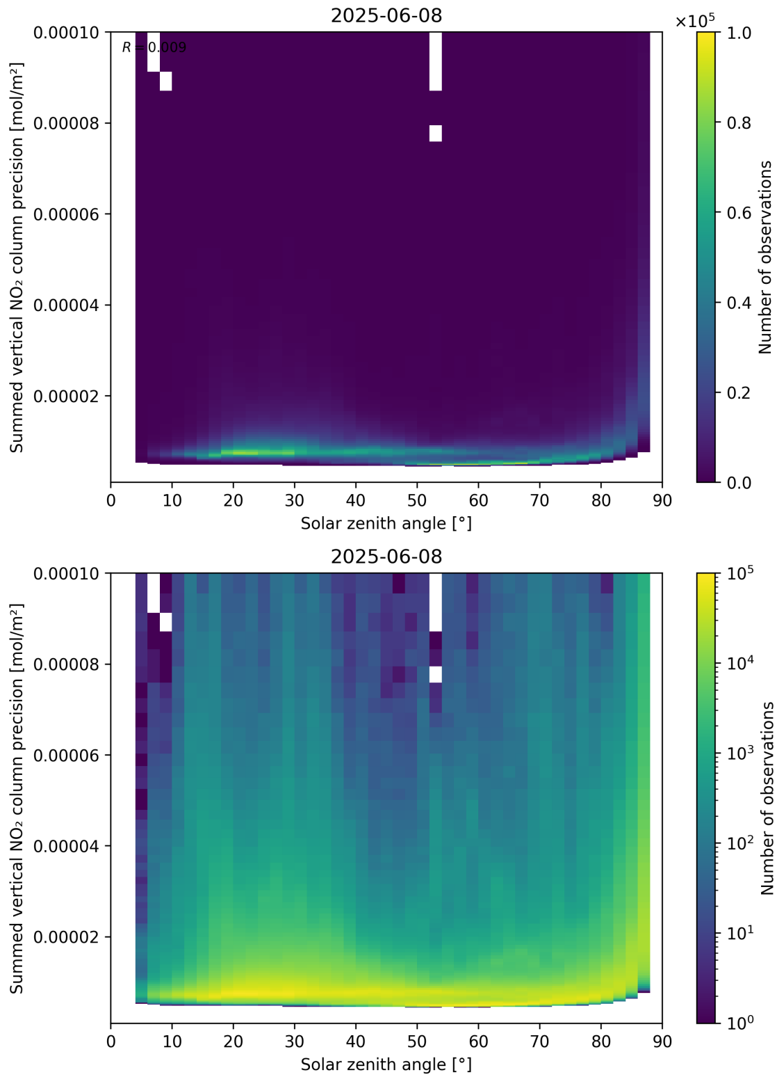
Figure 152: Scatter density plot of “Solar zenith angle” against “Summed vertical NO 2 column precision” for 2025-06-07 to 2025-06-09.
