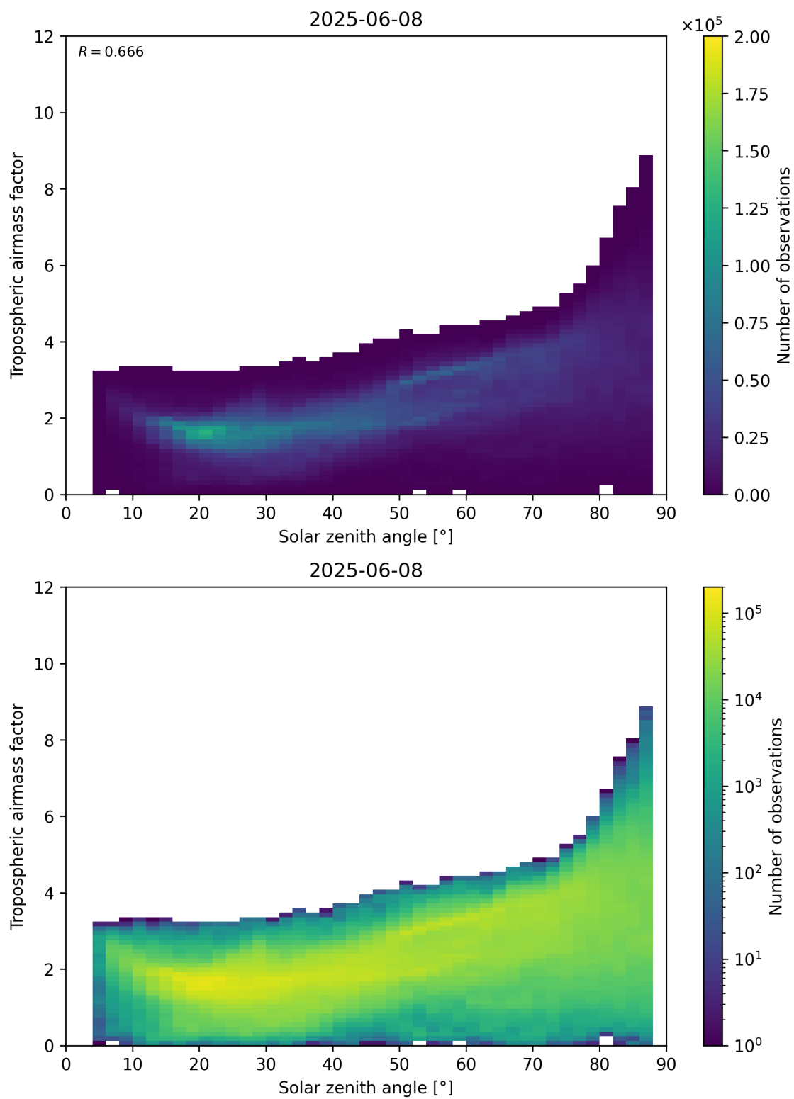
Figure 147: Scatter density plot of “Solar zenith angle” against “Tropospheric airmass factor” for 2025-06-07 to 2025-06-09.
