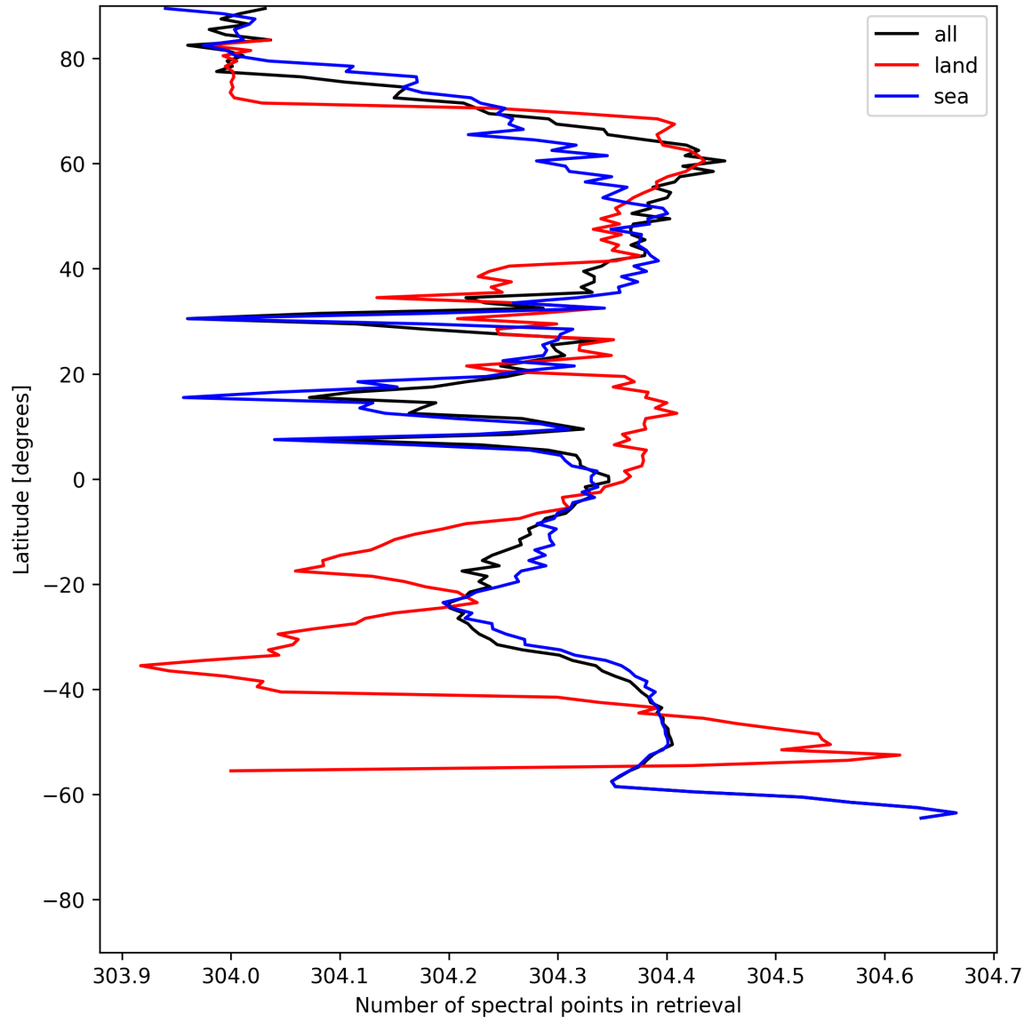
Figure 16: Zonal average of “Number of spectral points in retrieval” for 2025-06-07 to 2025-06-09.
