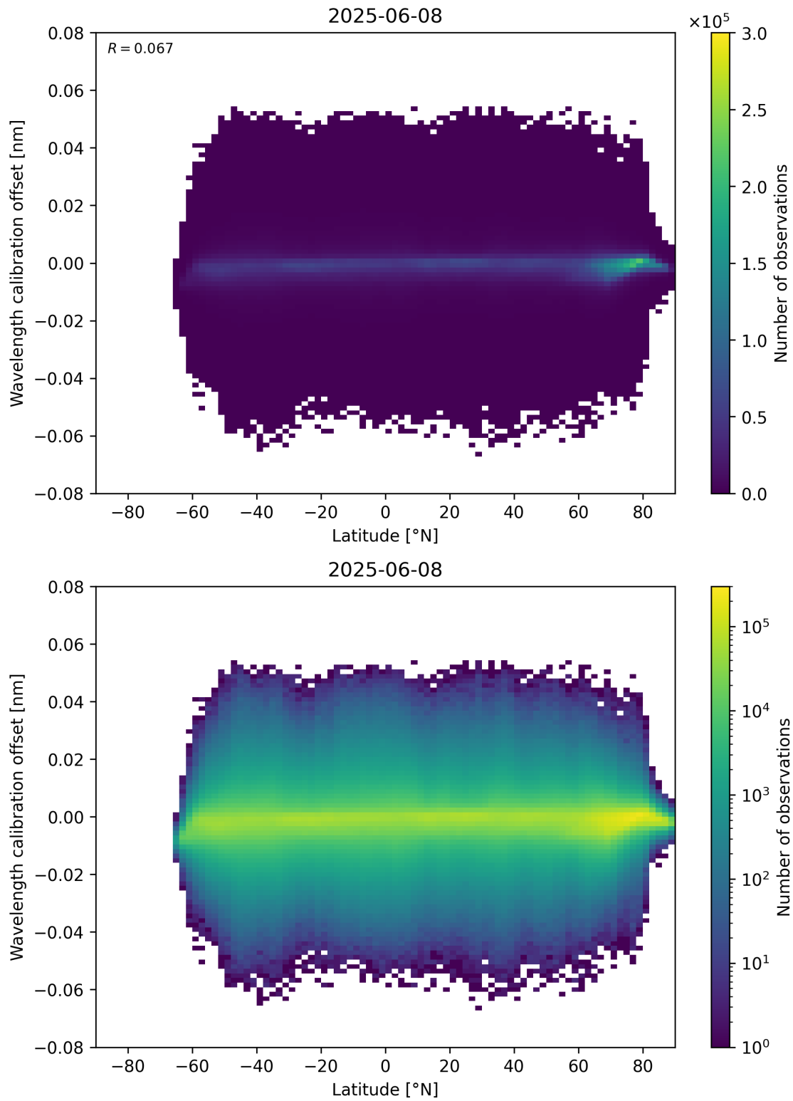
Figure 95: Scatter density plot of “Latitude” against “Wavelength calibration offset” for 2025-06-07 to 2025-06-09.
