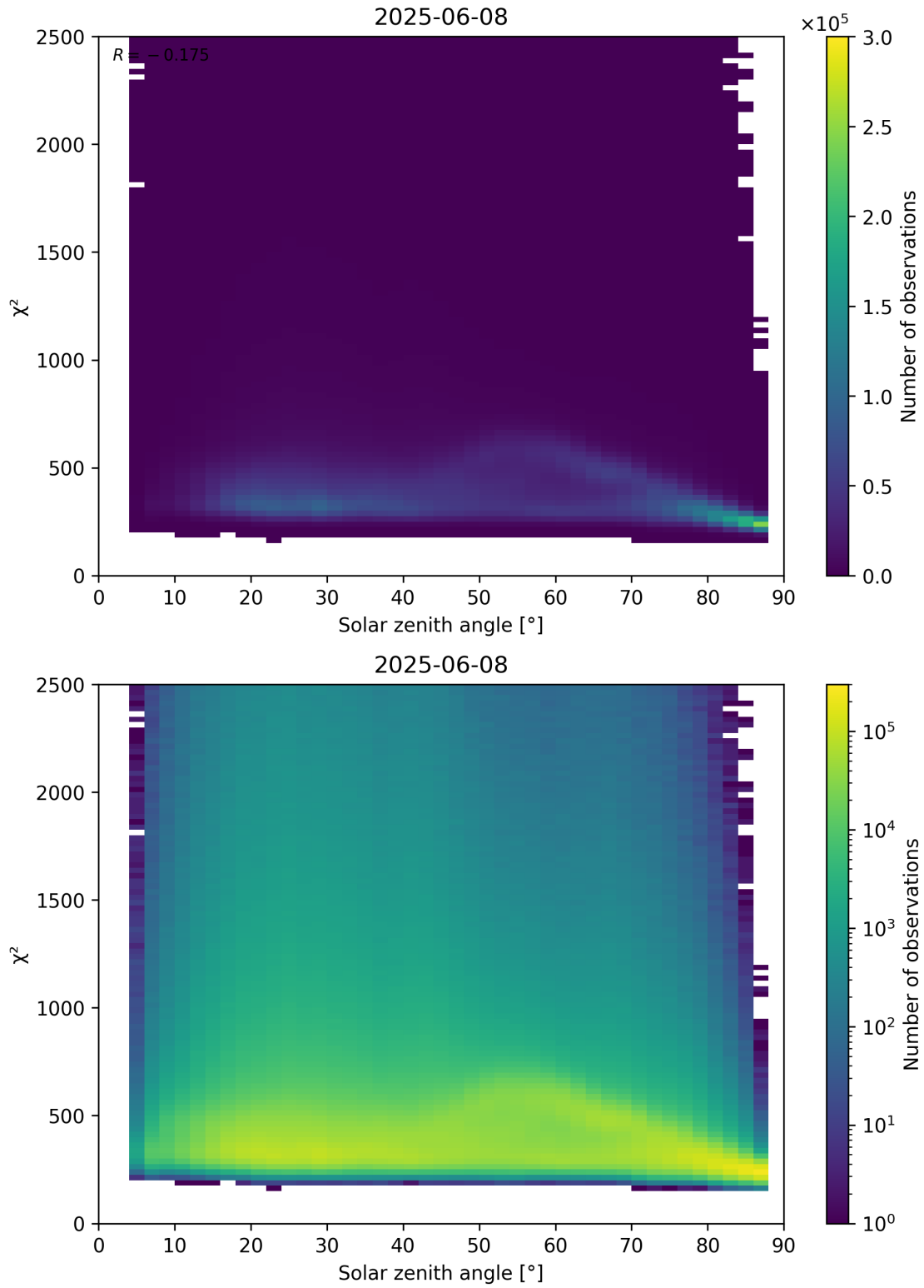
Figure 148: Scatter density plot of “Solar zenith angle” against “ \chi^2 ” for 2025-06-07 to 2025-06-09.
