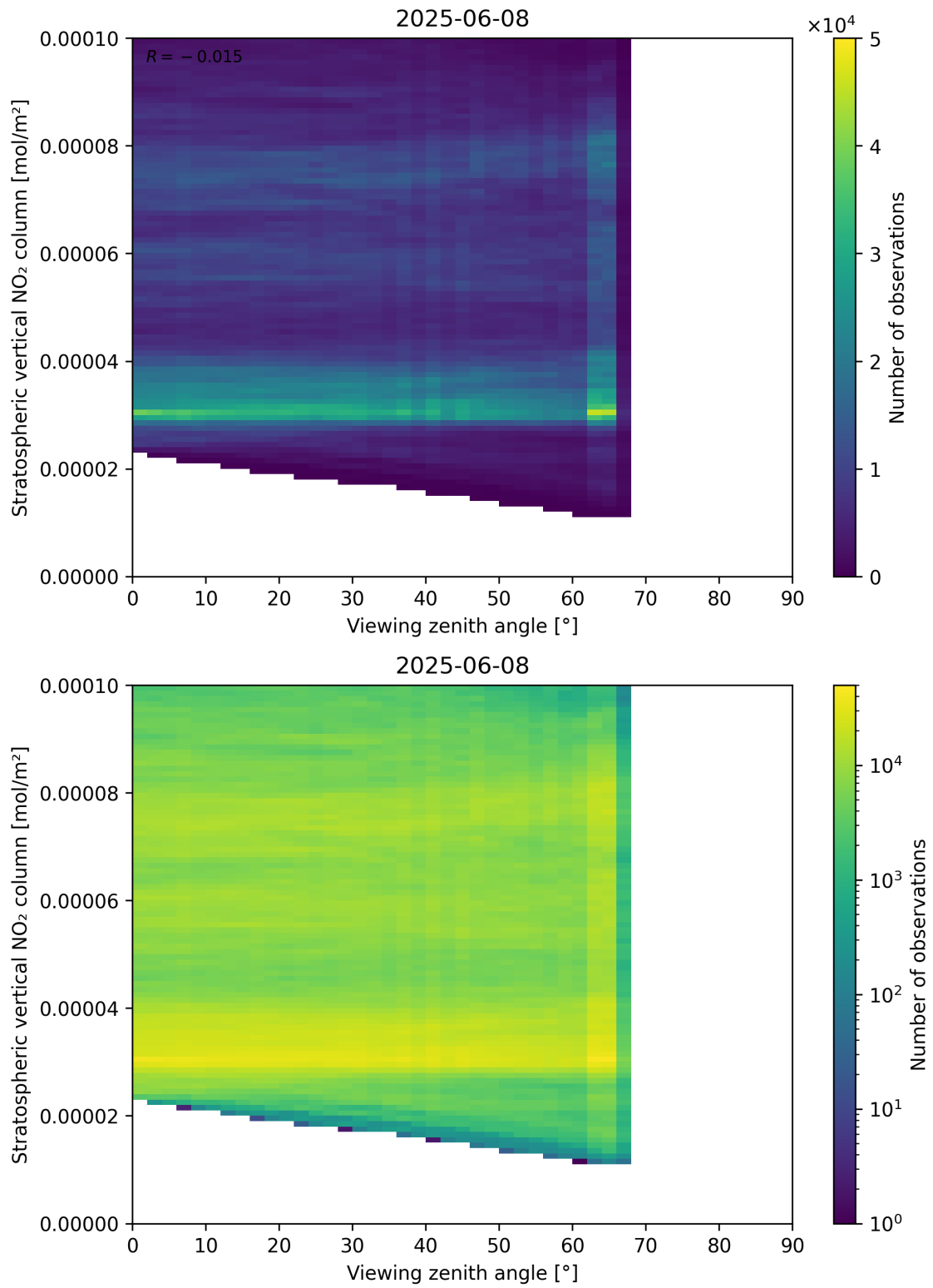
Figure 164: Scatter density plot of “Viewing zenith angle” against “Stratospheric vertical NO 2 column” for 2025-06-07 to 2025-06-09.
