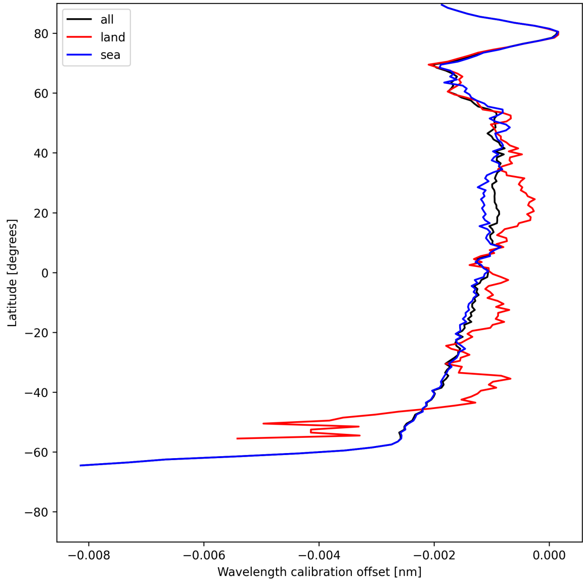
Figure 18: Zonal average of “Wavelength calibration offset” for 2025-06-07 to 2025-06-09.
