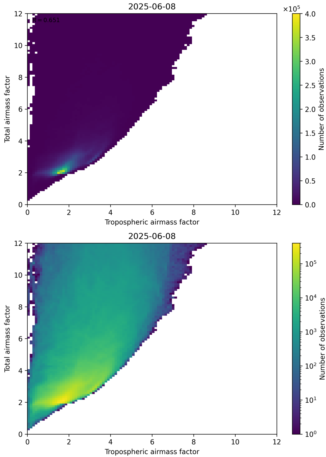
Figure 72: Scatter density plot of “Tropospheric airmass factor” against “Total airmass factor” for 2025-06-07 to 2025-06-09.
