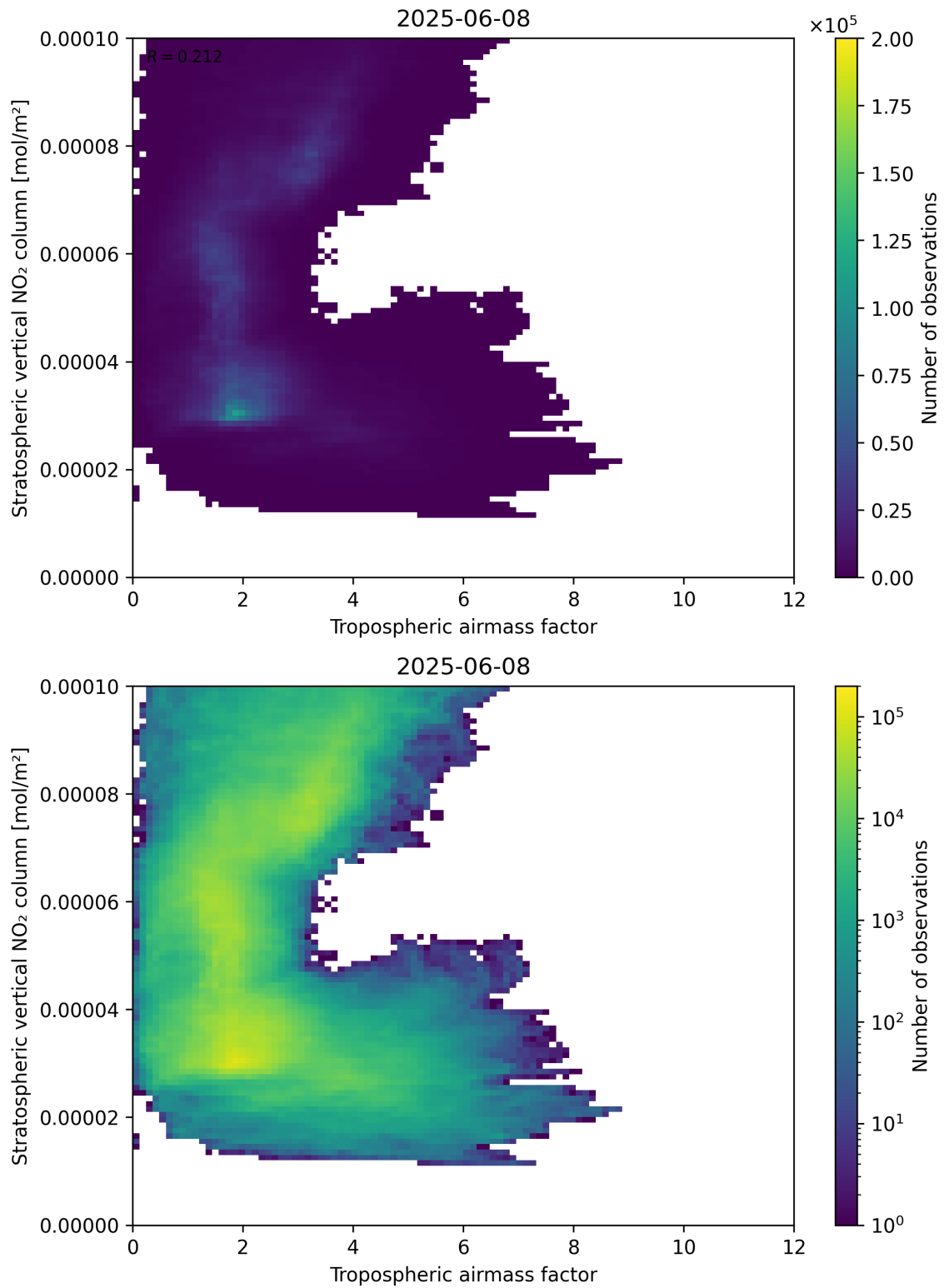
Figure 74: Scatter density plot of “Tropospheric air mass factor” against “Stratospheric vertical NO 2 column” for 2025-06-07 to 2025-06-09.
