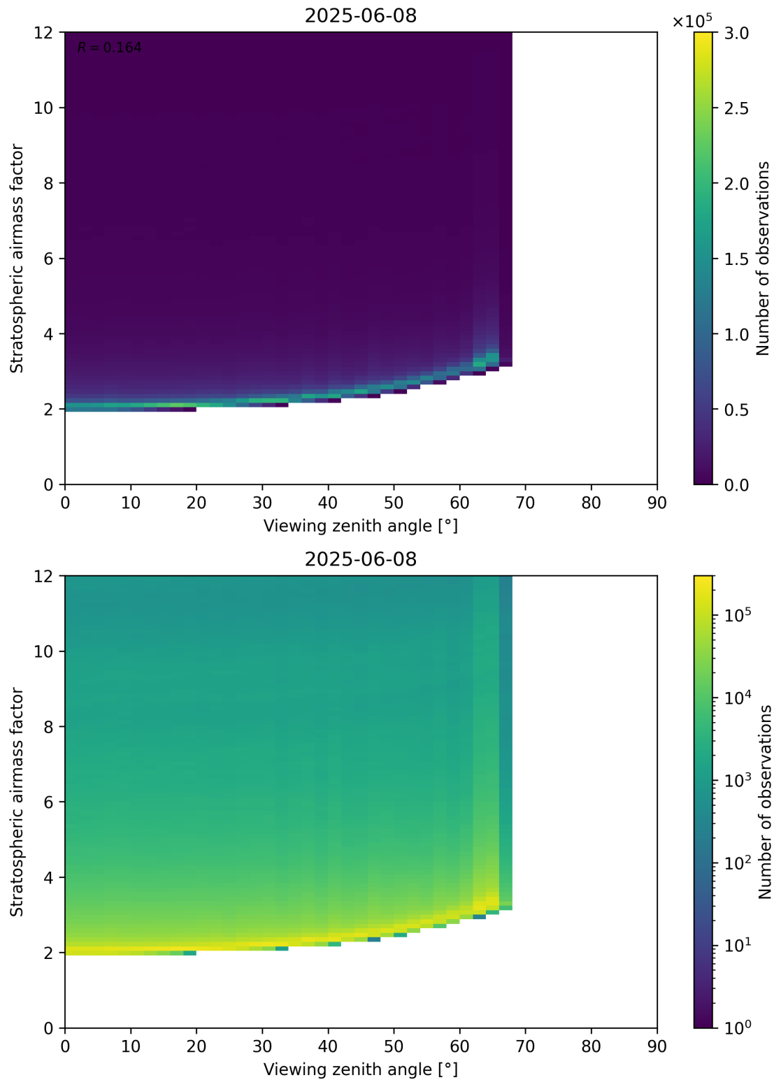
Figure 159: Scatter density plot of “Viewing zenith angle” against “Stratospheric airmass factor” for 2025-06-07 to 2025-06-09.
