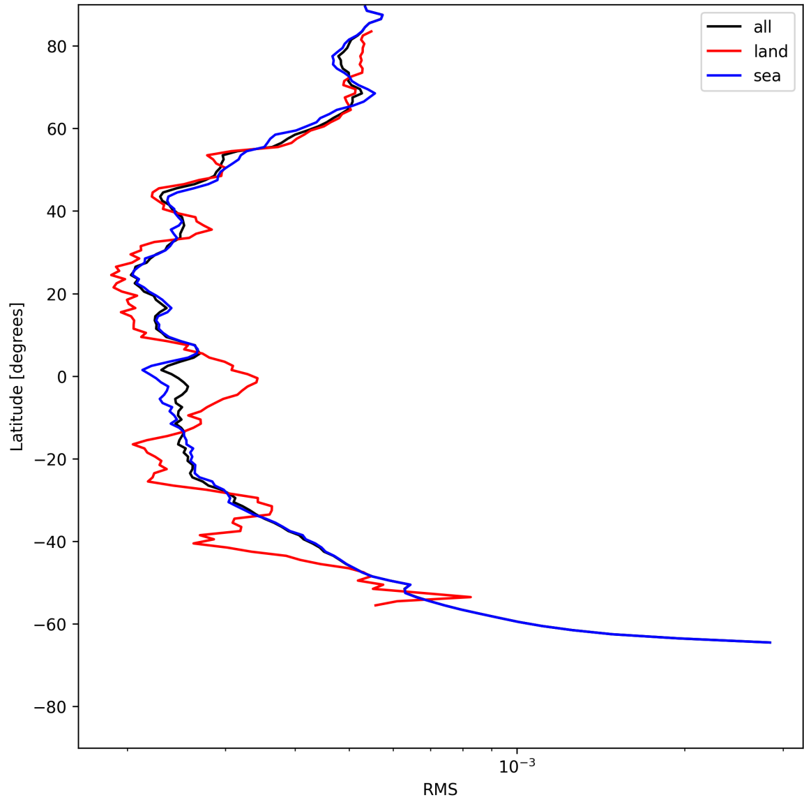
Figure 26: Zonal average of “RMS” for 2025-06-07 to 2025-06-09.
