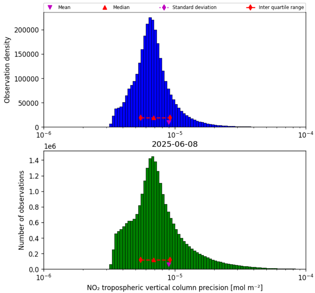
Figure 30: Histogram of "NO 2 tropospheric vertical column precision" for 2025-06-07 to 2025-06-09
