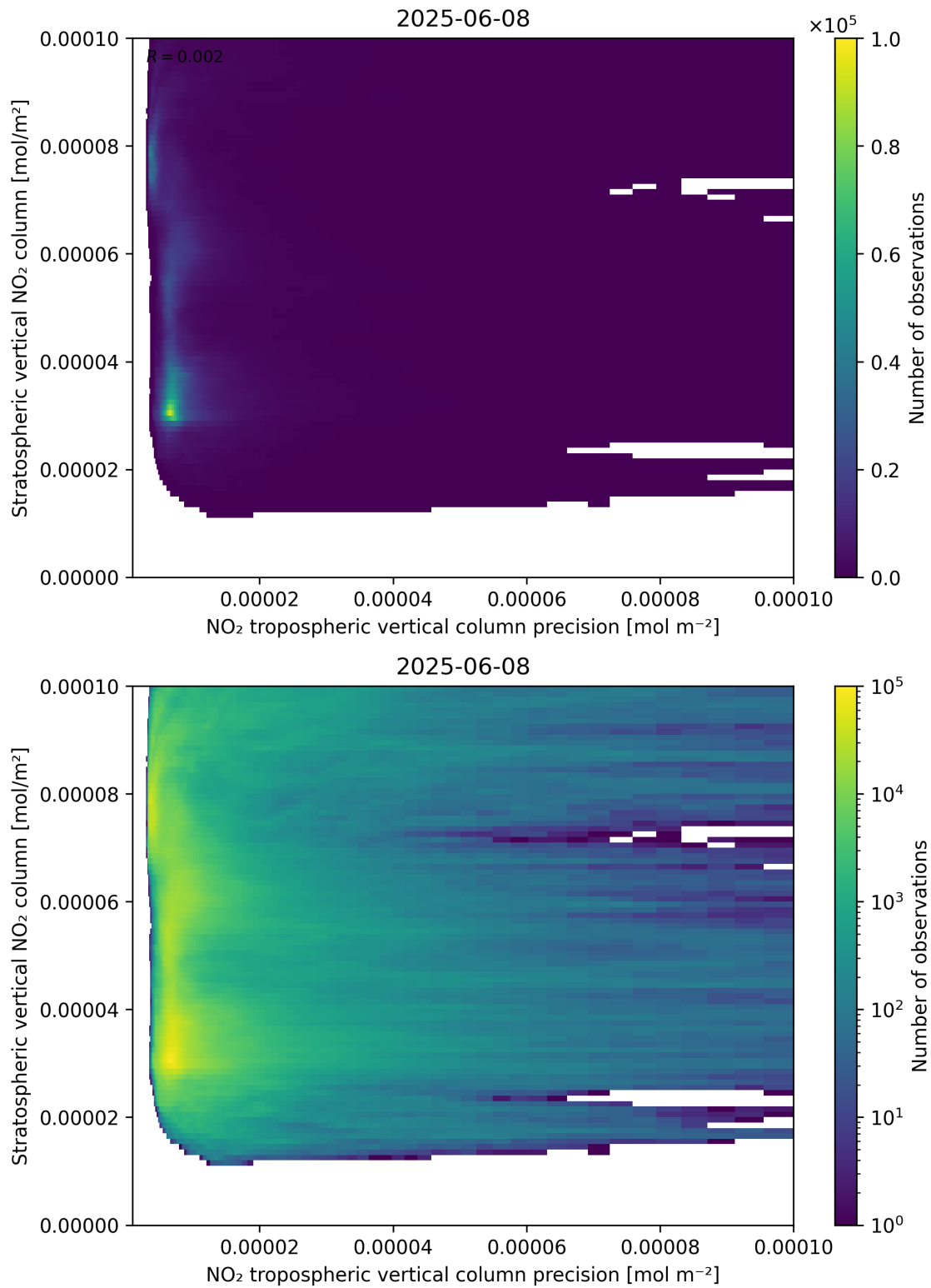
Figure 135: Scatter density plot of “NO 2 tropospheric vertical column precision” against “Stratospheric vertical NO 2 column” for 2025-06-07 to 2025-06-09.
