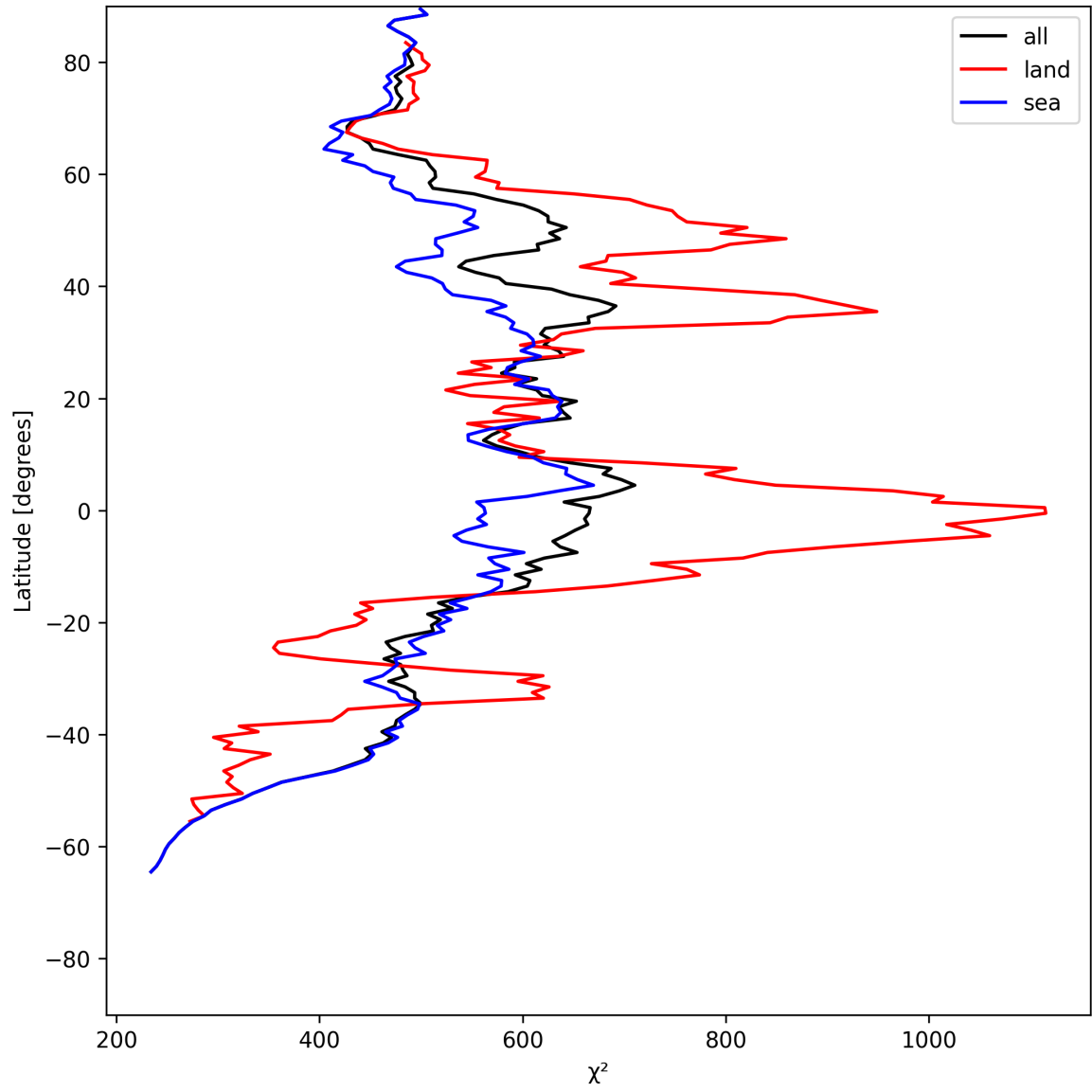
Figure 25: Zonal average of “ \chi^2 ” for 2025-06-07 to 2025-06-09.
