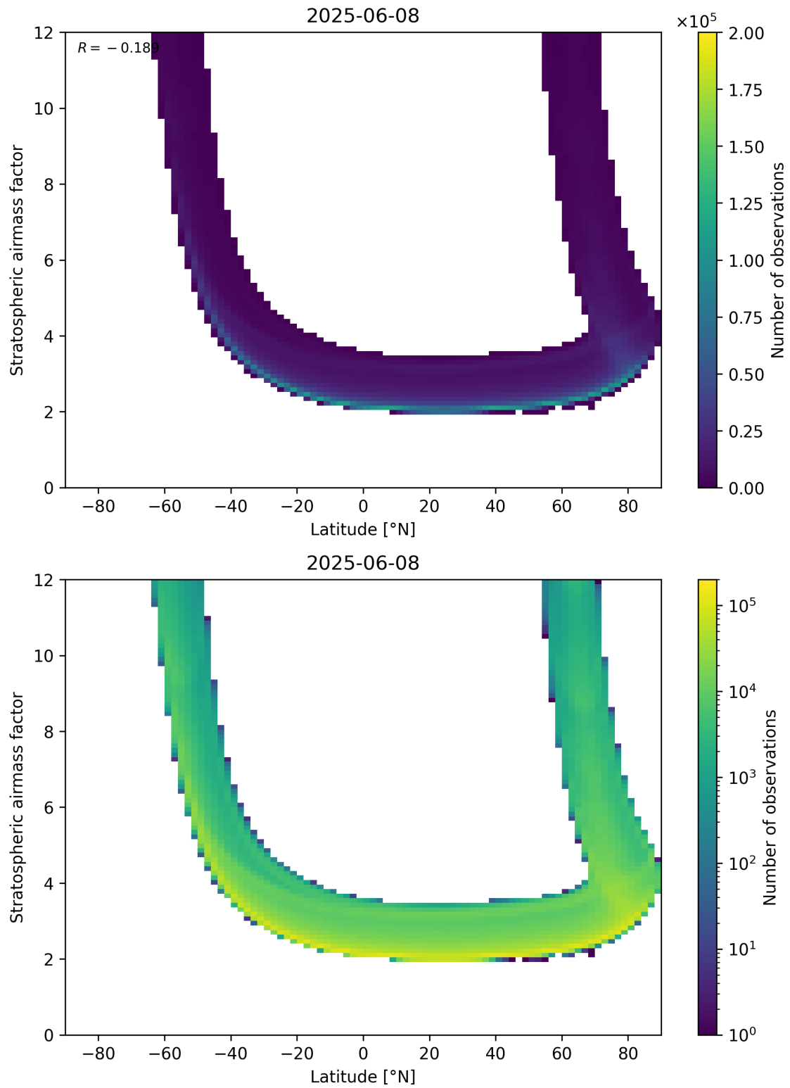
Figure 83: Scatter density plot of “Latitude” against “Stratospheric air mass factor” for 2025-06-07 to 2025-06-09.
