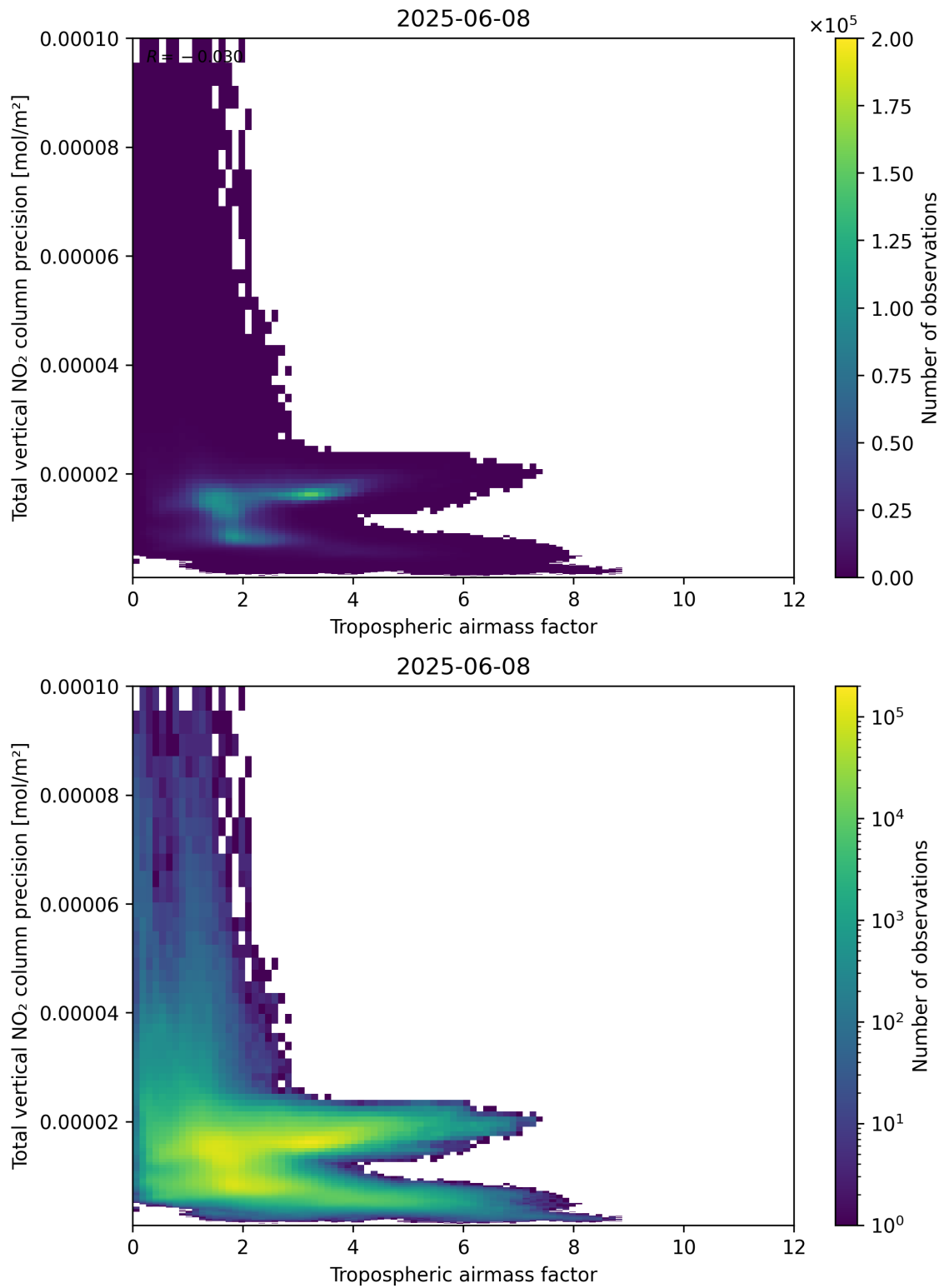
Figure 78: Scatter density plot of “Tropospheric airmass factor” against “Total vertical NO 2 column precision” for 2025-06-07 to 2025-06-09.
