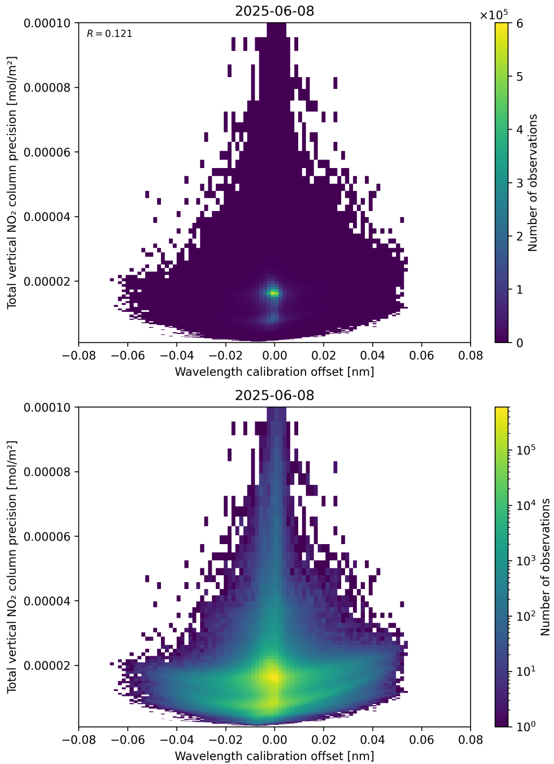
Figure 180: Scatter density plot of “Wavelength calibration offset” against “Total vertical NO 2 column precision” for 2025-06-07 to 2025-06-09.
