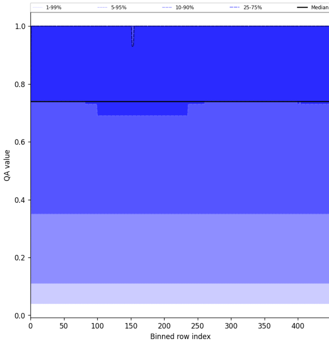
Figure 45: Along track statistics of “QA value” for 2025-06-07 to 2025-06-09
