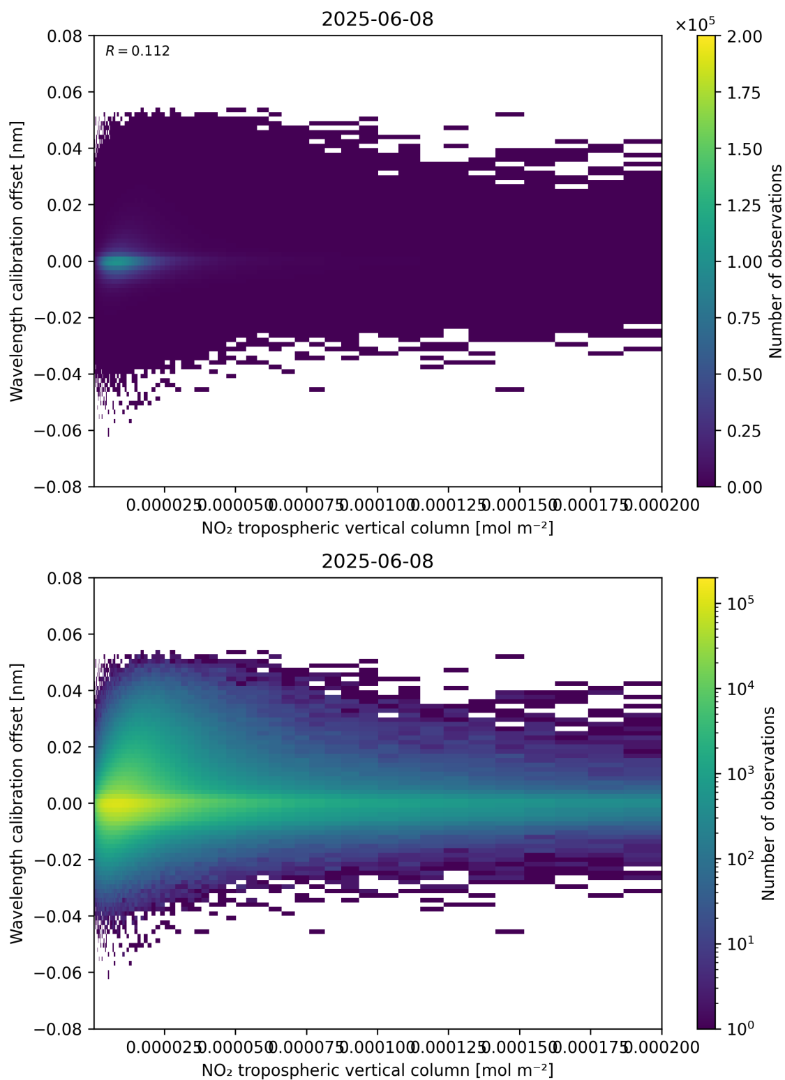
Figure 143: Scatter density plot of “NO 2 tropospheric vertical column” against “Wavelength calibration offset” for 2025-06-07 to 2025-06-09.
