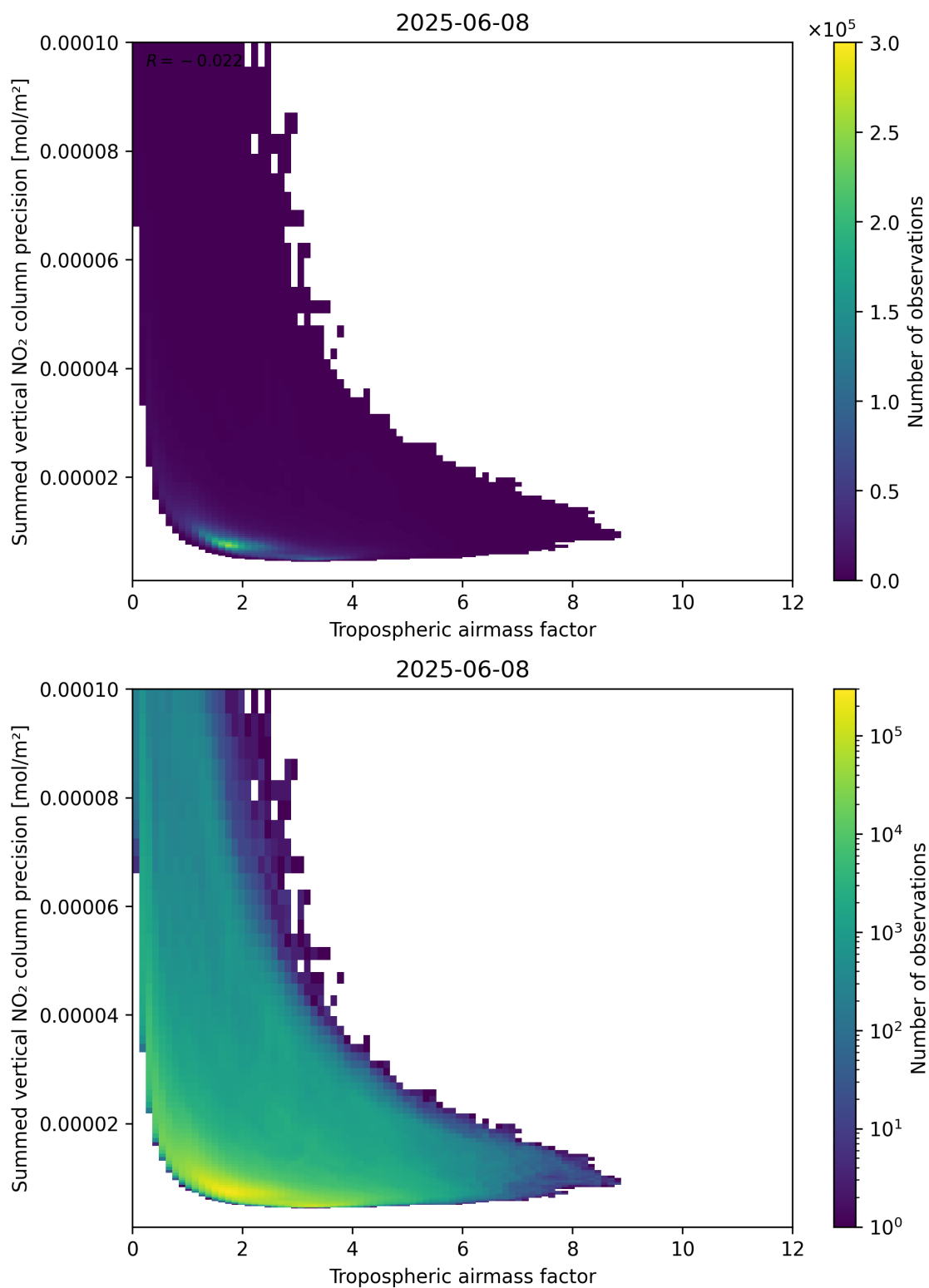
Figure 76: Scatter density plot of “Tropospheric air mass factor” against “Summed vertical NO 2 column precision” for 2025-06-07 to 2025-06-09.
