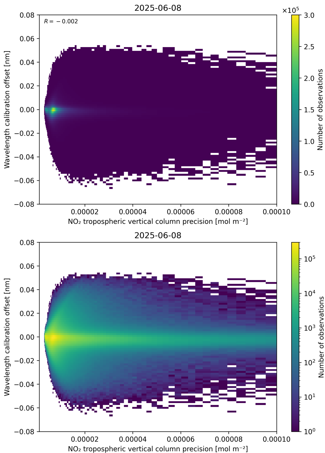
Figure 141: Scatter density plot of “NO 2 tropospheric vertical column precision” against “Wavelength calibration offset” for 2025-06-07 to 2025-06-09.
