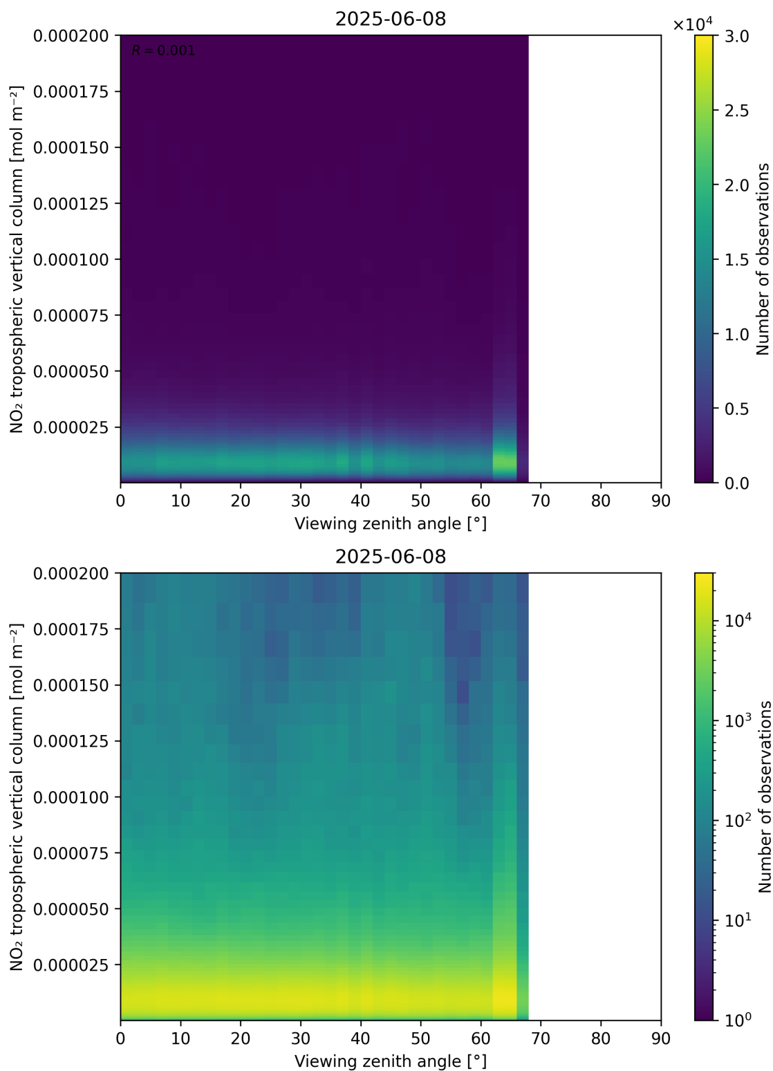
Figure 169: Scatter density plot of “Viewing zenith angle” against “NO 2 tropospheric vertical column” for 2025-06-07 to 2025-06-09.
