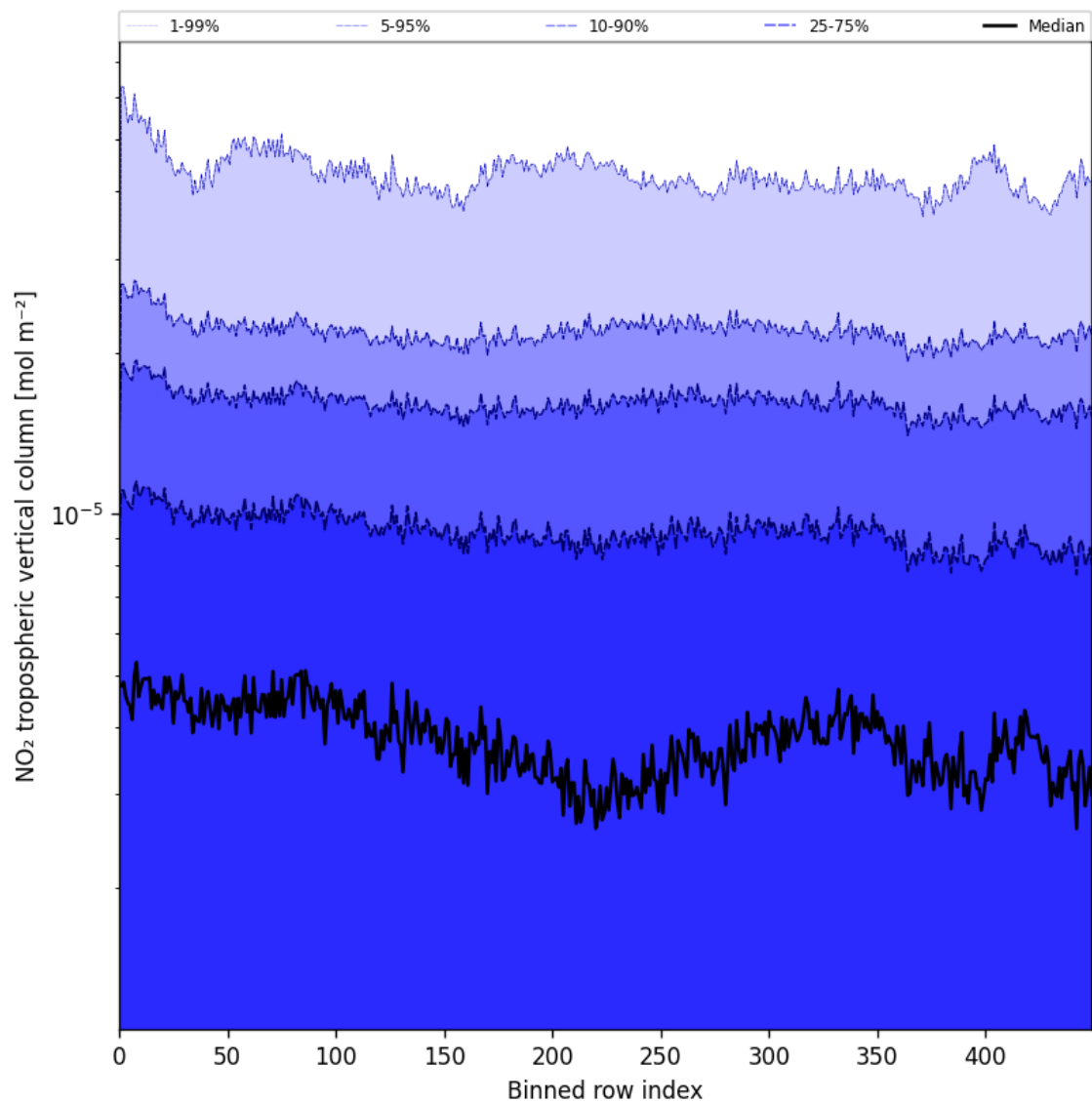
Figure 46: Along track statistics of “NO 2 tropospheric vertical column” for 2025-06-07 to 2025-06-09
