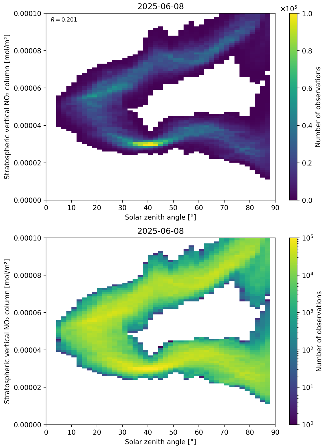
Figure 150: Scatter density plot of “Solar zenith angle” against “Stratospheric vertical \text{NO}_2 column” for 2025-06-07 to 2025-06-09.
