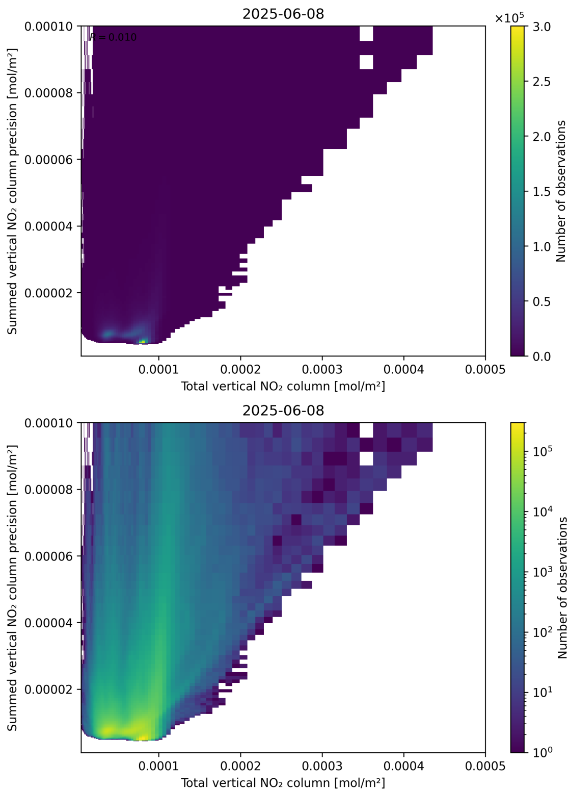
Figure 113: Scatter density plot of “Total vertical NO 2 column” against “Summed vertical NO 2 column precision” for 2025-06-07 to 2025-06-09.
