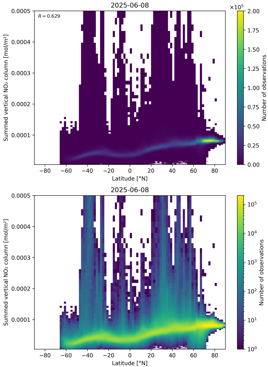
Figure 88: Scatter density plot of “Latitude” against “Summed vertical NO 2 column” for 2025-06-07 to 2025-06-09.
