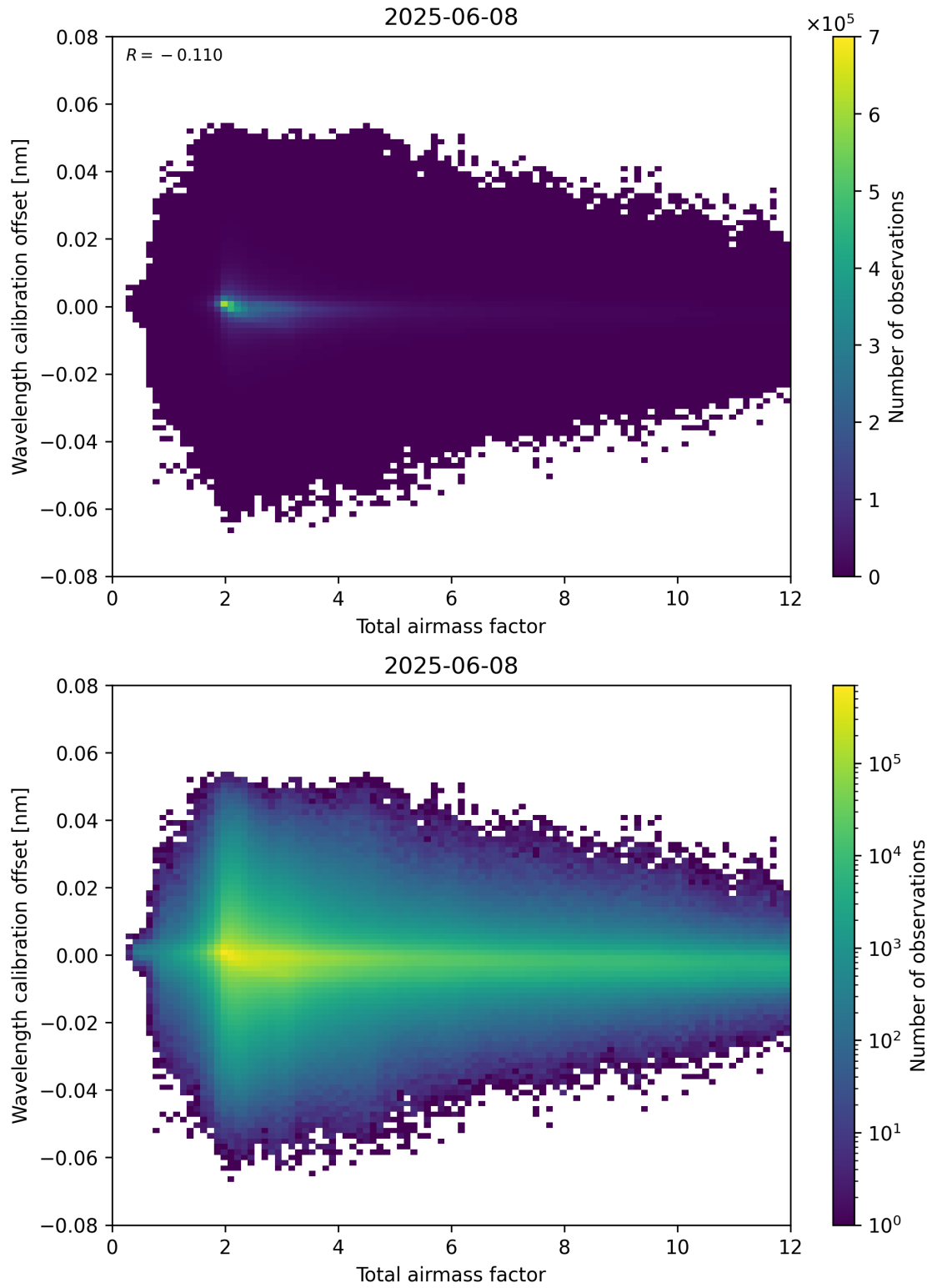
Figure 70: Scatter density plot of “Total airmass factor” against “Wavelength calibration offset” for 2025-06-07 to 2025-06-09.
