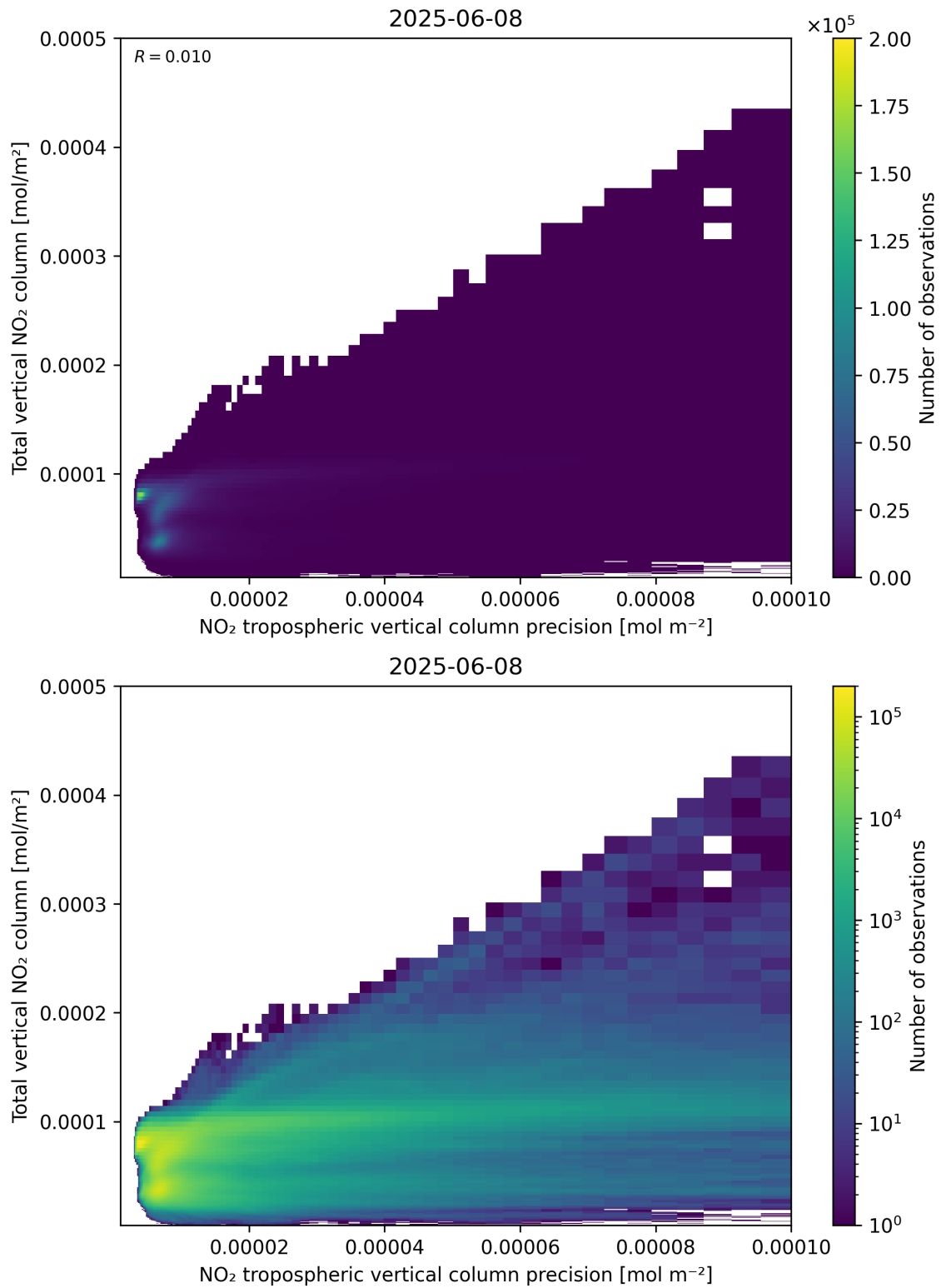
Figure 138: Scatter density plot of “NO 2 tropospheric vertical column precision” against “Total vertical NO 2 column” for 2025-06-07 to 2025-06-09.
