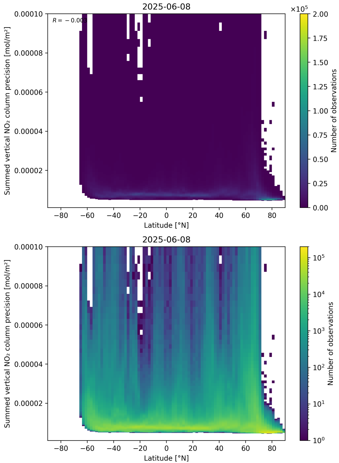
Figure 89: Scatter density plot of “Latitude” against “Summed vertical NO 2 column precision” for 2025-06-07 to 2025-06-09.
