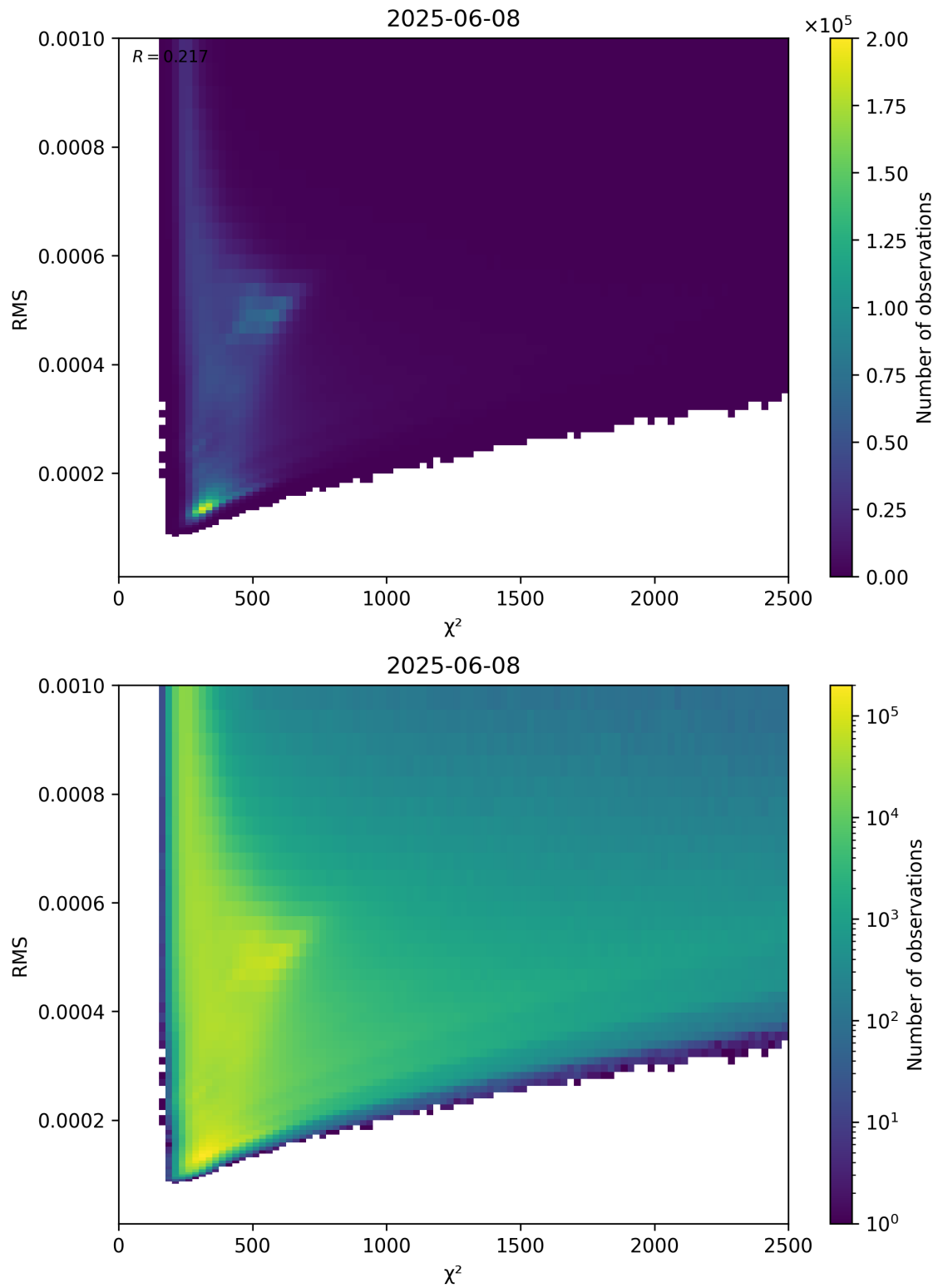
Figure 82: Scatter density plot of “ \chi^2 ” against “RMS” for 2025-06-07 to 2025-06-09.
