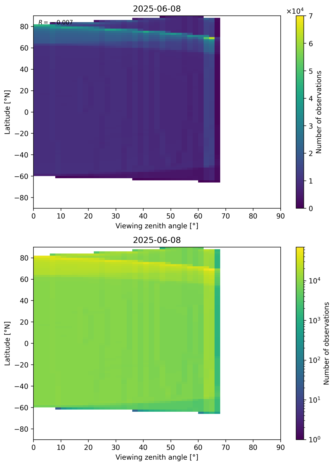
Figure 163: Scatter density plot of “Viewing zenith angle” against “Latitude” for 2025-06-07 to 2025-06-09.
