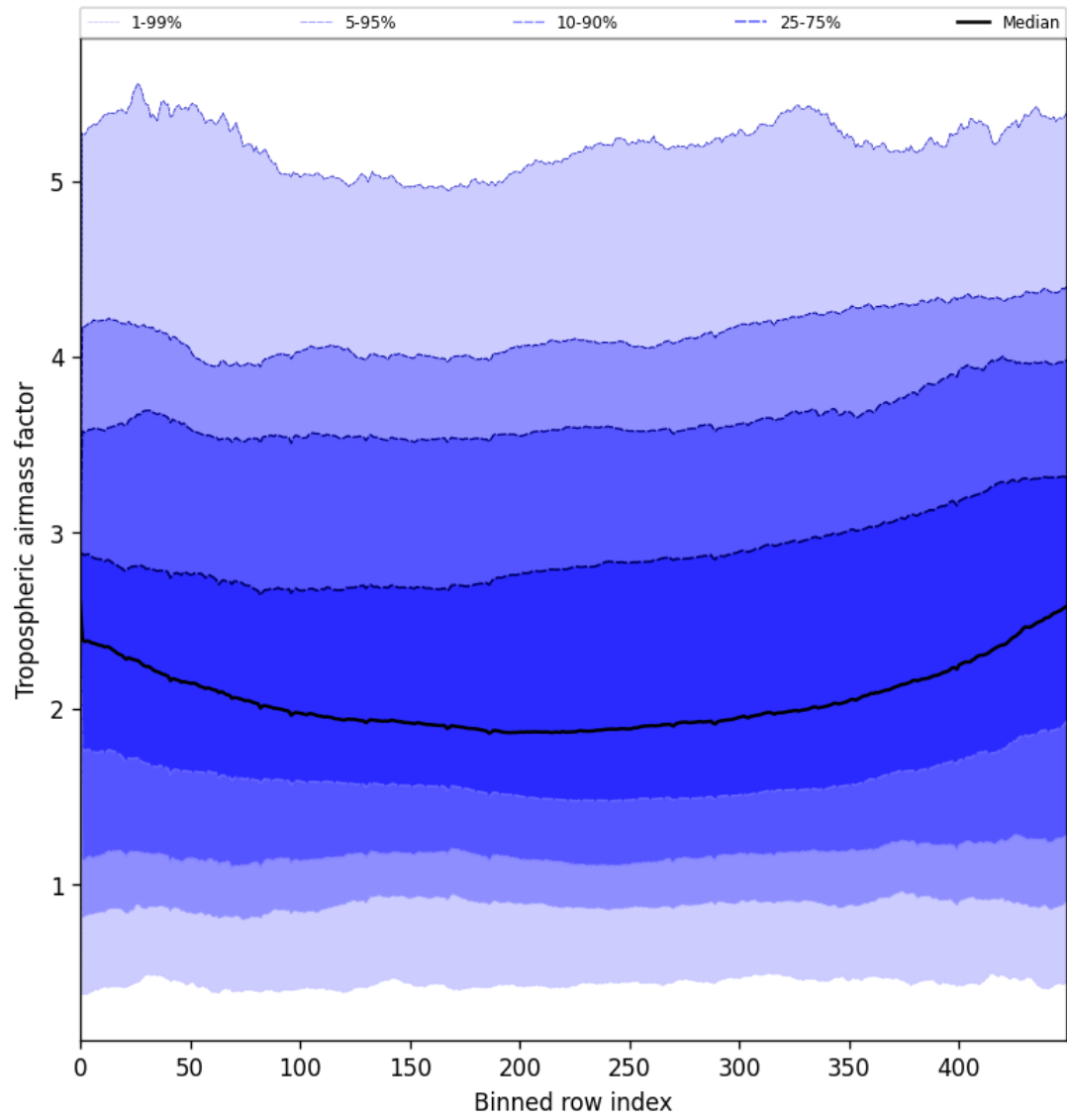
Figure 48: Along track statistics of “Tropospheric airmass factor” for 2025-06-07 to 2025-06-09
