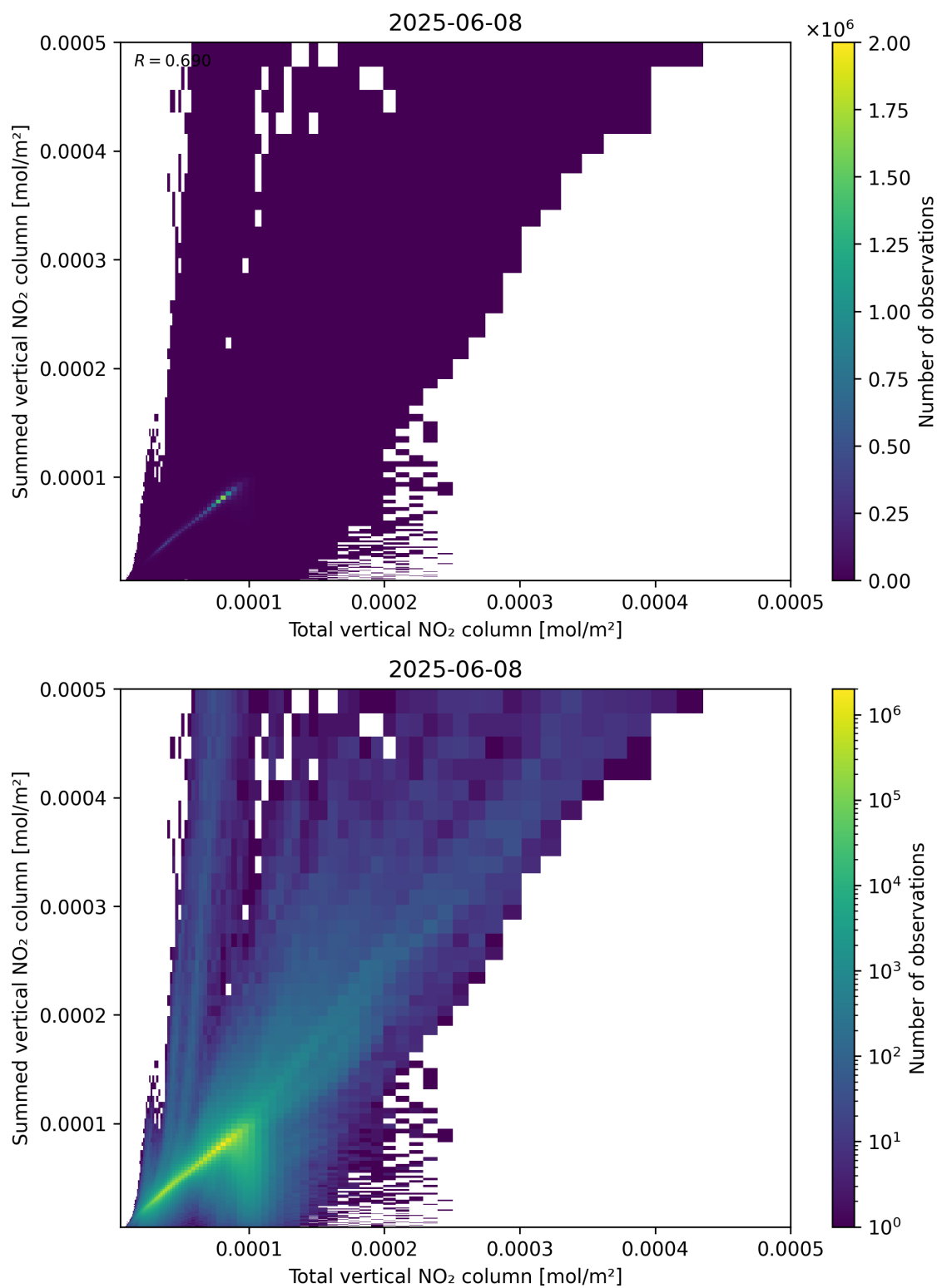
Figure 112: Scatter density plot of “Total vertical NO 2 column” against “Summed vertical NO 2 column” for 2025-06-07 to 2025-06-09.
