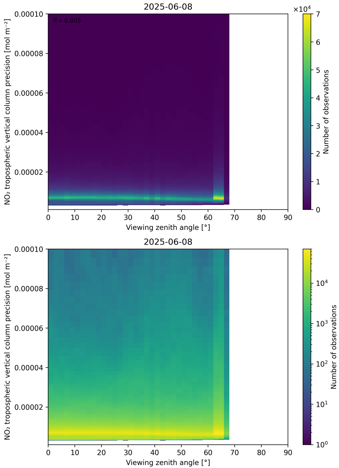
Figure 170: Scatter density plot of “Viewing zenith angle” against “NO 2 tropospheric vertical column precision” for 2025-06-07 to 2025-06-09.
