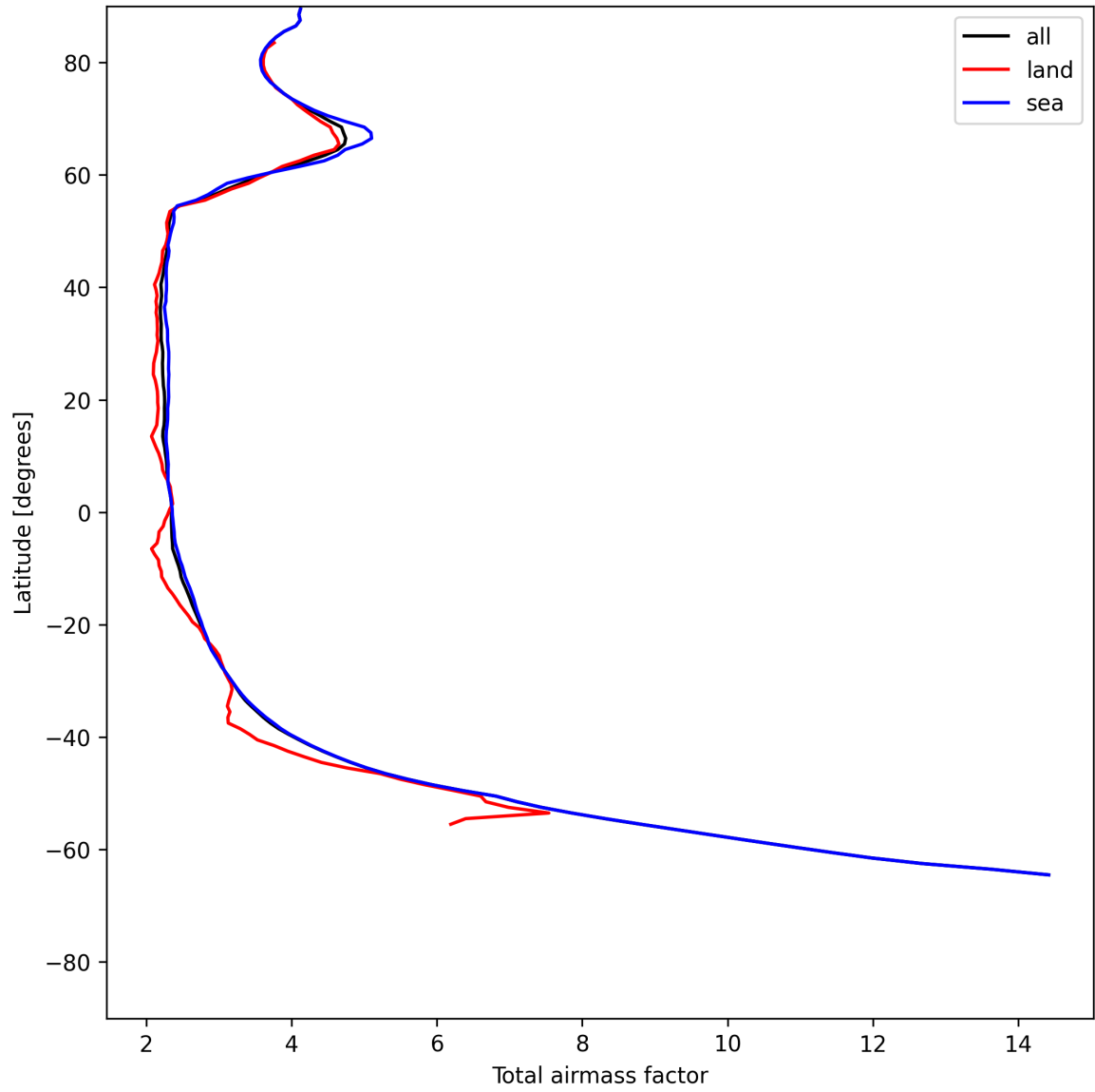
Figure 15: Zonal average of “Total airmass factor” for 2025-06-07 to 2025-06-09.
