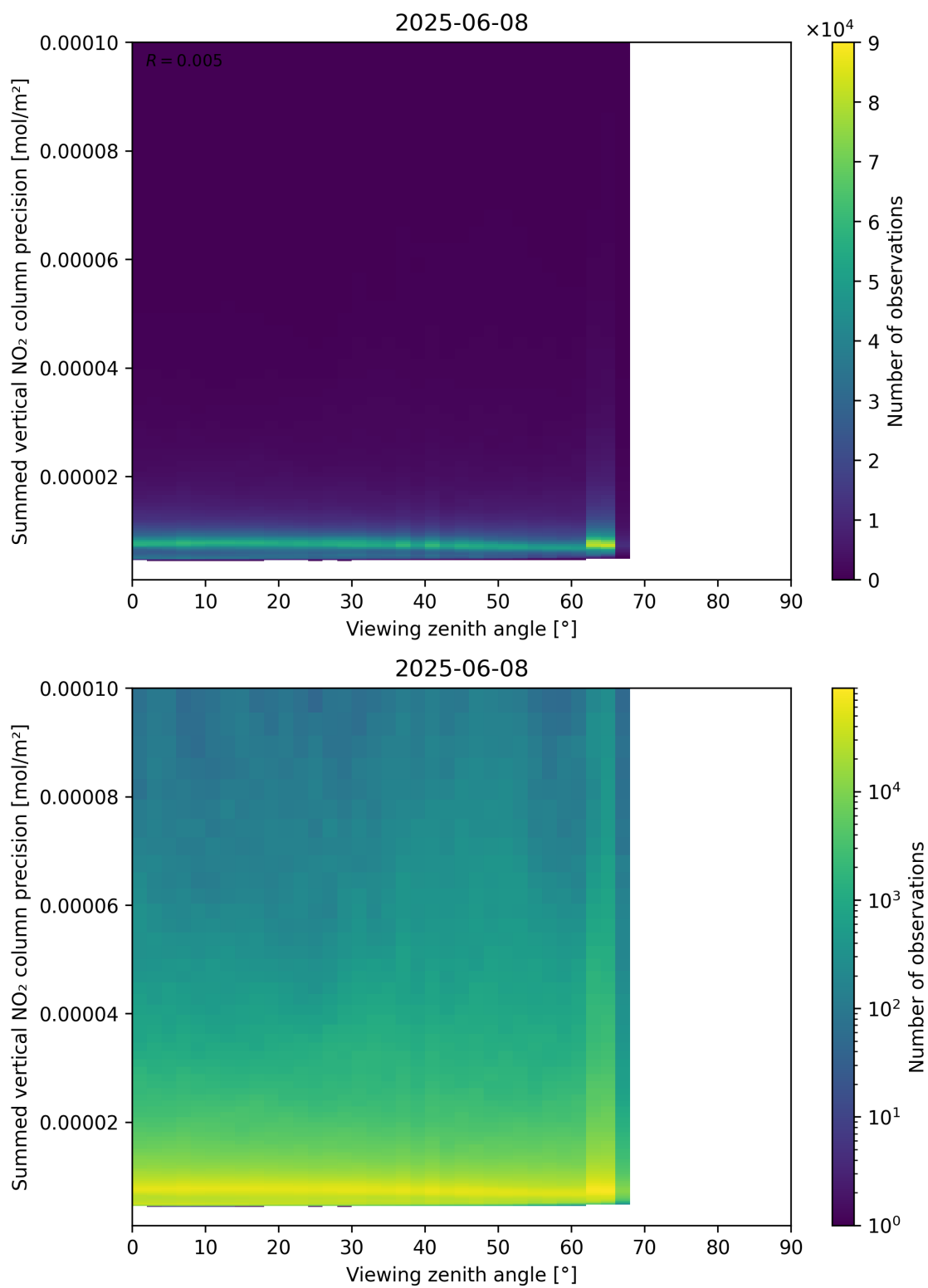
Figure 166: Scatter density plot of “Viewing zenith angle” against “Summed vertical NO 2 column precision” for 2025-06-07 to 2025-06-09.
