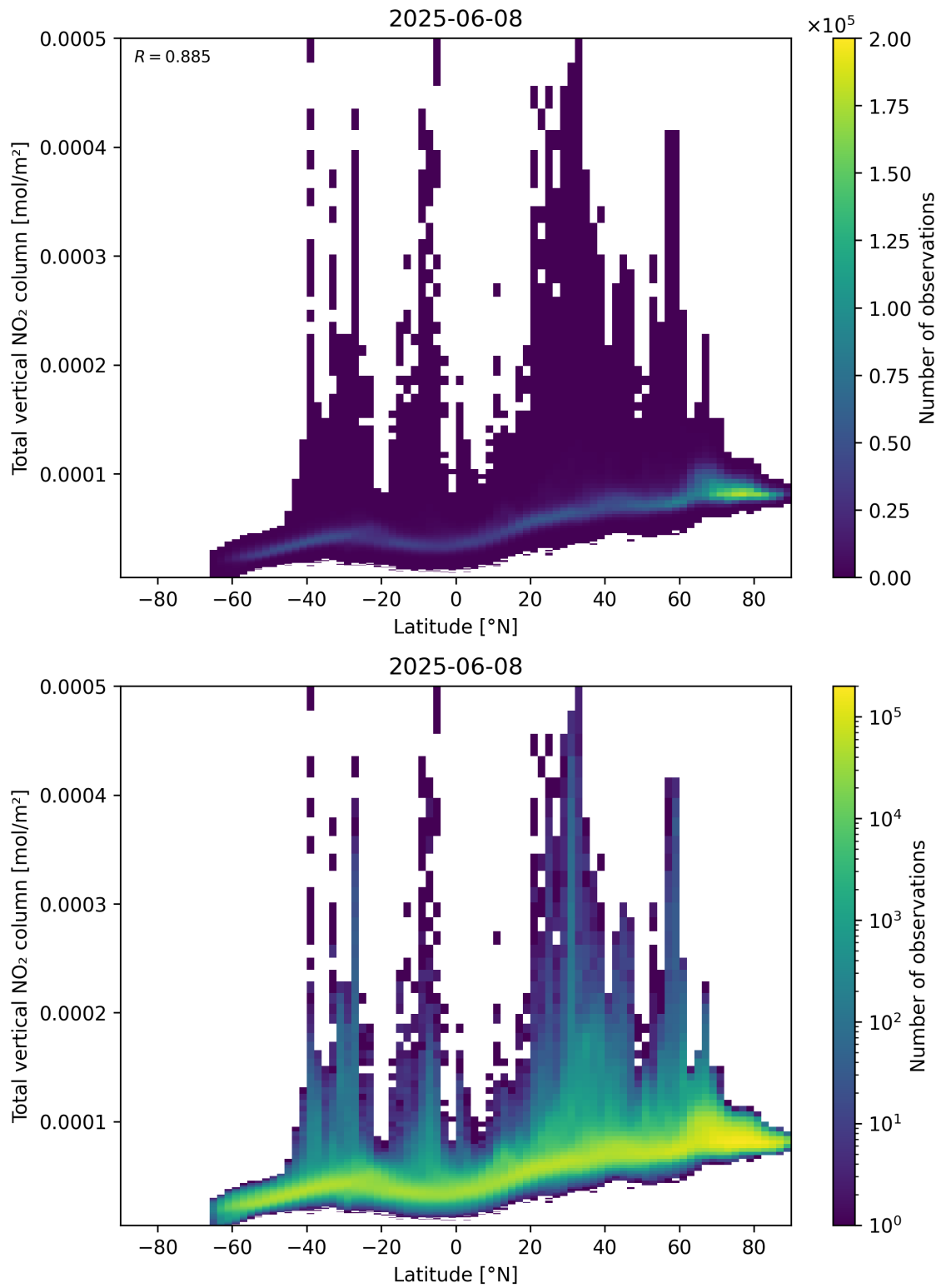
Figure 90: Scatter density plot of “Latitude” against “Total vertical NO 2 column” for 2025-06-07 to 2025-06-09.
