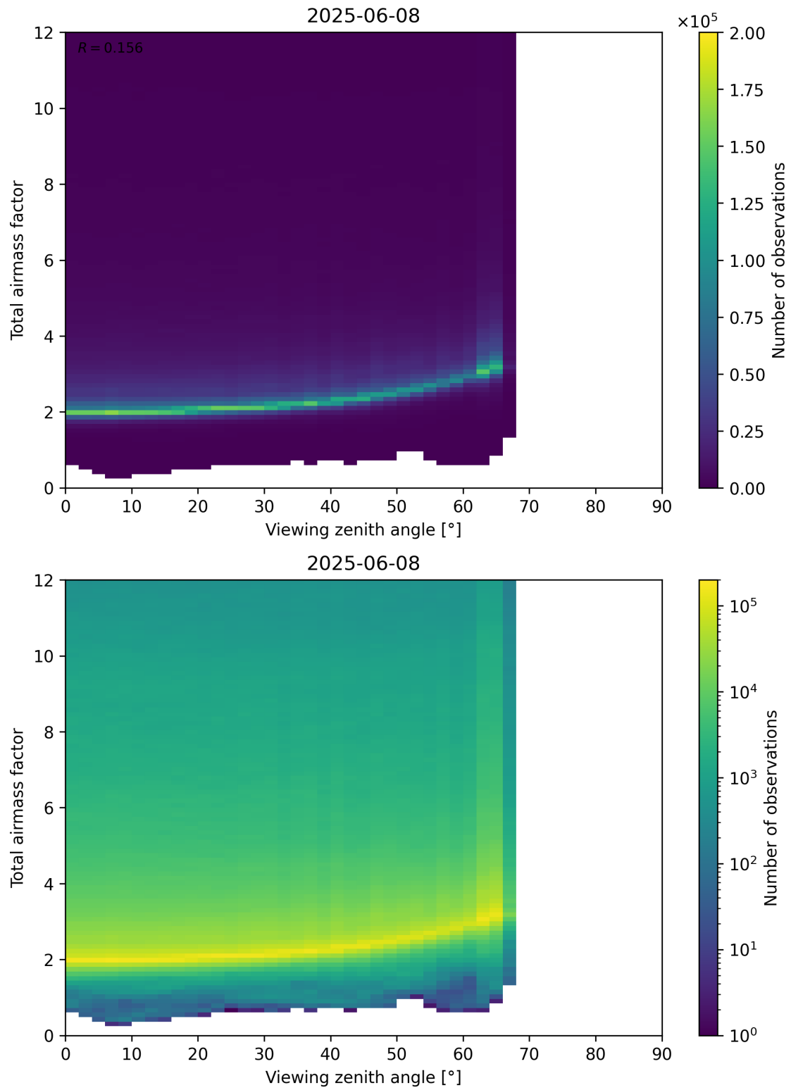
Figure 160: Scatter density plot of “Viewing zenith angle” against “Total airmass factor” for 2025-06-07 to 2025-06-09.
