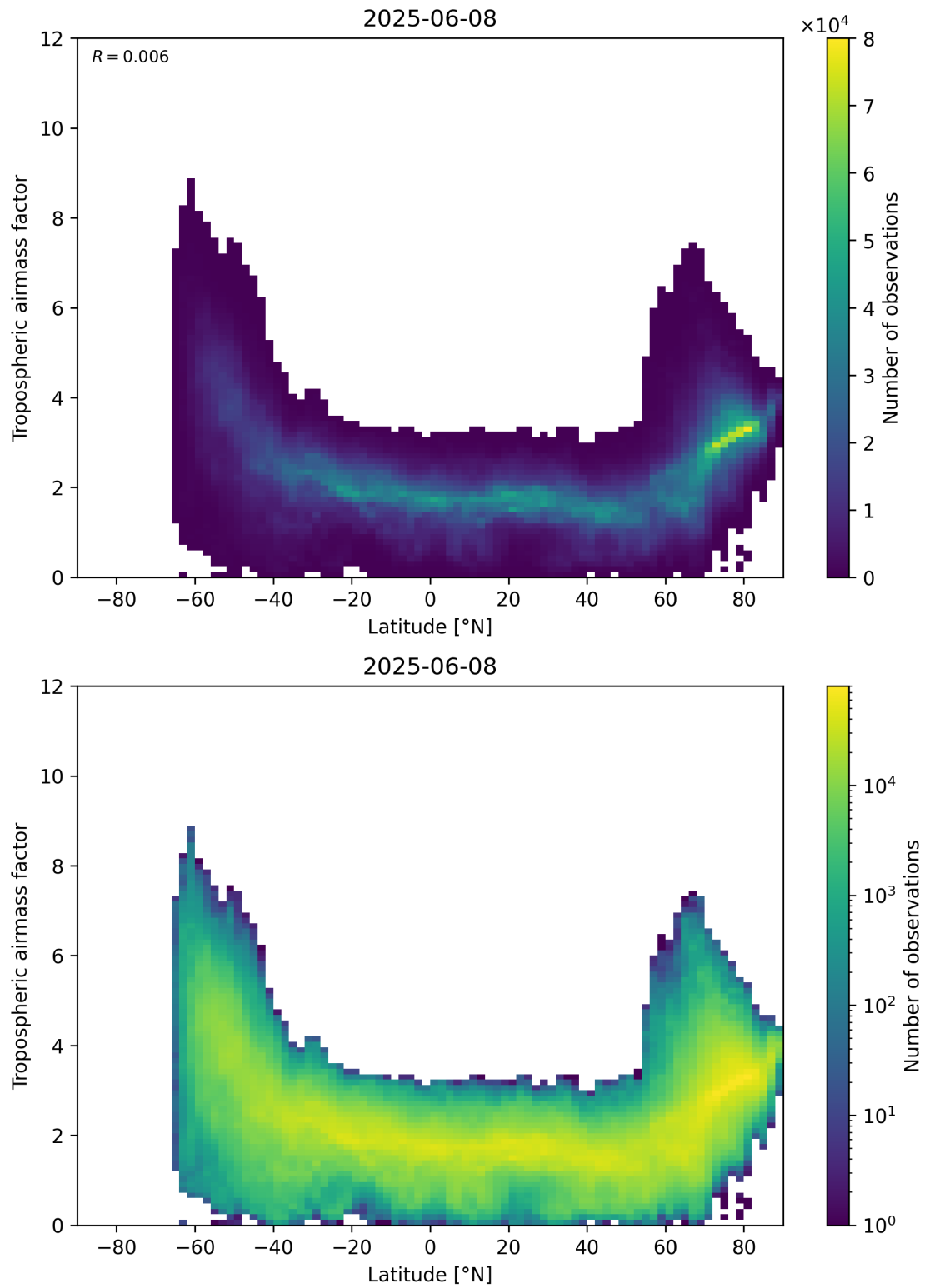
Figure 85: Scatter density plot of “Latitude” against “Tropospheric air mass factor” for 2025-06-07 to 2025-06-09.
