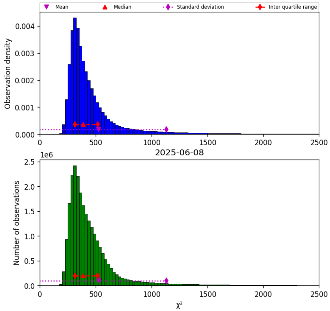
Figure 42: Histogram of “ \chi^2 ” for 2025-06-07 to 2025-06-09
