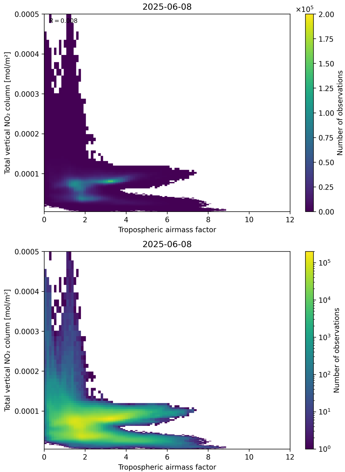
Figure 77: Scatter density plot of “Tropospheric airmass factor” against “Total vertical NO 2 column” for 2025-06-07 to 2025-06-09.
