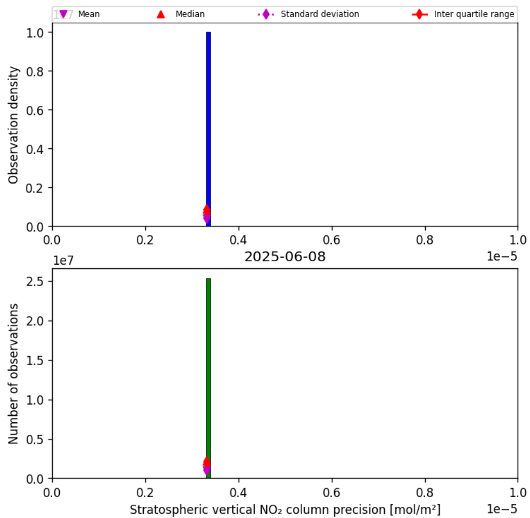
Figure 37: Histogram of “Stratospheric vertical NO 2 column precision” for 2025-06-07 to 2025-06-09
