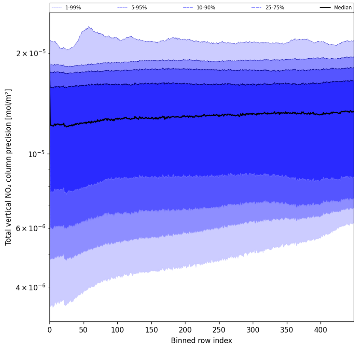
Figure 56: Along track statistics of “Total vertical NO 2 column precision” for 2025-06-07 to 2025-06-09
