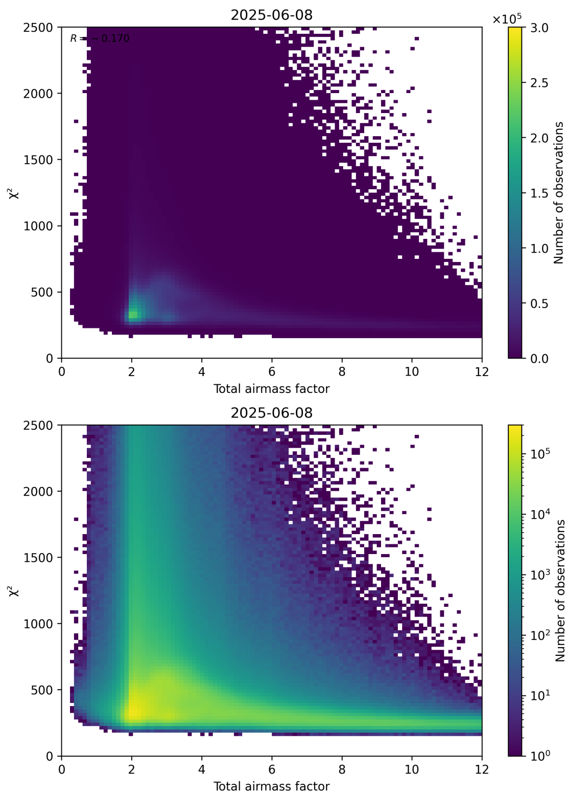
Figure 63: Scatter density plot of “Total airmass factor” against “ \chi^2 ” for 2025-06-07 to 2025-06-09.
