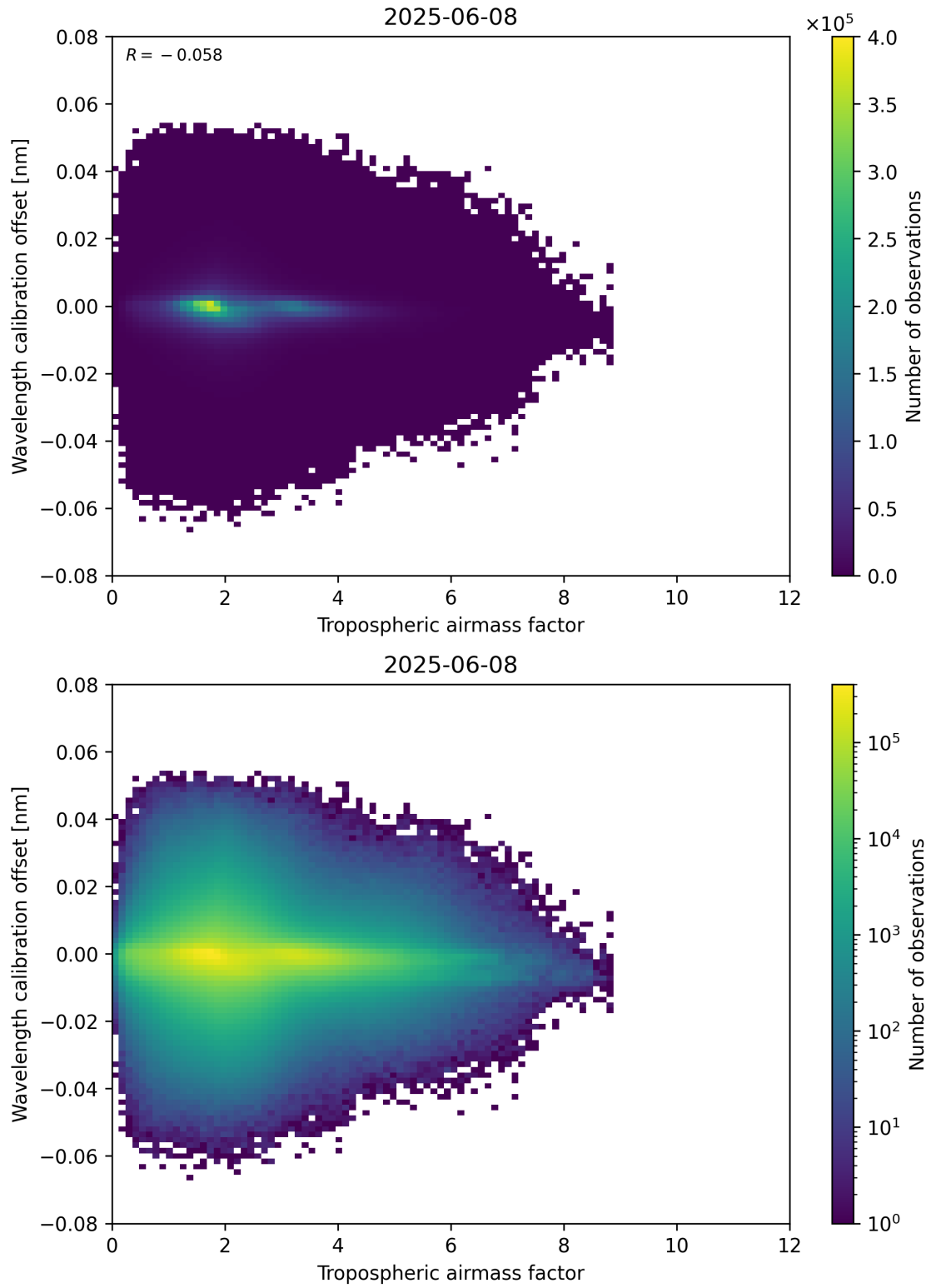
Figure 80: Scatter density plot of “Tropospheric airmass factor” against “Wavelength calibration offset” for 2025-06-07 to 2025-06-09.
