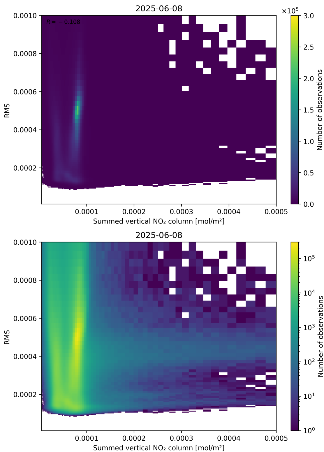
Figure 109: Scatter density plot of “Summed vertical NO 2 column” against “RMS” for 2025-06-07 to 2025-06-09.
