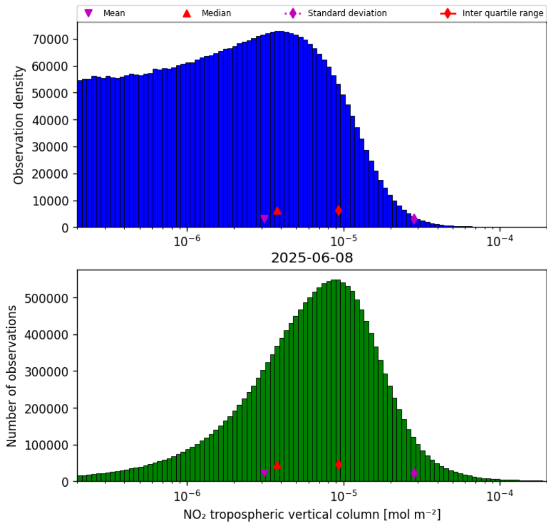
Figure 29: Histogram of “NO 2 tropospheric vertical column” for 2025-06-07 to 2025-06-09
