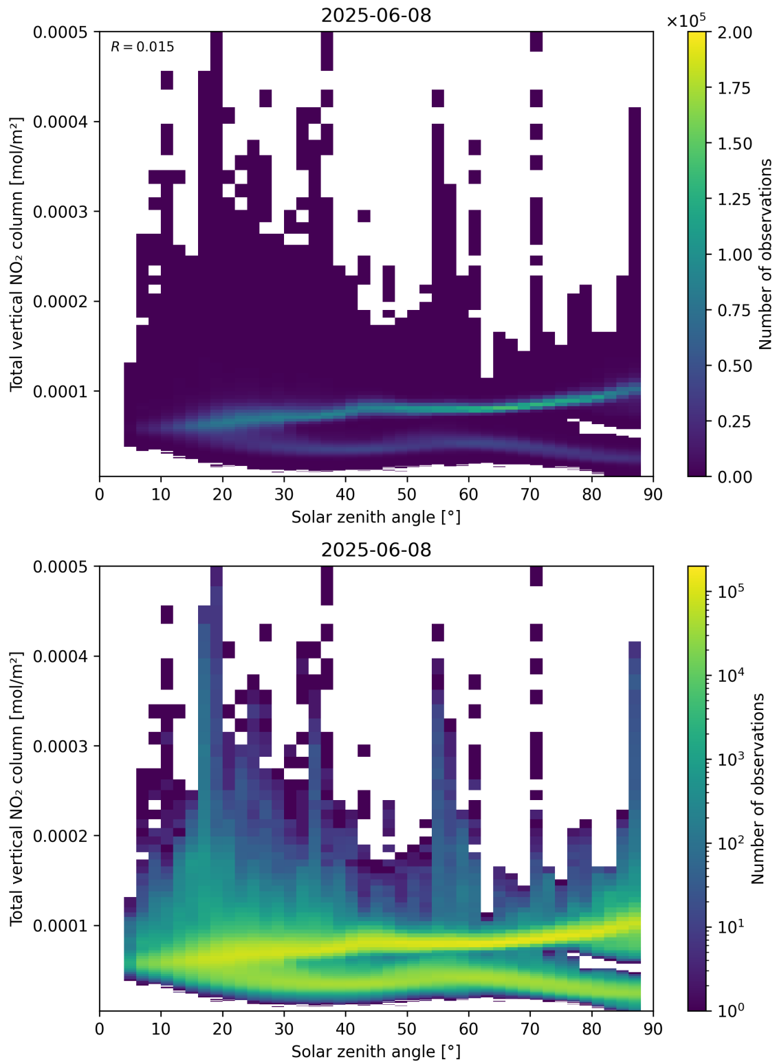
Figure 153: Scatter density plot of “Solar zenith angle” against “Total vertical NO 2 column” for 2025-06-07 to 2025-06-09.
