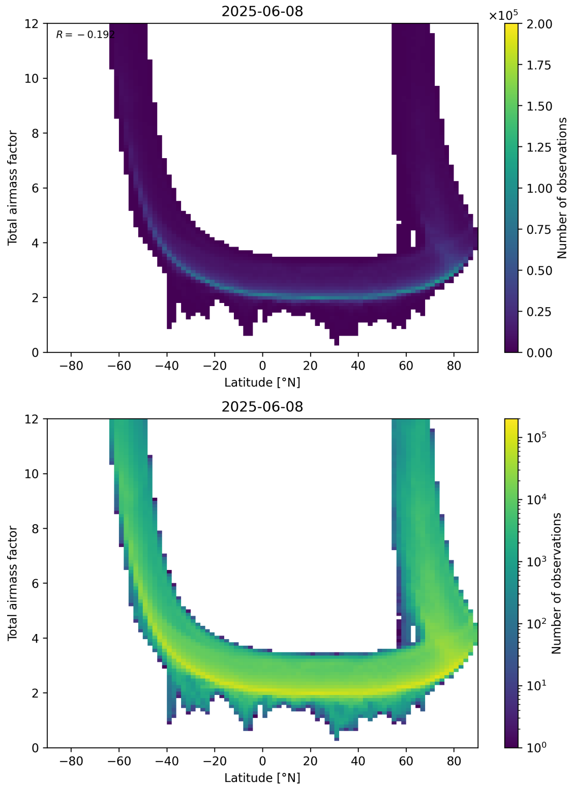
Figure 84: Scatter density plot of “Latitude” against “Total airmass factor” for 2025-06-07 to 2025-06-09.
