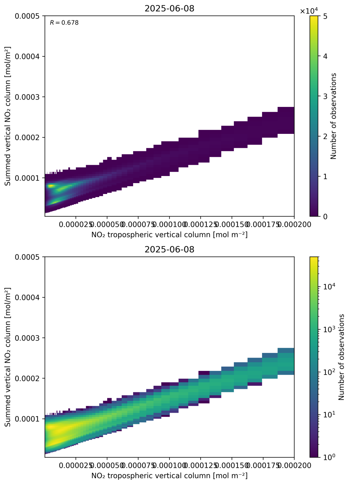
Figure 126: Scatter density plot of “NO 2 tropospheric vertical column” against “Summed vertical NO 2 column” for 2025-06-07 to 2025-06-09.
