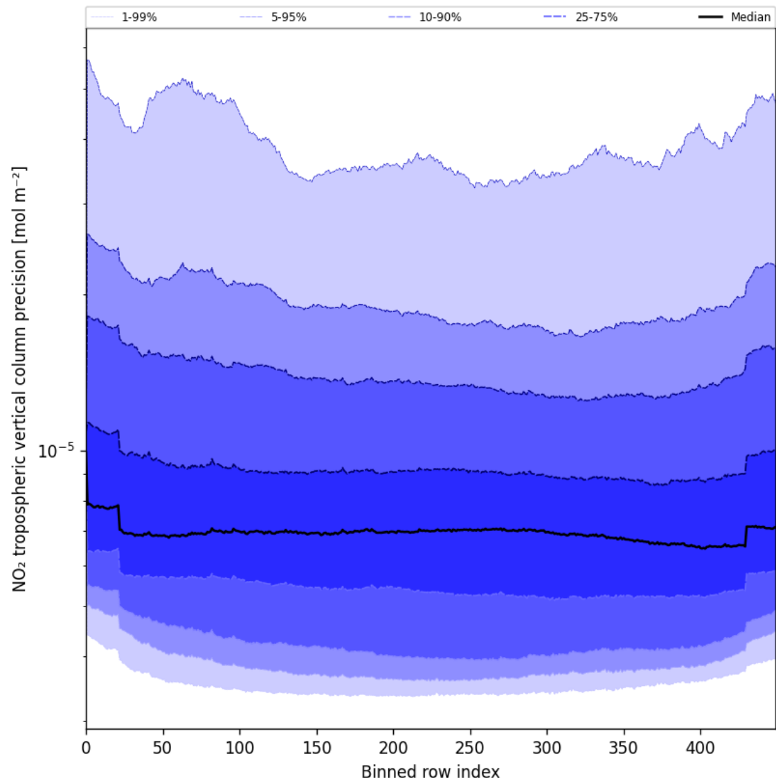
Figure 47: Along track statistics of “NO 2 tropospheric vertical column precision” for 2025-06-07 to 2025-06-09
