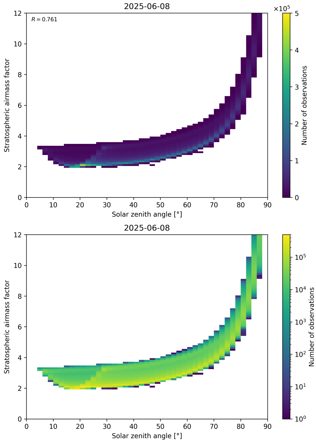
Figure 145: Scatter density plot of “Solar zenith angle” against “Stratospheric airmass factor” for 2025-06-07 to 2025-06-09.
