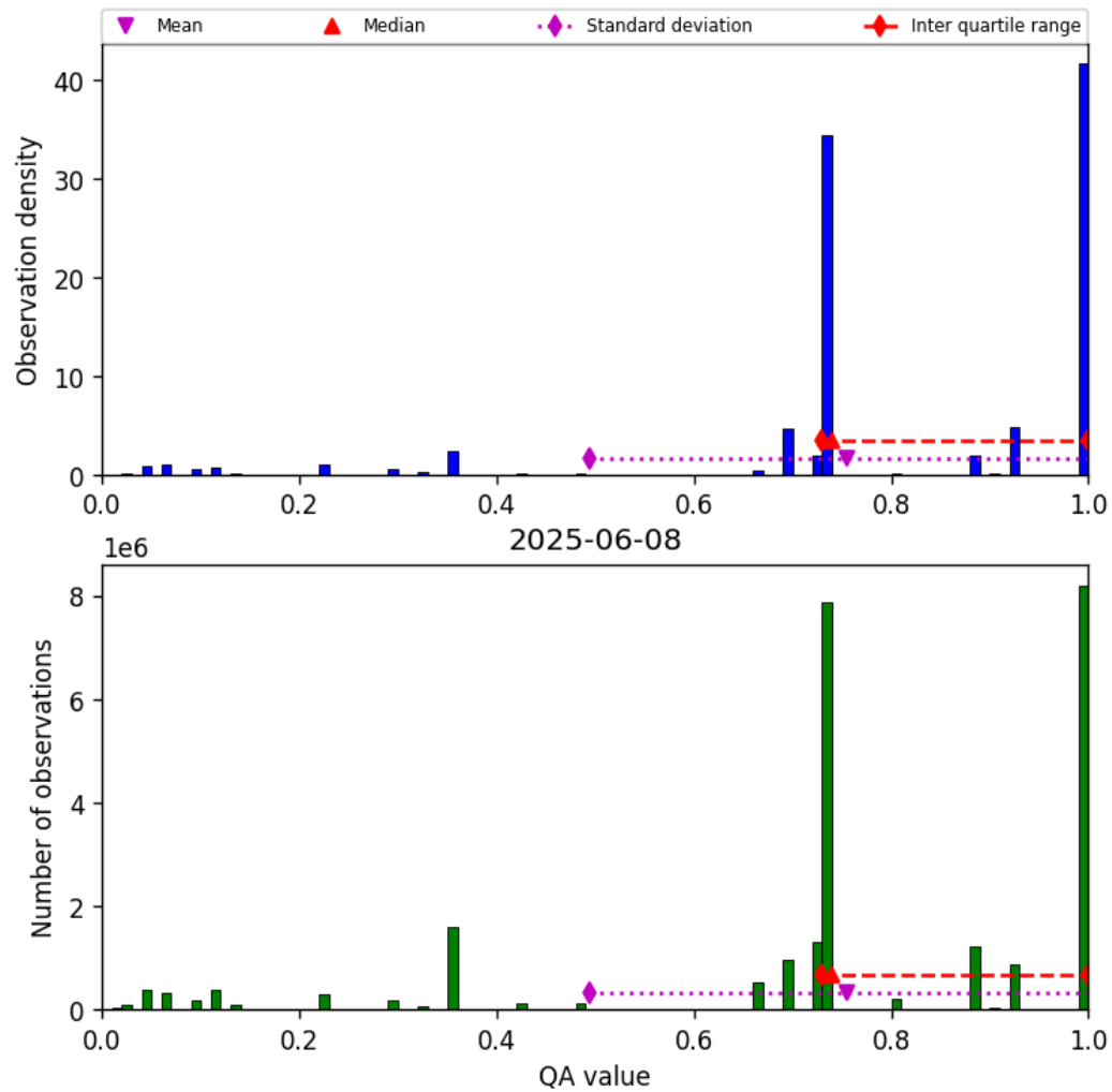
Figure 28: Histogram of “QA value” for 2025-06-07 to 2025-06-09
