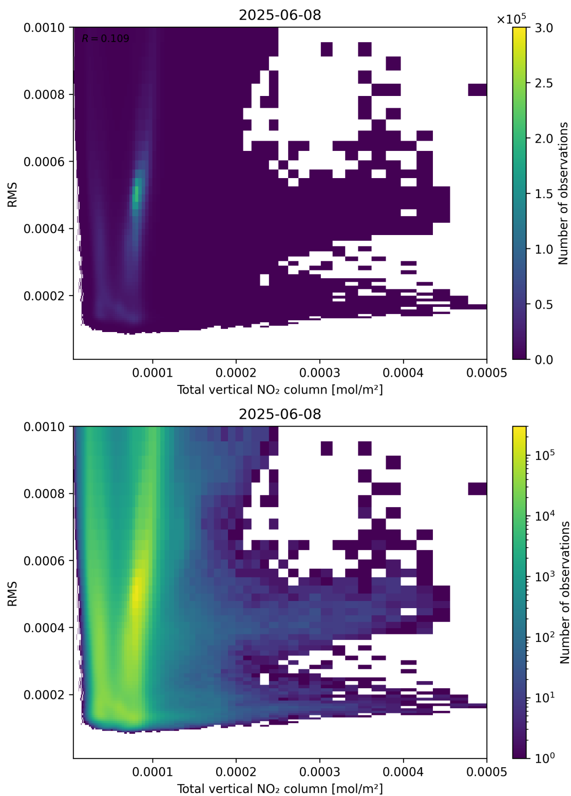
Figure 120: Scatter density plot of “Total vertical NO 2 column” against “RMS” for 2025-06-07 to 2025-06-09.
