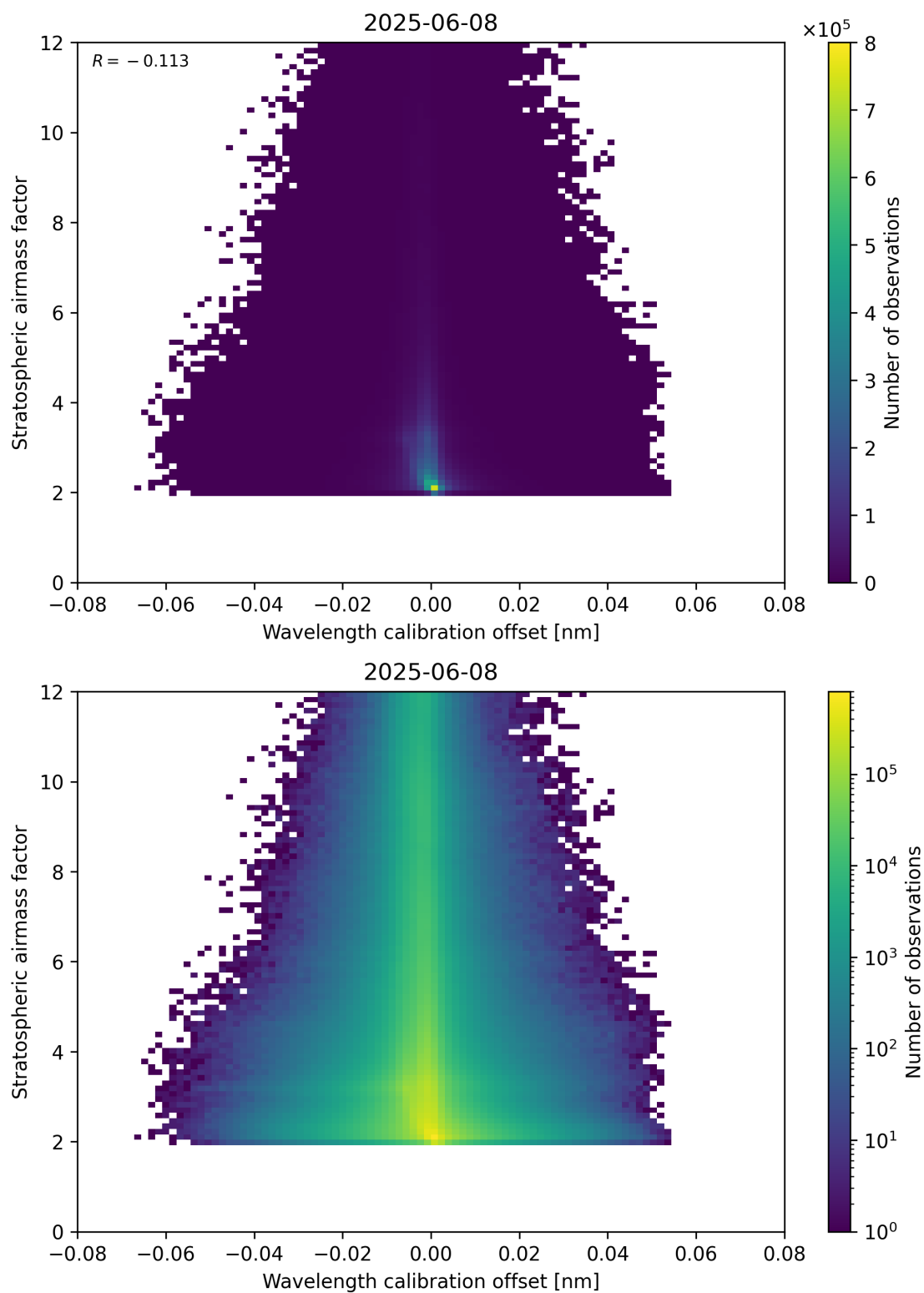
Figure 174: Scatter density plot of “Wavelength calibration offset” against “Stratospheric airmass factor” for 2025-06-07 to 2025-06-09.
