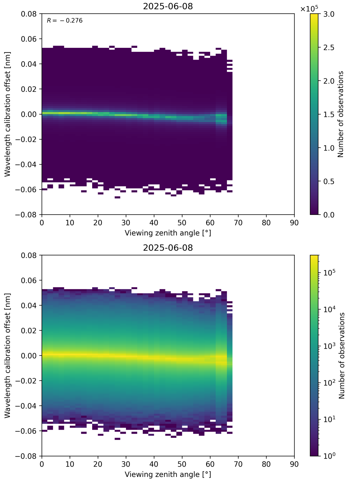
Figure 173: Scatter density plot of “Viewing zenith angle” against “Wavelength calibration offset” for 2025-06-07 to 2025-06-09.
