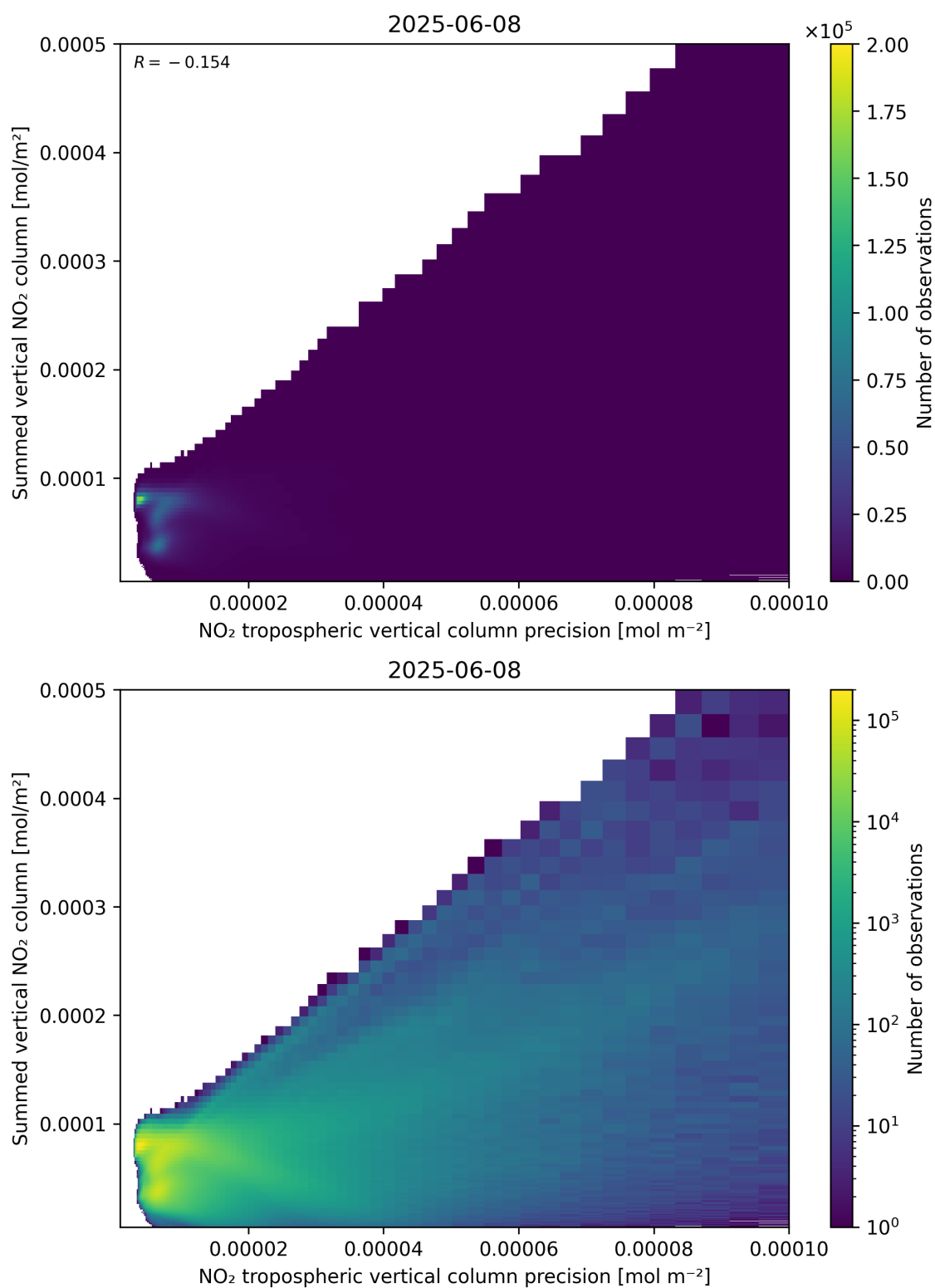
Figure 136: Scatter density plot of “NO 2 tropospheric vertical column precision” against “Summed vertical NO 2 column” for 2025-06-07 to 2025-06-09.
