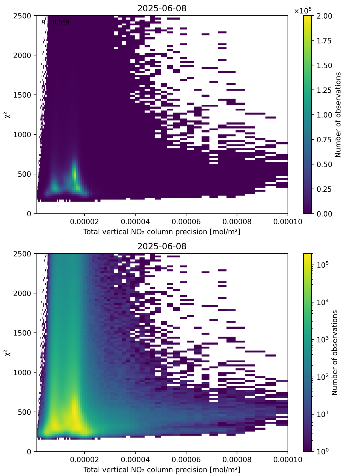
Figure 116: Scatter density plot of “Total vertical NO 2 column precision” against “ \chi^2 ” for 2025-06-07 to 2025-06-09.
