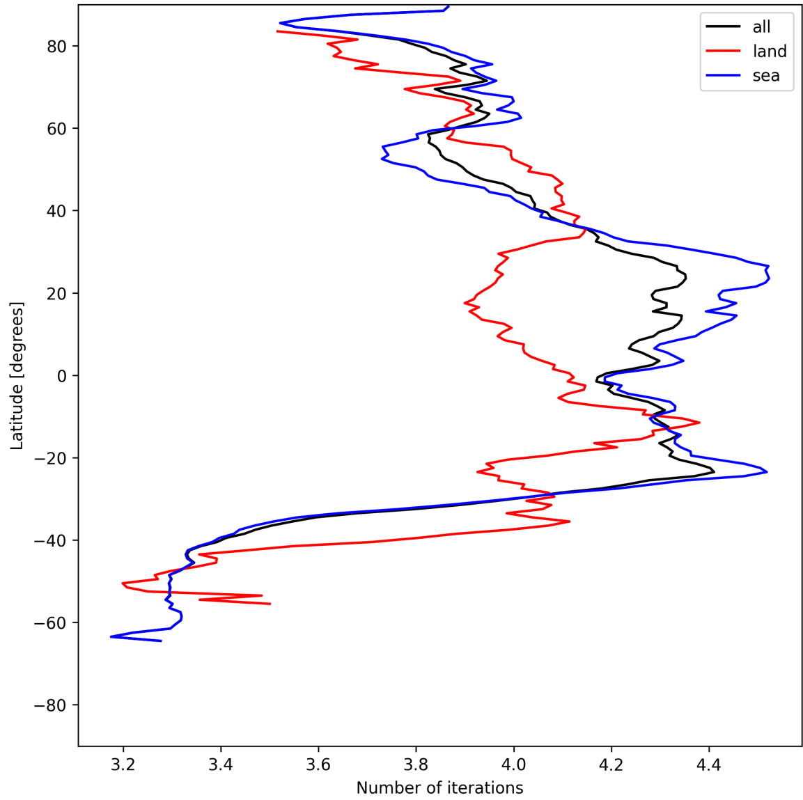
Figure 17: Zonal average of “Number of iterations” for 2025-06-07 to 2025-06-09.
