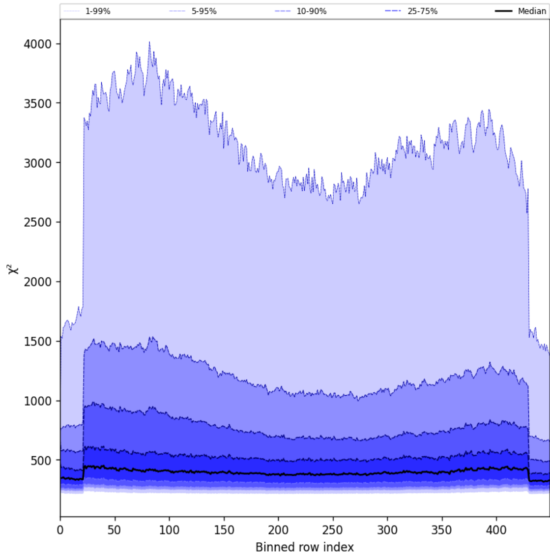
Figure 59: Along track statistics of “ \chi^2 ” for 2025-06-07 to 2025-06-09
