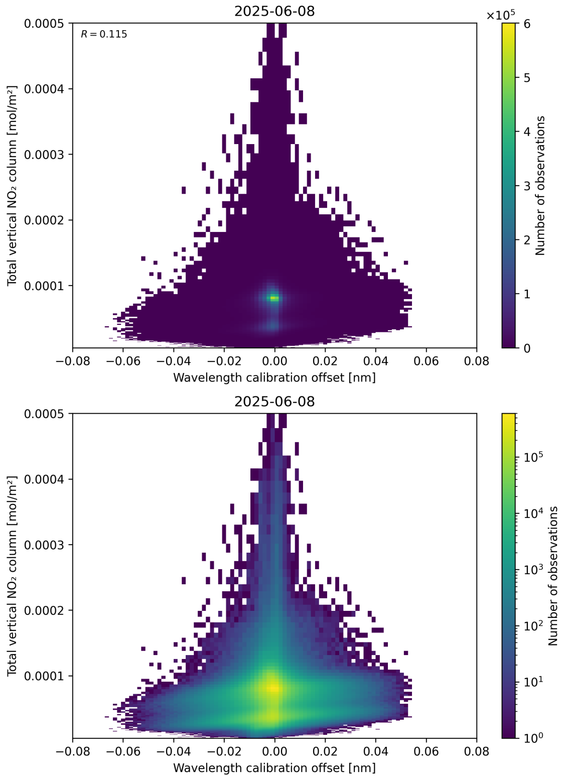
Figure 179: Scatter density plot of “Wavelength calibration offset” against “Total vertical NO 2 column” for 2025-06-07 to 2025-06-09.
