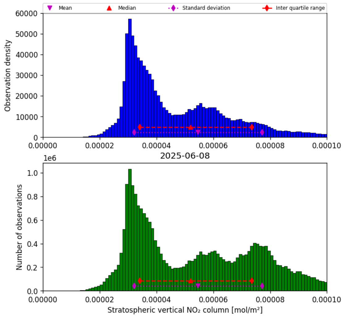
Figure 36: Histogram of “Stratospheric vertical NO 2 column” for 2025-06-07 to 2025-06-09
