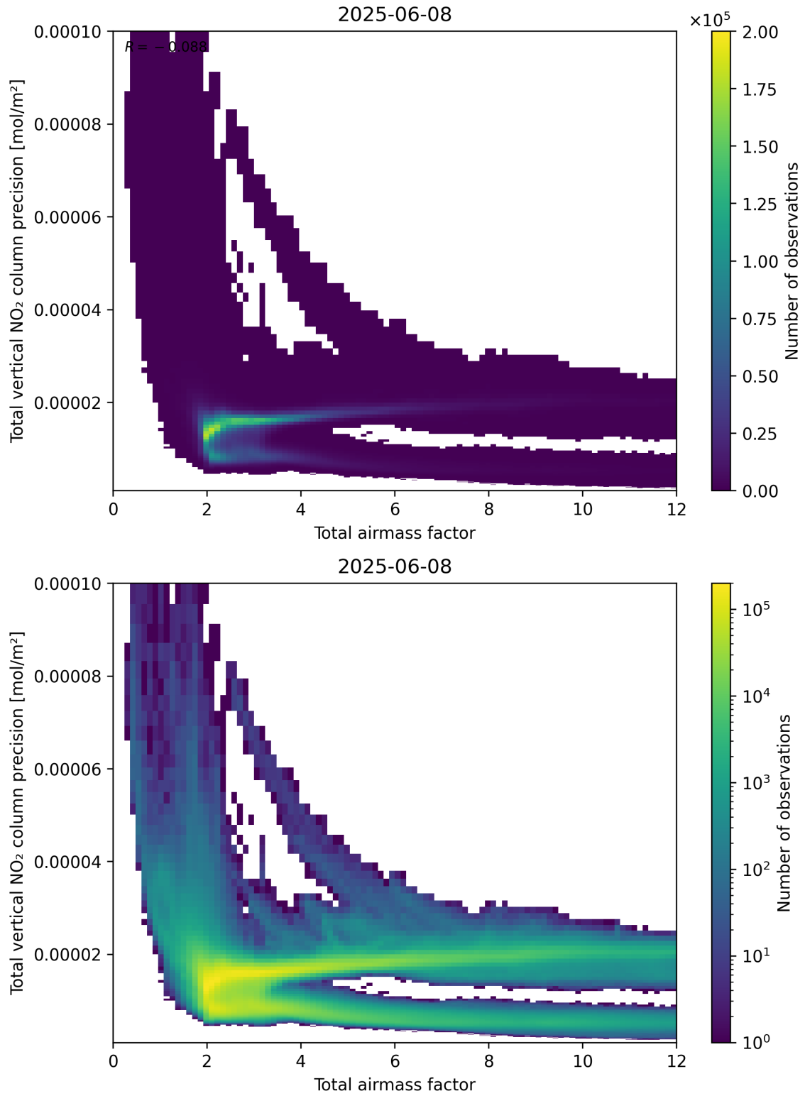
Figure 68: Scatter density plot of “Total airmass factor” against “Total vertical NO 2 column precision” for 2025-06-07 to 2025-06-09.
