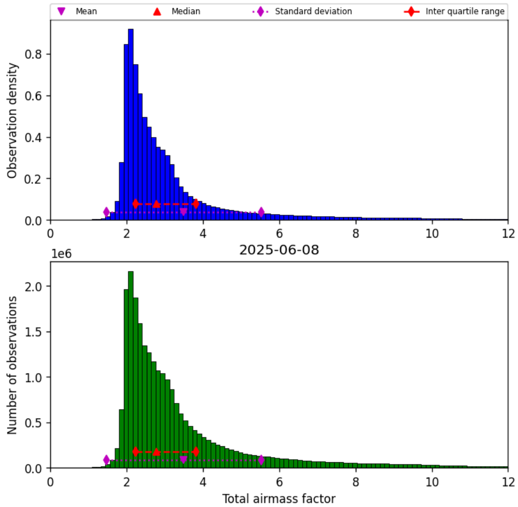
Figure 32: Histogram of “Total airmass factor” for 2025-06-07 to 2025-06-09
