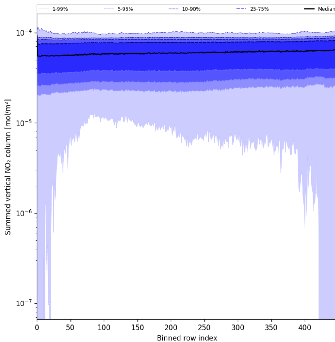
Figure 57: Along track statistics of “Summed vertical NO 2 column” for 2025-06-07 to 2025-06-09
