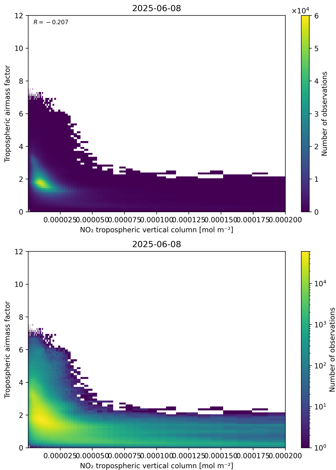
Figure 123: Scatter density plot of “NO 2 tropospheric vertical column” against “Tropospheric air mass factor” for 2025-06-07 to 2025-06-09.
