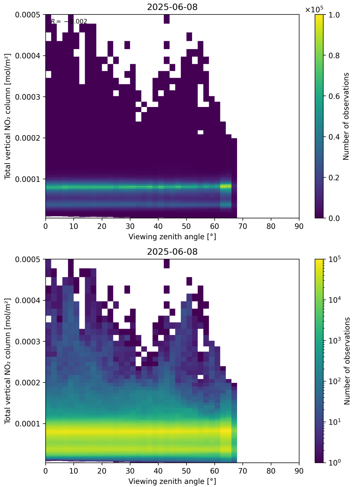
Figure 167: Scatter density plot of “Viewing zenith angle” against “Total vertical NO 2 column” for 2025-06-07 to 2025-06-09.
