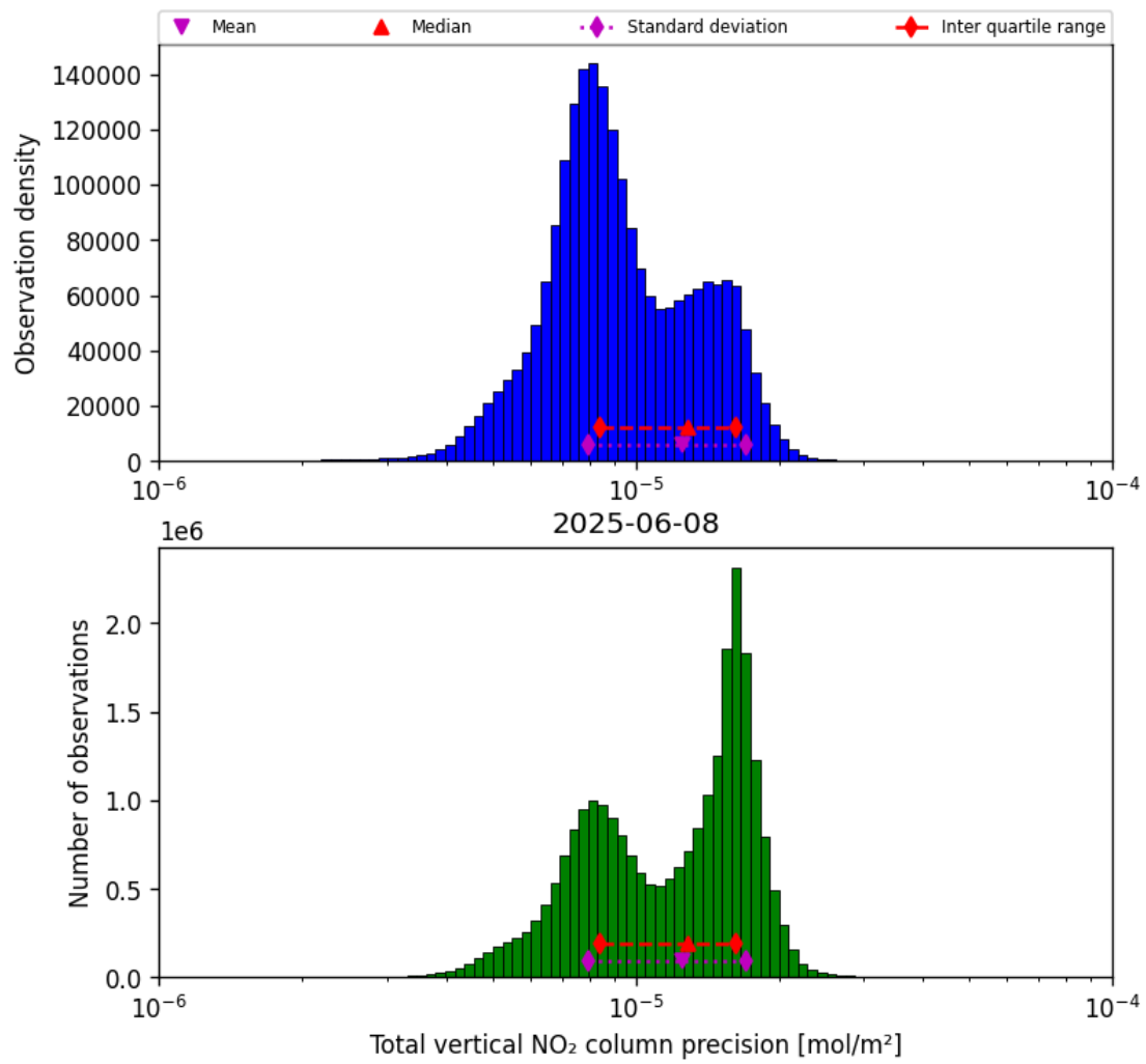
Figure 39: Histogram of “Total vertical NO 2 column precision” for 2025-06-07 to 2025-06-09
