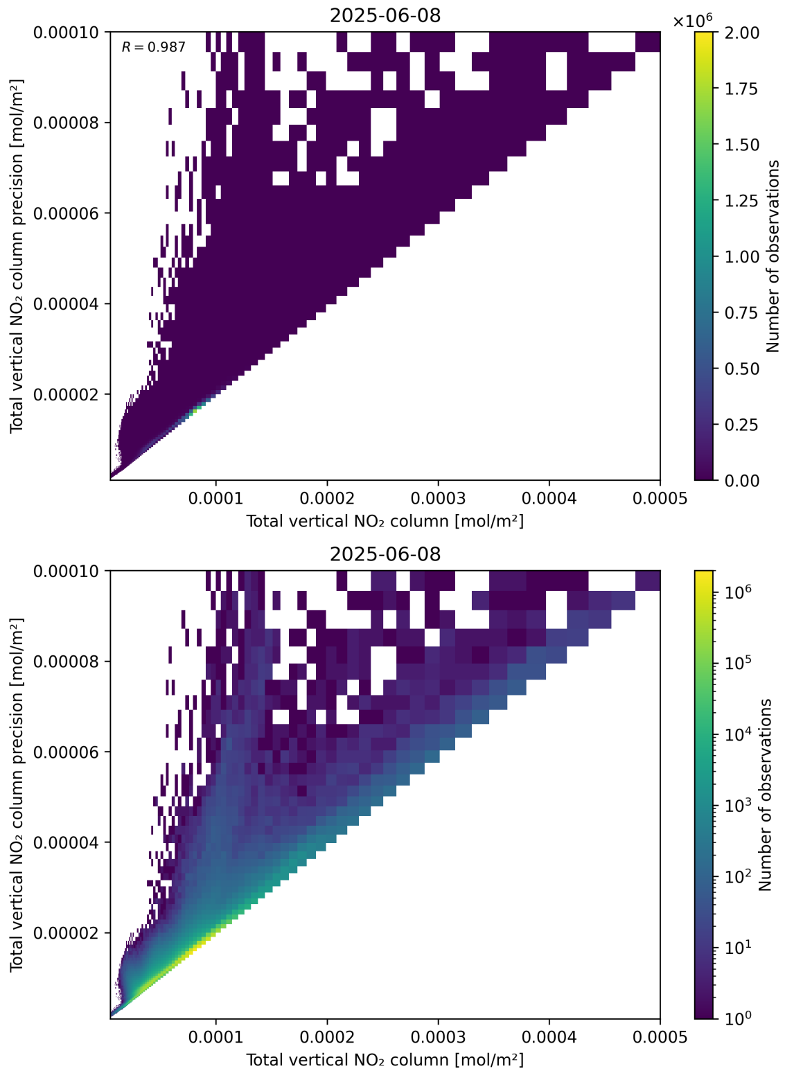
Figure 114: Scatter density plot of “Total vertical NO 2 column” against “Total vertical NO 2 column precision” for 2025-06-07 to 2025-06-09.
