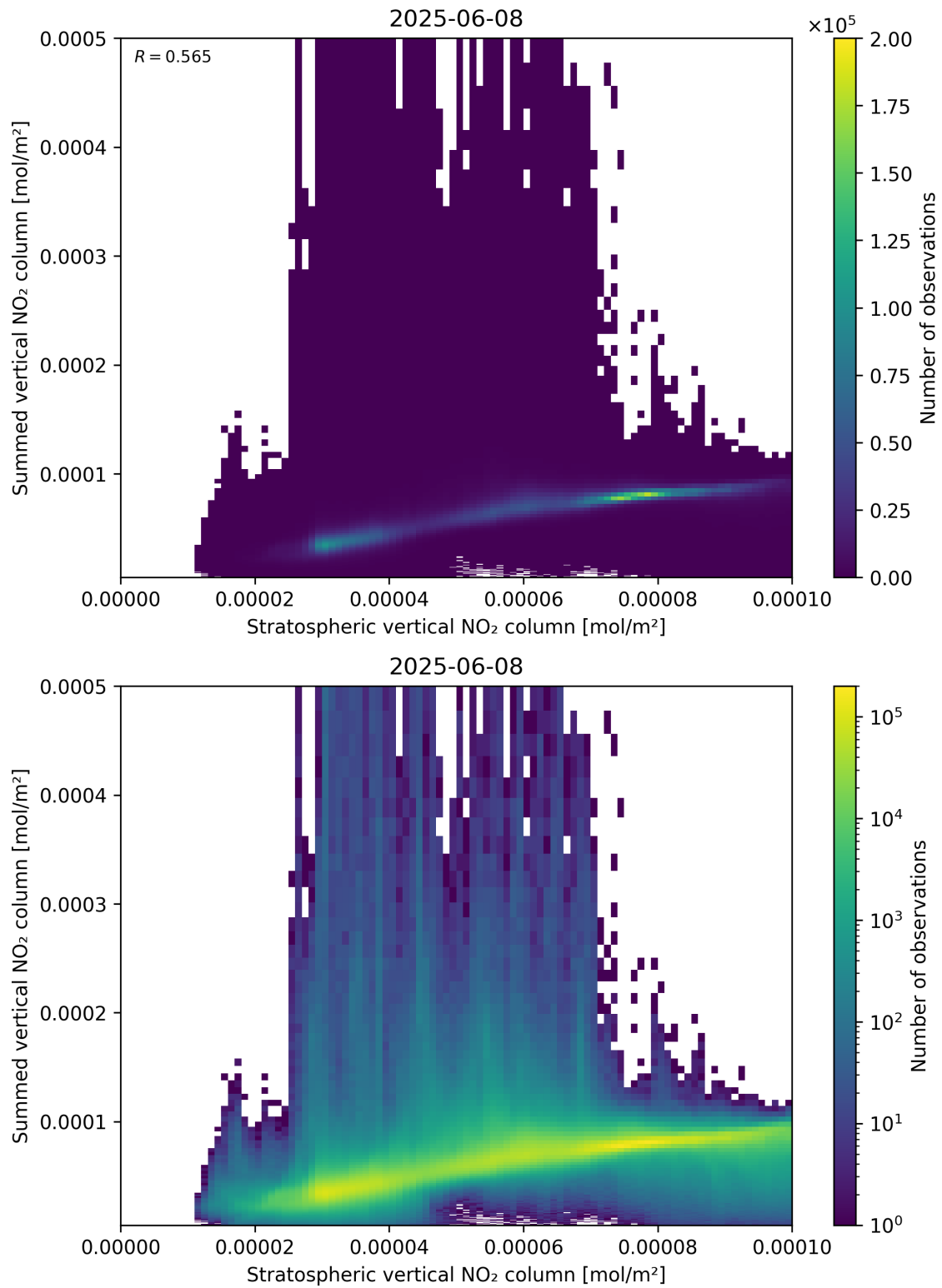
Figure 98: Scatter density plot of “Stratospheric vertical NO 2 column” against “Summed vertical NO 2 column” for 2025-06-07 to 2025-06-09.
