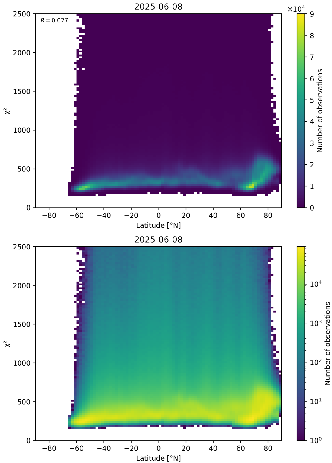
Figure 86: Scatter density plot of “Latitude” against “ \chi^2 ” for 2025-06-07 to 2025-06-09.
