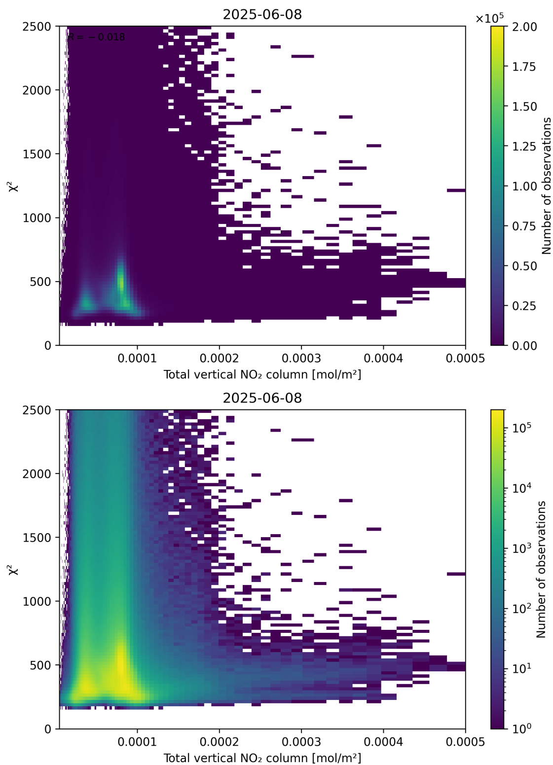
Figure 111: Scatter density plot of “Total vertical NO 2 column” against “ \chi^2 ” for 2025-06-07 to 2025-06-09.
