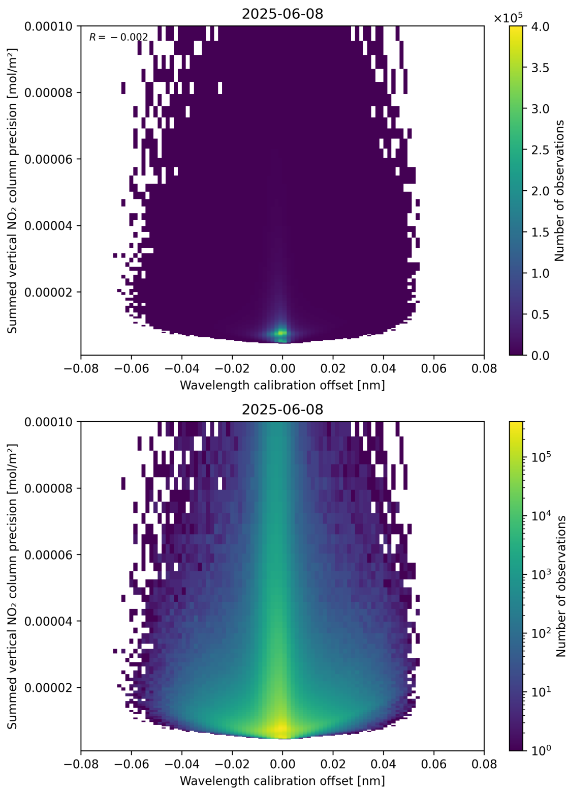
Figure 178: Scatter density plot of “Wavelength calibration offset” against “Summed vertical NO 2 column precision” for 2025-06-07 to 2025-06-09.
