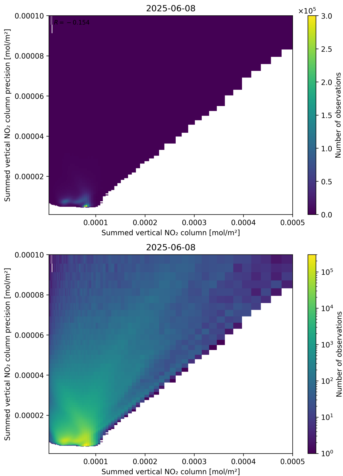
Figure 105: Scatter density plot of “Summed vertical NO 2 column” against “Summed vertical NO 2 column precision” for 2025-06-07 to 2025-06-09.
