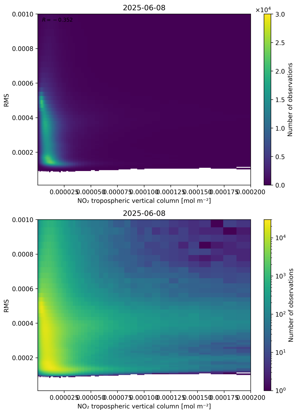
Figure 142: Scatter density plot of “NO 2 tropospheric vertical column” against “RMS” for 2025-06-07 to 2025-06-09.
