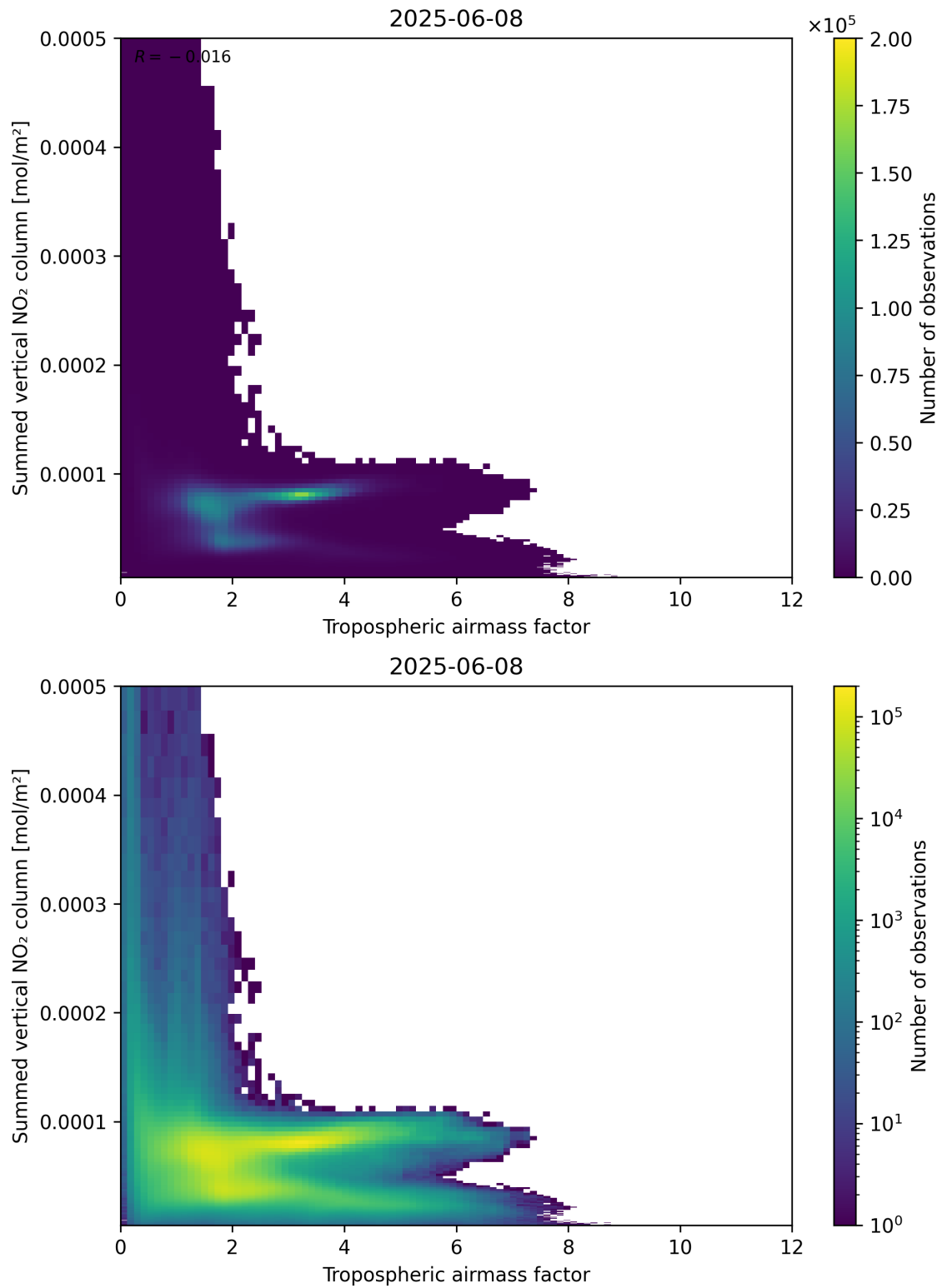
Figure 75: Scatter density plot of “Tropospheric airmass factor” against “Summed vertical NO 2 column” for 2025-06-07 to 2025-06-09.
