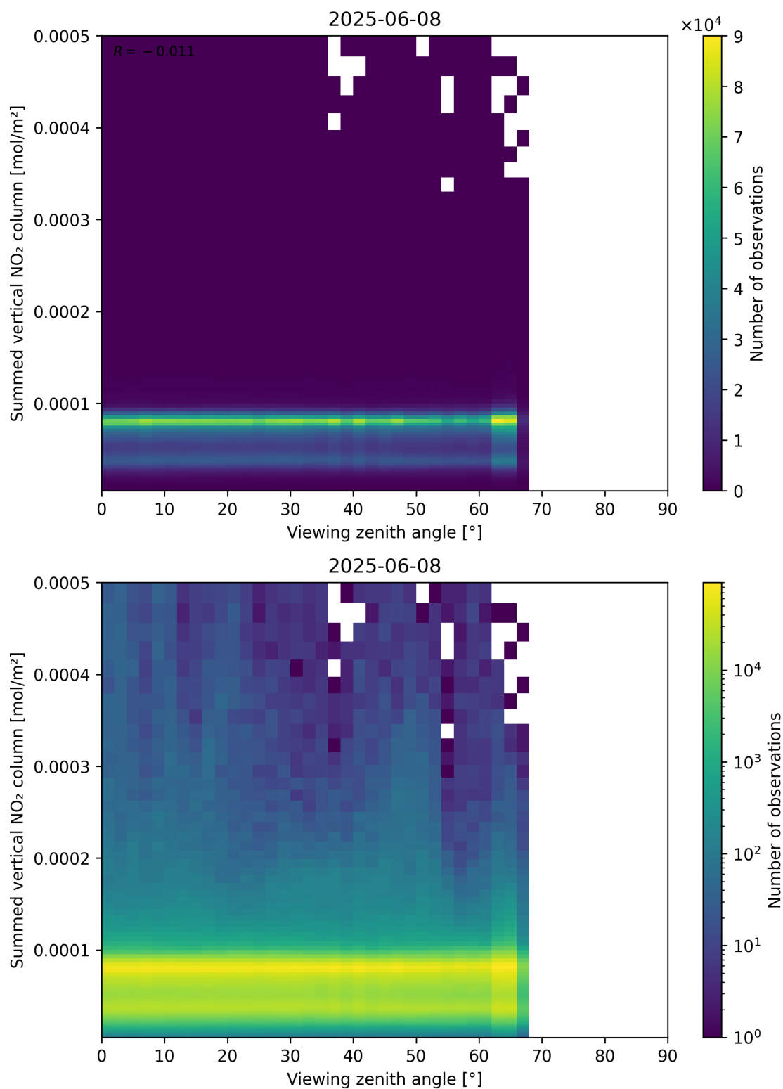
Figure 165: Scatter density plot of “Viewing zenith angle” against “Summed vertical NO 2 column” for 2025-06-07 to 2025-06-09.
