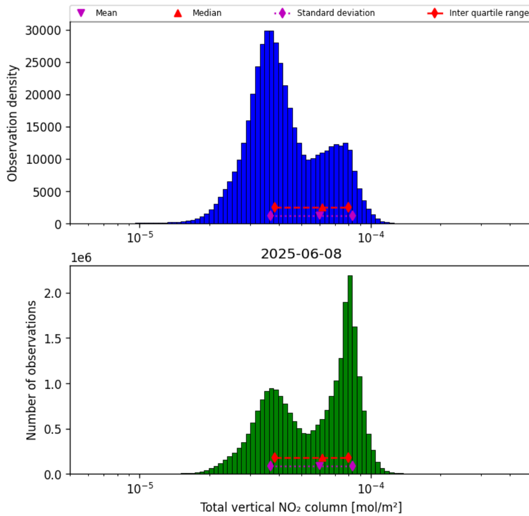
Figure 38: Histogram of “Total vertical NO 2 column” for 2025-06-07 to 2025-06-09
