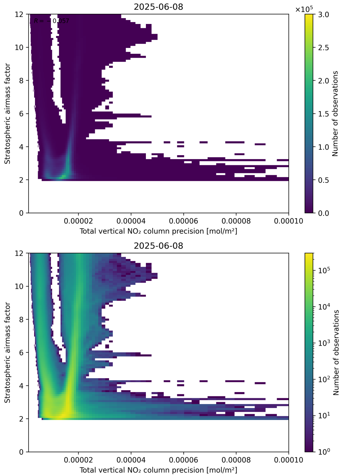
Figure 115: Scatter density plot of “Total vertical NO 2 column precision” against “Stratospheric air mass factor” for 2025-06-07 to 2025-06-09.
