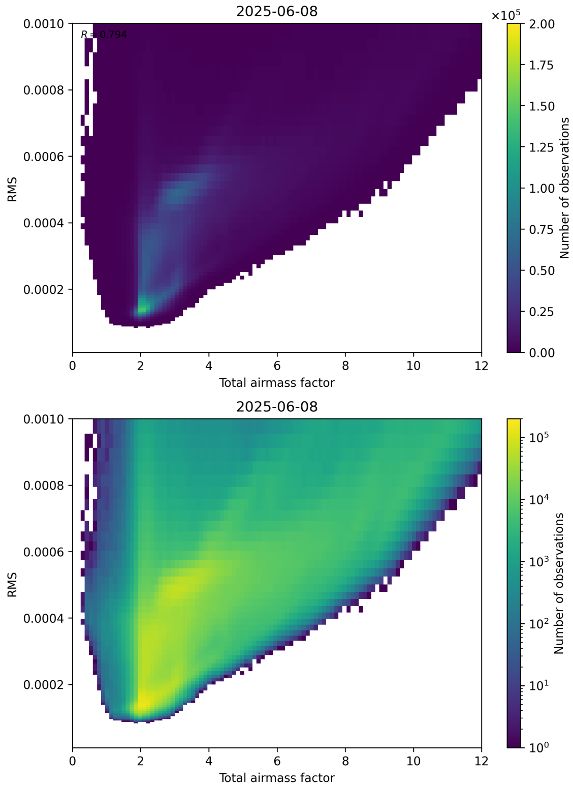
Figure 69: Scatter density plot of “Total airmass factor” against “RMS” for 2025-06-07 to 2025-06-09.
