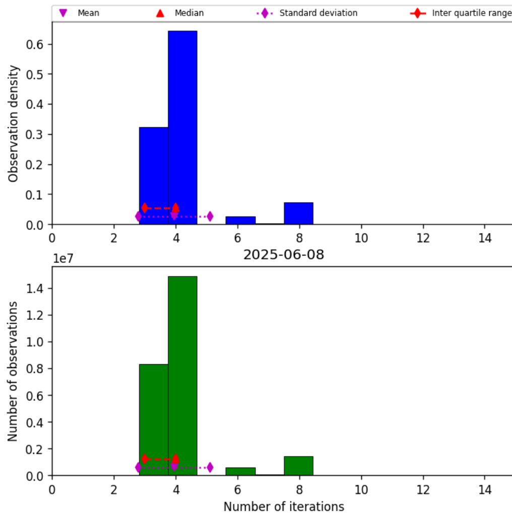
Figure 34: Histogram of “Number of iterations” for 2025-06-07 to 2025-06-09
