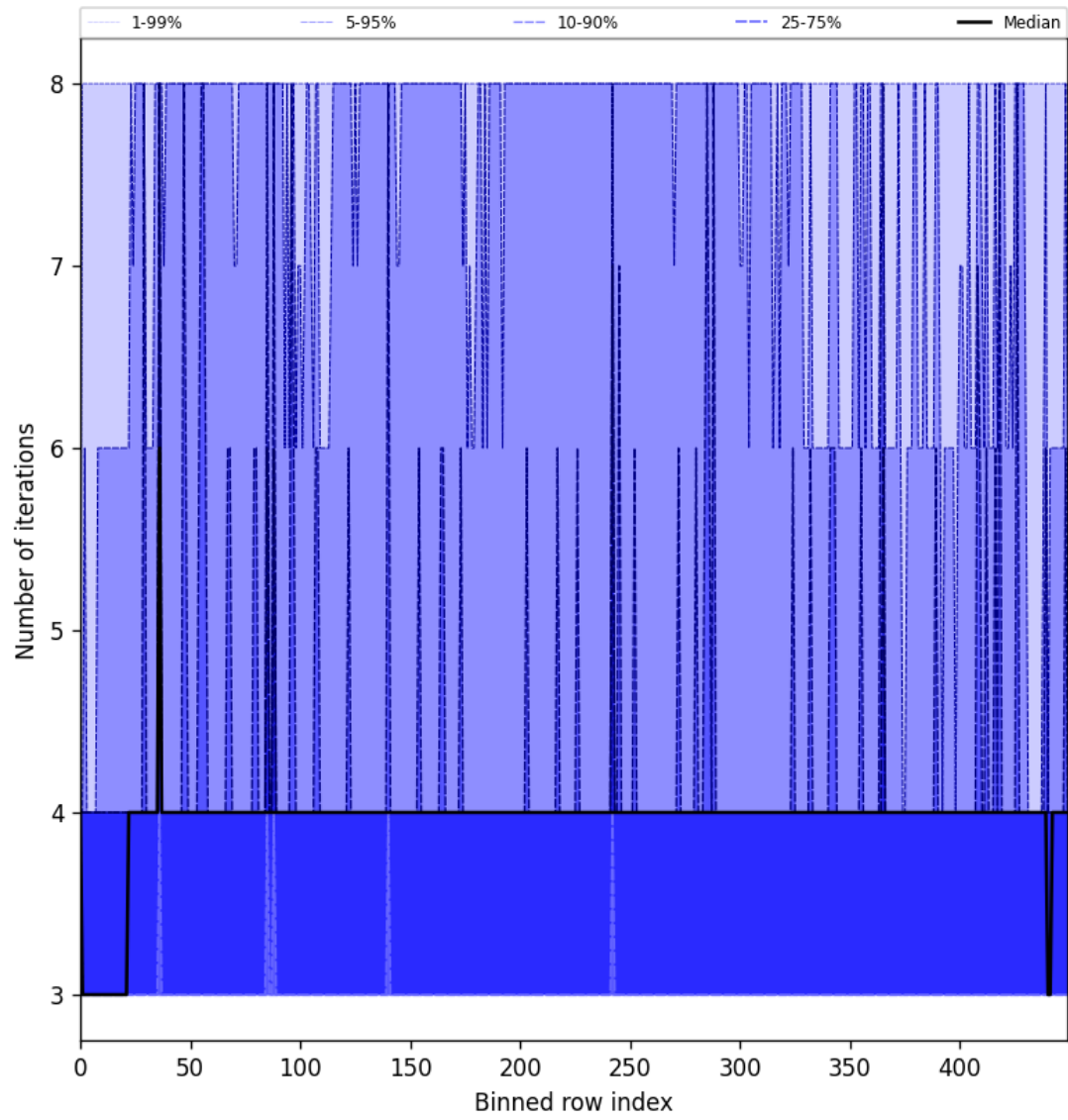
Figure 51: Along track statistics of “Number of iterations” for 2025-06-07 to 2025-06-09
