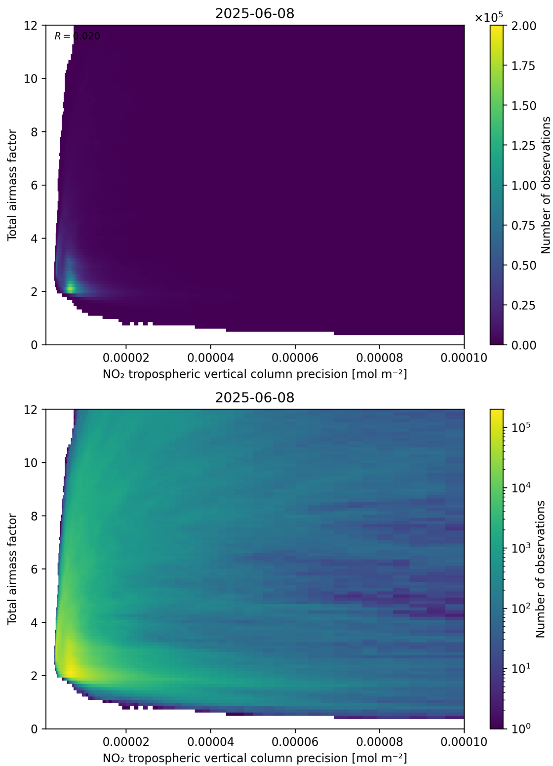
Figure 132: Scatter density plot of “NO 2 tropospheric vertical column precision” against “Total air mass factor” for 2025-06-07 to 2025-06-09.
