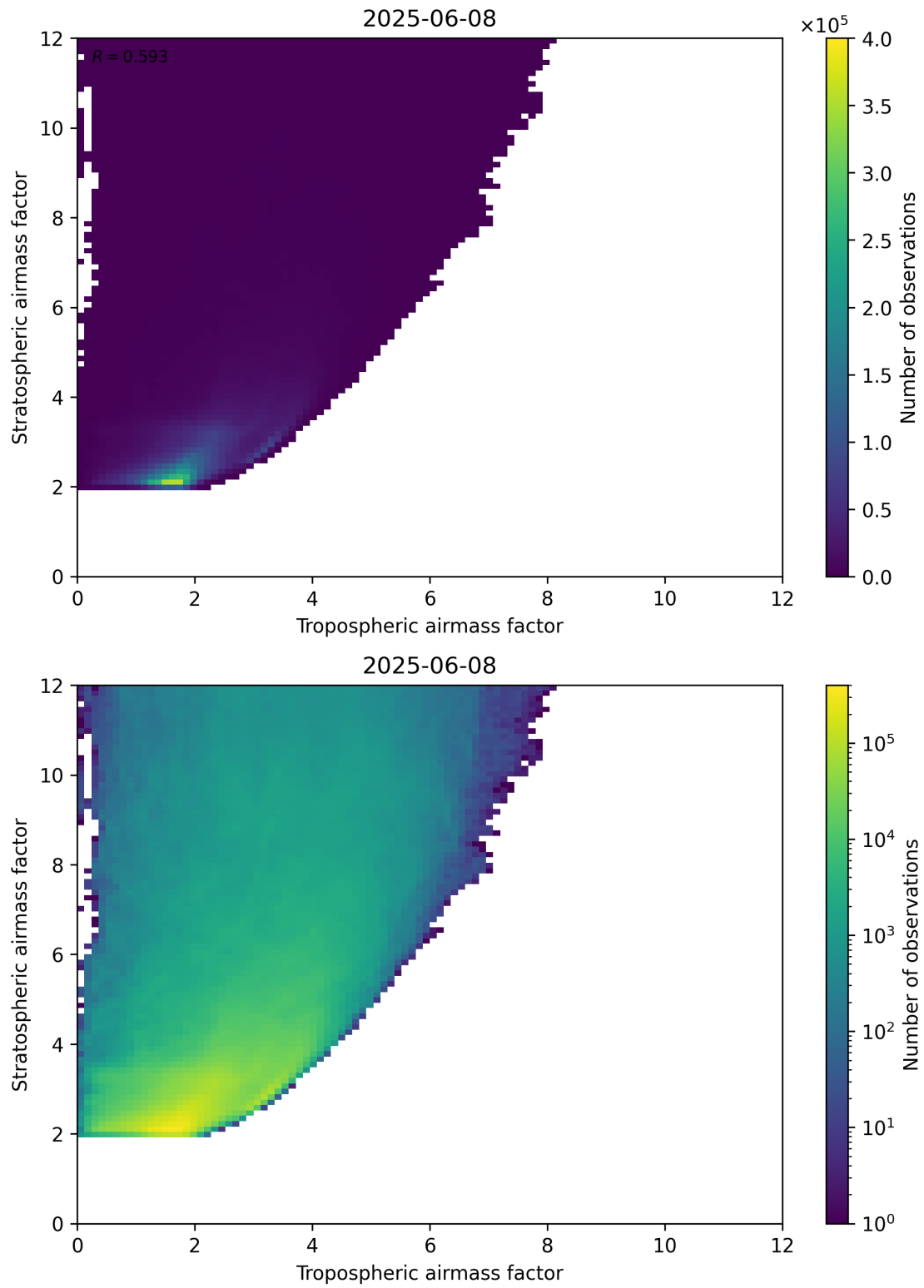
Figure 71: Scatter density plot of “Tropospheric airmass factor” against “Stratospheric airmass factor” for 2025-06-07 to 2025-06-09.
