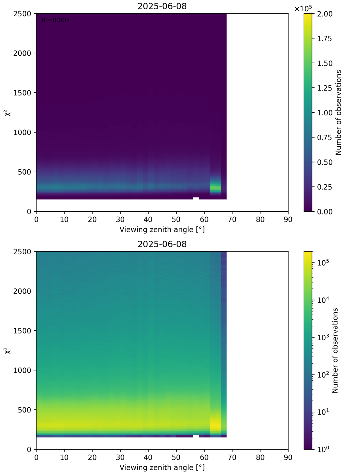
Figure 162: Scatter density plot of “Viewing zenith angle” against “ \chi^2 ” for 2025-06-07 to 2025-06-09.
