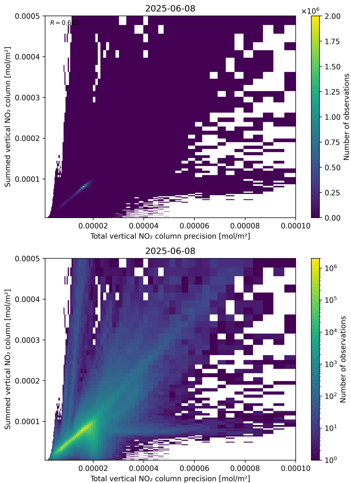
Figure 117: Scatter density plot of “Total vertical NO 2 column precision” against “Summed vertical NO 2 column” for 2025-06-07 to 2025-06-09.
