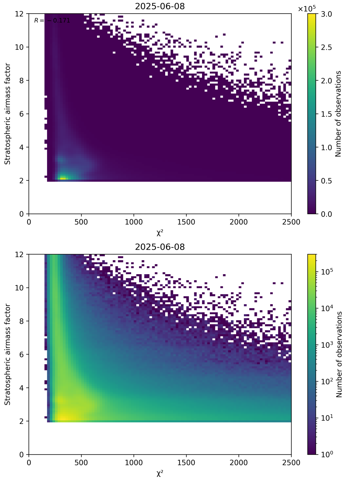
Figure 81: Scatter density plot of “ \chi^2 ” against “Stratospheric airmass factor” for 2025-06-07 to 2025-06-09.
