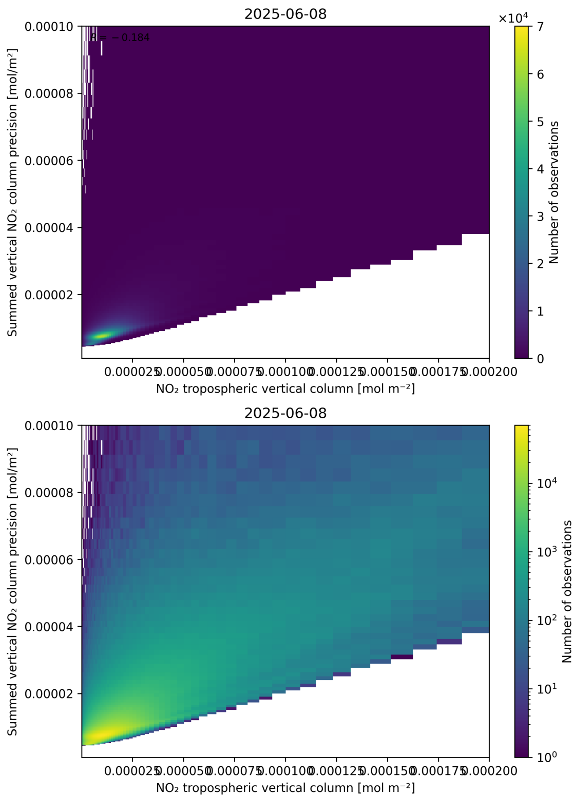
Figure 127: Scatter density plot of “NO 2 tropospheric vertical column” against “Summed vertical NO 2 column precision” for 2025-06-07 to 2025-06-09.
