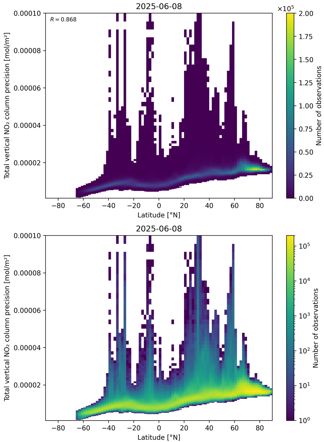
Figure 91: Scatter density plot of “Latitude” against “Total vertical NO 2 column precision” for 2025-06-07 to 2025-06-09.
