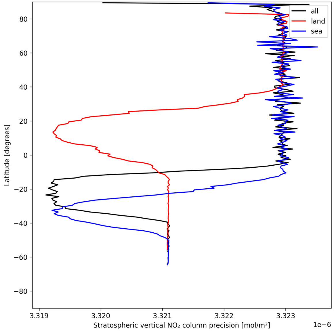
Figure 20: Zonal average of “Stratospheric vertical NO 2 column precision” for 2025-06-07 to 2025-06-09.
