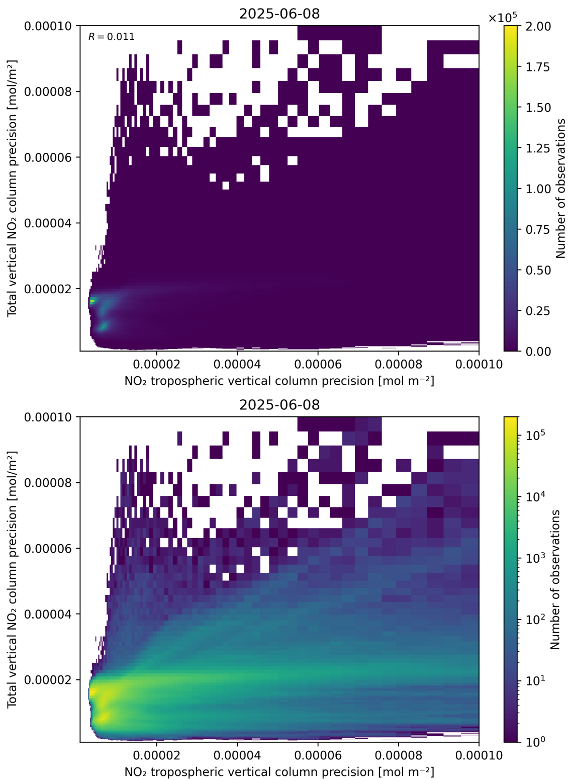
Figure 139: Scatter density plot of “NO 2 tropospheric vertical column precision” against “Total vertical NO 2 column precision” for 2025-06-07 to 2025-06-09.
