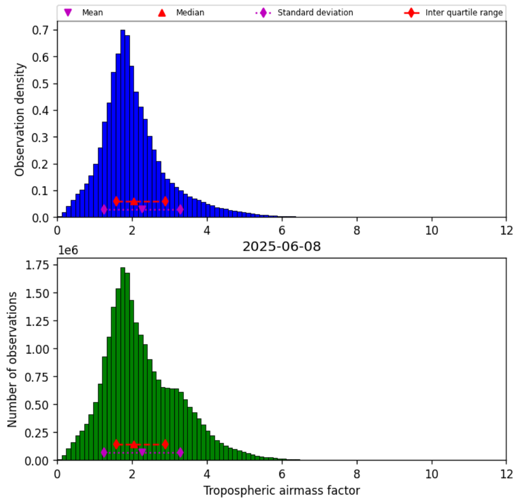
Figure 31: Histogram of “Tropospheric airmass factor” for 2025-06-07 to 2025-06-09
