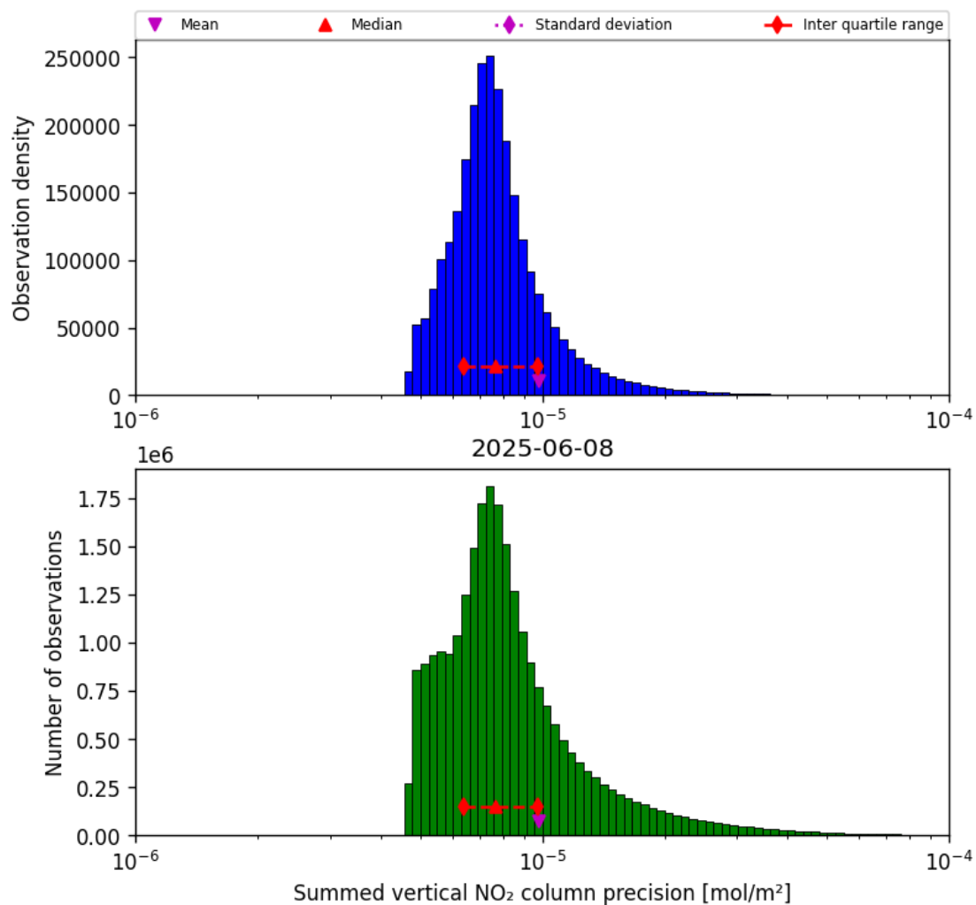
Figure 41: Histogram of "Summed vertical NO 2 column precision" for 2025-06-07 to 2025-06-09
