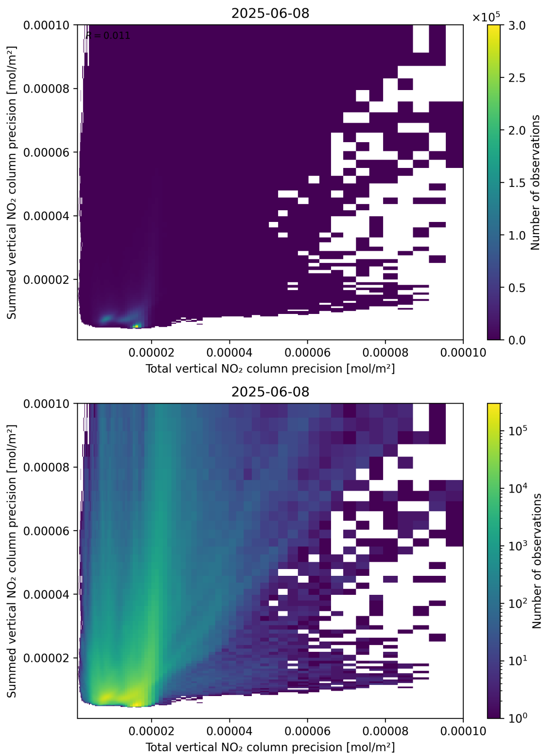
Figure 118: Scatter density plot of “Total vertical NO 2 column precision” against “Summed vertical NO 2 column precision” for 2025-06-07 to 2025-06-09.
