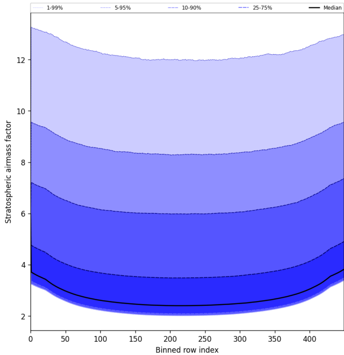
Figure 61: Along track statistics of “Stratospheric airmass factor” for 2025-06-07 to 2025-06-09
