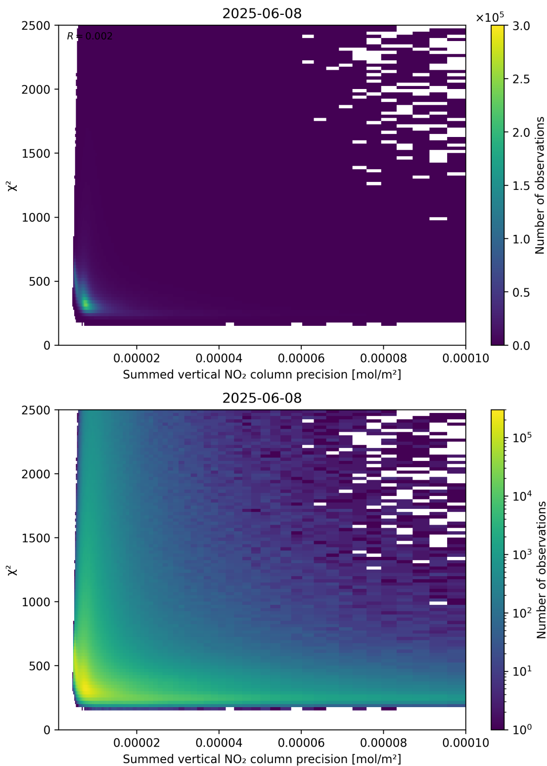
Figure 107: Scatter density plot of “Summed vertical NO 2 column precision” against “ \chi^2 ” for 2025-06-07 to 2025-06-09.
