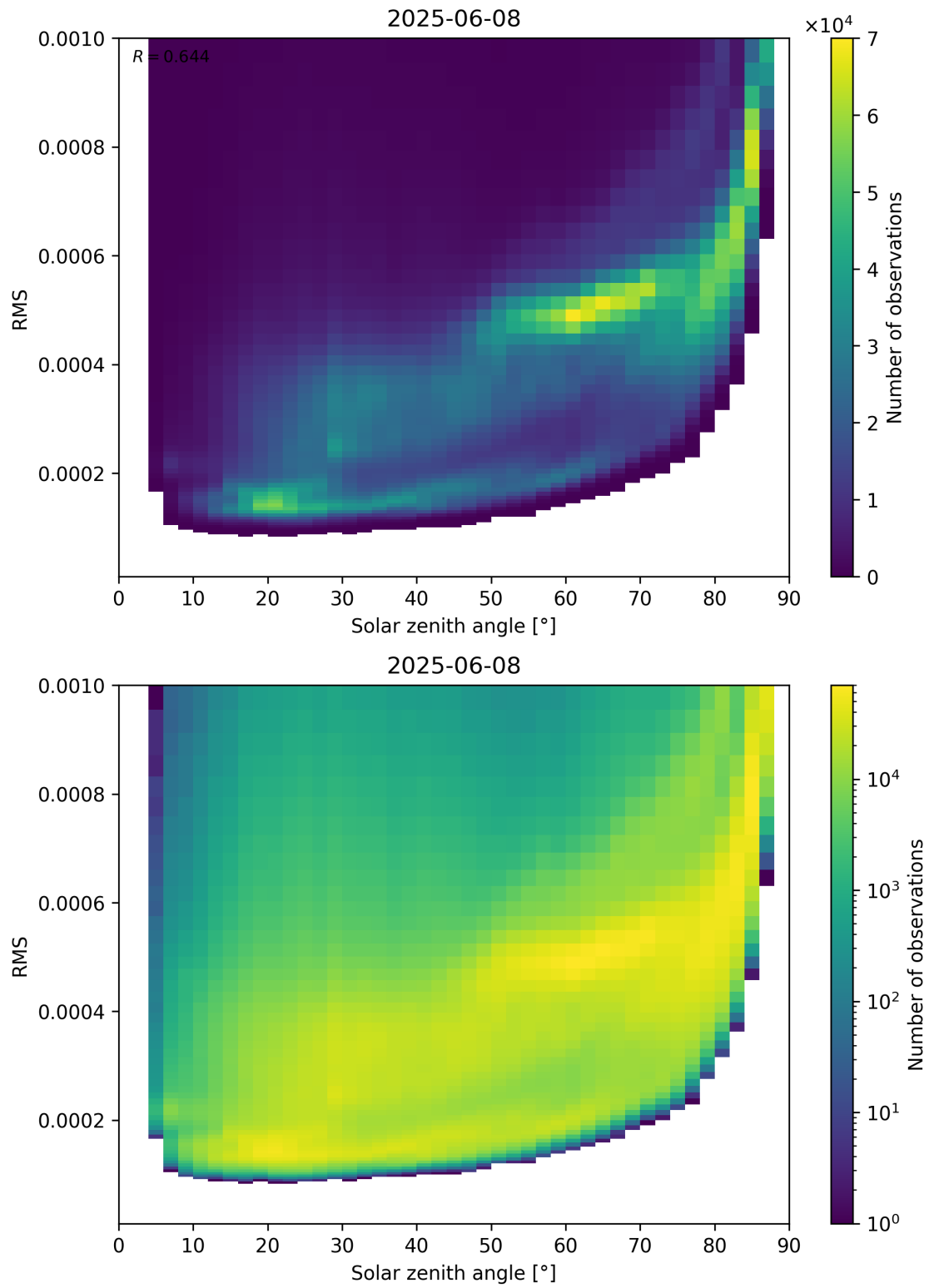
Figure 157: Scatter density plot of “Solar zenith angle” against “RMS” for 2025-06-07 to 2025-06-09.
