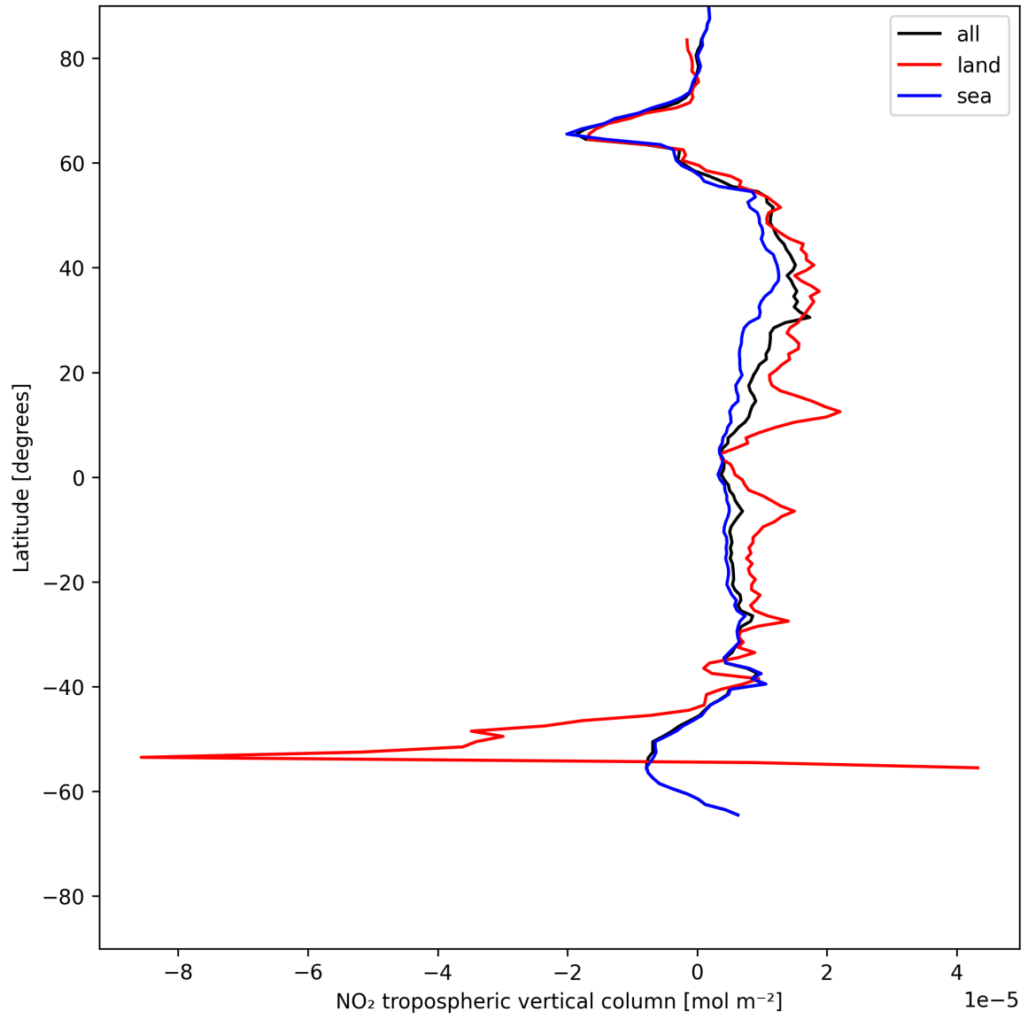
Figure 12: Zonal average of “NO 2 tropospheric vertical column” for 2025-06-07 to 2025-06-09.
