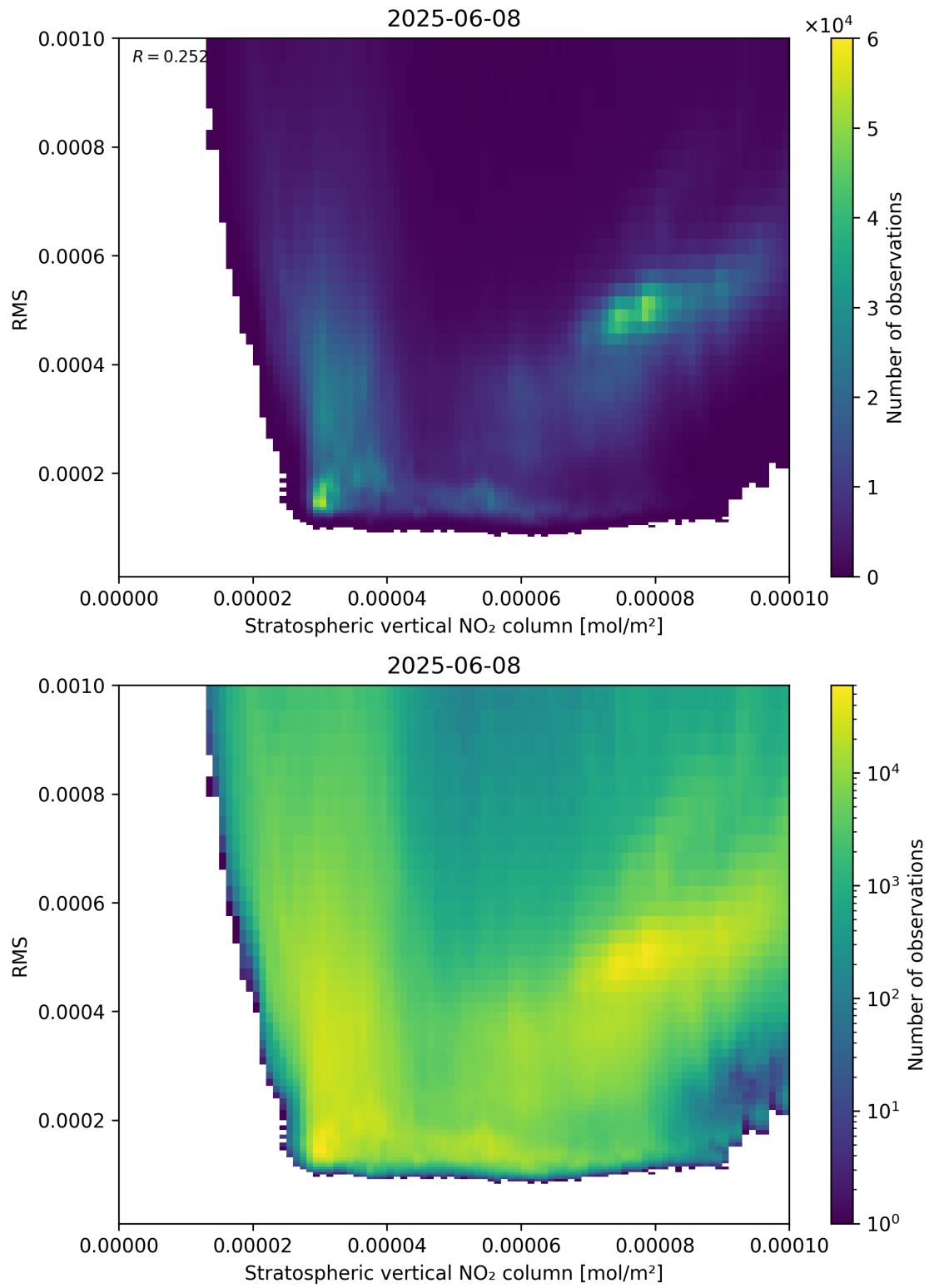
Figure 102: Scatter density plot of “Stratospheric vertical NO 2 column” against “RMS” for 2025-06-07 to 2025-06-09.
