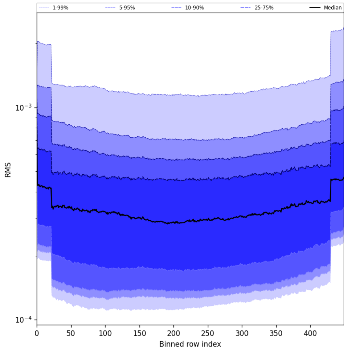
Figure 60: Along track statistics of “RMS” for 2025-06-07 to 2025-06-09
