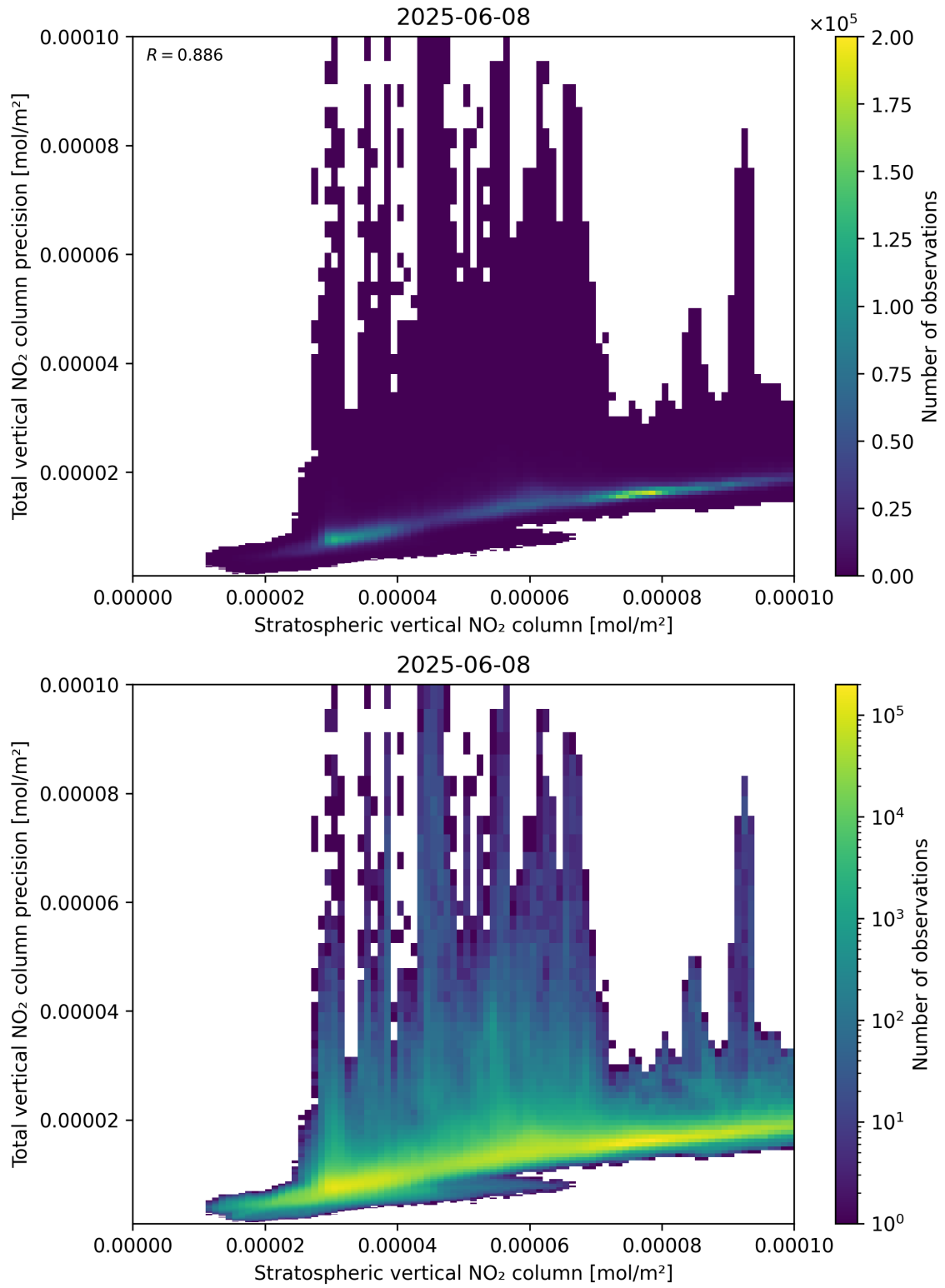
Figure 101: Scatter density plot of “Stratospheric vertical NO 2 column” against “Total vertical NO 2 column precision” for 2025-06-07 to 2025-06-09.
