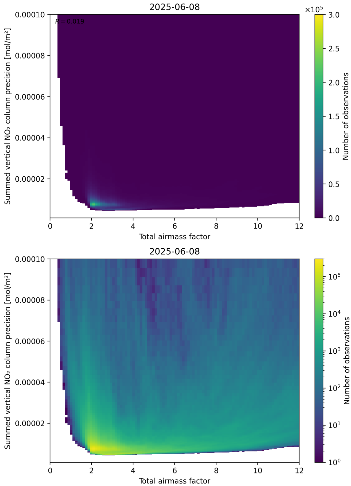
Figure 66: Scatter density plot of “Total airmass factor” against “Summed vertical NO 2 column precision” for 2025-06-07 to 2025-06-09.
