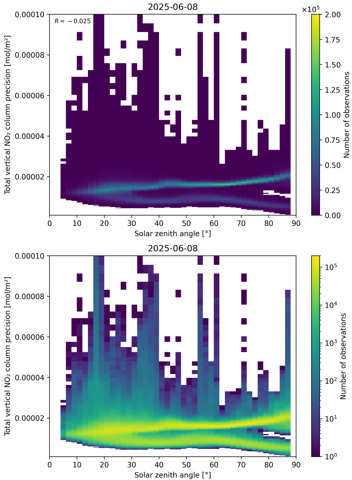
Figure 154: Scatter density plot of “Solar zenith angle” against “Total vertical NO 2 column precision” for 2025-06-07 to 2025-06-09.
