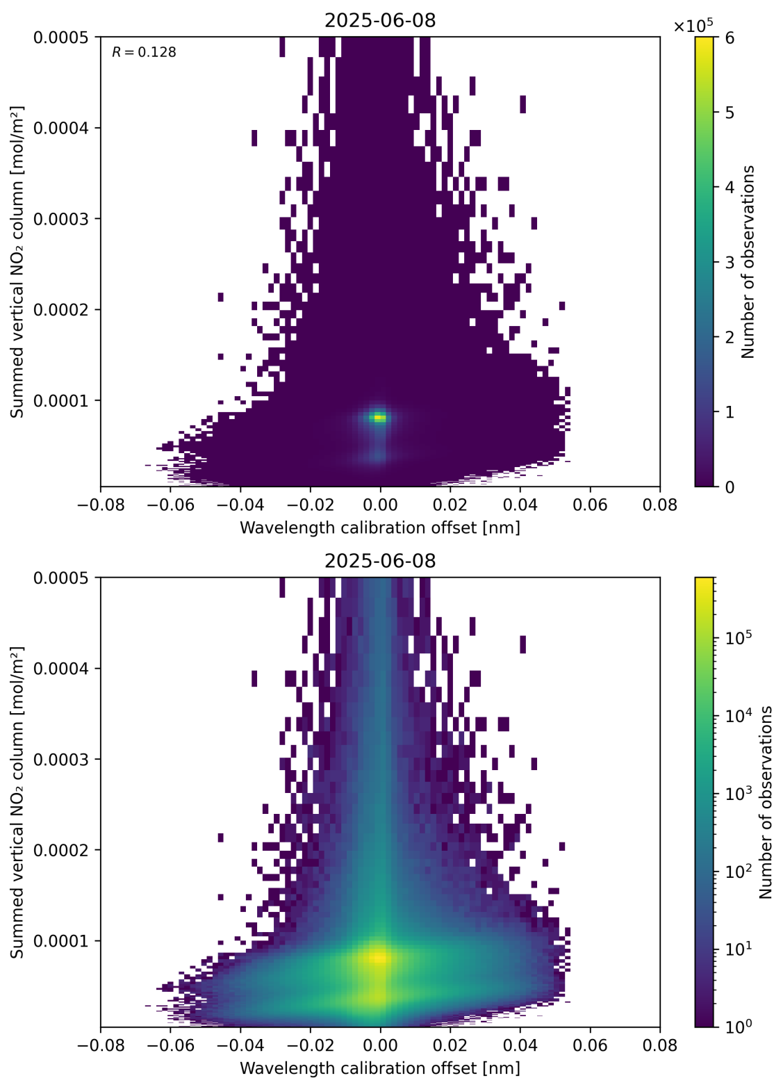
Figure 177: Scatter density plot of “Wavelength calibration offset” against “Summed vertical NO 2 column” for 2025-06-07 to 2025-06-09.
