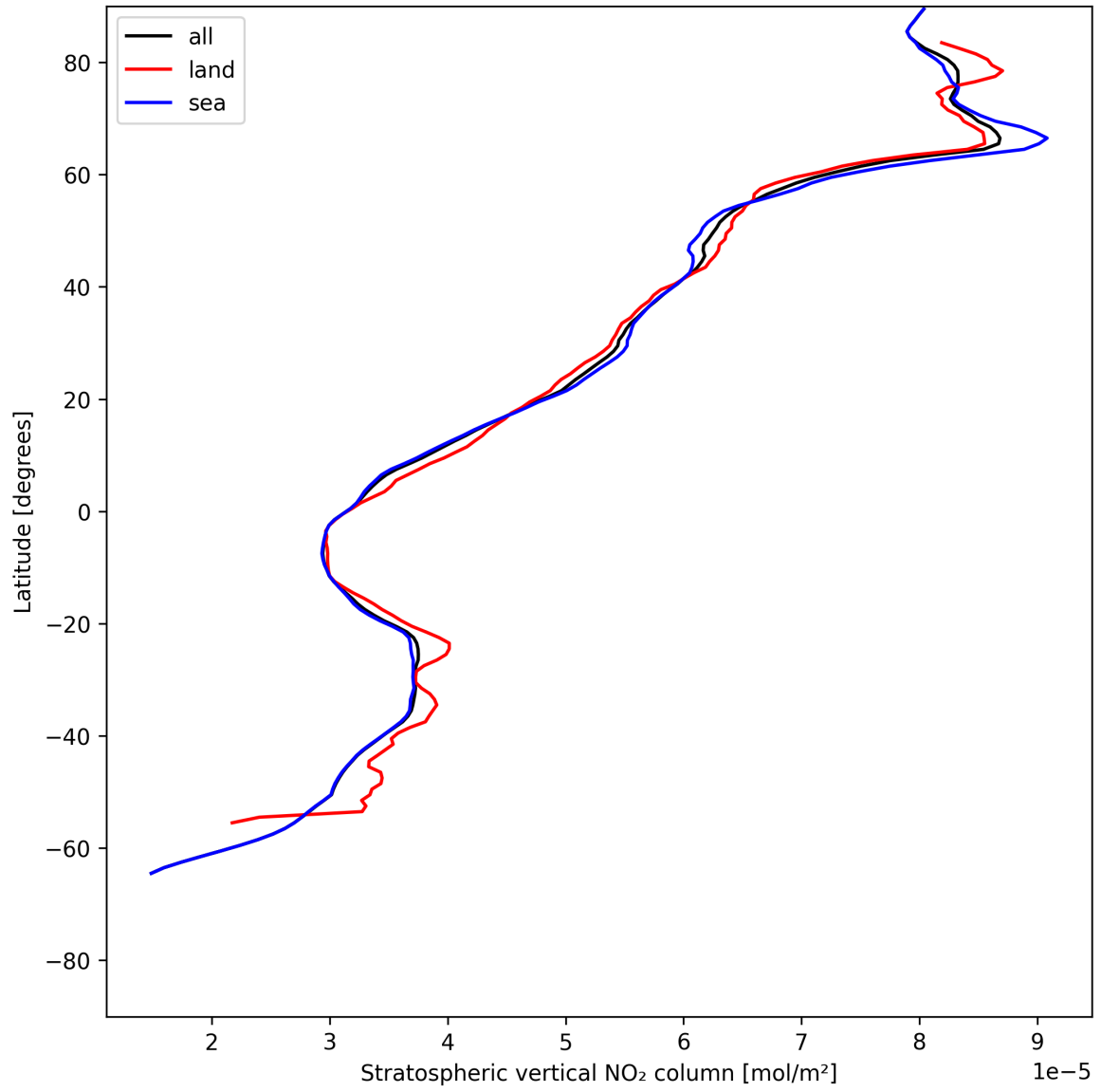
Figure 19: Zonal average of “Stratospheric vertical NO 2 column” for 2025-06-07 to 2025-06-09.
