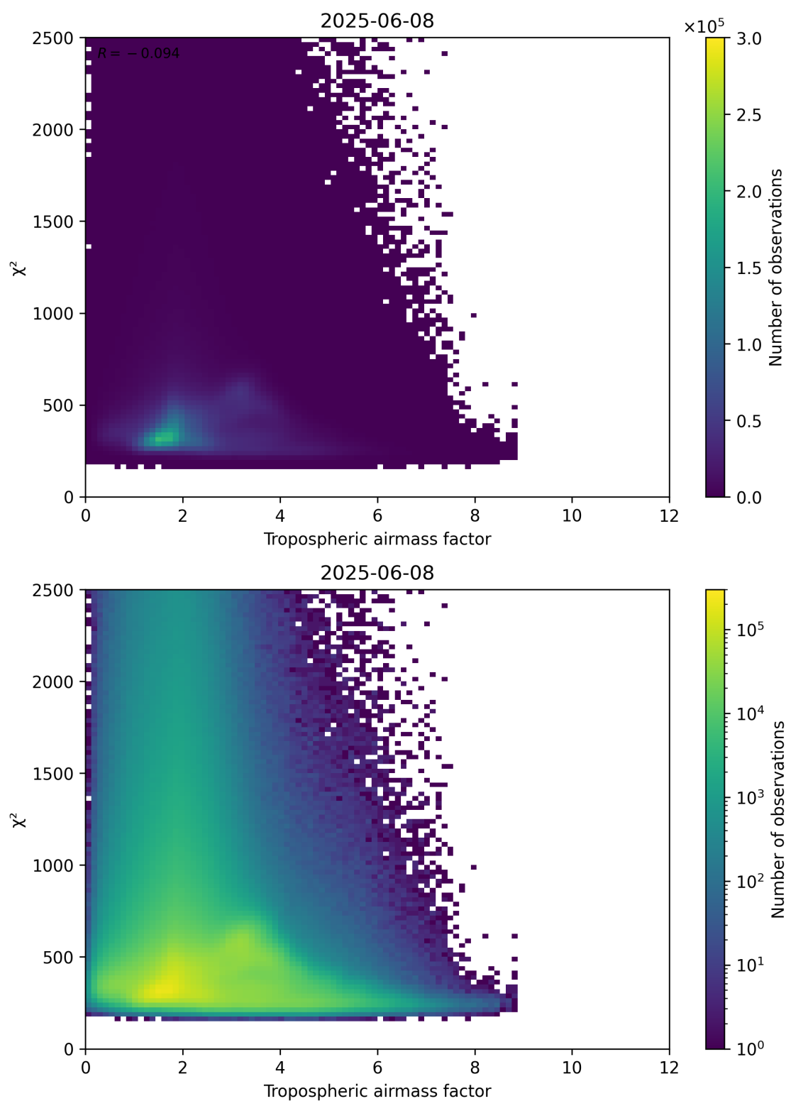
Figure 73: Scatter density plot of “Tropospheric airmass factor” against “ \chi^2 ” for 2025-06-07 to 2025-06-09.
