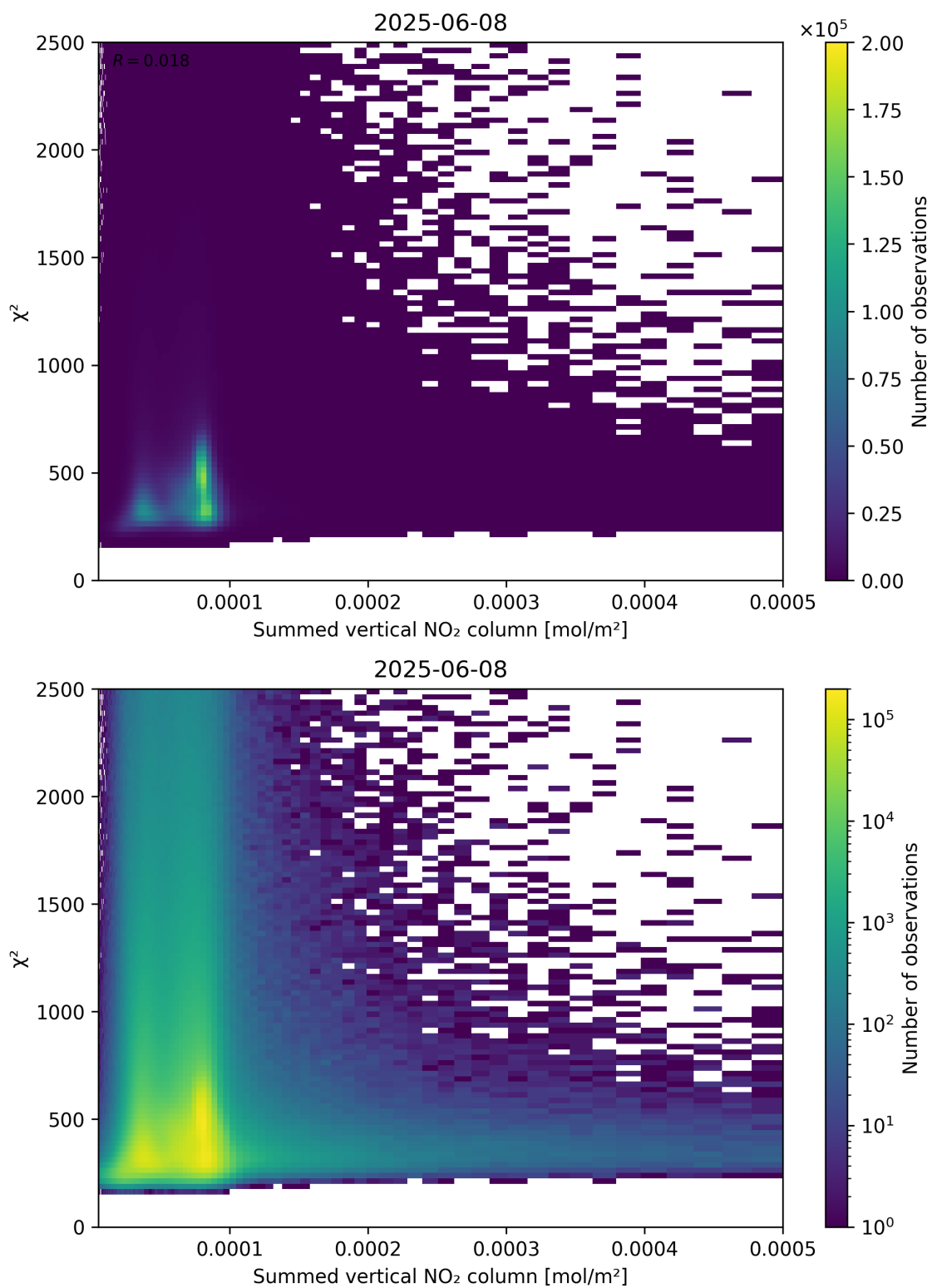
Figure 104: Scatter density plot of “Summed vertical NO 2 column” against “ \chi^2 ” for 2025-06-07 to 2025-06-09.
