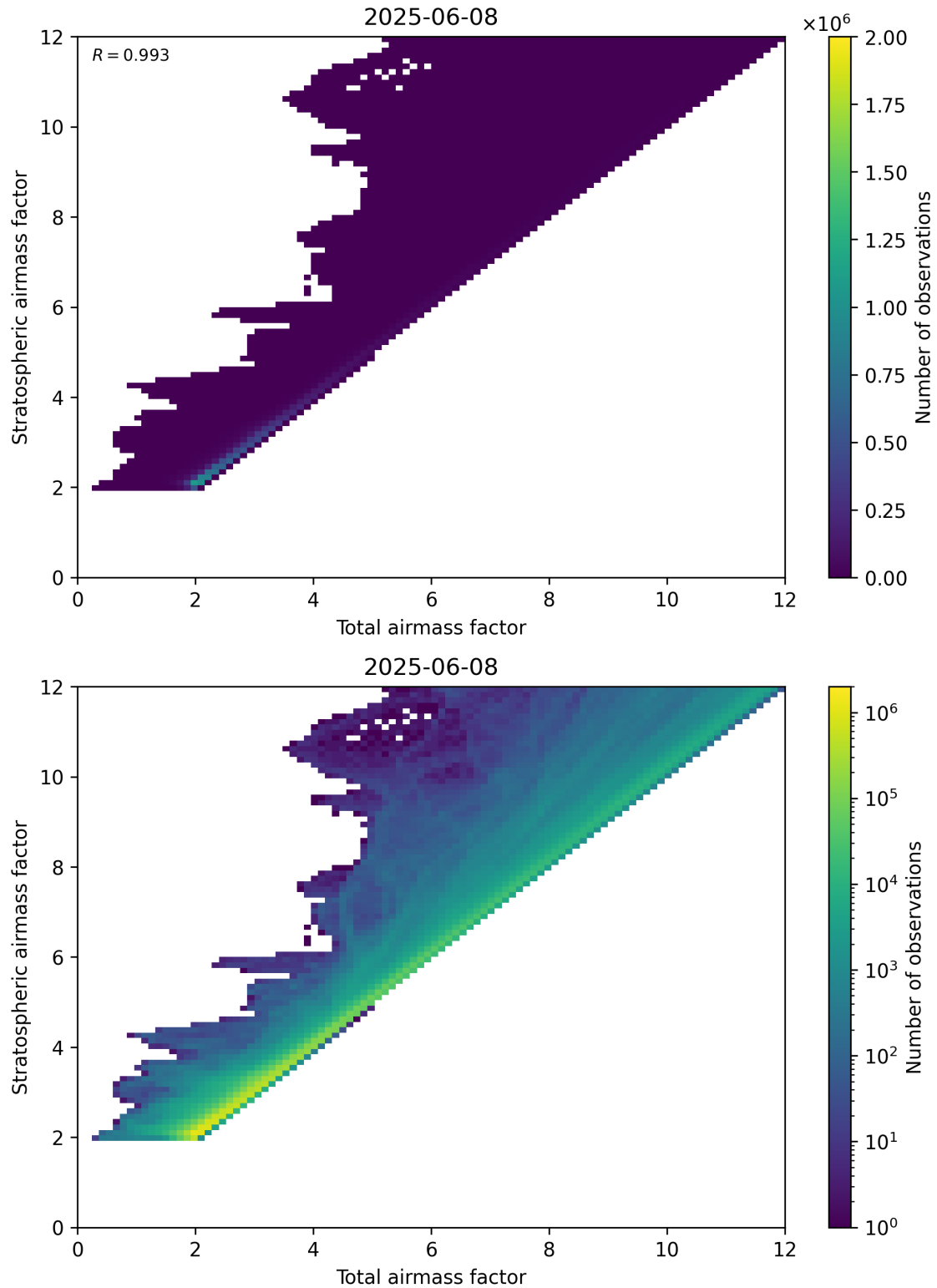
Figure 62: Scatter density plot of “Total airmass factor” against “Stratospheric airmass factor” for 2025-06-07 to 2025-06-09.
