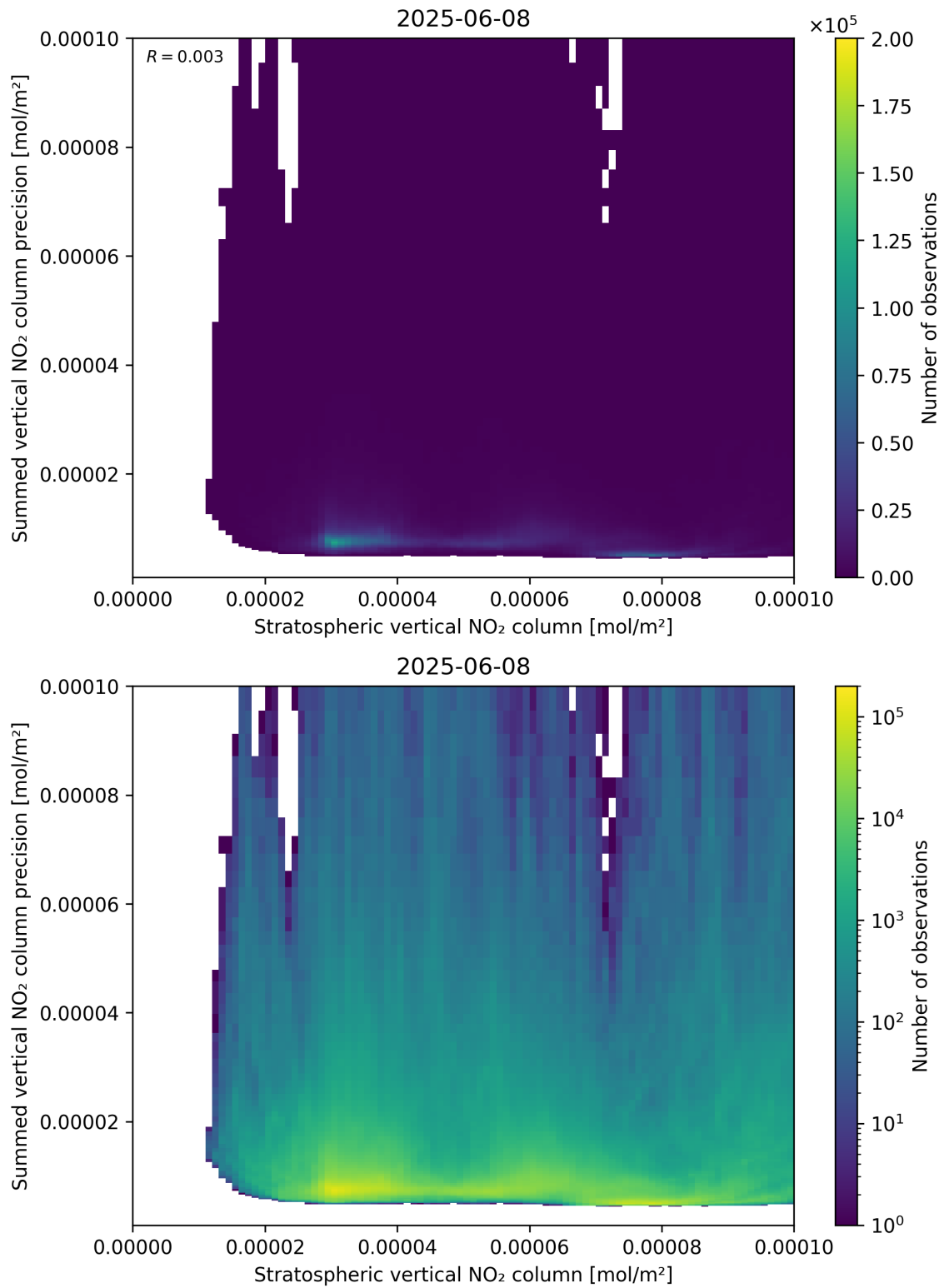
Figure 99: Scatter density plot of “Stratospheric vertical NO 2 column” against “Summed vertical NO 2 column precision” for 2025-06-07 to 2025-06-09.
