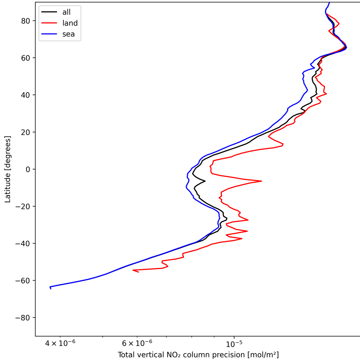
Figure 22: Zonal average of “Total vertical NO 2 column precision” for 2025-06-07 to 2025-06-09.
