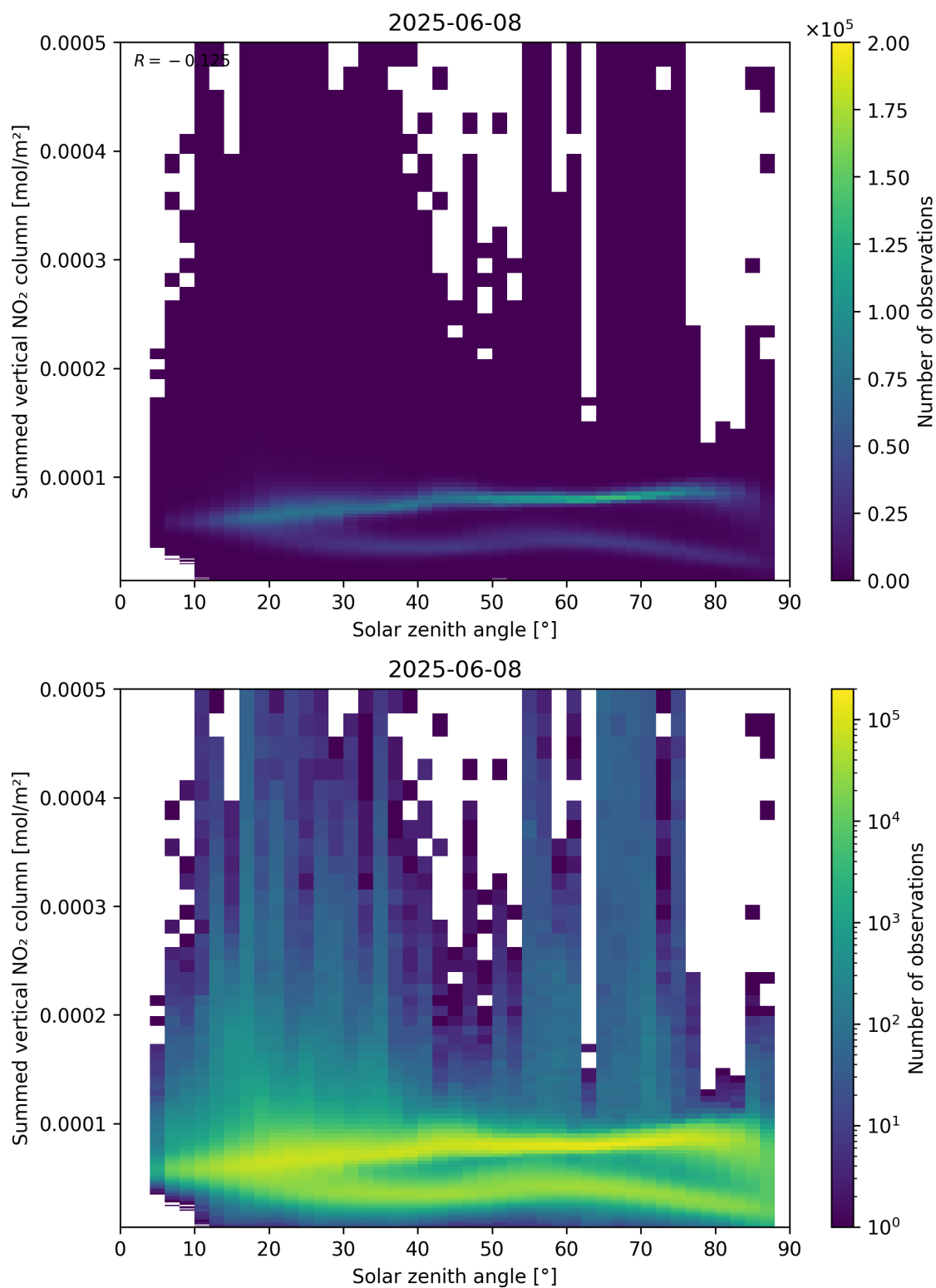
Figure 151: Scatter density plot of “Solar zenith angle” against “Summed vertical NO 2 column” for 2025-06-07 to 2025-06-09.
