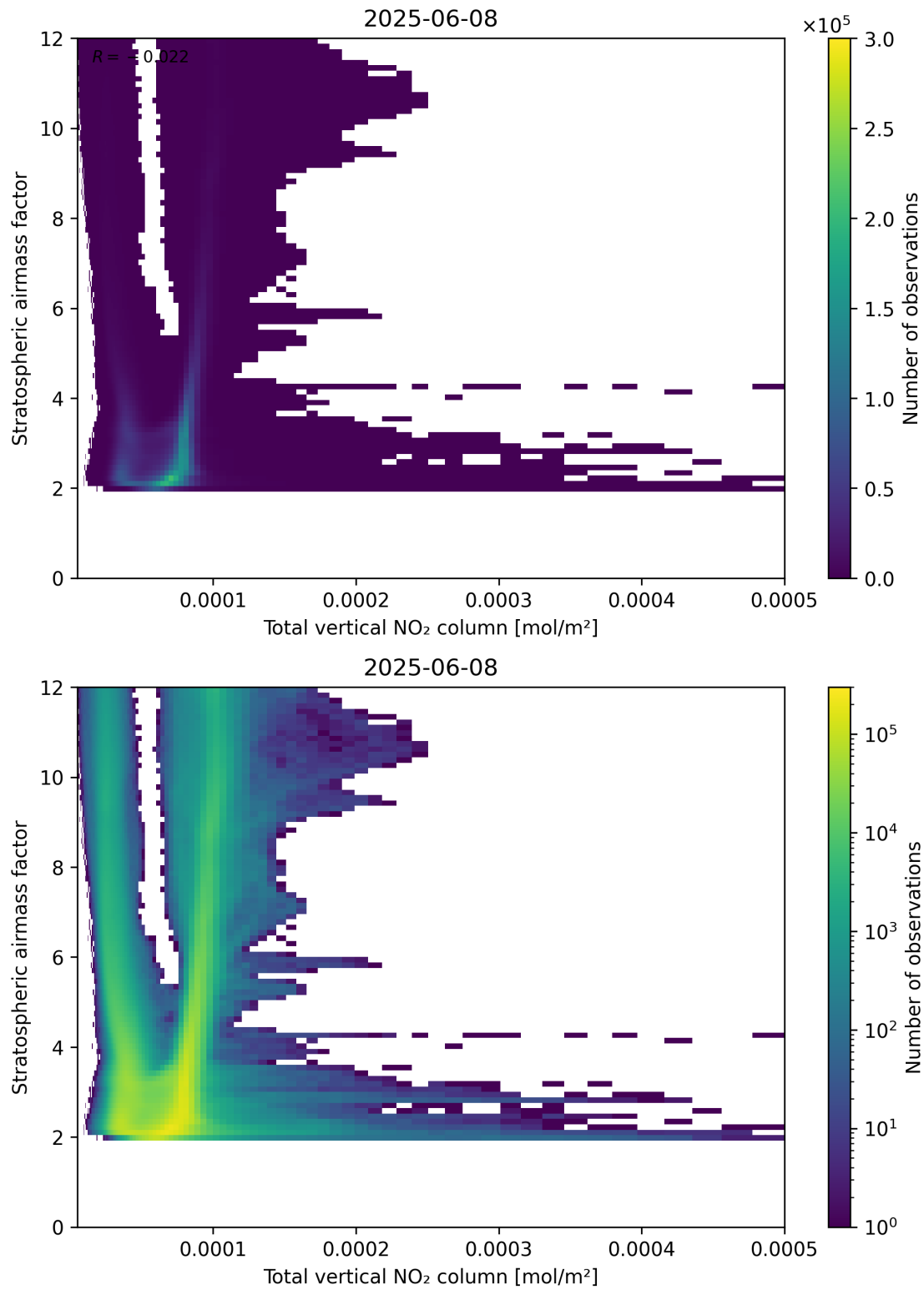
Figure 110: Scatter density plot of “Total vertical NO 2 column” against “Stratospheric airmass factor” for 2025-06-07 to 2025-06-09.
