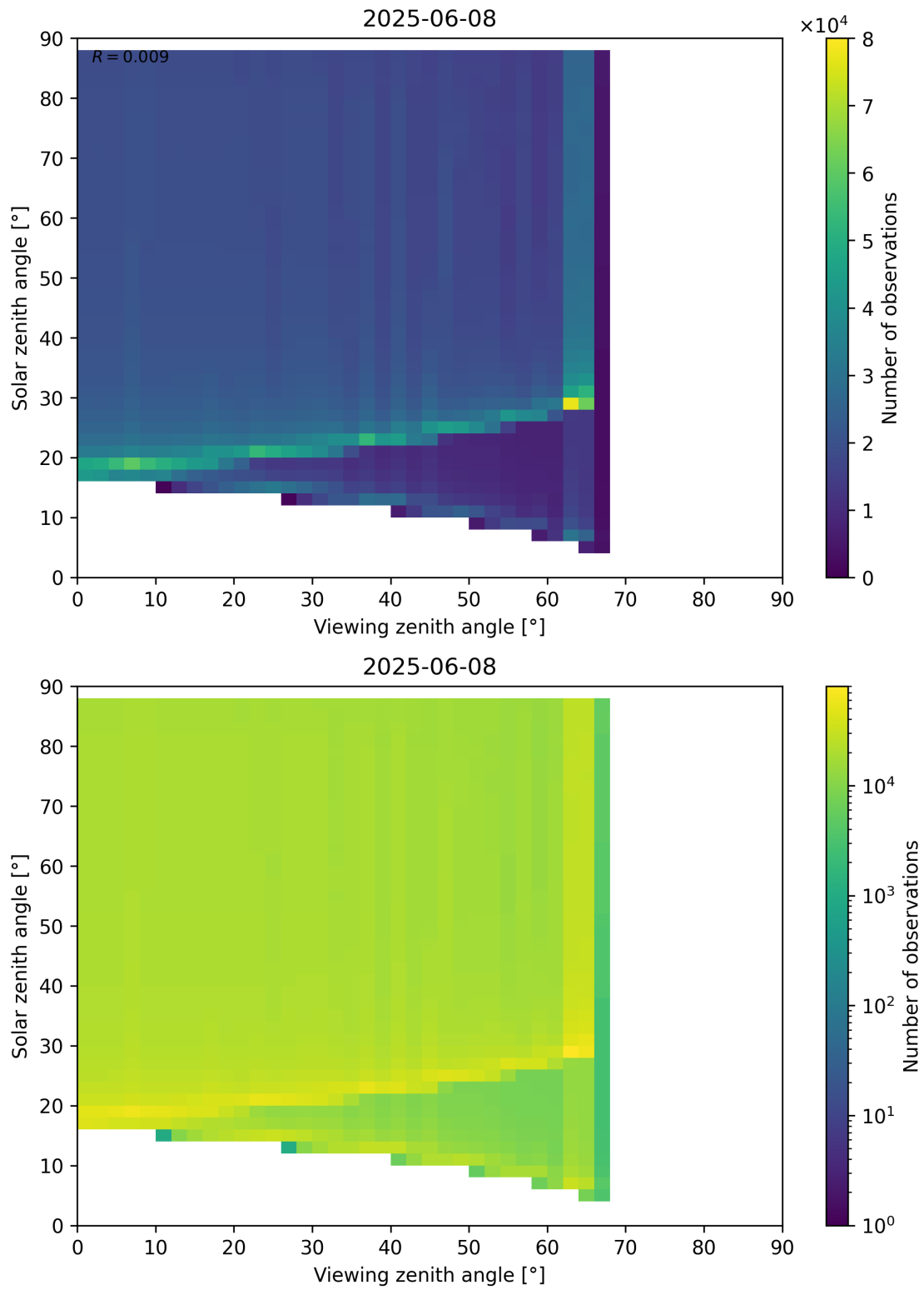
Figure 172: Scatter density plot of “Viewing zenith angle” against “Solar zenith angle” for 2025-06-07 to 2025-06-09.
