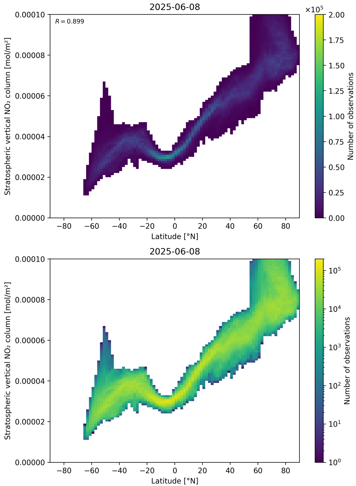
Figure 87: Scatter density plot of “Latitude” against “Stratospheric vertical \text{NO}_2 column” for 2025-06-07 to 2025-06-09.
