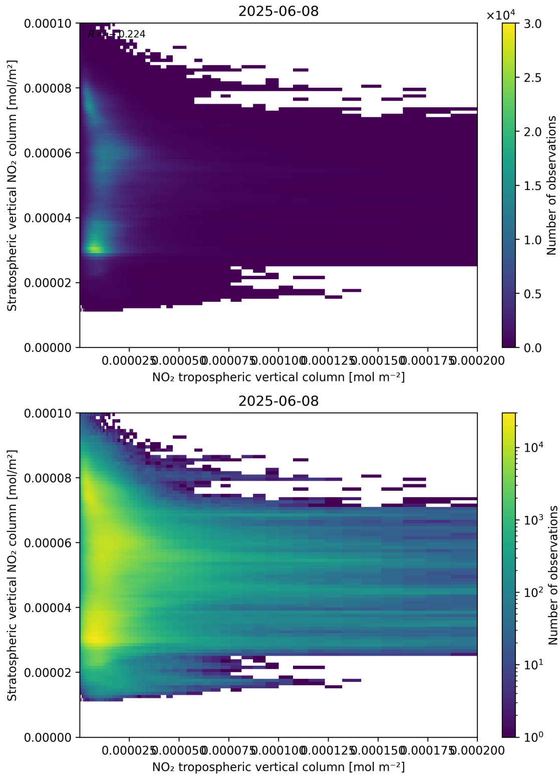
Figure 125: Scatter density plot of “NO 2 tropospheric vertical column” against “Stratospheric vertical NO 2 column” for 2025-06-07 to 2025-06-09.
