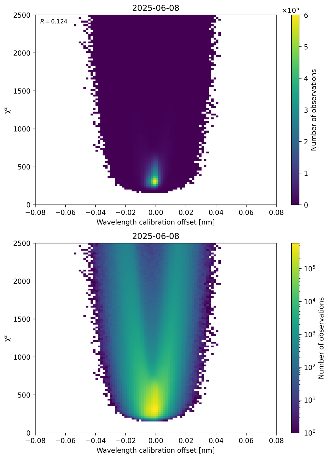
Figure 175: Scatter density plot of “Wavelength calibration offset” against “ \chi^2 ” for 2025-06-07 to 2025-06-09.
