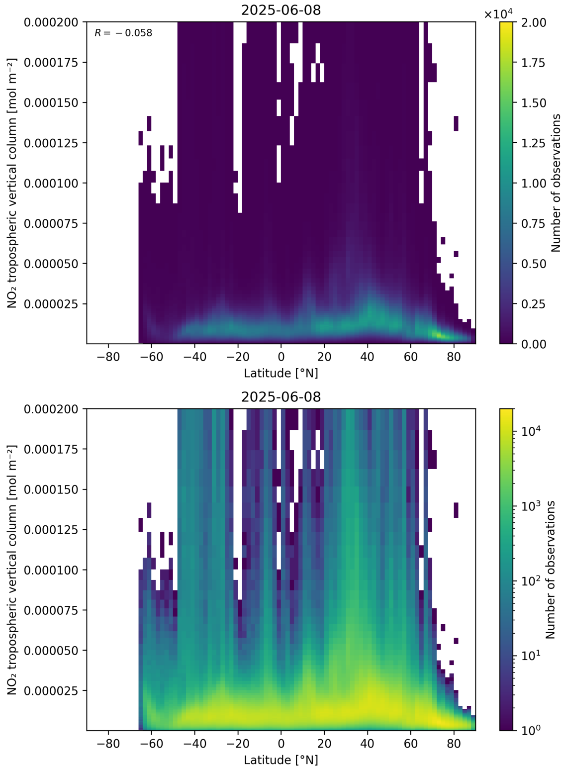
Figure 92: Scatter density plot of “Latitude” against “NO 2 tropospheric vertical column” for 2025-06-07 to 2025-06-09.
