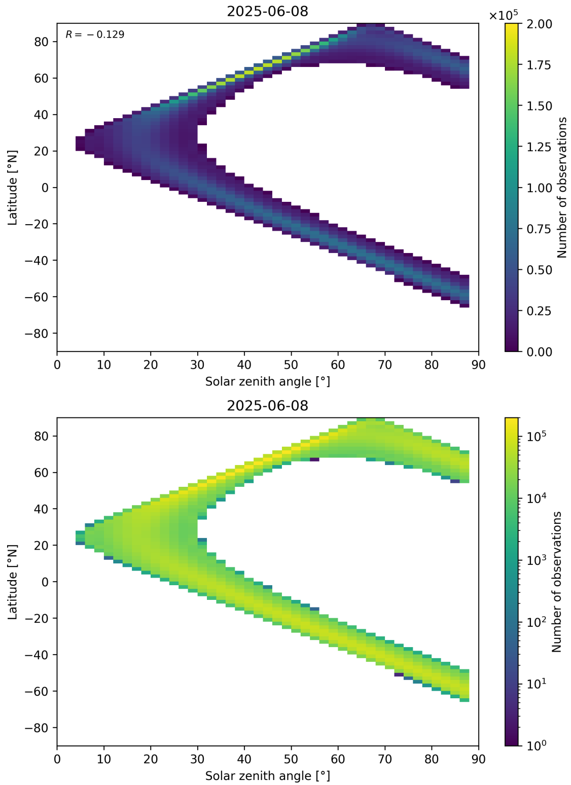
Figure 149: Scatter density plot of “Solar zenith angle” against “Latitude” for 2025-06-07 to 2025-06-09.
