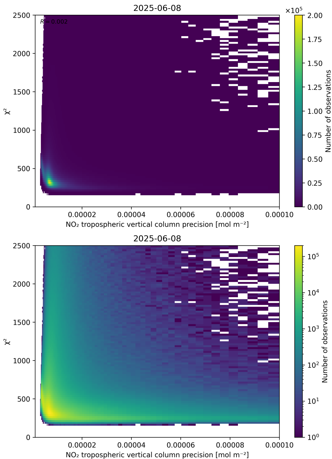
Figure 134: Scatter density plot of “NO 2 tropospheric vertical column precision” against “ \chi^2 ” for 2025-06-07 to 2025-06-09.
