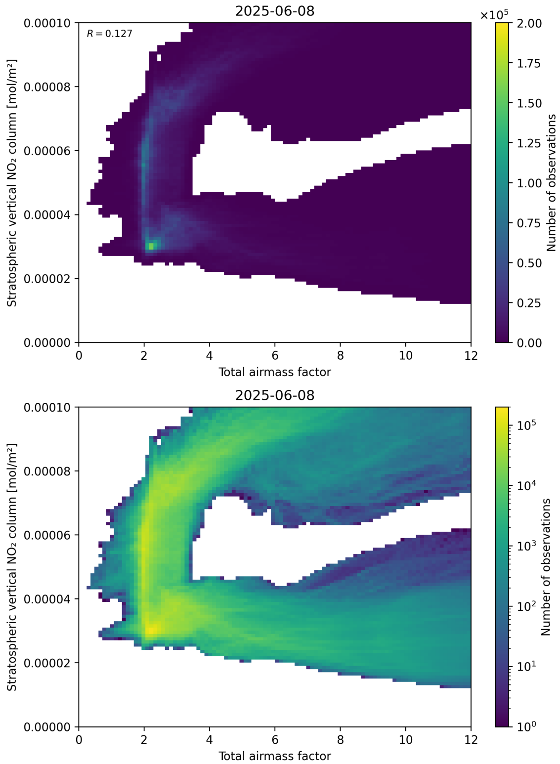
Figure 64: Scatter density plot of “Total airmass factor” against “Stratospheric vertical NO 2 column” for 2025-06-07 to 2025-06-09.
