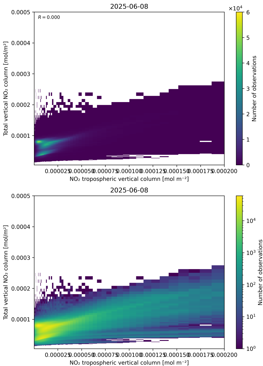
Figure 128: Scatter density plot of “NO 2 tropospheric vertical column” against “Total vertical NO 2 column” for 2025-06-07 to 2025-06-09.
