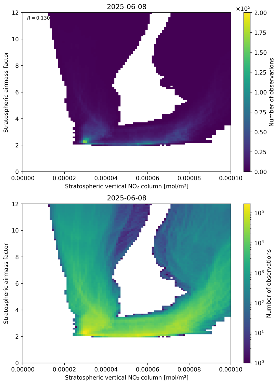
Figure 96: Scatter density plot of “Stratospheric vertical NO 2 column” against “Stratospheric airmass factor” for 2025-06-07 to 2025-06-09.
