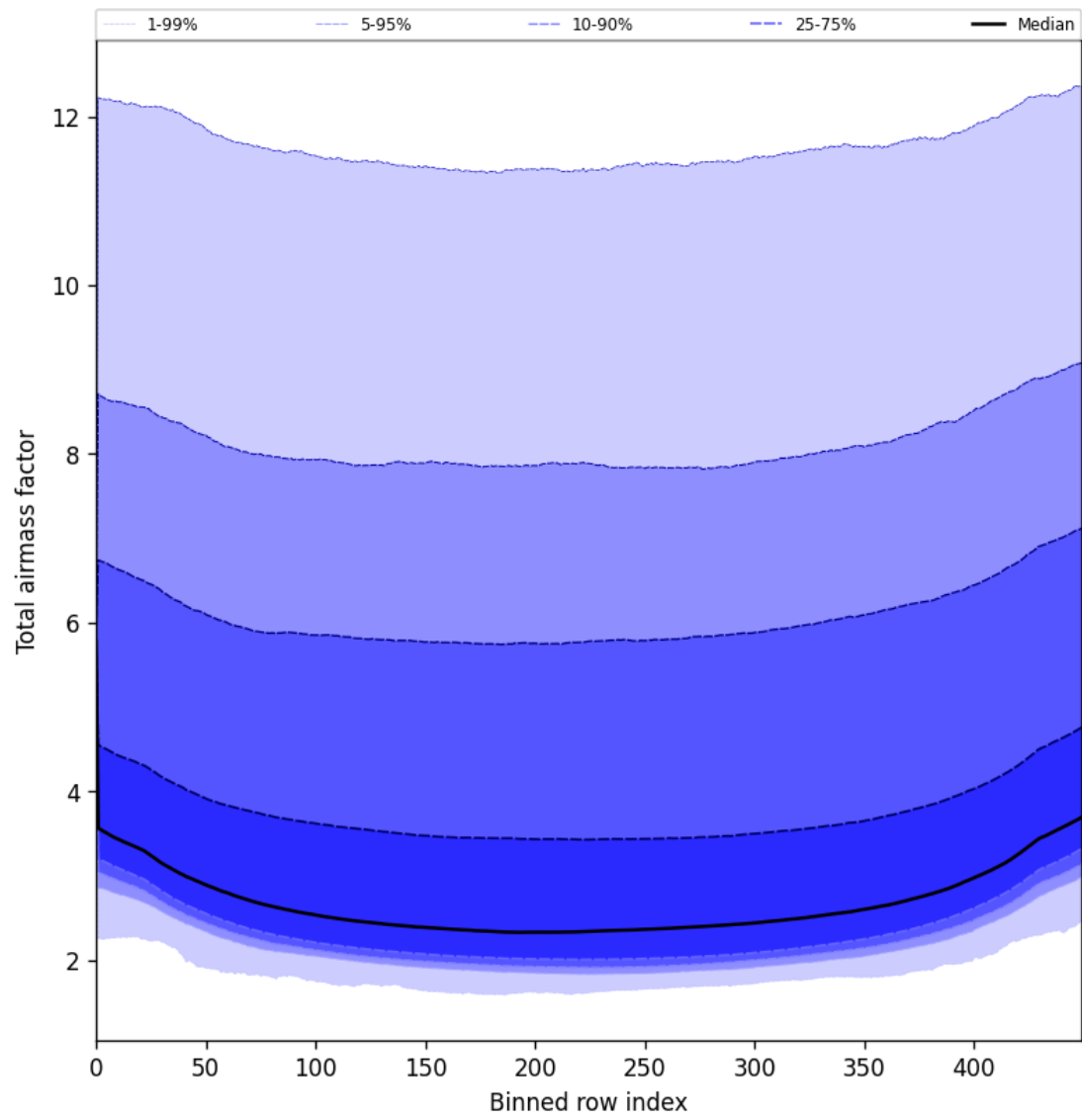
Figure 49: Along track statistics of “Total airmass factor” for 2025-06-07 to 2025-06-09
