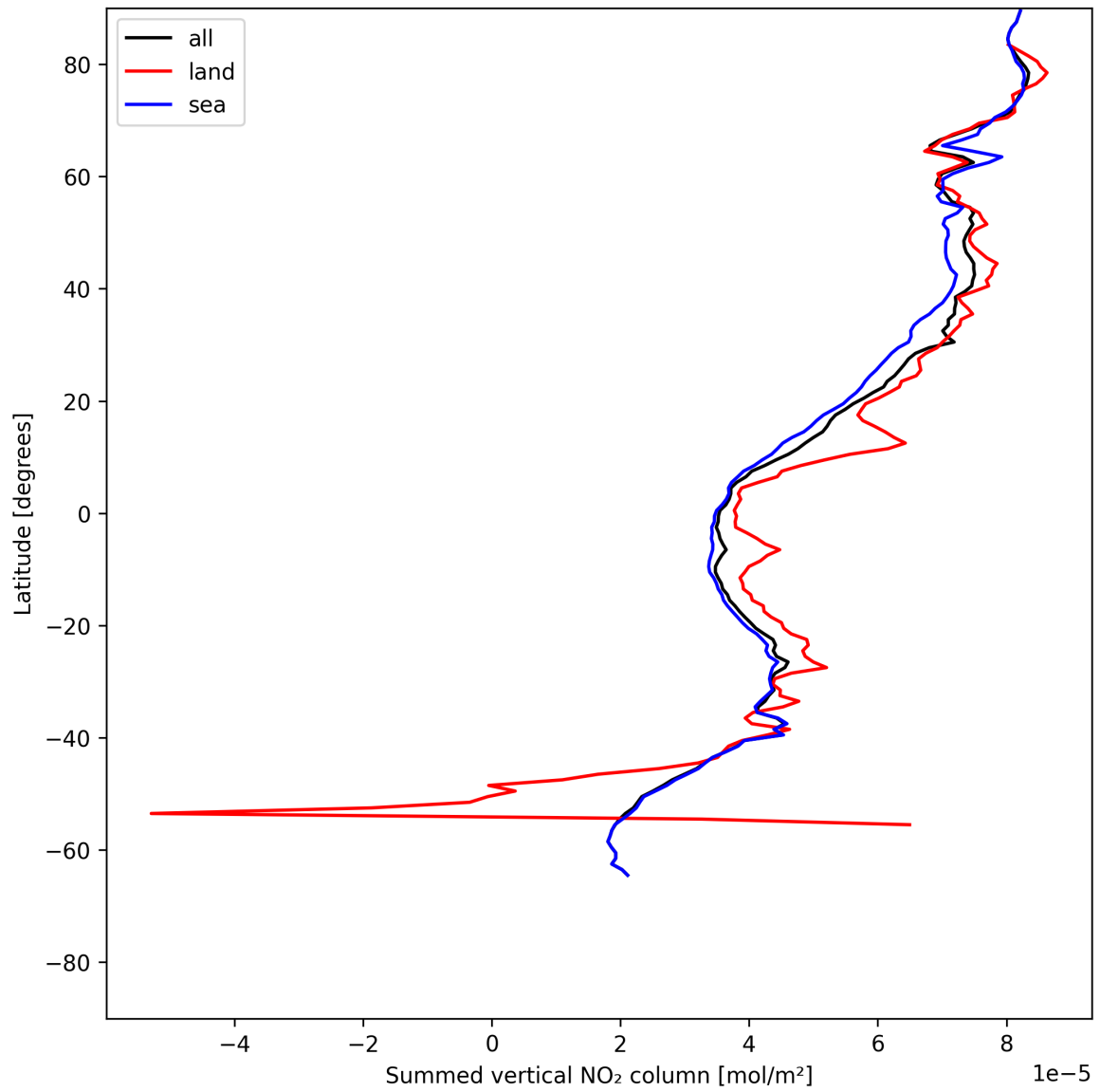
Figure 23: Zonal average of “Summed vertical NO 2 column” for 2025-06-07 to 2025-06-09.
