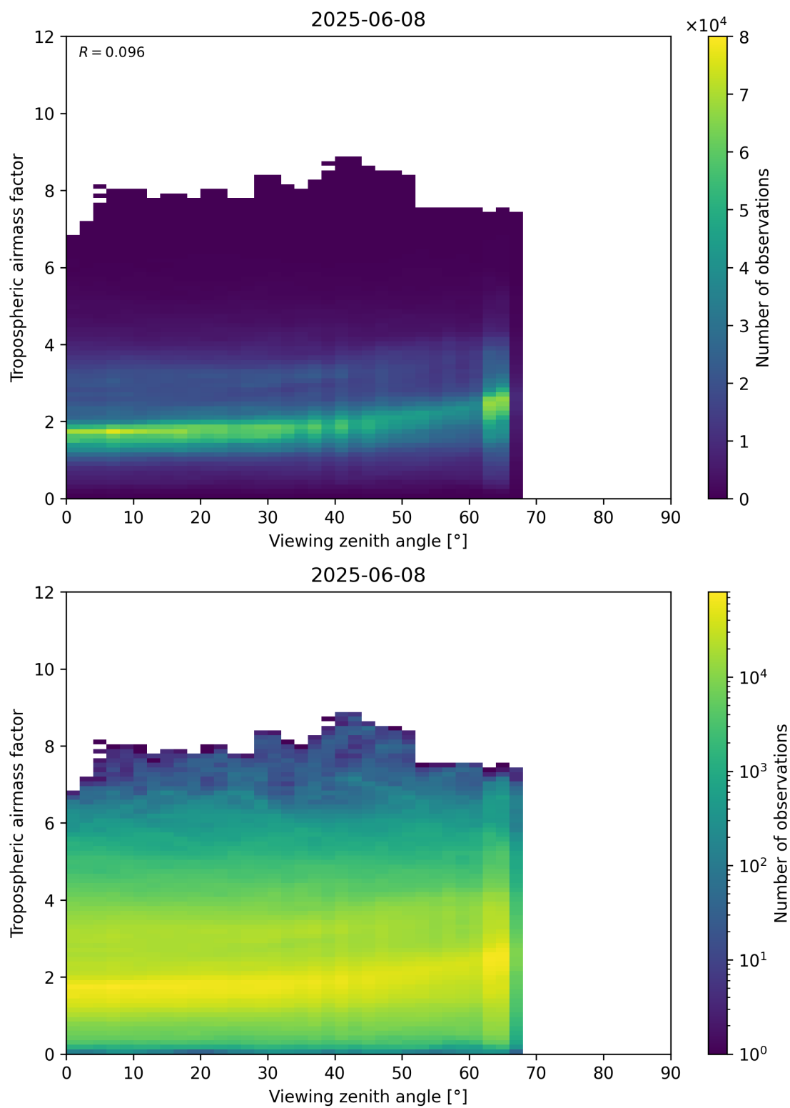
Figure 161: Scatter density plot of “Viewing zenith angle” against “Tropospheric airmass factor” for 2025-06-07 to 2025-06-09.
