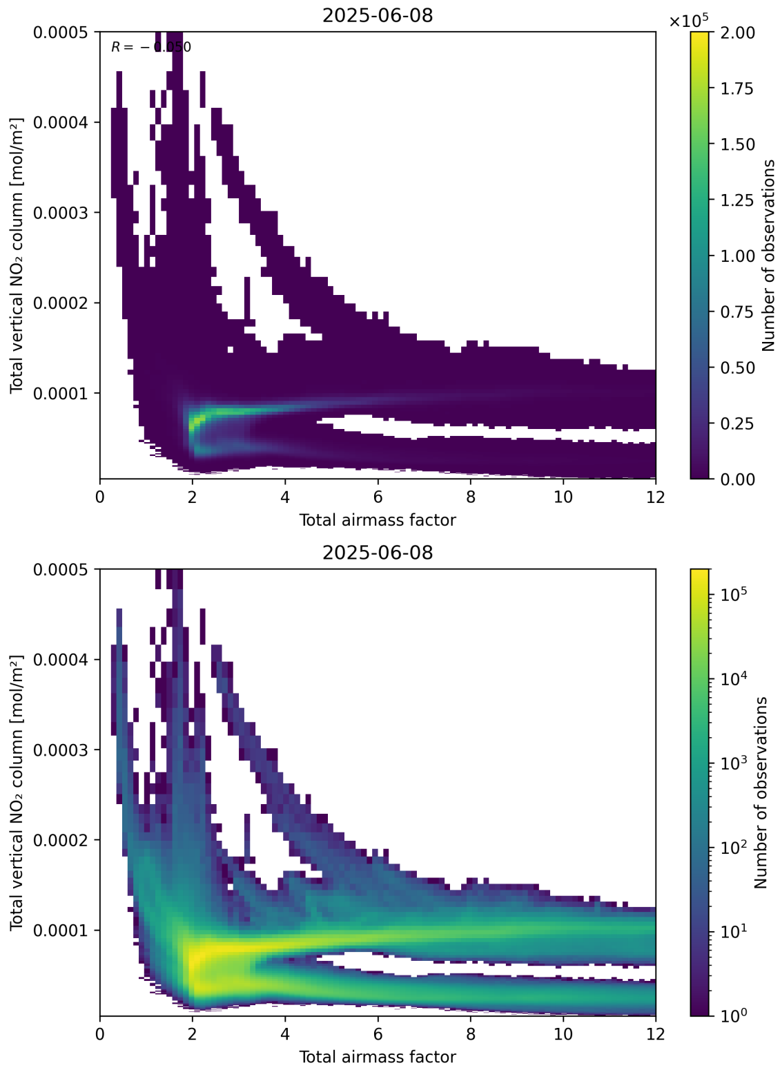
Figure 67: Scatter density plot of “Total airmass factor” against “Total vertical NO 2 column” for 2025-06-07 to 2025-06-09.
