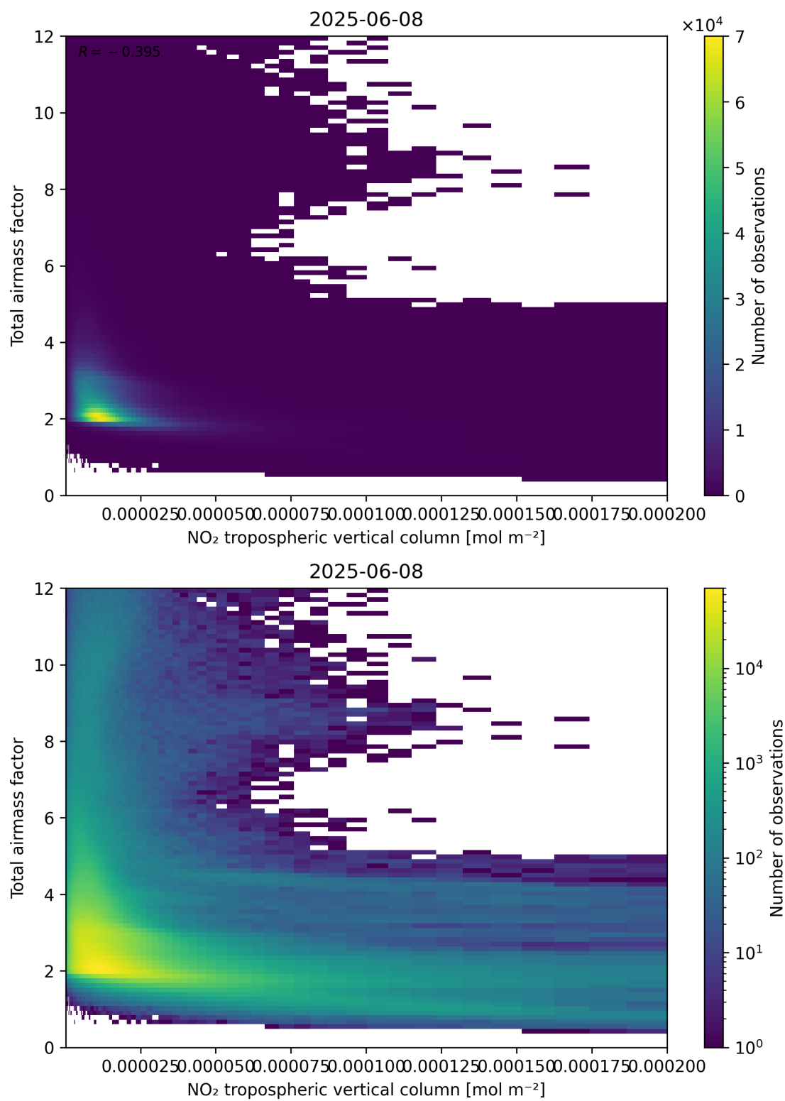
Figure 122: Scatter density plot of “NO 2 tropospheric vertical column” against “Total air mass factor” for 2025-06-07 to 2025-06-09.
