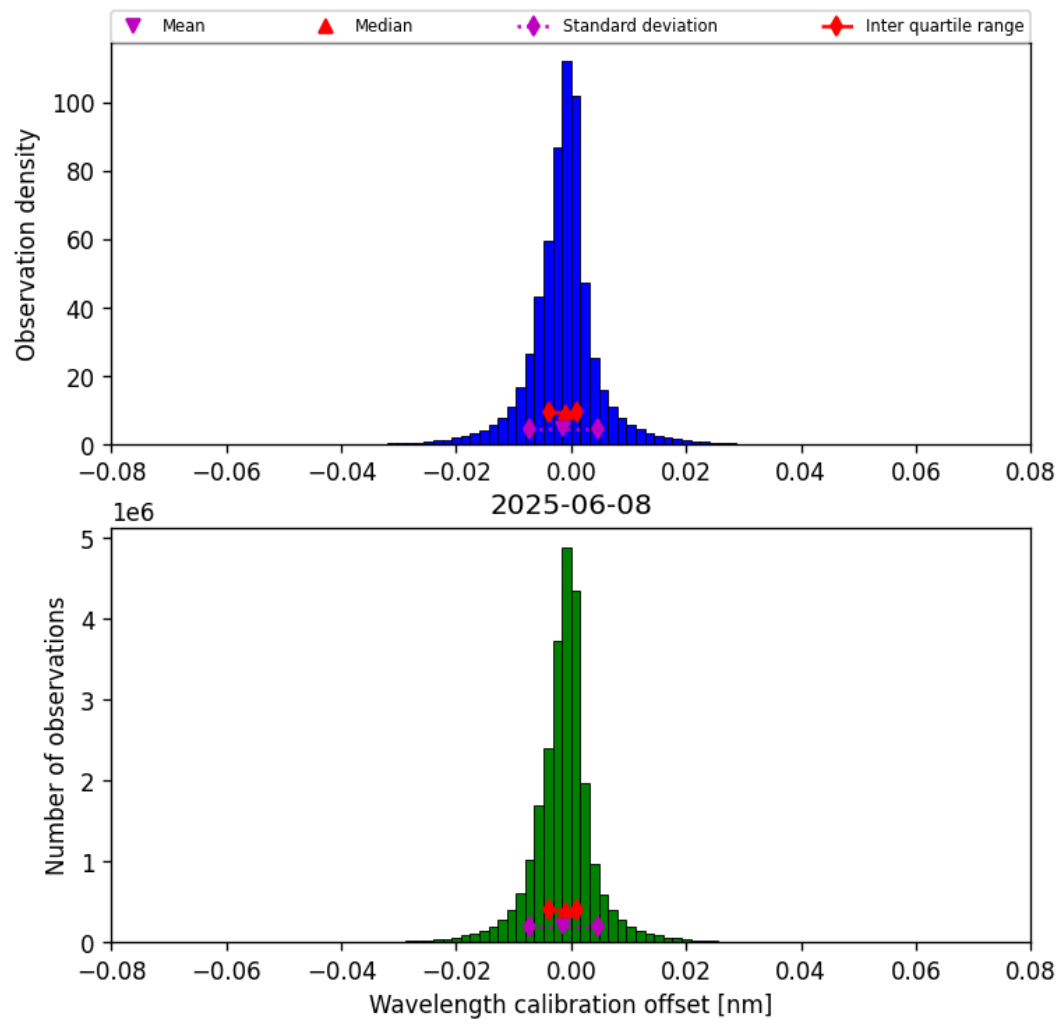
Figure 35: Histogram of “Wavelength calibration offset” for 2025-06-07 to 2025-06-09
