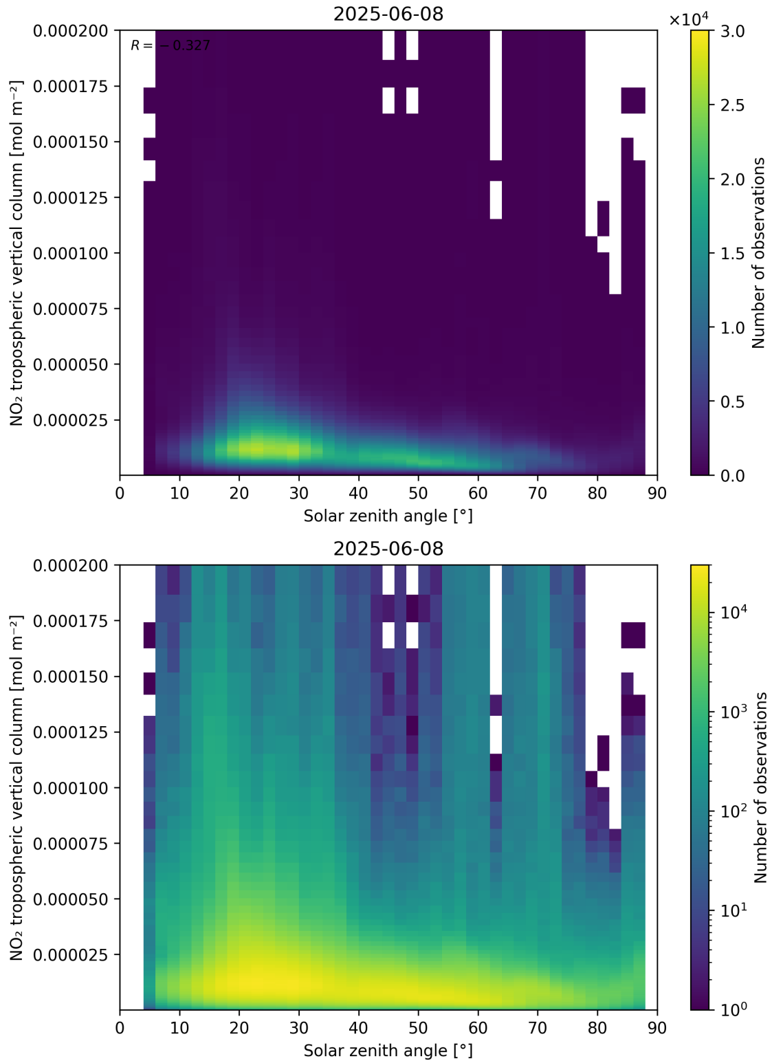
Figure 155: Scatter density plot of “Solar zenith angle” against “NO 2 tropospheric vertical column” for 2025-06-07 to 2025-06-09.
