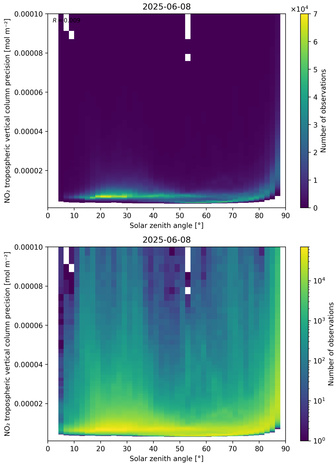
Figure 156: Scatter density plot of “Solar zenith angle” against “NO 2 tropospheric vertical column precision” for 2025-06-07 to 2025-06-09.
