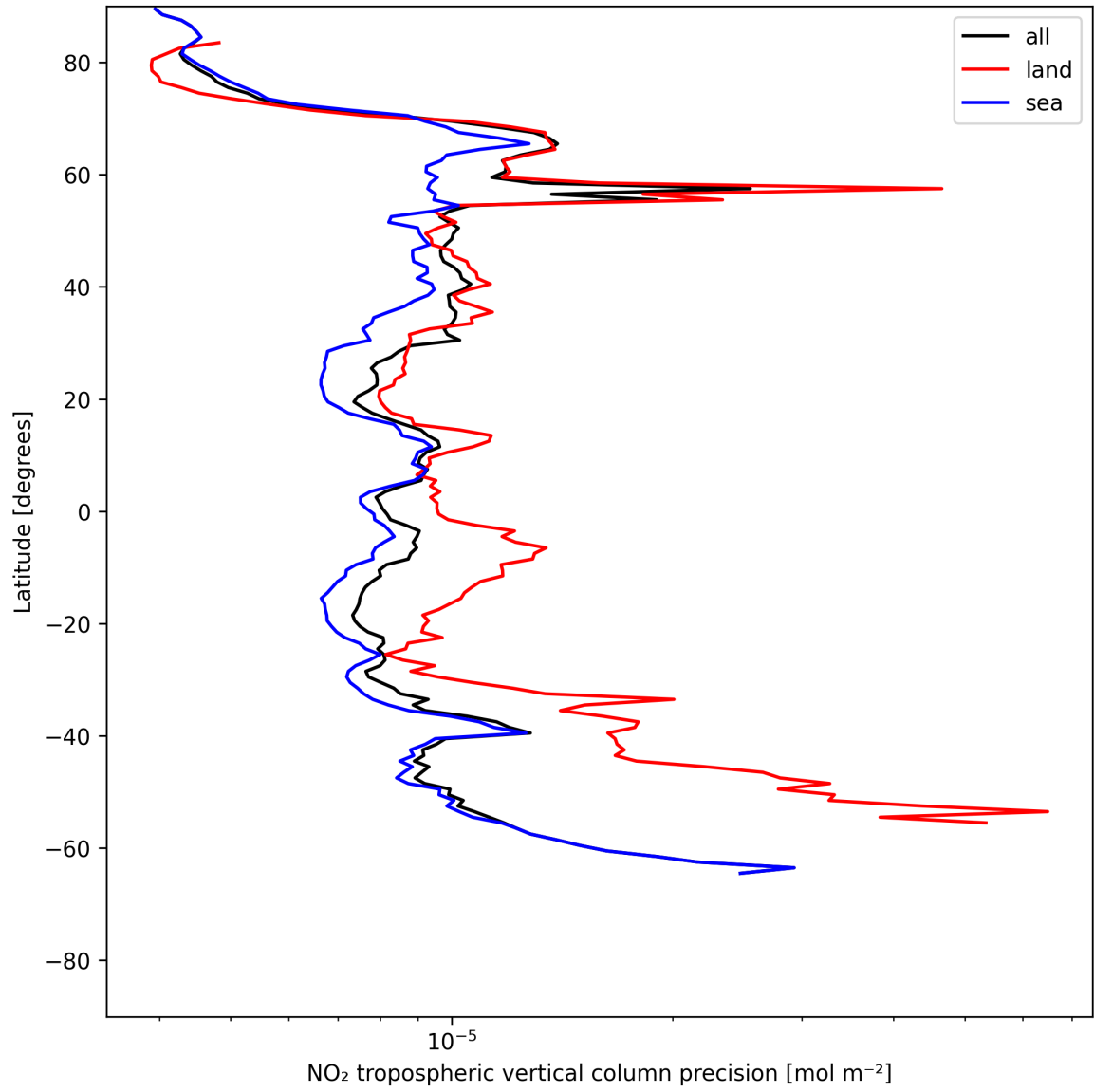
Figure 13: Zonal average of “NO 2 tropospheric vertical column precision” for 2025-06-07 to 2025-06-09.
