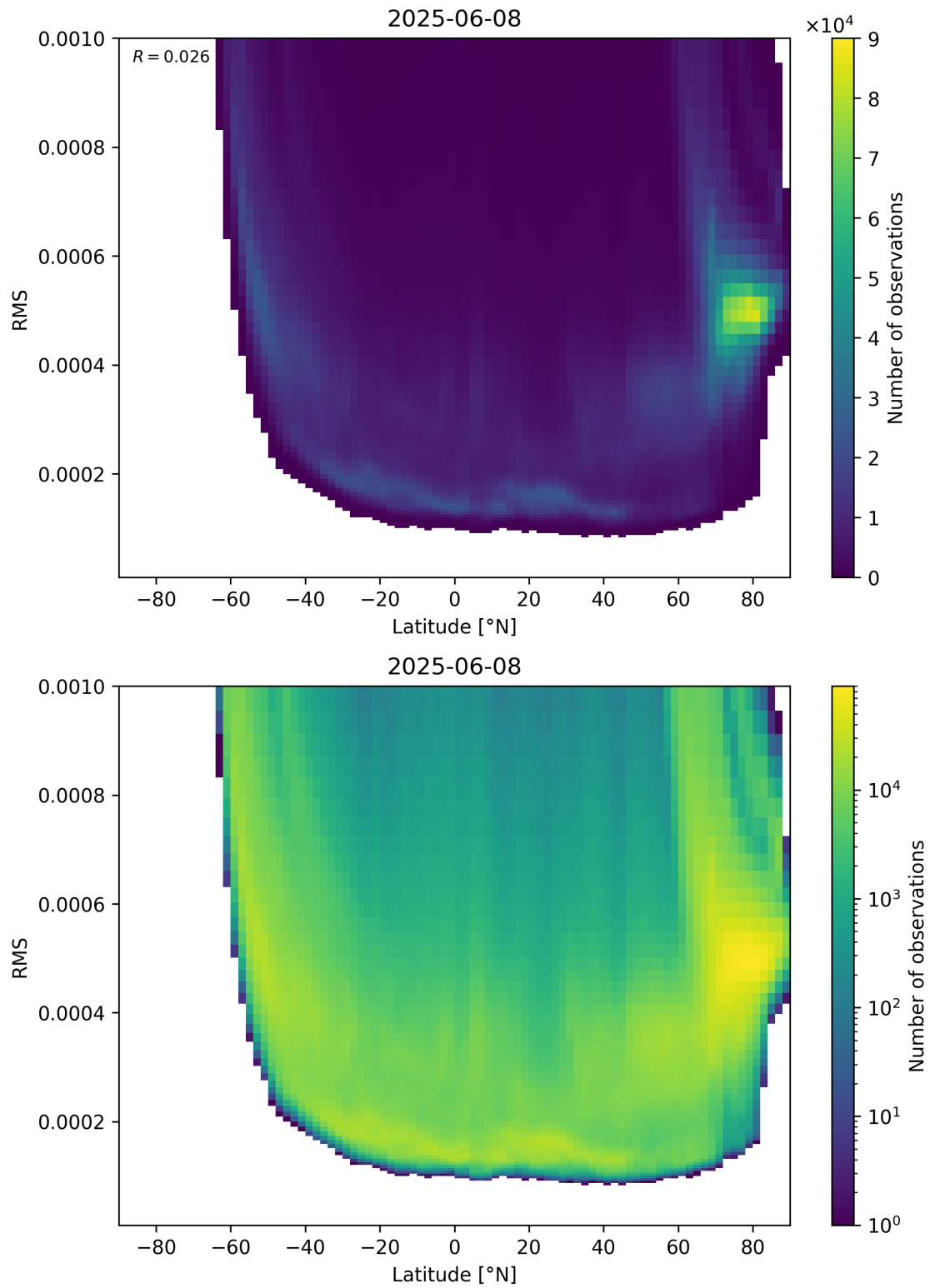
Figure 94: Scatter density plot of “Latitude” against “RMS” for 2025-06-07 to 2025-06-09.
