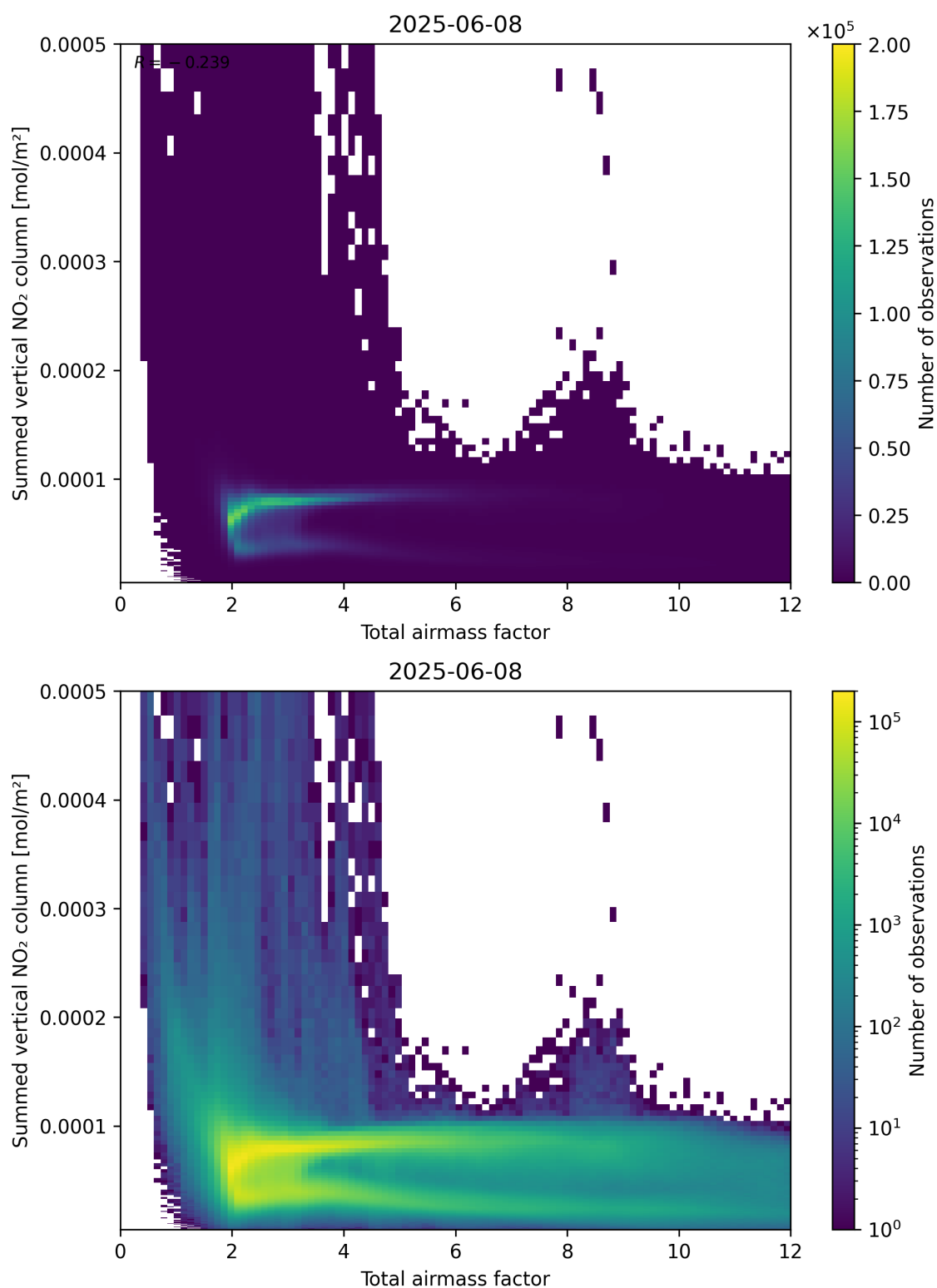
Figure 65: Scatter density plot of “Total airmass factor” against “Summed vertical NO 2 column” for 2025-06-07 to 2025-06-09.
