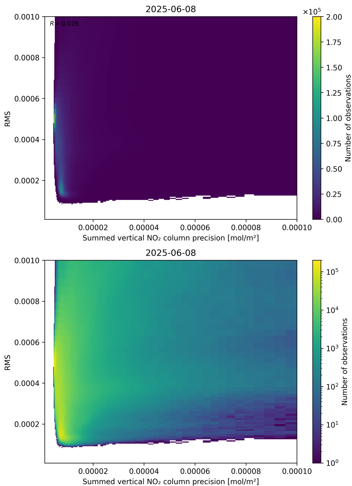
Figure 108: Scatter density plot of “Summed vertical NO 2 column precision” against “RMS” for 2025-06-07 to 2025-06-09.
