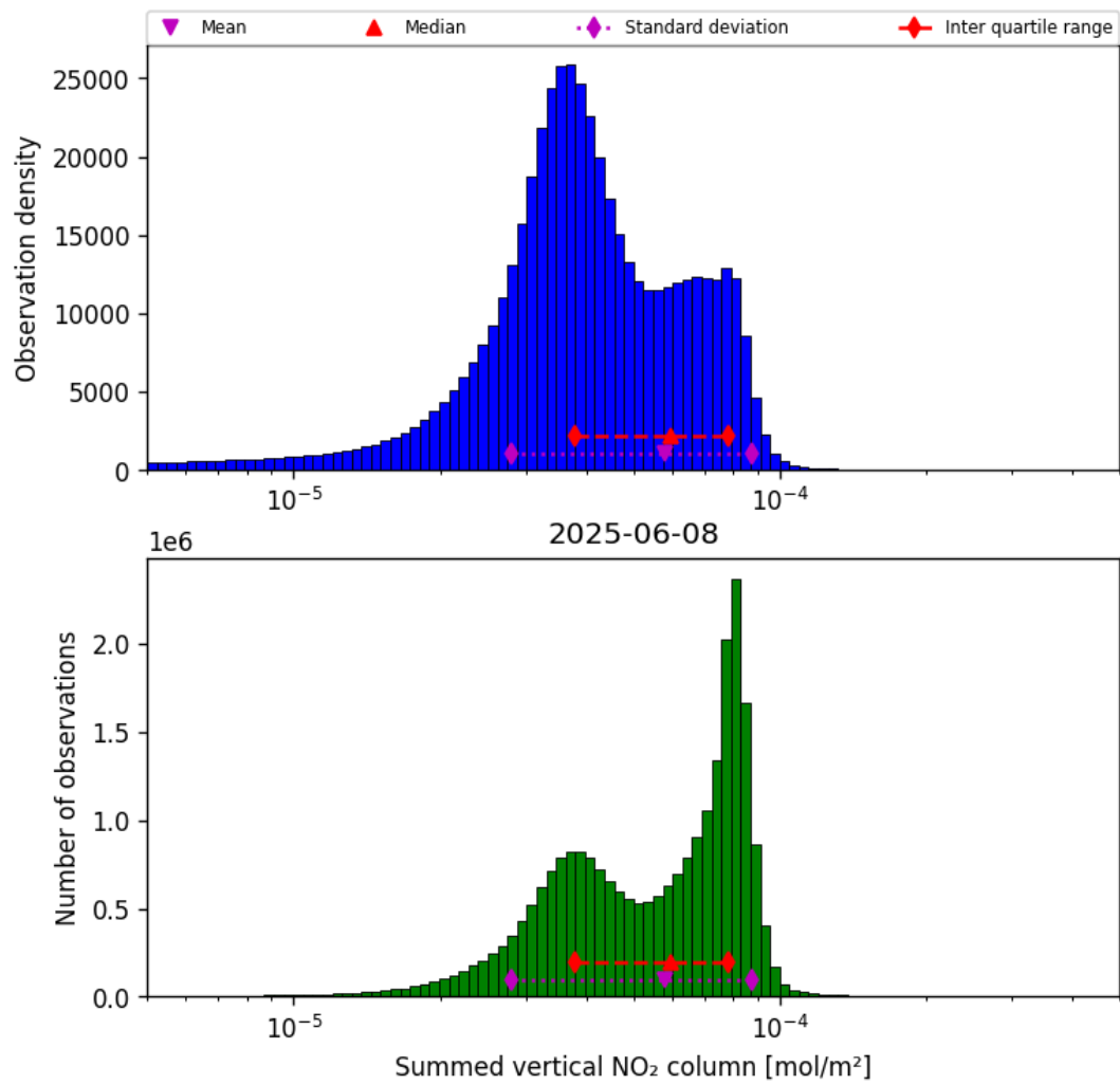
Figure 40: Histogram of “Summed vertical NO 2 column” for 2025-06-07 to 2025-06-09
