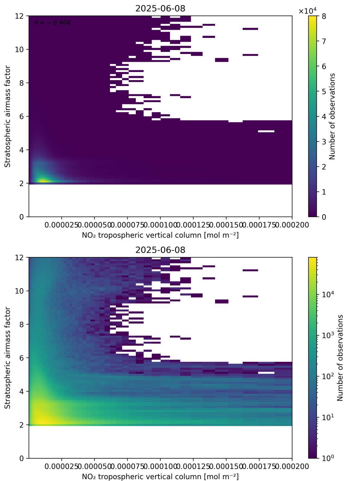
Figure 121: Scatter density plot of “NO 2 tropospheric vertical column” against “Stratospheric air mass factor” for 2025-06-07 to 2025-06-09.
