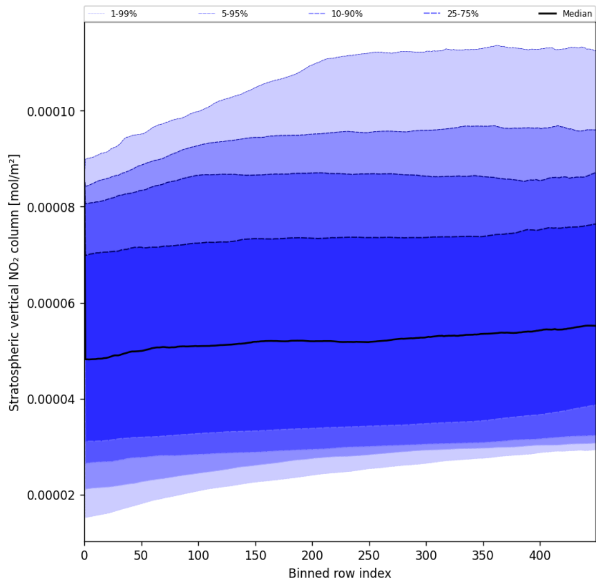
Figure 53: Along track statistics of “Stratospheric vertical NO 2 column” for 2025-06-07 to 2025-06-09
