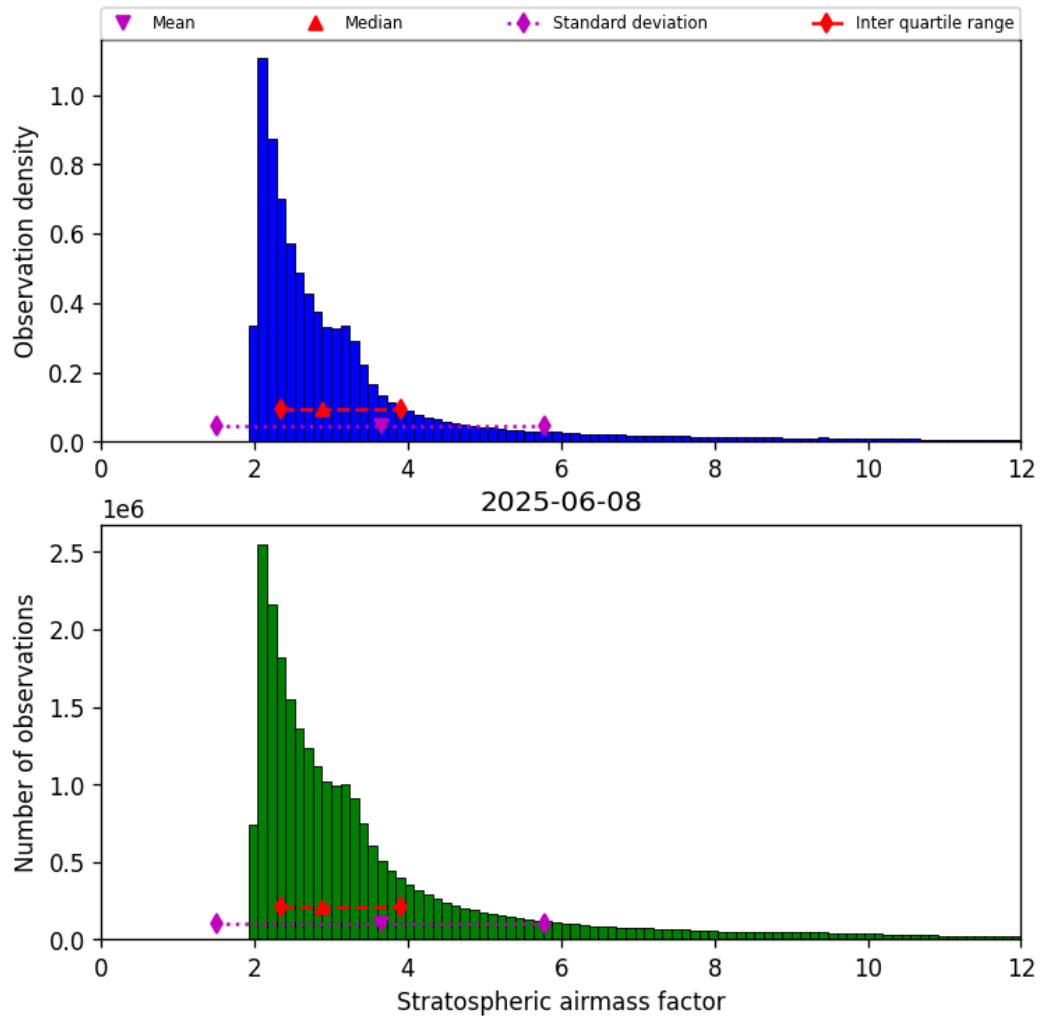
Figure 44: Histogram of “Stratospheric airmass factor” for 2025-06-07 to 2025-06-09
