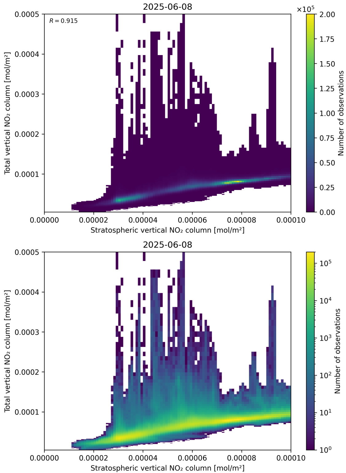
Figure 100: Scatter density plot of “Stratospheric vertical NO 2 column” against “Total vertical NO 2 column” for 2025-06-07 to 2025-06-09.
