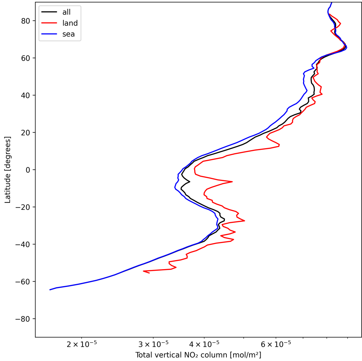
Figure 21: Zonal average of “Total vertical NO 2 column” for 2025-06-07 to 2025-06-09.
