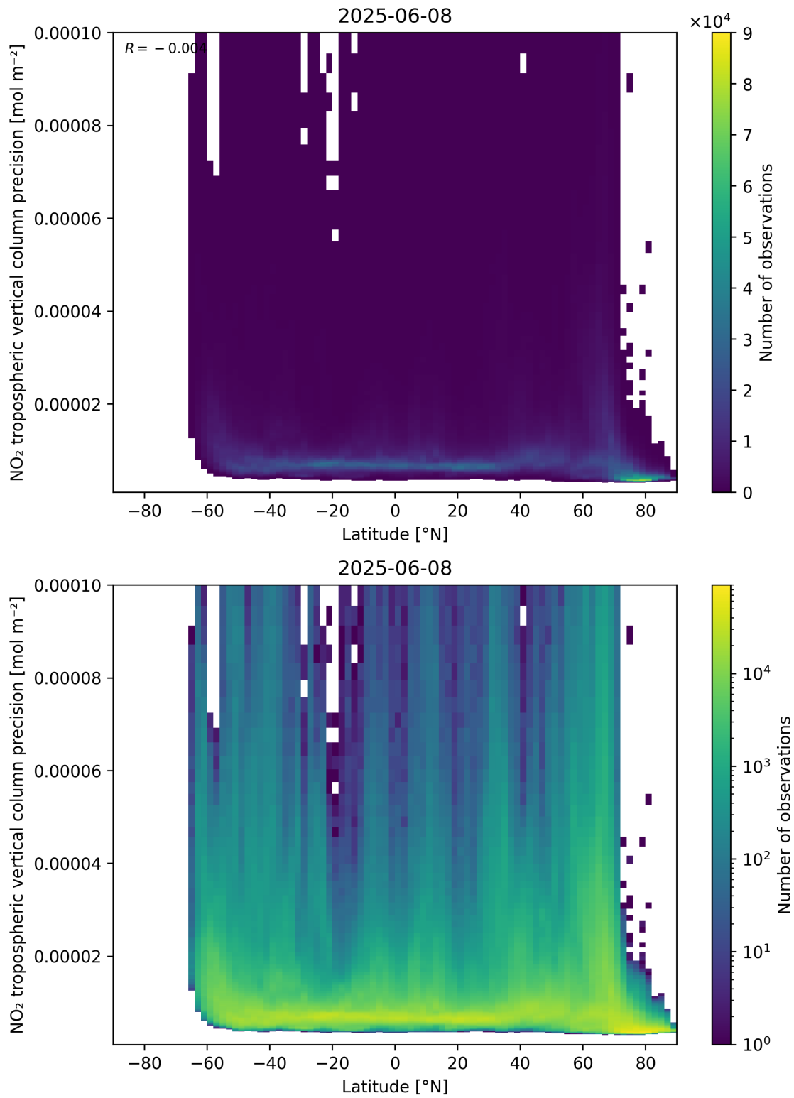
Figure 93: Scatter density plot of “Latitude” against “NO 2 tropospheric vertical column precision” for 2025-06-07 to 2025-06-09.
