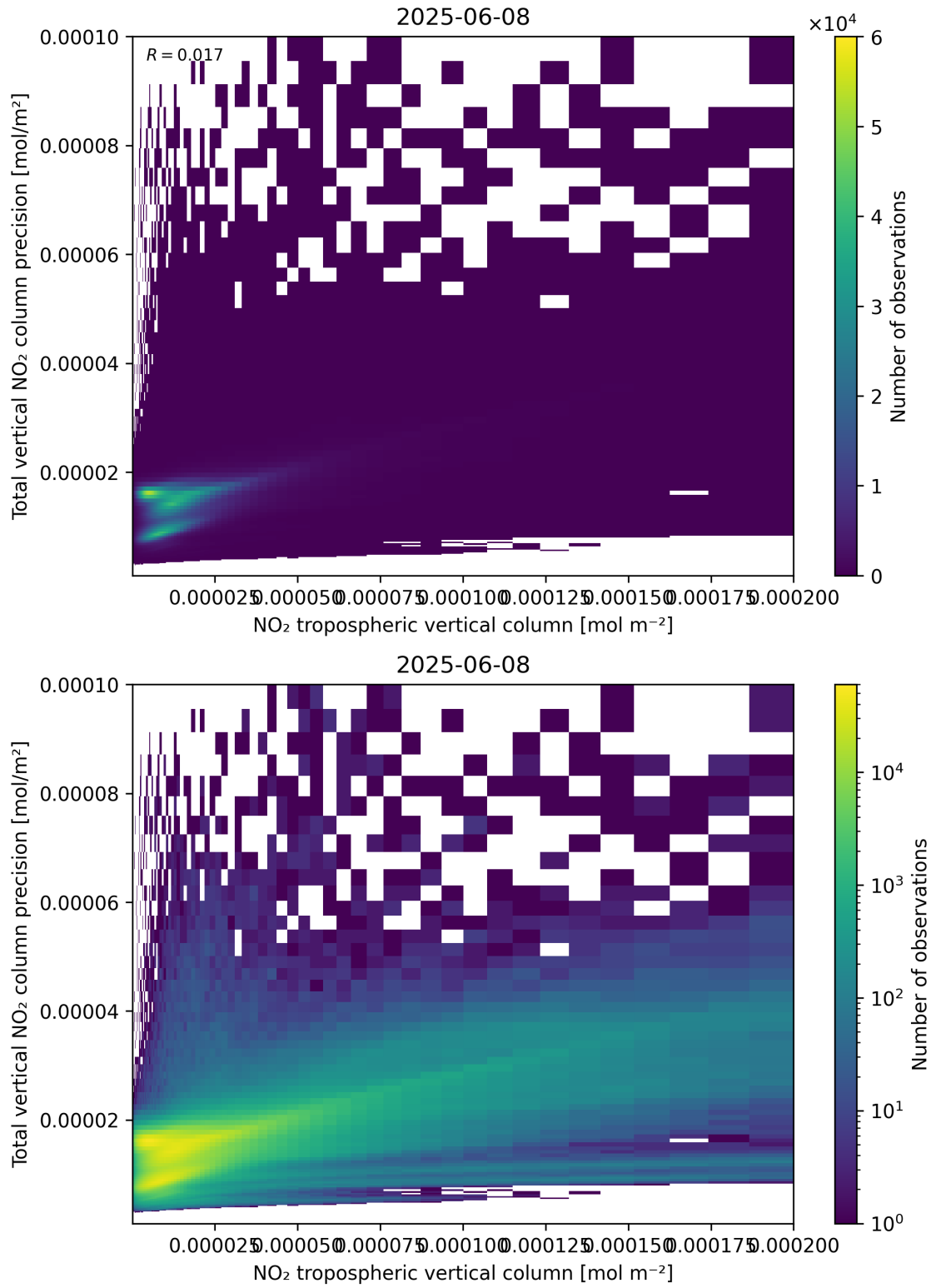
Figure 129: Scatter density plot of “NO 2 tropospheric vertical column” against “Total vertical NO 2 column precision” for 2025-06-07 to 2025-06-09.
