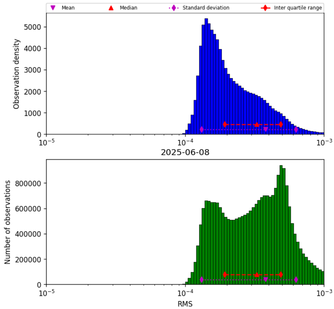
Figure 43: Histogram of “RMS” for 2025-06-07 to 2025-06-09
