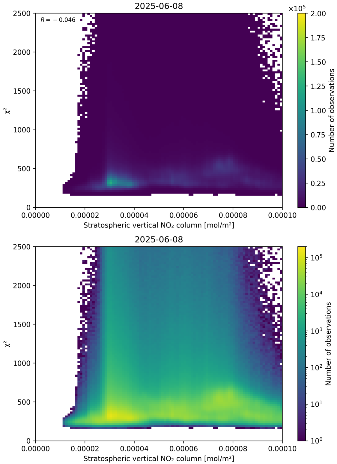
Figure 97: Scatter density plot of “Stratospheric vertical NO 2 column” against “ \chi^2 ” for 2025-06-07 to 2025-06-09.
