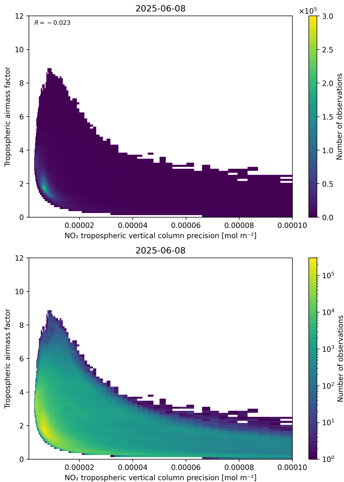
Figure 133: Scatter density plot of “NO 2 tropospheric vertical column precision” against “Tropospheric airmass factor” for 2025-06-07 to 2025-06-09.
