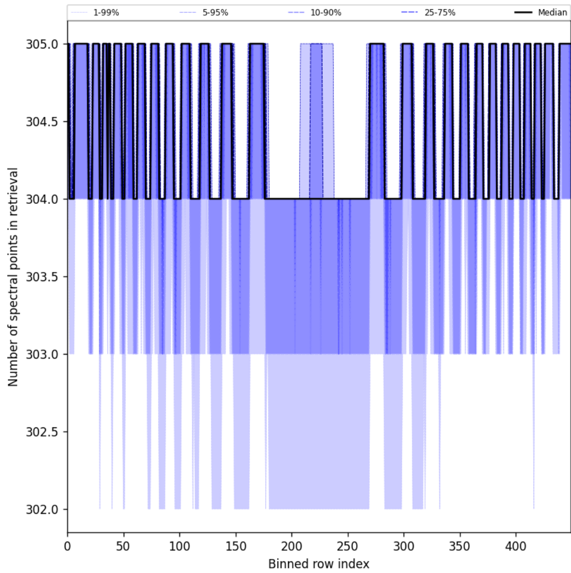
Figure 50: Along track statistics of “Number of spectral points in retrieval” for 2025-06-07 to 2025-06-09
