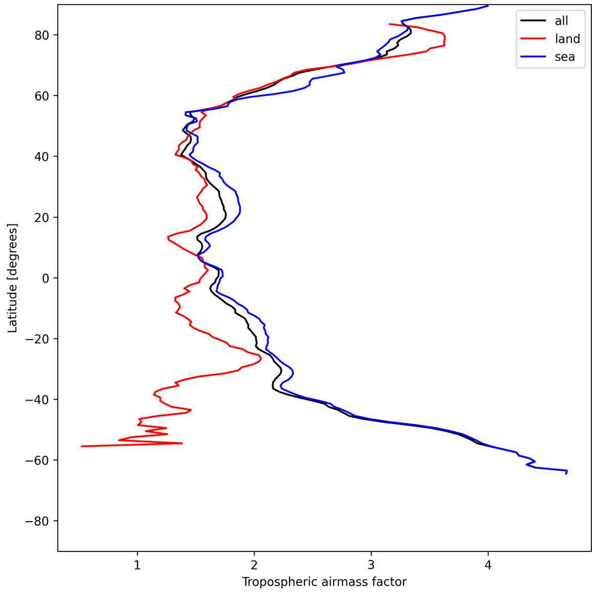
Figure 14: Zonal average of “Tropospheric airmass factor” for 2025-06-07 to 2025-06-09.
