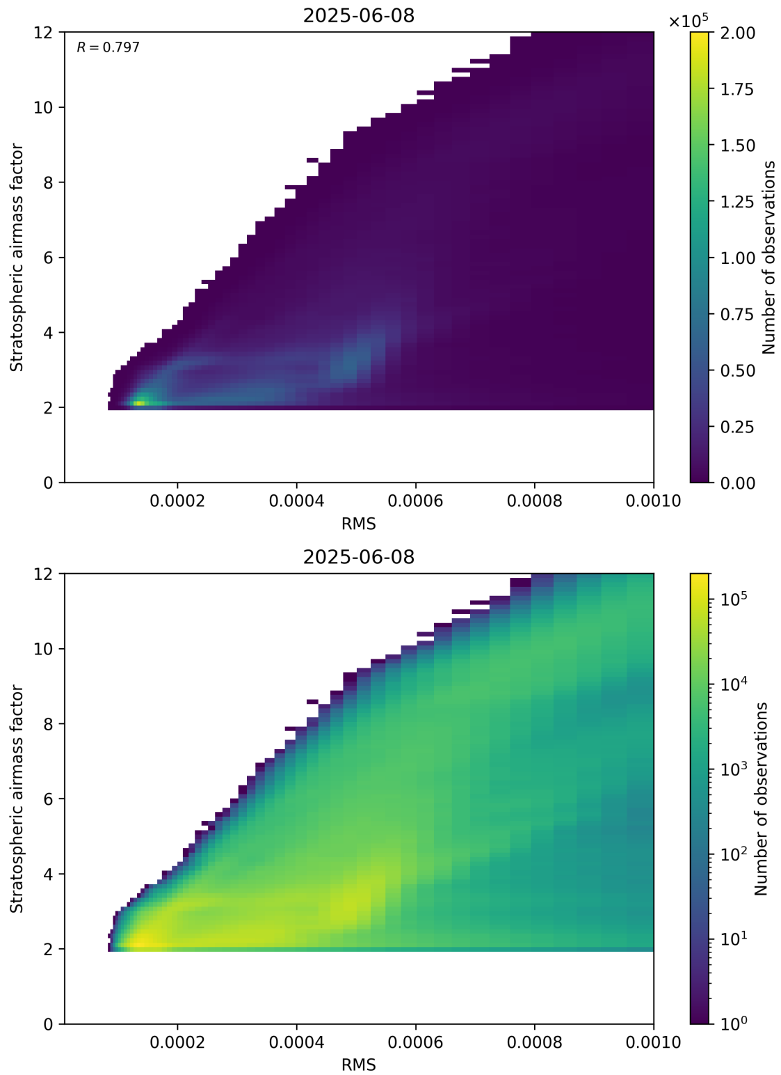
Figure 144: Scatter density plot of “RMS” against “Stratospheric airmass factor” for 2025-06-07 to 2025-06-09.
