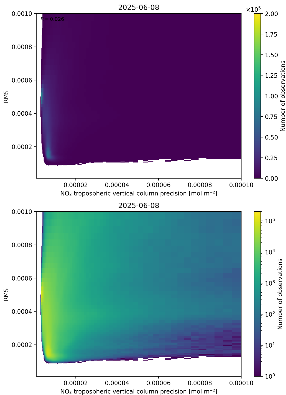
Figure 140: Scatter density plot of “NO 2 tropospheric vertical column precision” against “RMS” for 2025-06-07 to 2025-06-09.
