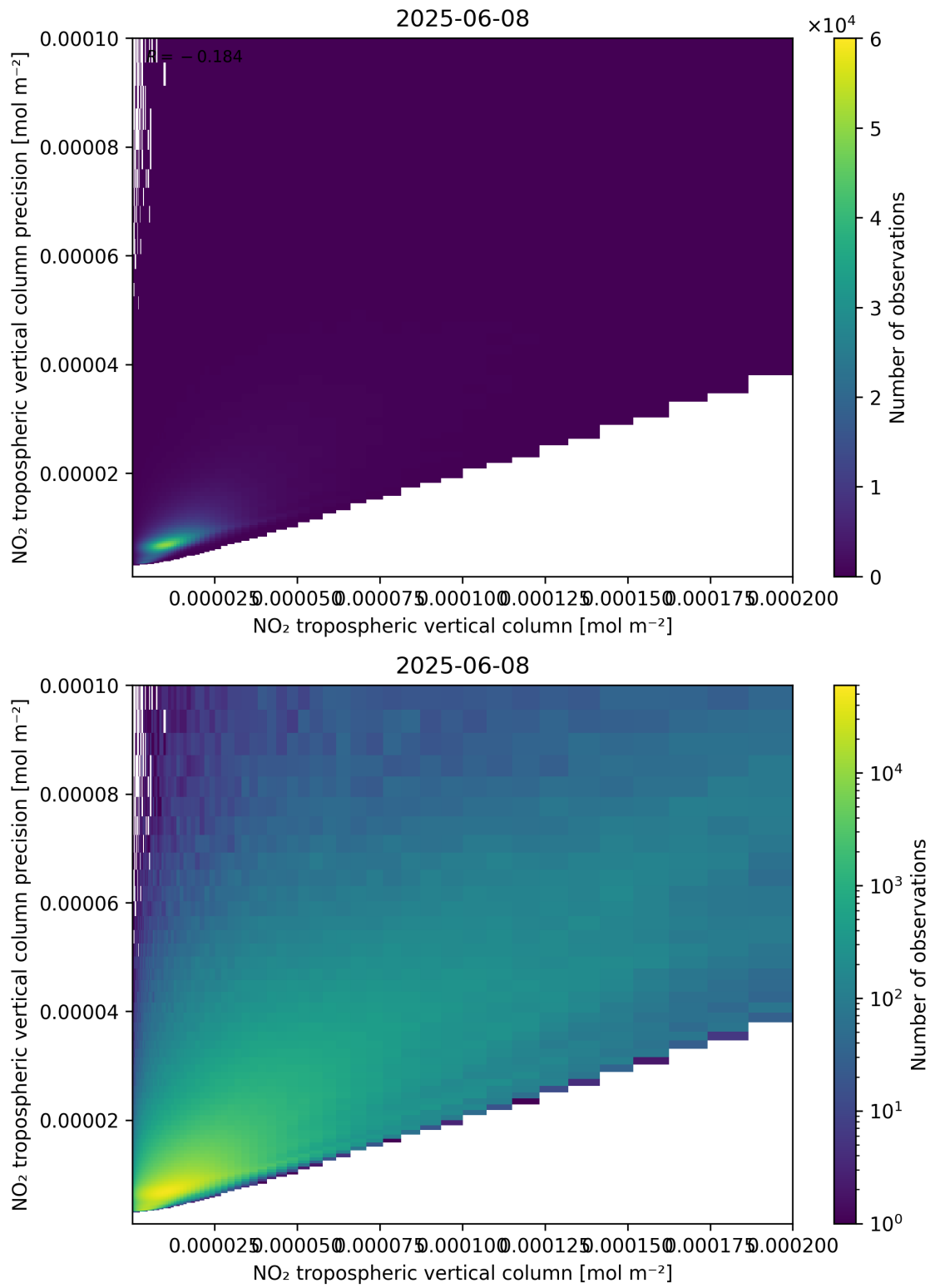
Figure 130: Scatter density plot of “NO 2 tropospheric vertical column” against “NO 2 tropospheric vertical column precision” for 2025-06-07 to 2025-06-09.
