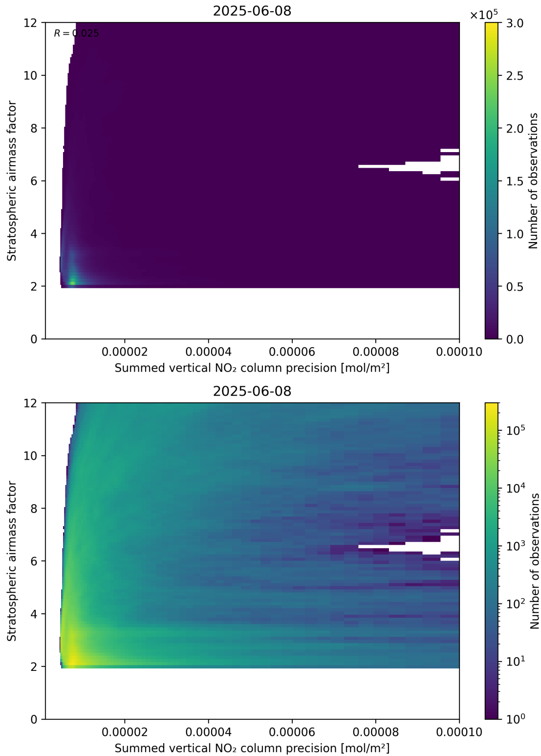
Figure 106: Scatter density plot of “Summed vertical NO 2 column precision” against “Stratospheric airmass factor” for 2025-06-07 to 2025-06-09.
