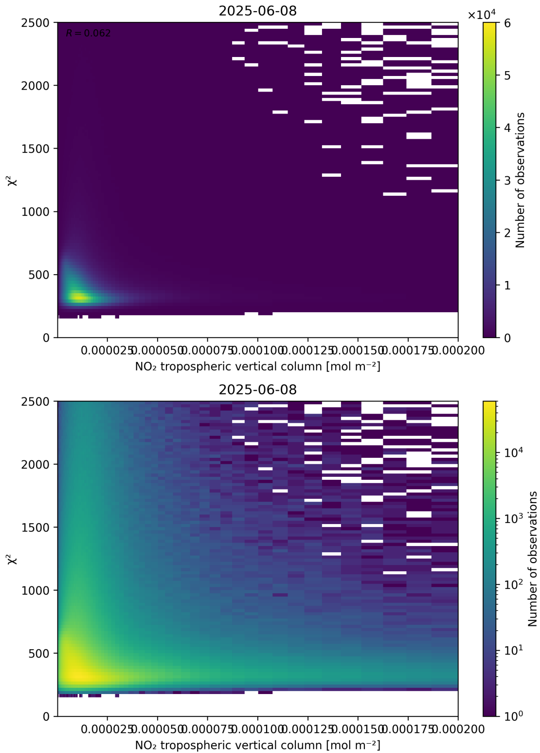
Figure 124: Scatter density plot of “NO 2 tropospheric vertical column” against “ \chi^2 ” for 2025-06-07 to 2025-06-09.
