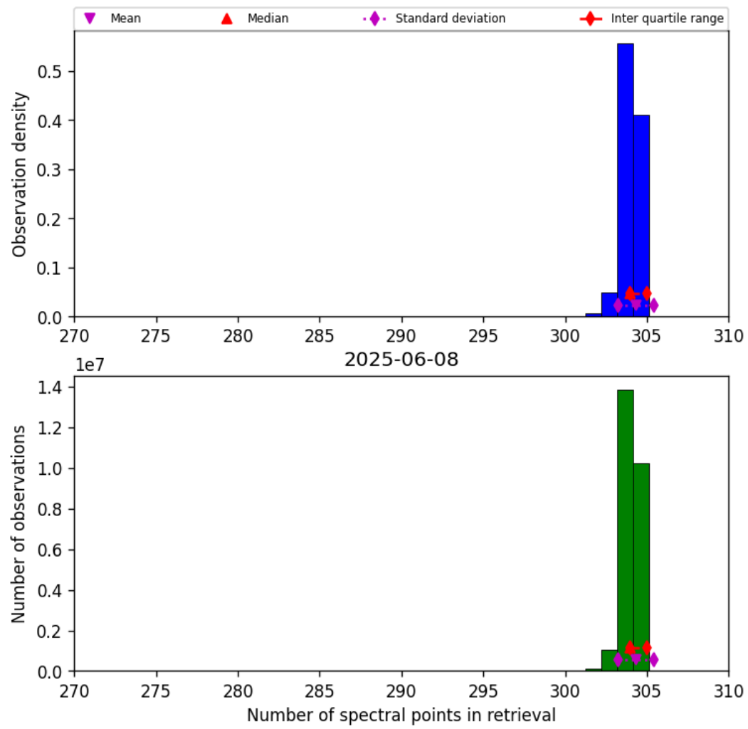
Figure 33: Histogram of “Number of spectral points in retrieval” for 2025-06-07 to 2025-06-09
