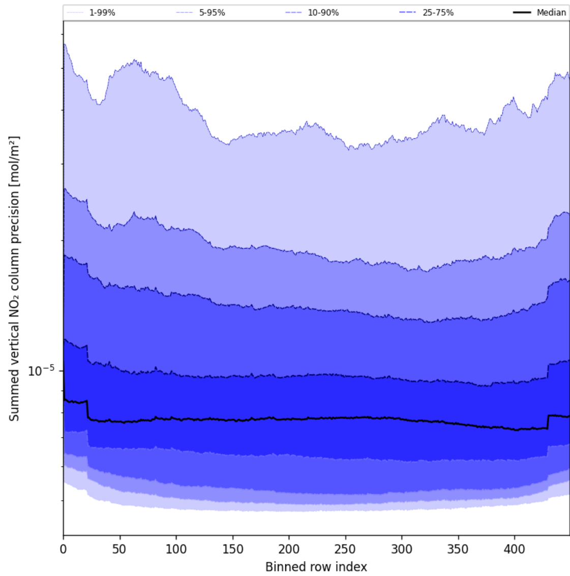
Figure 58: Along track statistics of “Summed vertical NO 2 column precision” for 2025-06-07 to 2025-06-09
