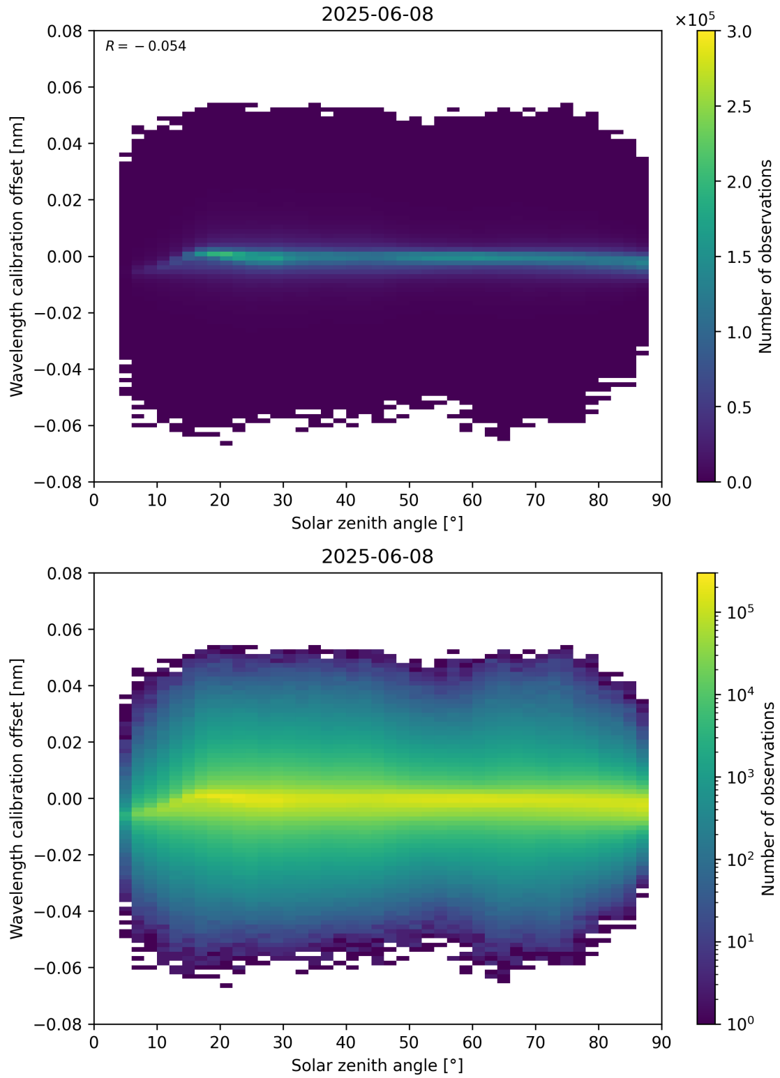
Figure 158: Scatter density plot of “Solar zenith angle” against “Wavelength calibration offset” for 2025-06-07 to 2025-06-09.
