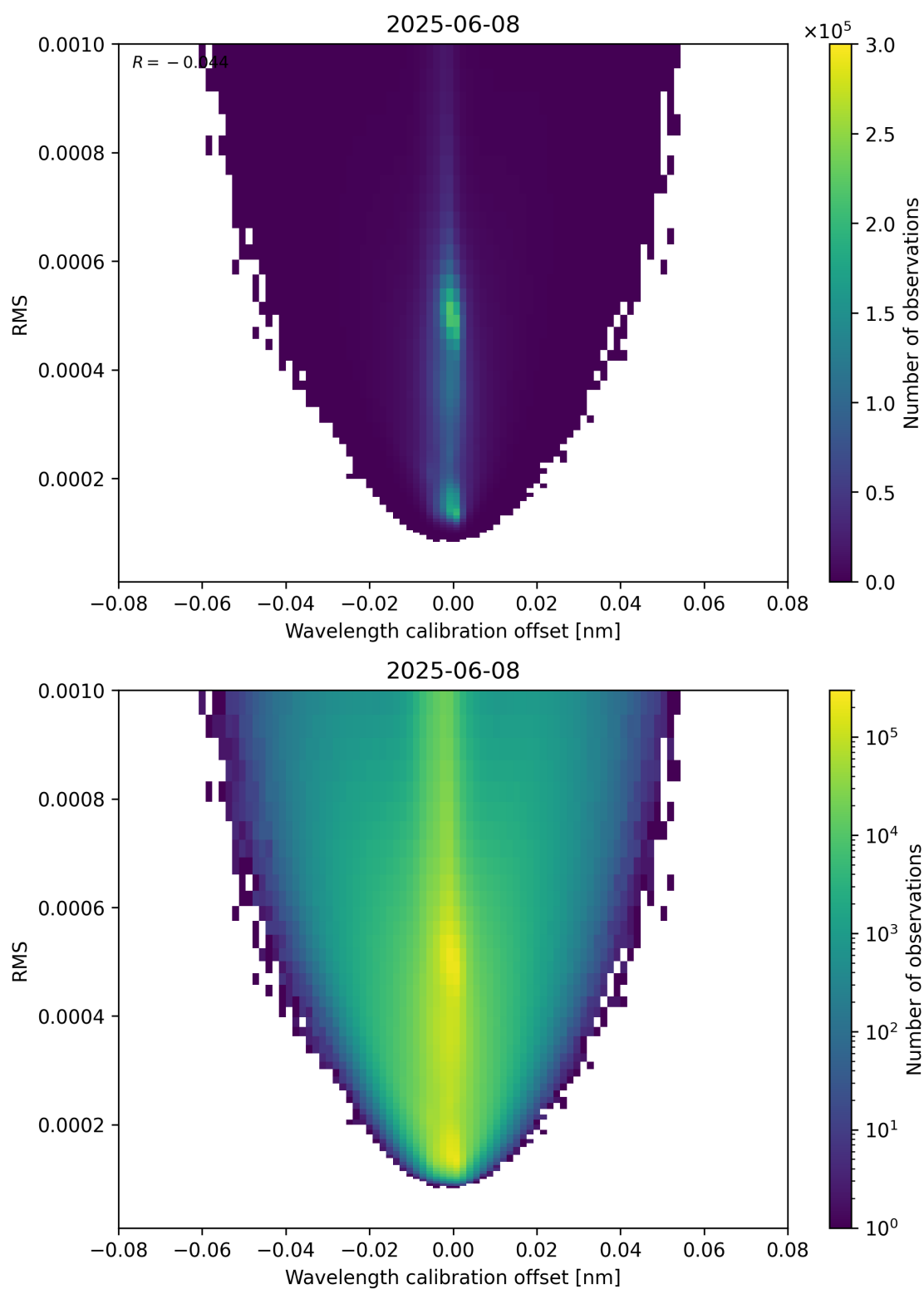
Figure 181: Scatter density plot of “Wavelength calibration offset” against “RMS” for 2025-06-07 to 2025-06-09.
