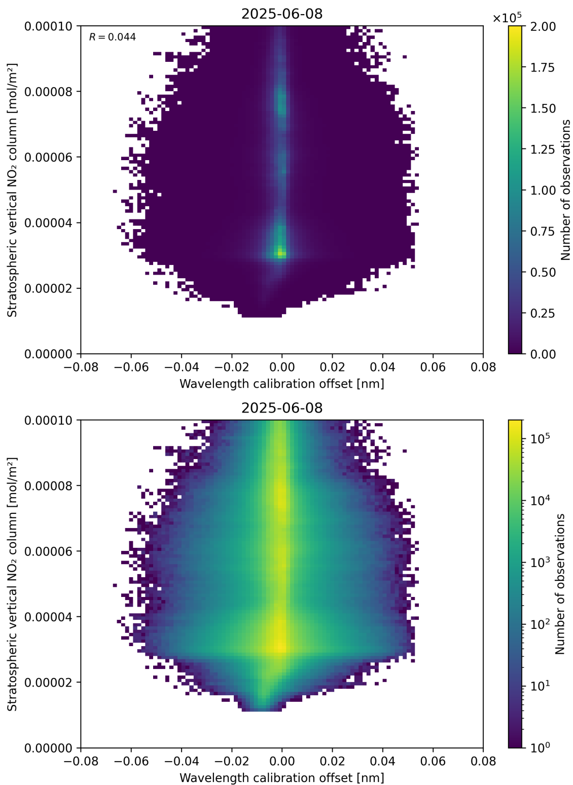
Figure 176: Scatter density plot of “Wavelength calibration offset” against “Stratospheric vertical NO 2 column” for 2025-06-07 to 2025-06-09.
