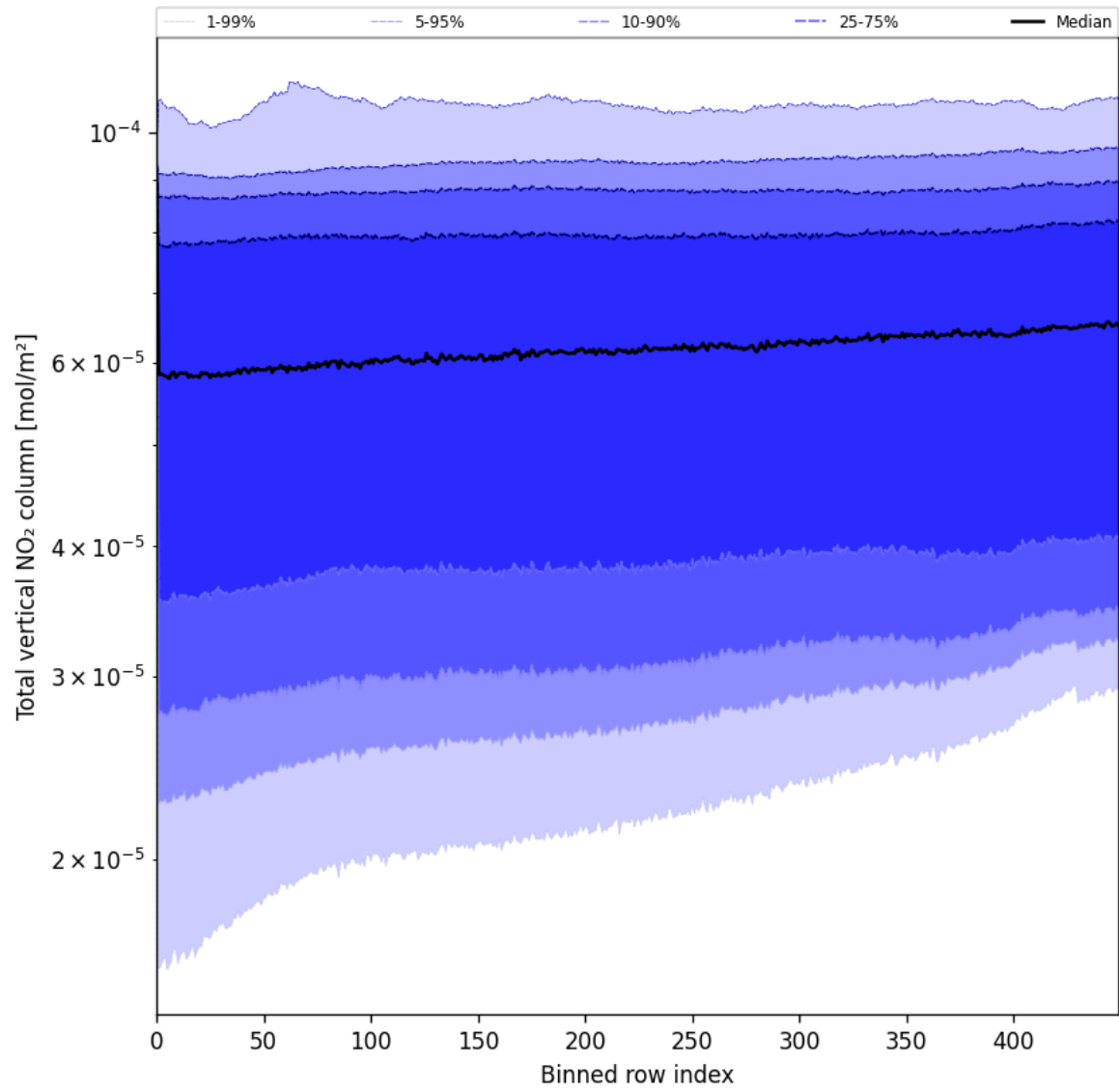
Figure 55: Along track statistics of “Total vertical NO 2 column” for 2025-06-07 to 2025-06-09
