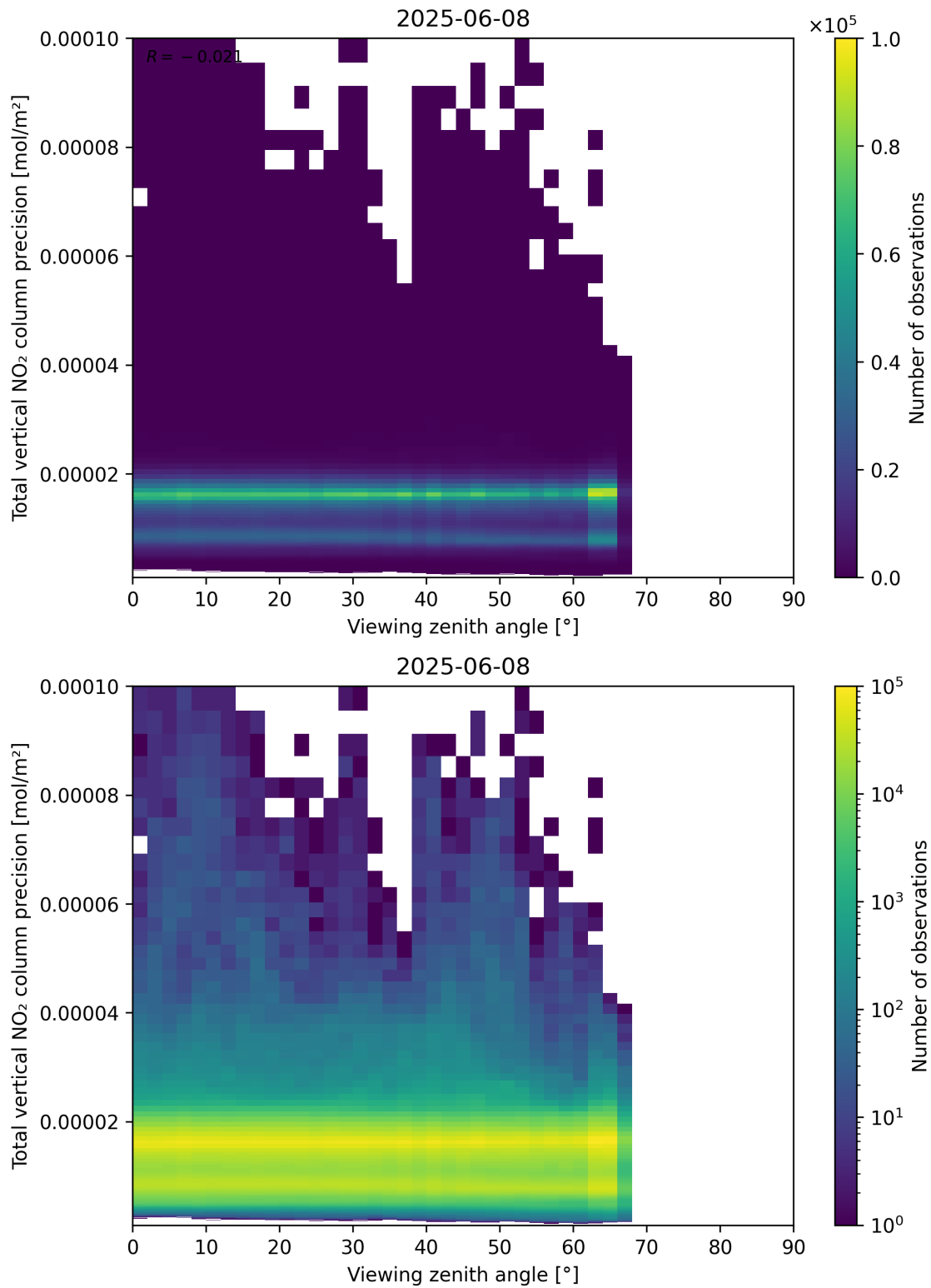
Figure 168: Scatter density plot of “Viewing zenith angle” against “Total vertical NO 2 column precision” for 2025-06-07 to 2025-06-09.
