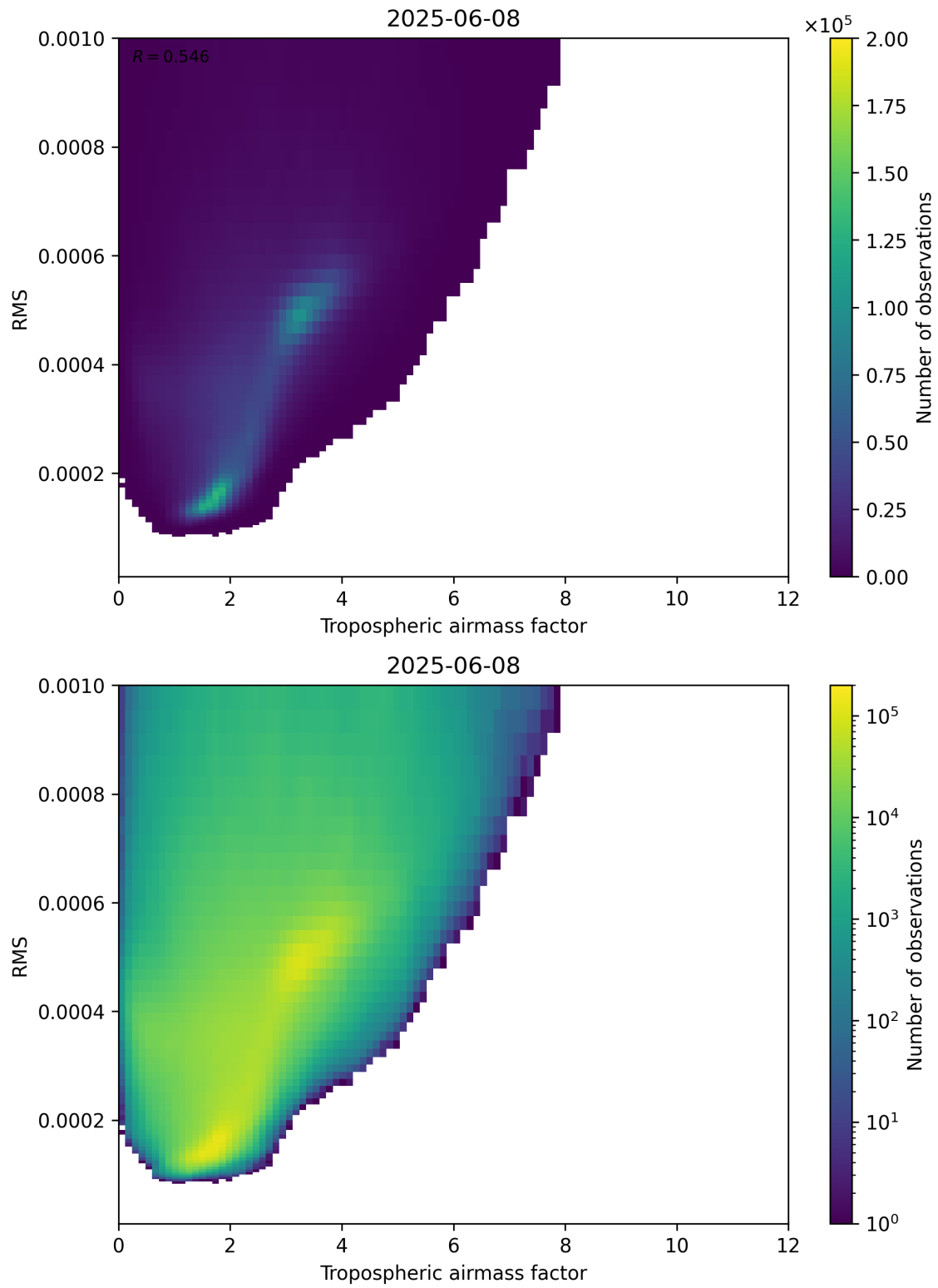
Figure 79: Scatter density plot of “Tropospheric airmass factor” against “RMS” for 2025-06-07 to 2025-06-09.
