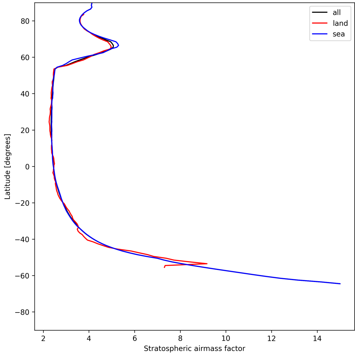
Figure 27: Zonal average of “Stratospheric airmass factor” for 2025-06-07 to 2025-06-09.
