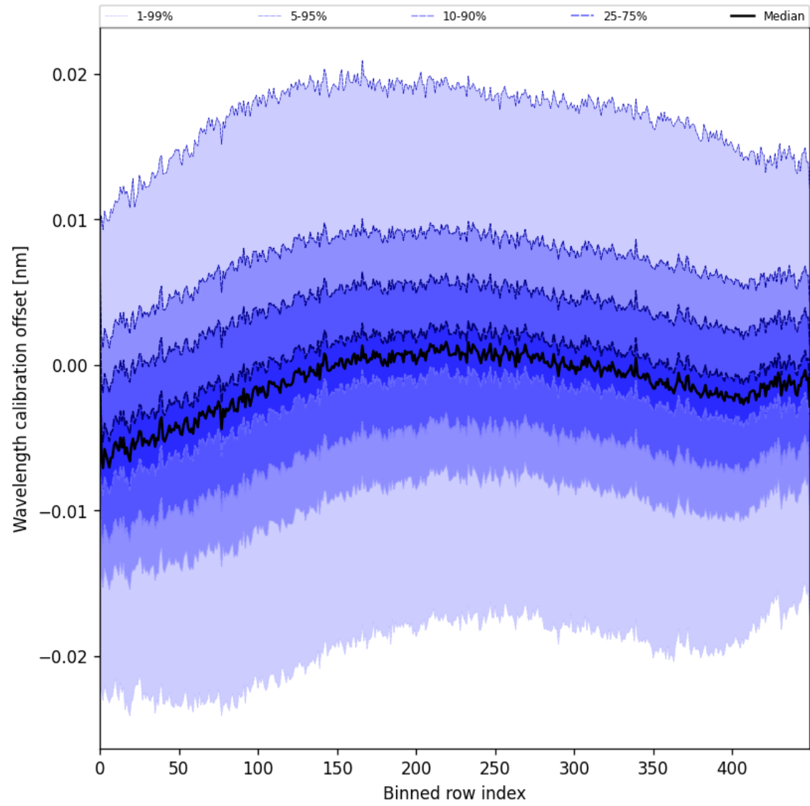
Figure 52: Along track statistics of “Wavelength calibration offset” for 2025-06-07 to 2025-06-09
