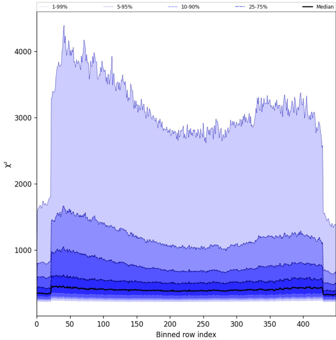
Figure 59: Along track statistics of “ \chi^2 ” for 2025-06-08 to 2025-06-10
