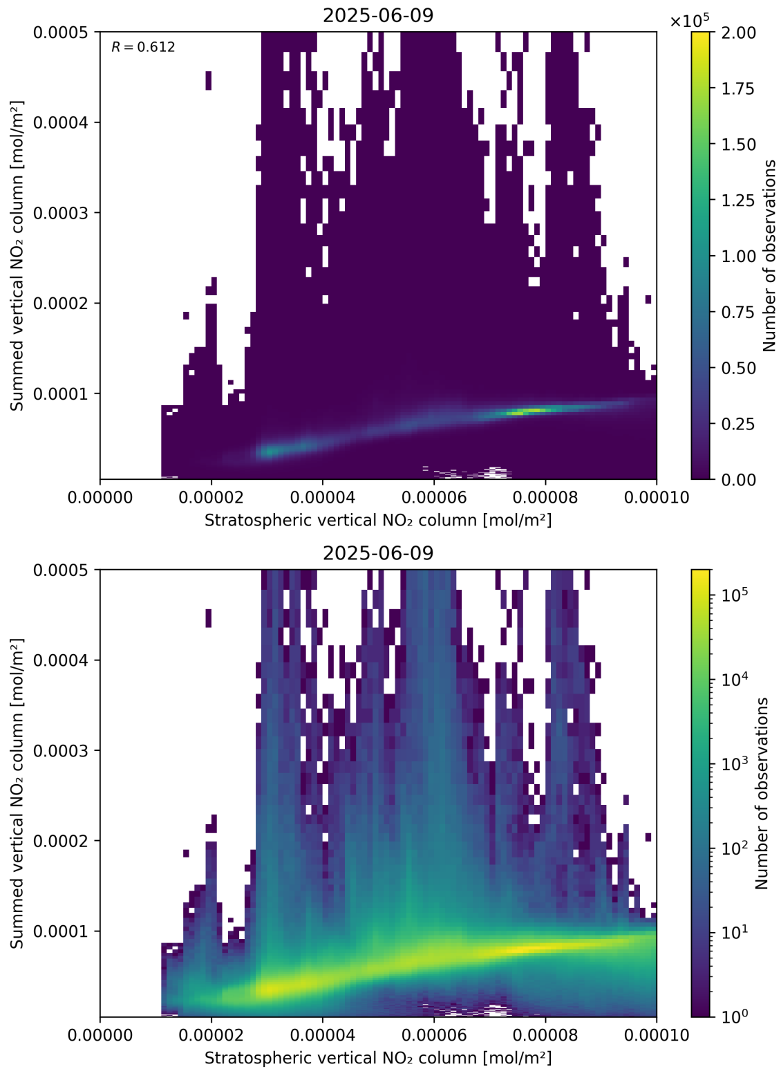
Figure 98: Scatter density plot of “Stratospheric vertical NO 2 column” against “Summed vertical NO 2 column” for 2025-06-08 to 2025-06-10.
