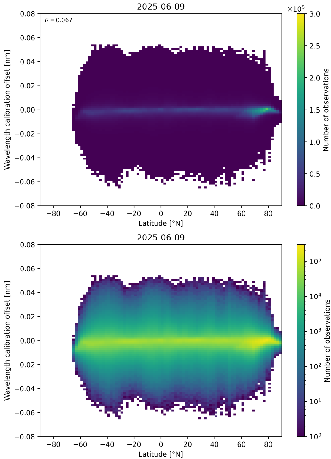
Figure 95: Scatter density plot of “Latitude” against “Wavelength calibration offset” for 2025-06-08 to 2025-06-10.
