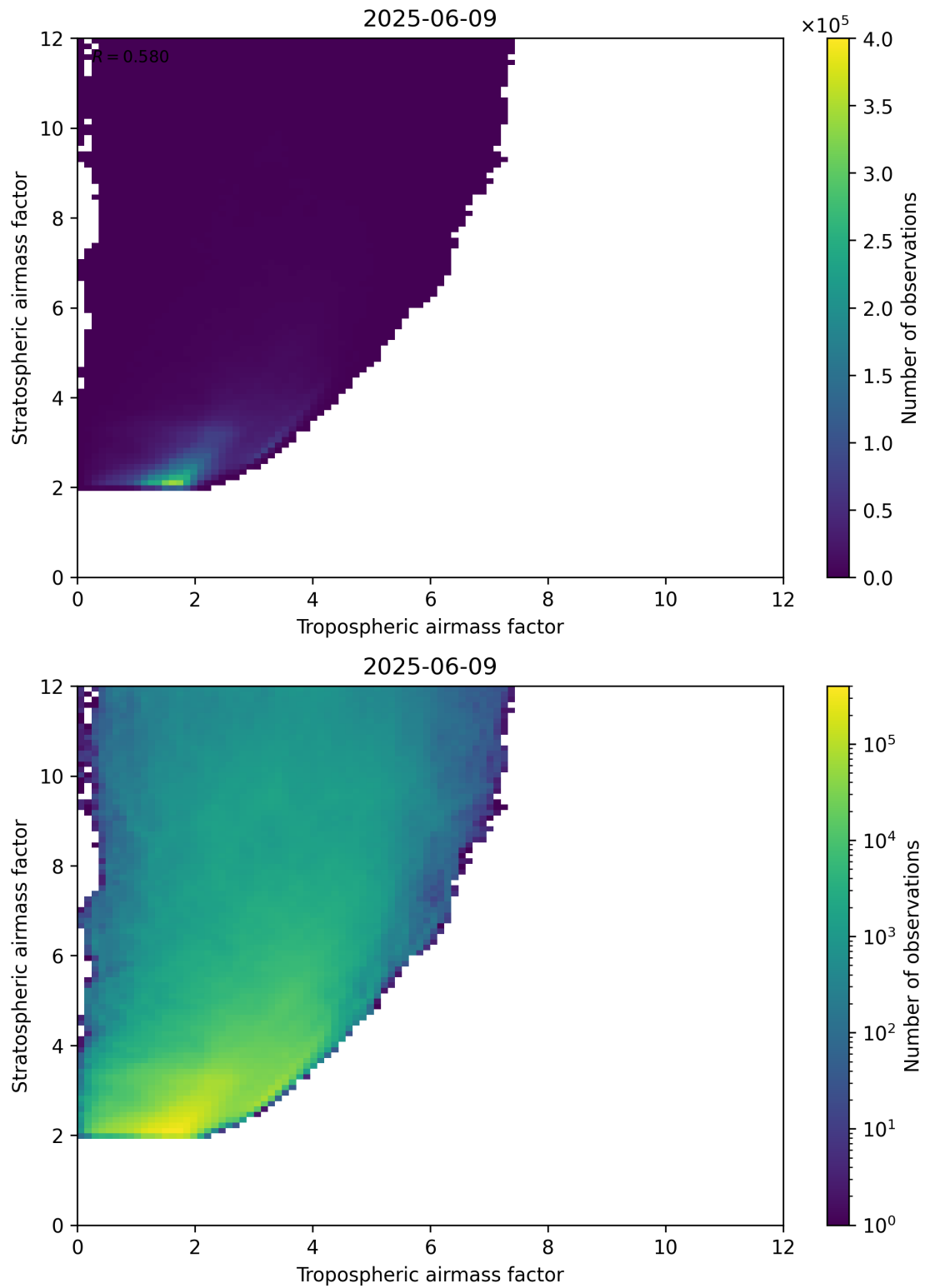
Figure 71: Scatter density plot of “Tropospheric airmass factor” against “Stratospheric airmass factor” for 2025-06-08 to 2025-06-10.
