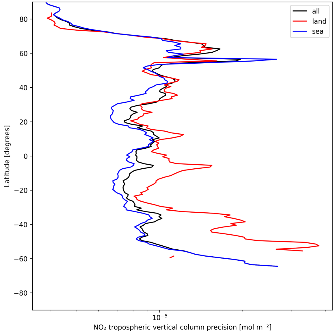
Figure 13: Zonal average of “NO 2 tropospheric vertical column precision” for 2025-06-08 to 2025-06-10.
