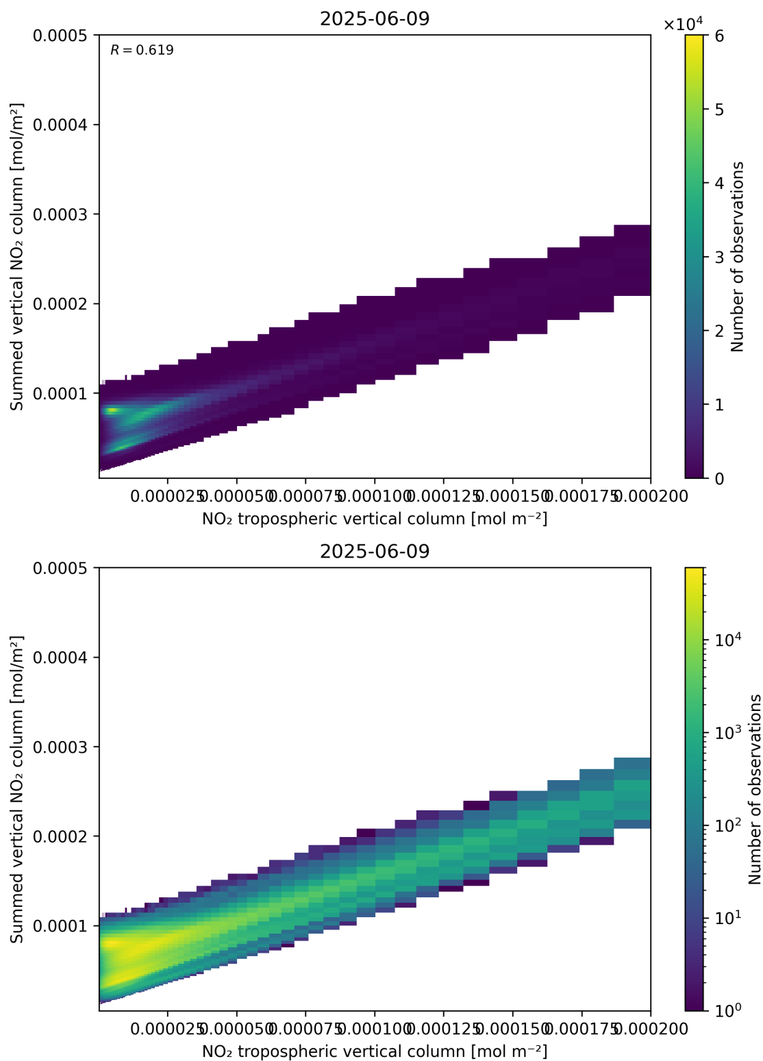
Figure 126: Scatter density plot of “NO 2 tropospheric vertical column” against “Summed vertical NO 2 column” for 2025-06-08 to 2025-06-10.
