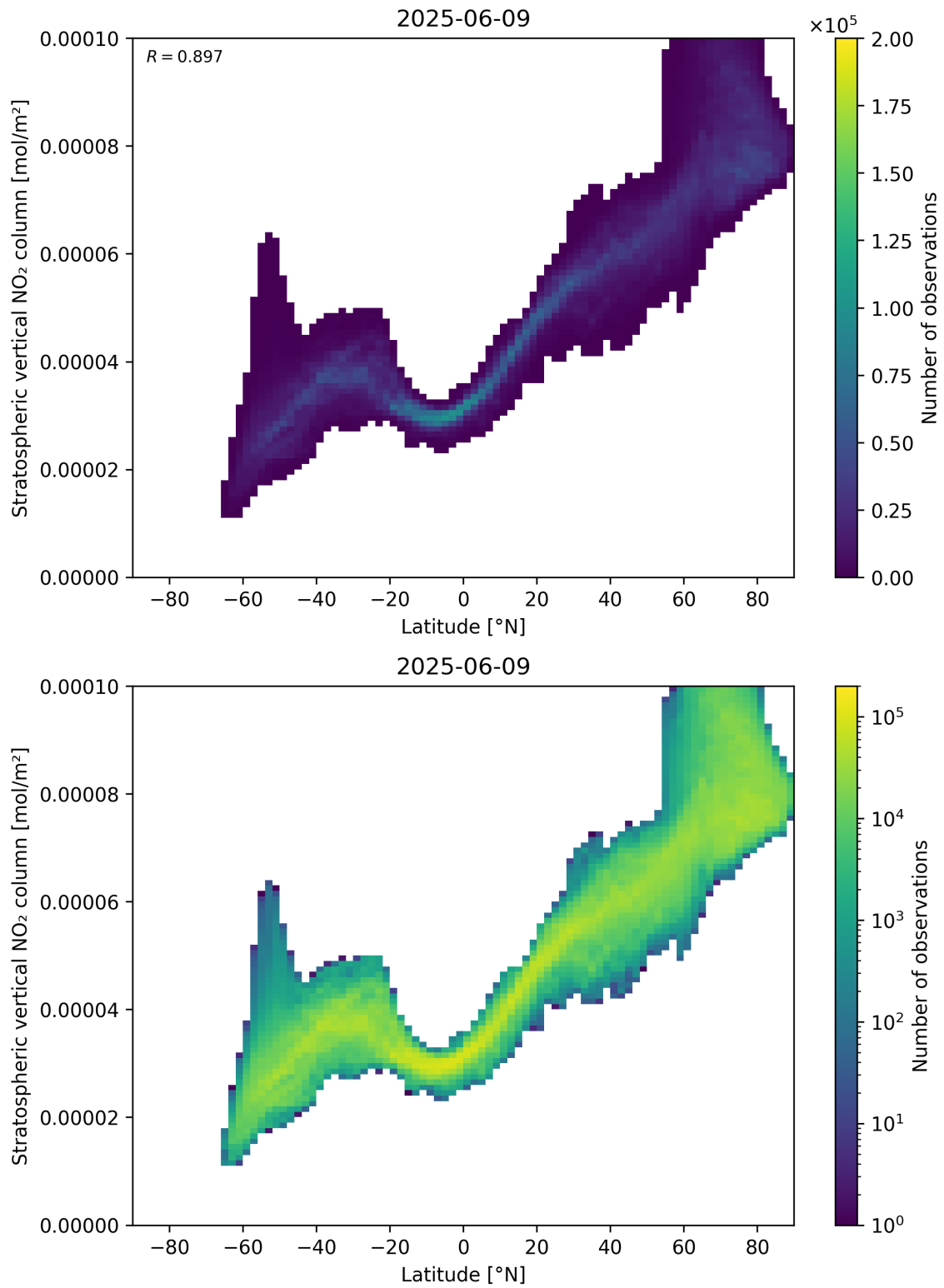
Figure 87: Scatter density plot of “Latitude” against “Stratospheric vertical \text{NO}_2 column” for 2025-06-08 to 2025-06-10.
