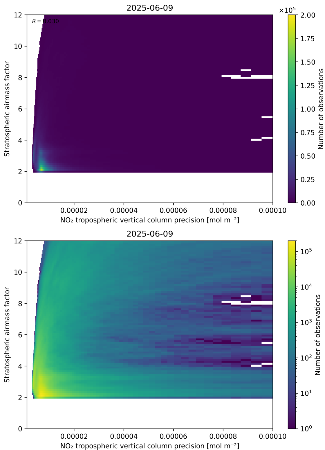
Figure 131: Scatter density plot of “NO 2 tropospheric vertical column precision” against “Stratospheric airmass factor” for 2025-06-08 to 2025-06-10.
