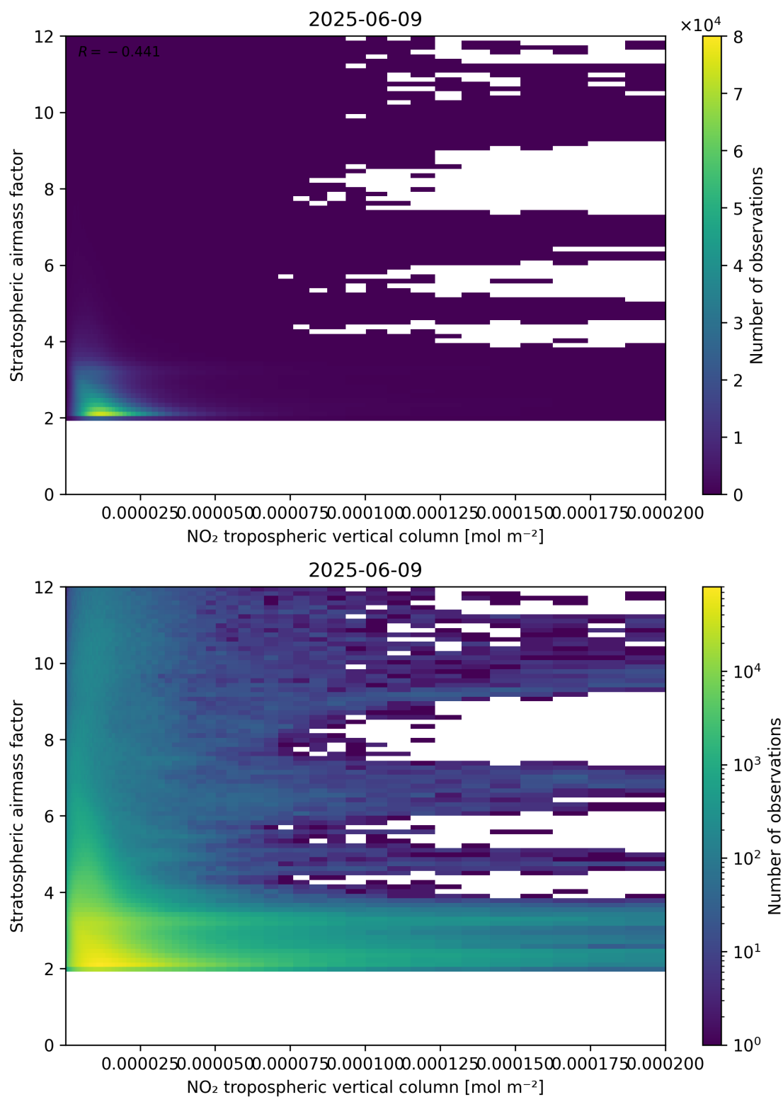
Figure 121: Scatter density plot of “NO 2 tropospheric vertical column” against “Stratospheric air mass factor” for 2025-06-08 to 2025-06-10.
