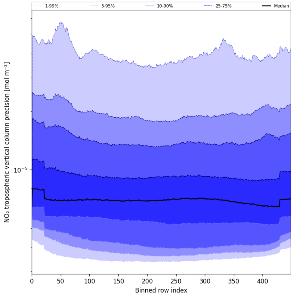
Figure 47: Along track statistics of “NO 2 tropospheric vertical column precision” for 2025-06-08 to 2025-06-10
