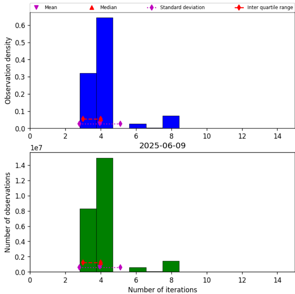
Figure 34: Histogram of “Number of iterations” for 2025-06-08 to 2025-06-10
