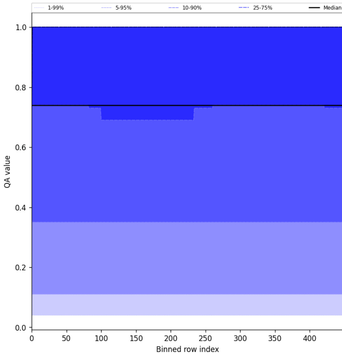
Figure 45: Along track statistics of “QA value” for 2025-06-08 to 2025-06-10
