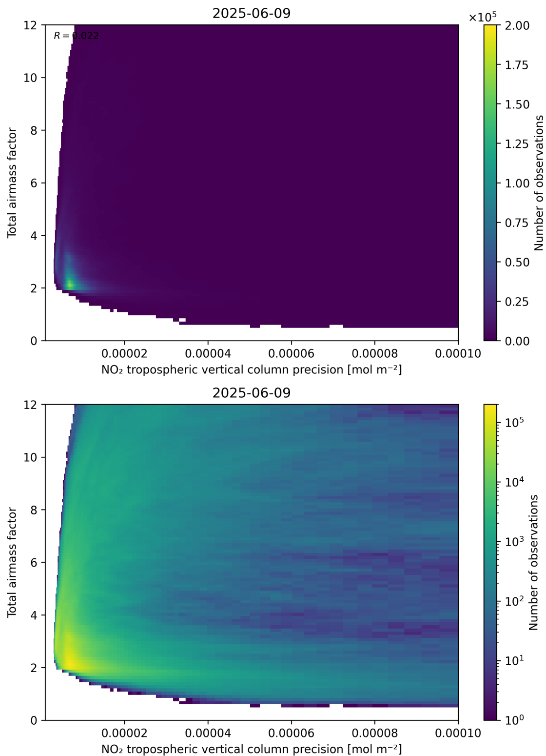
Figure 132: Scatter density plot of “NO 2 tropospheric vertical column precision” against “Total air mass factor” for 2025-06-08 to 2025-06-10.
