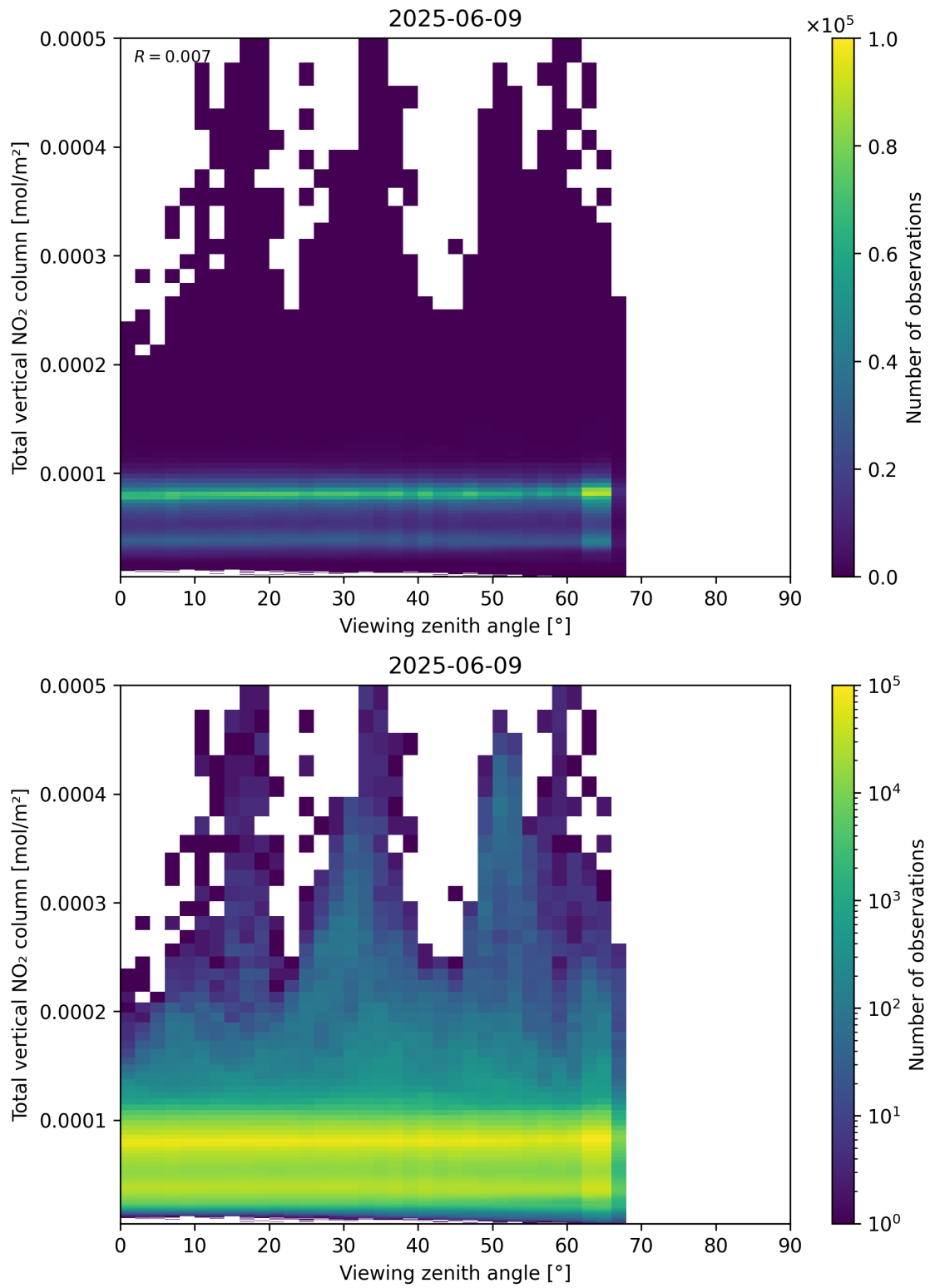
Figure 167: Scatter density plot of “Viewing zenith angle” against “Total vertical NO 2 column” for 2025-06-08 to 2025-06-10.
