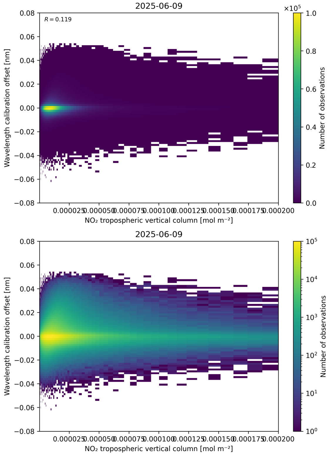
Figure 143: Scatter density plot of “NO 2 tropospheric vertical column” against “Wavelength calibration offset” for 2025-06-08 to 2025-06-10.
