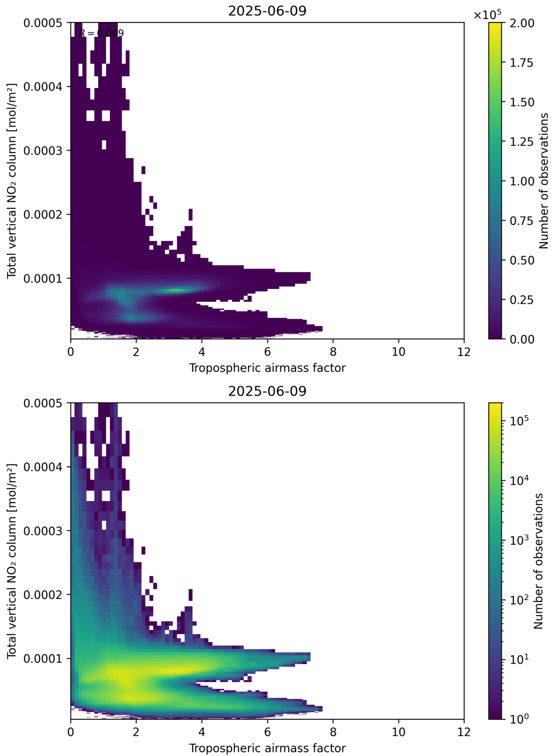
Figure 77: Scatter density plot of “Tropospheric airmass factor” against “Total vertical NO 2 column” for 2025-06-08 to 2025-06-10.
