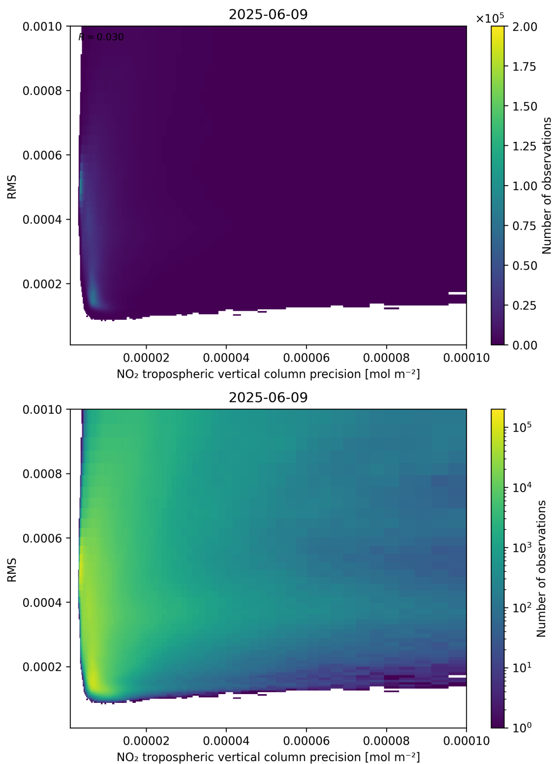
Figure 140: Scatter density plot of “NO 2 tropospheric vertical column precision” against “RMS” for 2025-06-08 to 2025-06-10.
