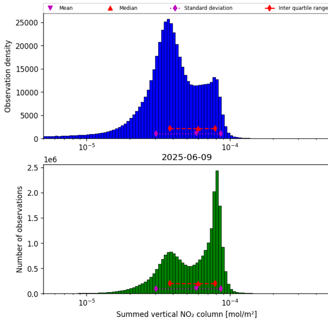
Figure 40: Histogram of “Summed vertical NO 2 column” for 2025-06-08 to 2025-06-10
