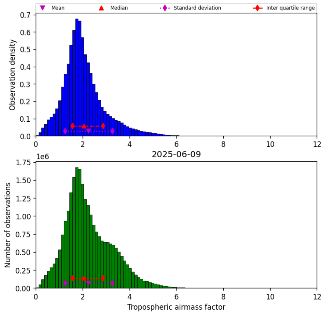
Figure 31: Histogram of “Tropospheric airmass factor” for 2025-06-08 to 2025-06-10
