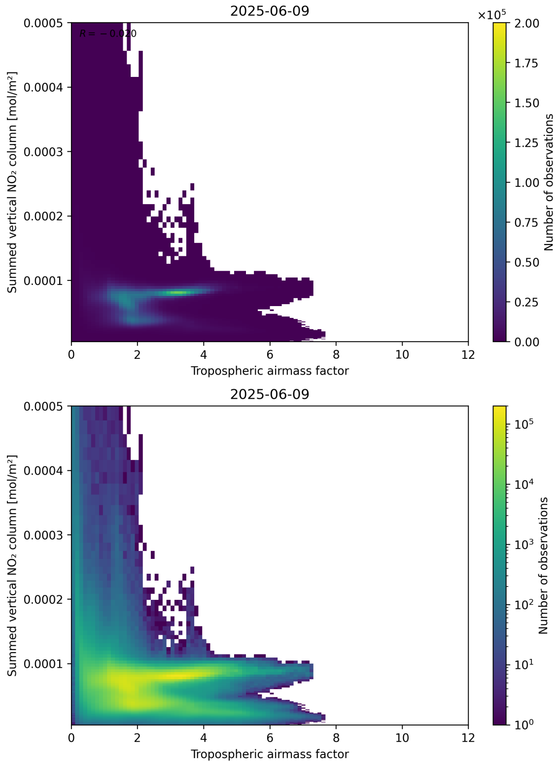
Figure 75: Scatter density plot of “Tropospheric airmass factor” against “Summed vertical NO 2 column” for 2025-06-08 to 2025-06-10.
