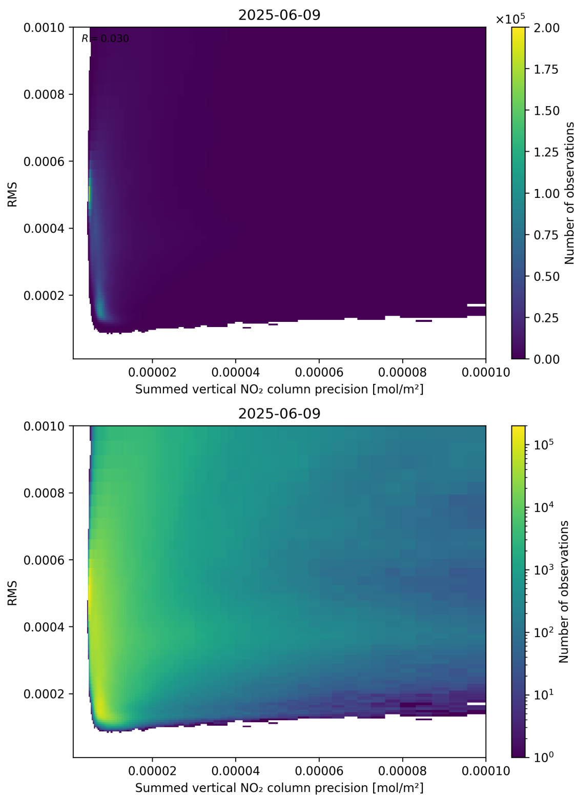
Figure 108: Scatter density plot of “Summed vertical NO 2 column precision” against “RMS” for 2025-06-08 to 2025-06-10.
