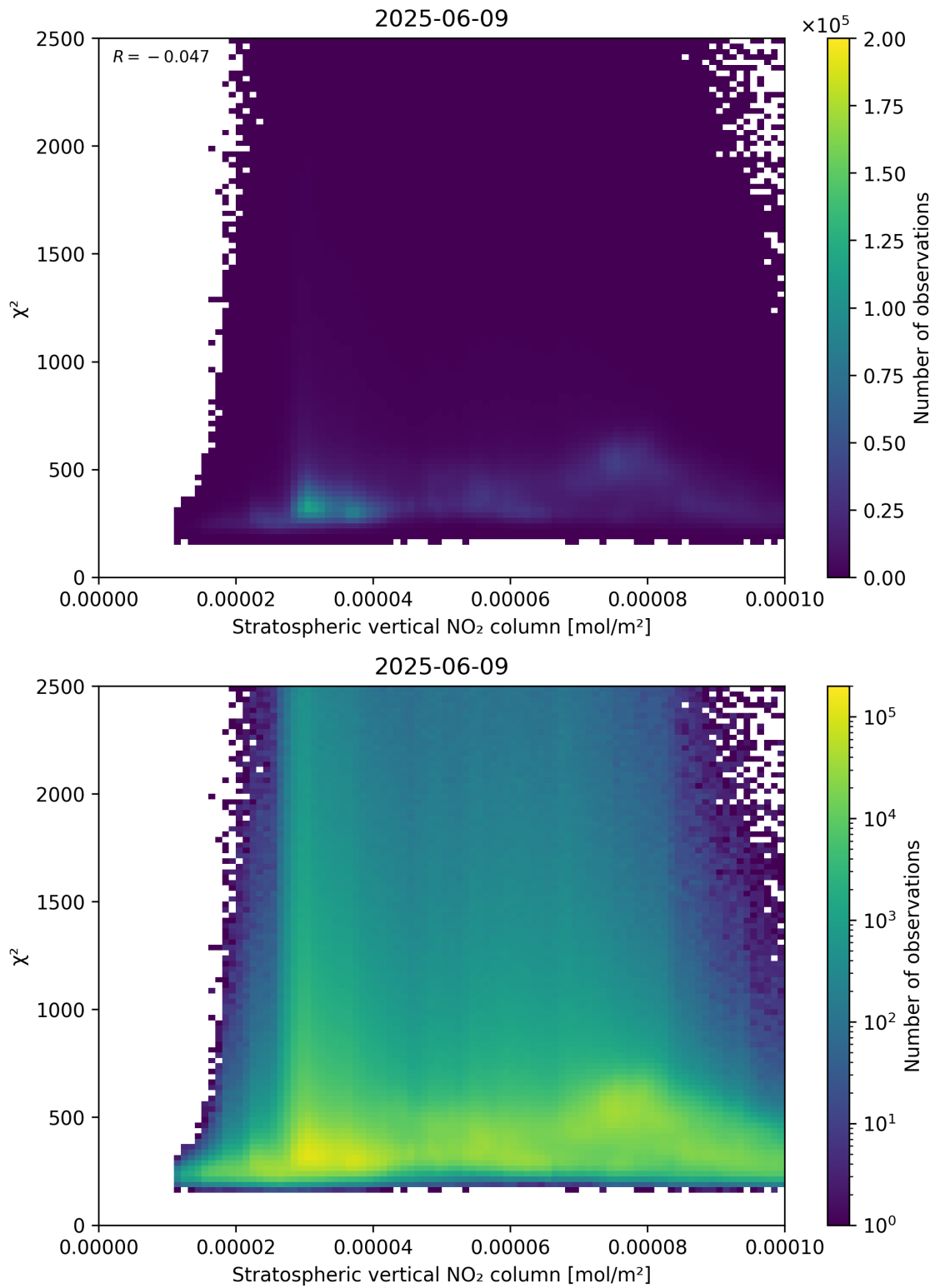
Figure 97: Scatter density plot of “Stratospheric vertical NO 2 column” against “ \chi^2 ” for 2025-06-08 to 2025-06-10.
