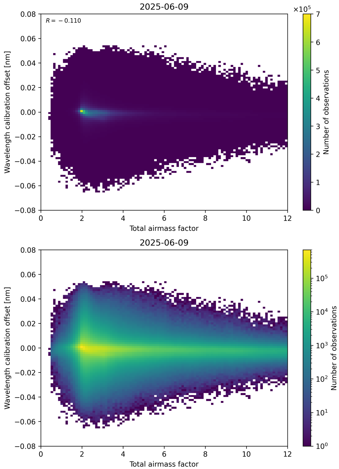
Figure 70: Scatter density plot of “Total airmass factor” against “Wavelength calibration offset” for 2025-06-08 to 2025-06-10.
