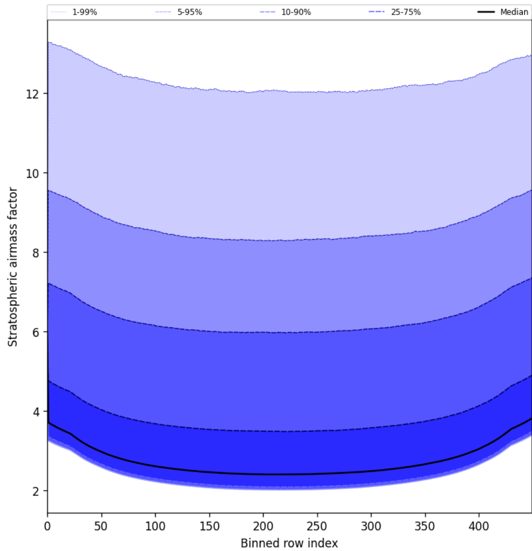
Figure 61: Along track statistics of “Stratospheric airmass factor” for 2025-06-08 to 2025-06-10
