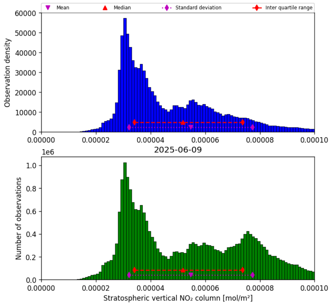
Figure 36: Histogram of “Stratospheric vertical NO 2 column” for 2025-06-08 to 2025-06-10
