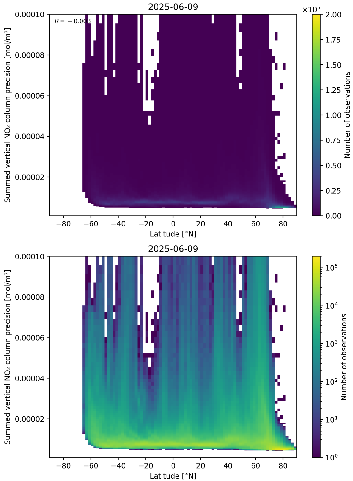
Figure 89: Scatter density plot of “Latitude” against “Summed vertical NO 2 column precision” for 2025-06-08 to 2025-06-10.
