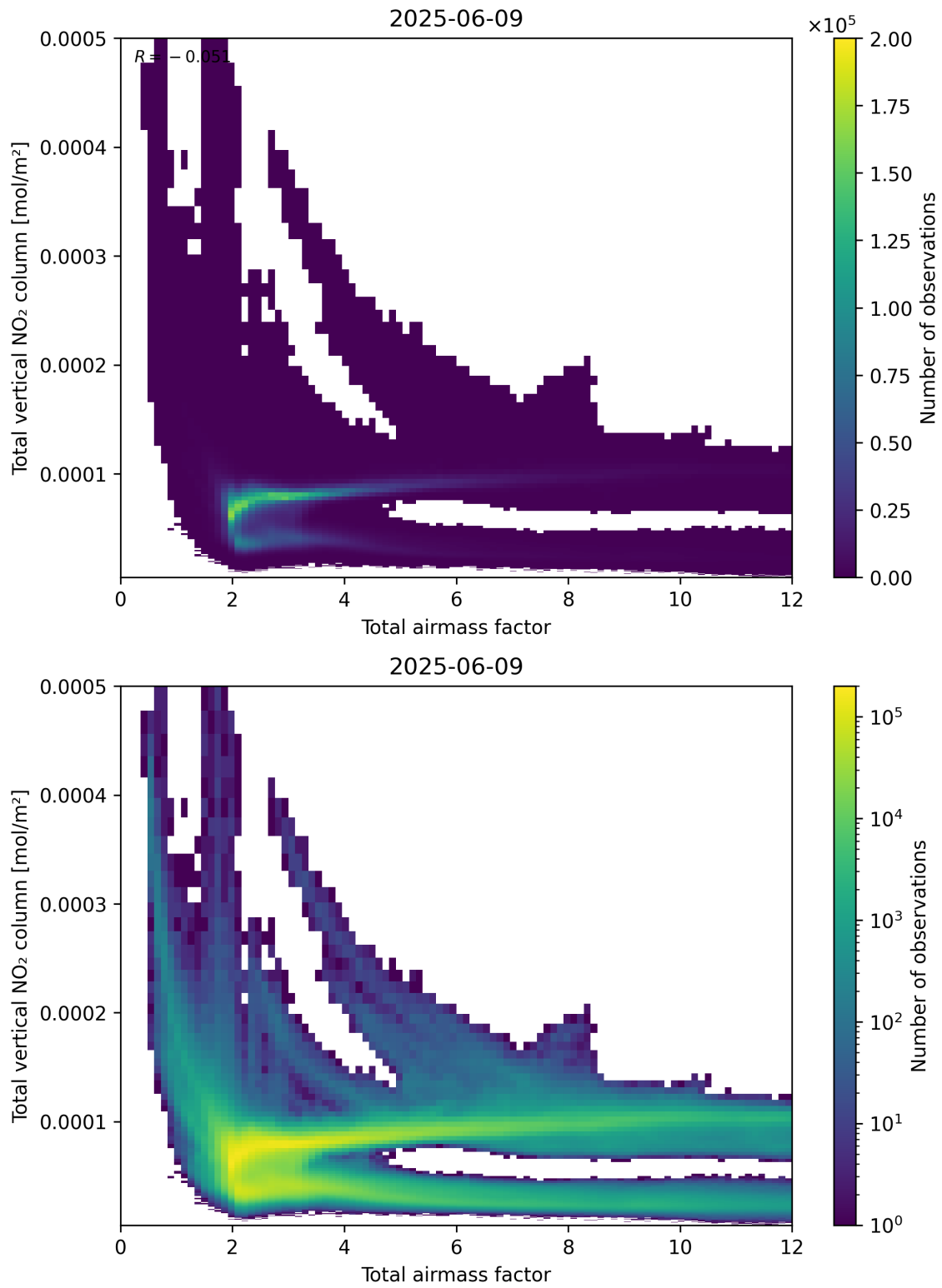
Figure 67: Scatter density plot of “Total airmass factor” against “Total vertical NO 2 column” for 2025-06-08 to 2025-06-10.
