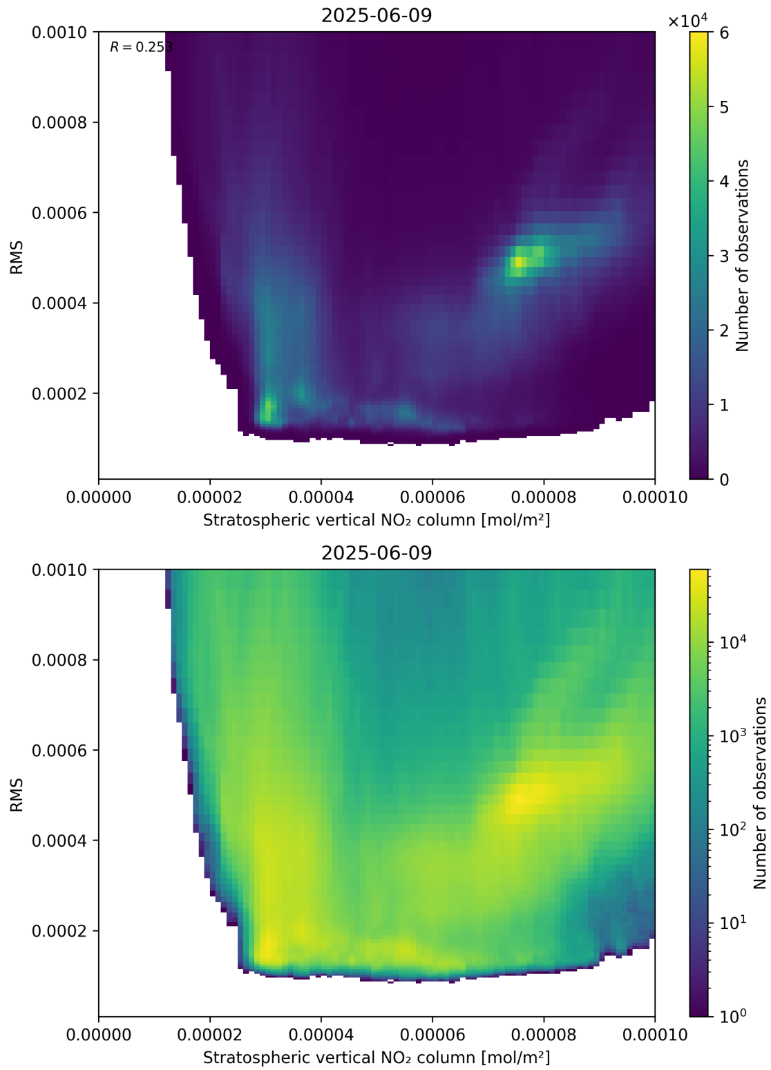
Figure 102: Scatter density plot of “Stratospheric vertical NO 2 column” against “RMS” for 2025-06-08 to 2025-06-10.
