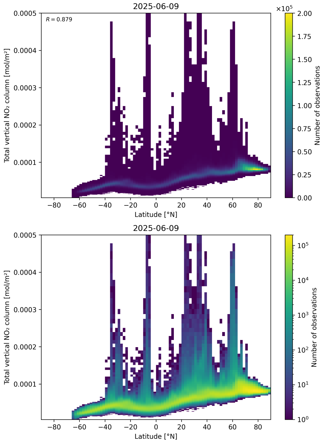
Figure 90: Scatter density plot of “Latitude” against “Total vertical NO 2 column” for 2025-06-08 to 2025-06-10.
