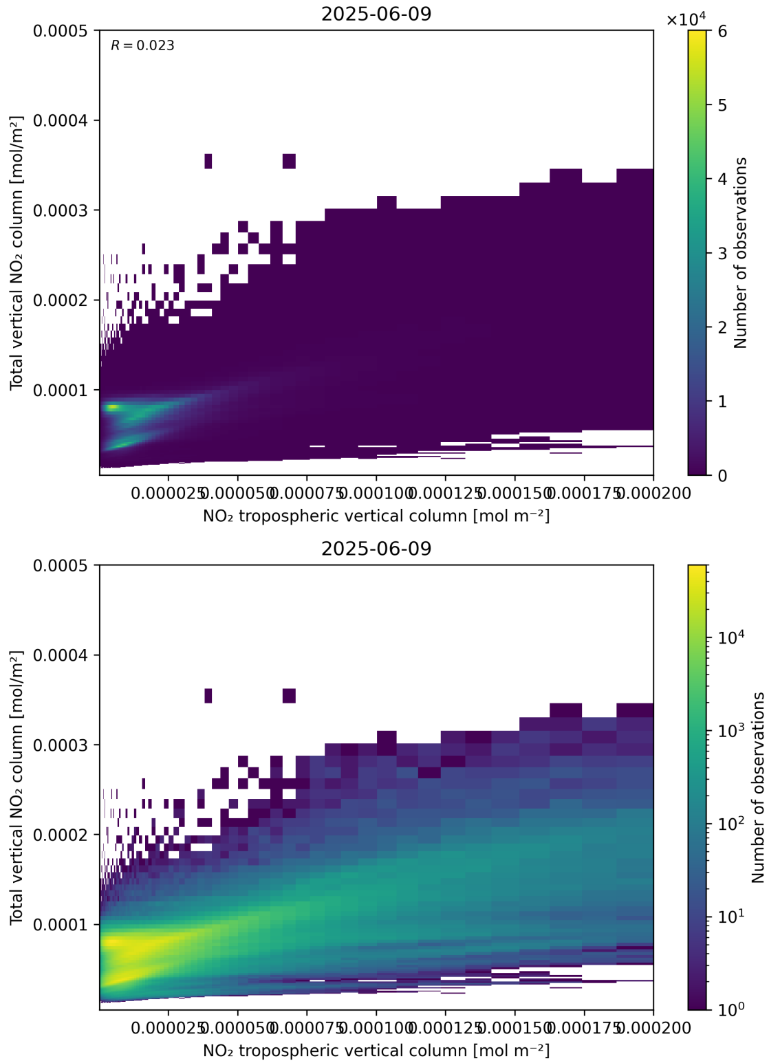
Figure 128: Scatter density plot of “NO 2 tropospheric vertical column” against “Total vertical NO 2 column” for 2025-06-08 to 2025-06-10.
