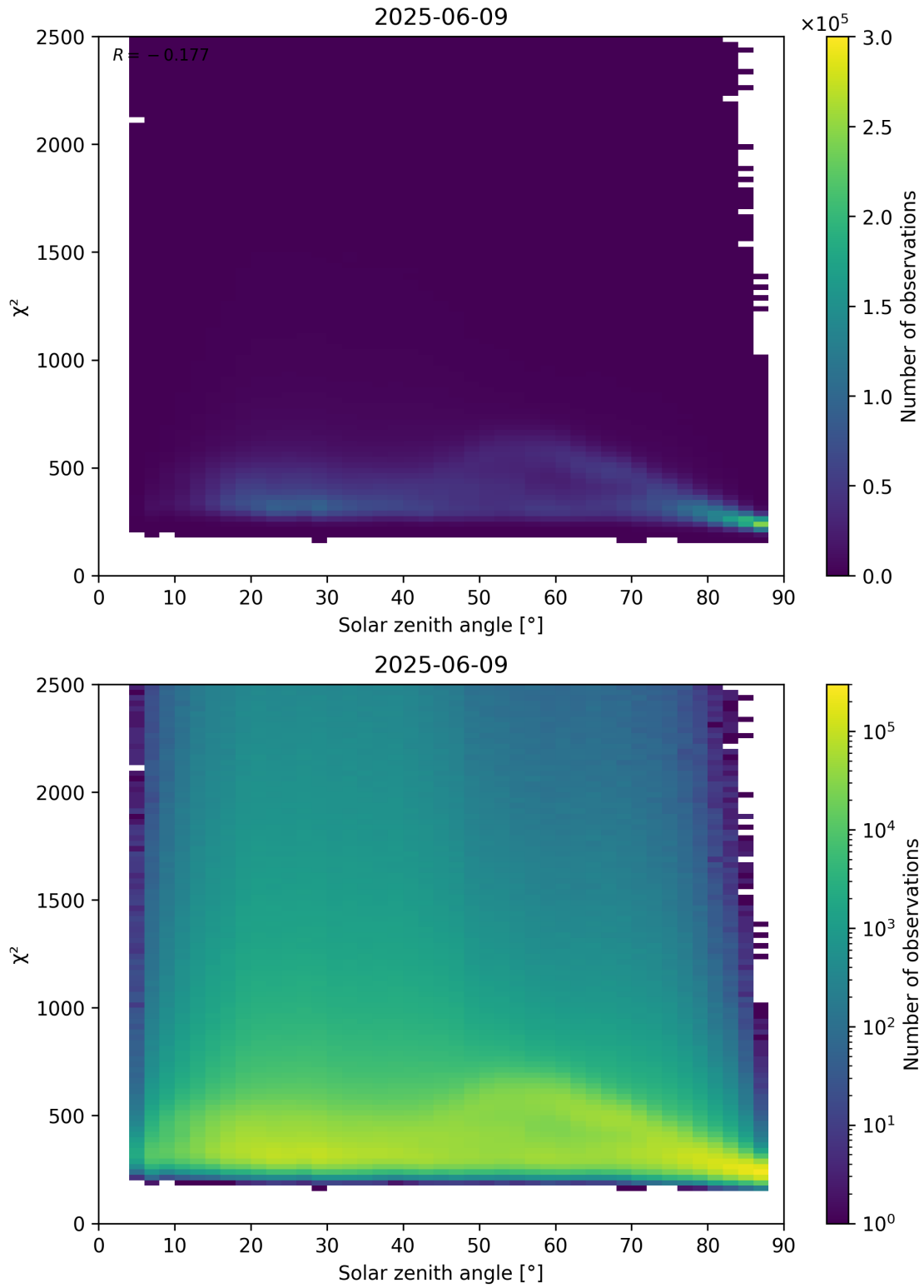
Figure 148: Scatter density plot of “Solar zenith angle” against “ \chi^2 ” for 2025-06-08 to 2025-06-10.
