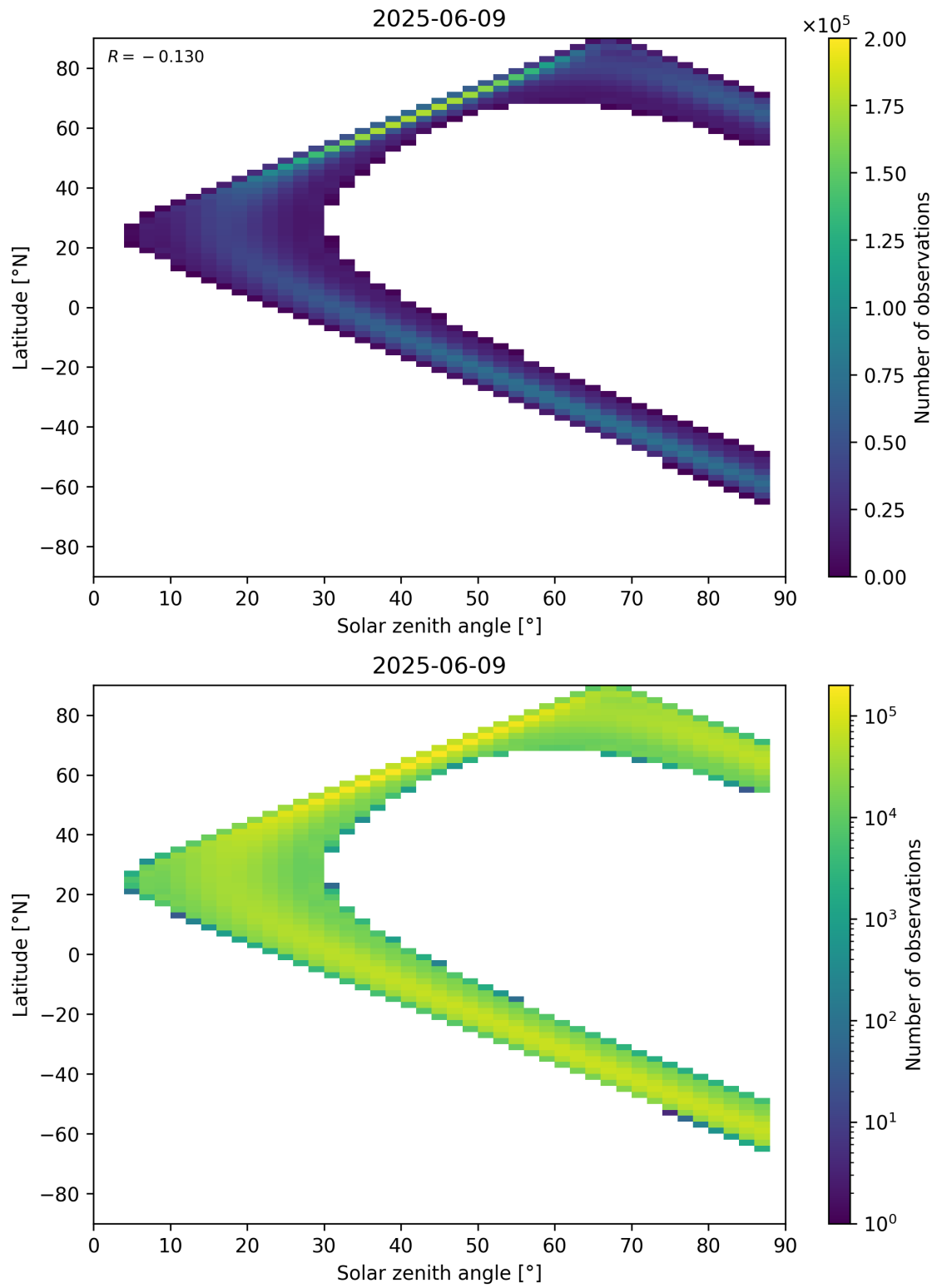
Figure 149: Scatter density plot of “Solar zenith angle” against “Latitude” for 2025-06-08 to 2025-06-10.
