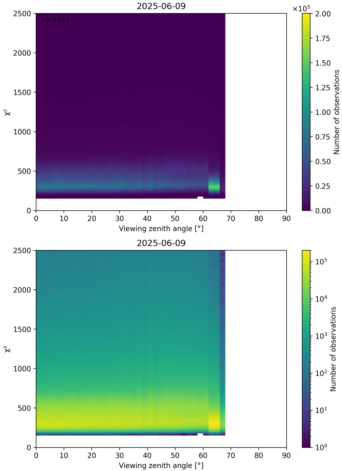
Figure 162: Scatter density plot of “Viewing zenith angle” against “ \chi^2 ” for 2025-06-08 to 2025-06-10.
