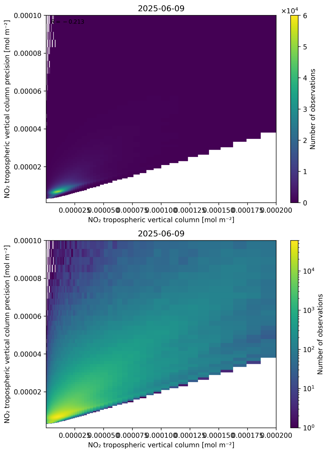
Figure 130: Scatter density plot of “NO 2 tropospheric vertical column” against “NO 2 tropospheric vertical column precision” for 2025-06-08 to 2025-06-10.
