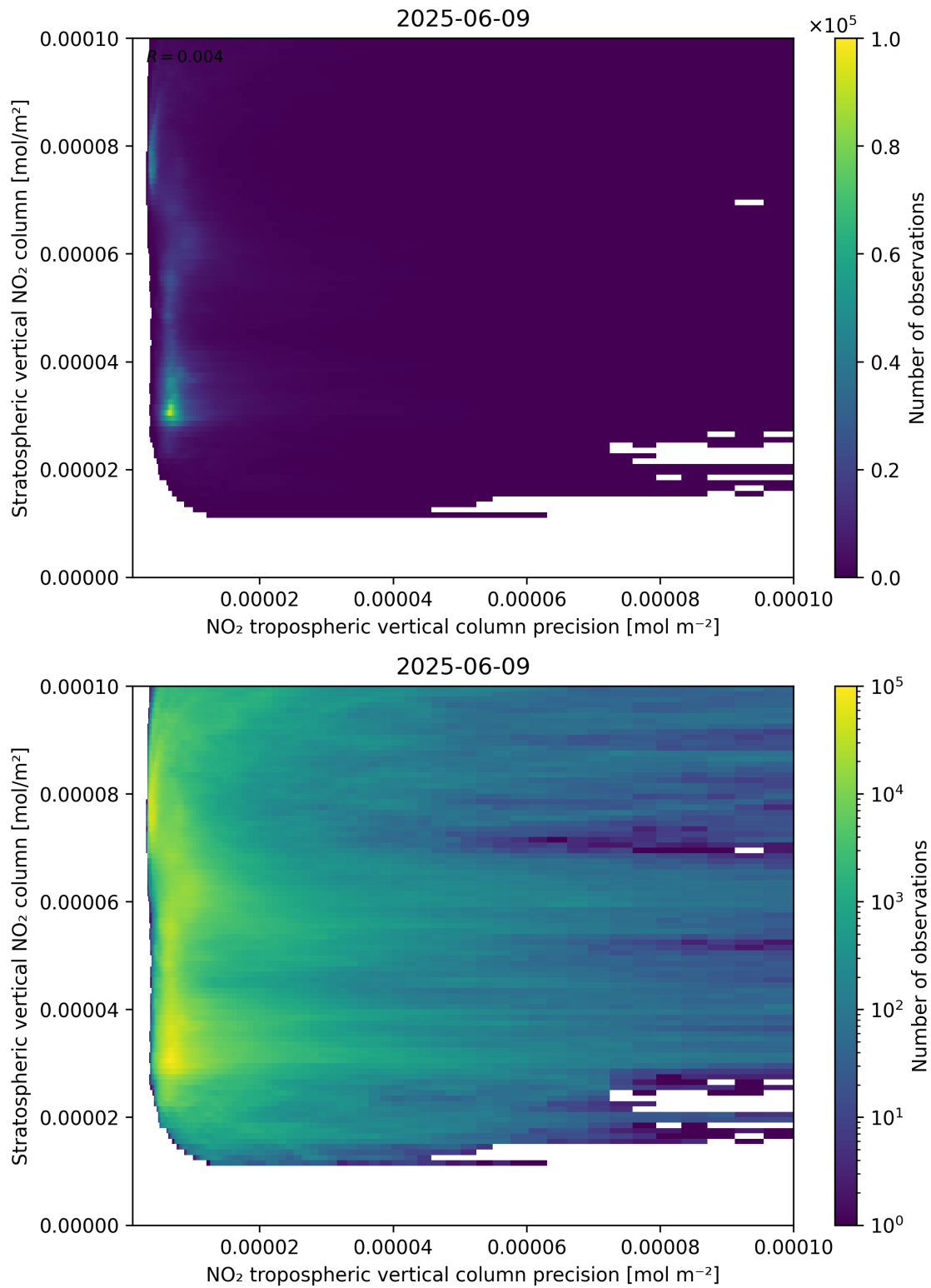
Figure 135: Scatter density plot of “NO 2 tropospheric vertical column precision” against “Stratospheric vertical NO 2 column” for 2025-06-08 to 2025-06-10.
