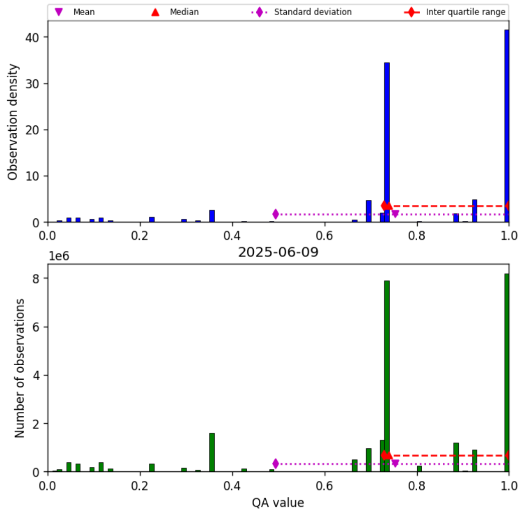
Figure 28: Histogram of “QA value” for 2025-06-08 to 2025-06-10
