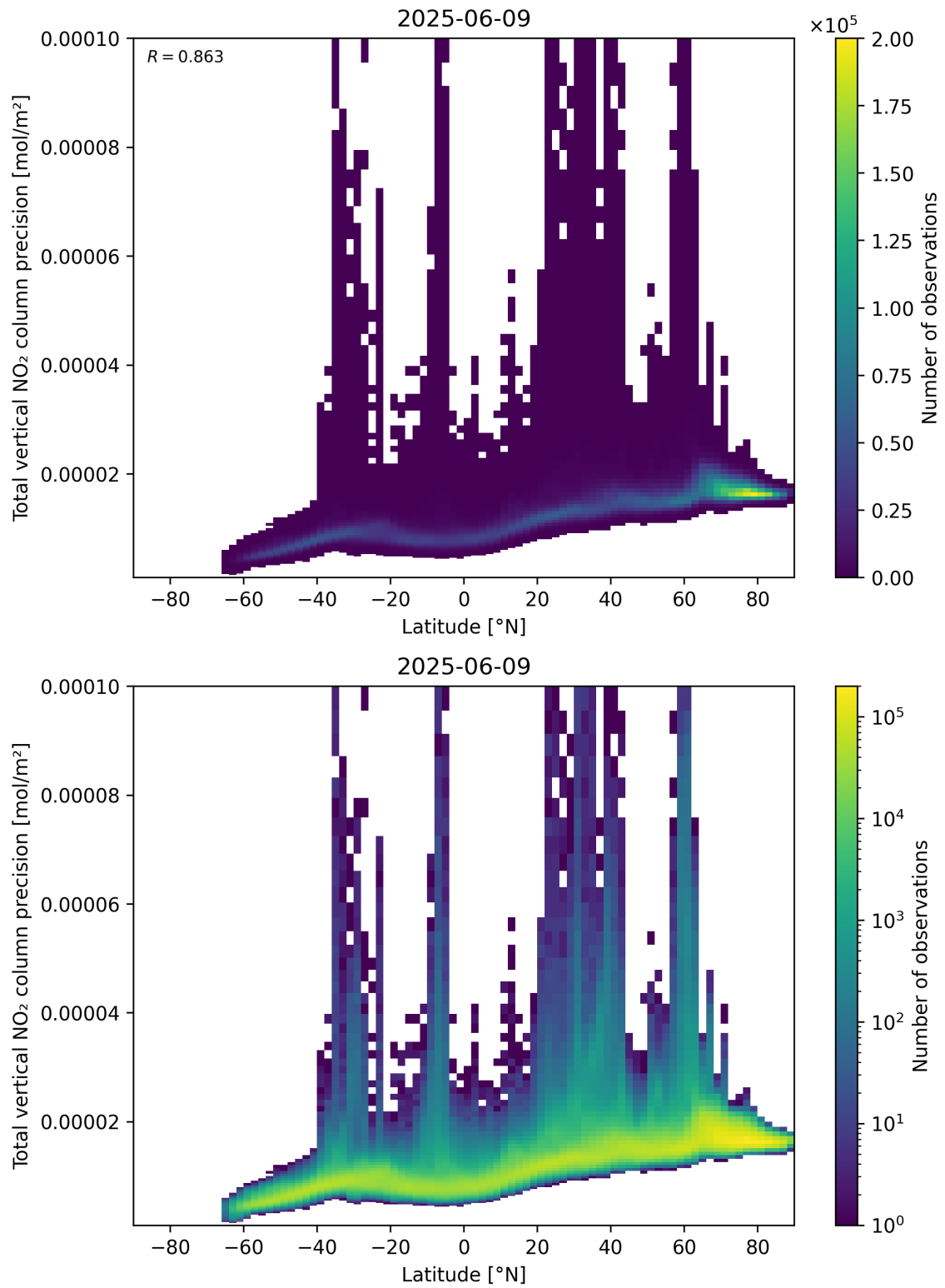
Figure 91: Scatter density plot of “Latitude” against “Total vertical NO 2 column precision” for 2025-06-08 to 2025-06-10.
