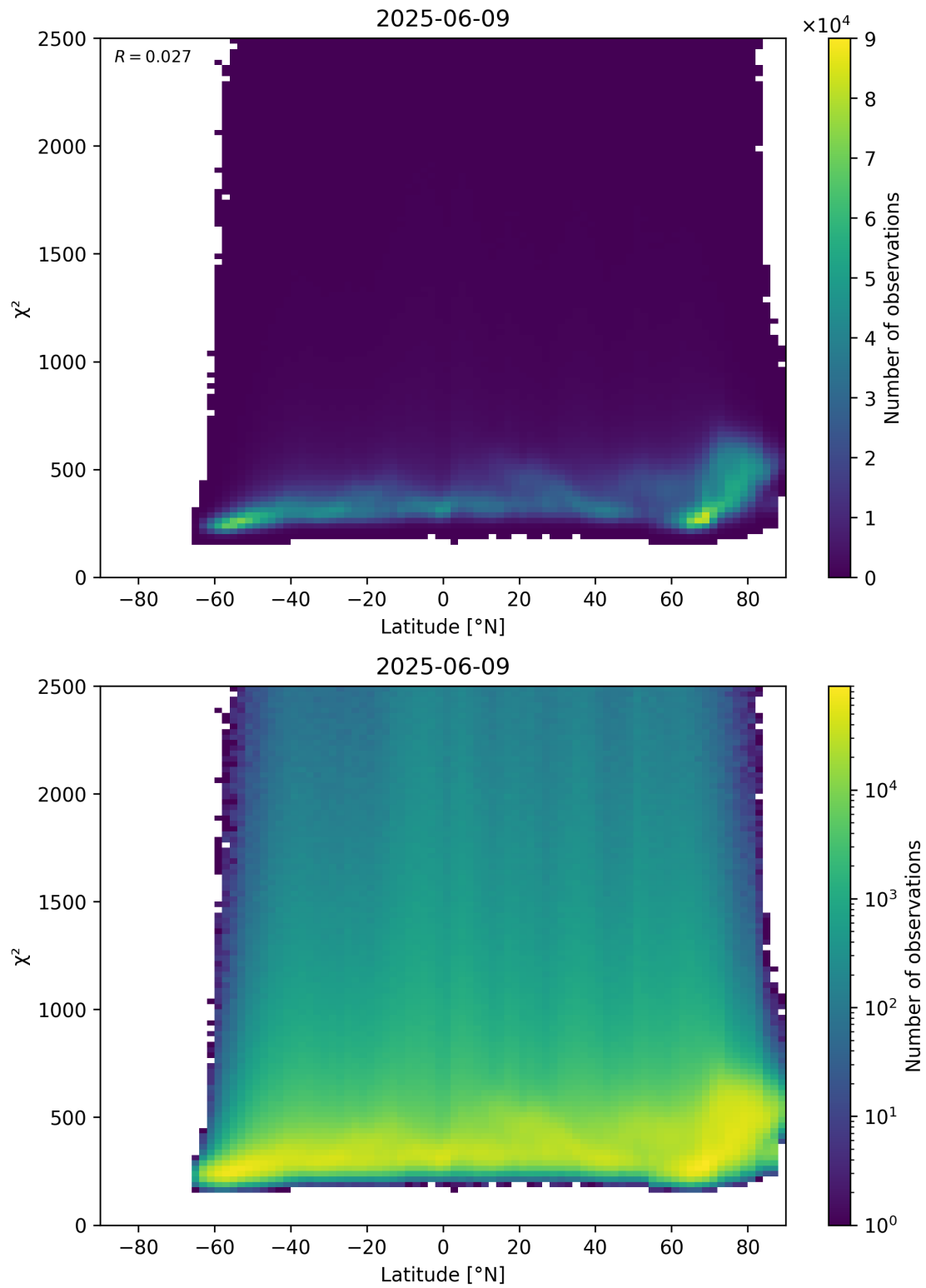
Figure 86: Scatter density plot of “Latitude” against “ \chi^2 ” for 2025-06-08 to 2025-06-10.
