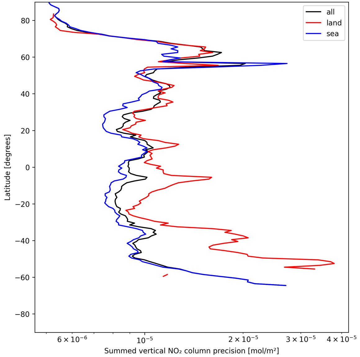
Figure 24: Zonal average of “Summed vertical NO 2 column precision” for 2025-06-08 to 2025-06-10.
