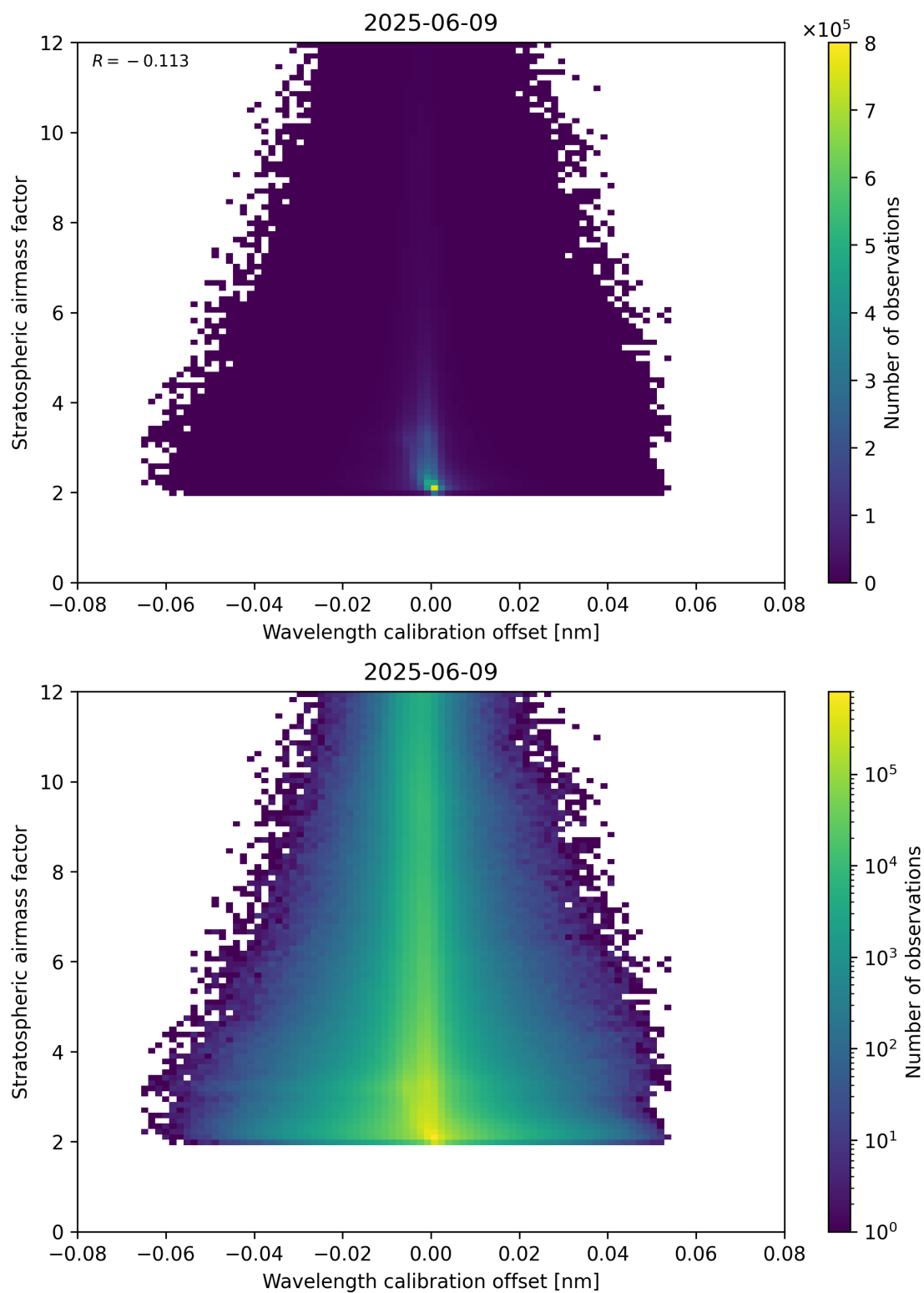
Figure 174: Scatter density plot of “Wavelength calibration offset” against “Stratospheric airmass factor” for 2025-06-08 to 2025-06-10.
