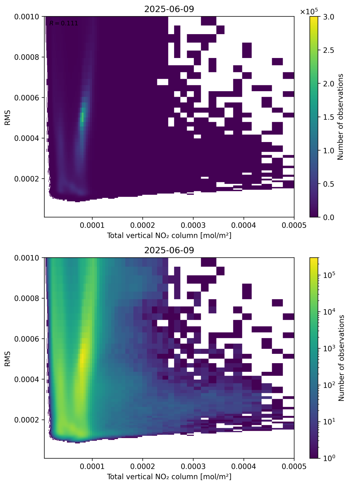
Figure 120: Scatter density plot of “Total vertical NO 2 column” against “RMS” for 2025-06-08 to 2025-06-10.
