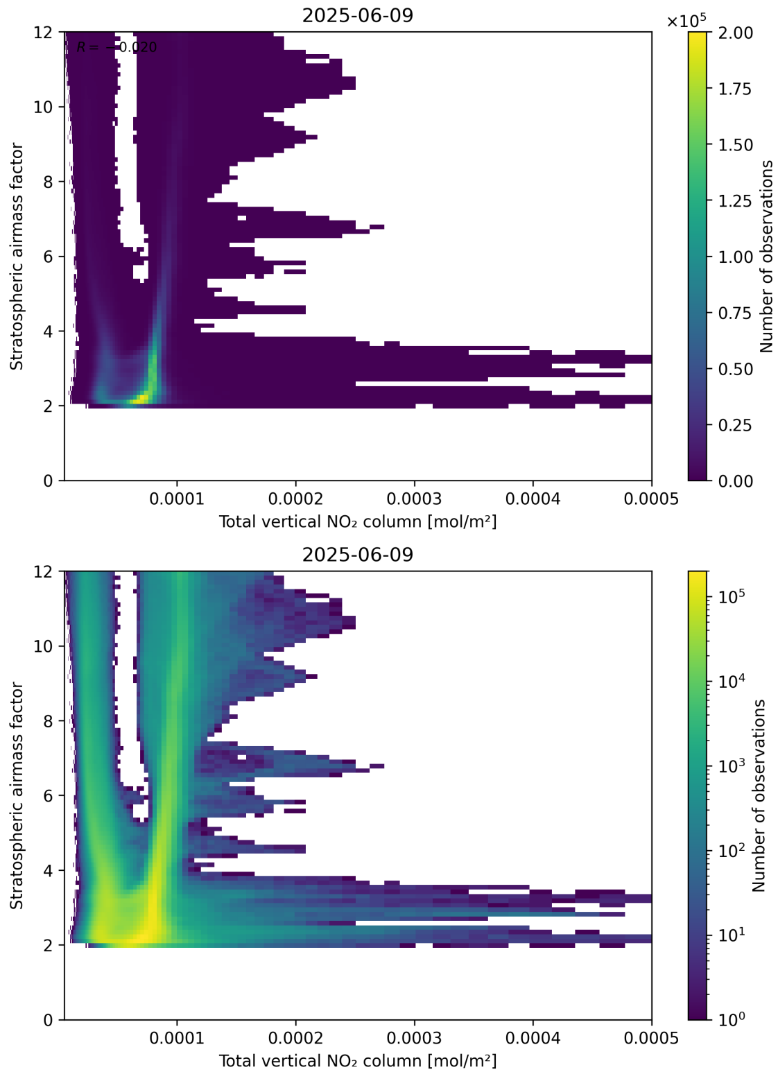
Figure 110: Scatter density plot of “Total vertical NO 2 column” against “Stratospheric airmass factor” for 2025-06-08 to 2025-06-10.
