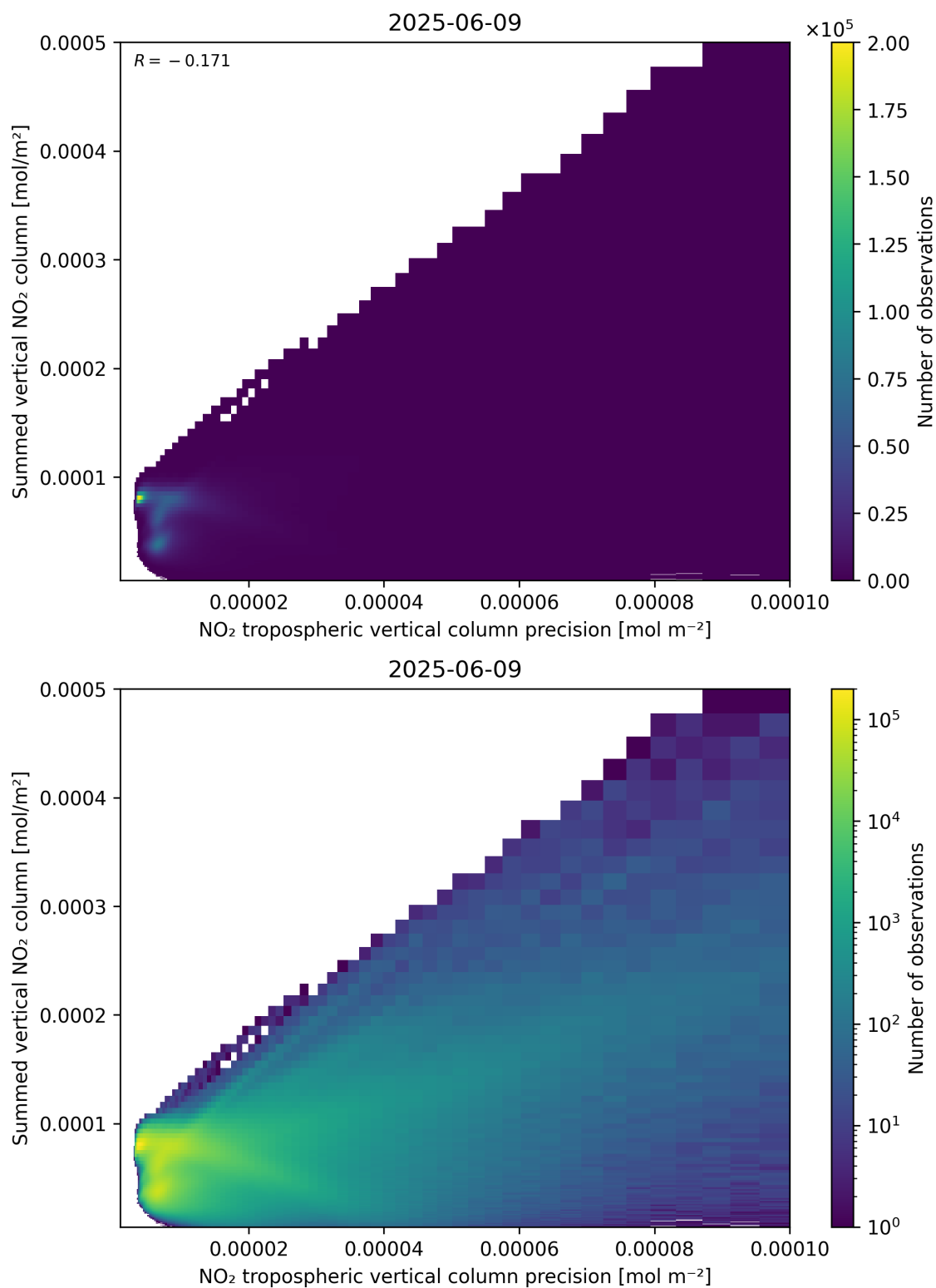
Figure 136: Scatter density plot of “NO 2 tropospheric vertical column precision” against “Summed vertical NO 2 column” for 2025-06-08 to 2025-06-10.
