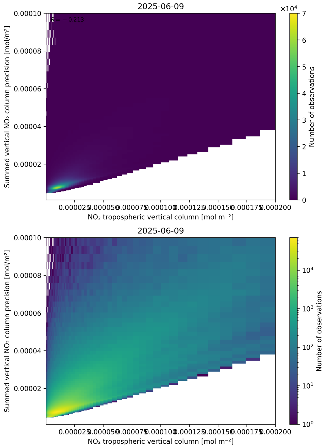
Figure 127: Scatter density plot of “NO 2 tropospheric vertical column” against “Summed vertical NO 2 column precision” for 2025-06-08 to 2025-06-10.
