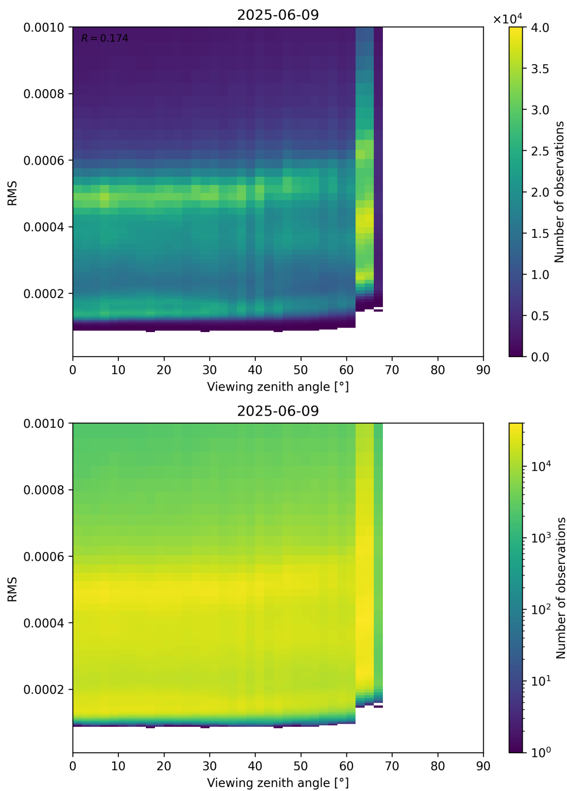
Figure 171: Scatter density plot of “Viewing zenith angle” against “RMS” for 2025-06-08 to 2025-06-10.
