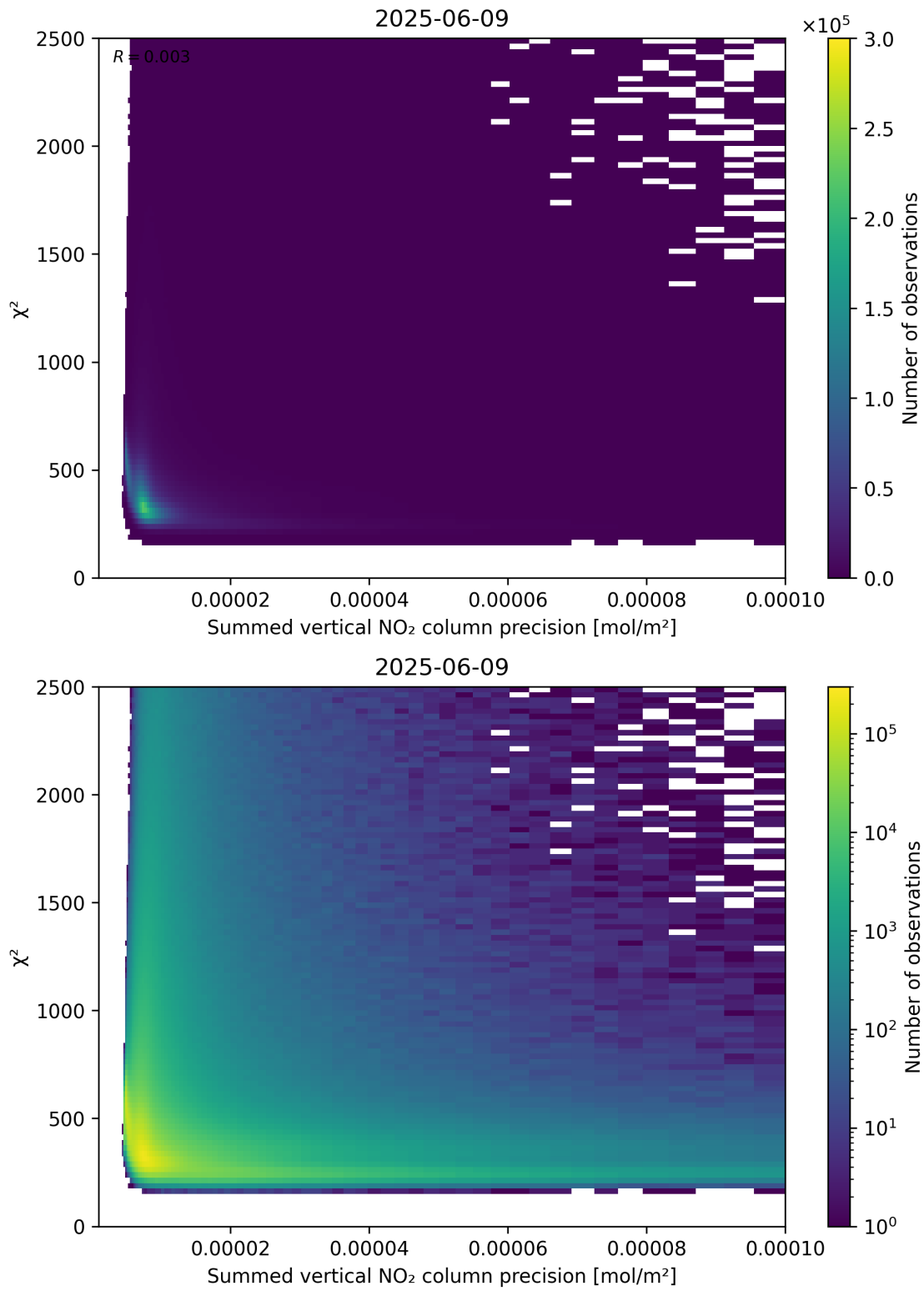
Figure 107: Scatter density plot of “Summed vertical NO 2 column precision” against “ \chi^2 ” for 2025-06-08 to 2025-06-10.
