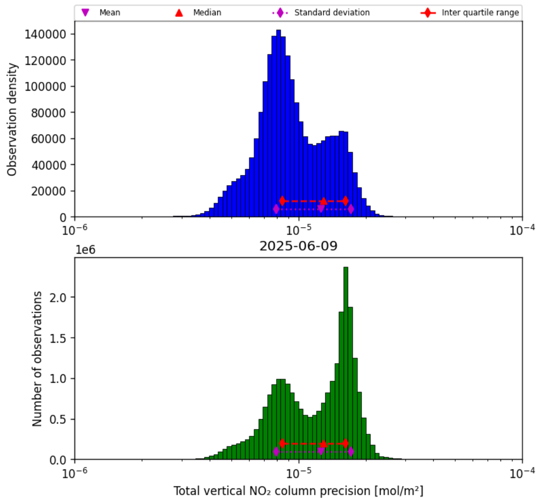
Figure 39: Histogram of “Total vertical NO 2 column precision” for 2025-06-08 to 2025-06-10
