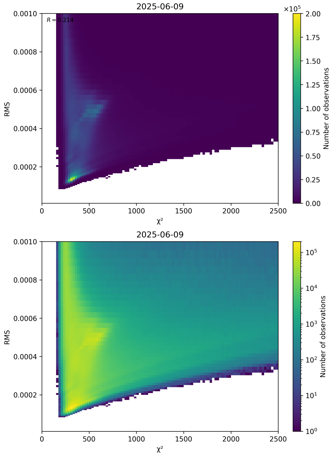
Figure 82: Scatter density plot of “ \chi^2 ” against “RMS” for 2025-06-08 to 2025-06-10.
