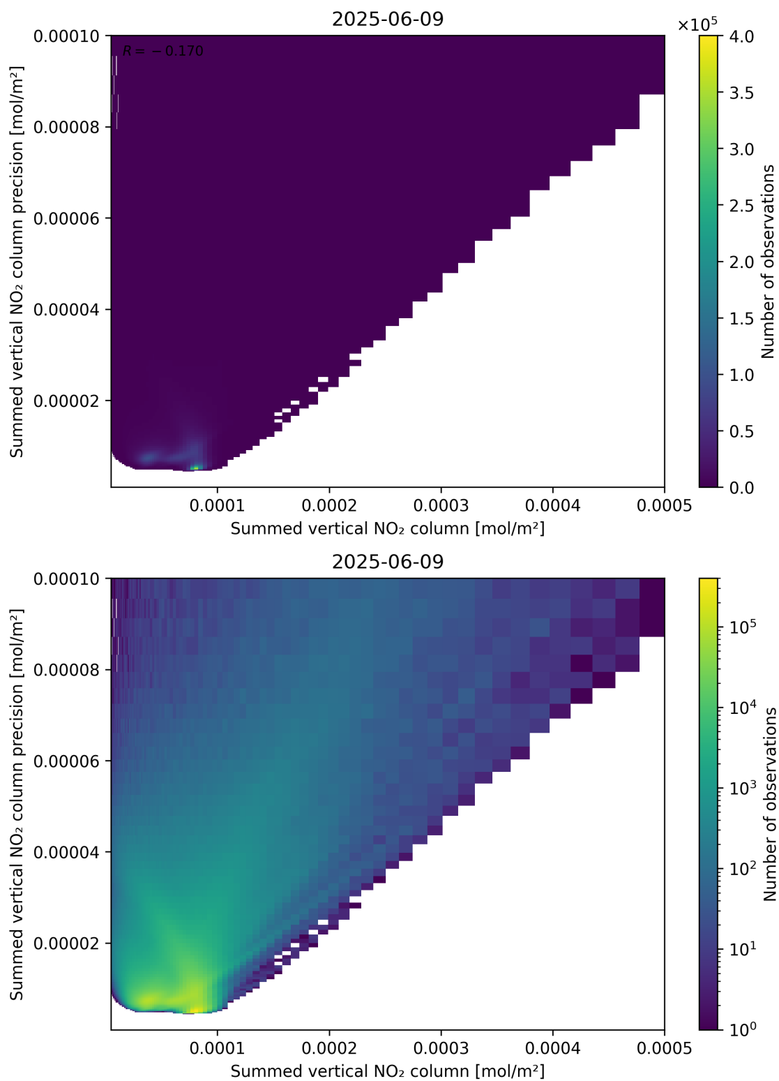
Figure 105: Scatter density plot of “Summed vertical NO 2 column” against “Summed vertical NO 2 column precision” for 2025-06-08 to 2025-06-10.
