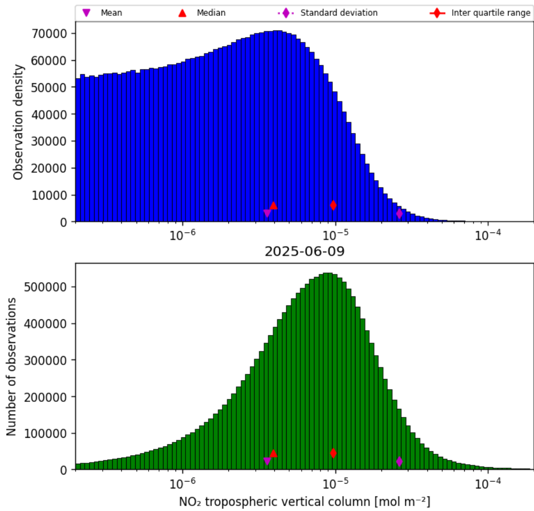
Figure 29: Histogram of “NO 2 tropospheric vertical column” for 2025-06-08 to 2025-06-10
