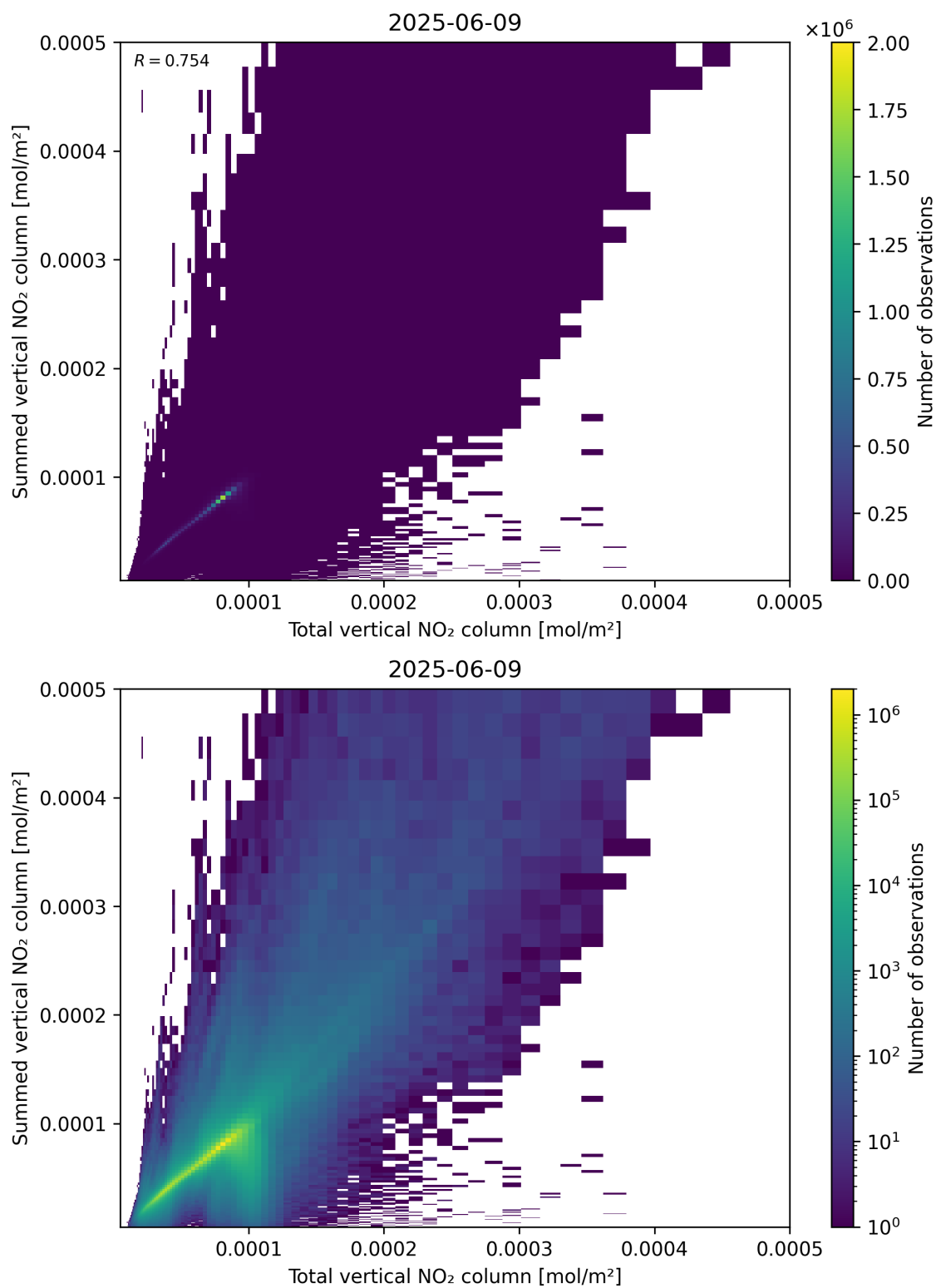
Figure 112: Scatter density plot of “Total vertical NO 2 column” against “Summed vertical NO 2 column” for 2025-06-08 to 2025-06-10.
