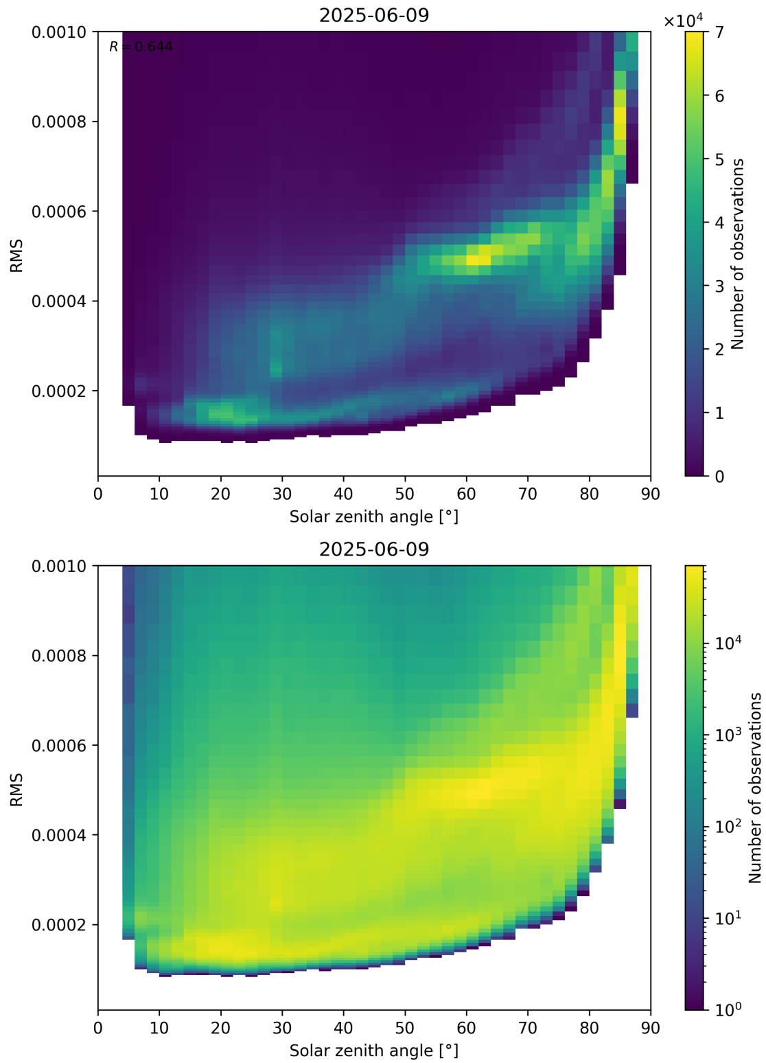
Figure 157: Scatter density plot of “Solar zenith angle” against “RMS” for 2025-06-08 to 2025-06-10.
