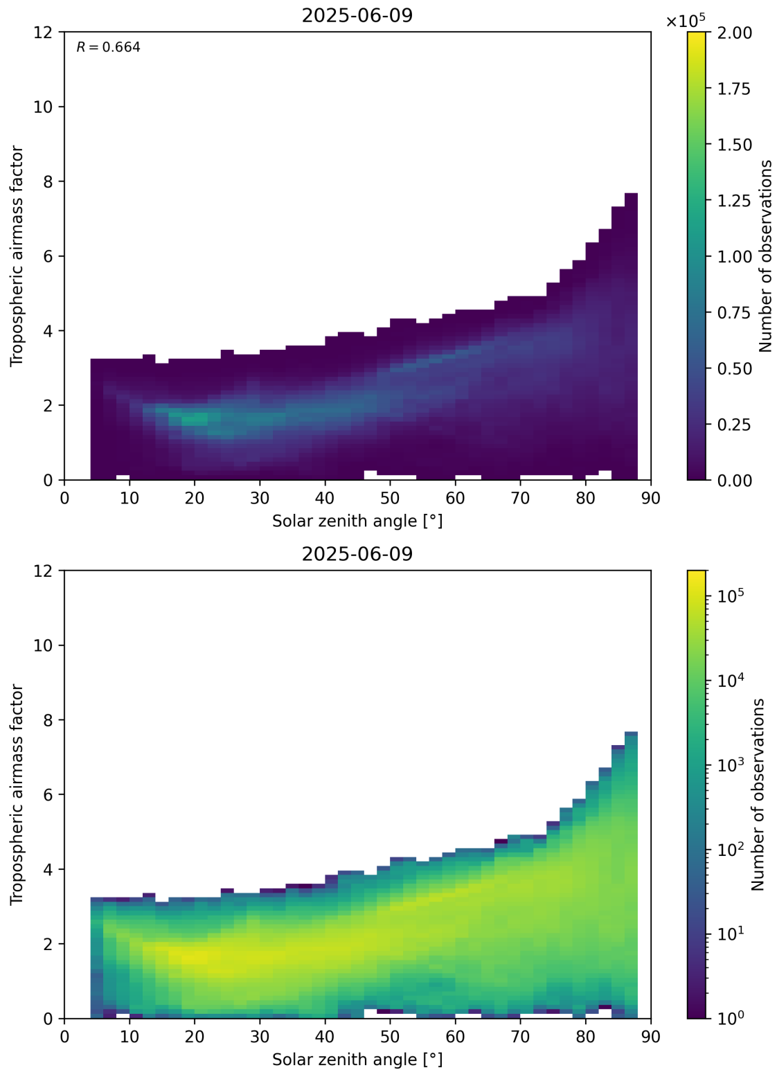
Figure 147: Scatter density plot of “Solar zenith angle” against “Tropospheric airmass factor” for 2025-06-08 to 2025-06-10.
