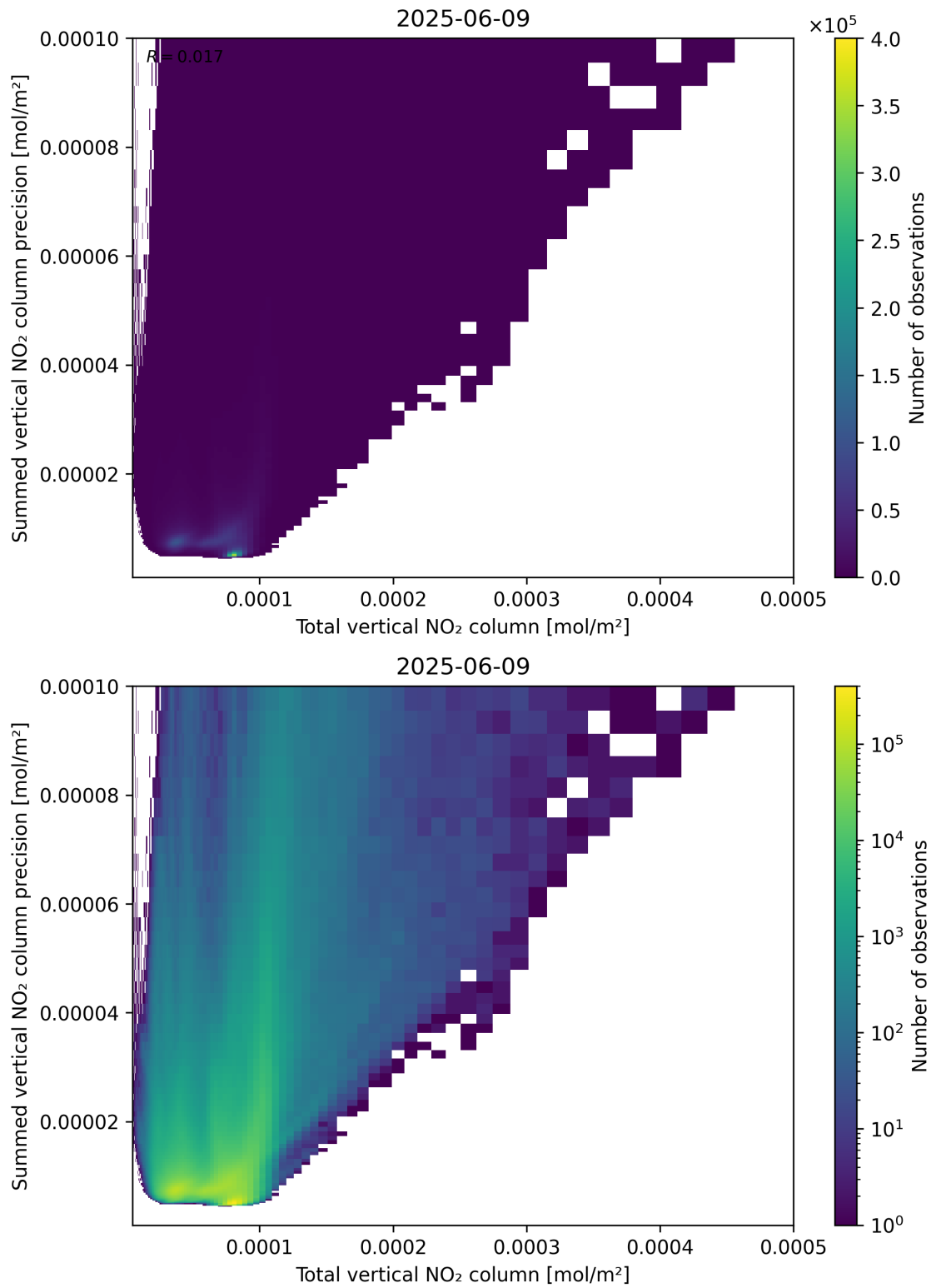
Figure 113: Scatter density plot of “Total vertical NO 2 column” against “Summed vertical NO 2 column precision” for 2025-06-08 to 2025-06-10.
