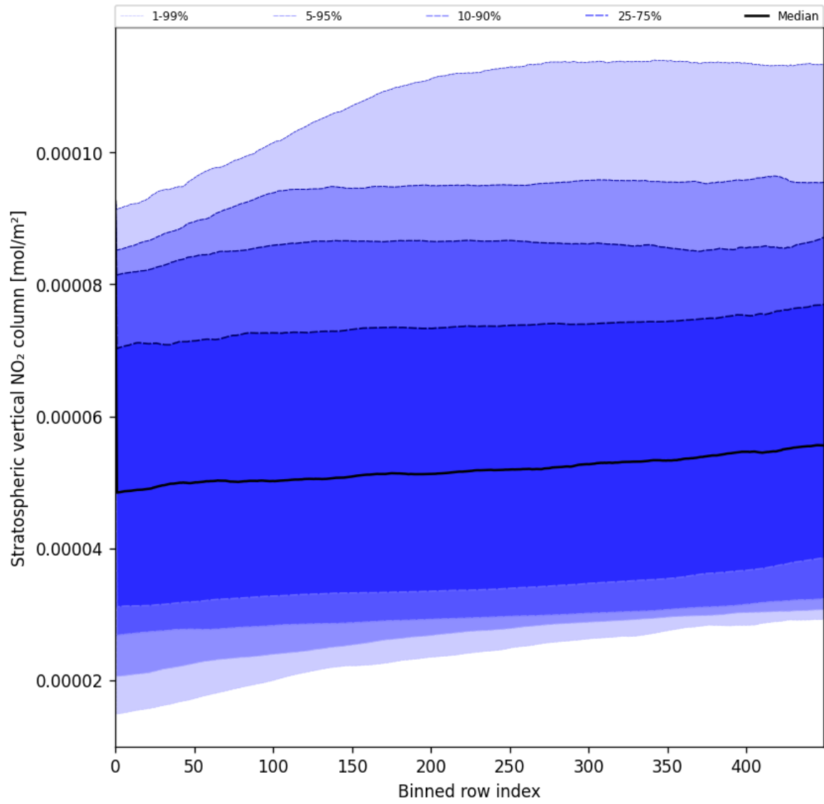
Figure 53: Along track statistics of “Stratospheric vertical NO 2 column” for 2025-06-08 to 2025-06-10
