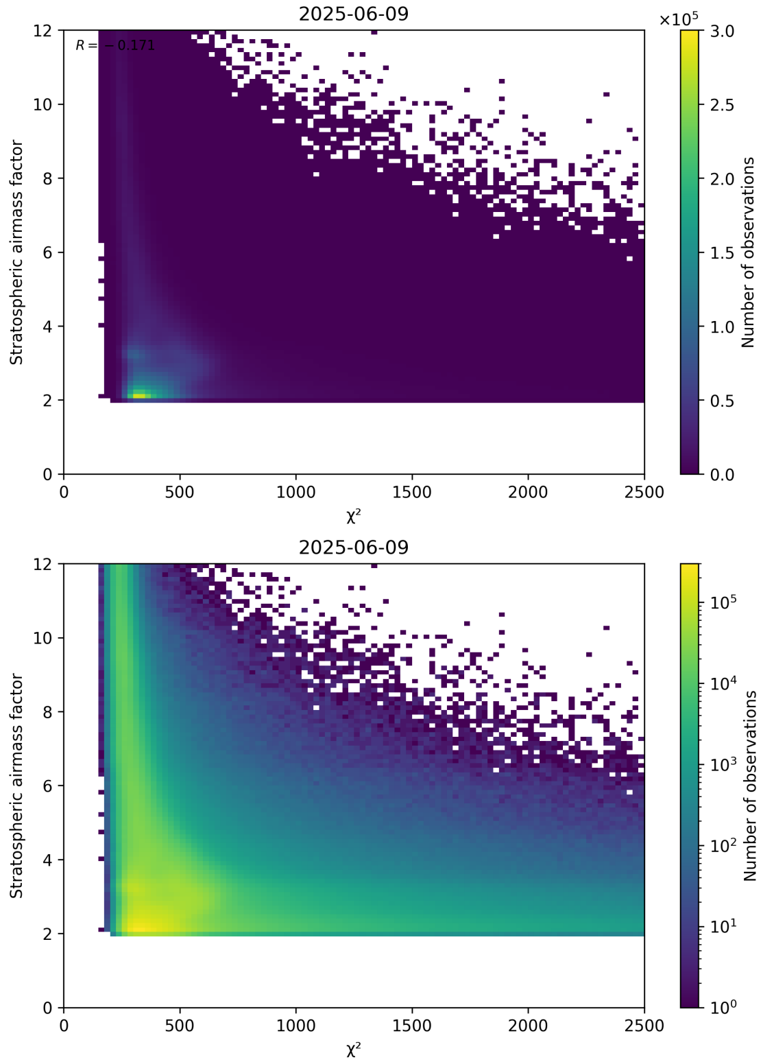
Figure 81: Scatter density plot of “ \chi^2 ” against “Stratospheric airmass factor” for 2025-06-08 to 2025-06-10.
