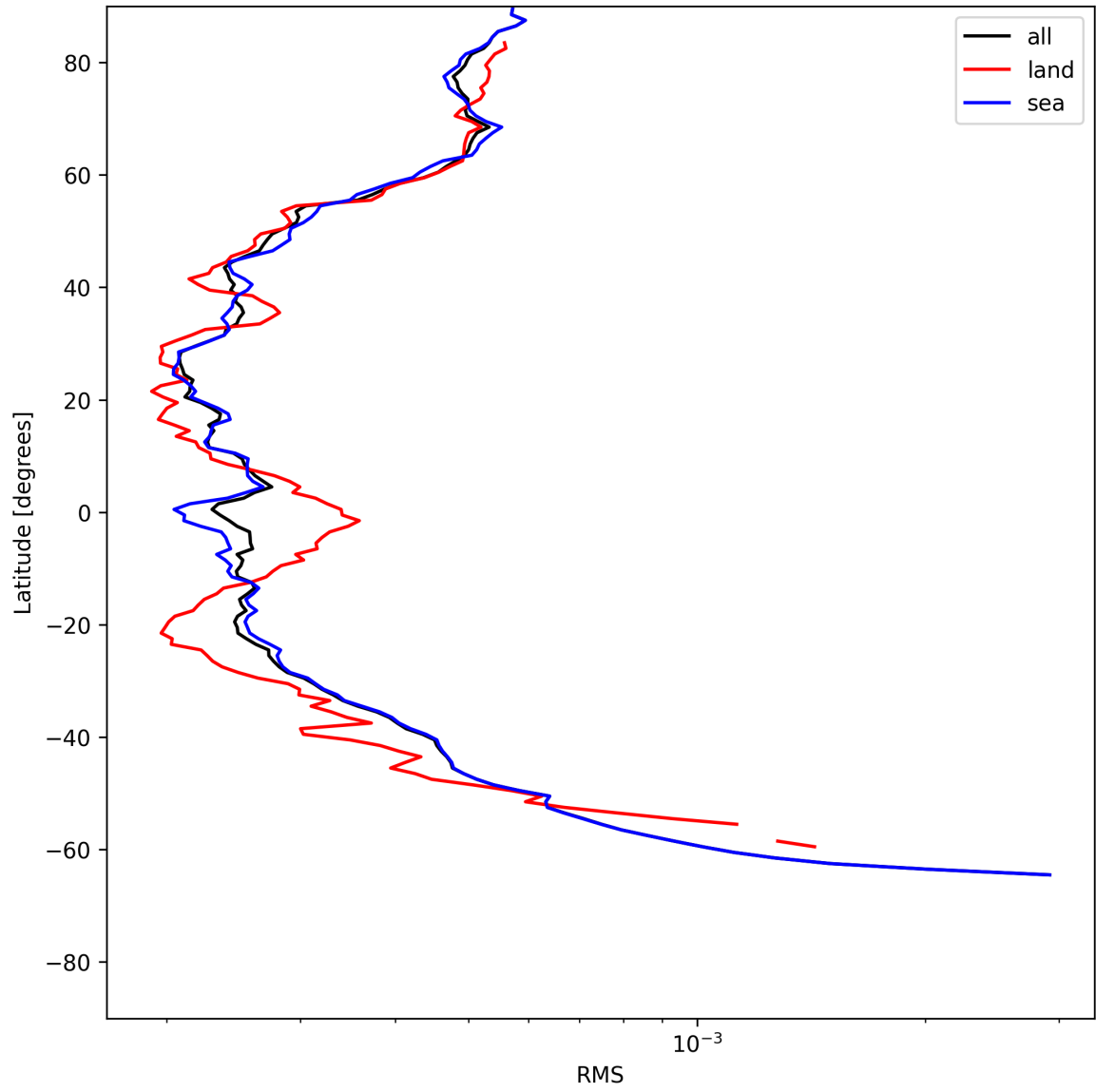
Figure 26: Zonal average of “RMS” for 2025-06-08 to 2025-06-10.
