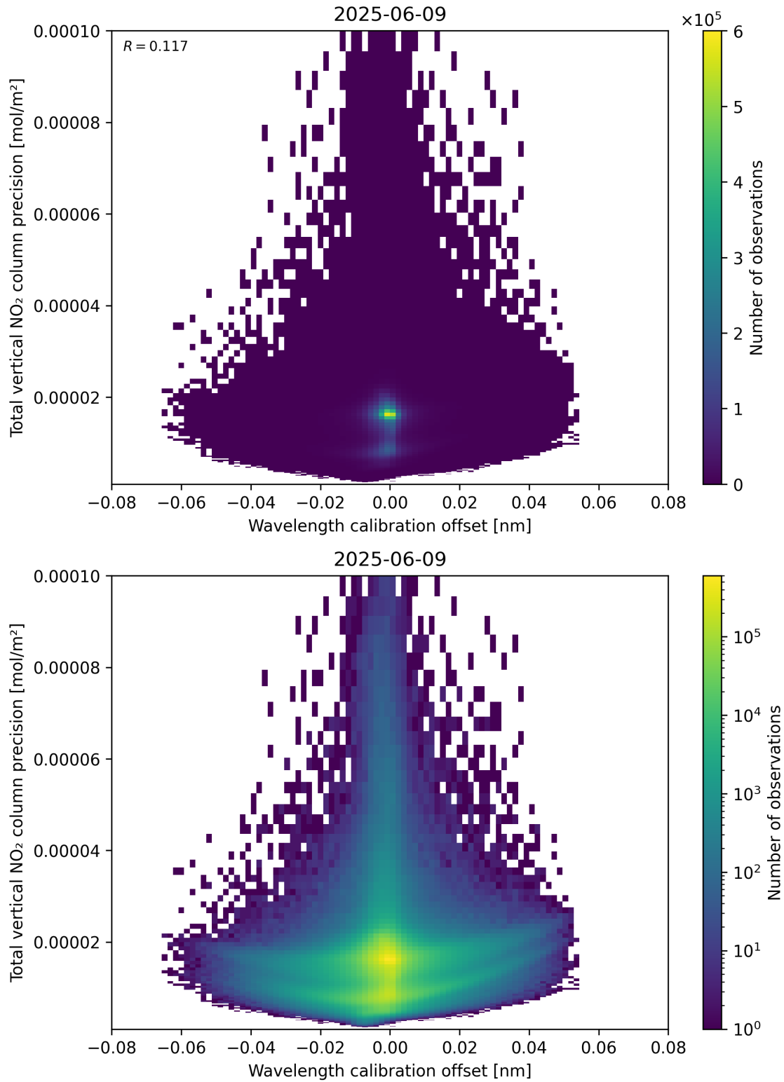
Figure 180: Scatter density plot of “Wavelength calibration offset” against “Total vertical NO 2 column precision” for 2025-06-08 to 2025-06-10.
