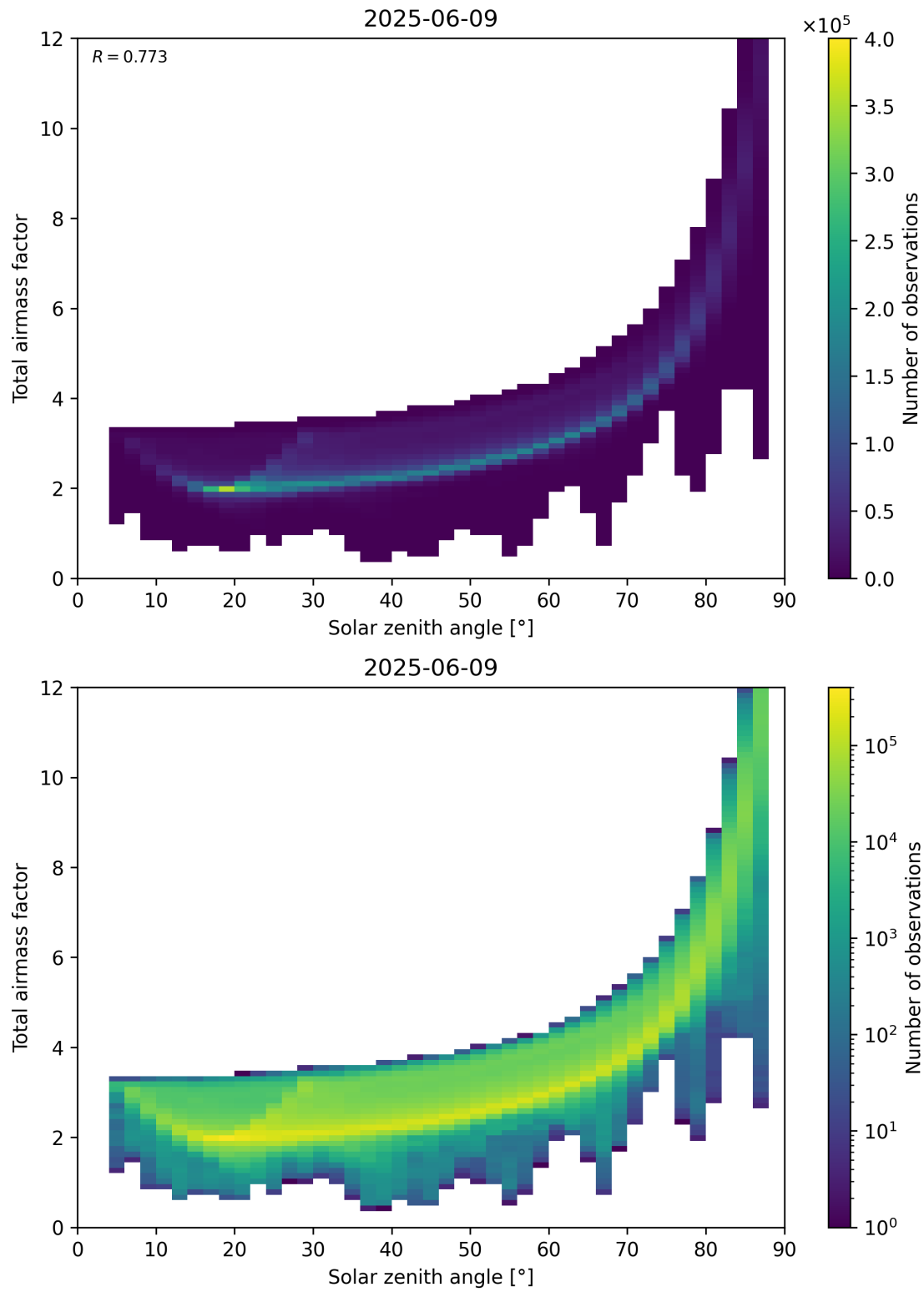
Figure 146: Scatter density plot of “Solar zenith angle” against “Total air mass factor” for 2025-06-08 to 2025-06-10.
