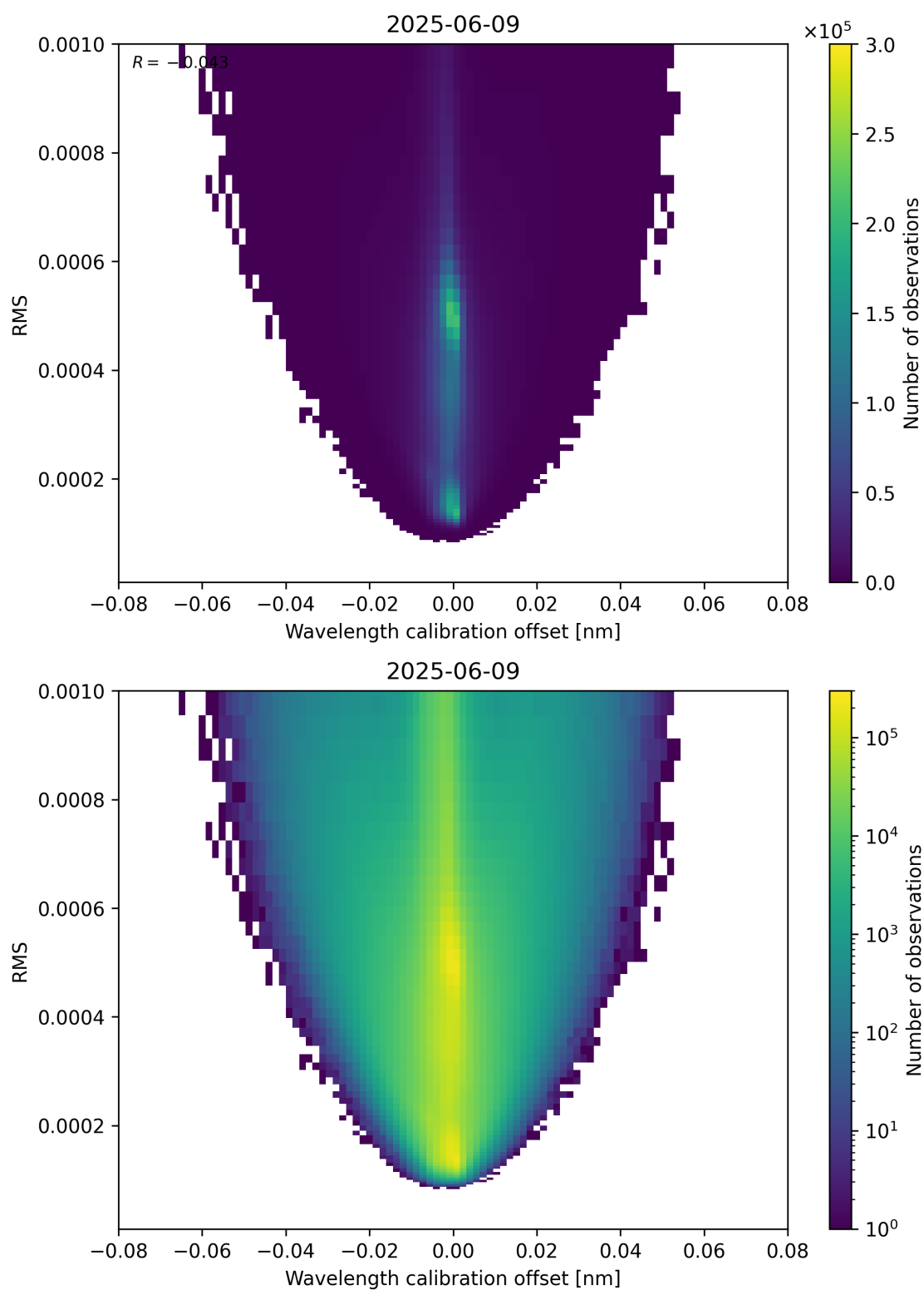
Figure 181: Scatter density plot of “Wavelength calibration offset” against “RMS” for 2025-06-08 to 2025-06-10.
