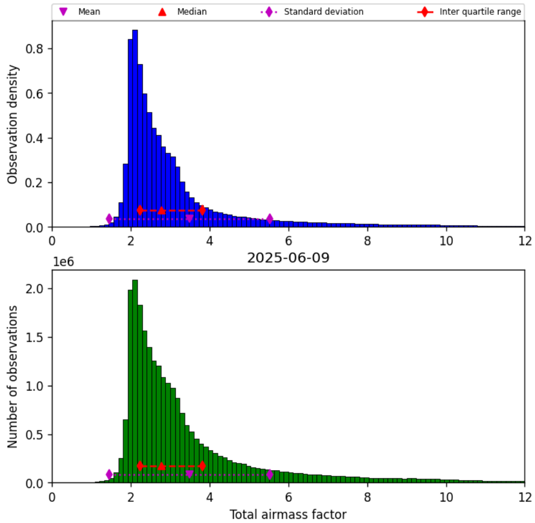
Figure 32: Histogram of “Total airmass factor” for 2025-06-08 to 2025-06-10
