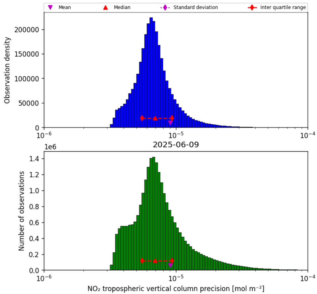
Figure 30: Histogram of “NO 2 tropospheric vertical column precision” for 2025-06-08 to 2025-06-10
