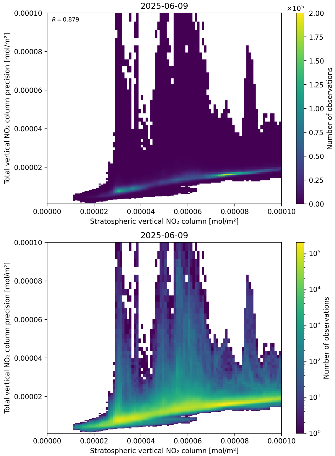
Figure 101: Scatter density plot of “Stratospheric vertical NO 2 column” against “Total vertical NO 2 column precision” for 2025-06-08 to 2025-06-10.
