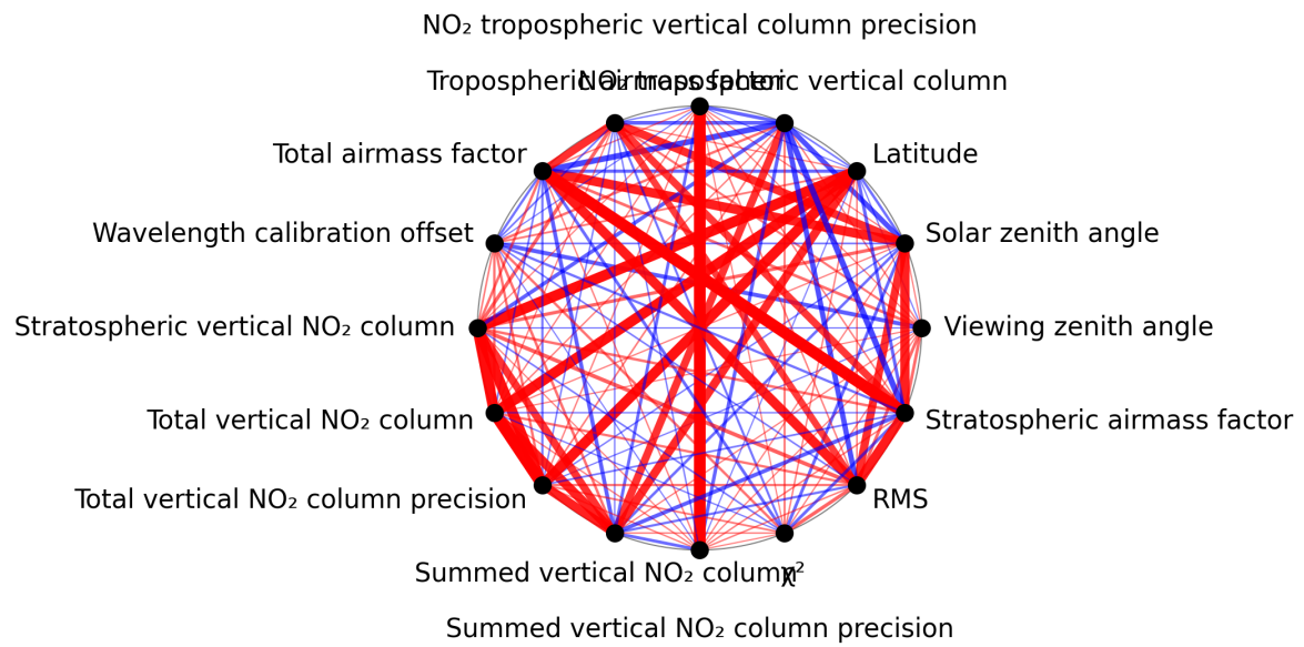
Figure 1: Map of correlation graph for 2025-06-08 to 2025-06-10.
