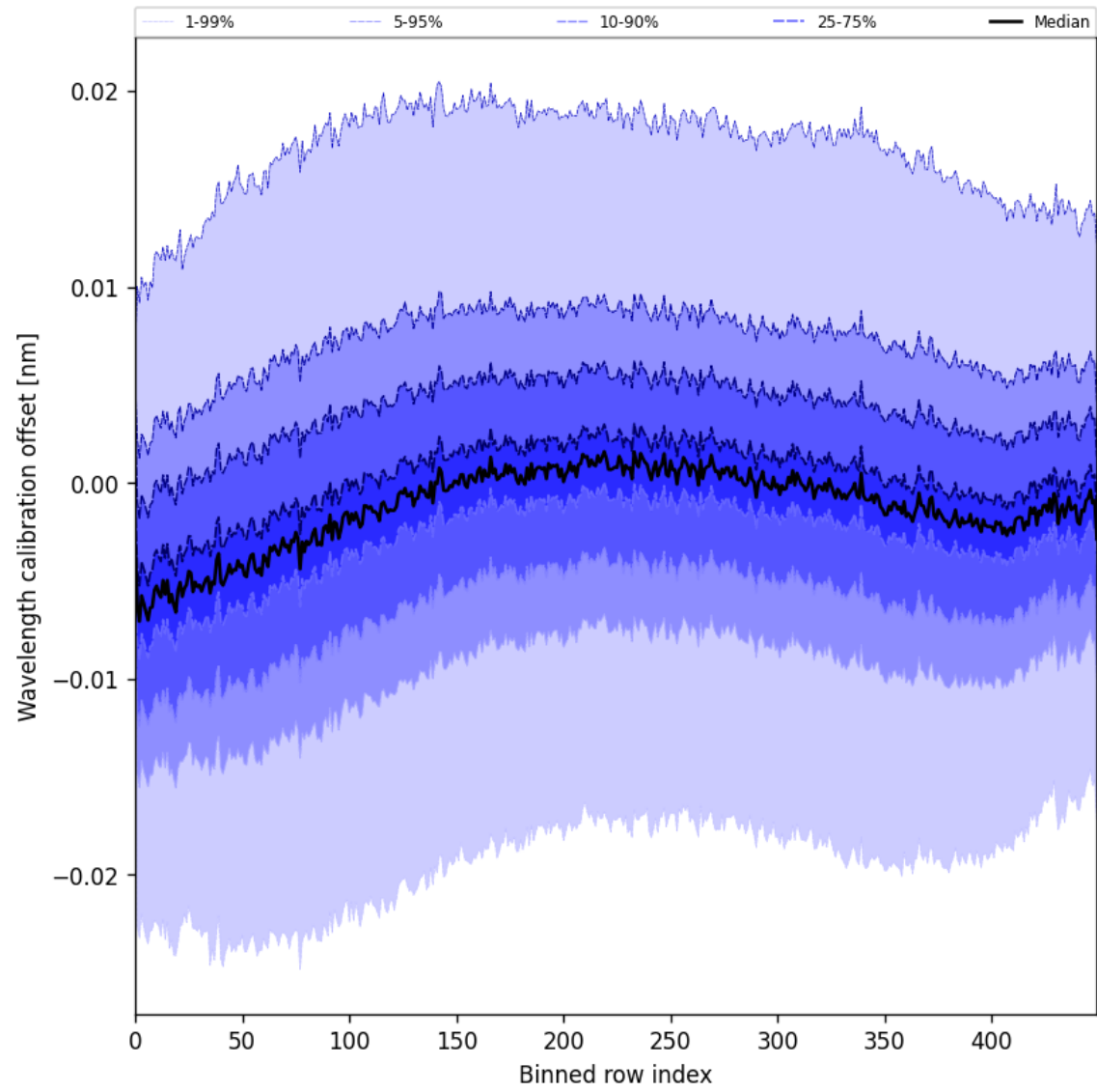
Figure 52: Along track statistics of “Wavelength calibration offset” for 2025-06-08 to 2025-06-10
