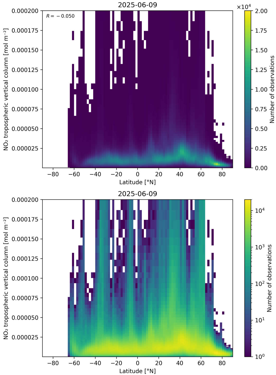
Figure 92: Scatter density plot of “Latitude” against “NO 2 tropospheric vertical column” for 2025-06-08 to 2025-06-10.
