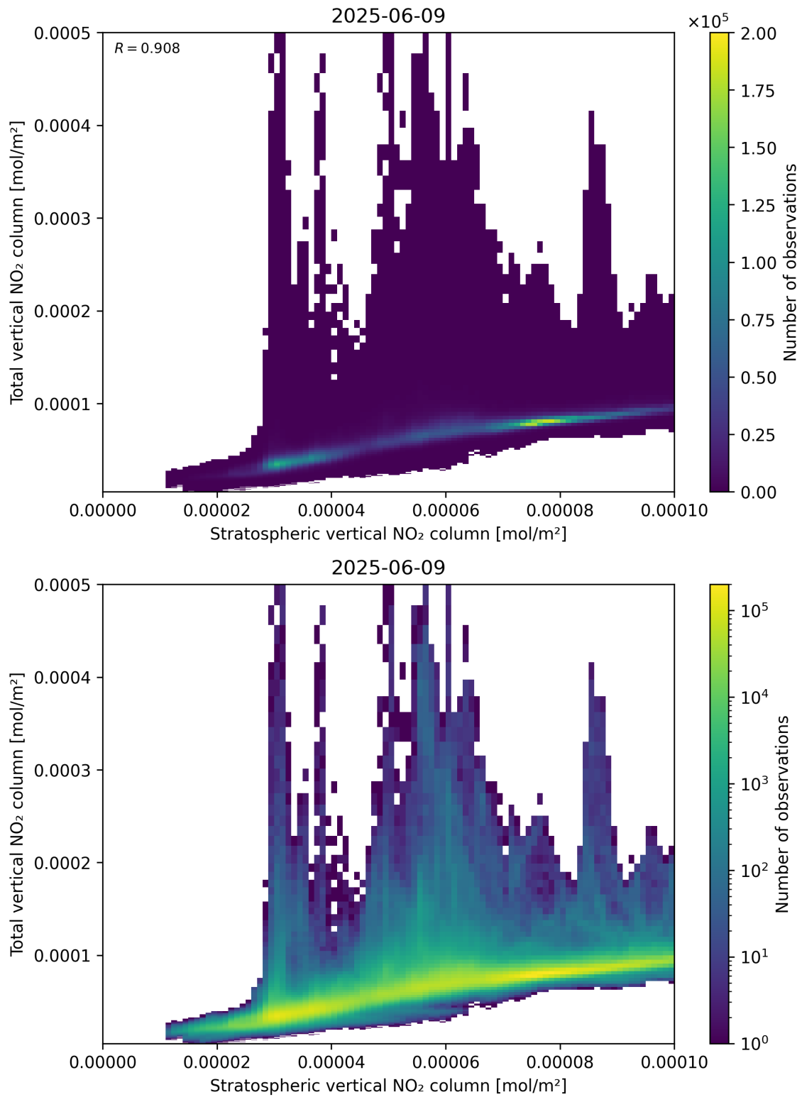
Figure 100: Scatter density plot of “Stratospheric vertical NO 2 column” against “Total vertical NO 2 column” for 2025-06-08 to 2025-06-10.
