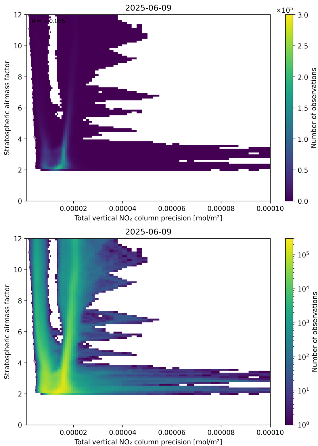
Figure 115: Scatter density plot of “Total vertical NO 2 column precision” against “Stratospheric air mass factor” for 2025-06-08 to 2025-06-10.
