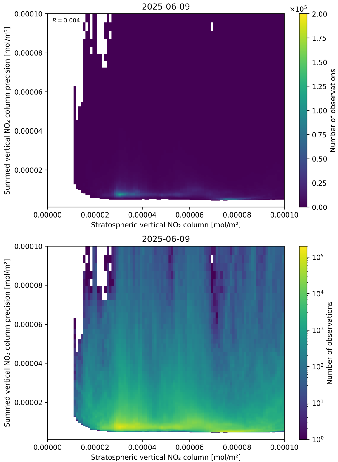
Figure 99: Scatter density plot of “Stratospheric vertical NO 2 column” against “Summed vertical NO 2 column precision” for 2025-06-08 to 2025-06-10.
