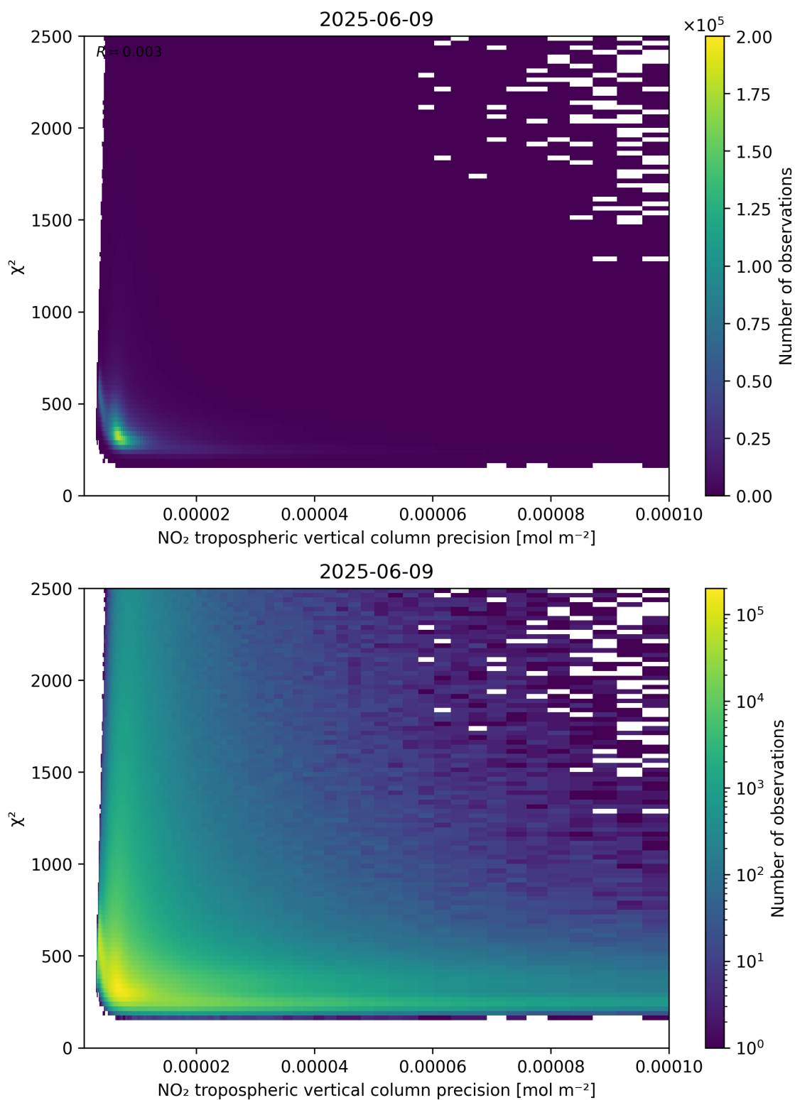
Figure 134: Scatter density plot of “NO 2 tropospheric vertical column precision” against “ \chi^2 ” for 2025-06-08 to 2025-06-10.
