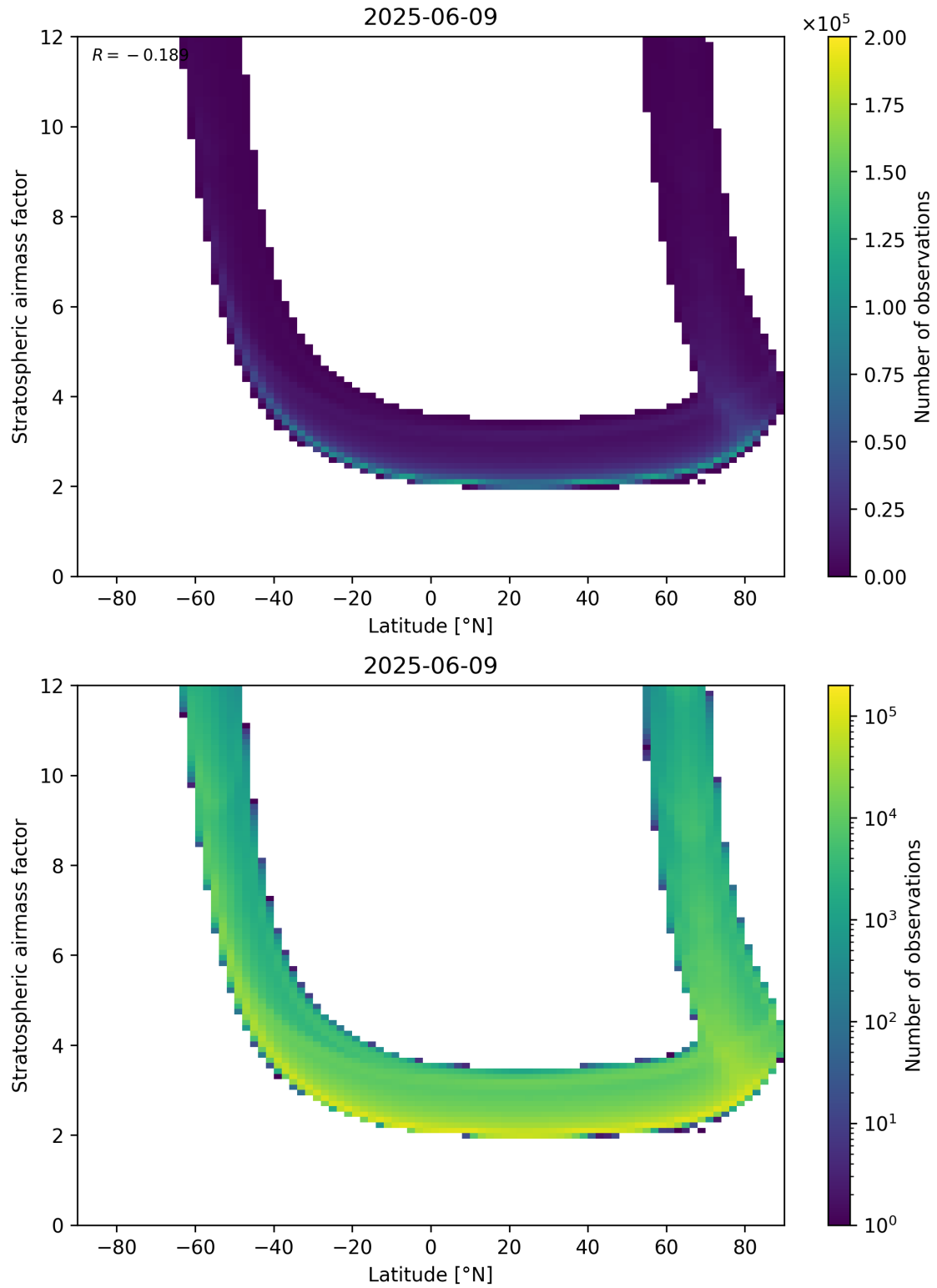
Figure 83: Scatter density plot of “Latitude” against “Stratospheric air mass factor” for 2025-06-08 to 2025-06-10.
