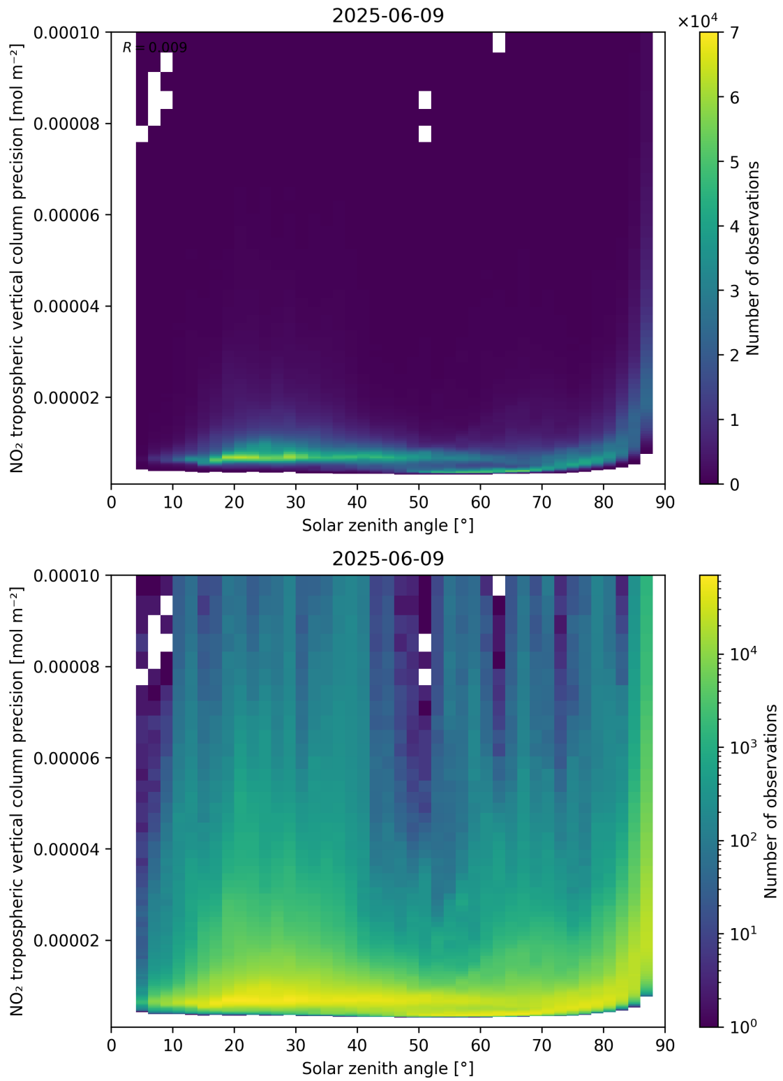
Figure 156: Scatter density plot of “Solar zenith angle” against “NO 2 tropospheric vertical column precision” for 2025-06-08 to 2025-06-10.
