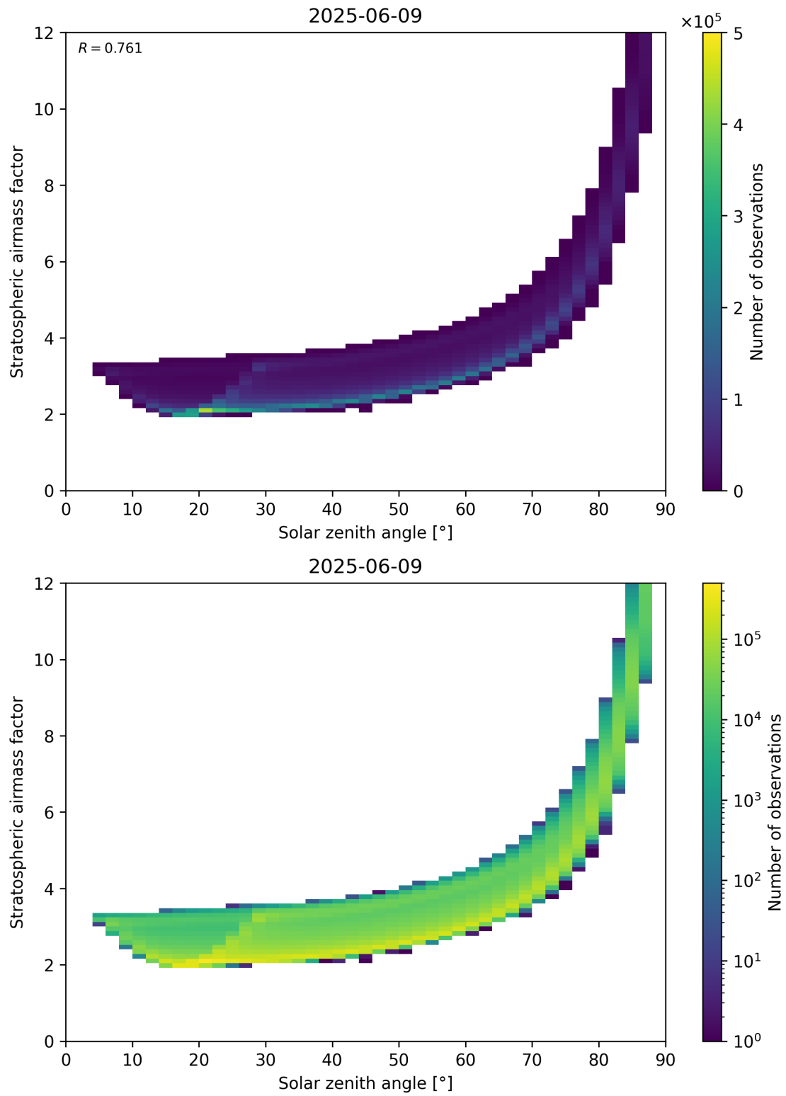
Figure 145: Scatter density plot of “Solar zenith angle” against “Stratospheric airmass factor” for 2025-06-08 to 2025-06-10.
