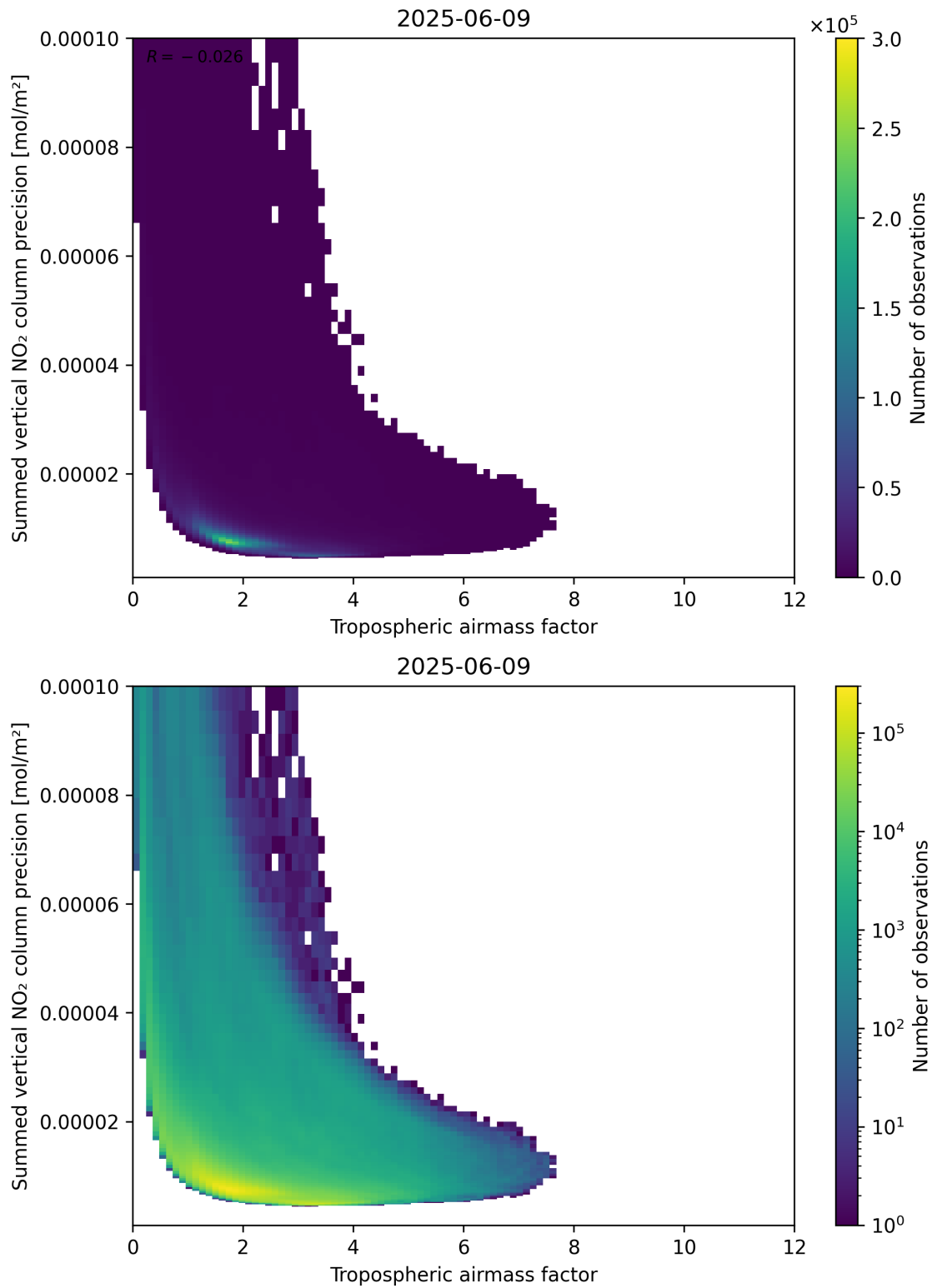
Figure 76: Scatter density plot of “Tropospheric air mass factor” against “Summed vertical NO 2 column precision” for 2025-06-08 to 2025-06-10.
