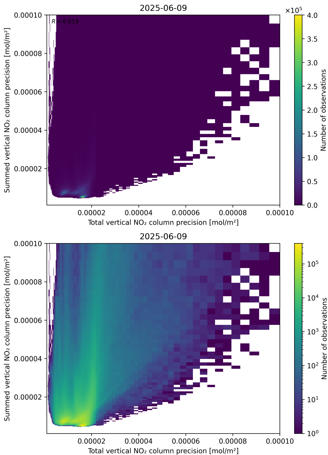
Figure 118: Scatter density plot of “Total vertical NO 2 column precision” against “Summed vertical NO 2 column precision” for 2025-06-08 to 2025-06-10.
