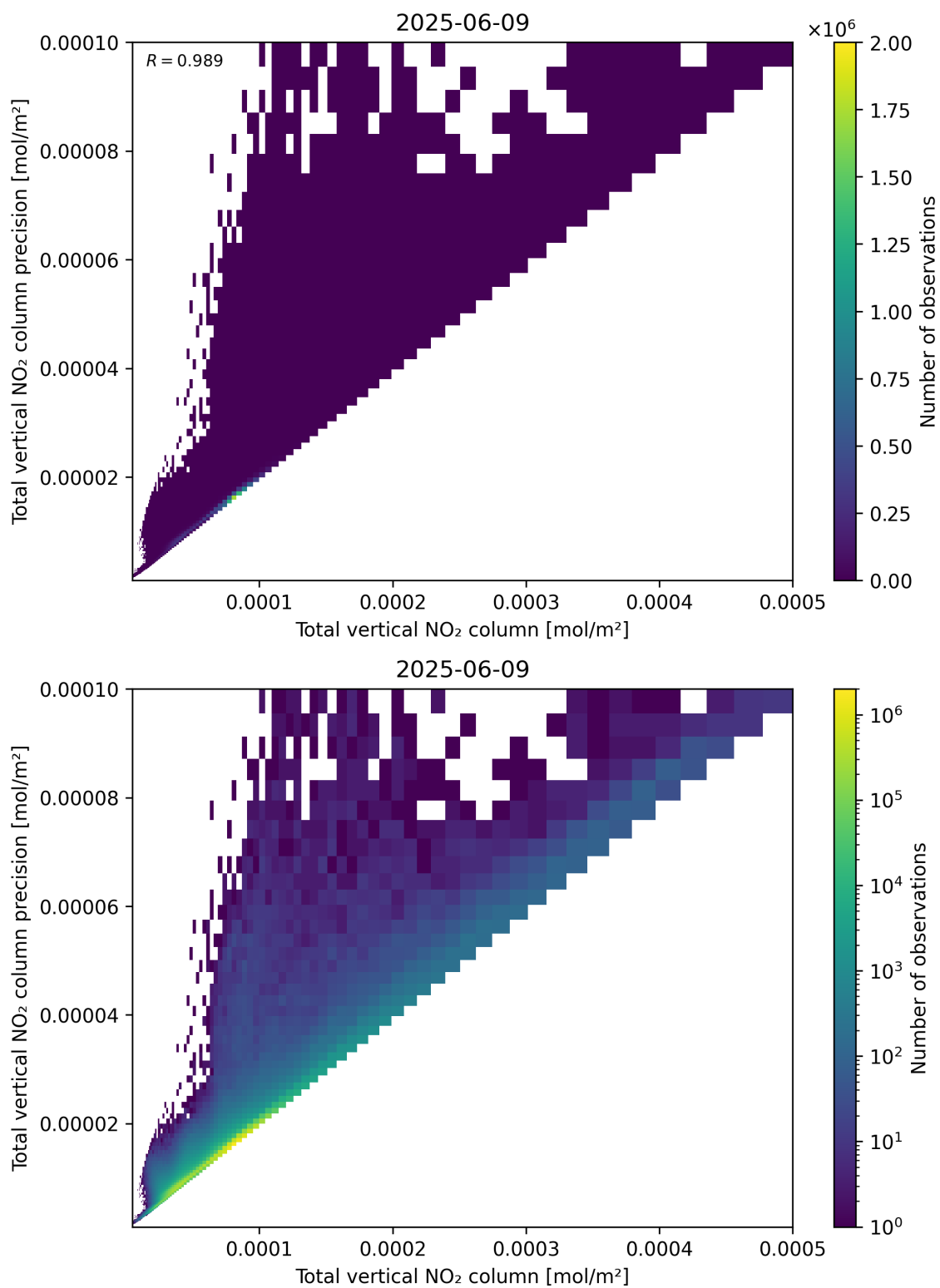
Figure 114: Scatter density plot of “Total vertical NO 2 column” against “Total vertical NO 2 column precision” for 2025-06-08 to 2025-06-10.
