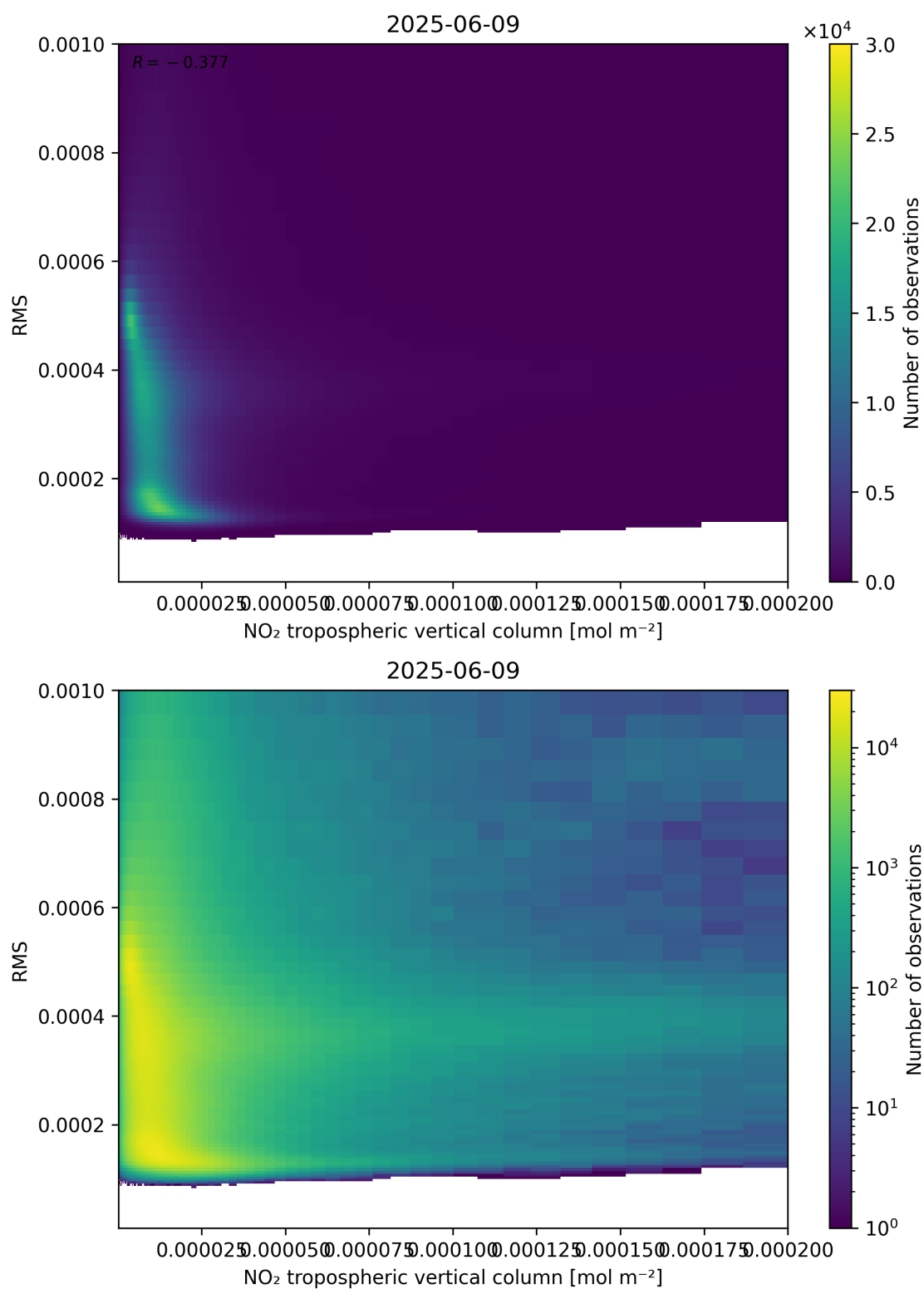
Figure 142: Scatter density plot of “NO 2 tropospheric vertical column” against “RMS” for 2025-06-08 to 2025-06-10.
