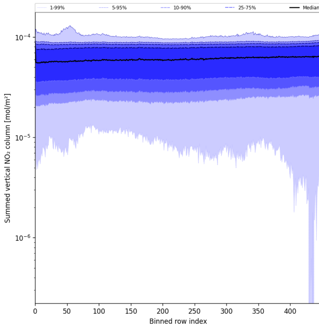
Figure 57: Along track statistics of “Summed vertical NO 2 column” for 2025-06-08 to 2025-06-10
