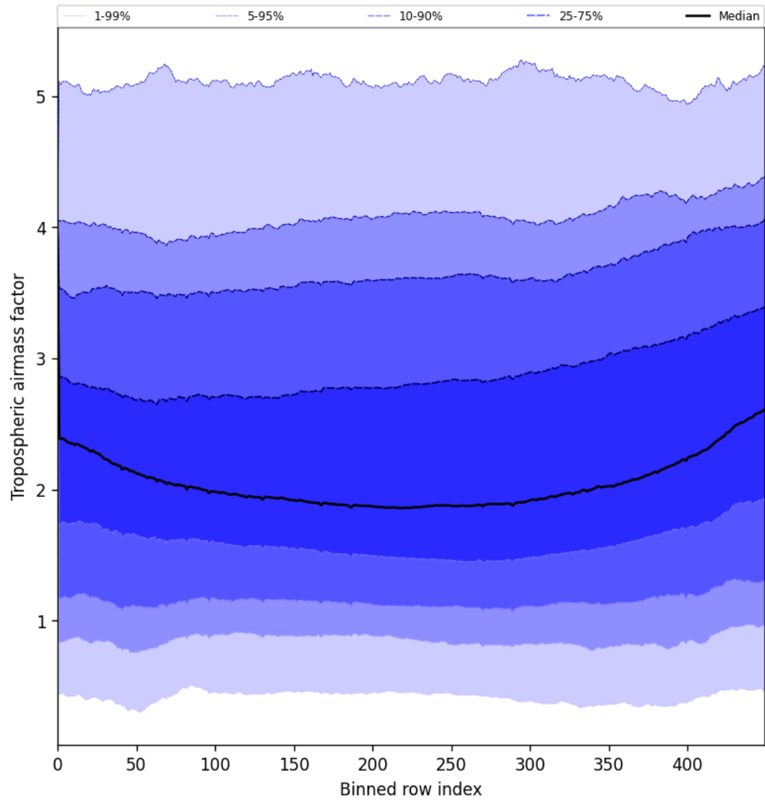
Figure 48: Along track statistics of “Tropospheric airmass factor” for 2025-06-08 to 2025-06-10
