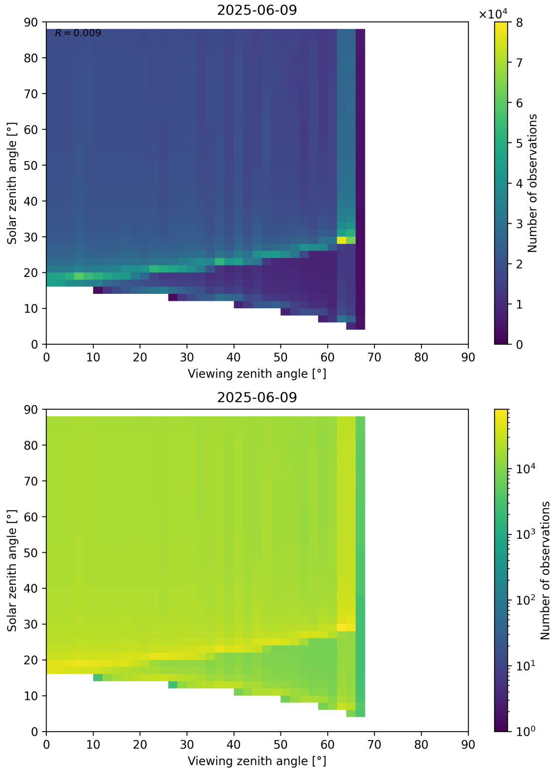
Figure 172: Scatter density plot of “Viewing zenith angle” against “Solar zenith angle” for 2025-06-08 to 2025-06-10.
