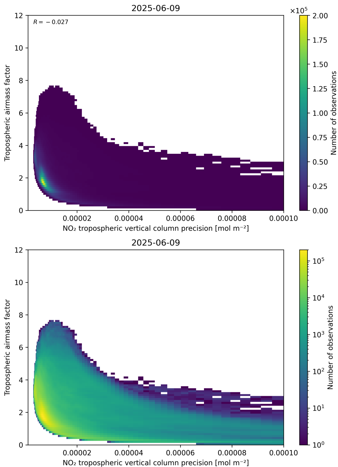
Figure 133: Scatter density plot of “NO 2 tropospheric vertical column precision” against “Tropospheric air mass factor” for 2025-06-08 to 2025-06-10.
