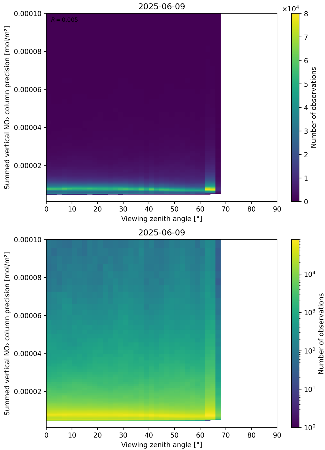
Figure 166: Scatter density plot of “Viewing zenith angle” against “Summed vertical NO 2 column precision” for 2025-06-08 to 2025-06-10.
