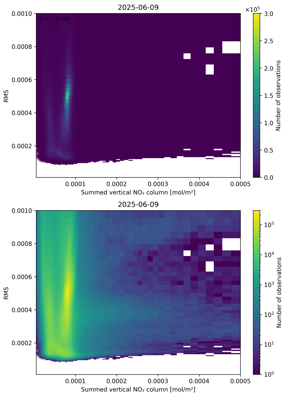
Figure 109: Scatter density plot of “Summed vertical NO 2 column” against “RMS” for 2025-06-08 to 2025-06-10.
