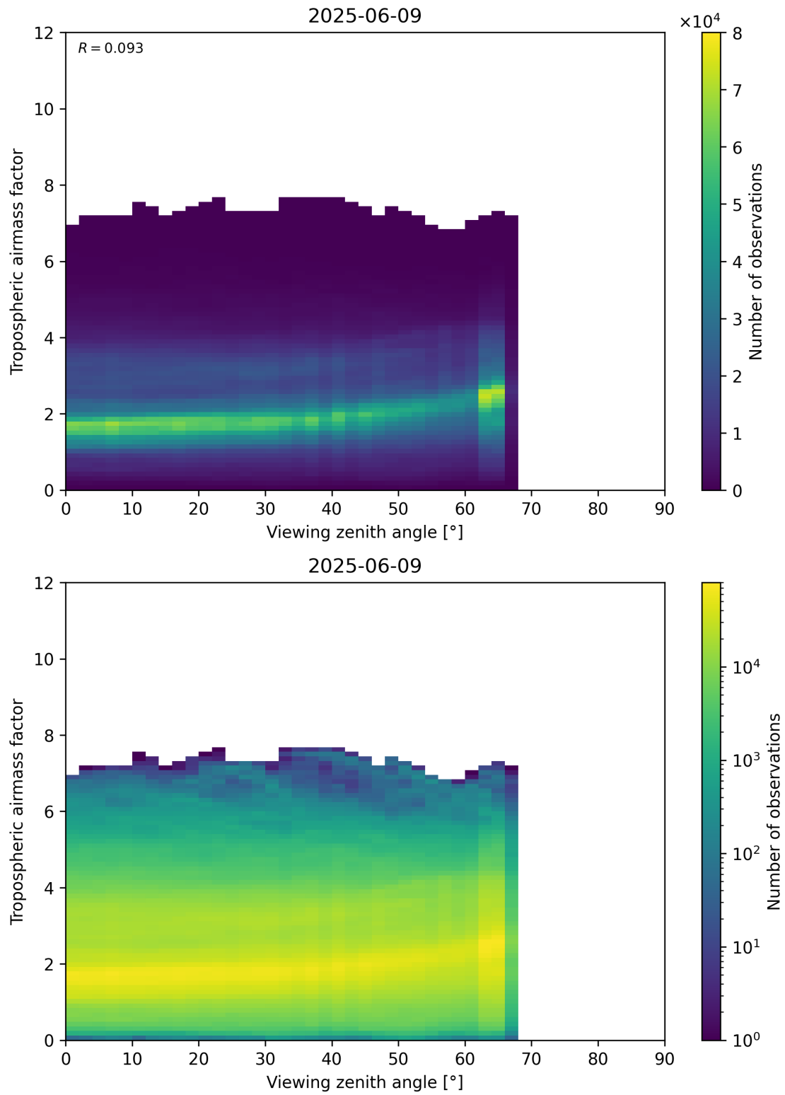
Figure 161: Scatter density plot of “Viewing zenith angle” against “Tropospheric airmass factor” for 2025-06-08 to 2025-06-10.
