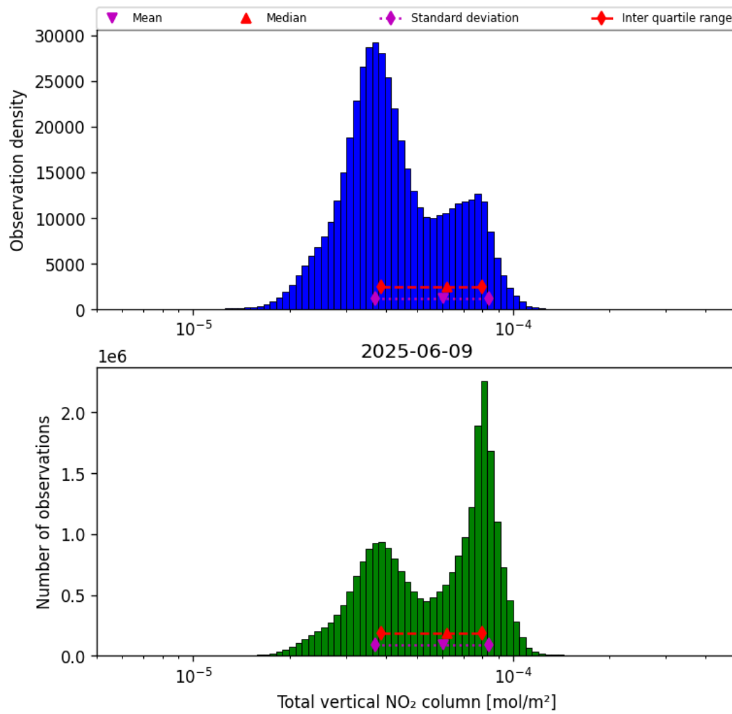
Figure 38: Histogram of “Total vertical NO 2 column” for 2025-06-08 to 2025-06-10
