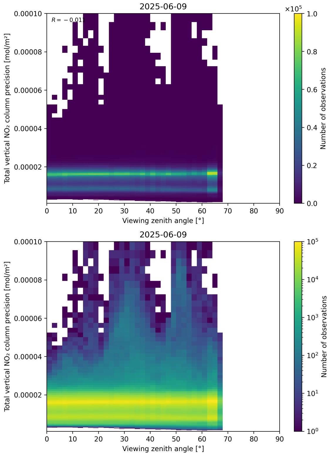
Figure 168: Scatter density plot of “Viewing zenith angle” against “Total vertical NO 2 column precision” for 2025-06-08 to 2025-06-10.
