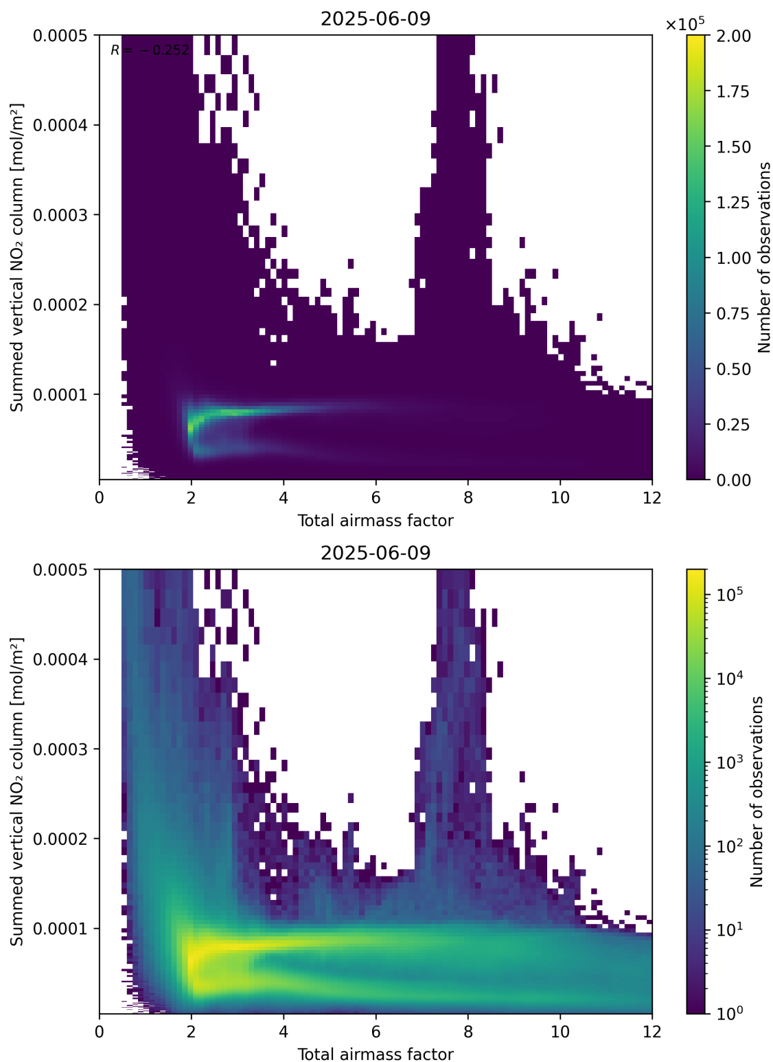
Figure 65: Scatter density plot of “Total airmass factor” against “Summed vertical NO 2 column” for 2025-06-08 to 2025-06-10.
