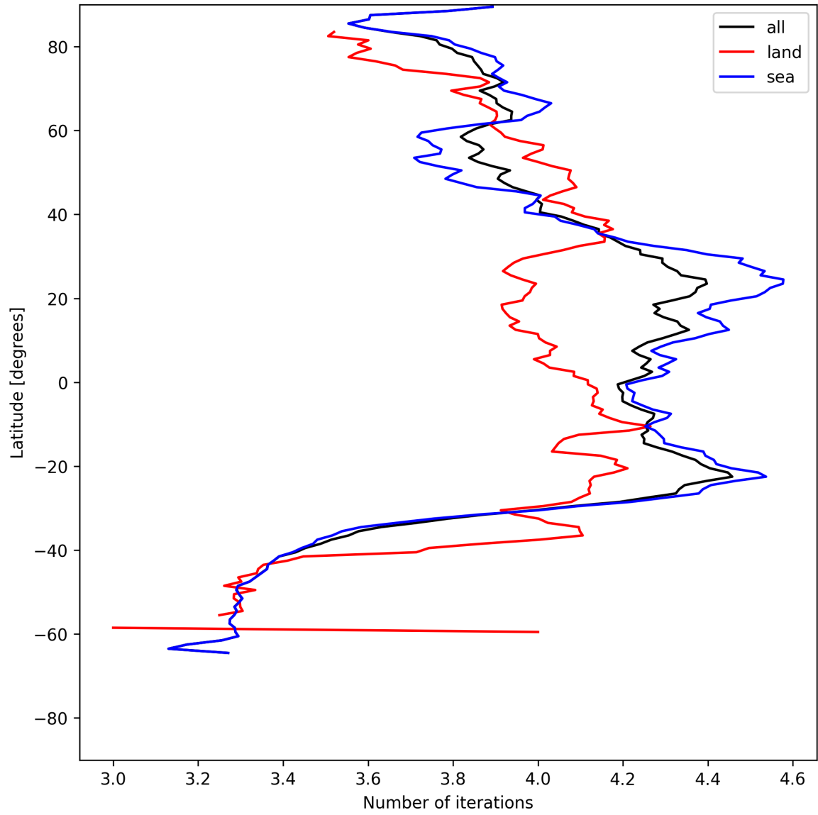
Figure 17: Zonal average of “Number of iterations” for 2025-06-08 to 2025-06-10.
