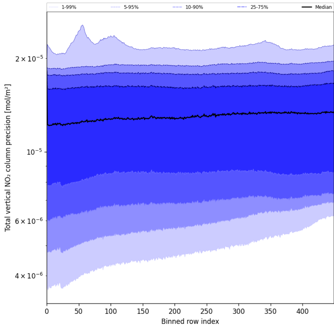
Figure 56: Along track statistics of “Total vertical NO 2 column precision” for 2025-06-08 to 2025-06-10
