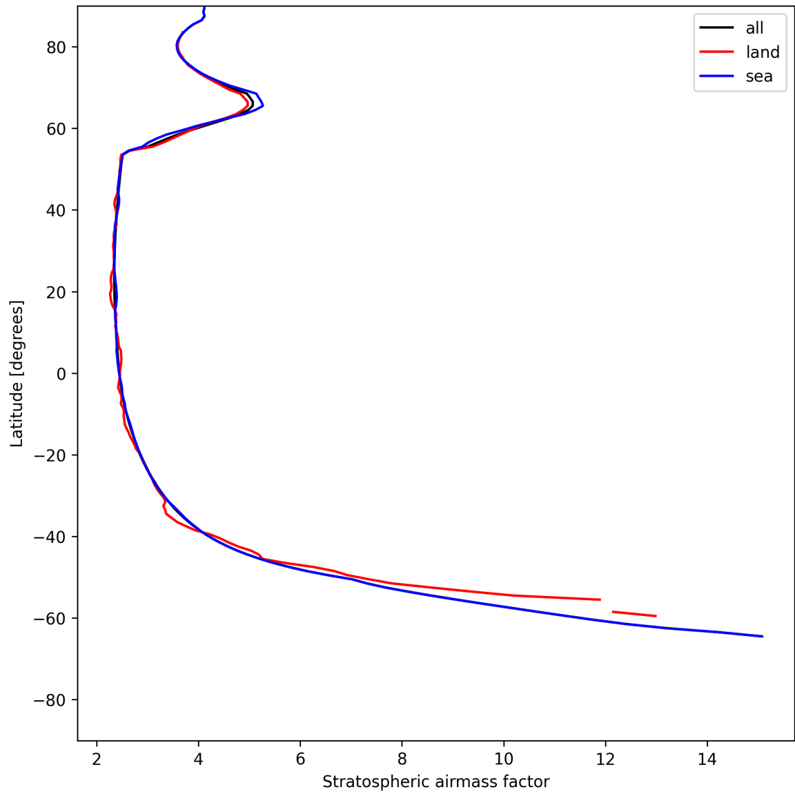
Figure 27: Zonal average of “Stratospheric airmass factor” for 2025-06-08 to 2025-06-10.
