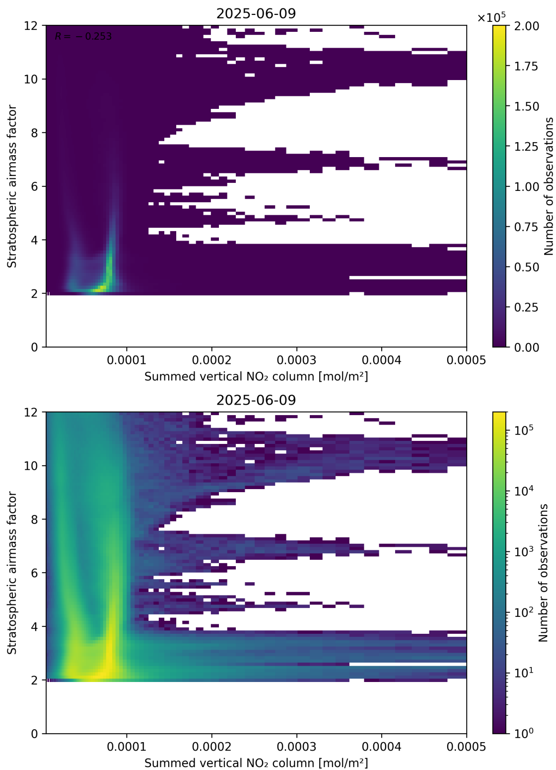
Figure 103: Scatter density plot of “Summed vertical NO 2 column” against “Stratospheric air mass factor” for 2025-06-08 to 2025-06-10.
