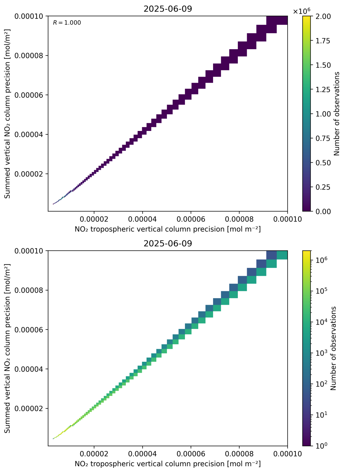
Figure 137: Scatter density plot of “NO 2 tropospheric vertical column precision” against “Summed vertical NO 2 column precision” for 2025-06-08 to 2025-06-10.
