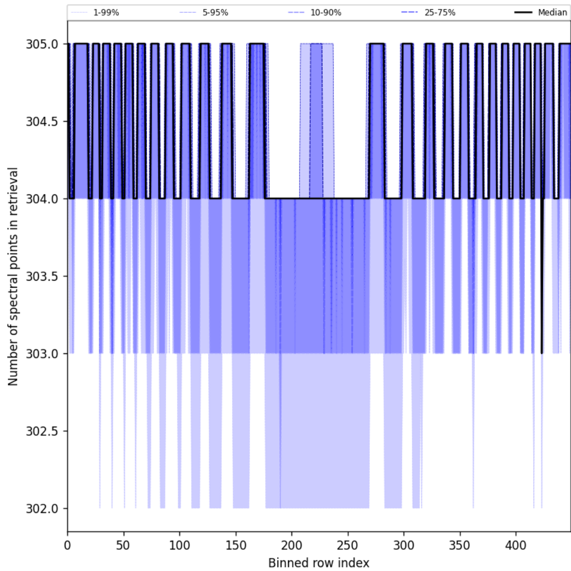
Figure 50: Along track statistics of “Number of spectral points in retrieval” for 2025-06-08 to 2025-06-10
