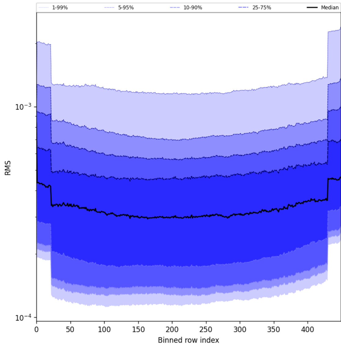
Figure 60: Along track statistics of “RMS” for 2025-06-08 to 2025-06-10
