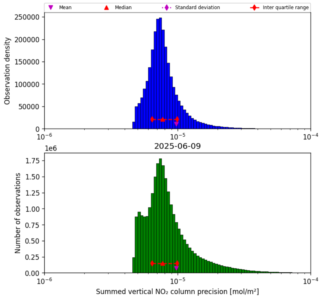
Figure 41: Histogram of "Summed vertical NO 2 column precision" for 2025-06-08 to 2025-06-10
