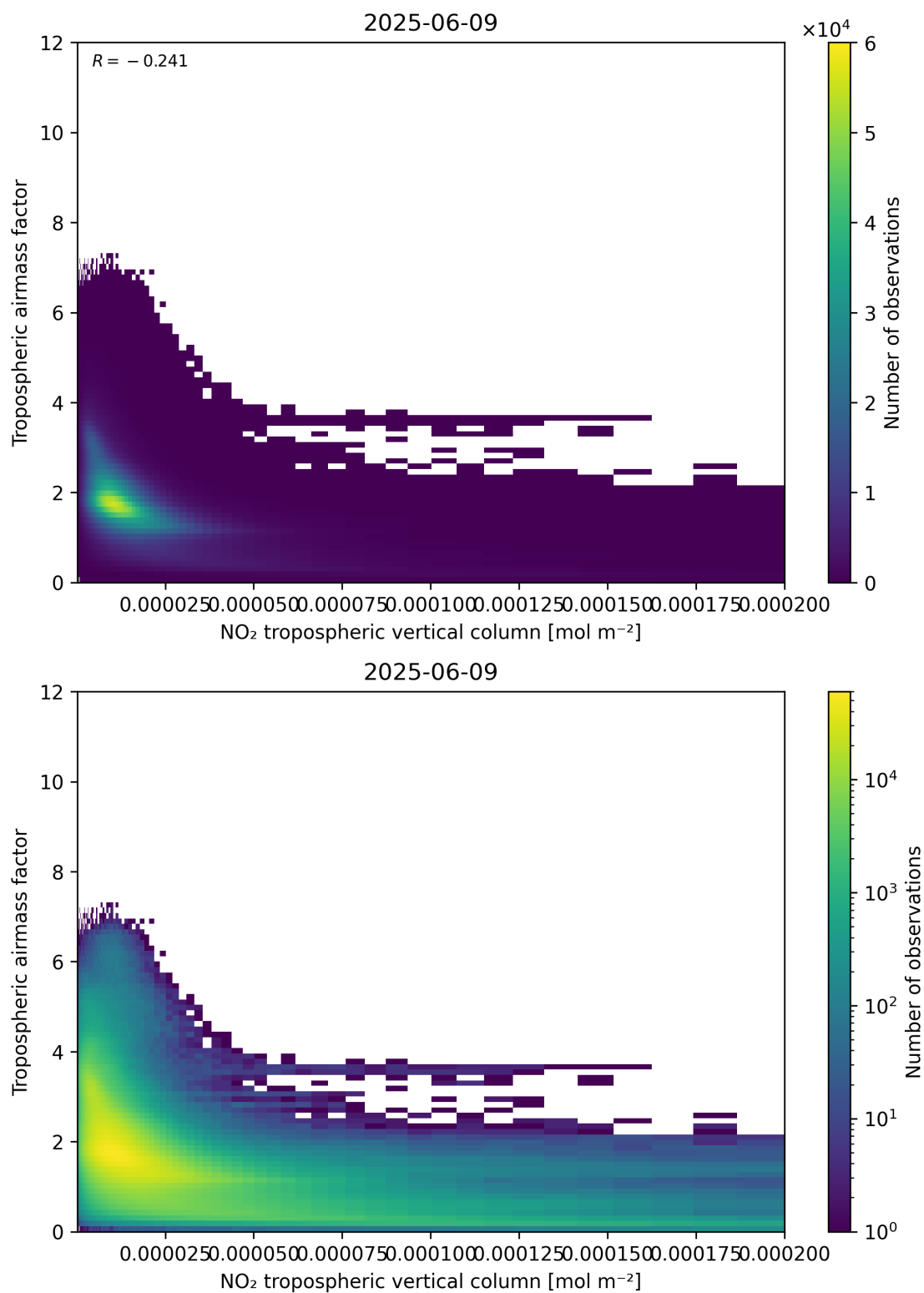
Figure 123: Scatter density plot of “NO 2 tropospheric vertical column” against “Tropospheric air mass factor” for 2025-06-08 to 2025-06-10.
