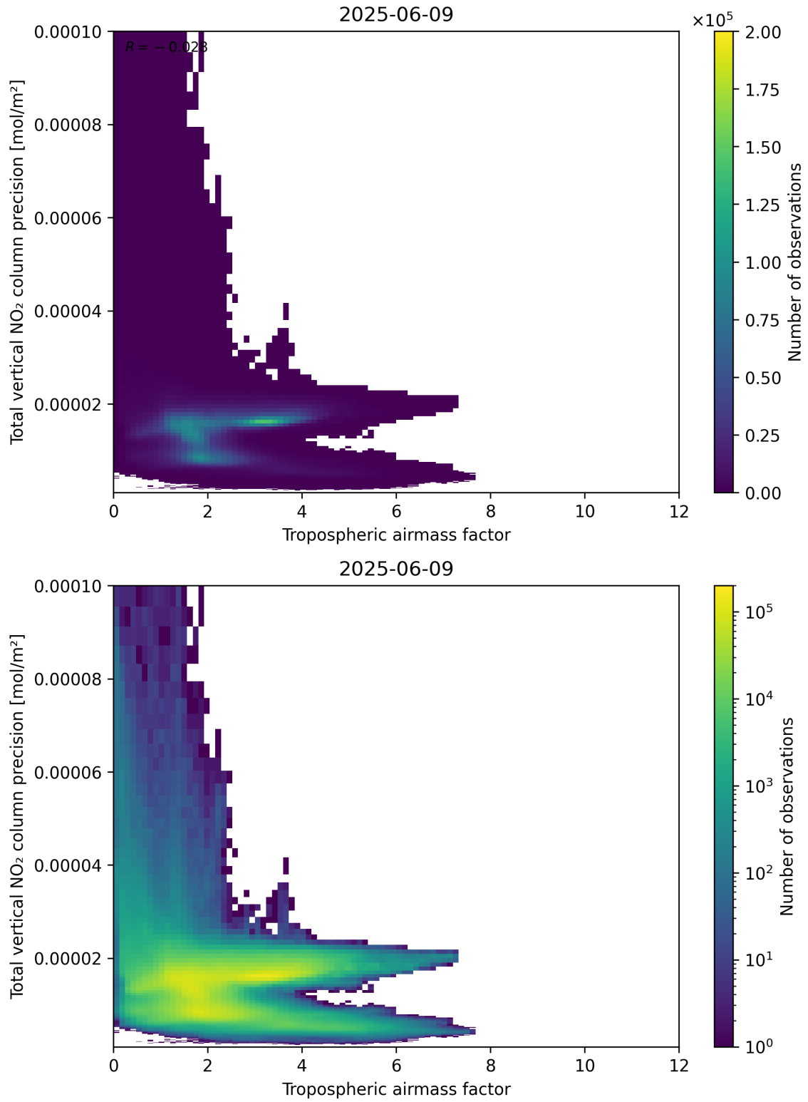
Figure 78: Scatter density plot of “Tropospheric air mass factor” against “Total vertical NO 2 column precision” for 2025-06-08 to 2025-06-10.
