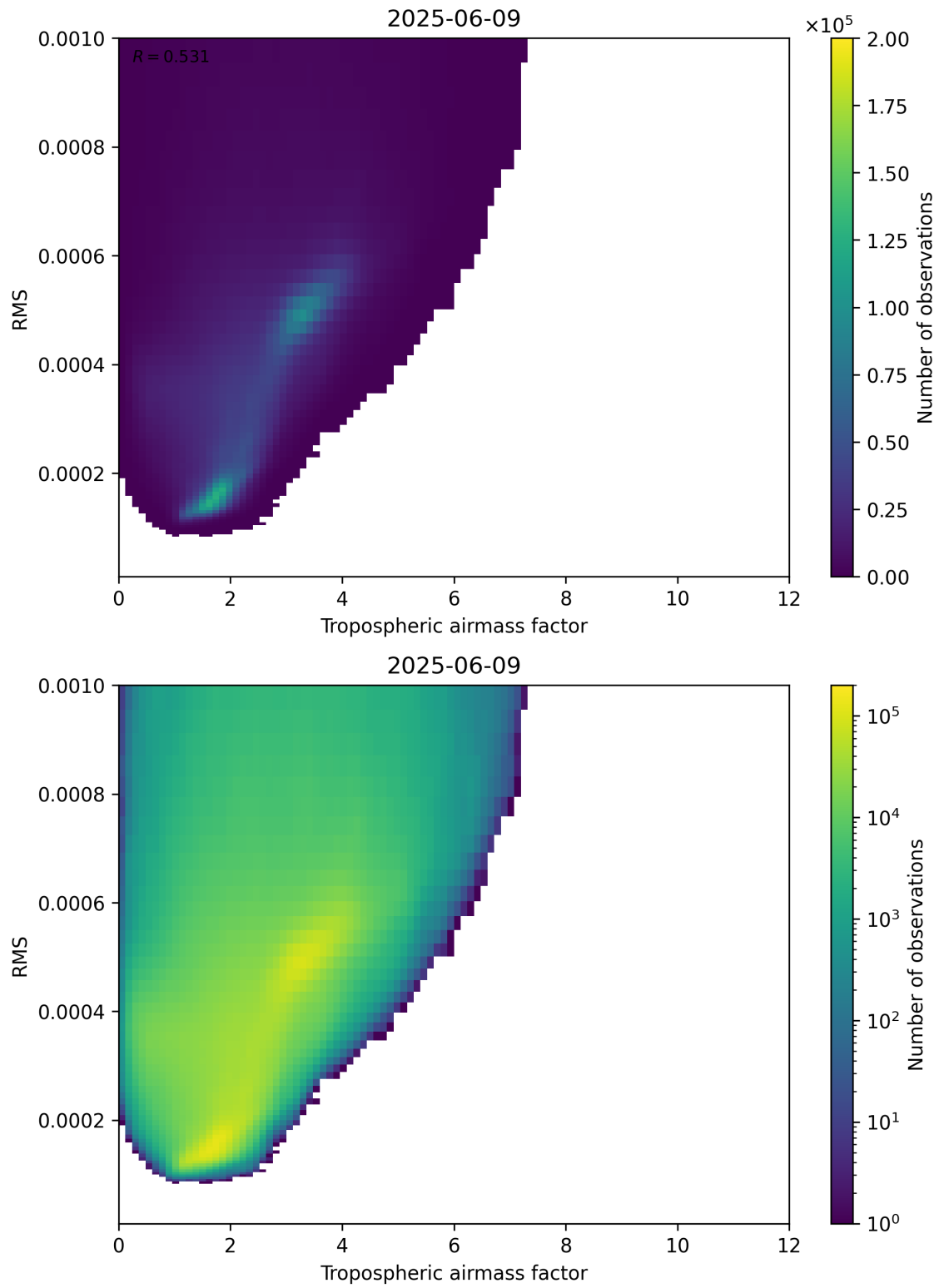
Figure 79: Scatter density plot of “Tropospheric airmass factor” against “RMS” for 2025-06-08 to 2025-06-10.
