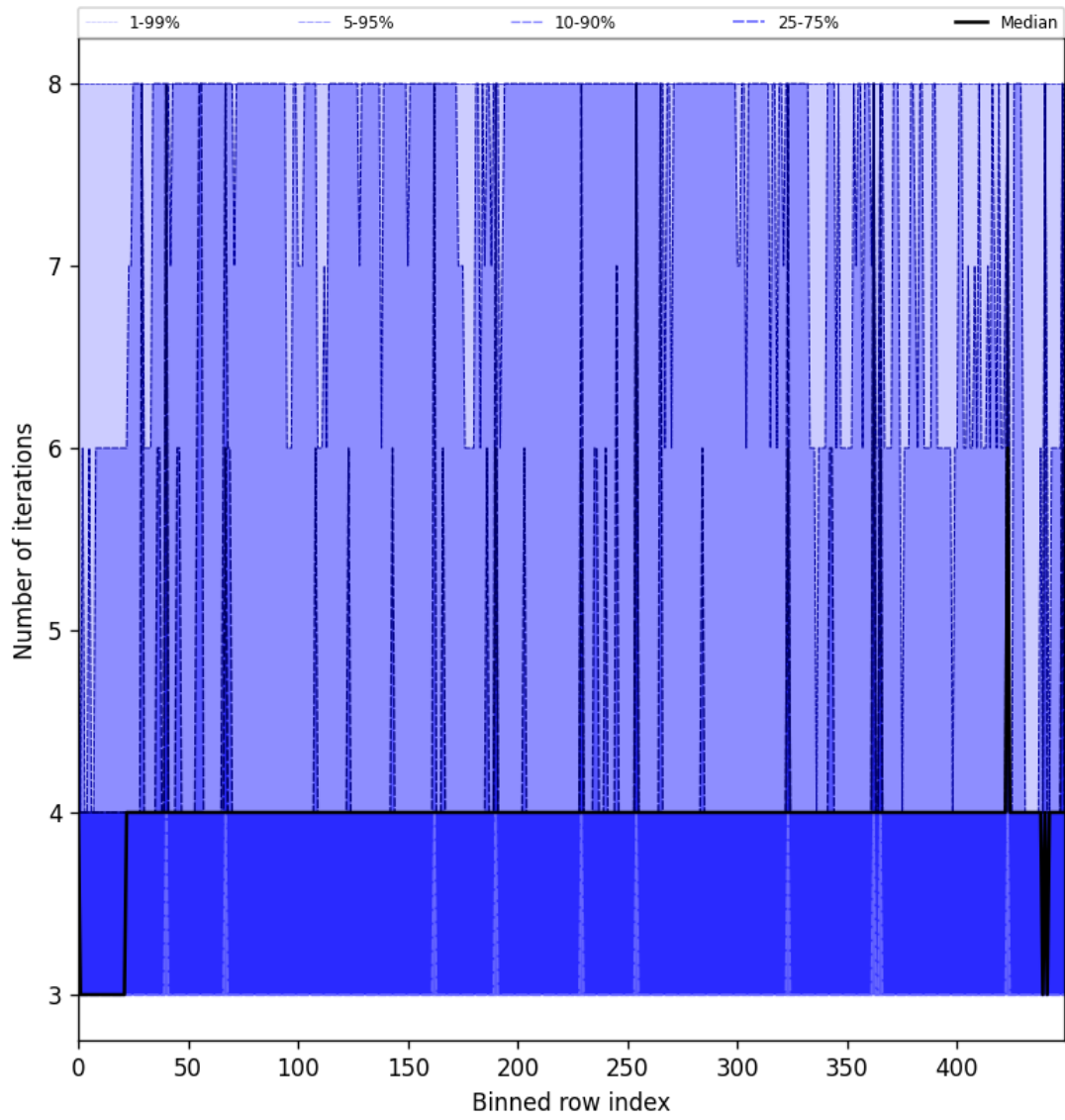
Figure 51: Along track statistics of “Number of iterations” for 2025-06-08 to 2025-06-10
