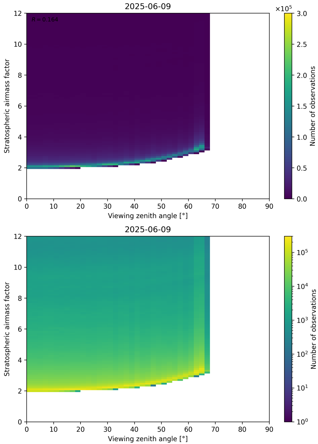
Figure 159: Scatter density plot of “Viewing zenith angle” against “Stratospheric airmass factor” for 2025-06-08 to 2025-06-10.
