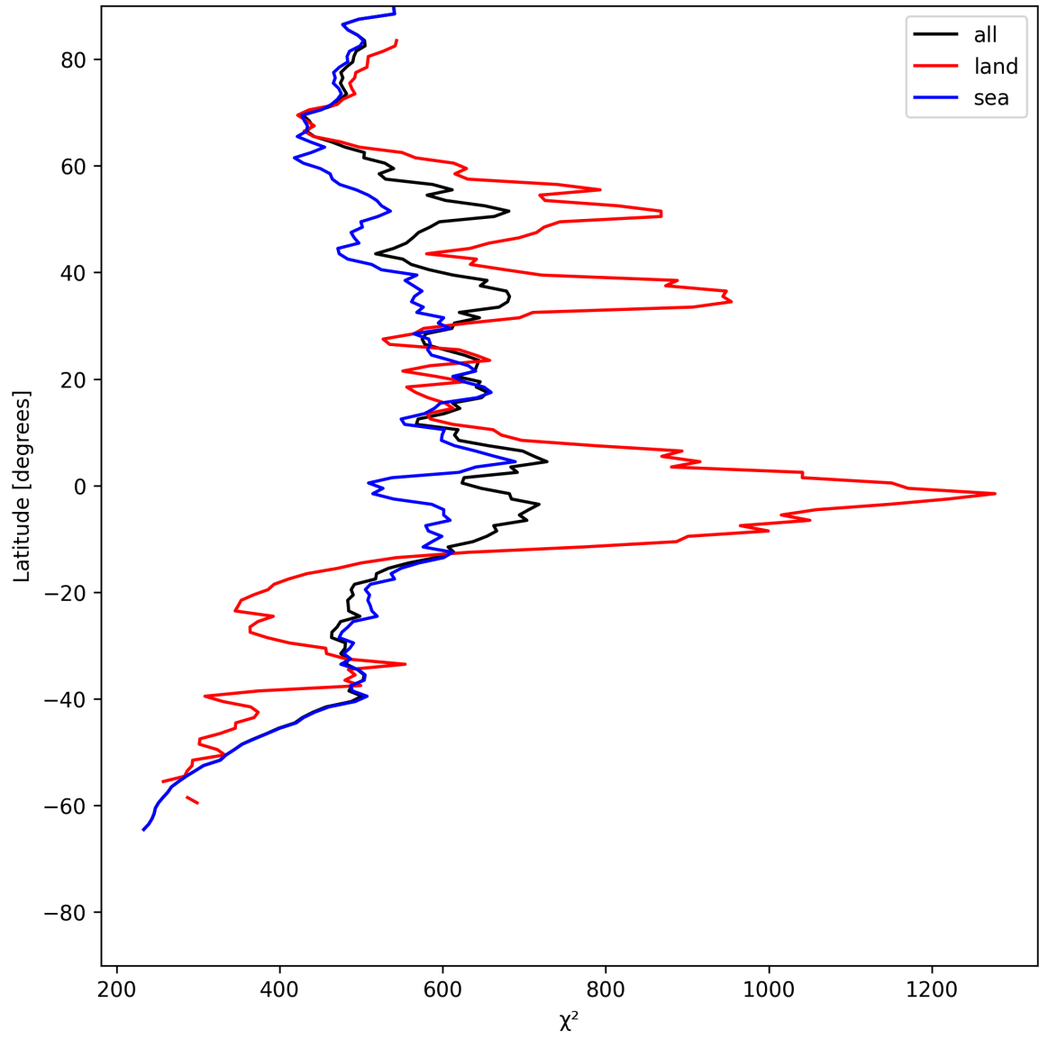
Figure 25: Zonal average of “ \chi^2 ” for 2025-06-08 to 2025-06-10.
