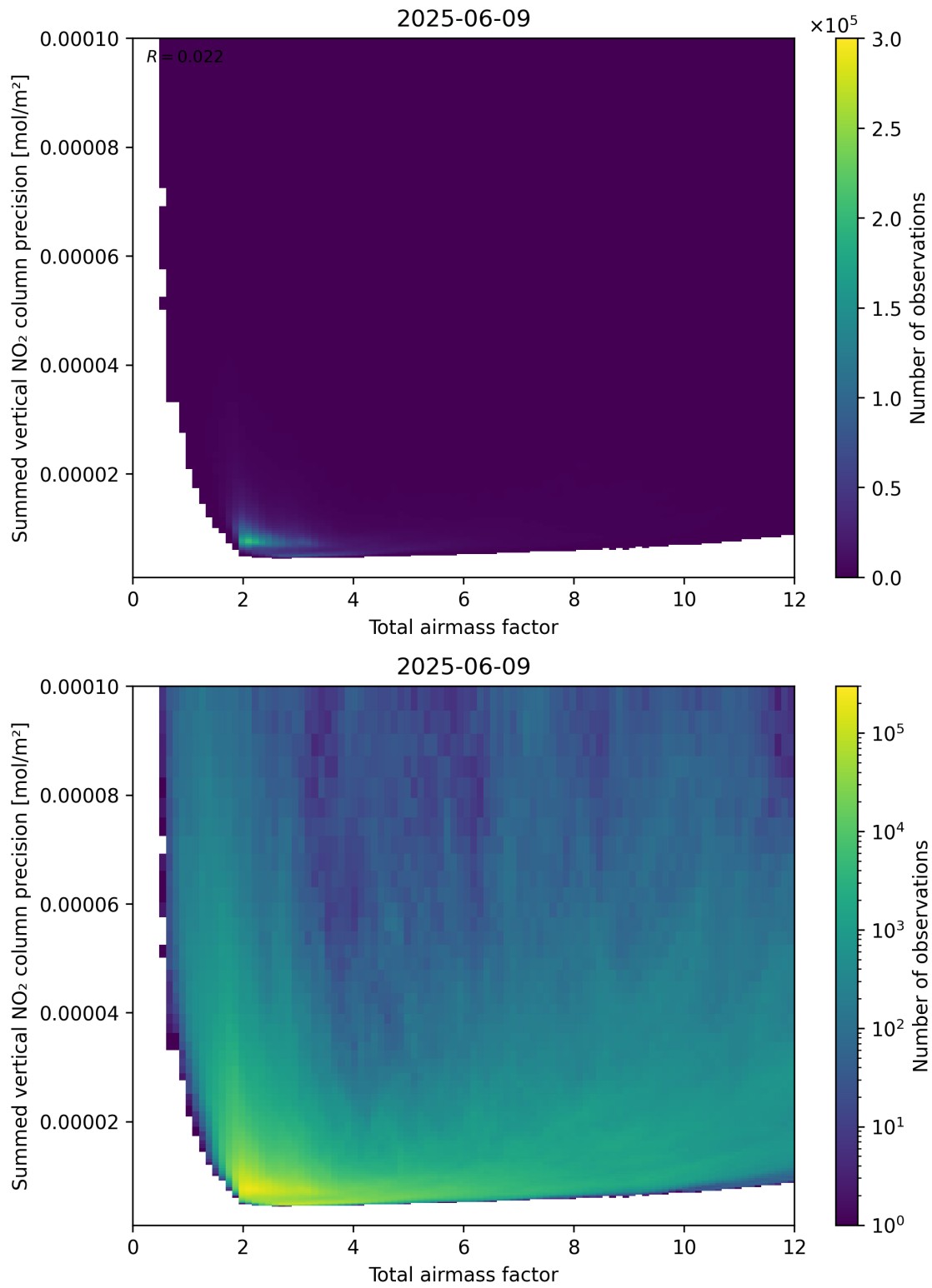
Figure 66: Scatter density plot of “Total airmass factor” against “Summed vertical NO 2 column precision” for 2025-06-08 to 2025-06-10.
