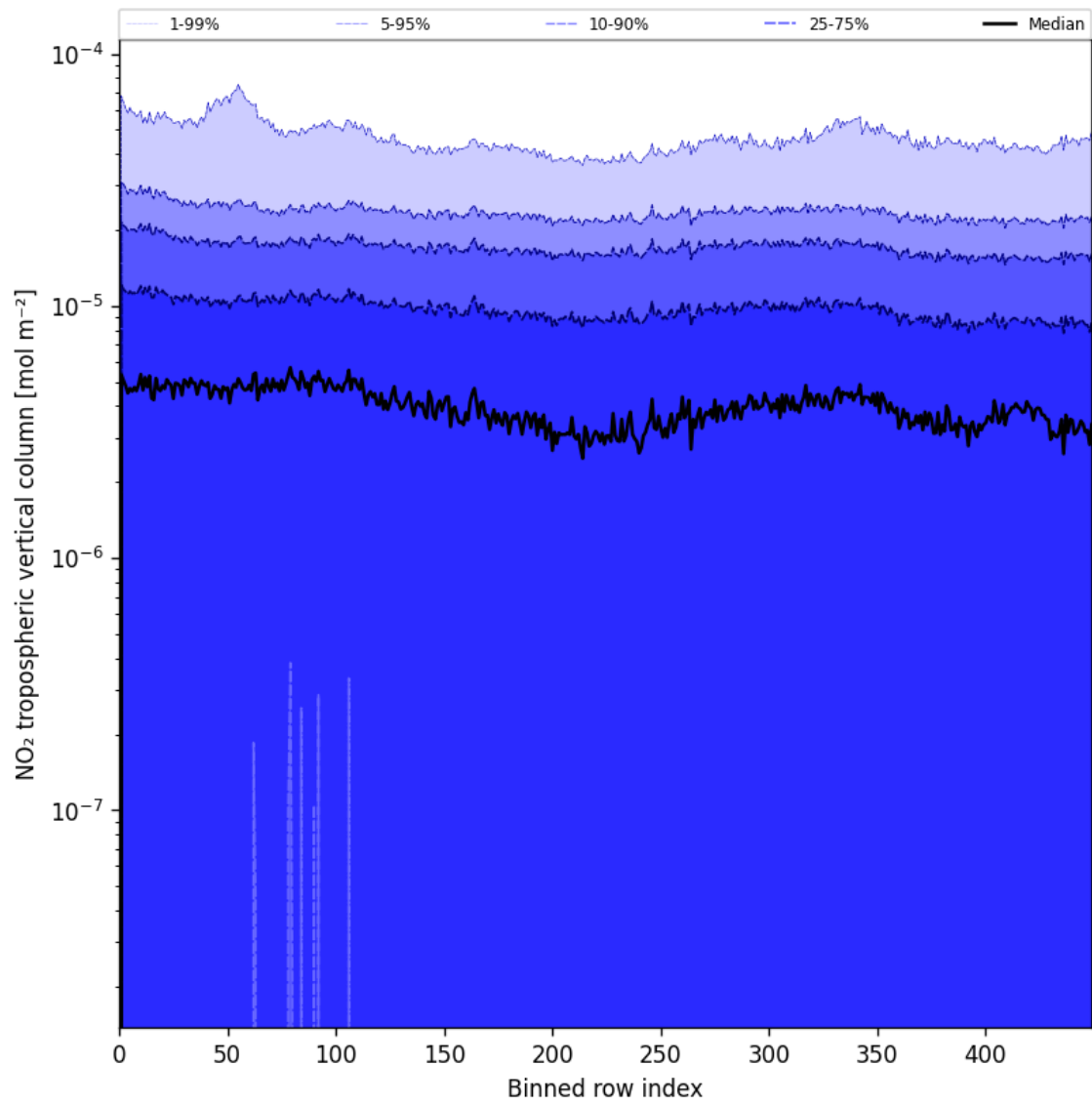
Figure 46: Along track statistics of “NO 2 tropospheric vertical column” for 2025-06-08 to 2025-06-10
