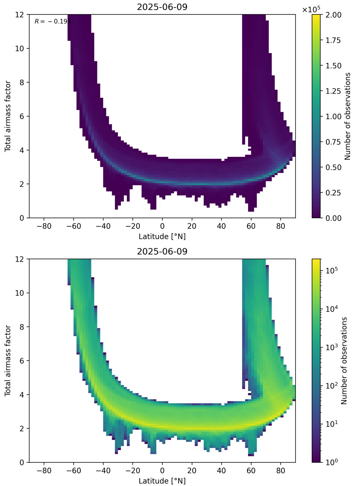
Figure 84: Scatter density plot of “Latitude” against “Total airmass factor” for 2025-06-08 to 2025-06-10.
