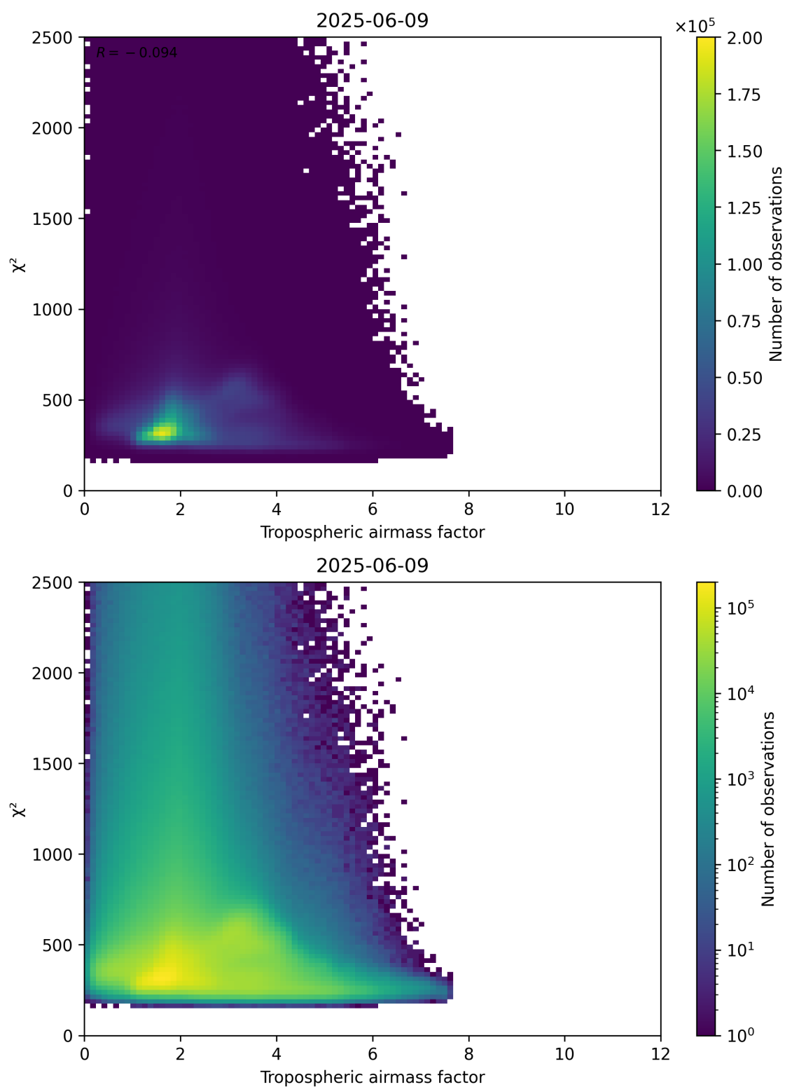
Figure 73: Scatter density plot of “Tropospheric airmass factor” against “ \chi^2 ” for 2025-06-08 to 2025-06-10.
