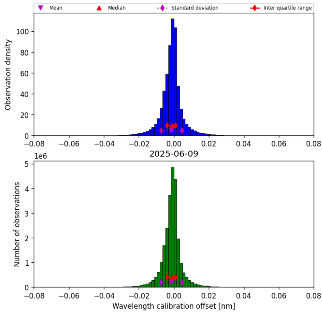
Figure 35: Histogram of “Wavelength calibration offset” for 2025-06-08 to 2025-06-10
