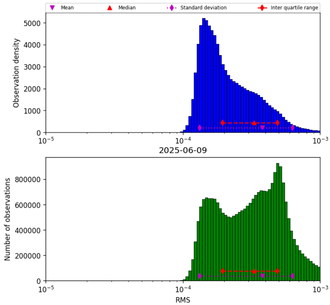
Figure 43: Histogram of “RMS” for 2025-06-08 to 2025-06-10
