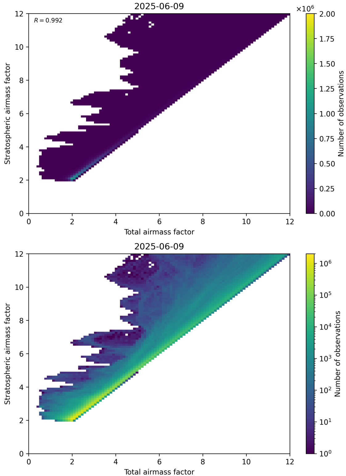
Figure 62: Scatter density plot of “Total airmass factor” against “Stratospheric airmass factor” for 2025-06-08 to 2025-06-10.
