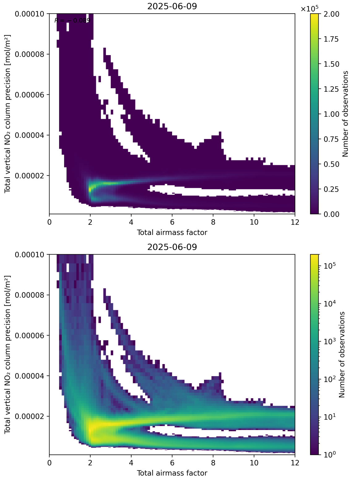
Figure 68: Scatter density plot of “Total airmass factor” against “Total vertical NO 2 column precision” for 2025-06-08 to 2025-06-10.
