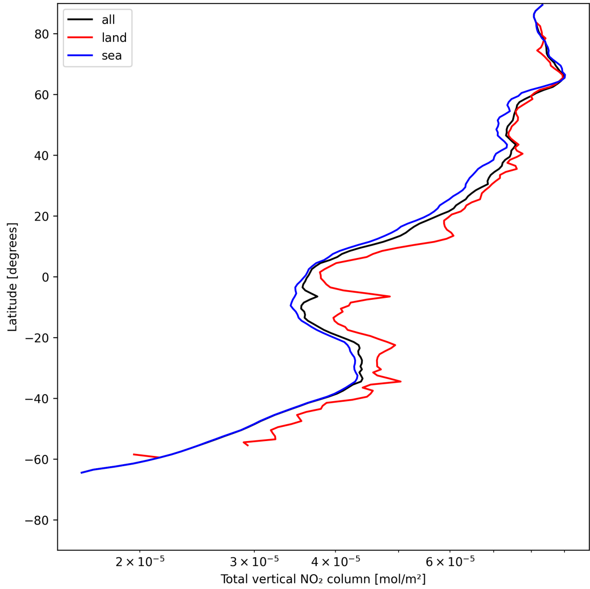
Figure 21: Zonal average of “Total vertical NO 2 column” for 2025-06-08 to 2025-06-10.
