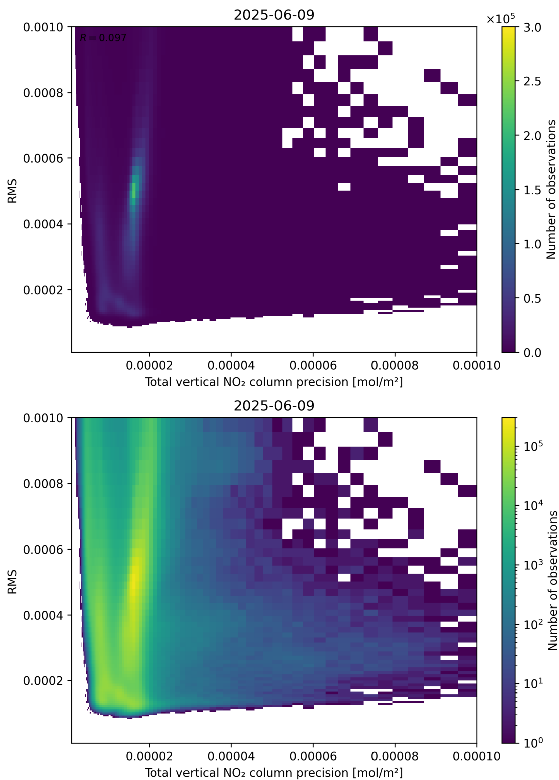
Figure 119: Scatter density plot of “Total vertical NO 2 column precision” against “RMS” for 2025-06-08 to 2025-06-10.
