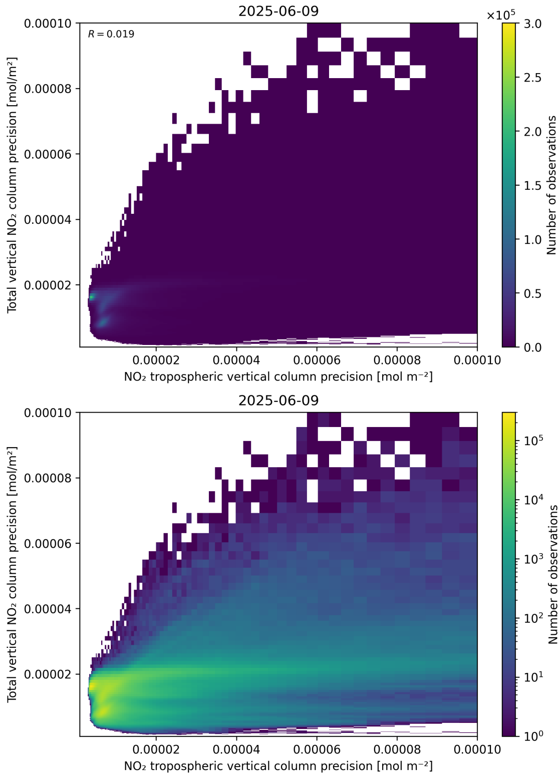
Figure 139: Scatter density plot of “NO 2 tropospheric vertical column precision” against “Total vertical NO 2 column precision” for 2025-06-08 to 2025-06-10.
