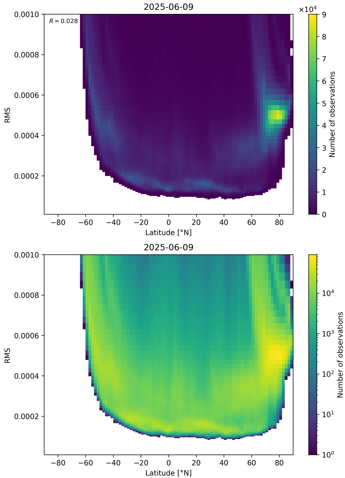
Figure 94: Scatter density plot of “Latitude” against “RMS” for 2025-06-08 to 2025-06-10.
