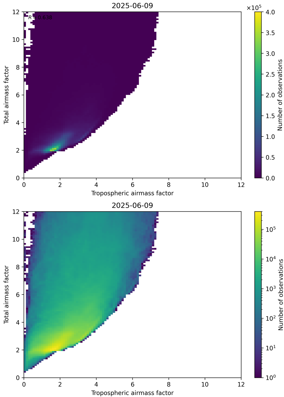
Figure 72: Scatter density plot of “Tropospheric airmass factor” against “Total airmass factor” for 2025-06-08 to 2025-06-10.
