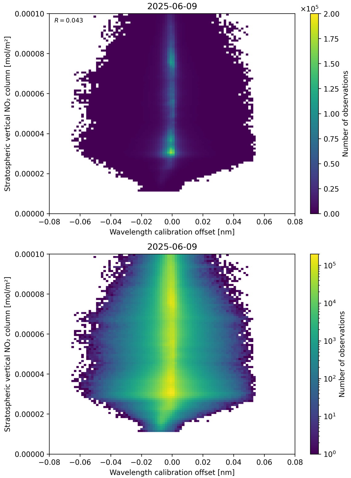
Figure 176: Scatter density plot of “Wavelength calibration offset” against “Stratospheric vertical NO 2 column” for 2025-06-08 to 2025-06-10.
