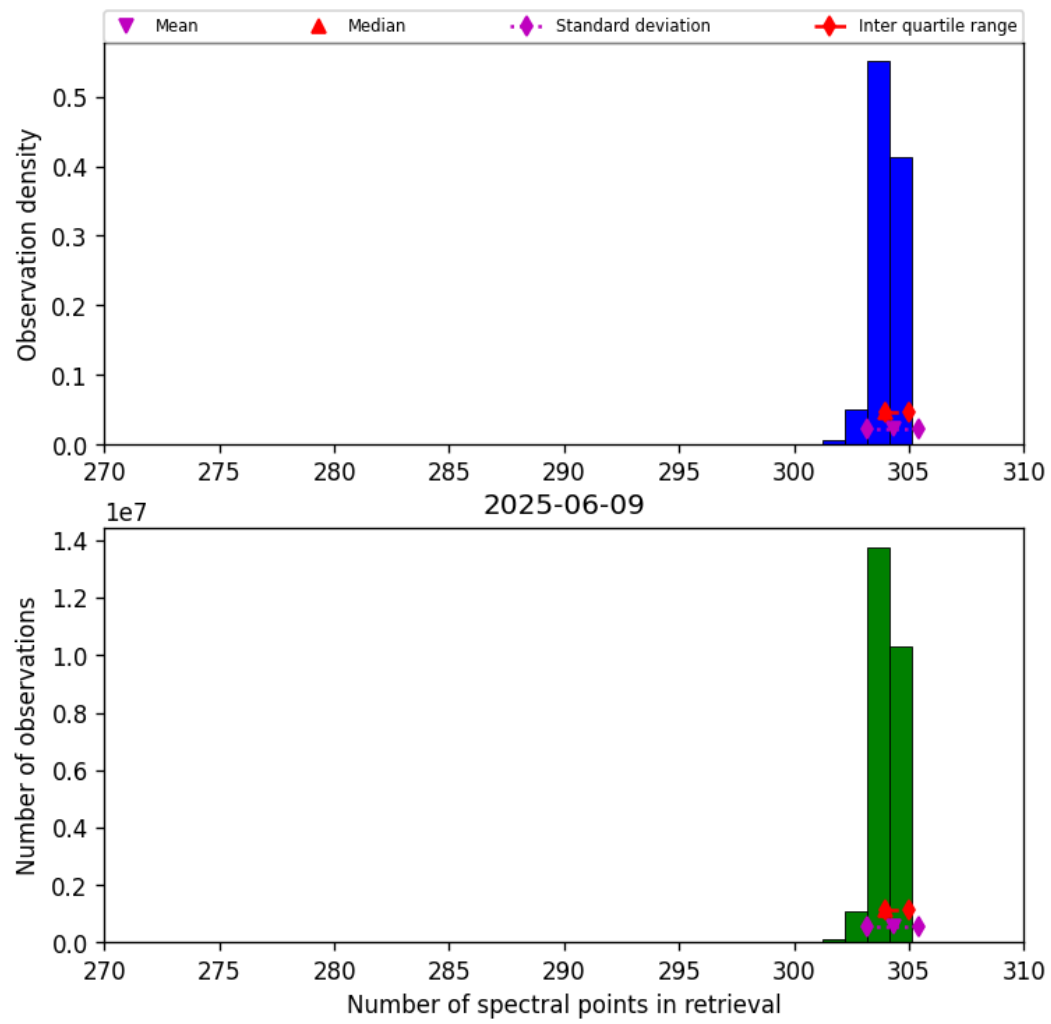
Figure 33: Histogram of “Number of spectral points in retrieval” for 2025-06-08 to 2025-06-10
