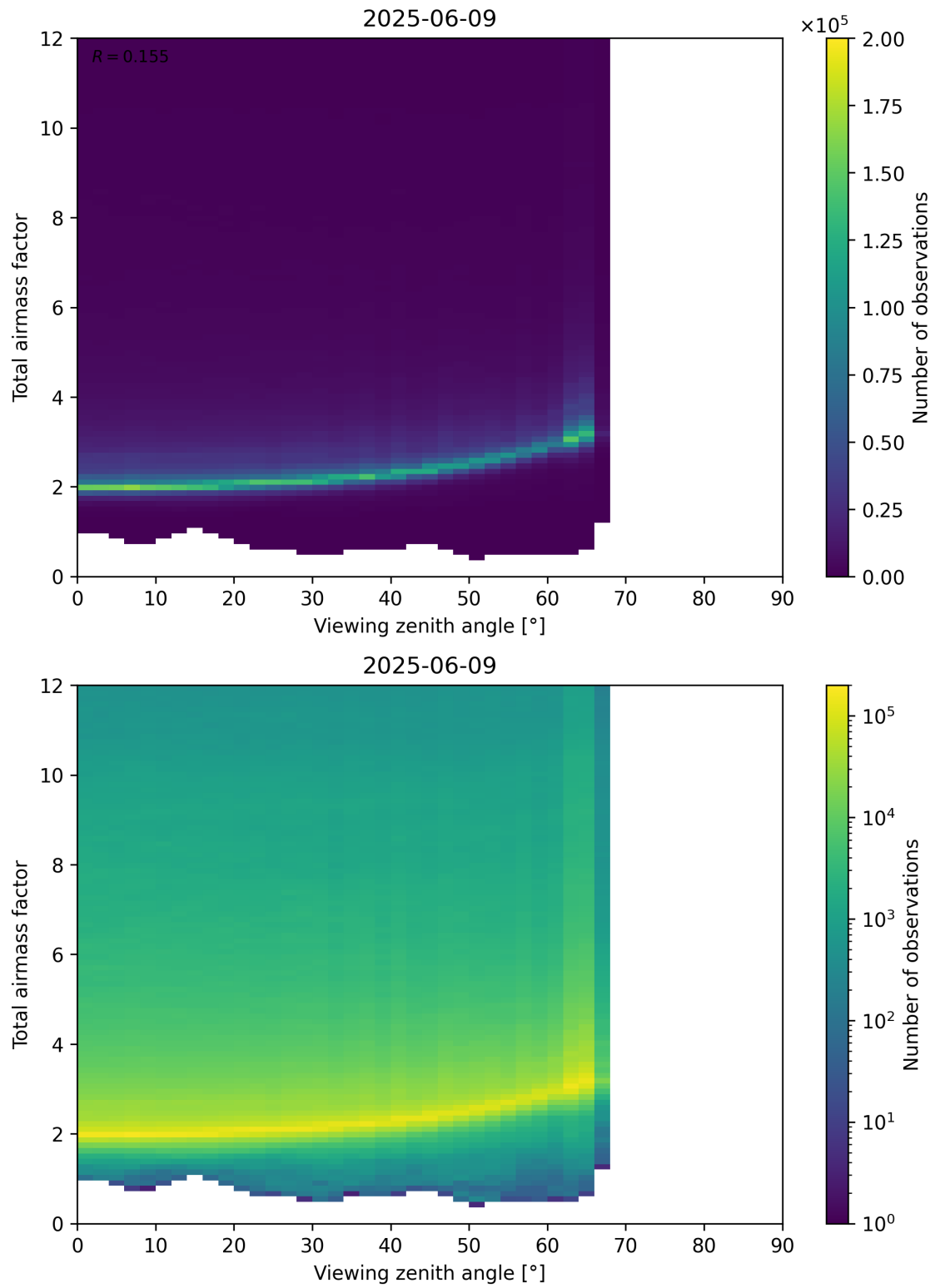
Figure 160: Scatter density plot of “Viewing zenith angle” against “Total airmass factor” for 2025-06-08 to 2025-06-10.
