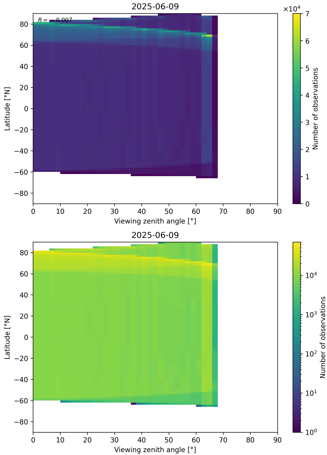
Figure 163: Scatter density plot of “Viewing zenith angle” against “Latitude” for 2025-06-08 to 2025-06-10.
