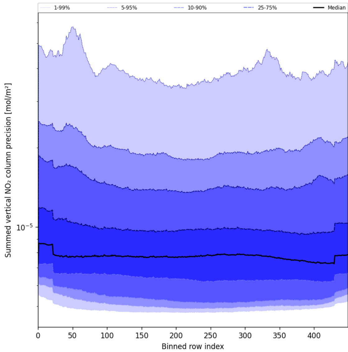
Figure 58: Along track statistics of “Summed vertical NO 2 column precision” for 2025-06-08 to 2025-06-10
