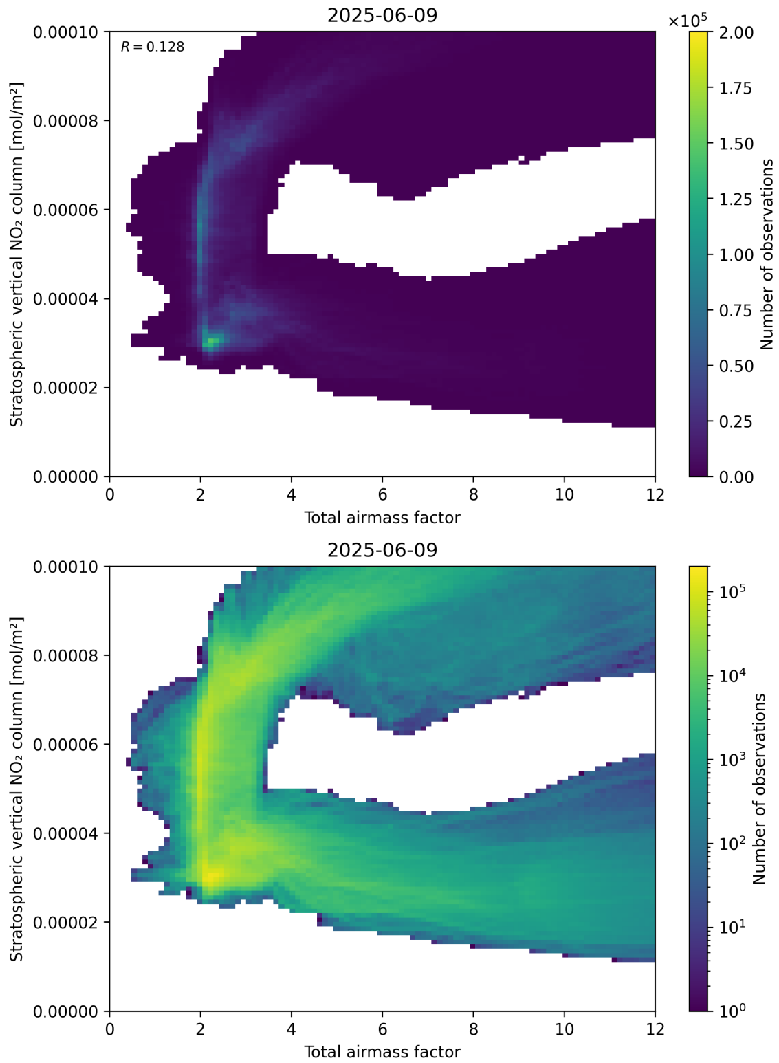
Figure 64: Scatter density plot of “Total airmass factor” against “Stratospheric vertical NO 2 column” for 2025-06-08 to 2025-06-10.
