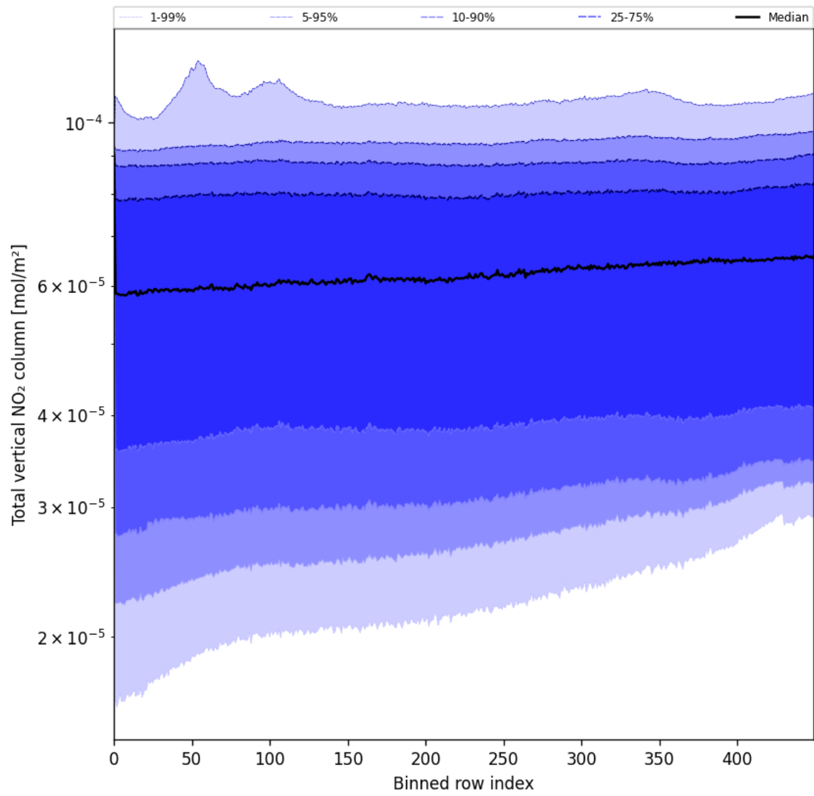
Figure 55: Along track statistics of “Total vertical NO 2 column” for 2025-06-08 to 2025-06-10
