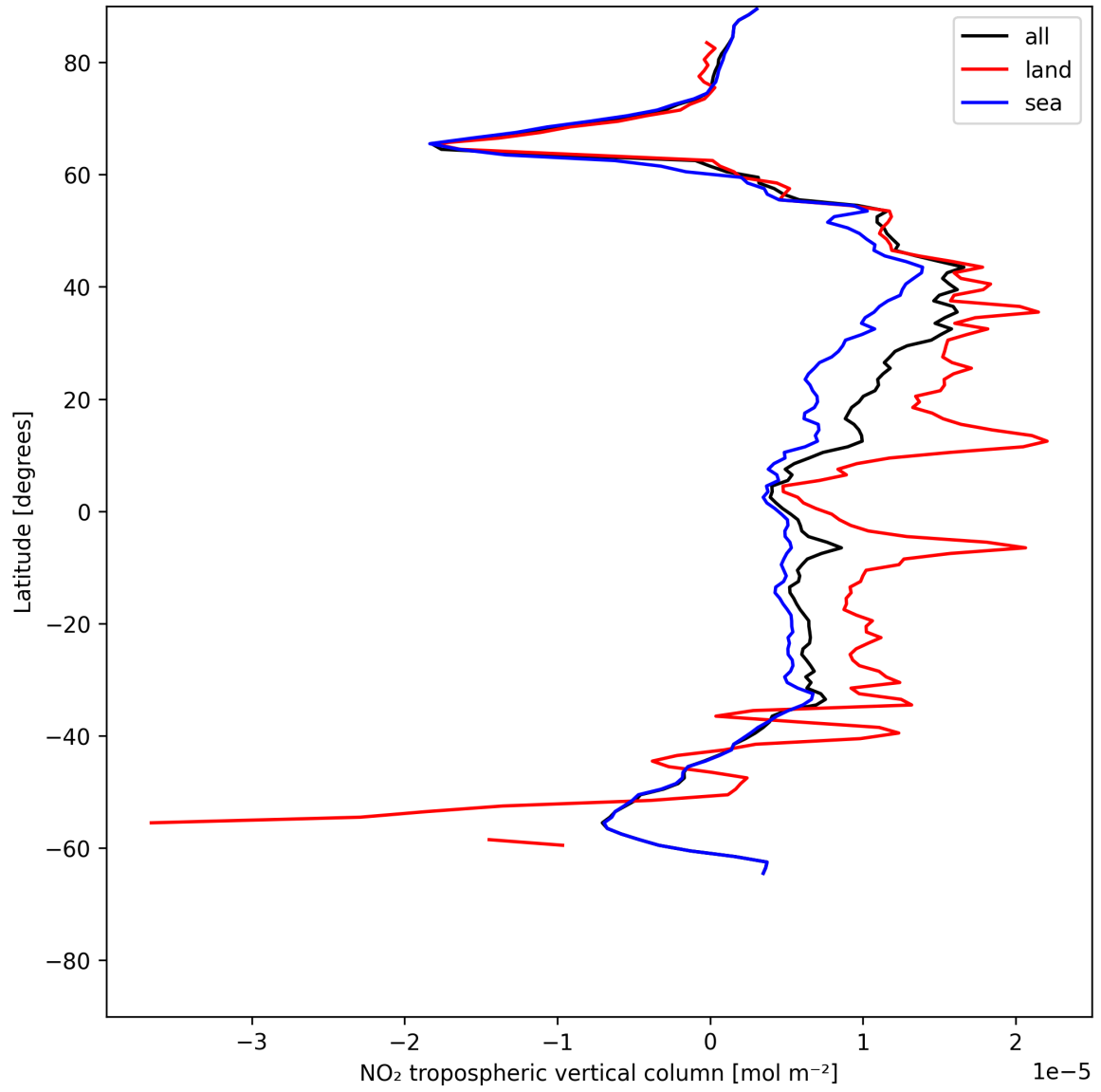
Figure 12: Zonal average of “NO 2 tropospheric vertical column” for 2025-06-08 to 2025-06-10.
