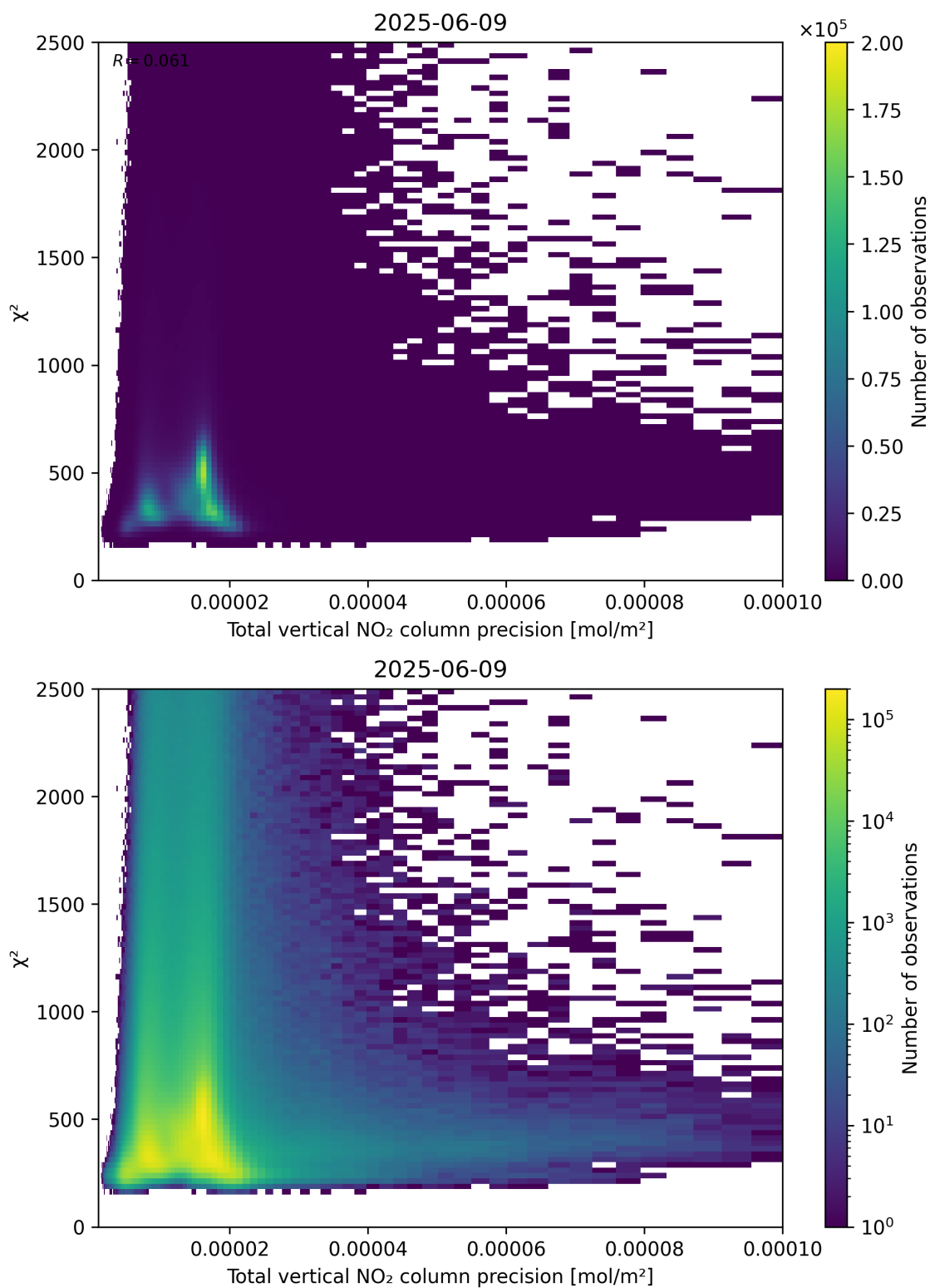
Figure 116: Scatter density plot of “Total vertical NO 2 column precision” against “ \chi^2 ” for 2025-06-08 to 2025-06-10.
