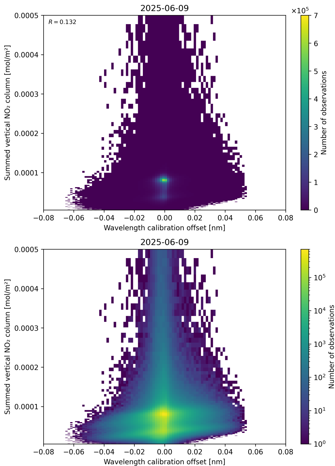
Figure 177: Scatter density plot of “Wavelength calibration offset” against “Summed vertical NO 2 column” for 2025-06-08 to 2025-06-10.
