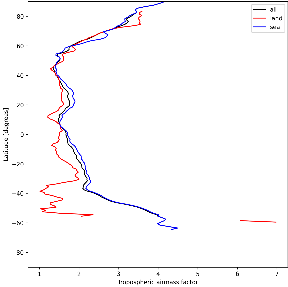
Figure 14: Zonal average of “Tropospheric airmass factor” for 2025-06-08 to 2025-06-10.
