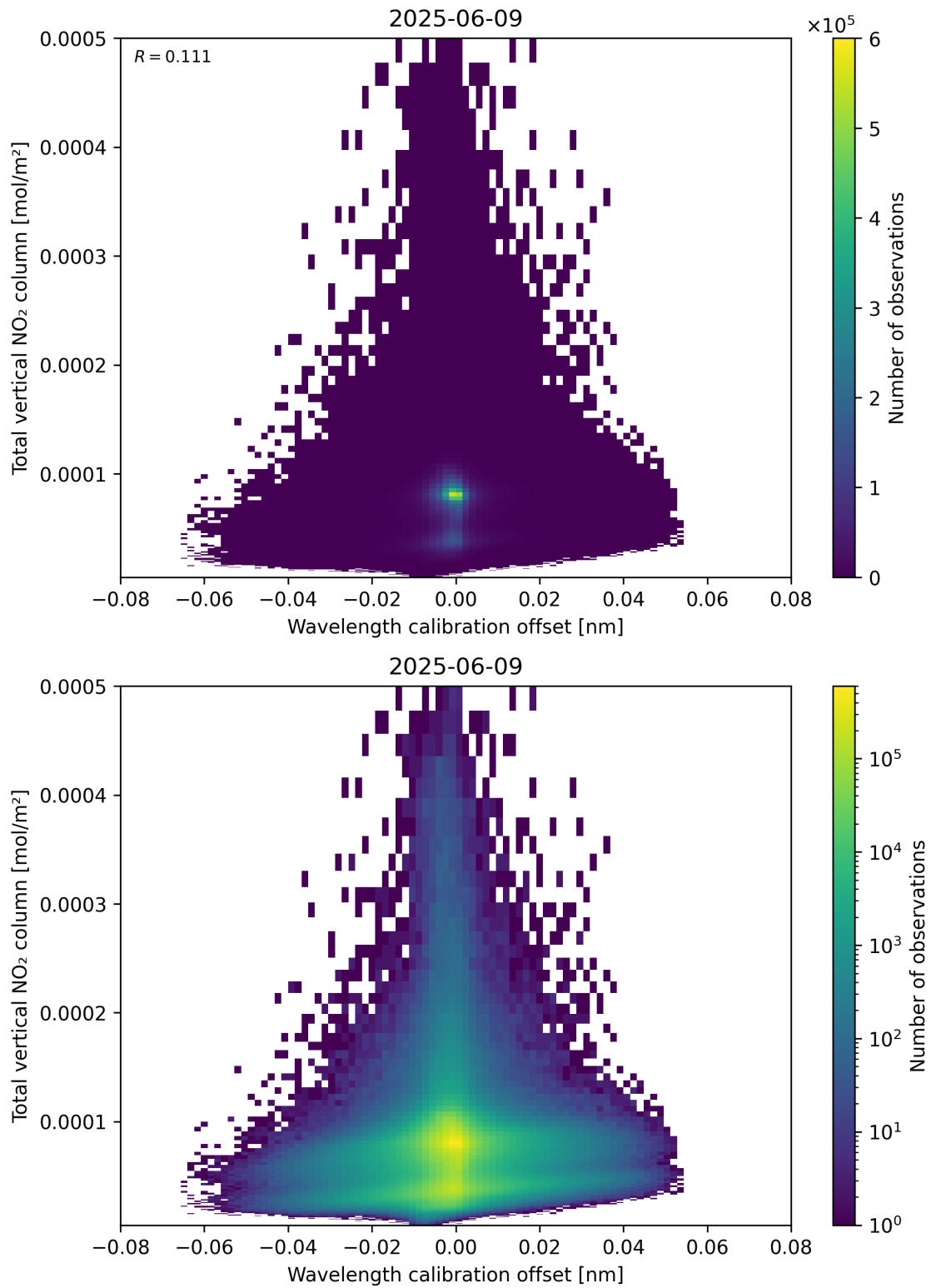
Figure 179: Scatter density plot of “Wavelength calibration offset” against “Total vertical NO 2 column” for 2025-06-08 to 2025-06-10.
