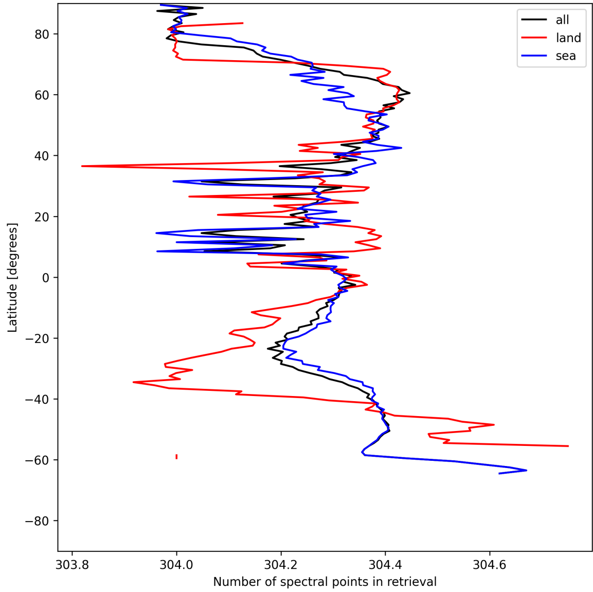
Figure 16: Zonal average of “Number of spectral points in retrieval” for 2025-06-08 to 2025-06-10.
