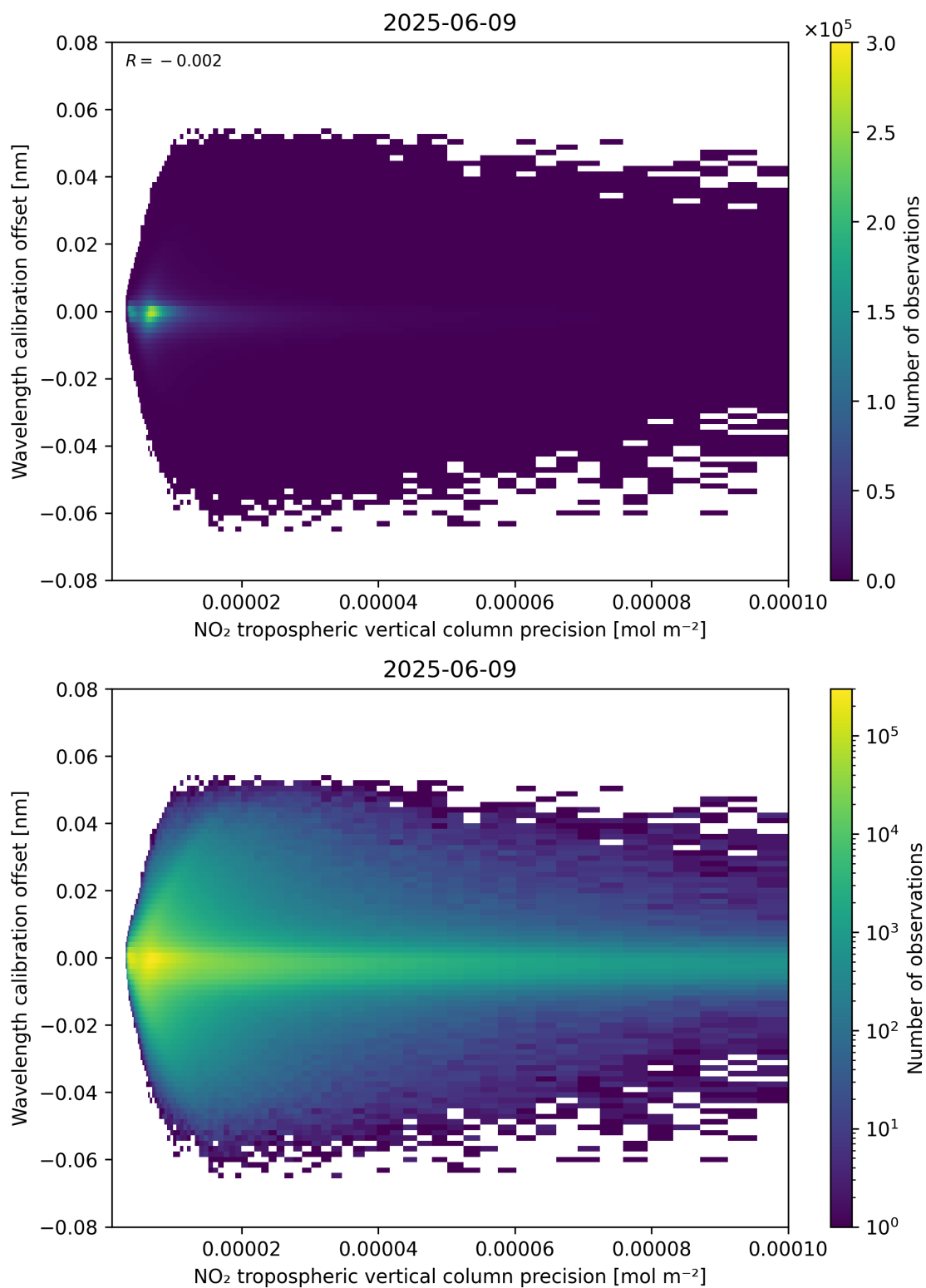
Figure 141: Scatter density plot of “NO 2 tropospheric vertical column precision” against “Wavelength calibration offset” for 2025-06-08 to 2025-06-10.
