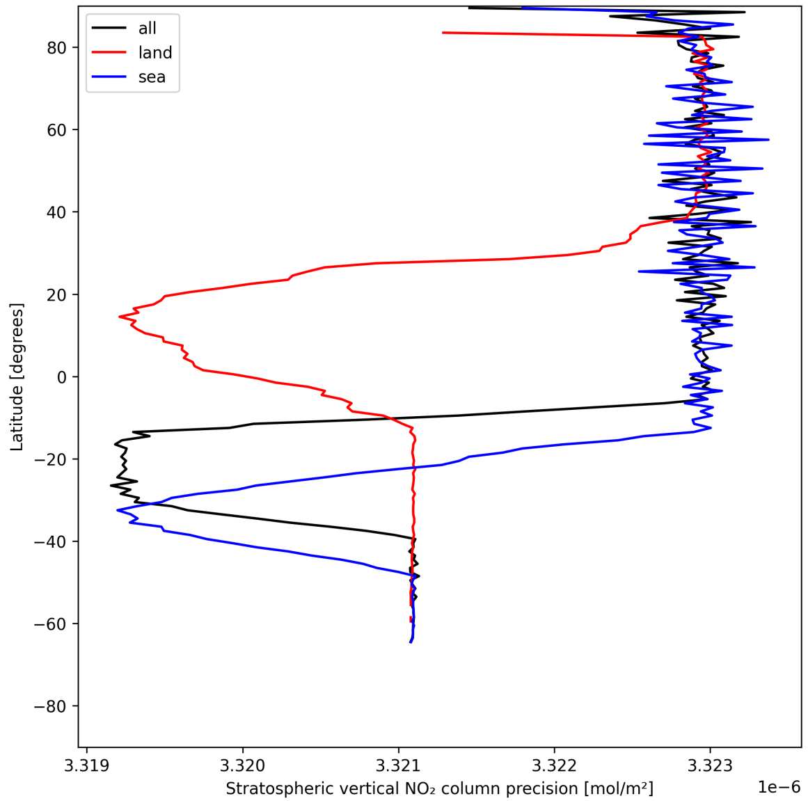
Figure 20: Zonal average of “Stratospheric vertical NO 2 column precision” for 2025-06-08 to 2025-06-10.
