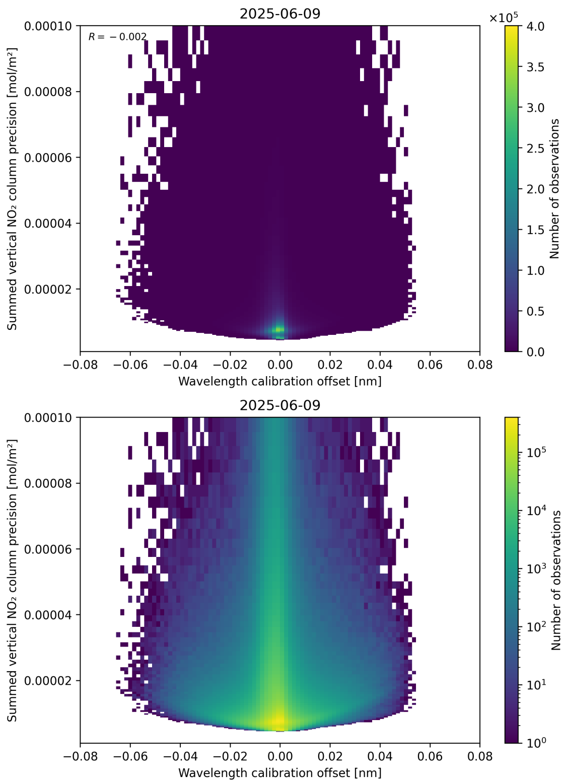
Figure 178: Scatter density plot of “Wavelength calibration offset” against “Summed vertical NO 2 column precision” for 2025-06-08 to 2025-06-10.
