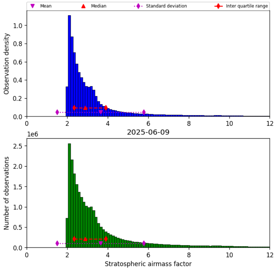
Figure 44: Histogram of “Stratospheric airmass factor” for 2025-06-08 to 2025-06-10
