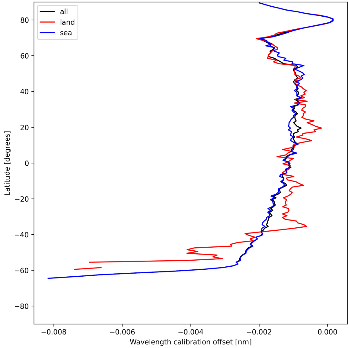
Figure 18: Zonal average of “Wavelength calibration offset” for 2025-06-08 to 2025-06-10.
