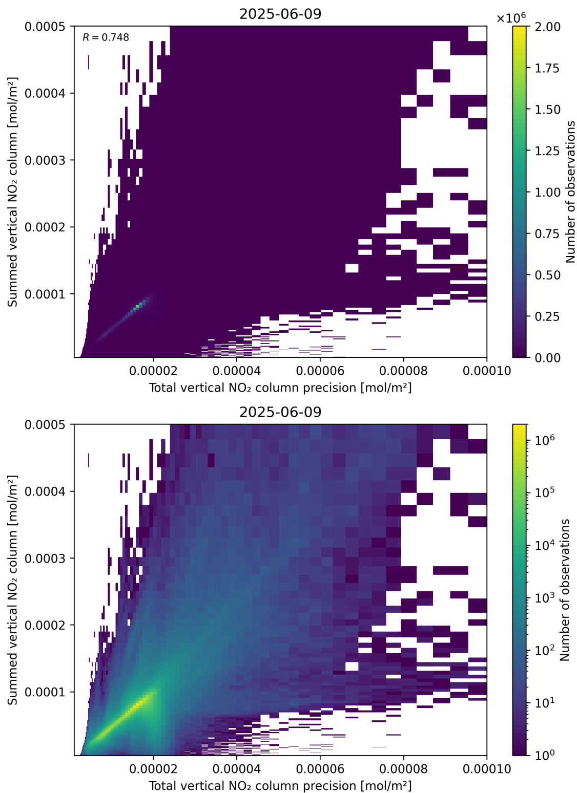
Figure 117: Scatter density plot of “Total vertical NO 2 column precision” against “Summed vertical NO 2 column” for 2025-06-08 to 2025-06-10.
