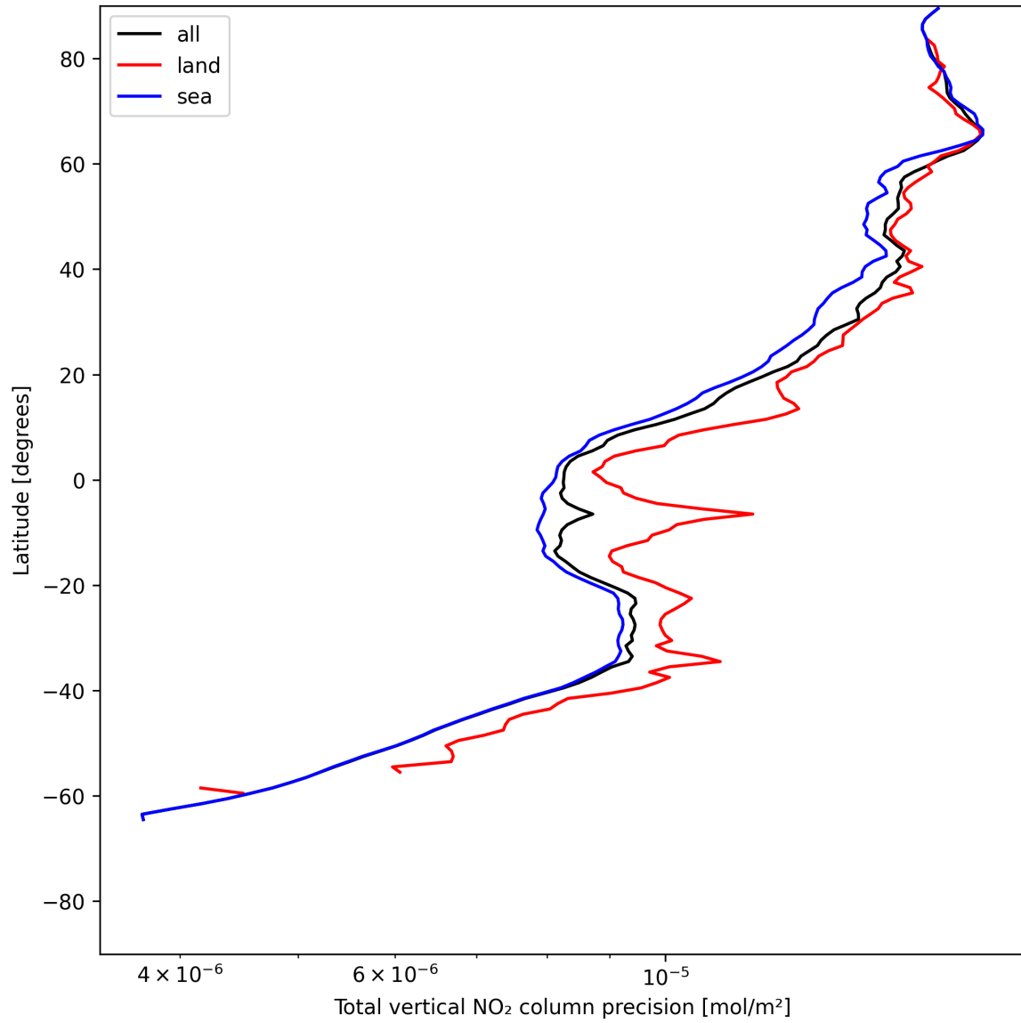
Figure 22: Zonal average of “Total vertical NO 2 column precision” for 2025-06-08 to 2025-06-10.
