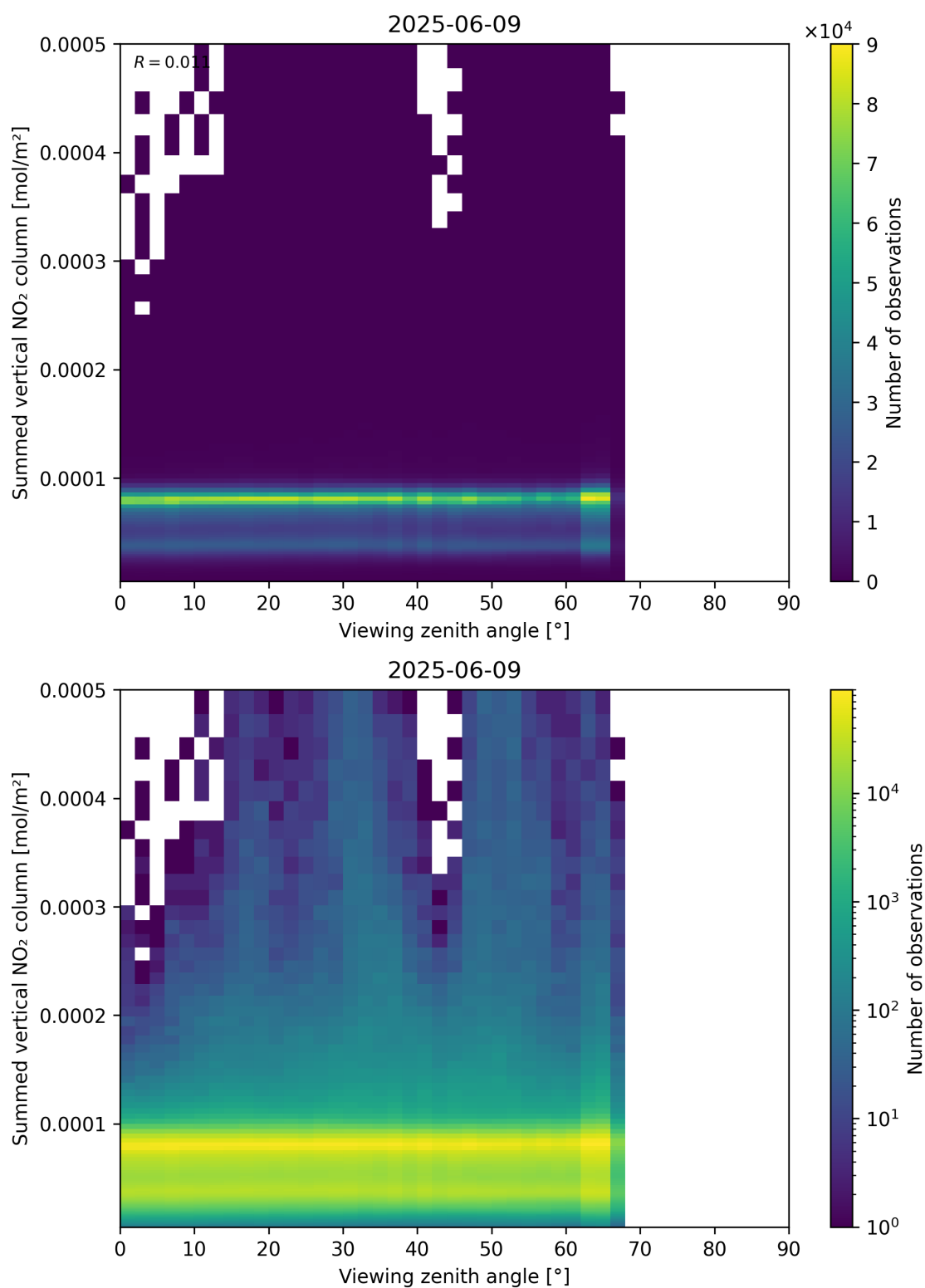
Figure 165: Scatter density plot of “Viewing zenith angle” against “Summed vertical NO 2 column” for 2025-06-08 to 2025-06-10.
