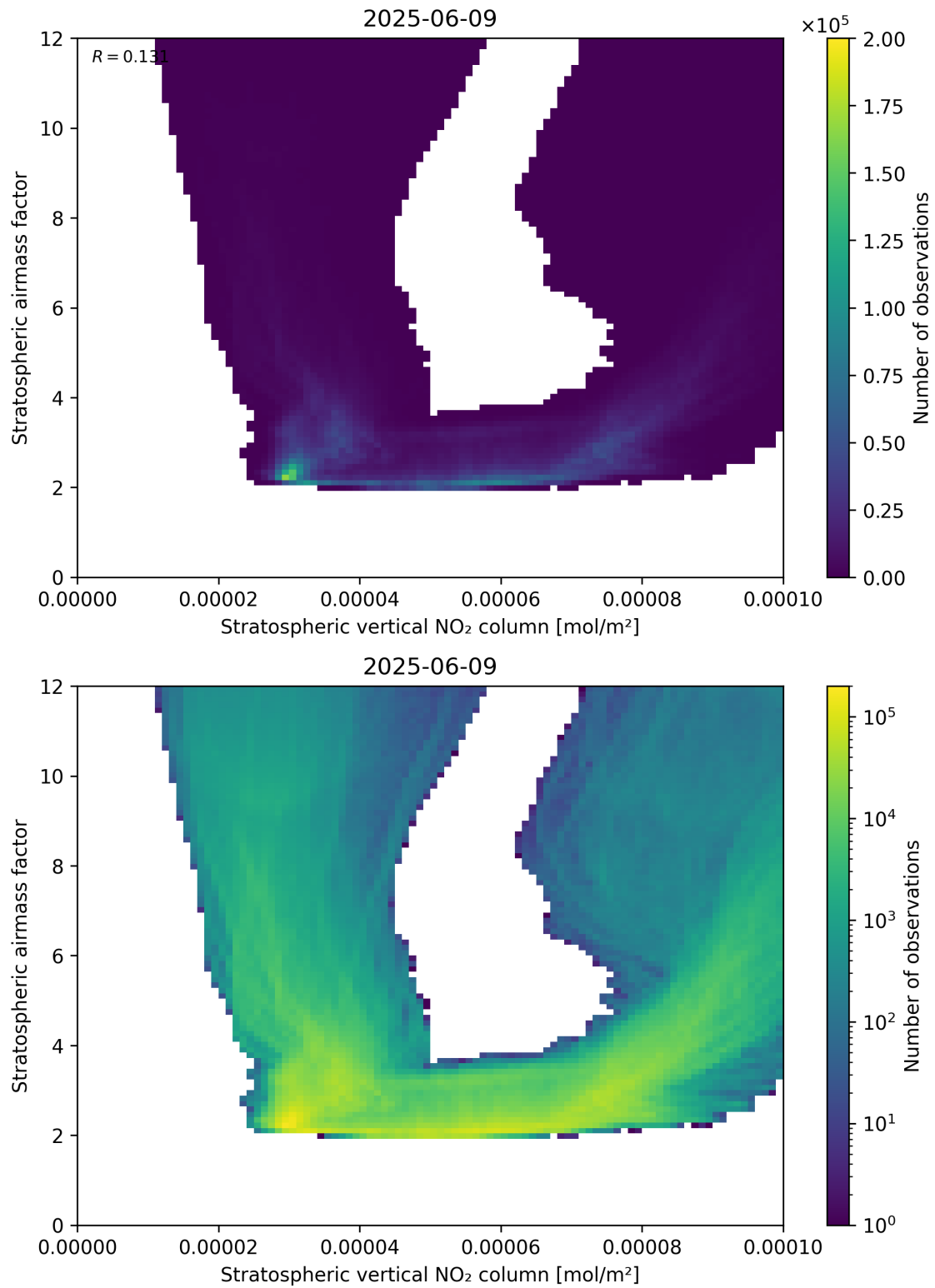
Figure 96: Scatter density plot of “Stratospheric vertical NO 2 column” against “Stratospheric airmass factor” for 2025-06-08 to 2025-06-10.
