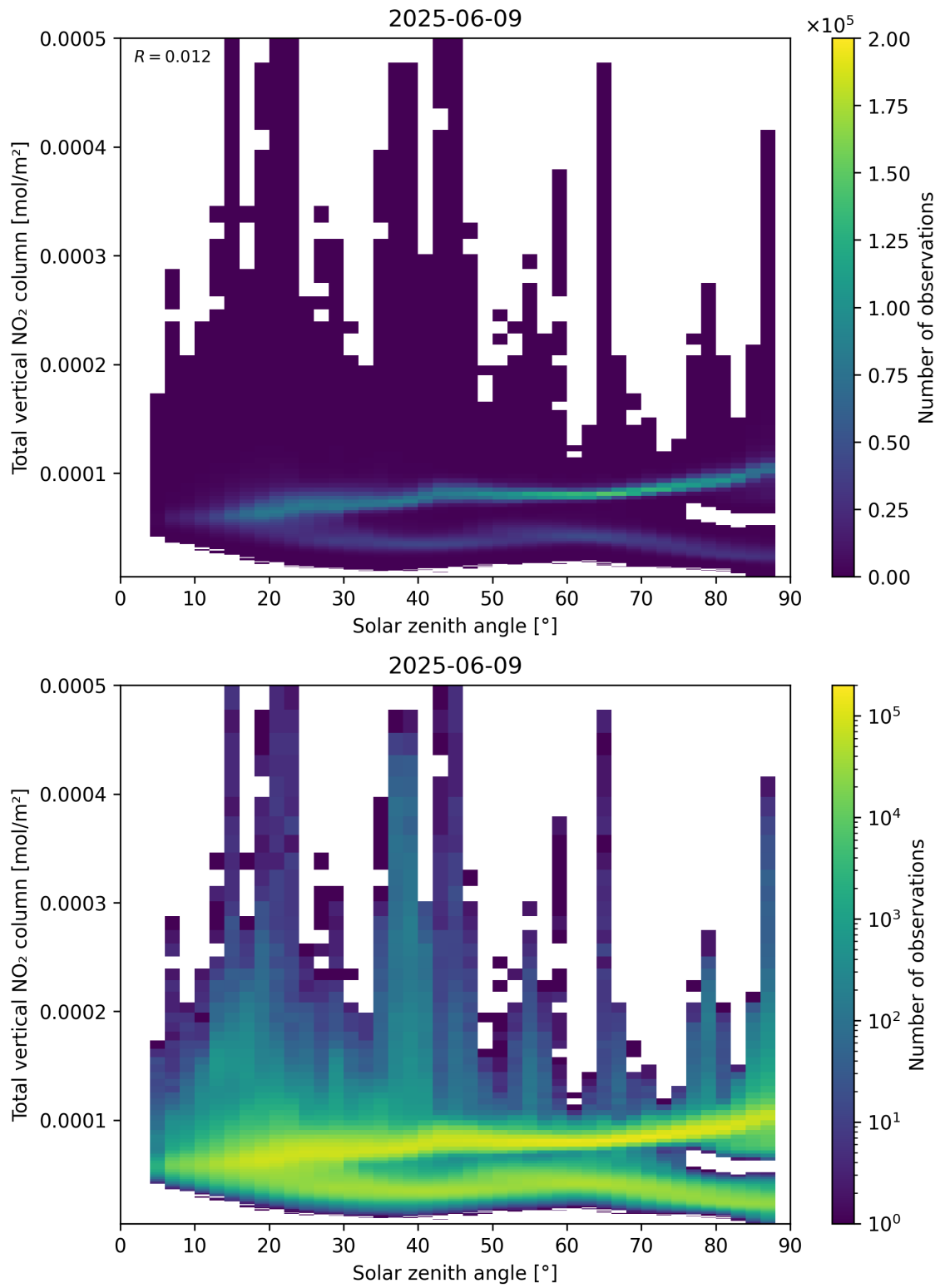
Figure 153: Scatter density plot of “Solar zenith angle” against “Total vertical NO 2 column” for 2025-06-08 to 2025-06-10.
