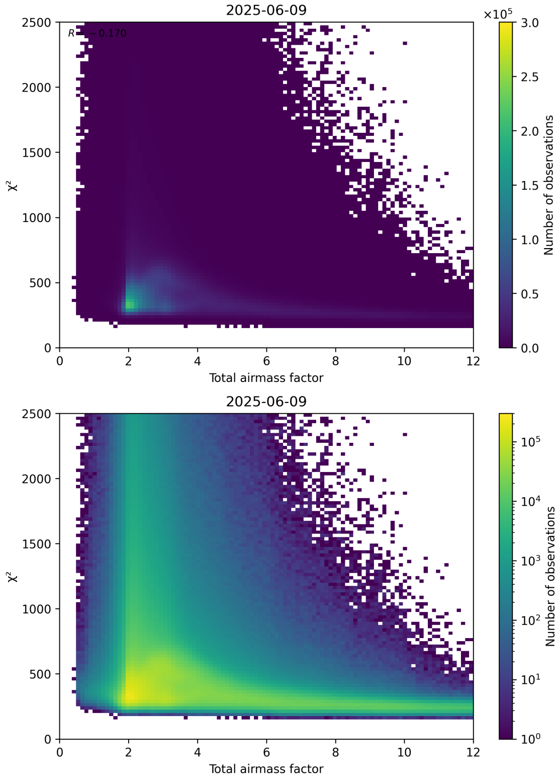
Figure 63: Scatter density plot of “Total airmass factor” against “ \chi^2 ” for 2025-06-08 to 2025-06-10.
