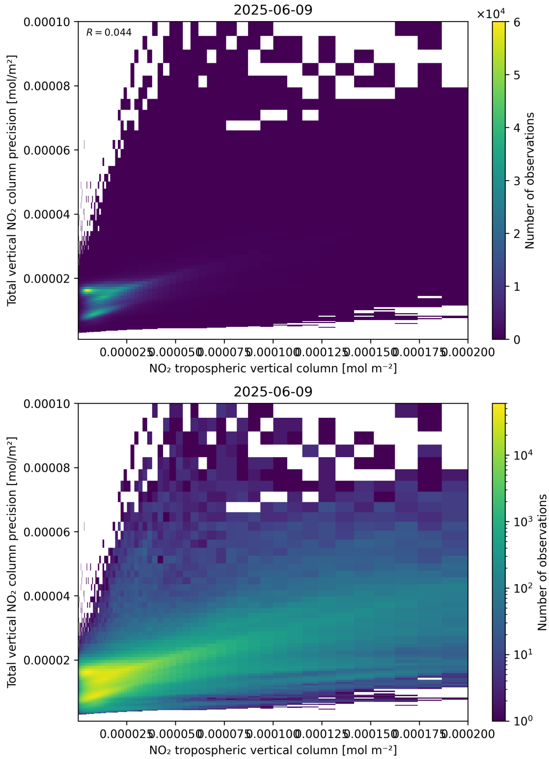
Figure 129: Scatter density plot of “NO 2 tropospheric vertical column” against “Total vertical NO 2 column precision” for 2025-06-08 to 2025-06-10.
