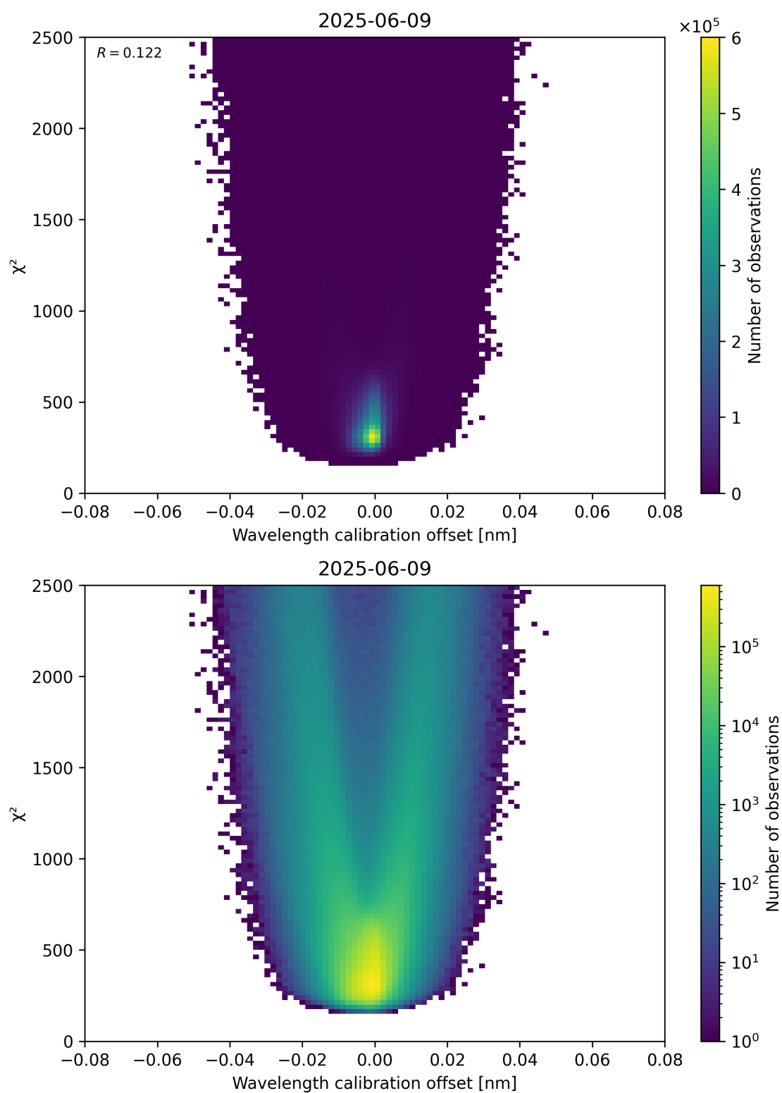
Figure 175: Scatter density plot of “Wavelength calibration offset” against “ \chi^2 ” for 2025-06-08 to 2025-06-10.
