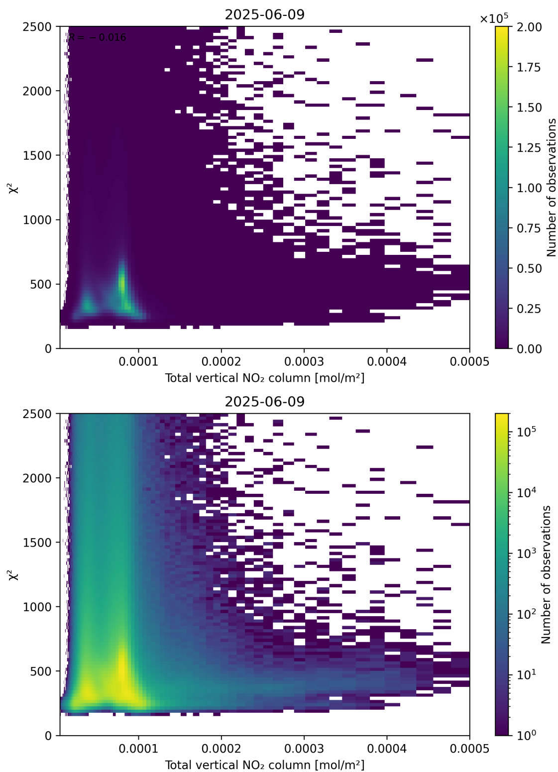
Figure 111: Scatter density plot of “Total vertical NO 2 column” against “ \chi^2 ” for 2025-06-08 to 2025-06-10.
