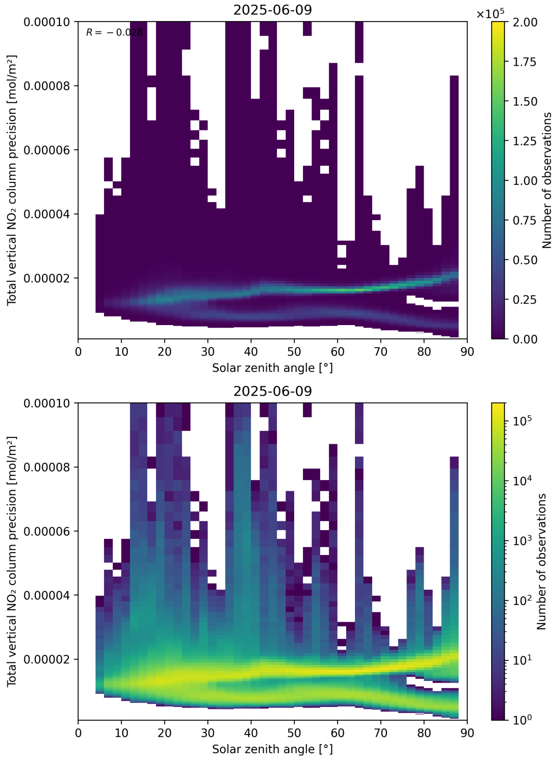
Figure 154: Scatter density plot of “Solar zenith angle” against “Total vertical NO 2 column precision” for 2025-06-08 to 2025-06-10.
