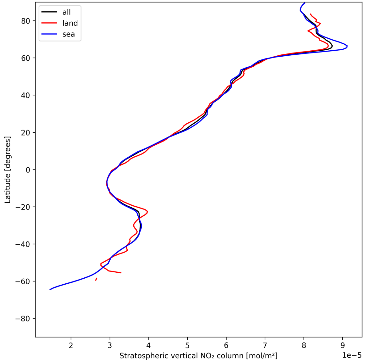
Figure 19: Zonal average of “Stratospheric vertical NO 2 column” for 2025-06-08 to 2025-06-10.
