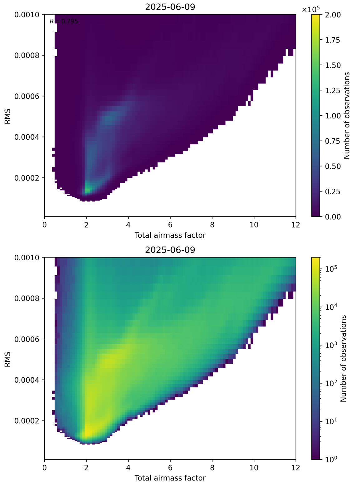
Figure 69: Scatter density plot of “Total airmass factor” against “RMS” for 2025-06-08 to 2025-06-10.
