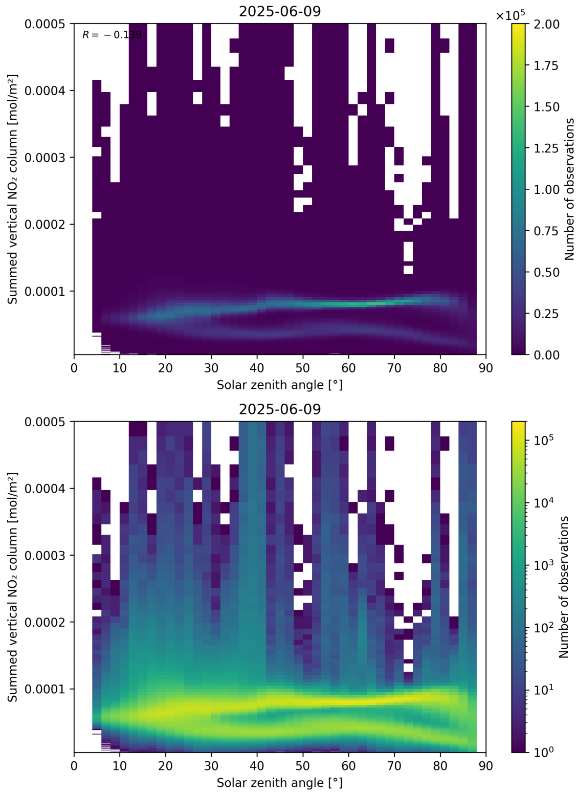
Figure 151: Scatter density plot of “Solar zenith angle” against “Summed vertical NO 2 column” for 2025-06-08 to 2025-06-10.
