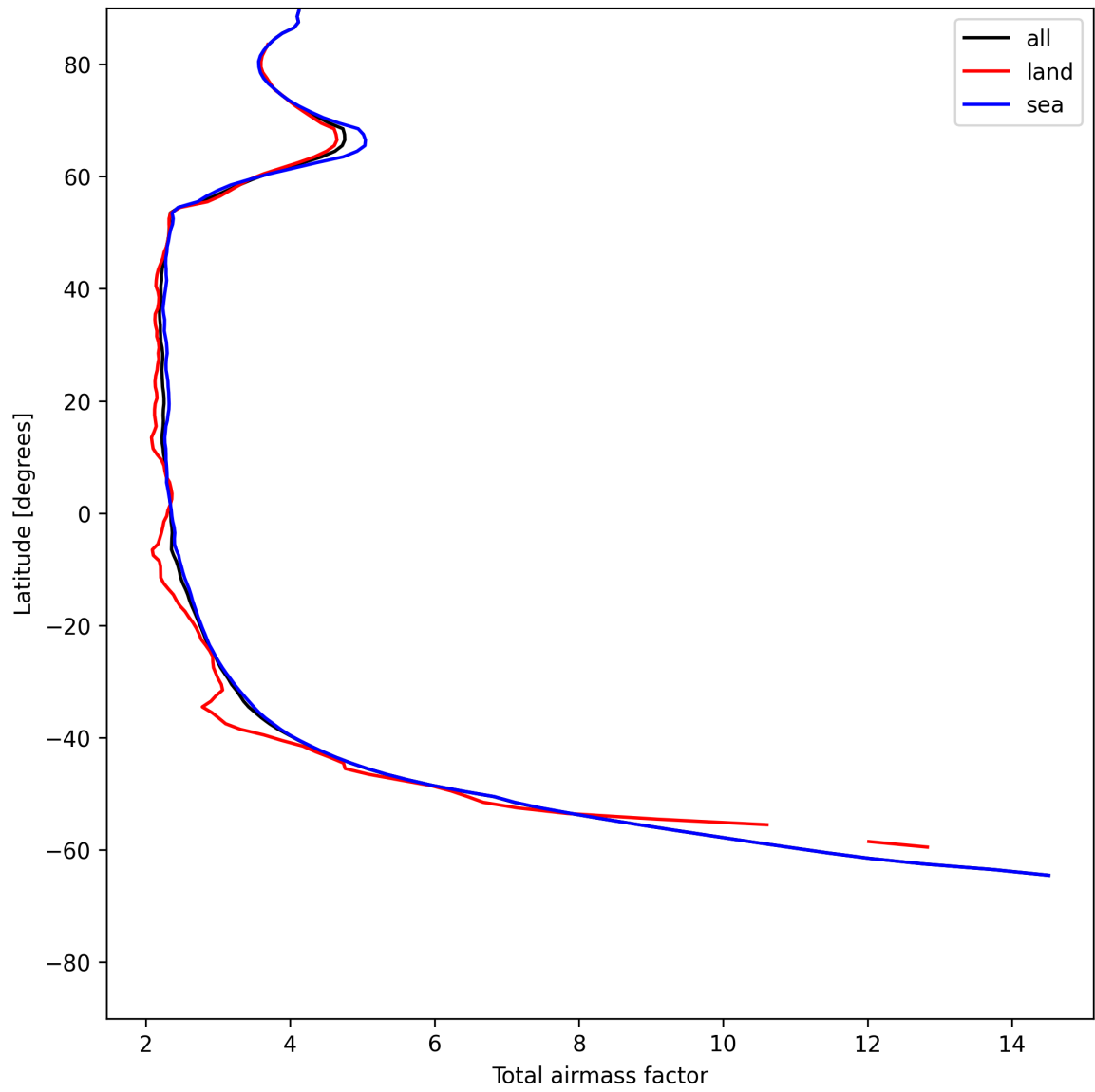
Figure 15: Zonal average of “Total airmass factor” for 2025-06-08 to 2025-06-10.
