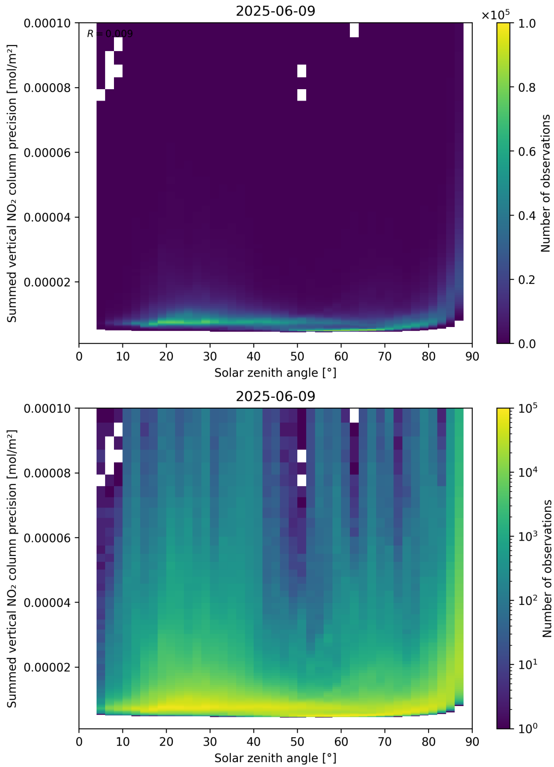
Figure 152: Scatter density plot of “Solar zenith angle” against “Summed vertical NO 2 column precision” for 2025-06-08 to 2025-06-10.
