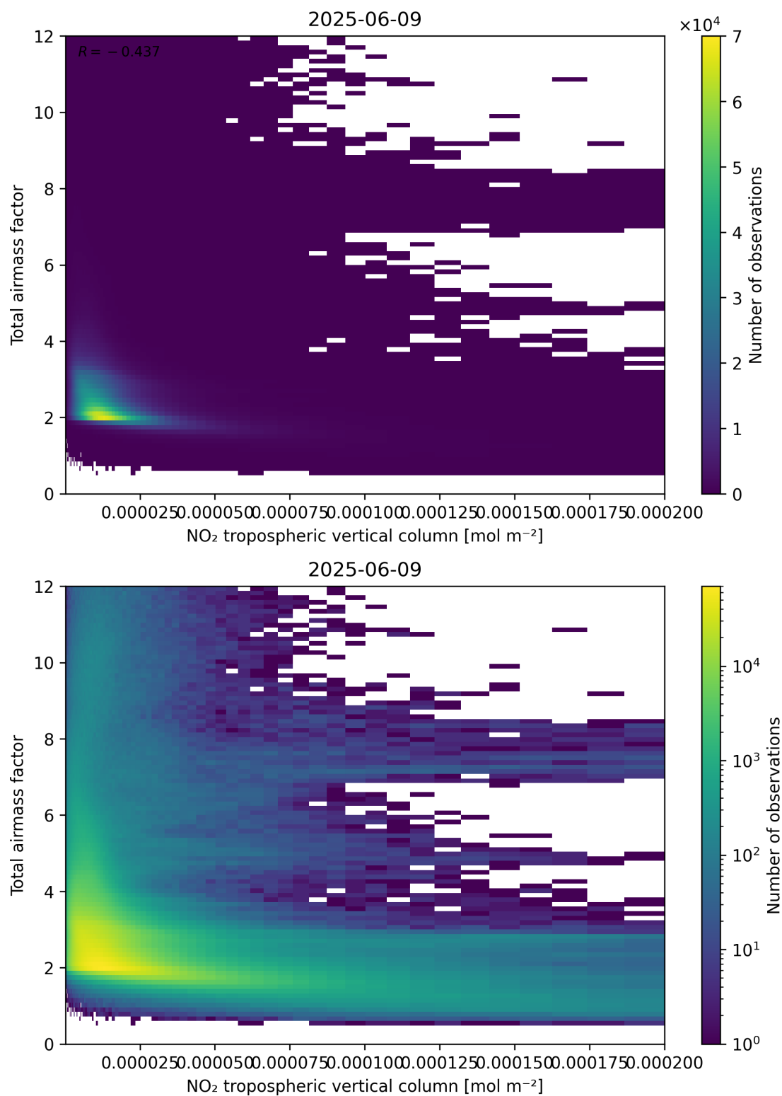
Figure 122: Scatter density plot of “NO 2 tropospheric vertical column” against “Total air mass factor” for 2025-06-08 to 2025-06-10.
