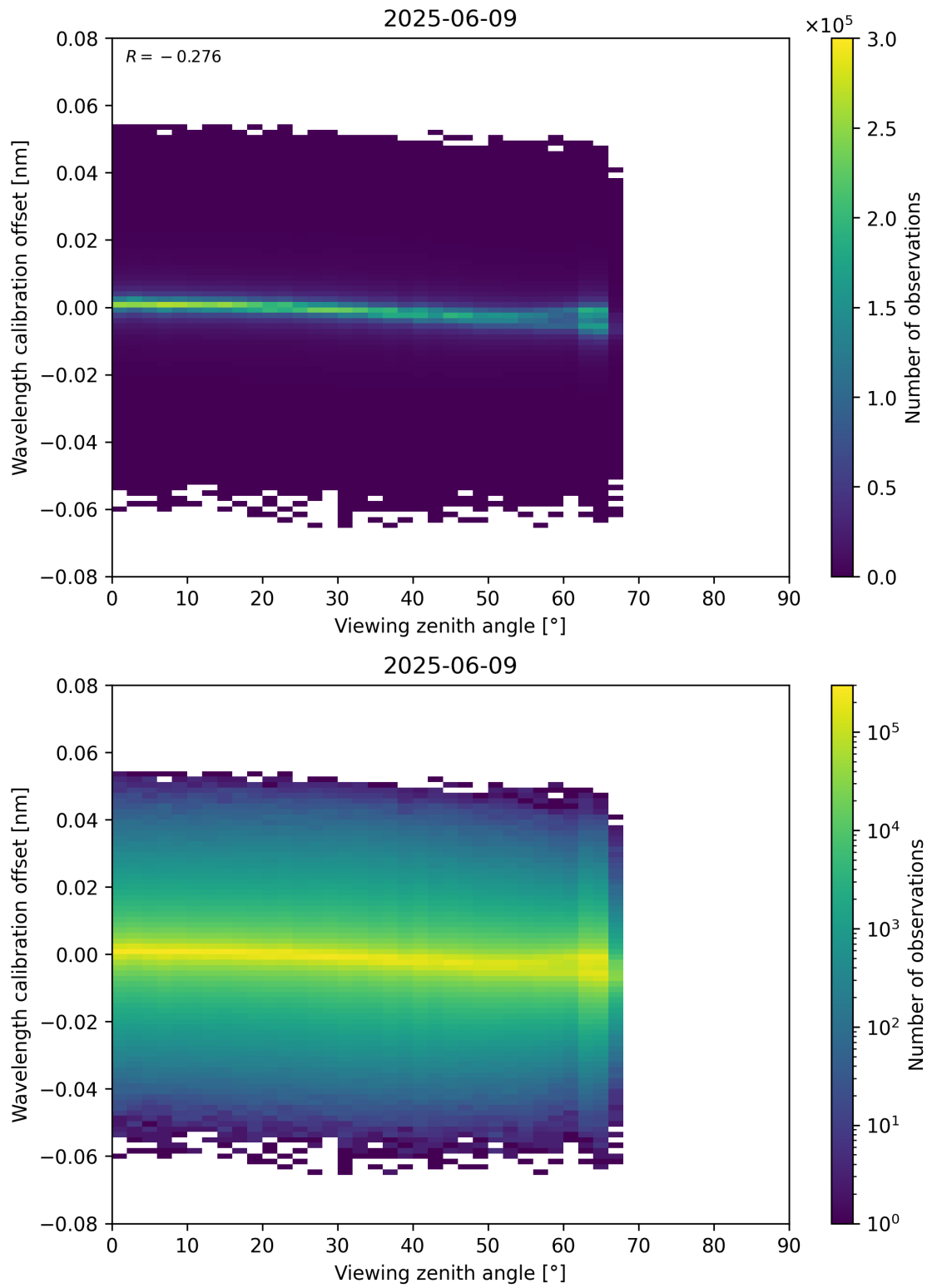
Figure 173: Scatter density plot of “Viewing zenith angle” against “Wavelength calibration offset” for 2025-06-08 to 2025-06-10.
