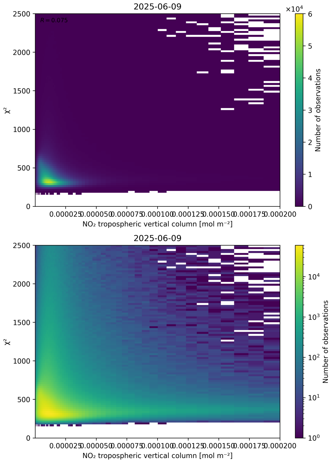
Figure 124: Scatter density plot of “NO 2 tropospheric vertical column” against “ \chi^2 ” for 2025-06-08 to 2025-06-10.
