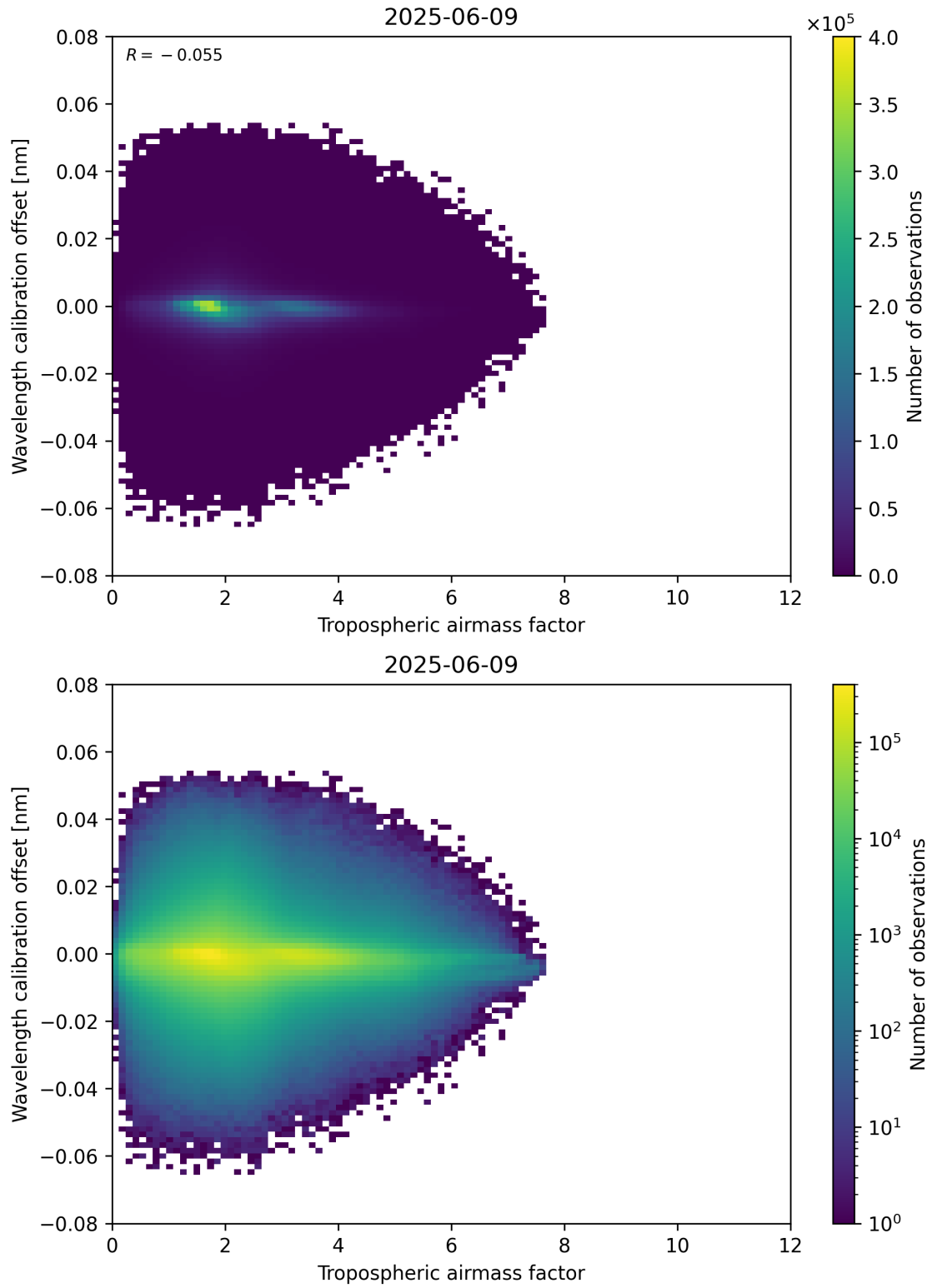
Figure 80: Scatter density plot of “Tropospheric airmass factor” against “Wavelength calibration offset” for 2025-06-08 to 2025-06-10.
