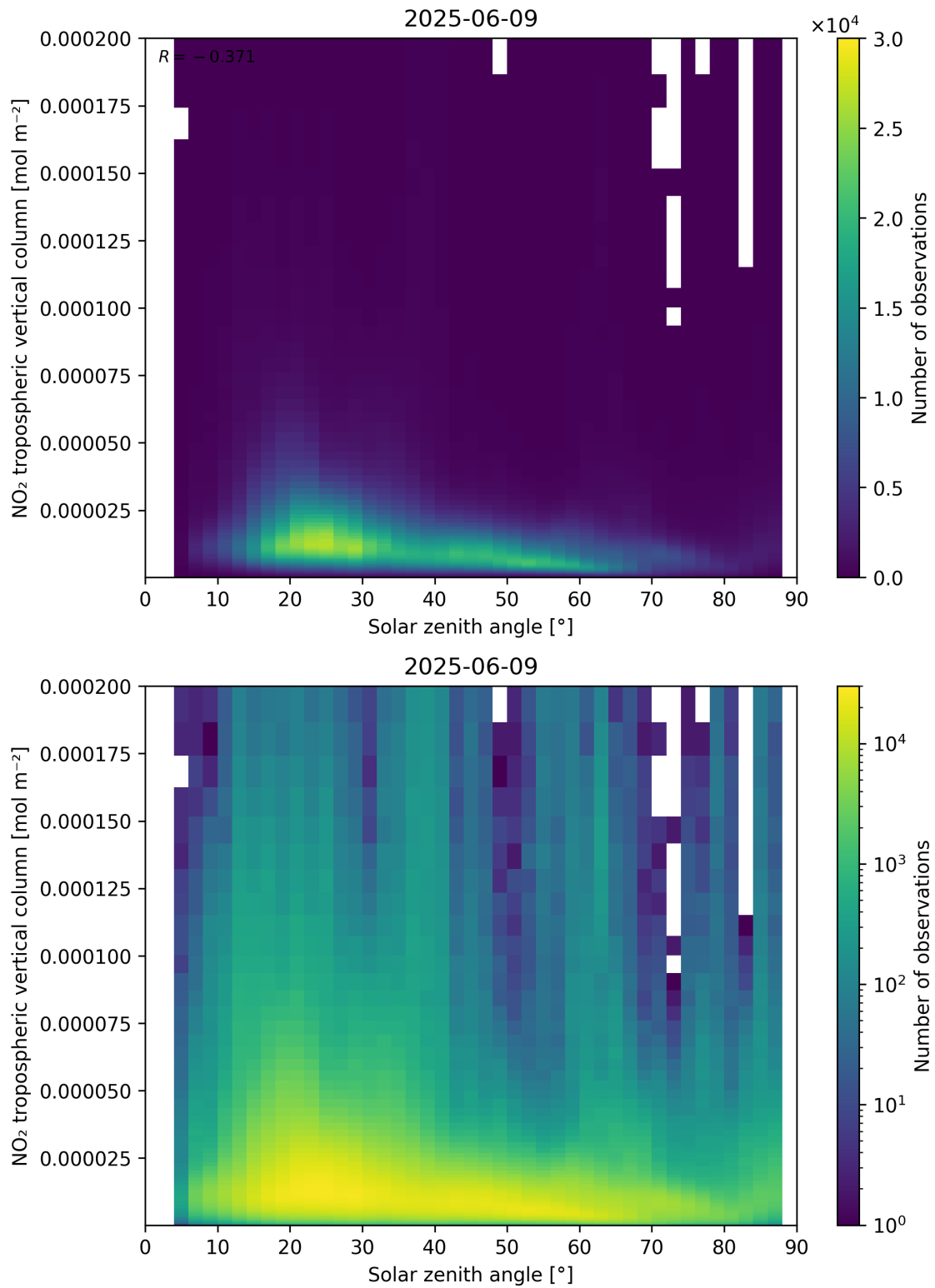
Figure 155: Scatter density plot of “Solar zenith angle” against “NO 2 tropospheric vertical column” for 2025-06-08 to 2025-06-10.
