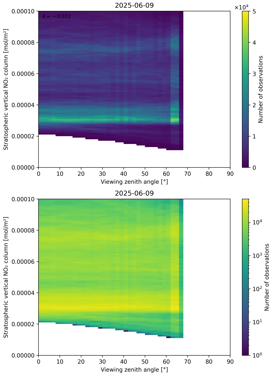
Figure 164: Scatter density plot of “Viewing zenith angle” against “Stratospheric vertical NO 2 column” for 2025-06-08 to 2025-06-10.
