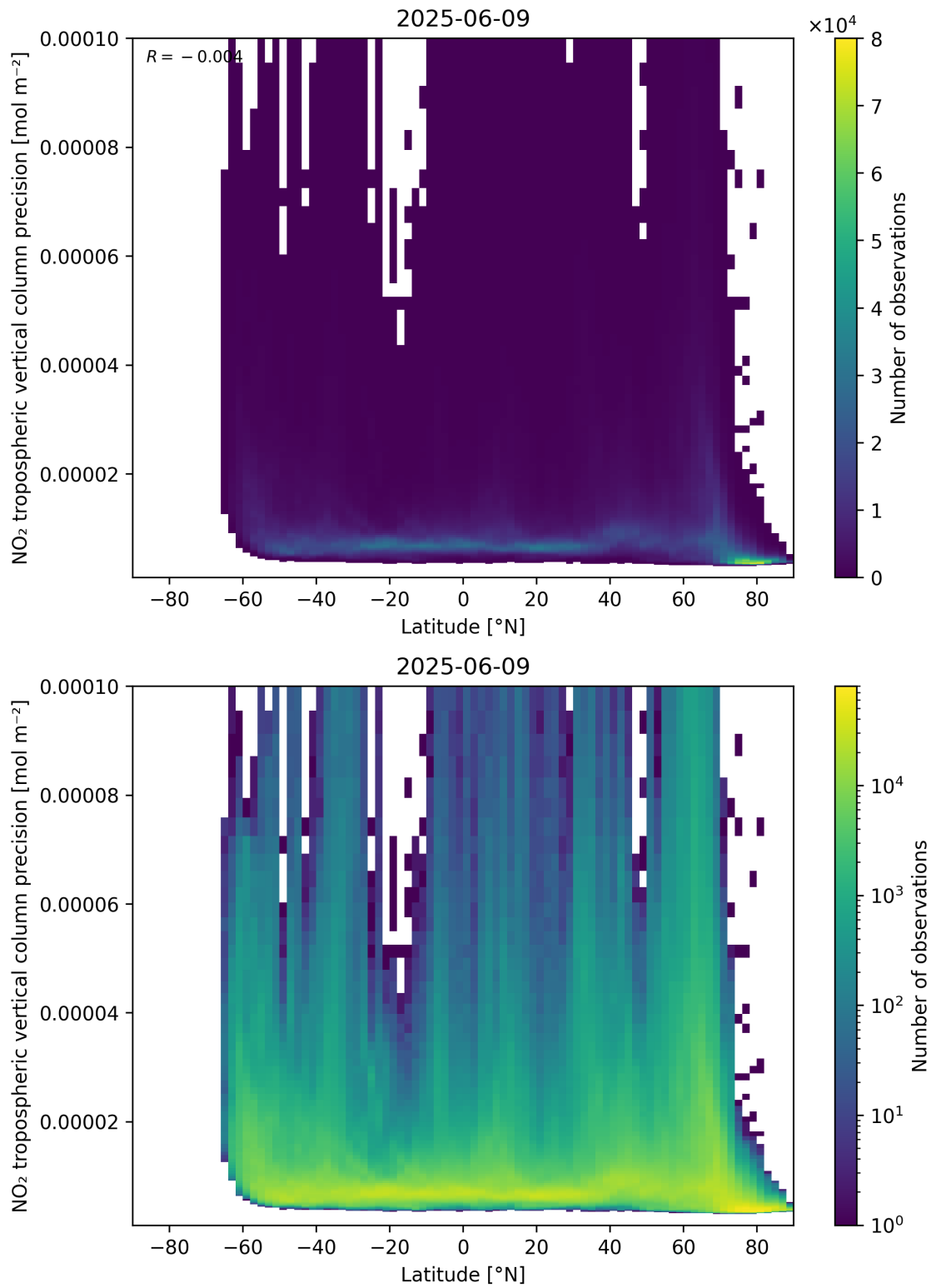
Figure 93: Scatter density plot of “Latitude” against “NO 2 tropospheric vertical column precision” for 2025-06-08 to 2025-06-10.
