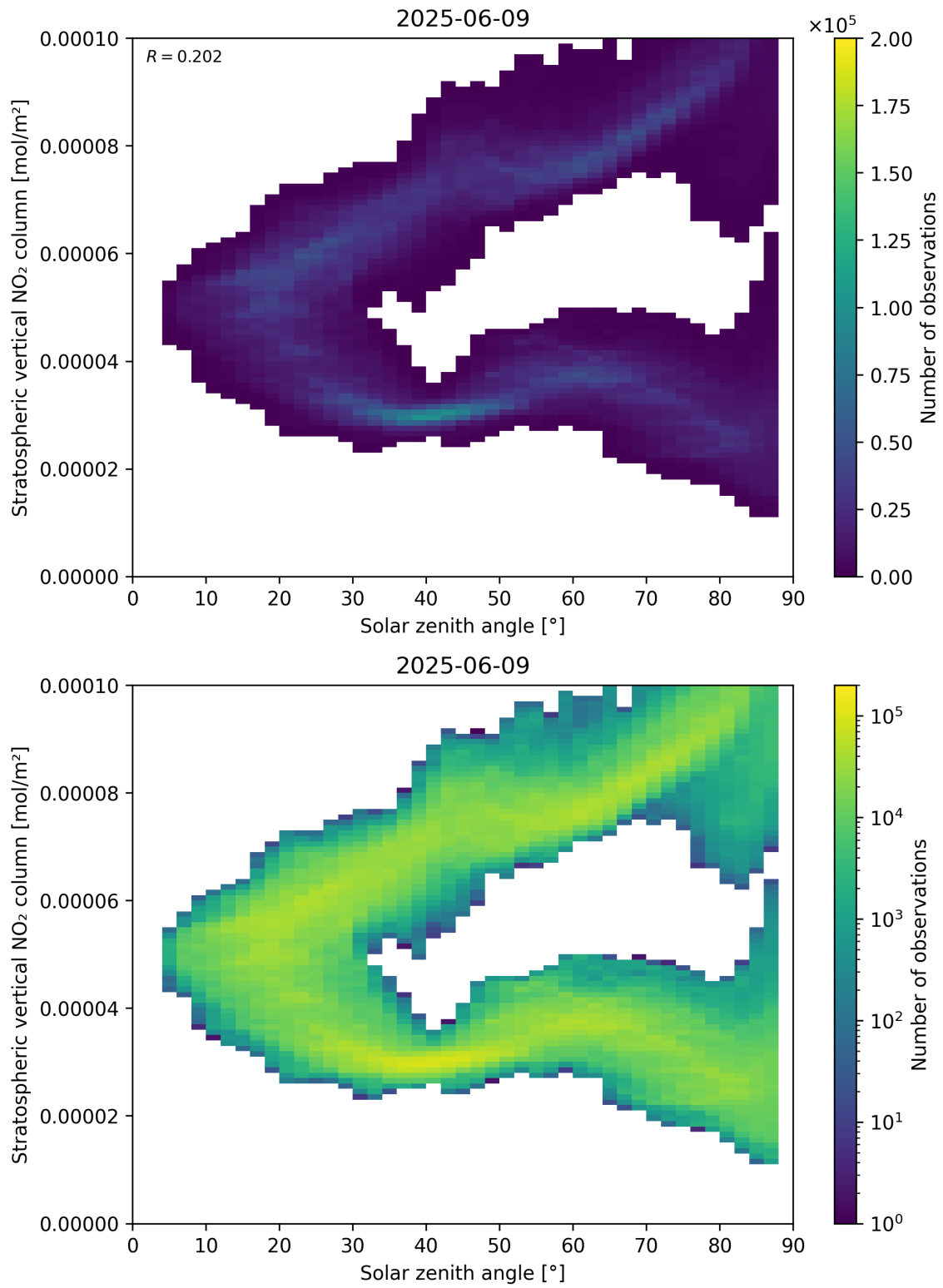
Figure 150: Scatter density plot of “Solar zenith angle” against “Stratospheric vertical NO 2 column” for 2025-06-08 to 2025-06-10.
