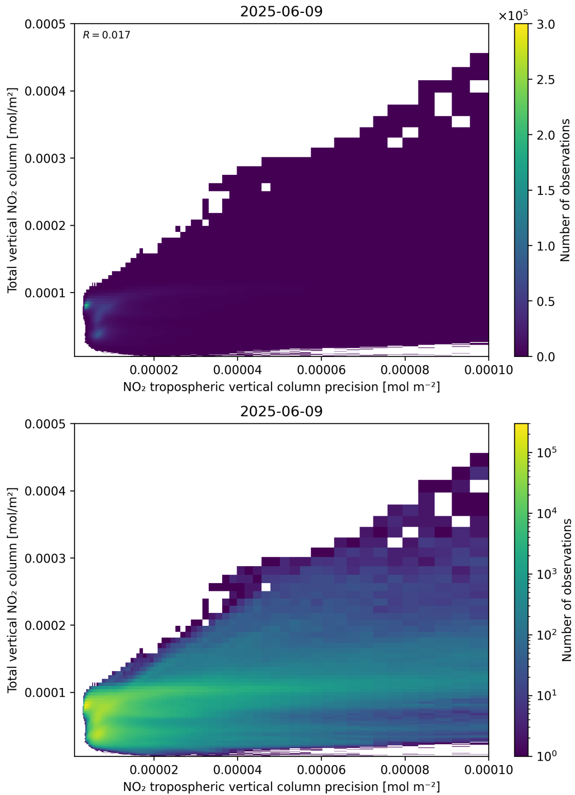
Figure 138: Scatter density plot of “NO 2 tropospheric vertical column precision” against “Total vertical NO 2 column” for 2025-06-08 to 2025-06-10.
