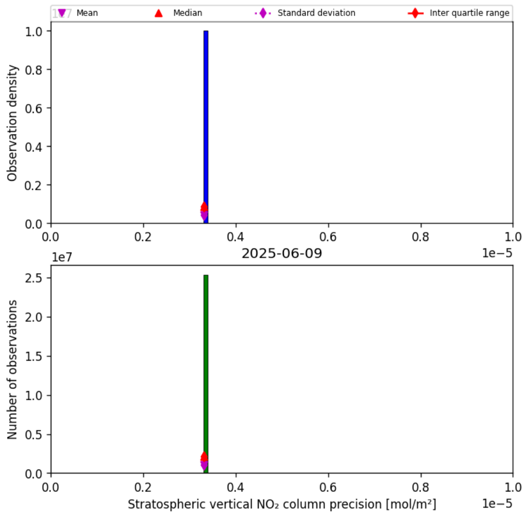
Figure 37: Histogram of “Stratospheric vertical NO 2 column precision” for 2025-06-08 to 2025-06-10
