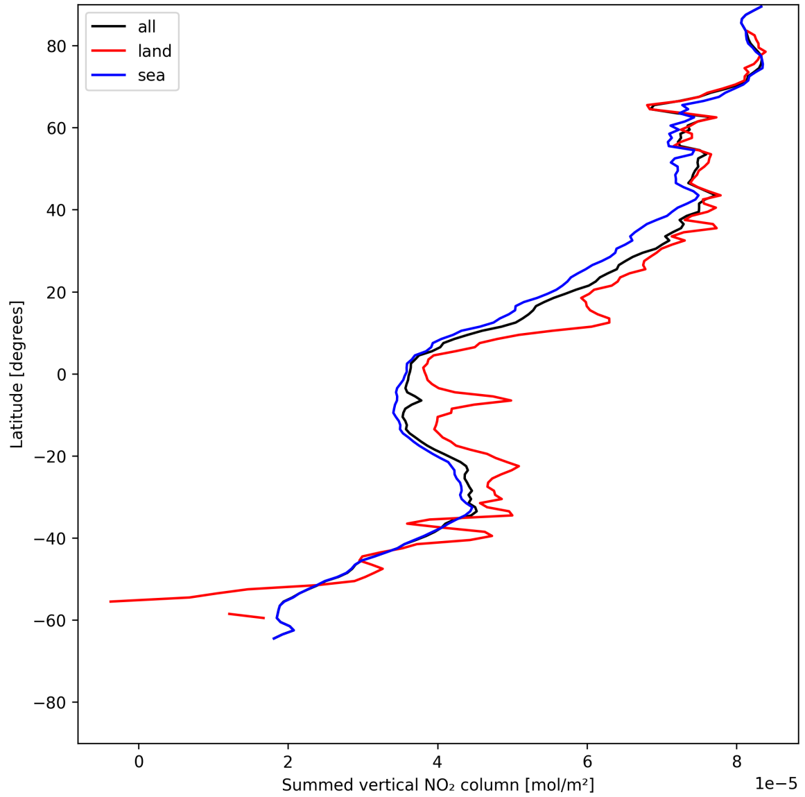
Figure 23: Zonal average of “Summed vertical NO 2 column” for 2025-06-08 to 2025-06-10.
