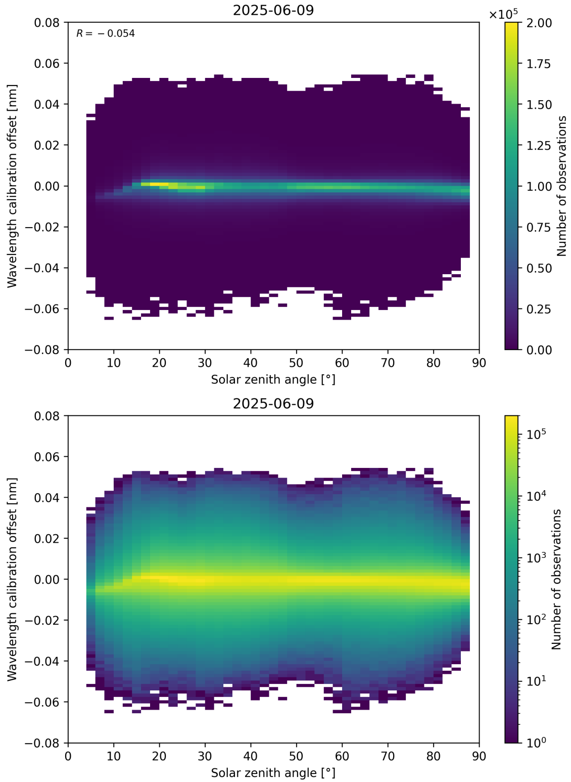
Figure 158: Scatter density plot of “Solar zenith angle” against “Wavelength calibration offset” for 2025-06-08 to 2025-06-10.
