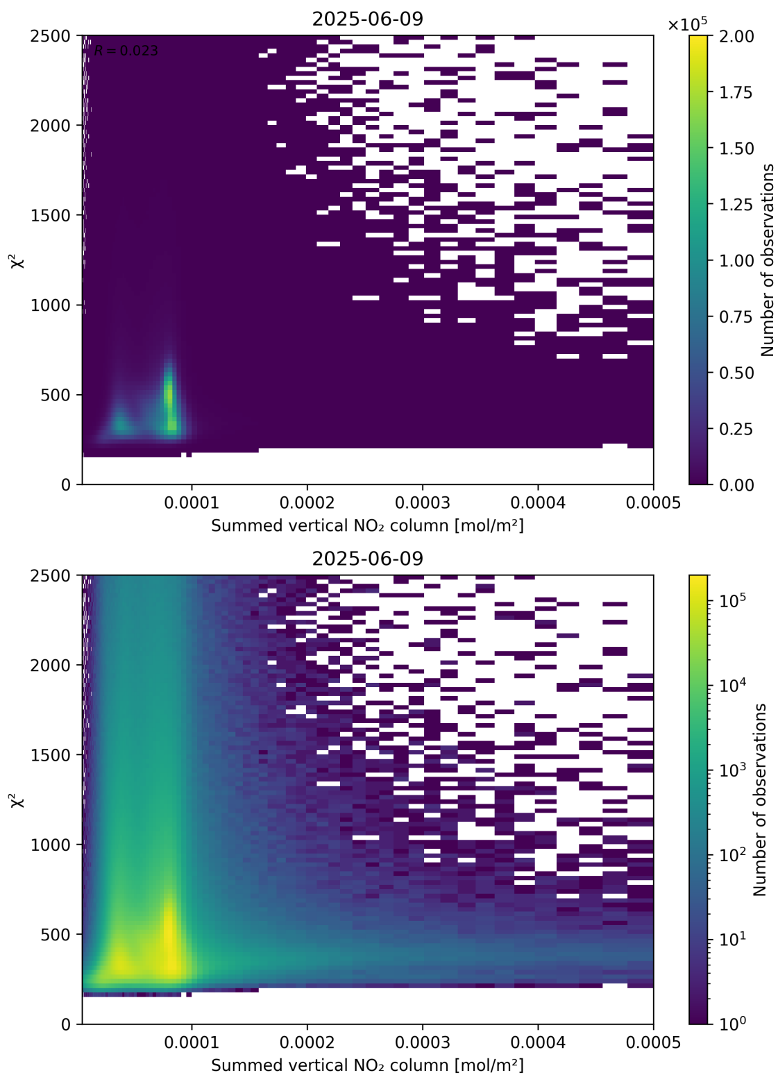
Figure 104: Scatter density plot of “Summed vertical NO 2 column” against “ \chi^2 ” for 2025-06-08 to 2025-06-10.
