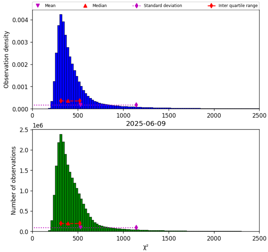
Figure 42: Histogram of “ \chi^2 ” for 2025-06-08 to 2025-06-10
