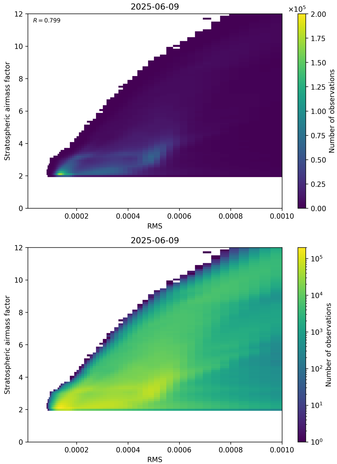
Figure 144: Scatter density plot of “RMS” against “Stratospheric airmass factor” for 2025-06-08 to 2025-06-10.
