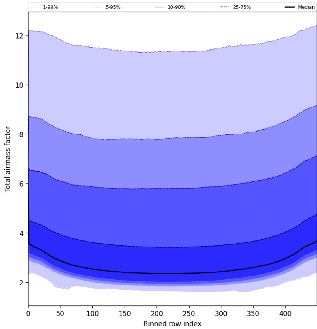
Figure 49: Along track statistics of “Total airmass factor” for 2025-06-08 to 2025-06-10
