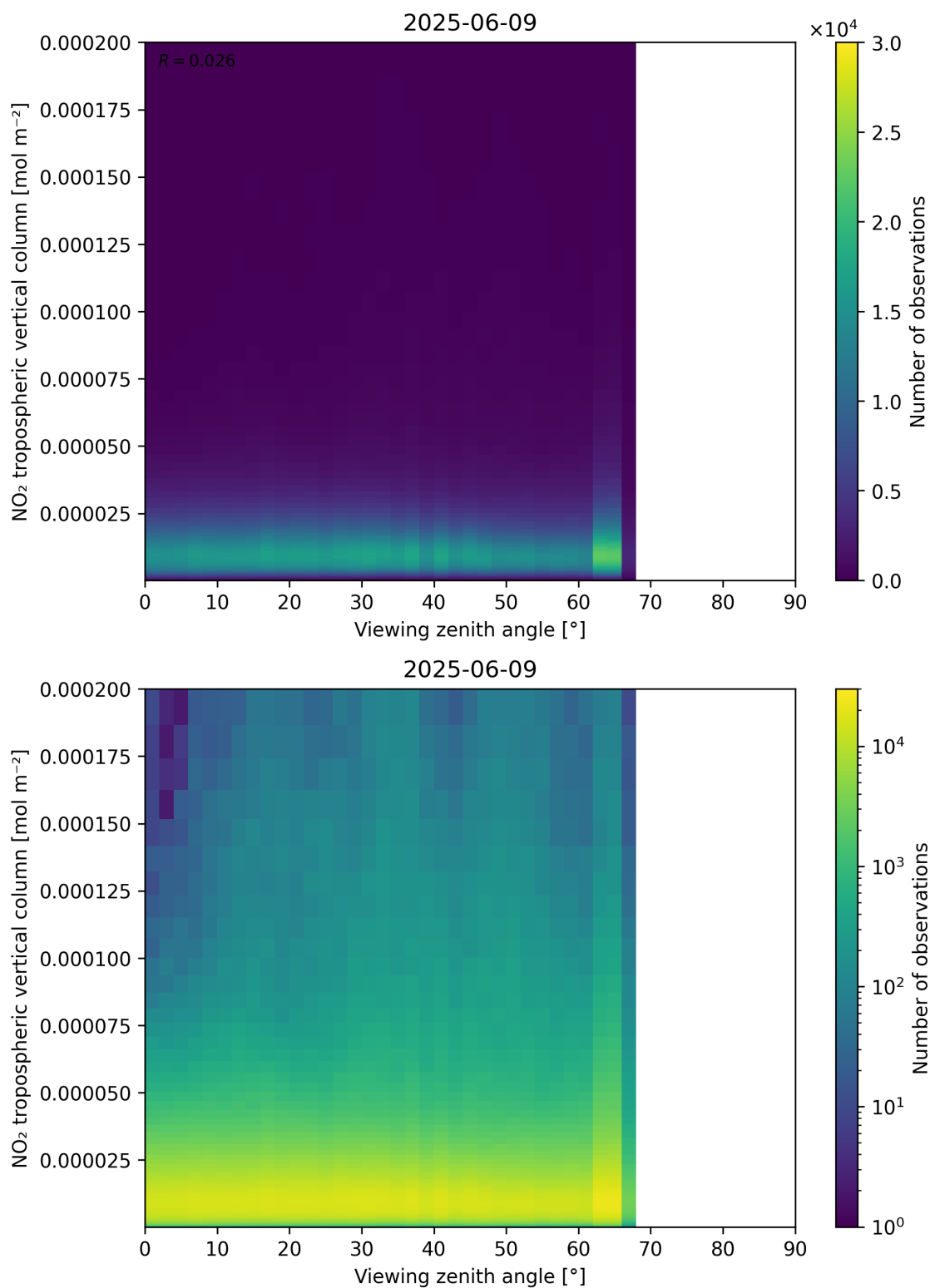
Figure 169: Scatter density plot of “Viewing zenith angle” against “NO 2 tropospheric vertical column” for 2025-06-08 to 2025-06-10.
