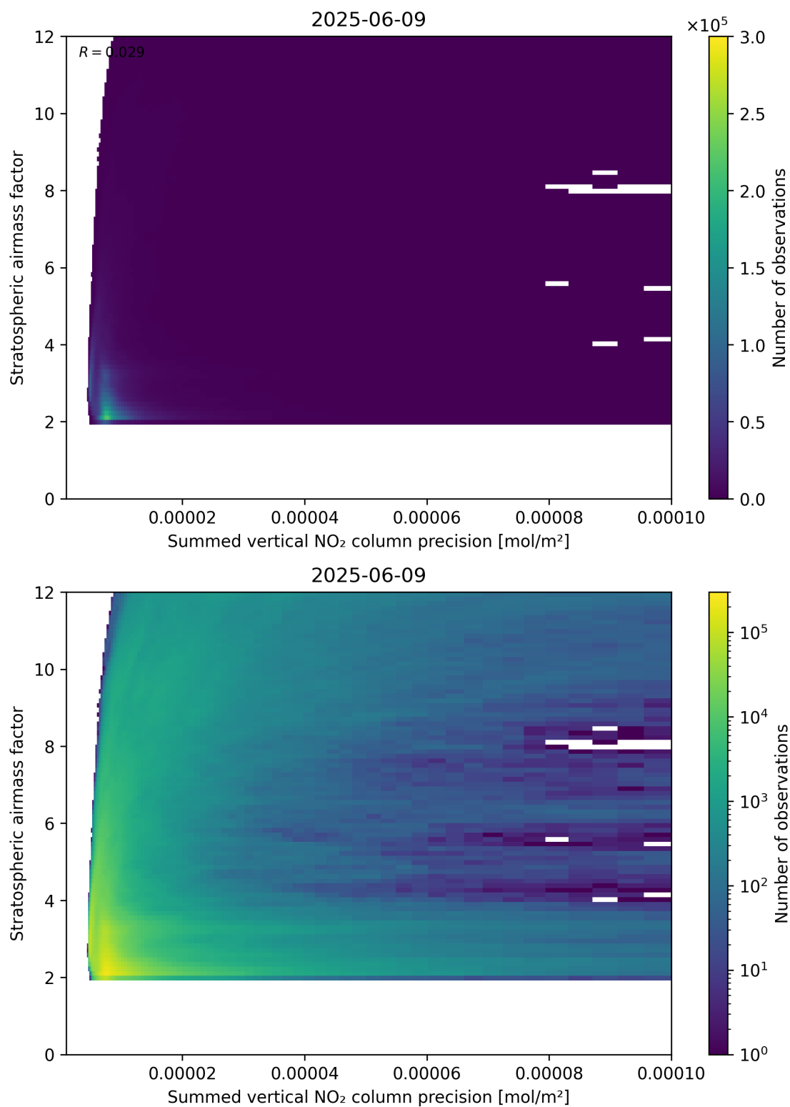
Figure 106: Scatter density plot of “Summed vertical NO 2 column precision” against “Stratospheric airmass factor” for 2025-06-08 to 2025-06-10.
