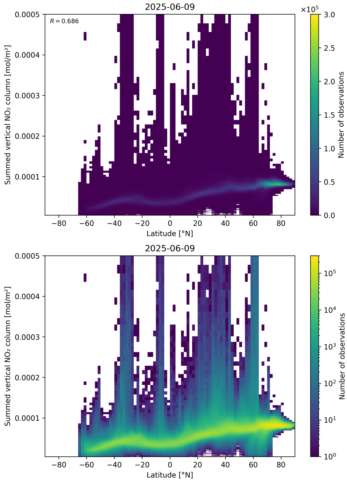
Figure 88: Scatter density plot of “Latitude” against “Summed vertical NO 2 column” for 2025-06-08 to 2025-06-10.
