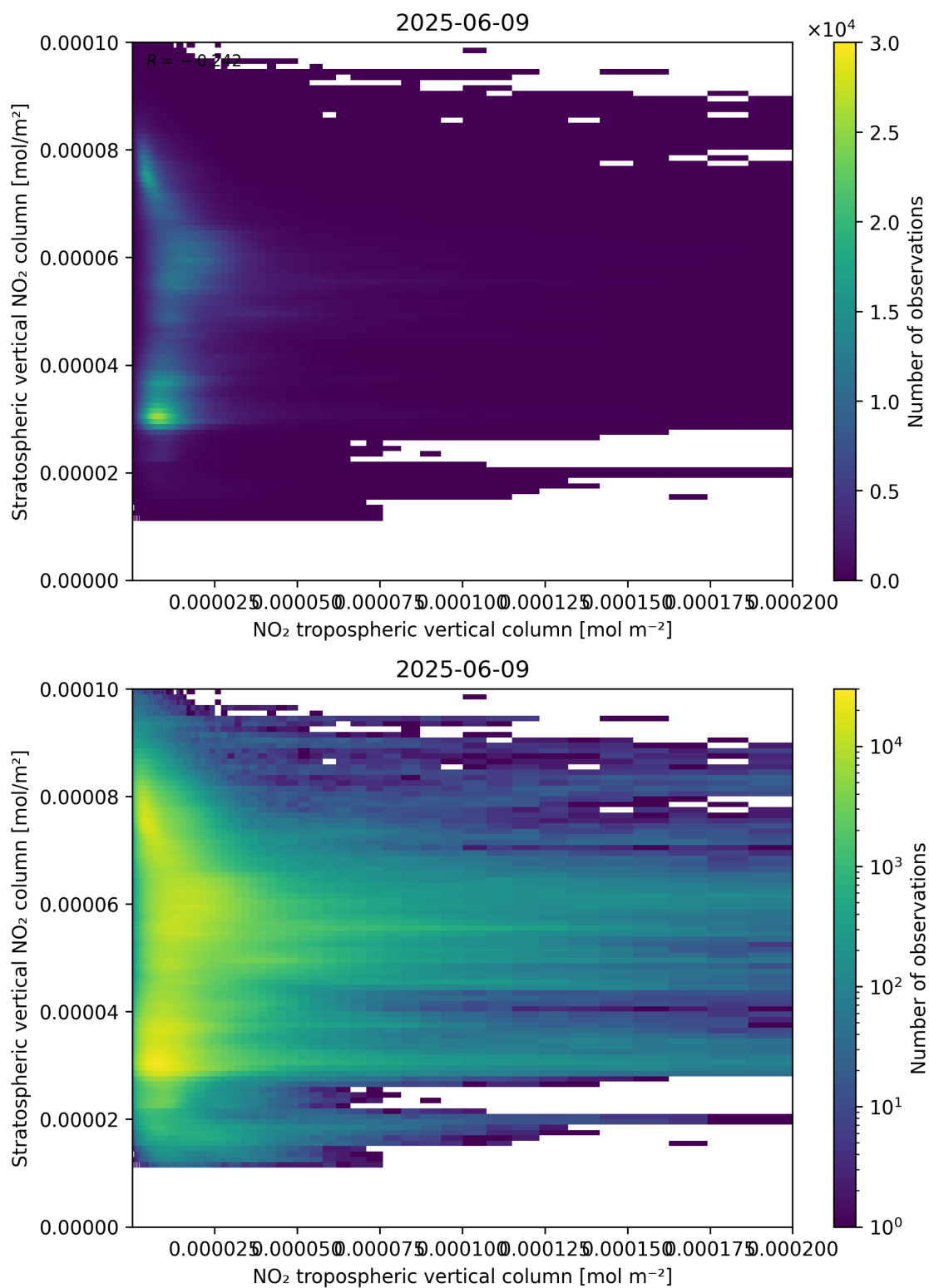
Figure 125: Scatter density plot of “NO 2 tropospheric vertical column” against “Stratospheric vertical NO 2 column” for 2025-06-08 to 2025-06-10.
