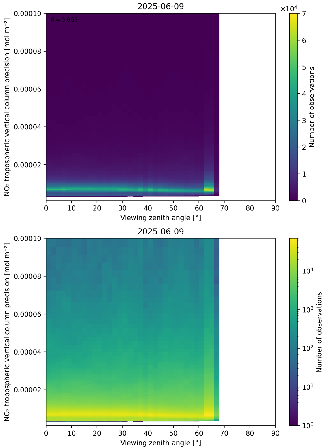
Figure 170: Scatter density plot of “Viewing zenith angle” against “NO 2 tropospheric vertical column precision” for 2025-06-08 to 2025-06-10.
