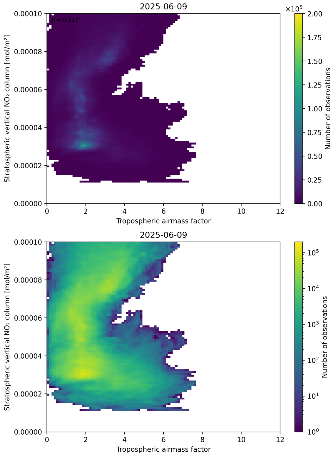
Figure 74: Scatter density plot of “Tropospheric airmass factor” against “Stratospheric vertical NO 2 column” for 2025-06-08 to 2025-06-10.
