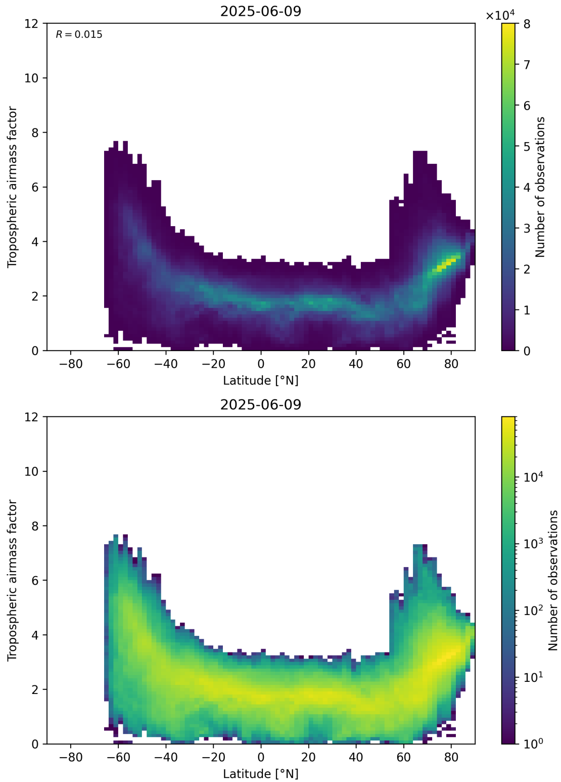
Figure 85: Scatter density plot of “Latitude” against “Tropospheric airmass factor” for 2025-06-08 to 2025-06-10.
