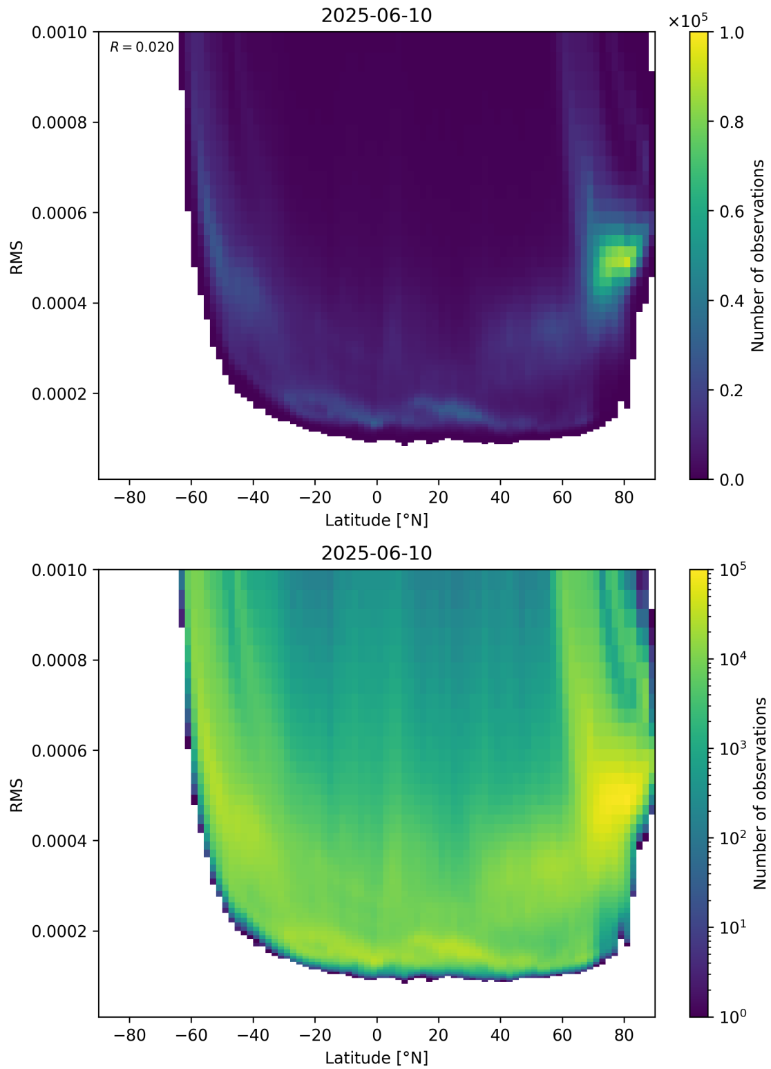
Figure 94: Scatter density plot of “Latitude” against “RMS” for 2025-06-09 to 2025-06-11.
