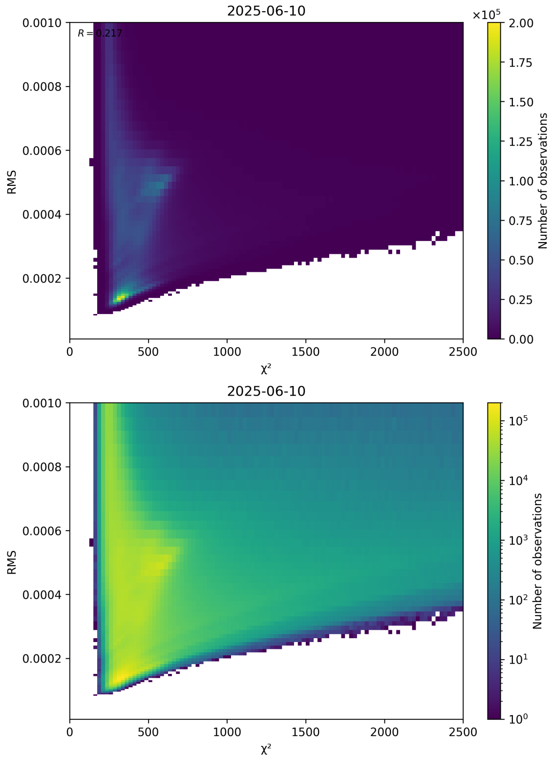
Figure 82: Scatter density plot of “ \chi^2 ” against “RMS” for 2025-06-09 to 2025-06-11.
