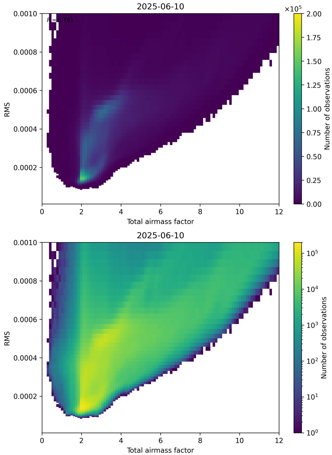
Figure 69: Scatter density plot of “Total airmass factor” against “RMS” for 2025-06-09 to 2025-06-11.
