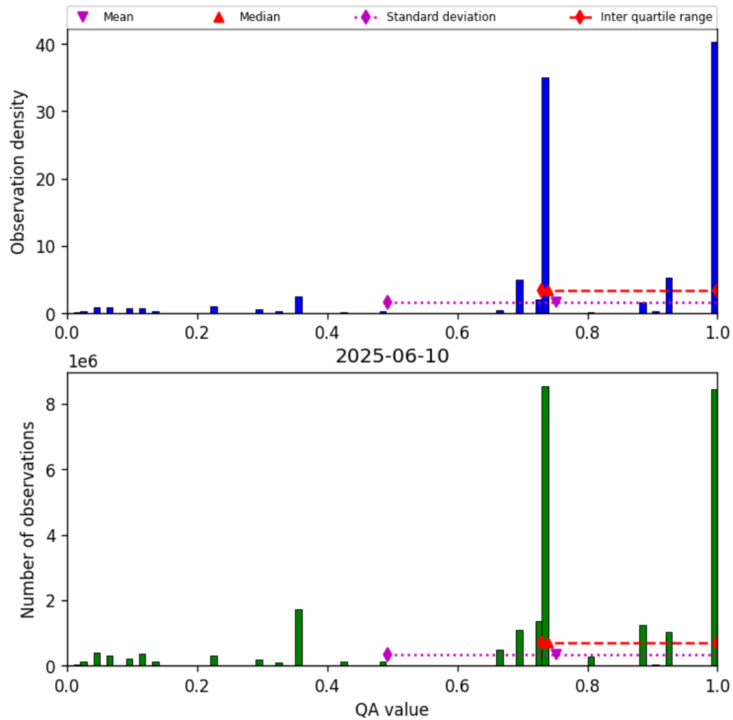
Figure 28: Histogram of “QA value” for 2025-06-09 to 2025-06-11
