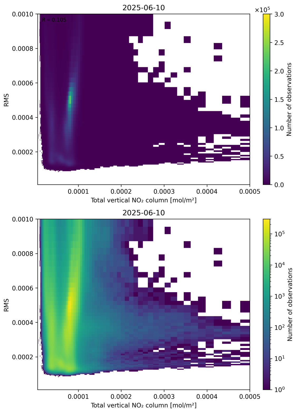
Figure 120: Scatter density plot of “Total vertical NO 2 column” against “RMS” for 2025-06-09 to 2025-06-11.
