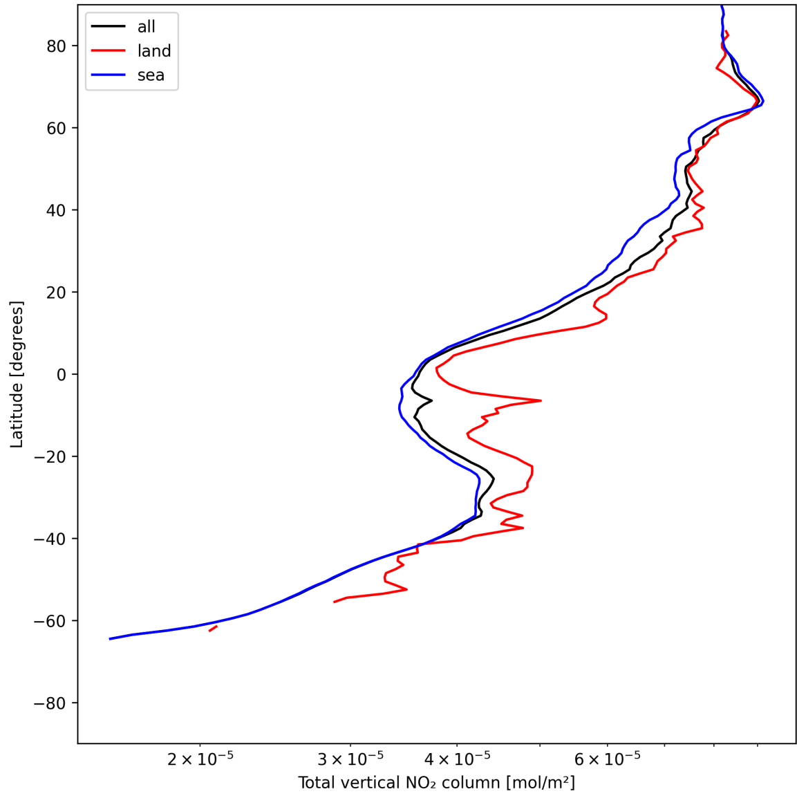
Figure 21: Zonal average of “Total vertical NO 2 column” for 2025-06-09 to 2025-06-11.
