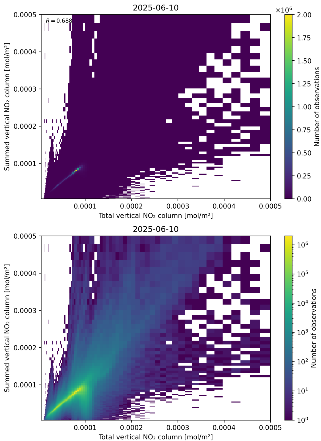
Figure 112: Scatter density plot of “Total vertical NO 2 column” against “Summed vertical NO 2 column” for 2025-06-09 to 2025-06-11.
