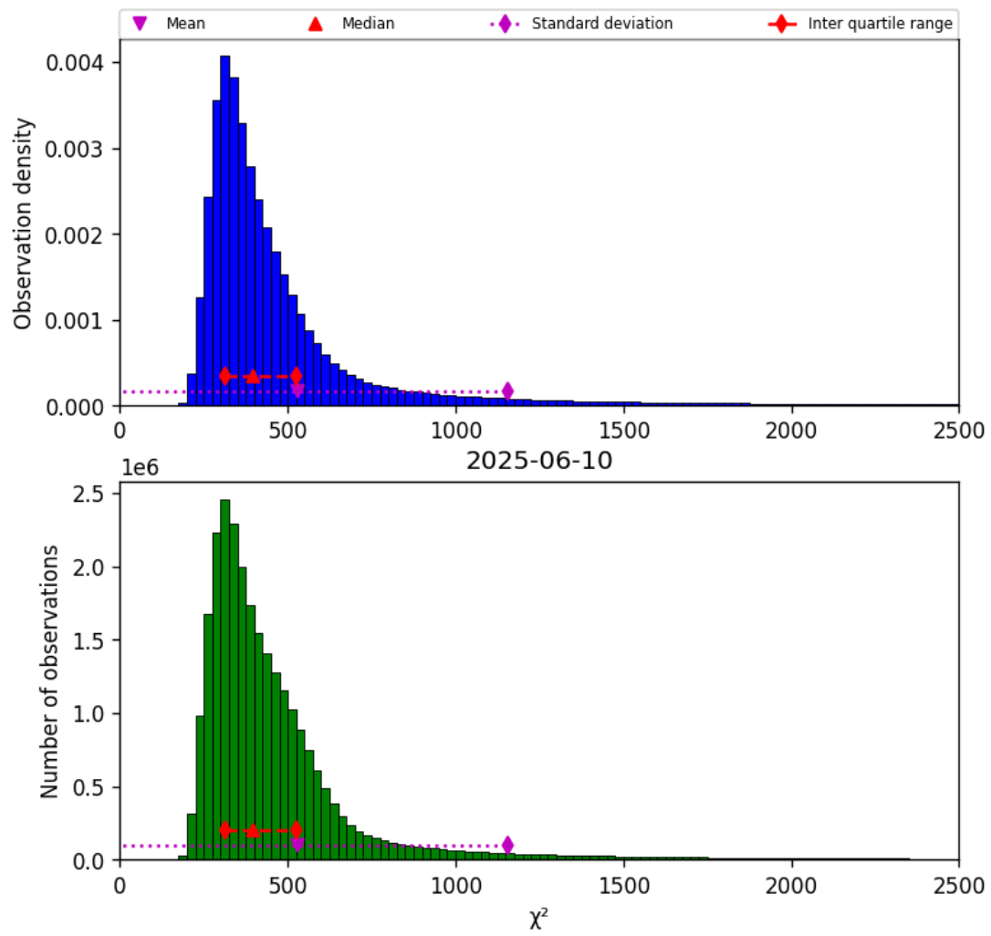
Figure 42: Histogram of “ \chi^2 ” for 2025-06-09 to 2025-06-11
