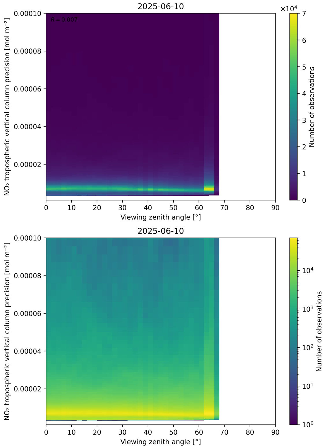
Figure 170: Scatter density plot of “Viewing zenith angle” against “NO 2 tropospheric vertical column precision” for 2025-06-09 to 2025-06-11.
