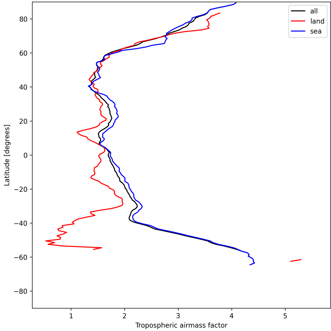
Figure 14: Zonal average of “Tropospheric airmass factor” for 2025-06-09 to 2025-06-11.
