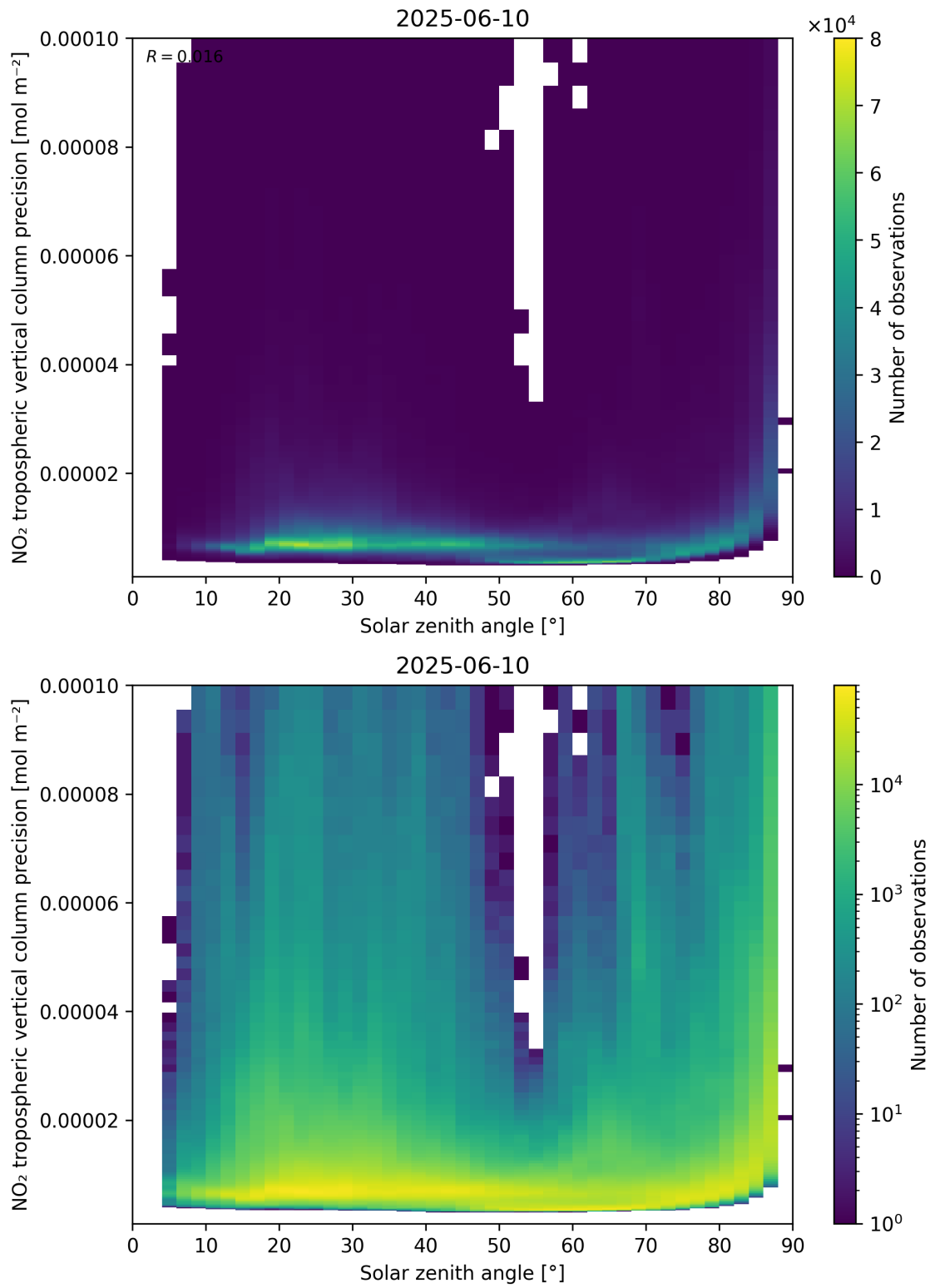
Figure 156: Scatter density plot of “Solar zenith angle” against “NO 2 tropospheric vertical column precision” for 2025-06-09 to 2025-06-11.
