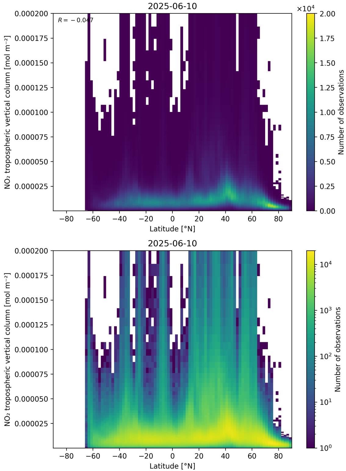
Figure 92: Scatter density plot of “Latitude” against “NO 2 tropospheric vertical column” for 2025-06-09 to 2025-06-11.
