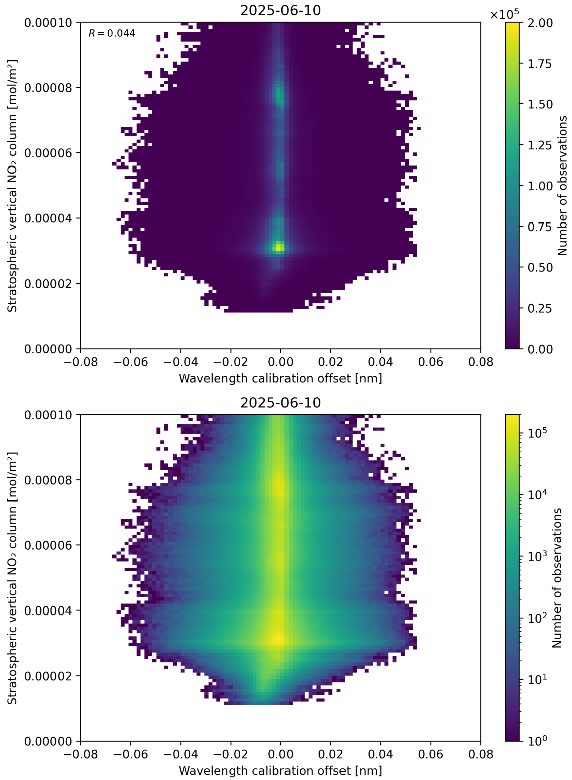
Figure 176: Scatter density plot of “Wavelength calibration offset” against “Stratospheric vertical NO 2 column” for 2025-06-09 to 2025-06-11.
