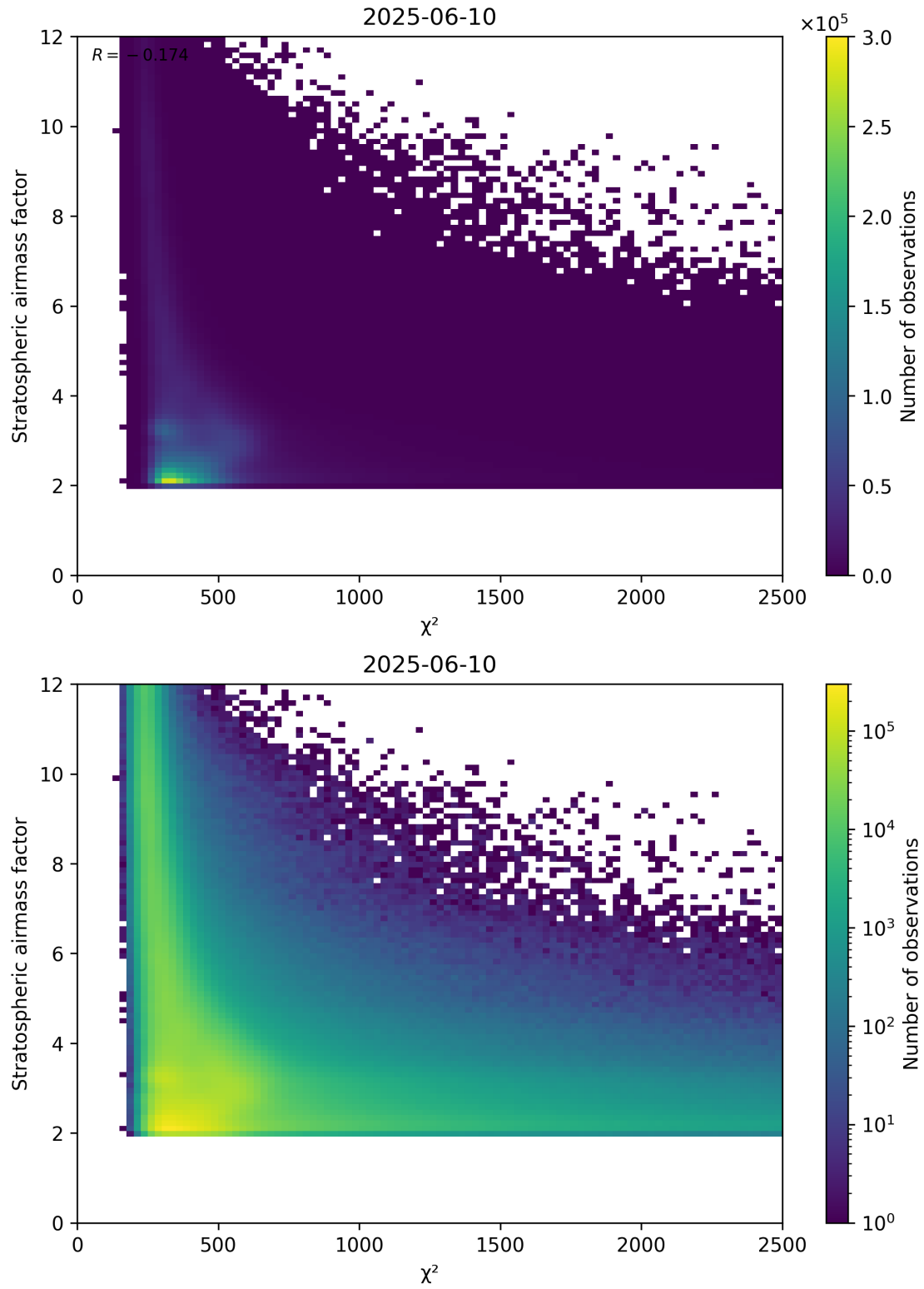
Figure 81: Scatter density plot of “ \chi^2 ” against “Stratospheric airmass factor” for 2025-06-09 to 2025-06-11.
