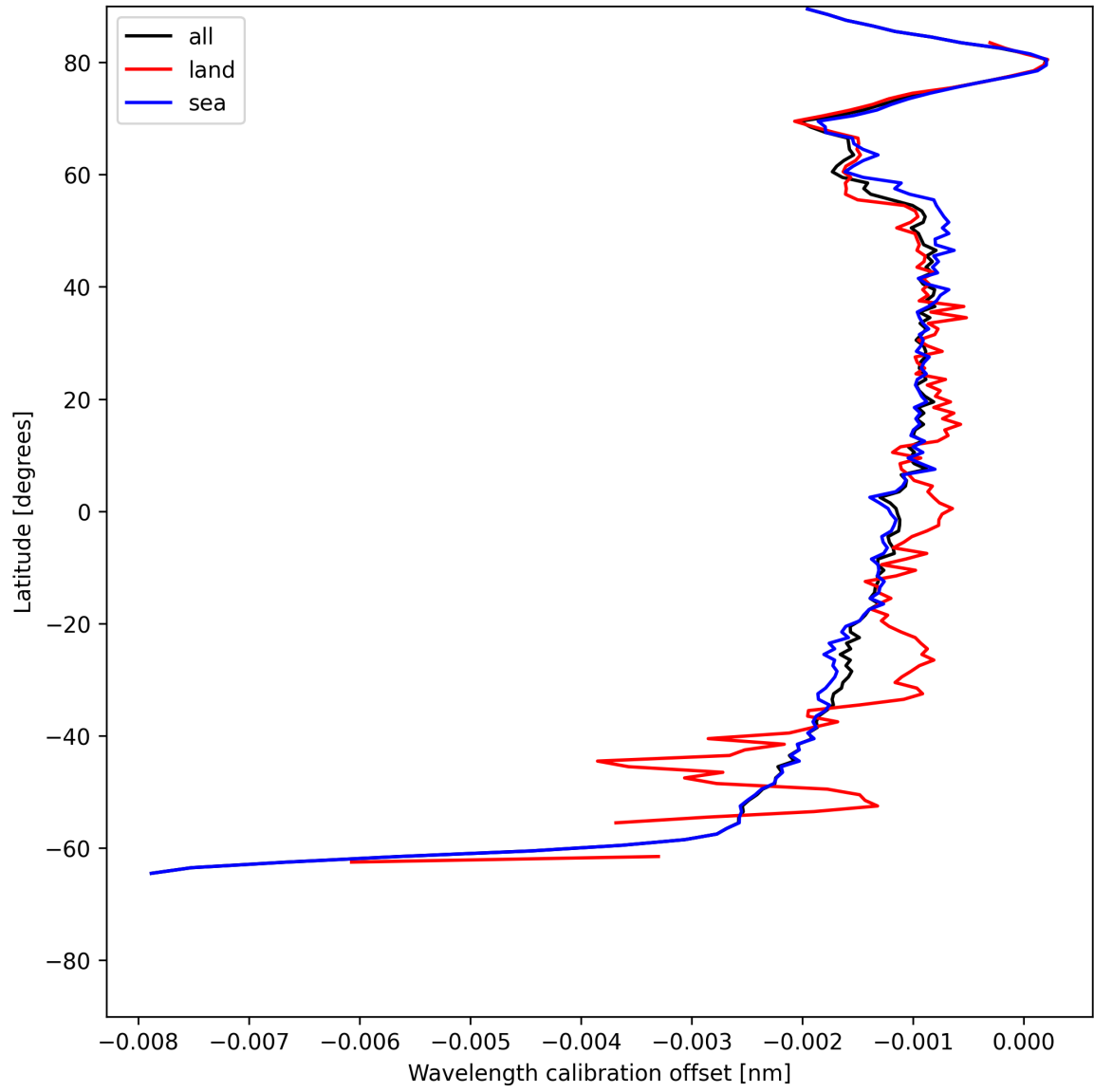
Figure 18: Zonal average of “Wavelength calibration offset” for 2025-06-09 to 2025-06-11.
