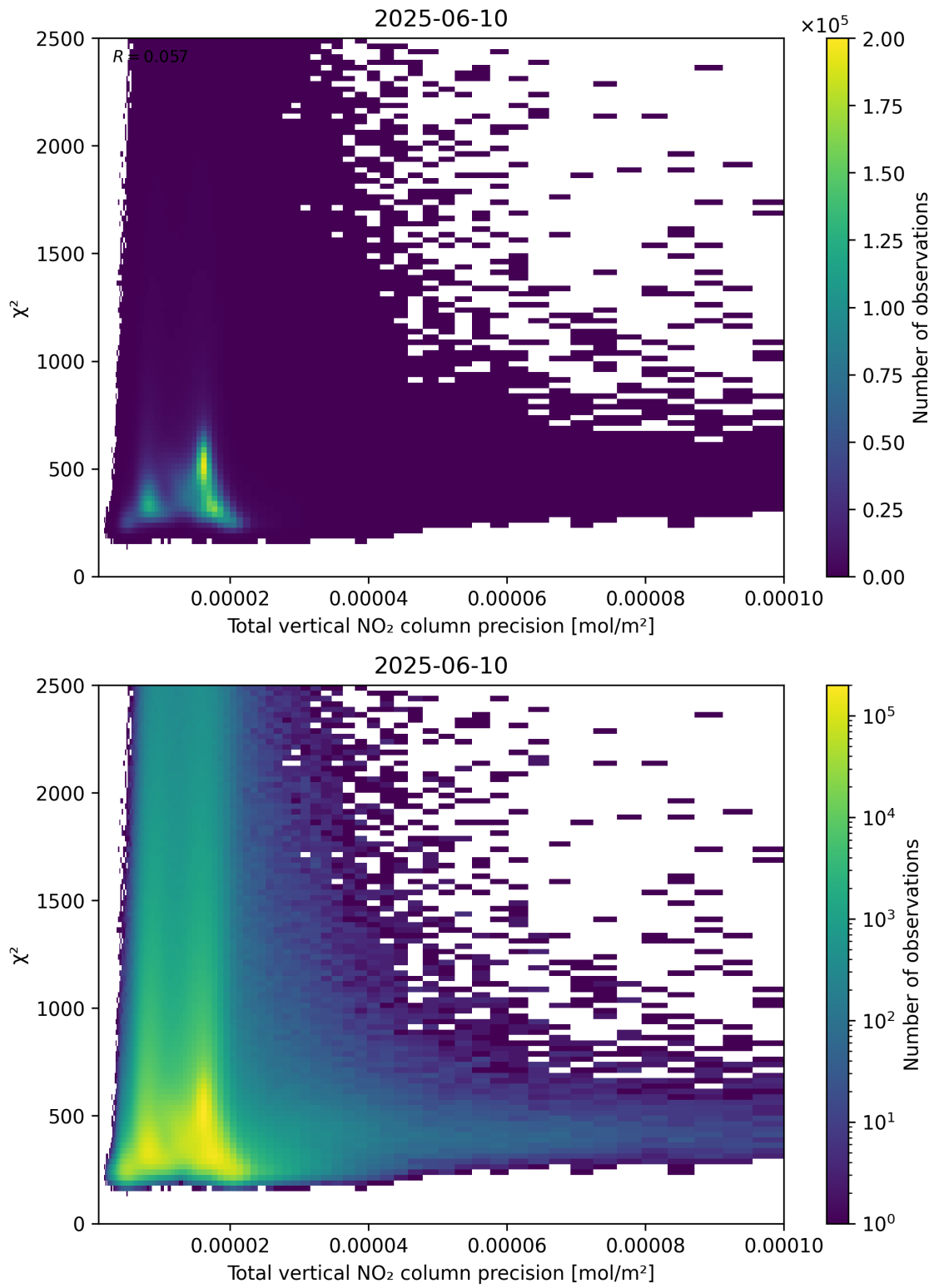
Figure 116: Scatter density plot of “Total vertical NO 2 column precision” against “ \chi^2 ” for 2025-06-09 to 2025-06-11.
