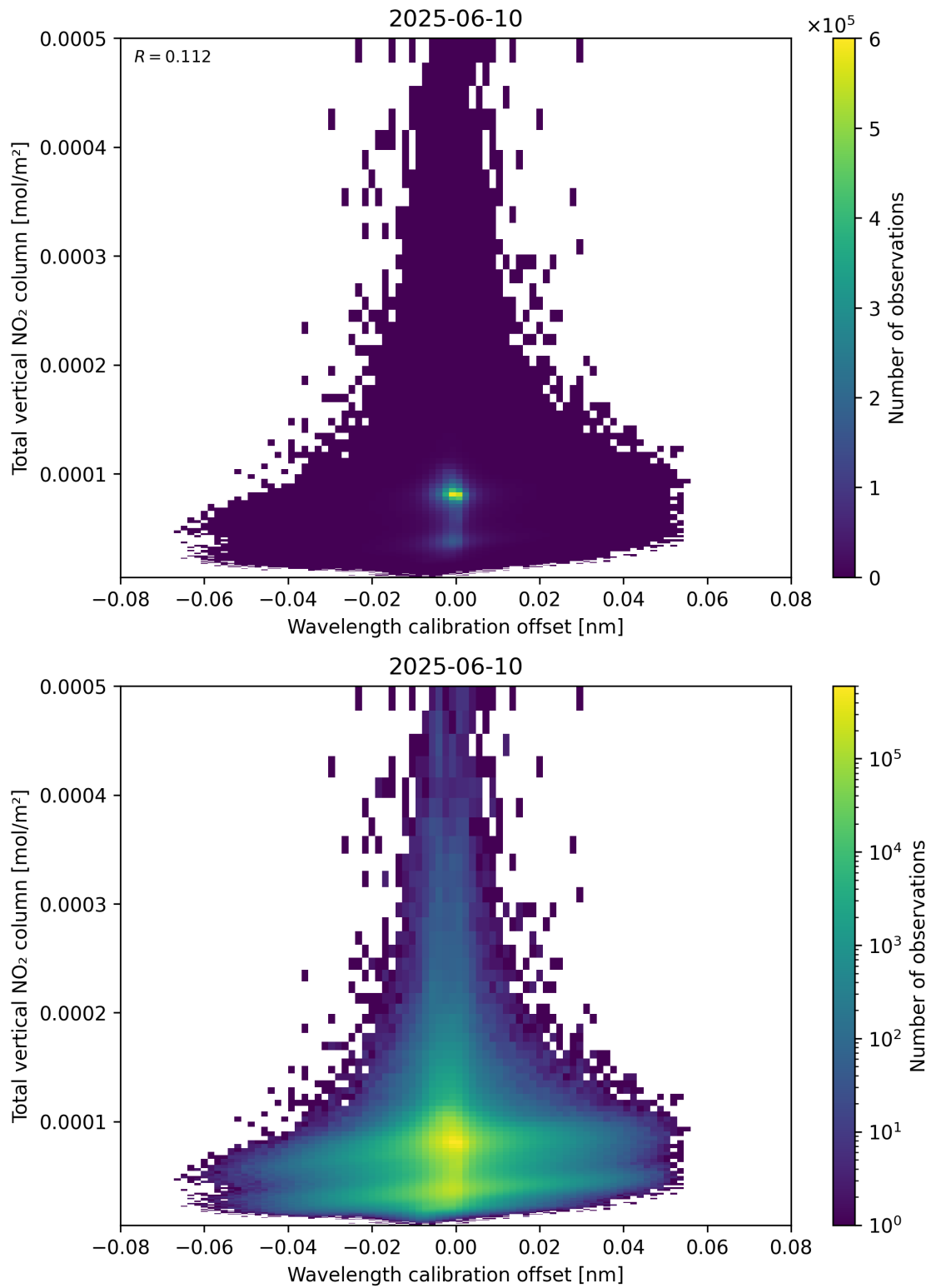
Figure 179: Scatter density plot of “Wavelength calibration offset” against “Total vertical NO 2 column” for 2025-06-09 to 2025-06-11.
