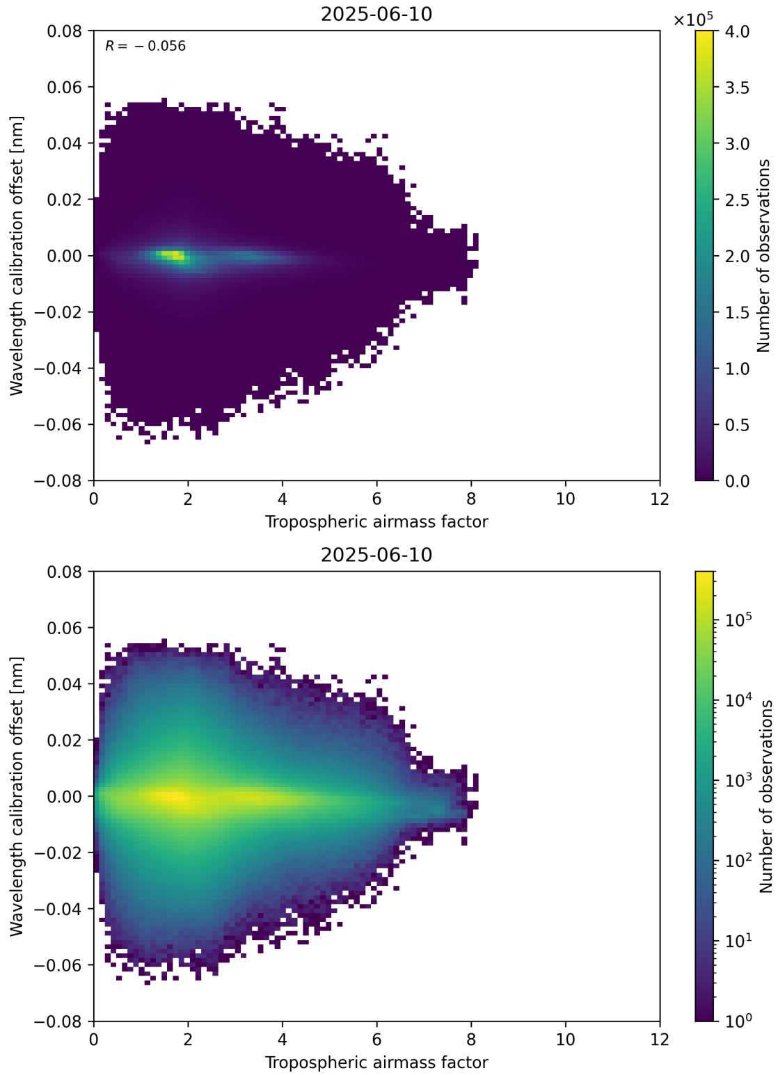
Figure 80: Scatter density plot of “Tropospheric airmass factor” against “Wavelength calibration offset” for 2025-06-09 to 2025-06-11.
