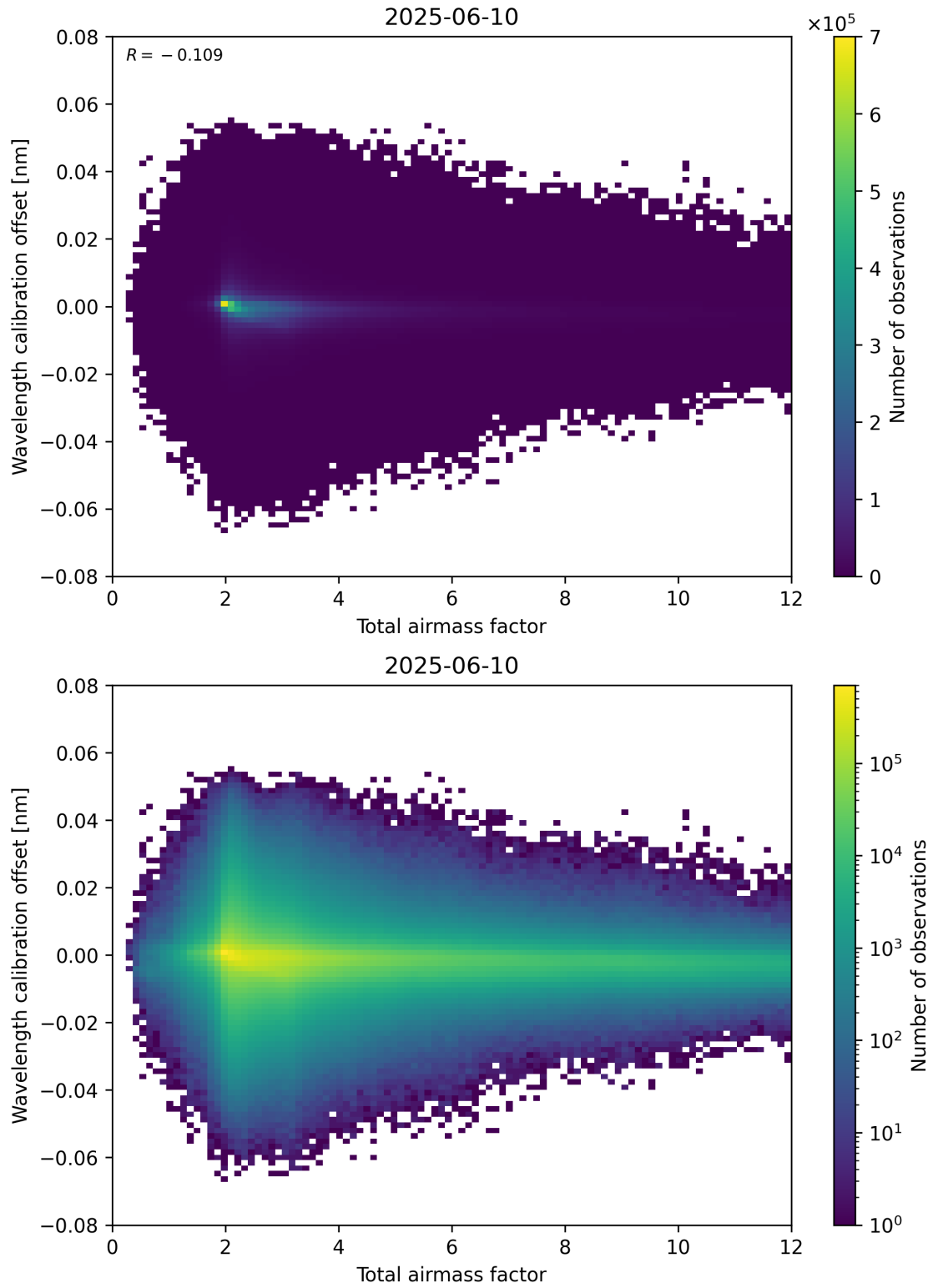
Figure 70: Scatter density plot of “Total airmass factor” against “Wavelength calibration offset” for 2025-06-09 to 2025-06-11.
