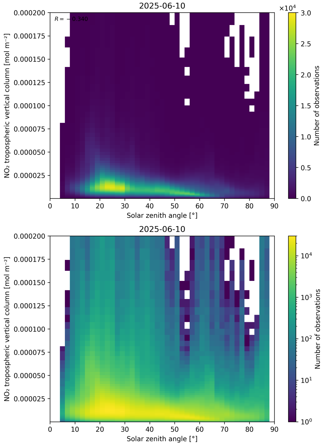
Figure 155: Scatter density plot of “Solar zenith angle” against “NO 2 tropospheric vertical column” for 2025-06-09 to 2025-06-11.
