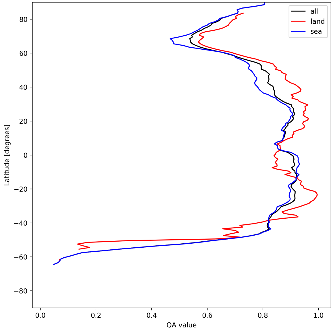
Figure 11: Zonal average of “QA value” for 2025-06-09 to 2025-06-11.
