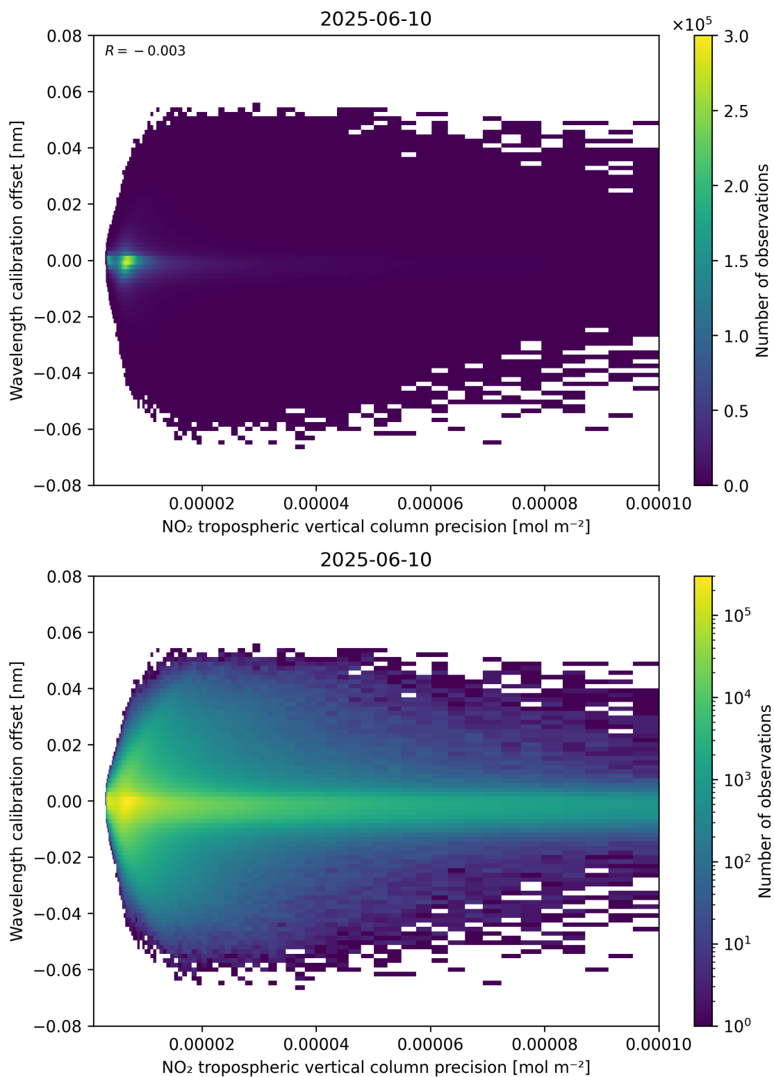
Figure 141: Scatter density plot of “NO 2 tropospheric vertical column precision” against “Wavelength calibration offset” for 2025-06-09 to 2025-06-11.
