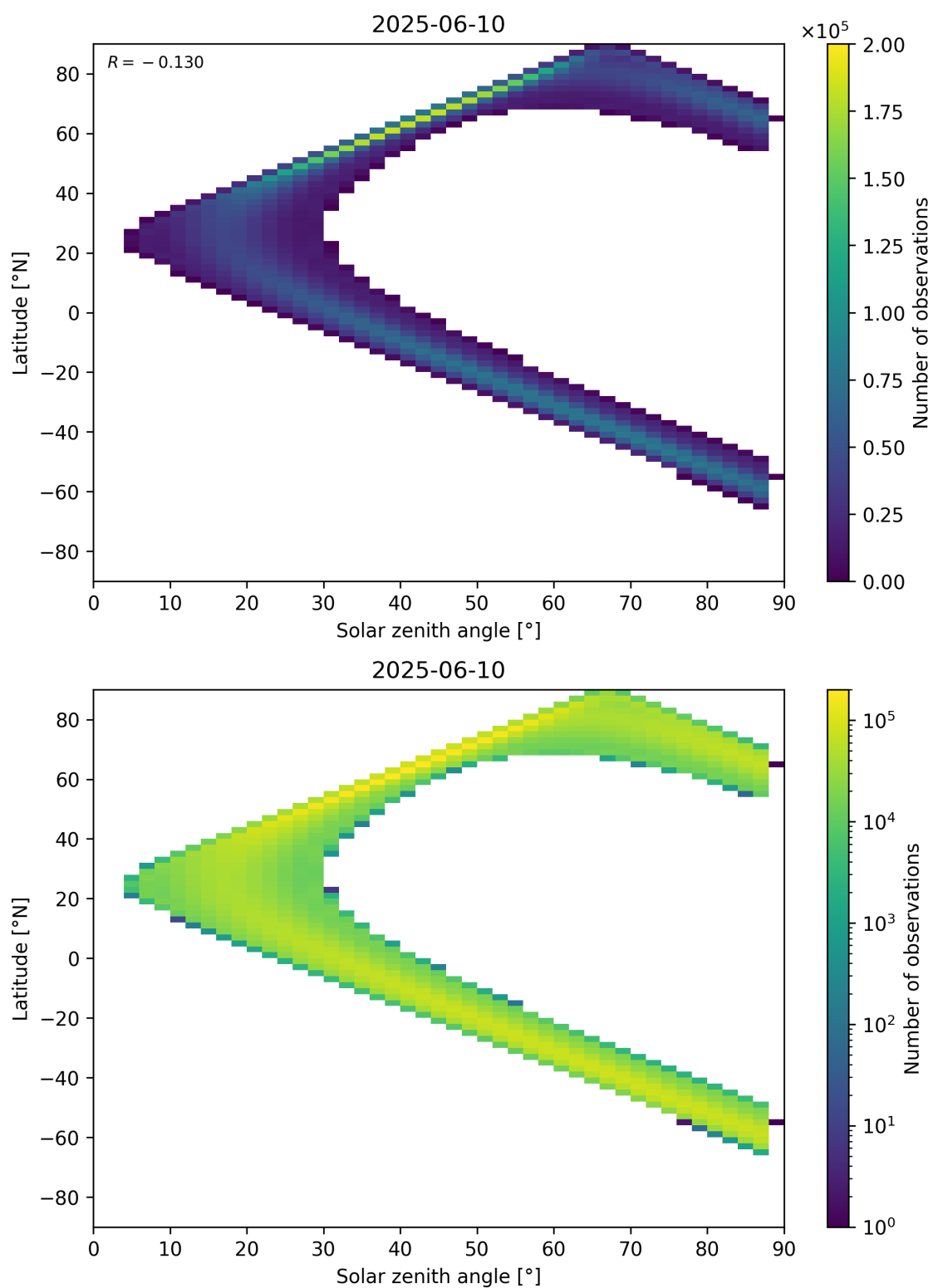
Figure 149: Scatter density plot of “Solar zenith angle” against “Latitude” for 2025-06-09 to 2025-06-11.
