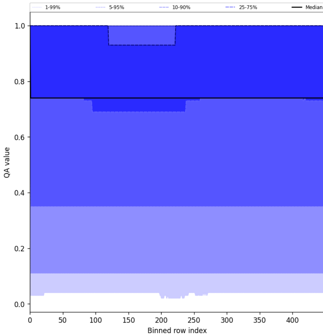
Figure 45: Along track statistics of “QA value” for 2025-06-09 to 2025-06-11
