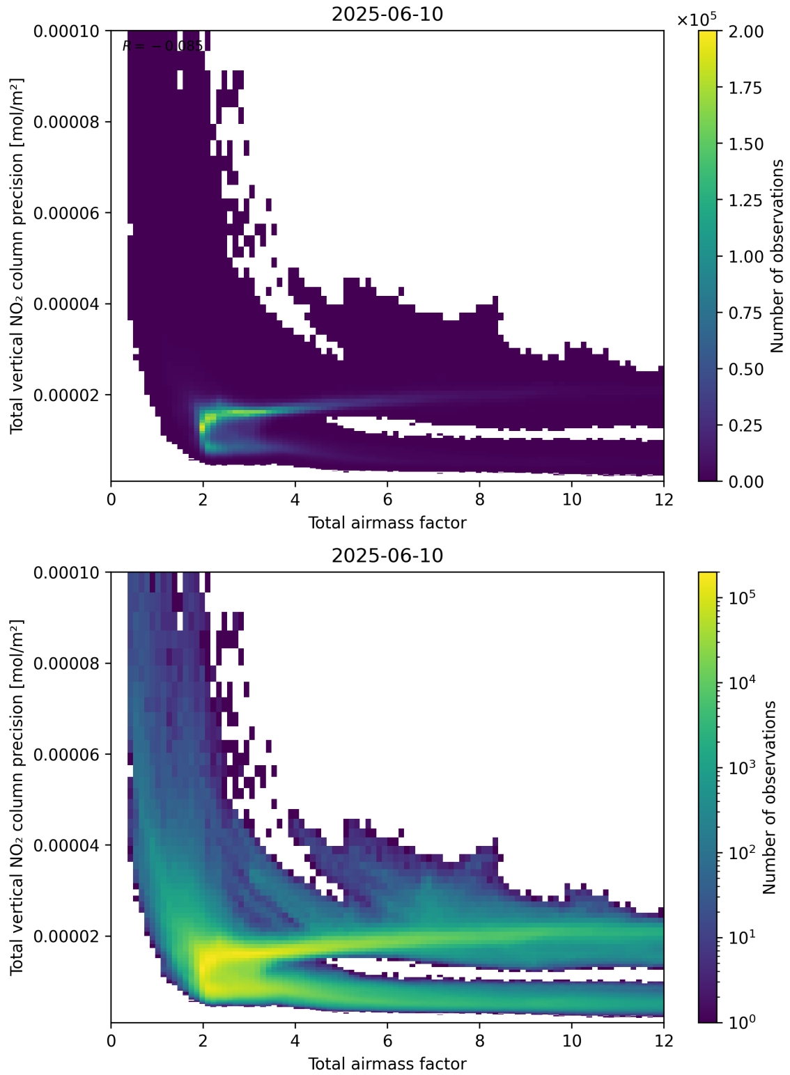
Figure 68: Scatter density plot of “Total airmass factor” against “Total vertical NO 2 column precision” for 2025-06-09 to 2025-06-11.
