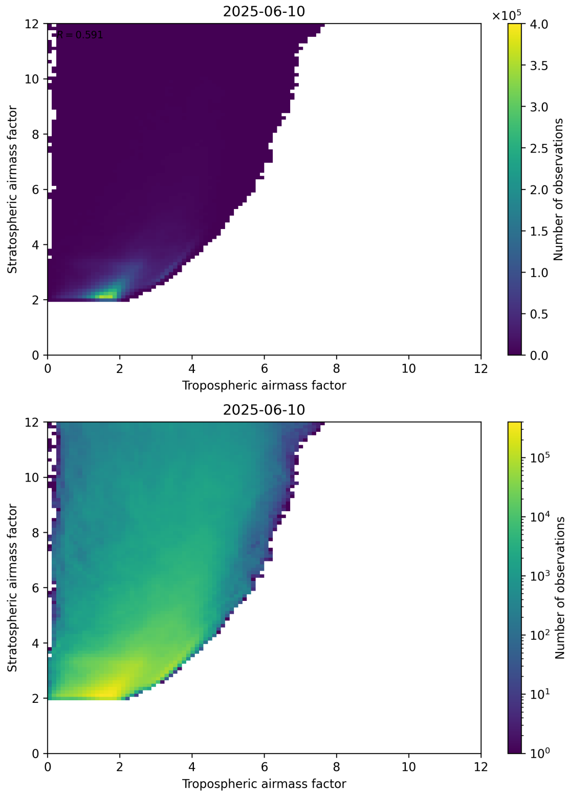
Figure 71: Scatter density plot of “Tropospheric airmass factor” against “Stratospheric airmass factor” for 2025-06-09 to 2025-06-11.
