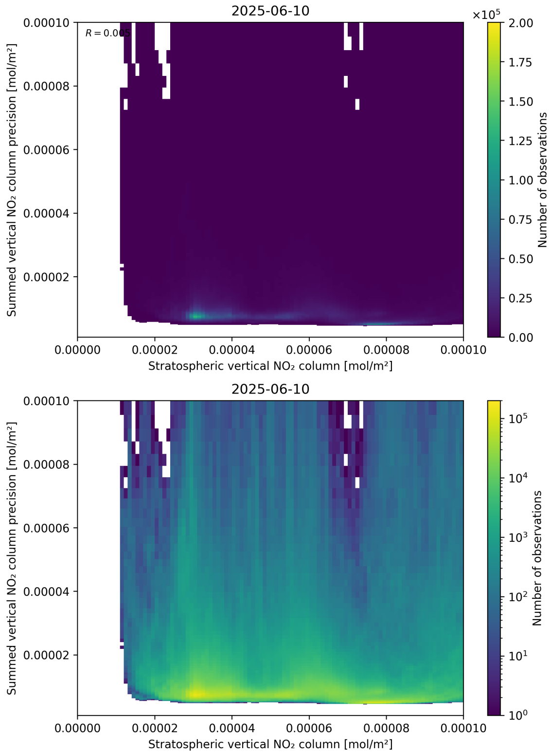
Figure 99: Scatter density plot of “Stratospheric vertical NO 2 column” against “Summed vertical NO 2 column precision” for 2025-06-09 to 2025-06-11.
