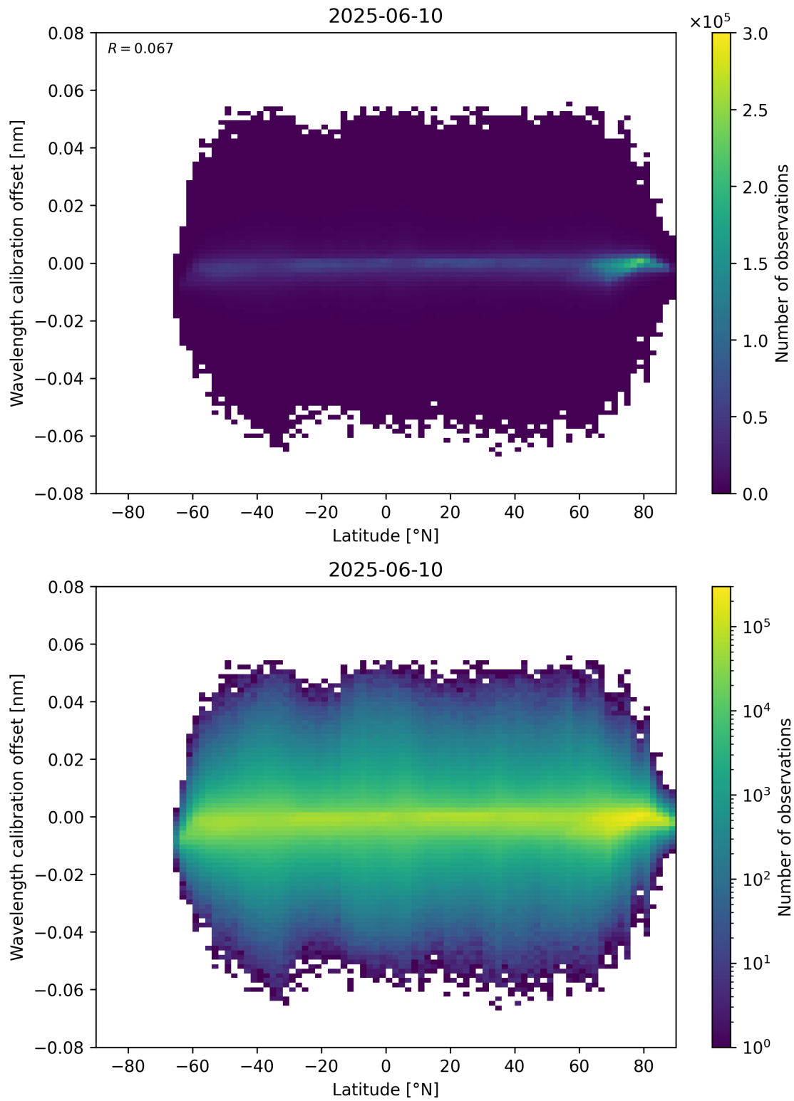
Figure 95: Scatter density plot of “Latitude” against “Wavelength calibration offset” for 2025-06-09 to 2025-06-11.
