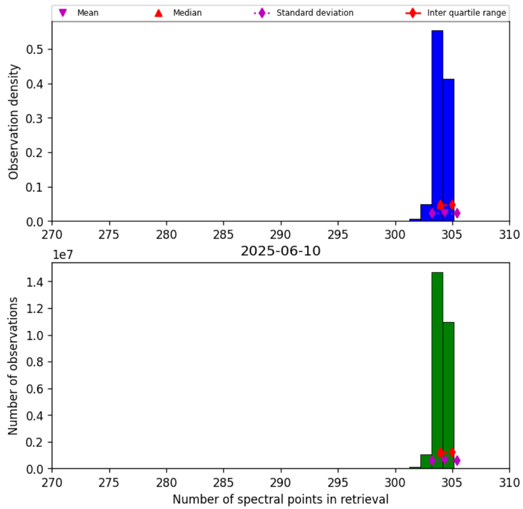
Figure 33: Histogram of “Number of spectral points in retrieval” for 2025-06-09 to 2025-06-11
