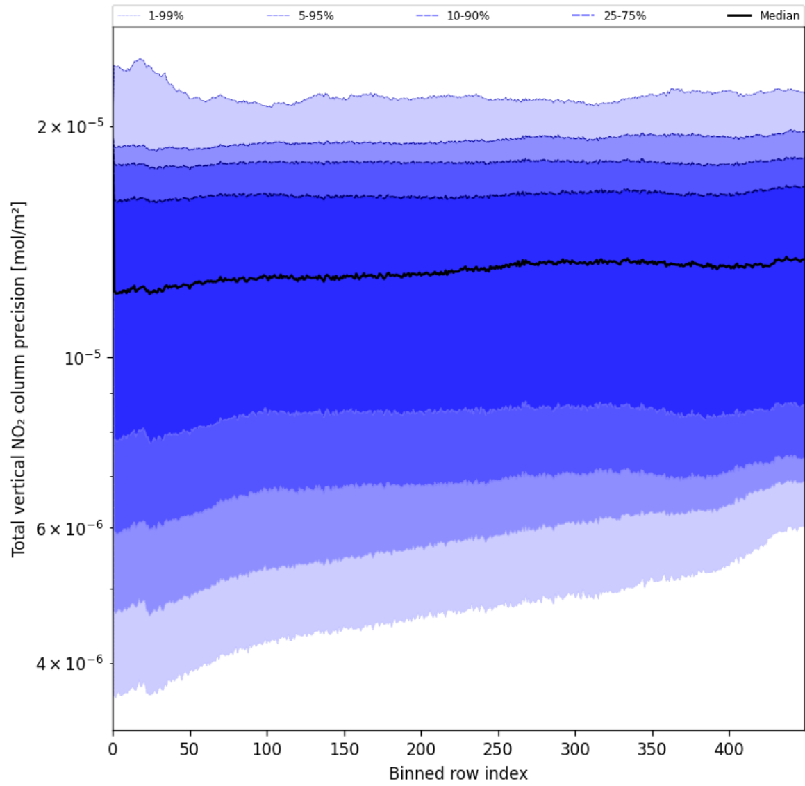
Figure 56: Along track statistics of “Total vertical NO 2 column precision” for 2025-06-09 to 2025-06-11
