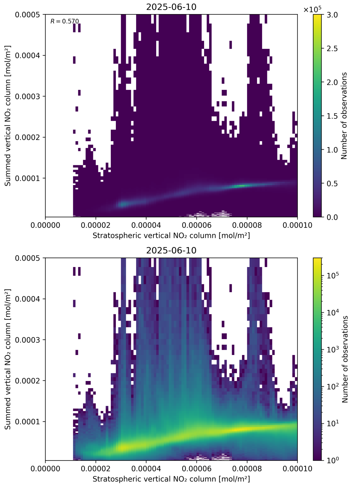
Figure 98: Scatter density plot of “Stratospheric vertical NO 2 column” against “Summed vertical NO 2 column” for 2025-06-09 to 2025-06-11.
