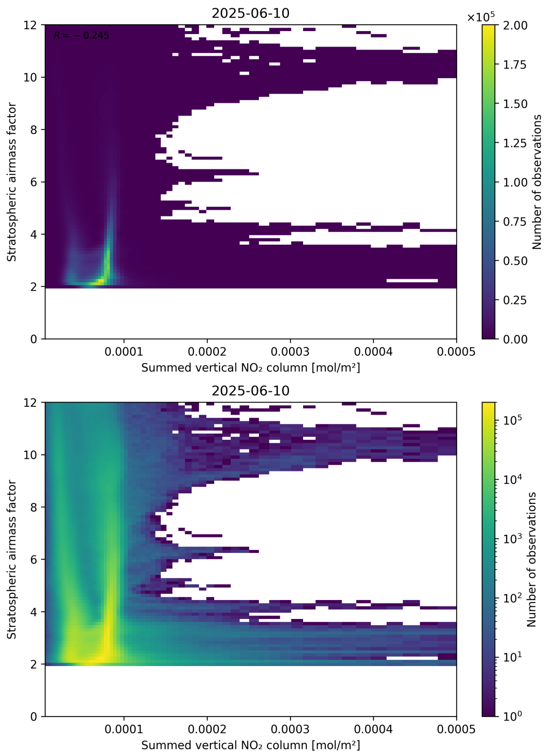
Figure 103: Scatter density plot of “Summed vertical NO 2 column” against “Stratospheric airmass factor” for 2025-06-09 to 2025-06-11.
