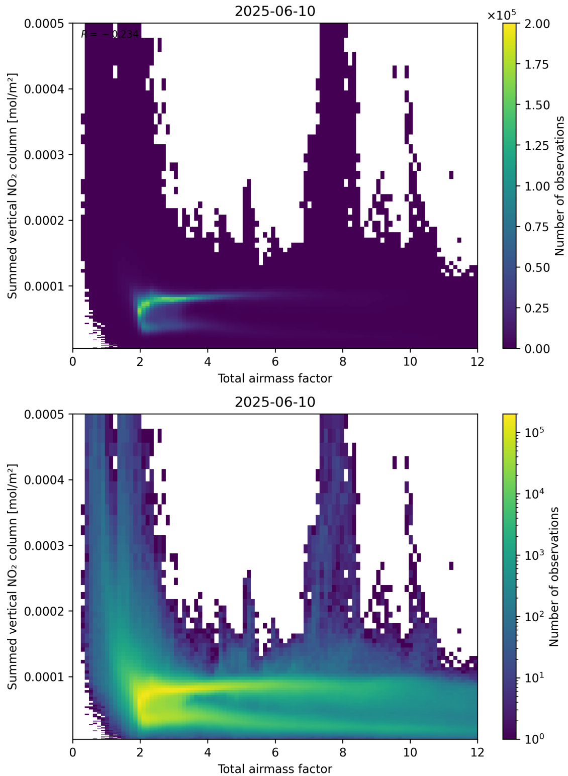
Figure 65: Scatter density plot of “Total airmass factor” against “Summed vertical NO 2 column” for 2025-06-09 to 2025-06-11.
