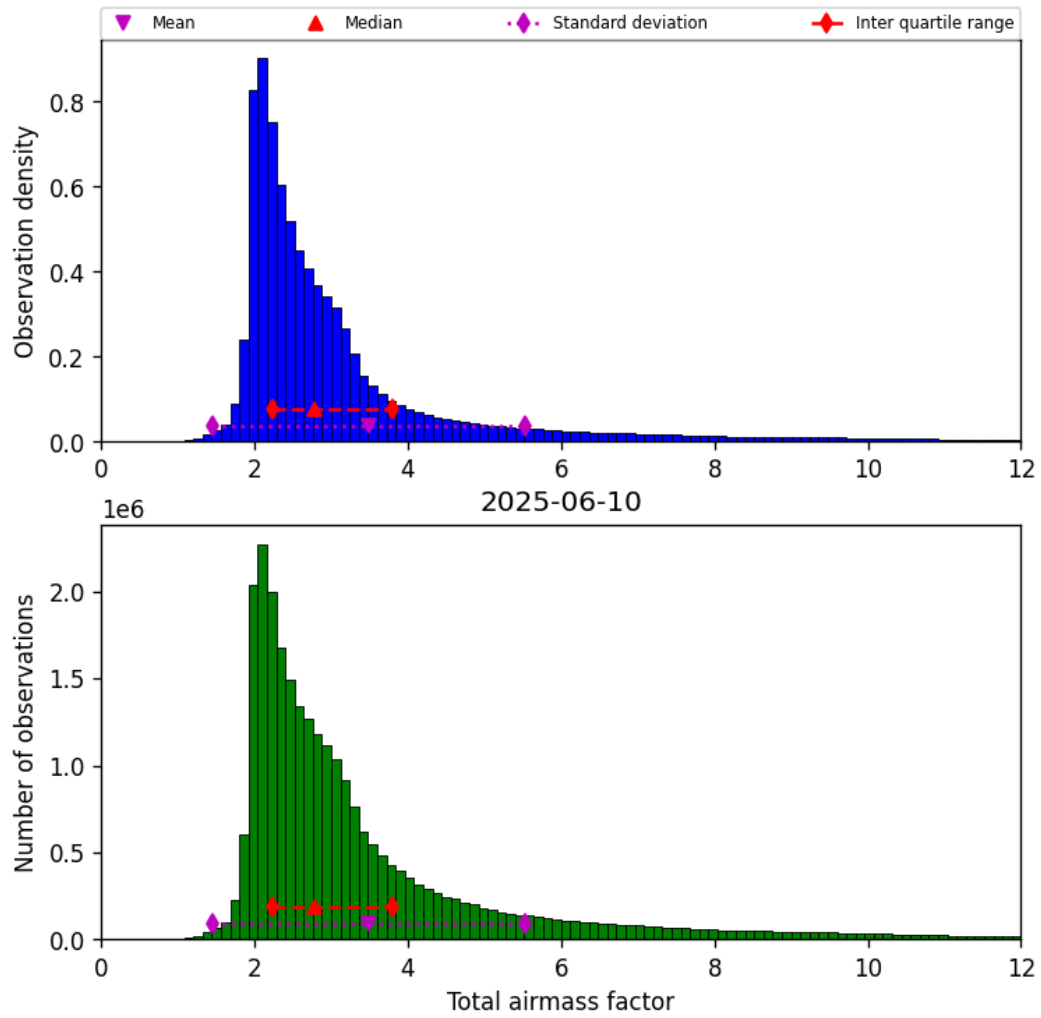
Figure 32: Histogram of “Total airmass factor” for 2025-06-09 to 2025-06-11
