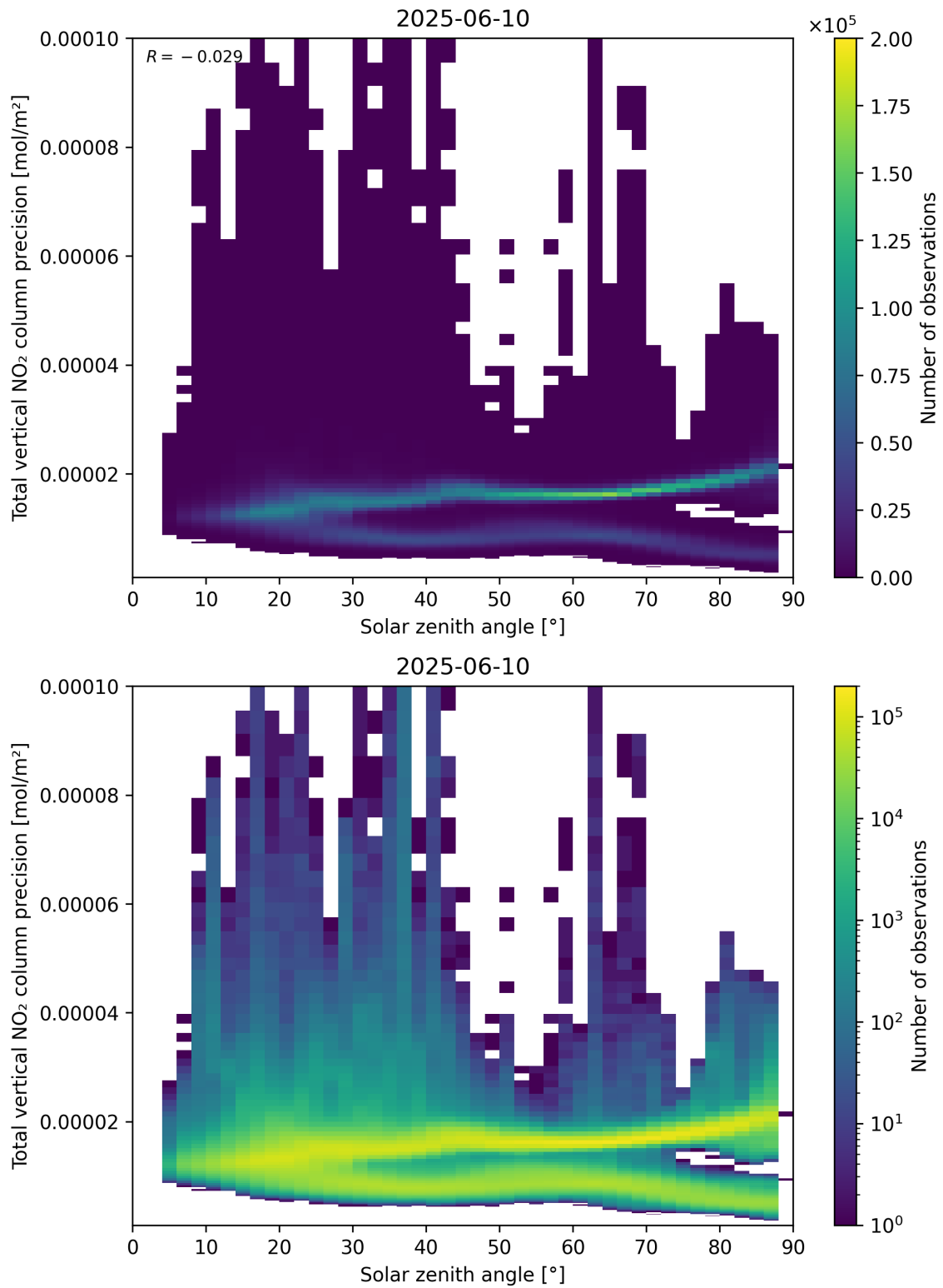
Figure 154: Scatter density plot of “Solar zenith angle” against “Total vertical NO 2 column precision” for 2025-06-09 to 2025-06-11.
