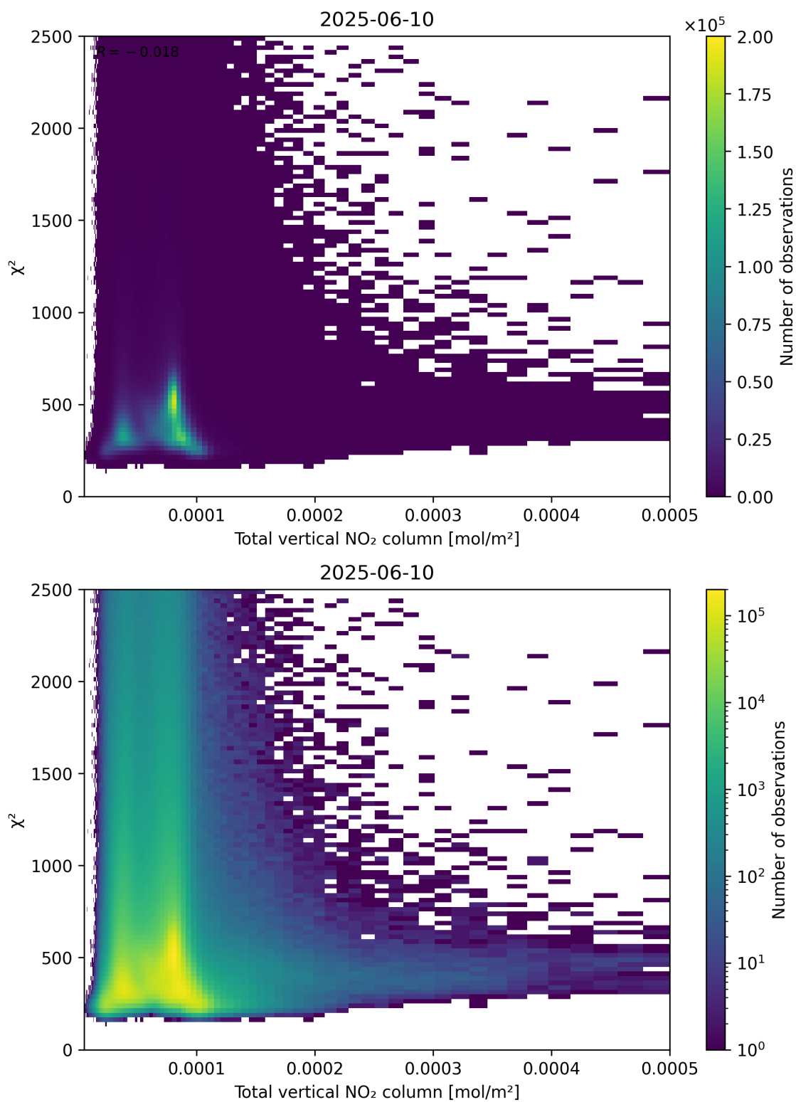
Figure 111: Scatter density plot of “Total vertical NO 2 column” against “ \chi^2 ” for 2025-06-09 to 2025-06-11.
