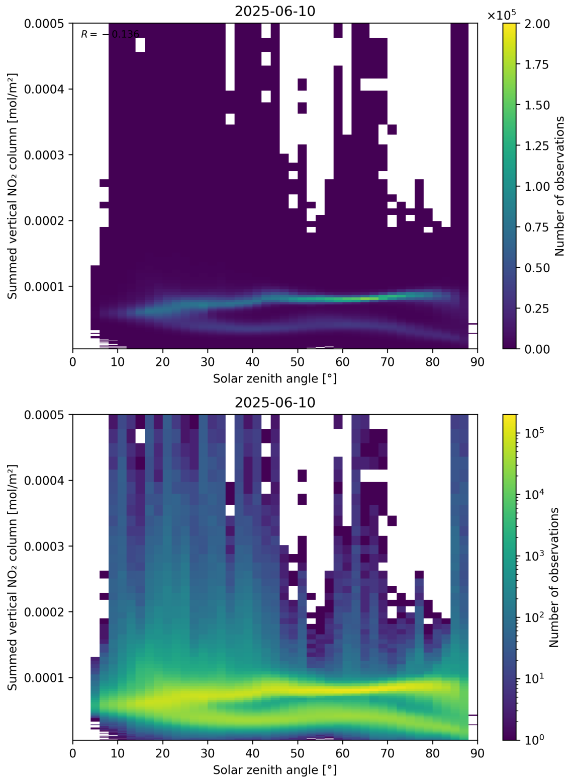
Figure 151: Scatter density plot of “Solar zenith angle” against “Summed vertical NO 2 column” for 2025-06-09 to 2025-06-11.
