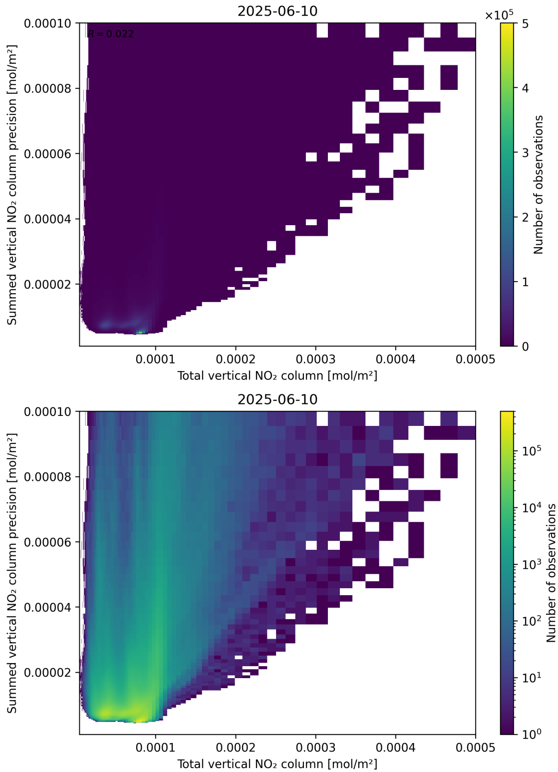
Figure 113: Scatter density plot of “Total vertical NO 2 column” against “Summed vertical NO 2 column precision” for 2025-06-09 to 2025-06-11.
