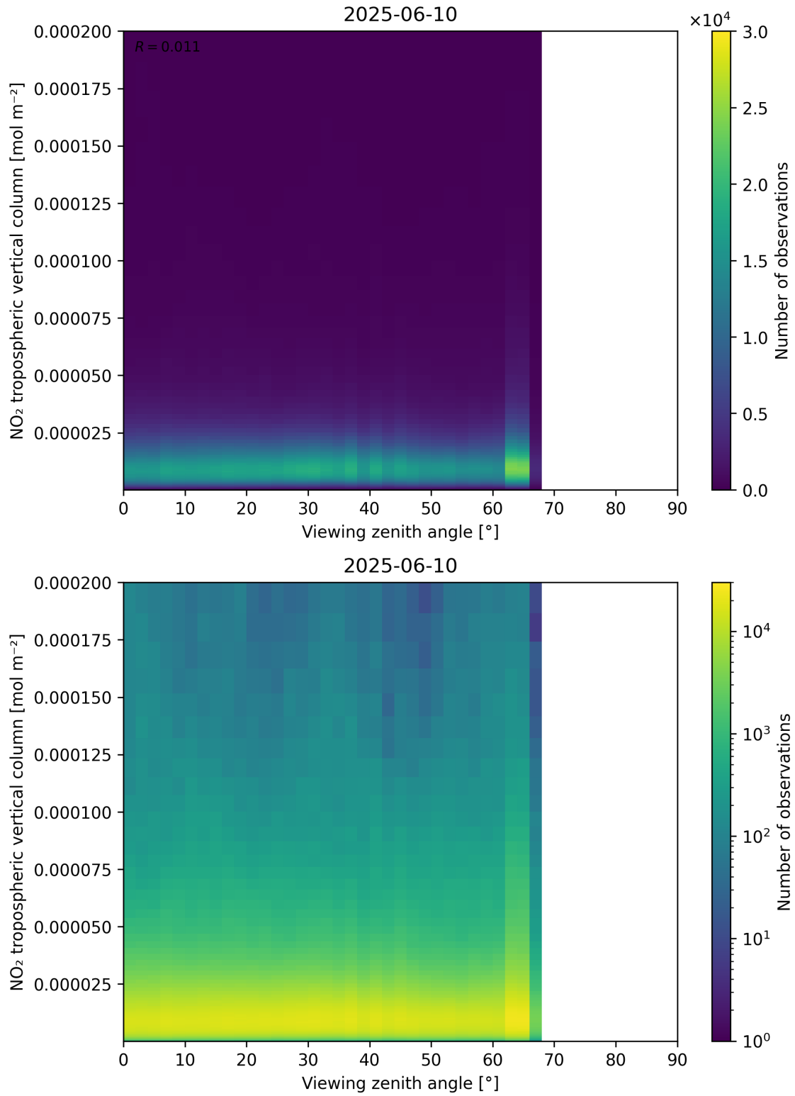
Figure 169: Scatter density plot of “Viewing zenith angle” against “NO 2 tropospheric vertical column” for 2025-06-09 to 2025-06-11.
