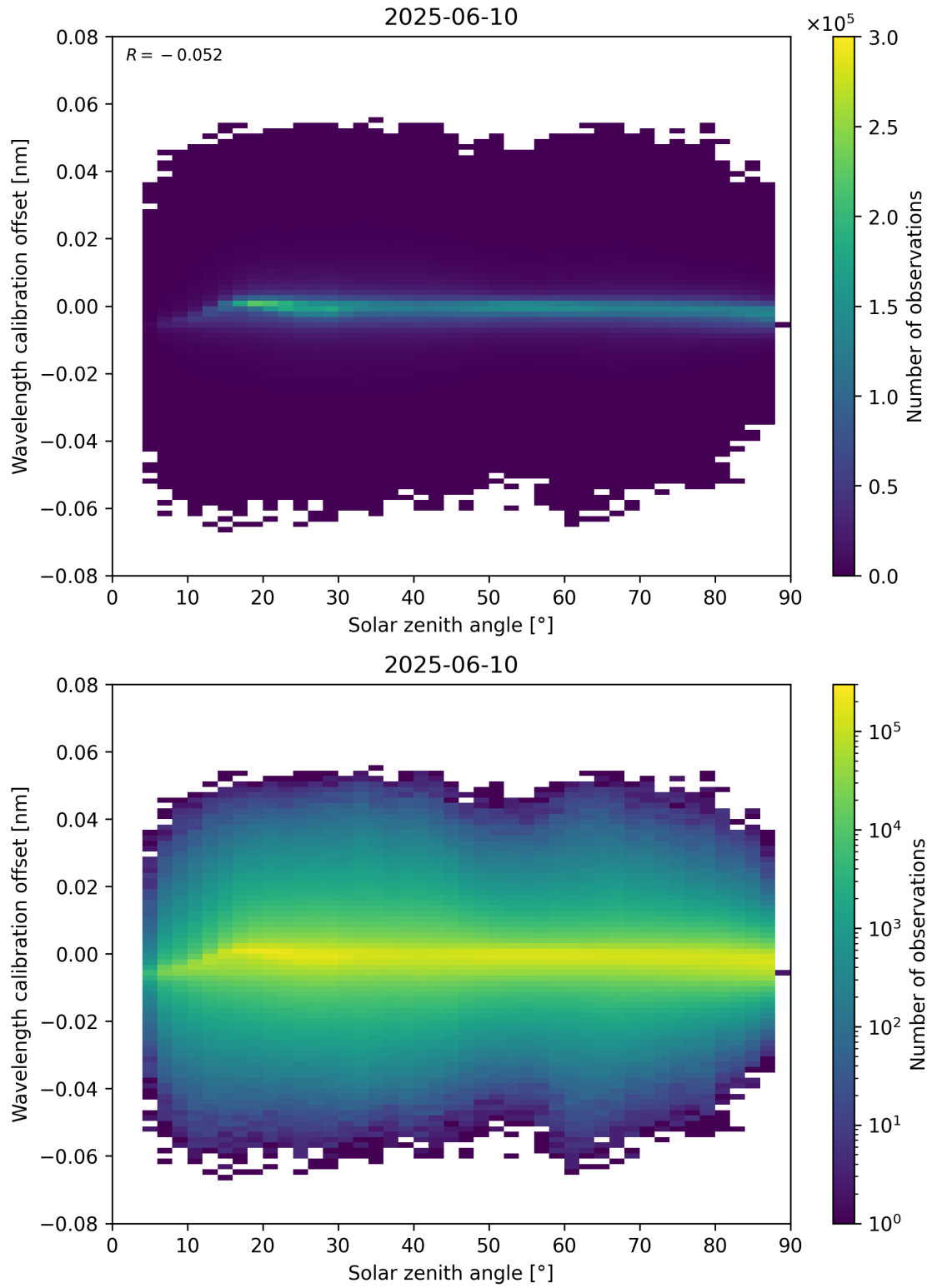
Figure 158: Scatter density plot of “Solar zenith angle” against “Wavelength calibration offset” for 2025-06-09 to 2025-06-11.
