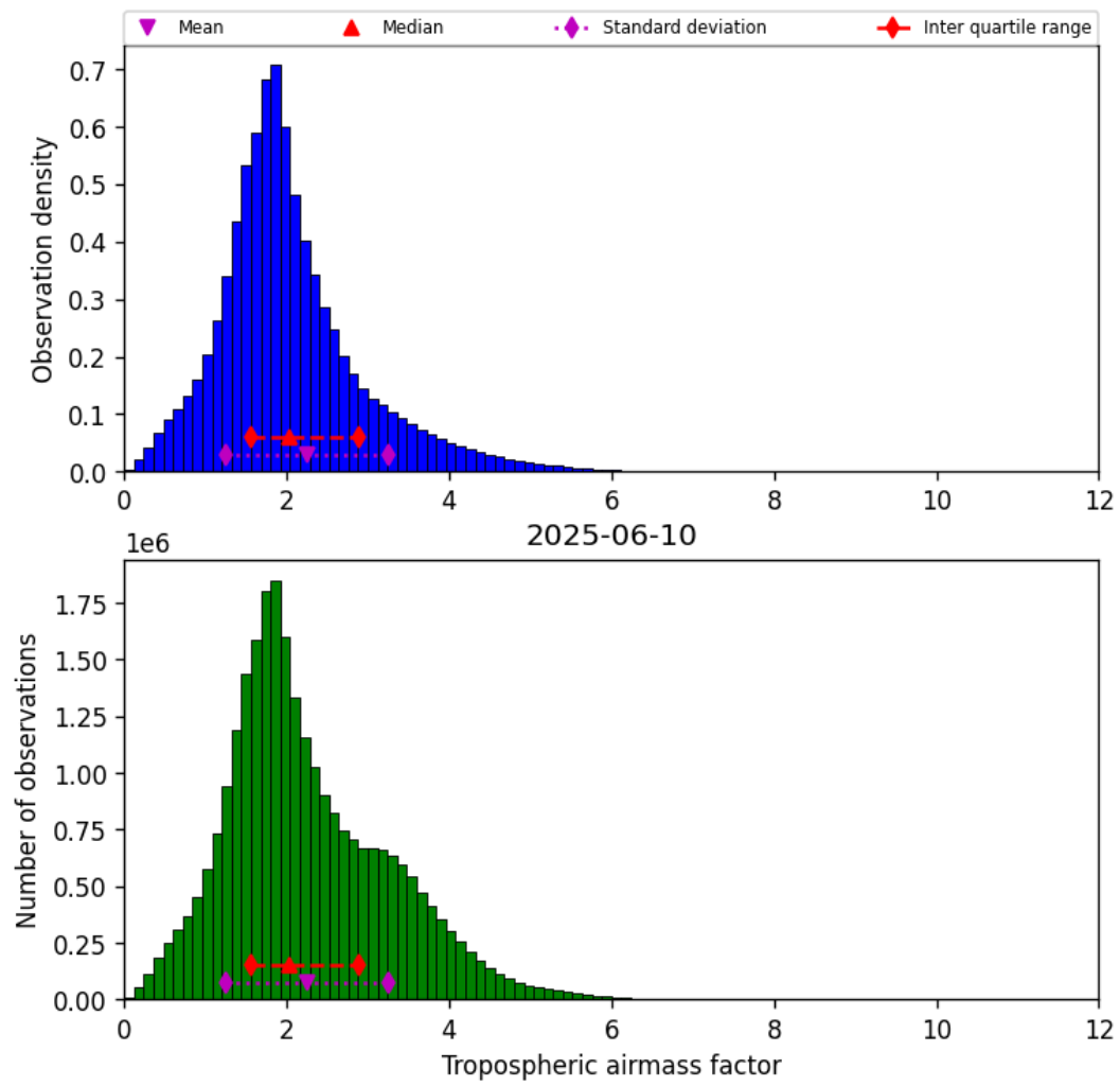
Figure 31: Histogram of “Tropospheric airmass factor” for 2025-06-09 to 2025-06-11
