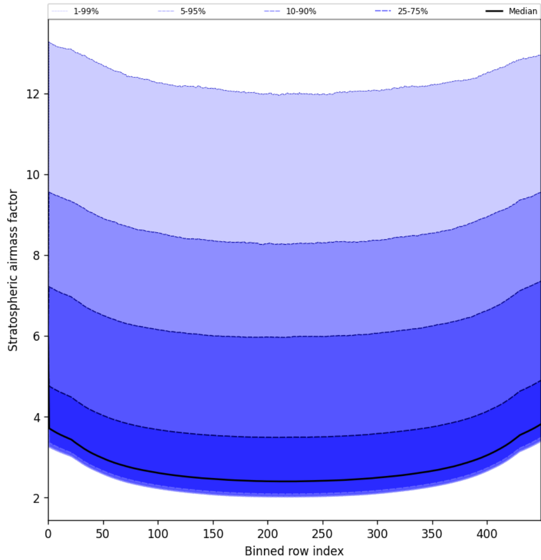
Figure 61: Along track statistics of “Stratospheric airmass factor” for 2025-06-09 to 2025-06-11
