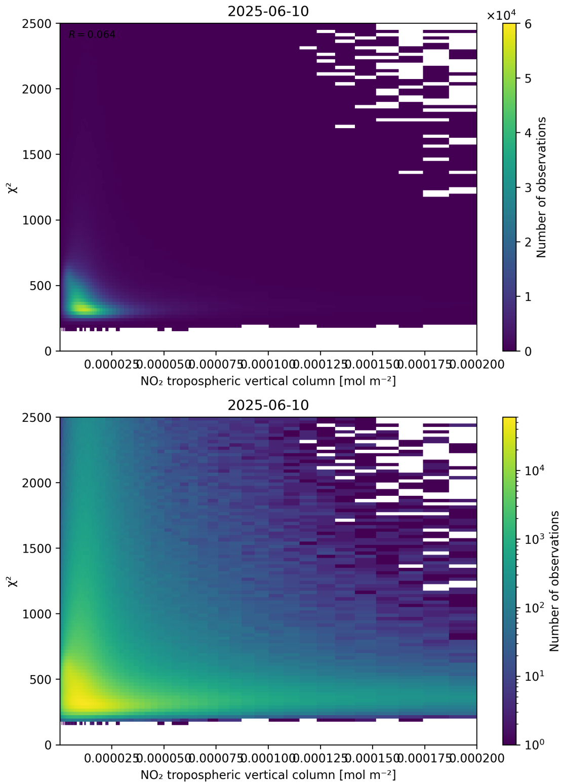
Figure 124: Scatter density plot of “NO 2 tropospheric vertical column” against “ \chi^2 ” for 2025-06-09 to 2025-06-11.
