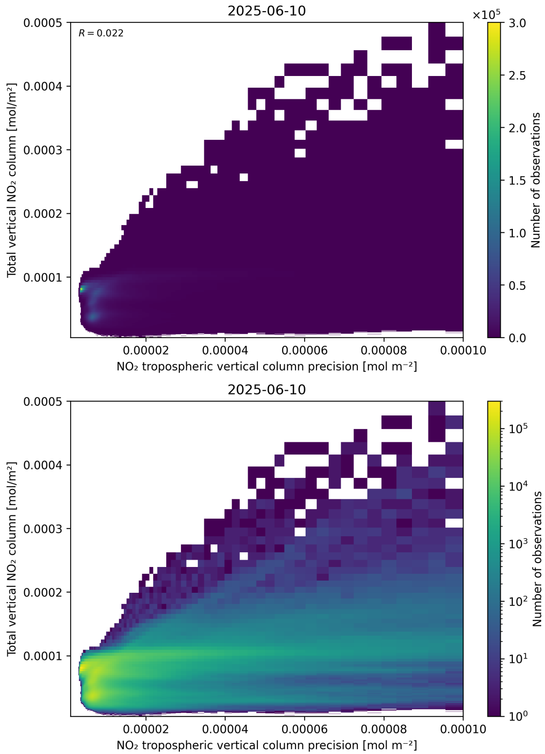
Figure 138: Scatter density plot of “NO 2 tropospheric vertical column precision” against “Total vertical NO 2 column” for 2025-06-09 to 2025-06-11.
