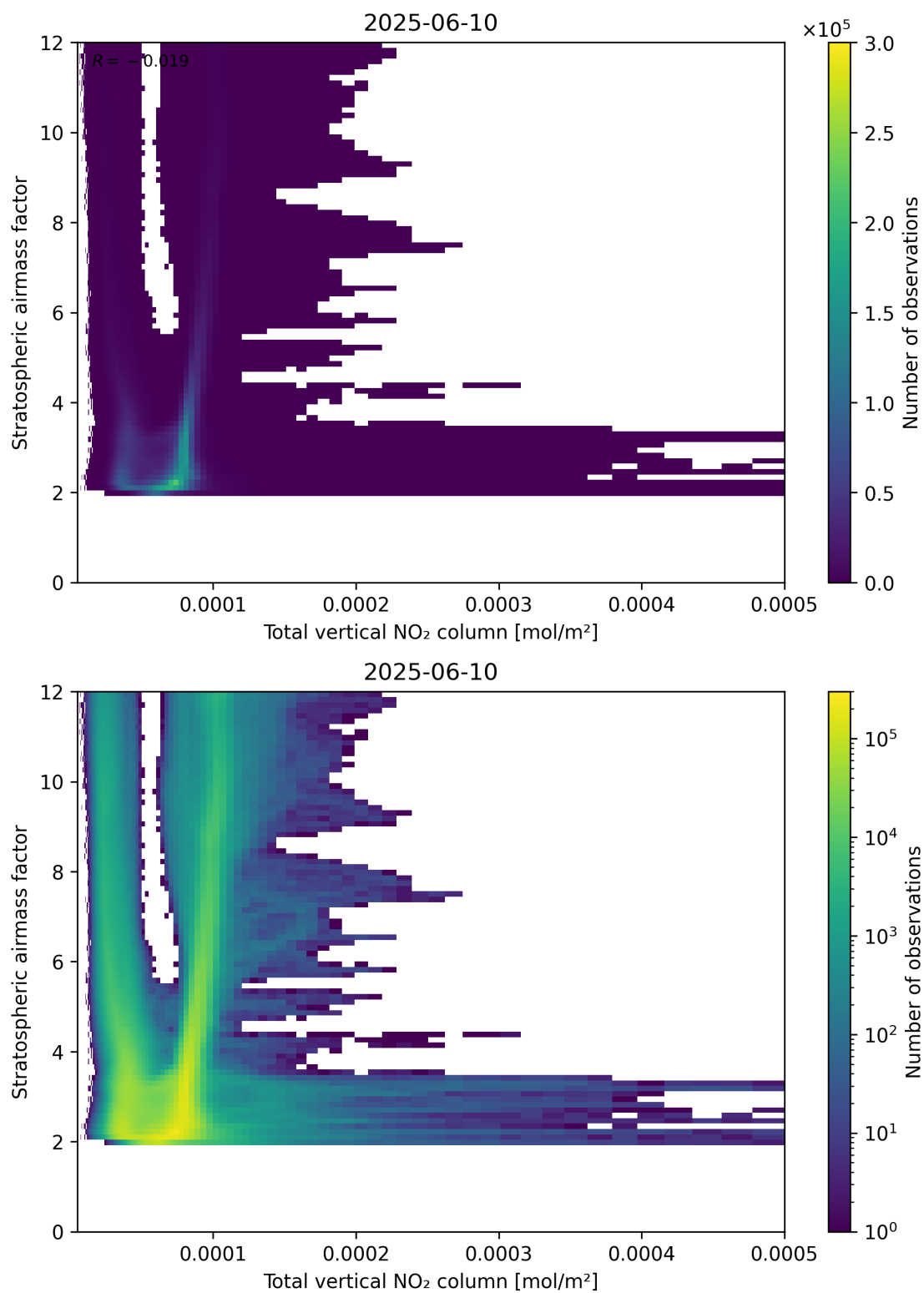
Figure 110: Scatter density plot of “Total vertical NO 2 column” against “Stratospheric airmass factor” for 2025-06-09 to 2025-06-11.
