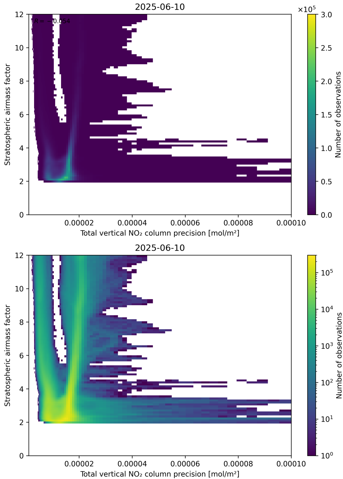
Figure 115: Scatter density plot of “Total vertical NO 2 column precision” against “Stratospheric air mass factor” for 2025-06-09 to 2025-06-11.
