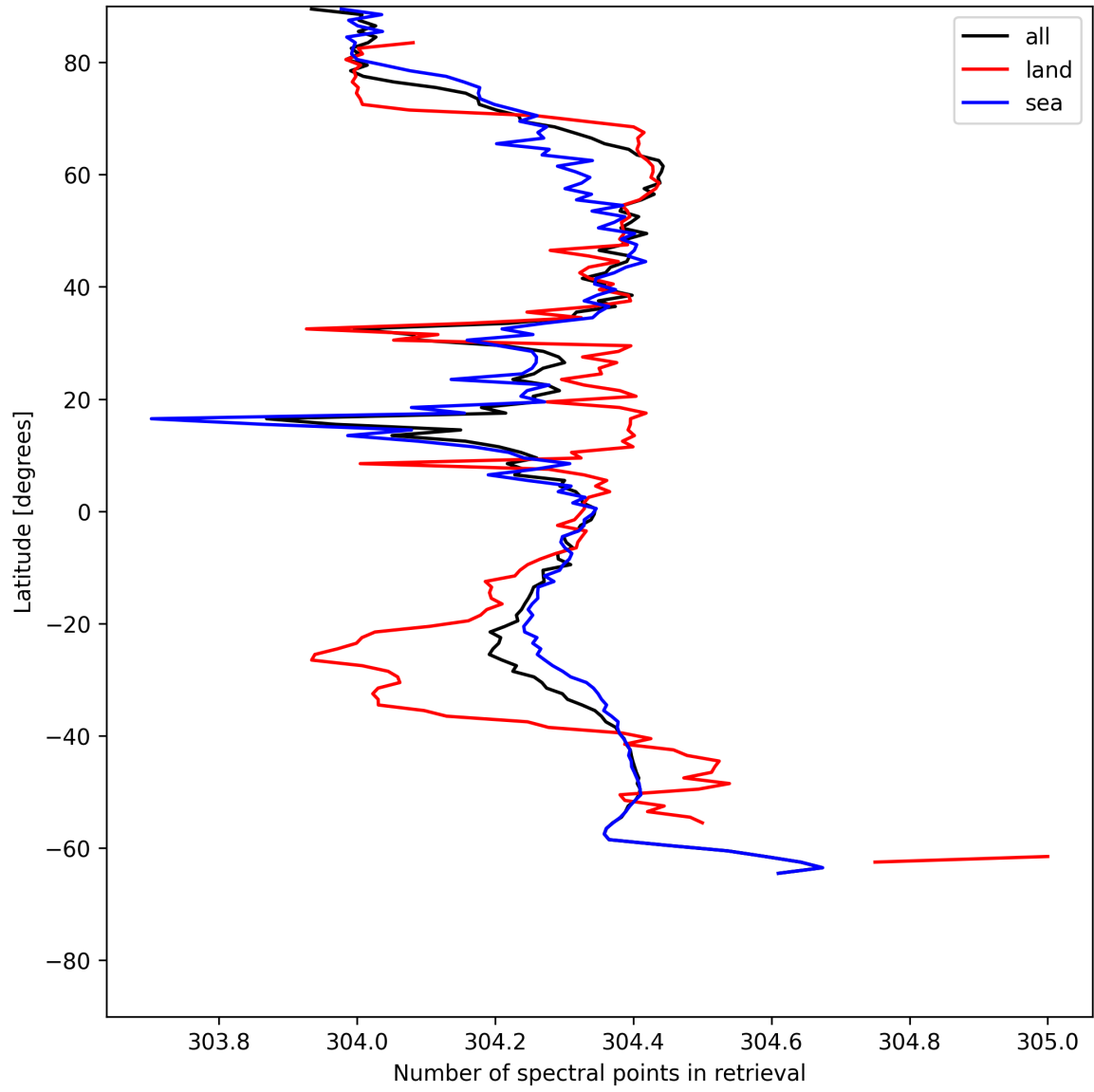
Figure 16: Zonal average of “Number of spectral points in retrieval” for 2025-06-09 to 2025-06-11.
