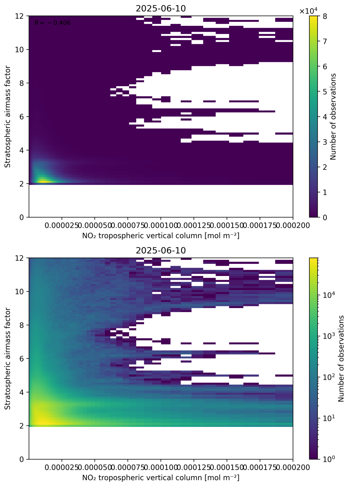
Figure 121: Scatter density plot of “NO 2 tropospheric vertical column” against “Stratospheric air mass factor” for 2025-06-09 to 2025-06-11.
