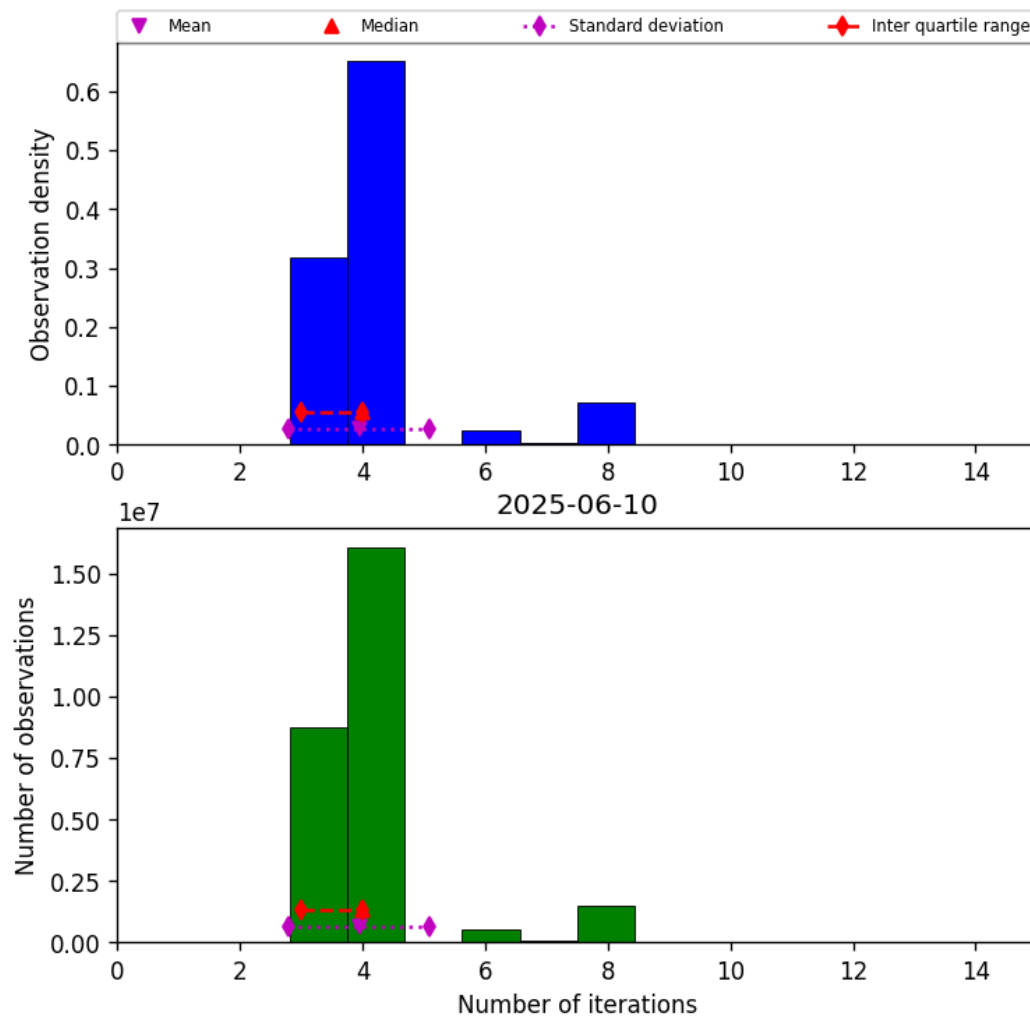
Figure 34: Histogram of “Number of iterations” for 2025-06-09 to 2025-06-11
