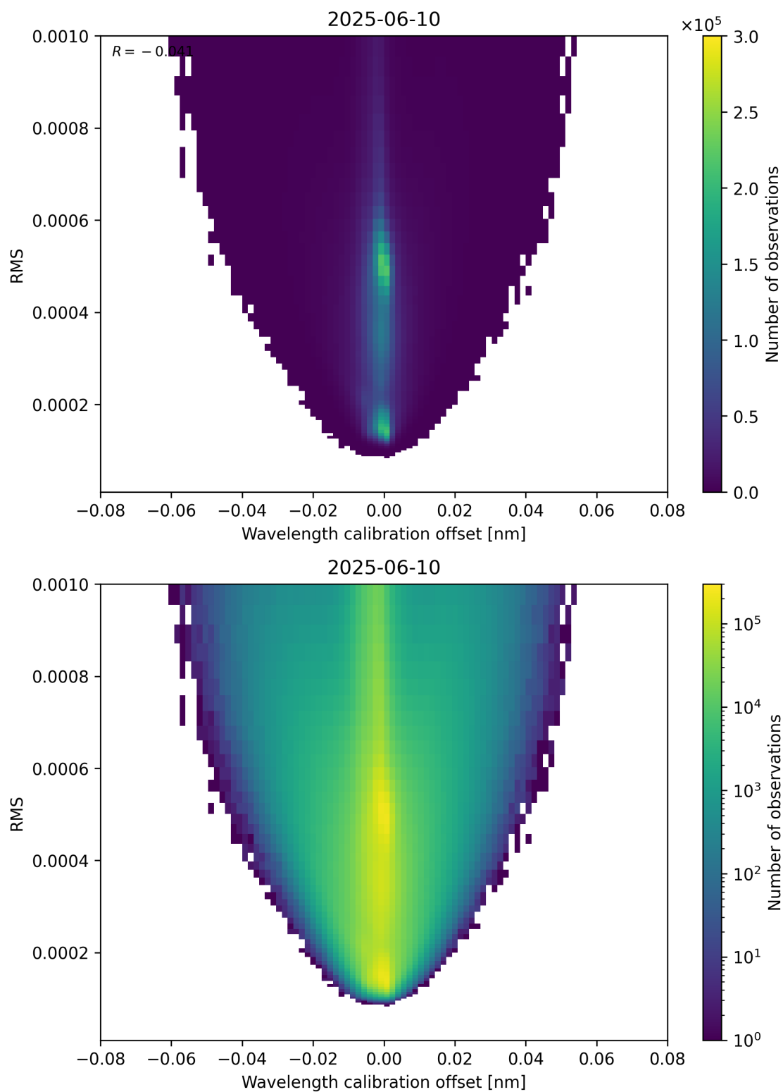
Figure 181: Scatter density plot of “Wavelength calibration offset” against “RMS” for 2025-06-09 to 2025-06-11.
