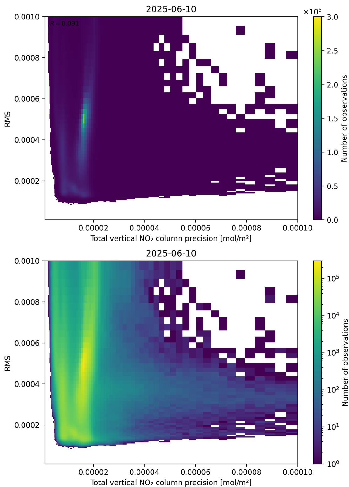
Figure 119: Scatter density plot of “Total vertical NO 2 column precision” against “RMS” for 2025-06-09 to 2025-06-11.
