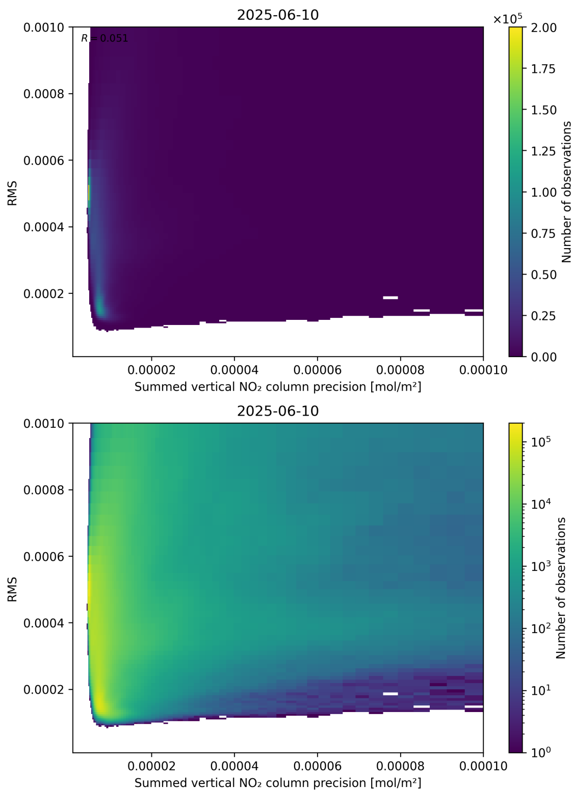
Figure 108: Scatter density plot of “Summed vertical NO 2 column precision” against “RMS” for 2025-06-09 to 2025-06-11.
