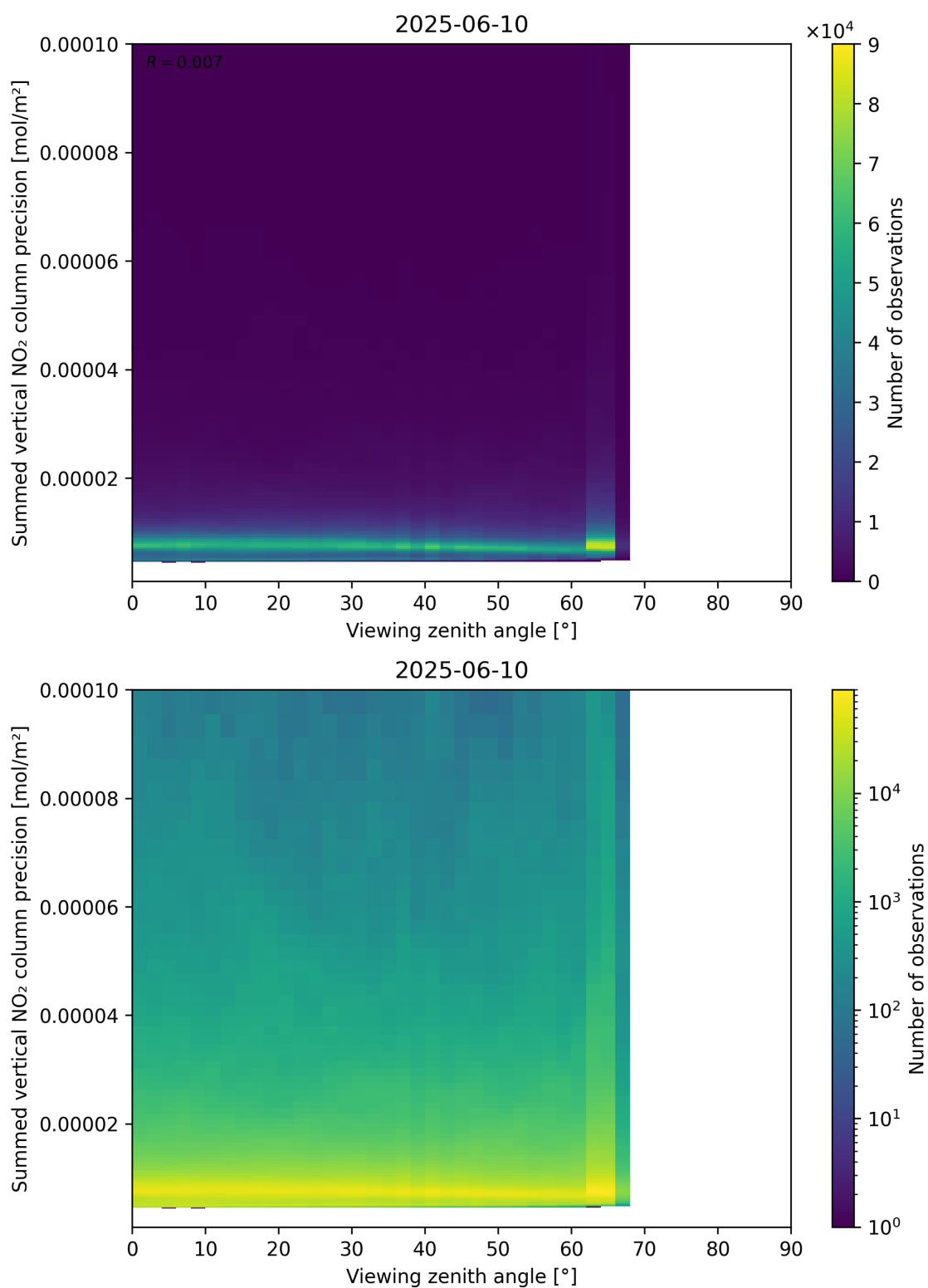
Figure 166: Scatter density plot of “Viewing zenith angle” against “Summed vertical NO 2 column precision” for 2025-06-09 to 2025-06-11.
