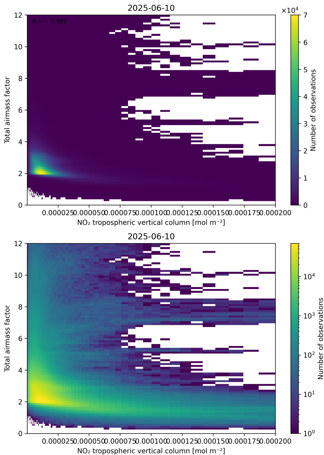
Figure 122: Scatter density plot of “NO 2 tropospheric vertical column” against “Total air mass factor” for 2025-06-09 to 2025-06-11.
