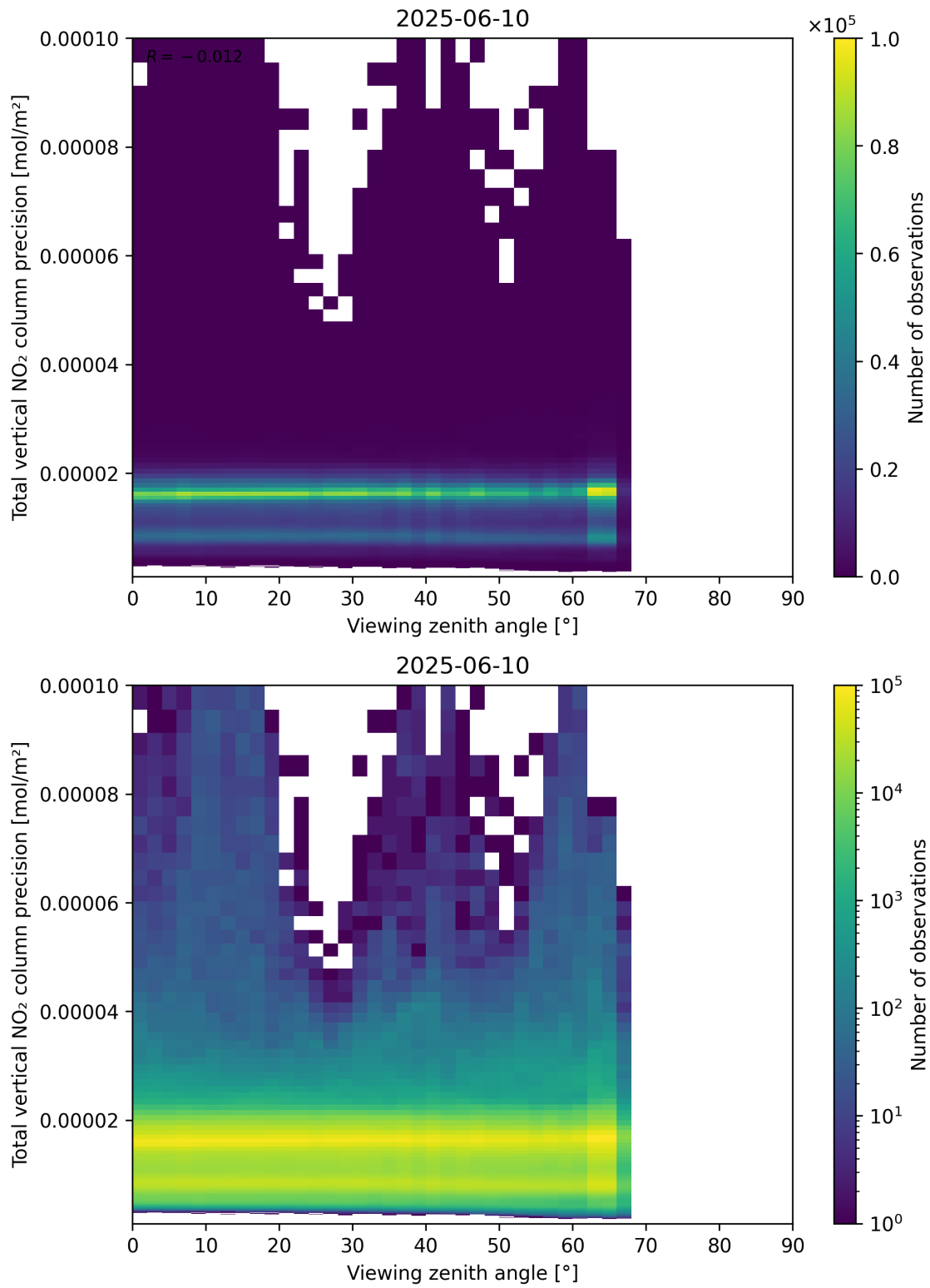
Figure 168: Scatter density plot of “Viewing zenith angle” against “Total vertical NO 2 column precision” for 2025-06-09 to 2025-06-11.
