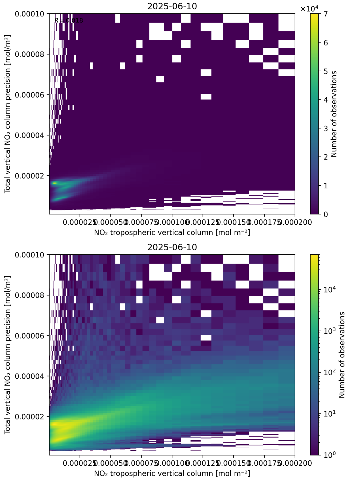
Figure 129: Scatter density plot of “NO 2 tropospheric vertical column” against “Total vertical NO 2 column precision” for 2025-06-09 to 2025-06-11.
