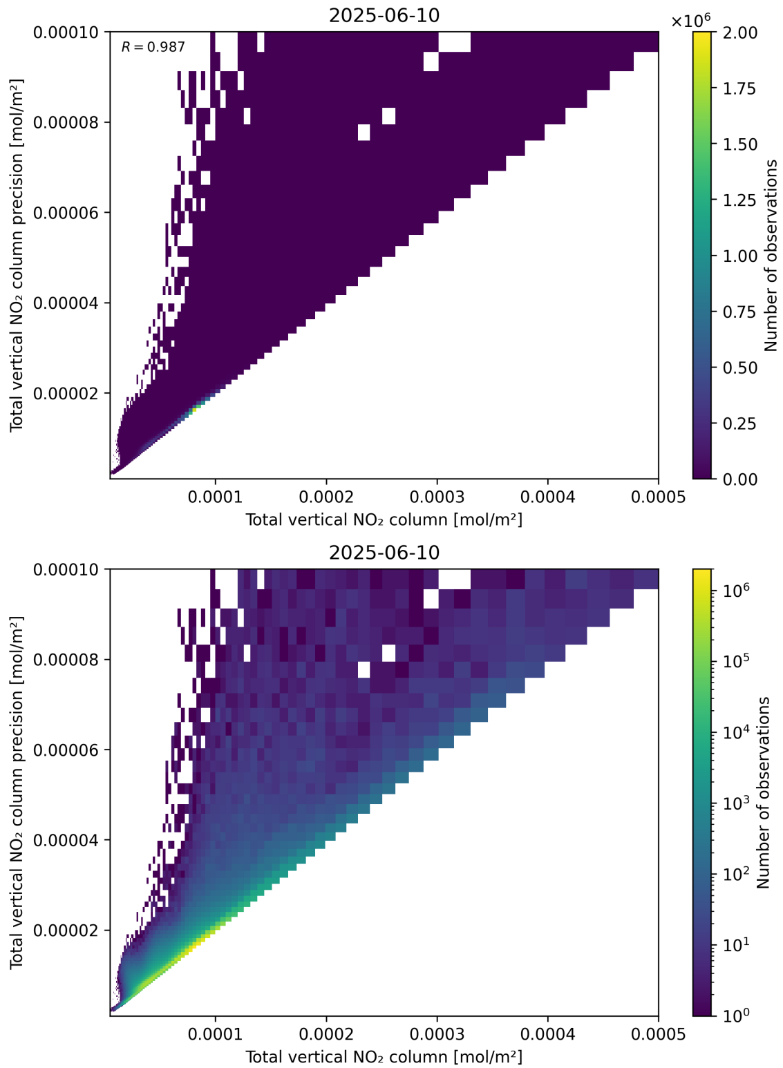
Figure 114: Scatter density plot of “Total vertical NO 2 column” against “Total vertical NO 2 column precision” for 2025-06-09 to 2025-06-11.
