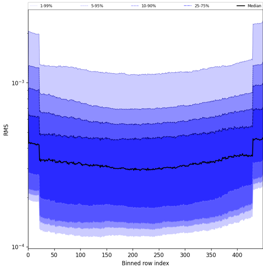
Figure 60: Along track statistics of “RMS” for 2025-06-09 to 2025-06-11
