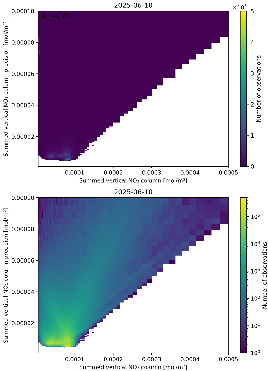
Figure 105: Scatter density plot of “Summed vertical NO 2 column” against “Summed vertical NO 2 column precision” for 2025-06-09 to 2025-06-11.
