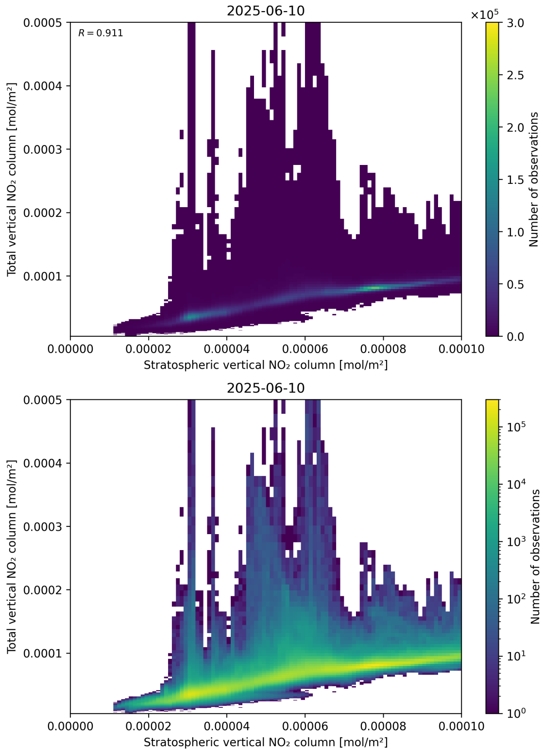
Figure 100: Scatter density plot of “Stratospheric vertical NO 2 column” against “Total vertical NO 2 column” for 2025-06-09 to 2025-06-11.
