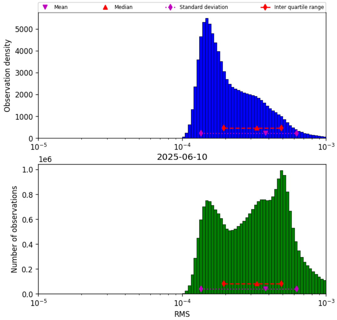
Figure 43: Histogram of “RMS” for 2025-06-09 to 2025-06-11
