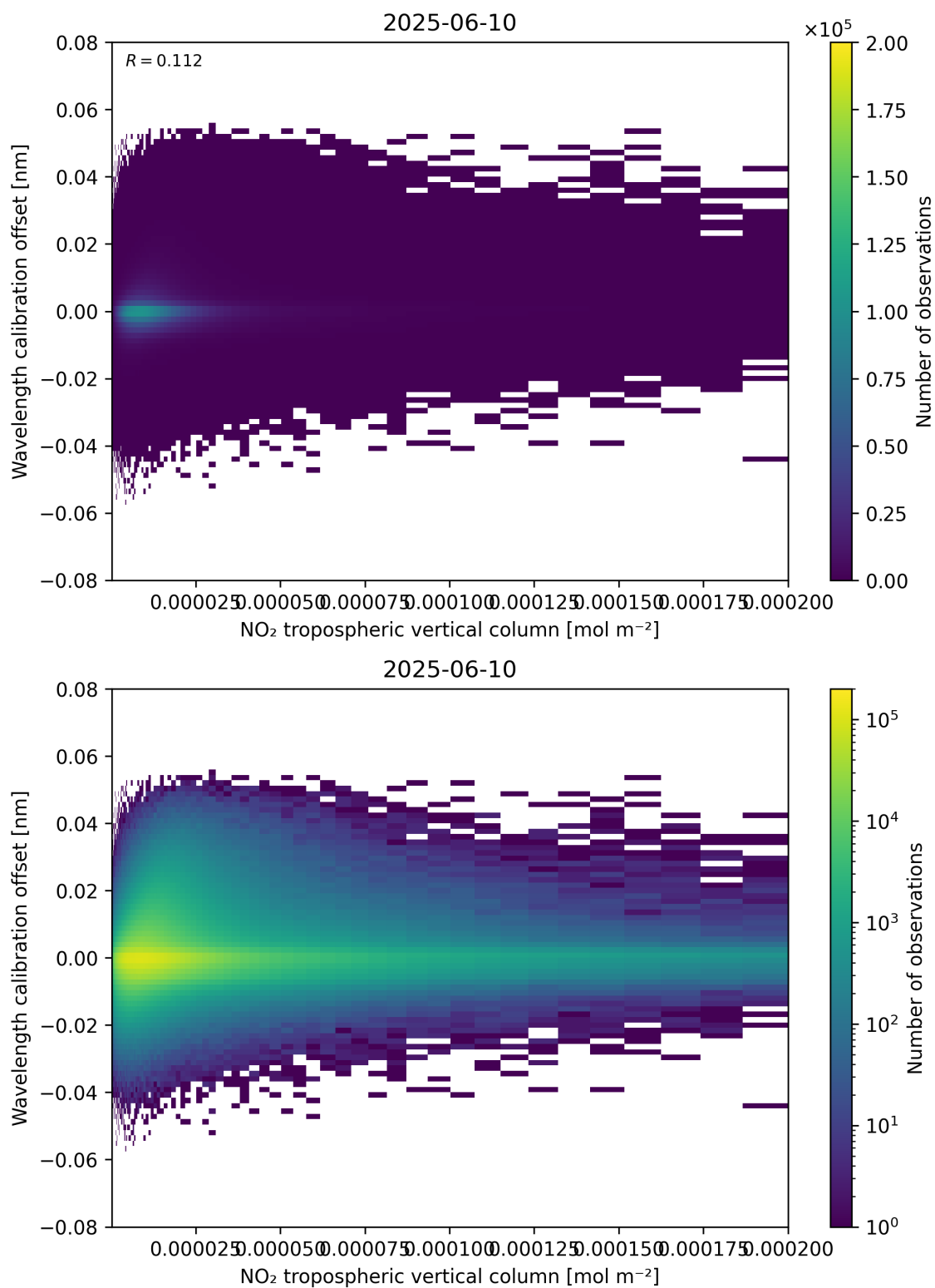
Figure 143: Scatter density plot of “NO 2 tropospheric vertical column” against “Wavelength calibration offset” for 2025-06-09 to 2025-06-11.
