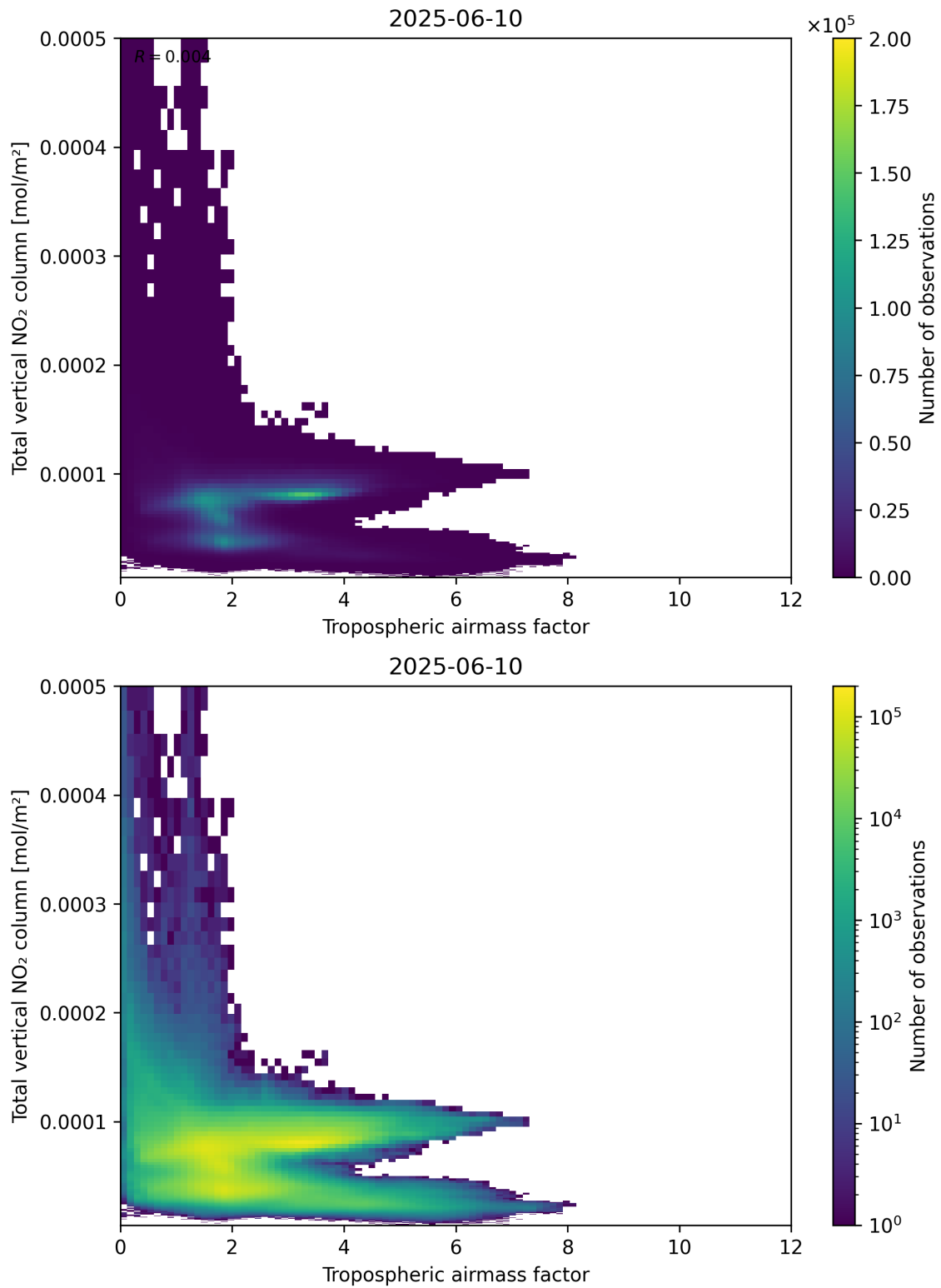
Figure 77: Scatter density plot of “Tropospheric airmass factor” against “Total vertical NO 2 column” for 2025-06-09 to 2025-06-11.
