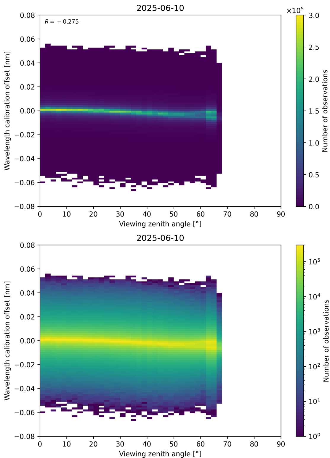
Figure 173: Scatter density plot of “Viewing zenith angle” against “Wavelength calibration offset” for 2025-06-09 to 2025-06-11.
