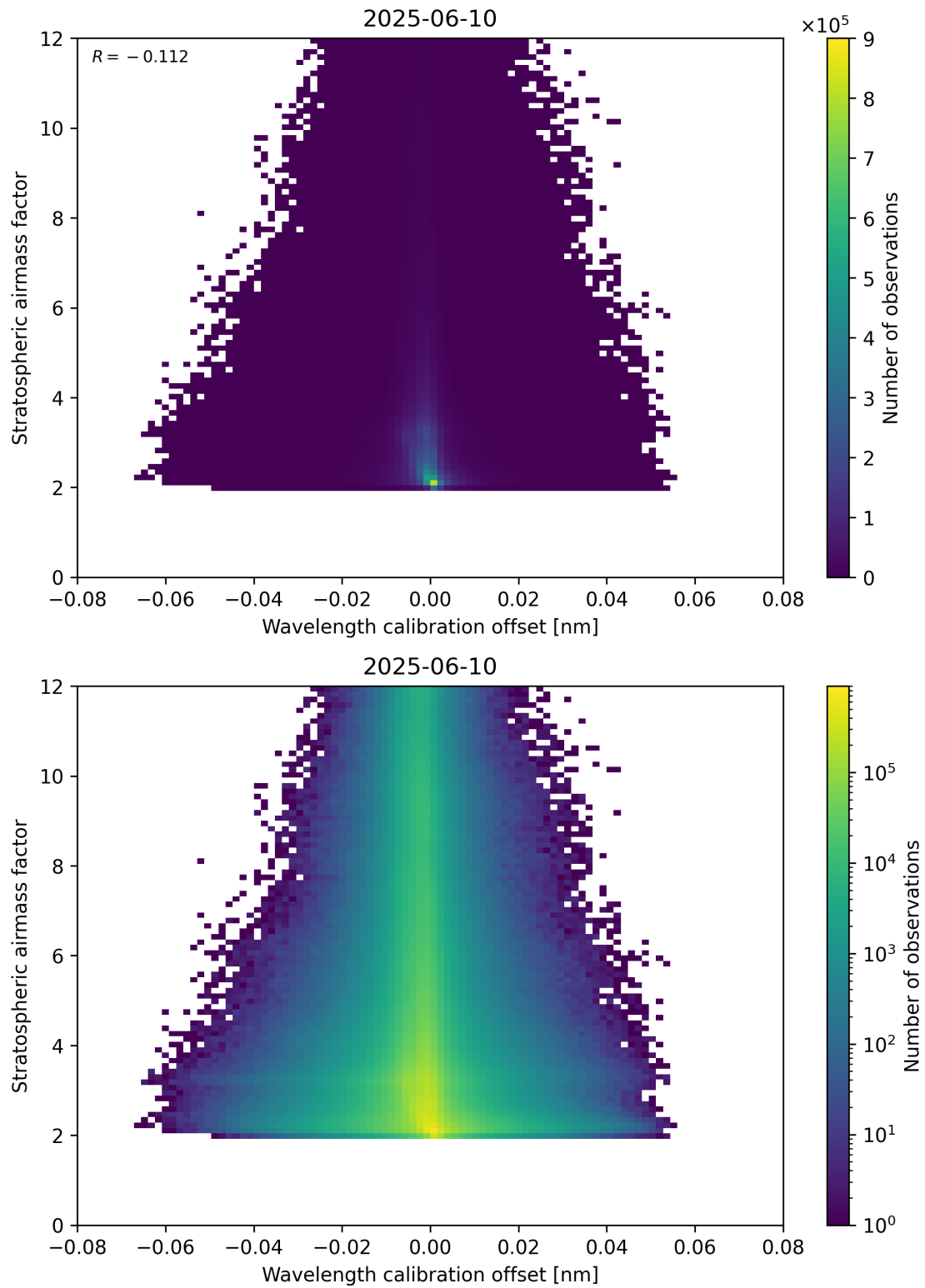
Figure 174: Scatter density plot of “Wavelength calibration offset” against “Stratospheric airmass factor” for 2025-06-09 to 2025-06-11.
