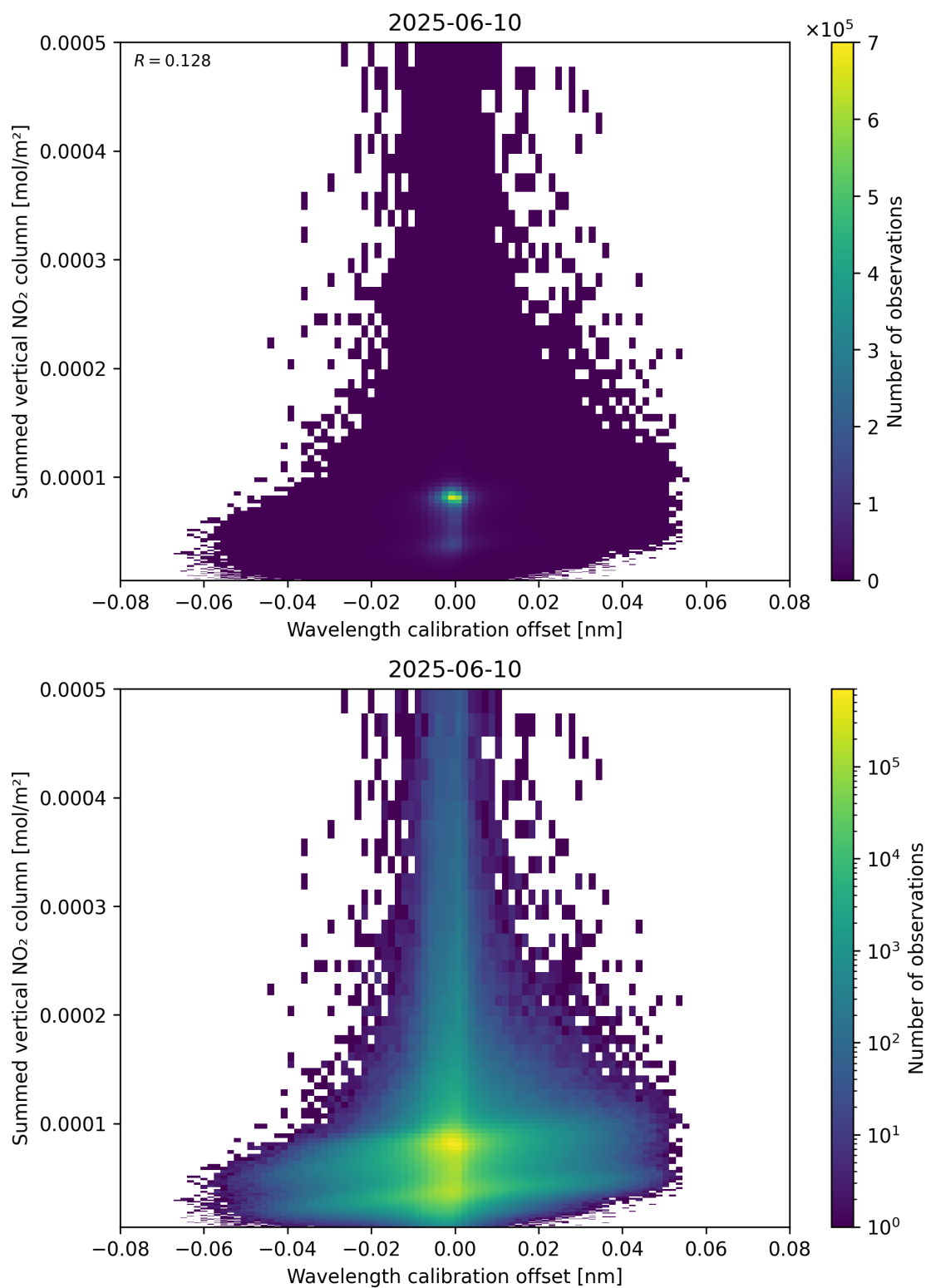
Figure 177: Scatter density plot of “Wavelength calibration offset” against “Summed vertical NO 2 column” for 2025-06-09 to 2025-06-11.
