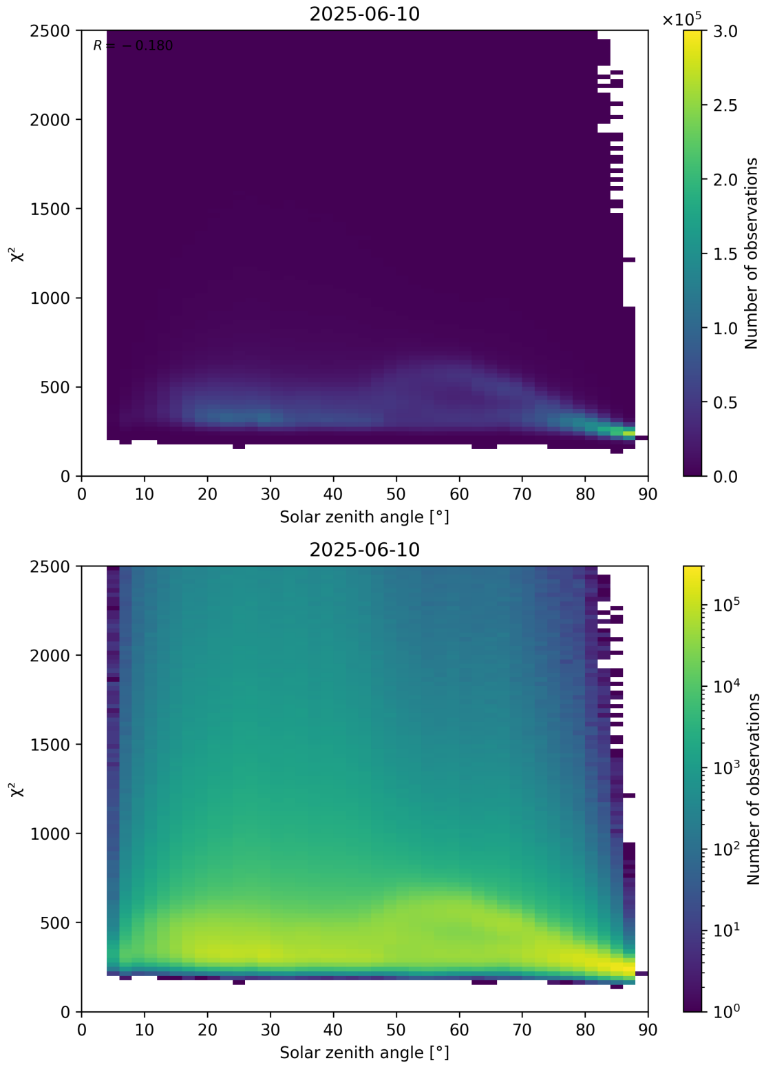
Figure 148: Scatter density plot of “Solar zenith angle” against “ \chi^2 ” for 2025-06-09 to 2025-06-11.
