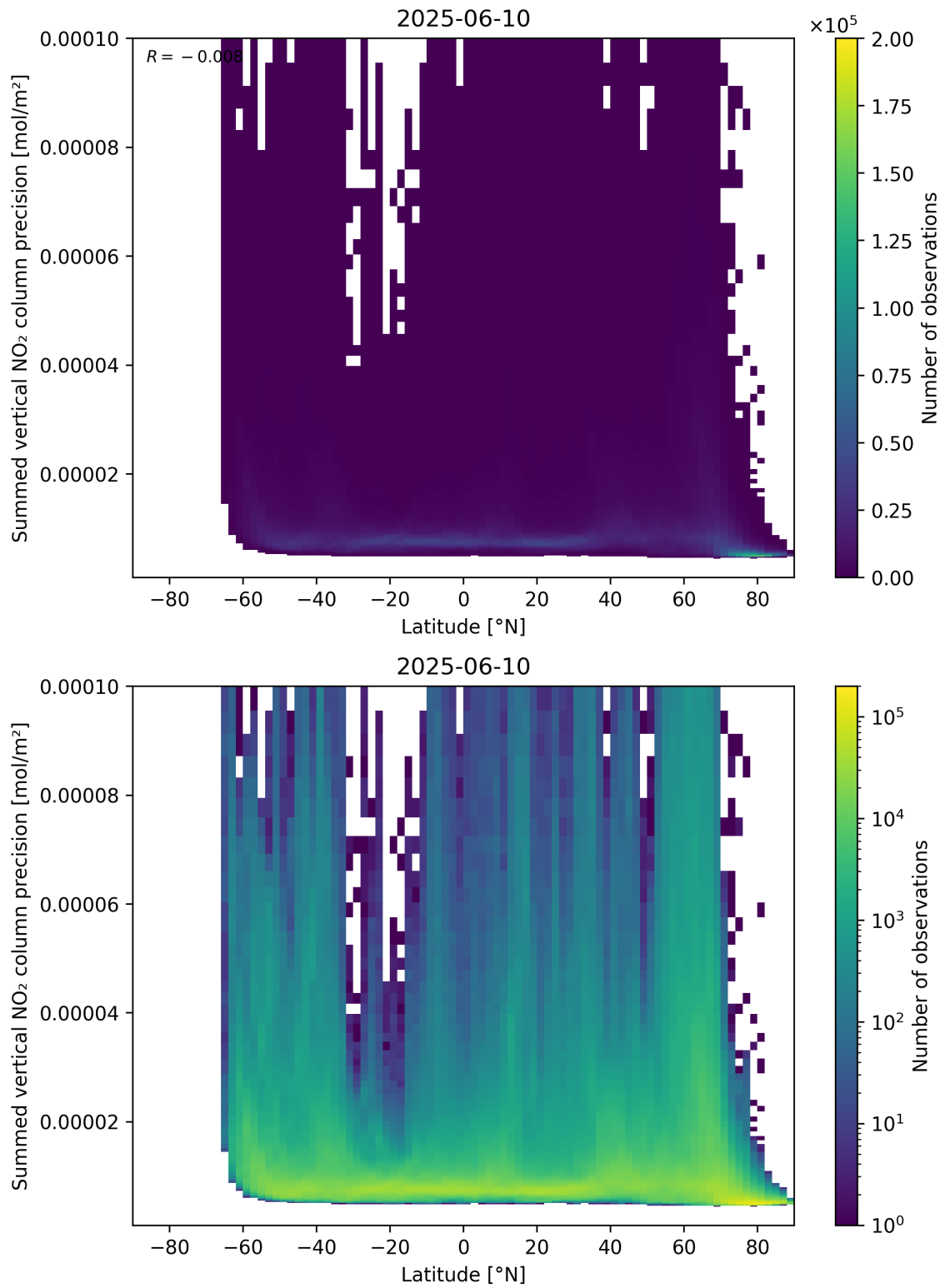
Figure 89: Scatter density plot of “Latitude” against “Summed vertical NO 2 column precision” for 2025-06-09 to 2025-06-11.
