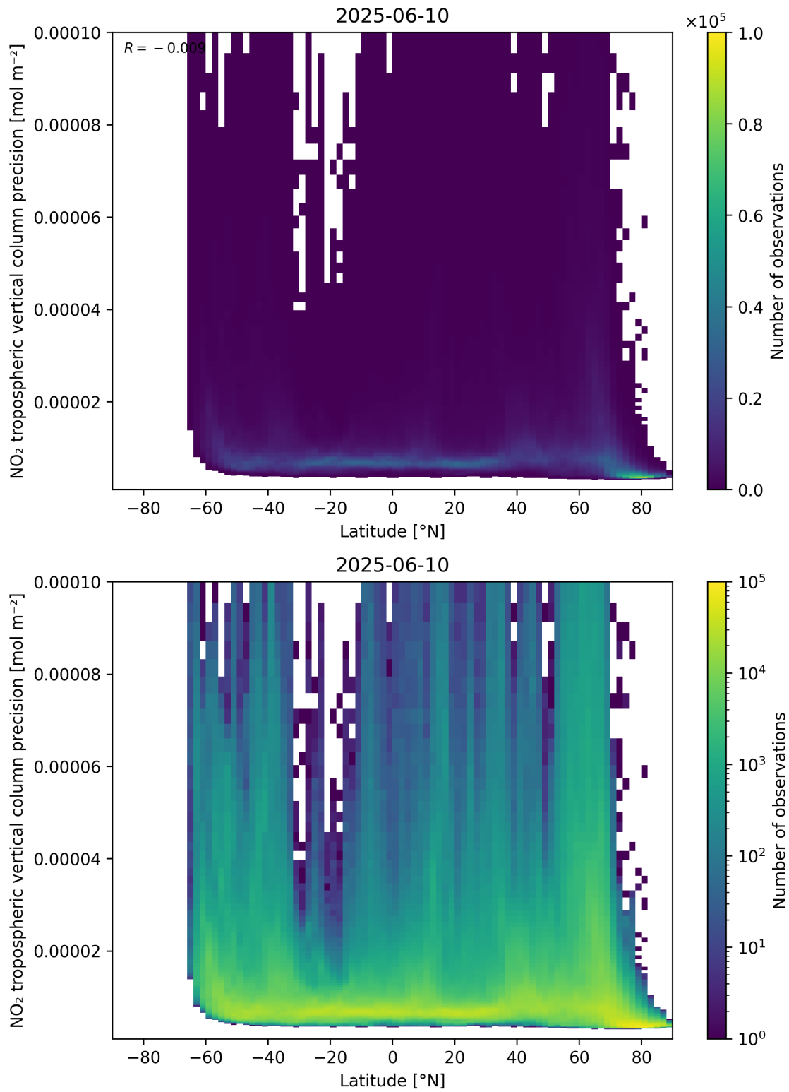
Figure 93: Scatter density plot of “Latitude” against “NO 2 tropospheric vertical column precision” for 2025-06-09 to 2025-06-11.
