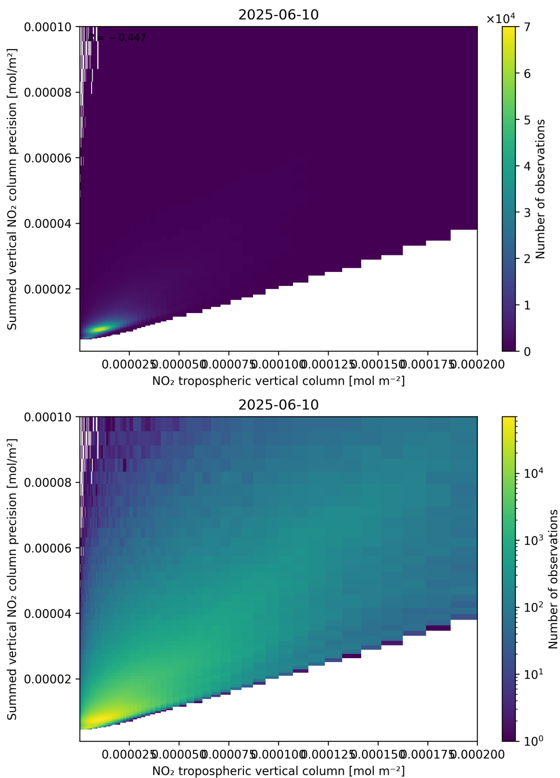
Figure 127: Scatter density plot of “NO 2 tropospheric vertical column” against “Summed vertical NO 2 column precision” for 2025-06-09 to 2025-06-11.
