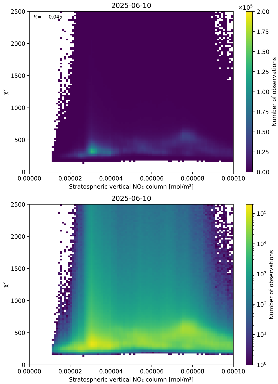
Figure 97: Scatter density plot of “Stratospheric vertical NO 2 column” against “ \chi^2 ” for 2025-06-09 to 2025-06-11.
