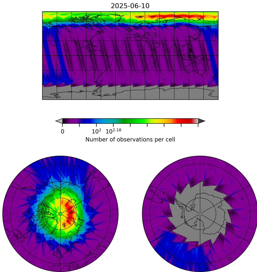
Figure 10: Map of the number of observations for 2025-06-09 to 2025-06-11
