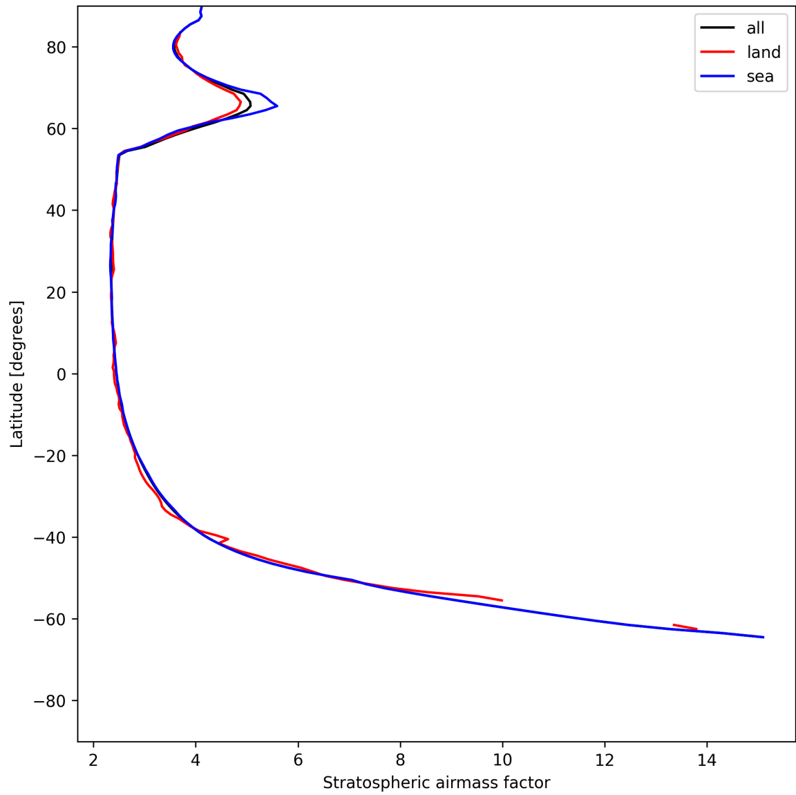
Figure 27: Zonal average of “Stratospheric airmass factor” for 2025-06-09 to 2025-06-11.
