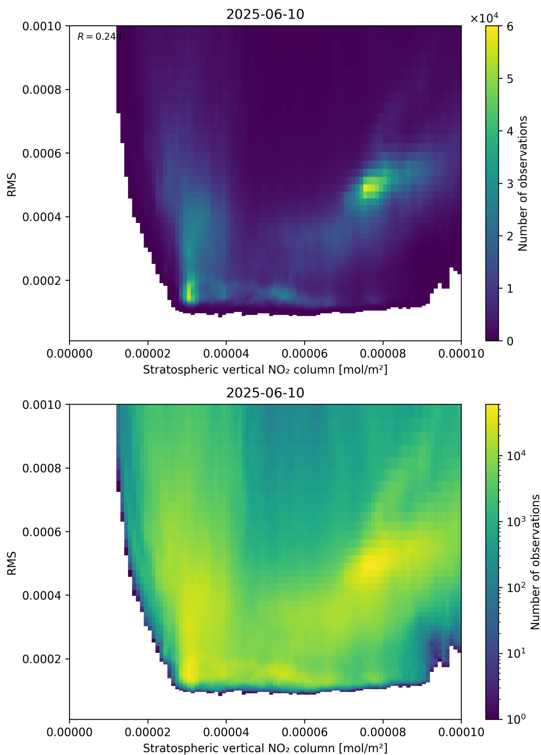
Figure 102: Scatter density plot of “Stratospheric vertical NO 2 column” against “RMS” for 2025-06-09 to 2025-06-11.
