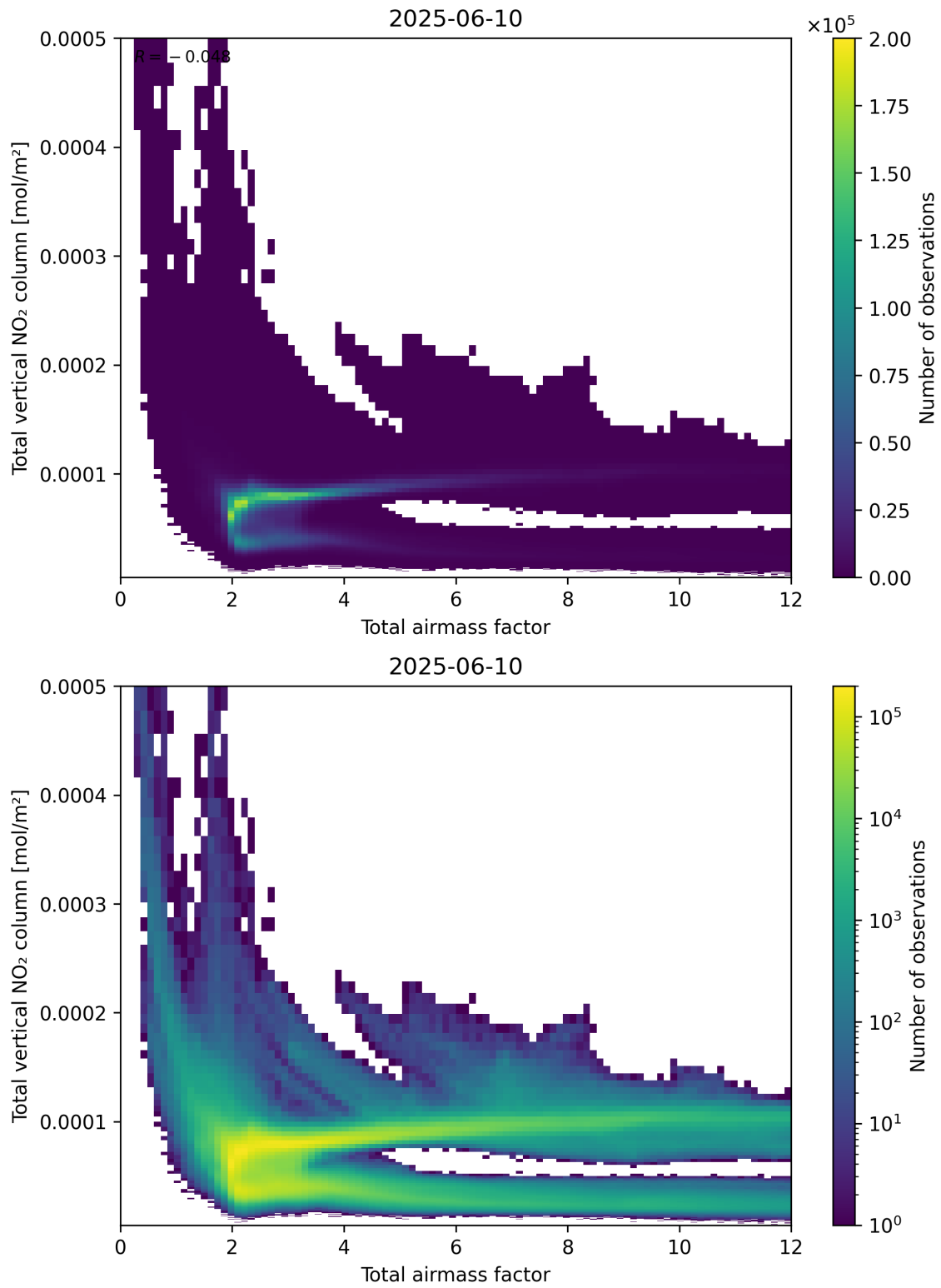
Figure 67: Scatter density plot of “Total airmass factor” against “Total vertical NO 2 column” for 2025-06-09 to 2025-06-11.
