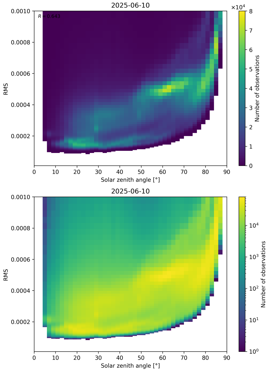
Figure 157: Scatter density plot of “Solar zenith angle” against “RMS” for 2025-06-09 to 2025-06-11.
