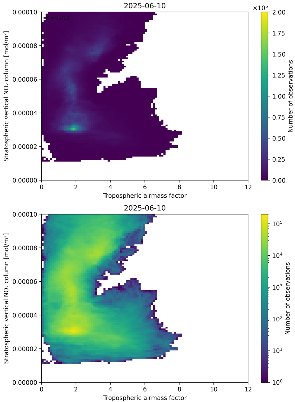
Figure 74: Scatter density plot of “Tropospheric air mass factor” against “Stratospheric vertical NO 2 column” for 2025-06-09 to 2025-06-11.
