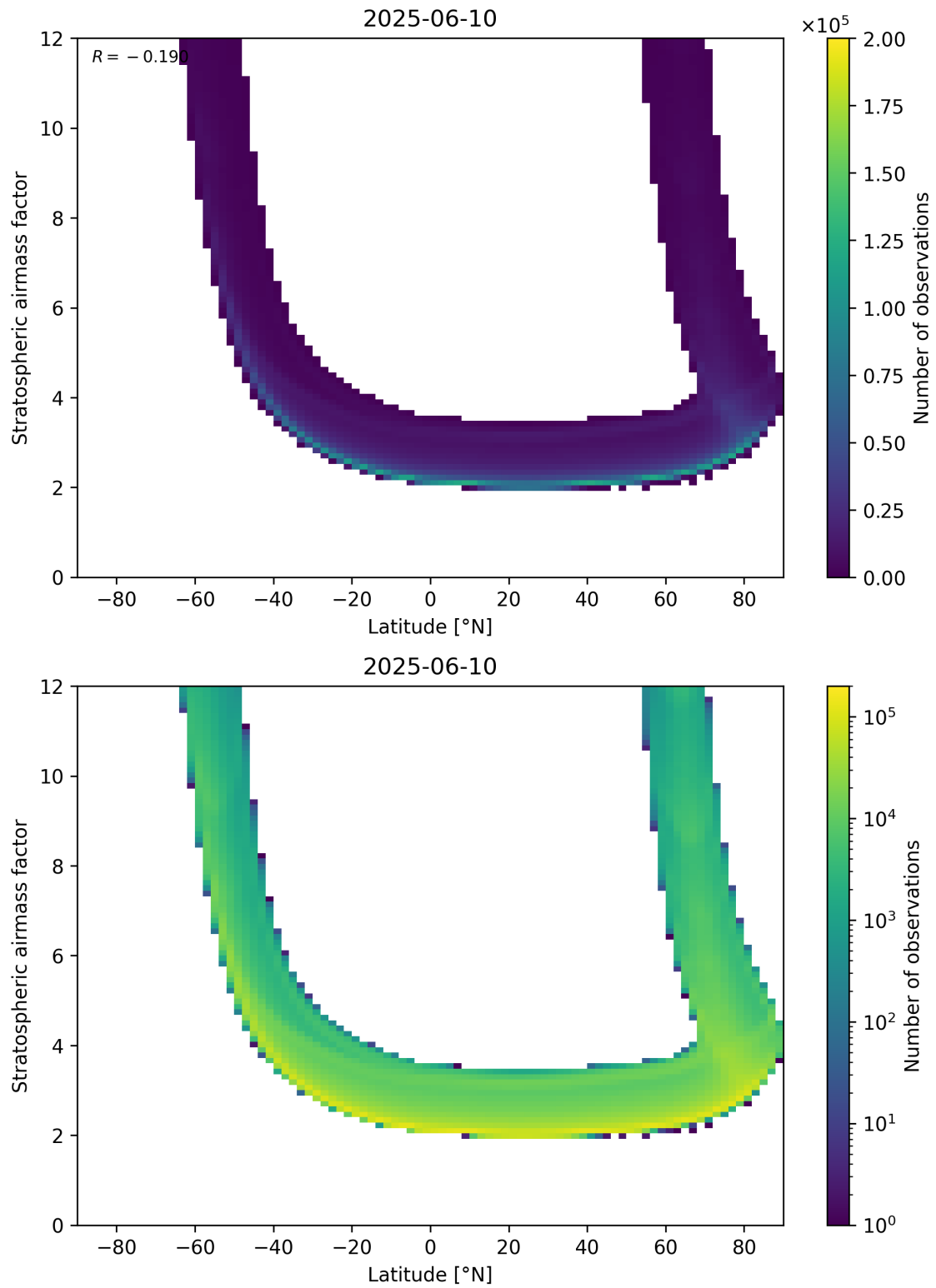
Figure 83: Scatter density plot of “Latitude” against “Stratospheric air mass factor” for 2025-06-09 to 2025-06-11.
