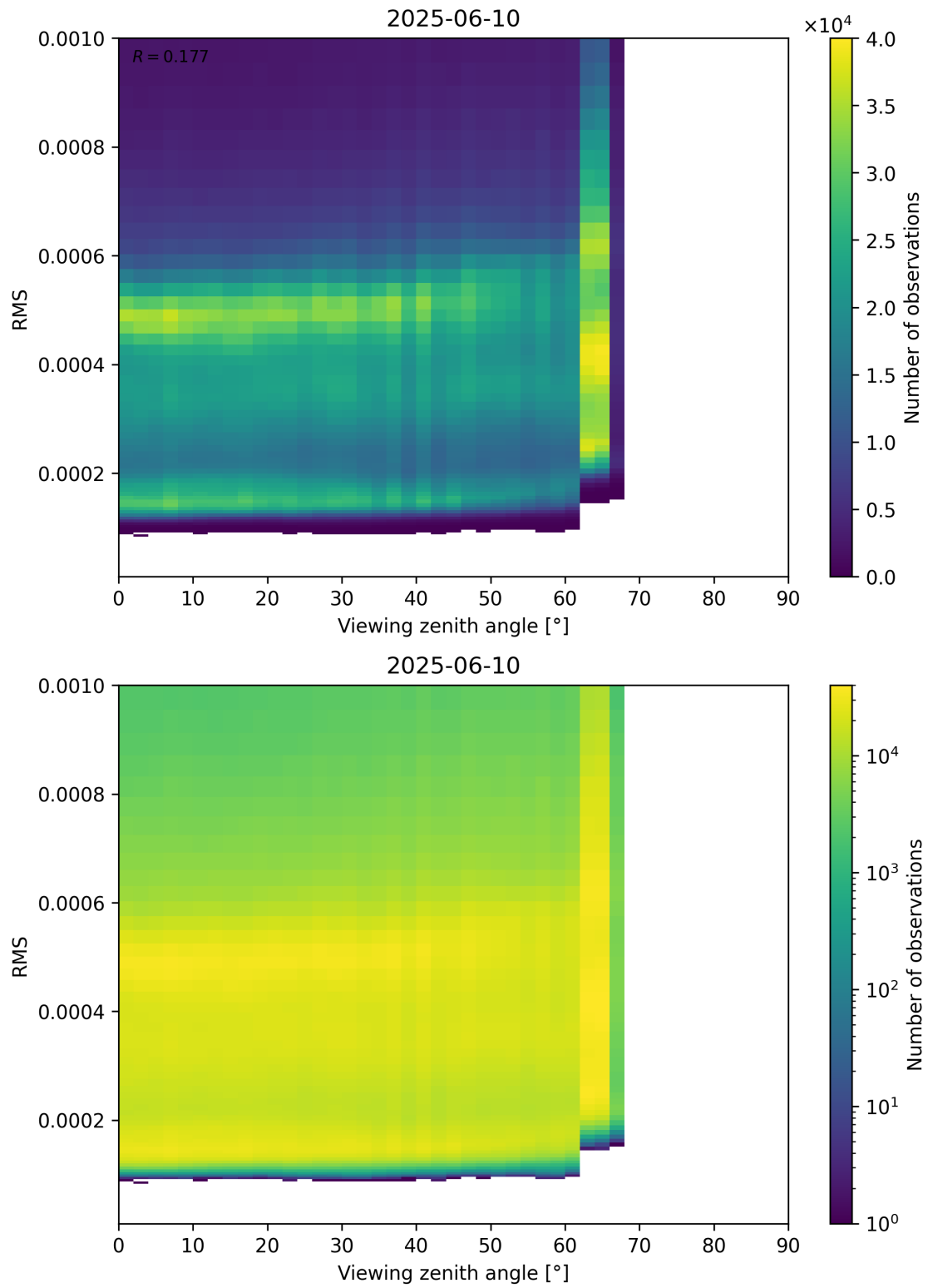
Figure 171: Scatter density plot of “Viewing zenith angle” against “RMS” for 2025-06-09 to 2025-06-11.
