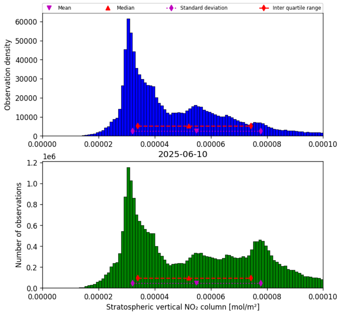
Figure 36: Histogram of “Stratospheric vertical NO 2 column” for 2025-06-09 to 2025-06-11
