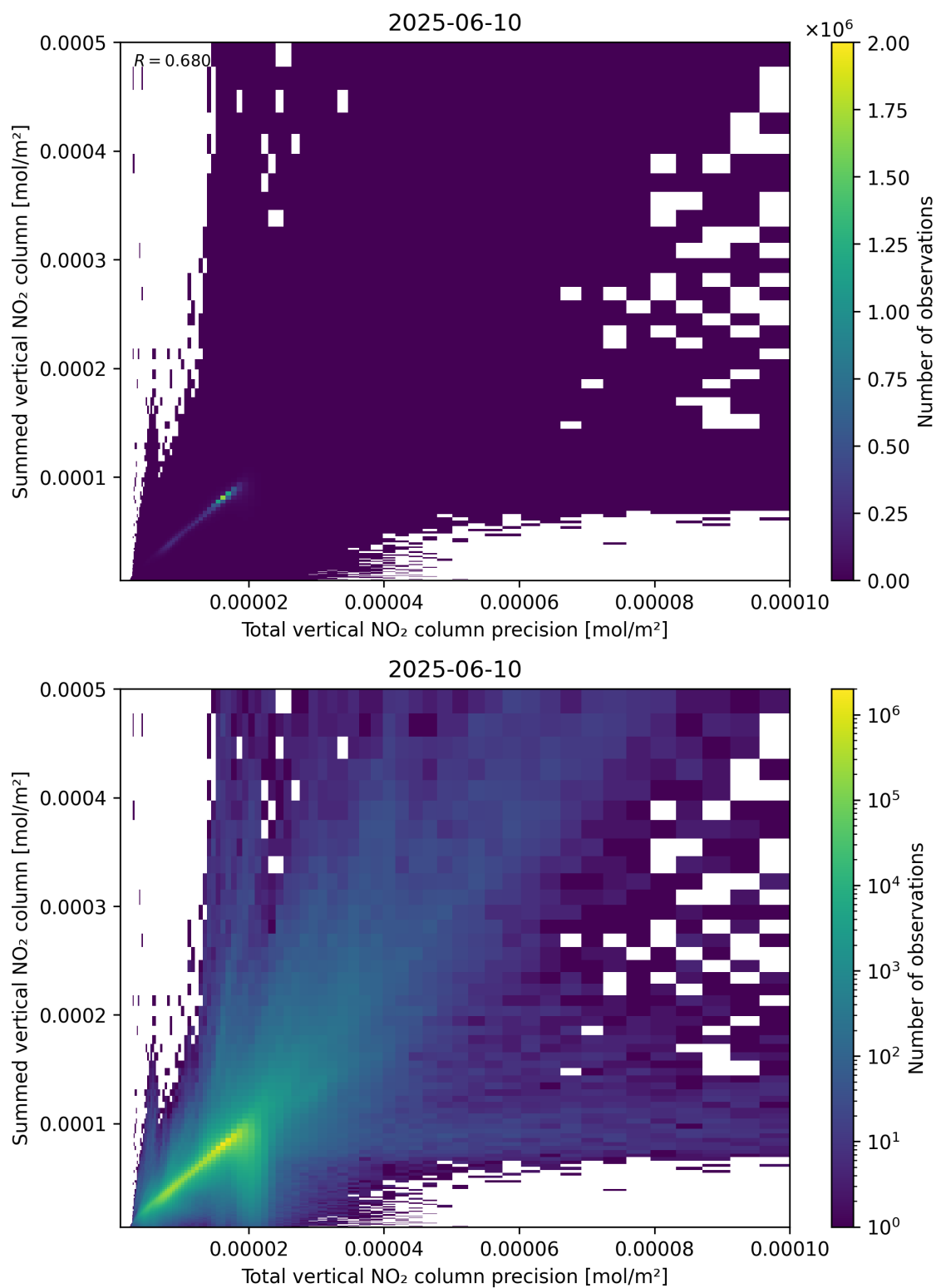
Figure 117: Scatter density plot of “Total vertical NO 2 column precision” against “Summed vertical NO 2 column” for 2025-06-09 to 2025-06-11.
