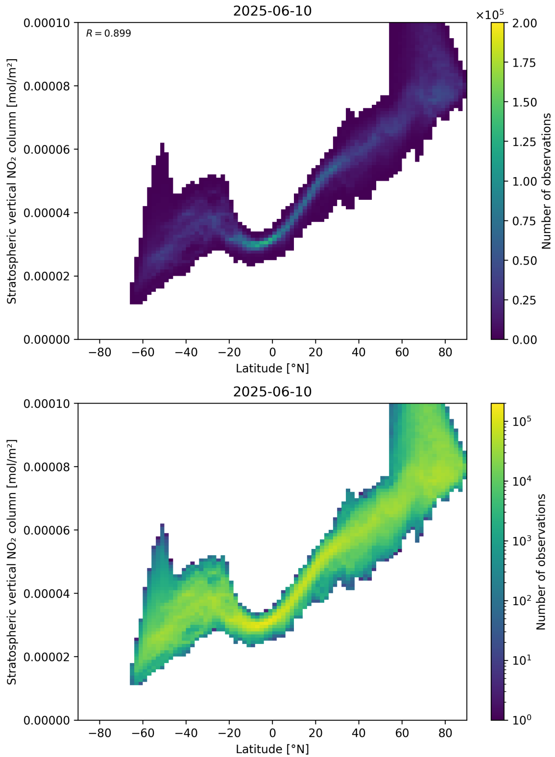
Figure 87: Scatter density plot of “Latitude” against “Stratospheric vertical \text{NO}_2 column” for 2025-06-09 to 2025-06-11.
