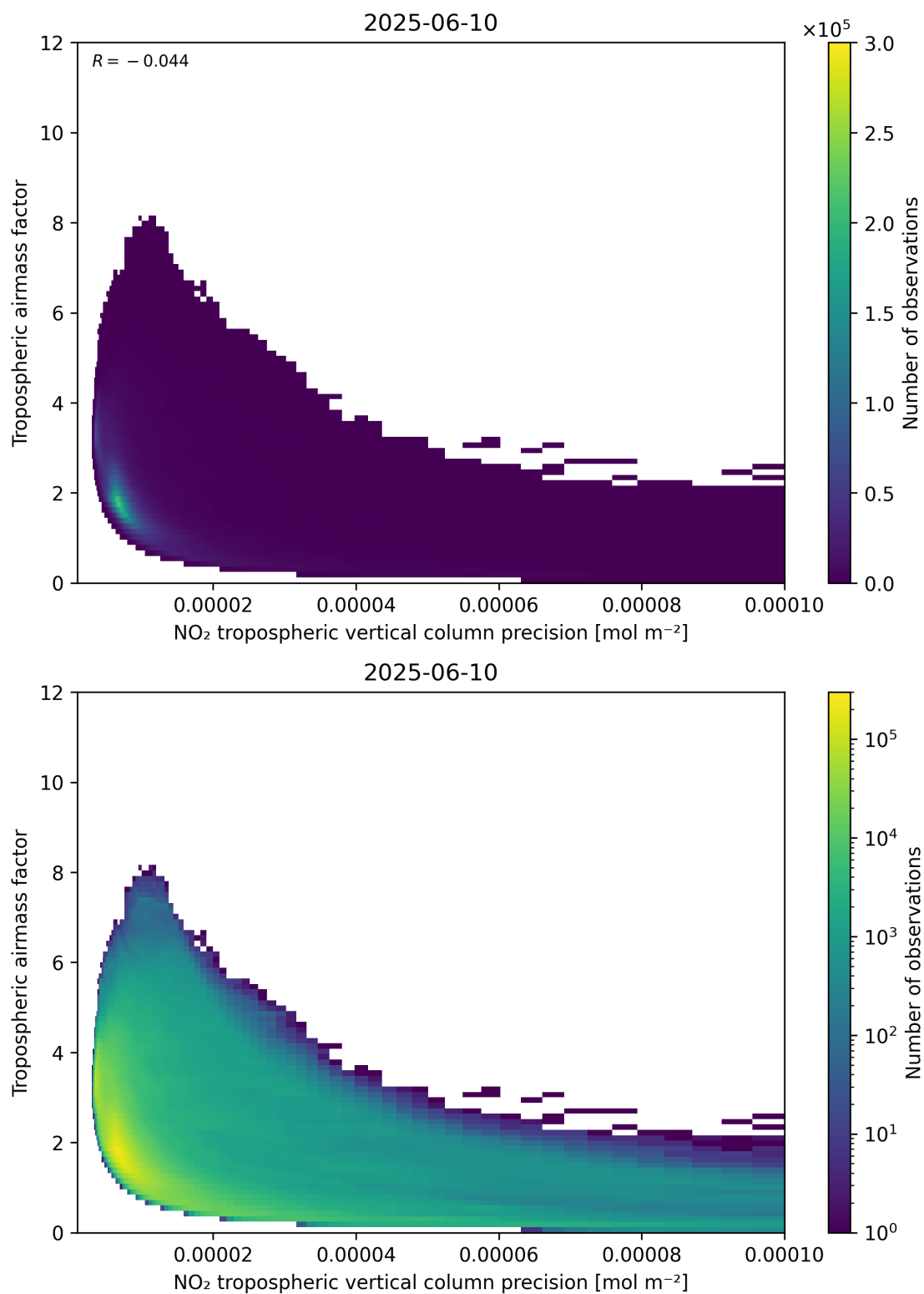
Figure 133: Scatter density plot of “NO 2 tropospheric vertical column precision” against “Tropospheric airmass factor” for 2025-06-09 to 2025-06-11.
