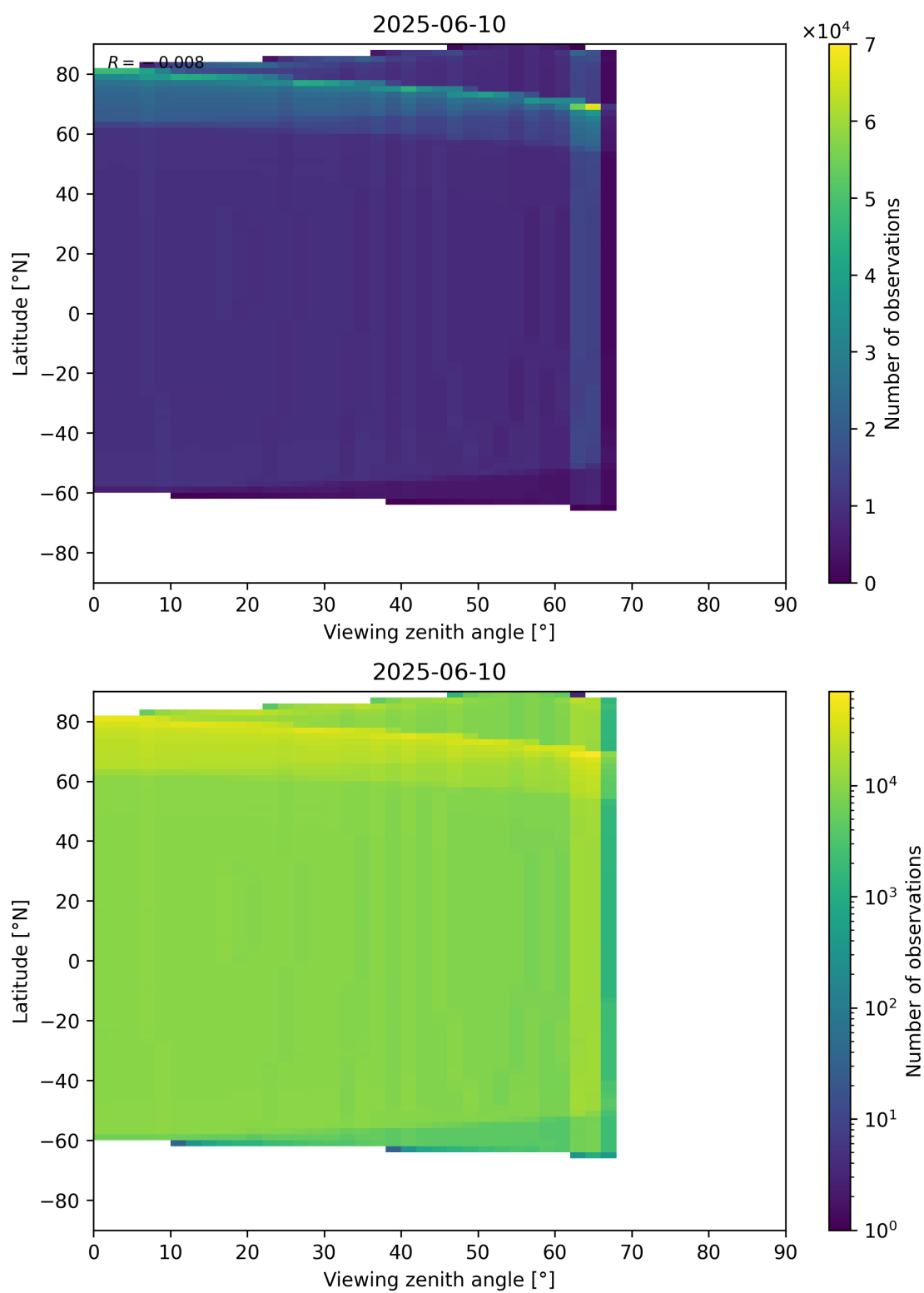
Figure 163: Scatter density plot of “Viewing zenith angle” against “Latitude” for 2025-06-09 to 2025-06-11.
