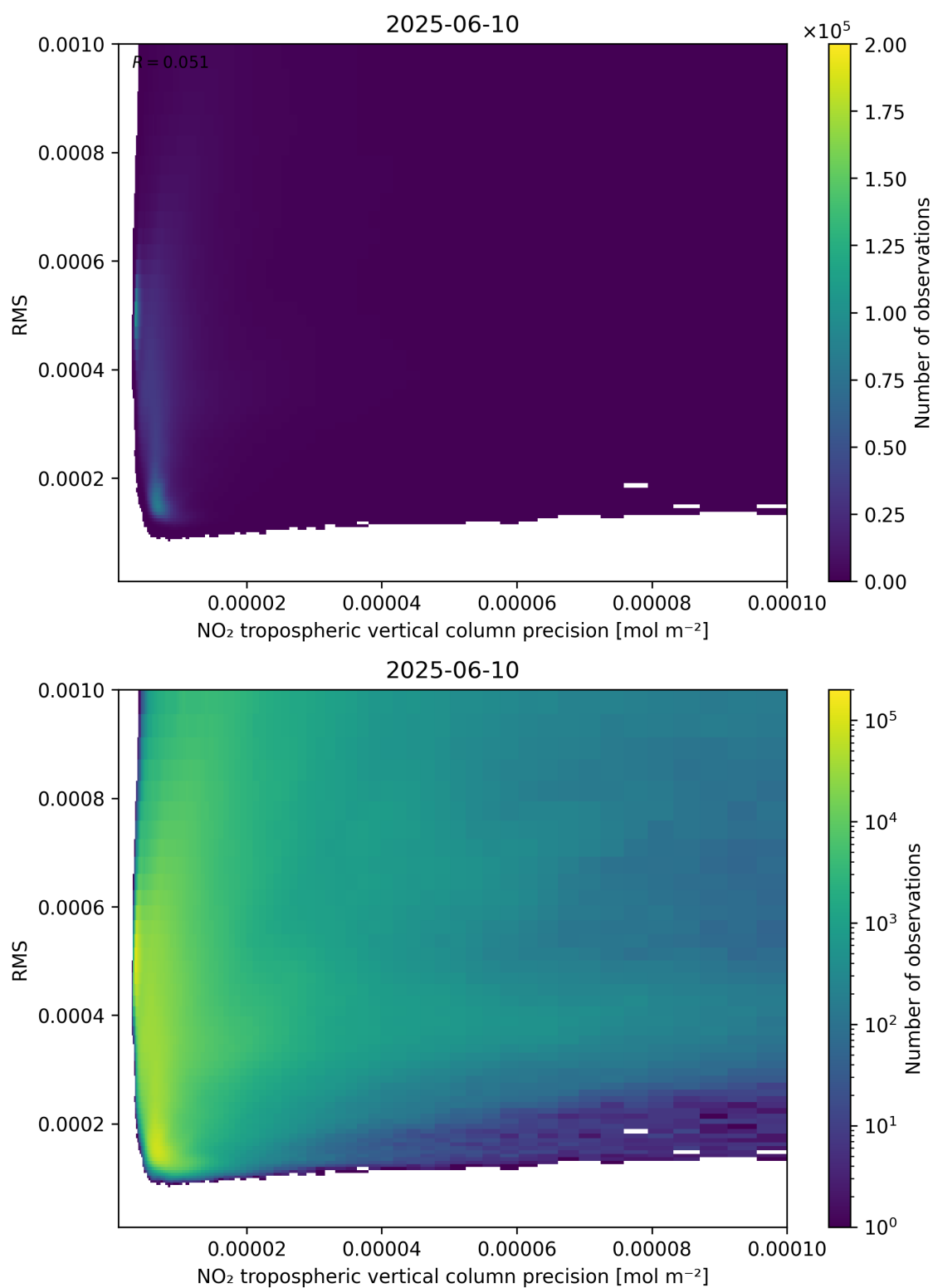
Figure 140: Scatter density plot of “NO 2 tropospheric vertical column precision” against “RMS” for 2025-06-09 to 2025-06-11.
