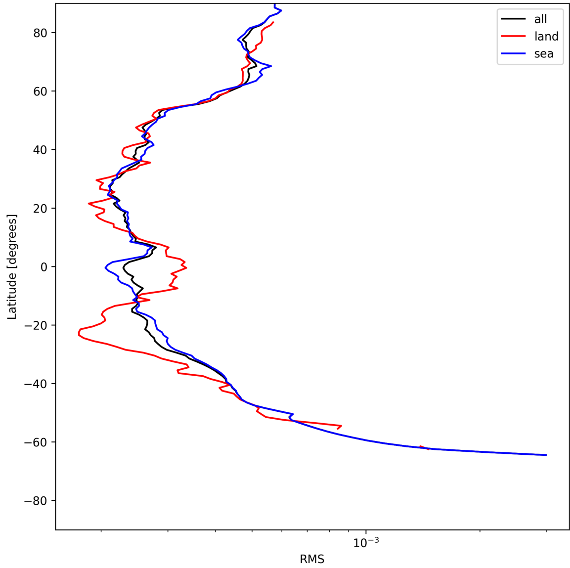
Figure 26: Zonal average of “RMS” for 2025-06-09 to 2025-06-11.
