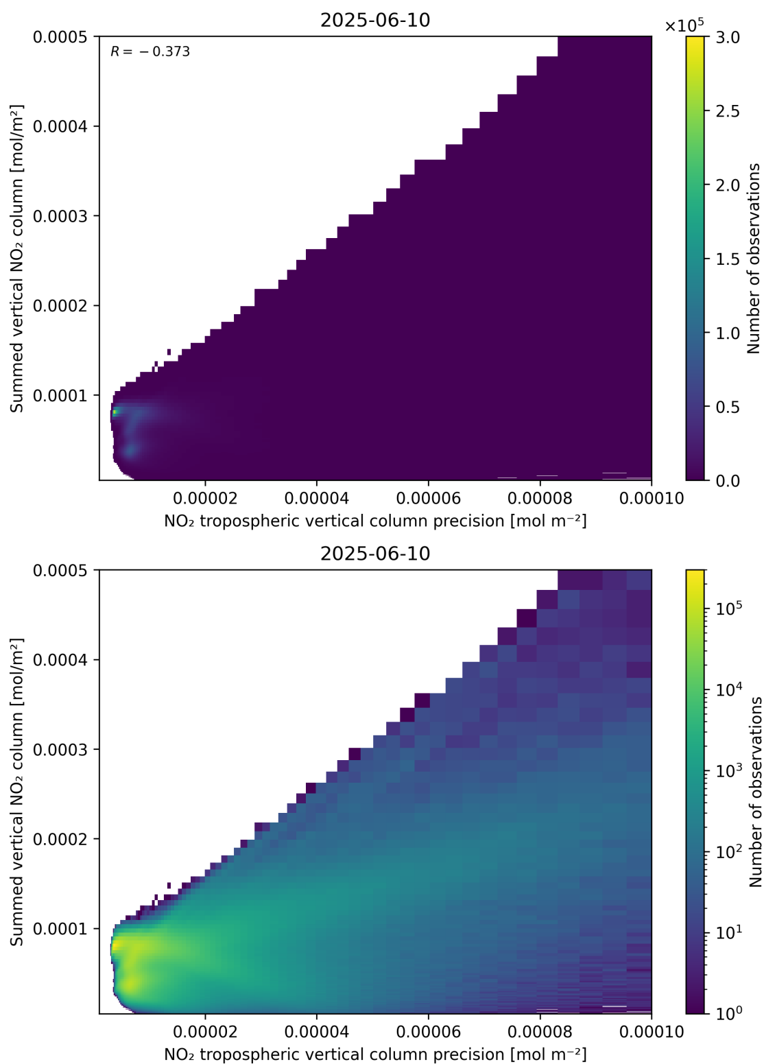
Figure 136: Scatter density plot of “NO 2 tropospheric vertical column precision” against “Summed vertical NO 2 column” for 2025-06-09 to 2025-06-11.
