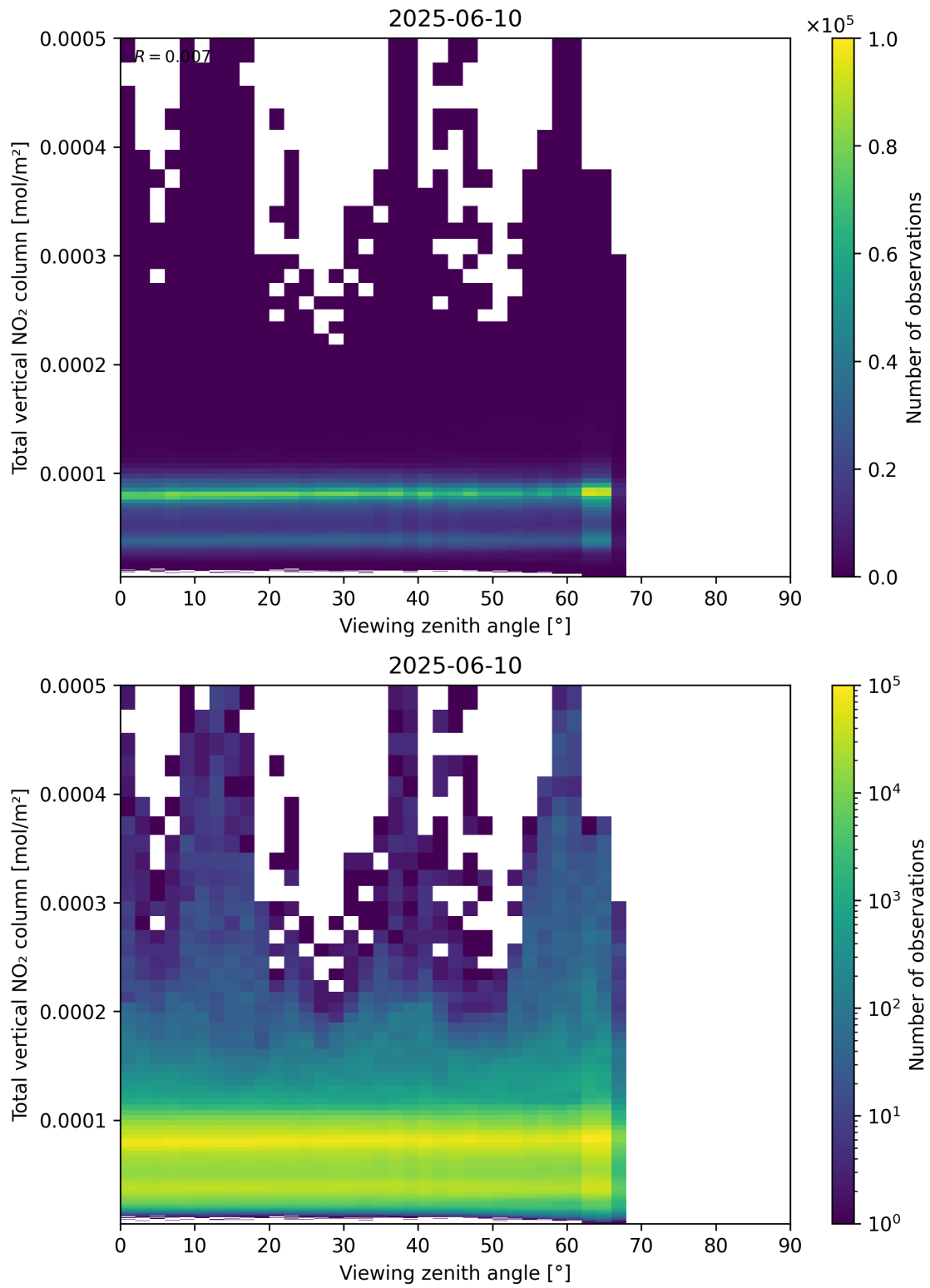
Figure 167: Scatter density plot of “Viewing zenith angle” against “Total vertical NO 2 column” for 2025-06-09 to 2025-06-11.
