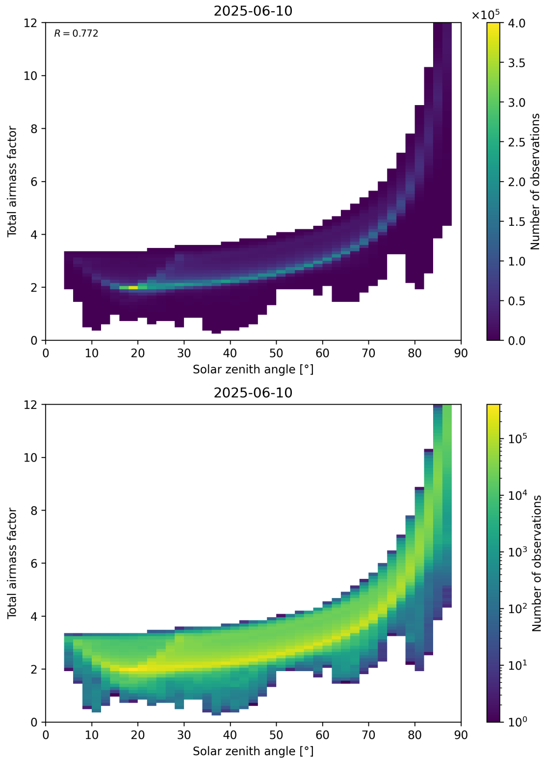
Figure 146: Scatter density plot of “Solar zenith angle” against “Total air mass factor” for 2025-06-09 to 2025-06-11.
