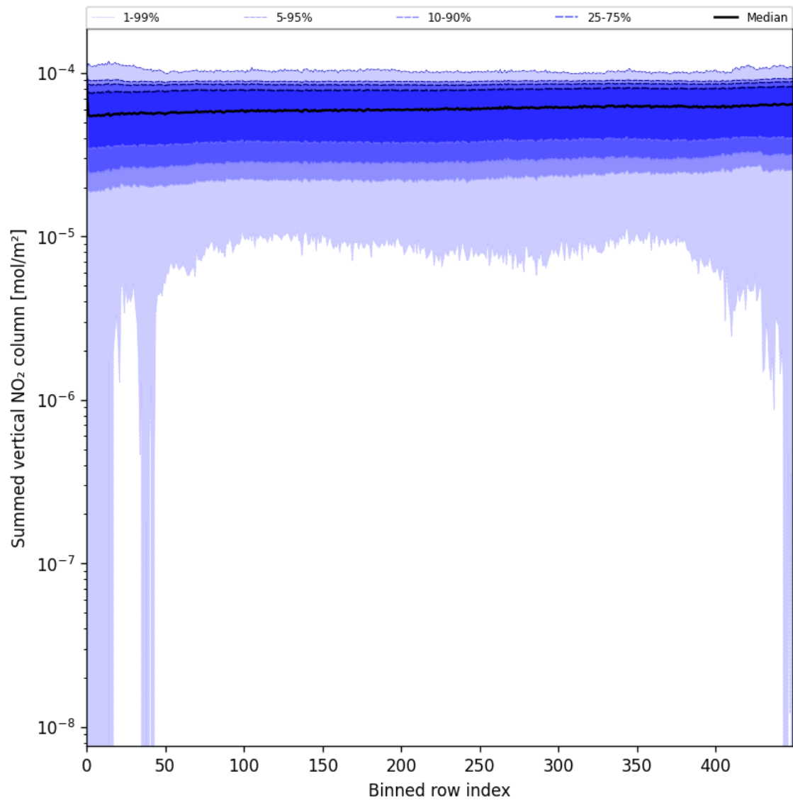
Figure 57: Along track statistics of “Summed vertical NO 2 column” for 2025-06-09 to 2025-06-11
