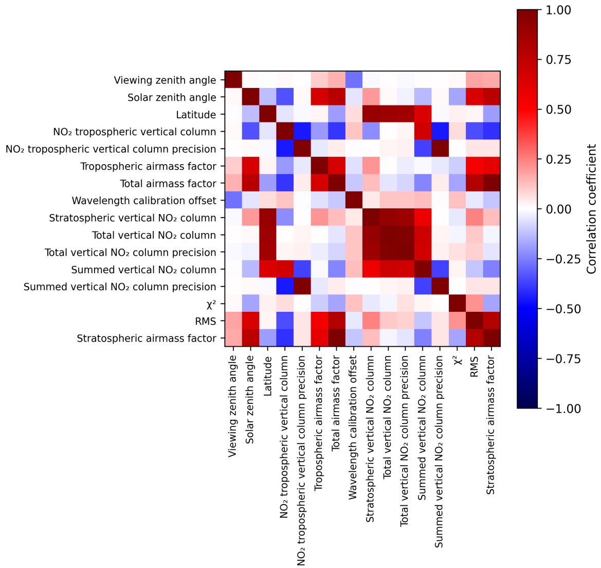
Figure 2: Map of correlation matrix for 2025-06-09 to 2025-06-11.
