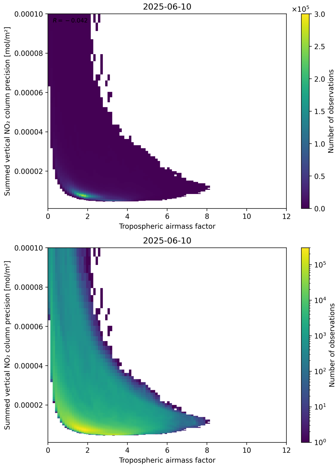
Figure 76: Scatter density plot of “Tropospheric air mass factor” against “Summed vertical NO 2 column precision” for 2025-06-09 to 2025-06-11.
