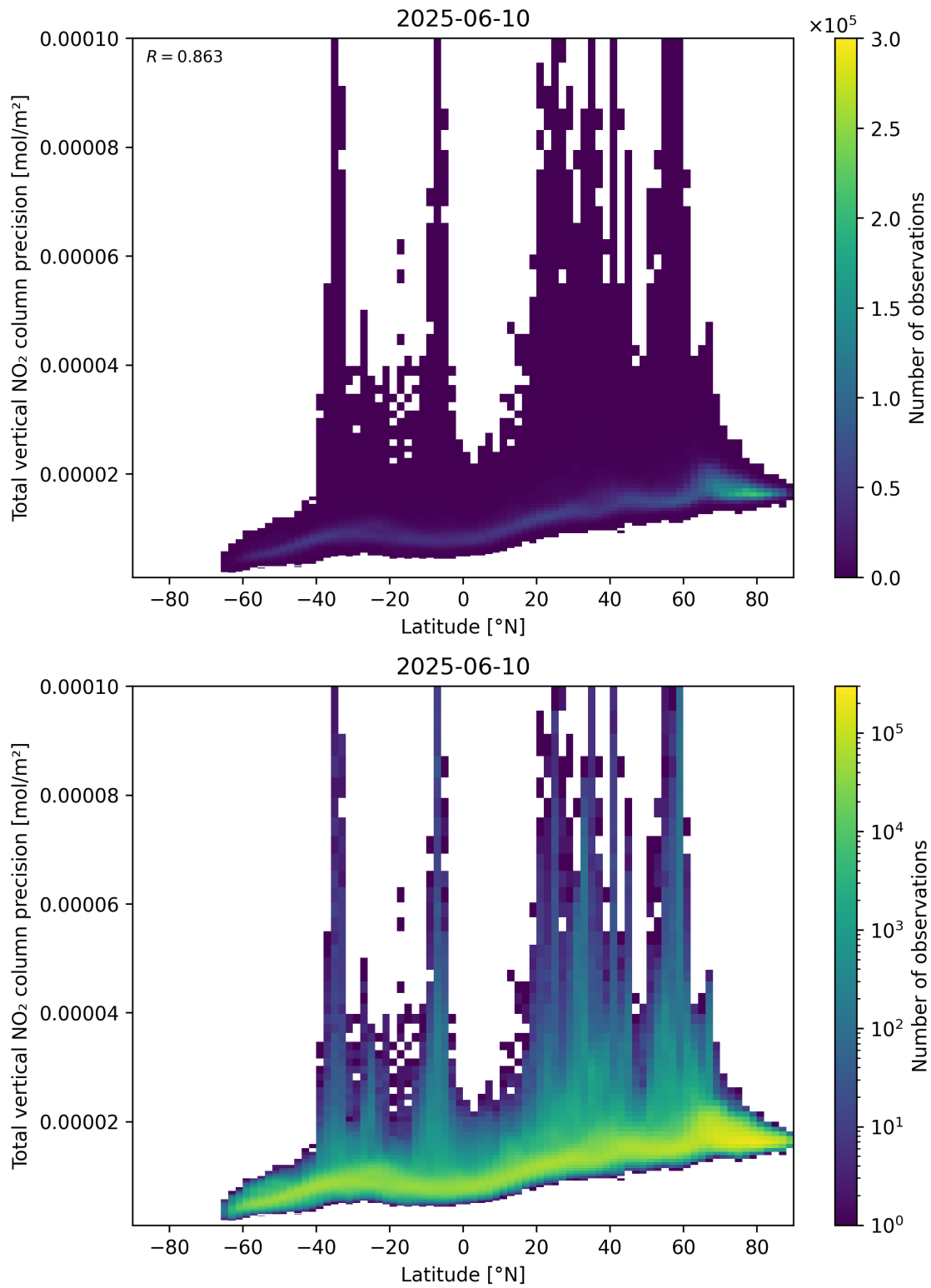
Figure 91: Scatter density plot of “Latitude” against “Total vertical NO 2 column precision” for 2025-06-09 to 2025-06-11.
