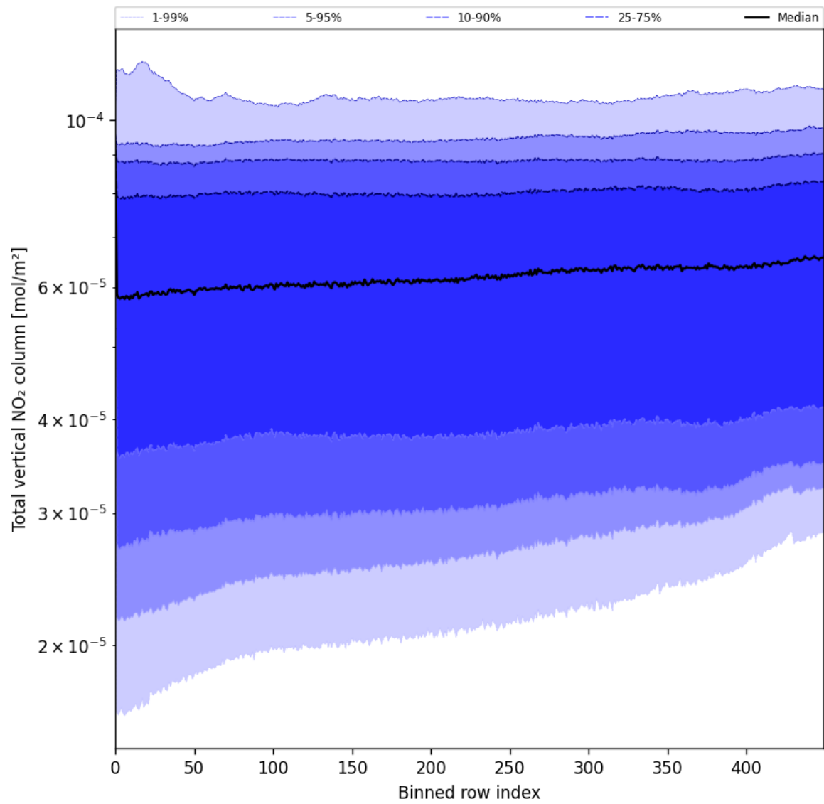
Figure 55: Along track statistics of “Total vertical NO 2 column” for 2025-06-09 to 2025-06-11
