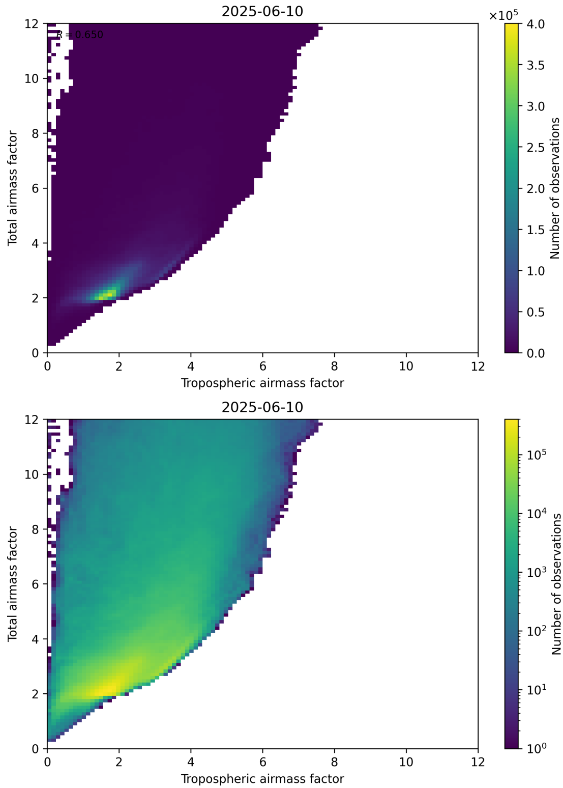
Figure 72: Scatter density plot of “Tropospheric airmass factor” against “Total airmass factor” for 2025-06-09 to 2025-06-11.
