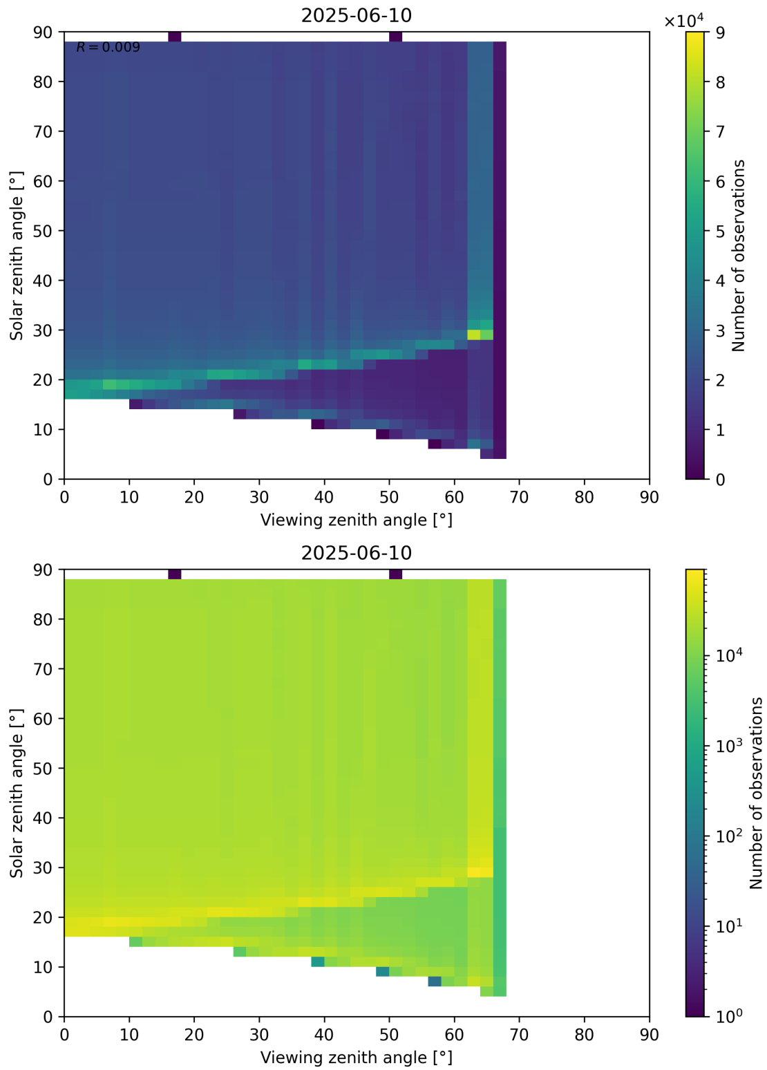
Figure 172: Scatter density plot of “Viewing zenith angle” against “Solar zenith angle” for 2025-06-09 to 2025-06-11.
