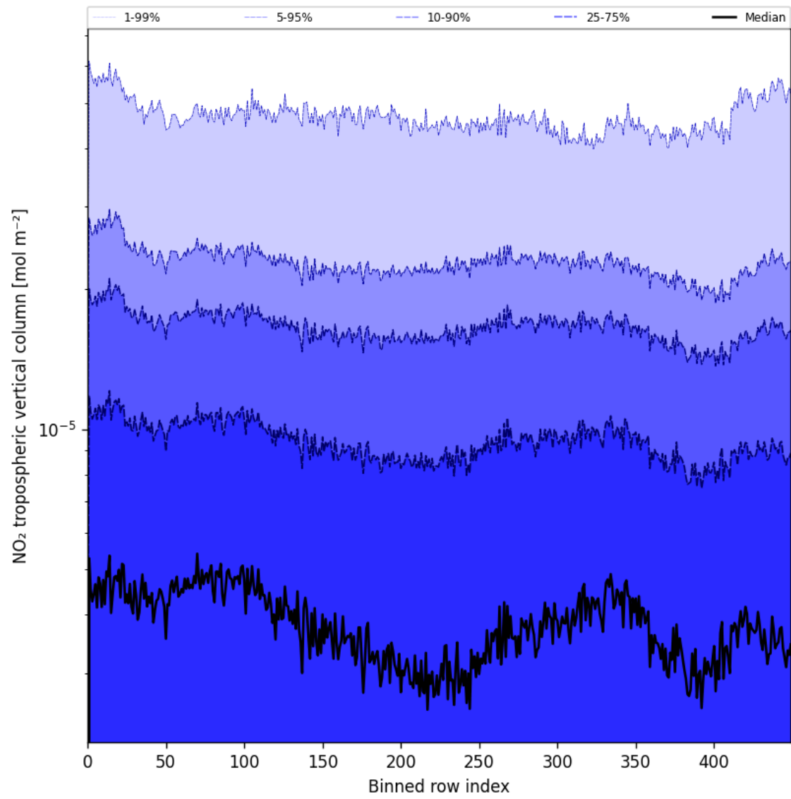
Figure 46: Along track statistics of “NO 2 tropospheric vertical column” for 2025-06-09 to 2025-06-11
