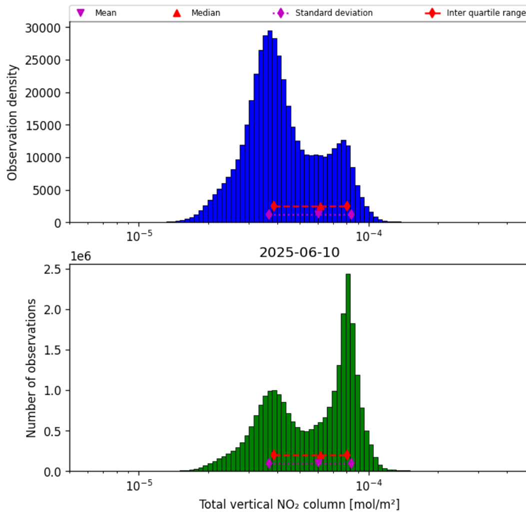
Figure 38: Histogram of “Total vertical NO 2 column” for 2025-06-09 to 2025-06-11
