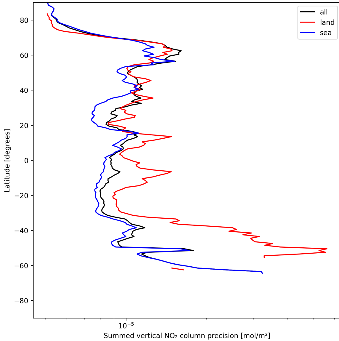
Figure 24: Zonal average of “Summed vertical NO 2 column precision” for 2025-06-09 to 2025-06-11.
