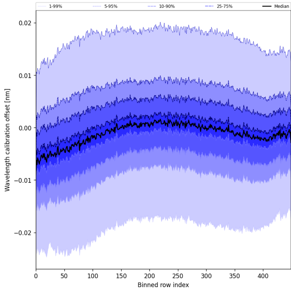
Figure 52: Along track statistics of “Wavelength calibration offset” for 2025-06-09 to 2025-06-11
