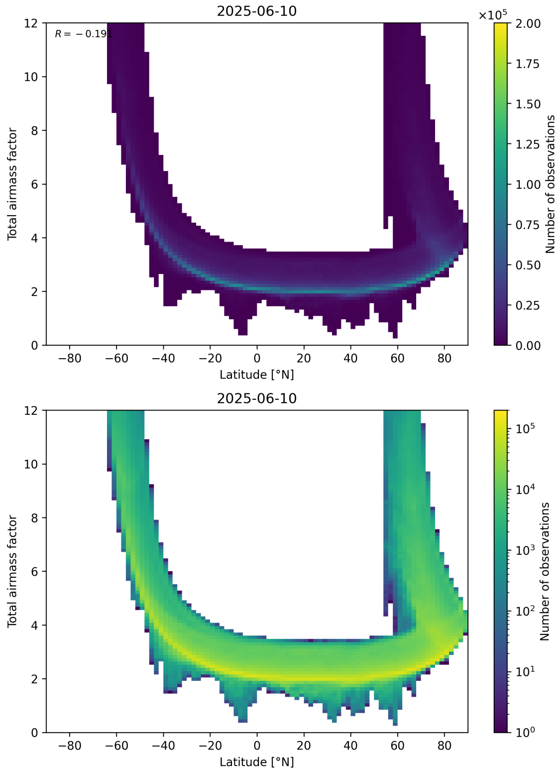
Figure 84: Scatter density plot of “Latitude” against “Total airmass factor” for 2025-06-09 to 2025-06-11.
