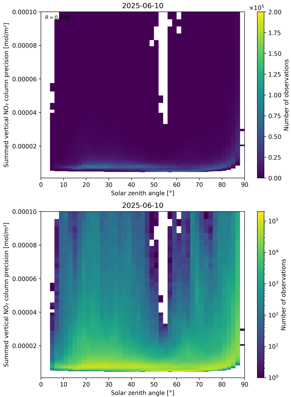
Figure 152: Scatter density plot of “Solar zenith angle” against “Summed vertical NO 2 column precision” for 2025-06-09 to 2025-06-11.
