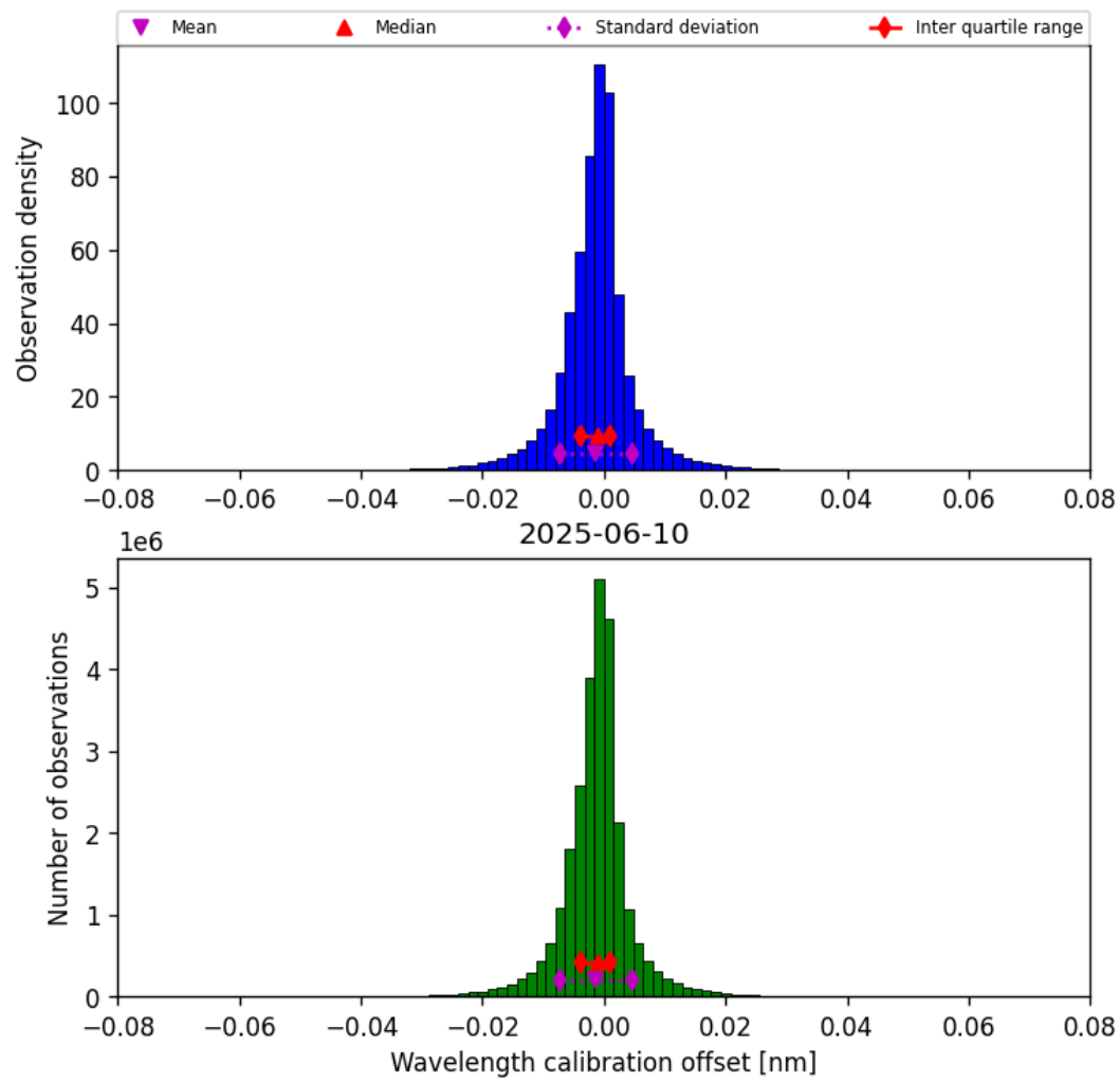
Figure 35: Histogram of “Wavelength calibration offset” for 2025-06-09 to 2025-06-11
