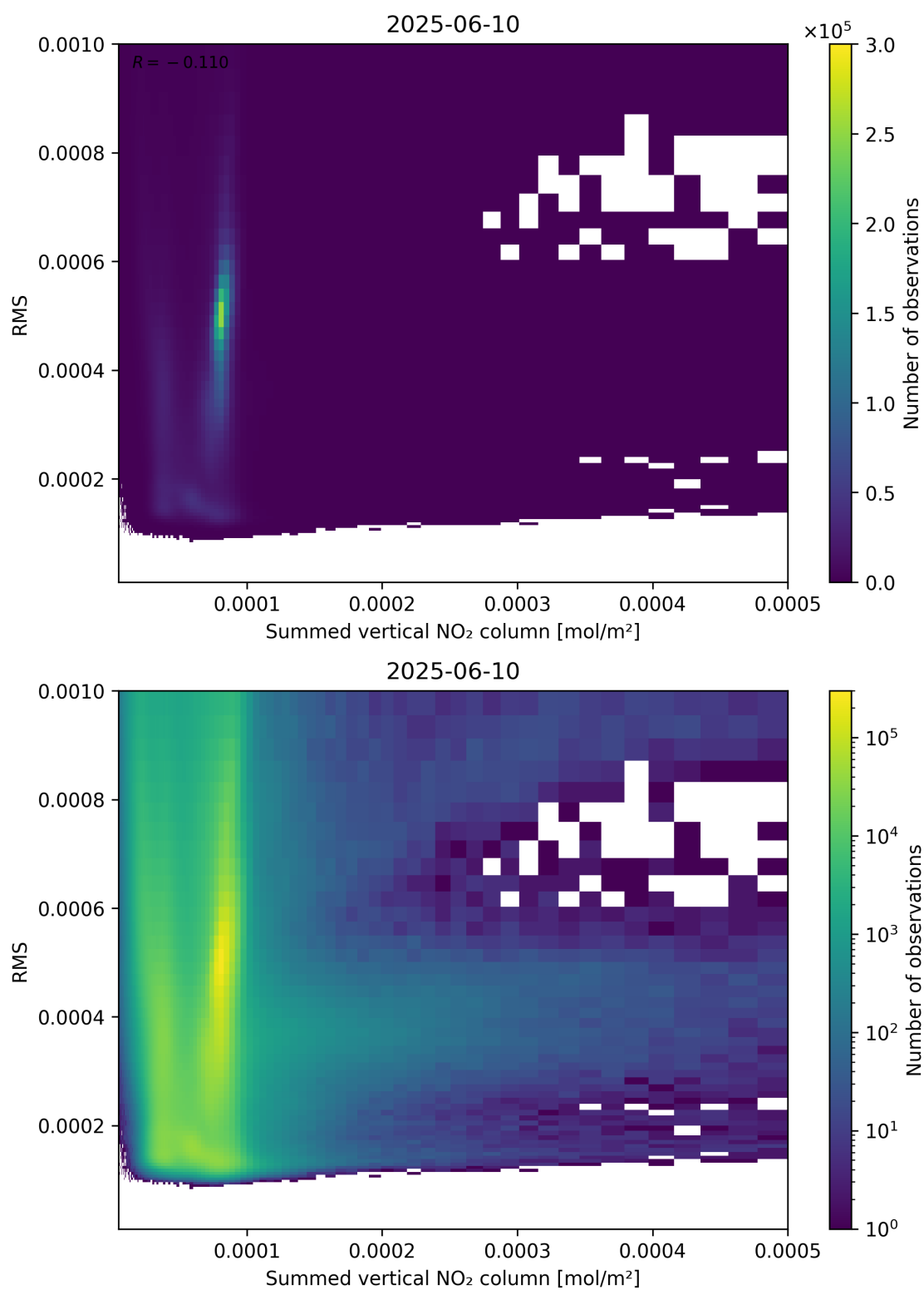
Figure 109: Scatter density plot of “Summed vertical NO 2 column” against “RMS” for 2025-06-09 to 2025-06-11.
