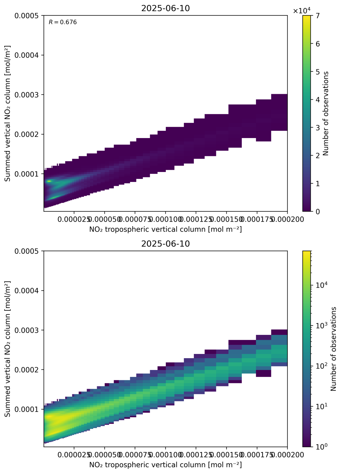
Figure 126: Scatter density plot of “NO 2 tropospheric vertical column” against “Summed vertical NO 2 column” for 2025-06-09 to 2025-06-11.
