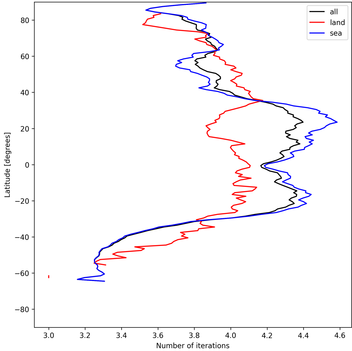
Figure 17: Zonal average of “Number of iterations” for 2025-06-09 to 2025-06-11.
