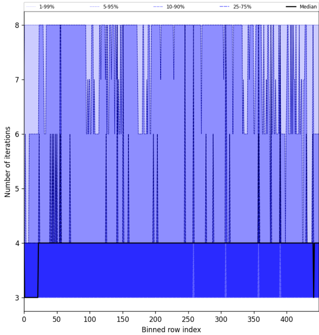
Figure 51: Along track statistics of “Number of iterations” for 2025-06-09 to 2025-06-11
