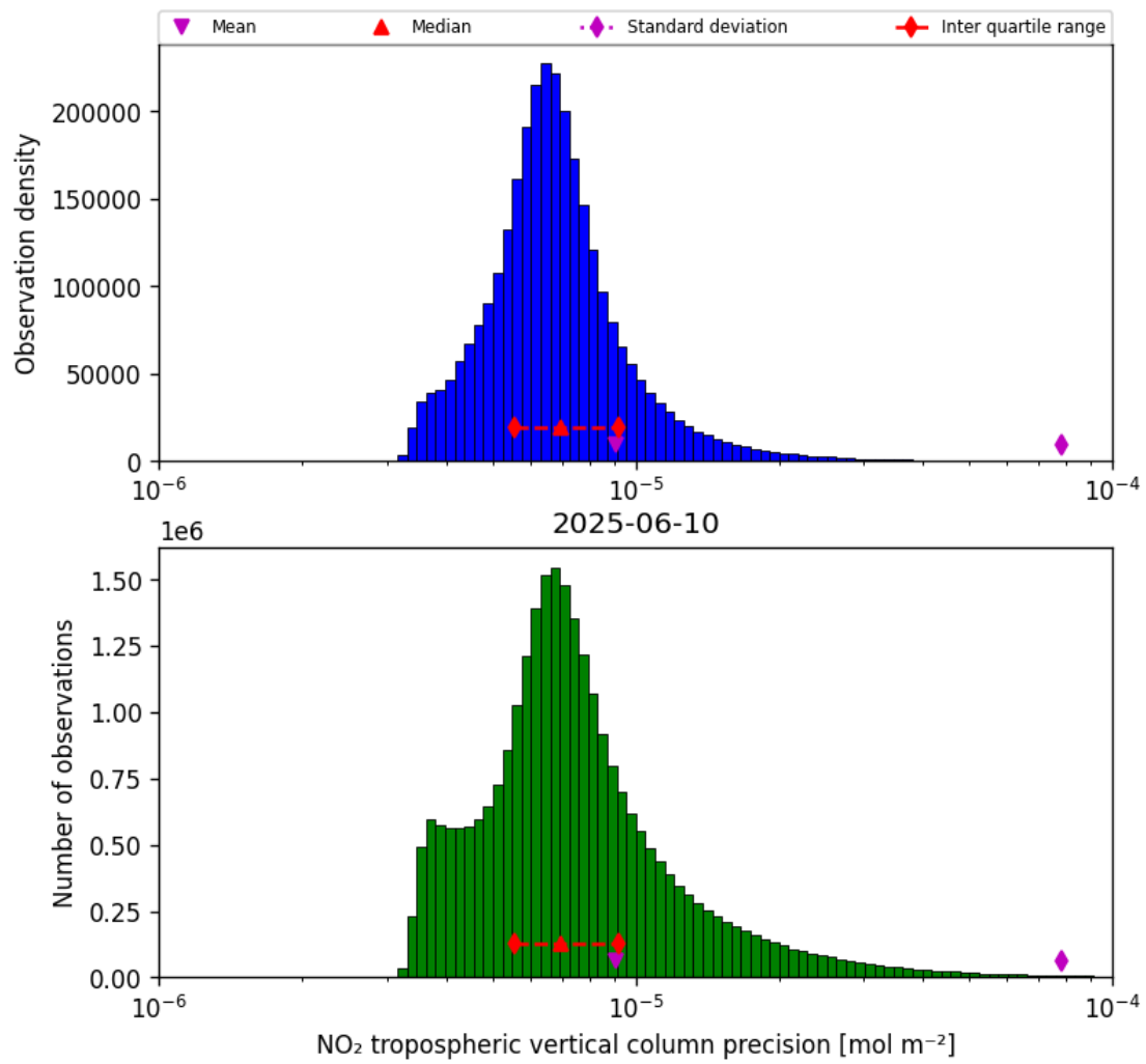
Figure 30: Histogram of “NO 2 tropospheric vertical column precision” for 2025-06-09 to 2025-06-11
