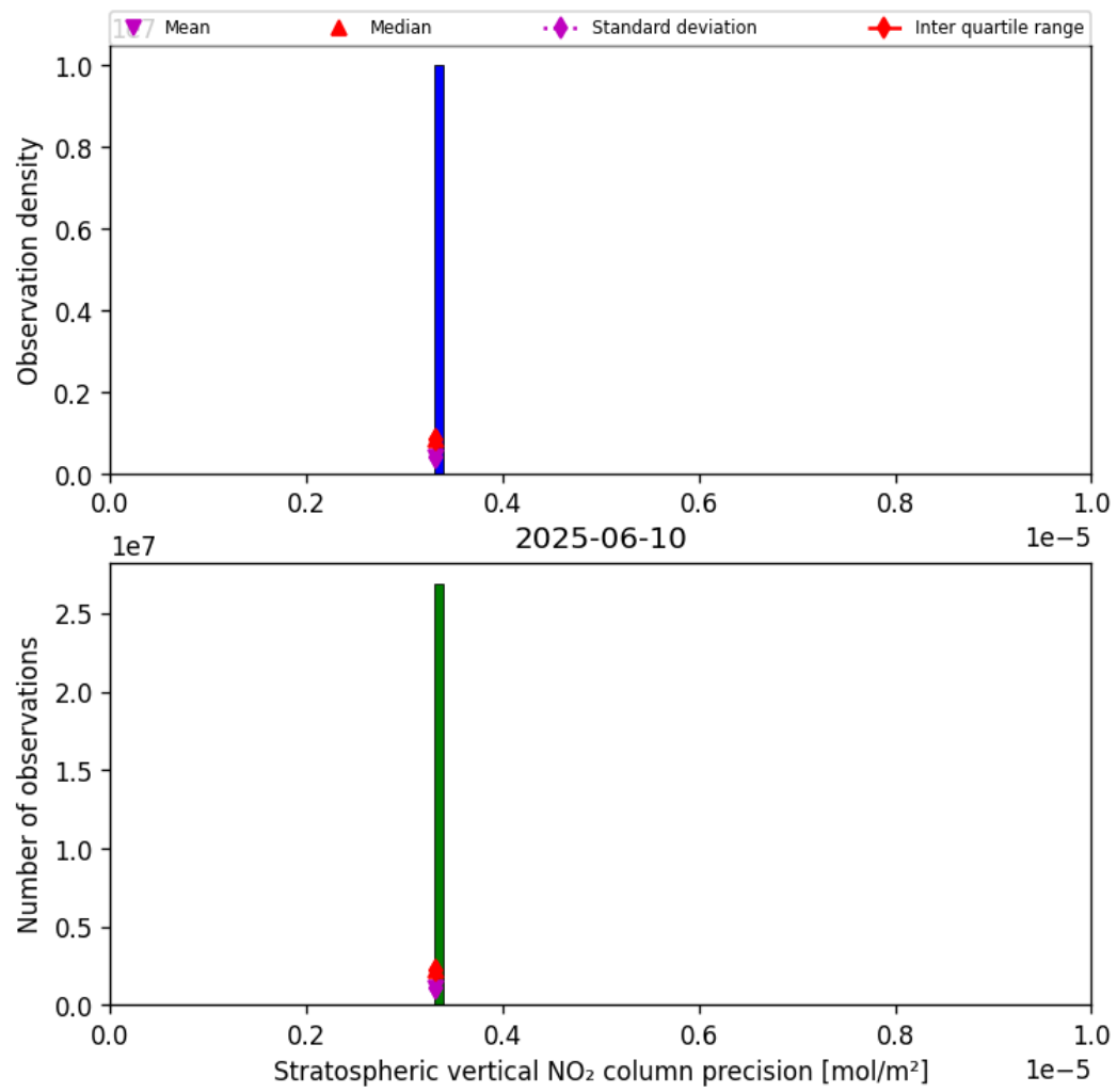
Figure 37: Histogram of “Stratospheric vertical NO 2 column precision” for 2025-06-09 to 2025-06-11
