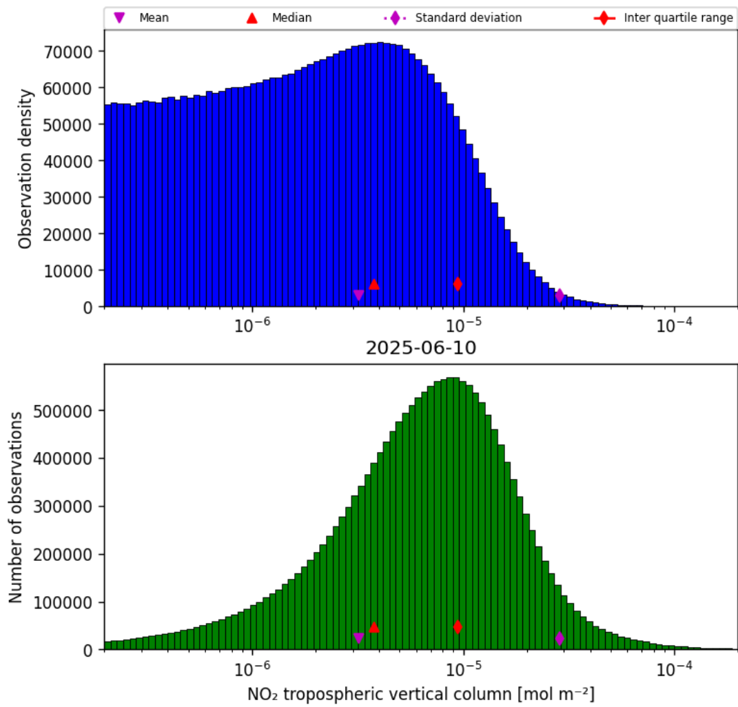
Figure 29: Histogram of “NO 2 tropospheric vertical column” for 2025-06-09 to 2025-06-11
