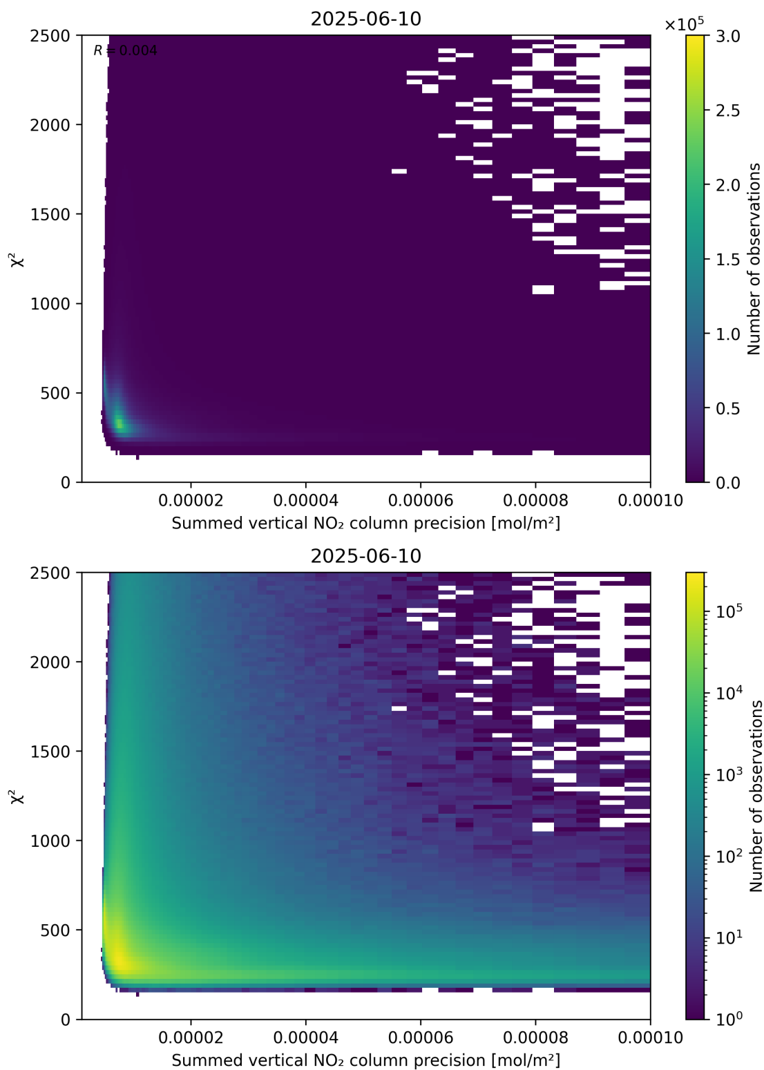
Figure 107: Scatter density plot of “Summed vertical NO 2 column precision” against “ \chi^2 ” for 2025-06-09 to 2025-06-11.
