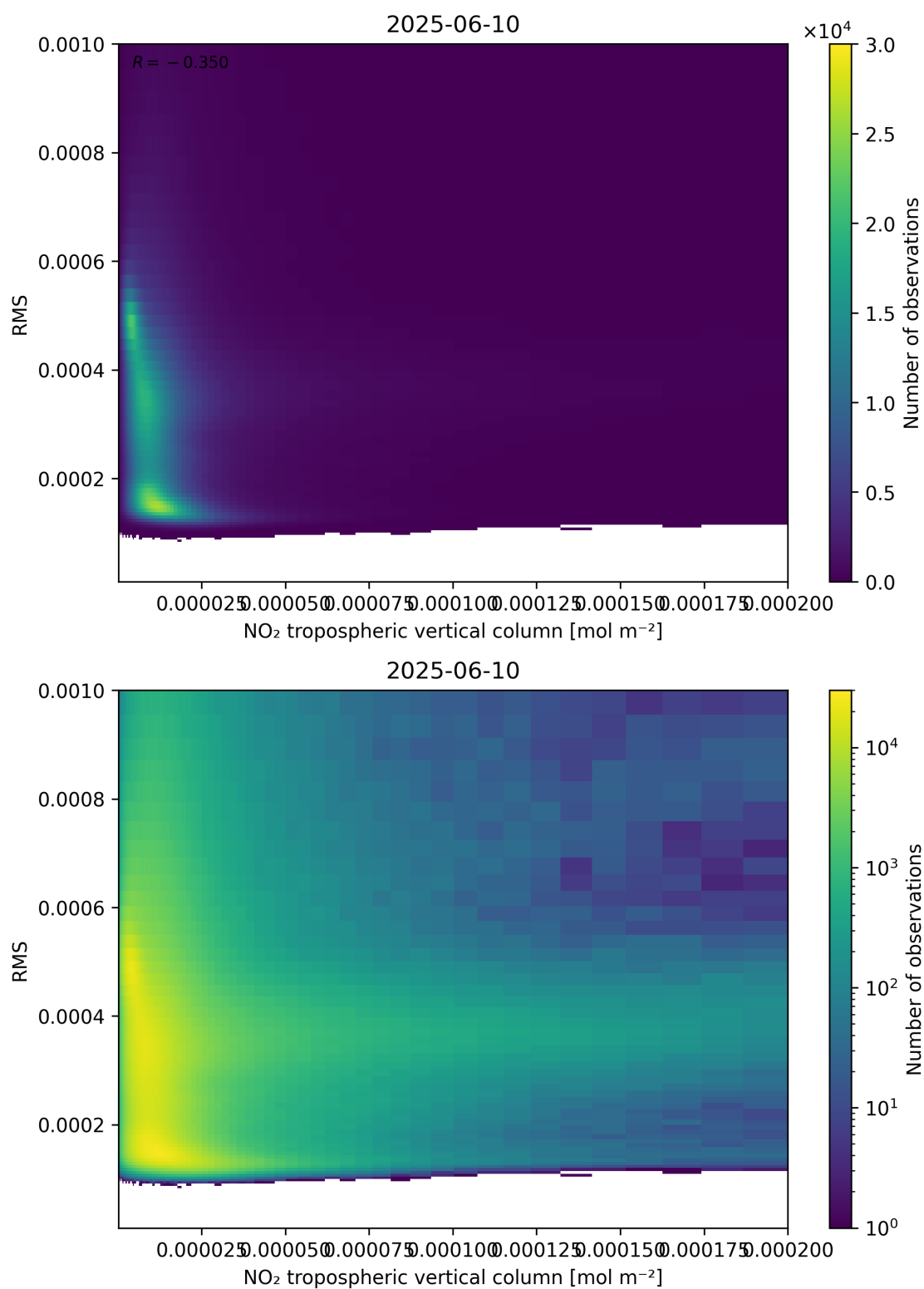
Figure 142: Scatter density plot of “NO 2 tropospheric vertical column” against “RMS” for 2025-06-09 to 2025-06-11.
