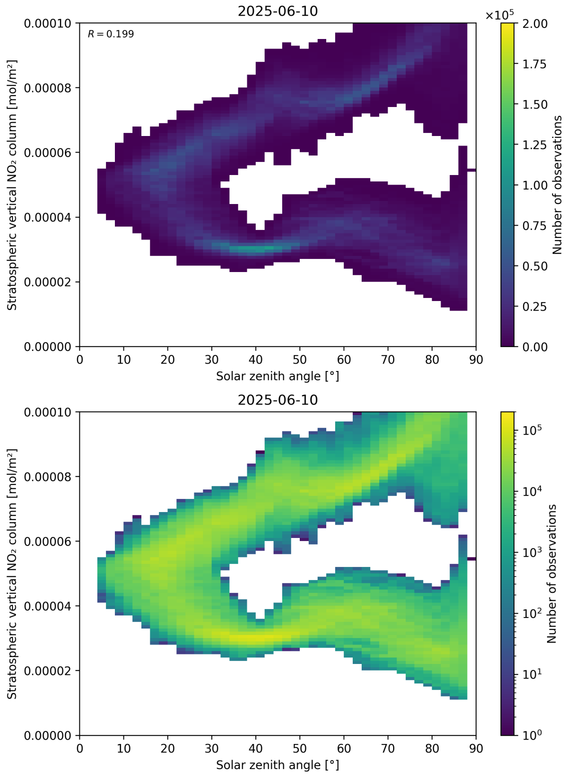
Figure 150: Scatter density plot of “Solar zenith angle” against “Stratospheric vertical NO 2 column” for 2025-06-09 to 2025-06-11.
