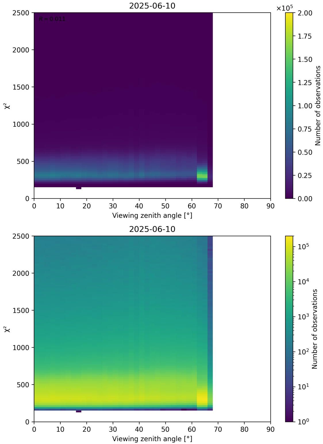
Figure 162: Scatter density plot of “Viewing zenith angle” against “ \chi^2 ” for 2025-06-09 to 2025-06-11.
