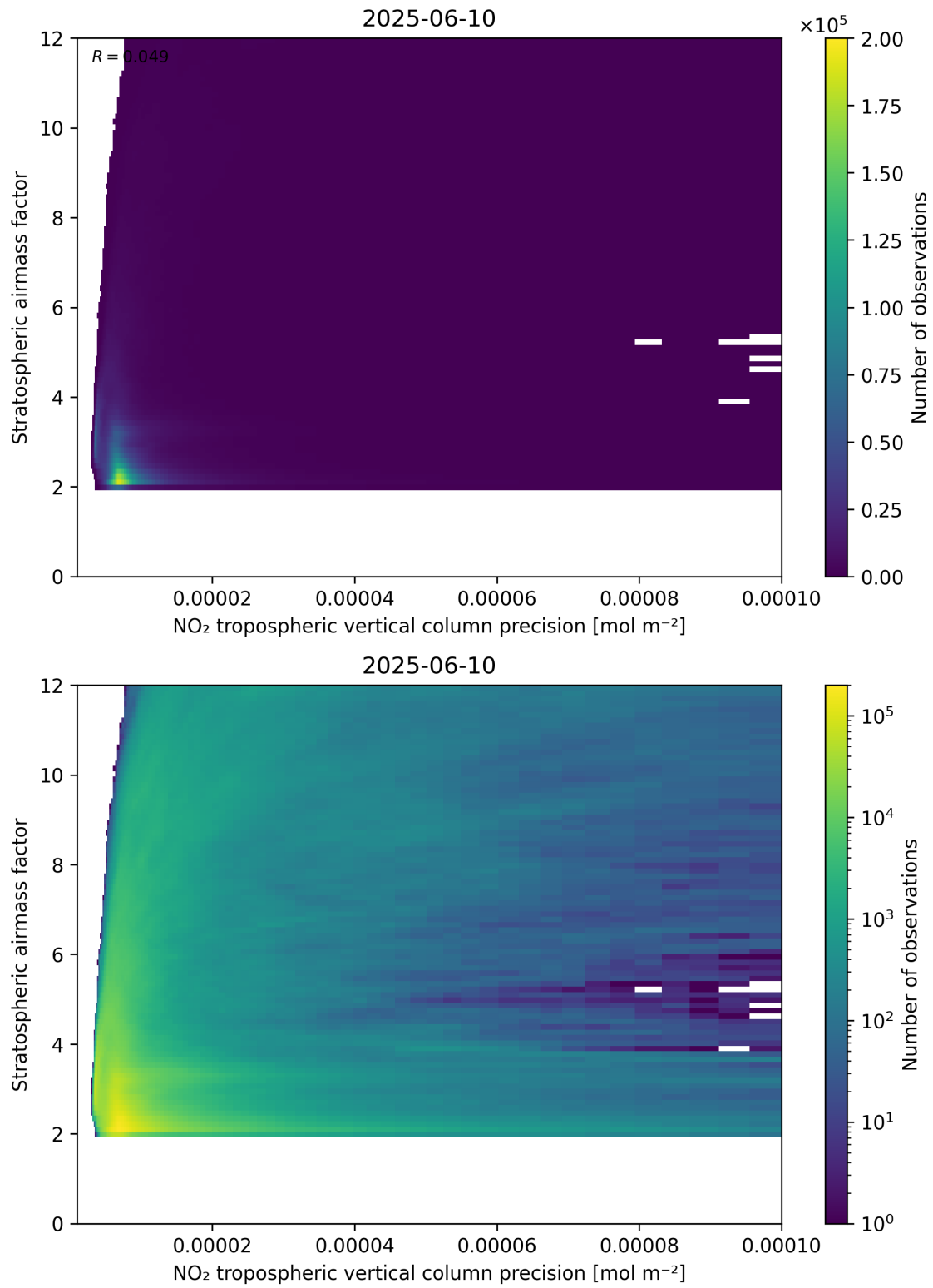
Figure 131: Scatter density plot of “NO 2 tropospheric vertical column precision” against “Stratospheric airmass factor” for 2025-06-09 to 2025-06-11.
