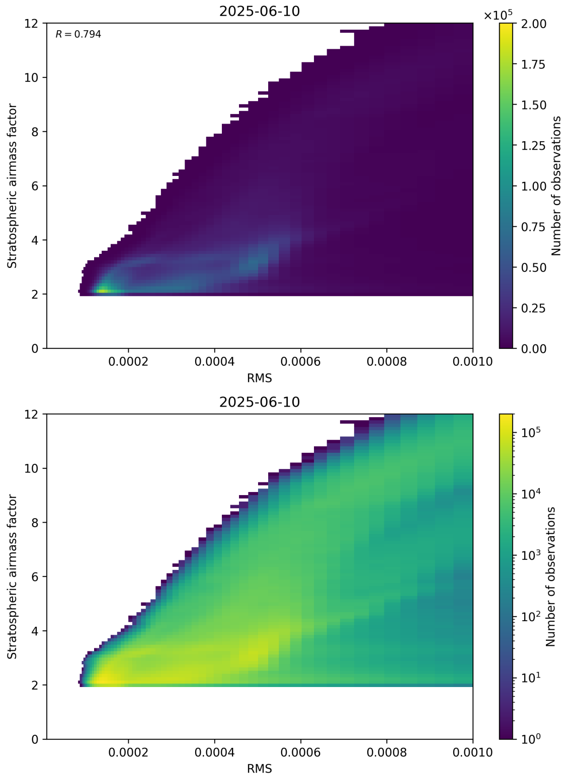
Figure 144: Scatter density plot of “RMS” against “Stratospheric airmass factor” for 2025-06-09 to 2025-06-11.
