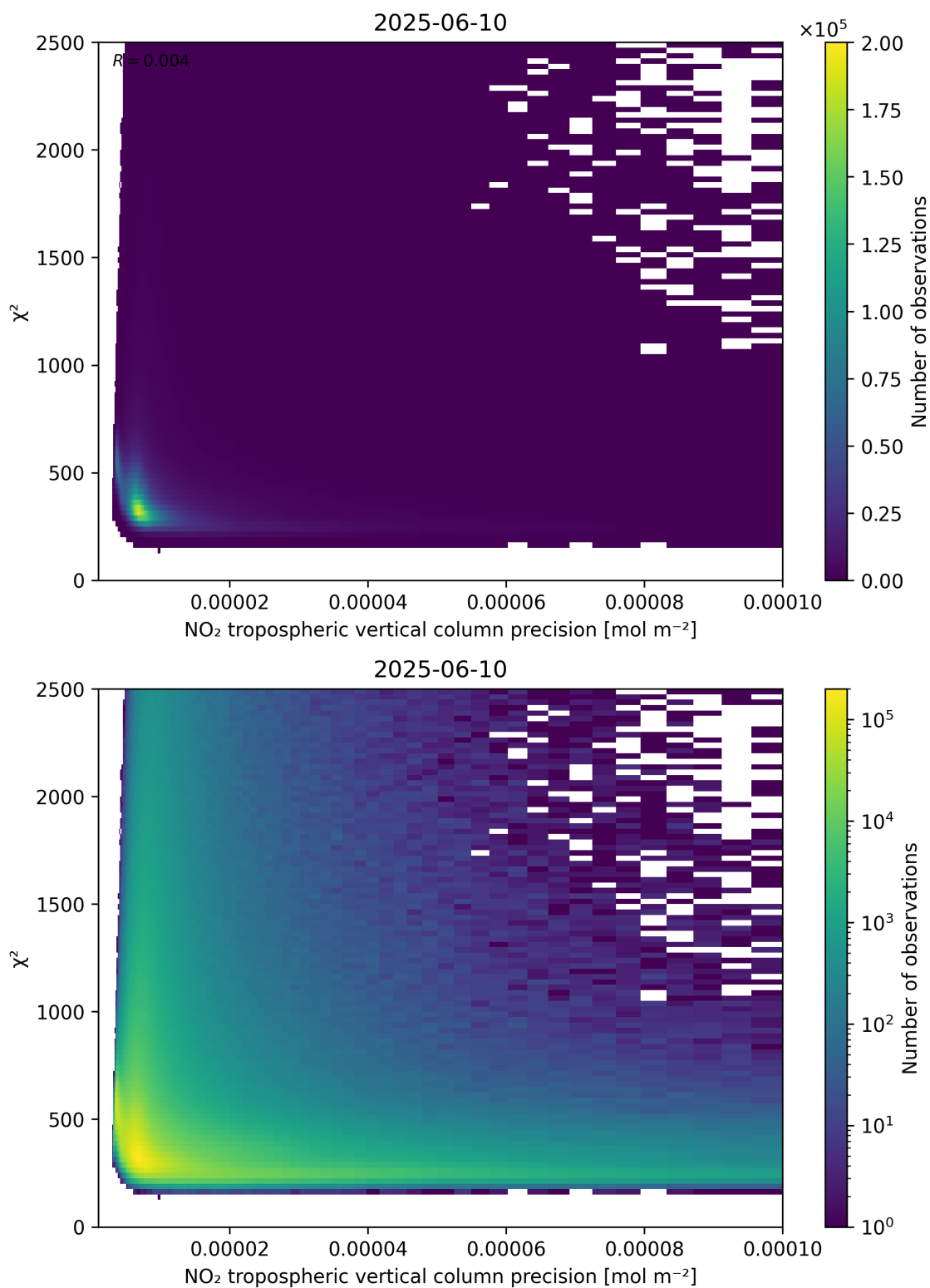
Figure 134: Scatter density plot of “NO 2 tropospheric vertical column precision” against “ \chi^2 ” for 2025-06-09 to 2025-06-11.
