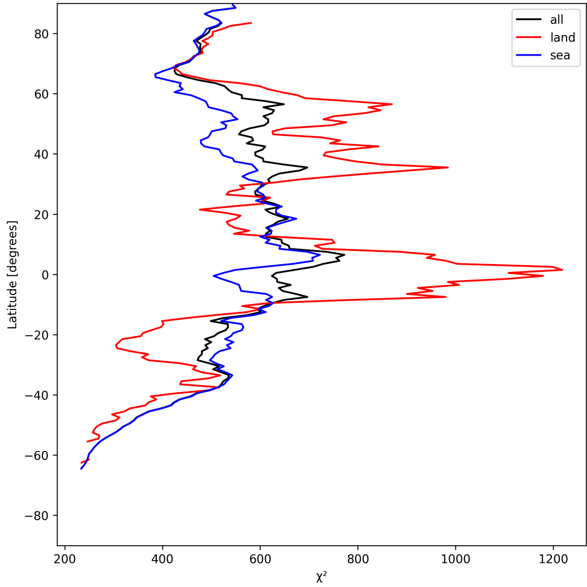
Figure 25: Zonal average of “ \chi^2 ” for 2025-06-09 to 2025-06-11.
