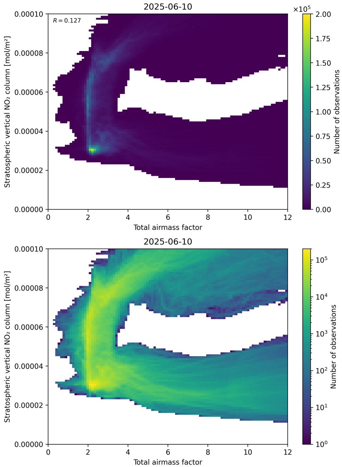
Figure 64: Scatter density plot of “Total airmass factor” against “Stratospheric vertical NO 2 column” for 2025-06-09 to 2025-06-11.
