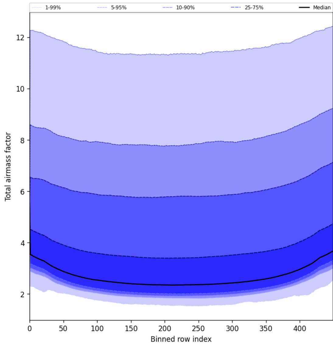
Figure 49: Along track statistics of “Total airmass factor” for 2025-06-09 to 2025-06-11
