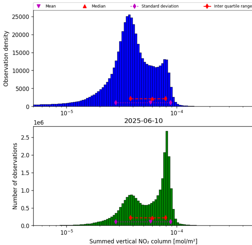
Figure 40: Histogram of “Summed vertical NO 2 column” for 2025-06-09 to 2025-06-11
