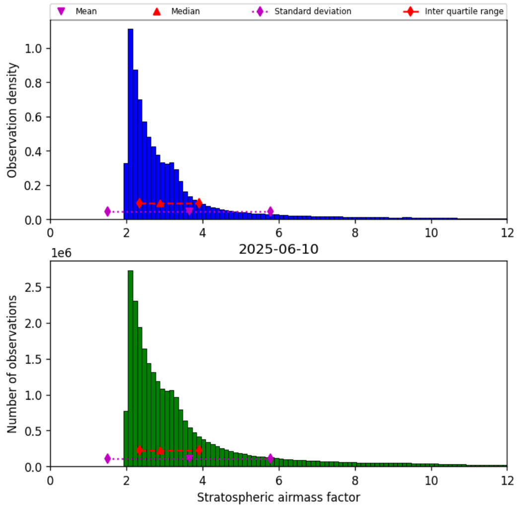
Figure 44: Histogram of “Stratospheric airmass factor” for 2025-06-09 to 2025-06-11
