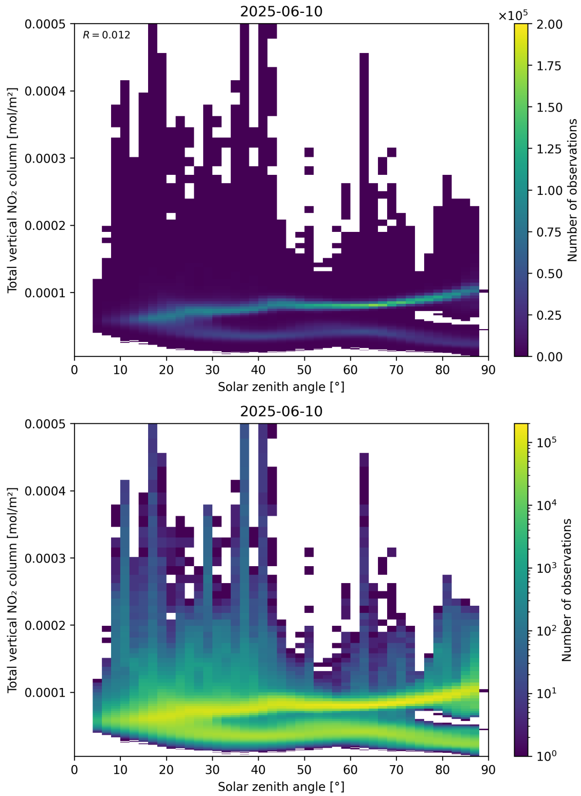
Figure 153: Scatter density plot of “Solar zenith angle” against “Total vertical NO 2 column” for 2025-06-09 to 2025-06-11.
