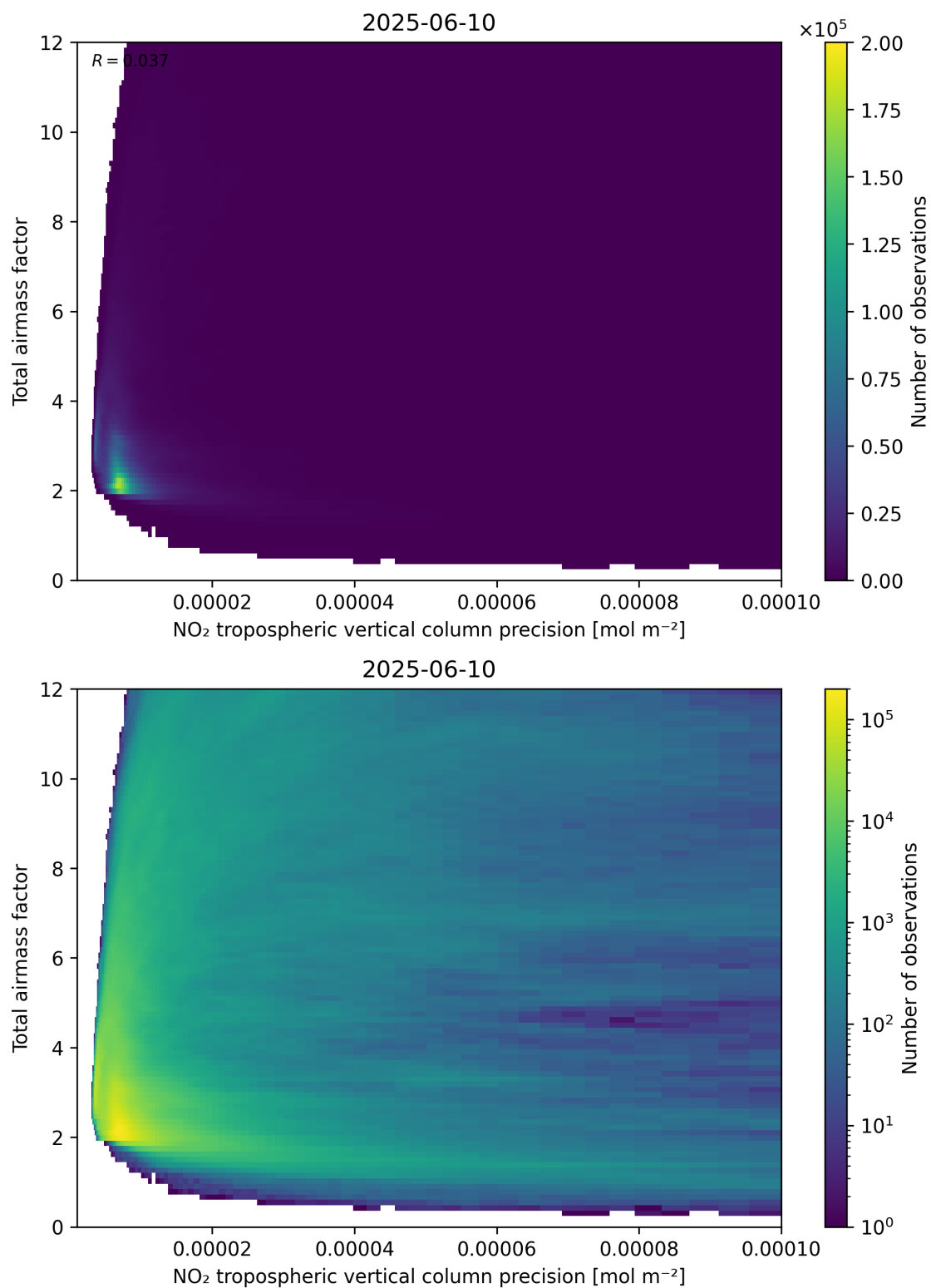
Figure 132: Scatter density plot of “NO 2 tropospheric vertical column precision” against “Total air mass factor” for 2025-06-09 to 2025-06-11.
