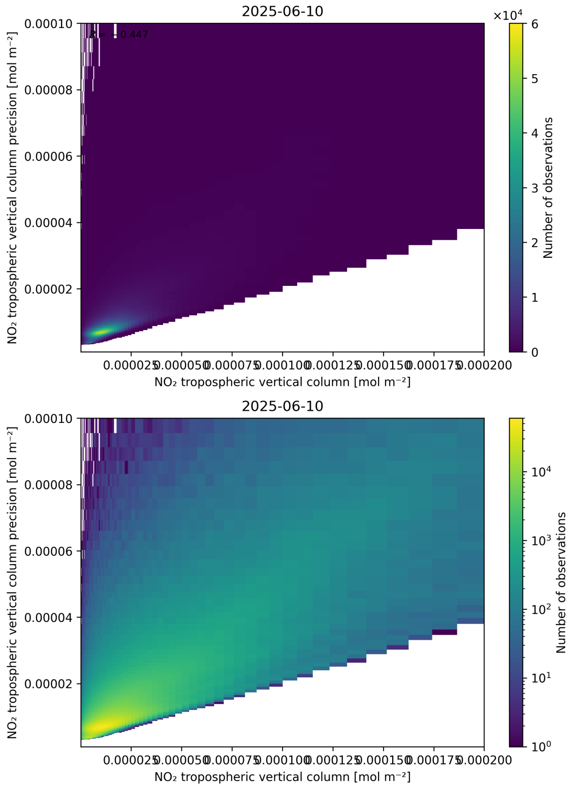
Figure 130: Scatter density plot of “NO 2 tropospheric vertical column” against “NO 2 tropospheric vertical column precision” for 2025-06-09 to 2025-06-11.
