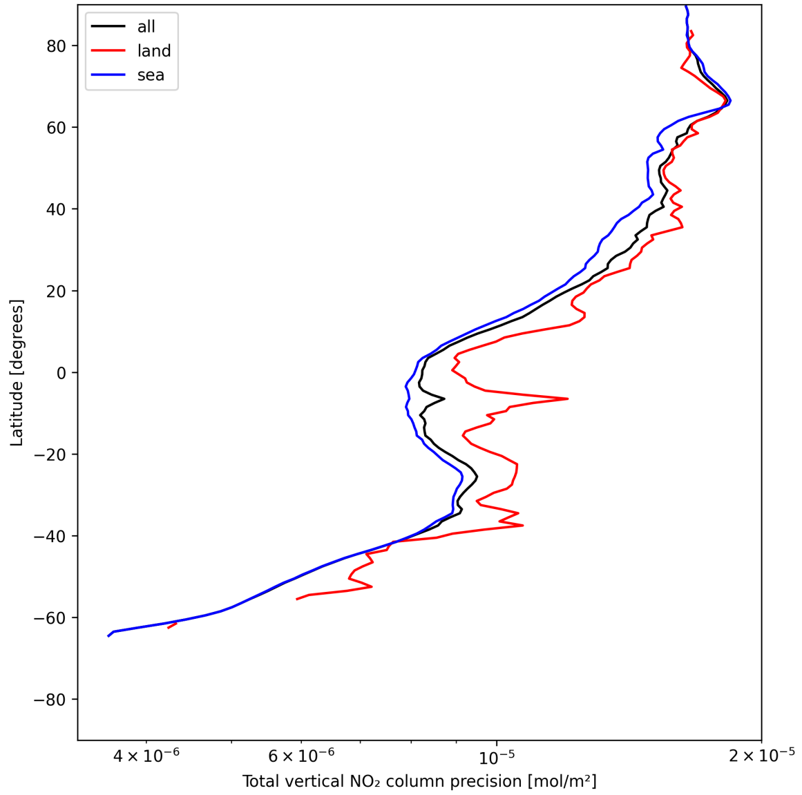
Figure 22: Zonal average of “Total vertical NO 2 column precision” for 2025-06-09 to 2025-06-11.
