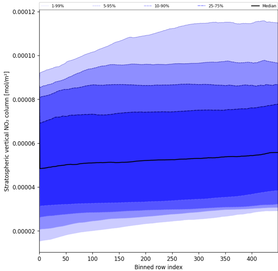
Figure 53: Along track statistics of “Stratospheric vertical NO 2 column” for 2025-06-09 to 2025-06-11
