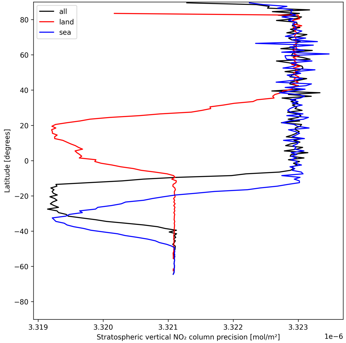
Figure 20: Zonal average of “Stratospheric vertical NO 2 column precision” for 2025-06-09 to 2025-06-11.
