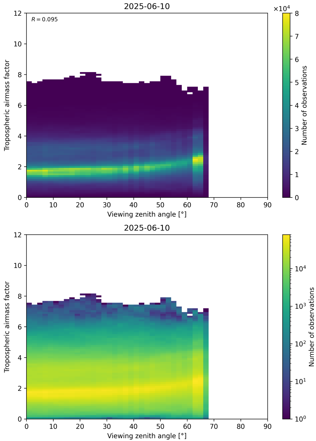
Figure 161: Scatter density plot of “Viewing zenith angle” against “Tropospheric airmass factor” for 2025-06-09 to 2025-06-11.
