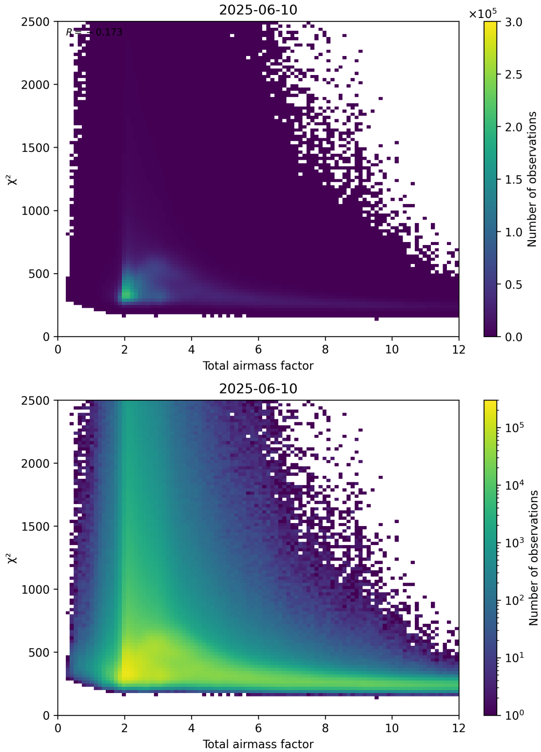
Figure 63: Scatter density plot of “Total airmass factor” against “ \chi^2 ” for 2025-06-09 to 2025-06-11.
