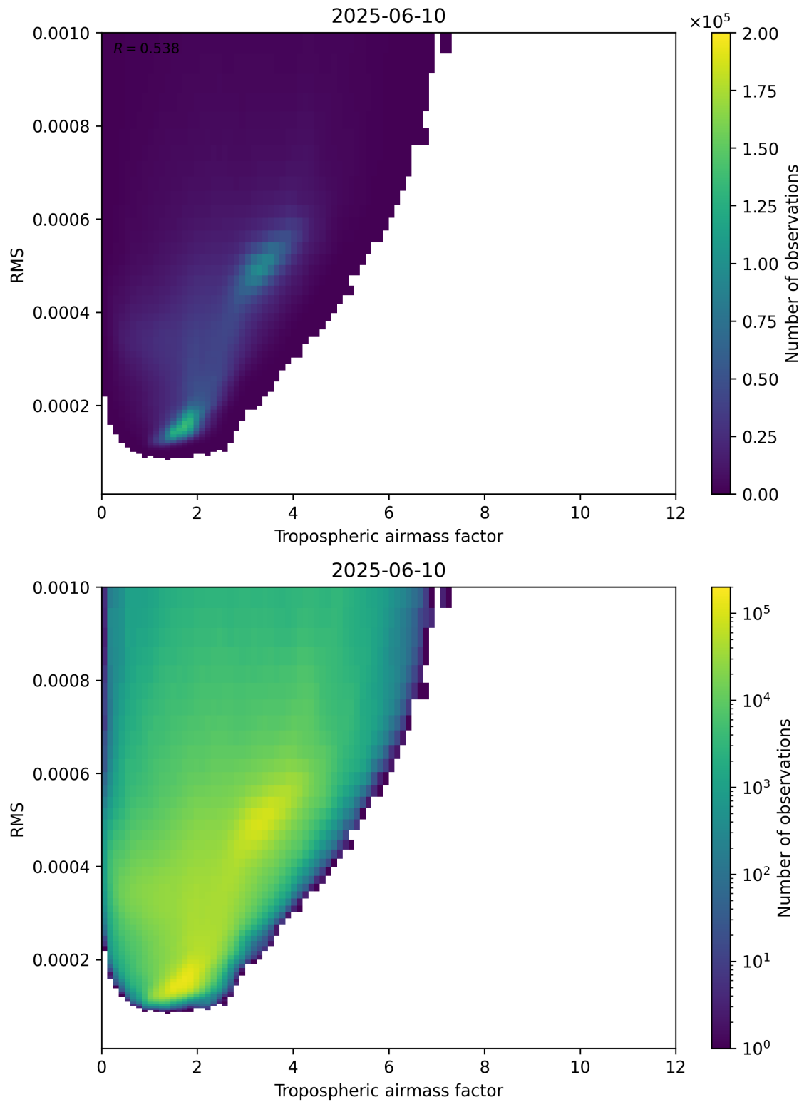
Figure 79: Scatter density plot of “Tropospheric airmass factor” against “RMS” for 2025-06-09 to 2025-06-11.
