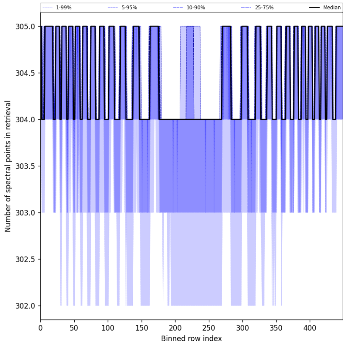
Figure 50: Along track statistics of “Number of spectral points in retrieval” for 2025-06-09 to 2025-06-11
