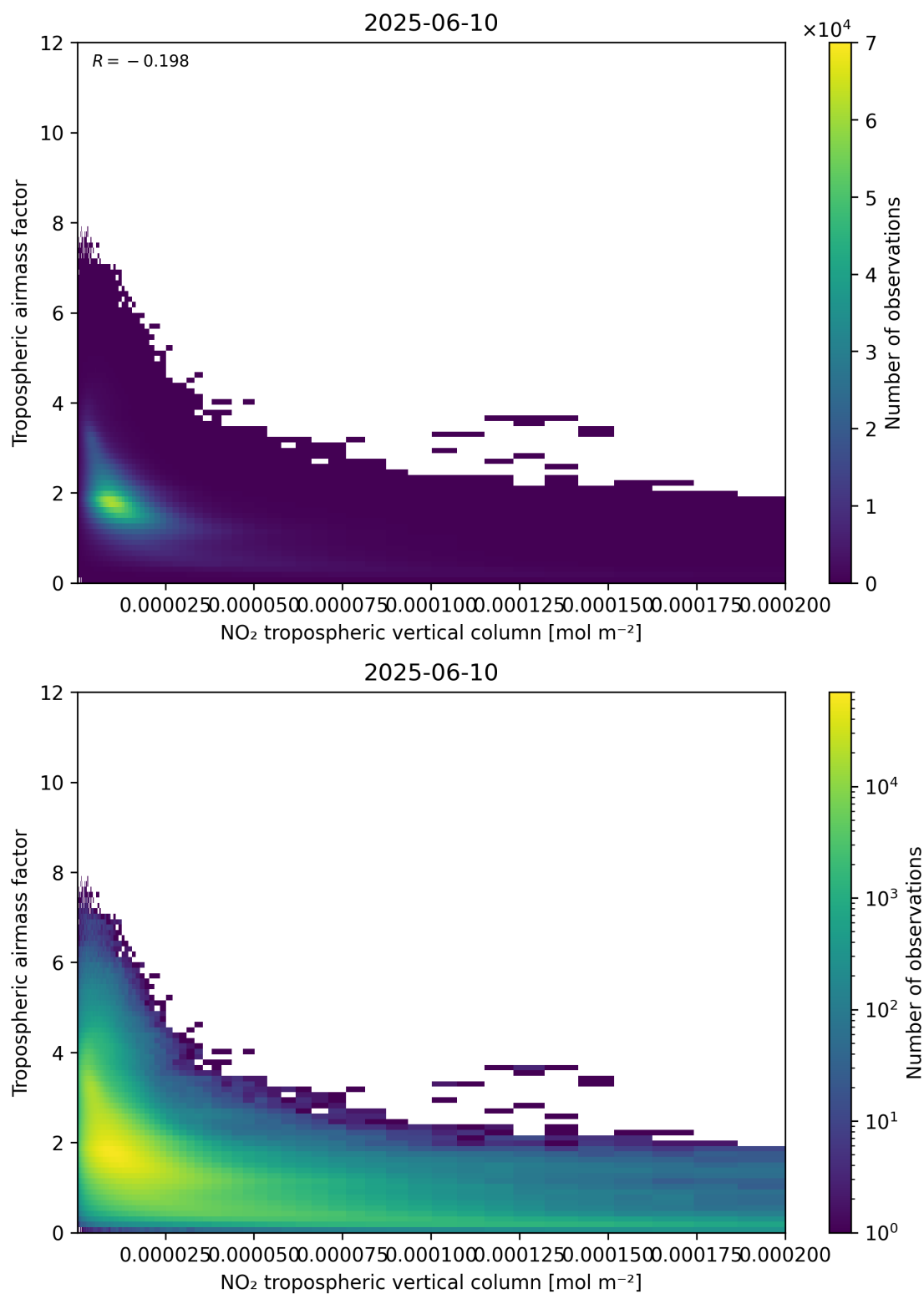
Figure 123: Scatter density plot of “NO 2 tropospheric vertical column” against “Tropospheric air mass factor” for 2025-06-09 to 2025-06-11.
