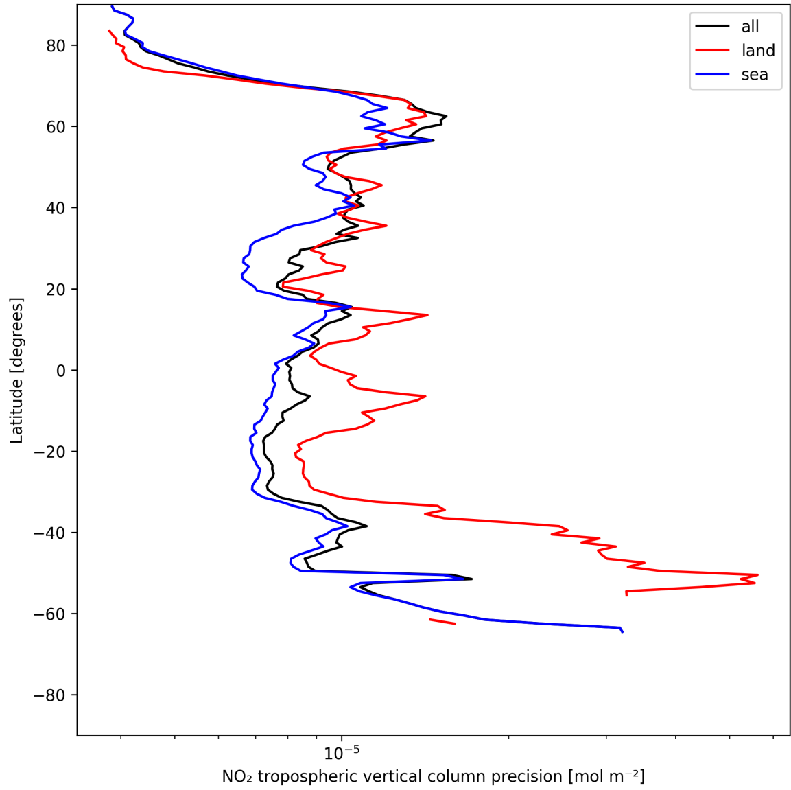
Figure 13: Zonal average of “NO 2 tropospheric vertical column precision” for 2025-06-09 to 2025-06-11.
