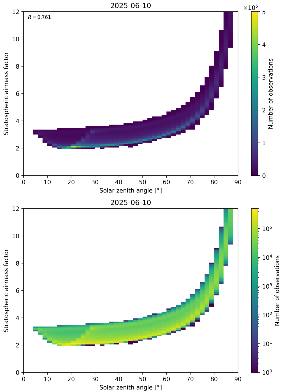
Figure 145: Scatter density plot of “Solar zenith angle” against “Stratospheric airmass factor” for 2025-06-09 to 2025-06-11.
