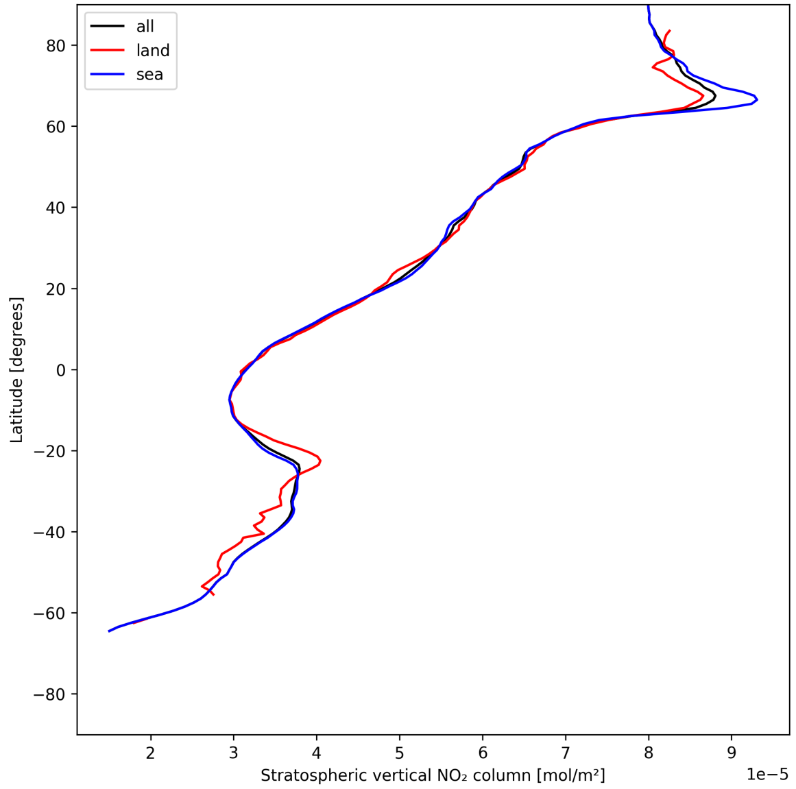
Figure 19: Zonal average of “Stratospheric vertical NO 2 column” for 2025-06-09 to 2025-06-11.
