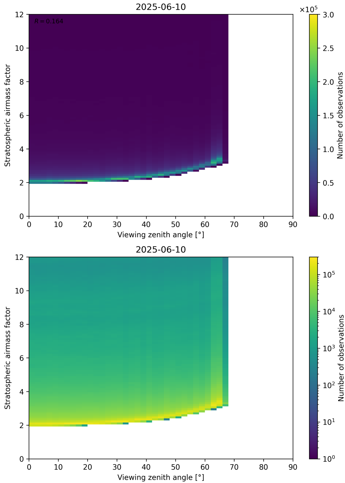
Figure 159: Scatter density plot of “Viewing zenith angle” against “Stratospheric airmass factor” for 2025-06-09 to 2025-06-11.
