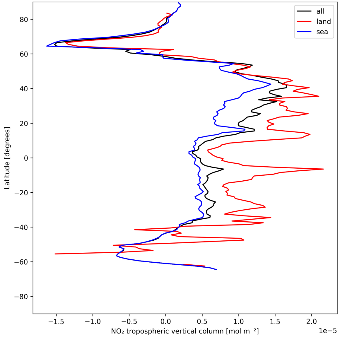
Figure 12: Zonal average of “NO 2 tropospheric vertical column” for 2025-06-09 to 2025-06-11.
