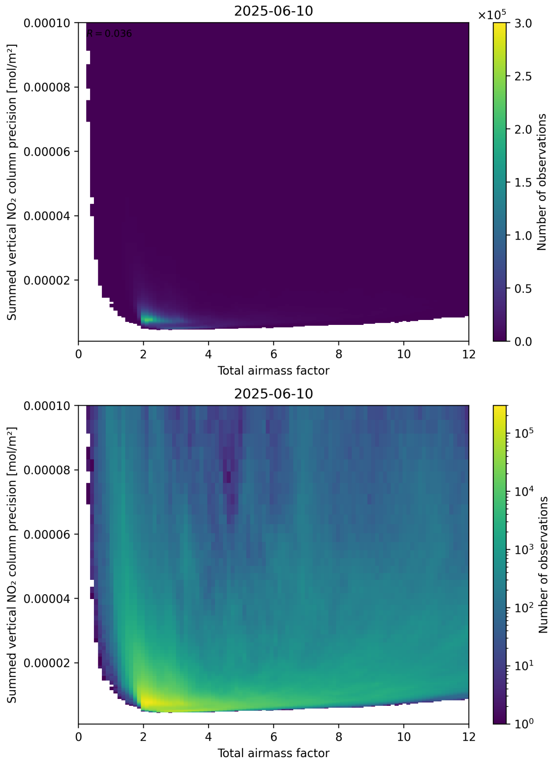
Figure 66: Scatter density plot of “Total airmass factor” against “Summed vertical NO 2 column precision” for 2025-06-09 to 2025-06-11.
