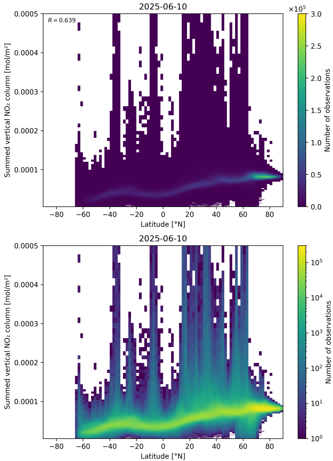
Figure 88: Scatter density plot of “Latitude” against “Summed vertical NO 2 column” for 2025-06-09 to 2025-06-11.
