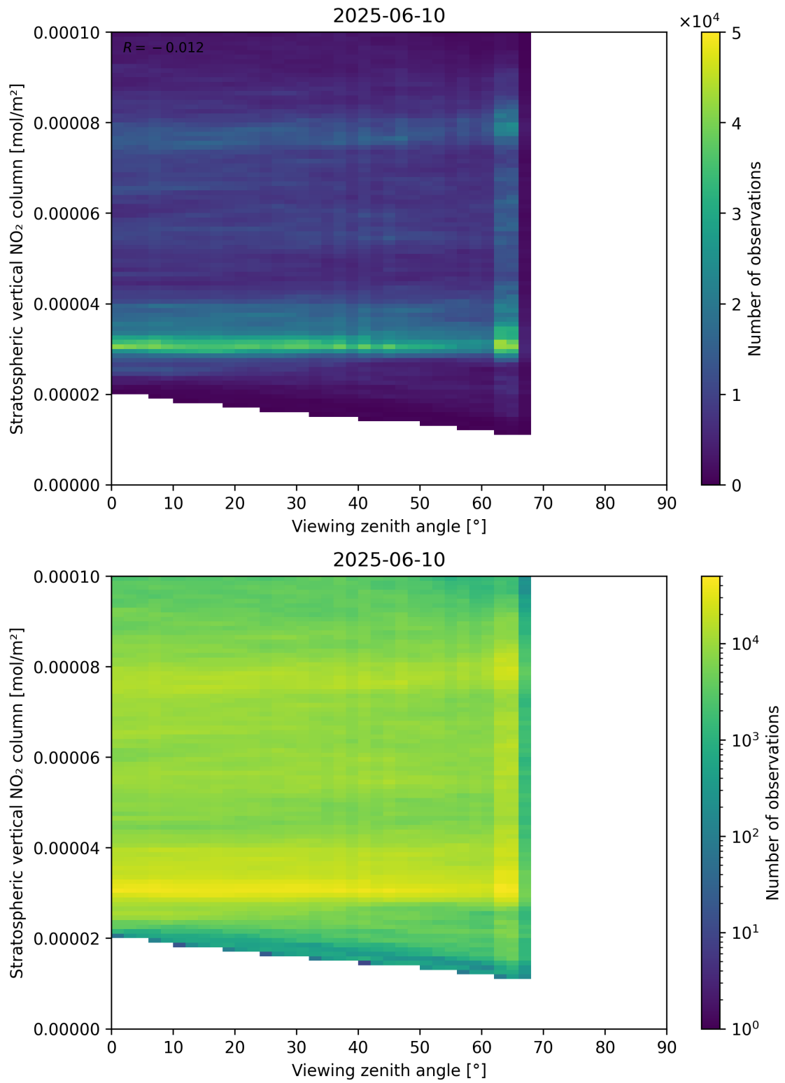
Figure 164: Scatter density plot of “Viewing zenith angle” against “Stratospheric vertical NO 2 column” for 2025-06-09 to 2025-06-11.
