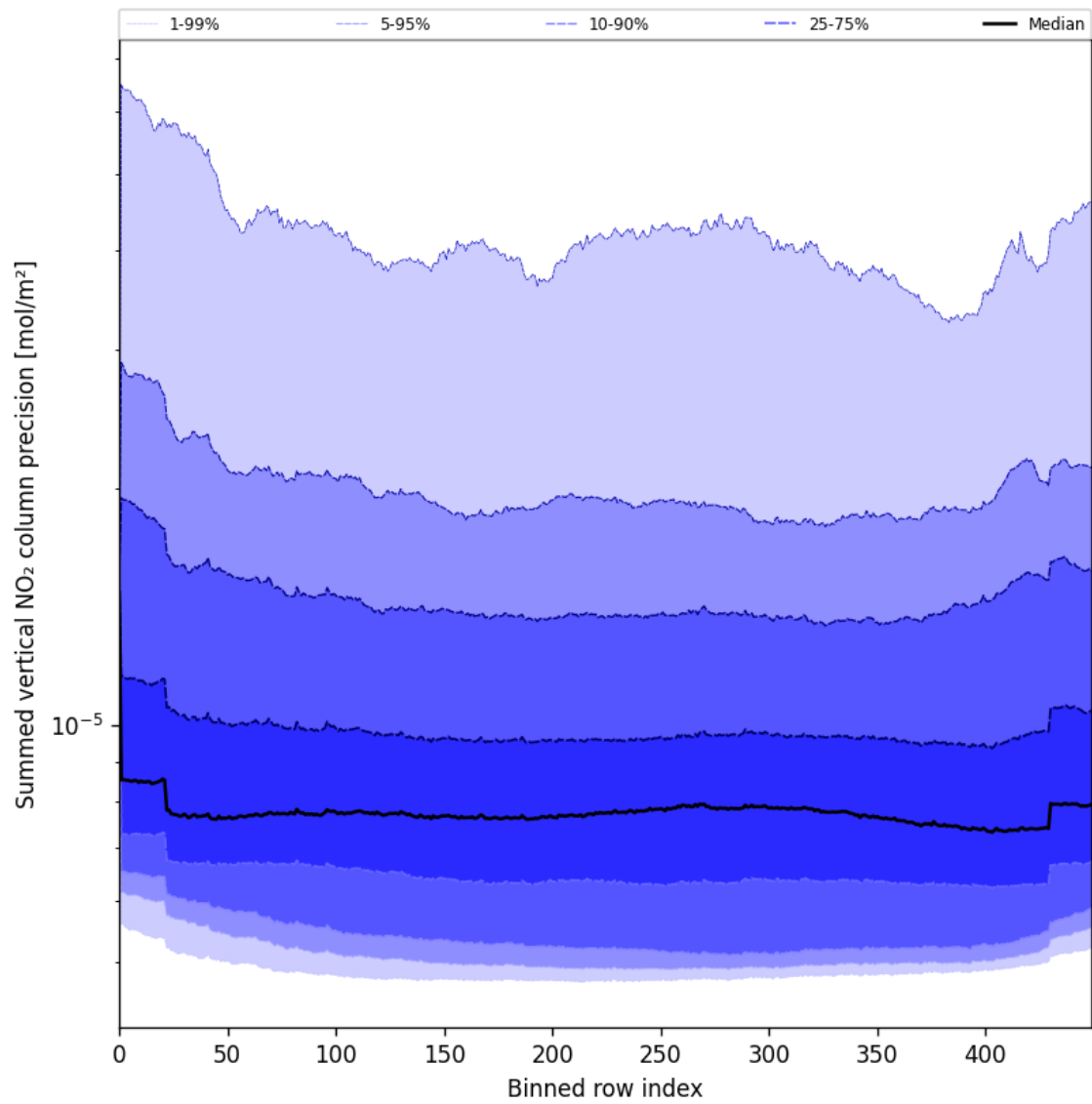
Figure 58: Along track statistics of “Summed vertical NO 2 column precision” for 2025-06-09 to 2025-06-11
