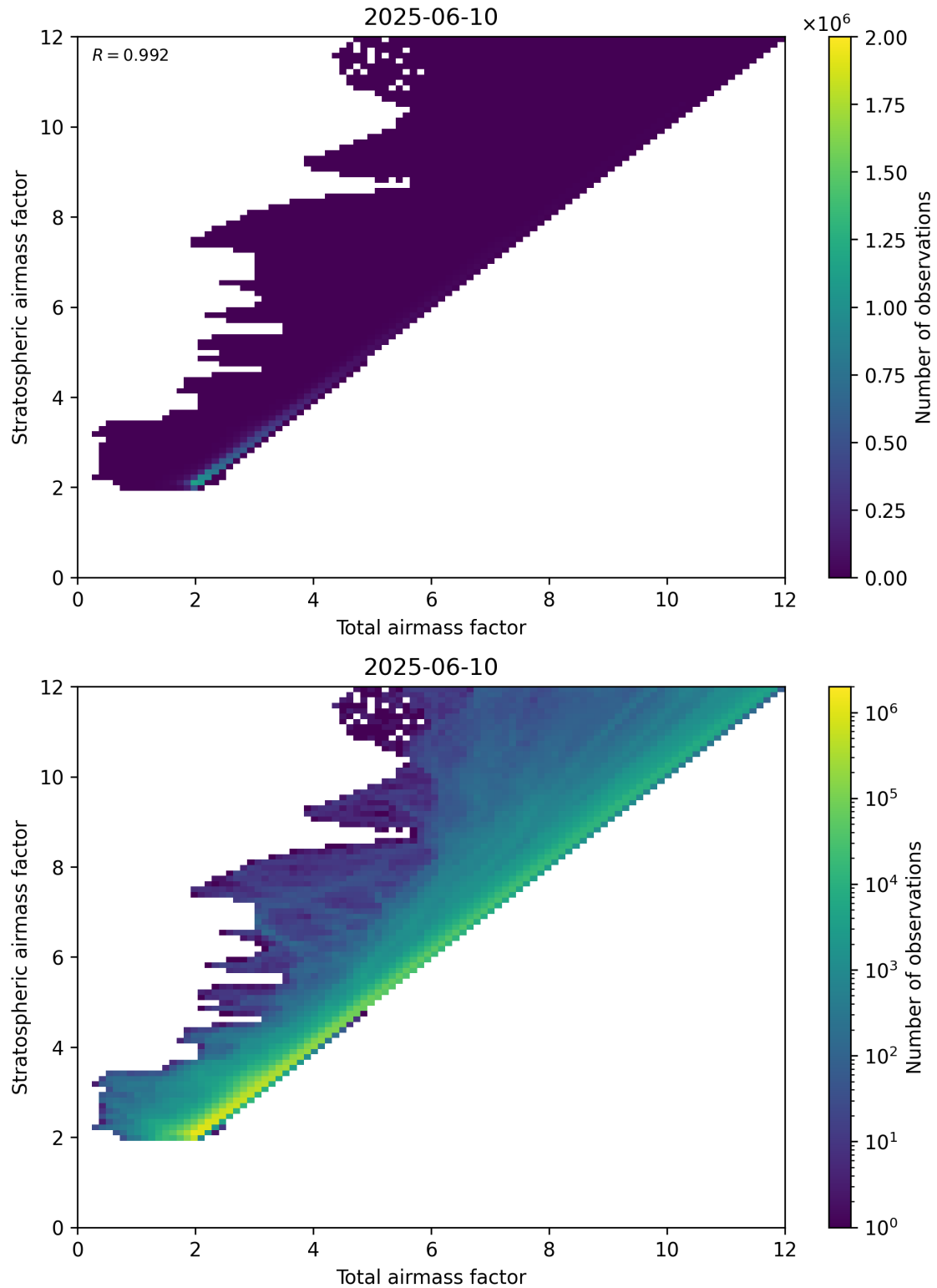
Figure 62: Scatter density plot of “Total air mass factor” against “Stratospheric air mass factor” for 2025-06-09 to 2025-06-11.
