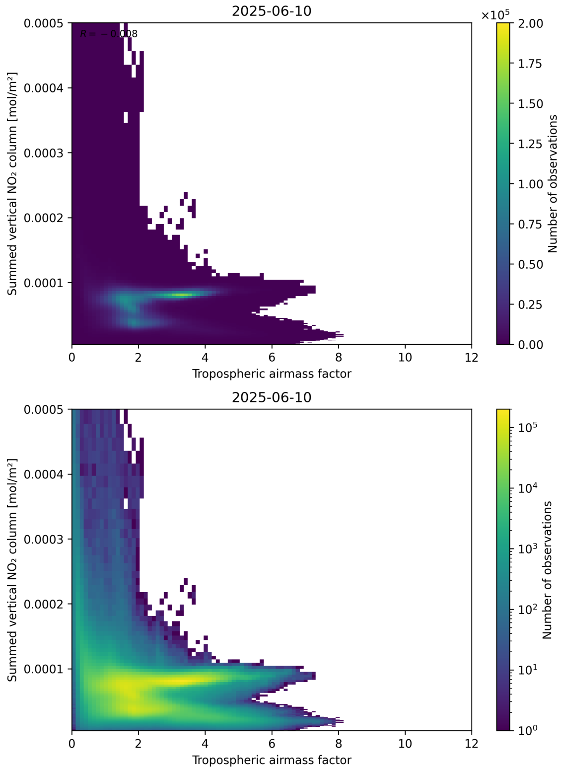
Figure 75: Scatter density plot of “Tropospheric airmass factor” against “Summed vertical NO 2 column” for 2025-06-09 to 2025-06-11.
