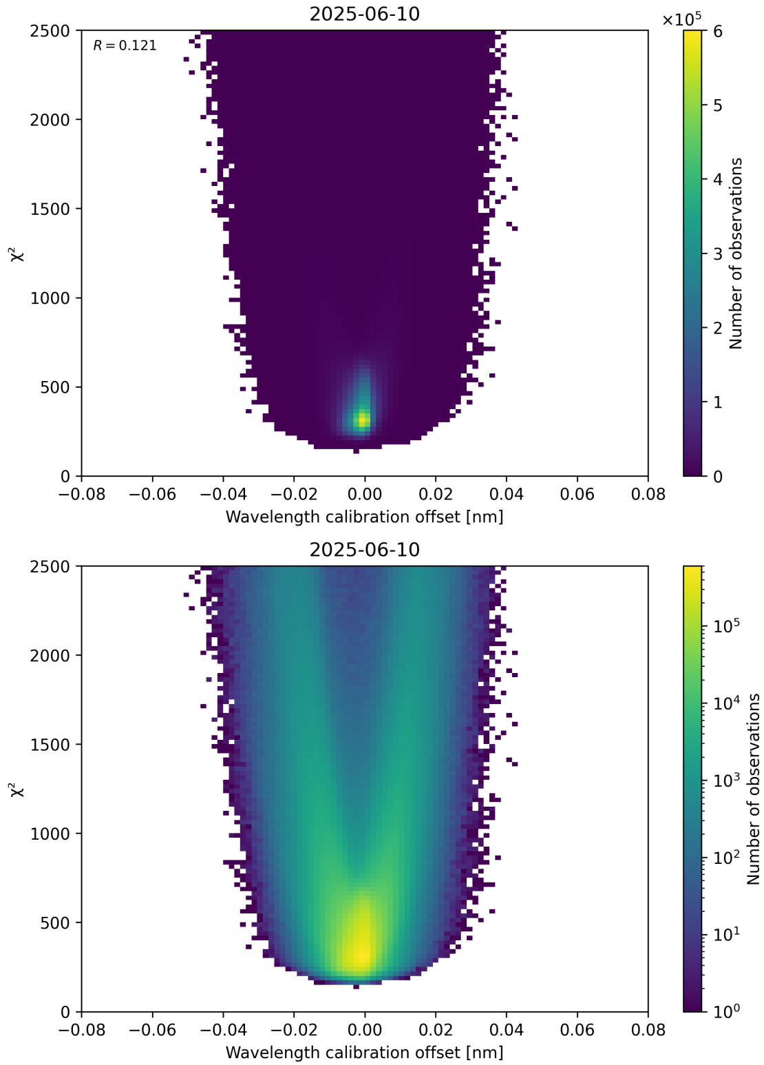
Figure 175: Scatter density plot of “Wavelength calibration offset” against “ \chi^2 ” for 2025-06-09 to 2025-06-11.
