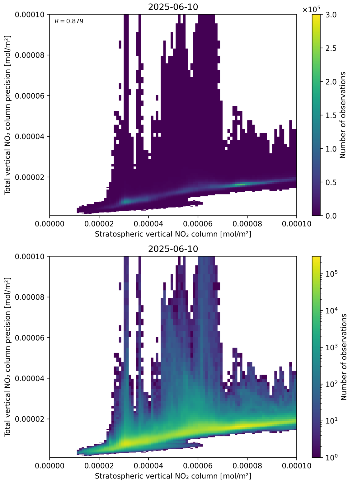
Figure 101: Scatter density plot of “Stratospheric vertical NO 2 column” against “Total vertical NO 2 column precision” for 2025-06-09 to 2025-06-11.
