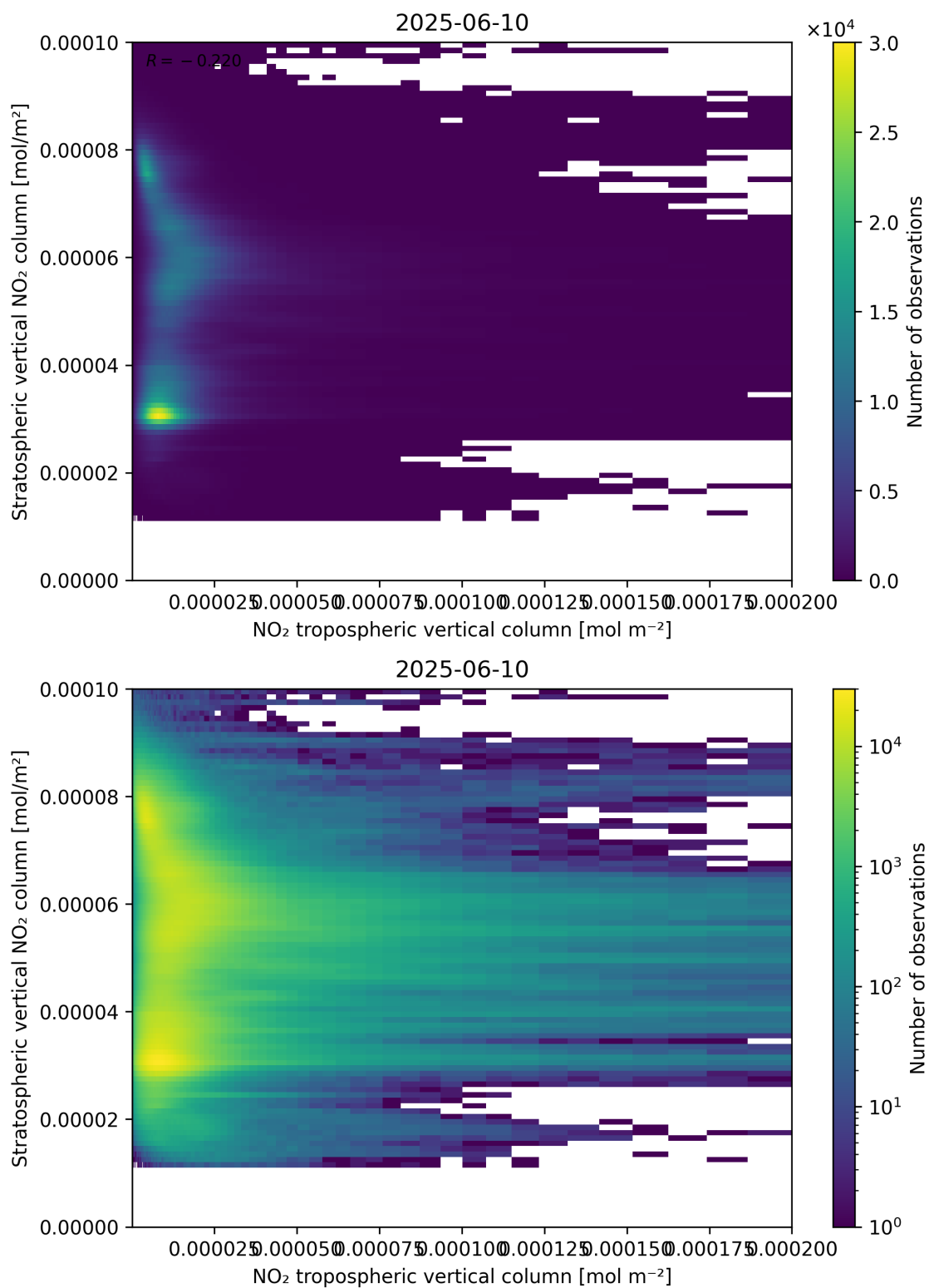
Figure 125: Scatter density plot of “NO 2 tropospheric vertical column” against “Stratospheric vertical NO 2 column” for 2025-06-09 to 2025-06-11.
