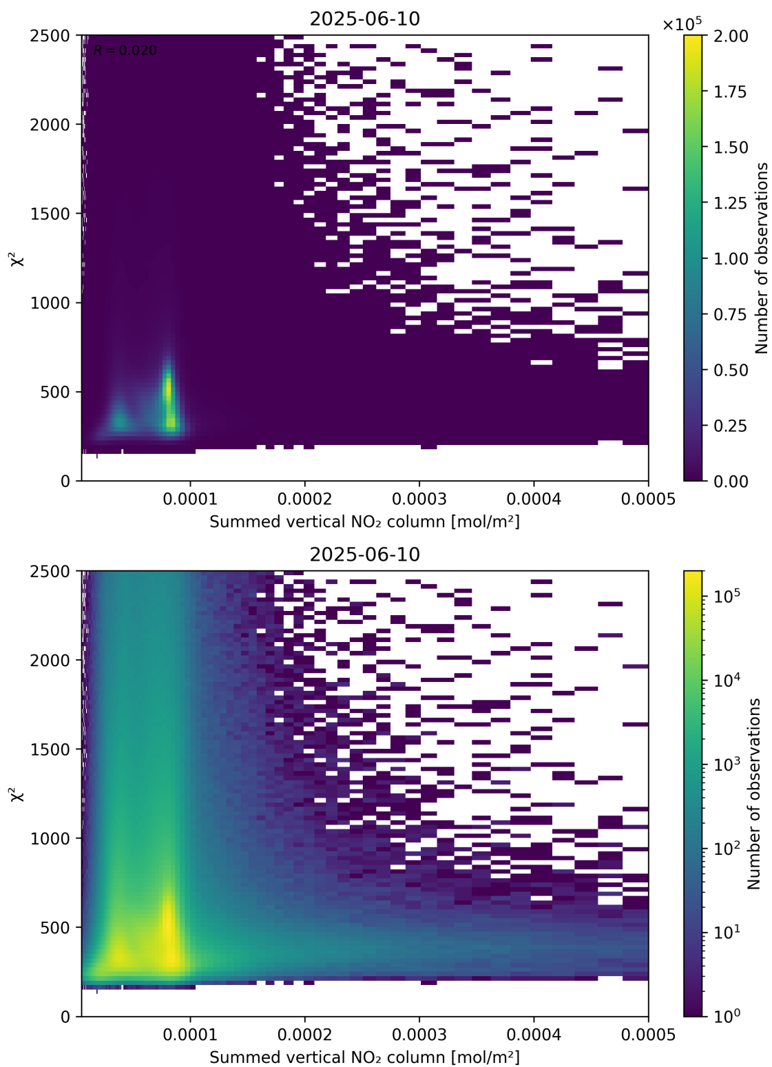
Figure 104: Scatter density plot of “Summed vertical NO 2 column” against “ \chi^2 ” for 2025-06-09 to 2025-06-11.
