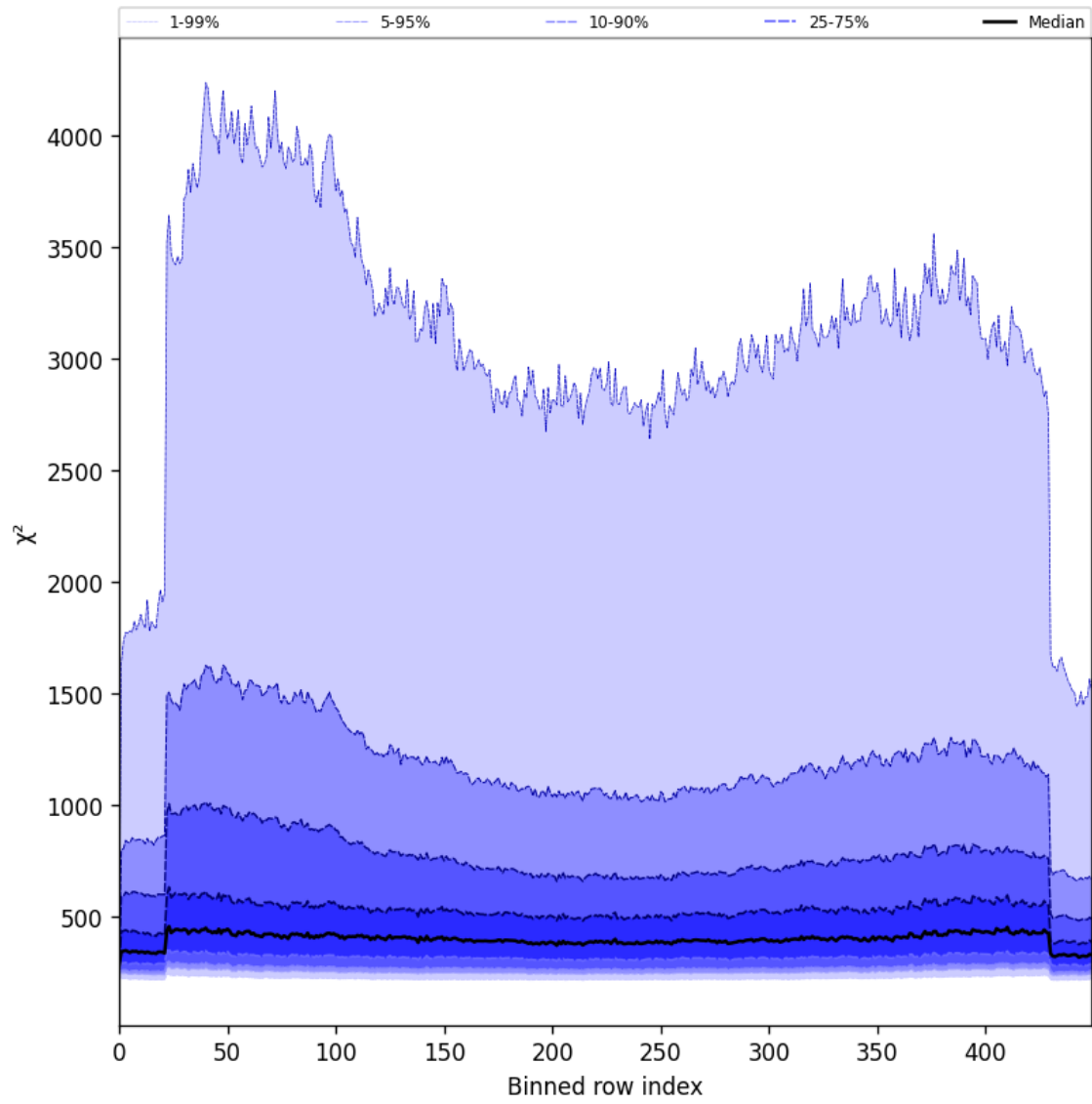
Figure 59: Along track statistics of “ \chi^2 ” for 2025-06-09 to 2025-06-11
