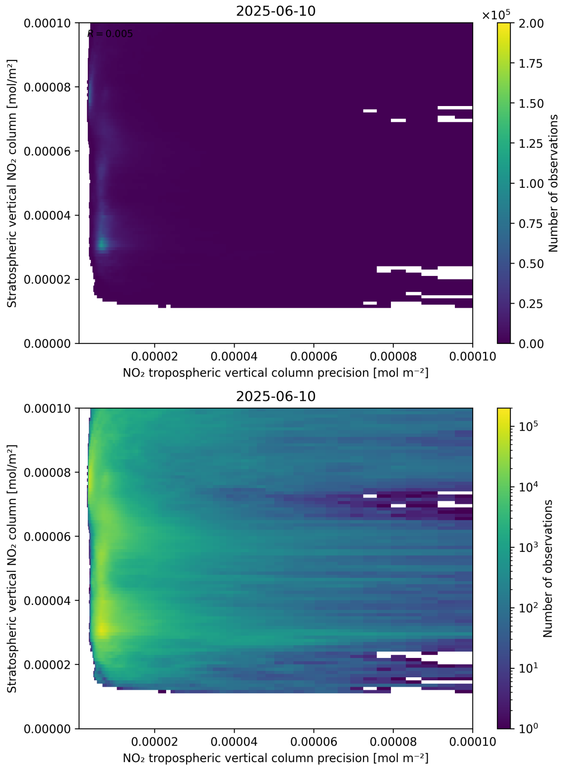
Figure 135: Scatter density plot of “NO 2 tropospheric vertical column precision” against “Stratospheric vertical NO 2 column” for 2025-06-09 to 2025-06-11.
