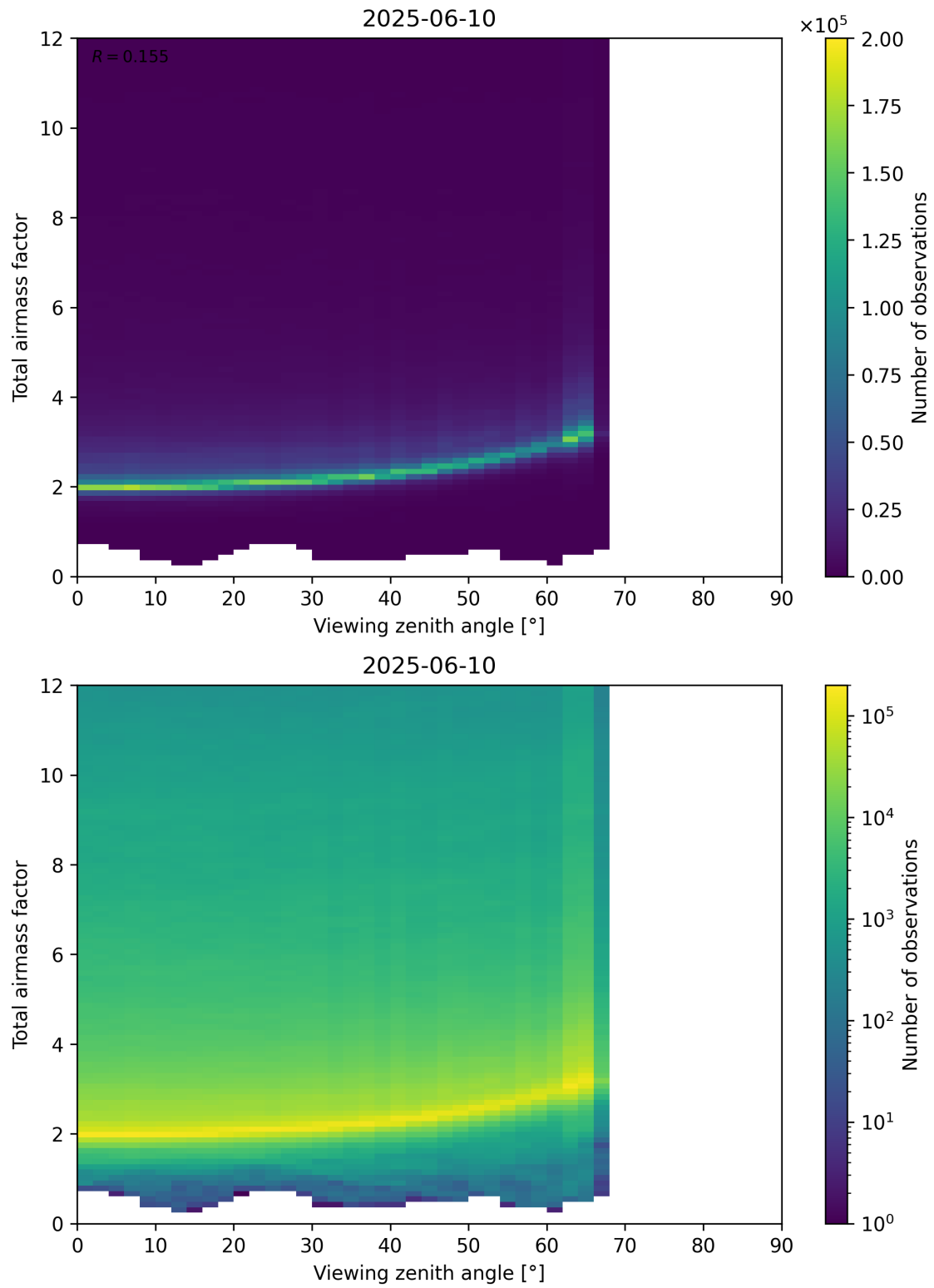
Figure 160: Scatter density plot of “Viewing zenith angle” against “Total airmass factor” for 2025-06-09 to 2025-06-11.
