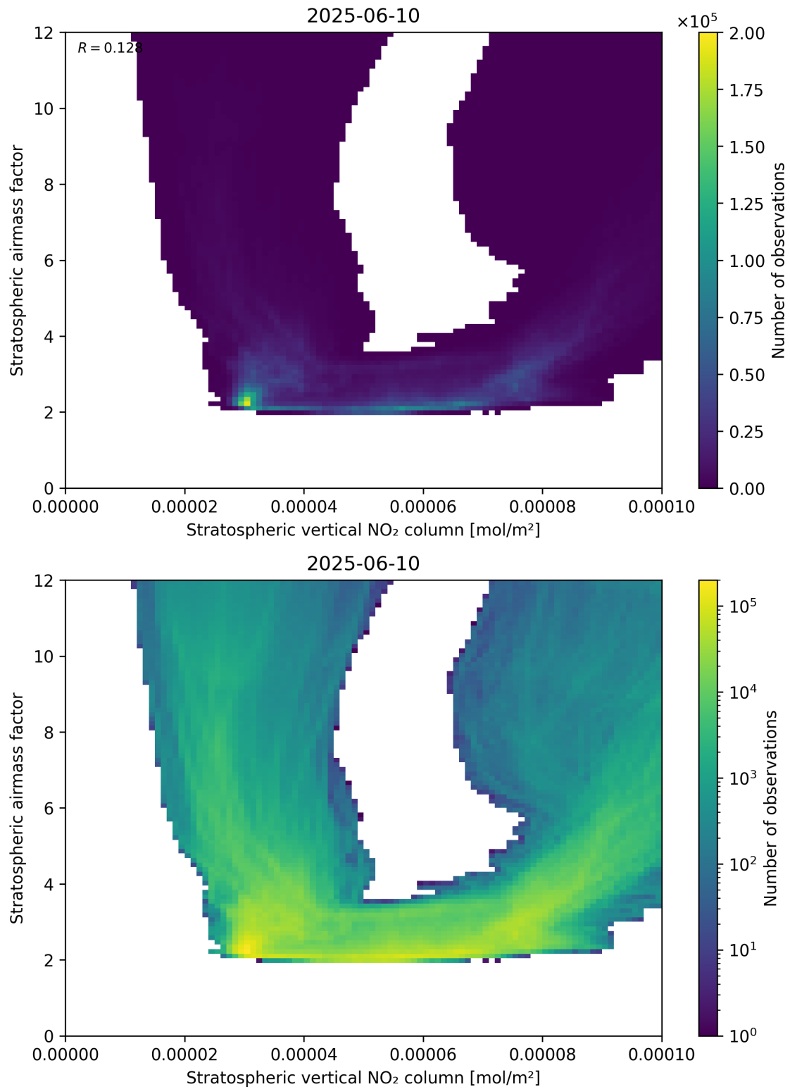
Figure 96: Scatter density plot of “Stratospheric vertical NO 2 column” against “Stratospheric airmass factor” for 2025-06-09 to 2025-06-11.
