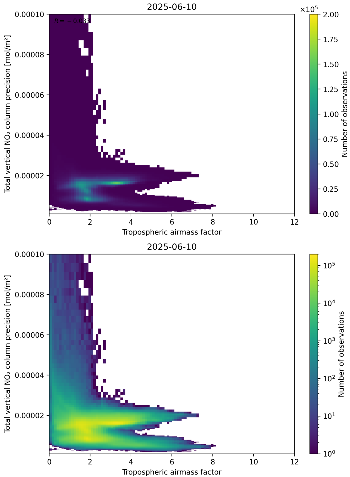
Figure 78: Scatter density plot of “Tropospheric airmass factor” against “Total vertical NO 2 column precision” for 2025-06-09 to 2025-06-11.
