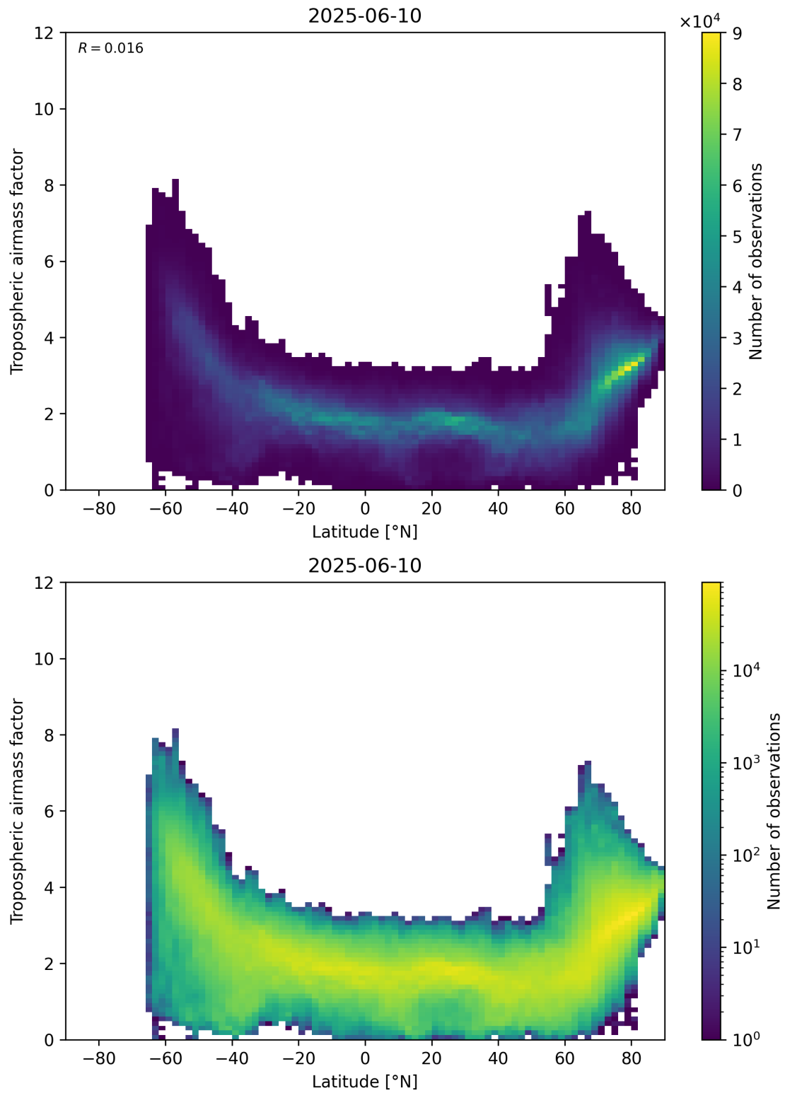
Figure 85: Scatter density plot of “Latitude” against “Tropospheric air mass factor” for 2025-06-09 to 2025-06-11.
