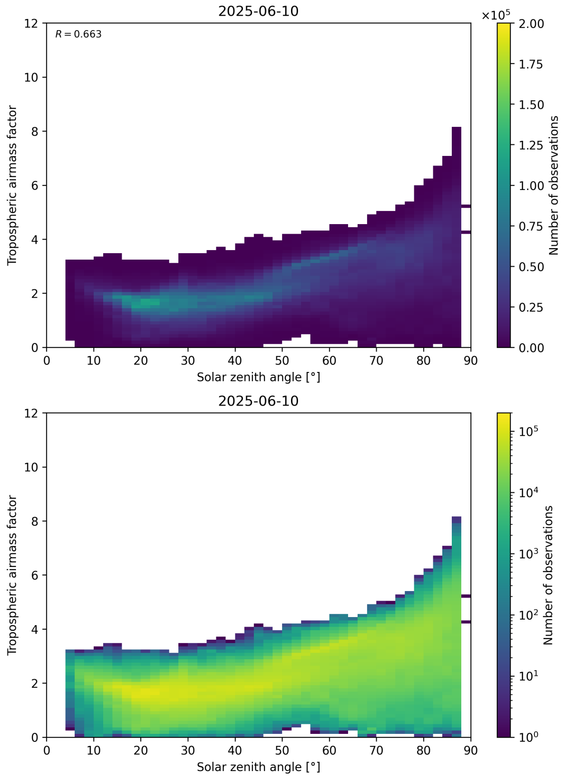
Figure 147: Scatter density plot of “Solar zenith angle” against “Tropospheric airmass factor” for 2025-06-09 to 2025-06-11.
