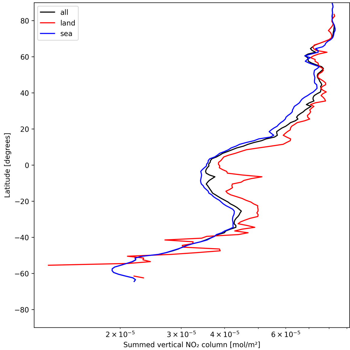
Figure 23: Zonal average of “Summed vertical NO 2 column” for 2025-06-09 to 2025-06-11.
