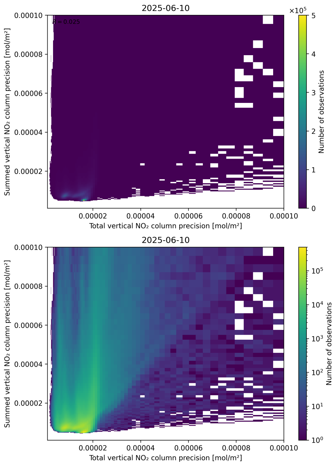
Figure 118: Scatter density plot of “Total vertical NO 2 column precision” against “Summed vertical NO 2 column precision” for 2025-06-09 to 2025-06-11.
