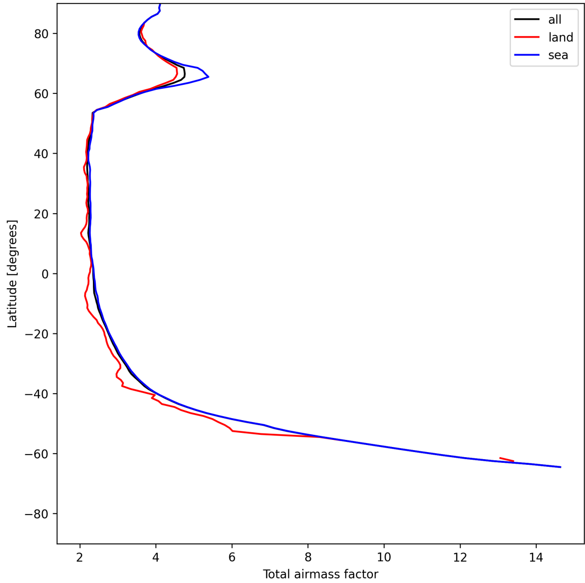
Figure 15: Zonal average of “Total airmass factor” for 2025-06-09 to 2025-06-11.
