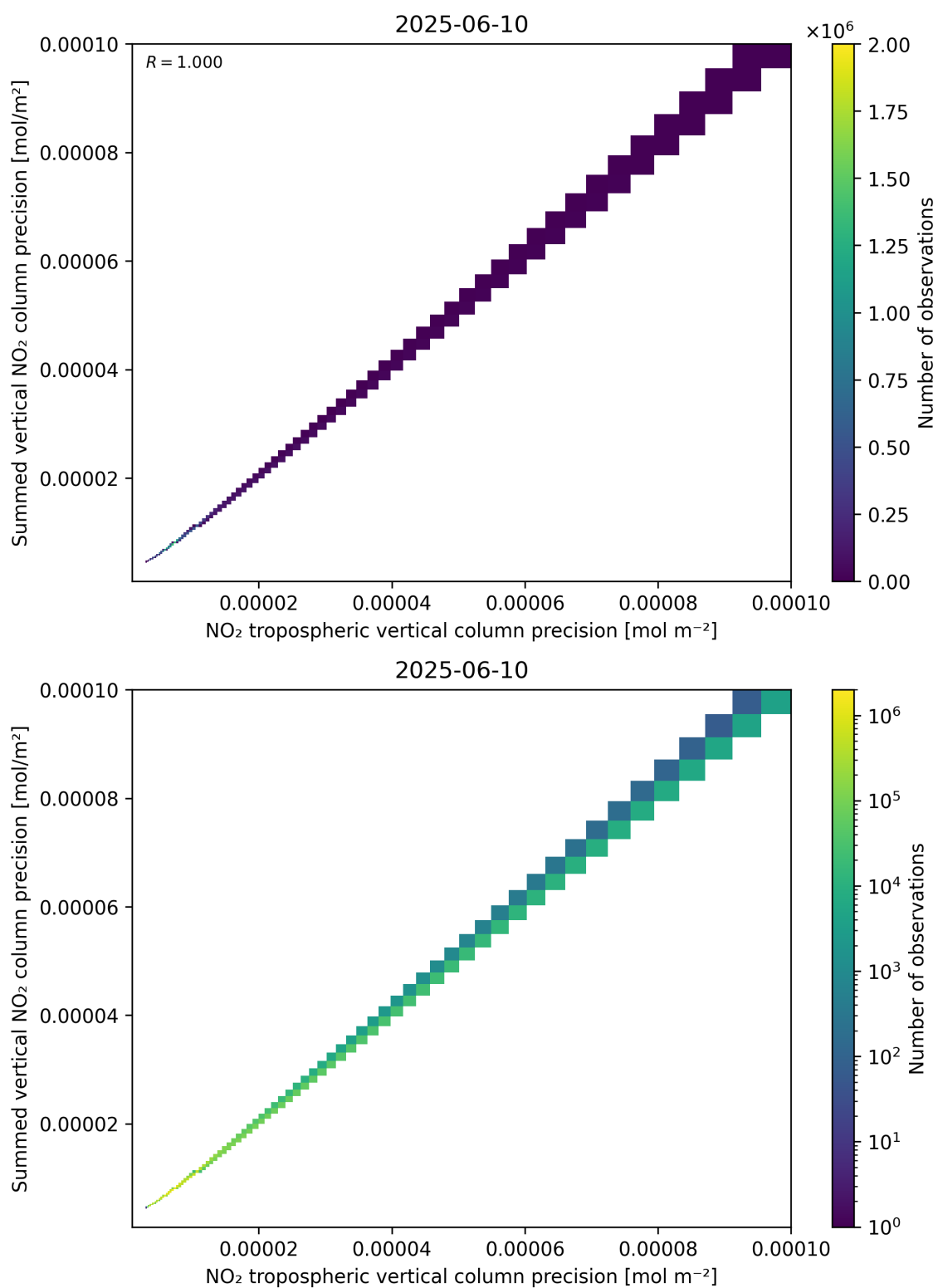
Figure 137: Scatter density plot of “NO 2 tropospheric vertical column precision” against “Summed vertical NO 2 column precision” for 2025-06-09 to 2025-06-11.
