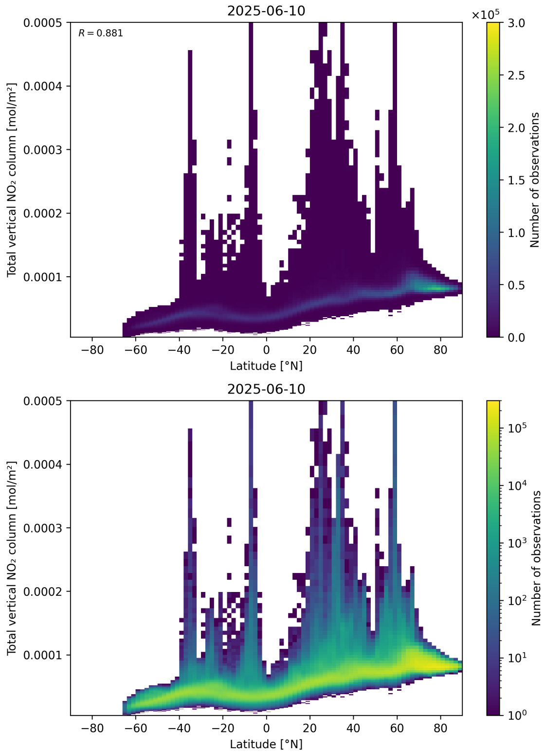
Figure 90: Scatter density plot of “Latitude” against “Total vertical NO 2 column” for 2025-06-09 to 2025-06-11.
