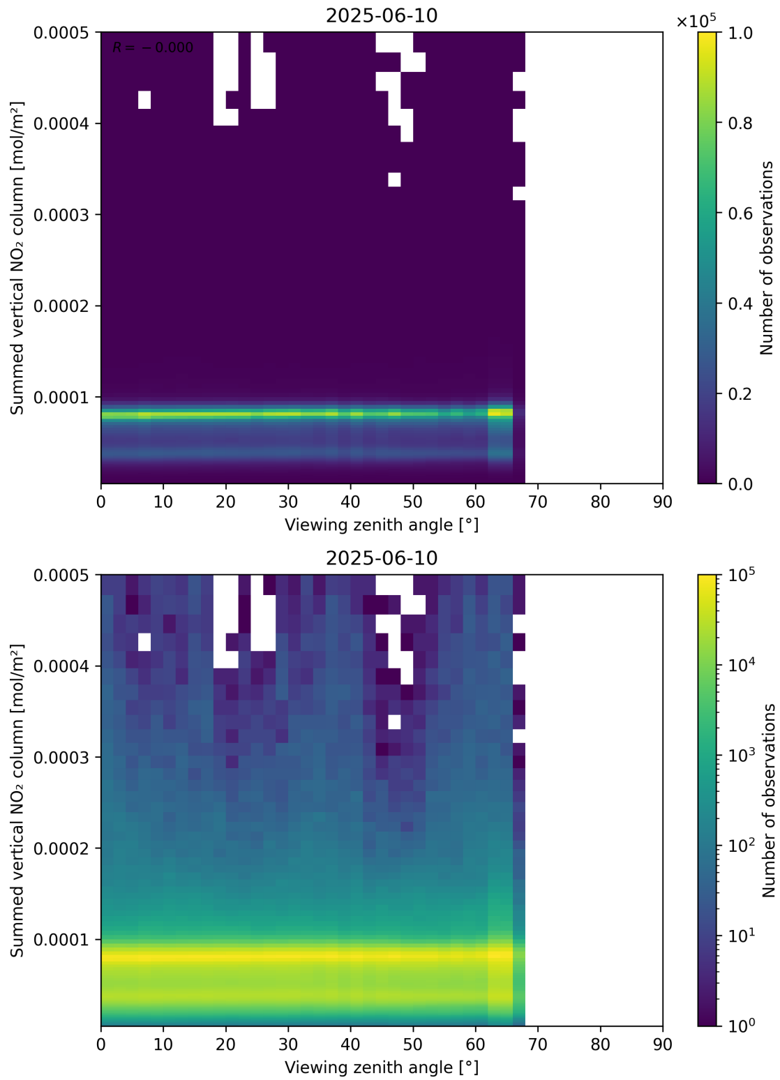
Figure 165: Scatter density plot of “Viewing zenith angle” against “Summed vertical NO 2 column” for 2025-06-09 to 2025-06-11.
