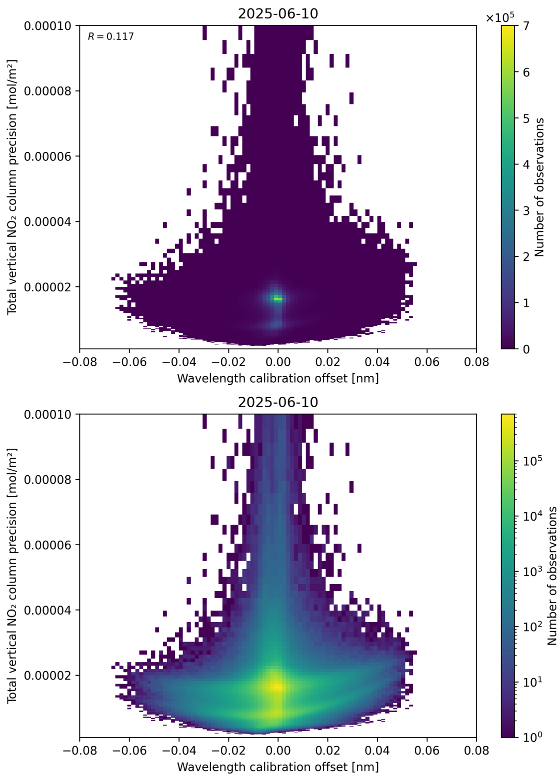
Figure 180: Scatter density plot of “Wavelength calibration offset” against “Total vertical NO 2 column precision” for 2025-06-09 to 2025-06-11.
