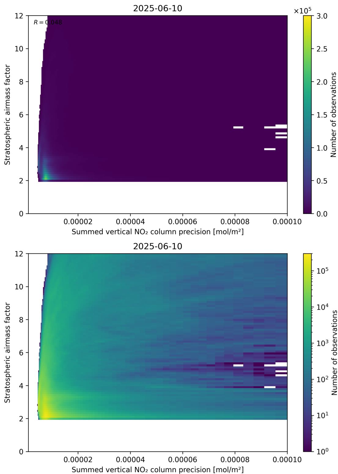
Figure 106: Scatter density plot of “Summed vertical NO 2 column precision” against “Stratospheric airmass factor” for 2025-06-09 to 2025-06-11.
