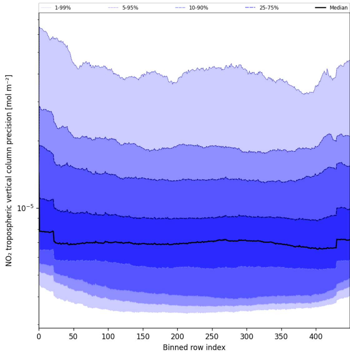
Figure 47: Along track statistics of “NO 2 tropospheric vertical column precision” for 2025-06-09 to 2025-06-11
