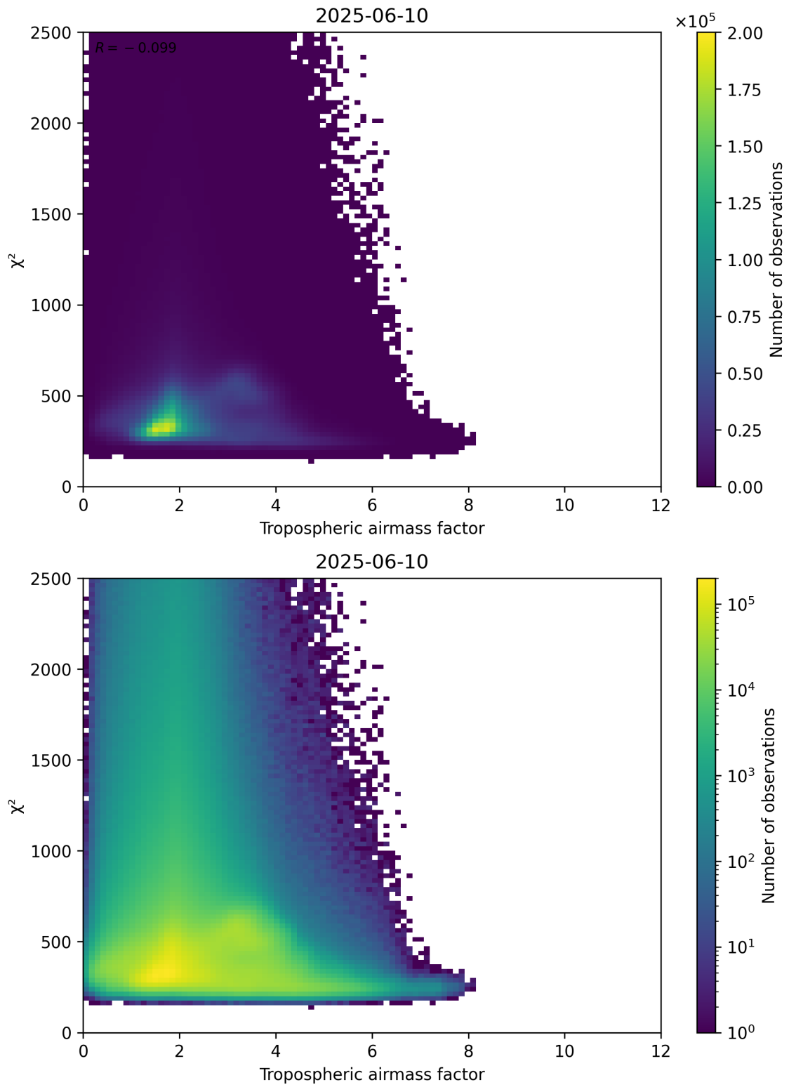
Figure 73: Scatter density plot of “Tropospheric airmass factor” against “ \chi^2 ” for 2025-06-09 to 2025-06-11.
