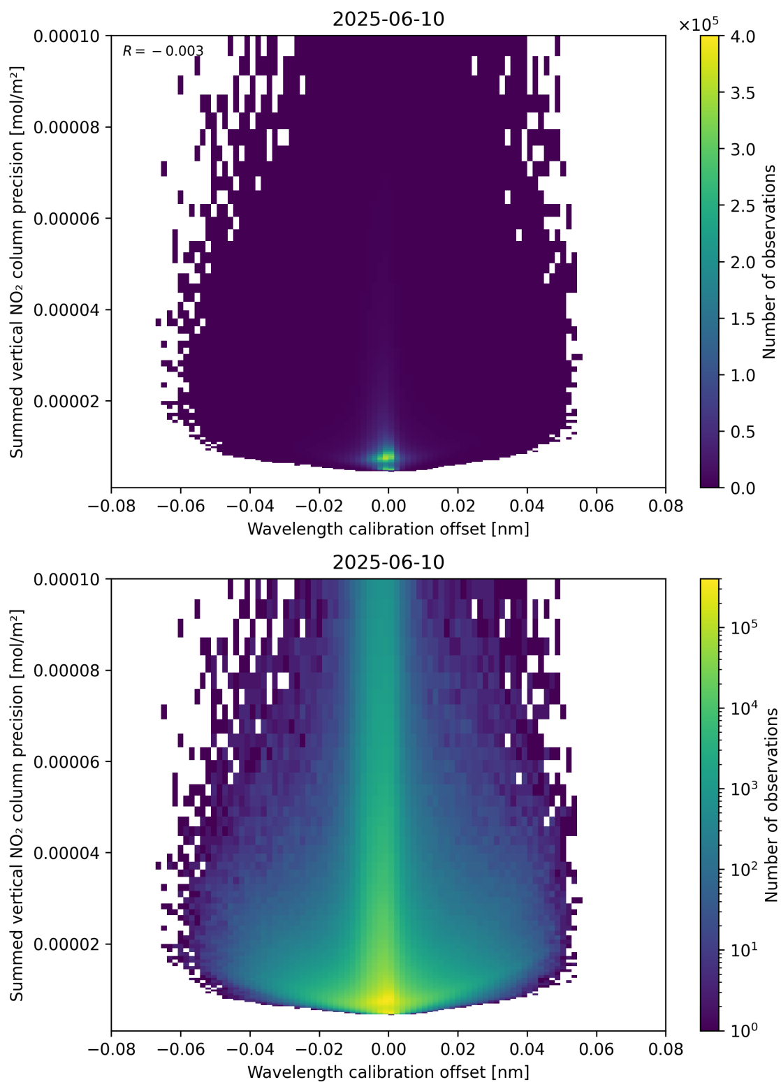
Figure 178: Scatter density plot of “Wavelength calibration offset” against “Summed vertical NO 2 column precision” for 2025-06-09 to 2025-06-11.
