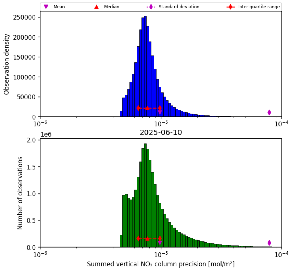
Figure 41: Histogram of "Summed vertical NO 2 column precision" for 2025-06-09 to 2025-06-11
