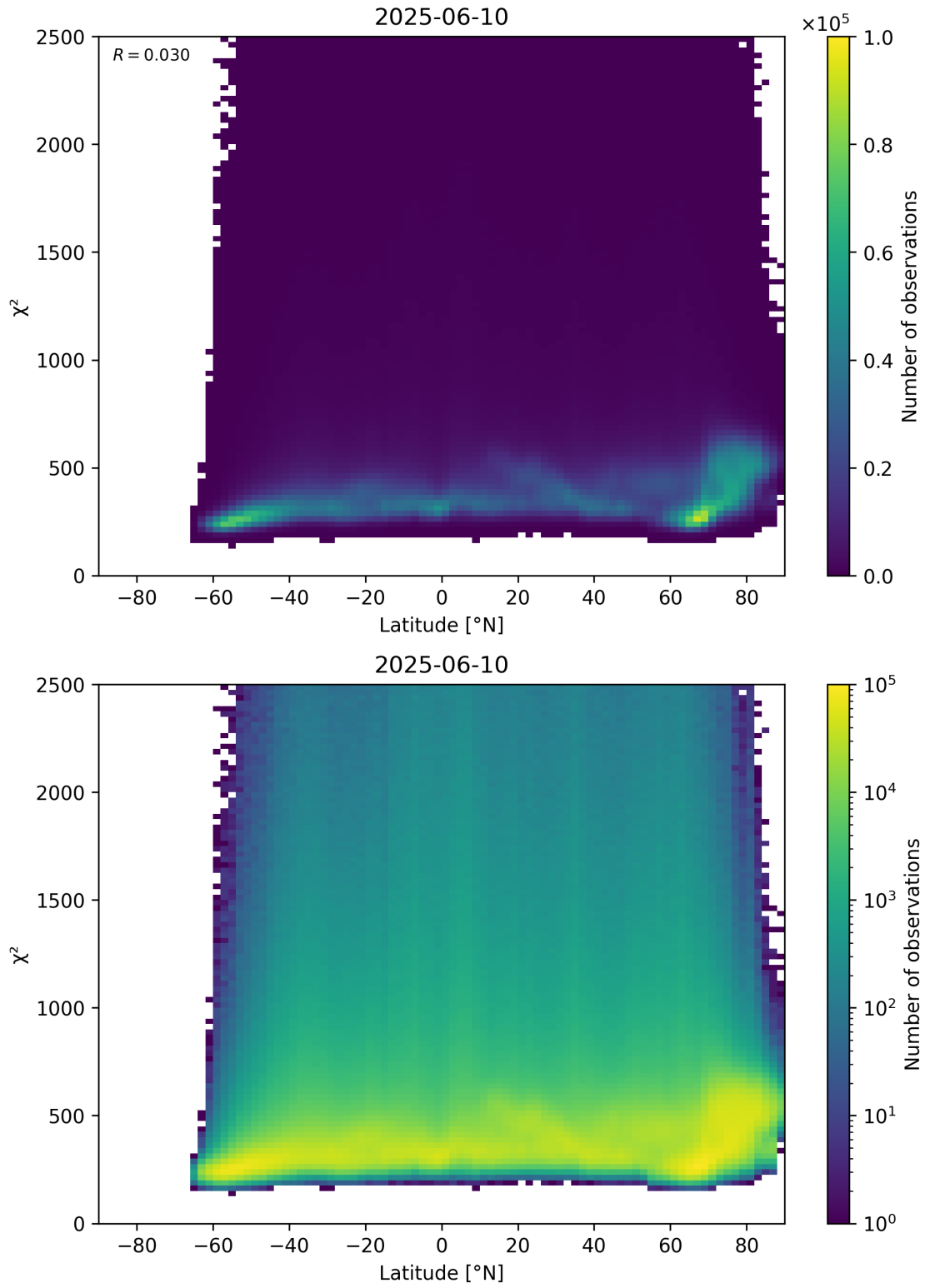
Figure 86: Scatter density plot of “Latitude” against “ \chi^2 ” for 2025-06-09 to 2025-06-11.
