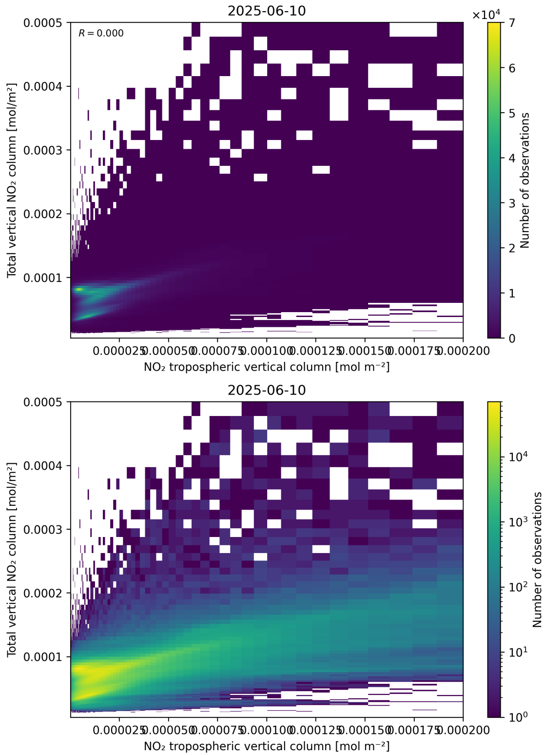
Figure 128: Scatter density plot of “NO 2 tropospheric vertical column” against “Total vertical NO 2 column” for 2025-06-09 to 2025-06-11.
