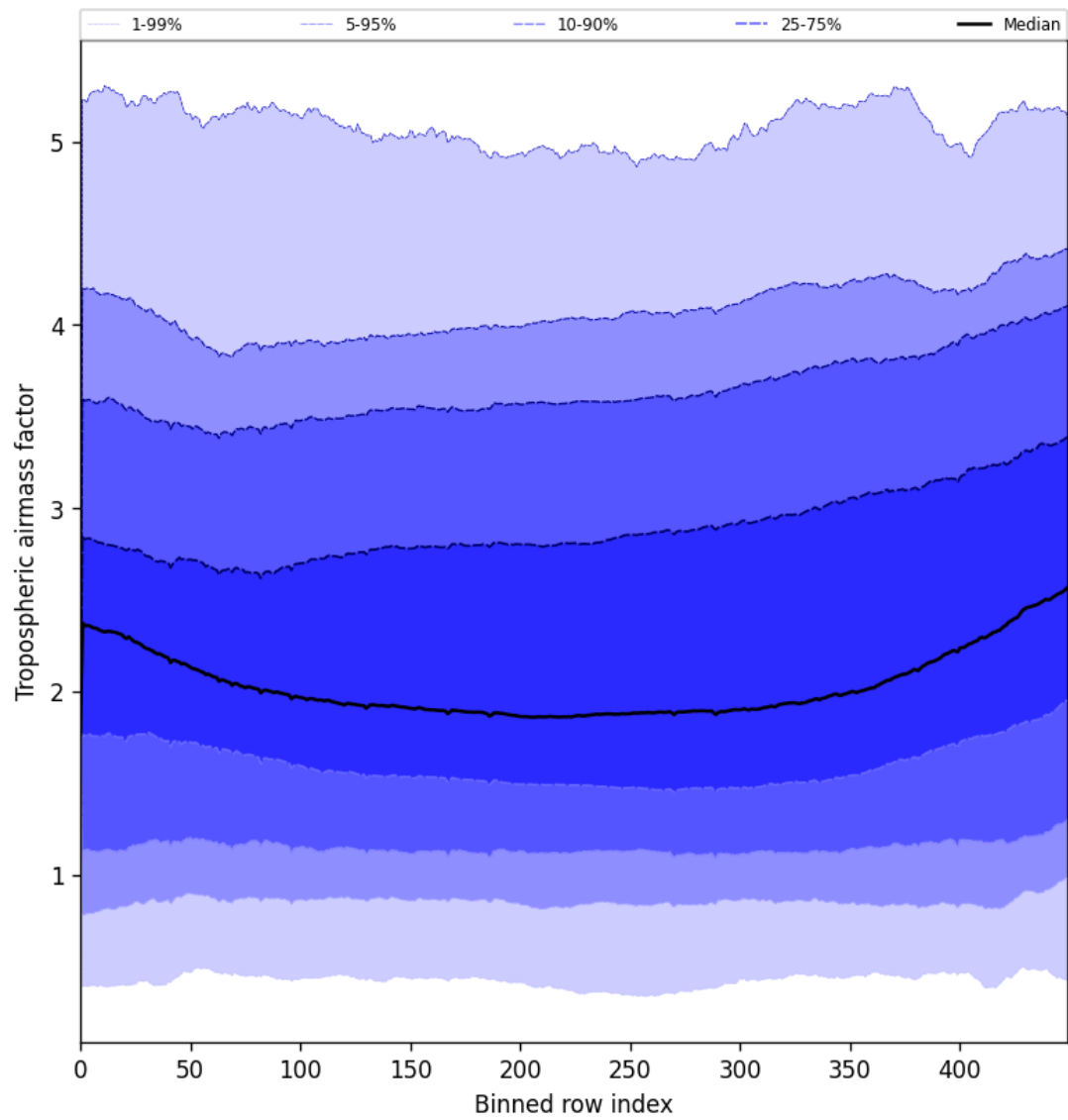
Figure 48: Along track statistics of “Tropospheric airmass factor” for 2025-06-09 to 2025-06-11
