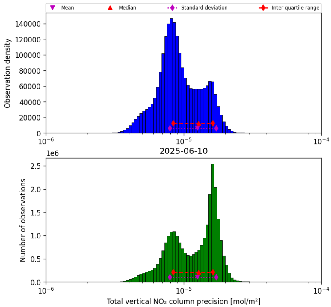
Figure 39: Histogram of “Total vertical NO 2 column precision” for 2025-06-09 to 2025-06-11
