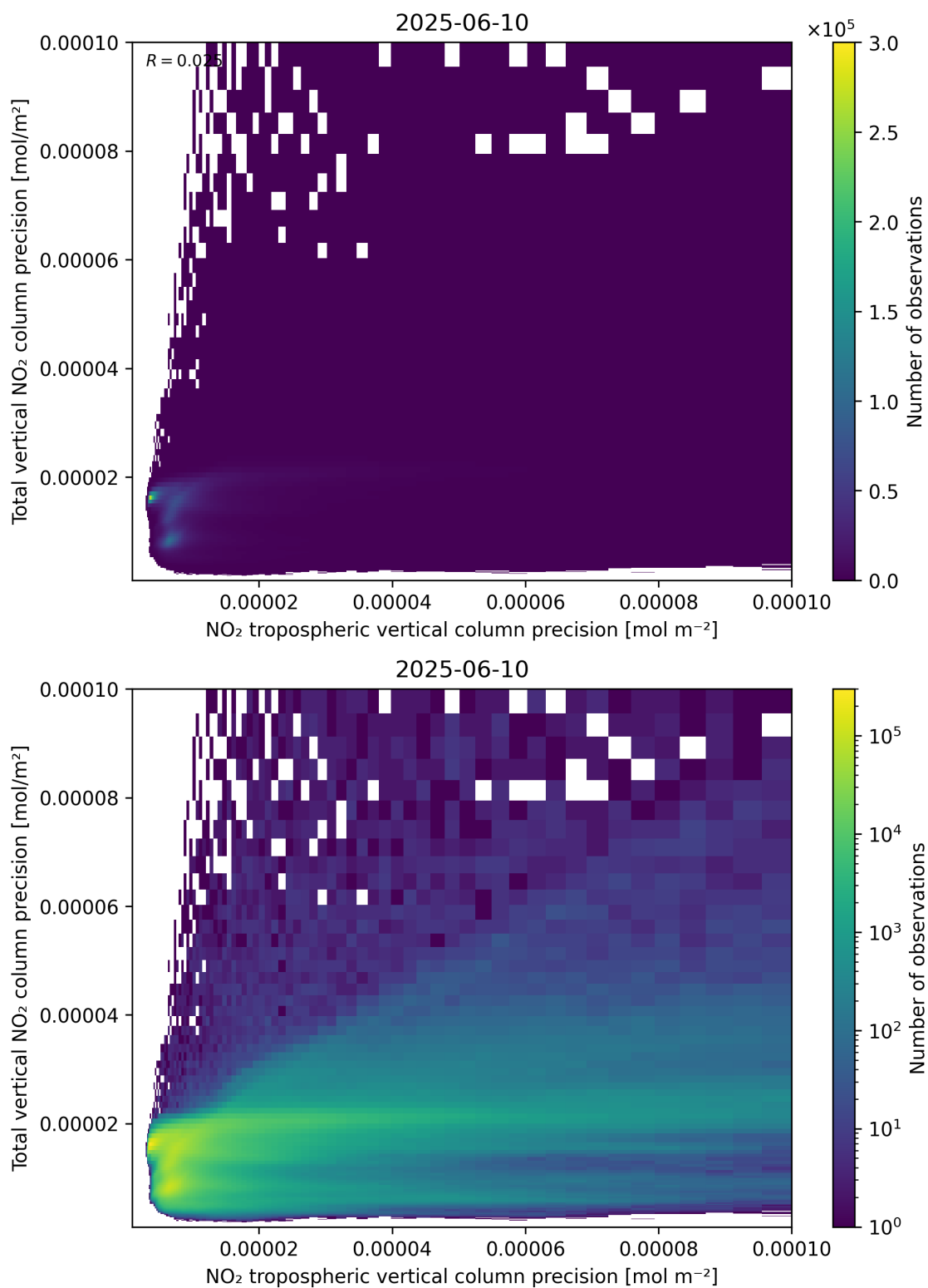
Figure 139: Scatter density plot of “NO 2 tropospheric vertical column precision” against “Total vertical NO 2 column precision” for 2025-06-09 to 2025-06-11.
