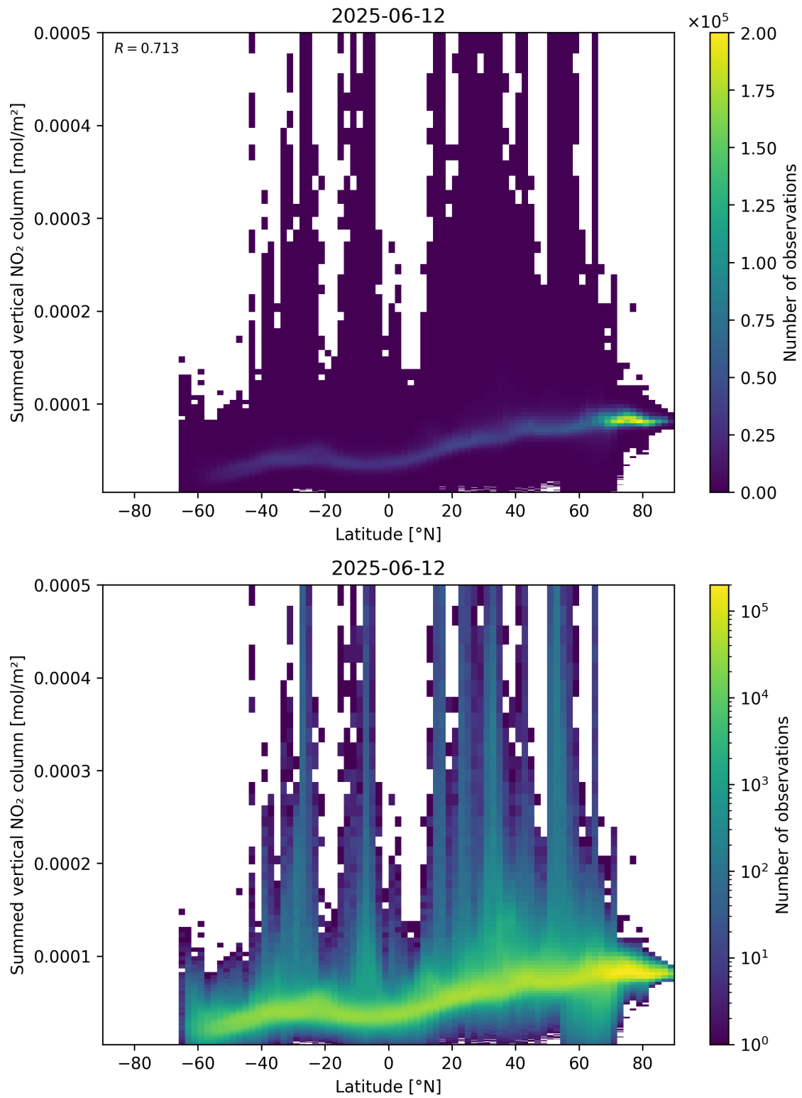
Figure 88: Scatter density plot of “Latitude” against “Summed vertical NO 2 column” for 2025-06-11 to 2025-06-13.
