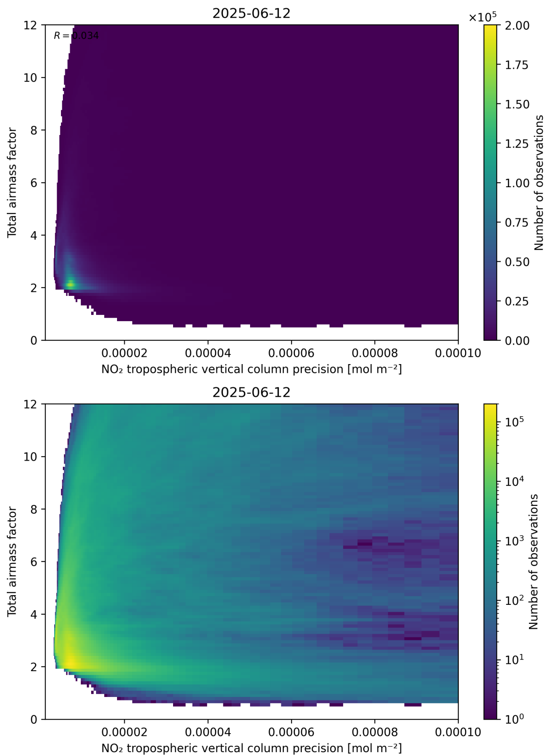
Figure 132: Scatter density plot of “NO 2 tropospheric vertical column precision” against “Total air mass factor” for 2025-06-11 to 2025-06-13.
