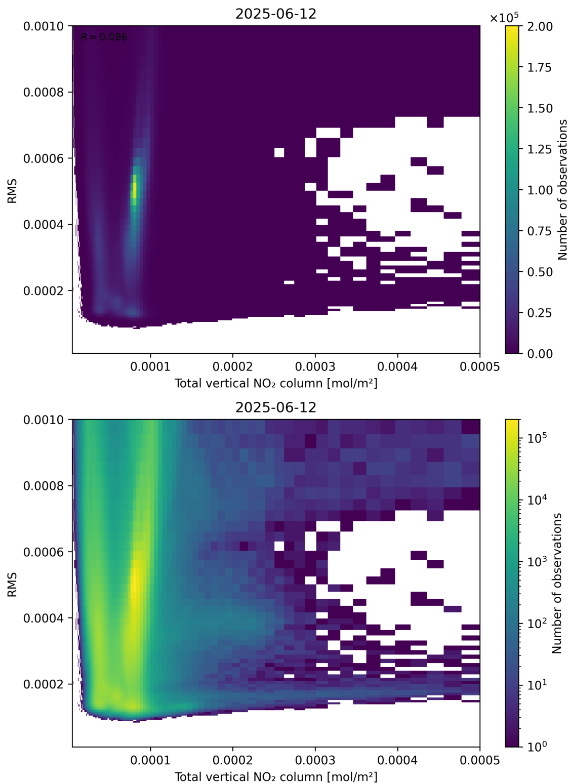
Figure 120: Scatter density plot of “Total vertical NO 2 column” against “RMS” for 2025-06-11 to 2025-06-13.
