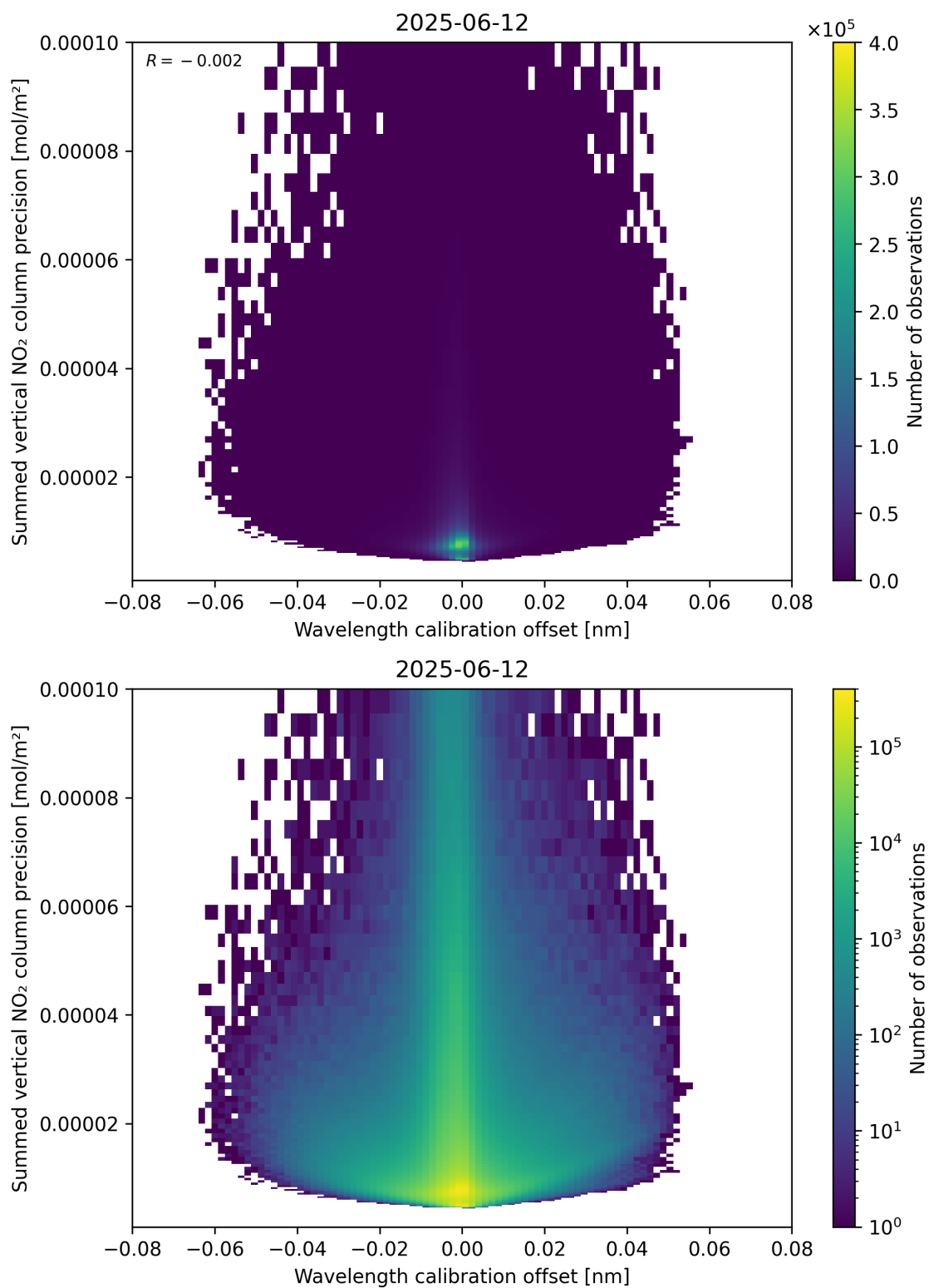
Figure 178: Scatter density plot of “Wavelength calibration offset” against “Summed vertical NO 2 column precision” for 2025-06-11 to 2025-06-13.
