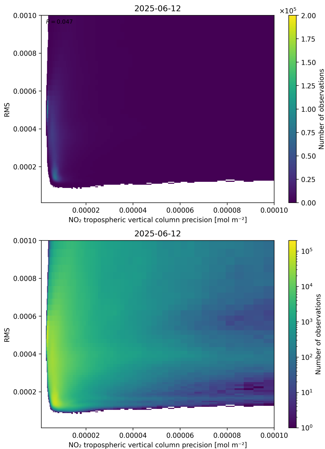
Figure 140: Scatter density plot of “NO 2 tropospheric vertical column precision” against “RMS” for 2025-06-11 to 2025-06-13.
