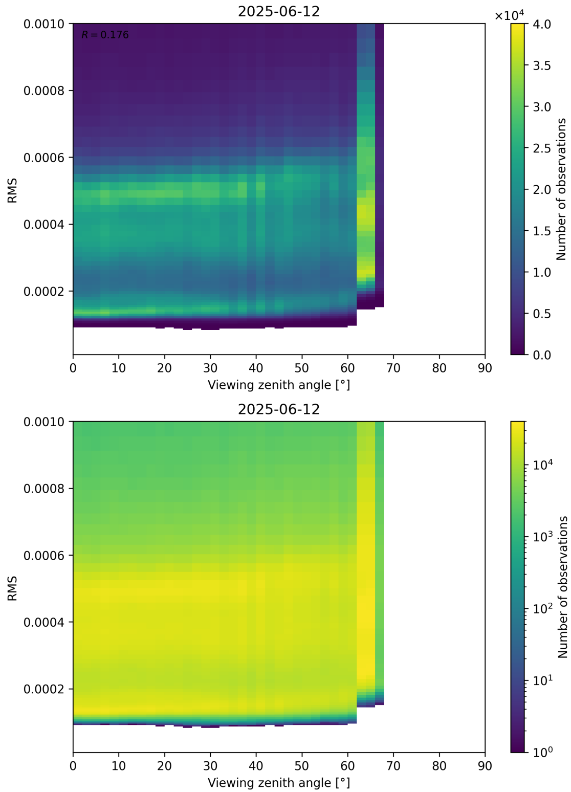
Figure 171: Scatter density plot of “Viewing zenith angle” against “RMS” for 2025-06-11 to 2025-06-13.
