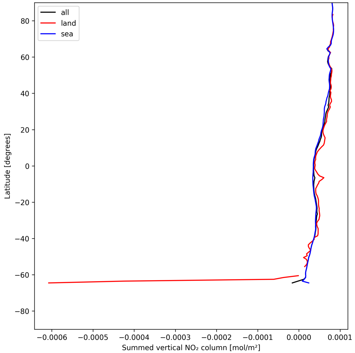
Figure 23: Zonal average of “Summed vertical NO 2 column” for 2025-06-11 to 2025-06-13.
