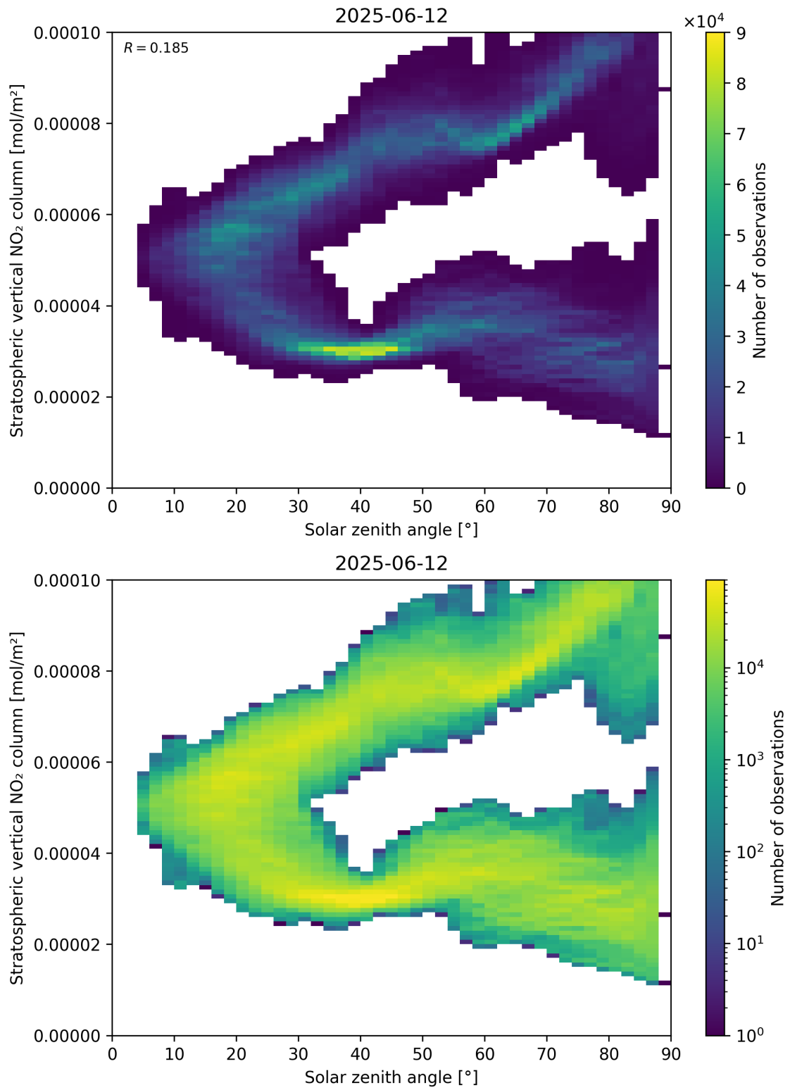
Figure 150: Scatter density plot of “Solar zenith angle” against “Stratospheric vertical NO 2 column” for 2025-06-11 to 2025-06-13.
