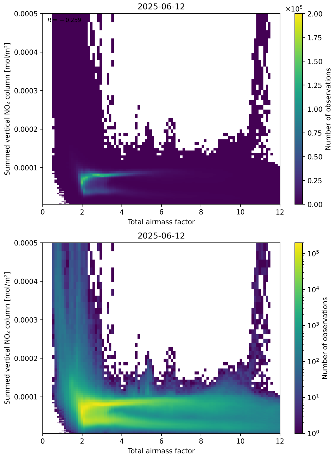
Figure 65: Scatter density plot of “Total airmass factor” against “Summed vertical NO 2 column” for 2025-06-11 to 2025-06-13.
