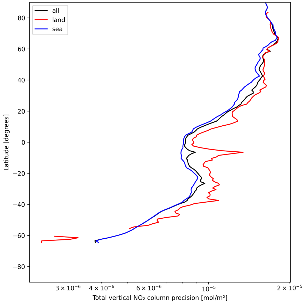
Figure 22: Zonal average of “Total vertical NO 2 column precision” for 2025-06-11 to 2025-06-13.
