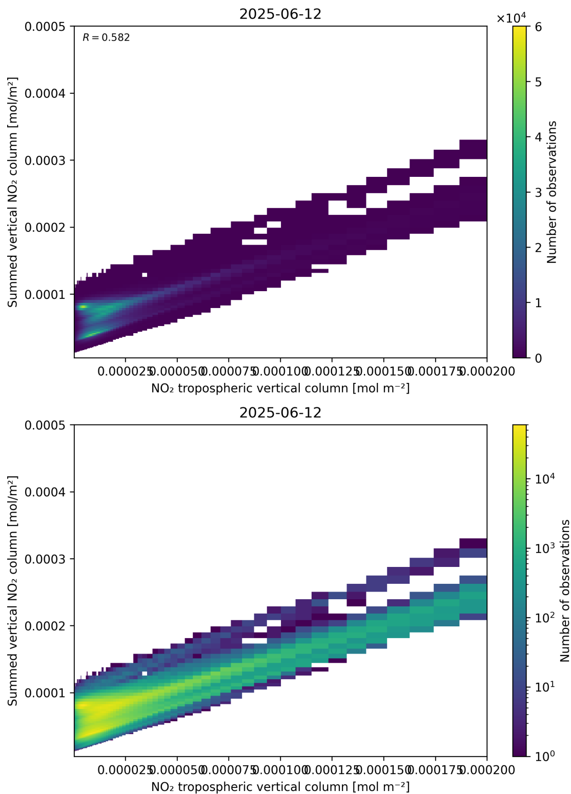
Figure 126: Scatter density plot of “NO 2 tropospheric vertical column” against “Summed vertical NO 2 column” for 2025-06-11 to 2025-06-13.
