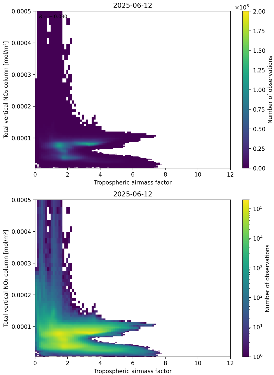
Figure 77: Scatter density plot of “Tropospheric airmass factor” against “Total vertical NO 2 column” for 2025-06-11 to 2025-06-13.
