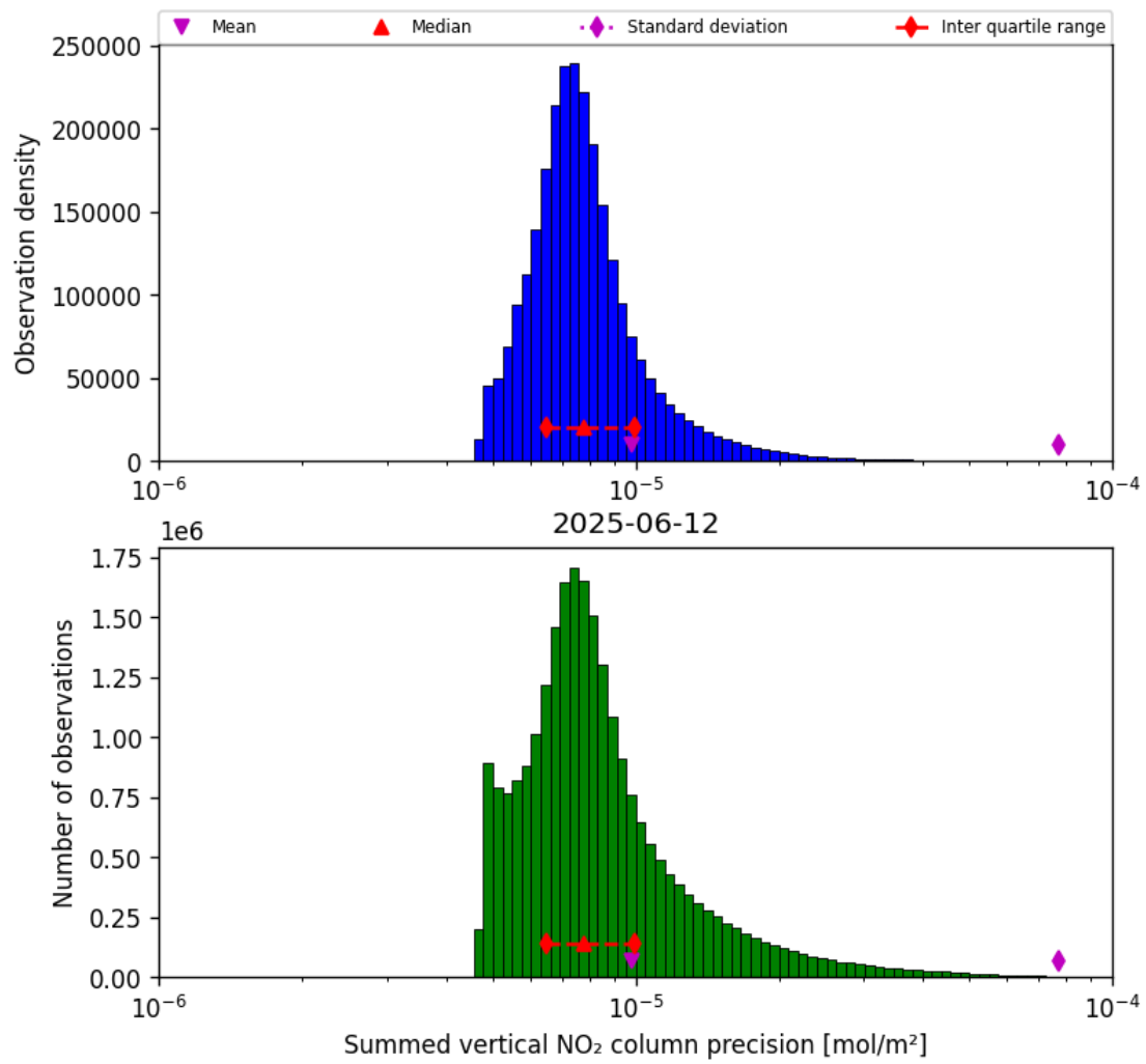
Figure 41: Histogram of “Summed vertical NO 2 column precision” for 2025-06-11 to 2025-06-13
