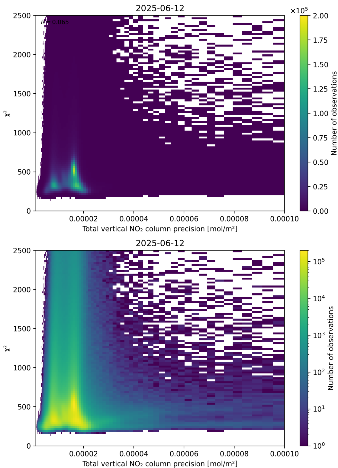
Figure 116: Scatter density plot of “Total vertical NO 2 column precision” against “ \chi^2 ” for 2025-06-11 to 2025-06-13.
