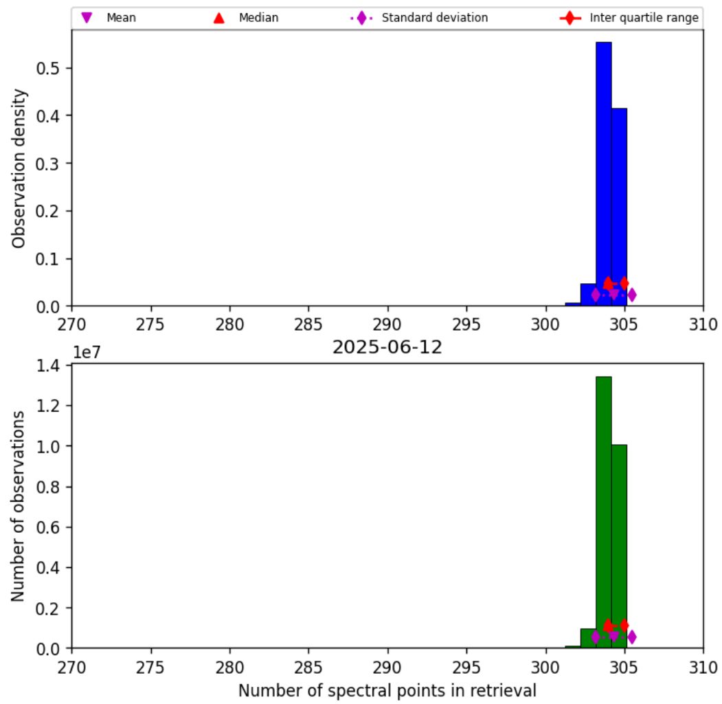
Figure 33: Histogram of “Number of spectral points in retrieval” for 2025-06-11 to 2025-06-13
