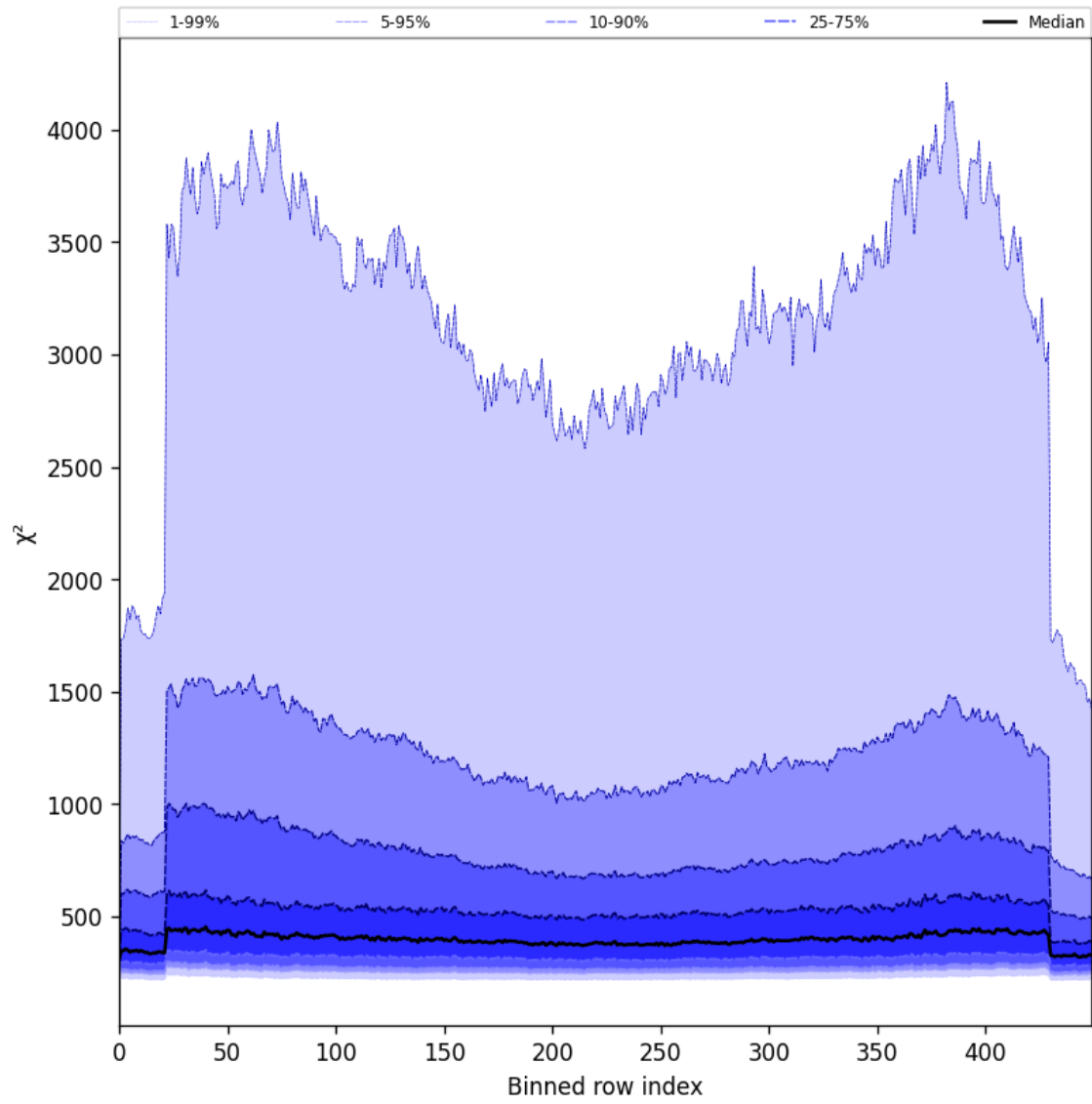
Figure 59: Along track statistics of “ \chi^2 ” for 2025-06-11 to 2025-06-13
