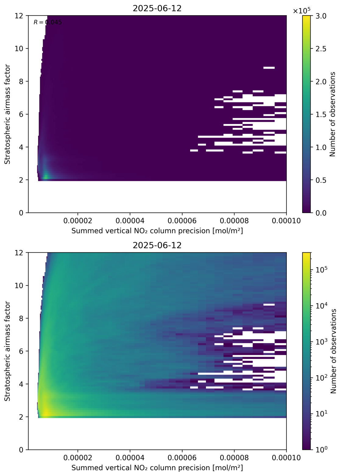
Figure 106: Scatter density plot of “Summed vertical NO 2 column precision” against “Stratospheric airmass factor” for 2025-06-11 to 2025-06-13.
