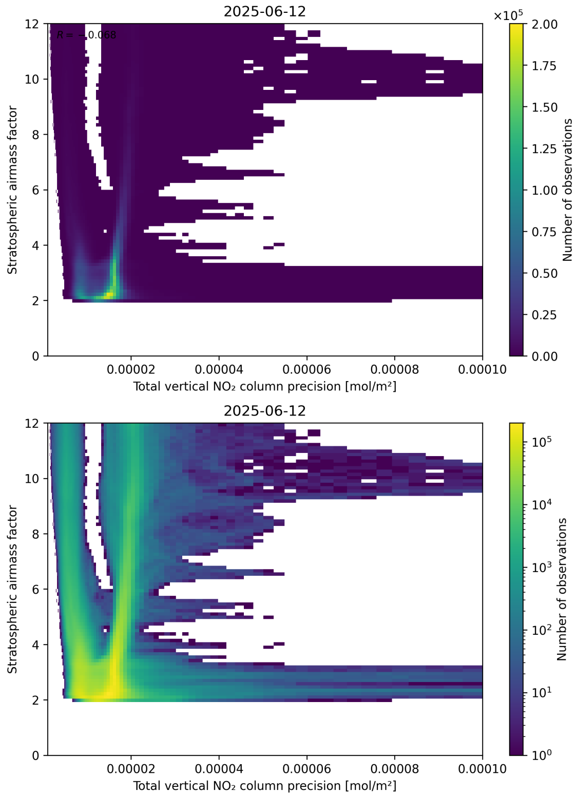
Figure 115: Scatter density plot of “Total vertical NO 2 column precision” against “Stratospheric air mass factor” for 2025-06-11 to 2025-06-13.
