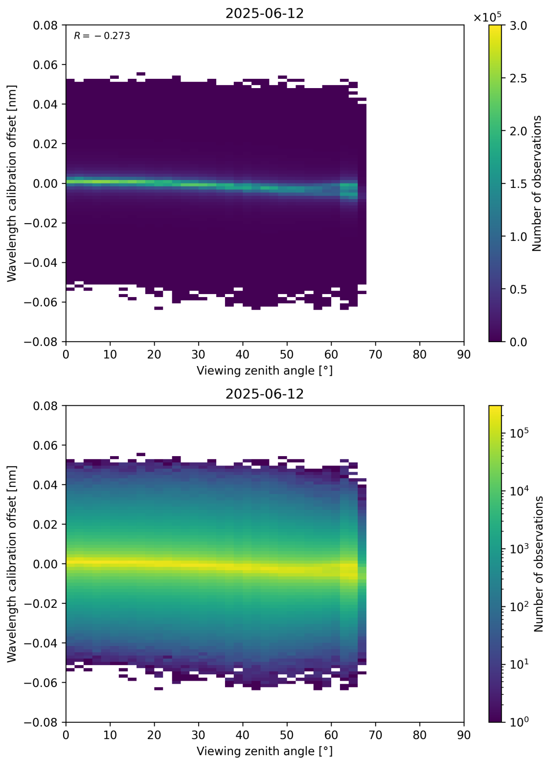
Figure 173: Scatter density plot of “Viewing zenith angle” against “Wavelength calibration offset” for 2025-06-11 to 2025-06-13.
