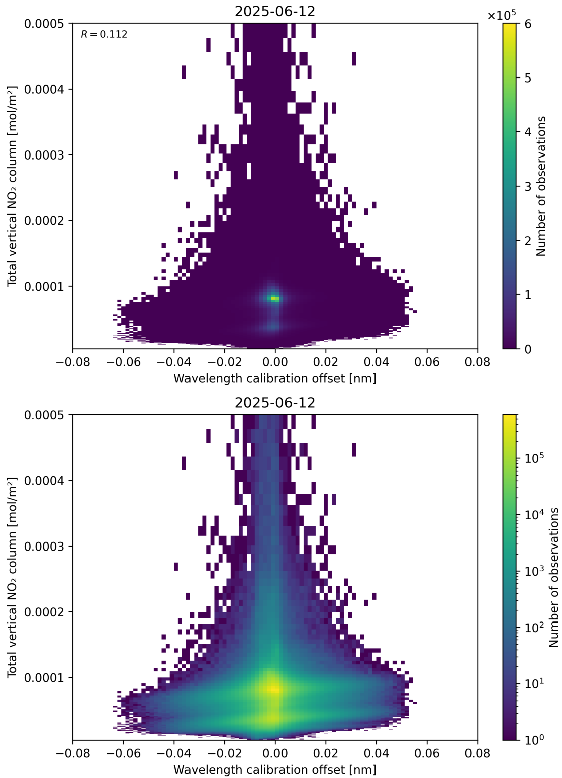
Figure 179: Scatter density plot of “Wavelength calibration offset” against “Total vertical NO 2 column” for 2025-06-11 to 2025-06-13.
