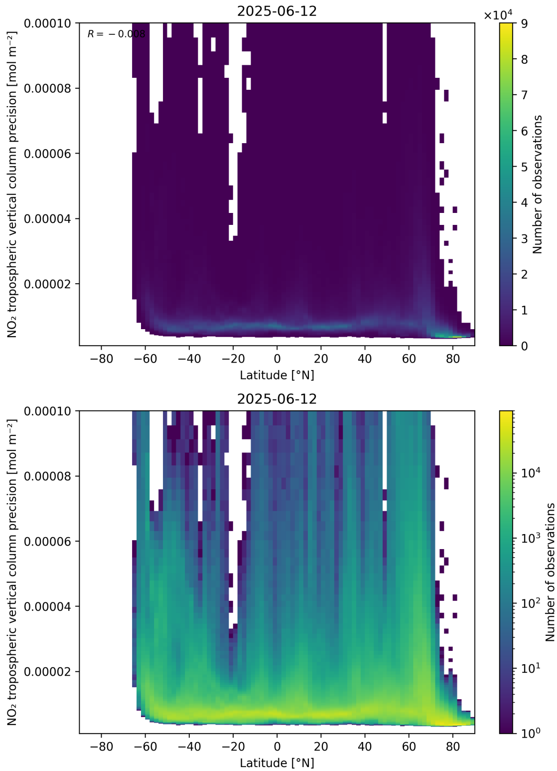
Figure 93: Scatter density plot of “Latitude” against “NO 2 tropospheric vertical column precision” for 2025-06-11 to 2025-06-13.
