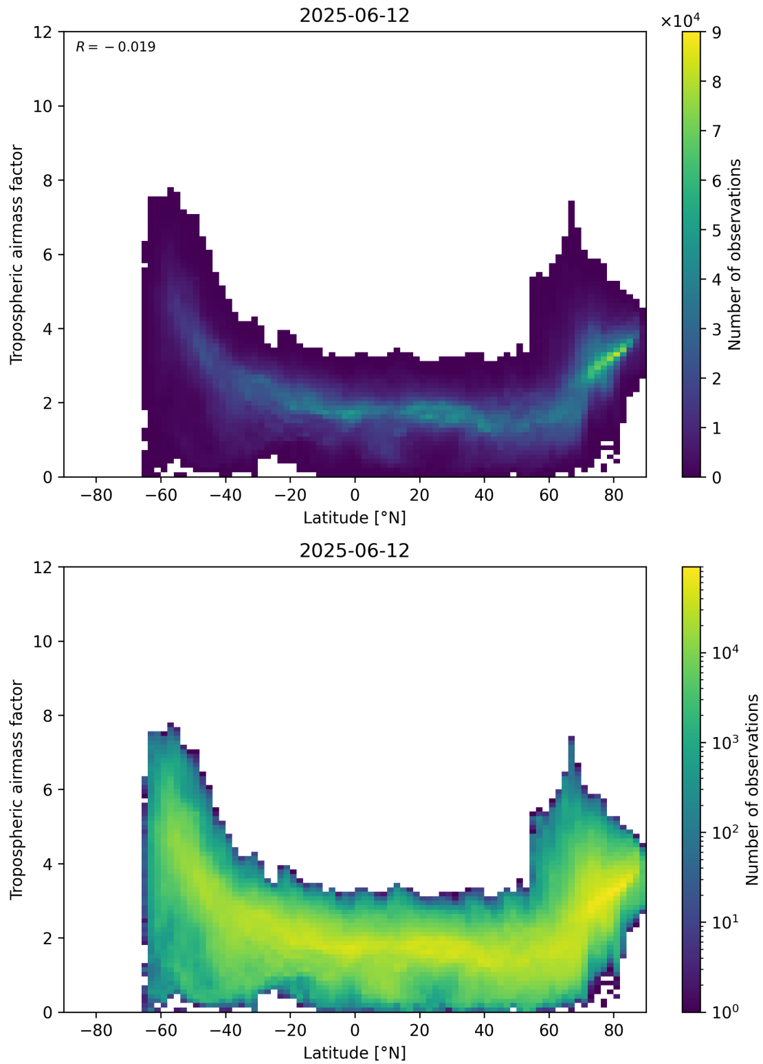
Figure 85: Scatter density plot of “Latitude” against “Tropospheric air mass factor” for 2025-06-11 to 2025-06-13.
