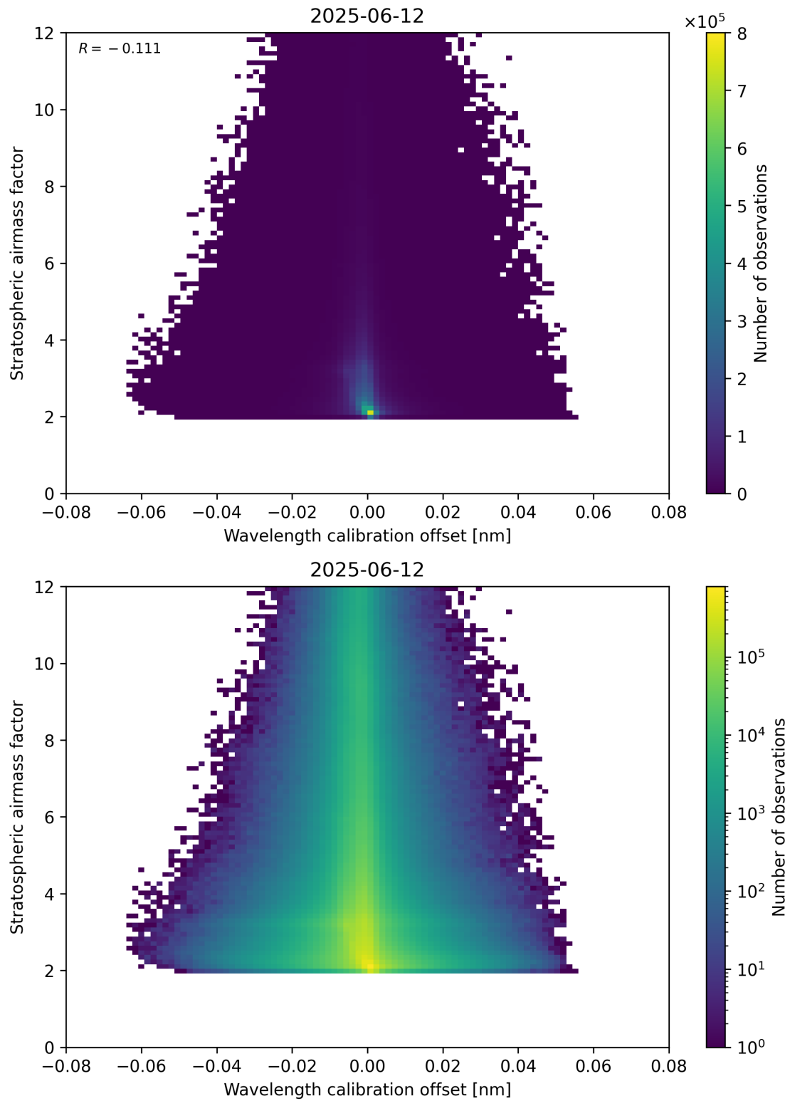
Figure 174: Scatter density plot of “Wavelength calibration offset” against “Stratospheric airmass factor” for 2025-06-11 to 2025-06-13.
