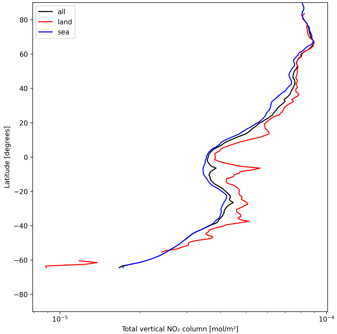
Figure 21: Zonal average of “Total vertical NO 2 column” for 2025-06-11 to 2025-06-13.
