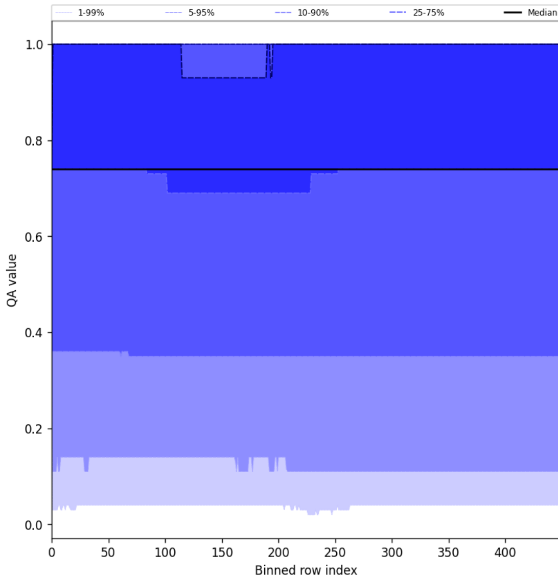
Figure 45: Along track statistics of “QA value” for 2025-06-11 to 2025-06-13
