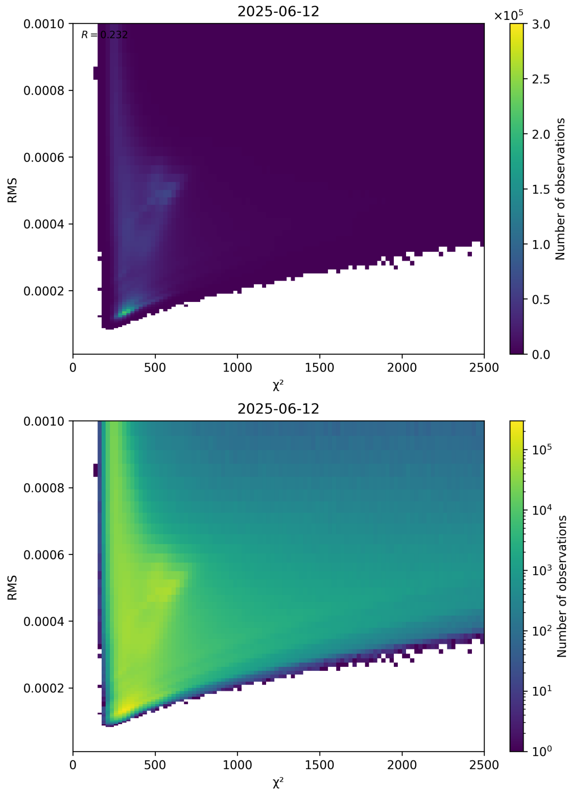
Figure 82: Scatter density plot of “ \chi^2 ” against “RMS” for 2025-06-11 to 2025-06-13.
