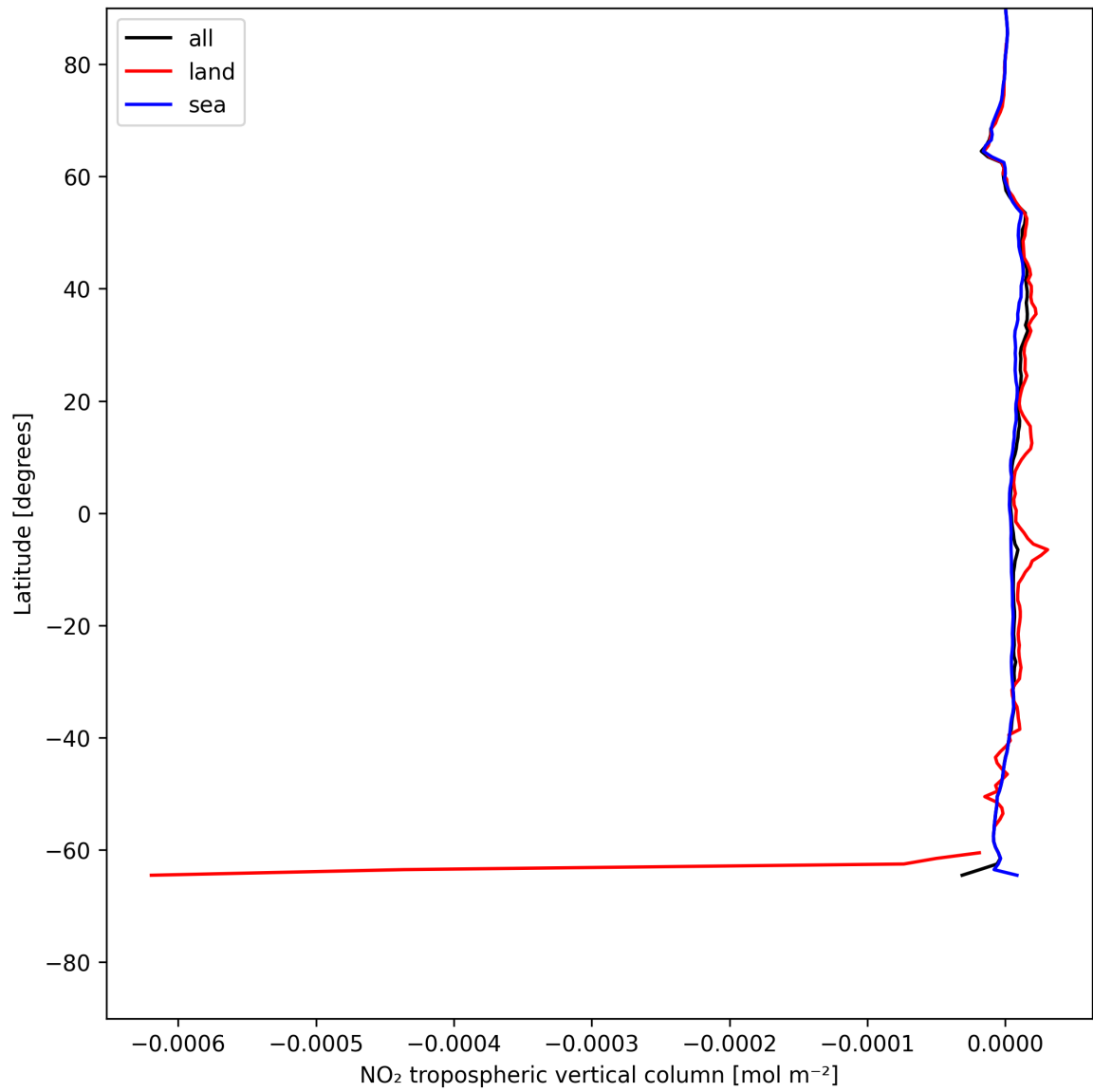
Figure 12: Zonal average of “NO 2 tropospheric vertical column” for 2025-06-11 to 2025-06-13.
