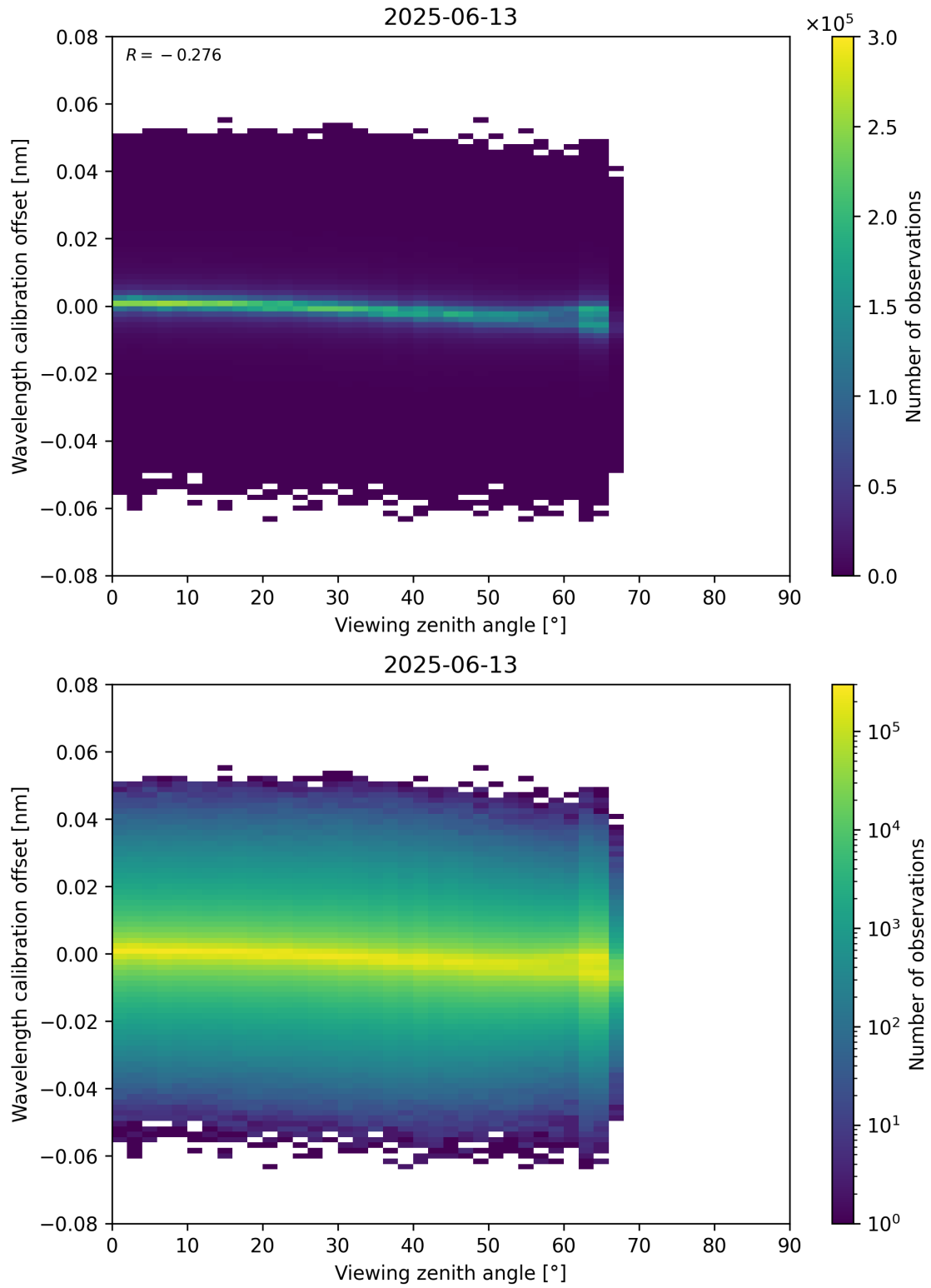
Figure 173: Scatter density plot of “Viewing zenith angle” against “Wavelength calibration offset” for 2025-06-12 to 2025-06-14.
