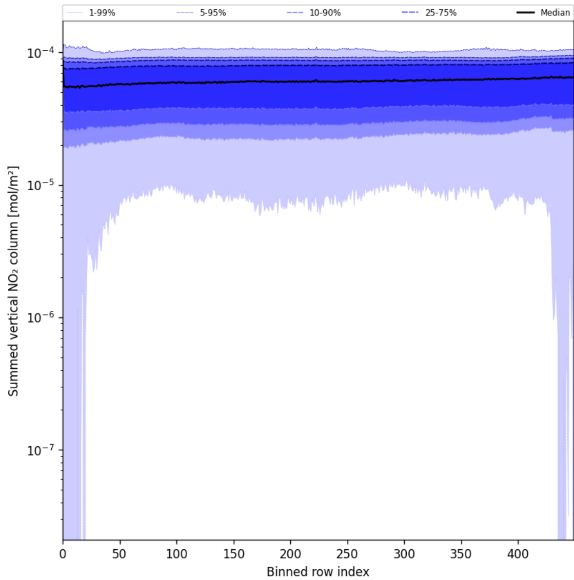
Figure 57: Along track statistics of “Summed vertical NO 2 column” for 2025-06-12 to 2025-06-14
