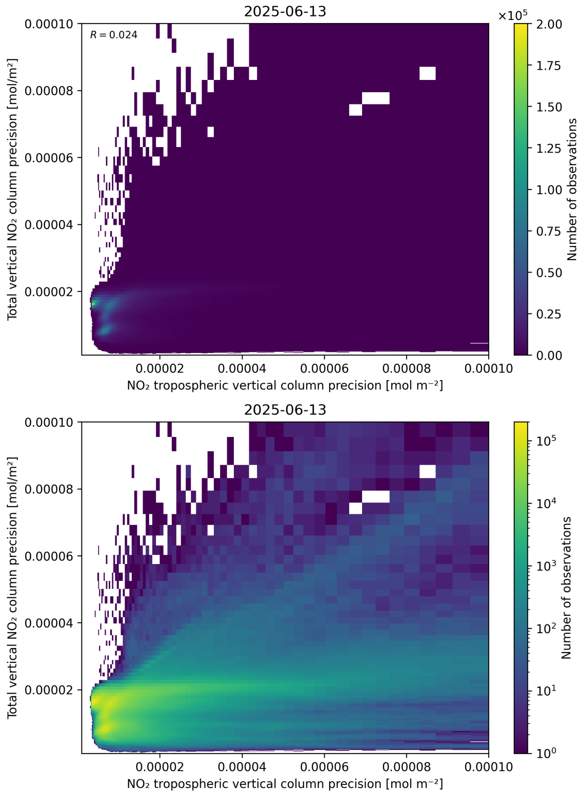
Figure 139: Scatter density plot of “NO 2 tropospheric vertical column precision” against “Total vertical NO 2 column precision” for 2025-06-12 to 2025-06-14.
