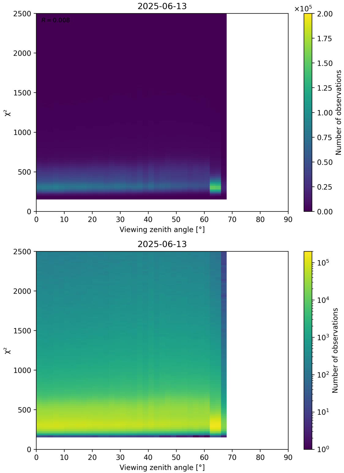
Figure 162: Scatter density plot of “Viewing zenith angle” against “ \chi^2 ” for 2025-06-12 to 2025-06-14.
