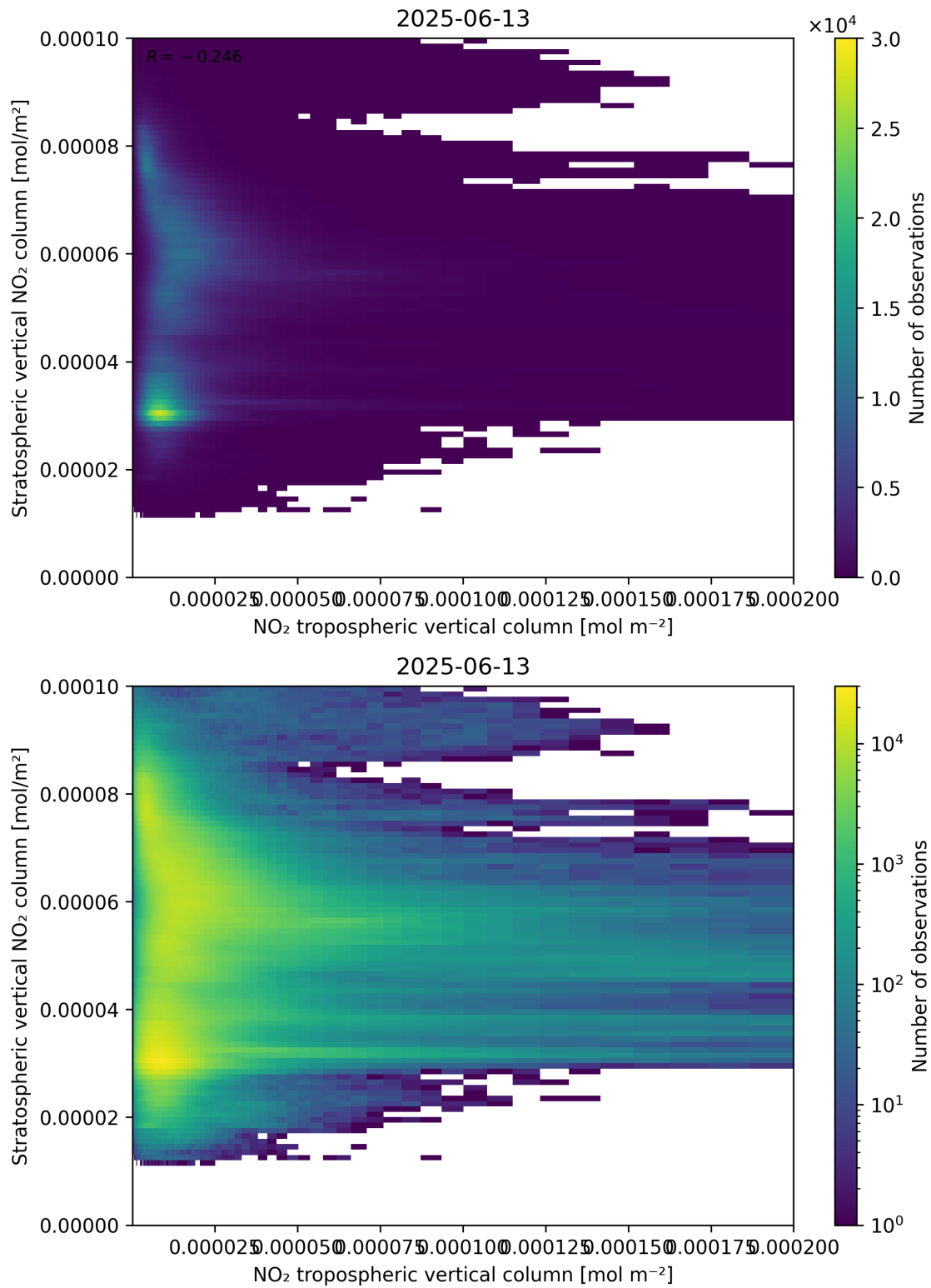
Figure 125: Scatter density plot of “NO 2 tropospheric vertical column” against “Stratospheric vertical NO 2 column” for 2025-06-12 to 2025-06-14.
