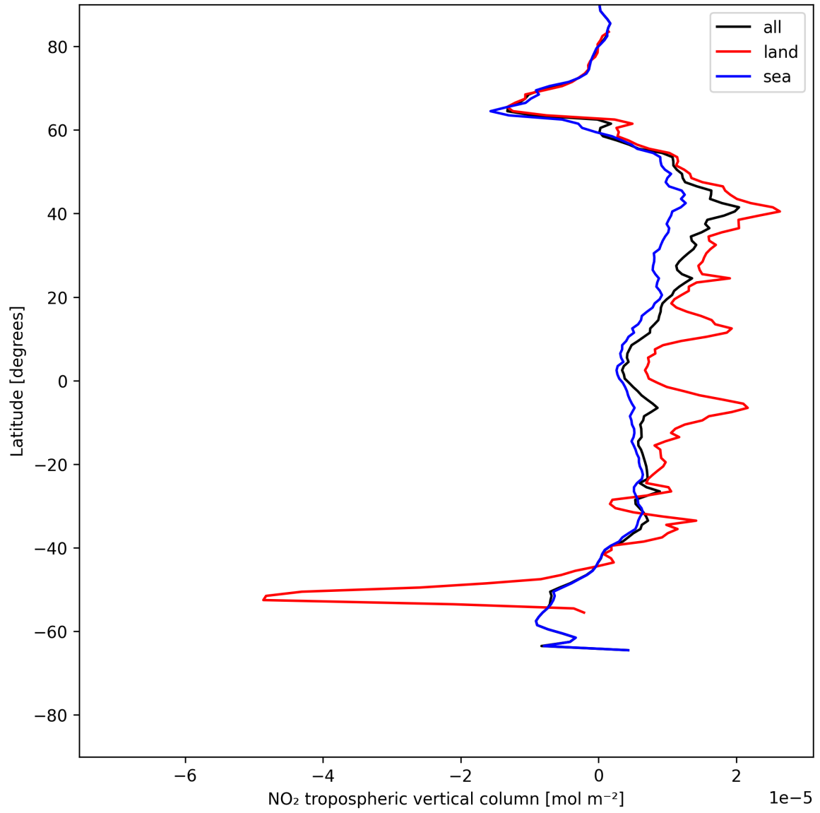
Figure 12: Zonal average of “NO 2 tropospheric vertical column” for 2025-06-12 to 2025-06-14.
