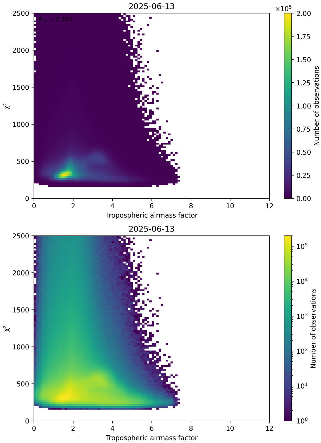
Figure 73: Scatter density plot of “Tropospheric airmass factor” against “ \chi^2 ” for 2025-06-12 to 2025-06-14.
