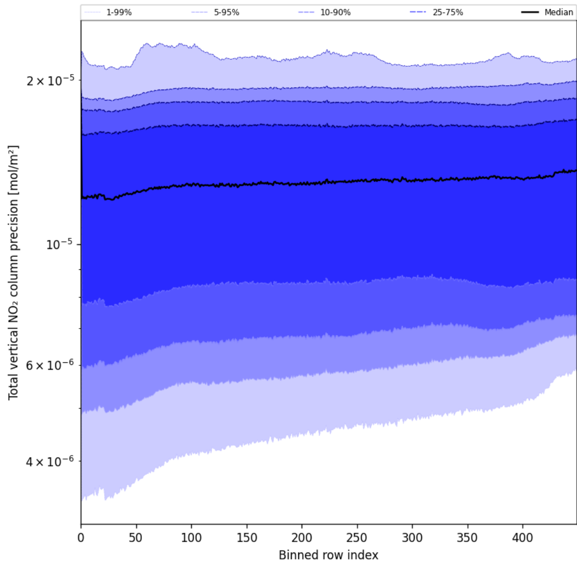
Figure 56: Along track statistics of “Total vertical NO 2 column precision” for 2025-06-12 to 2025-06-14
