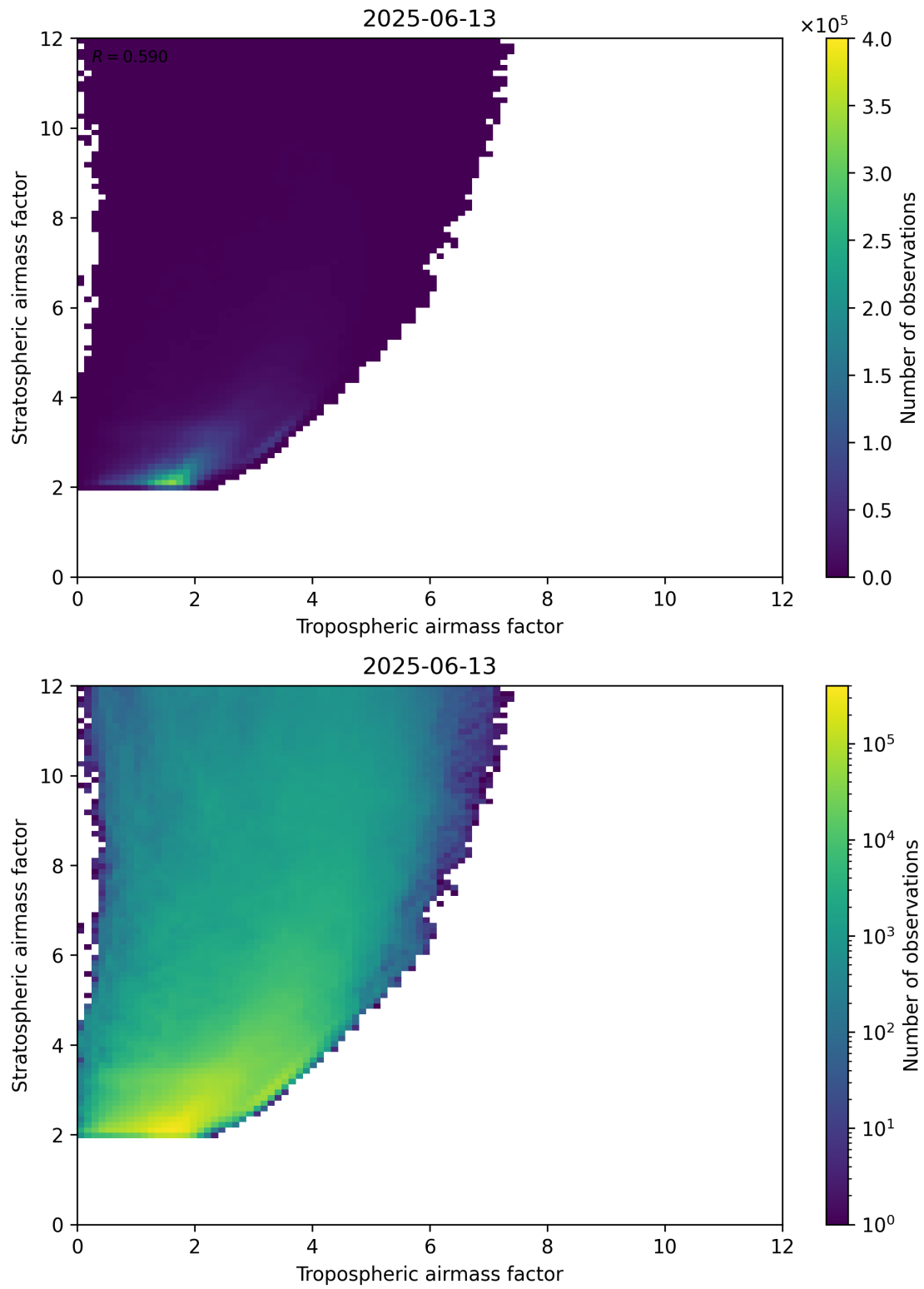
Figure 71: Scatter density plot of “Tropospheric airmass factor” against “Stratospheric airmass factor” for 2025-06-12 to 2025-06-14.
