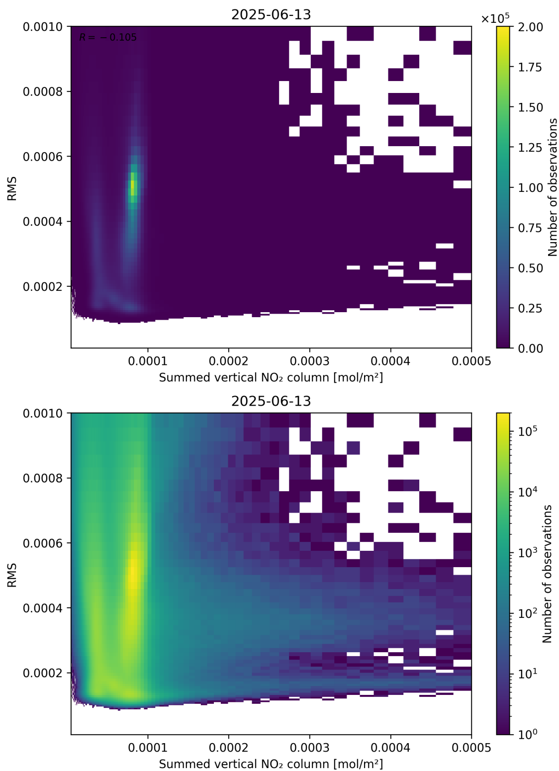
Figure 109: Scatter density plot of “Summed vertical NO 2 column” against “RMS” for 2025-06-12 to 2025-06-14.
