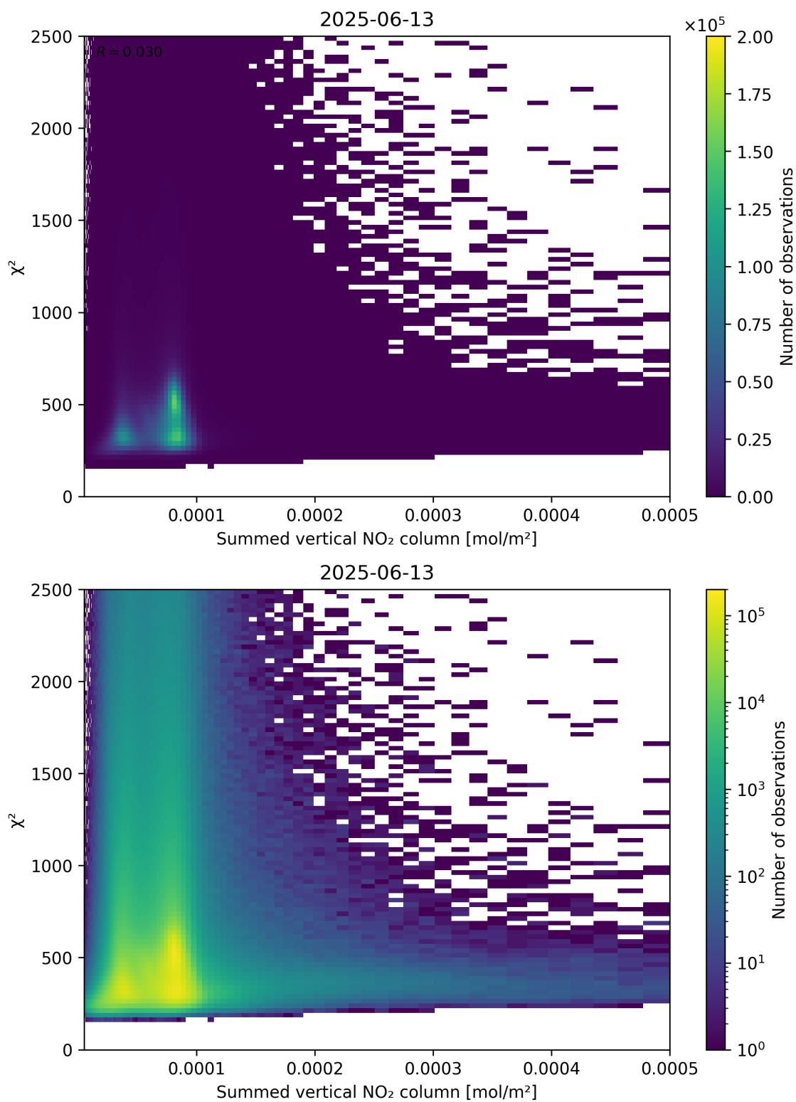
Figure 104: Scatter density plot of “Summed vertical NO 2 column” against “ \chi^2 ” for 2025-06-12 to 2025-06-14.
