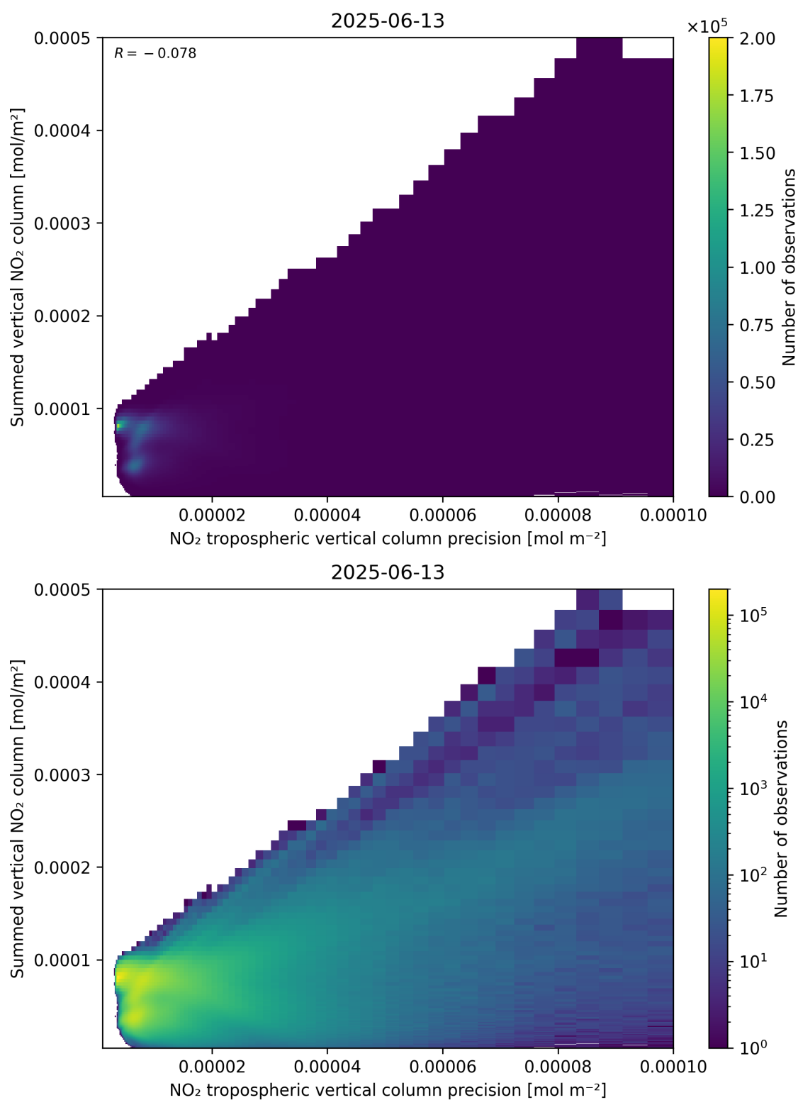
Figure 136: Scatter density plot of “NO 2 tropospheric vertical column precision” against “Summed vertical NO 2 column” for 2025-06-12 to 2025-06-14.
