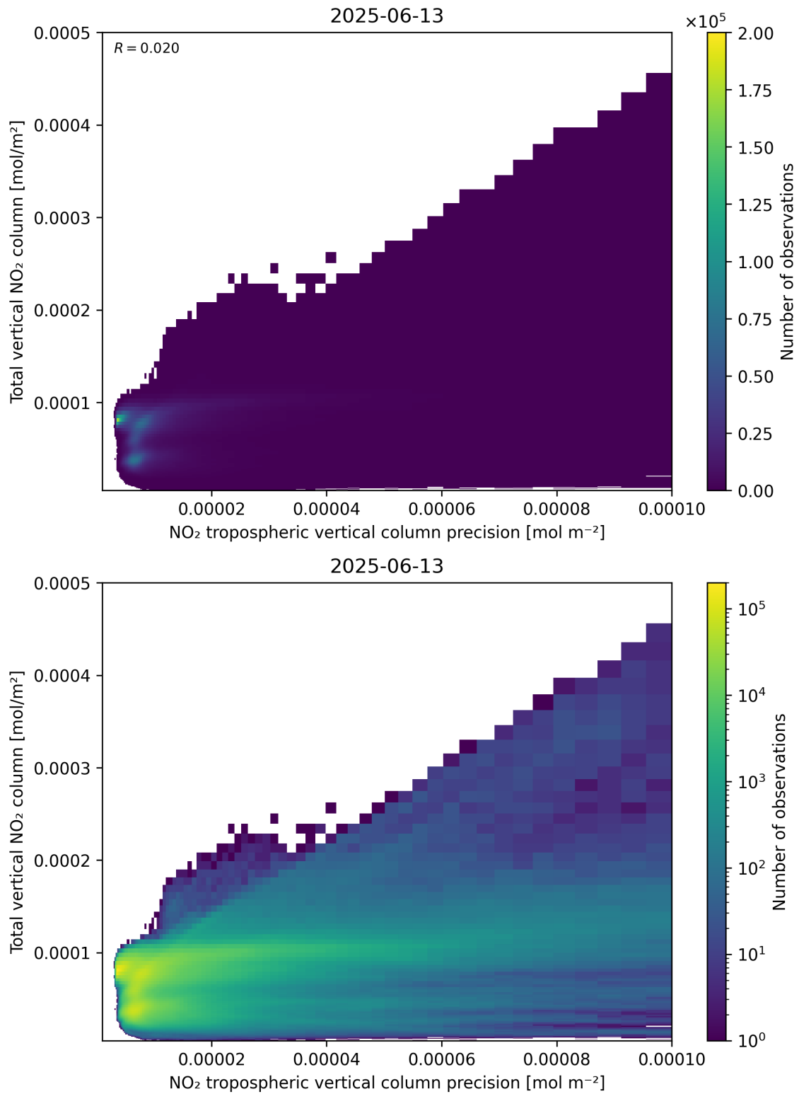
Figure 138: Scatter density plot of “NO 2 tropospheric vertical column precision” against “Total vertical NO 2 column” for 2025-06-12 to 2025-06-14.
