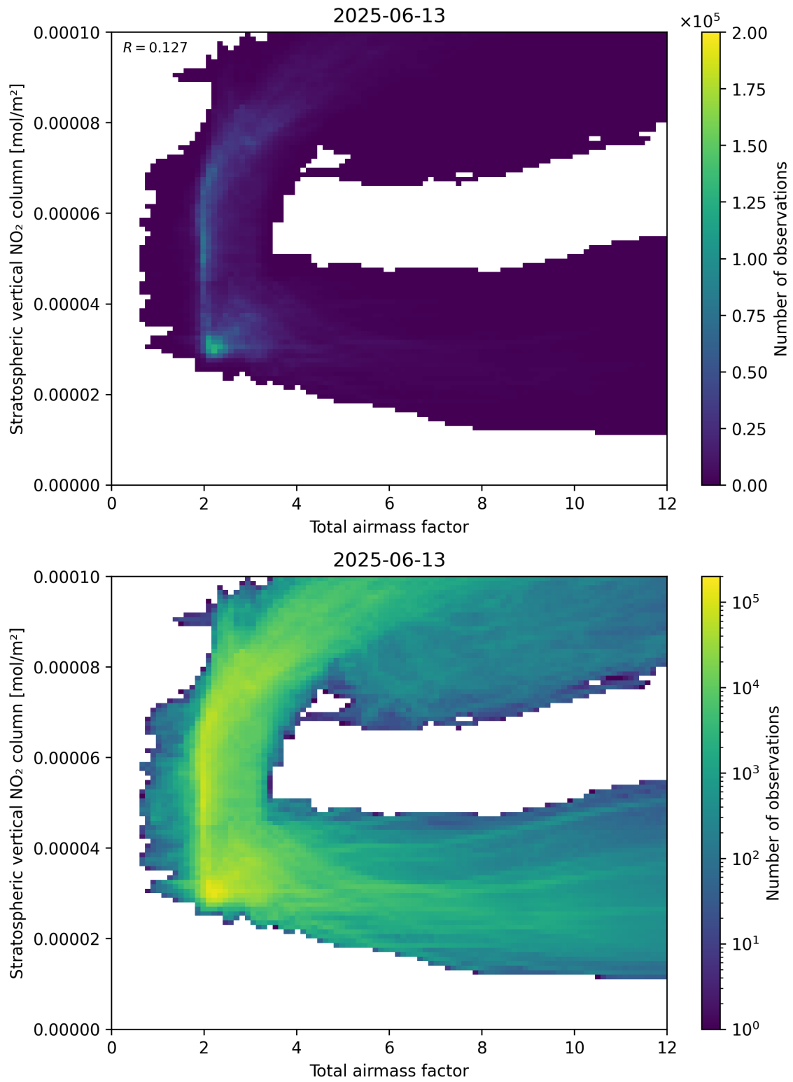
Figure 64: Scatter density plot of “Total airmass factor” against “Stratospheric vertical NO 2 column” for 2025-06-12 to 2025-06-14.
