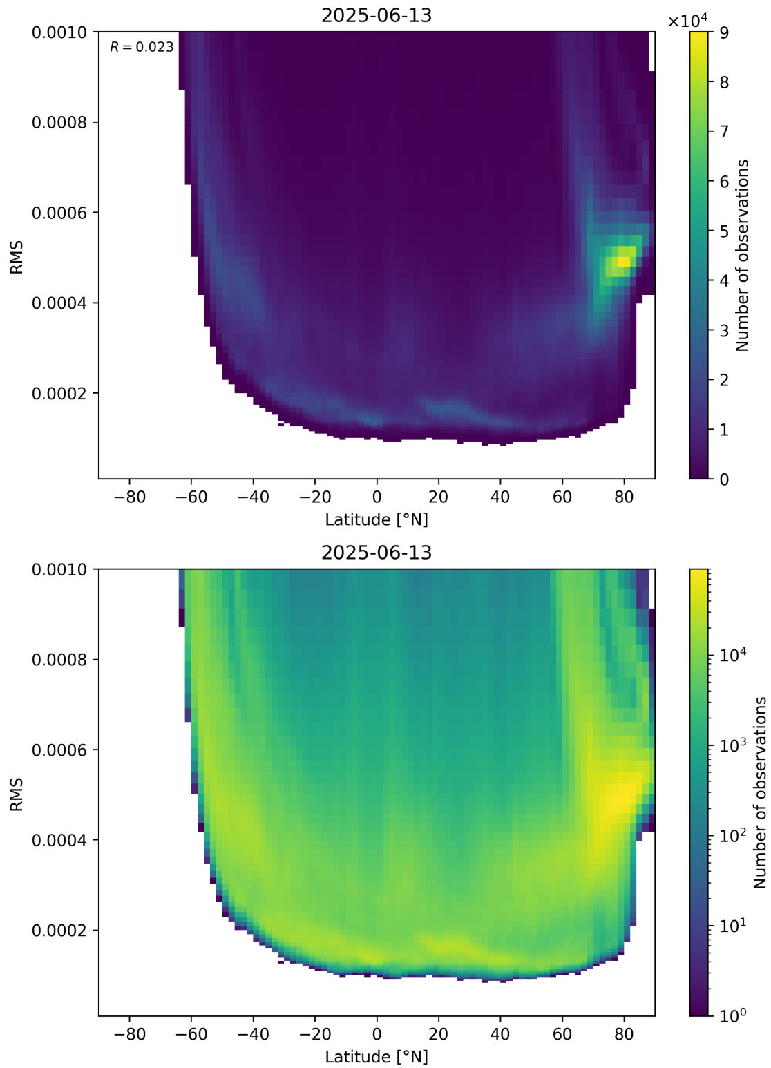
Figure 94: Scatter density plot of “Latitude” against “RMS” for 2025-06-12 to 2025-06-14.
