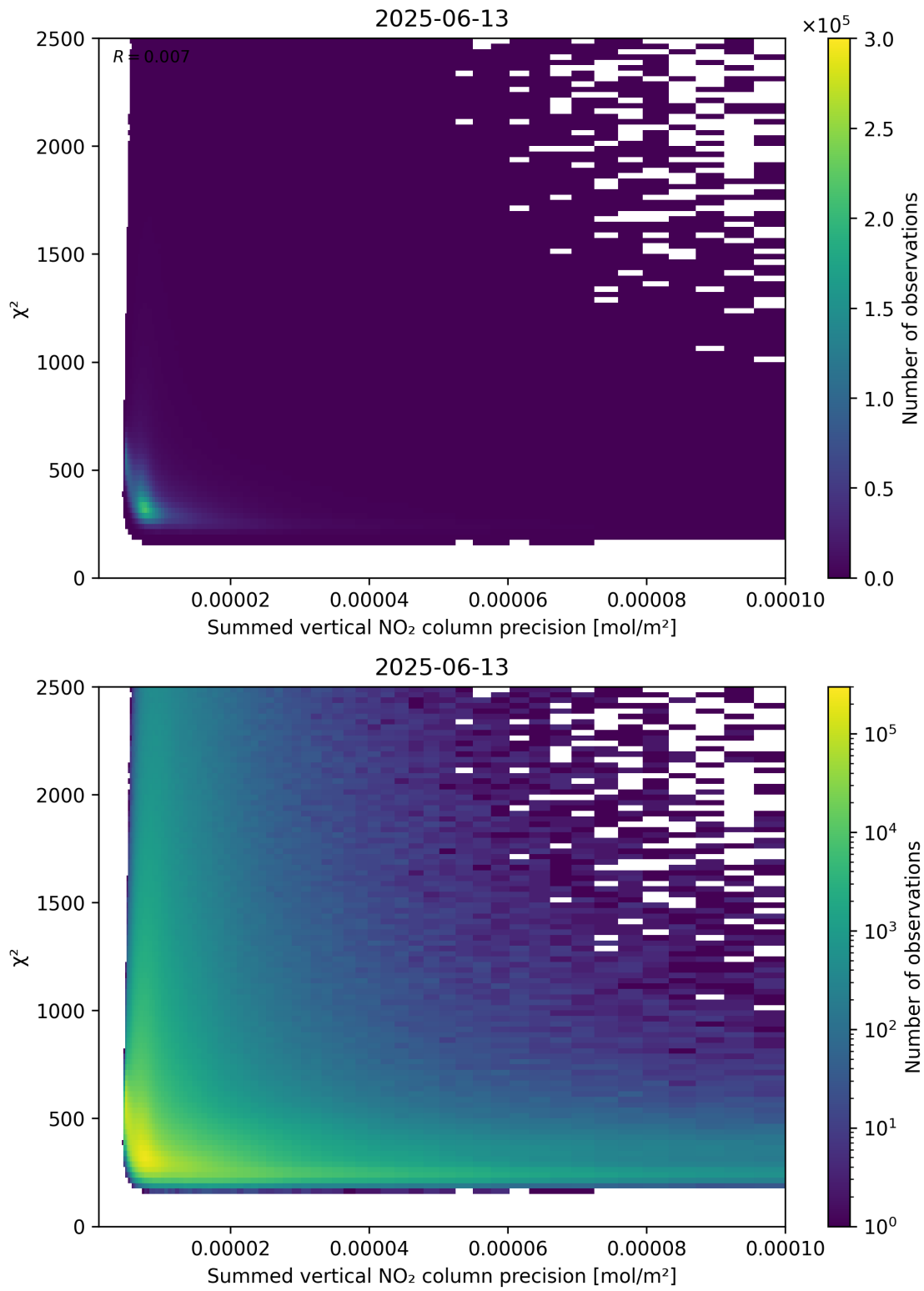
Figure 107: Scatter density plot of “Summed vertical NO 2 column precision” against “ \chi^2 ” for 2025-06-12 to 2025-06-14.
