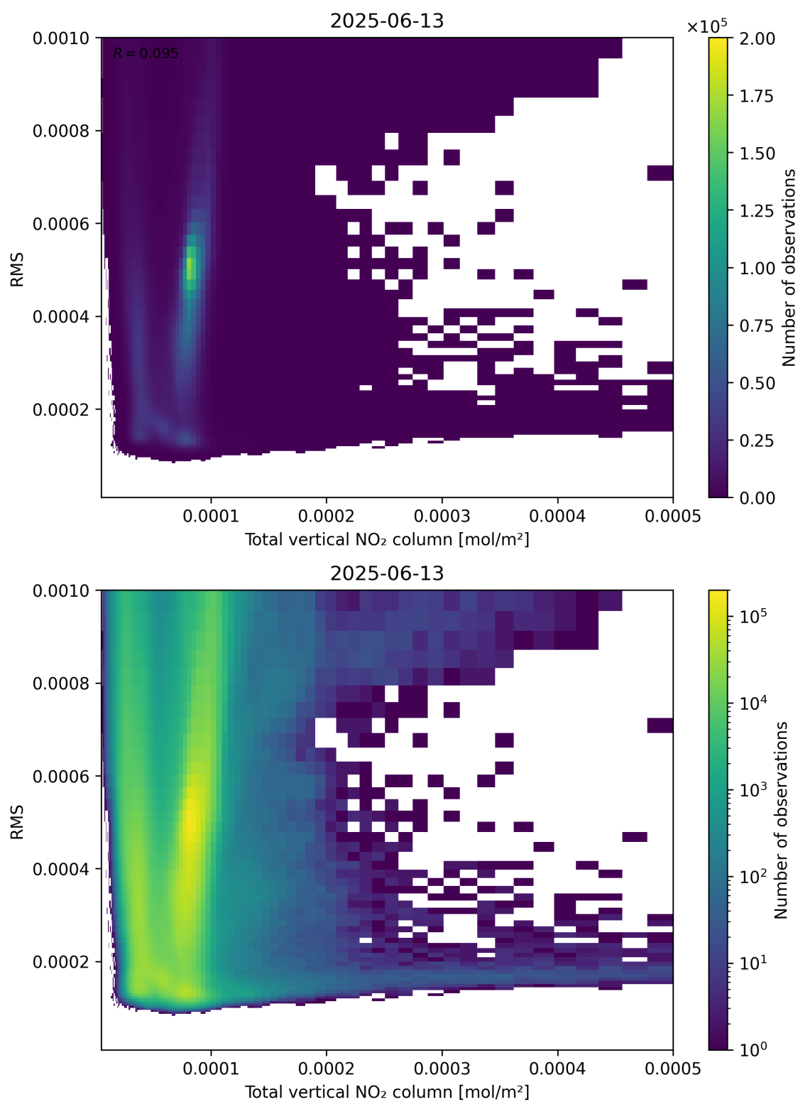
Figure 120: Scatter density plot of “Total vertical NO 2 column” against “RMS” for 2025-06-12 to 2025-06-14.
