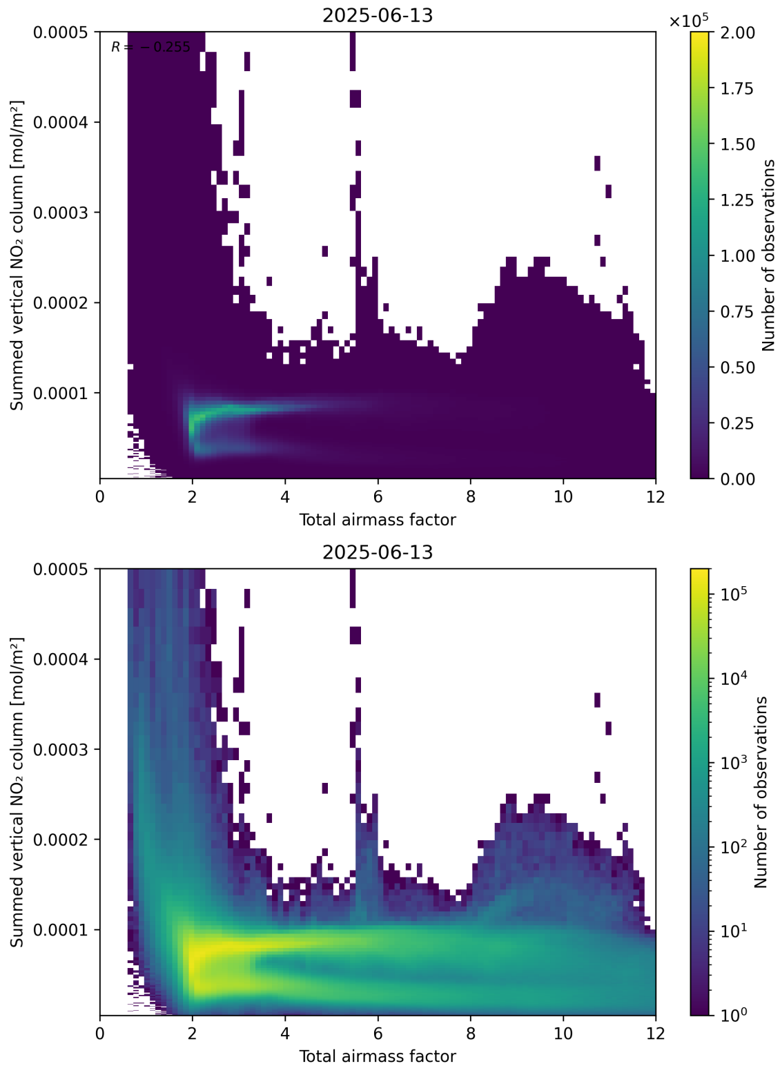
Figure 65: Scatter density plot of “Total airmass factor” against “Summed vertical NO 2 column” for 2025-06-12 to 2025-06-14.
