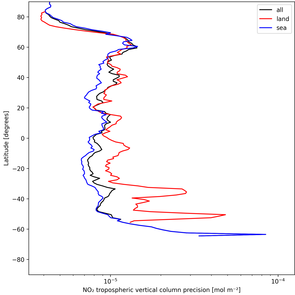
Figure 13: Zonal average of “NO 2 tropospheric vertical column precision” for 2025-06-12 to 2025-06-14.
