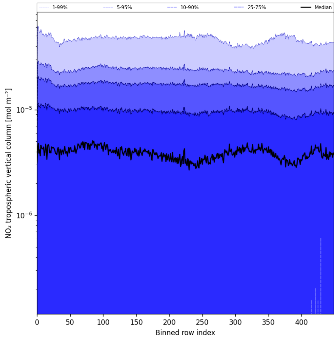
Figure 46: Along track statistics of “NO 2 tropospheric vertical column” for 2025-06-12 to 2025-06-14
