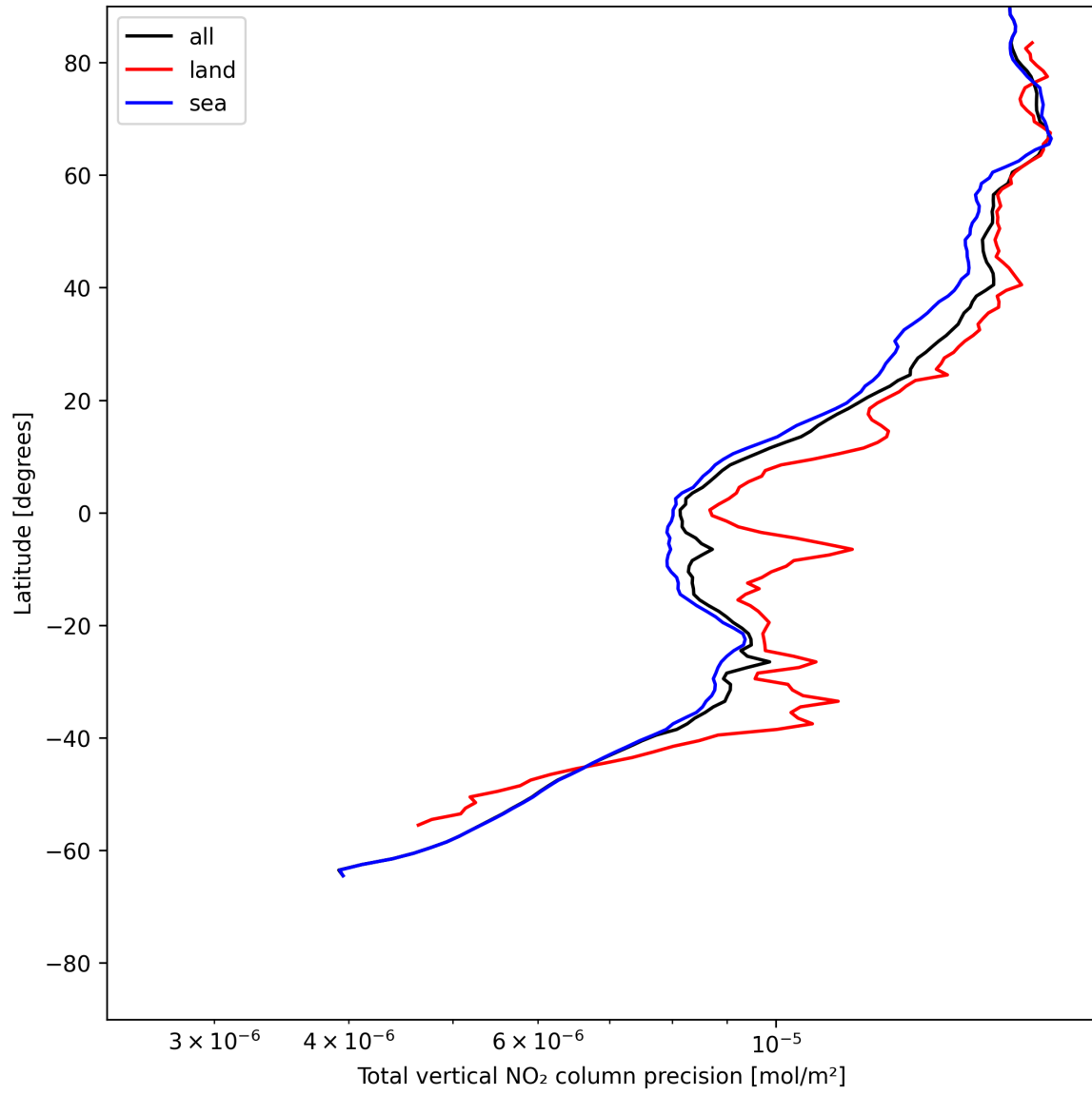
Figure 22: Zonal average of “Total vertical NO 2 column precision” for 2025-06-12 to 2025-06-14.
