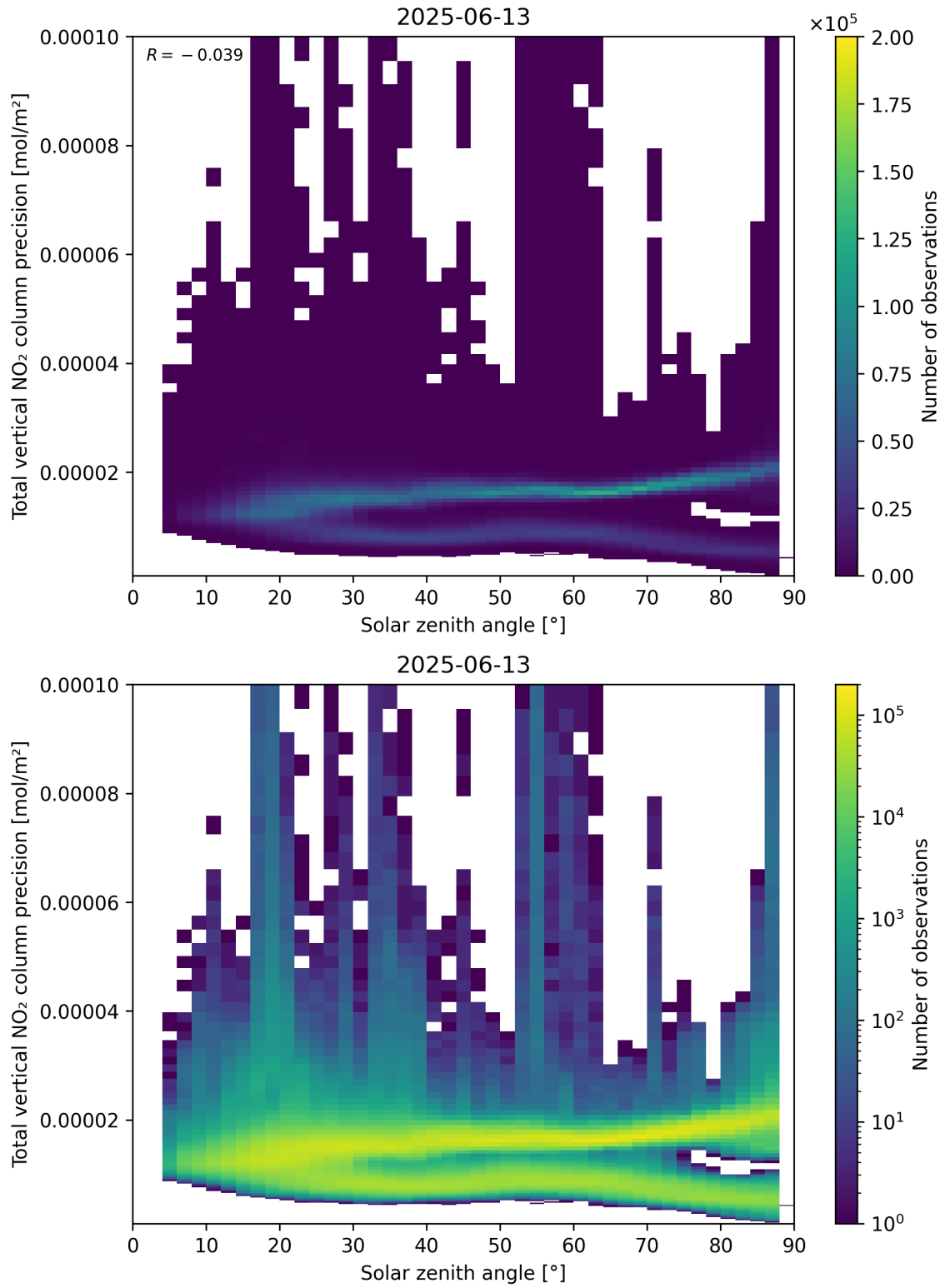
Figure 154: Scatter density plot of “Solar zenith angle” against “Total vertical NO 2 column precision” for 2025-06-12 to 2025-06-14.
