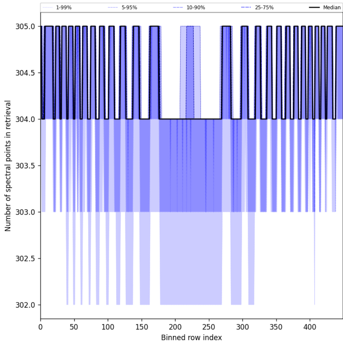
Figure 50: Along track statistics of “Number of spectral points in retrieval” for 2025-06-12 to 2025-06-14
