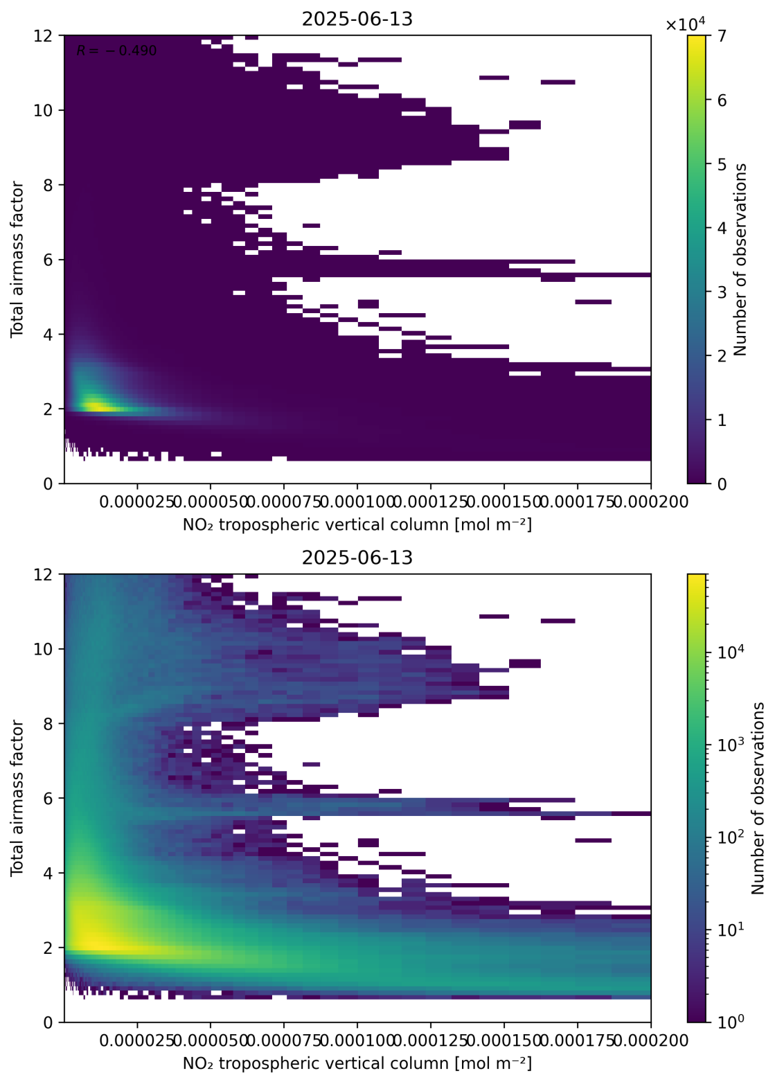
Figure 122: Scatter density plot of “NO 2 tropospheric vertical column” against “Total air mass factor” for 2025-06-12 to 2025-06-14.
