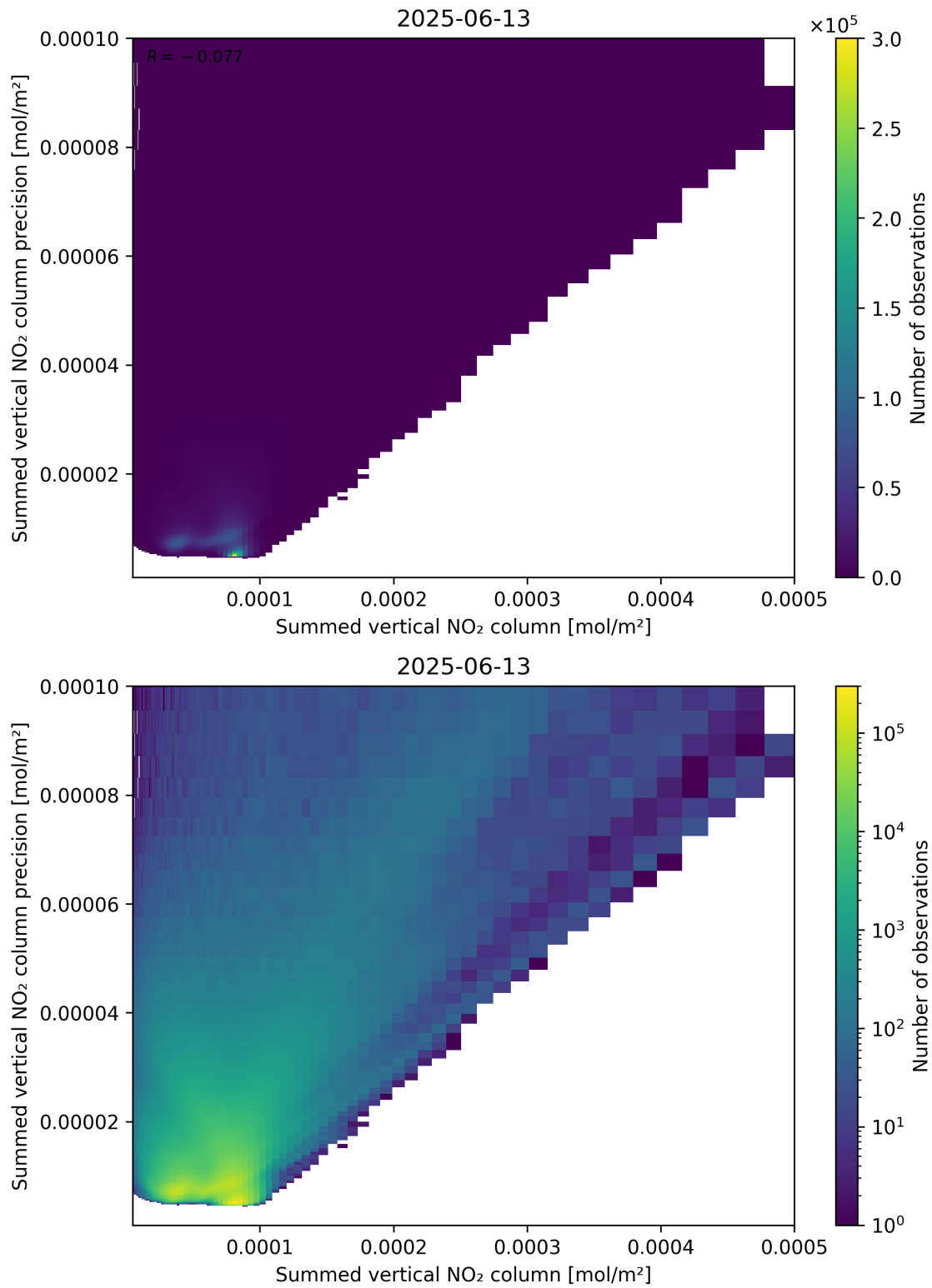
Figure 105: Scatter density plot of “Summed vertical NO 2 column” against “Summed vertical NO 2 column precision” for 2025-06-12 to 2025-06-14.
