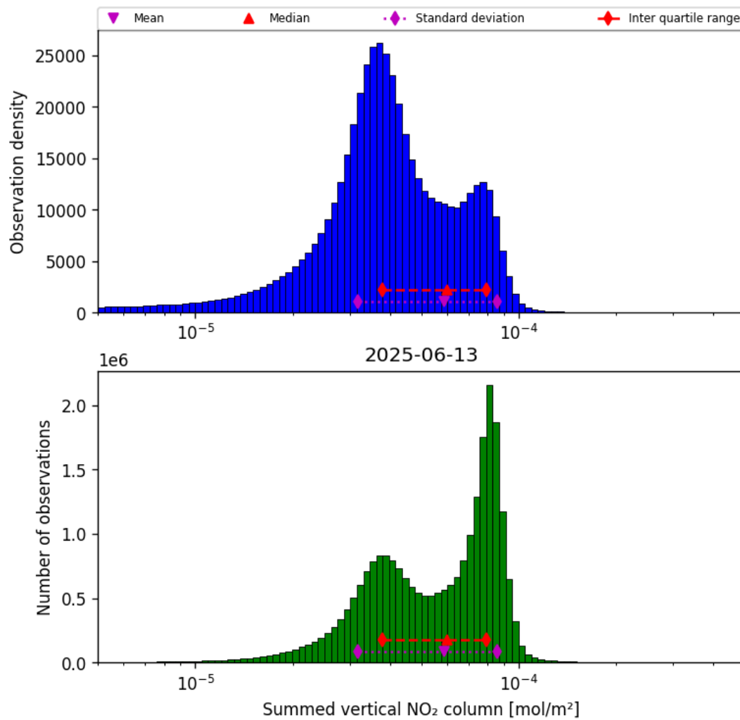
Figure 40: Histogram of “Summed vertical NO 2 column” for 2025-06-12 to 2025-06-14
