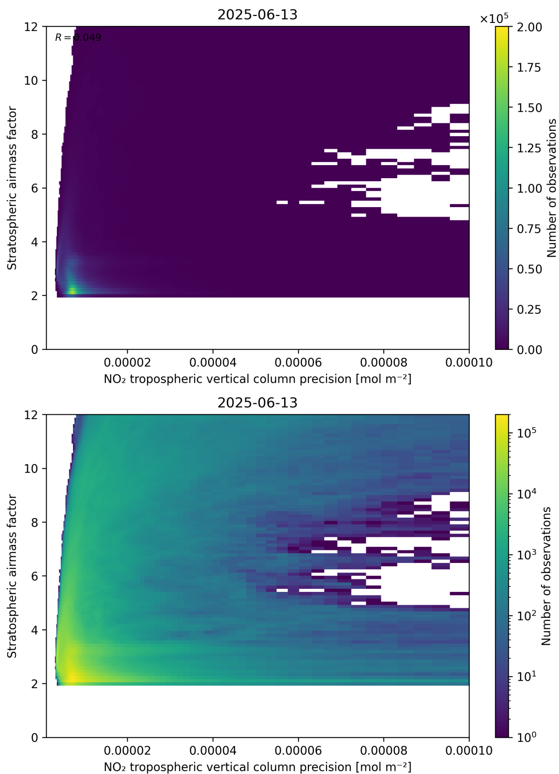
Figure 131: Scatter density plot of “NO 2 tropospheric vertical column precision” against “Stratospheric airmass factor” for 2025-06-12 to 2025-06-14.
