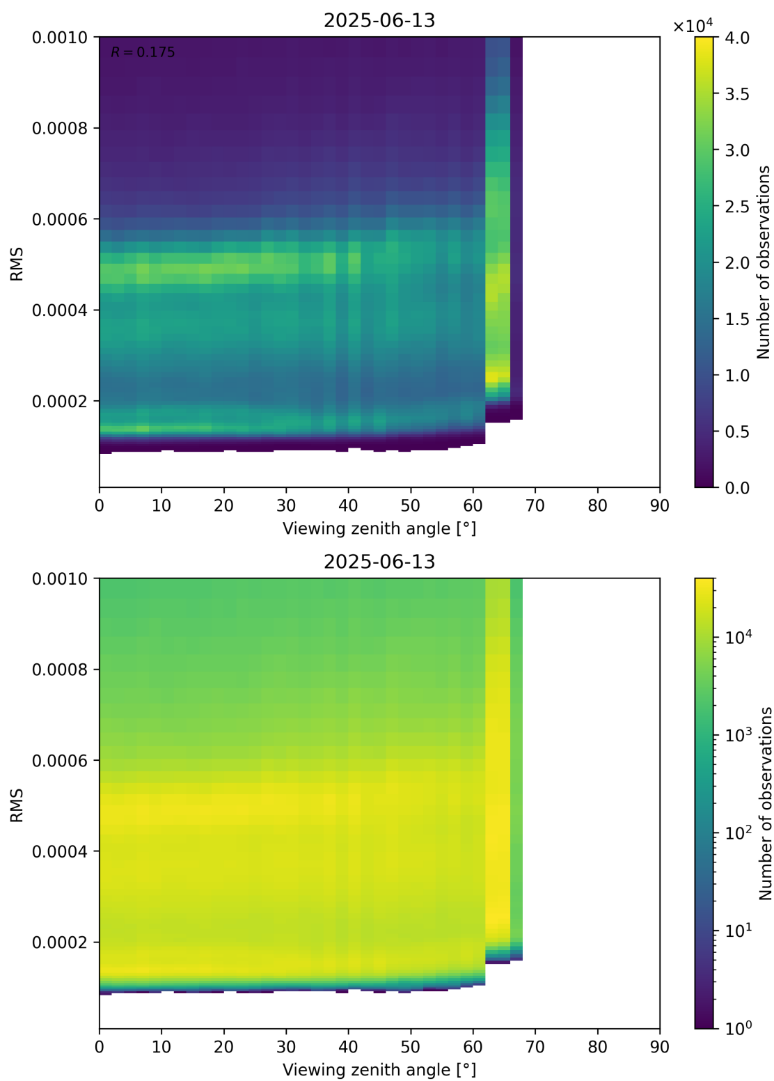
Figure 171: Scatter density plot of “Viewing zenith angle” against “RMS” for 2025-06-12 to 2025-06-14.
