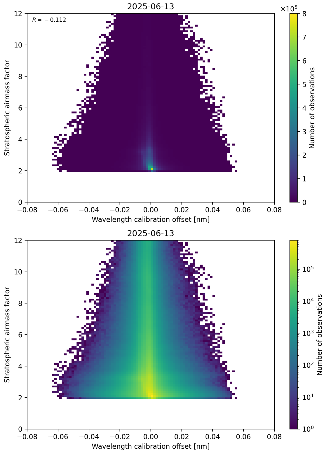
Figure 174: Scatter density plot of “Wavelength calibration offset” against “Stratospheric airmass factor” for 2025-06-12 to 2025-06-14.
