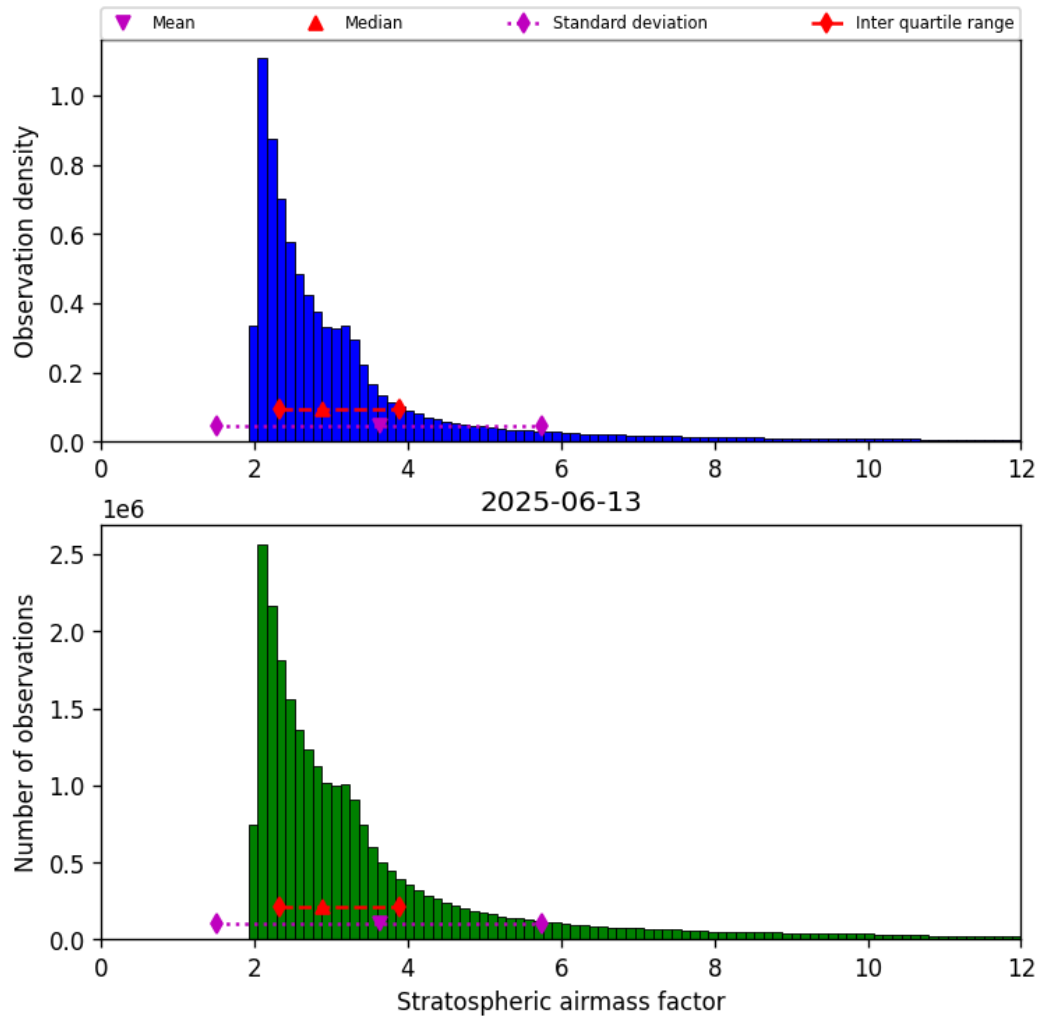
Figure 44: Histogram of “Stratospheric airmass factor” for 2025-06-12 to 2025-06-14
