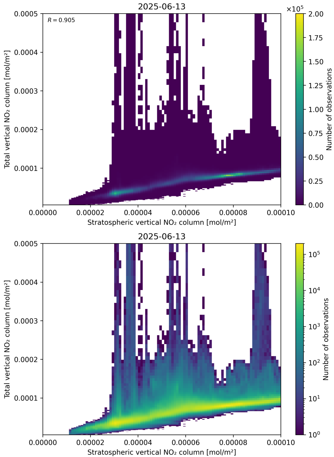
Figure 100: Scatter density plot of “Stratospheric vertical NO 2 column” against “Total vertical NO 2 column” for 2025-06-12 to 2025-06-14.
