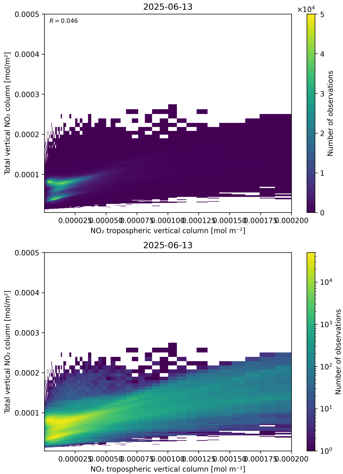
Figure 128: Scatter density plot of “NO 2 tropospheric vertical column” against “Total vertical NO 2 column” for 2025-06-12 to 2025-06-14.
