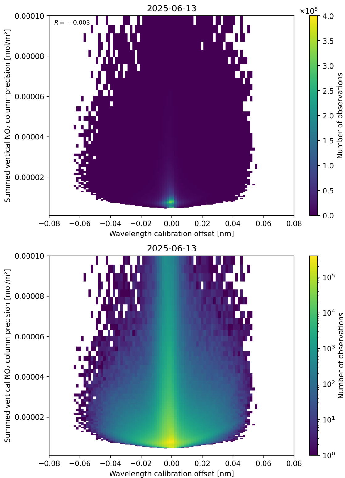
Figure 178: Scatter density plot of “Wavelength calibration offset” against “Summed vertical NO 2 column precision” for 2025-06-12 to 2025-06-14.
