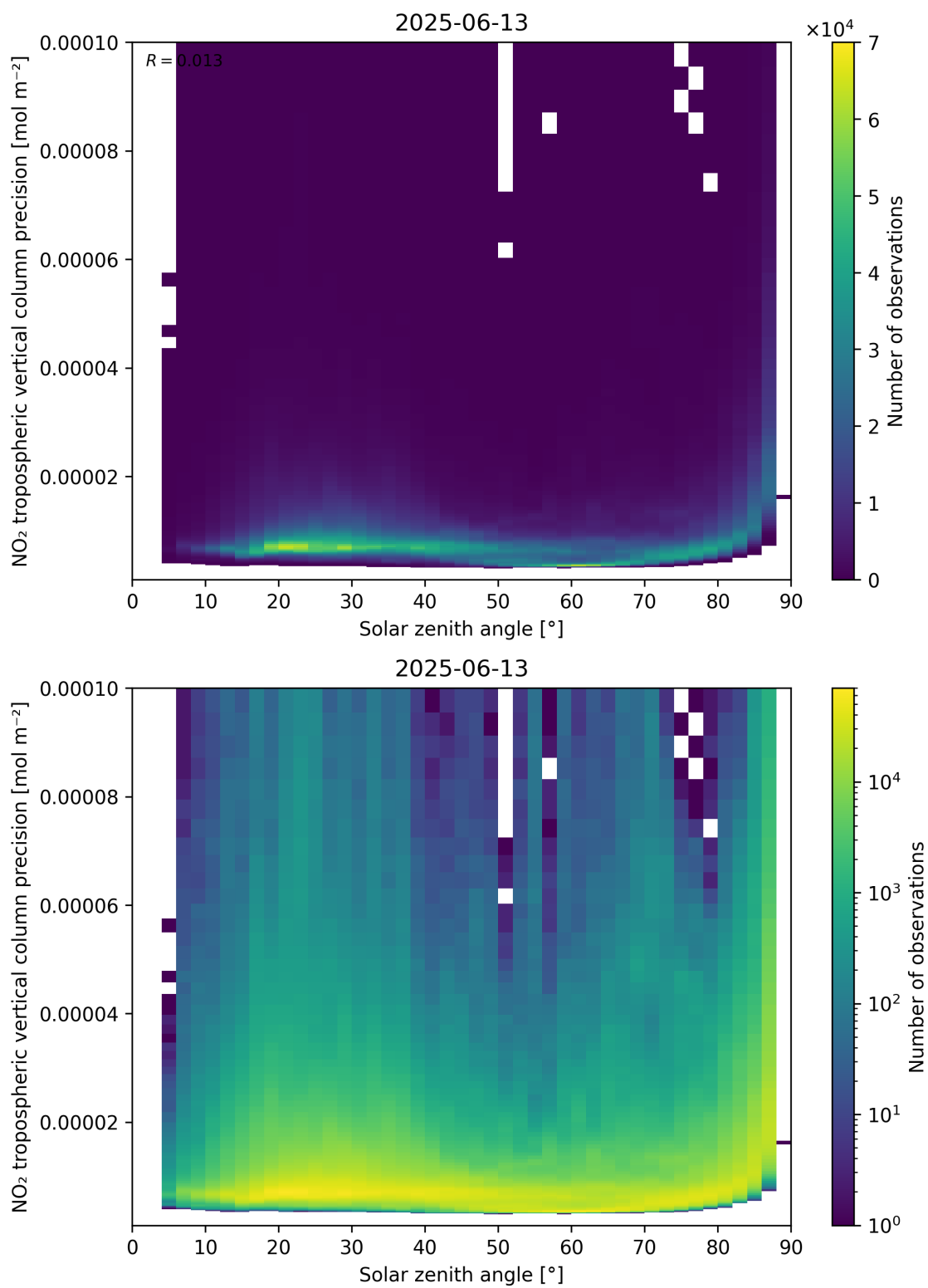
Figure 156: Scatter density plot of “Solar zenith angle” against “NO 2 tropospheric vertical column precision” for 2025-06-12 to 2025-06-14.
