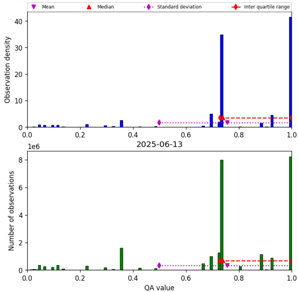
Figure 28: Histogram of “QA value” for 2025-06-12 to 2025-06-14
