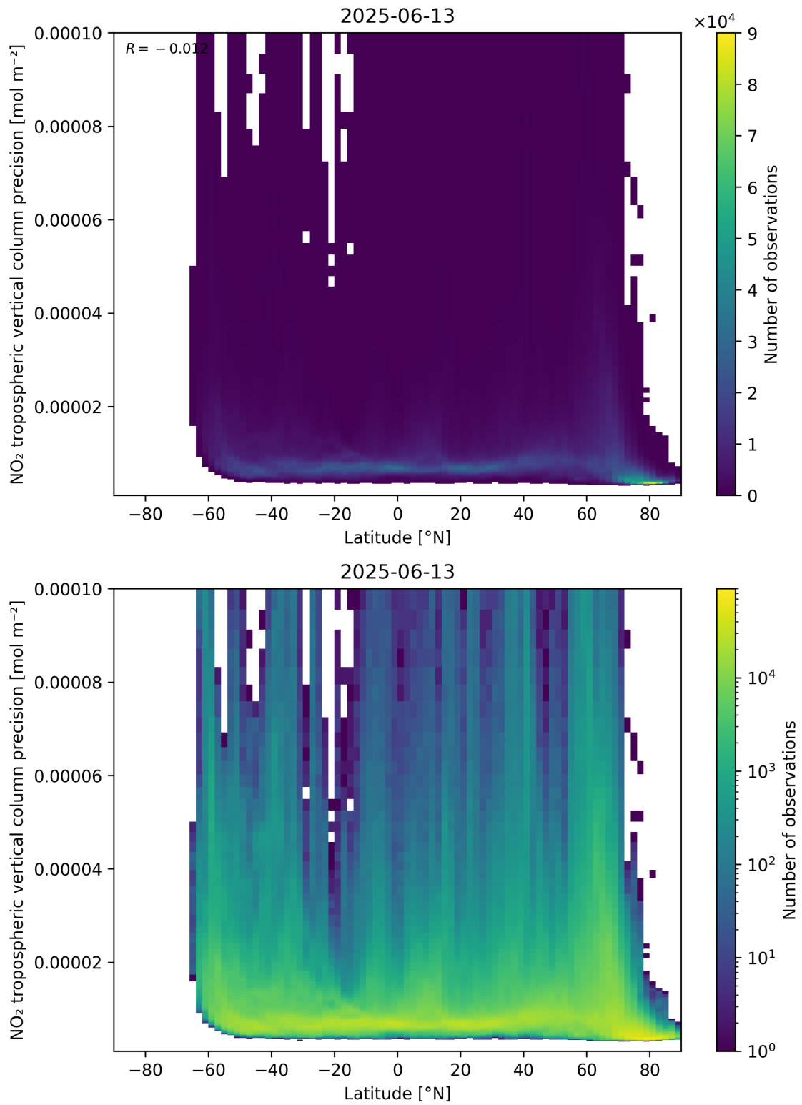
Figure 93: Scatter density plot of “Latitude” against “NO 2 tropospheric vertical column precision” for 2025-06-12 to 2025-06-14.
