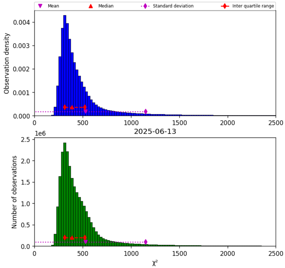
Figure 42: Histogram of “ \chi^2 ” for 2025-06-12 to 2025-06-14
