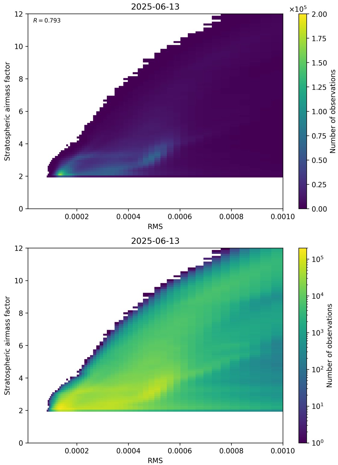
Figure 144: Scatter density plot of “RMS” against “Stratospheric airmass factor” for 2025-06-12 to 2025-06-14.
