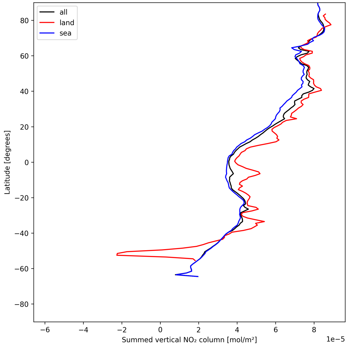
Figure 23: Zonal average of “Summed vertical NO 2 column” for 2025-06-12 to 2025-06-14.
