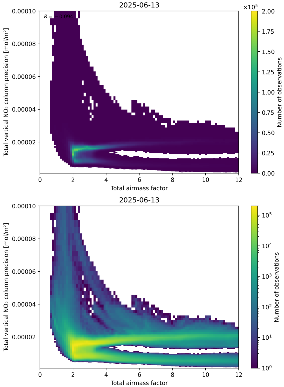
Figure 68: Scatter density plot of “Total airmass factor” against “Total vertical NO 2 column precision” for 2025-06-12 to 2025-06-14.
