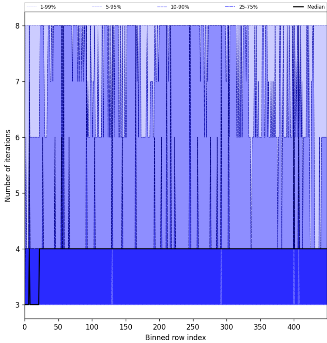
Figure 51: Along track statistics of “Number of iterations” for 2025-06-12 to 2025-06-14
