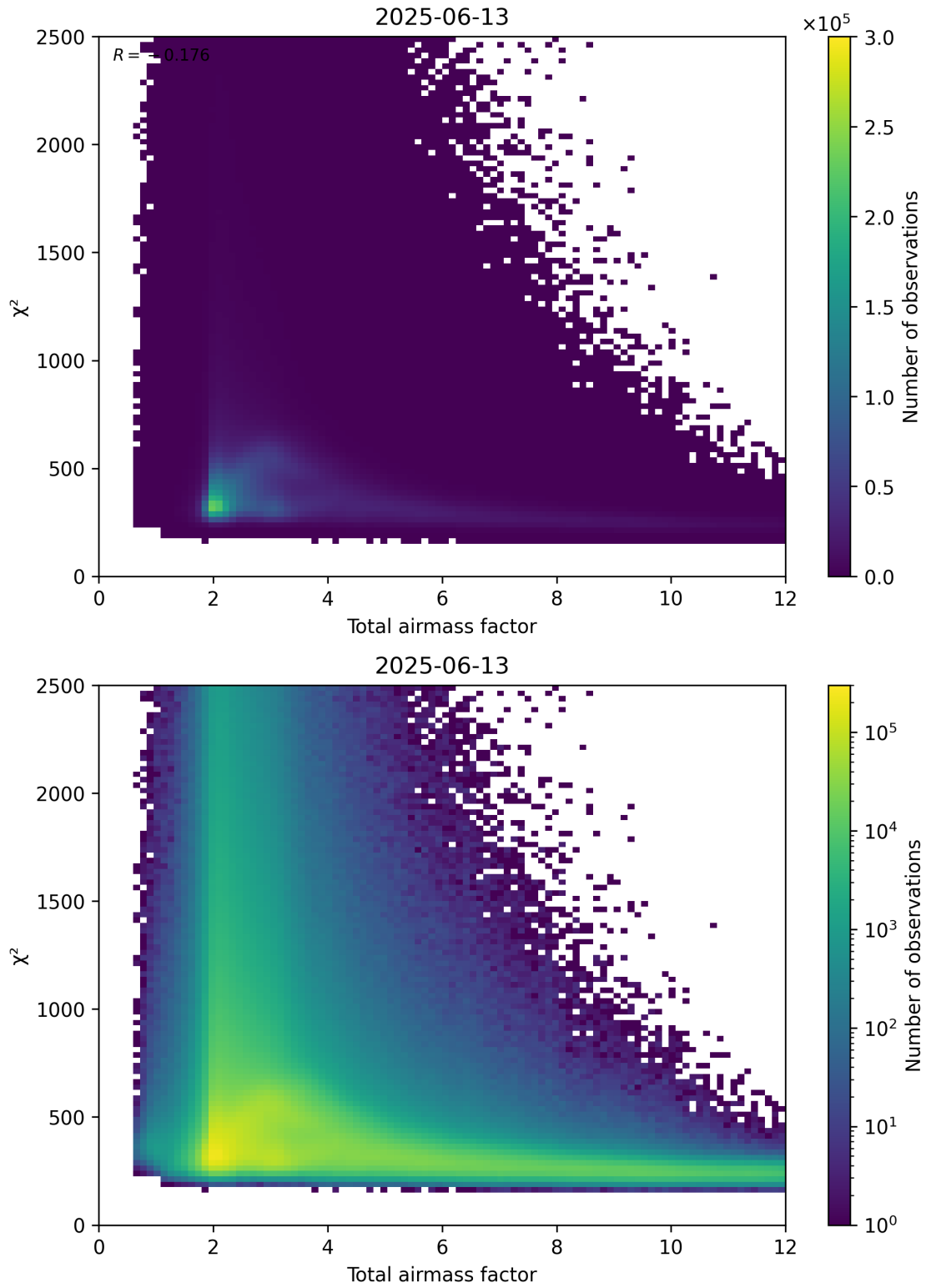
Figure 63: Scatter density plot of “Total airmass factor” against “ \chi^2 ” for 2025-06-12 to 2025-06-14.
