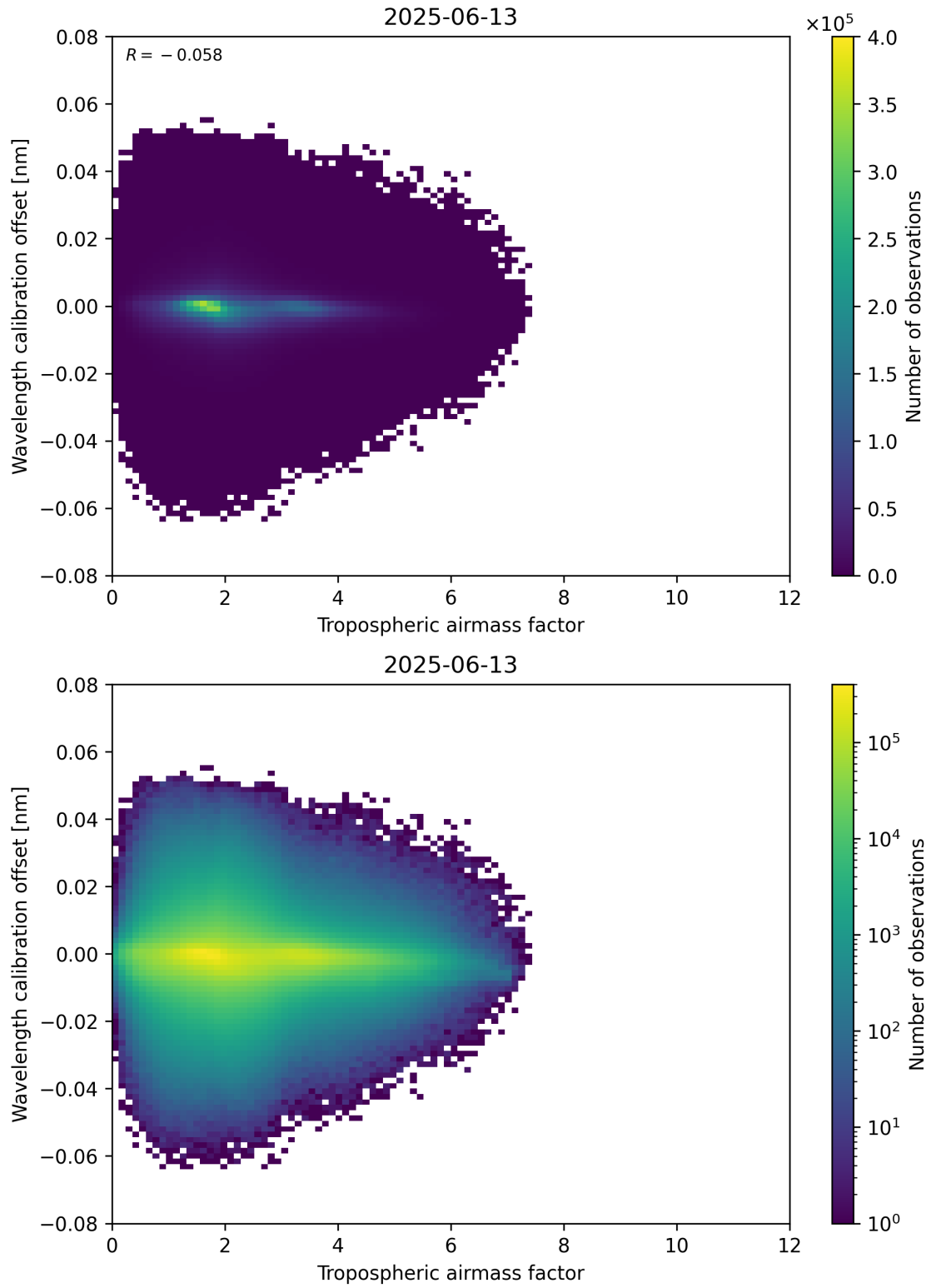
Figure 80: Scatter density plot of “Tropospheric airmass factor” against “Wavelength calibration offset” for 2025-06-12 to 2025-06-14.
