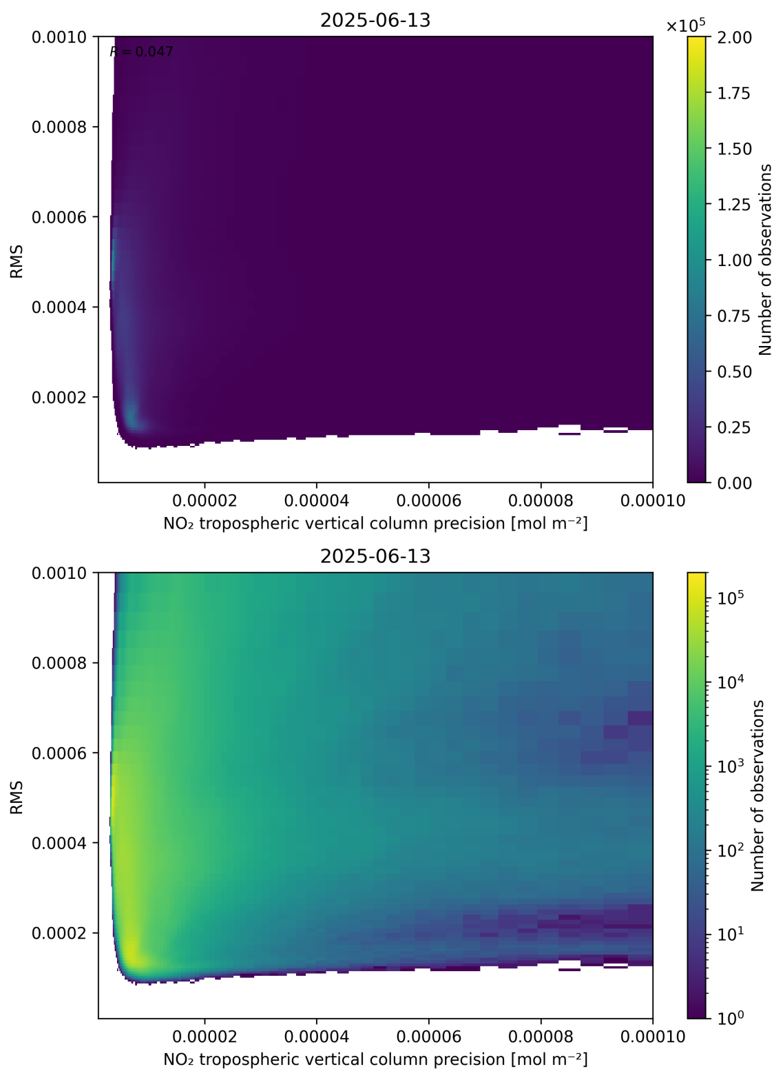
Figure 140: Scatter density plot of “NO 2 tropospheric vertical column precision” against “RMS” for 2025-06-12 to 2025-06-14.
