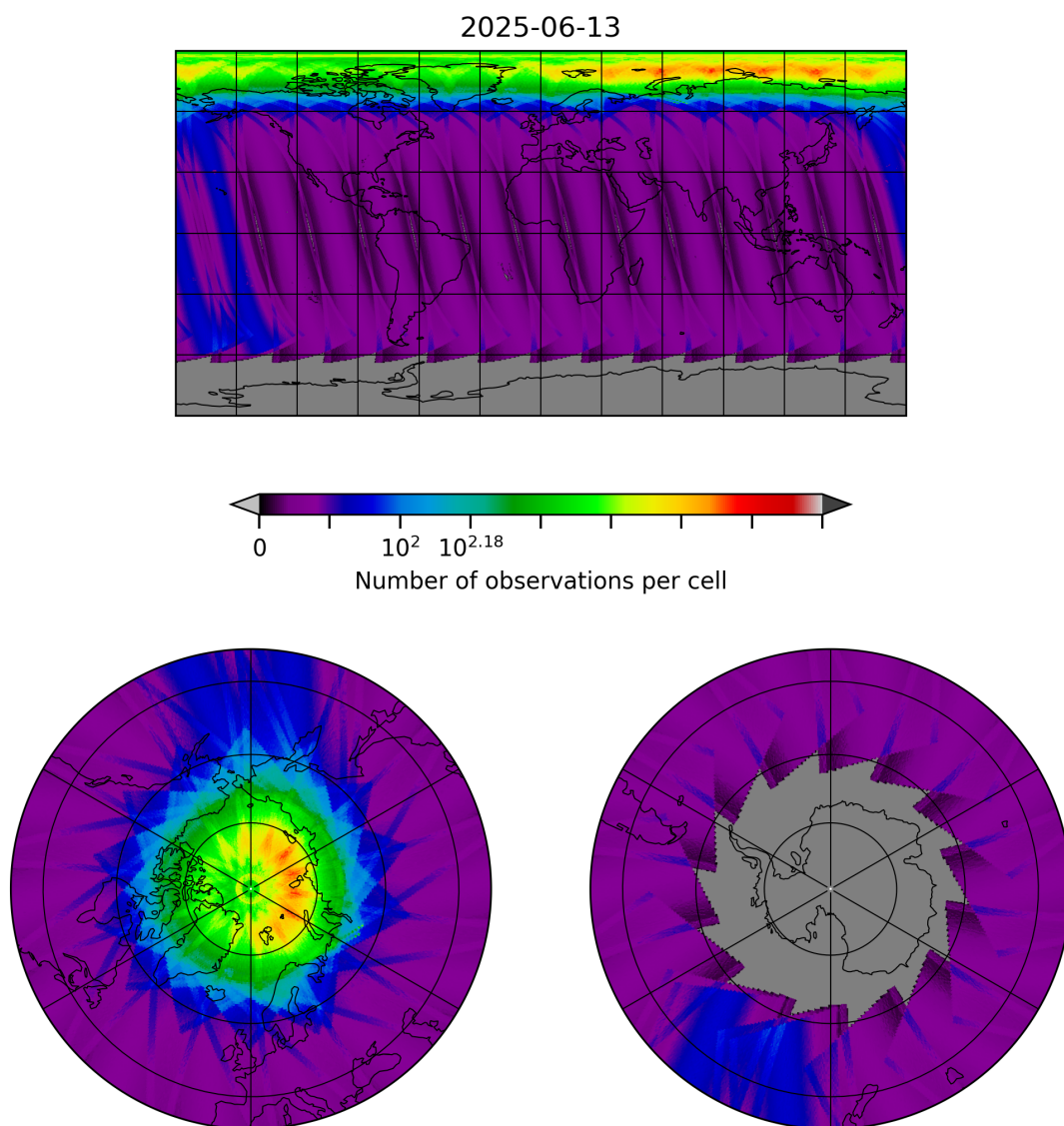
Figure 10: Map of the number of observations for 2025-06-12 to 2025-06-14
