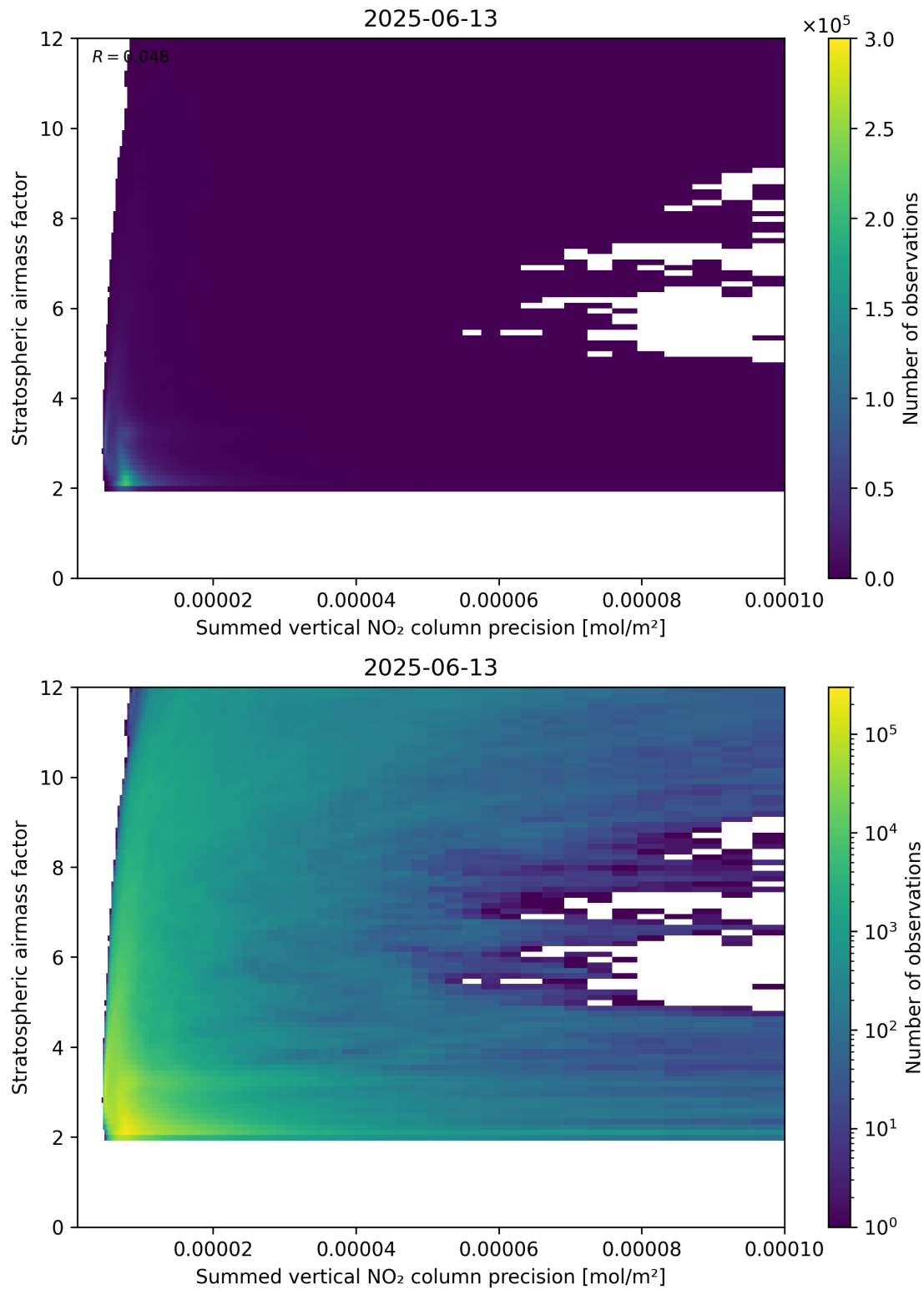
Figure 106: Scatter density plot of “Summed vertical NO 2 column precision” against “Stratospheric airmass factor” for 2025-06-12 to 2025-06-14.
