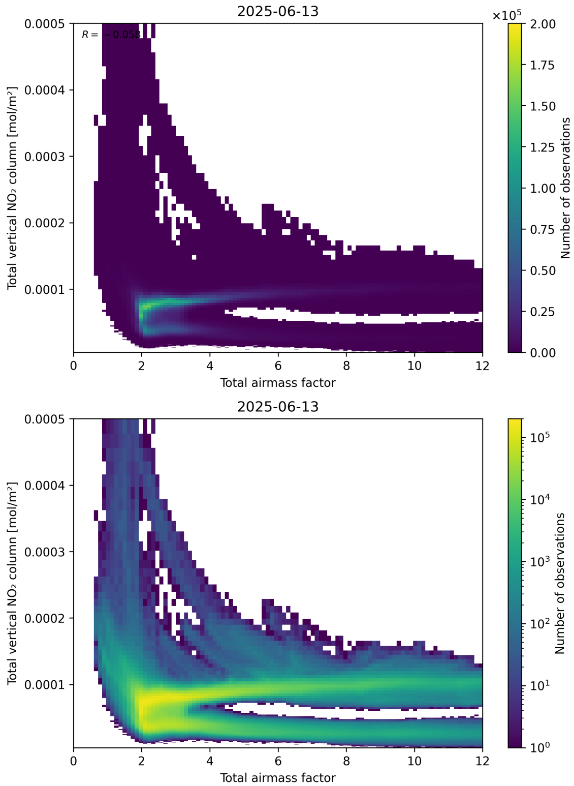
Figure 67: Scatter density plot of “Total airmass factor” against “Total vertical NO 2 column” for 2025-06-12 to 2025-06-14.
