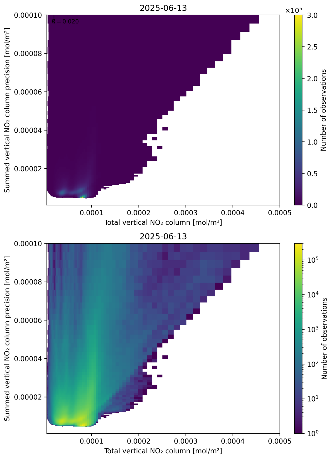
Figure 113: Scatter density plot of “Total vertical NO 2 column” against “Summed vertical NO 2 column precision” for 2025-06-12 to 2025-06-14.
