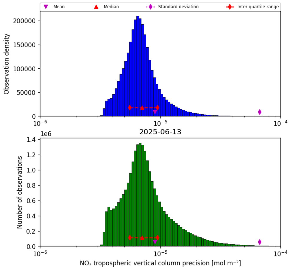
Figure 30: Histogram of “NO 2 tropospheric vertical column precision” for 2025-06-12 to 2025-06-14
