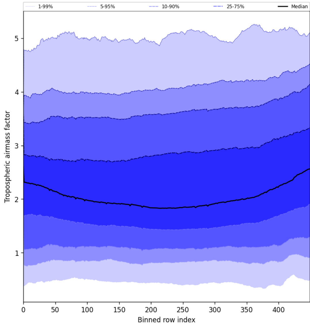
Figure 48: Along track statistics of “Tropospheric airmass factor” for 2025-06-12 to 2025-06-14
