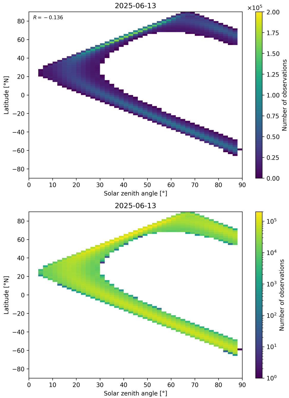
Figure 149: Scatter density plot of “Solar zenith angle” against “Latitude” for 2025-06-12 to 2025-06-14.
