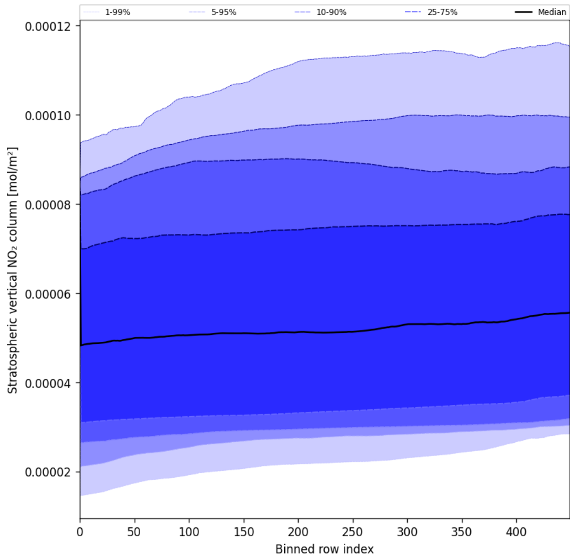
Figure 53: Along track statistics of “Stratospheric vertical NO 2 column” for 2025-06-12 to 2025-06-14
