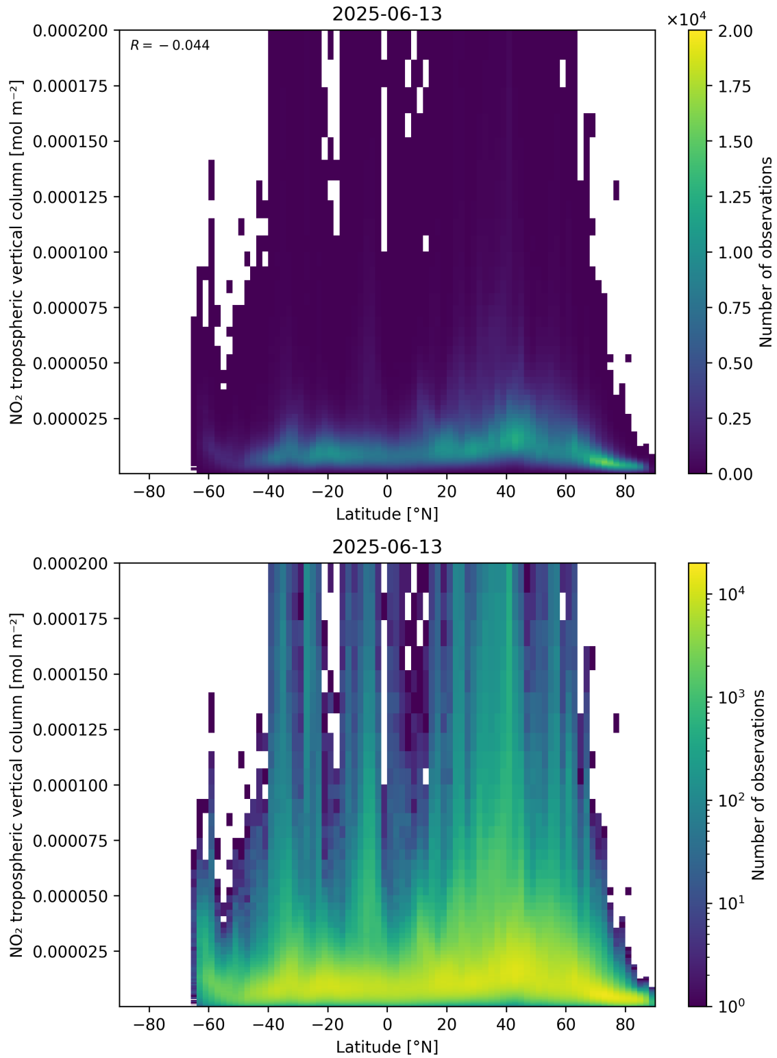
Figure 92: Scatter density plot of “Latitude” against “NO 2 tropospheric vertical column” for 2025-06-12 to 2025-06-14.
