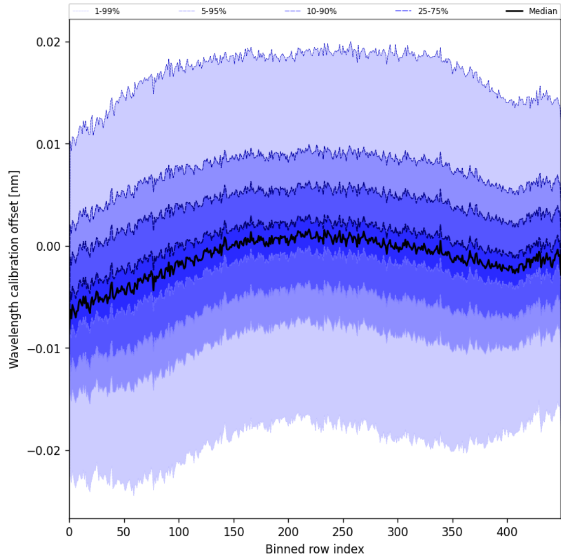
Figure 52: Along track statistics of “Wavelength calibration offset” for 2025-06-12 to 2025-06-14
