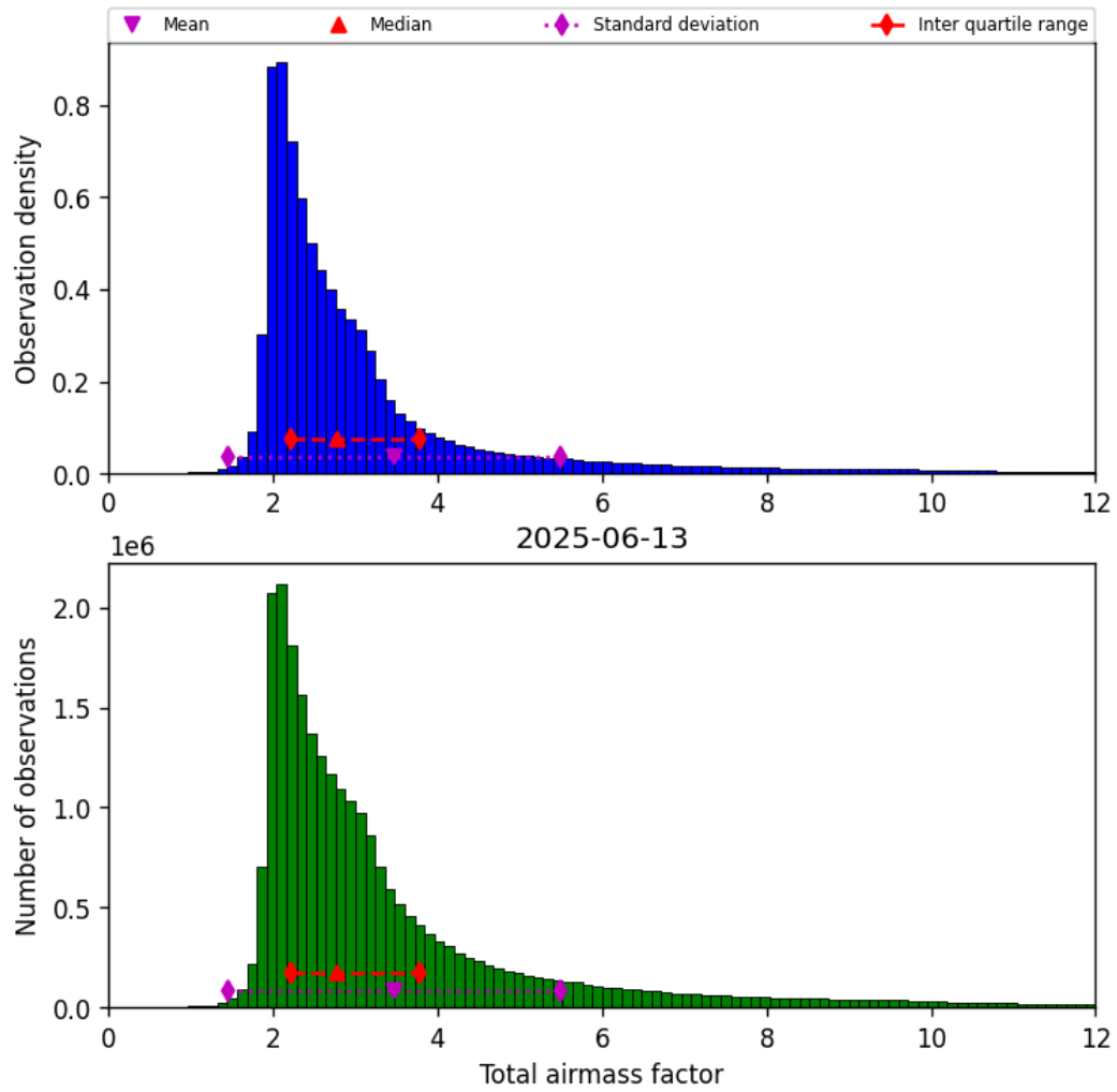
Figure 32: Histogram of “Total airmass factor” for 2025-06-12 to 2025-06-14
