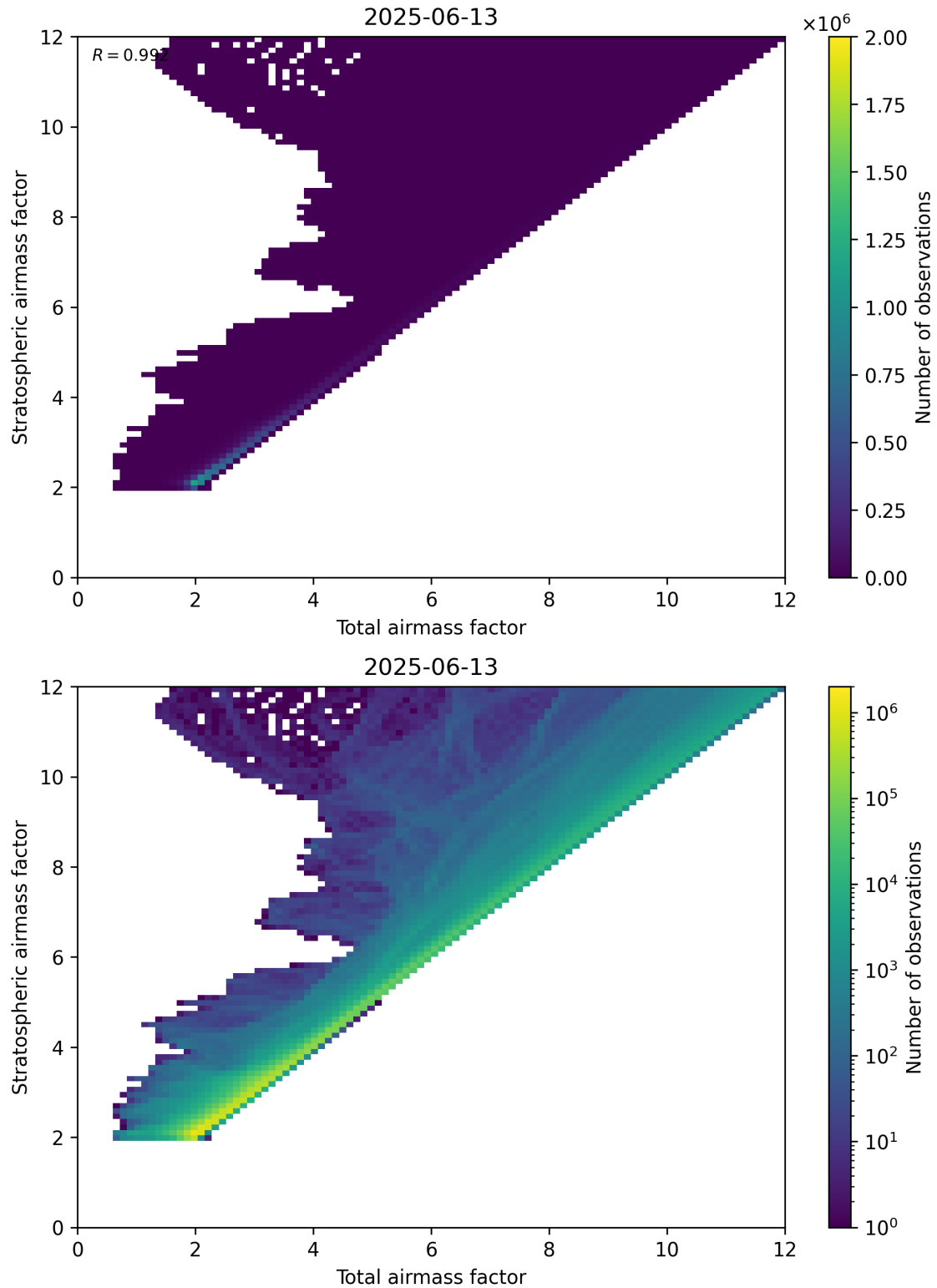
Figure 62: Scatter density plot of “Total airmass factor” against “Stratospheric airmass factor” for 2025-06-12 to 2025-06-14.
