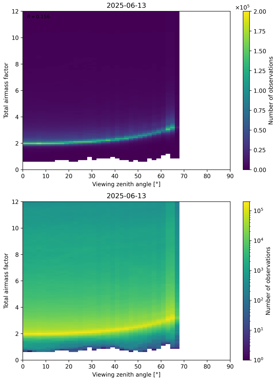
Figure 160: Scatter density plot of “Viewing zenith angle” against “Total airmass factor” for 2025-06-12 to 2025-06-14.
