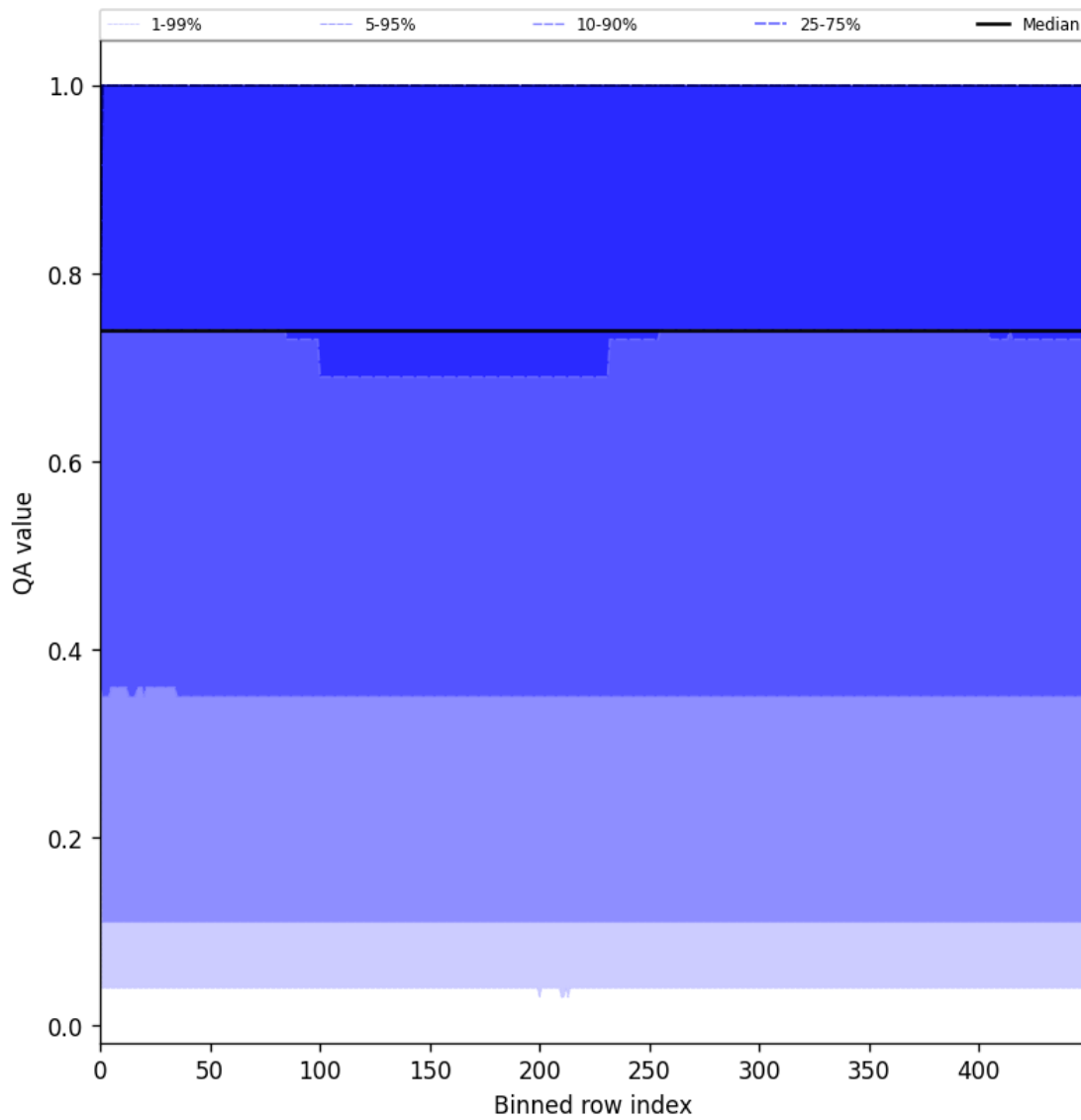
Figure 45: Along track statistics of “QA value” for 2025-06-12 to 2025-06-14
