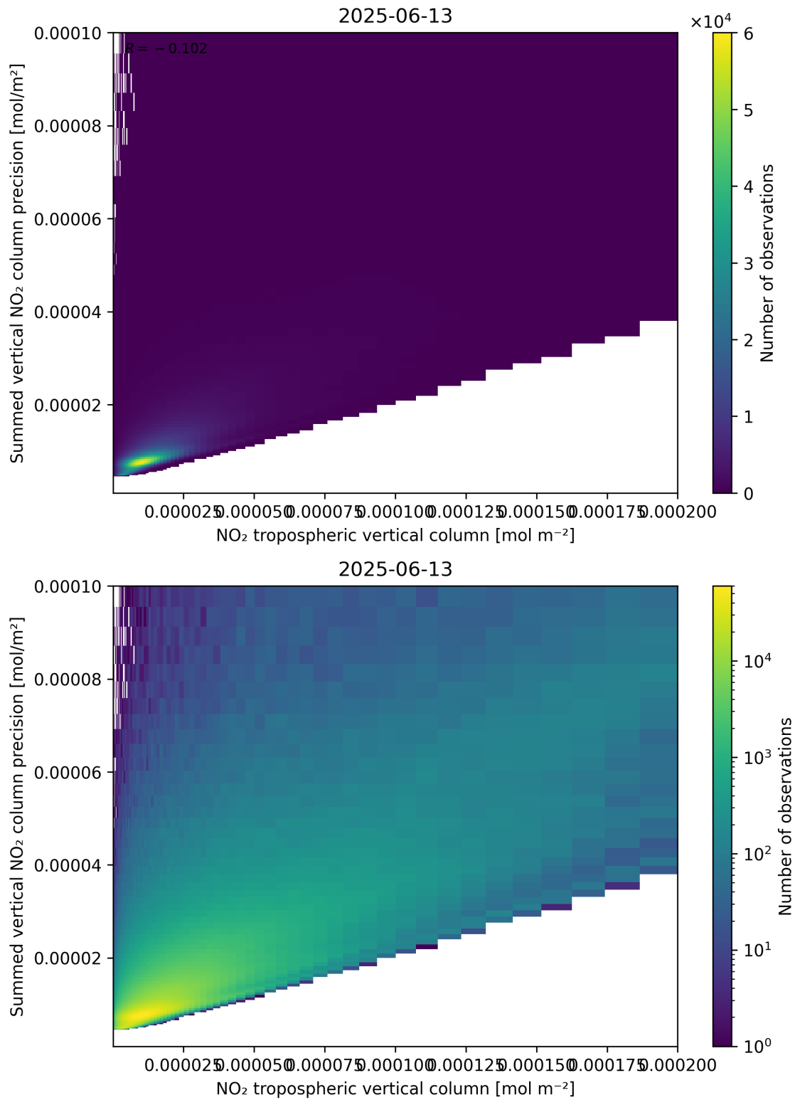
Figure 127: Scatter density plot of “NO 2 tropospheric vertical column” against “Summed vertical NO 2 column precision” for 2025-06-12 to 2025-06-14.
