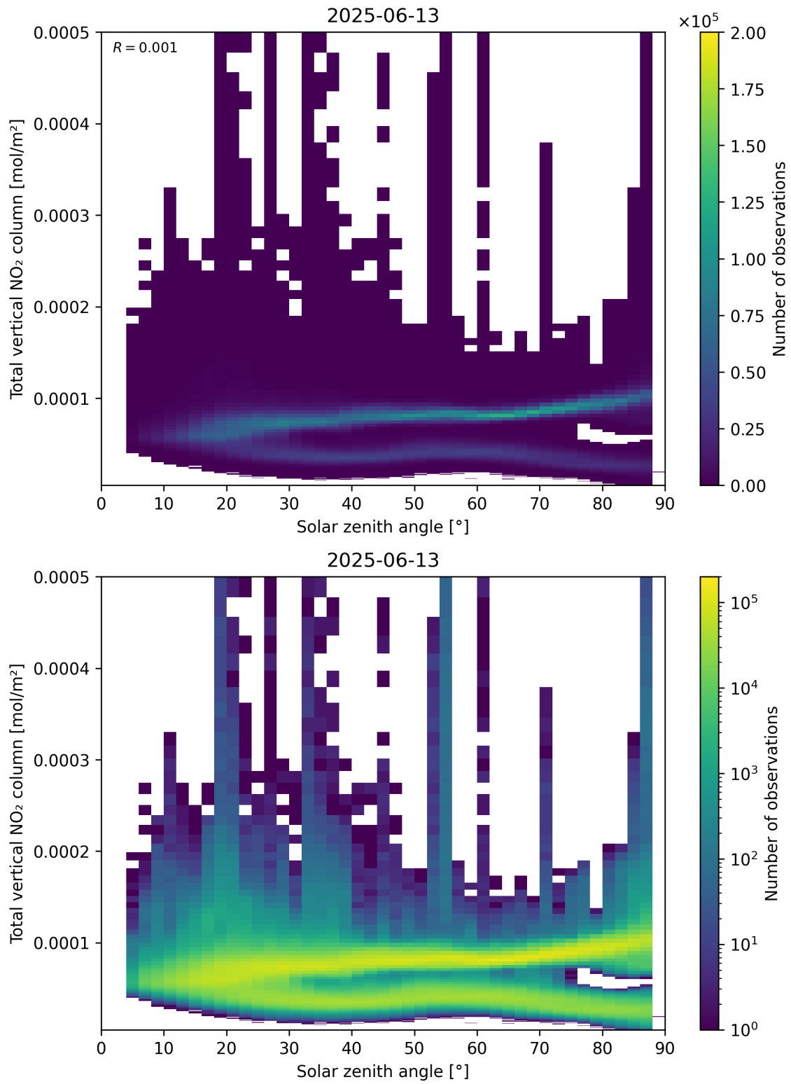
Figure 153: Scatter density plot of “Solar zenith angle” against “Total vertical NO 2 column” for 2025-06-12 to 2025-06-14.
