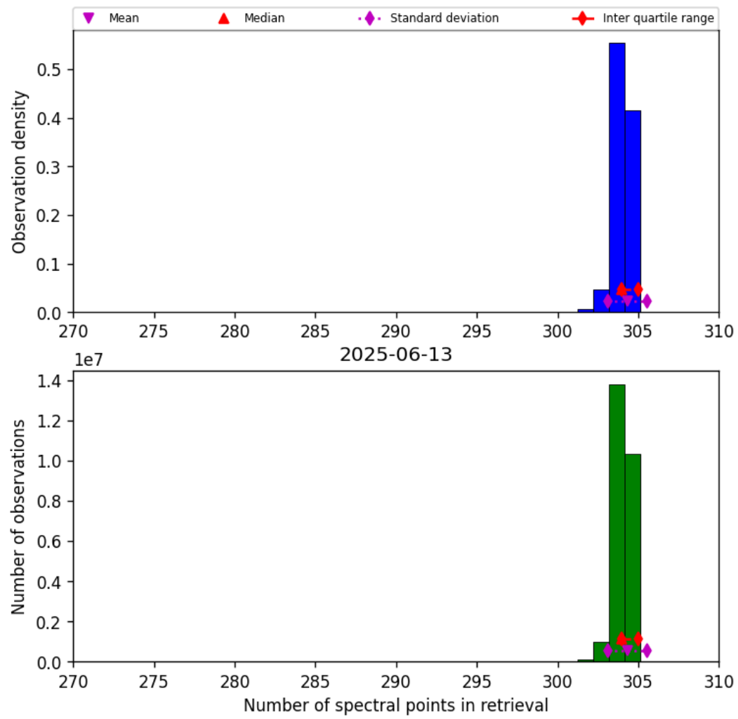
Figure 33: Histogram of “Number of spectral points in retrieval” for 2025-06-12 to 2025-06-14
