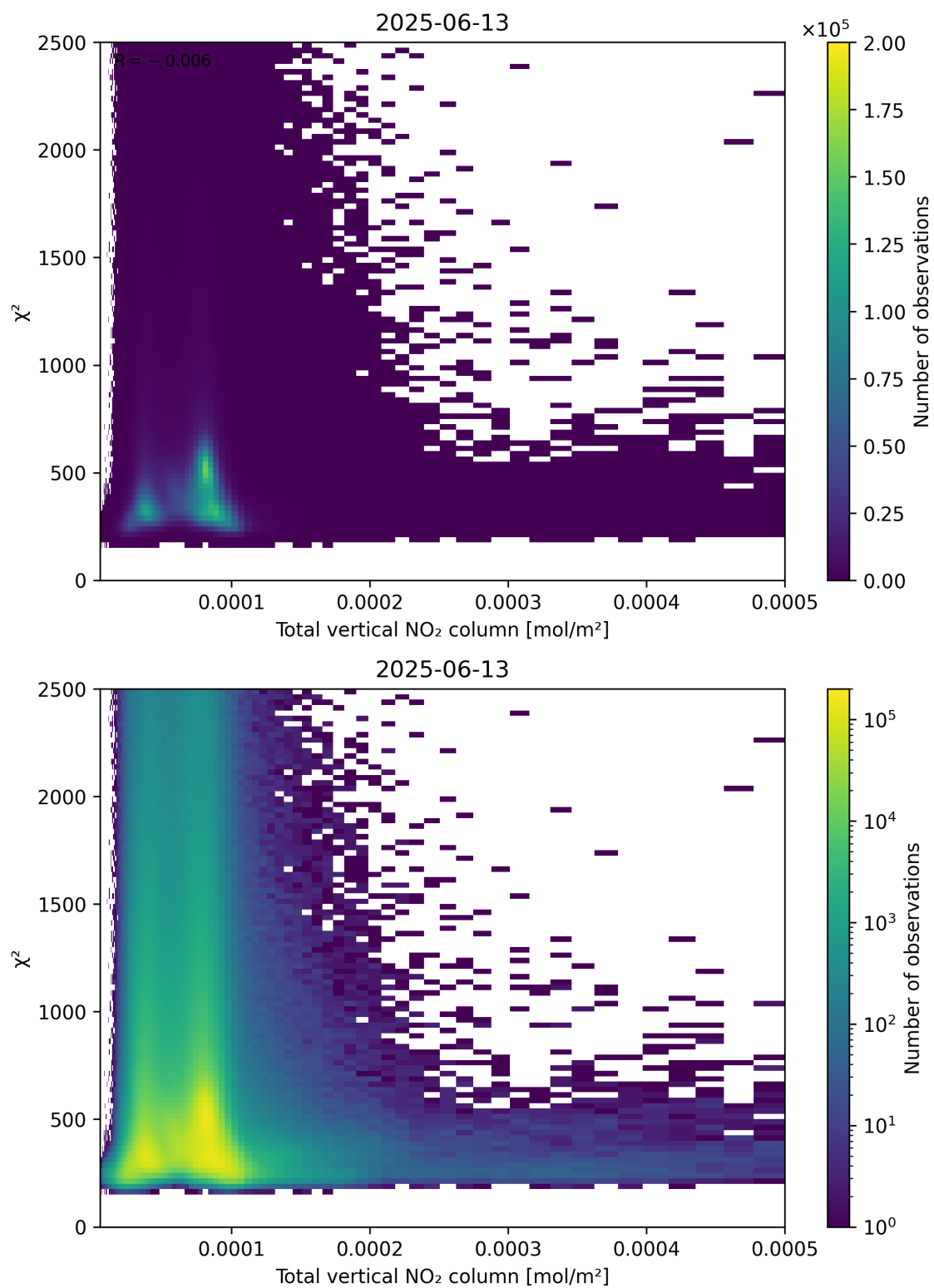
Figure 111: Scatter density plot of “Total vertical NO 2 column” against “ \chi^2 ” for 2025-06-12 to 2025-06-14.
