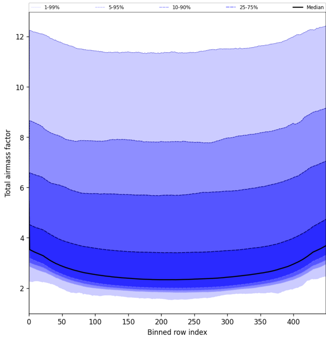
Figure 49: Along track statistics of “Total airmass factor” for 2025-06-12 to 2025-06-14
