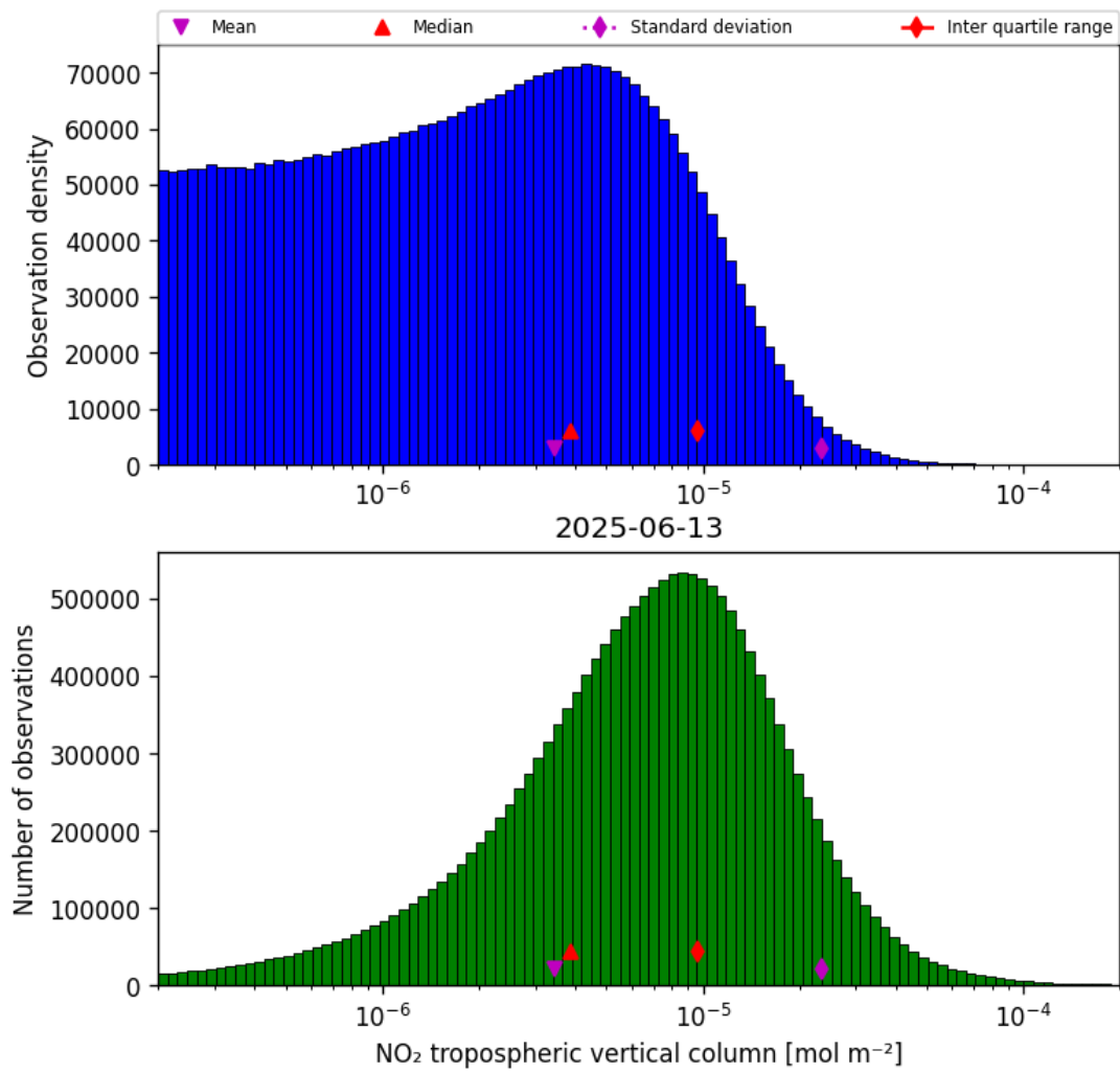
Figure 29: Histogram of “NO 2 tropospheric vertical column” for 2025-06-12 to 2025-06-14
