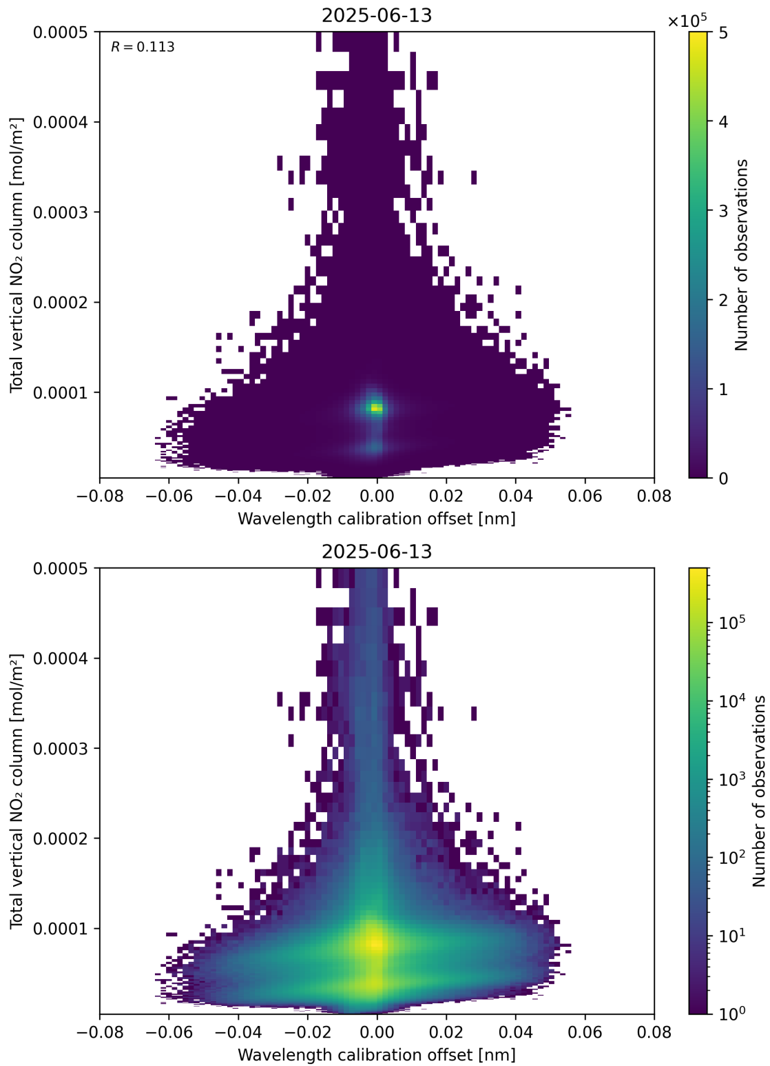
Figure 179: Scatter density plot of “Wavelength calibration offset” against “Total vertical NO 2 column” for 2025-06-12 to 2025-06-14.
