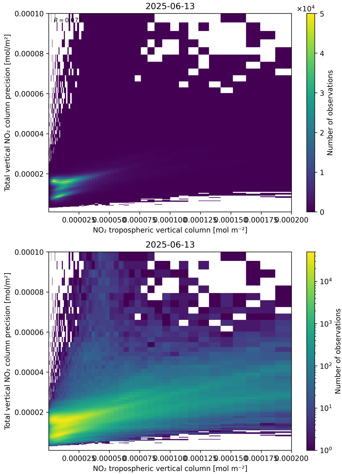
Figure 129: Scatter density plot of “NO 2 tropospheric vertical column” against “Total vertical NO 2 column precision” for 2025-06-12 to 2025-06-14.
