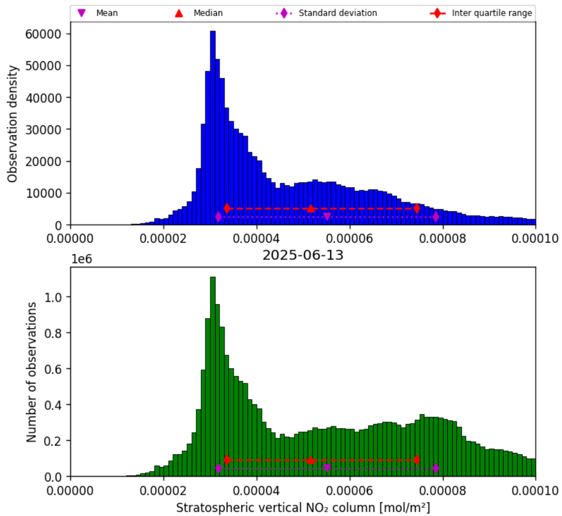
Figure 36: Histogram of “Stratospheric vertical NO 2 column” for 2025-06-12 to 2025-06-14
