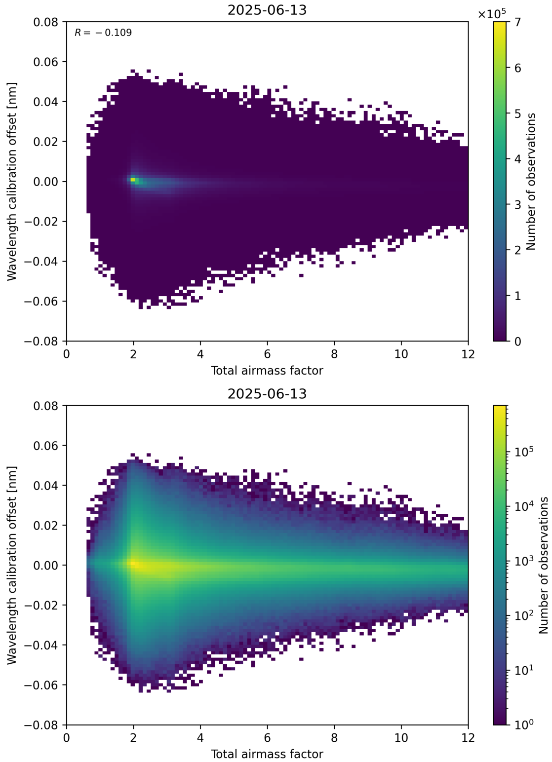
Figure 70: Scatter density plot of “Total airmass factor” against “Wavelength calibration offset” for 2025-06-12 to 2025-06-14.
