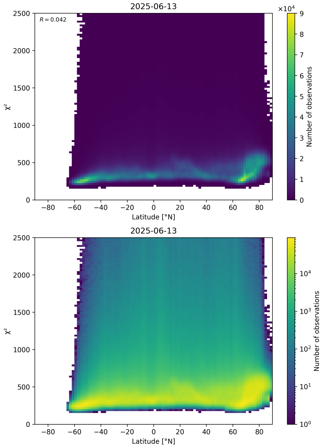
Figure 86: Scatter density plot of “Latitude” against “ \chi^2 ” for 2025-06-12 to 2025-06-14.
