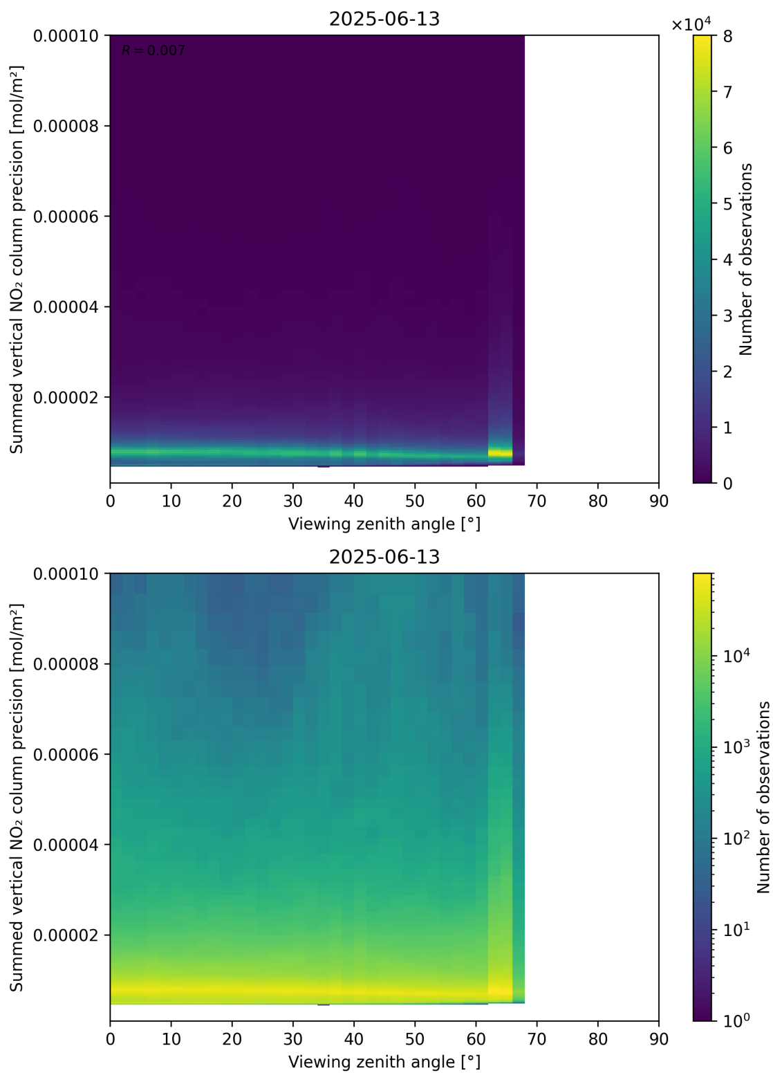
Figure 166: Scatter density plot of “Viewing zenith angle” against “Summed vertical NO 2 column precision” for 2025-06-12 to 2025-06-14.
