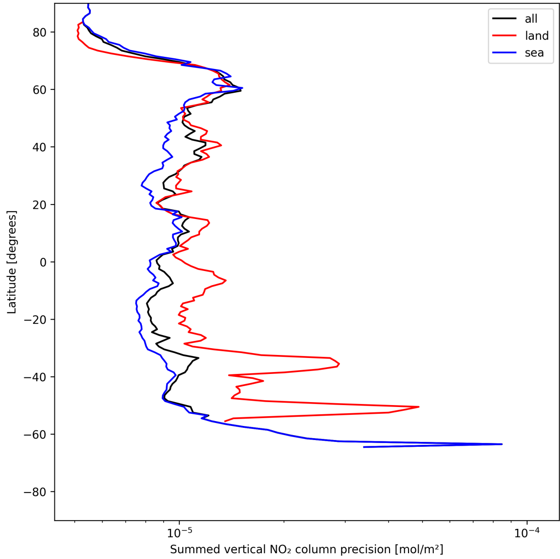
Figure 24: Zonal average of “Summed vertical NO 2 column precision” for 2025-06-12 to 2025-06-14.
