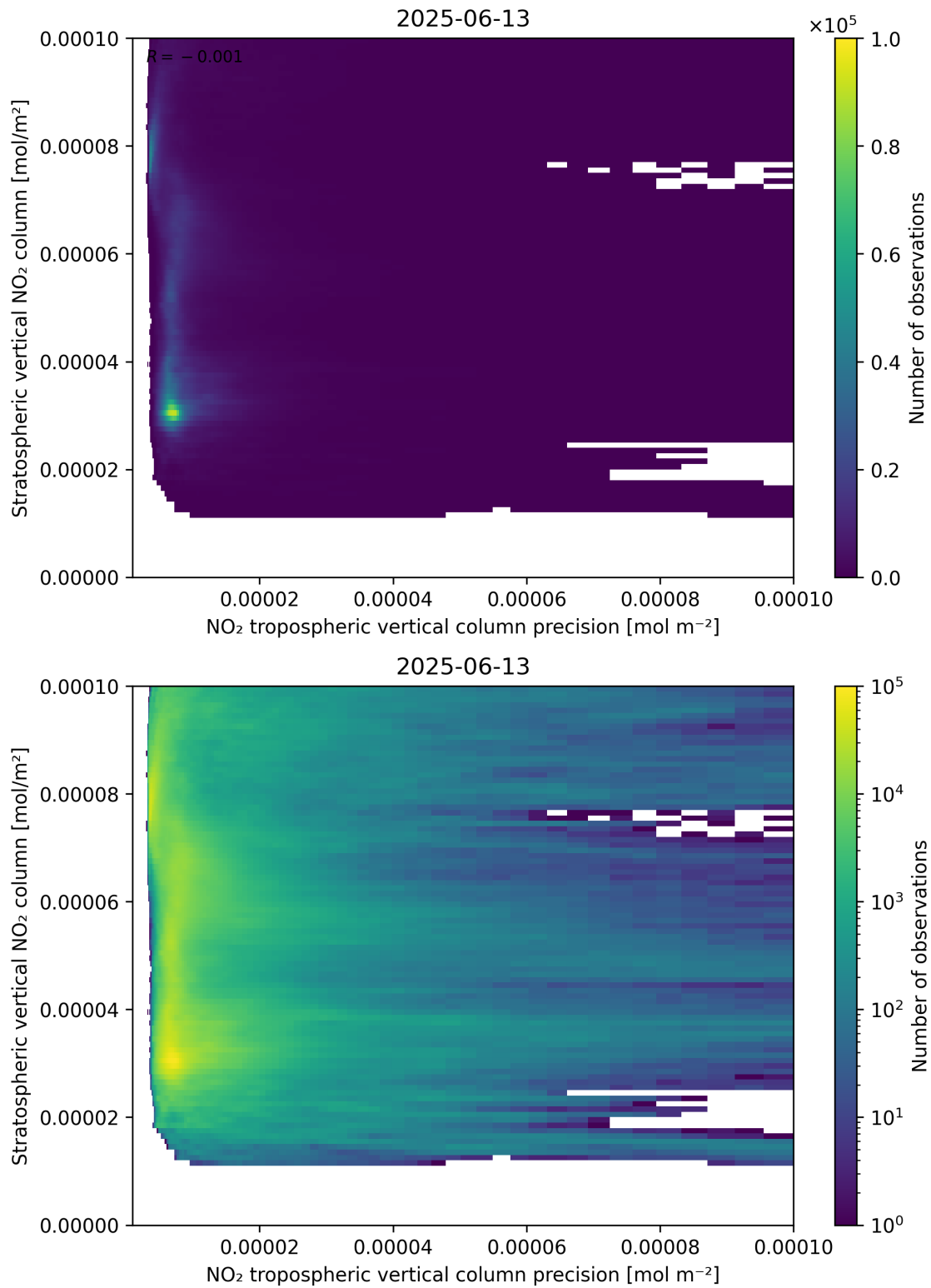
Figure 135: Scatter density plot of “NO 2 tropospheric vertical column precision” against “Stratospheric vertical NO 2 column” for 2025-06-12 to 2025-06-14.
