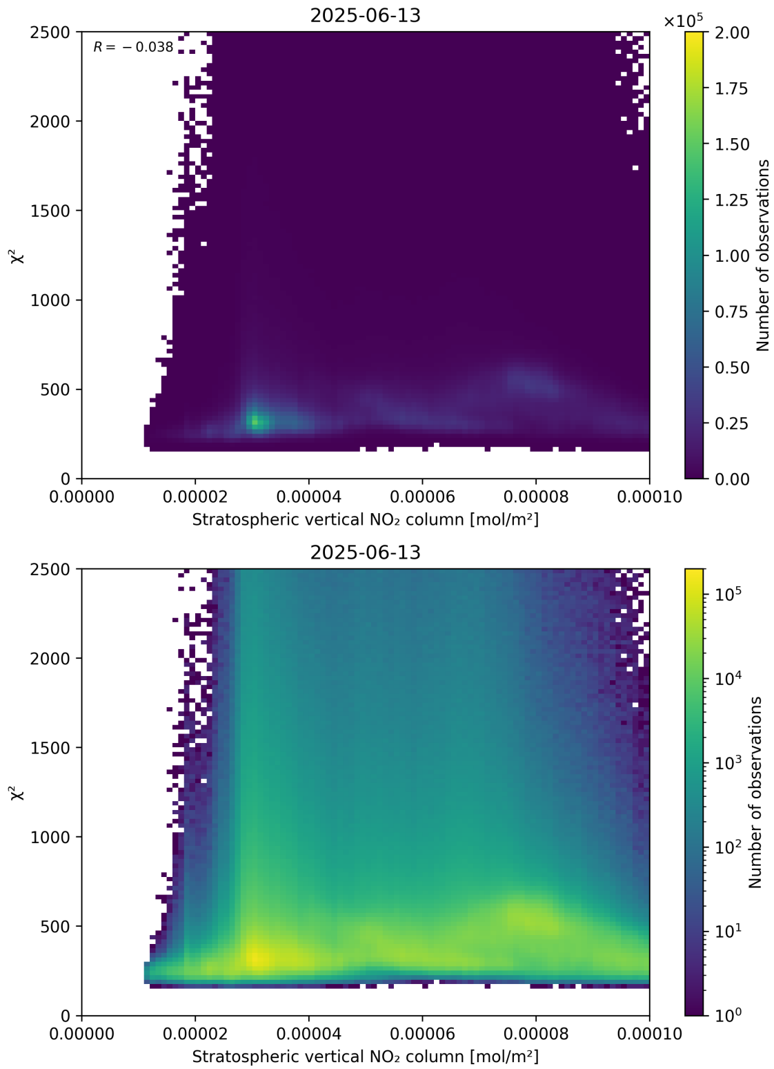
Figure 97: Scatter density plot of “Stratospheric vertical NO 2 column” against “ \chi^2 ” for 2025-06-12 to 2025-06-14.
