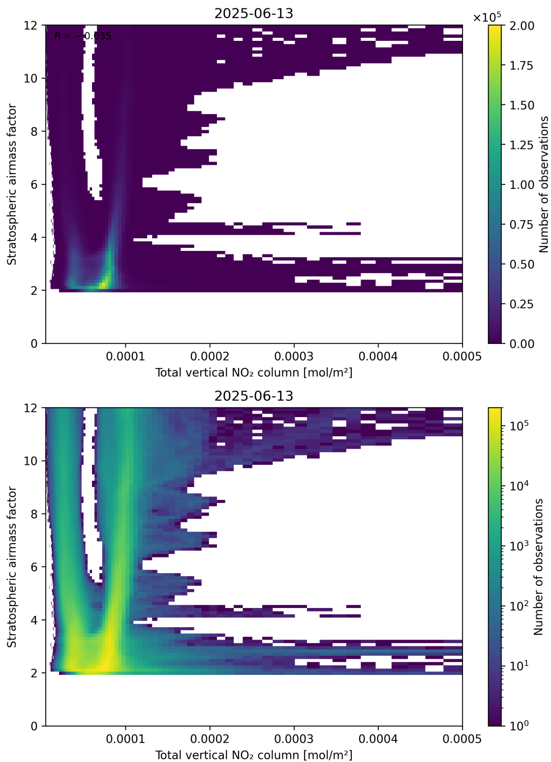
Figure 110: Scatter density plot of “Total vertical NO 2 column” against “Stratospheric airmass factor” for 2025-06-12 to 2025-06-14.
