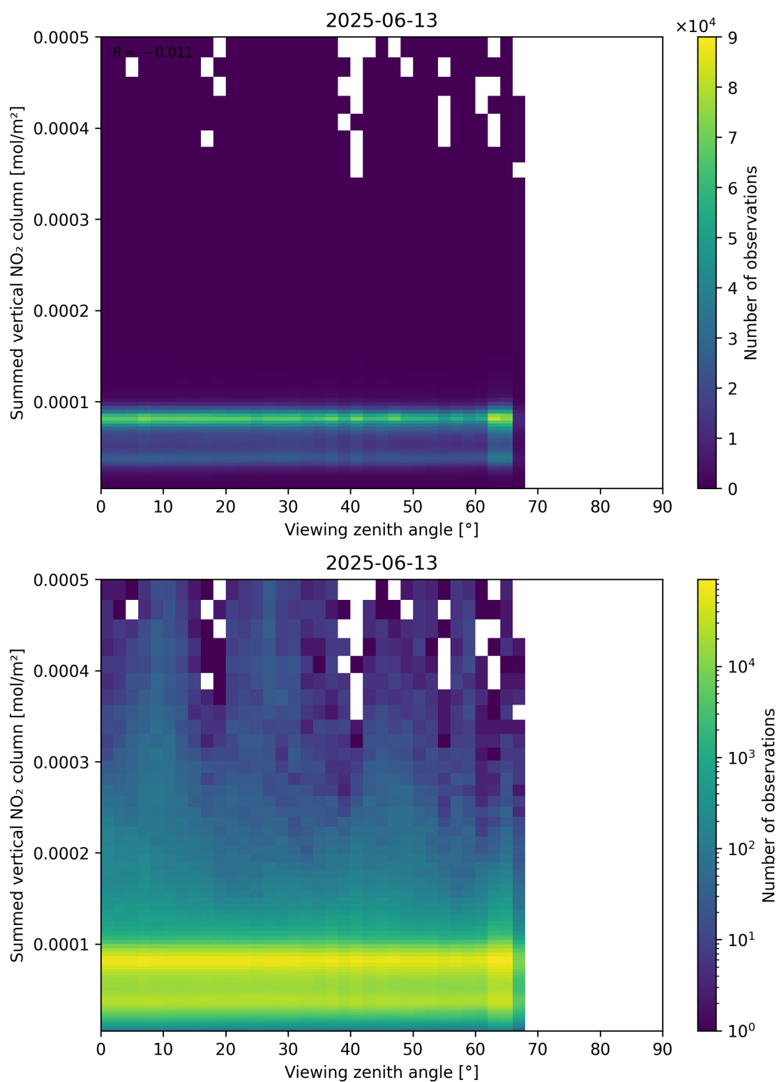
Figure 165: Scatter density plot of “Viewing zenith angle” against “Summed vertical NO 2 column” for 2025-06-12 to 2025-06-14.
