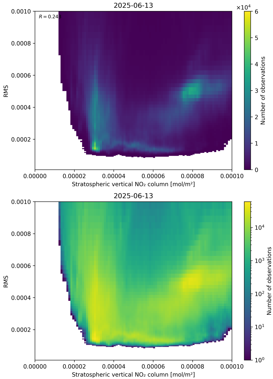
Figure 102: Scatter density plot of “Stratospheric vertical NO 2 column” against “RMS” for 2025-06-12 to 2025-06-14.
