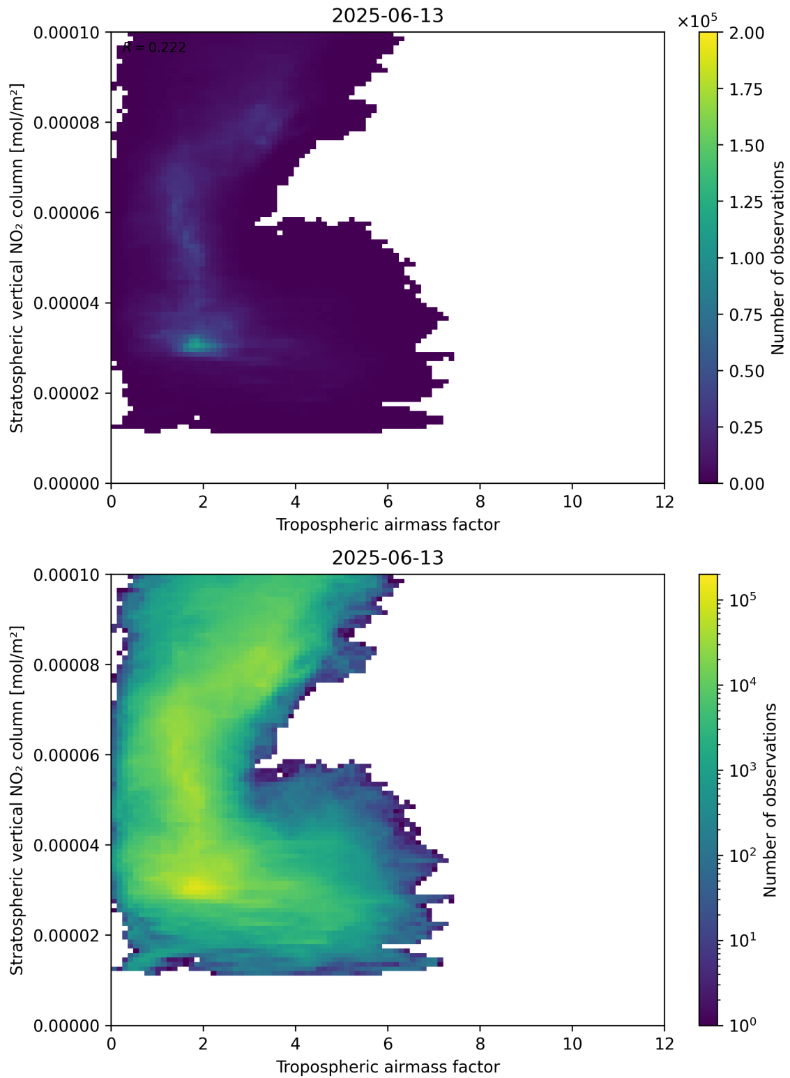
Figure 74: Scatter density plot of “Tropospheric airmass factor” against “Stratospheric vertical NO 2 column” for 2025-06-12 to 2025-06-14.
