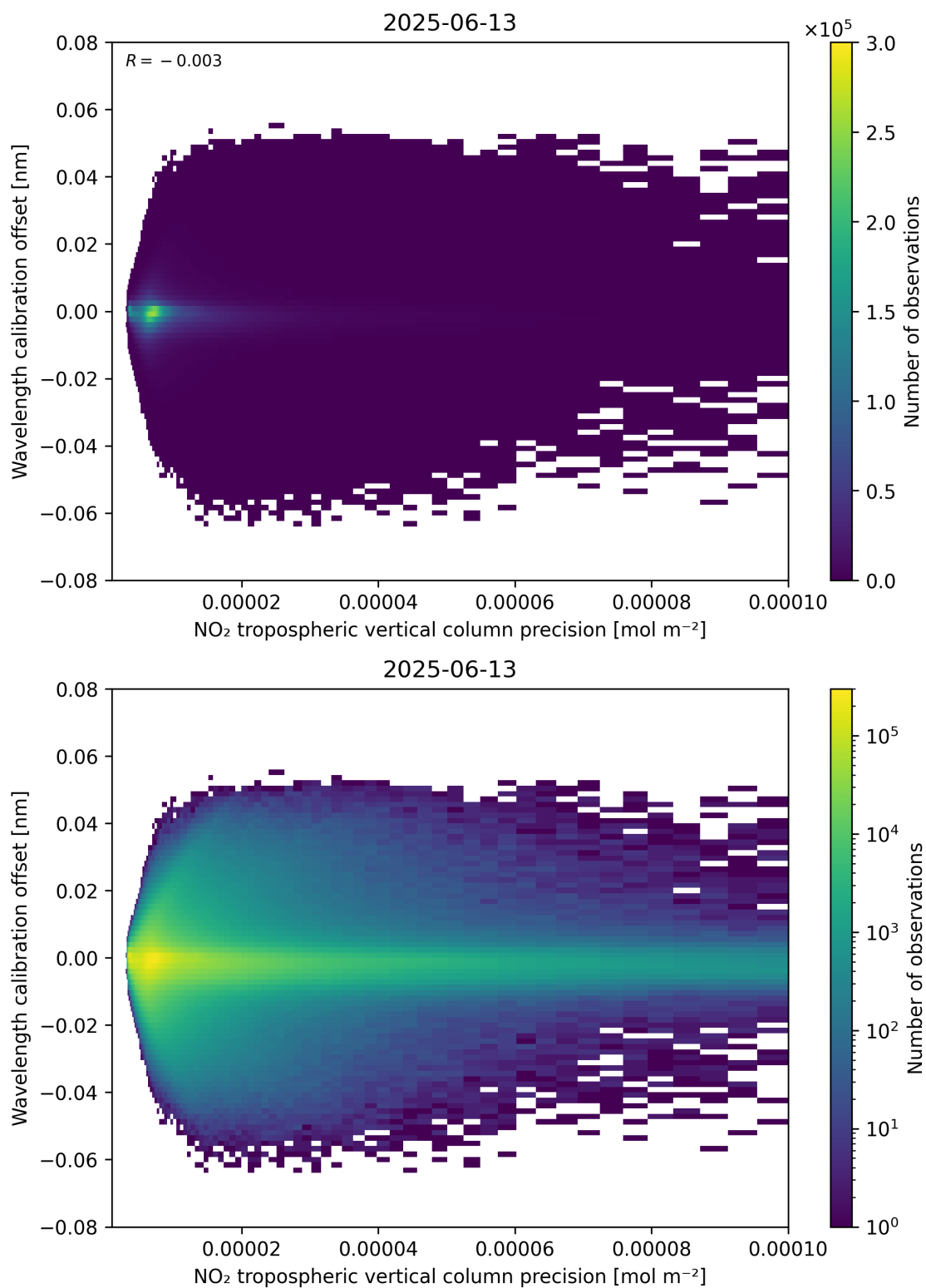
Figure 141: Scatter density plot of “NO 2 tropospheric vertical column precision” against “Wavelength calibration offset” for 2025-06-12 to 2025-06-14.
