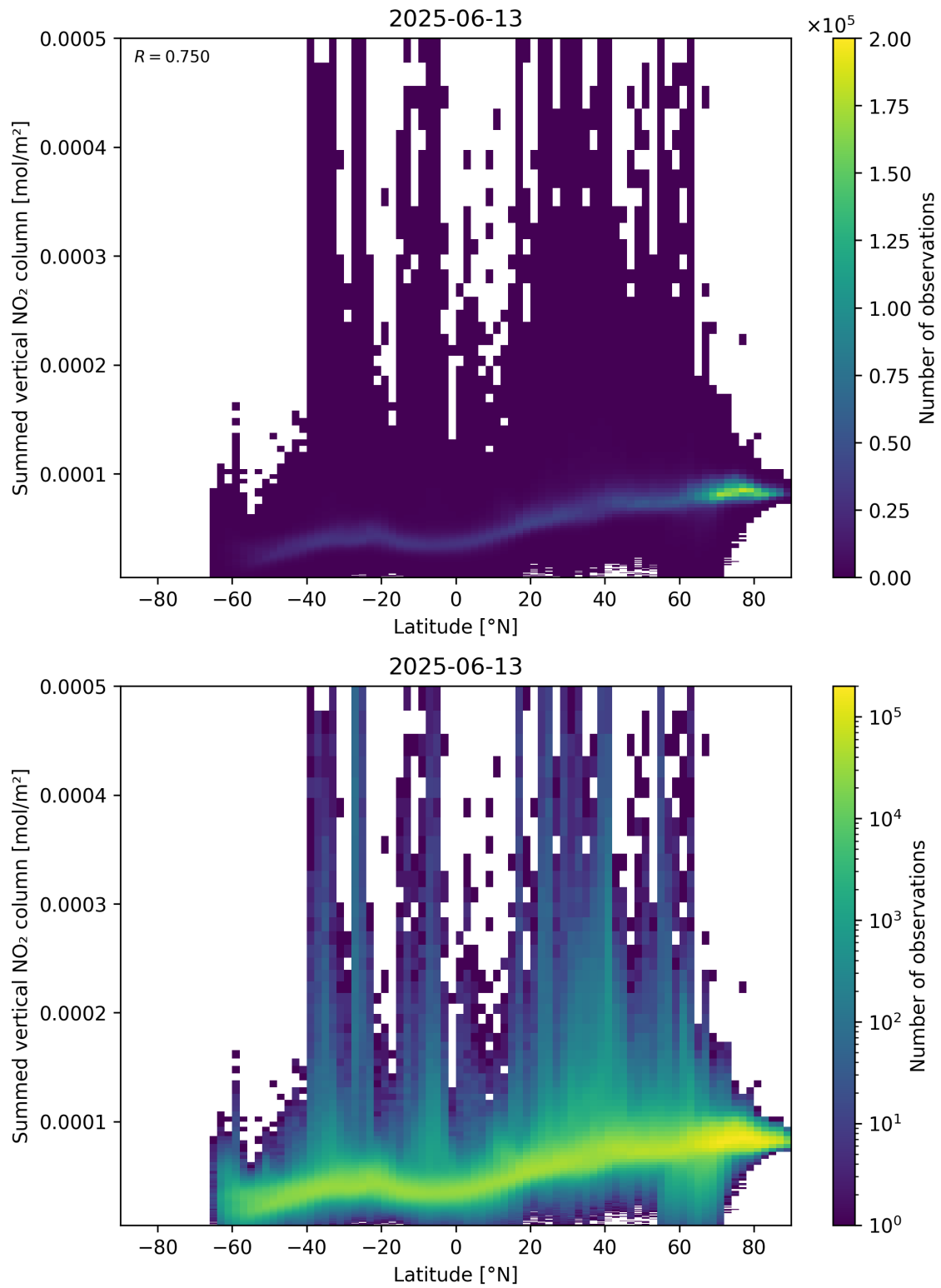
Figure 88: Scatter density plot of “Latitude” against “Summed vertical NO 2 column” for 2025-06-12 to 2025-06-14.
