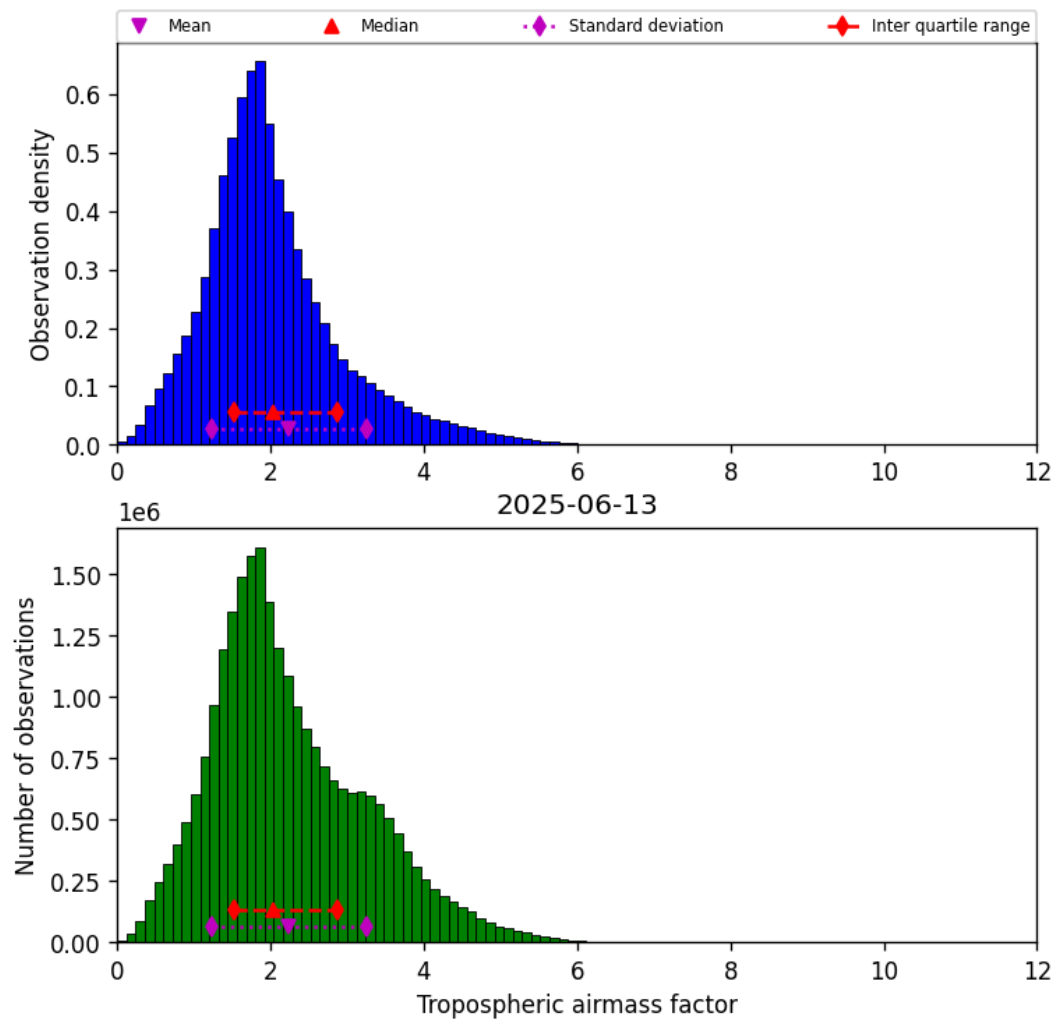
Figure 31: Histogram of “Tropospheric airmass factor” for 2025-06-12 to 2025-06-14
