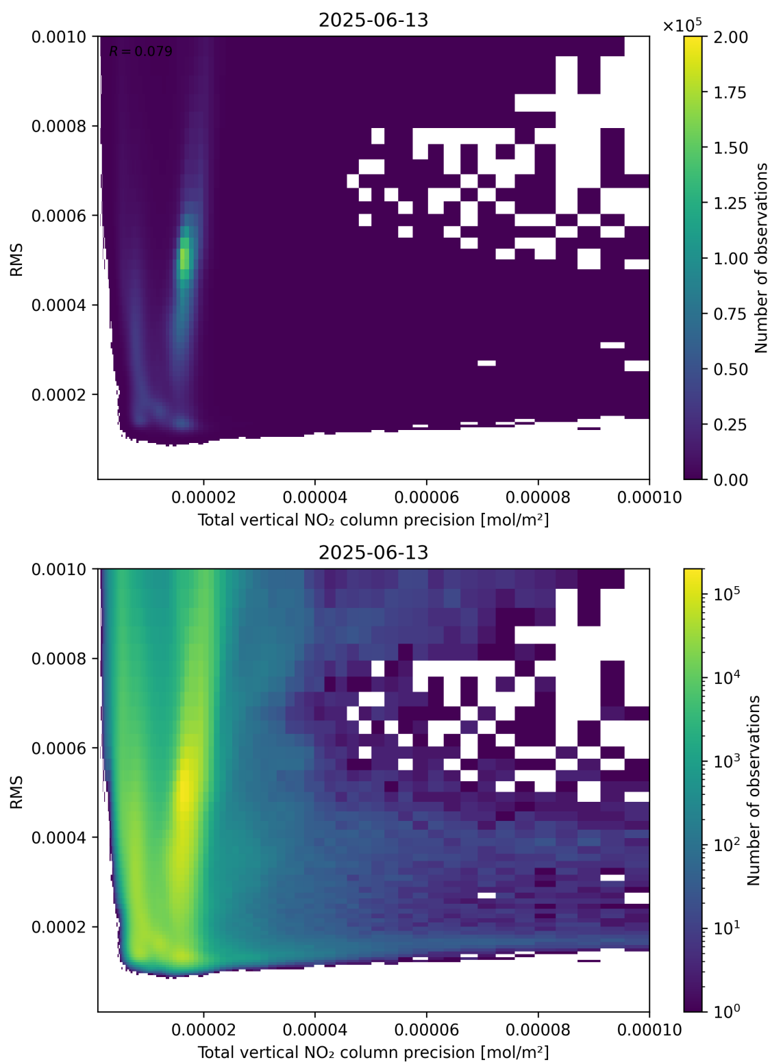
Figure 119: Scatter density plot of “Total vertical NO 2 column precision” against “RMS” for 2025-06-12 to 2025-06-14.
