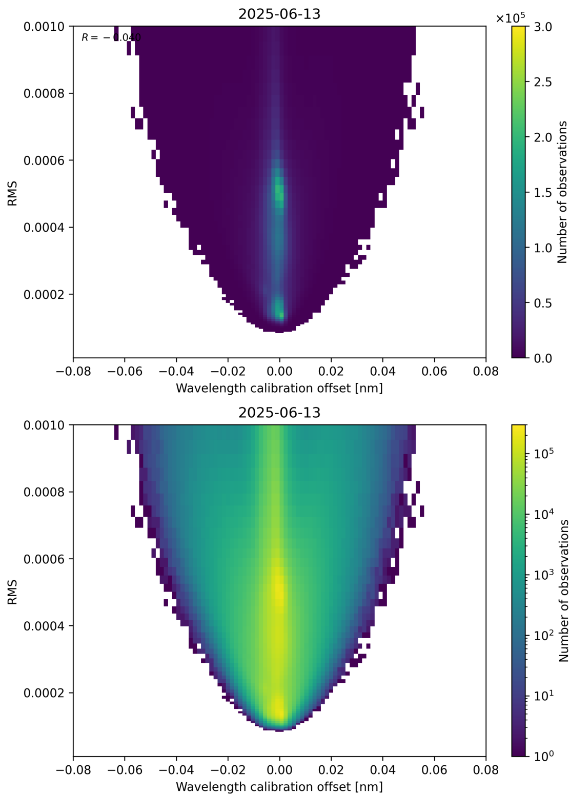
Figure 181: Scatter density plot of “Wavelength calibration offset” against “RMS” for 2025-06-12 to 2025-06-14.
