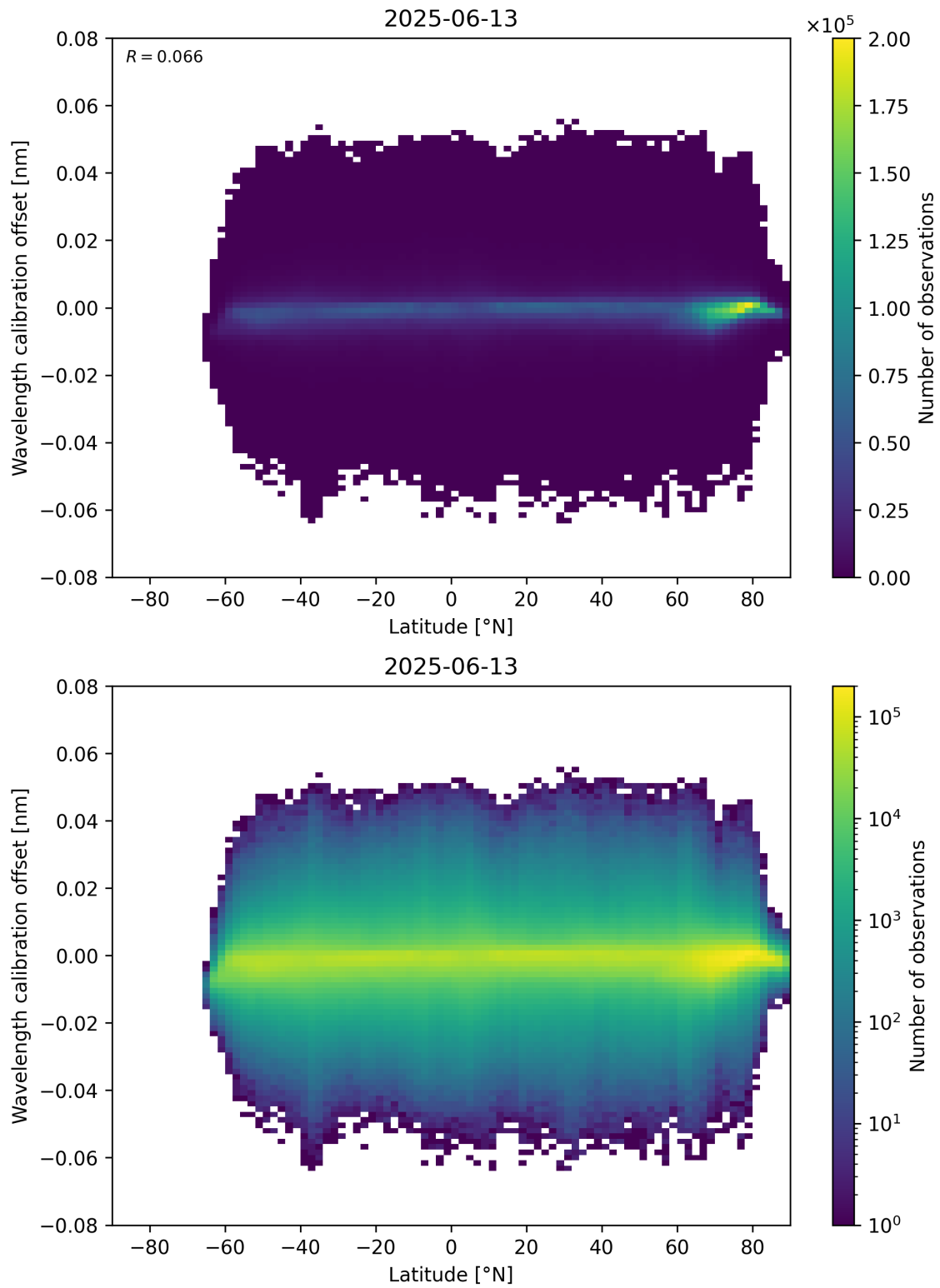
Figure 95: Scatter density plot of “Latitude” against “Wavelength calibration offset” for 2025-06-12 to 2025-06-14.
