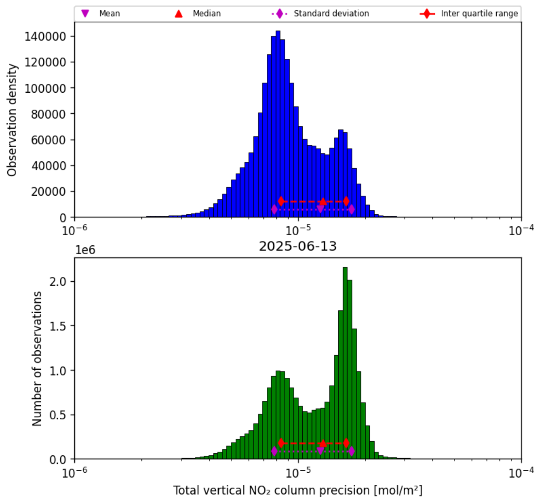
Figure 39: Histogram of "Total vertical NO 2 column precision" for 2025-06-12 to 2025-06-14
