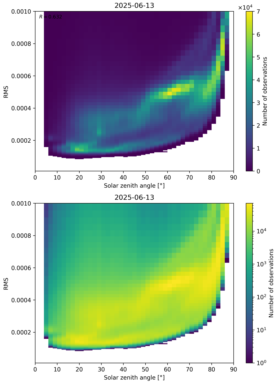
Figure 157: Scatter density plot of “Solar zenith angle” against “RMS” for 2025-06-12 to 2025-06-14.
