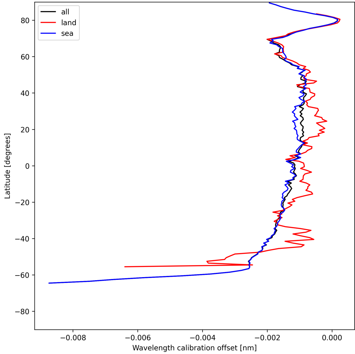
Figure 18: Zonal average of “Wavelength calibration offset” for 2025-06-12 to 2025-06-14.
