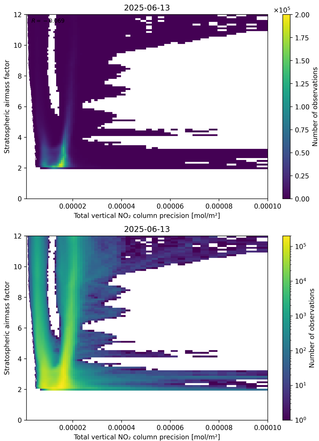
Figure 115: Scatter density plot of “Total vertical NO 2 column precision” against “Stratospheric air mass factor” for 2025-06-12 to 2025-06-14.
