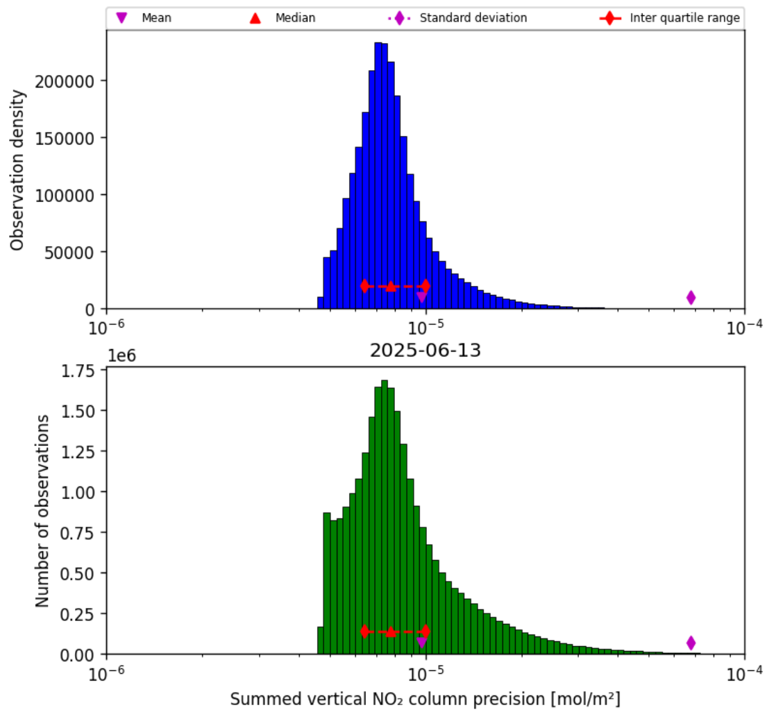
Figure 41: Histogram of "Summed vertical NO 2 column precision" for 2025-06-12 to 2025-06-14
