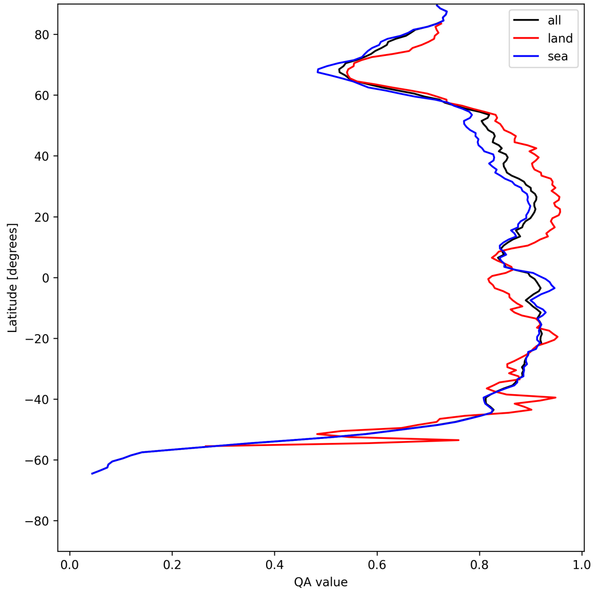
Figure 11: Zonal average of “QA value” for 2025-06-12 to 2025-06-14.
