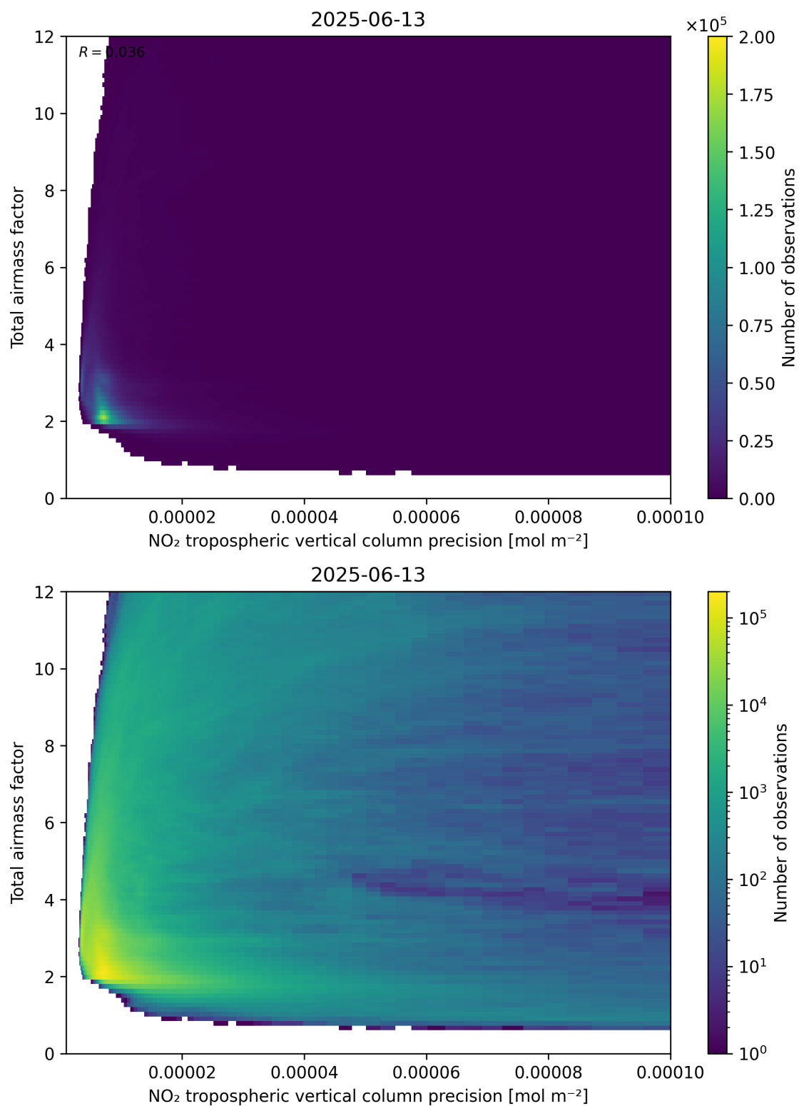
Figure 132: Scatter density plot of “NO 2 tropospheric vertical column precision” against “Total air mass factor” for 2025-06-12 to 2025-06-14.
