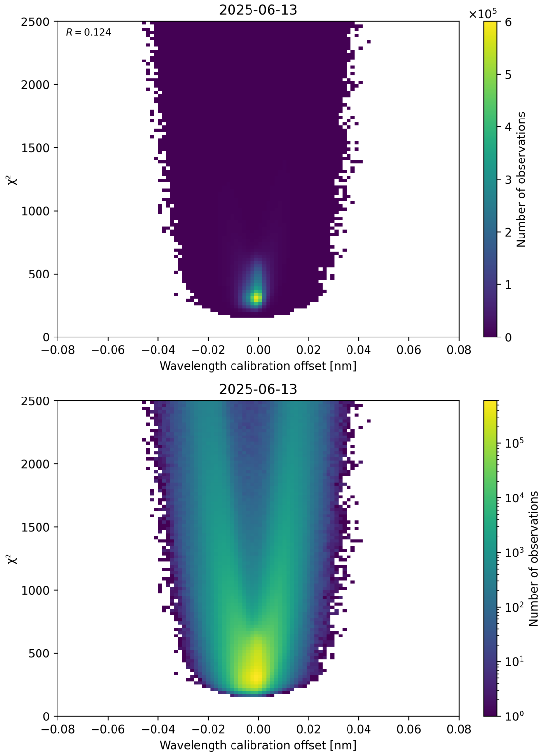
Figure 175: Scatter density plot of “Wavelength calibration offset” against “ \chi^2 ” for 2025-06-12 to 2025-06-14.
