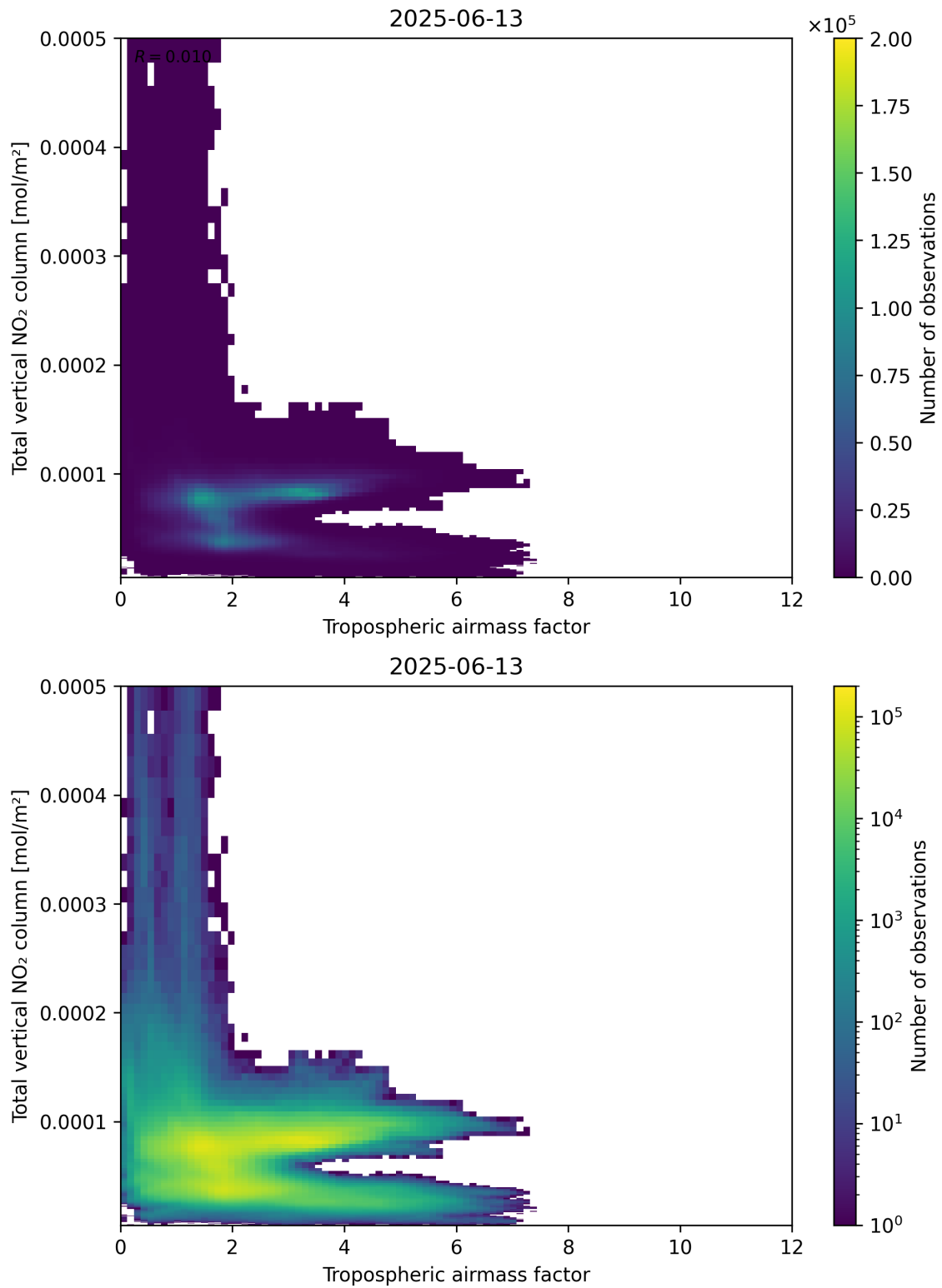
Figure 77: Scatter density plot of “Tropospheric airmass factor” against “Total vertical NO 2 column” for 2025-06-12 to 2025-06-14.
