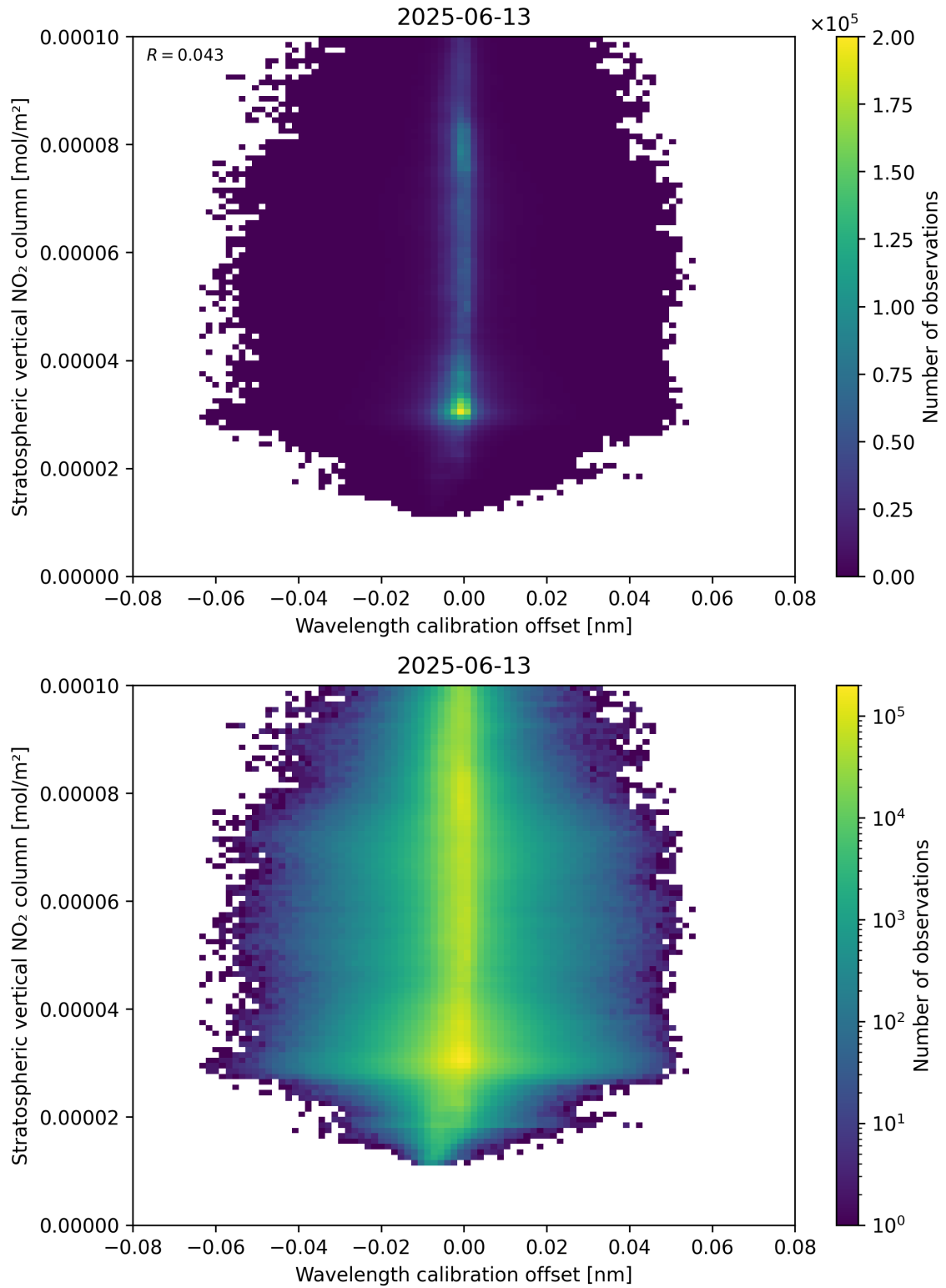
Figure 176: Scatter density plot of “Wavelength calibration offset” against “Stratospheric vertical NO 2 column” for 2025-06-12 to 2025-06-14.
