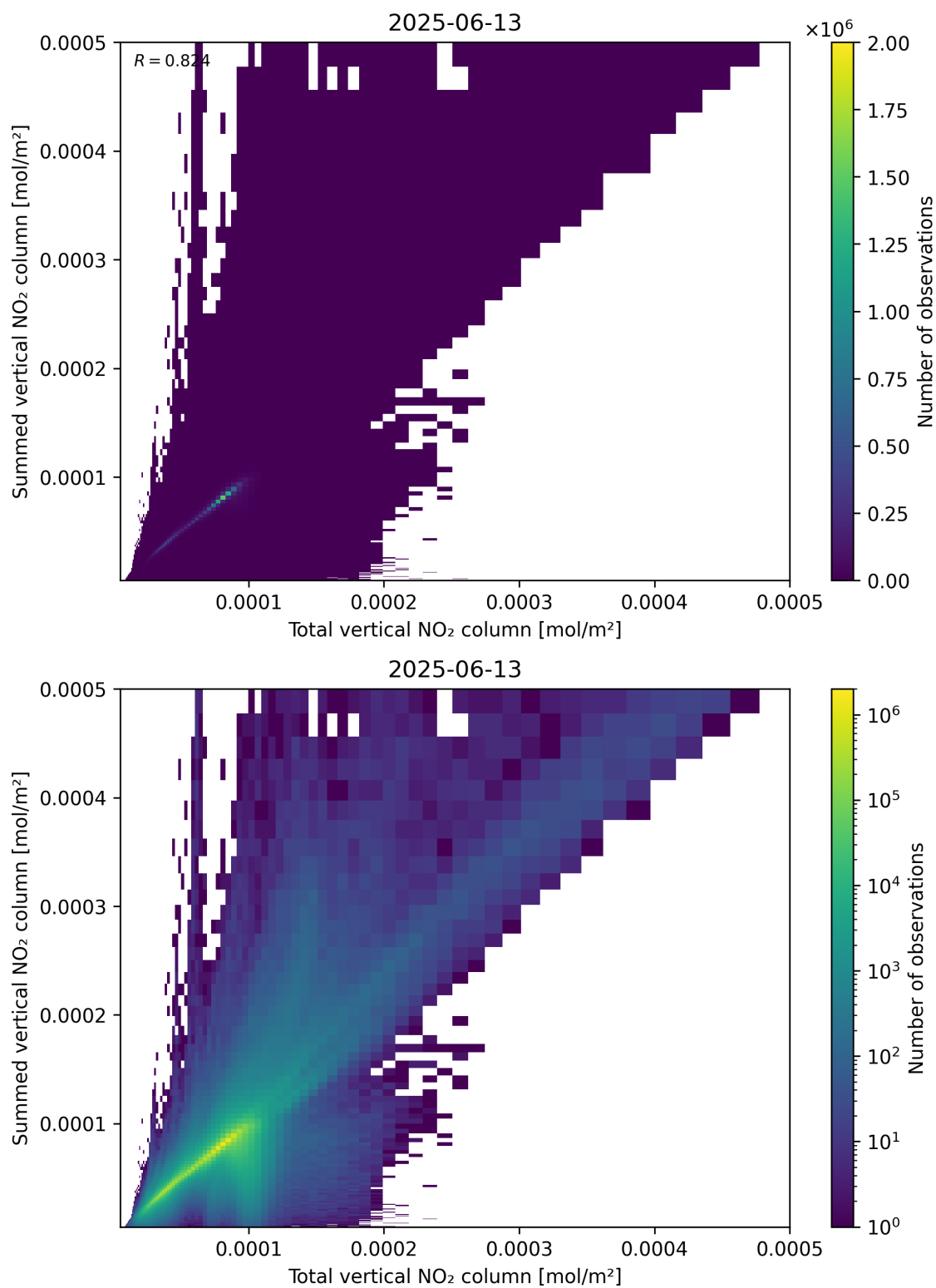
Figure 112: Scatter density plot of “Total vertical NO 2 column” against “Summed vertical NO 2 column” for 2025-06-12 to 2025-06-14.
