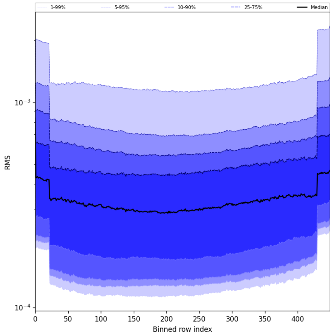
Figure 60: Along track statistics of “RMS” for 2025-06-12 to 2025-06-14
