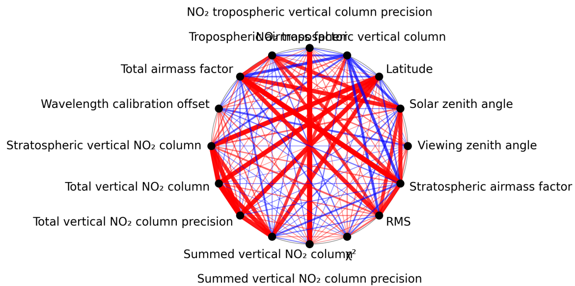
Figure 1: Map of correlation graph for 2025-06-12 to 2025-06-14.
