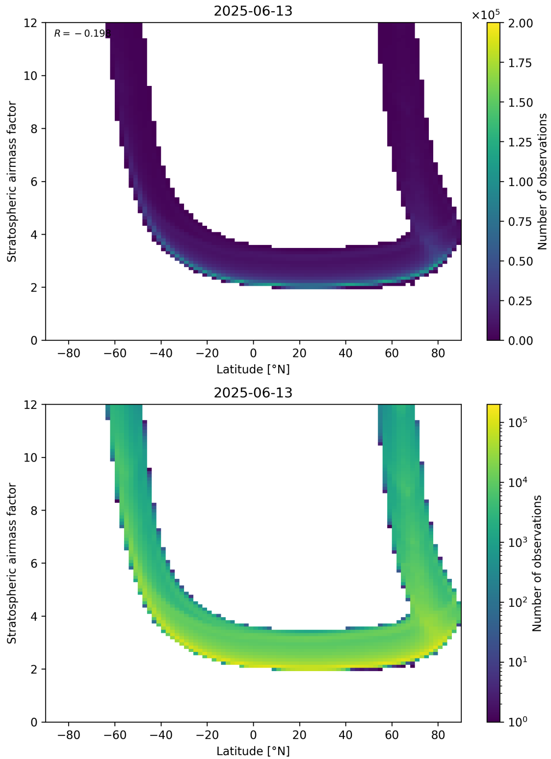
Figure 83: Scatter density plot of “Latitude” against “Stratospheric air mass factor” for 2025-06-12 to 2025-06-14.
