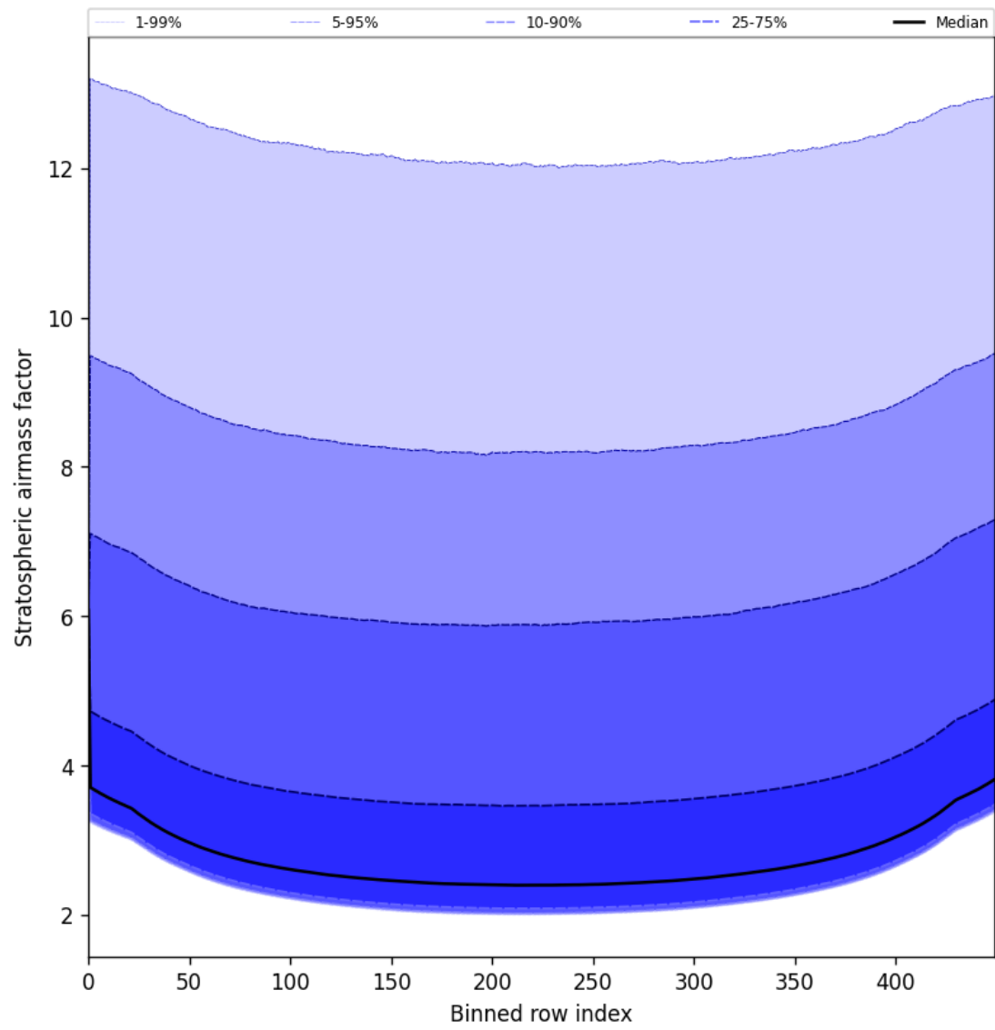
Figure 61: Along track statistics of “Stratospheric airmass factor” for 2025-06-12 to 2025-06-14
