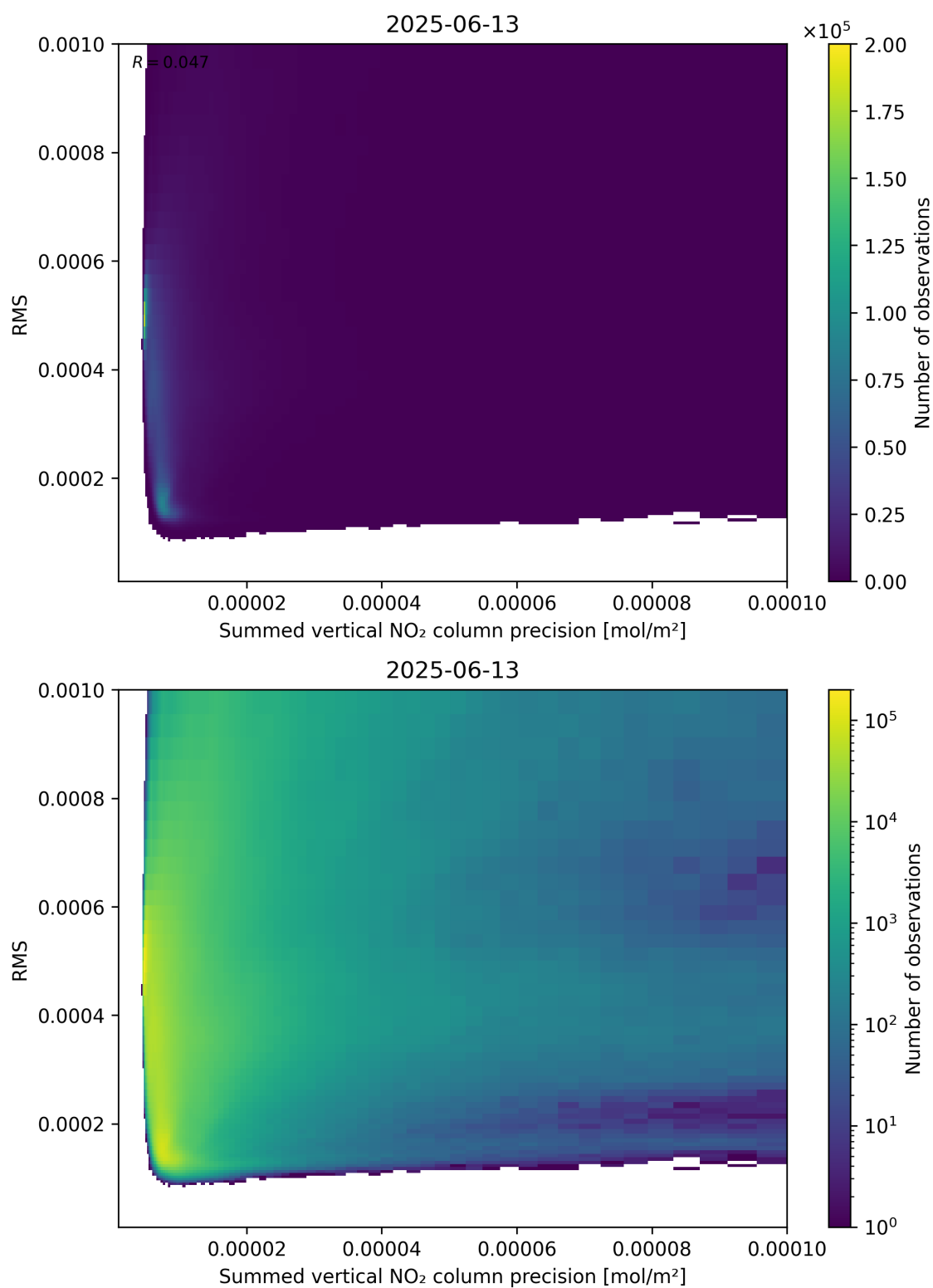
Figure 108: Scatter density plot of “Summed vertical NO 2 column precision” against “RMS” for 2025-06-12 to 2025-06-14.
