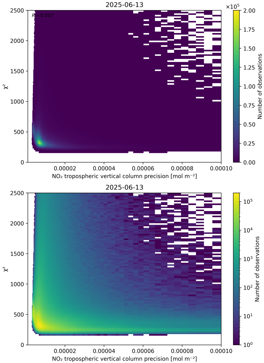
Figure 134: Scatter density plot of “NO 2 tropospheric vertical column precision” against “ \chi^2 ” for 2025-06-12 to 2025-06-14.
