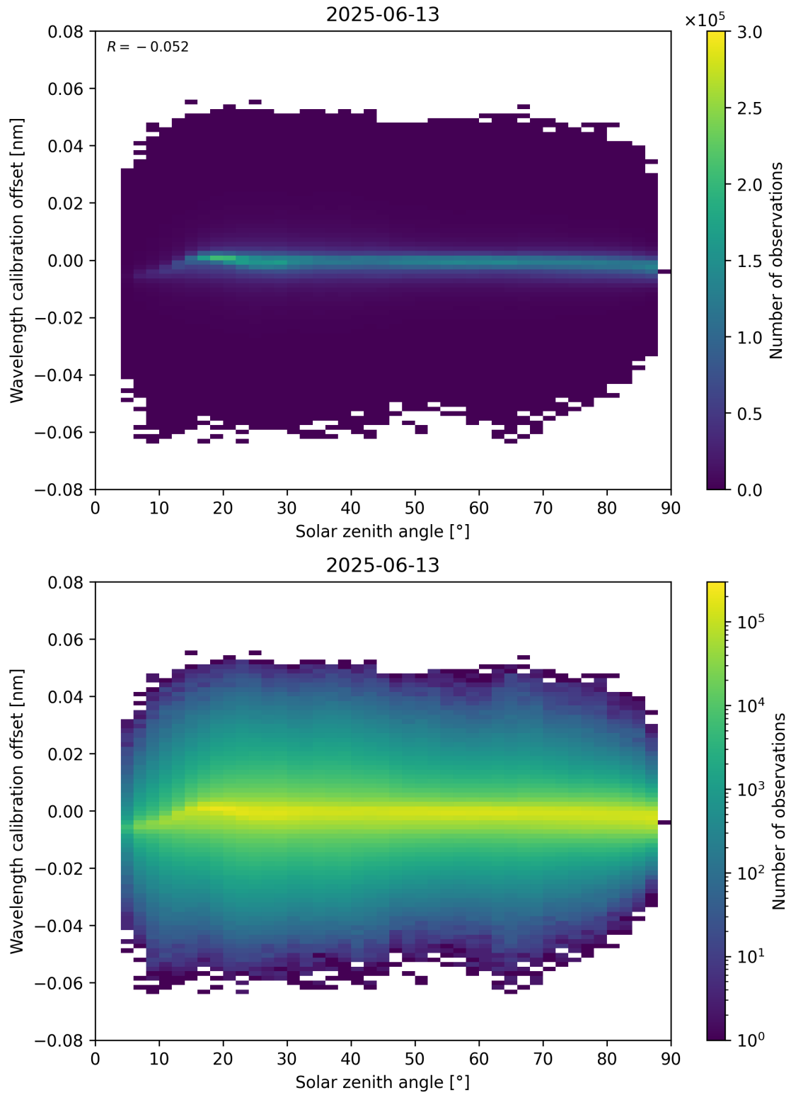
Figure 158: Scatter density plot of “Solar zenith angle” against “Wavelength calibration offset” for 2025-06-12 to 2025-06-14.
