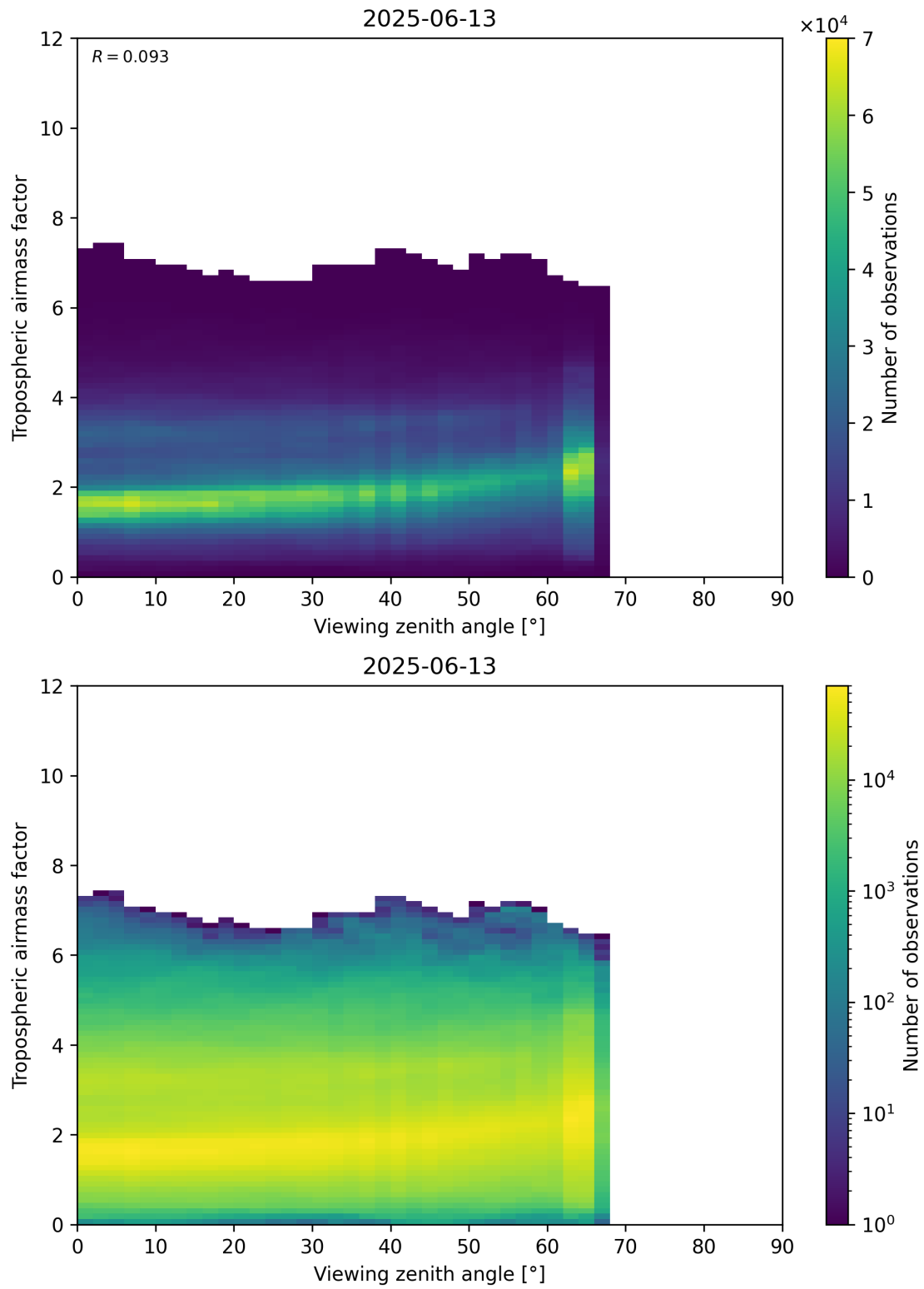
Figure 161: Scatter density plot of “Viewing zenith angle” against “Tropospheric airmass factor” for 2025-06-12 to 2025-06-14.
