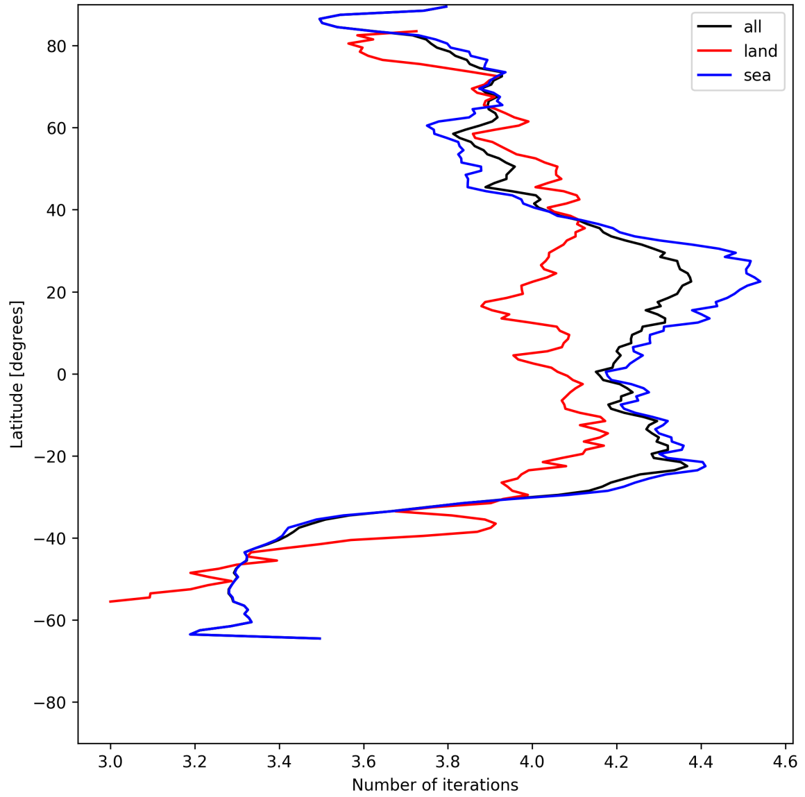
Figure 17: Zonal average of “Number of iterations” for 2025-06-12 to 2025-06-14.
