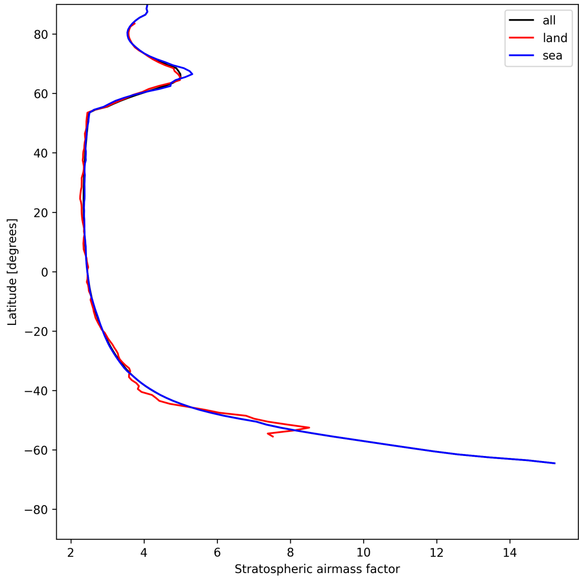
Figure 27: Zonal average of “Stratospheric air mass factor” for 2025-06-12 to 2025-06-14.
