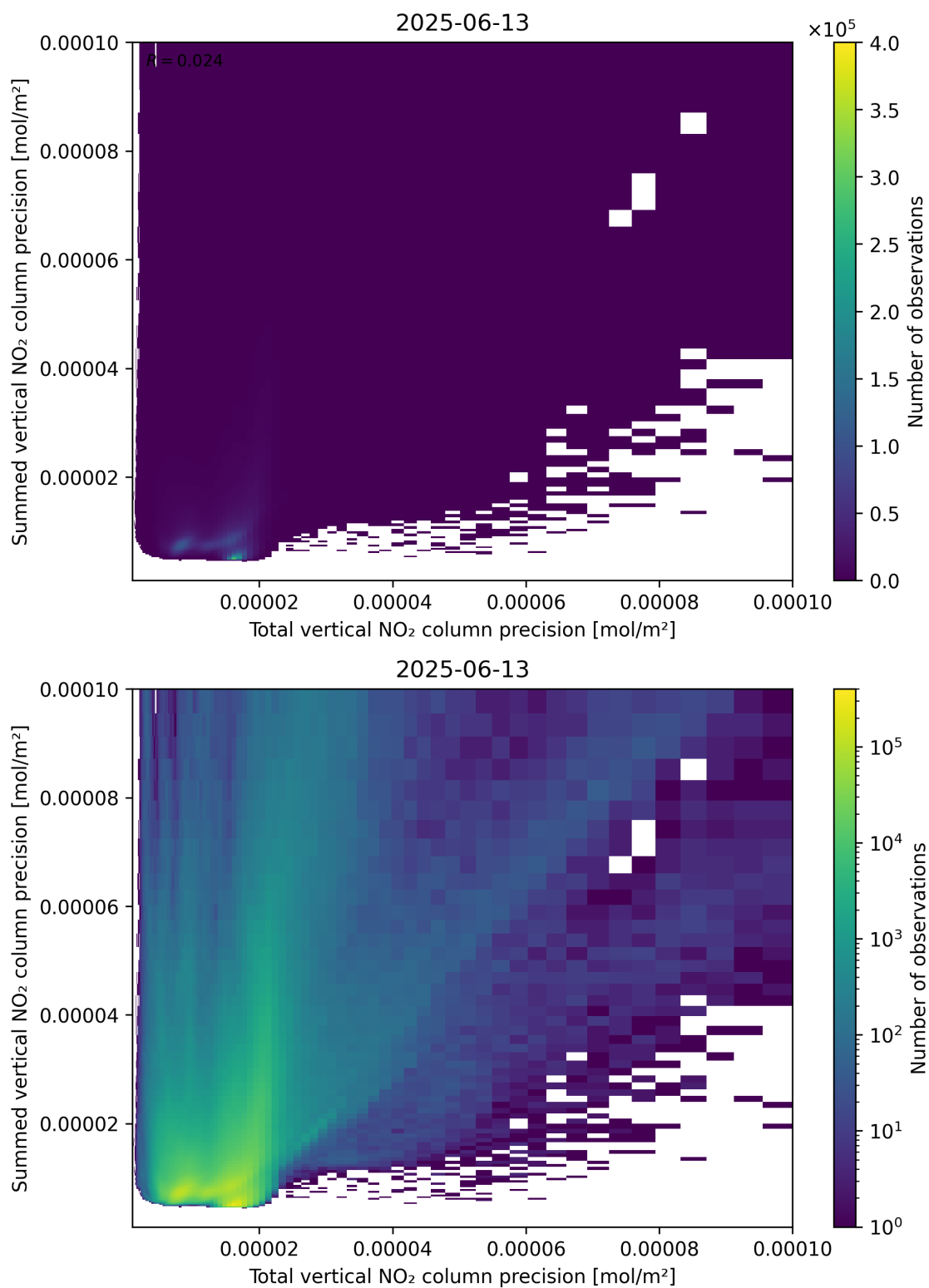
Figure 118: Scatter density plot of “Total vertical NO 2 column precision” against “Summed vertical NO 2 column precision” for 2025-06-12 to 2025-06-14.
