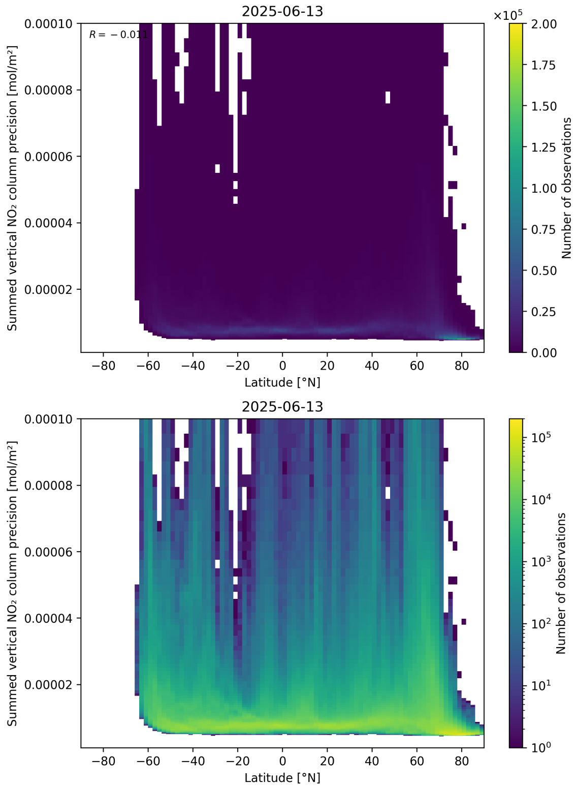
Figure 89: Scatter density plot of “Latitude” against “Summed vertical NO 2 column precision” for 2025-06-12 to 2025-06-14.
