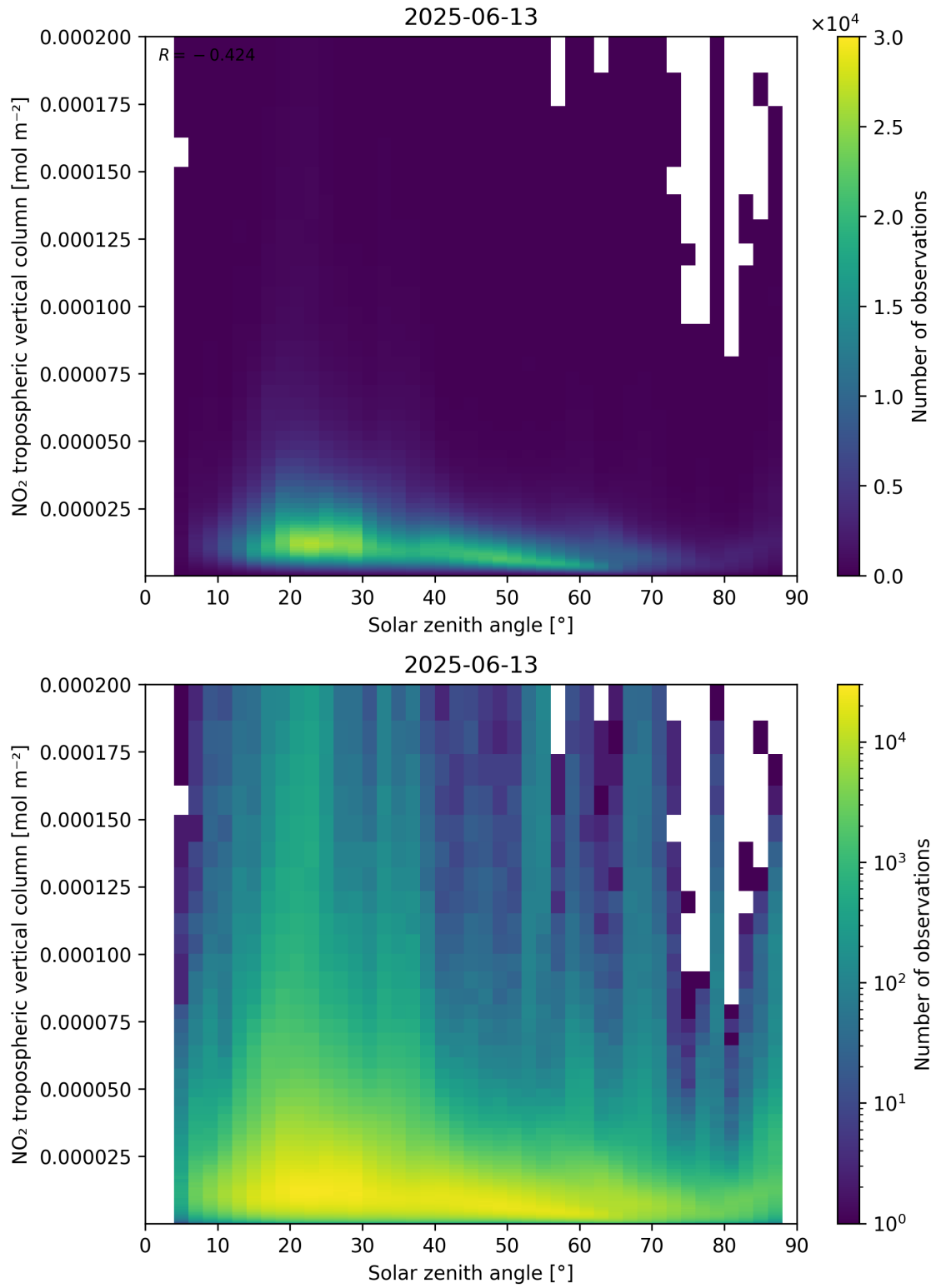
Figure 155: Scatter density plot of “Solar zenith angle” against “NO 2 tropospheric vertical column” for 2025-06-12 to 2025-06-14.
