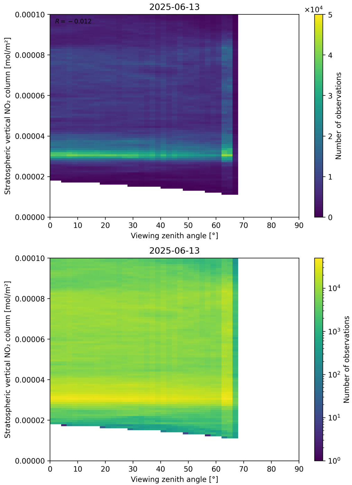
Figure 164: Scatter density plot of “Viewing zenith angle” against “Stratospheric vertical NO 2 column” for 2025-06-12 to 2025-06-14.
