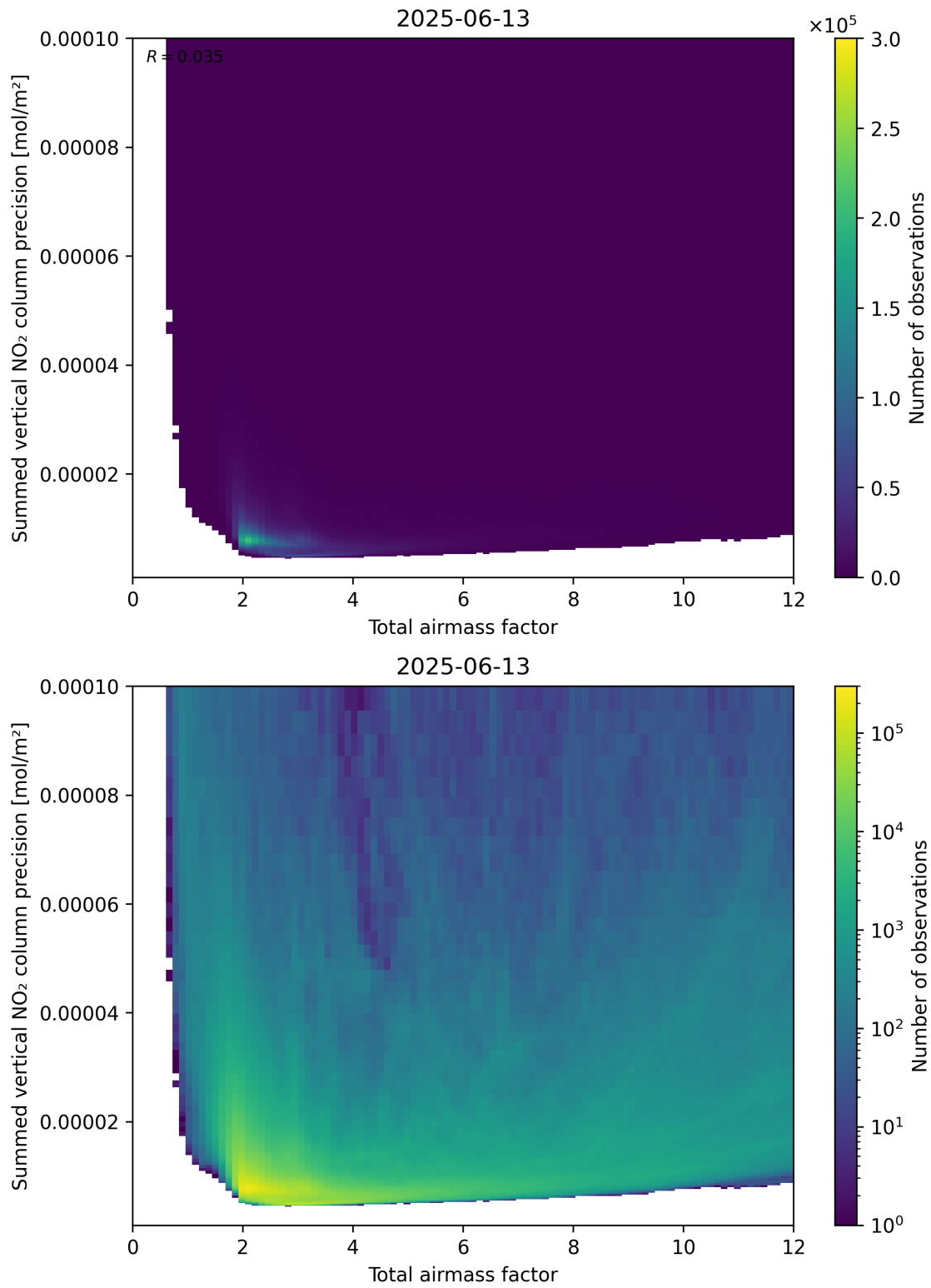
Figure 66: Scatter density plot of “Total airmass factor” against “Summed vertical NO 2 column precision” for 2025-06-12 to 2025-06-14.
