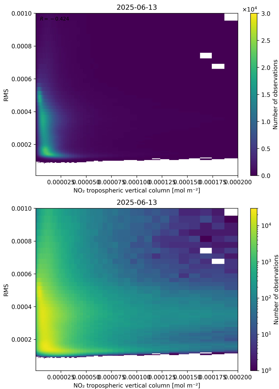
Figure 142: Scatter density plot of “NO 2 tropospheric vertical column” against “RMS” for 2025-06-12 to 2025-06-14.
