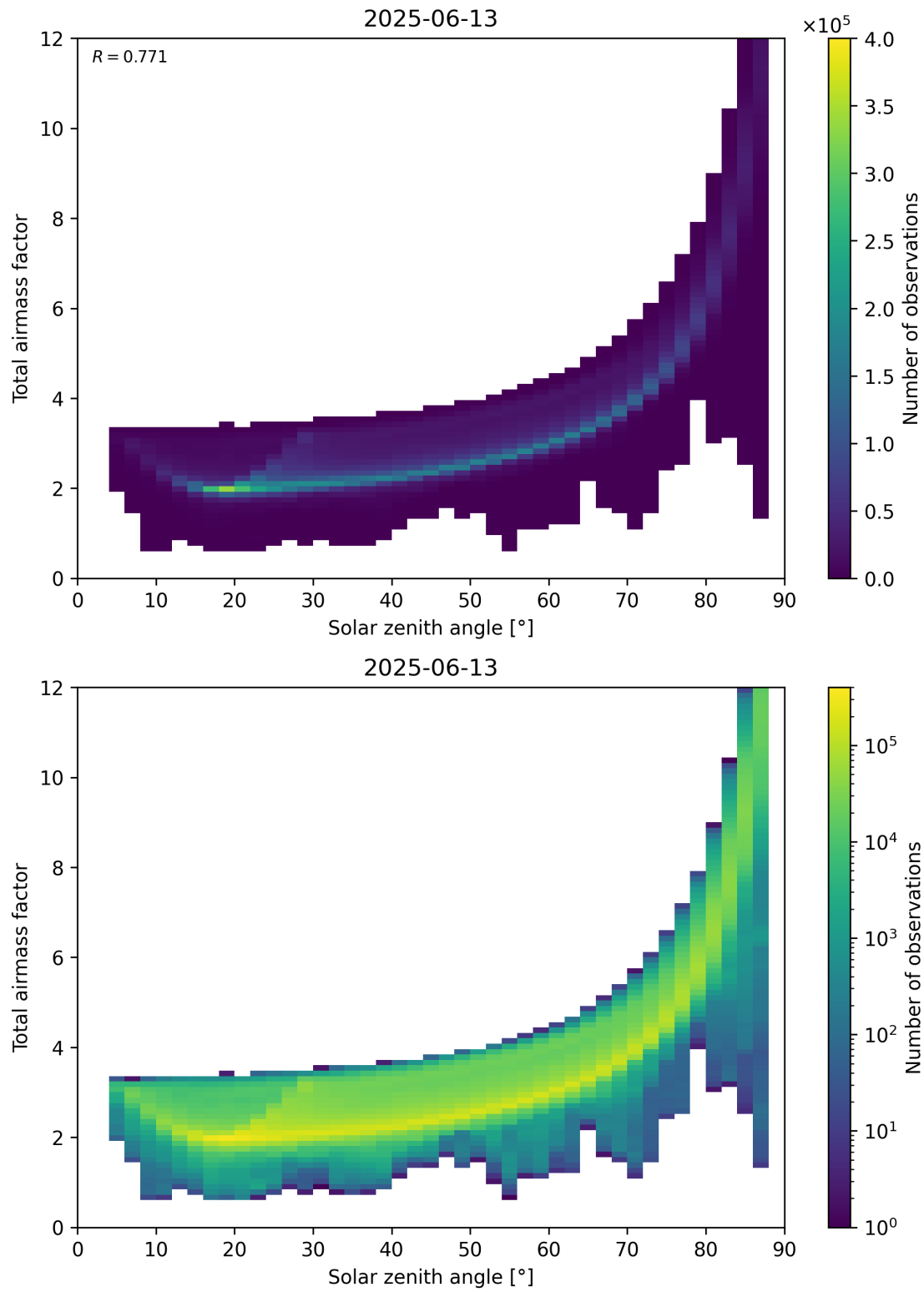
Figure 146: Scatter density plot of “Solar zenith angle” against “Total air mass factor” for 2025-06-12 to 2025-06-14.
