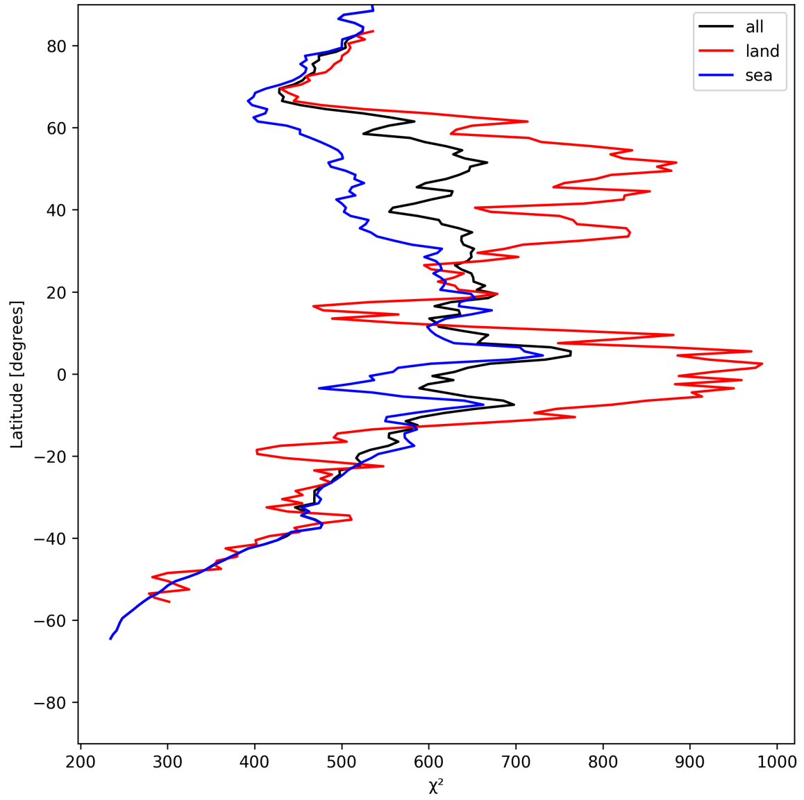
Figure 25: Zonal average of “ \chi^2 ” for 2025-06-12 to 2025-06-14.
