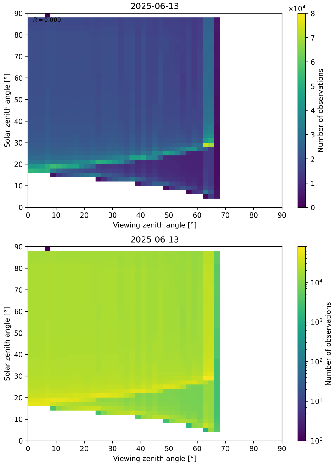
Figure 172: Scatter density plot of “Viewing zenith angle” against “Solar zenith angle” for 2025-06-12 to 2025-06-14.
