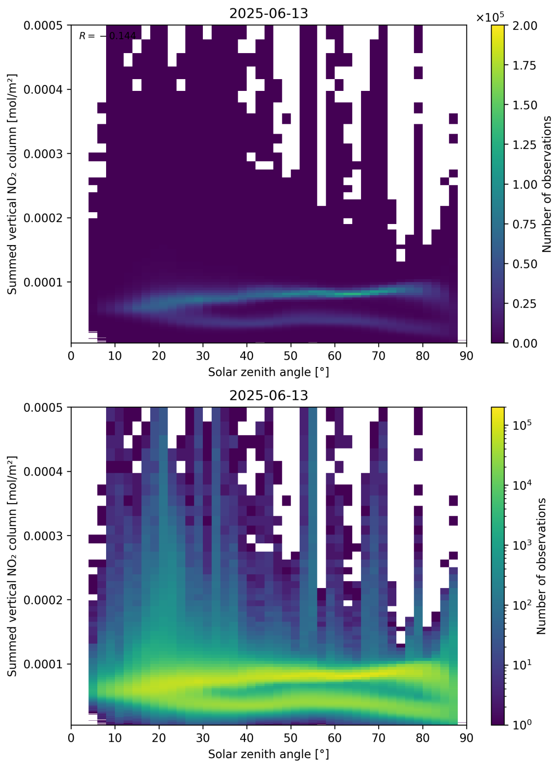
Figure 151: Scatter density plot of “Solar zenith angle” against “Summed vertical NO 2 column” for 2025-06-12 to 2025-06-14.
