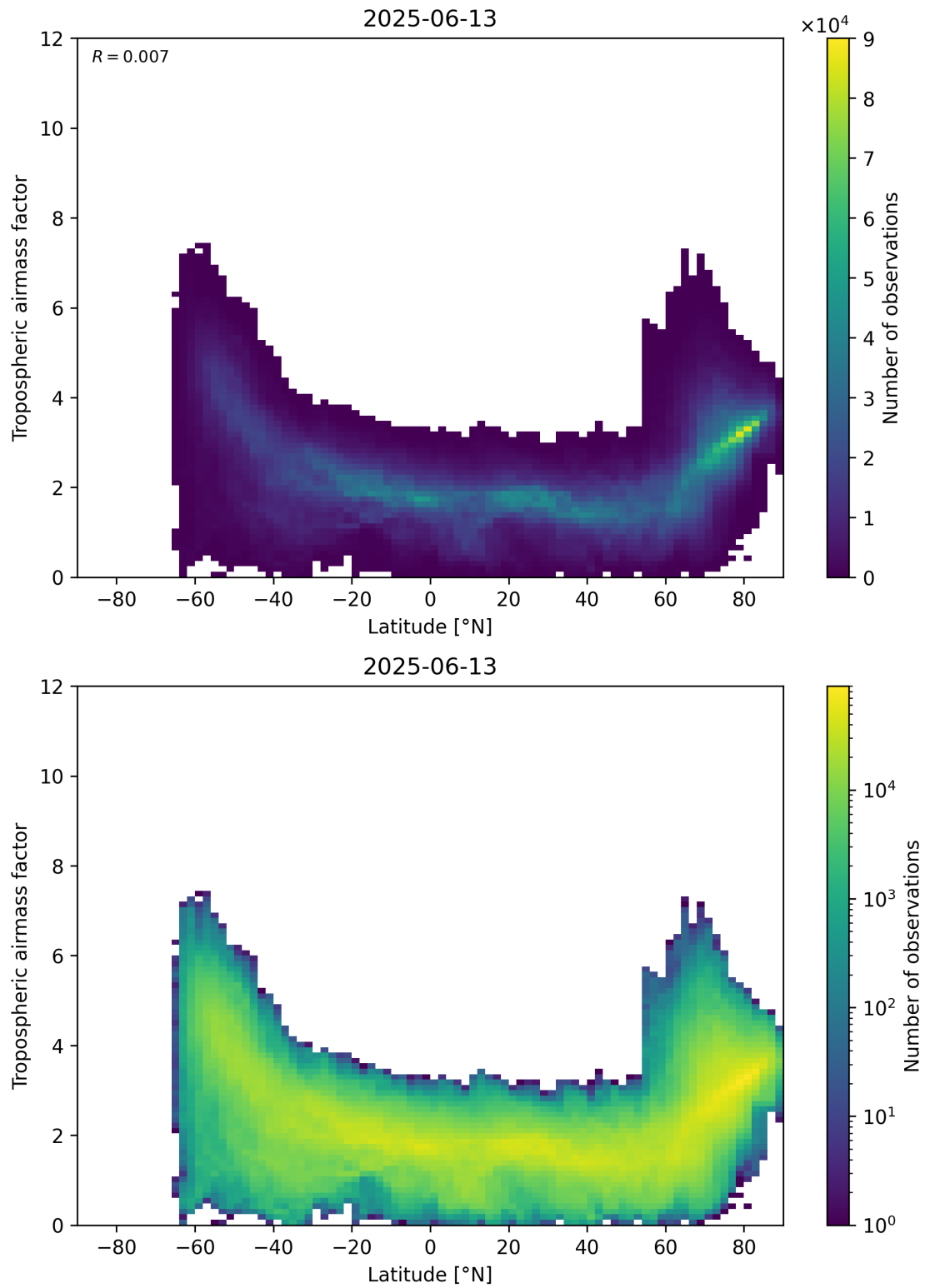
Figure 85: Scatter density plot of “Latitude” against “Tropospheric air mass factor” for 2025-06-12 to 2025-06-14.
