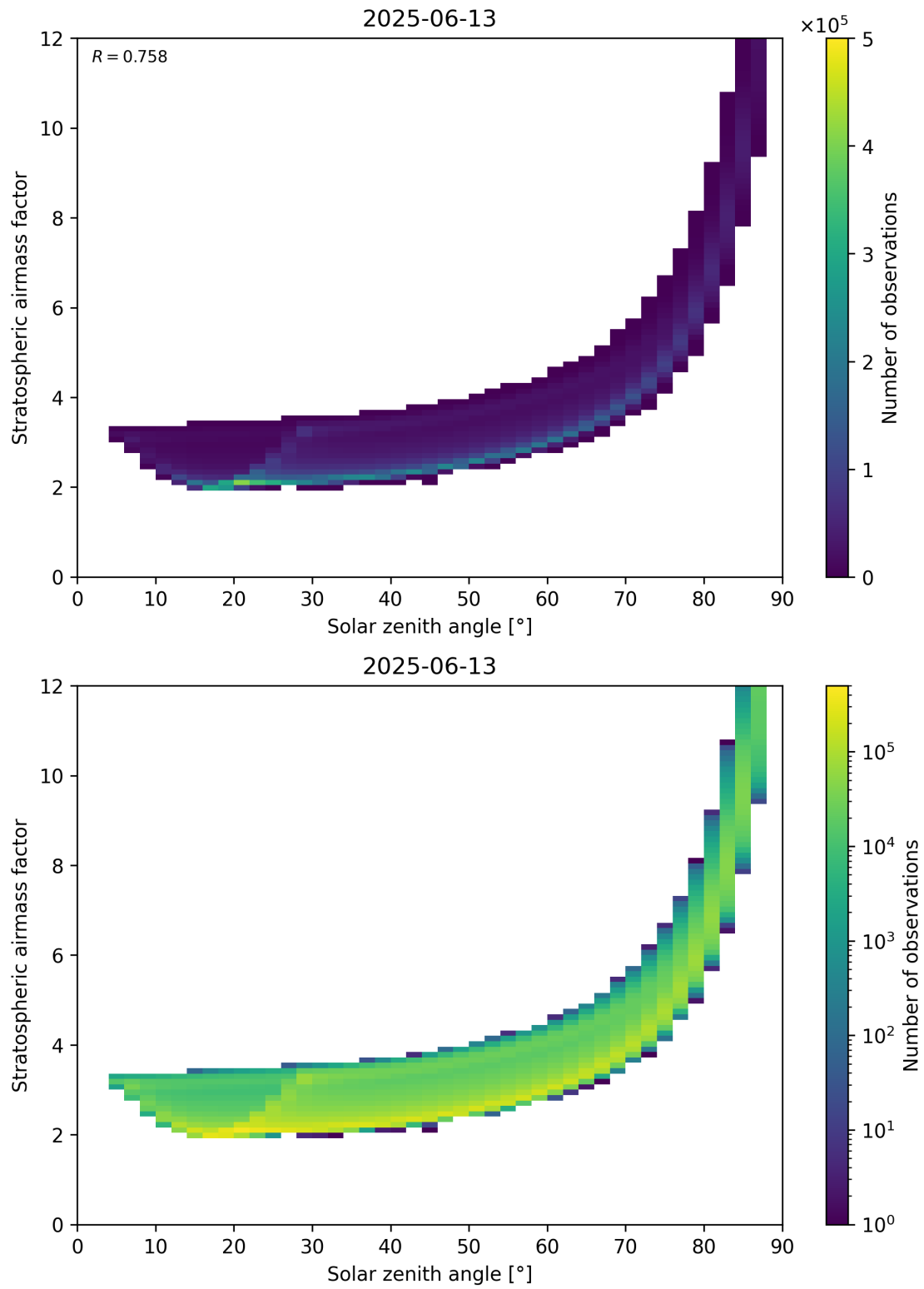
Figure 145: Scatter density plot of “Solar zenith angle” against “Stratospheric airmass factor” for 2025-06-12 to 2025-06-14.
