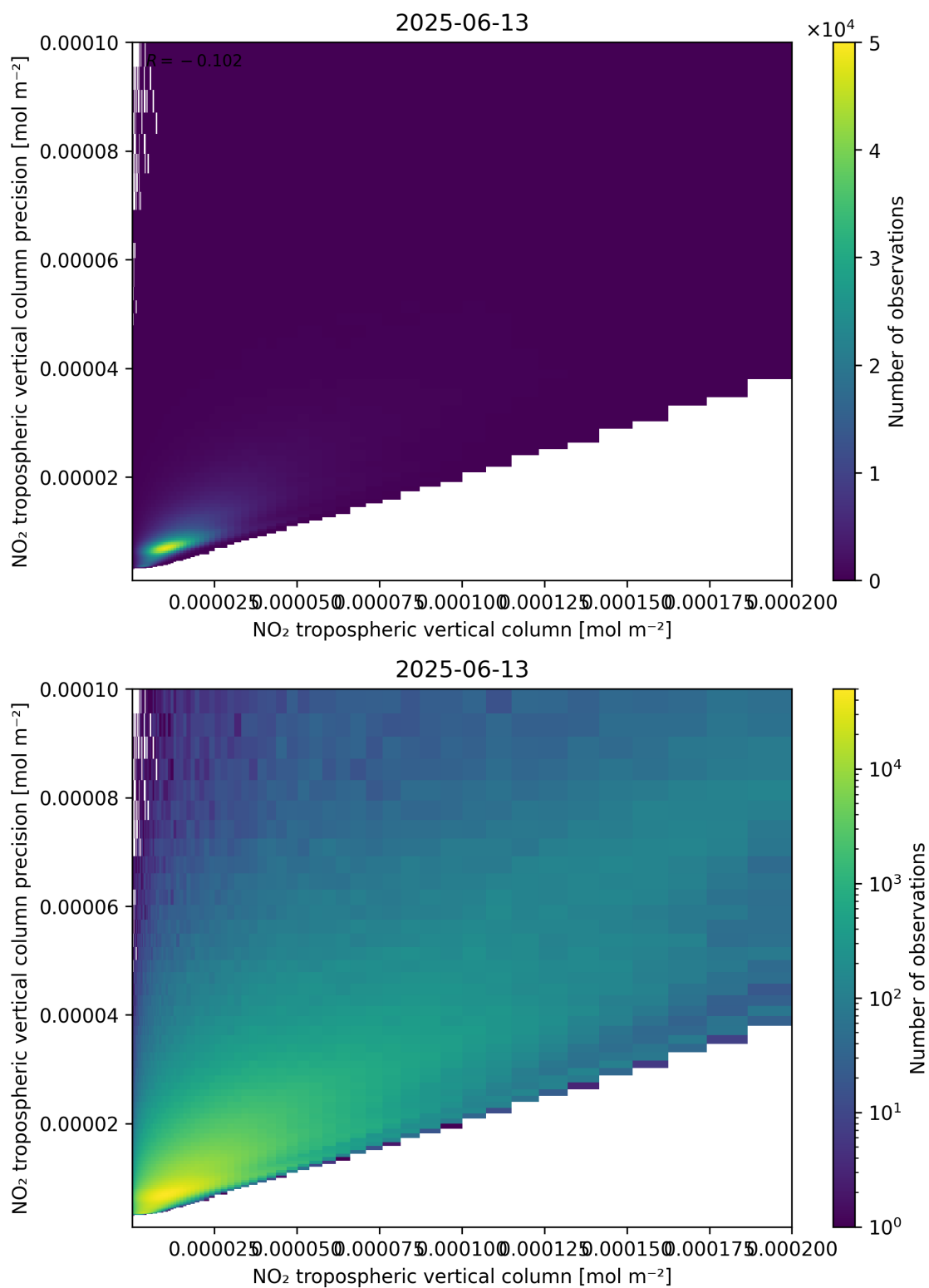
Figure 130: Scatter density plot of “NO 2 tropospheric vertical column” against “NO 2 tropospheric vertical column precision” for 2025-06-12 to 2025-06-14.
