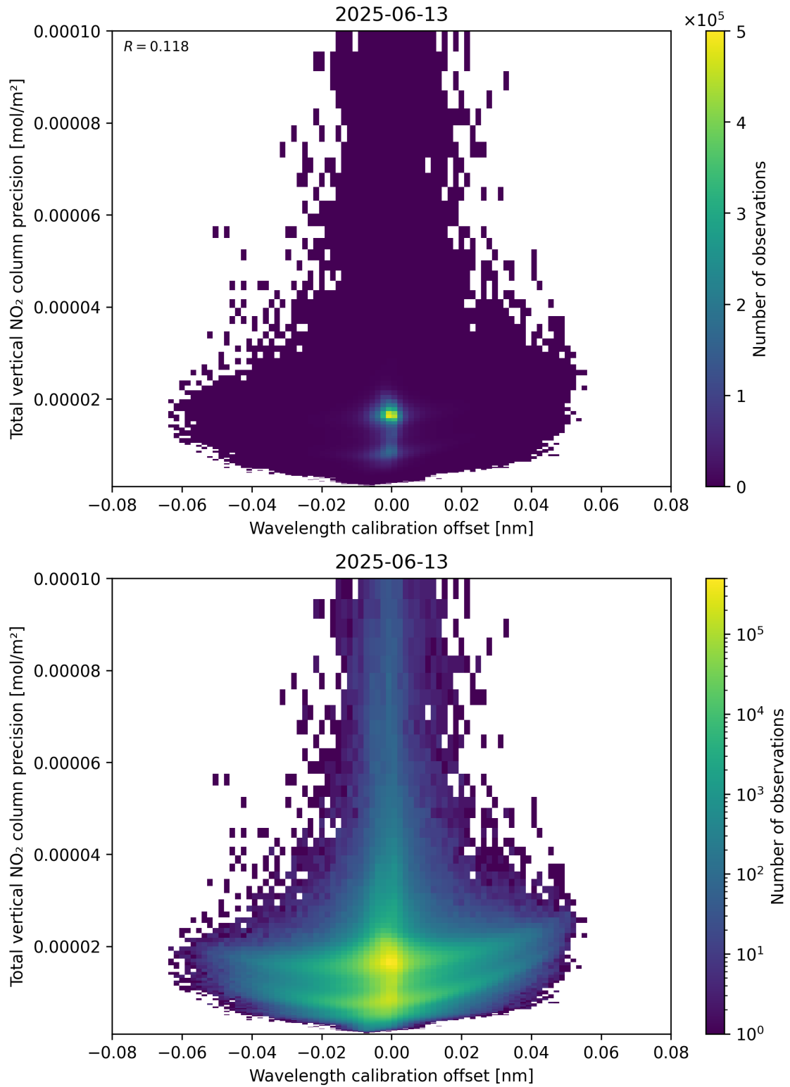
Figure 180: Scatter density plot of “Wavelength calibration offset” against “Total vertical NO 2 column precision” for 2025-06-12 to 2025-06-14.
