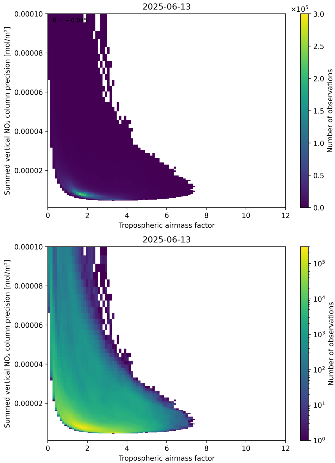
Figure 76: Scatter density plot of “Tropospheric air mass factor” against “Summed vertical NO 2 column precision” for 2025-06-12 to 2025-06-14.
