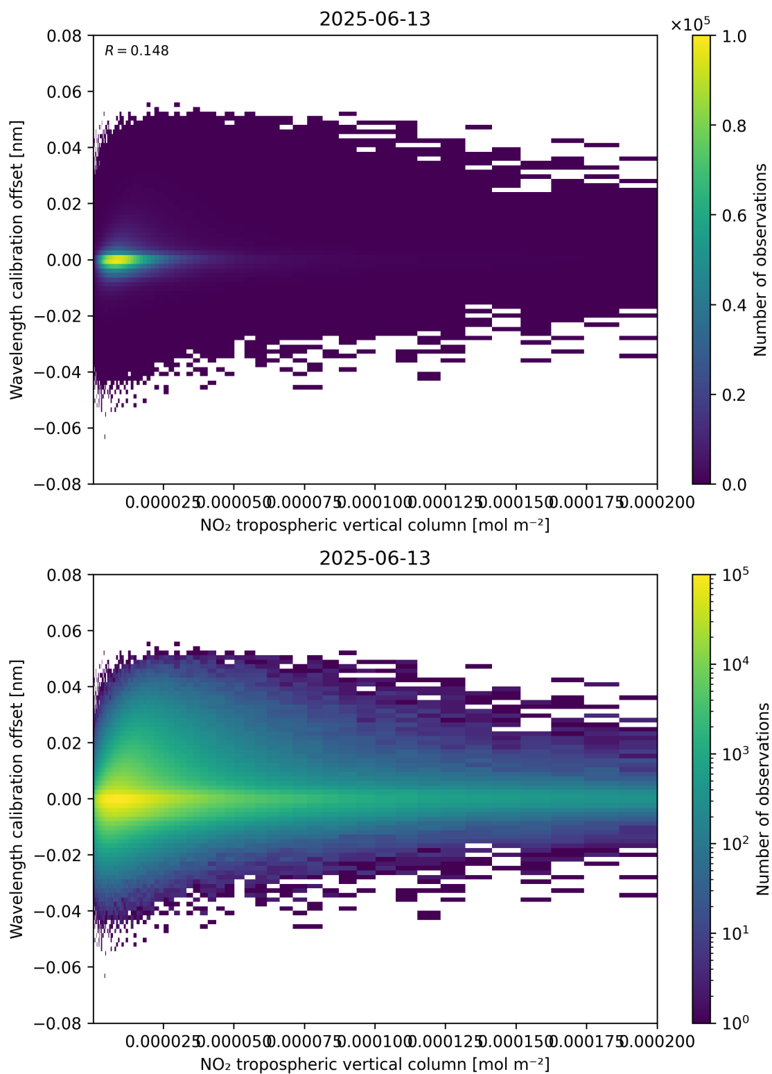
Figure 143: Scatter density plot of “NO 2 tropospheric vertical column” against “Wavelength calibration offset” for 2025-06-12 to 2025-06-14.
