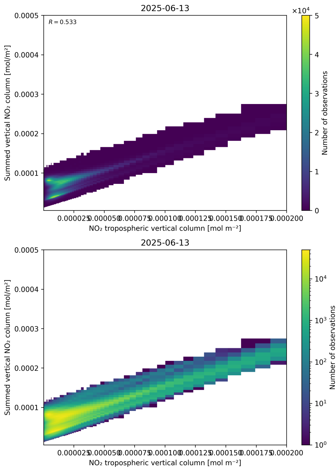
Figure 126: Scatter density plot of “NO 2 tropospheric vertical column” against “Summed vertical NO 2 column” for 2025-06-12 to 2025-06-14.
