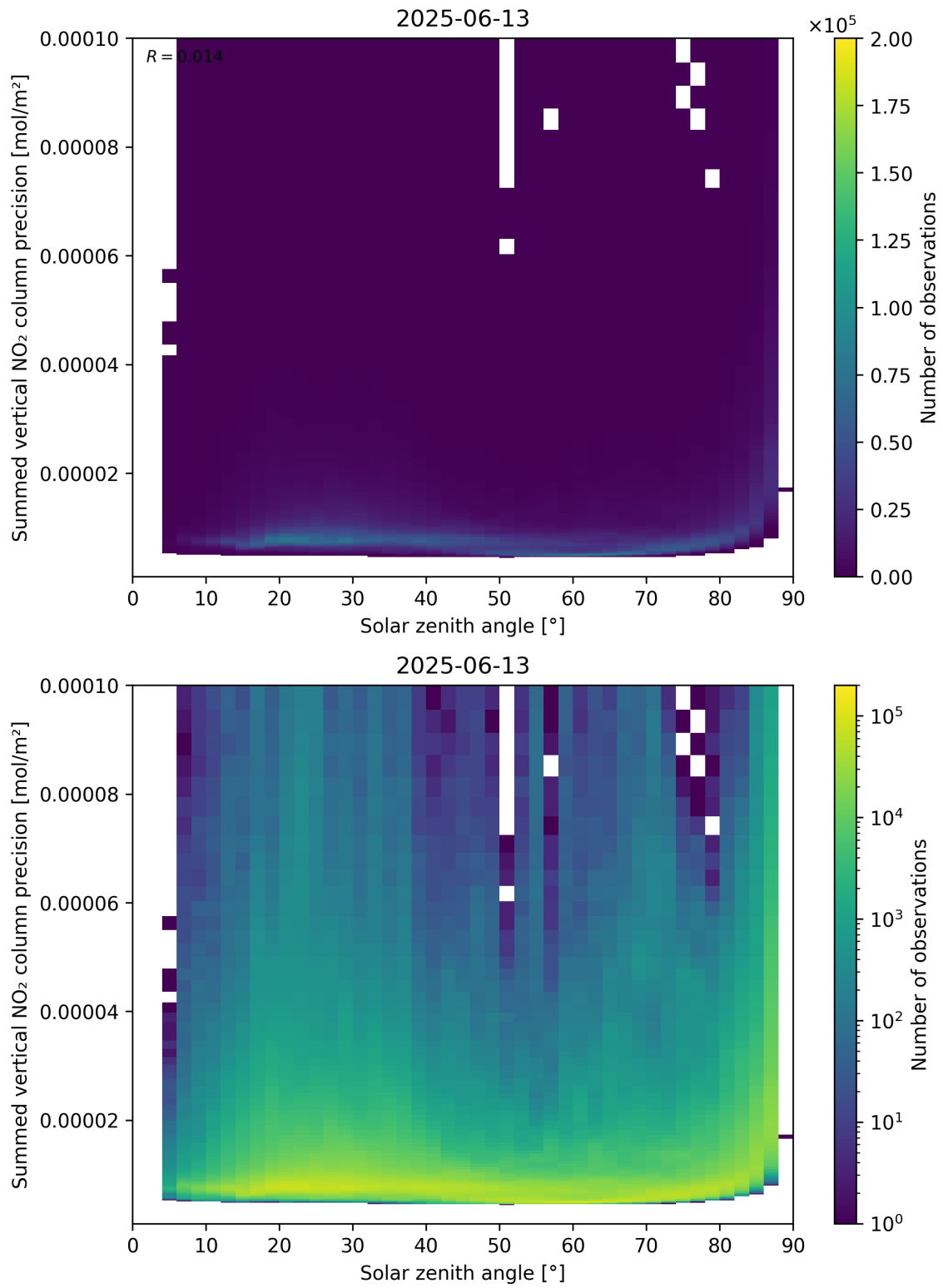
Figure 152: Scatter density plot of “Solar zenith angle” against “Summed vertical NO 2 column precision” for 2025-06-12 to 2025-06-14.
