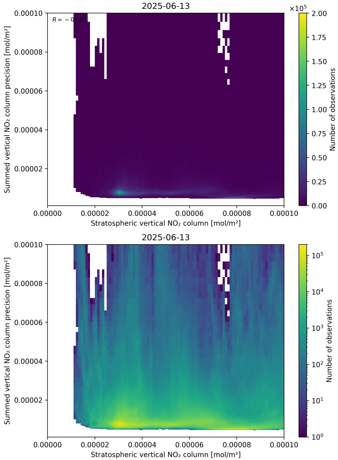
Figure 99: Scatter density plot of “Stratospheric vertical NO 2 column” against “Summed vertical NO 2 column precision” for 2025-06-12 to 2025-06-14.
