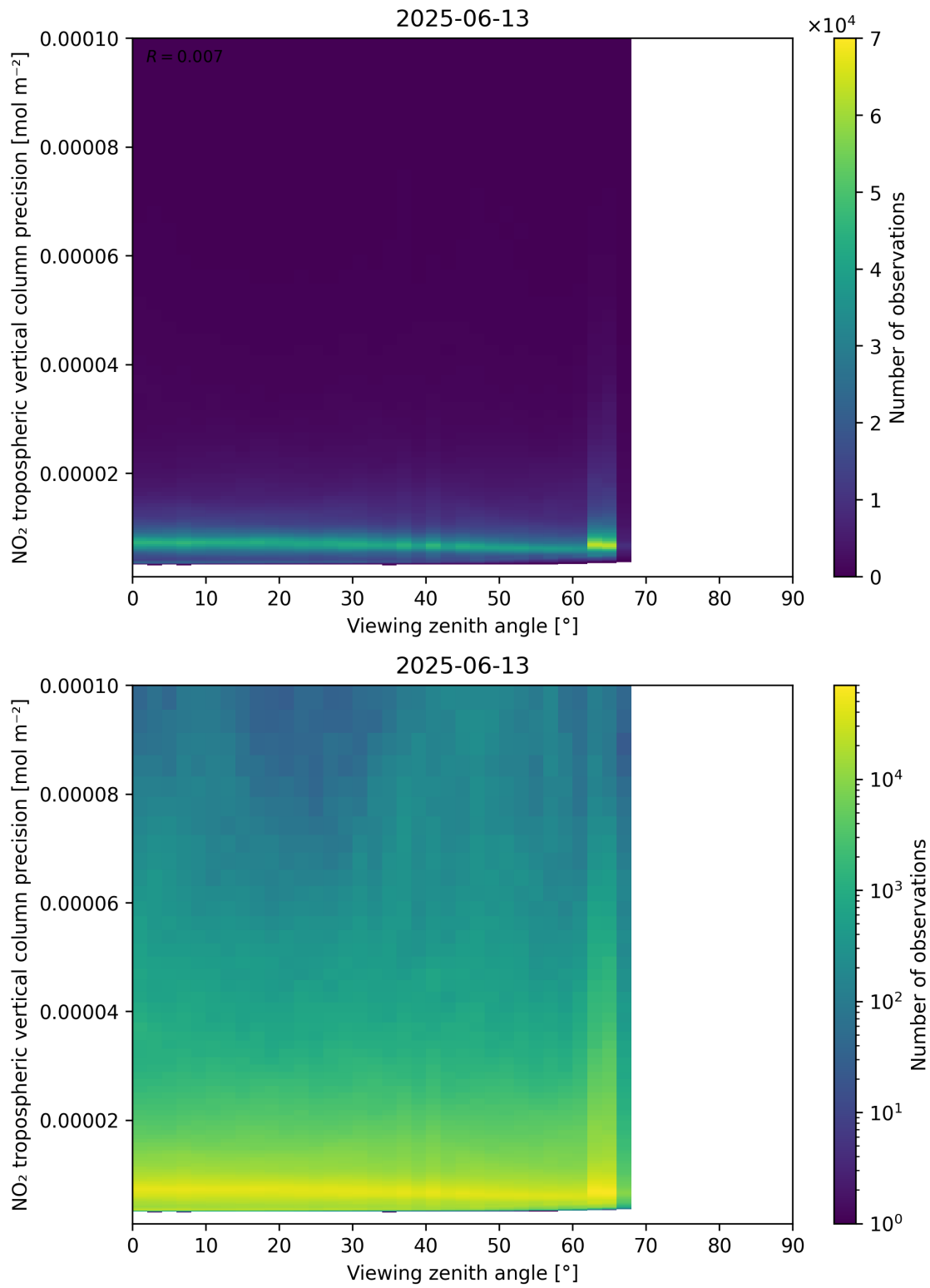
Figure 170: Scatter density plot of “Viewing zenith angle” against “NO 2 tropospheric vertical column precision” for 2025-06-12 to 2025-06-14.
