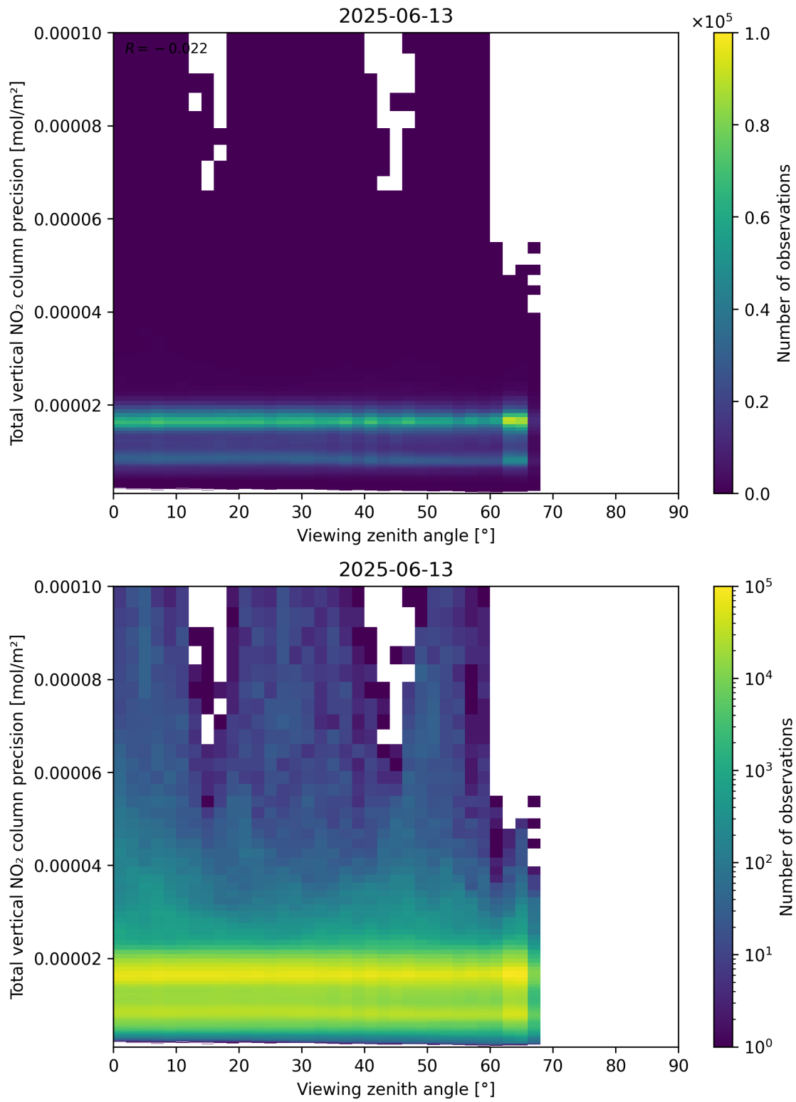
Figure 168: Scatter density plot of “Viewing zenith angle” against “Total vertical NO 2 column precision” for 2025-06-12 to 2025-06-14.
