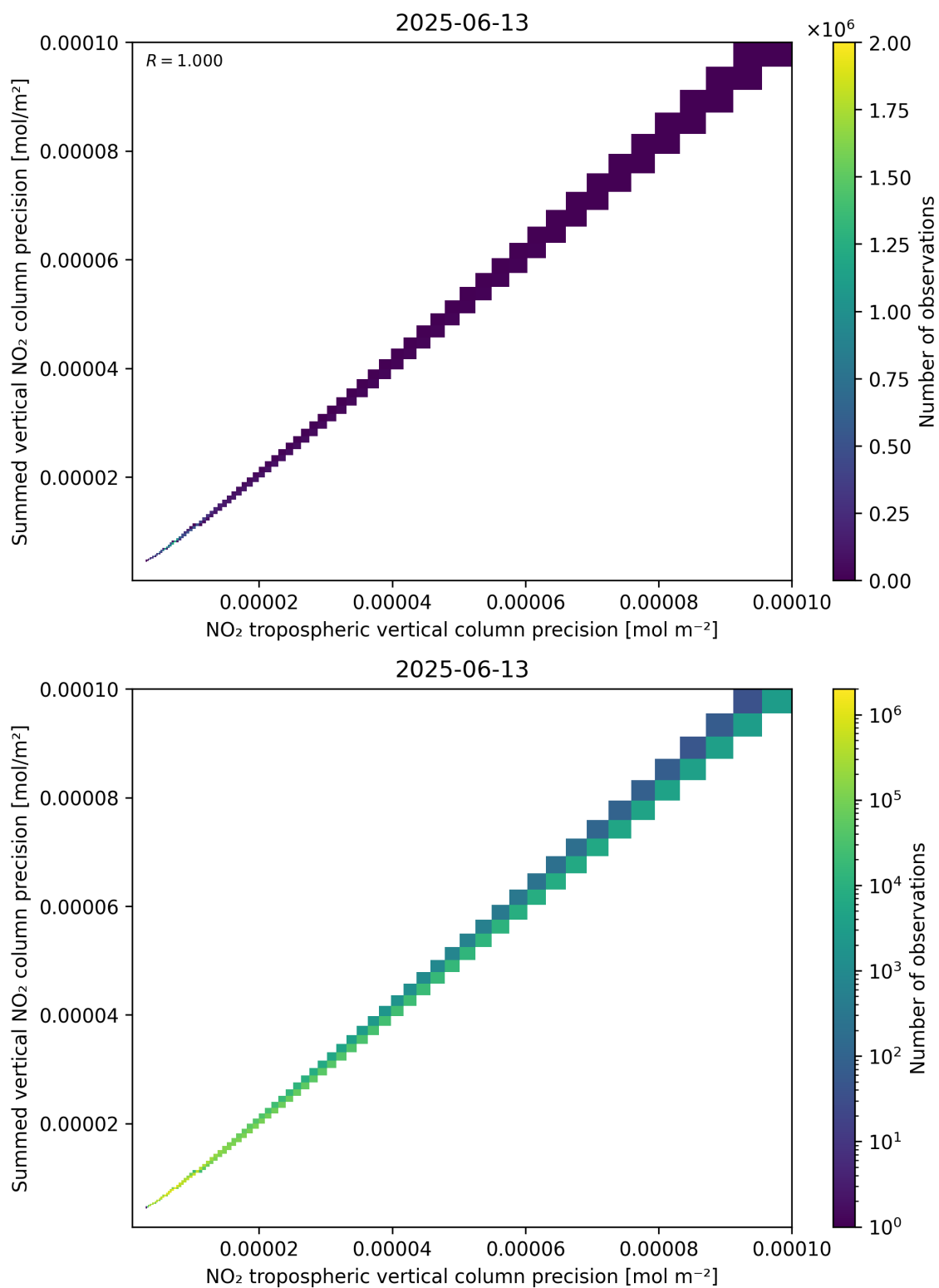
Figure 137: Scatter density plot of “NO 2 tropospheric vertical column precision” against “Summed vertical NO 2 column precision” for 2025-06-12 to 2025-06-14.
