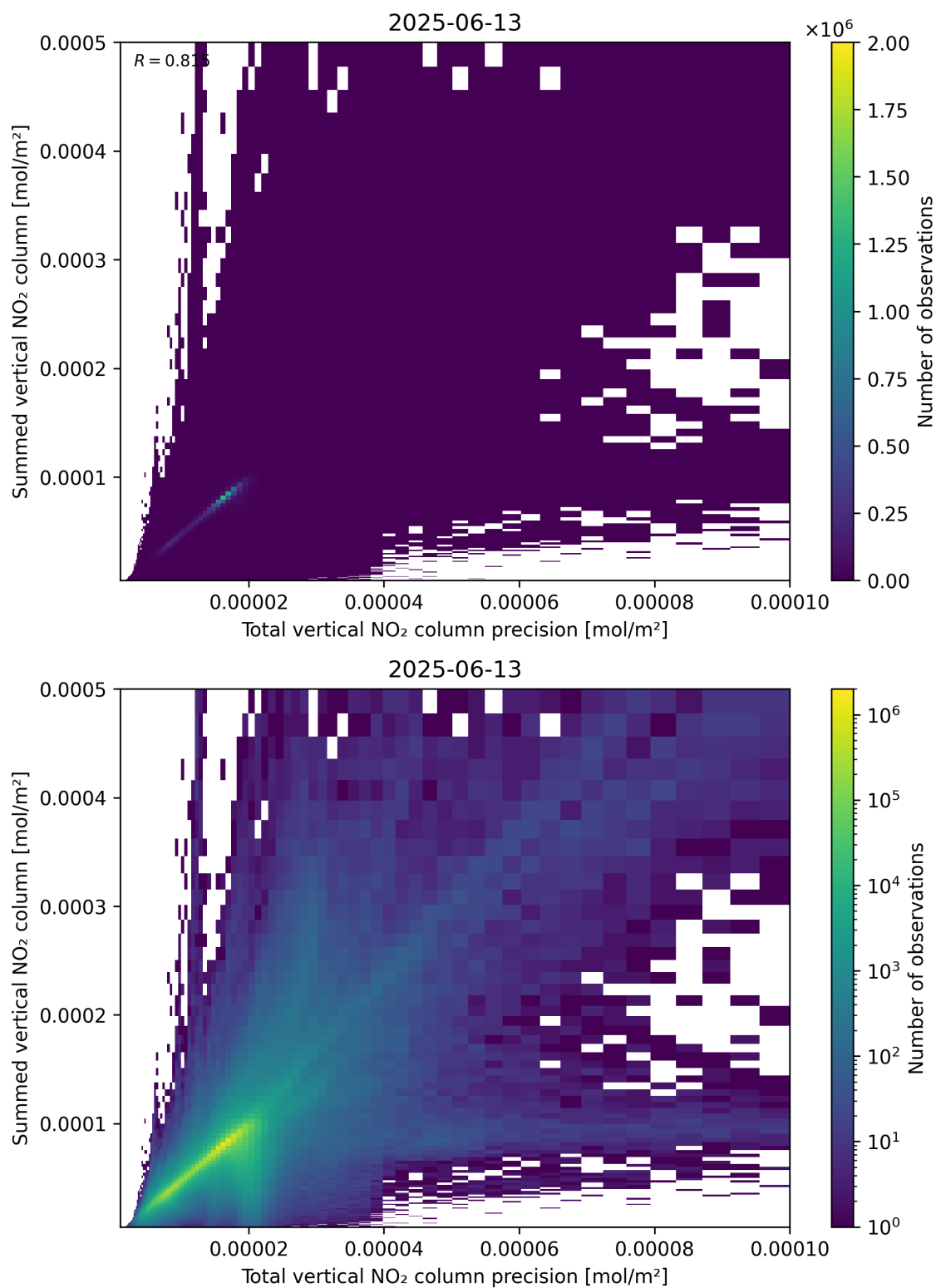
Figure 117: Scatter density plot of “Total vertical NO 2 column precision” against “Summed vertical NO 2 column” for 2025-06-12 to 2025-06-14.
