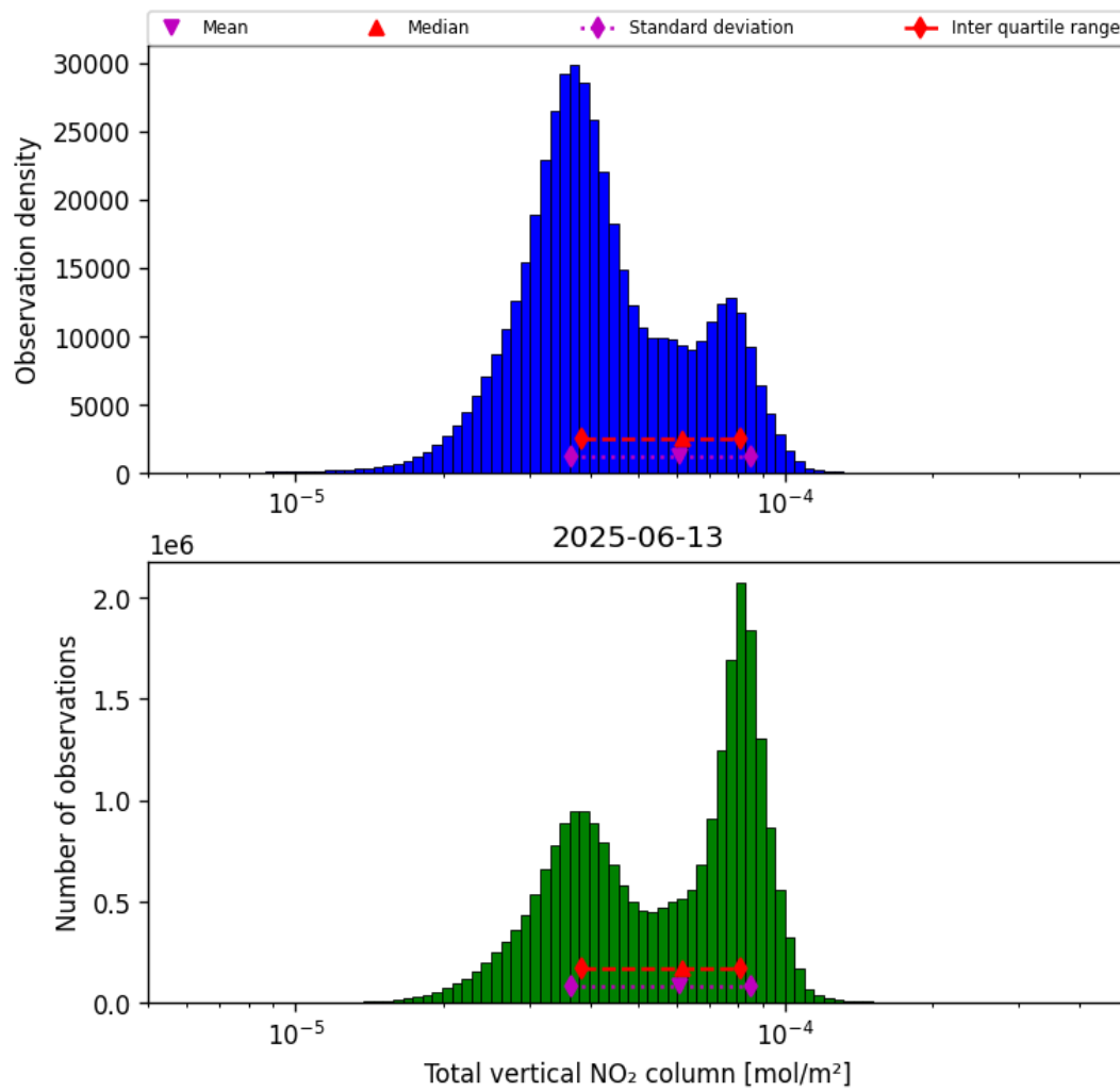
Figure 38: Histogram of “Total vertical NO 2 column” for 2025-06-12 to 2025-06-14
