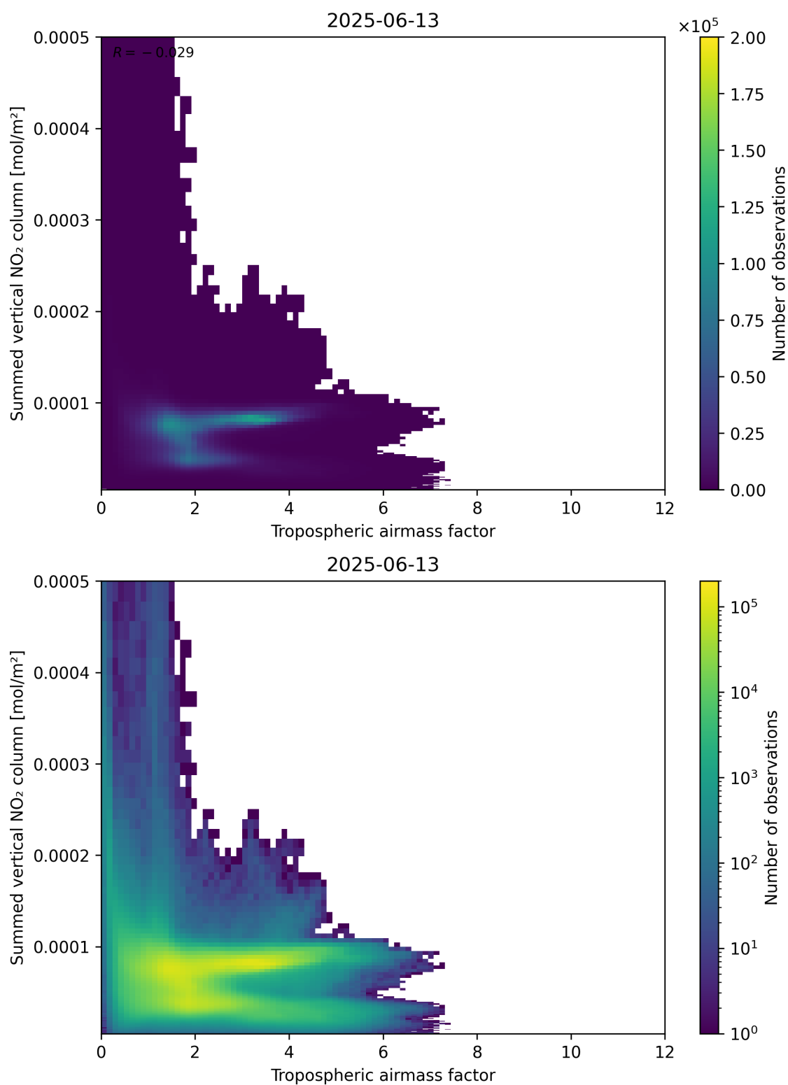
Figure 75: Scatter density plot of “Tropospheric air mass factor” against “Summed vertical NO 2 column” for 2025-06-12 to 2025-06-14.
