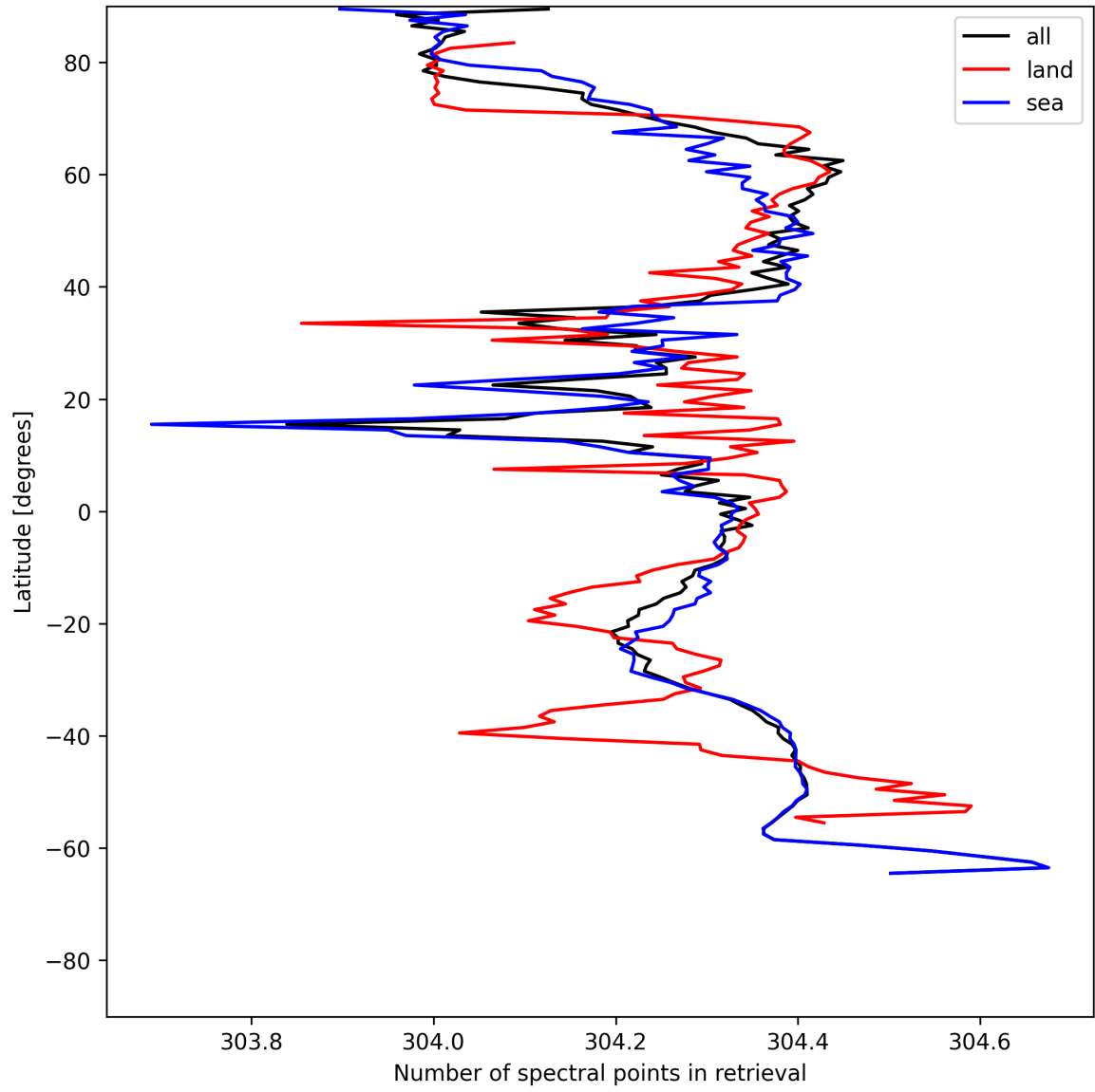
Figure 16: Zonal average of “Number of spectral points in retrieval” for 2025-06-12 to 2025-06-14.
