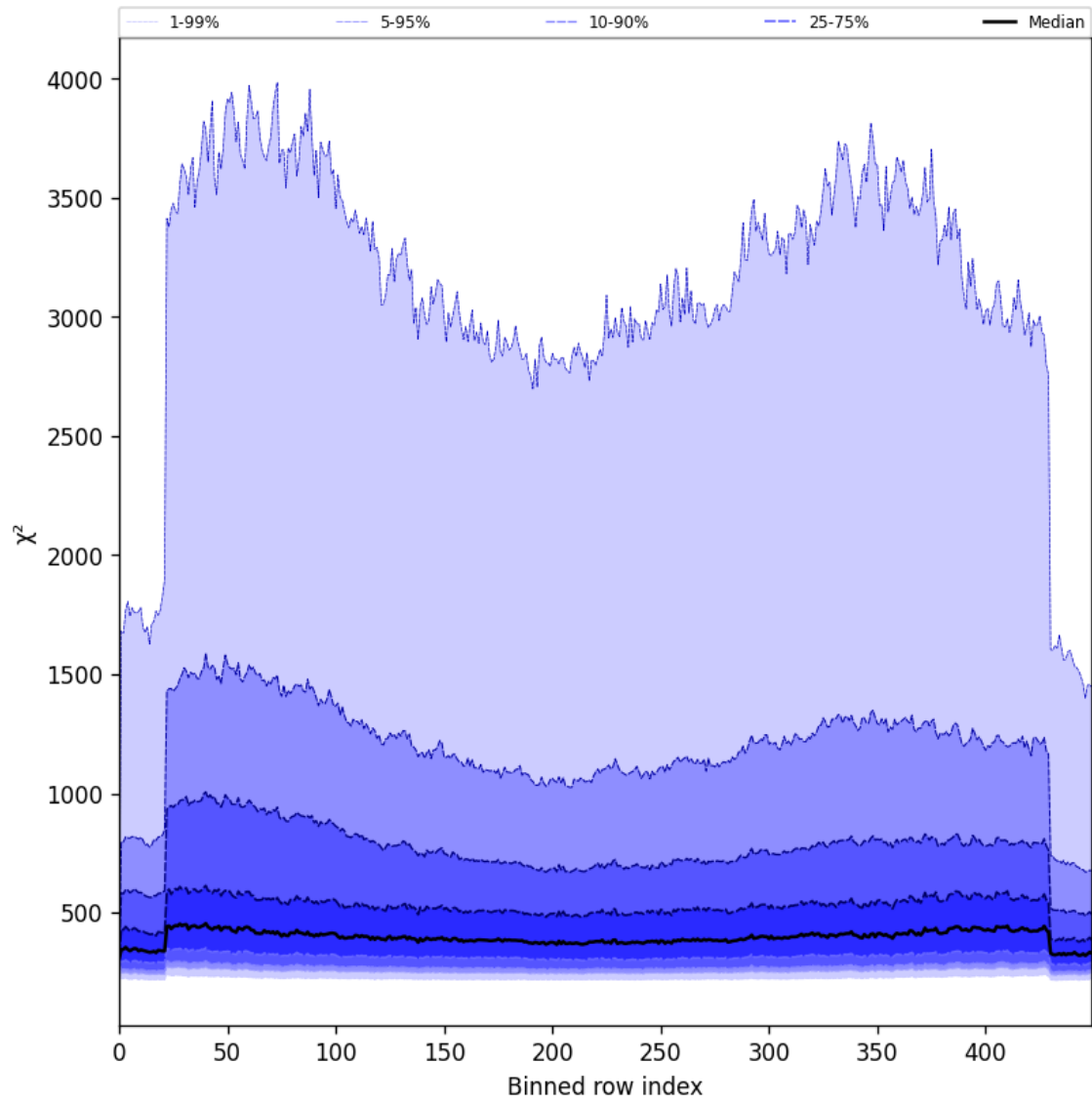
Figure 59: Along track statistics of “ \chi^2 ” for 2025-06-12 to 2025-06-14
