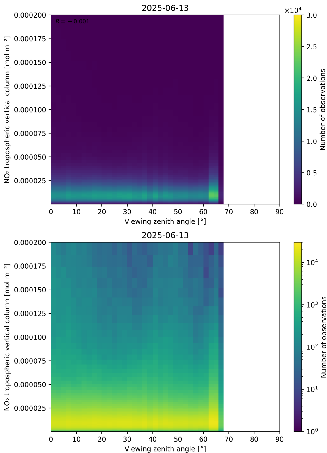
Figure 169: Scatter density plot of “Viewing zenith angle” against “NO 2 tropospheric vertical column” for 2025-06-12 to 2025-06-14.
