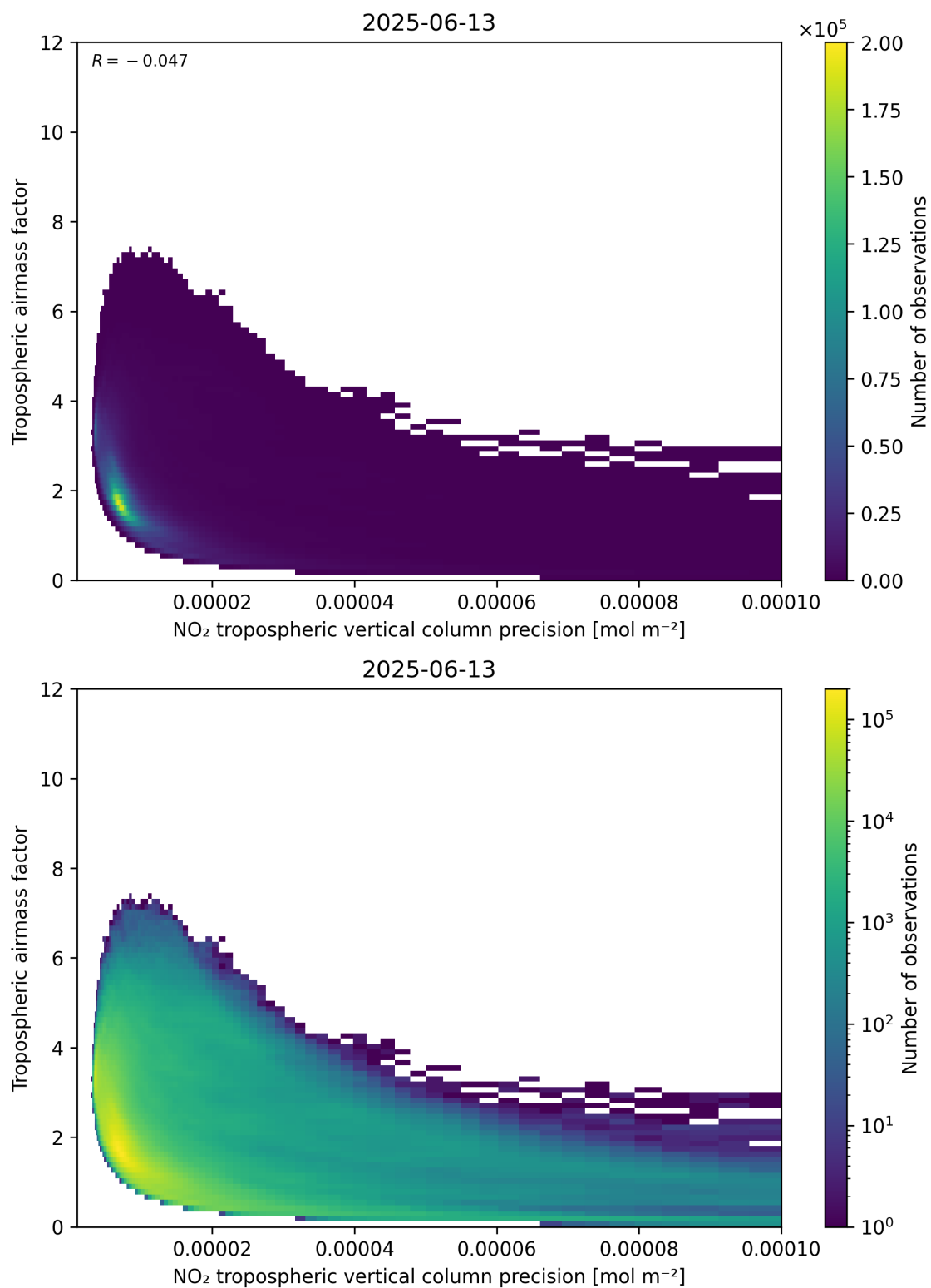
Figure 133: Scatter density plot of “NO 2 tropospheric vertical column precision” against “Tropospheric air mass factor” for 2025-06-12 to 2025-06-14.
