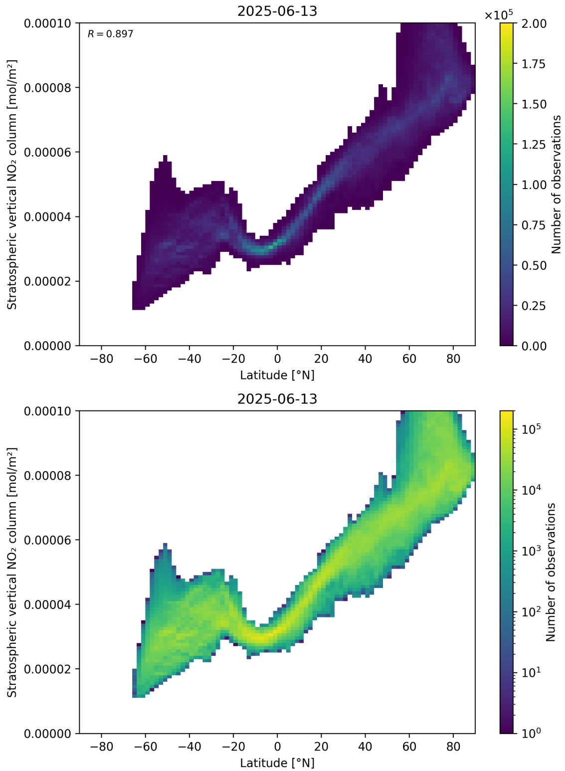
Figure 87: Scatter density plot of “Latitude” against “Stratospheric vertical NO 2 column” for 2025-06-12 to 2025-06-14.
