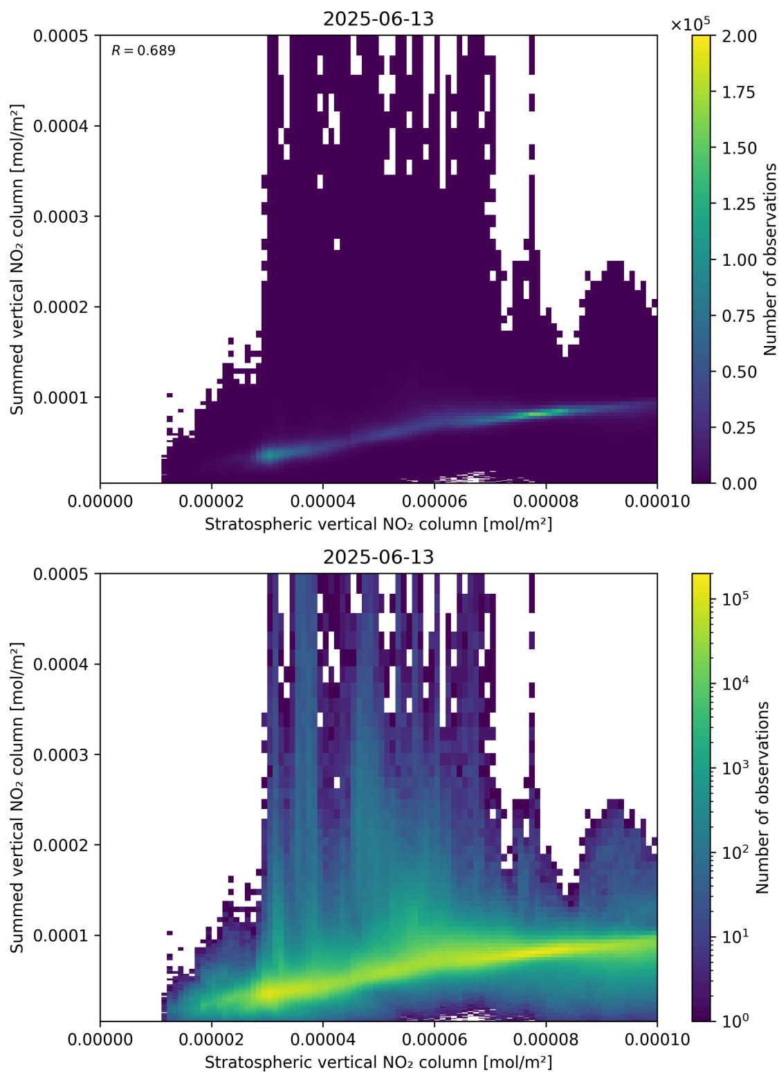
Figure 98: Scatter density plot of “Stratospheric vertical NO 2 column” against “Summed vertical NO 2 column” for 2025-06-12 to 2025-06-14.
