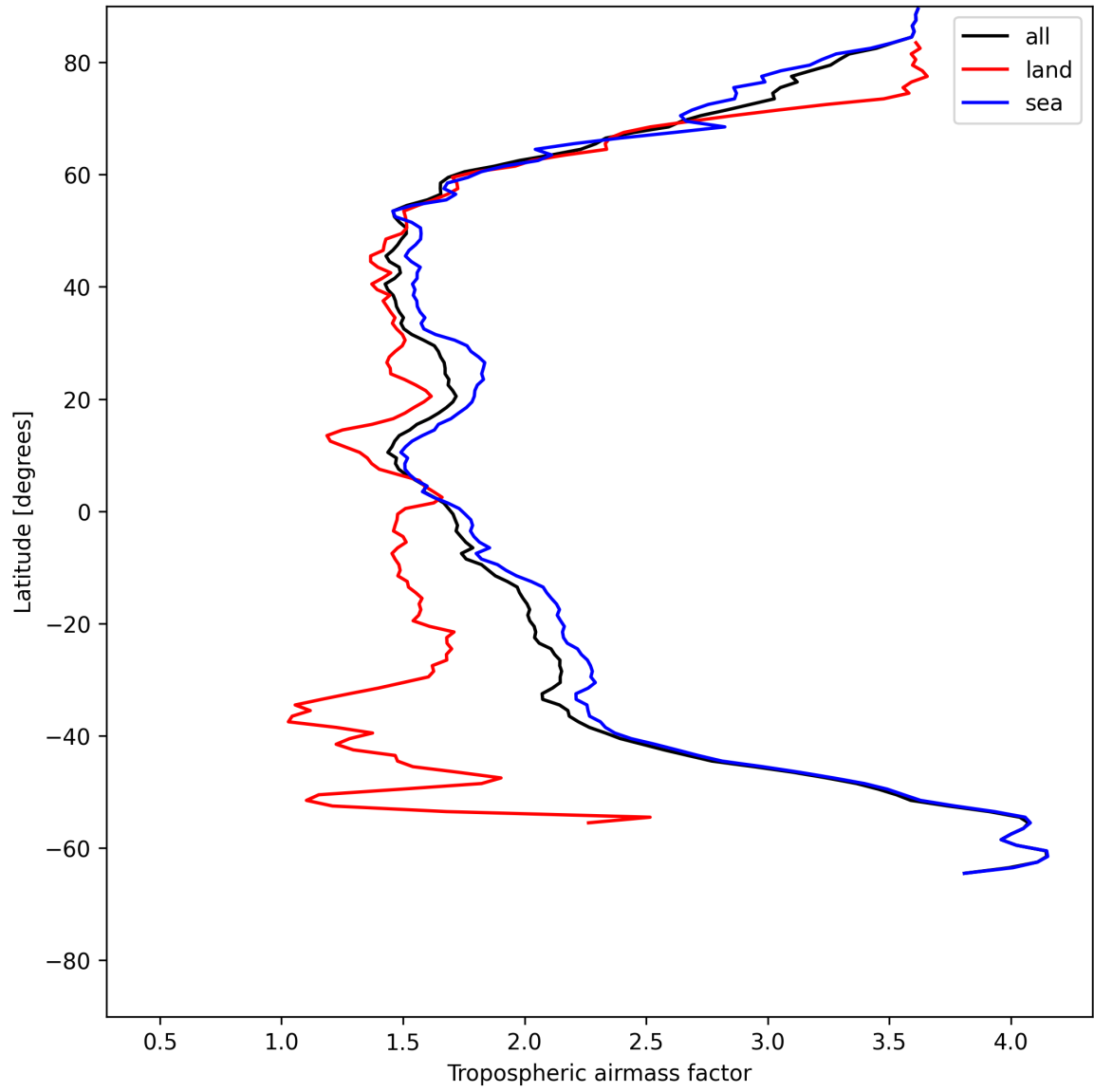
Figure 14: Zonal average of “Tropospheric airmass factor” for 2025-06-12 to 2025-06-14.
