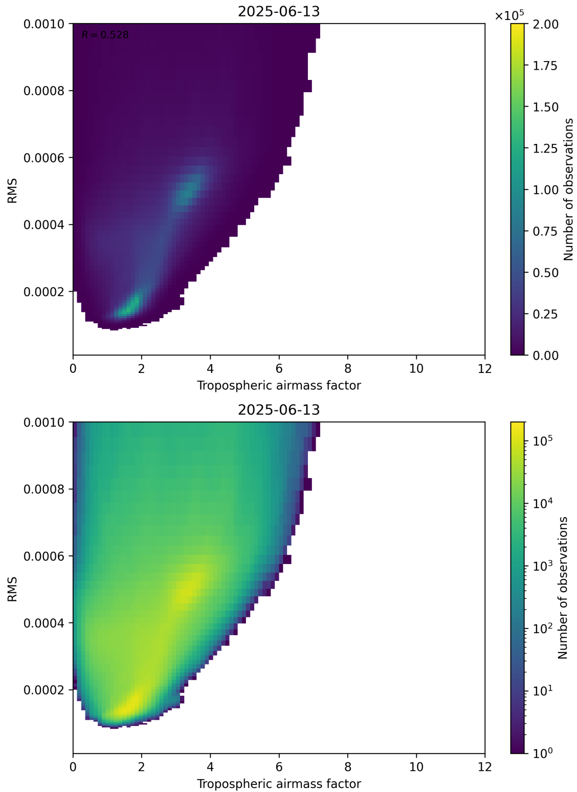
Figure 79: Scatter density plot of “Tropospheric airmass factor” against “RMS” for 2025-06-12 to 2025-06-14.
