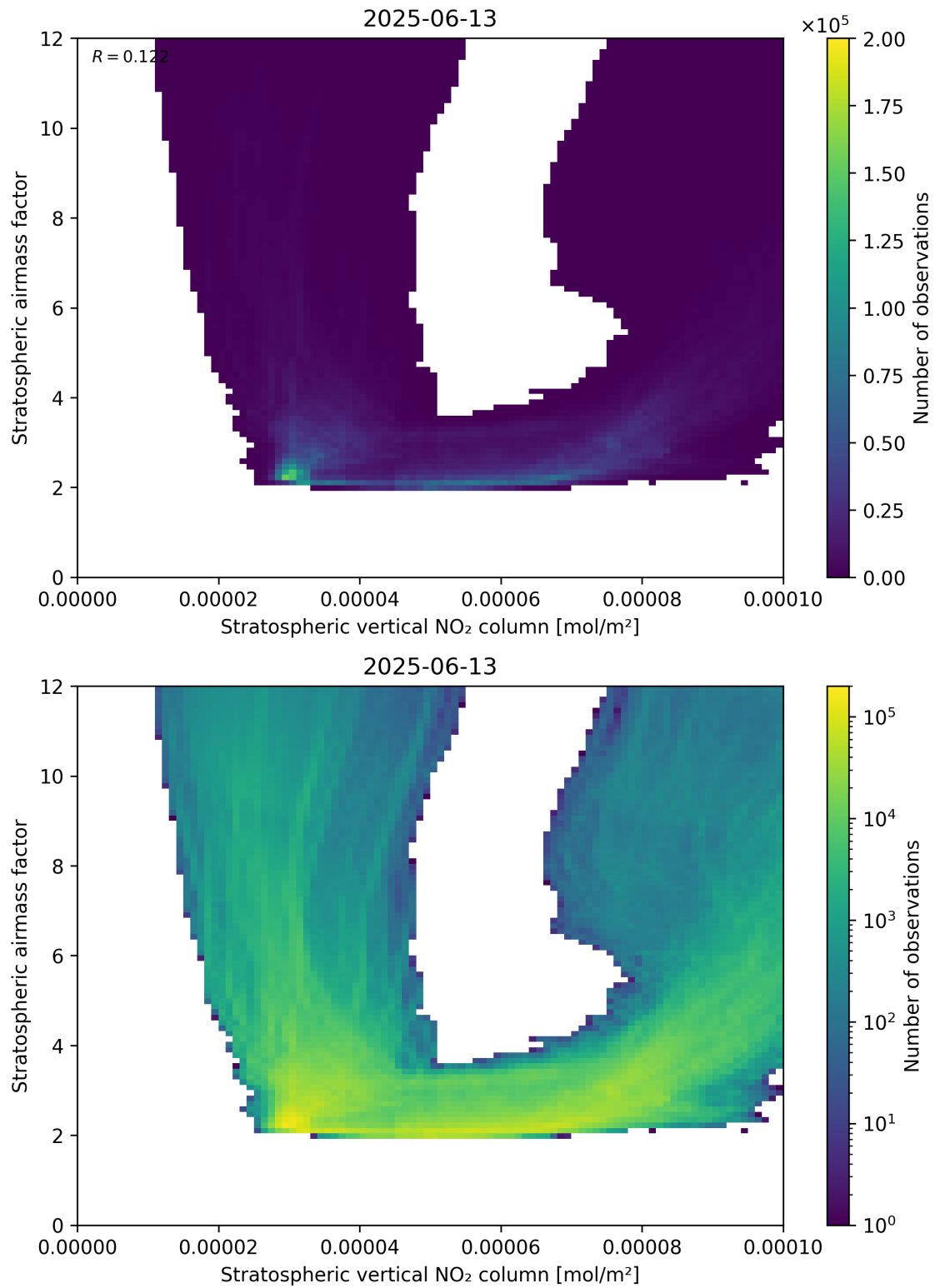
Figure 96: Scatter density plot of “Stratospheric vertical NO 2 column” against “Stratospheric airmass factor” for 2025-06-12 to 2025-06-14.
