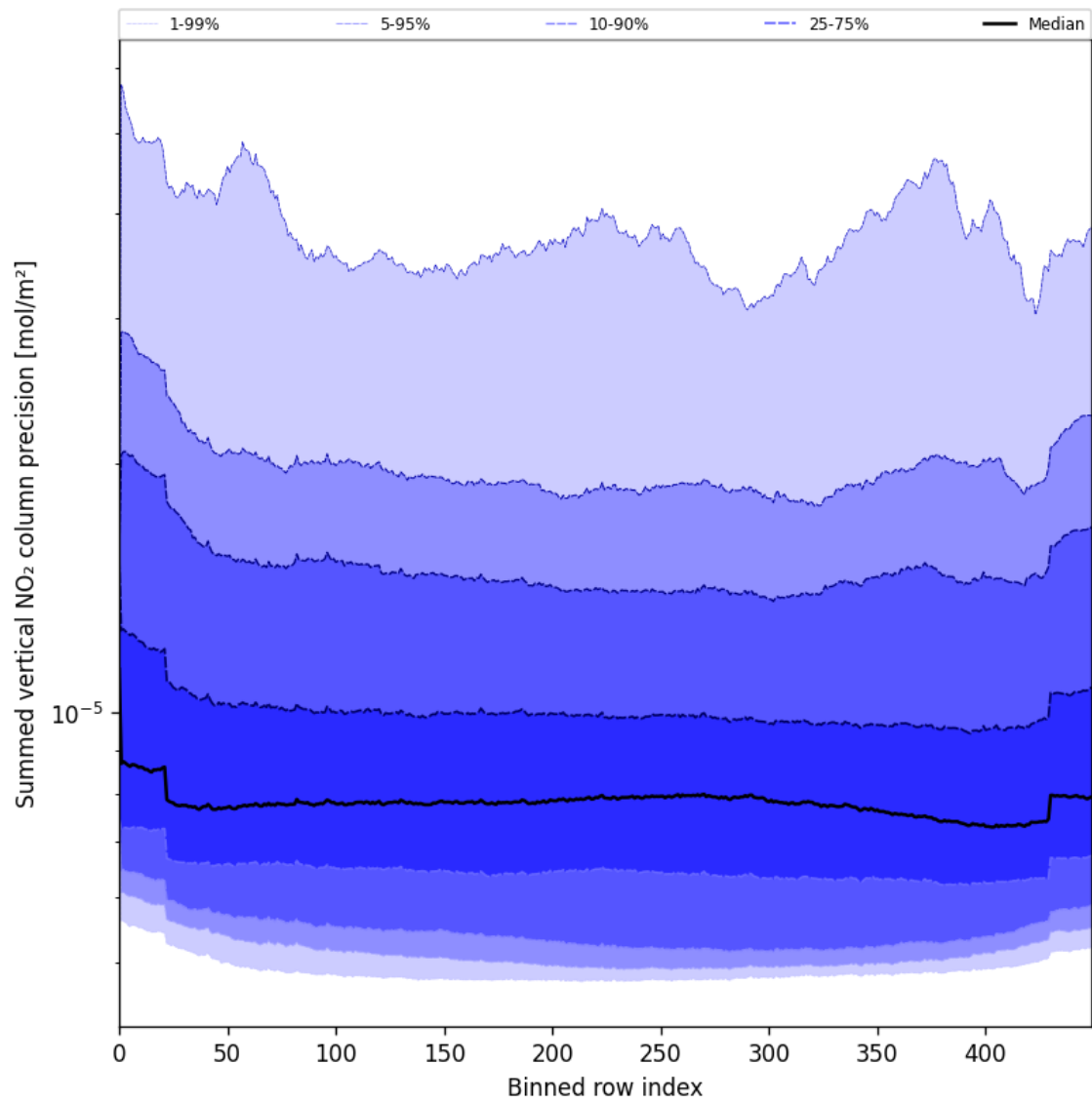
Figure 58: Along track statistics of “Summed vertical NO 2 column precision” for 2025-06-12 to 2025-06-14
