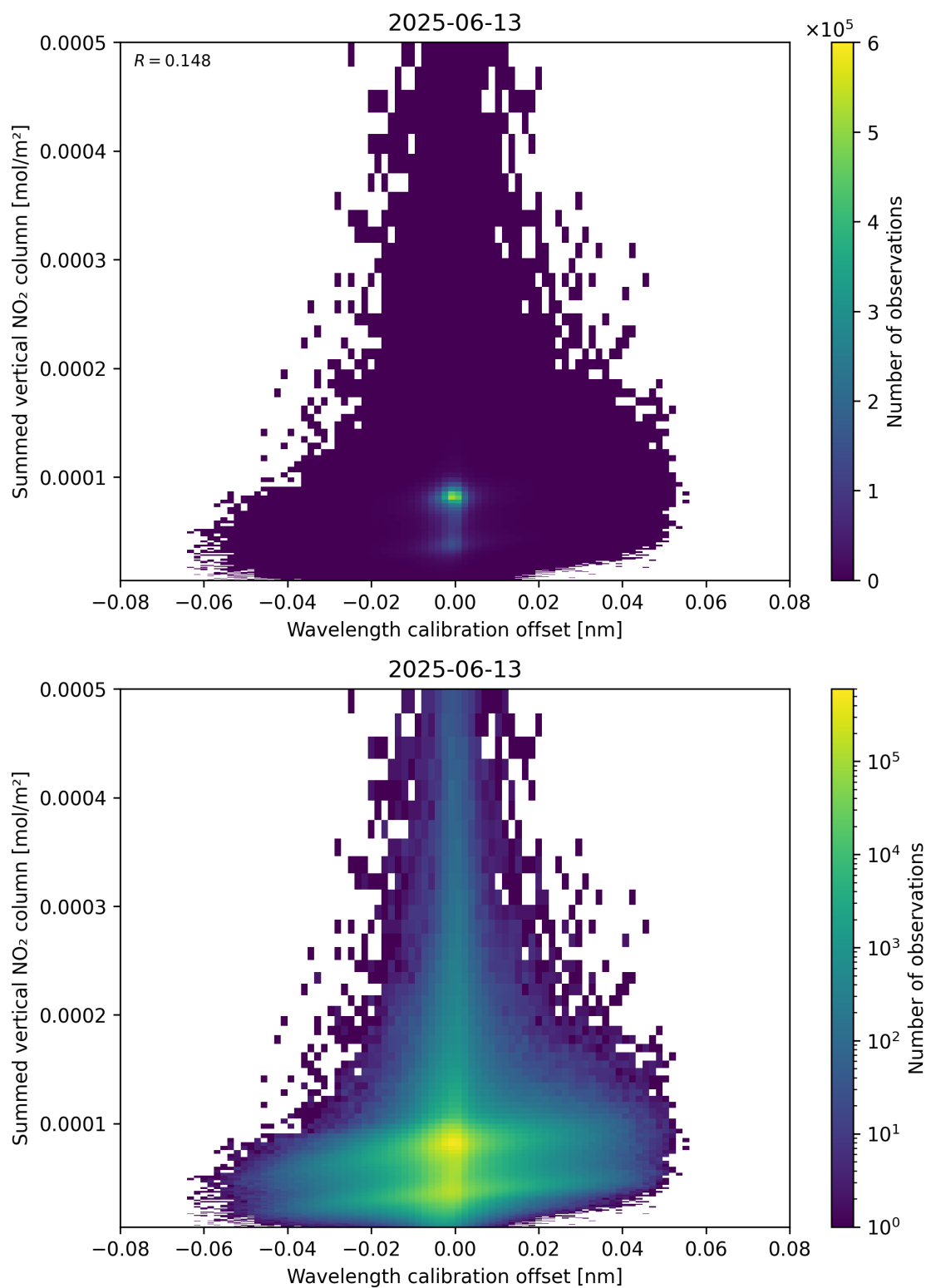
Figure 177: Scatter density plot of “Wavelength calibration offset” against “Summed vertical NO 2 column” for 2025-06-12 to 2025-06-14.
