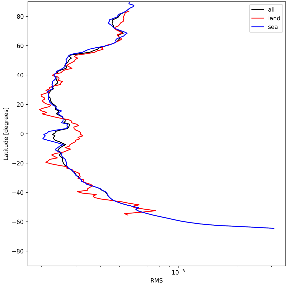
Figure 26: Zonal average of “RMS” for 2025-06-12 to 2025-06-14.
