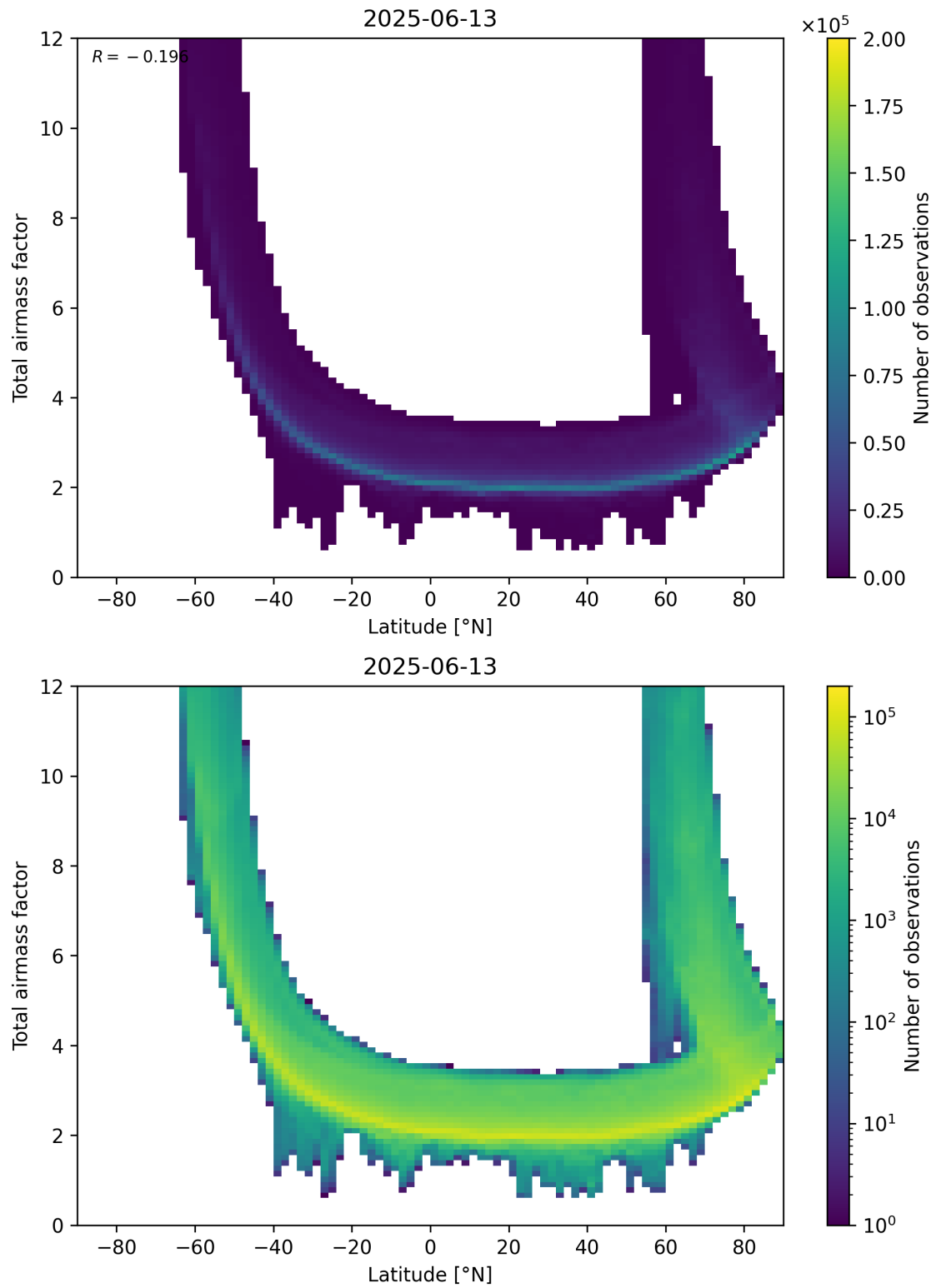
Figure 84: Scatter density plot of “Latitude” against “Total airmass factor” for 2025-06-12 to 2025-06-14.
