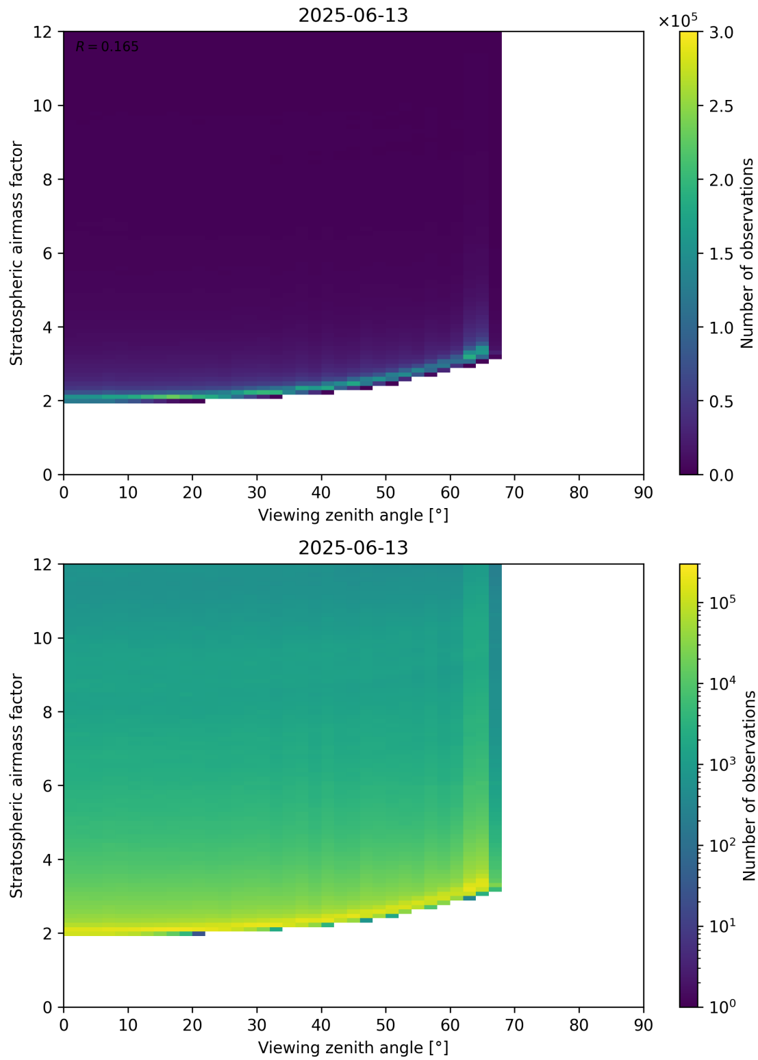
Figure 159: Scatter density plot of “Viewing zenith angle” against “Stratospheric airmass factor” for 2025-06-12 to 2025-06-14.
