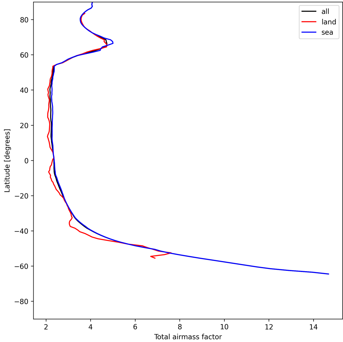
Figure 15: Zonal average of “Total airmass factor” for 2025-06-12 to 2025-06-14.
