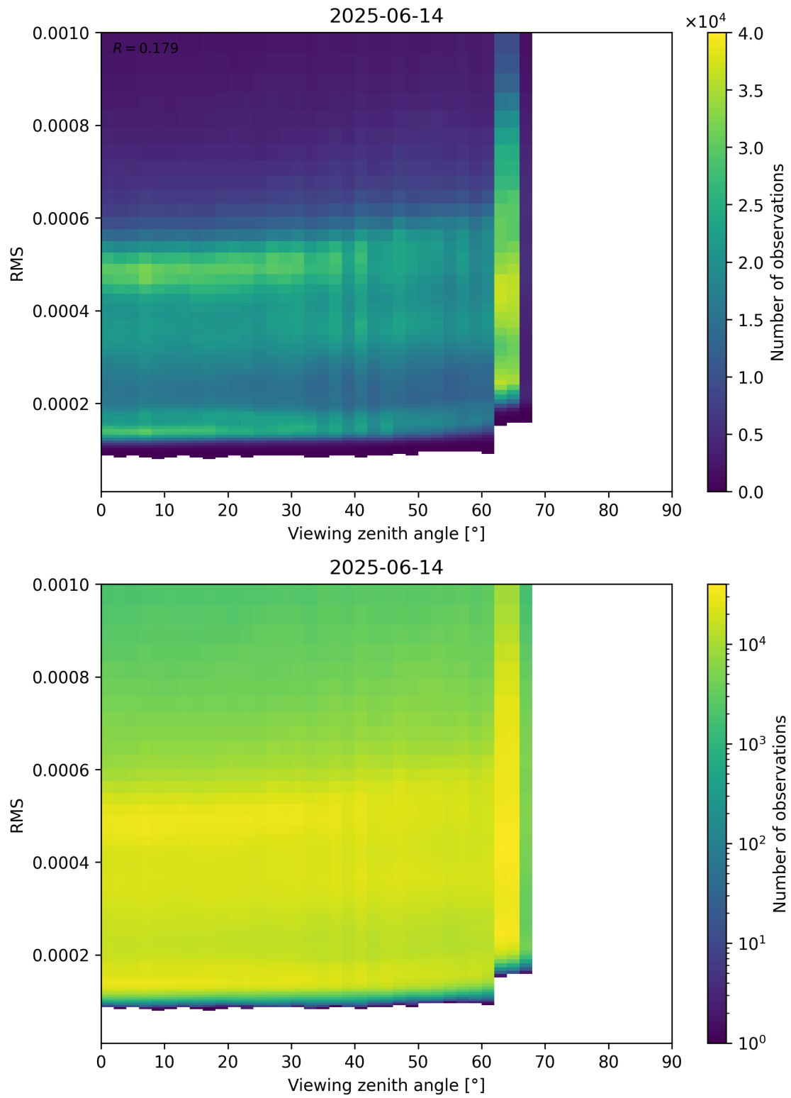
Figure 171: Scatter density plot of “Viewing zenith angle” against “RMS” for 2025-06-13 to 2025-06-15.
