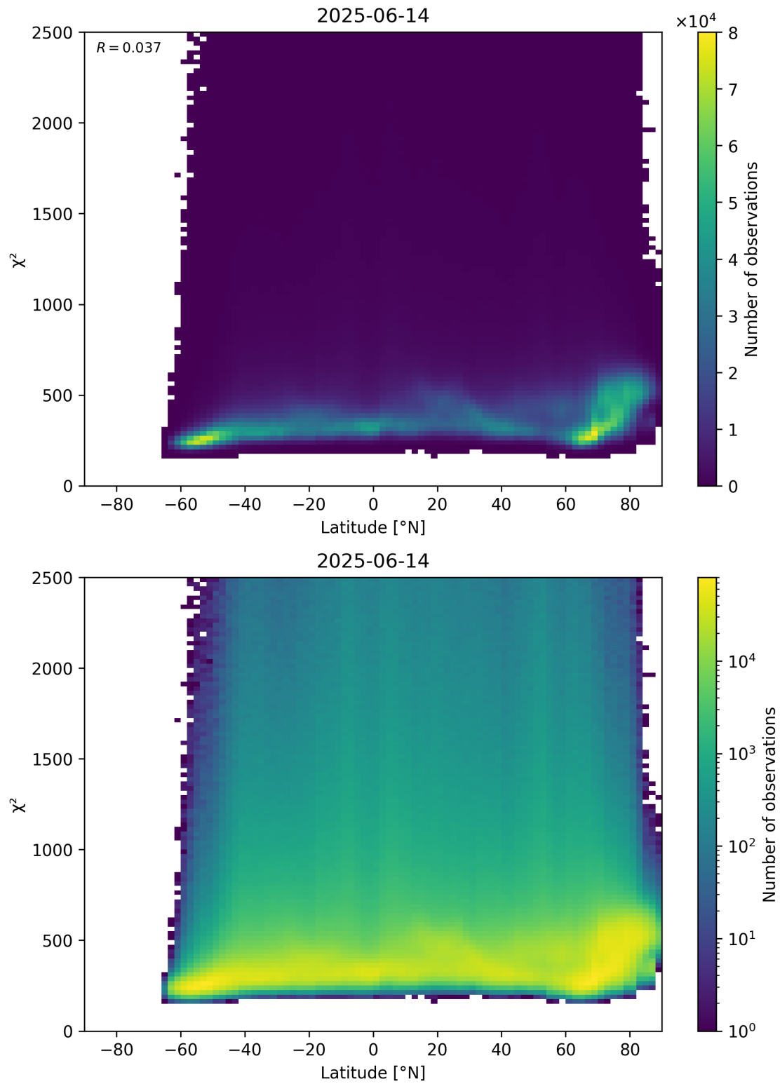
Figure 86: Scatter density plot of “Latitude” against “ \chi^2 ” for 2025-06-13 to 2025-06-15.
