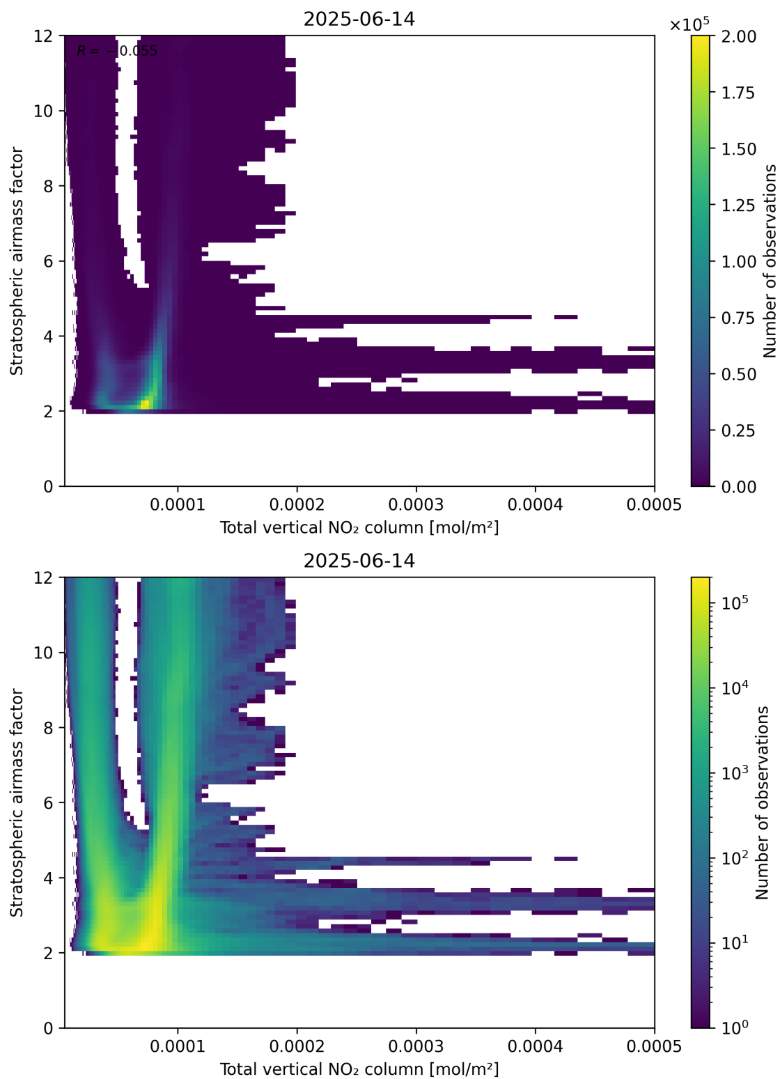
Figure 110: Scatter density plot of “Total vertical NO 2 column” against “Stratospheric airmass factor” for 2025-06-13 to 2025-06-15.
