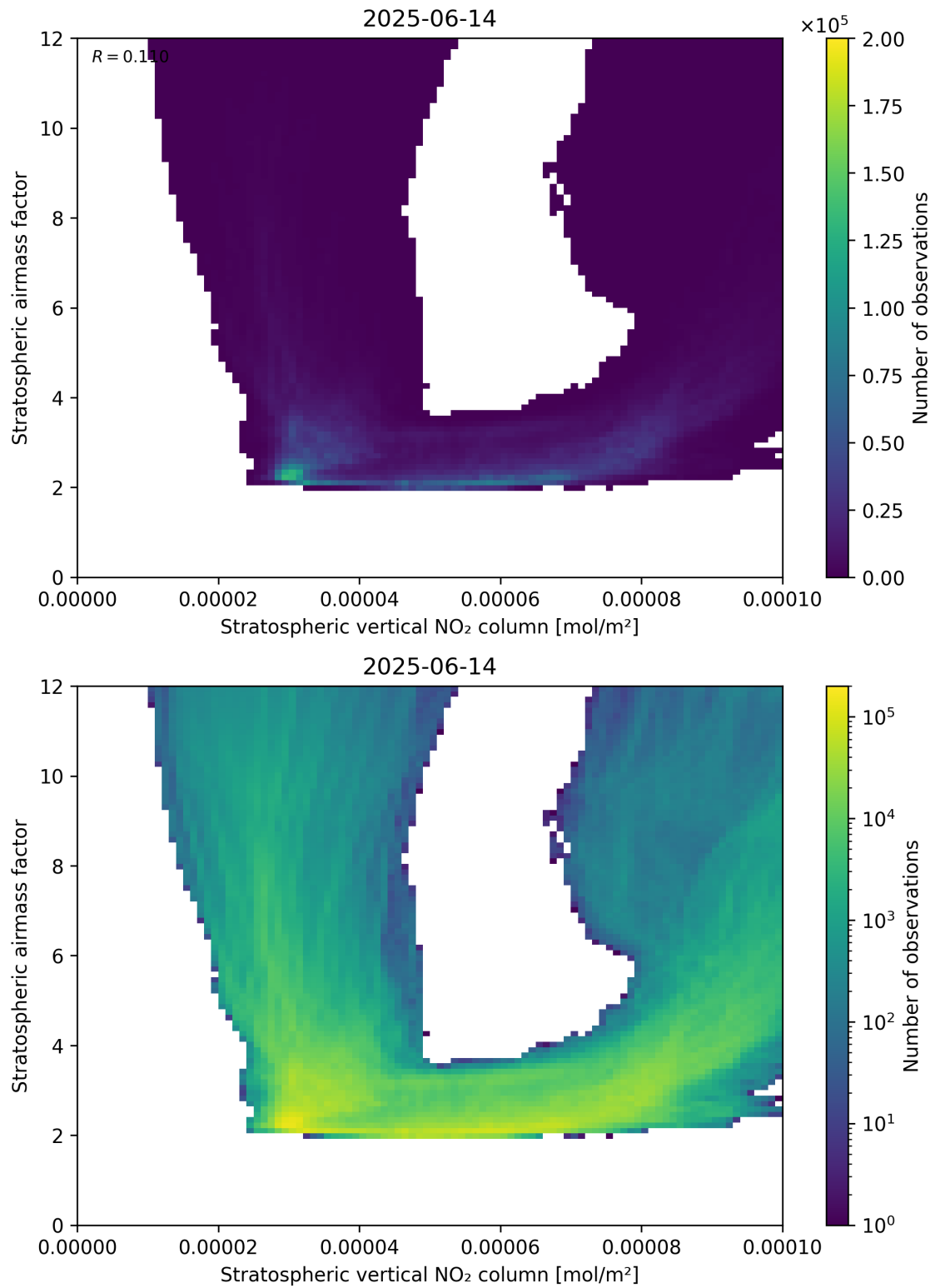
Figure 96: Scatter density plot of “Stratospheric vertical NO 2 column” against “Stratospheric airmass factor” for 2025-06-13 to 2025-06-15.
