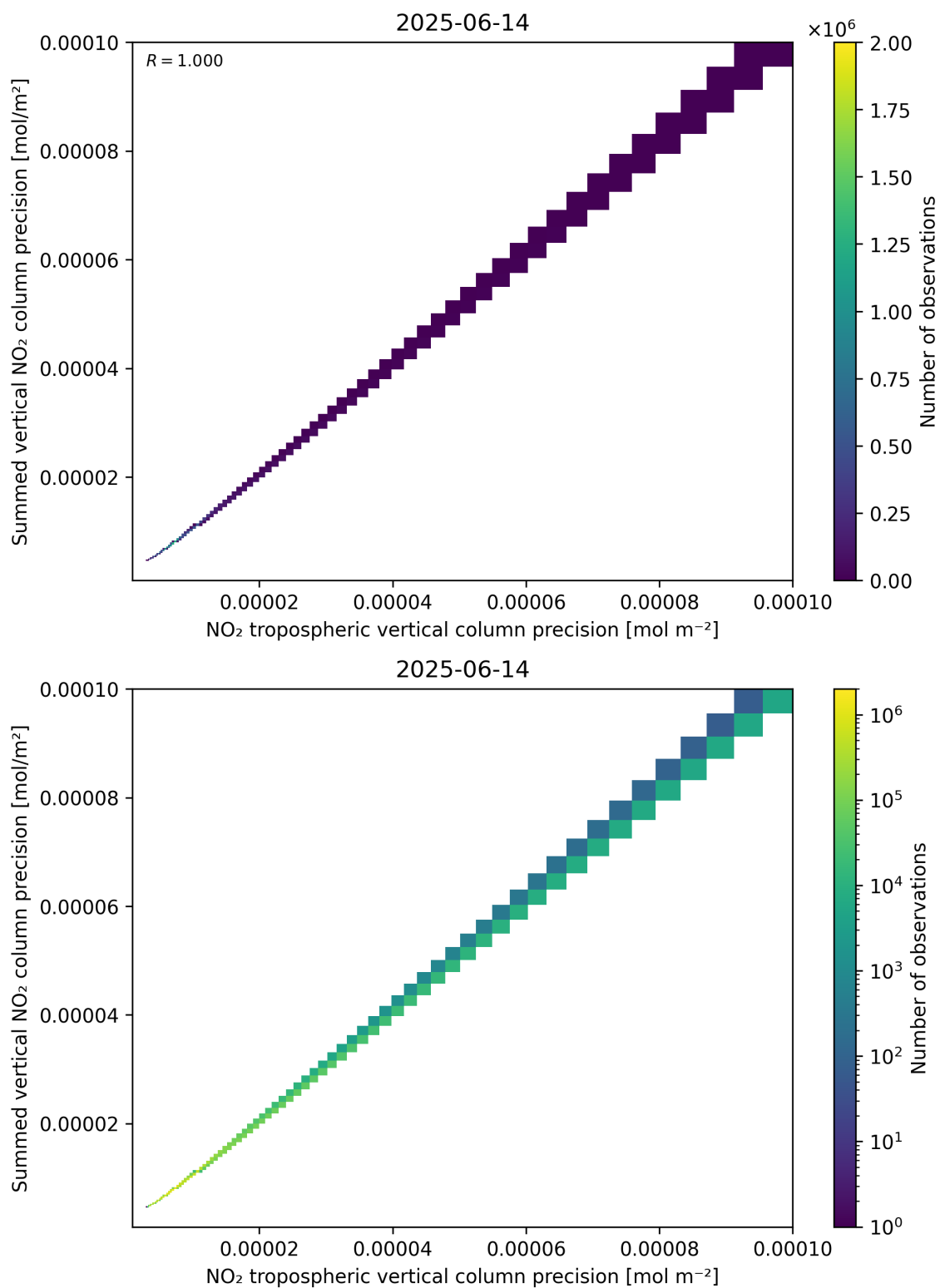
Figure 137: Scatter density plot of “NO 2 tropospheric vertical column precision” against “Summed vertical NO 2 column precision” for 2025-06-13 to 2025-06-15.
