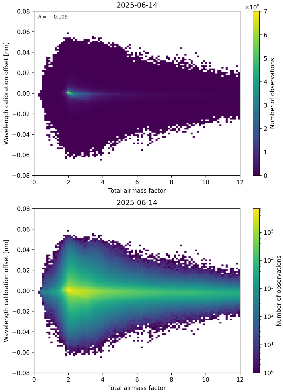
Figure 70: Scatter density plot of “Total airmass factor” against “Wavelength calibration offset” for 2025-06-13 to 2025-06-15.
