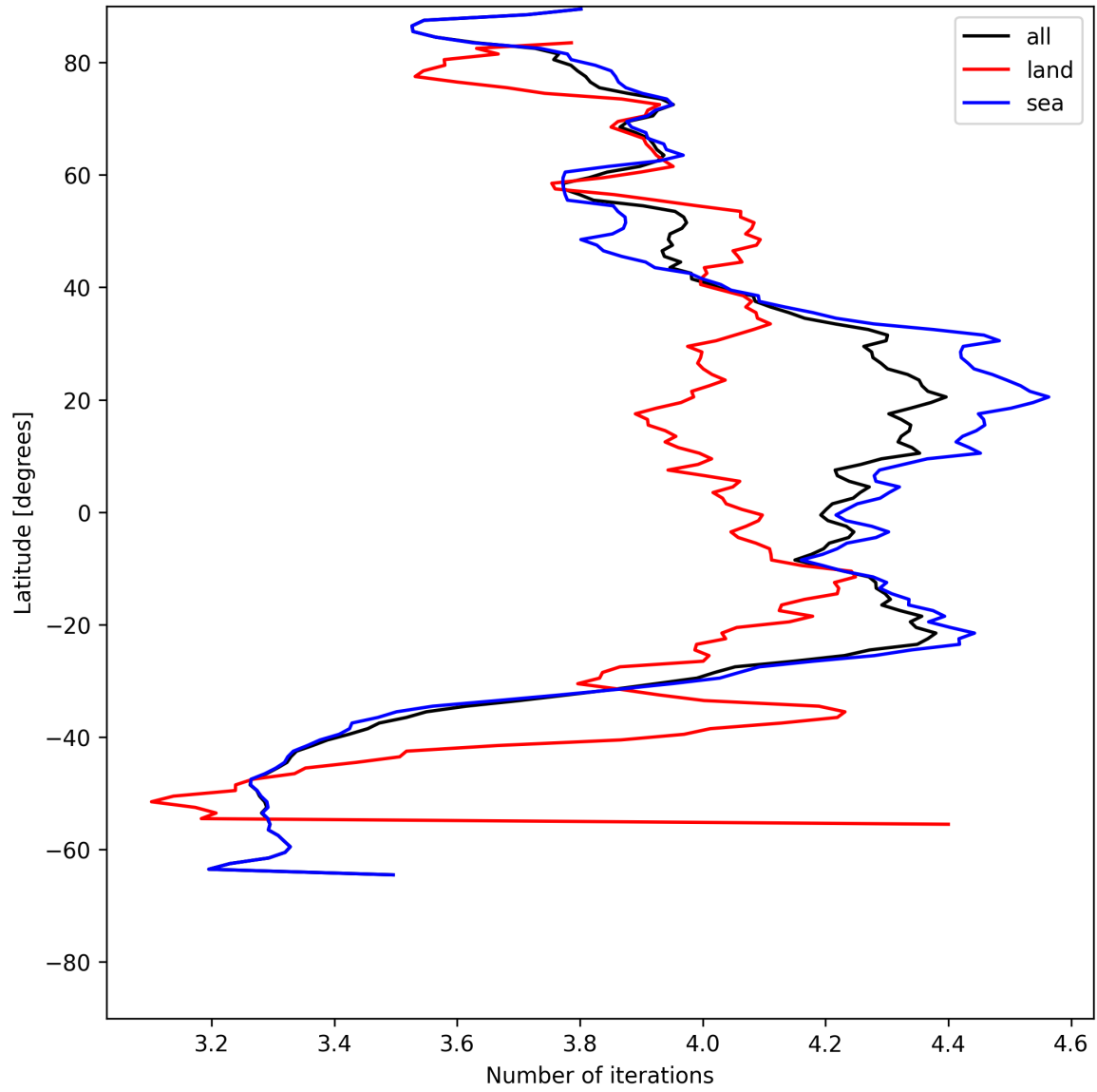
Figure 17: Zonal average of “Number of iterations” for 2025-06-13 to 2025-06-15.
