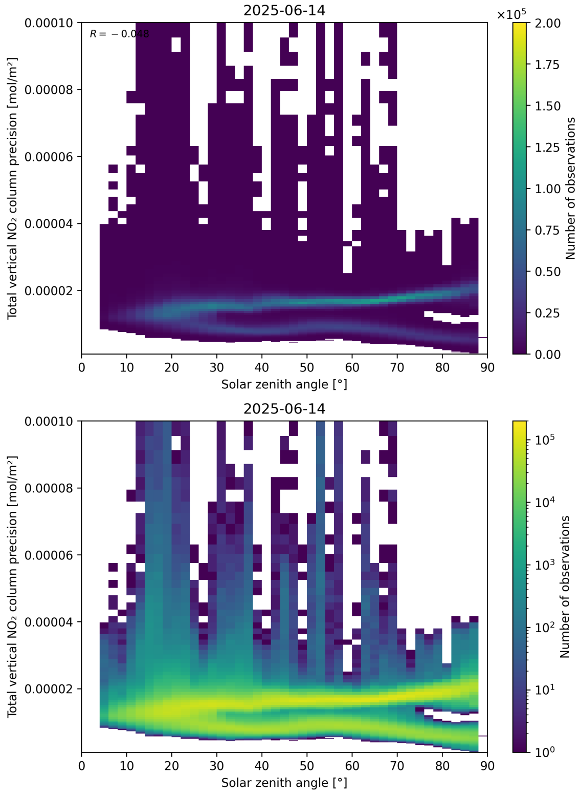
Figure 154: Scatter density plot of “Solar zenith angle” against “Total vertical NO 2 column precision” for 2025-06-13 to 2025-06-15.
