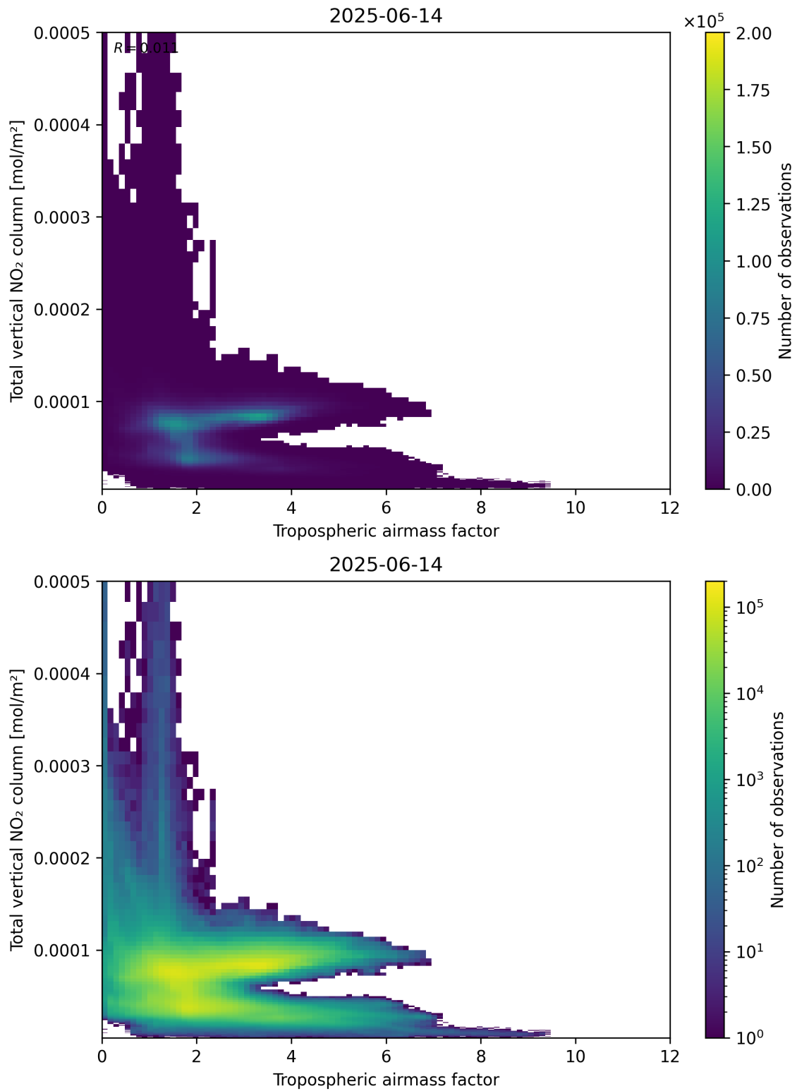
Figure 77: Scatter density plot of “Tropospheric airmass factor” against “Total vertical \text{NO}_2 column” for 2025-06-13 to 2025-06-15.
