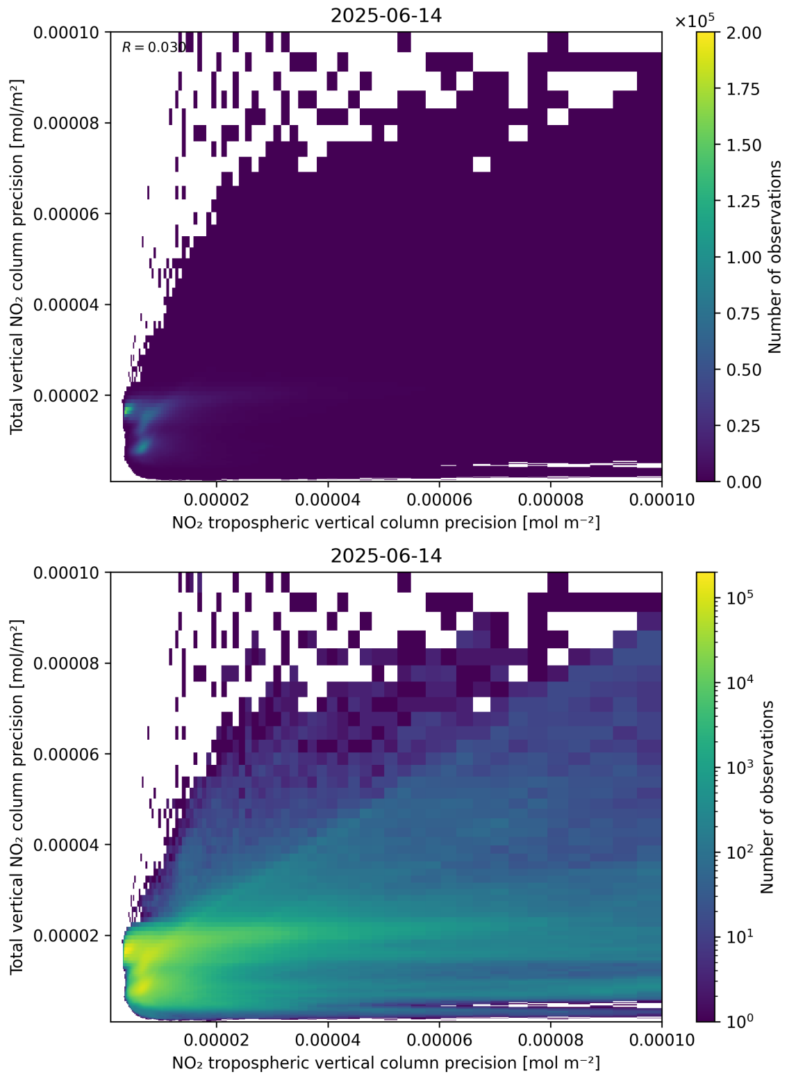
Figure 139: Scatter density plot of “NO 2 tropospheric vertical column precision” against “Total vertical NO 2 column precision” for 2025-06-13 to 2025-06-15.
