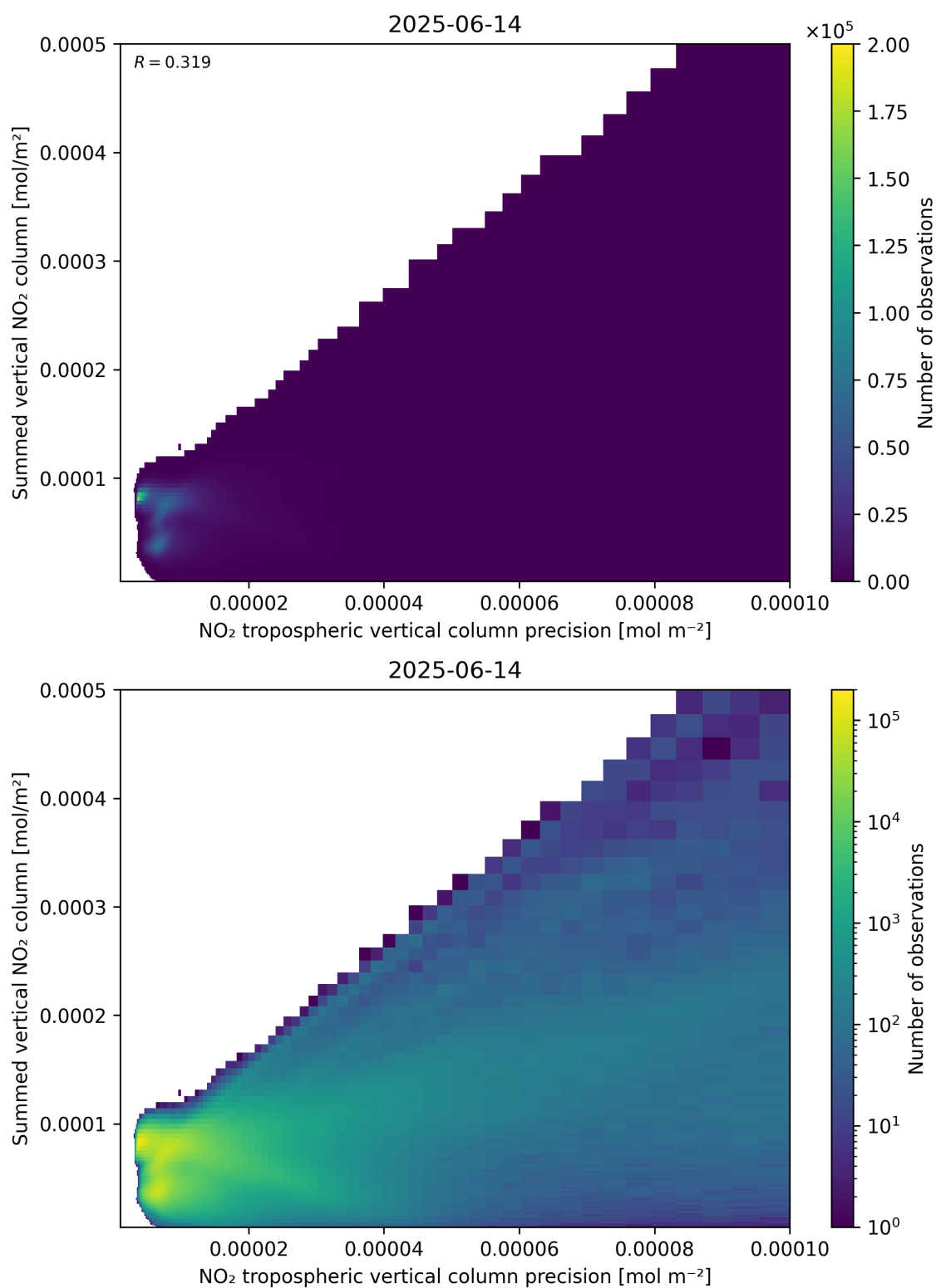
Figure 136: Scatter density plot of “NO 2 tropospheric vertical column precision” against “Summed vertical NO 2 column” for 2025-06-13 to 2025-06-15.
