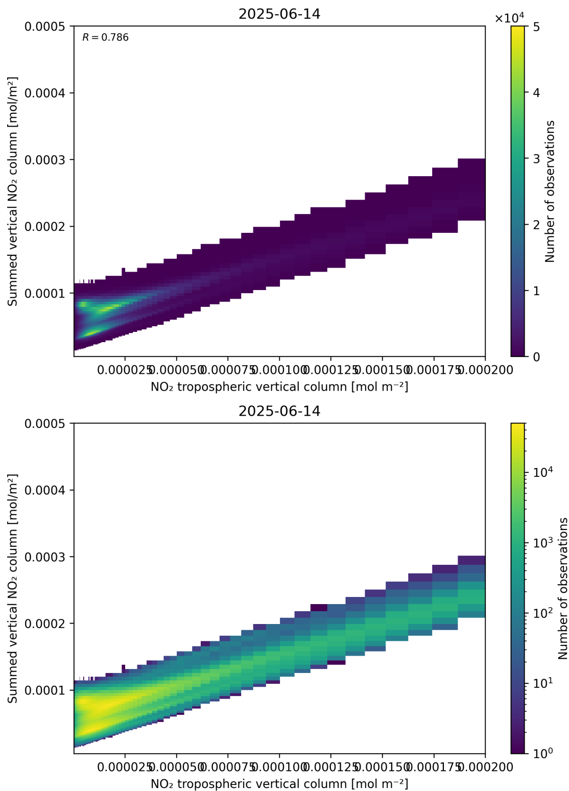
Figure 126: Scatter density plot of “NO 2 tropospheric vertical column” against “Summed vertical NO 2 column” for 2025-06-13 to 2025-06-15.
