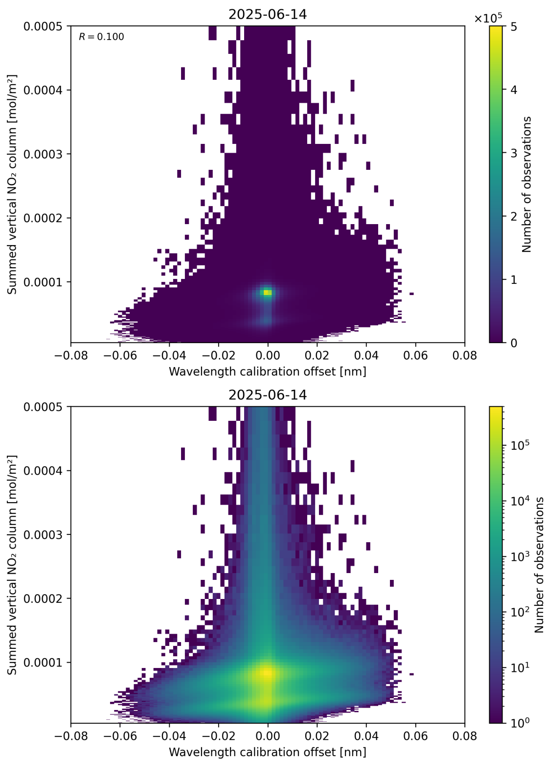
Figure 177: Scatter density plot of “Wavelength calibration offset” against “Summed vertical NO 2 column” for 2025-06-13 to 2025-06-15.
