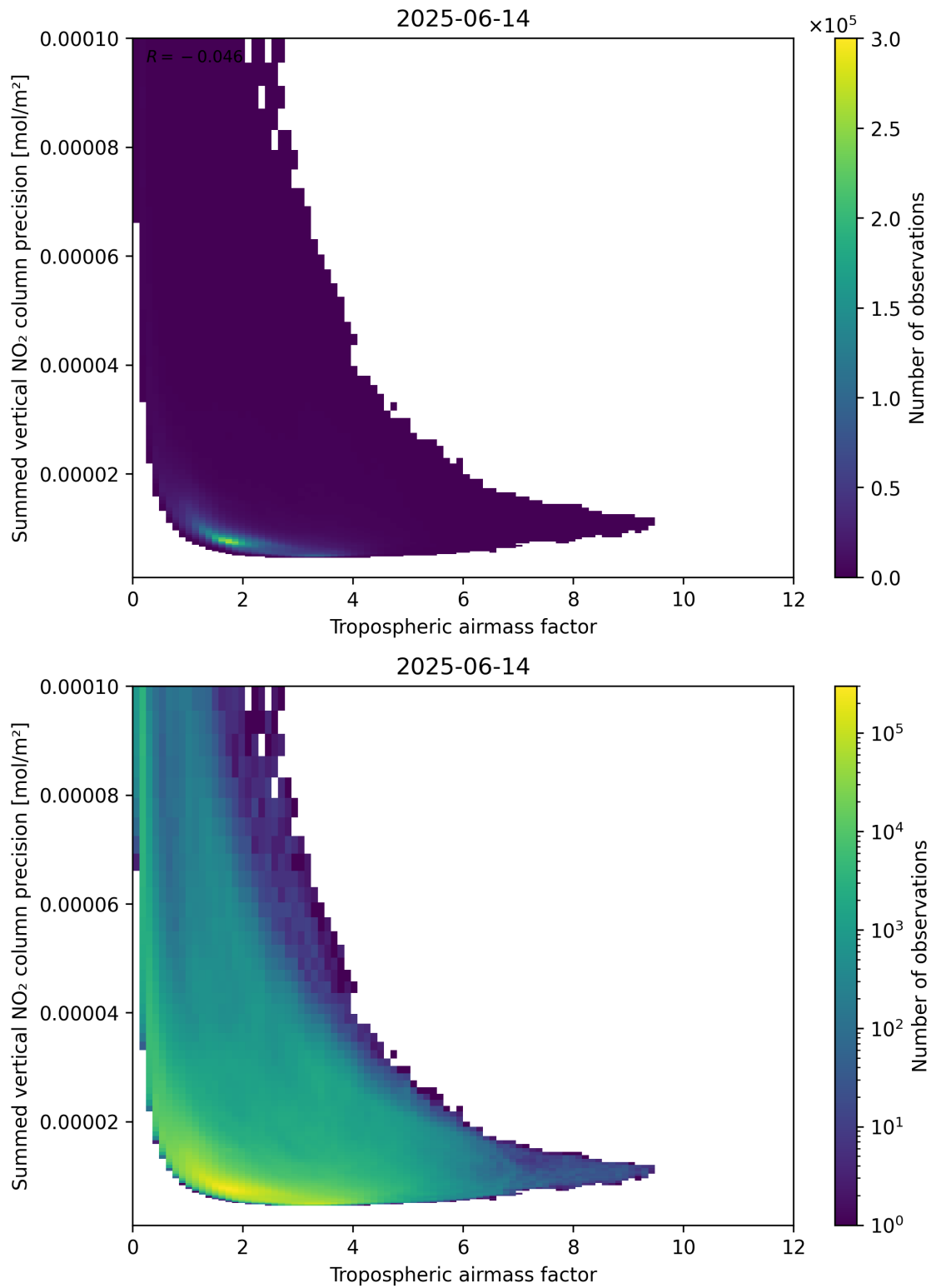
Figure 76: Scatter density plot of “Tropospheric air mass factor” against “Summed vertical NO 2 column precision” for 2025-06-13 to 2025-06-15.
