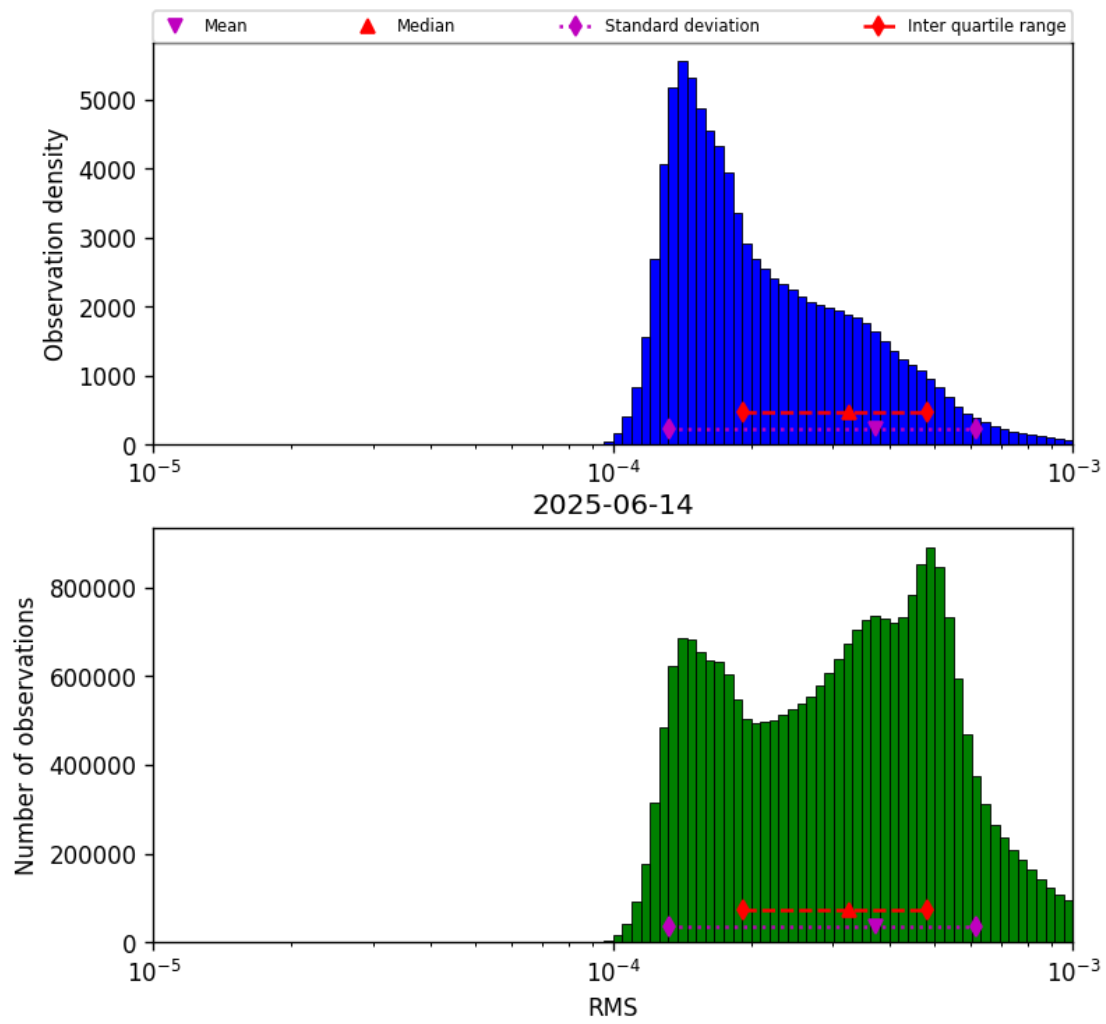
Figure 43: Histogram of “RMS” for 2025-06-13 to 2025-06-15
