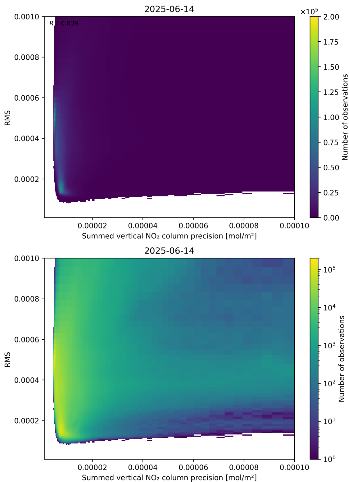
Figure 108: Scatter density plot of “Summed vertical NO 2 column precision” against “RMS” for 2025-06-13 to 2025-06-15.
