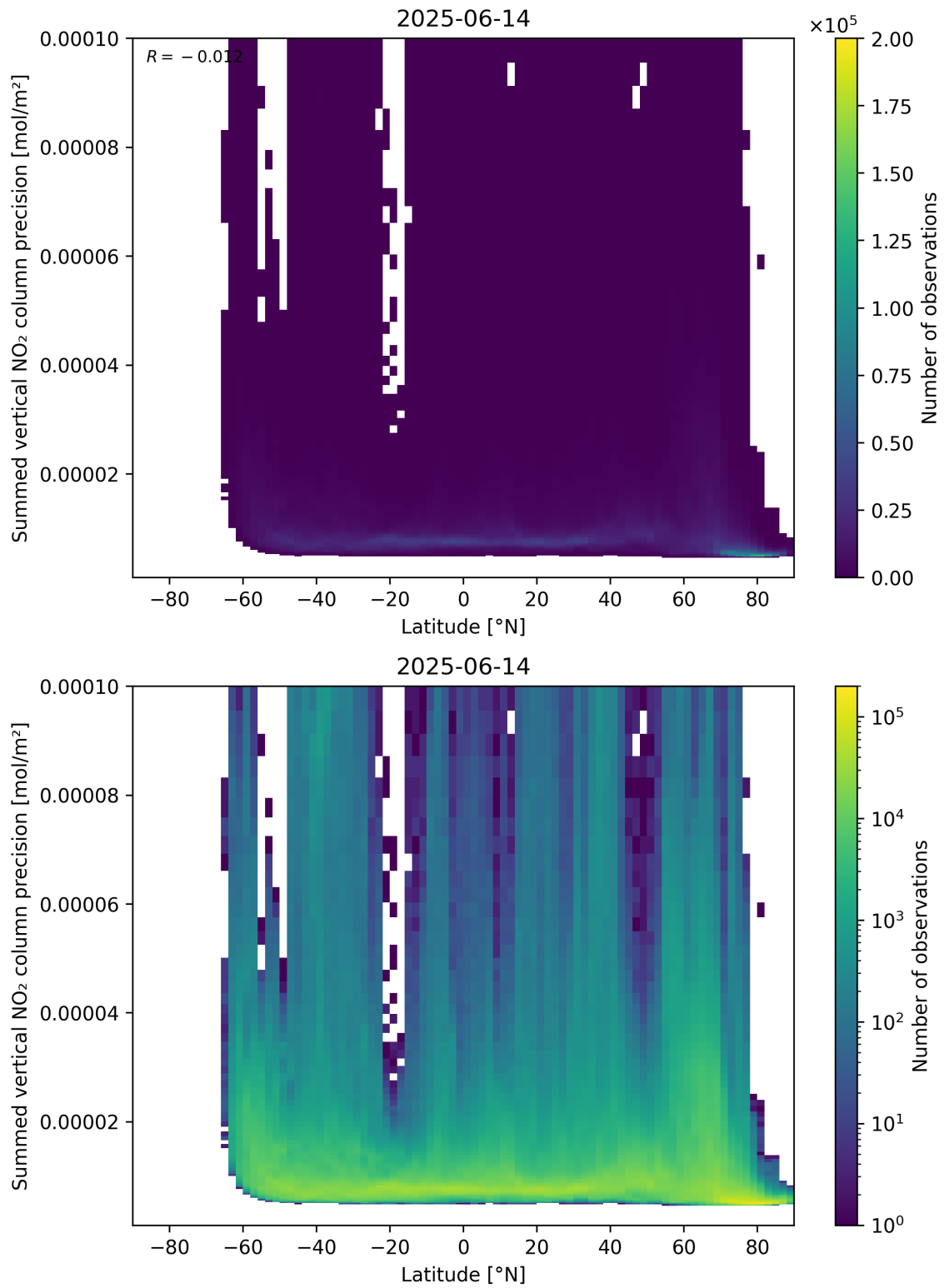
Figure 89: Scatter density plot of “Latitude” against “Summed vertical NO 2 column precision” for 2025-06-13 to 2025-06-15.
