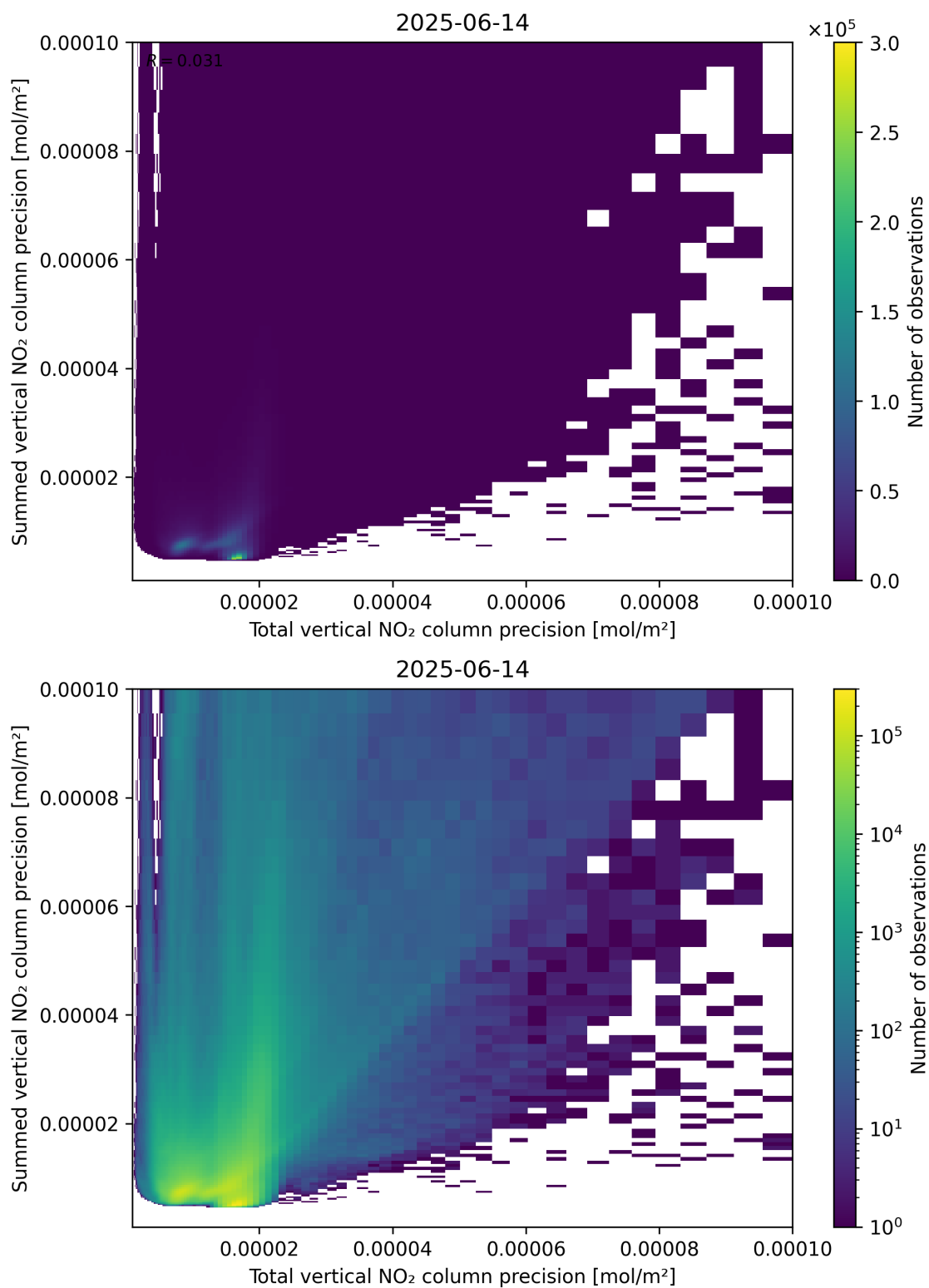
Figure 118: Scatter density plot of “Total vertical NO 2 column precision” against “Summed vertical NO 2 column precision” for 2025-06-13 to 2025-06-15.
