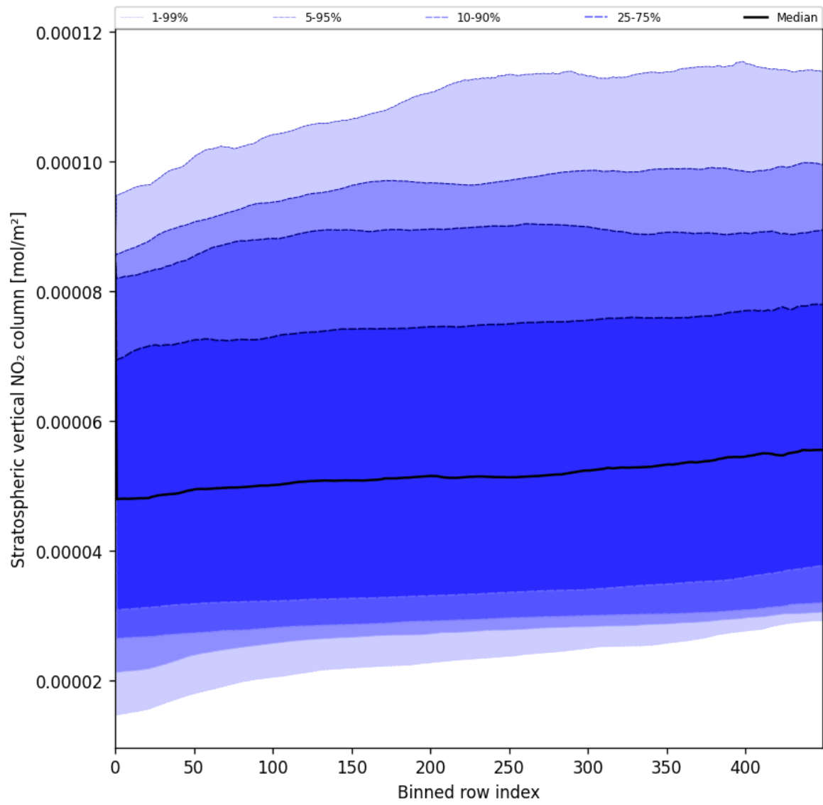
Figure 53: Along track statistics of “Stratospheric vertical NO 2 column” for 2025-06-13 to 2025-06-15
