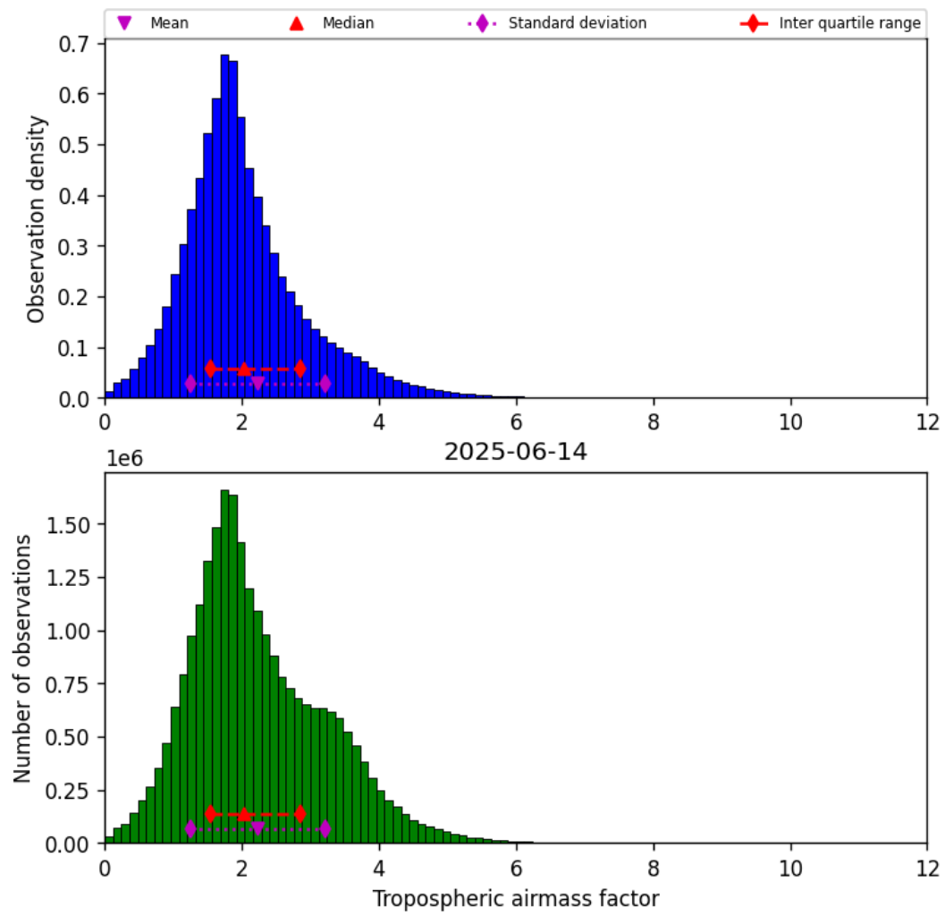
Figure 31: Histogram of “Tropospheric airmass factor” for 2025-06-13 to 2025-06-15
