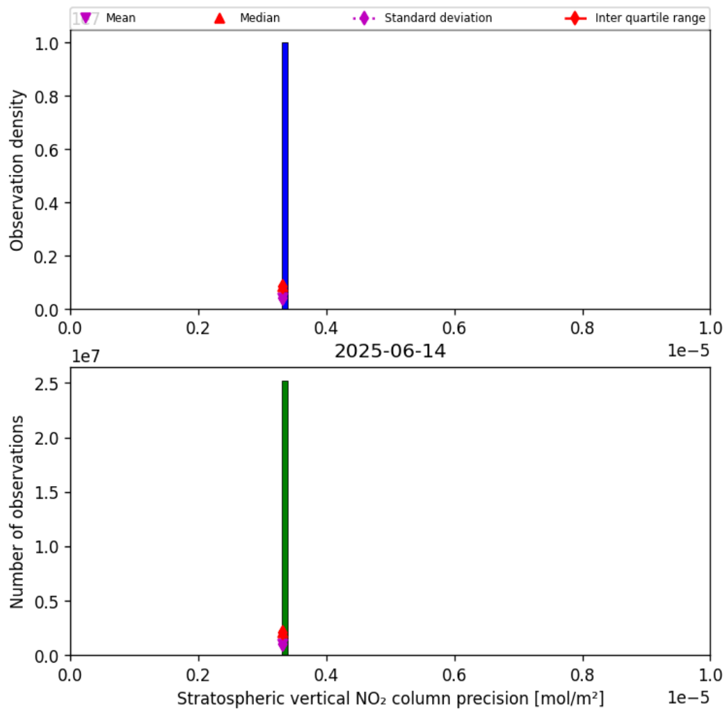
Figure 37: Histogram of “Stratospheric vertical NO 2 column precision” for 2025-06-13 to 2025-06-15
