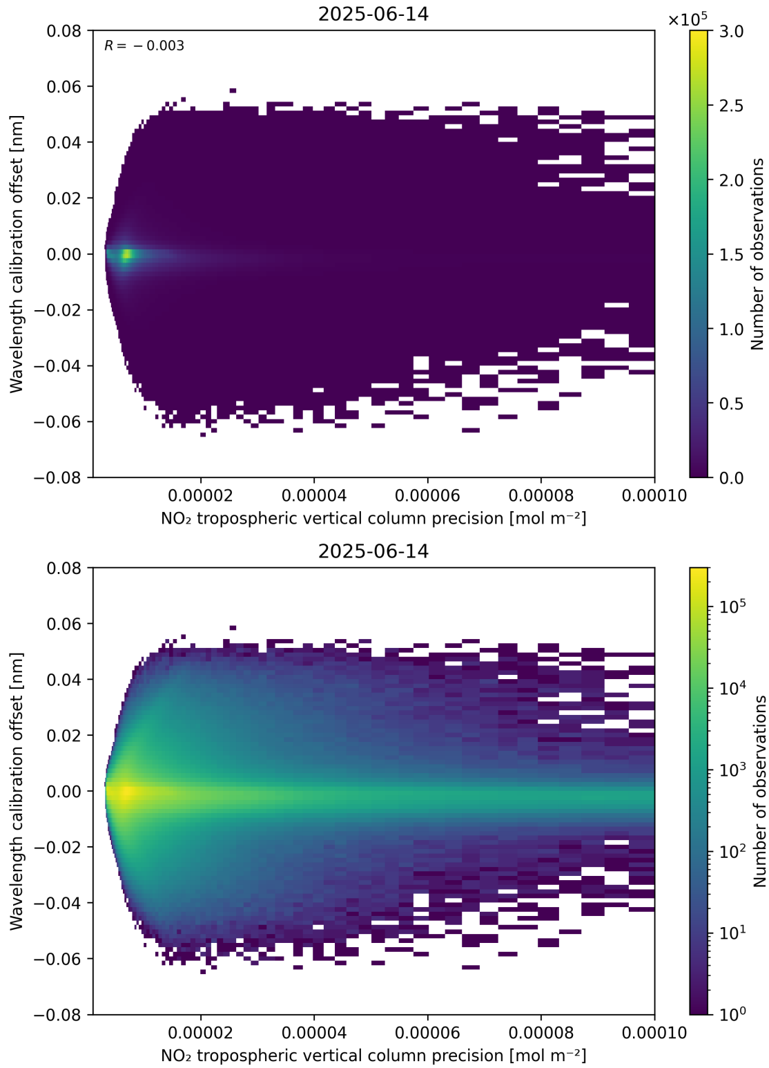
Figure 141: Scatter density plot of “NO 2 tropospheric vertical column precision” against “Wavelength calibration offset” for 2025-06-13 to 2025-06-15.
