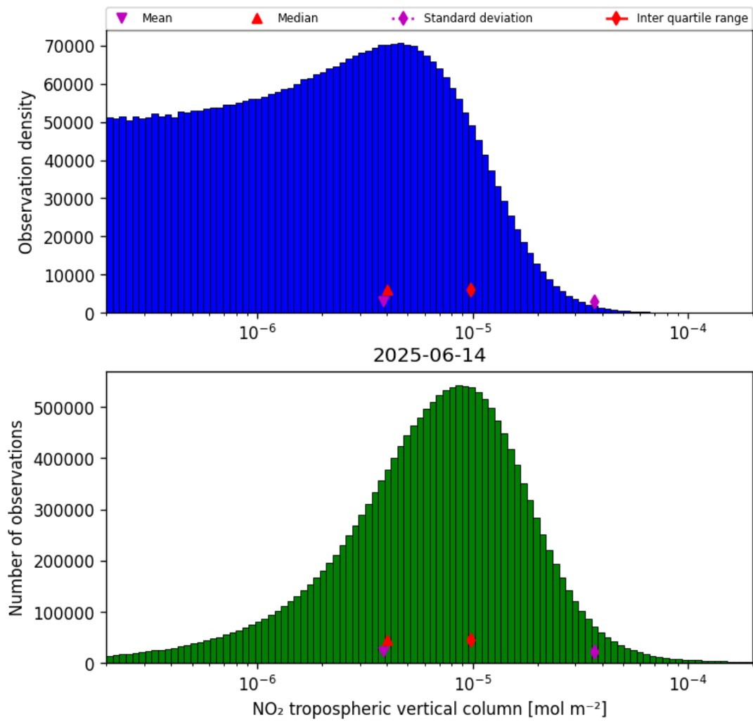
Figure 29: Histogram of “NO 2 tropospheric vertical column” for 2025-06-13 to 2025-06-15
