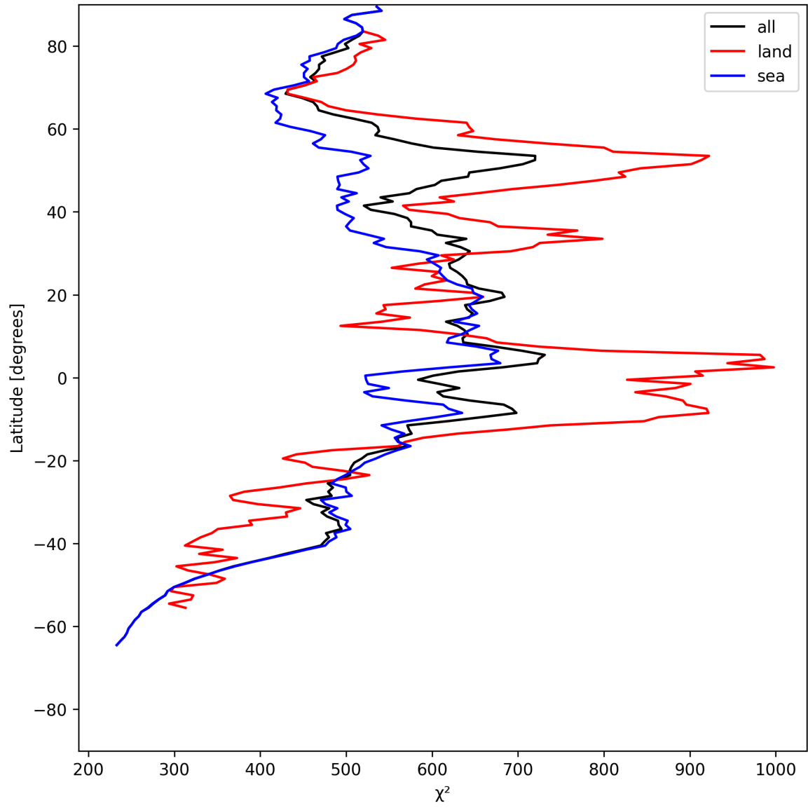
Figure 25: Zonal average of “ \chi^2 ” for 2025-06-13 to 2025-06-15.
