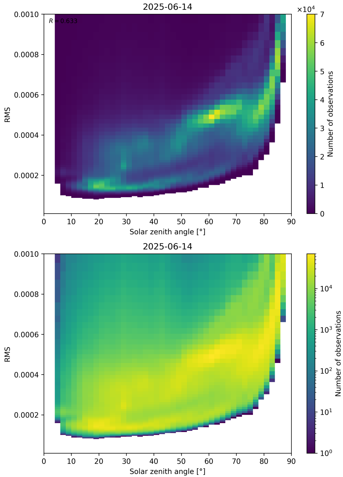
Figure 157: Scatter density plot of “Solar zenith angle” against “RMS” for 2025-06-13 to 2025-06-15.
