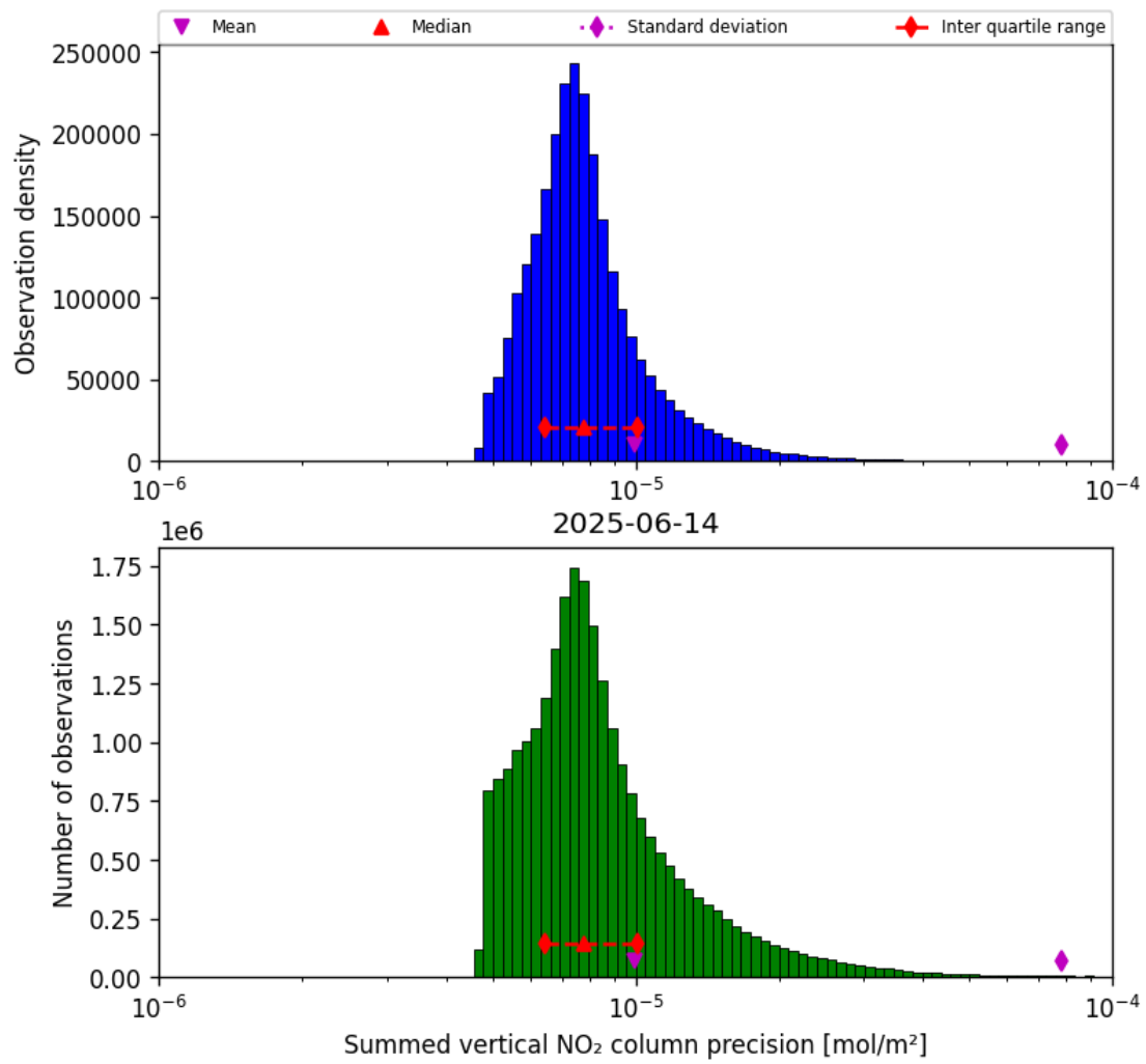
Figure 41: Histogram of "Summed vertical NO 2 column precision" for 2025-06-13 to 2025-06-15
