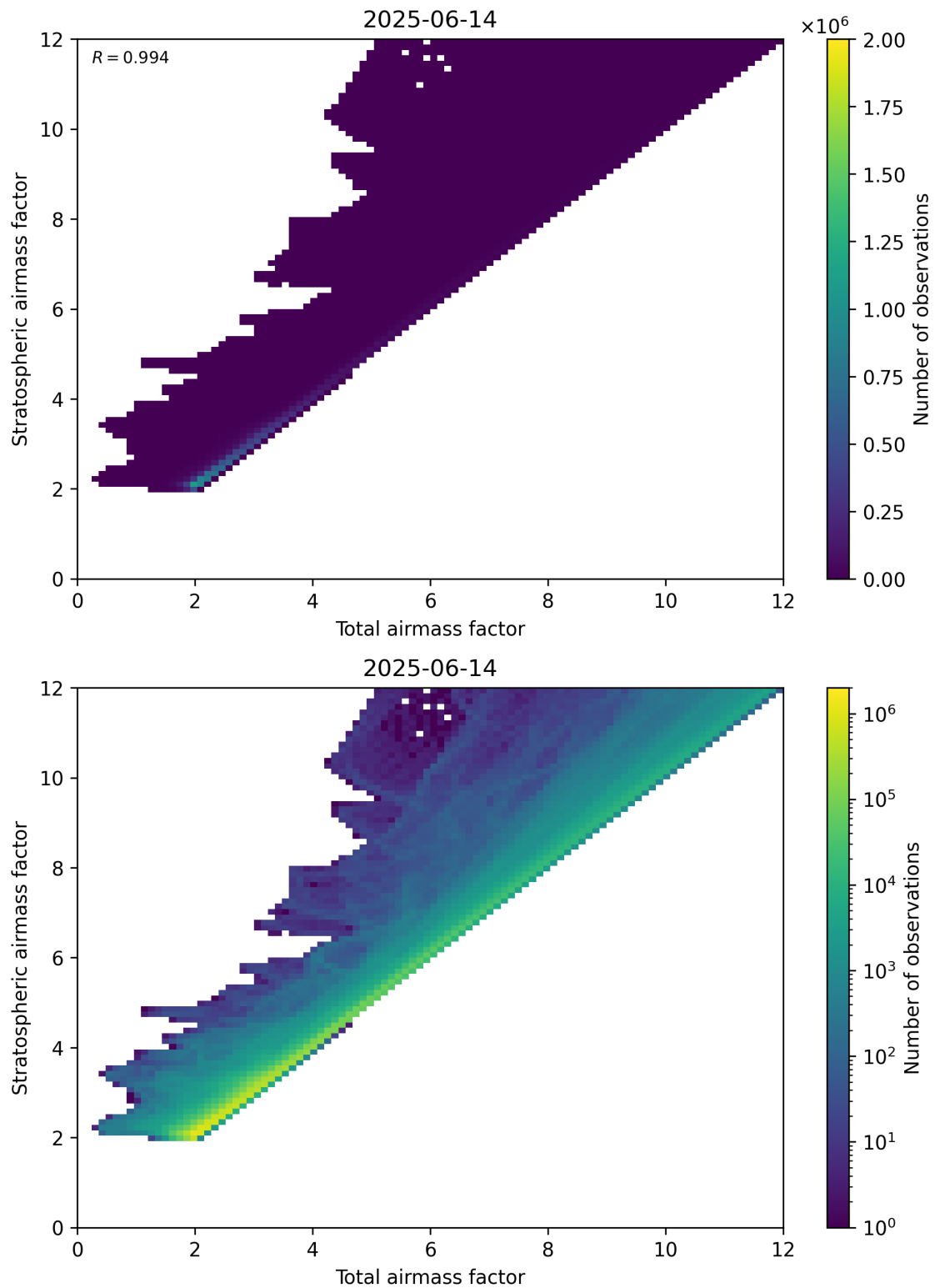
Figure 62: Scatter density plot of “Total airmass factor” against “Stratospheric airmass factor” for 2025-06-13 to 2025-06-15.
