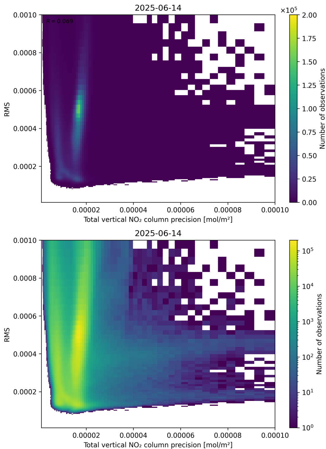
Figure 119: Scatter density plot of “Total vertical NO 2 column precision” against “RMS” for 2025-06-13 to 2025-06-15.
