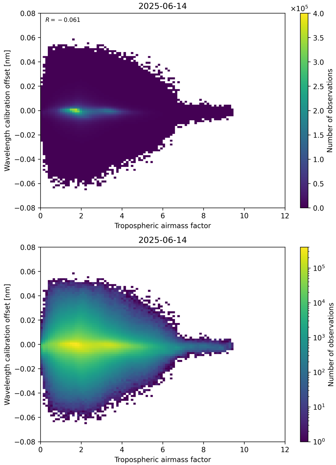
Figure 80: Scatter density plot of “Tropospheric airmass factor” against “Wavelength calibration offset” for 2025-06-13 to 2025-06-15.
