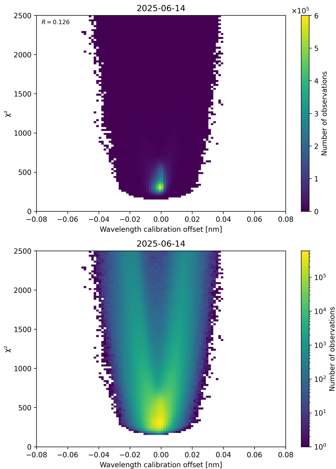
Figure 175: Scatter density plot of “Wavelength calibration offset” against “ \chi^2 ” for 2025-06-13 to 2025-06-15.
