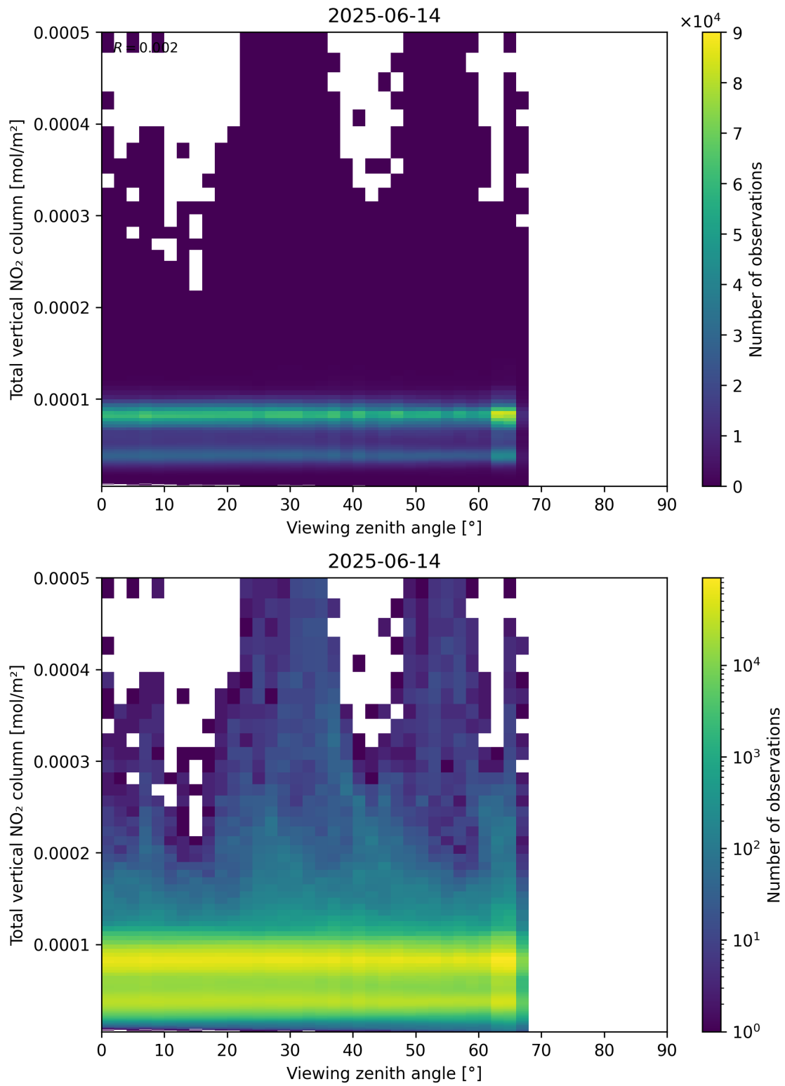
Figure 167: Scatter density plot of “Viewing zenith angle” against “Total vertical NO 2 column” for 2025-06-13 to 2025-06-15.
