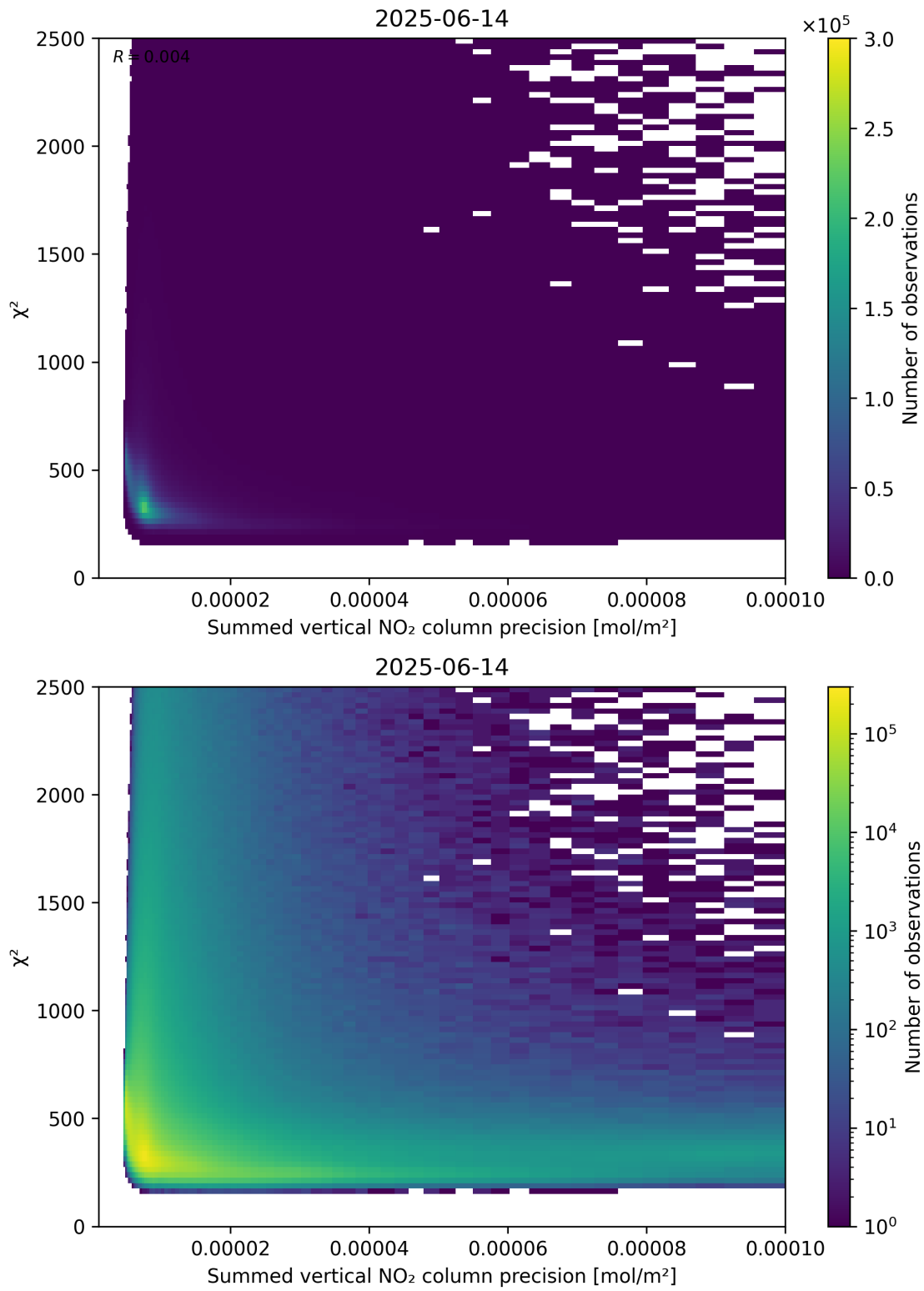
Figure 107: Scatter density plot of “Summed vertical NO 2 column precision” against “ \chi^2 ” for 2025-06-13 to 2025-06-15.
