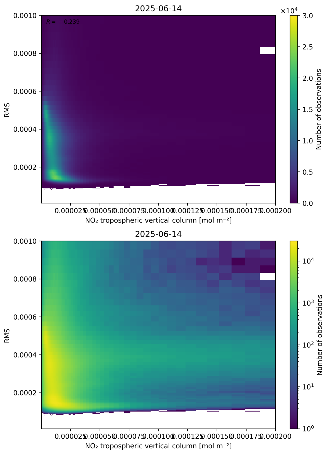
Figure 142: Scatter density plot of “NO 2 tropospheric vertical column” against “RMS” for 2025-06-13 to 2025-06-15.
