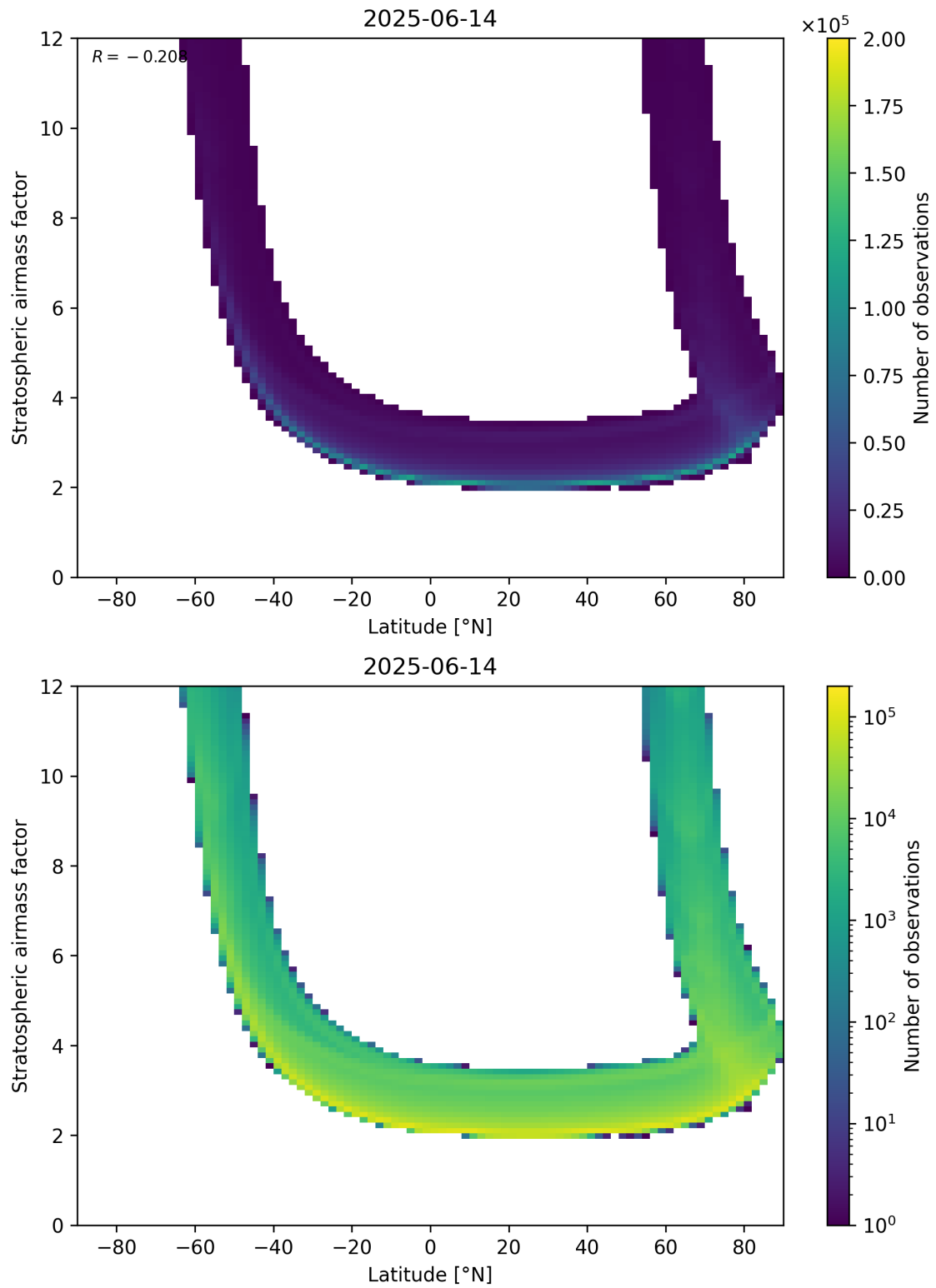
Figure 83: Scatter density plot of “Latitude” against “Stratospheric air mass factor” for 2025-06-13 to 2025-06-15.
