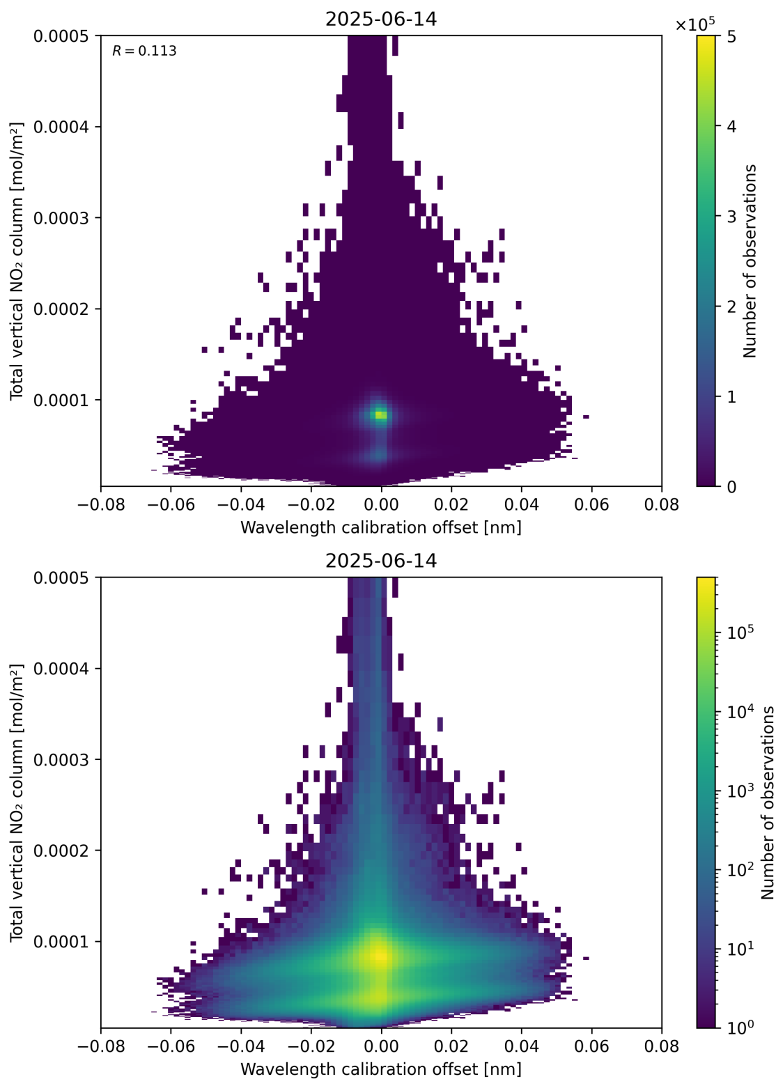
Figure 179: Scatter density plot of “Wavelength calibration offset” against “Total vertical NO 2 column” for 2025-06-13 to 2025-06-15.
