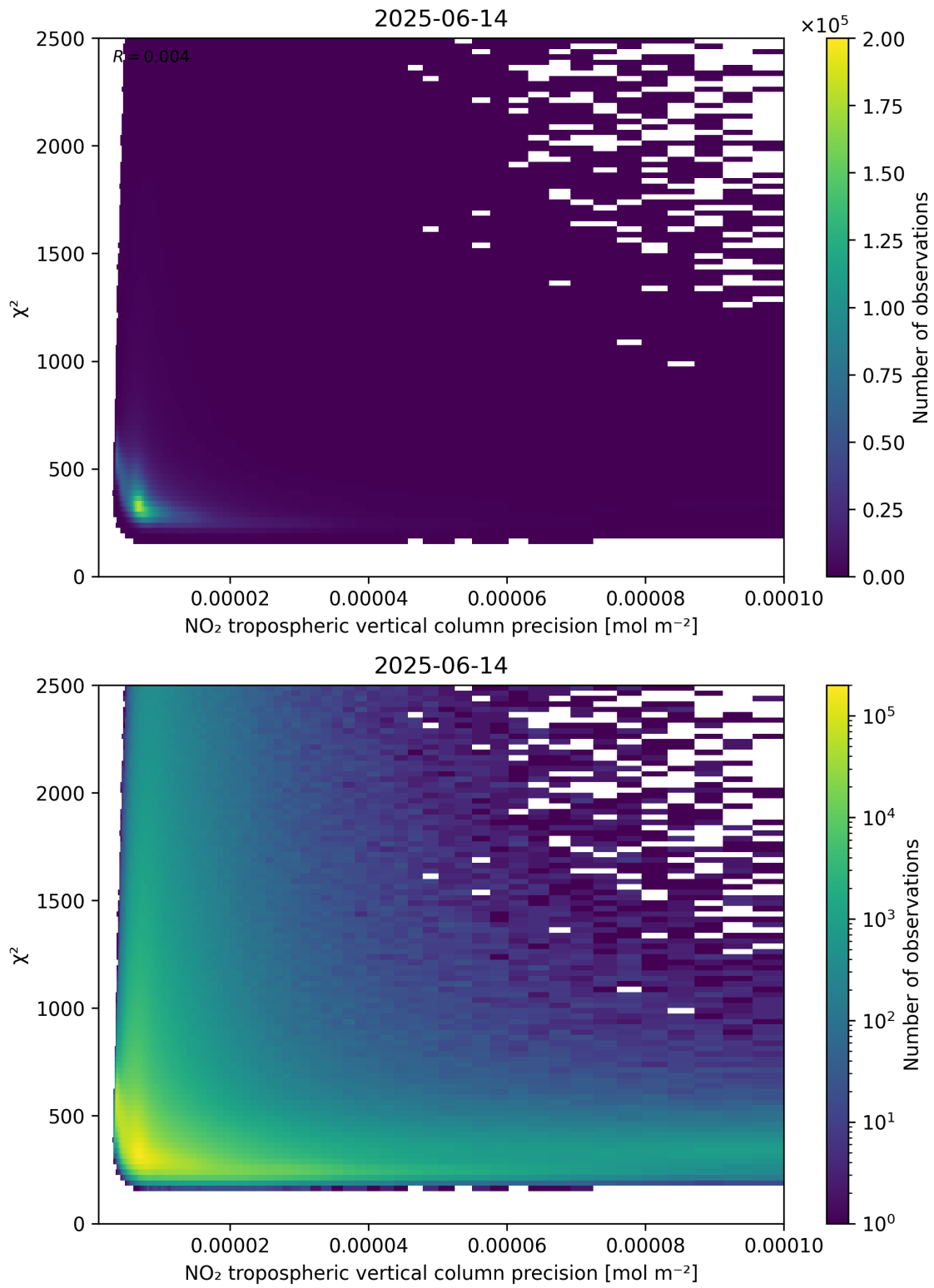
Figure 134: Scatter density plot of “NO 2 tropospheric vertical column precision” against “ \chi^2 ” for 2025-06-13 to 2025-06-15.
