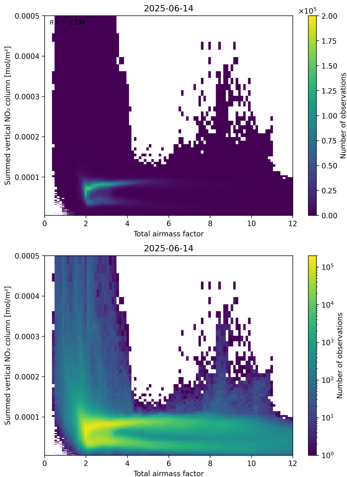
Figure 65: Scatter density plot of “Total airmass factor” against “Summed vertical NO 2 column” for 2025-06-13 to 2025-06-15.
