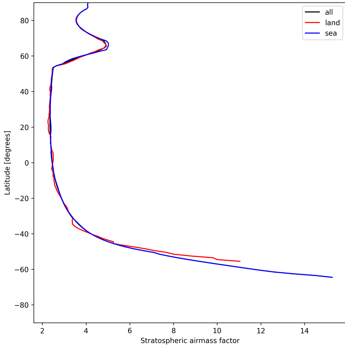
Figure 27: Zonal average of “Stratospheric airmass factor” for 2025-06-13 to 2025-06-15.
