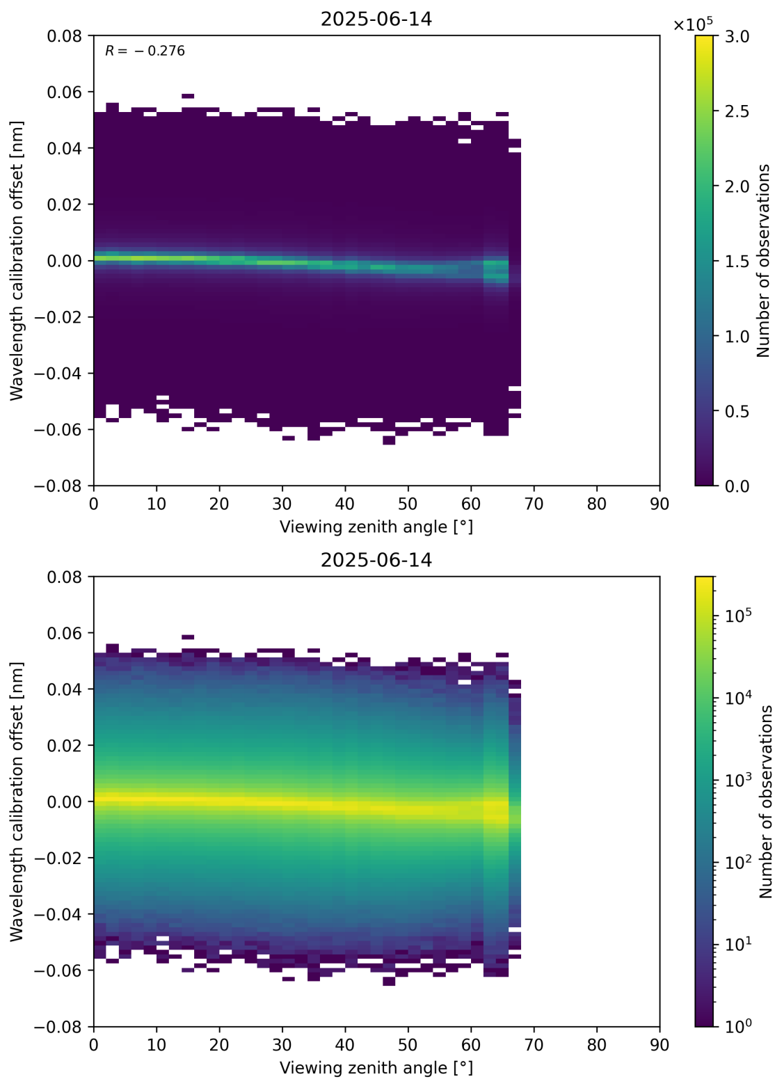
Figure 173: Scatter density plot of “Viewing zenith angle” against “Wavelength calibration offset” for 2025-06-13 to 2025-06-15.
