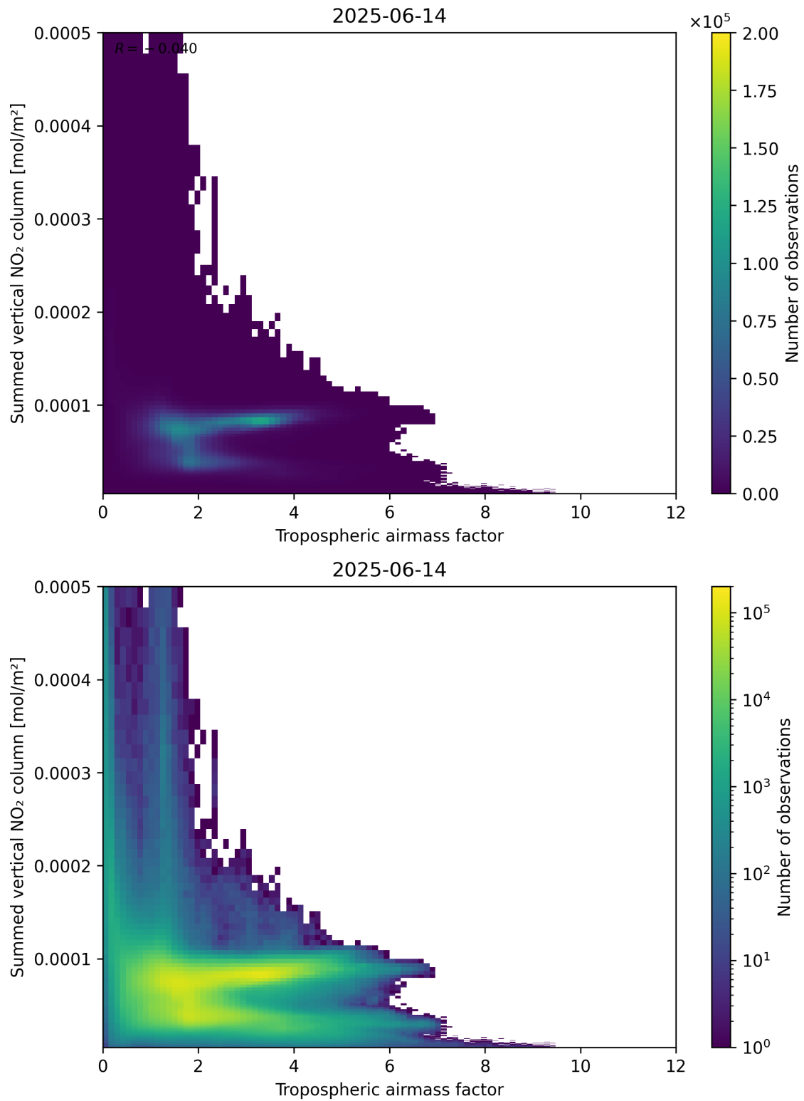
Figure 75: Scatter density plot of “Tropospheric air mass factor” against “Summed vertical NO 2 column” for 2025-06-13 to 2025-06-15.
