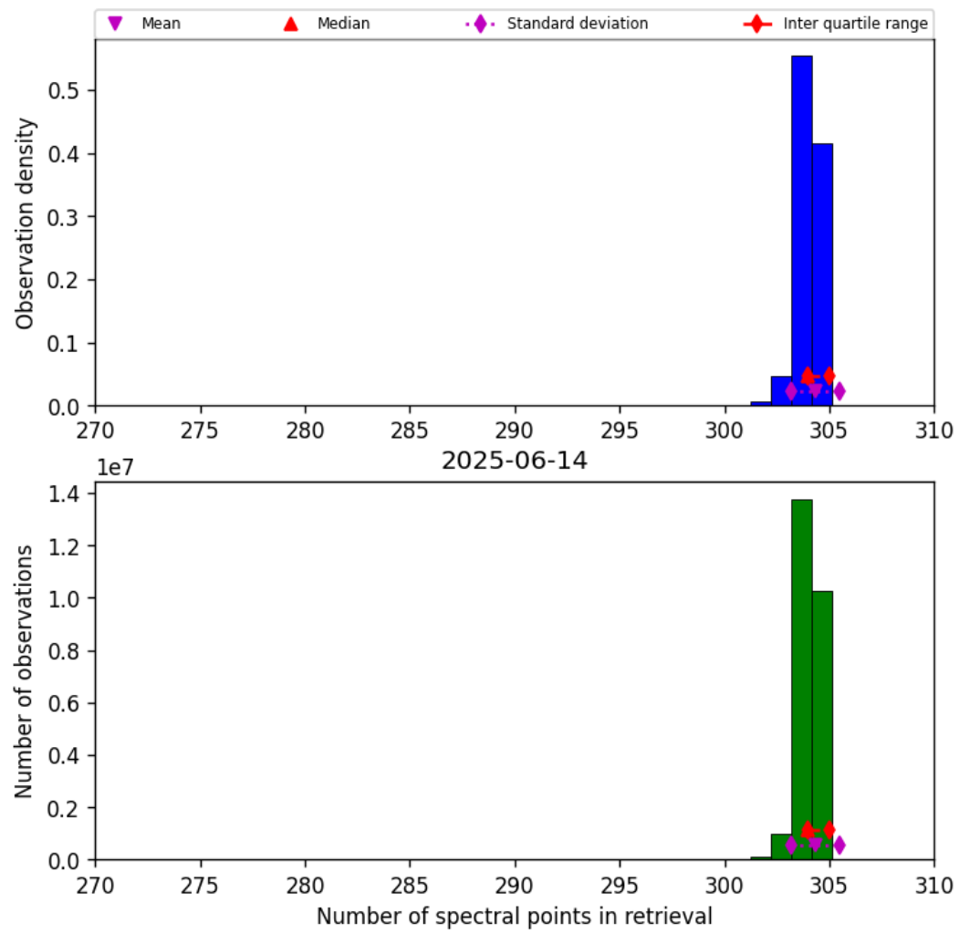
Figure 33: Histogram of “Number of spectral points in retrieval” for 2025-06-13 to 2025-06-15
