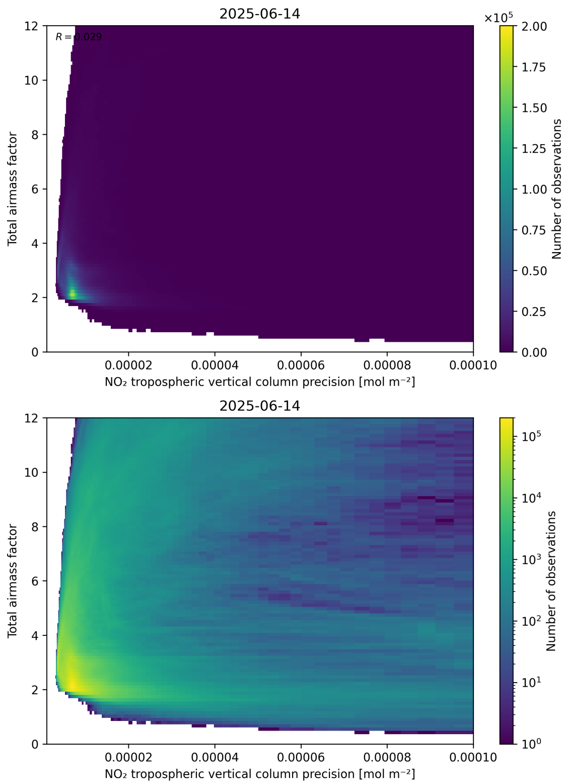
Figure 132: Scatter density plot of “NO 2 tropospheric vertical column precision” against “Total air mass factor” for 2025-06-13 to 2025-06-15.
