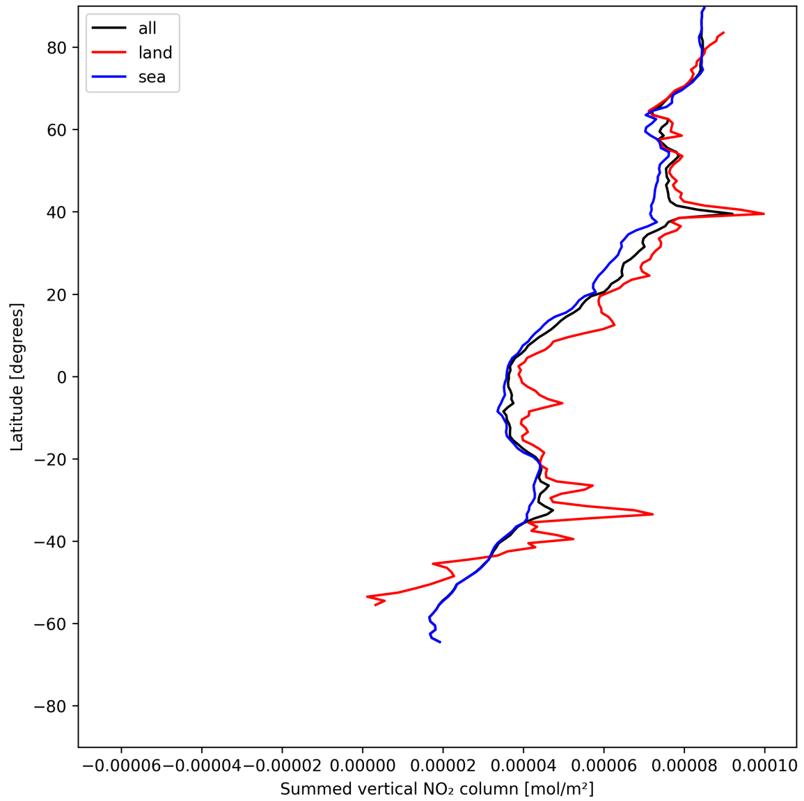
Figure 23: Zonal average of “Summed vertical NO 2 column” for 2025-06-13 to 2025-06-15.
