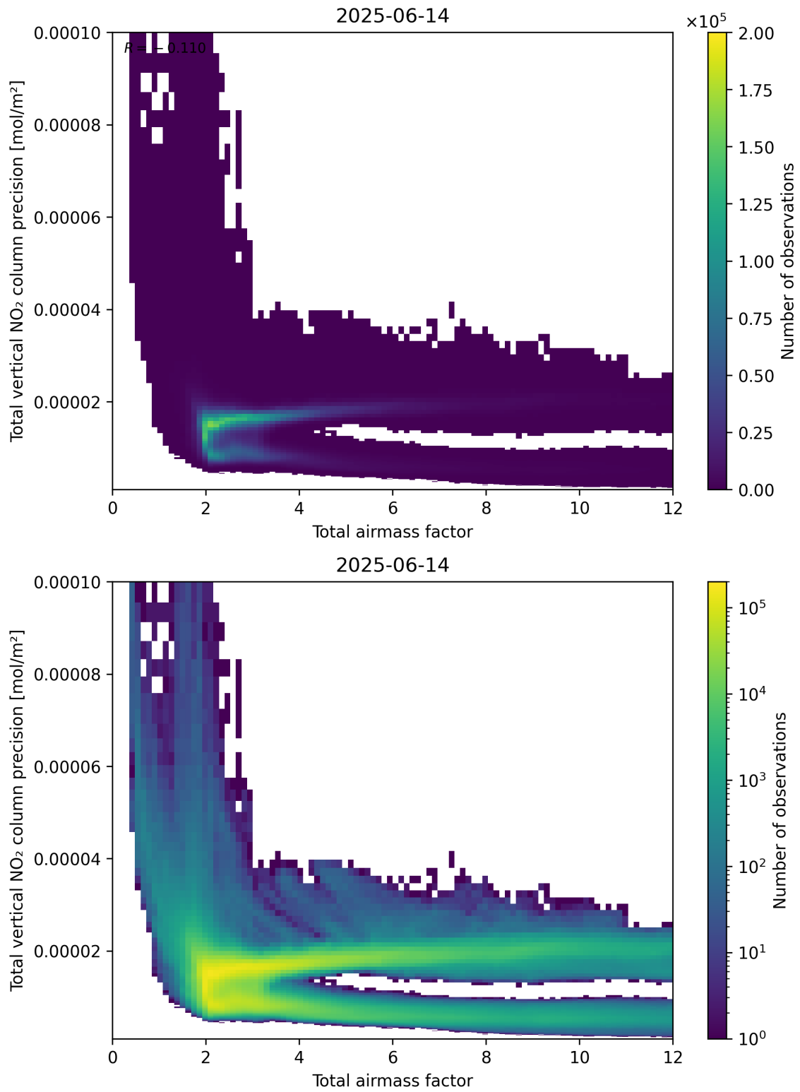
Figure 68: Scatter density plot of “Total airmass factor” against “Total vertical NO 2 column precision” for 2025-06-13 to 2025-06-15.
