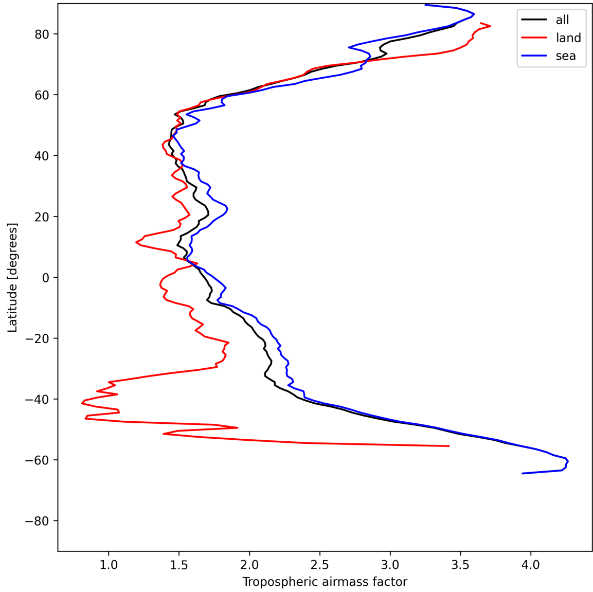
Figure 14: Zonal average of “Tropospheric airmass factor” for 2025-06-13 to 2025-06-15.
