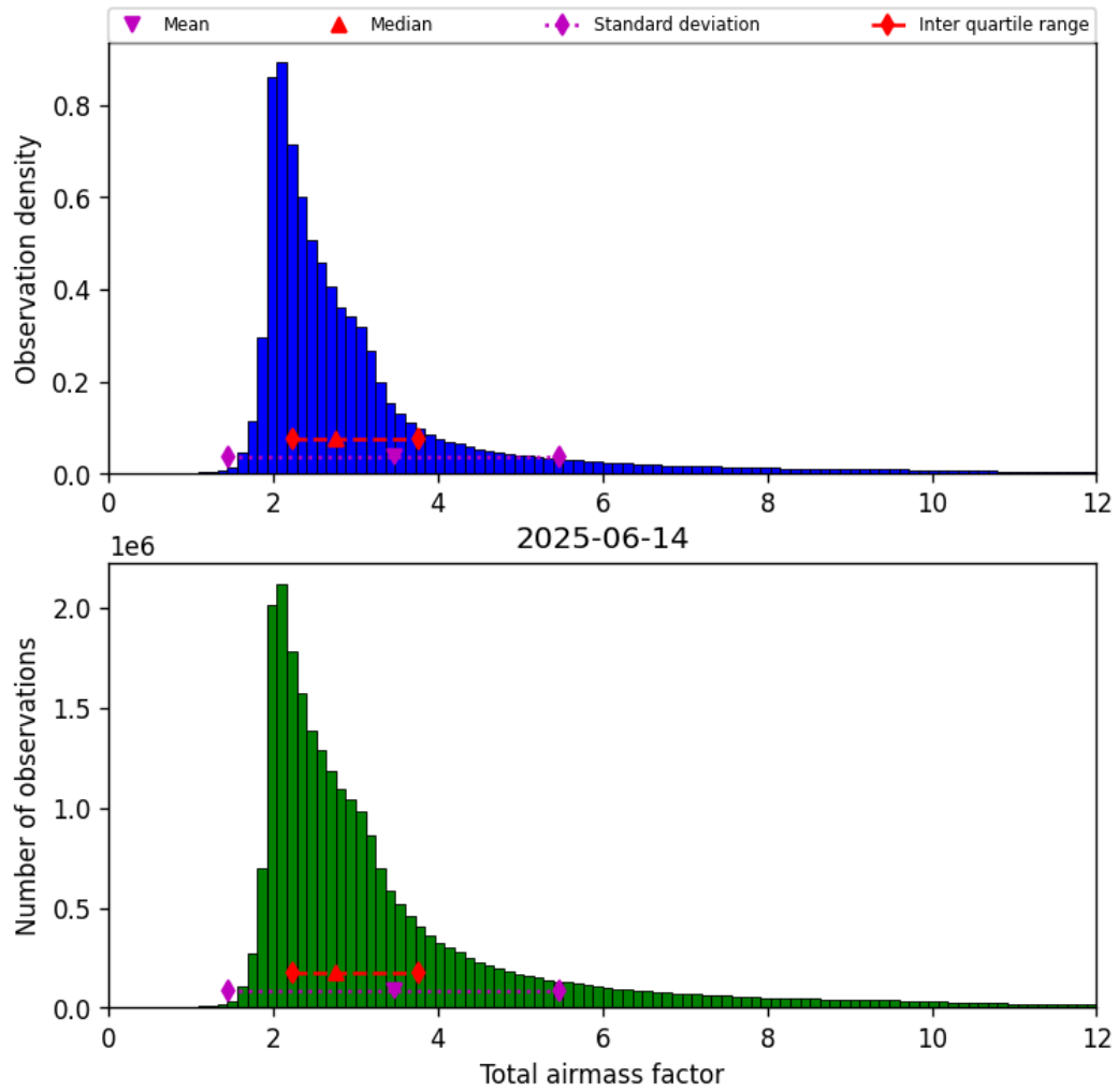
Figure 32: Histogram of “Total airmass factor” for 2025-06-13 to 2025-06-15
