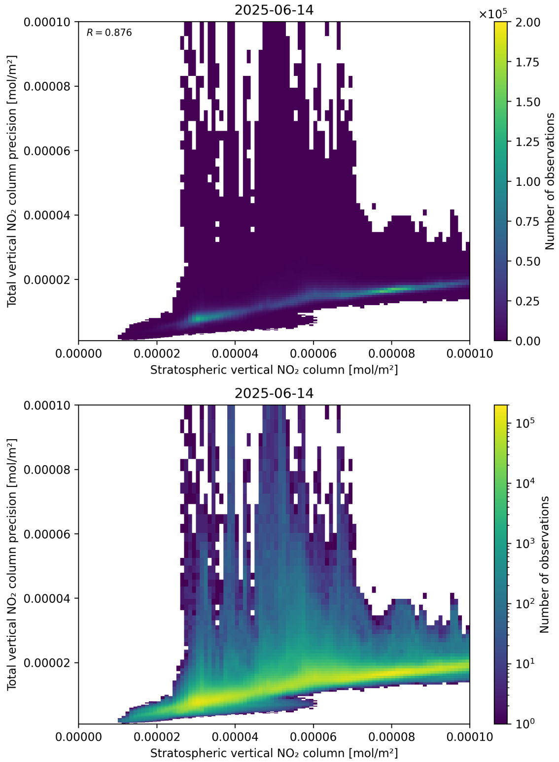
Figure 101: Scatter density plot of “Stratospheric vertical NO 2 column” against “Total vertical NO 2 column precision” for 2025-06-13 to 2025-06-15.
