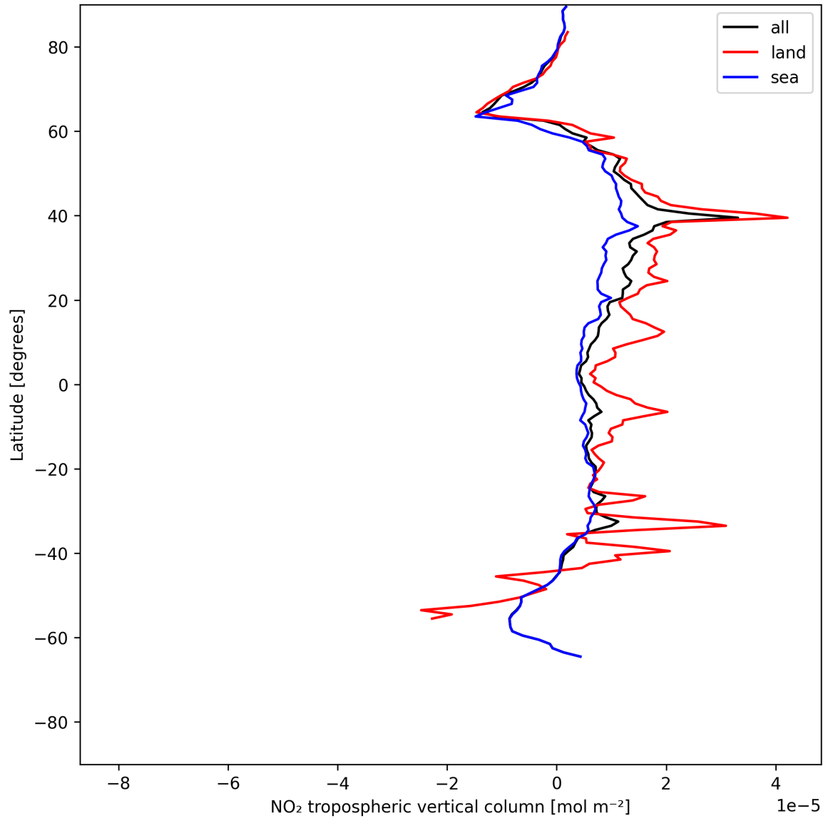
Figure 12: Zonal average of “NO 2 tropospheric vertical column” for 2025-06-13 to 2025-06-15.
