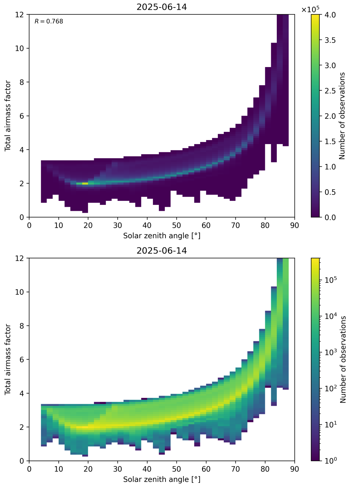
Figure 146: Scatter density plot of “Solar zenith angle” against “Total air mass factor” for 2025-06-13 to 2025-06-15.
