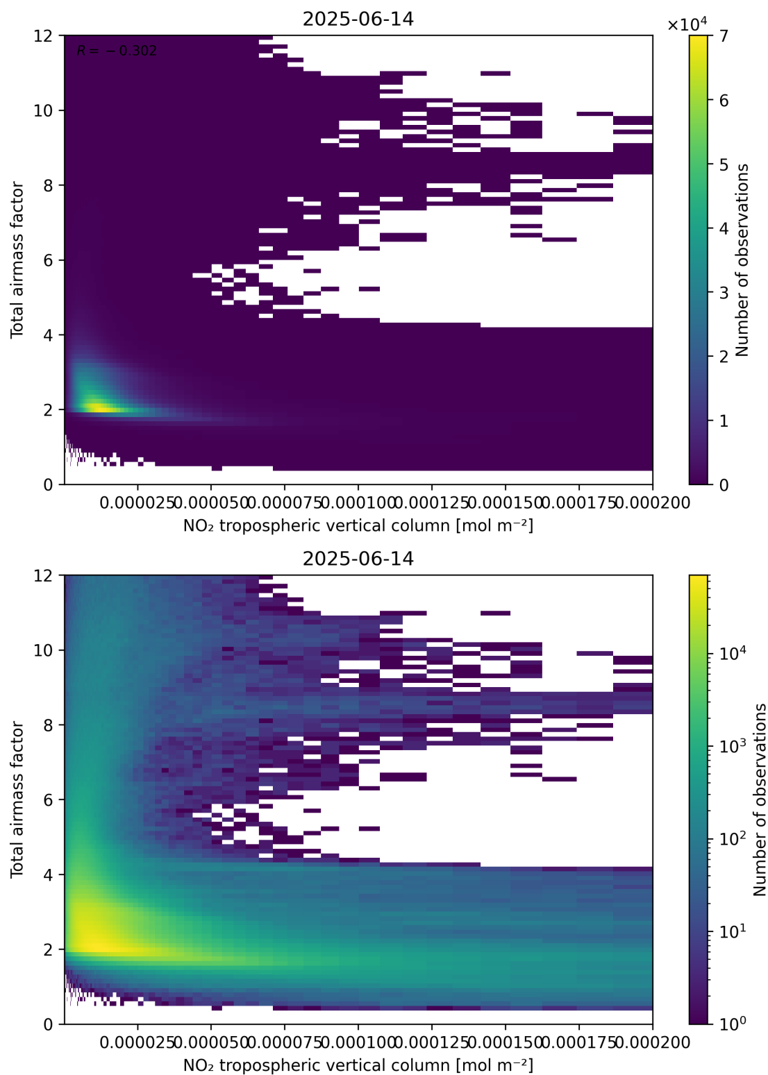
Figure 122: Scatter density plot of “NO 2 tropospheric vertical column” against “Total air mass factor” for 2025-06-13 to 2025-06-15.
