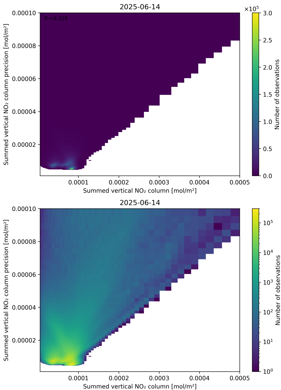
Figure 105: Scatter density plot of “Summed vertical NO 2 column” against “Summed vertical NO 2 column precision” for 2025-06-13 to 2025-06-15.
