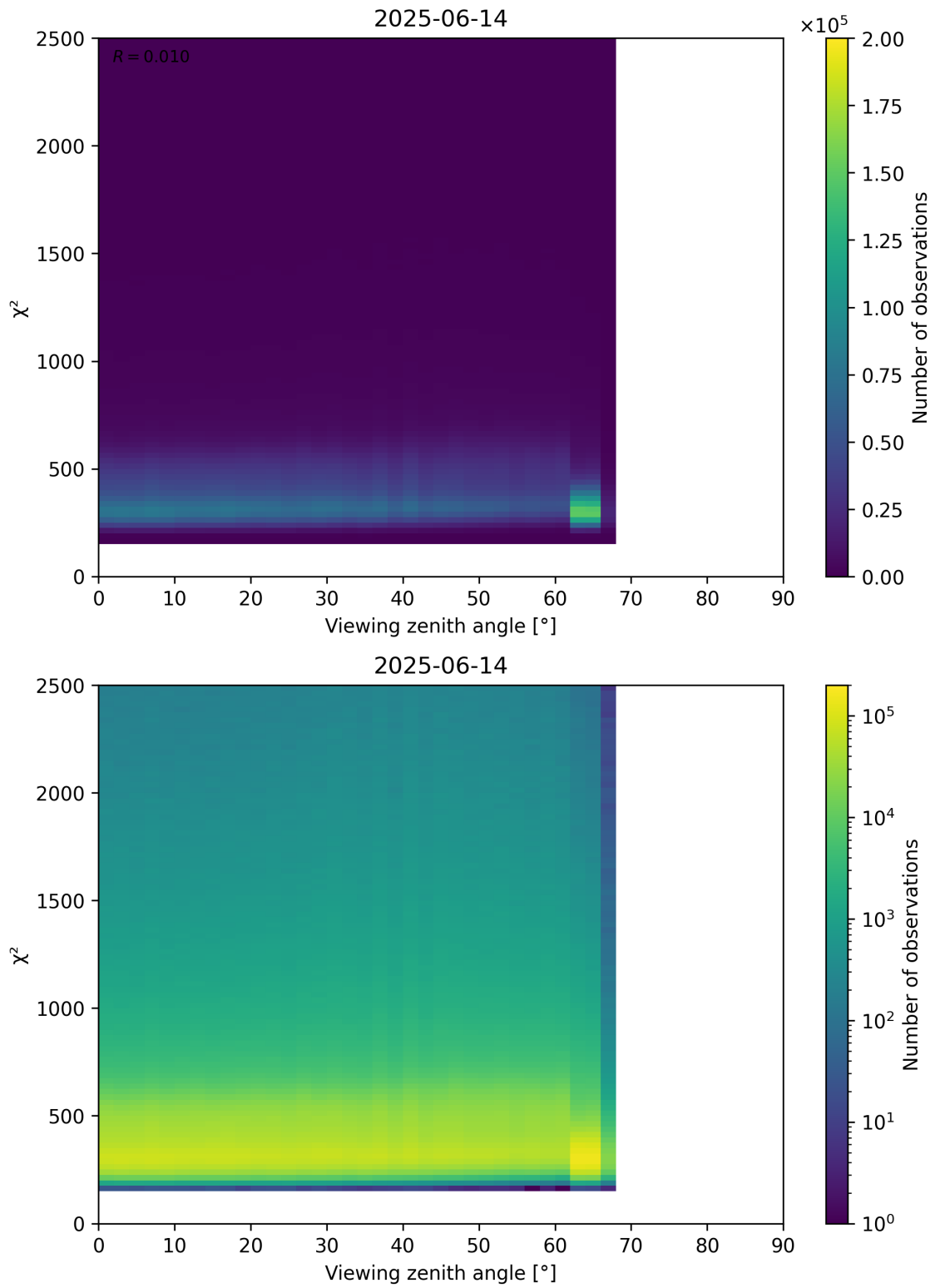
Figure 162: Scatter density plot of “Viewing zenith angle” against “ \chi^2 ” for 2025-06-13 to 2025-06-15.
