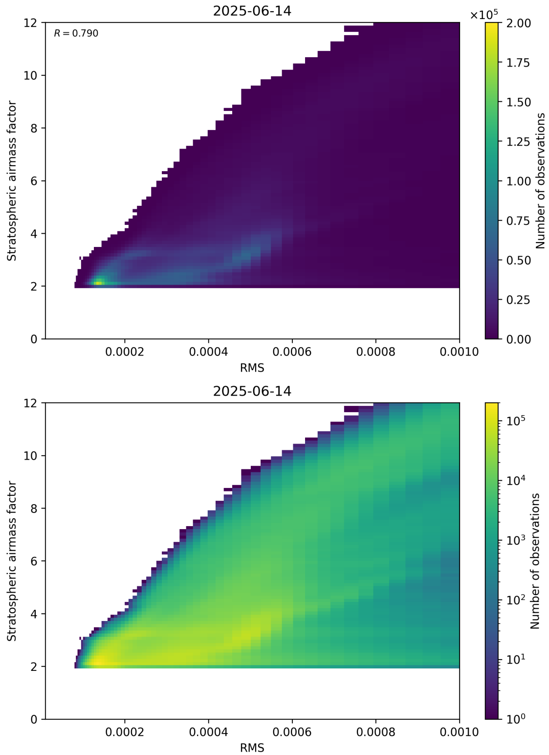
Figure 144: Scatter density plot of “RMS” against “Stratospheric airmass factor” for 2025-06-13 to 2025-06-15.
