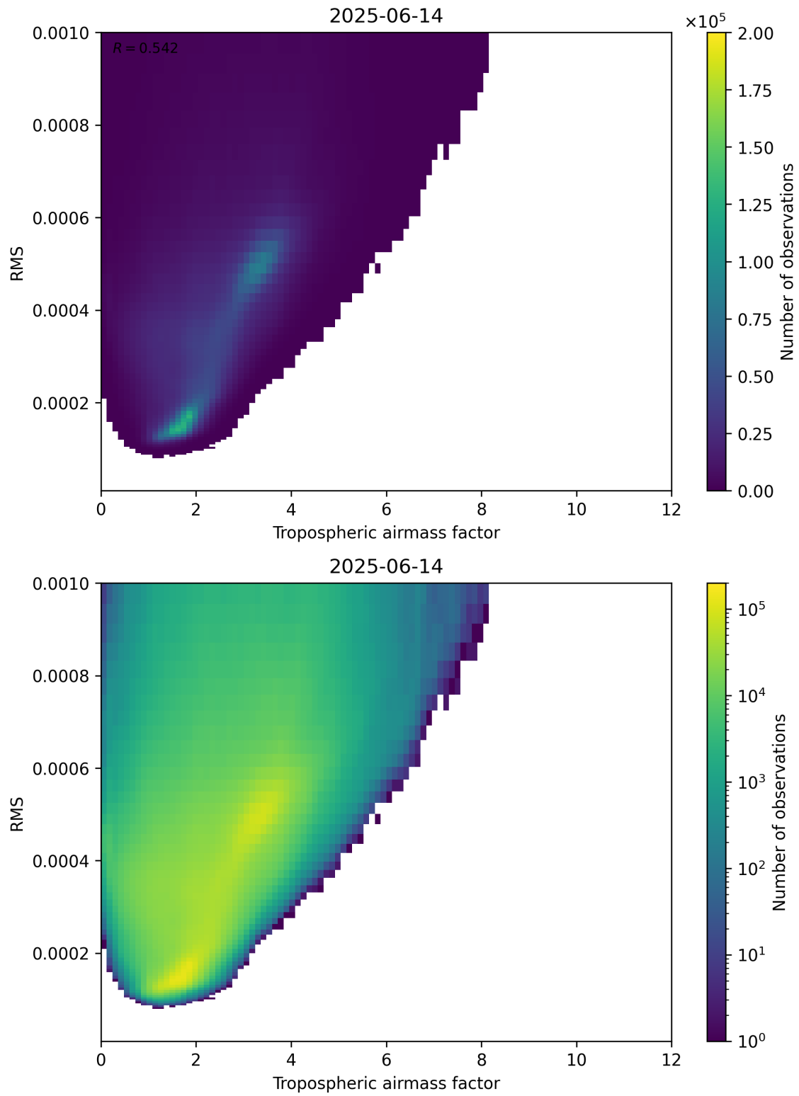
Figure 79: Scatter density plot of “Tropospheric airmass factor” against “RMS” for 2025-06-13 to 2025-06-15.
