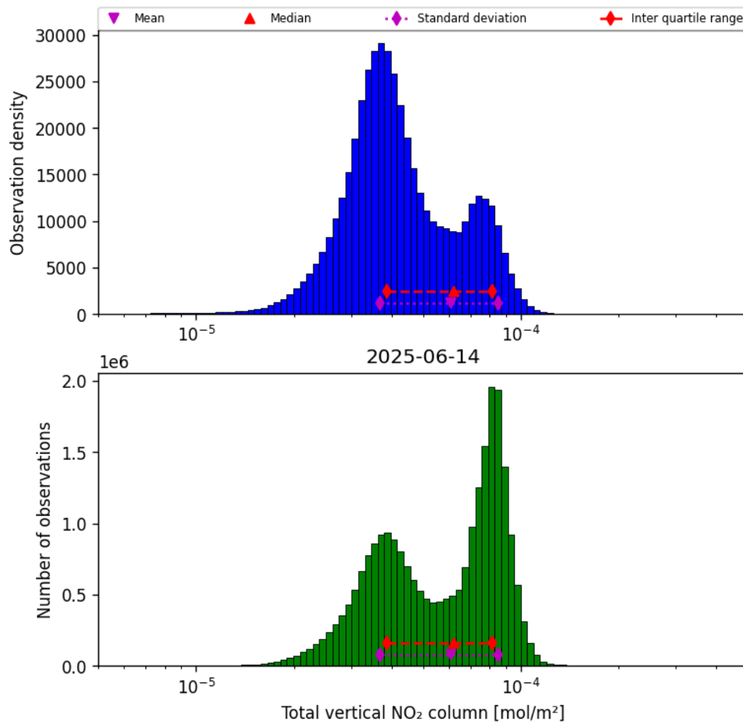
Figure 38: Histogram of “Total vertical NO 2 column” for 2025-06-13 to 2025-06-15
