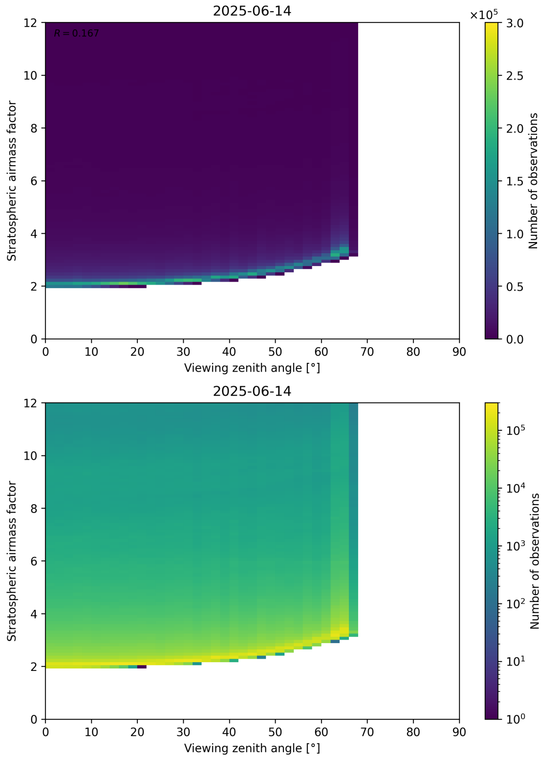
Figure 159: Scatter density plot of “Viewing zenith angle” against “Stratospheric airmass factor” for 2025-06-13 to 2025-06-15.
