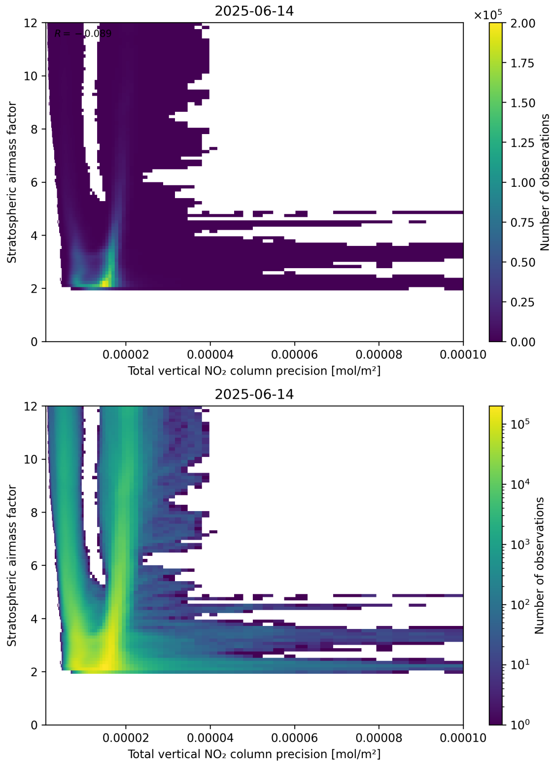
Figure 115: Scatter density plot of “Total vertical NO 2 column precision” against “Stratospheric air mass factor” for 2025-06-13 to 2025-06-15.
