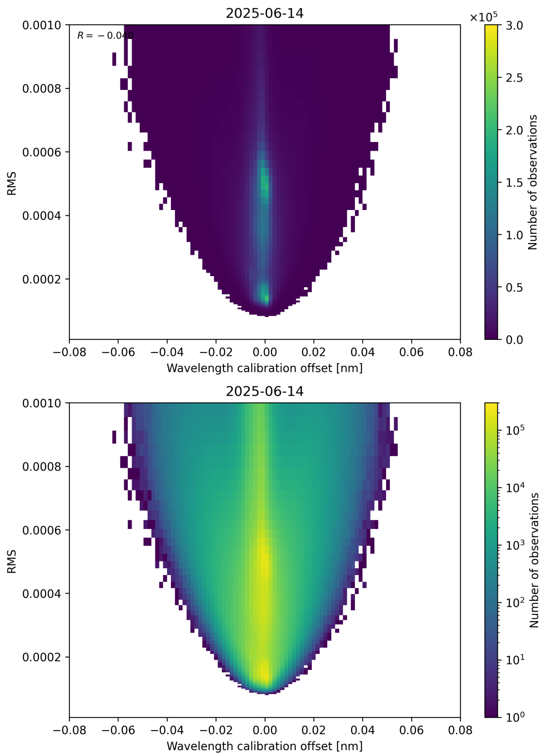
Figure 181: Scatter density plot of “Wavelength calibration offset” against “RMS” for 2025-06-13 to 2025-06-15.
