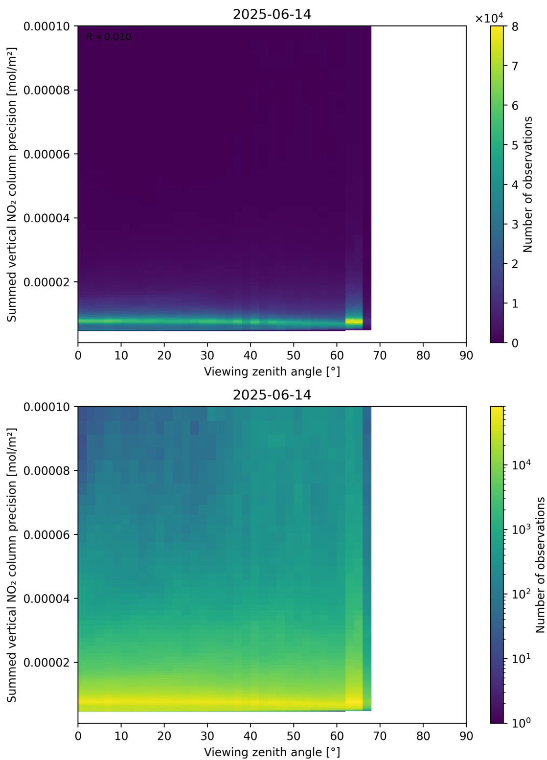
Figure 166: Scatter density plot of “Viewing zenith angle” against “Summed vertical NO 2 column precision” for 2025-06-13 to 2025-06-15.
