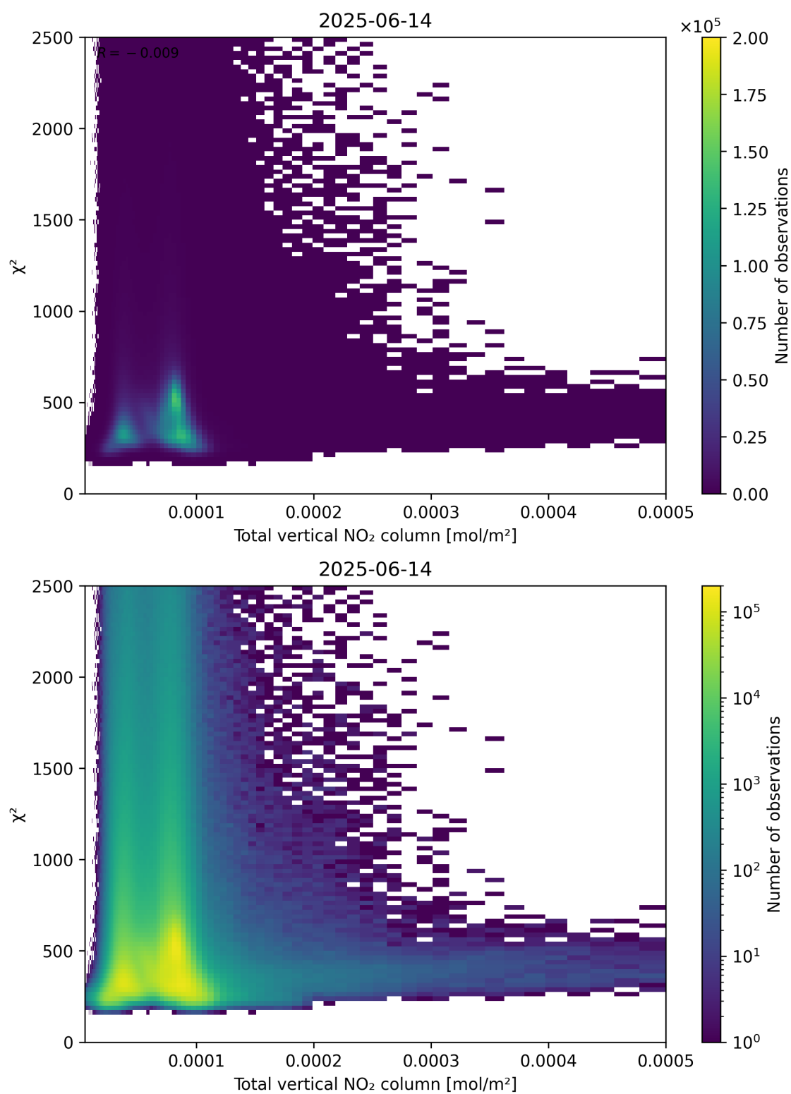
Figure 111: Scatter density plot of “Total vertical NO 2 column” against “ \chi^2 ” for 2025-06-13 to 2025-06-15.
