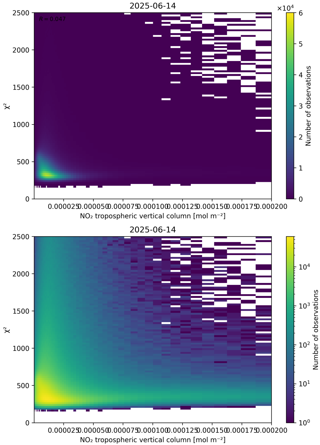
Figure 124: Scatter density plot of “NO 2 tropospheric vertical column” against “ \chi^2 ” for 2025-06-13 to 2025-06-15.
