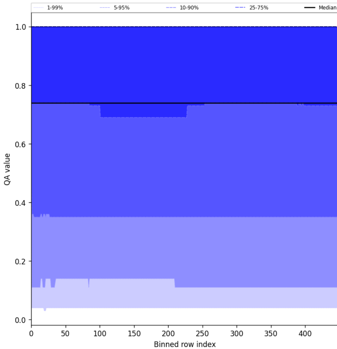
Figure 45: Along track statistics of “QA value” for 2025-06-13 to 2025-06-15
