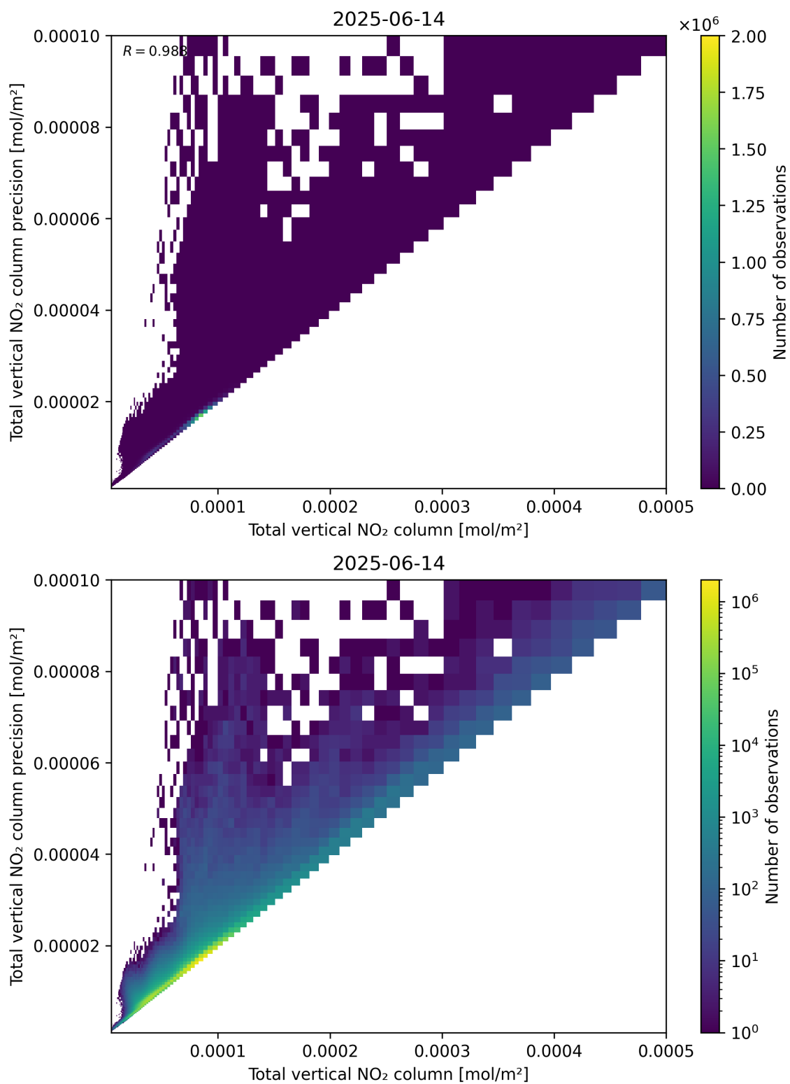
Figure 114: Scatter density plot of “Total vertical NO 2 column” against “Total vertical NO 2 column precision” for 2025-06-13 to 2025-06-15.
