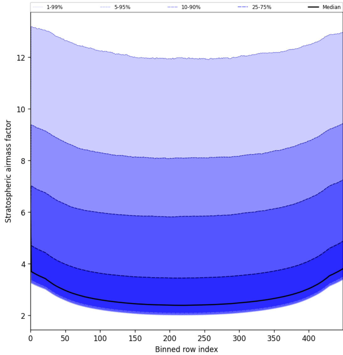
Figure 61: Along track statistics of “Stratospheric airmass factor” for 2025-06-13 to 2025-06-15
