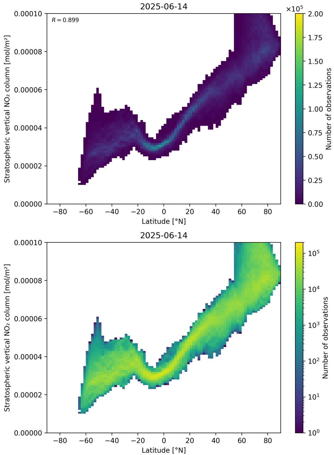
Figure 87: Scatter density plot of “Latitude” against “Stratospheric vertical NO 2 column” for 2025-06-13 to 2025-06-15.
