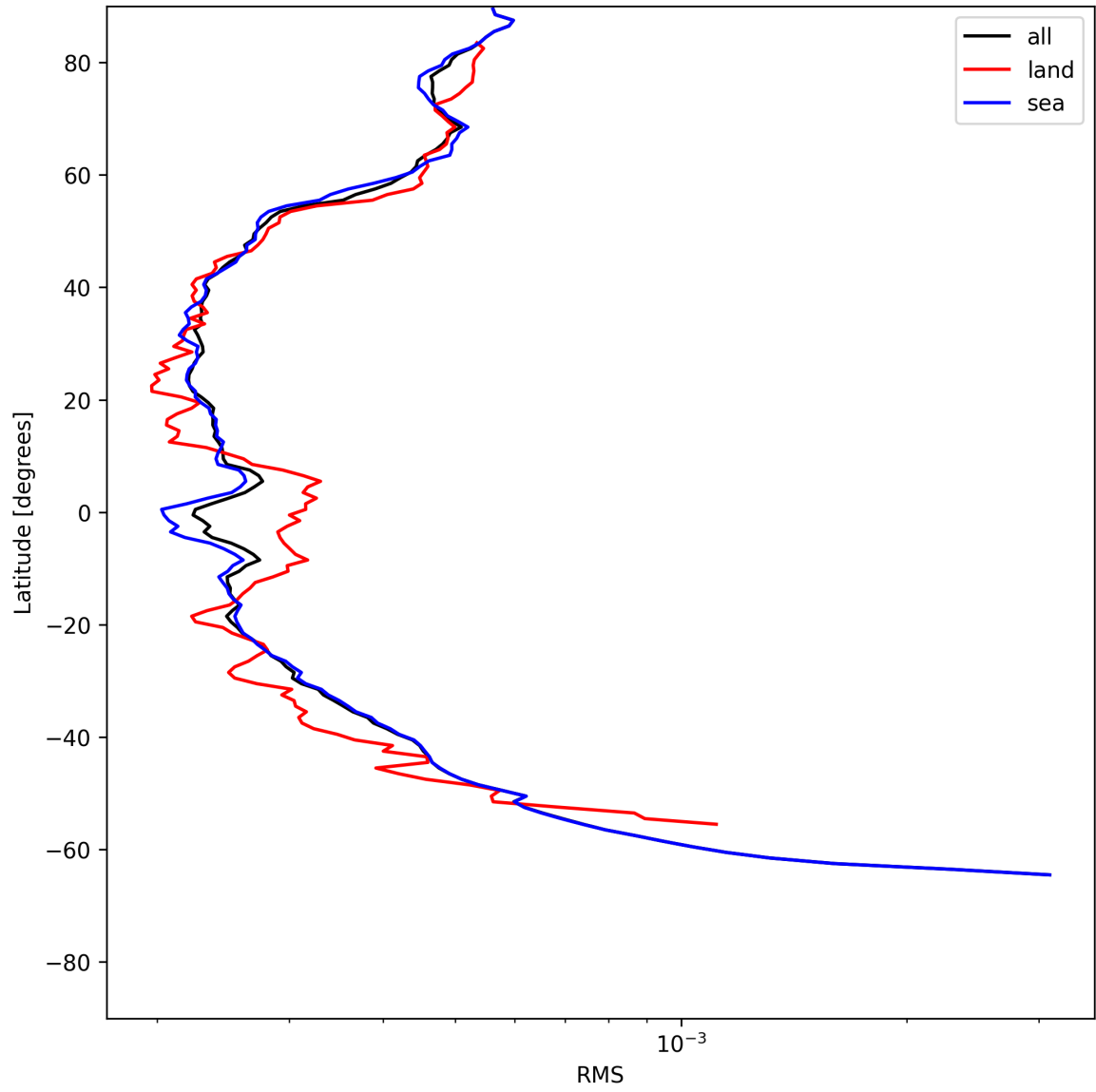
Figure 26: Zonal average of “RMS” for 2025-06-13 to 2025-06-15.
