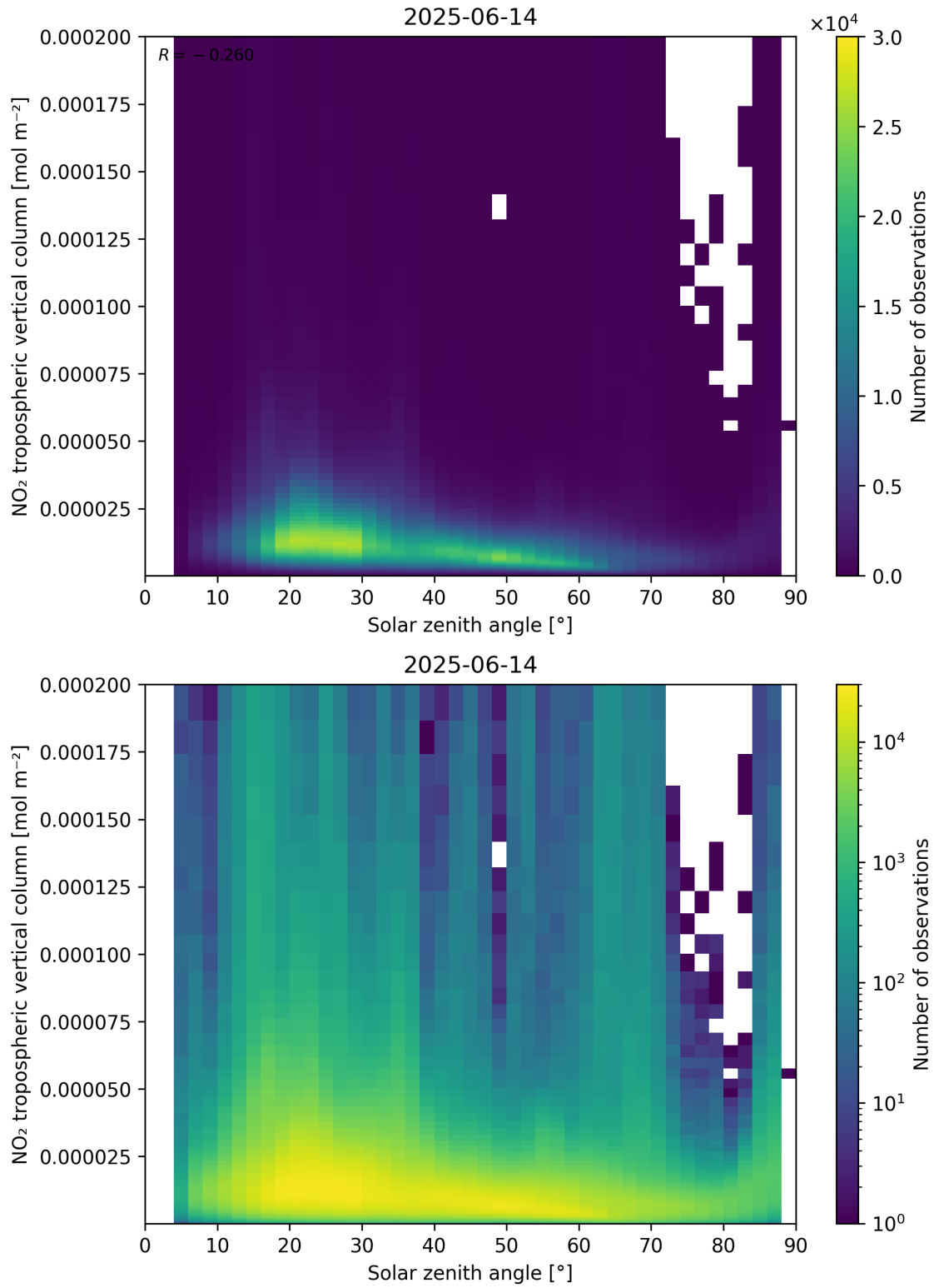
Figure 155: Scatter density plot of “Solar zenith angle” against “NO 2 tropospheric vertical column” for 2025-06-13 to 2025-06-15.
