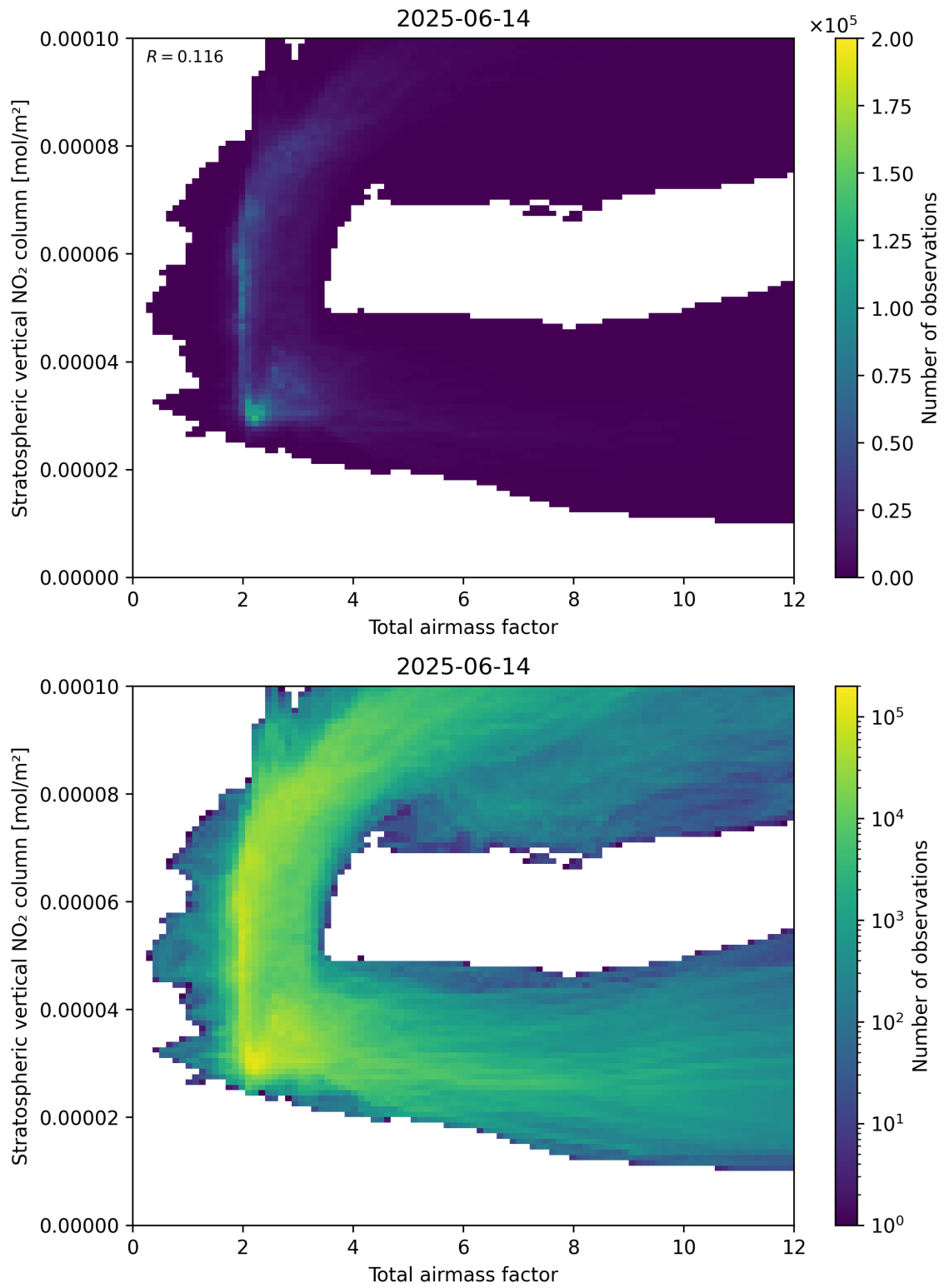
Figure 64: Scatter density plot of “Total airmass factor” against “Stratospheric vertical NO 2 column” for 2025-06-13 to 2025-06-15.
