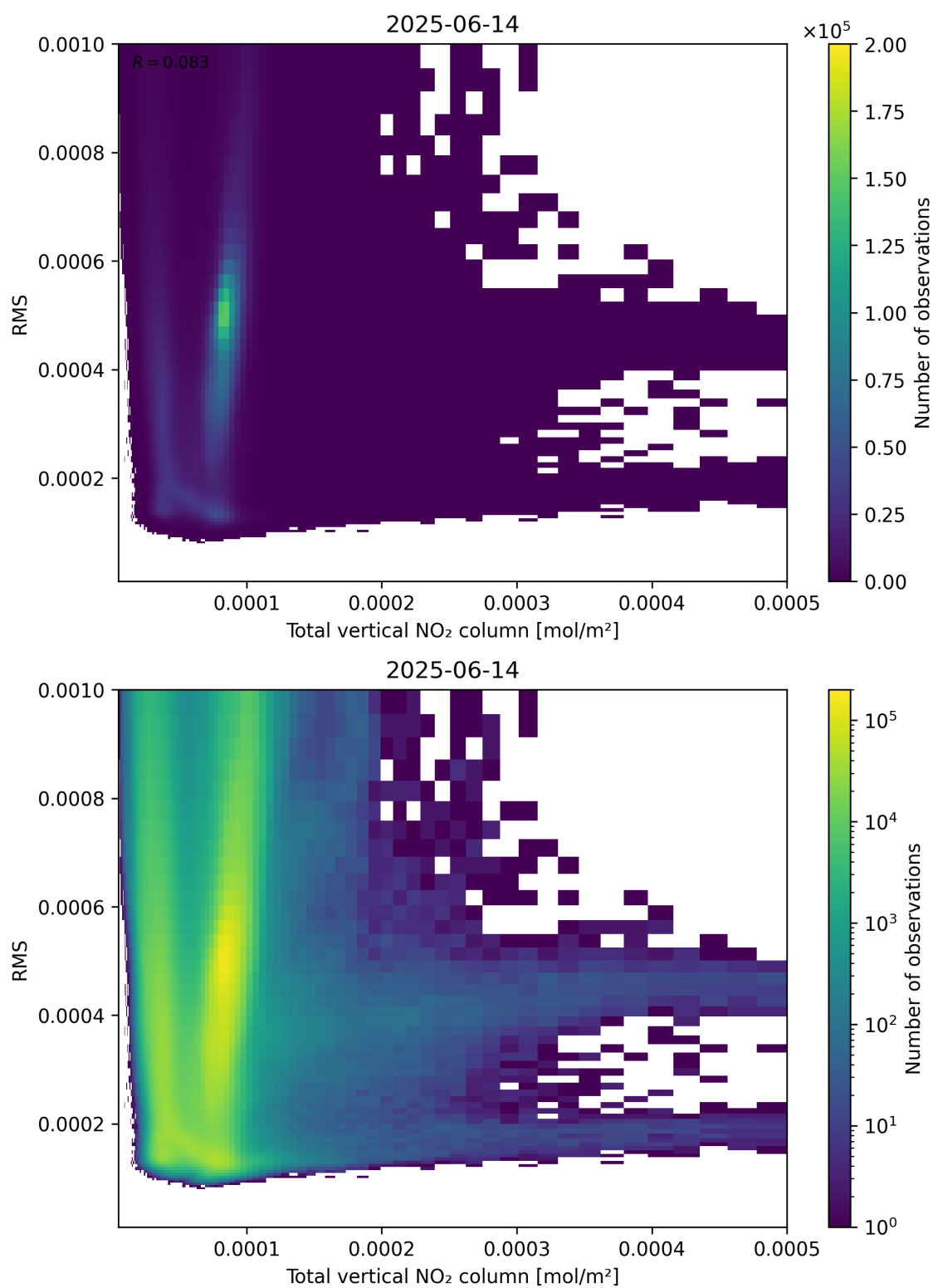
Figure 120: Scatter density plot of “Total vertical NO 2 column” against “RMS” for 2025-06-13 to 2025-06-15.
