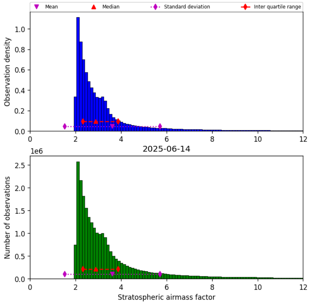
Figure 44: Histogram of “Stratospheric airmass factor” for 2025-06-13 to 2025-06-15
