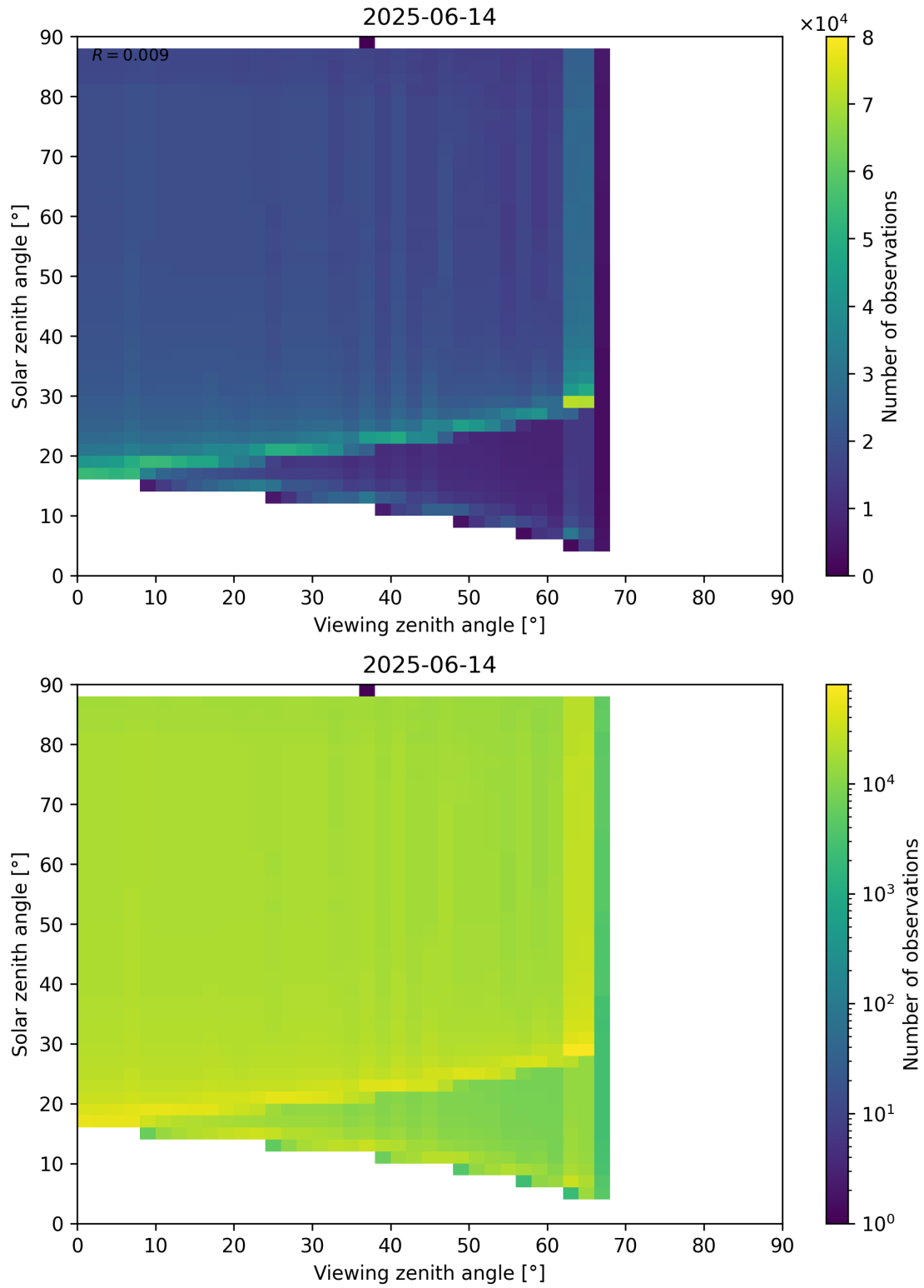
Figure 172: Scatter density plot of “Viewing zenith angle” against “Solar zenith angle” for 2025-06-13 to 2025-06-15.
