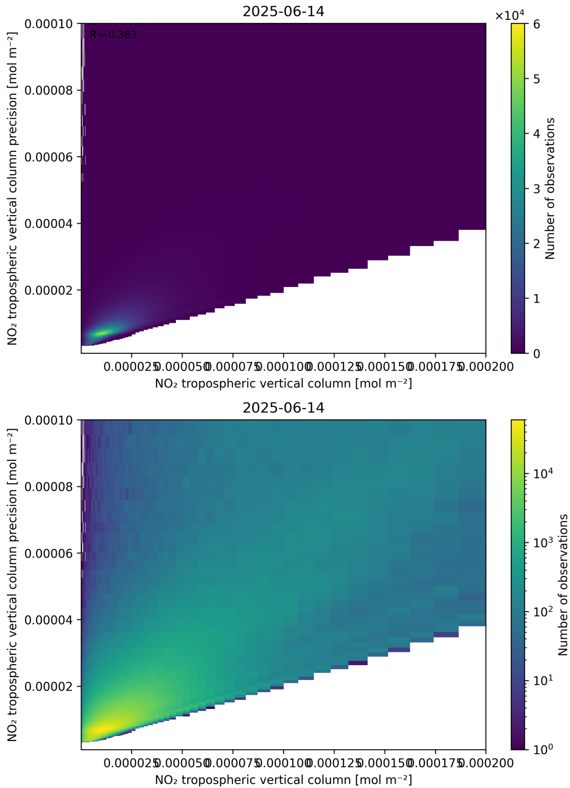
Figure 130: Scatter density plot of “NO 2 tropospheric vertical column” against “NO 2 tropospheric vertical column precision” for 2025-06-13 to 2025-06-15.
