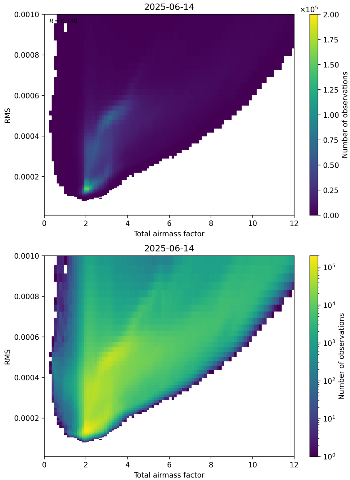
Figure 69: Scatter density plot of “Total airmass factor” against “RMS” for 2025-06-13 to 2025-06-15.
