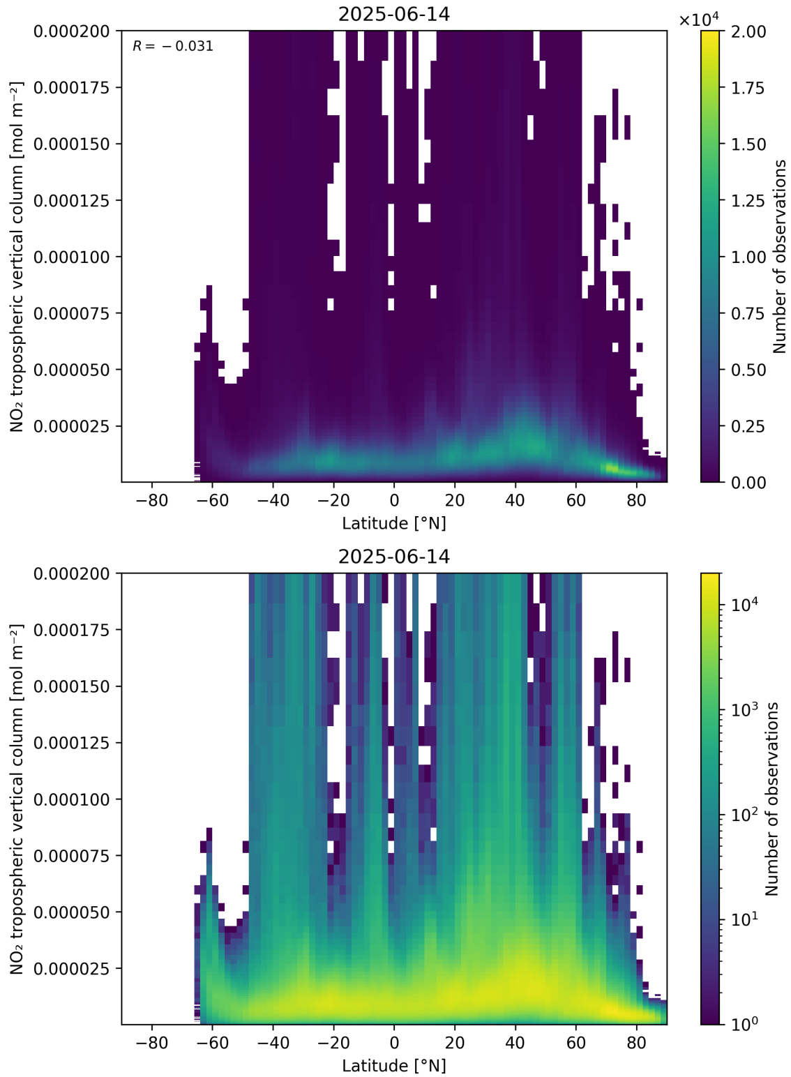
Figure 92: Scatter density plot of “Latitude” against “NO 2 tropospheric vertical column” for 2025-06-13 to 2025-06-15.
