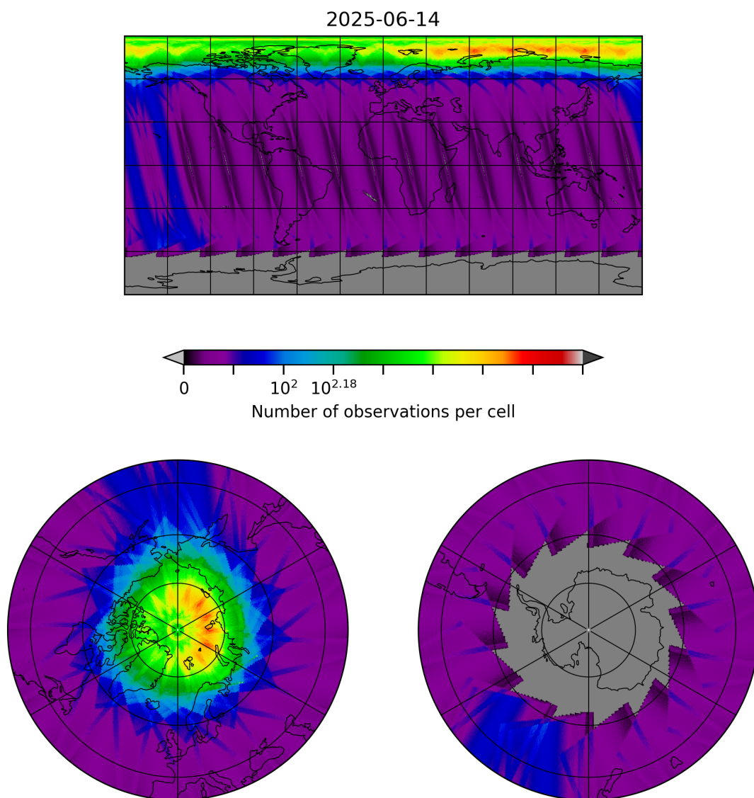
Figure 10: Map of the number of observations for 2025-06-13 to 2025-06-15
