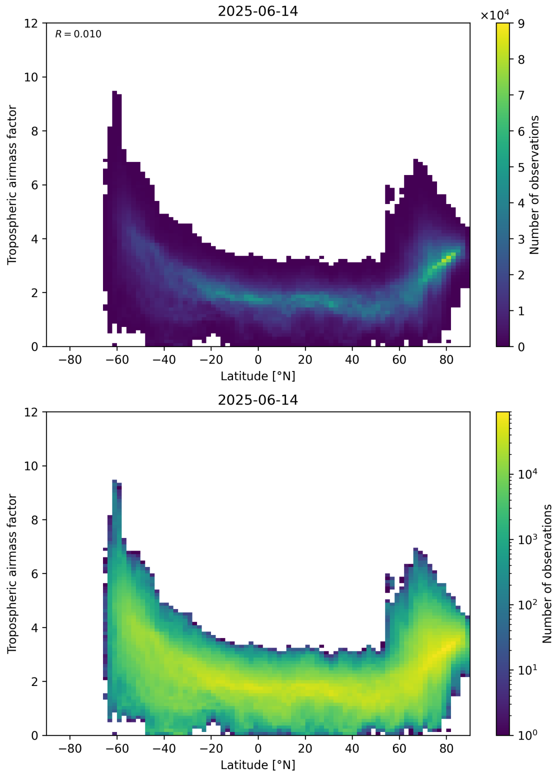
Figure 85: Scatter density plot of “Latitude” against “Tropospheric air mass factor” for 2025-06-13 to 2025-06-15.
