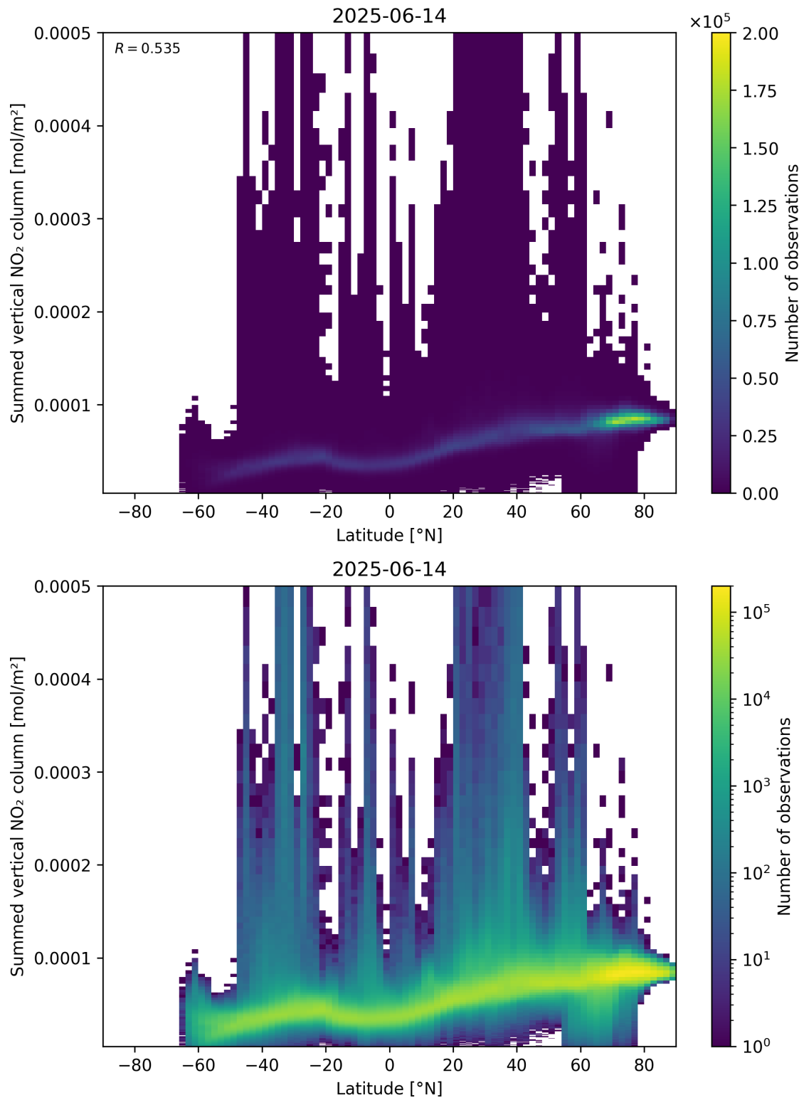
Figure 88: Scatter density plot of “Latitude” against “Summed vertical NO 2 column” for 2025-06-13 to 2025-06-15.
