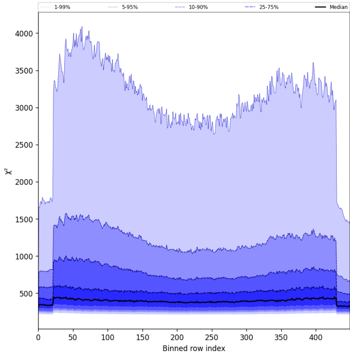
Figure 59: Along track statistics of “ \chi^2 ” for 2025-06-13 to 2025-06-15
