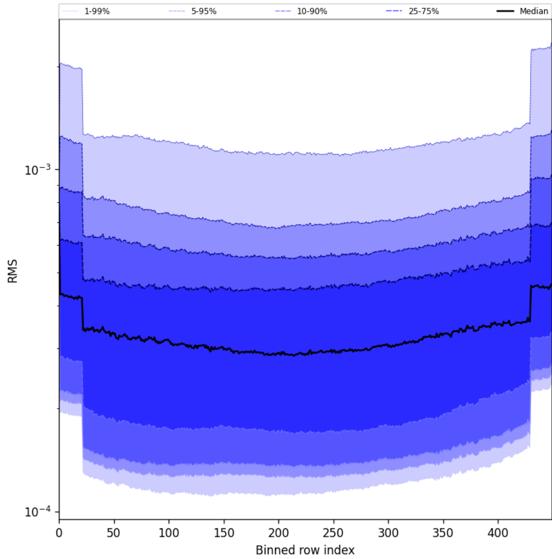
Figure 60: Along track statistics of “RMS” for 2025-06-13 to 2025-06-15
