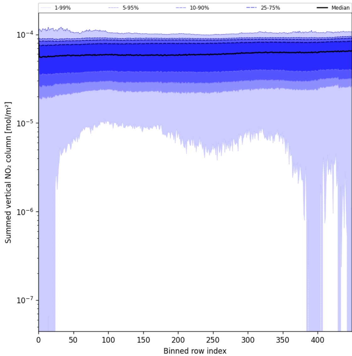
Figure 57: Along track statistics of “Summed vertical NO 2 column” for 2025-06-13 to 2025-06-15
