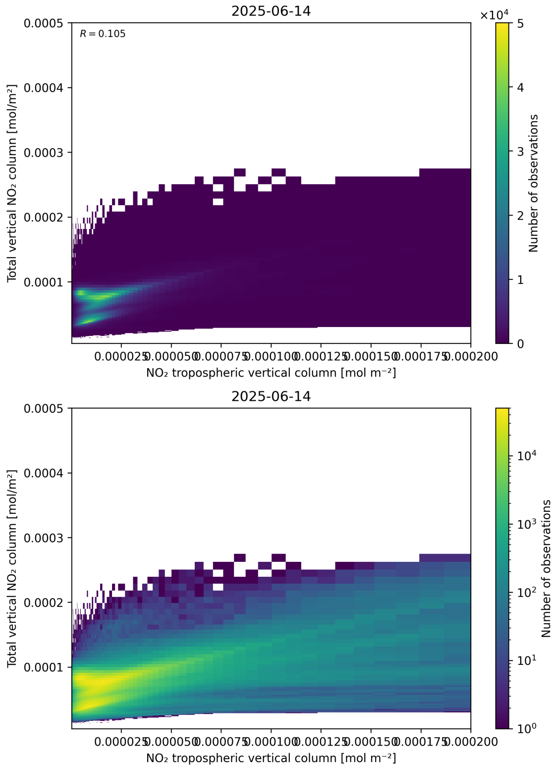
Figure 128: Scatter density plot of “NO 2 tropospheric vertical column” against “Total vertical NO 2 column” for 2025-06-13 to 2025-06-15.
