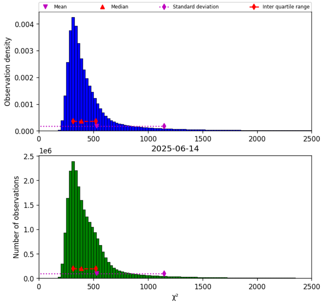
Figure 42: Histogram of “ \chi^2 ” for 2025-06-13 to 2025-06-15
