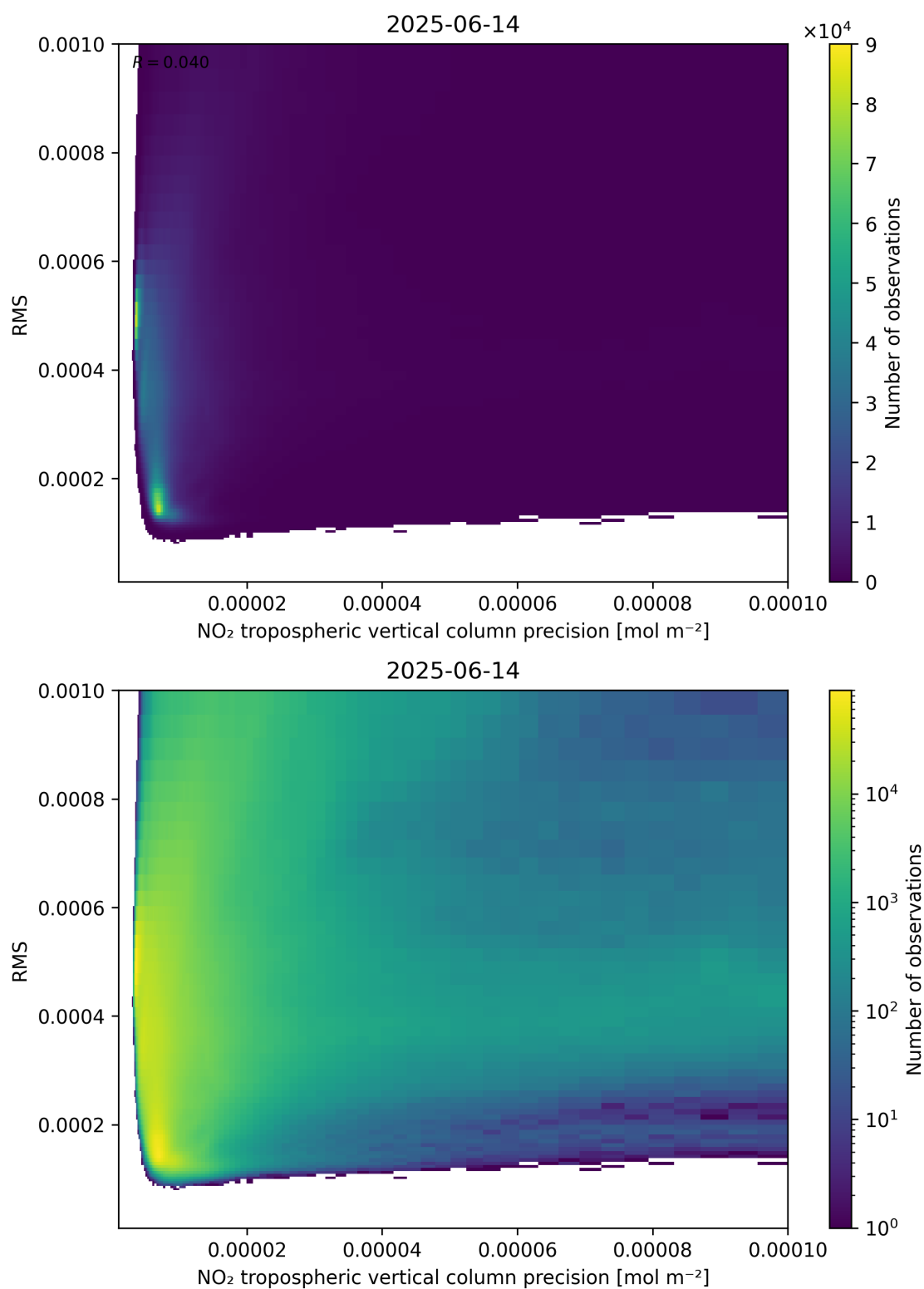
Figure 140: Scatter density plot of “NO 2 tropospheric vertical column precision” against “RMS” for 2025-06-13 to 2025-06-15.
