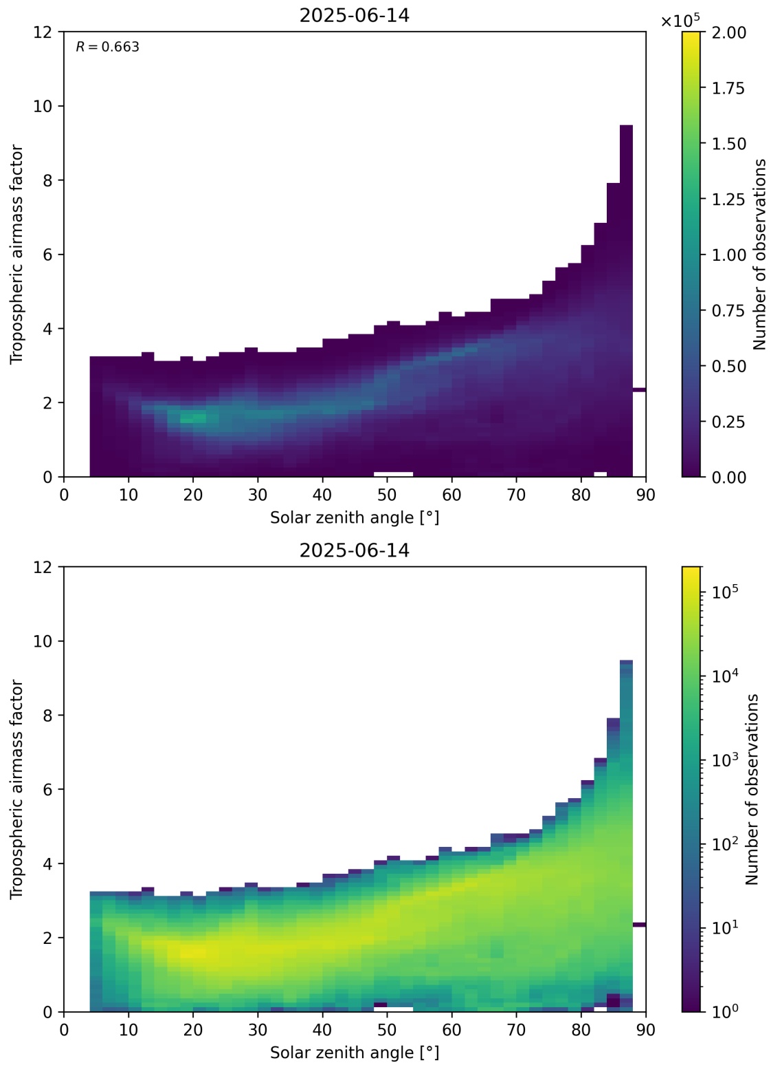
Figure 147: Scatter density plot of “Solar zenith angle” against “Tropospheric airmass factor” for 2025-06-13 to 2025-06-15.
