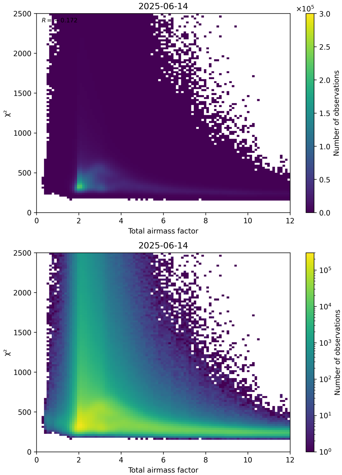
Figure 63: Scatter density plot of “Total airmass factor” against “ \chi^2 ” for 2025-06-13 to 2025-06-15.
