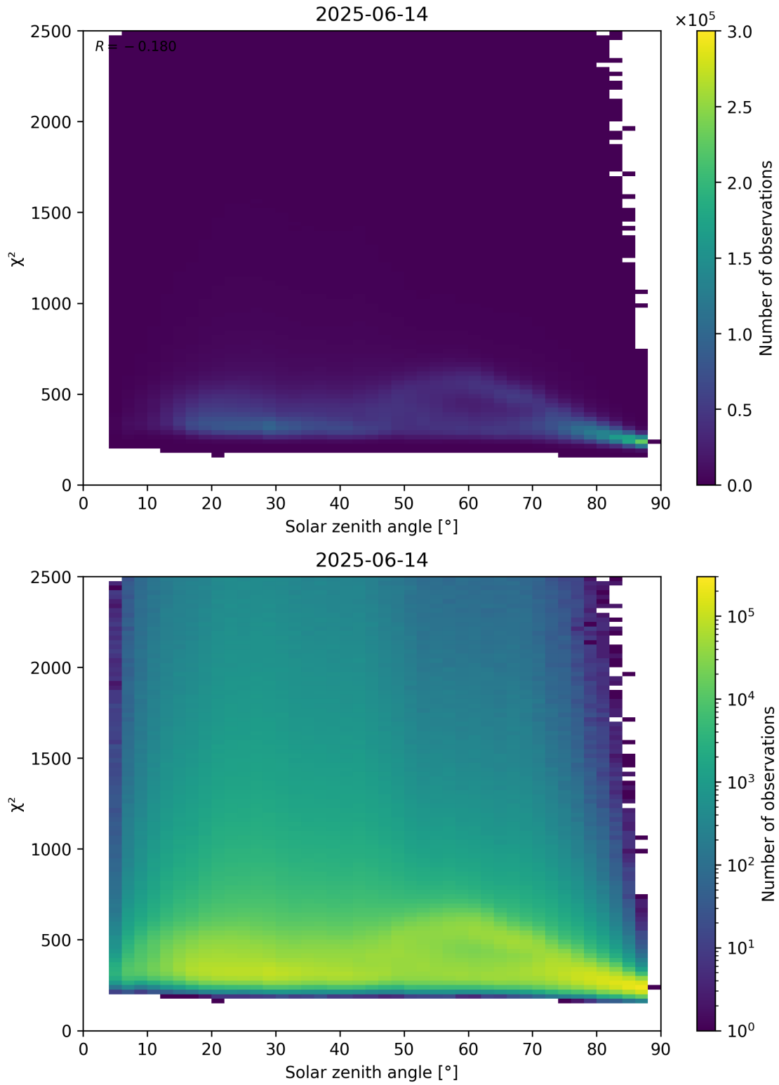
Figure 148: Scatter density plot of “Solar zenith angle” against “ \chi^2 ” for 2025-06-13 to 2025-06-15.
