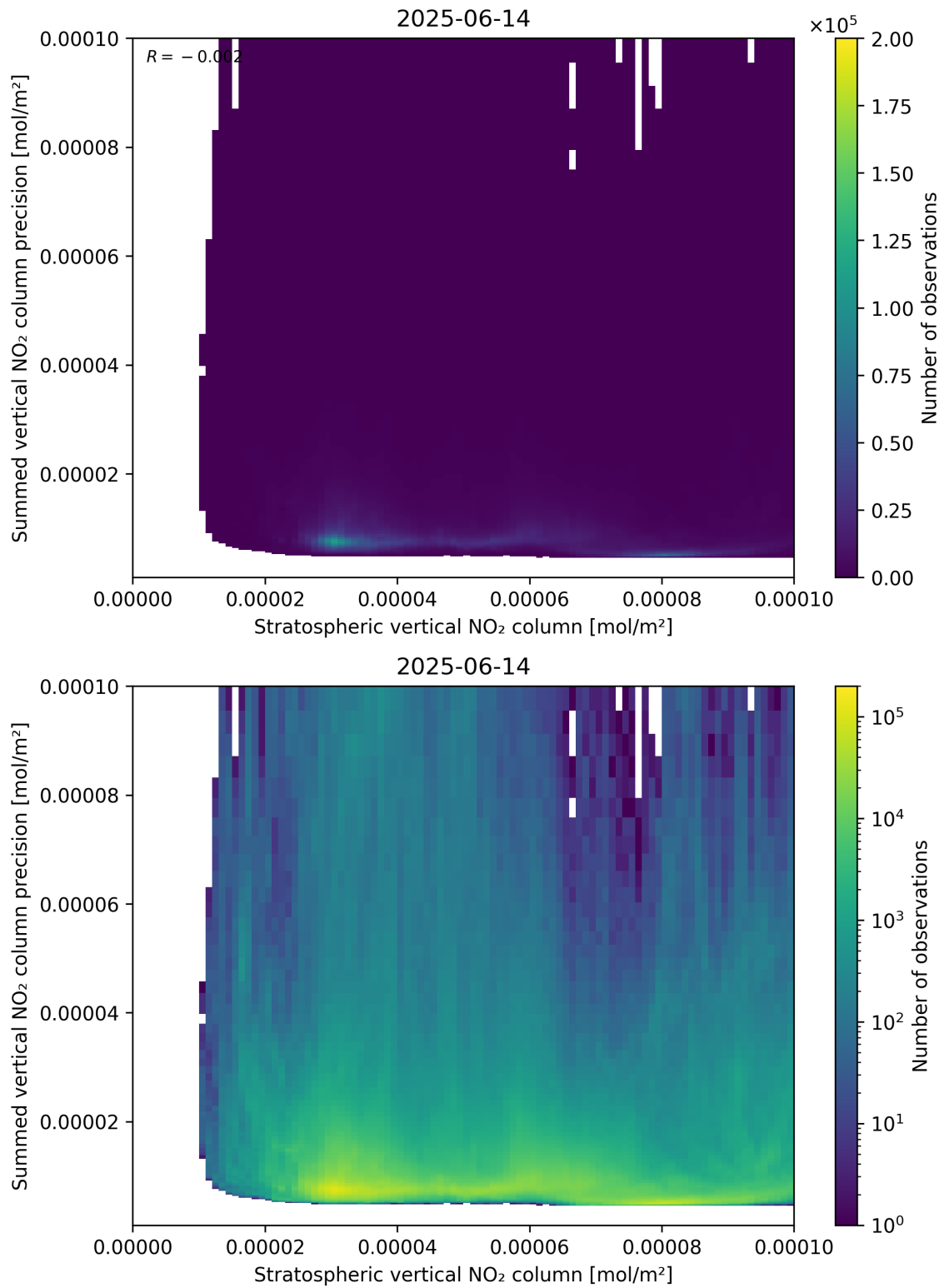
Figure 99: Scatter density plot of “Stratospheric vertical NO 2 column” against “Summed vertical NO 2 column precision” for 2025-06-13 to 2025-06-15.
