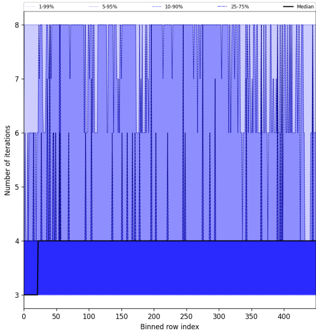
Figure 51: Along track statistics of “Number of iterations” for 2025-06-13 to 2025-06-15
