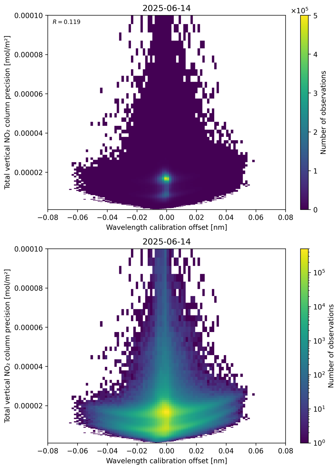
Figure 180: Scatter density plot of “Wavelength calibration offset” against “Total vertical NO 2 column precision” for 2025-06-13 to 2025-06-15.
