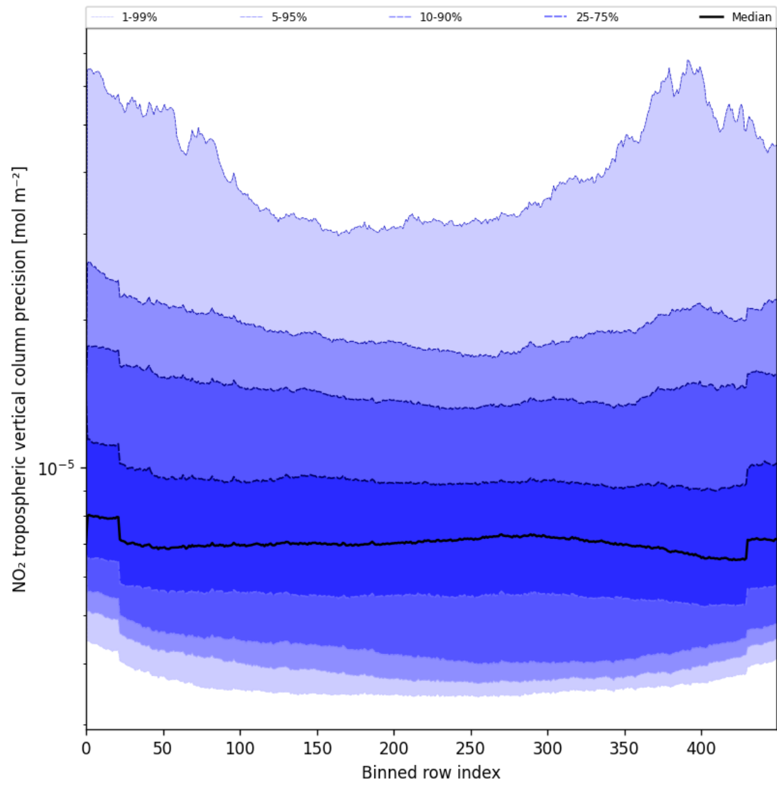
Figure 47: Along track statistics of “NO 2 tropospheric vertical column precision” for 2025-06-13 to 2025-06-15
