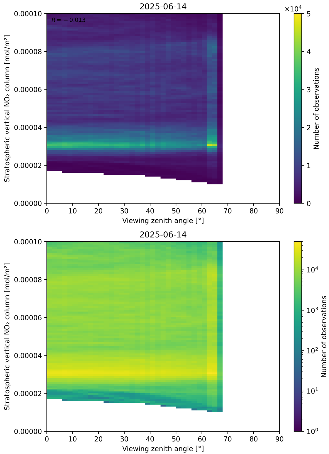
Figure 164: Scatter density plot of “Viewing zenith angle” against “Stratospheric vertical NO 2 column” for 2025-06-13 to 2025-06-15.
