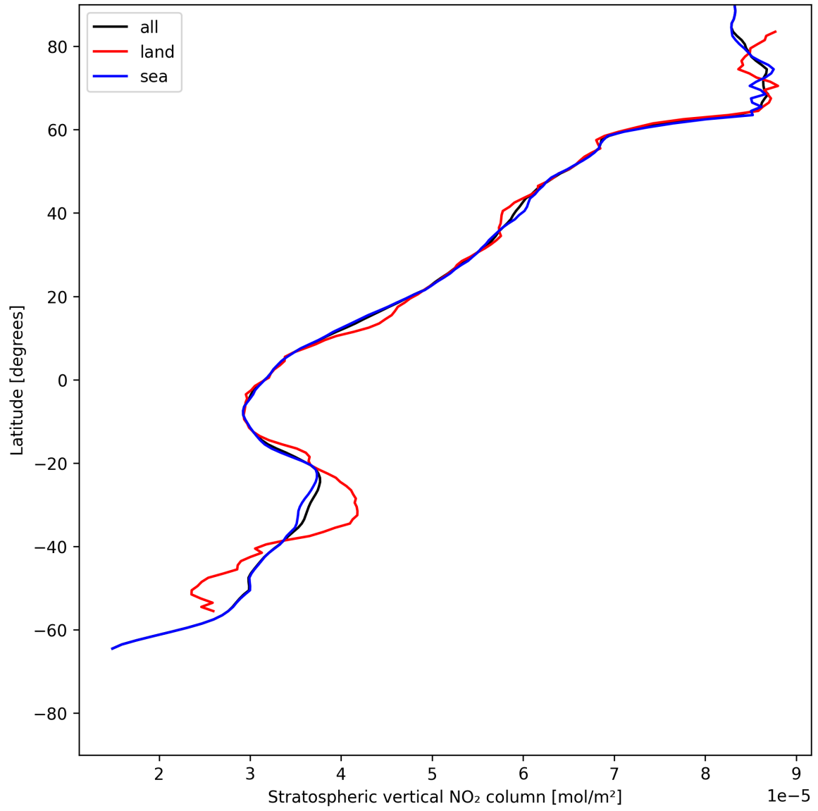
Figure 19: Zonal average of “Stratospheric vertical NO 2 column” for 2025-06-13 to 2025-06-15.
