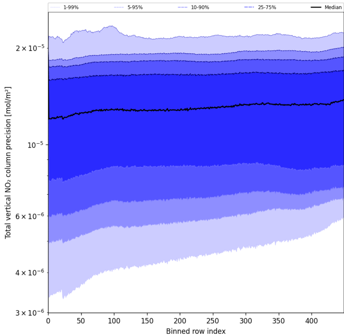
Figure 56: Along track statistics of "Total vertical NO 2 column precision" for 2025-06-13 to 2025-06-15
