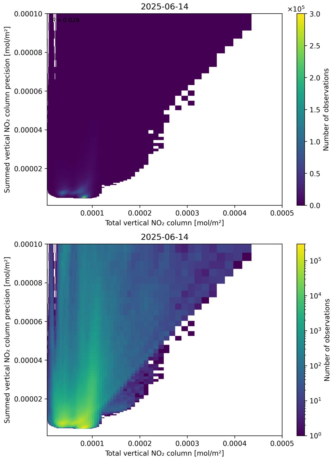
Figure 113: Scatter density plot of “Total vertical NO 2 column” against “Summed vertical NO 2 column precision” for 2025-06-13 to 2025-06-15.
