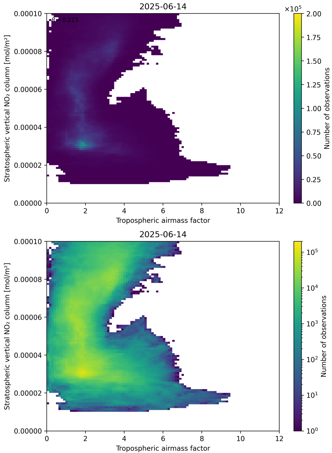
Figure 74: Scatter density plot of “Tropospheric air mass factor” against “Stratospheric vertical NO 2 column” for 2025-06-13 to 2025-06-15.
