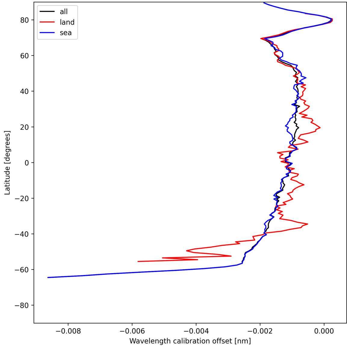
Figure 18: Zonal average of “Wavelength calibration offset” for 2025-06-13 to 2025-06-15.
