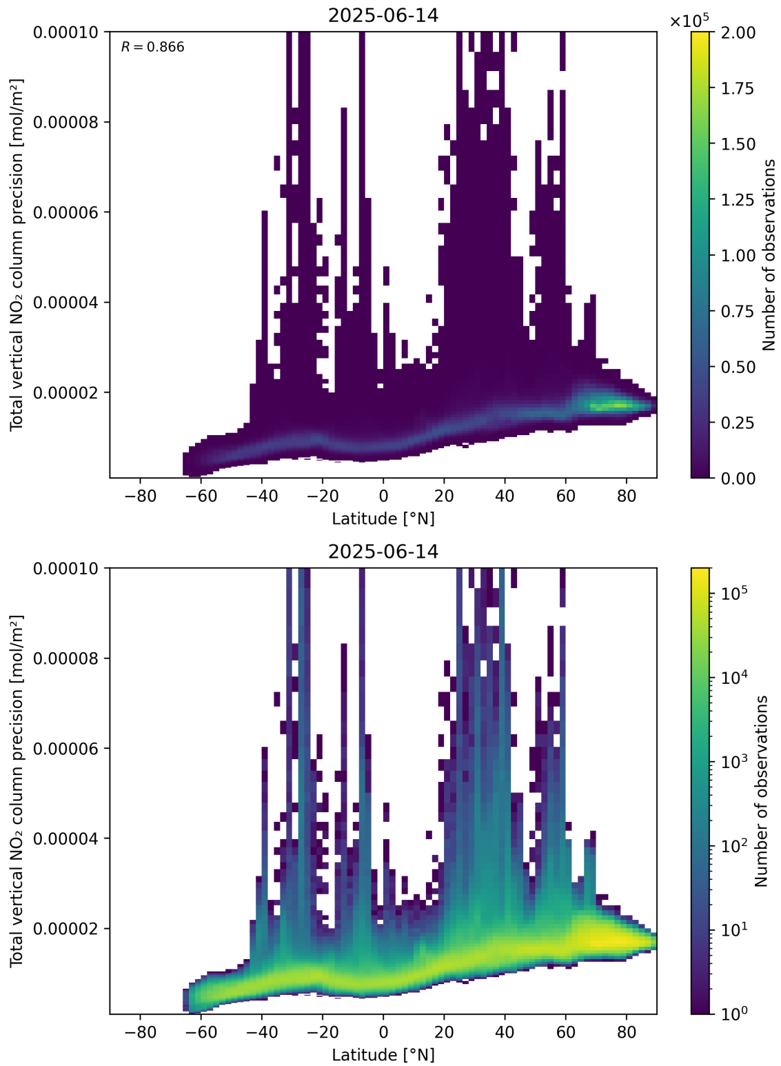
Figure 91: Scatter density plot of “Latitude” against “Total vertical NO 2 column precision” for 2025-06-13 to 2025-06-15.
