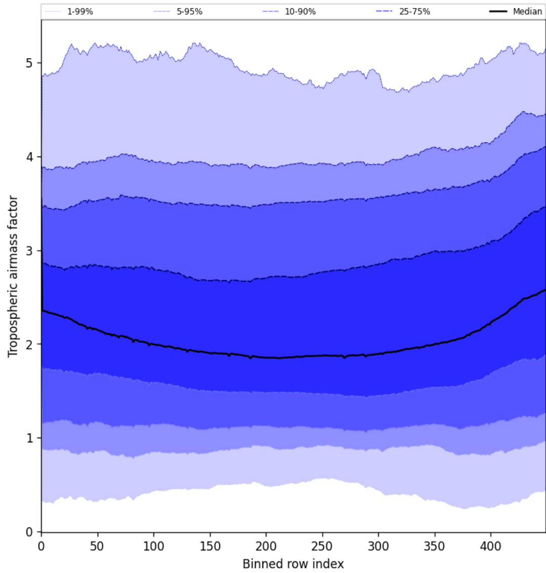
Figure 48: Along track statistics of “Tropospheric airmass factor” for 2025-06-13 to 2025-06-15
