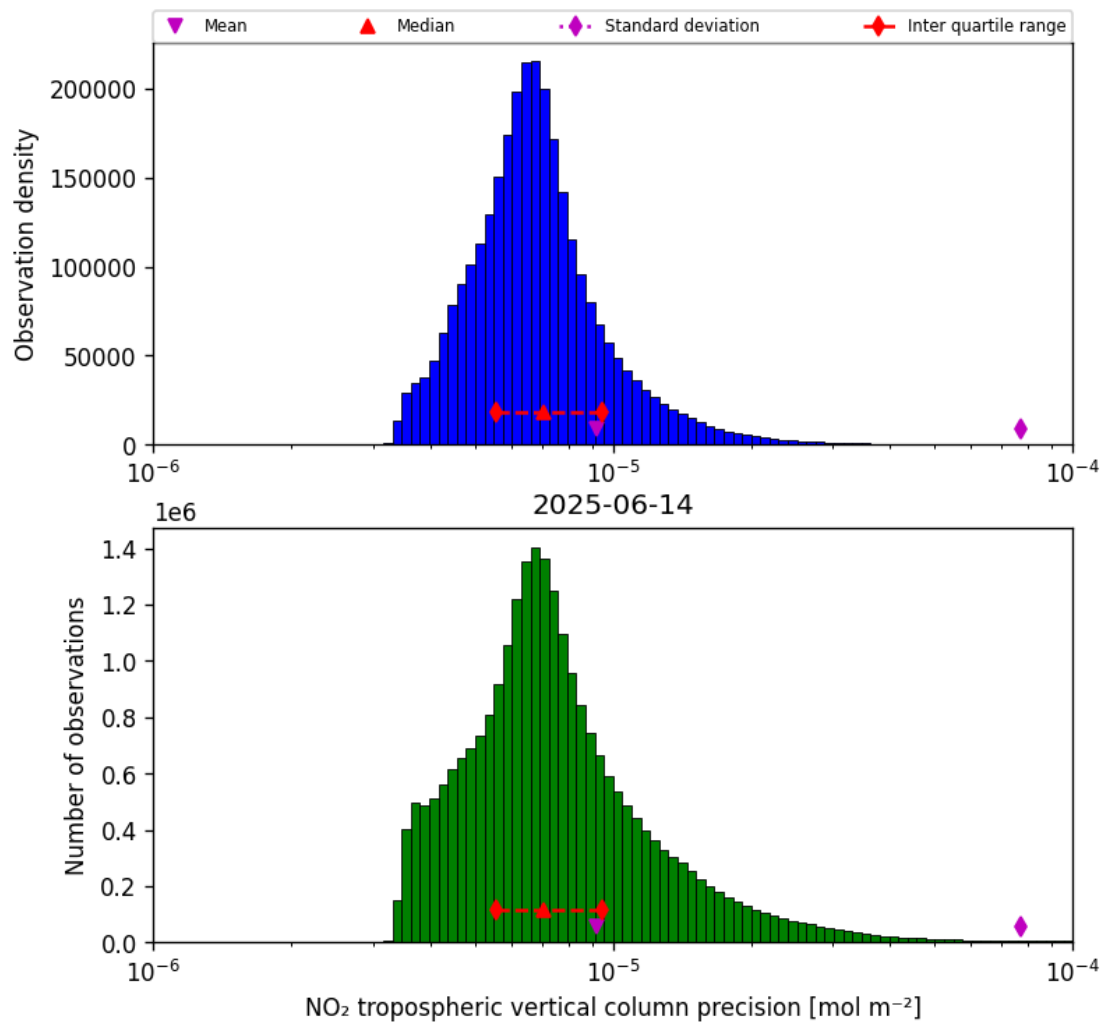
Figure 30: Histogram of “NO 2 tropospheric vertical column precision” for 2025-06-13 to 2025-06-15
