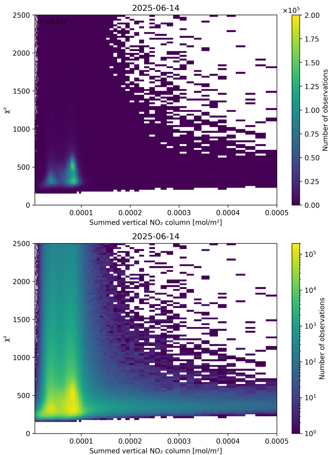
Figure 104: Scatter density plot of “Summed vertical NO 2 column” against “ \chi^2 ” for 2025-06-13 to 2025-06-15.
