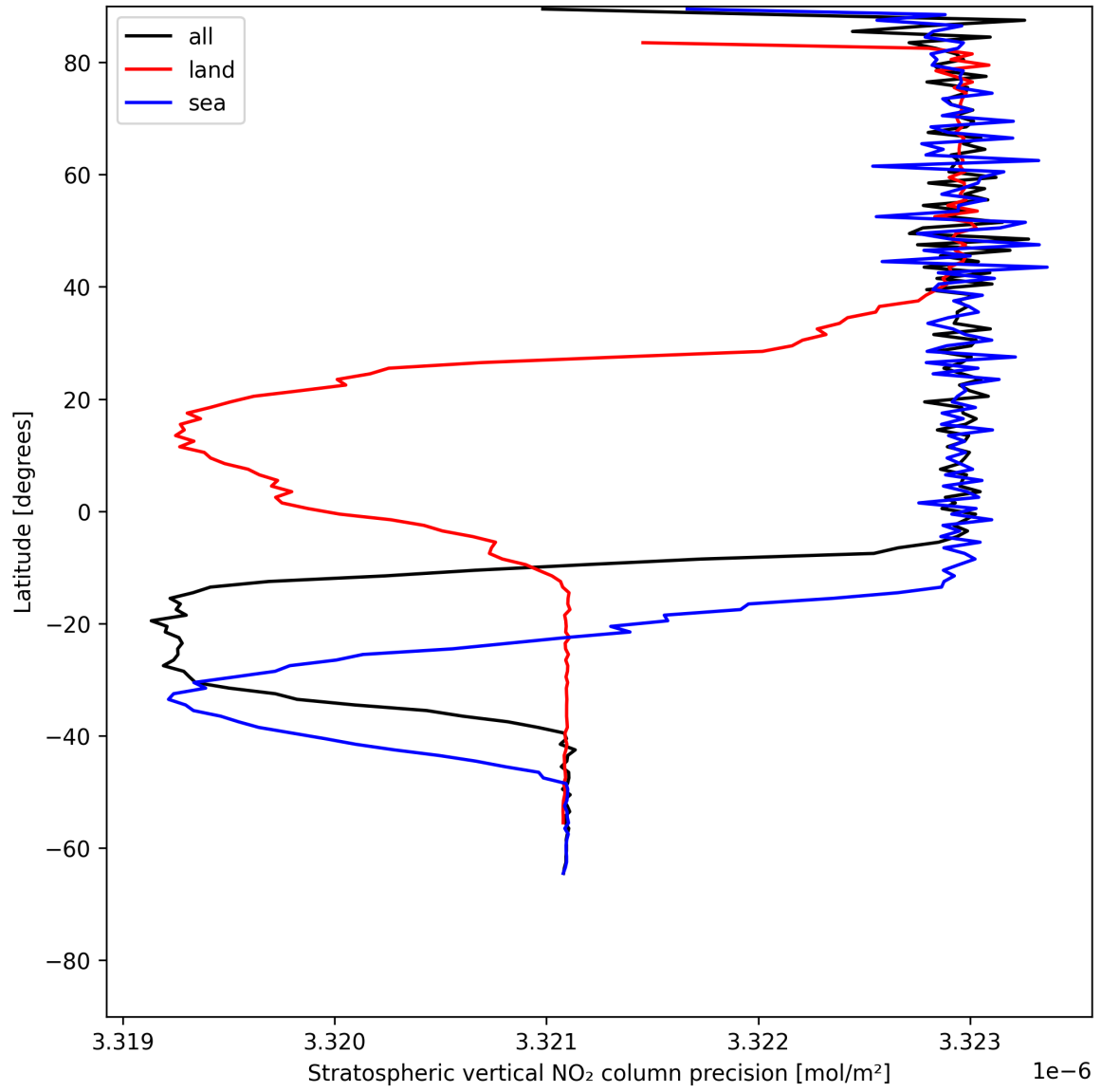
Figure 20: Zonal average of “Stratospheric vertical NO 2 column precision” for 2025-06-13 to 2025-06-15.
