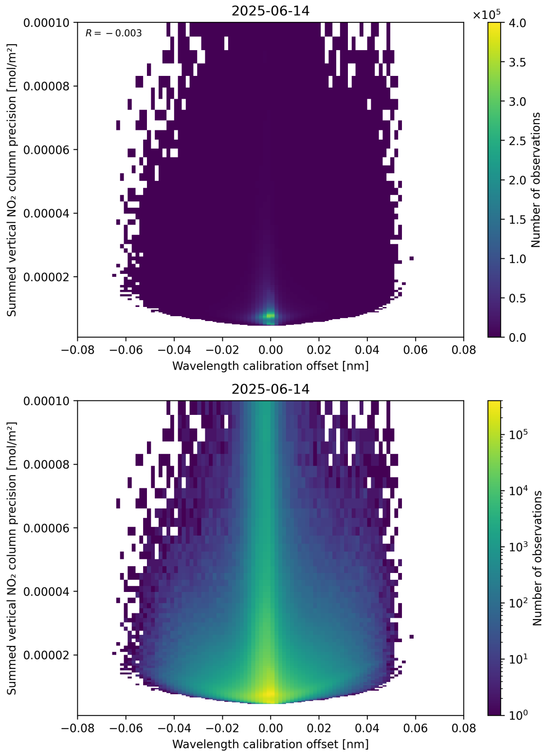
Figure 178: Scatter density plot of “Wavelength calibration offset” against “Summed vertical NO 2 column precision” for 2025-06-13 to 2025-06-15.
