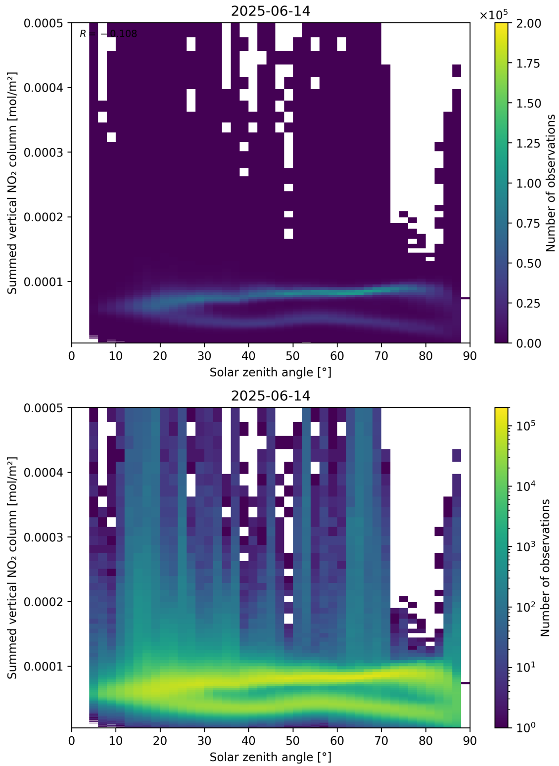
Figure 151: Scatter density plot of “Solar zenith angle” against “Summed vertical NO 2 column” for 2025-06-13 to 2025-06-15.
