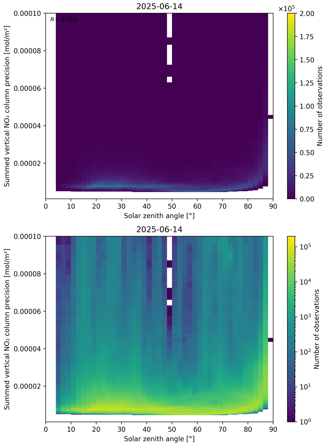
Figure 152: Scatter density plot of “Solar zenith angle” against “Summed vertical NO 2 column precision” for 2025-06-13 to 2025-06-15.
