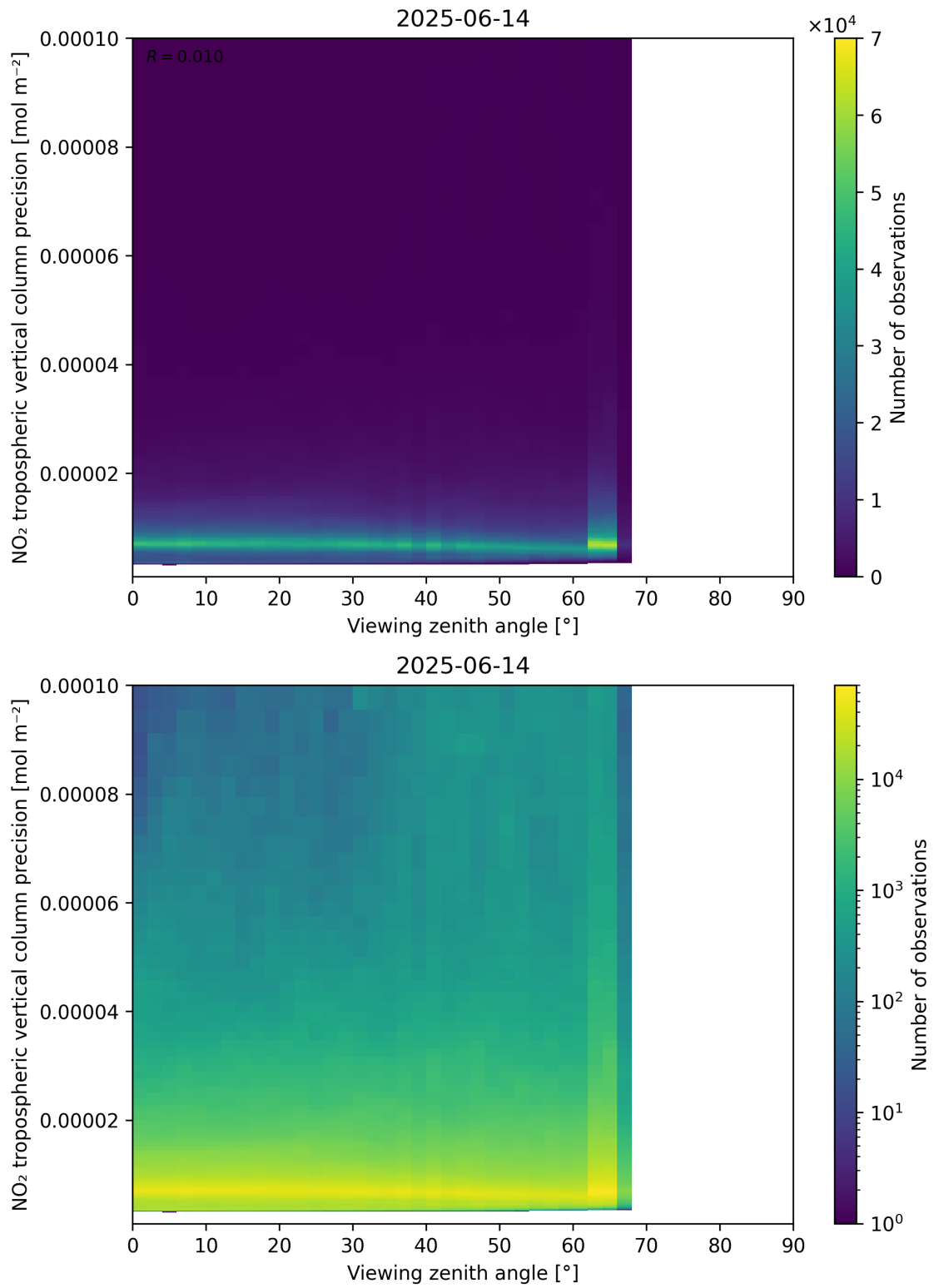
Figure 170: Scatter density plot of “Viewing zenith angle” against “NO 2 tropospheric vertical column precision” for 2025-06-13 to 2025-06-15.
