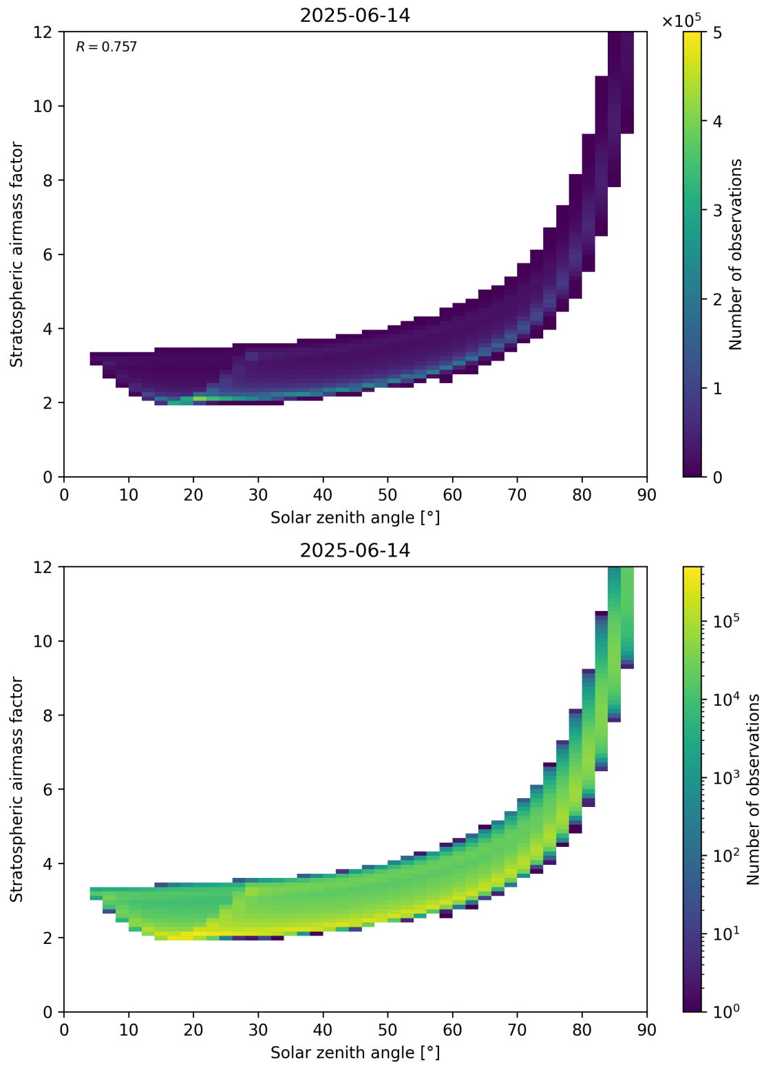
Figure 145: Scatter density plot of “Solar zenith angle” against “Stratospheric airmass factor” for 2025-06-13 to 2025-06-15.
