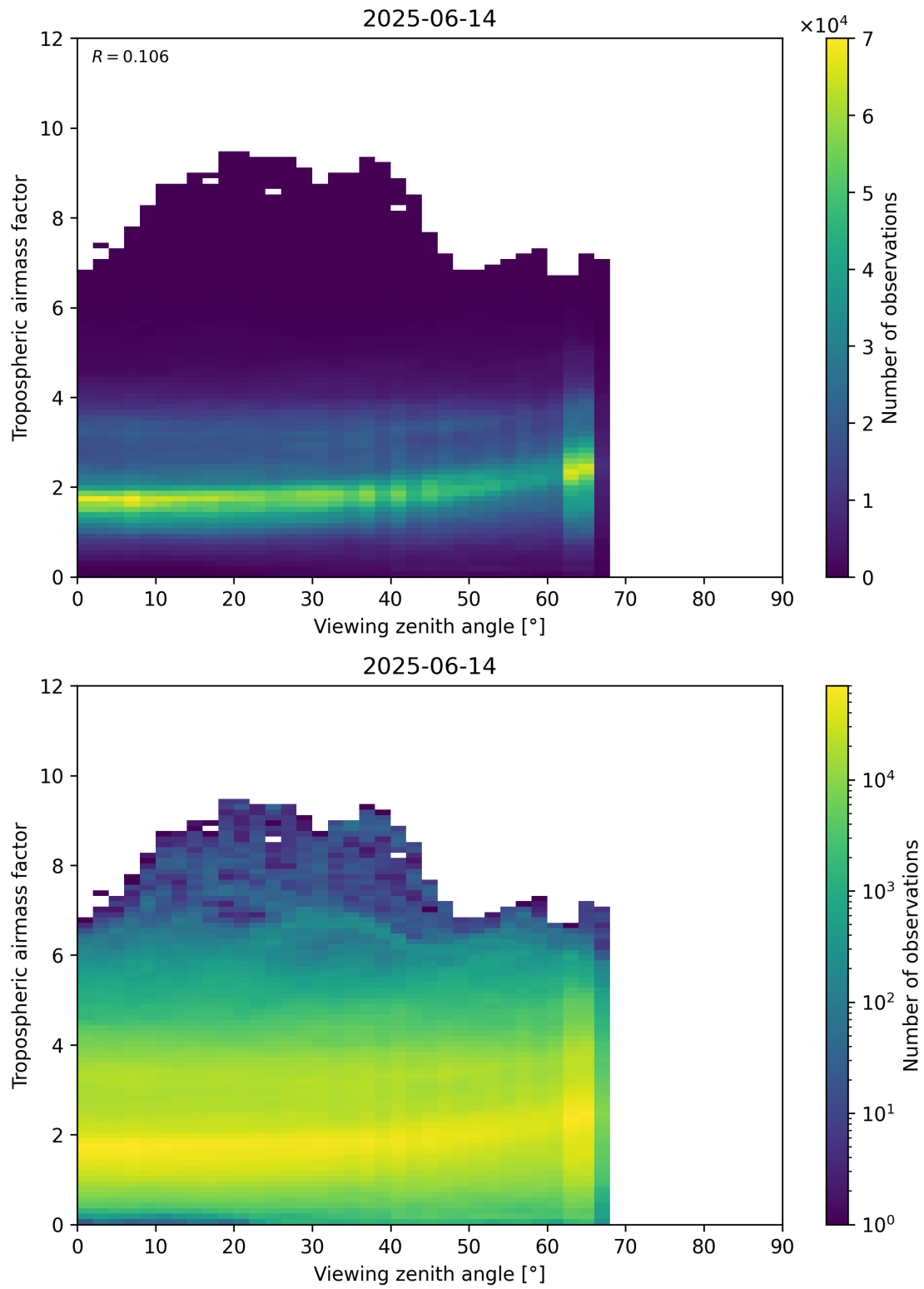
Figure 161: Scatter density plot of “Viewing zenith angle” against “Tropospheric airmass factor” for 2025-06-13 to 2025-06-15.
