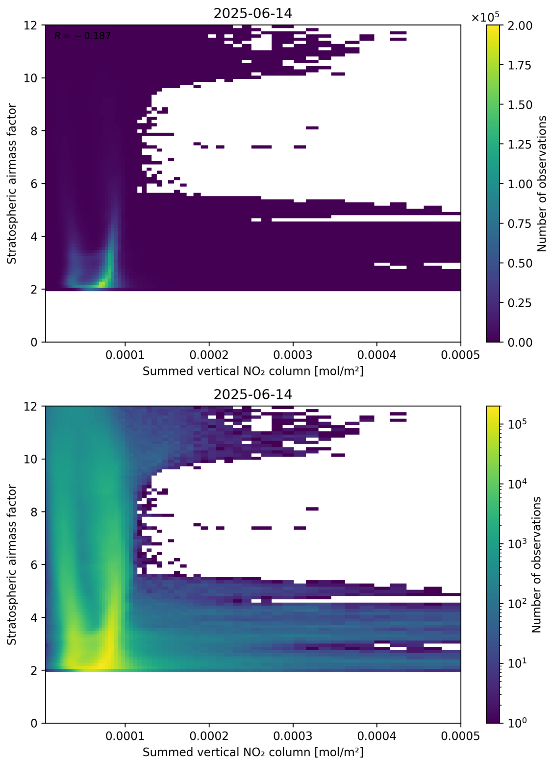
Figure 103: Scatter density plot of “Summed vertical NO 2 column” against “Stratospheric airmass factor” for 2025-06-13 to 2025-06-15.
