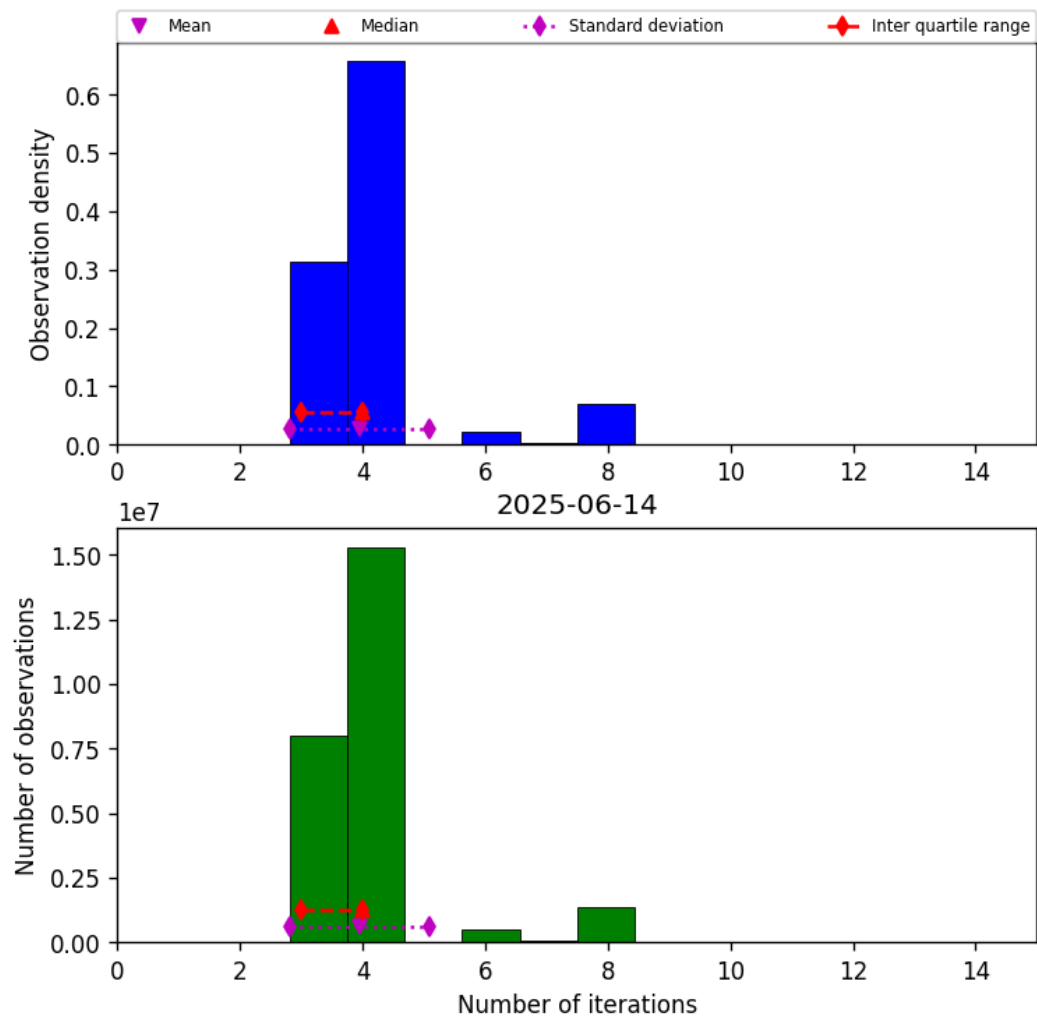
Figure 34: Histogram of “Number of iterations” for 2025-06-13 to 2025-06-15
