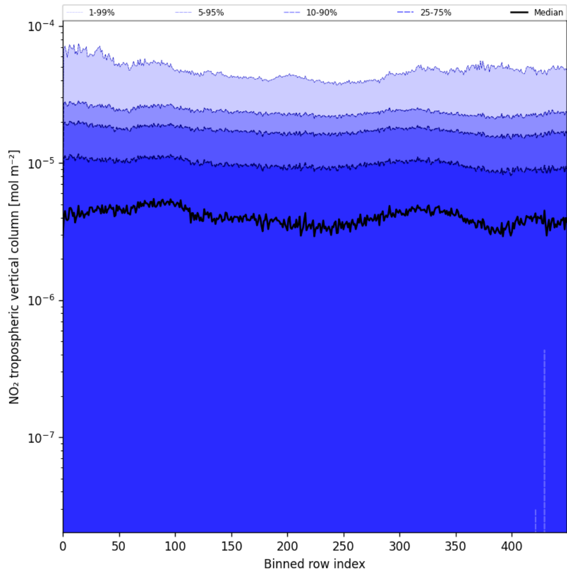
Figure 46: Along track statistics of “NO 2 tropospheric vertical column” for 2025-06-13 to 2025-06-15
