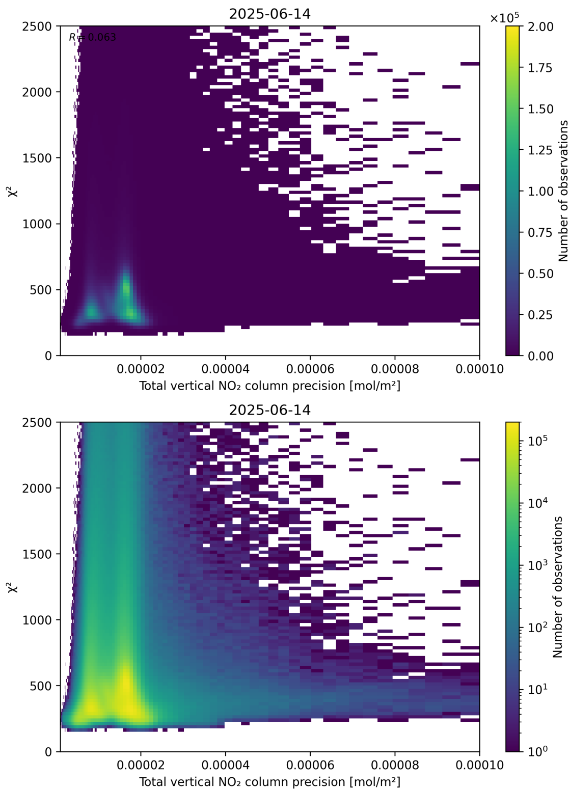
Figure 116: Scatter density plot of “Total vertical NO 2 column precision” against “ \chi^2 ” for 2025-06-13 to 2025-06-15.
