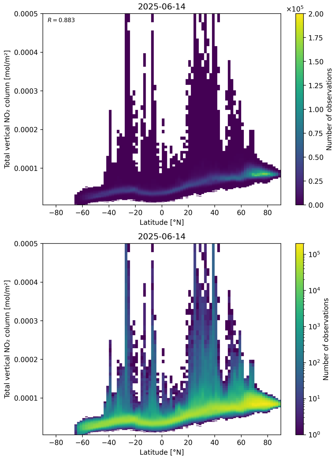
Figure 90: Scatter density plot of “Latitude” against “Total vertical NO 2 column” for 2025-06-13 to 2025-06-15.
