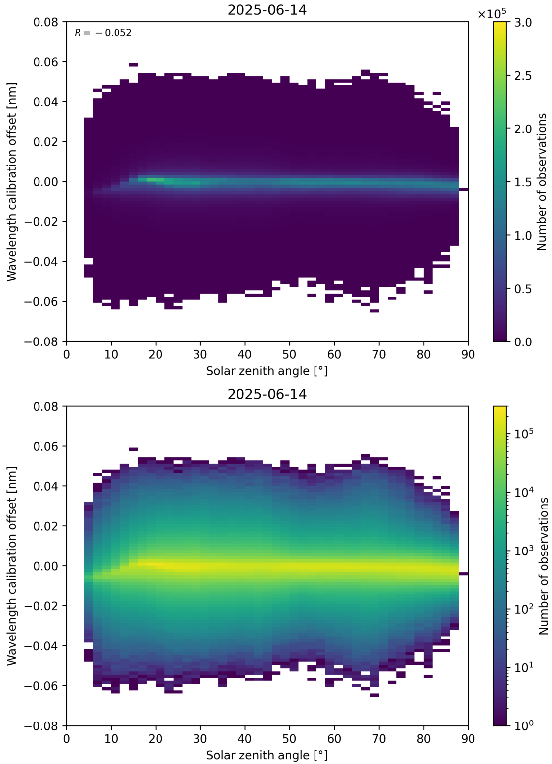
Figure 158: Scatter density plot of “Solar zenith angle” against “Wavelength calibration offset” for 2025-06-13 to 2025-06-15.
