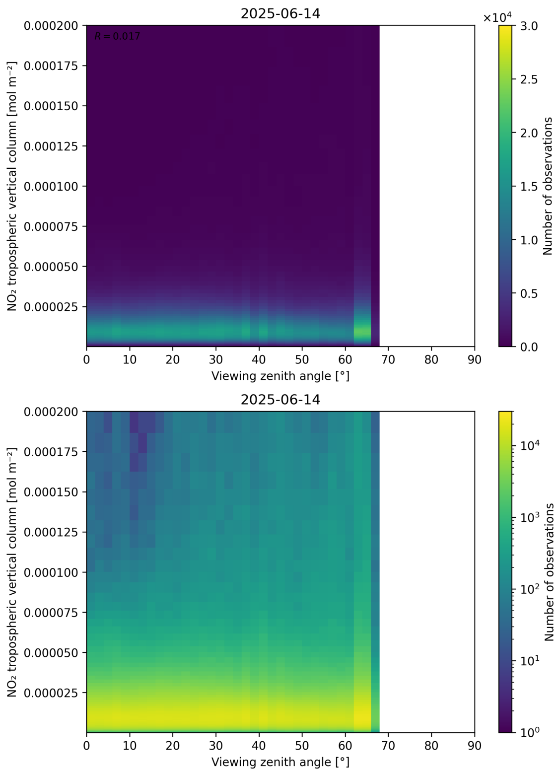
Figure 169: Scatter density plot of “Viewing zenith angle” against “NO 2 tropospheric vertical column” for 2025-06-13 to 2025-06-15.
