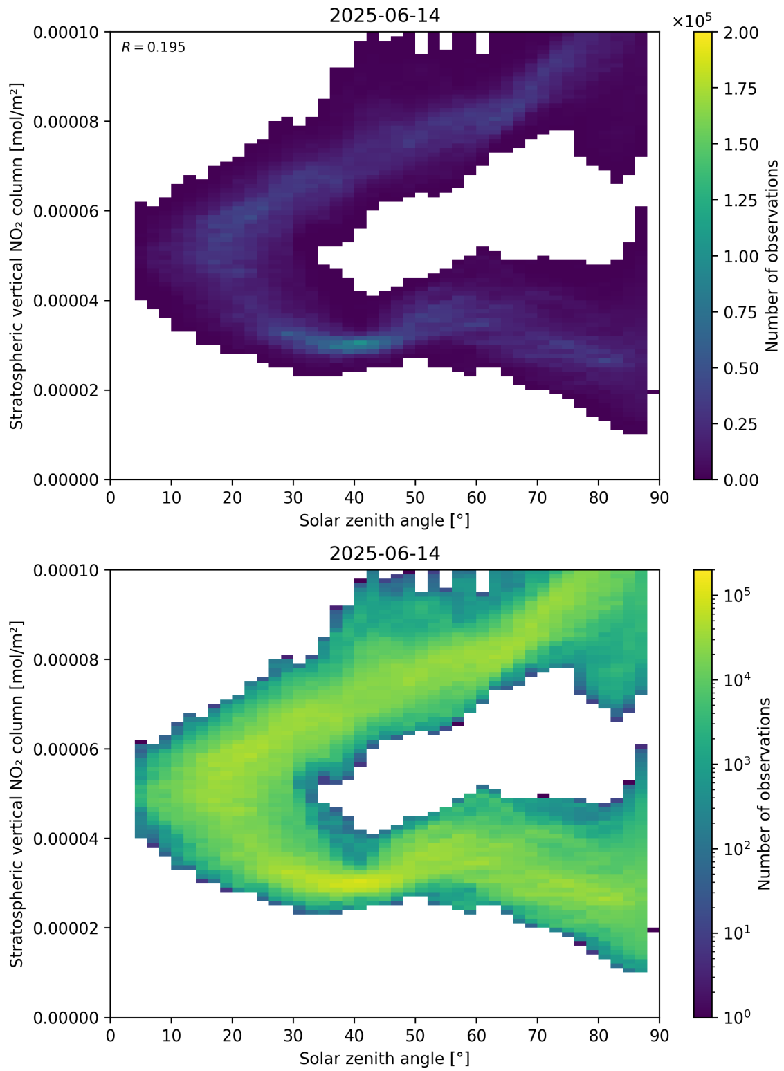
Figure 150: Scatter density plot of “Solar zenith angle” against “Stratospheric vertical NO 2 column” for 2025-06-13 to 2025-06-15.
