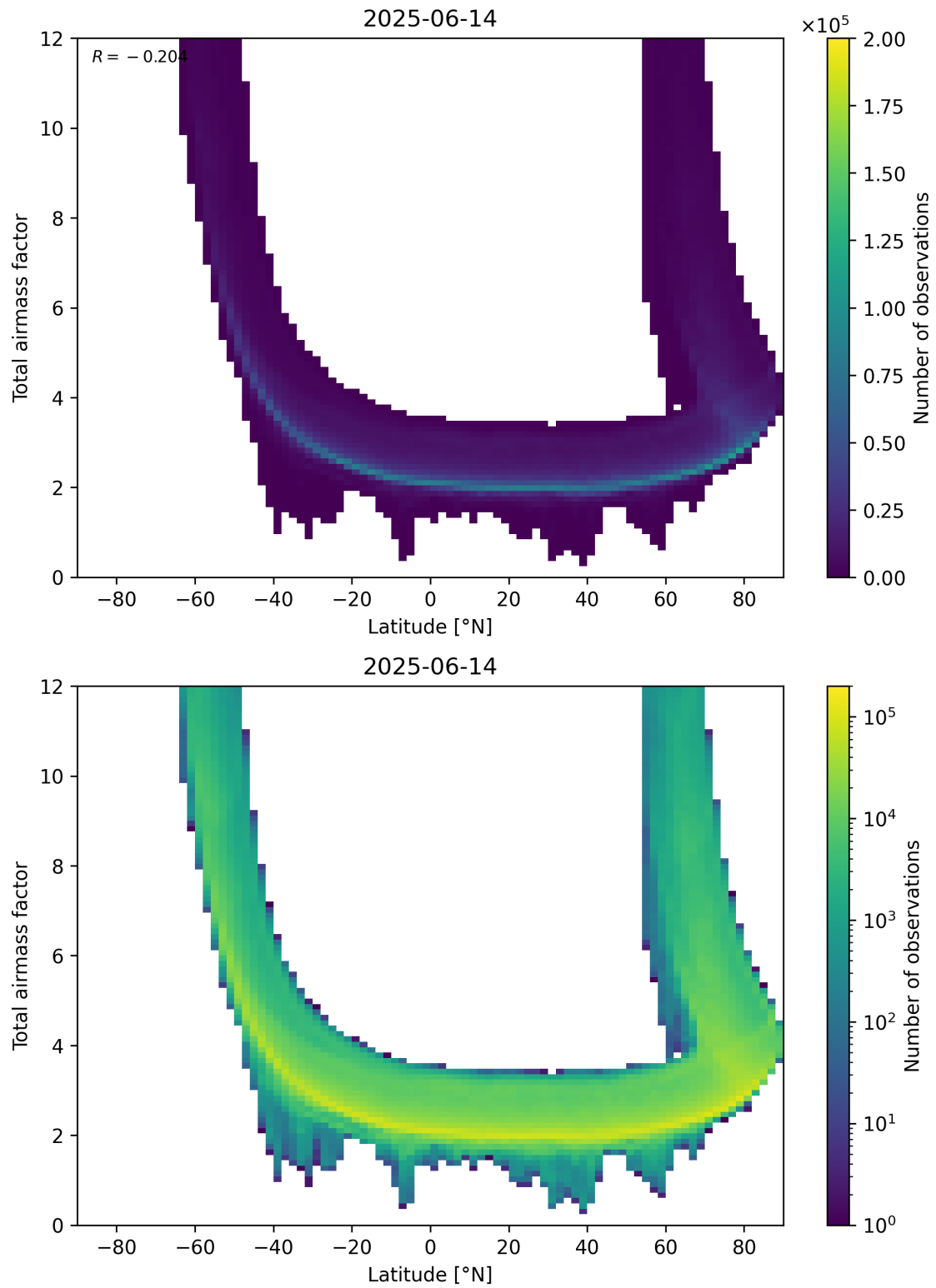
Figure 84: Scatter density plot of “Latitude” against “Total airmass factor” for 2025-06-13 to 2025-06-15.
