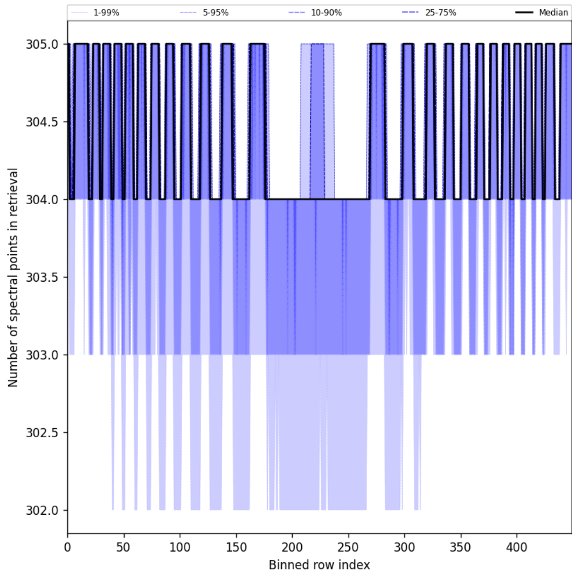
Figure 50: Along track statistics of “Number of spectral points in retrieval” for 2025-06-13 to 2025-06-15
