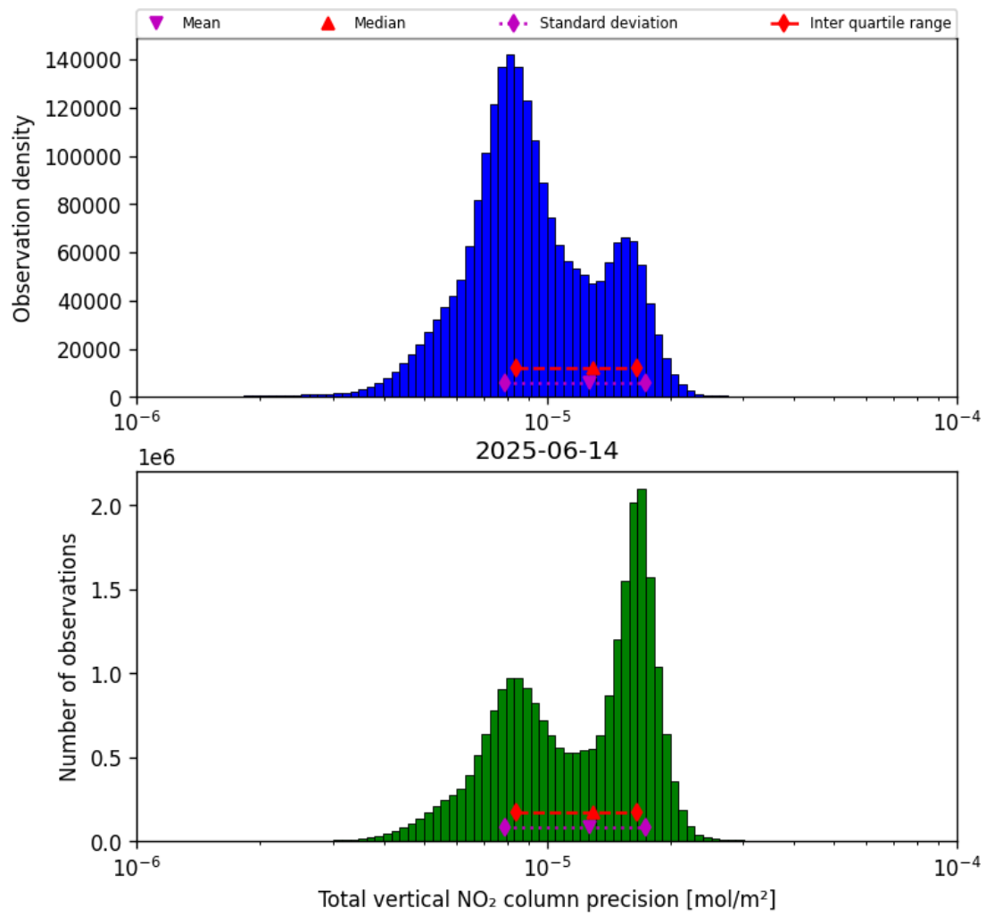
Figure 39: Histogram of “Total vertical NO 2 column precision” for 2025-06-13 to 2025-06-15
