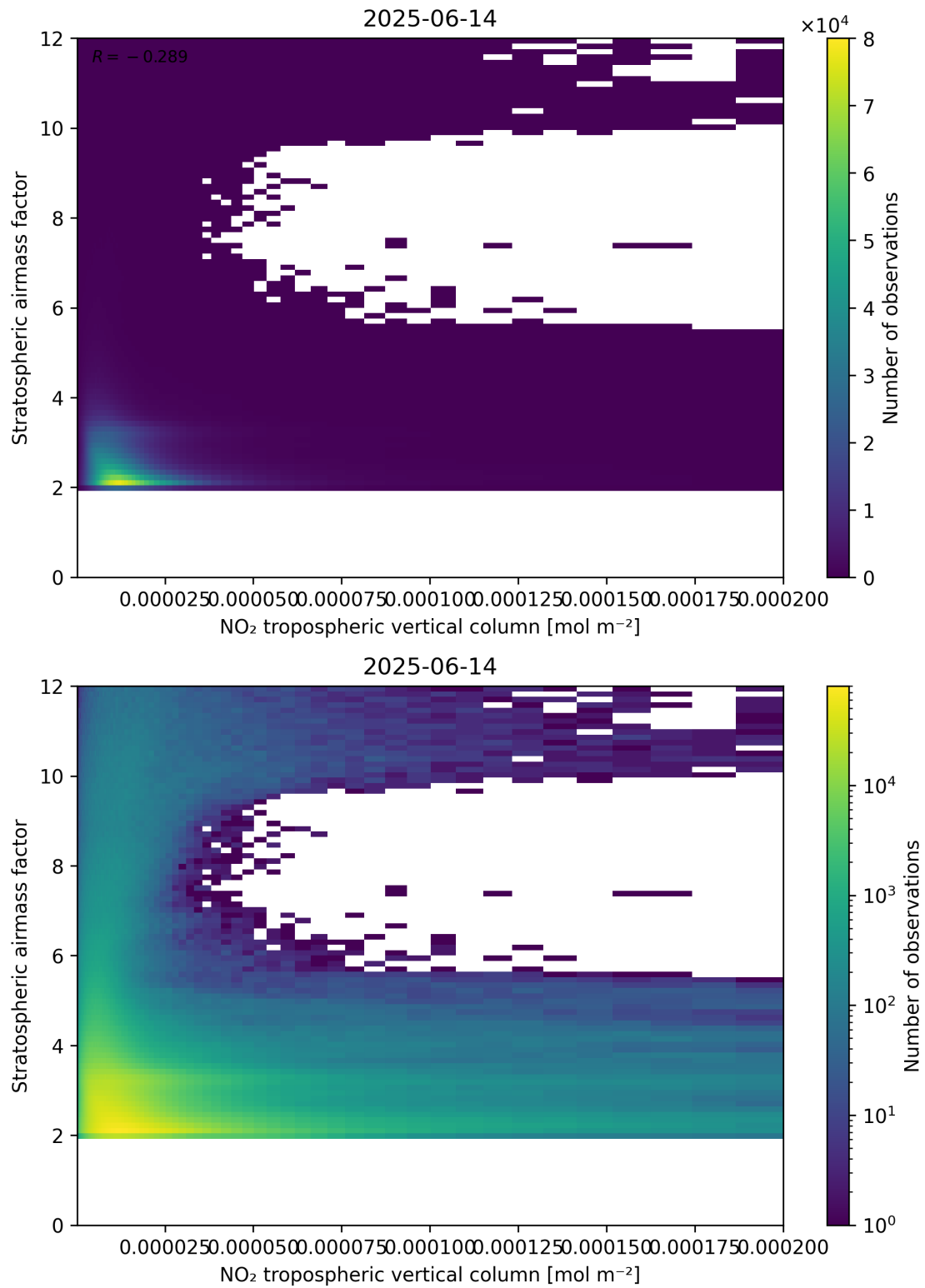
Figure 121: Scatter density plot of “NO 2 tropospheric vertical column” against “Stratospheric air mass factor” for 2025-06-13 to 2025-06-15.
