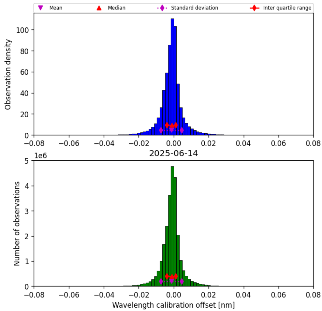
Figure 35: Histogram of “Wavelength calibration offset” for 2025-06-13 to 2025-06-15
