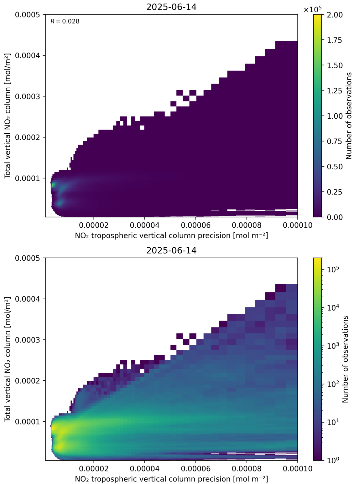
Figure 138: Scatter density plot of “NO 2 tropospheric vertical column precision” against “Total vertical NO 2 column” for 2025-06-13 to 2025-06-15.
