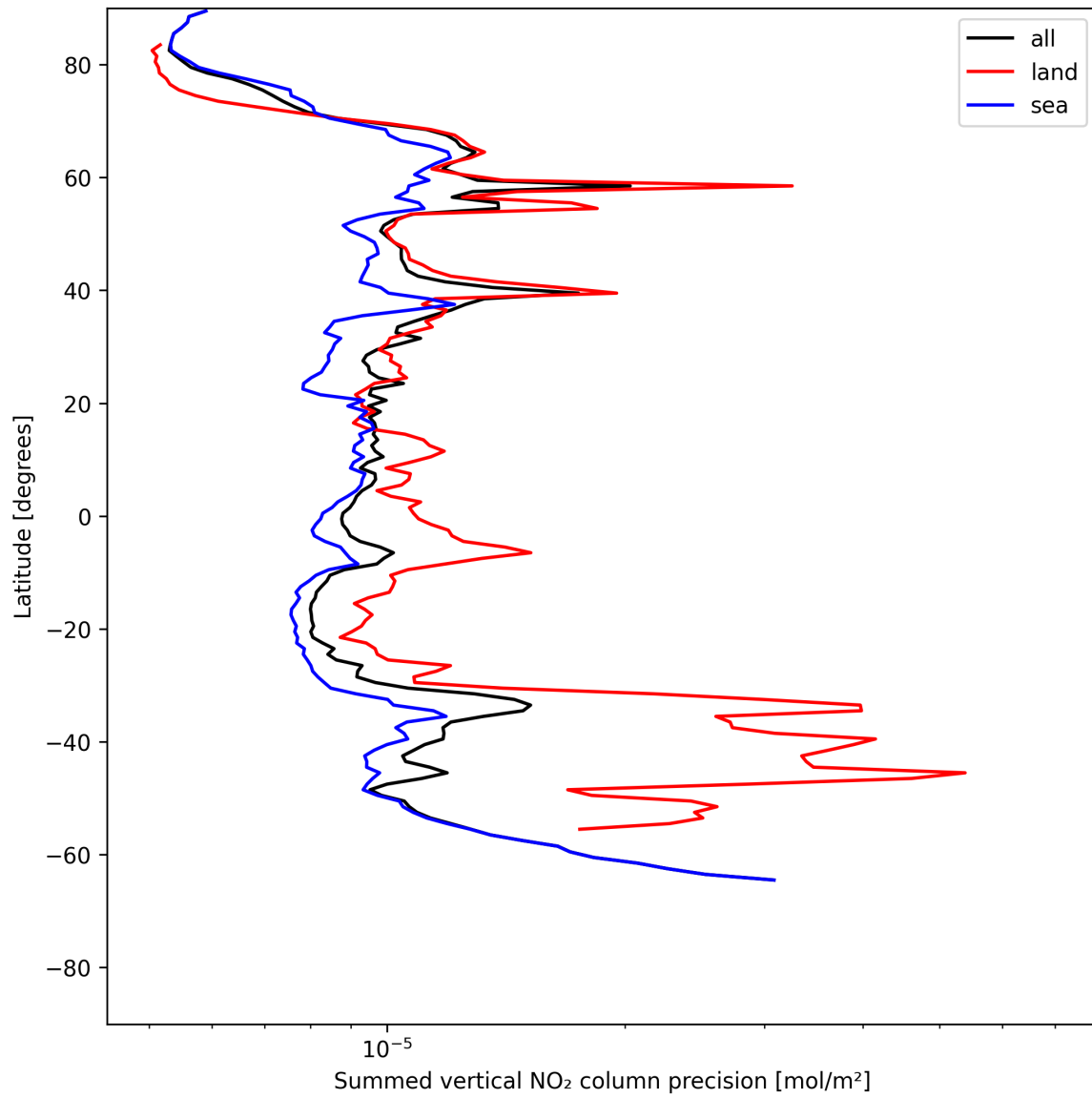
Figure 24: Zonal average of “Summed vertical NO 2 column precision” for 2025-06-13 to 2025-06-15.
