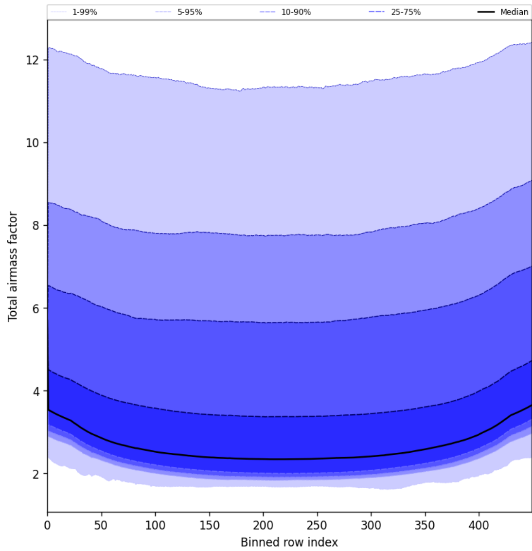
Figure 49: Along track statistics of “Total airmass factor” for 2025-06-13 to 2025-06-15
