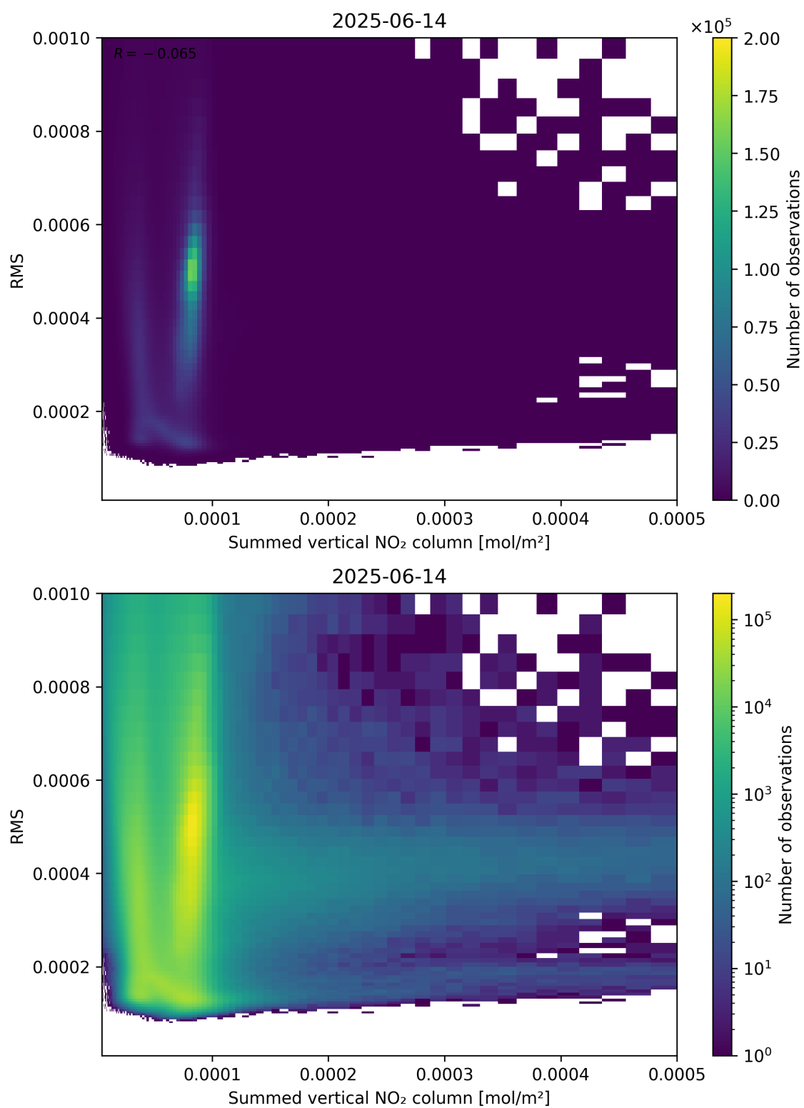
Figure 109: Scatter density plot of “Summed vertical NO 2 column” against “RMS” for 2025-06-13 to 2025-06-15.
