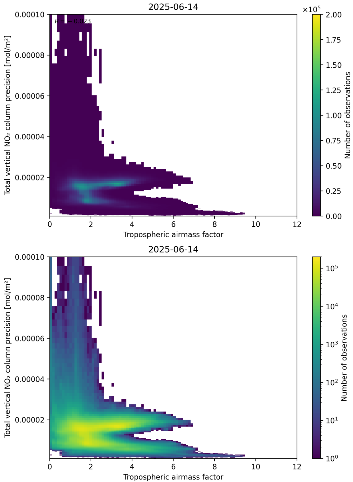
Figure 78: Scatter density plot of “Tropospheric air mass factor” against “Total vertical NO 2 column precision” for 2025-06-13 to 2025-06-15.
