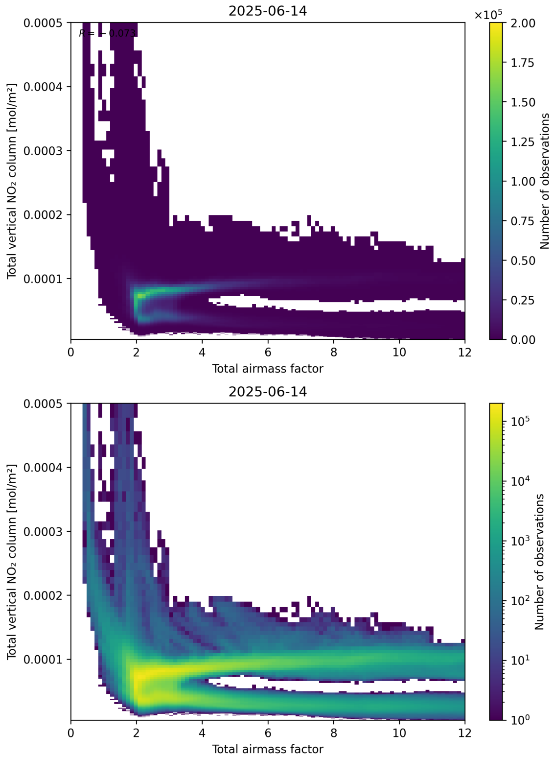
Figure 67: Scatter density plot of “Total air mass factor” against “Total vertical NO 2 column” for 2025-06-13 to 2025-06-15.
