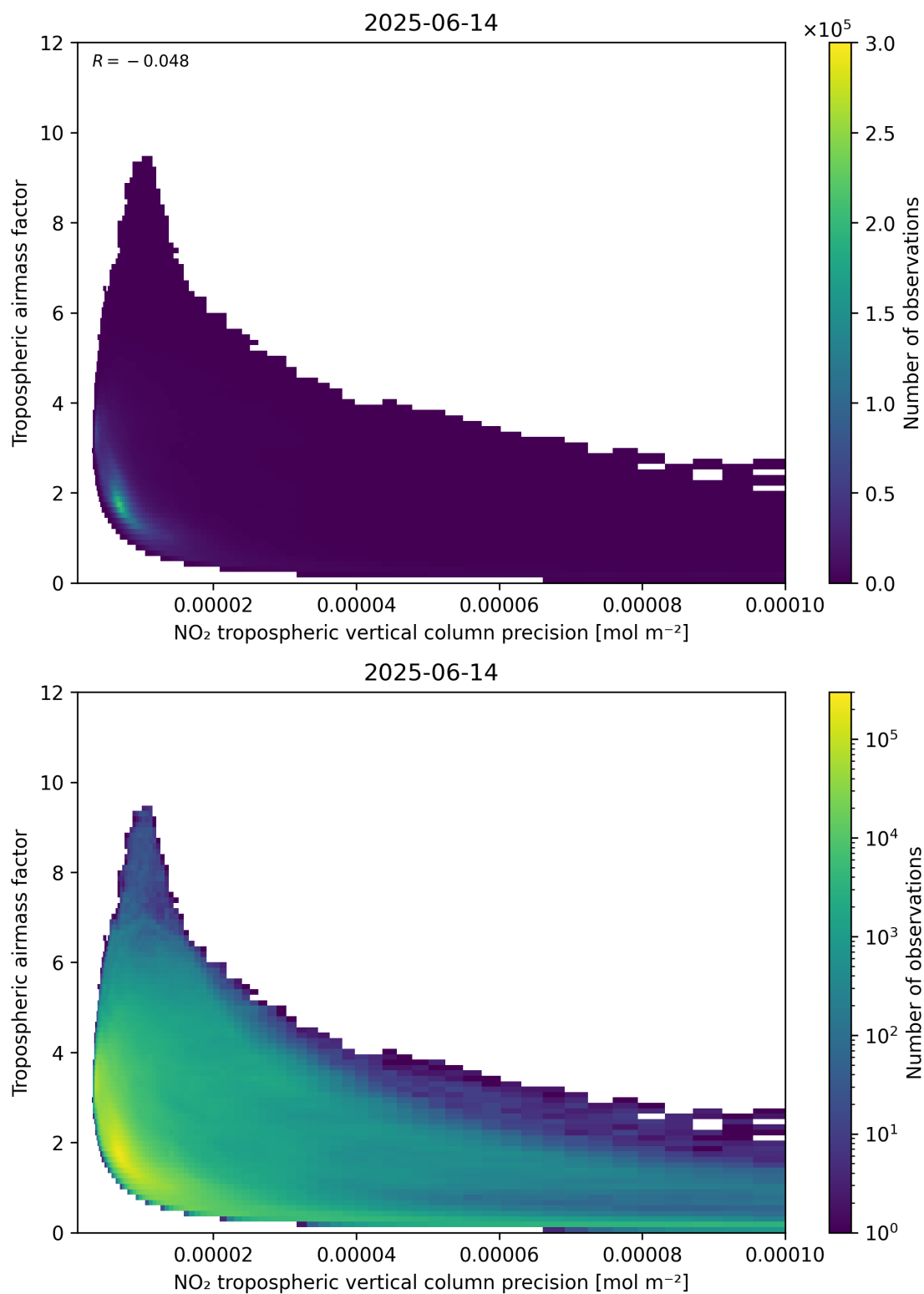
Figure 133: Scatter density plot of “NO 2 tropospheric vertical column precision” against “Tropospheric airmass factor” for 2025-06-13 to 2025-06-15.
