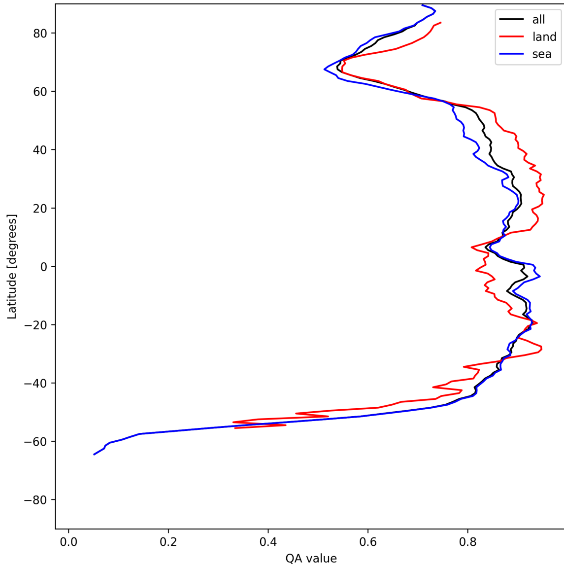
Figure 11: Zonal average of “QA value” for 2025-06-13 to 2025-06-15.
