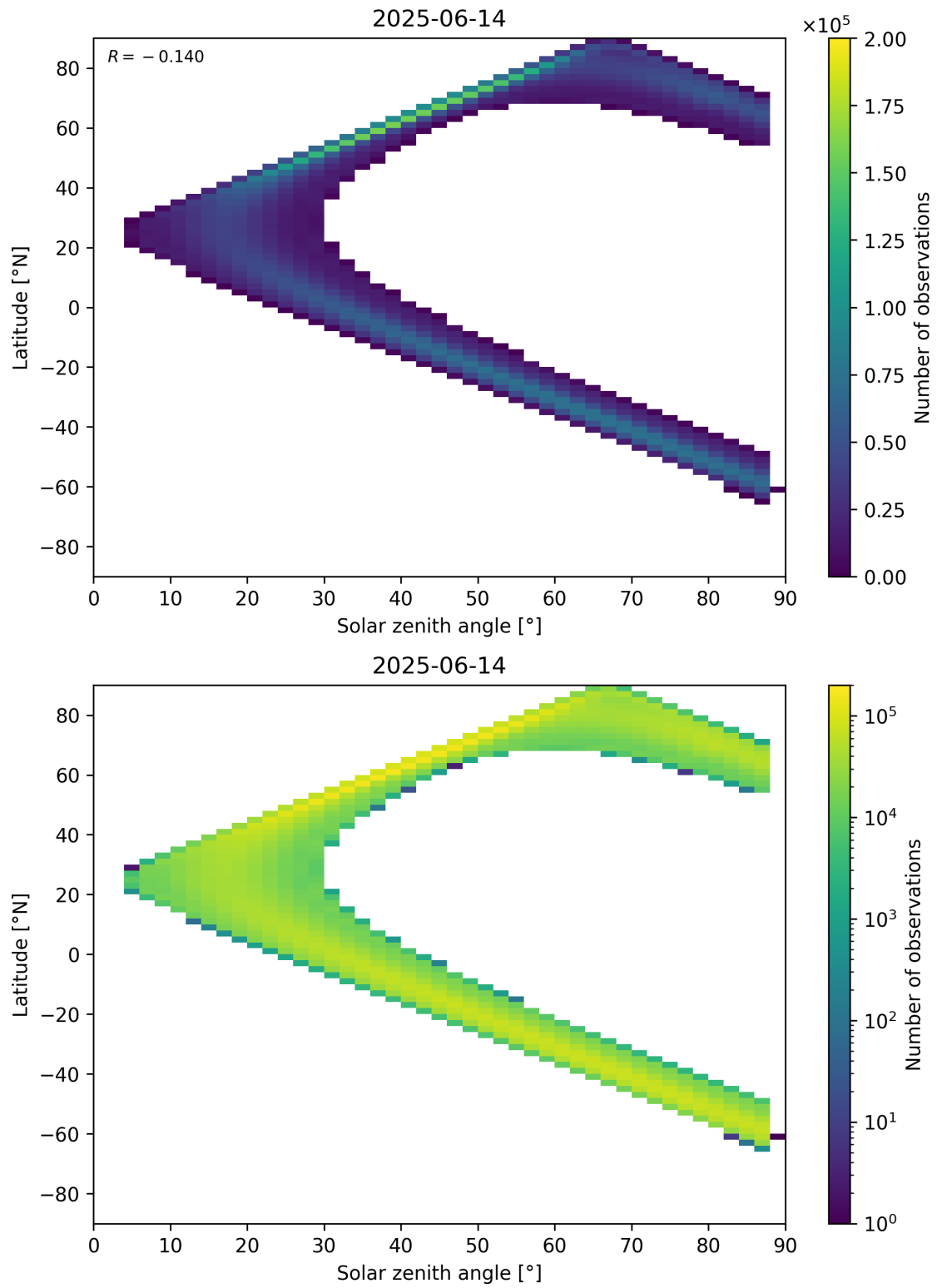
Figure 149: Scatter density plot of “Solar zenith angle” against “Latitude” for 2025-06-13 to 2025-06-15.
