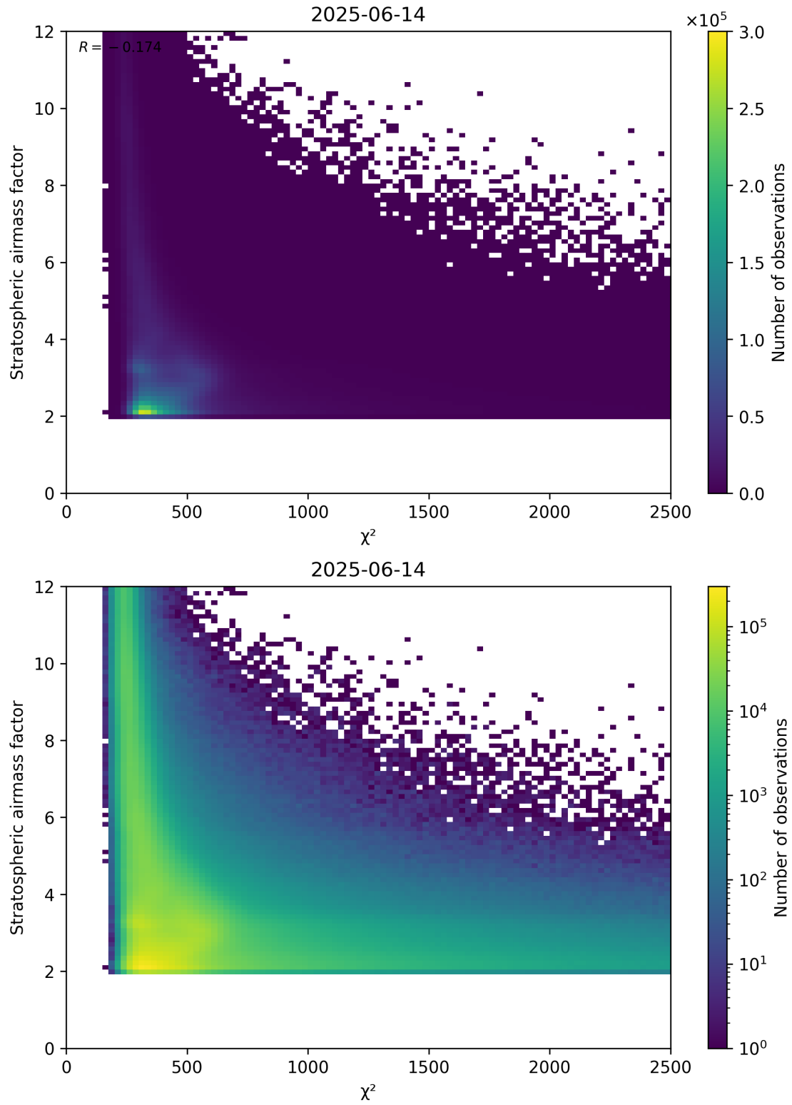
Figure 81: Scatter density plot of “ \chi^2 ” against “Stratospheric airmass factor” for 2025-06-13 to 2025-06-15.
