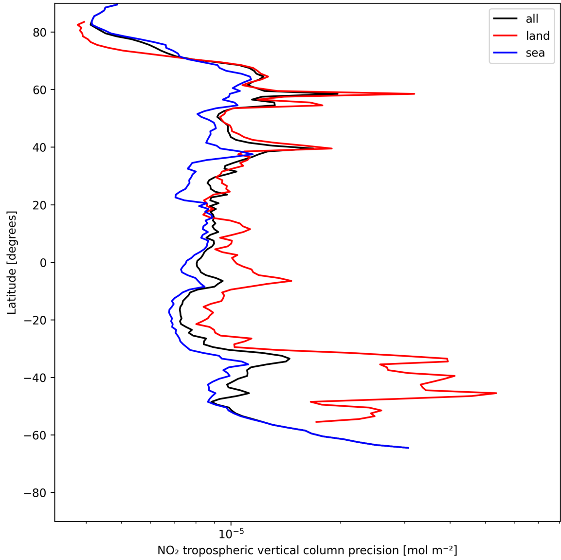
Figure 13: Zonal average of "NO 2 tropospheric vertical column precision" for 2025-06-13 to 2025-06-15.
