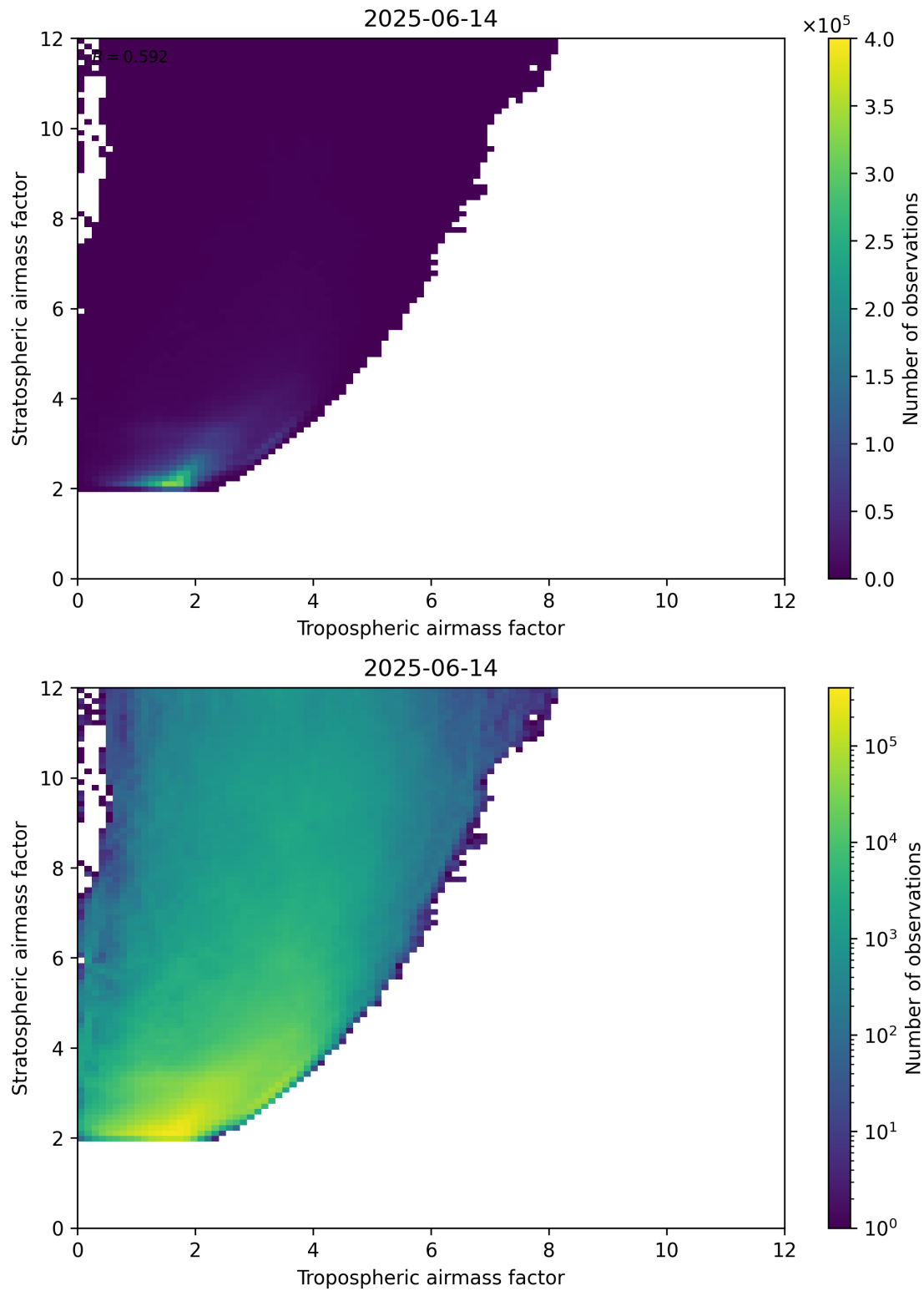
Figure 71: Scatter density plot of “Tropospheric airmass factor” against “Stratospheric airmass factor” for 2025-06-13 to 2025-06-15.
