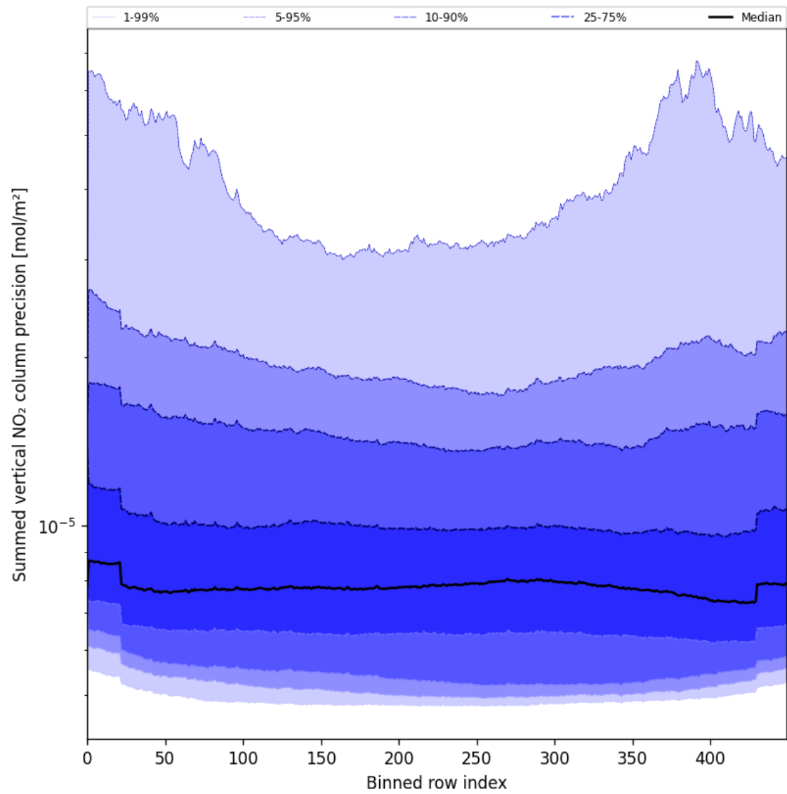
Figure 58: Along track statistics of “Summed vertical NO 2 column precision” for 2025-06-13 to 2025-06-15
