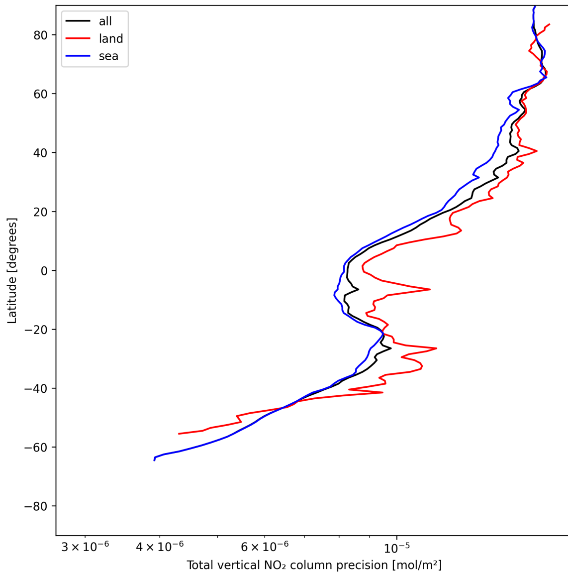
Figure 22: Zonal average of “Total vertical NO 2 column precision” for 2025-06-13 to 2025-06-15.
