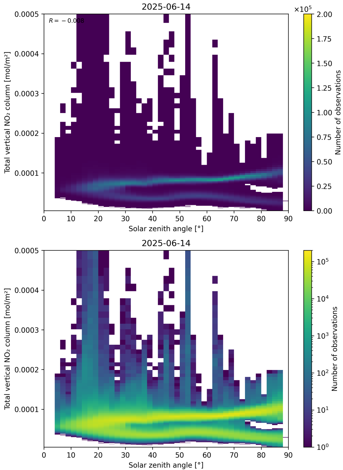
Figure 153: Scatter density plot of “Solar zenith angle” against “Total vertical NO 2 column” for 2025-06-13 to 2025-06-15.
