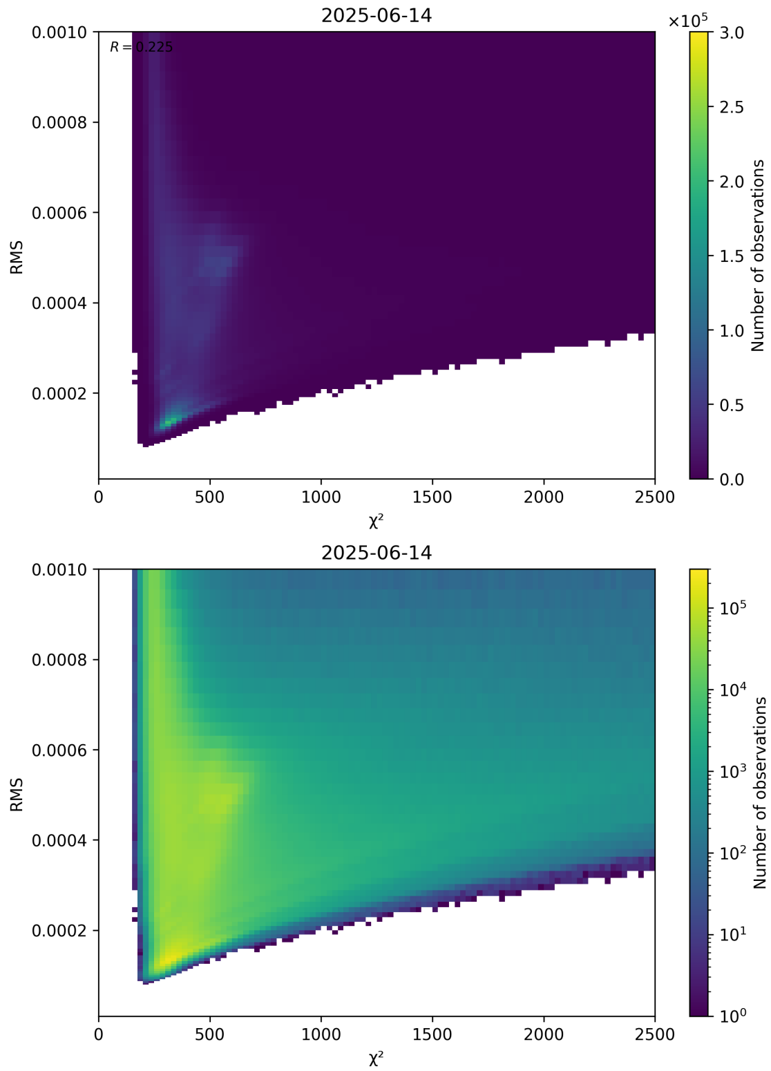
Figure 82: Scatter density plot of “ \chi^2 ” against “RMS” for 2025-06-13 to 2025-06-15.
