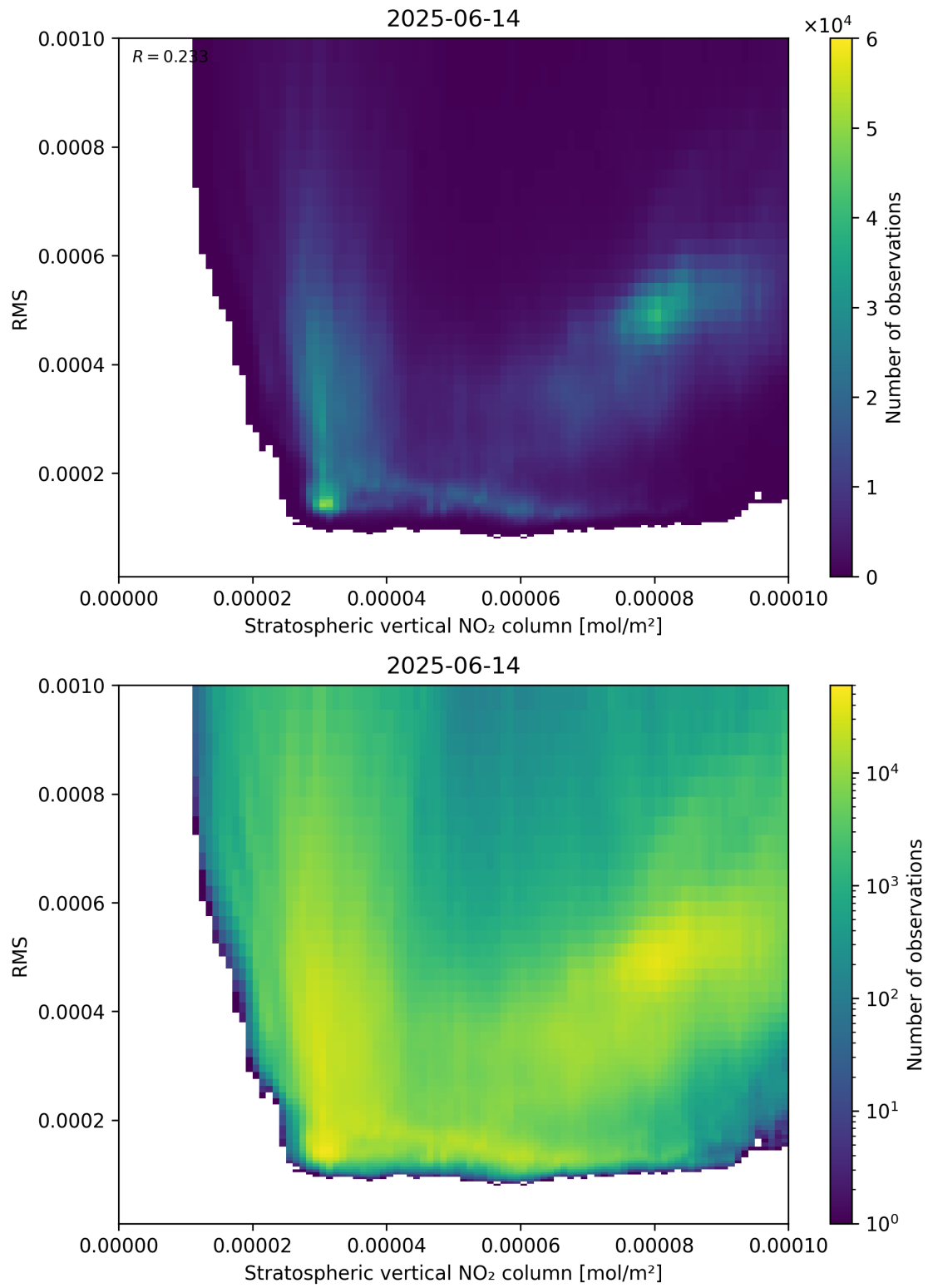
Figure 102: Scatter density plot of “Stratospheric vertical NO 2 column” against “RMS” for 2025-06-13 to 2025-06-15.
