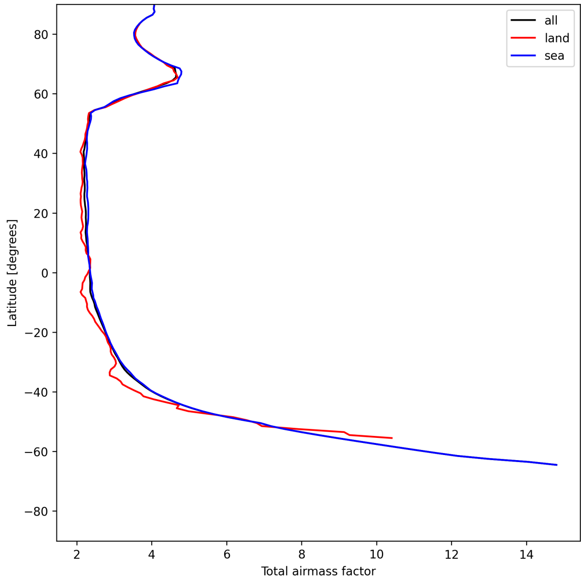
Figure 15: Zonal average of “Total airmass factor” for 2025-06-13 to 2025-06-15.
