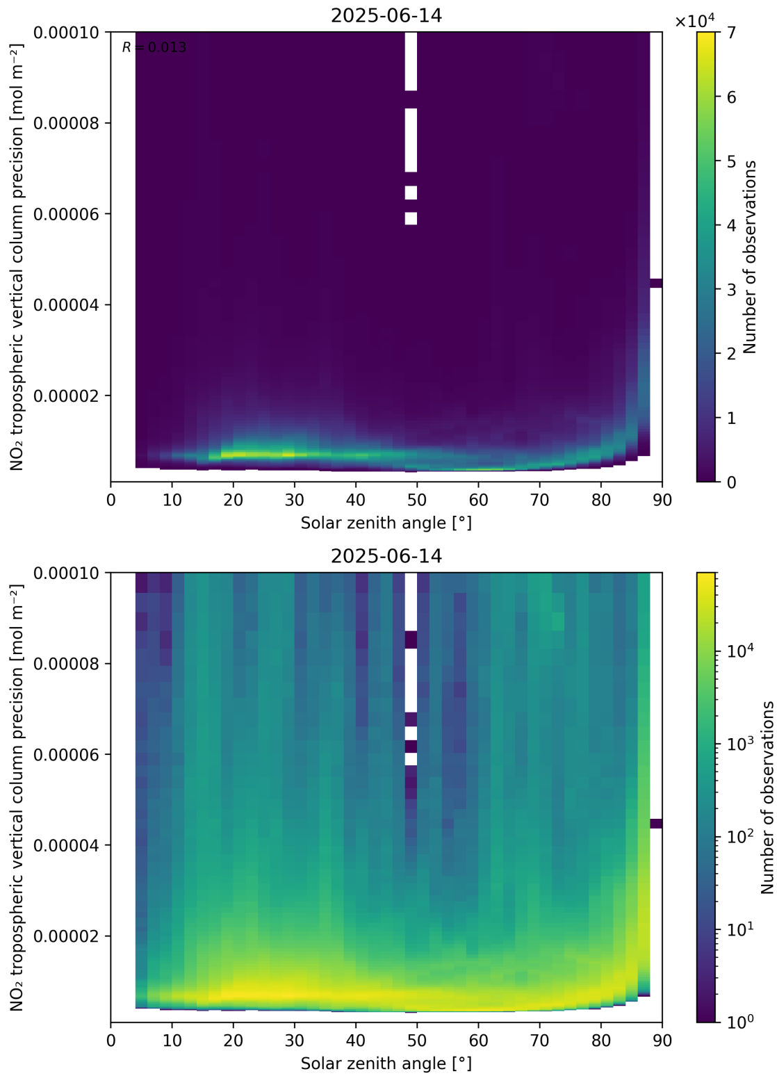
Figure 156: Scatter density plot of “Solar zenith angle” against “NO 2 tropospheric vertical column precision” for 2025-06-13 to 2025-06-15.
