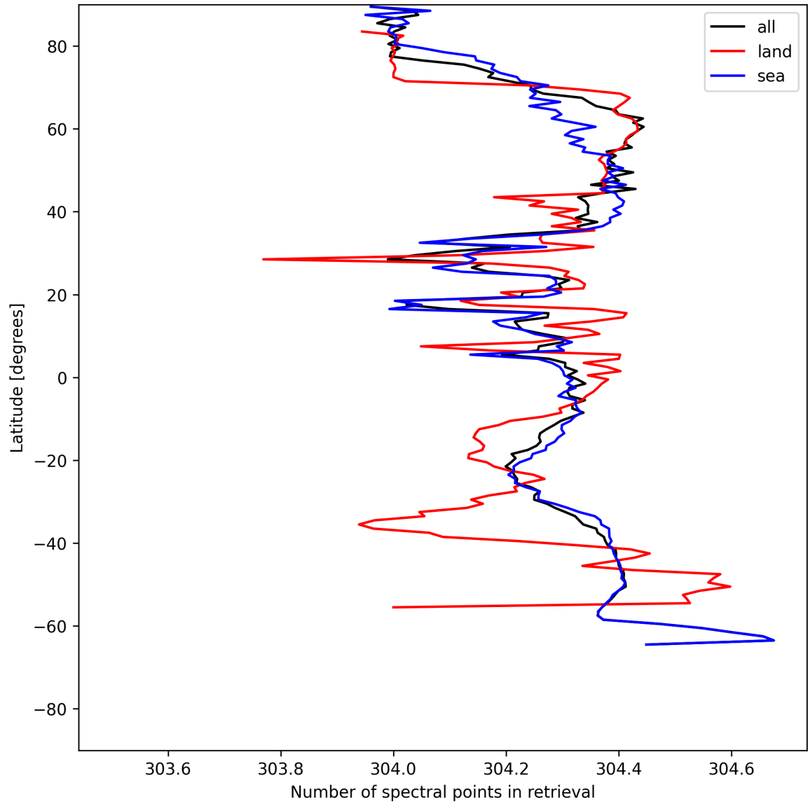
Figure 16: Zonal average of “Number of spectral points in retrieval” for 2025-06-13 to 2025-06-15.
