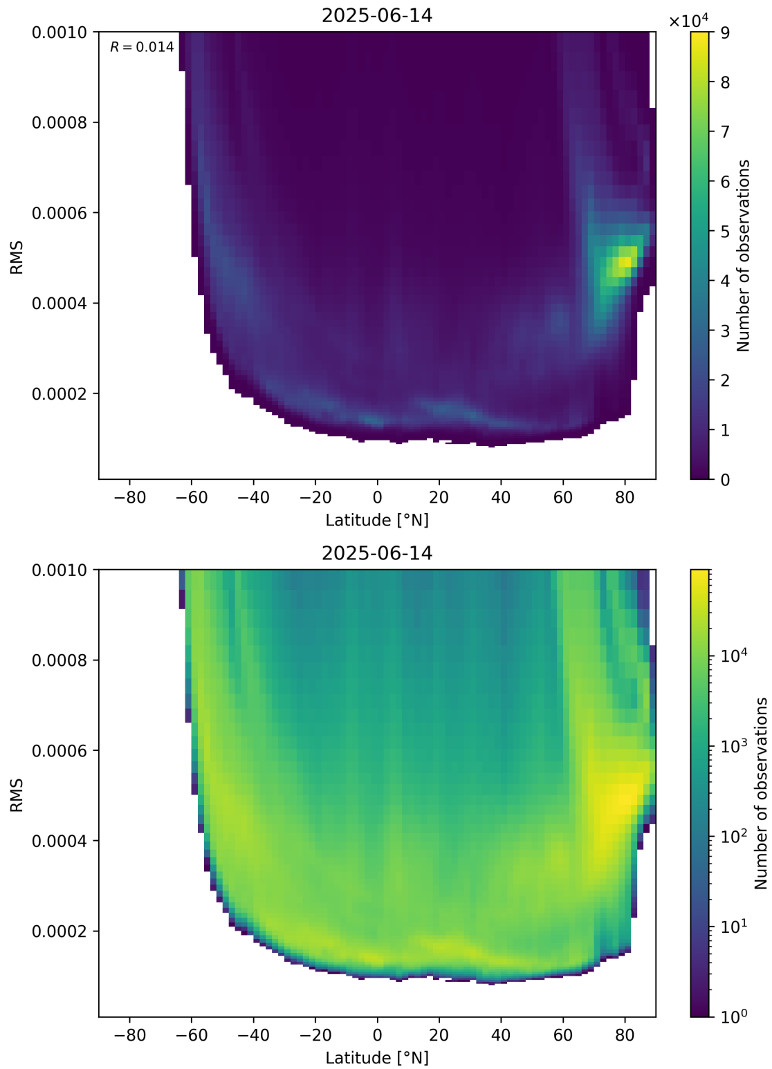
Figure 94: Scatter density plot of “Latitude” against “RMS” for 2025-06-13 to 2025-06-15.
