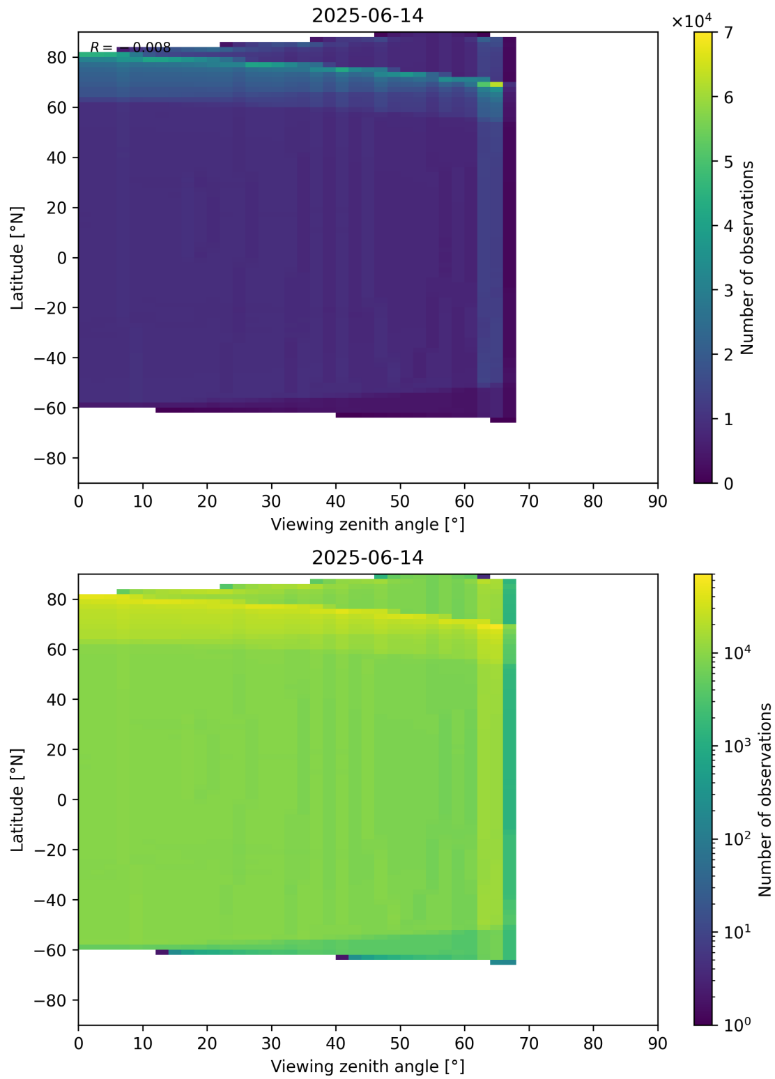
Figure 163: Scatter density plot of “Viewing zenith angle” against “Latitude” for 2025-06-13 to 2025-06-15.
