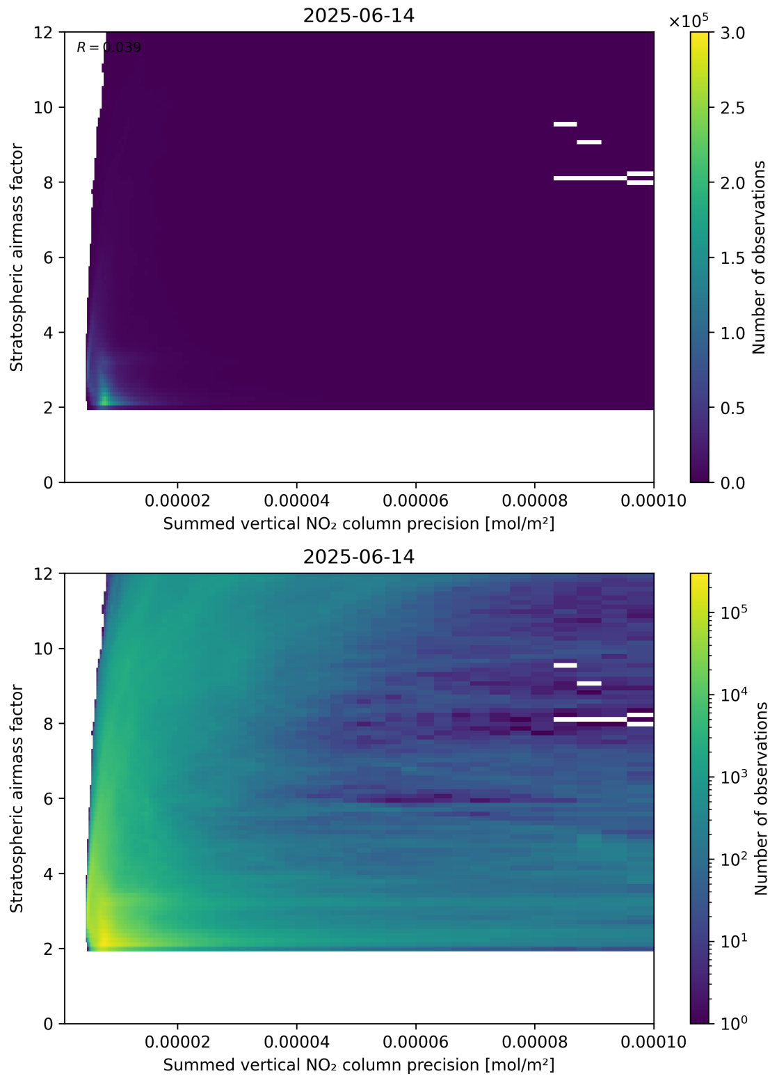
Figure 106: Scatter density plot of “Summed vertical NO 2 column precision” against “Stratospheric airmass factor” for 2025-06-13 to 2025-06-15.
