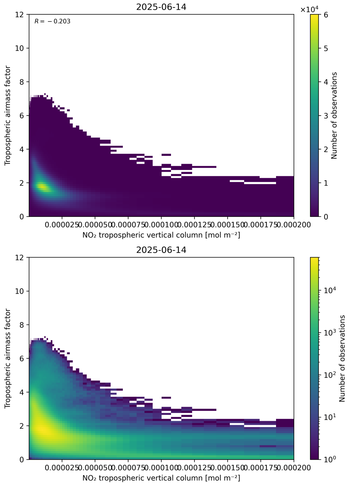
Figure 123: Scatter density plot of “NO 2 tropospheric vertical column” against “Tropospheric air mass factor” for 2025-06-13 to 2025-06-15.
