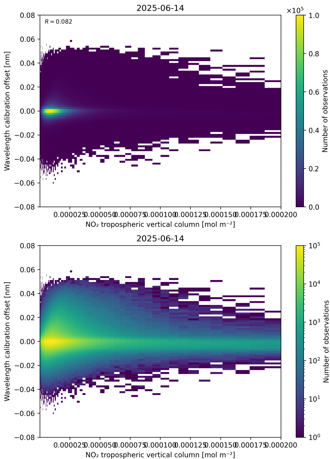
Figure 143: Scatter density plot of “NO 2 tropospheric vertical column” against “Wavelength calibration offset” for 2025-06-13 to 2025-06-15.
