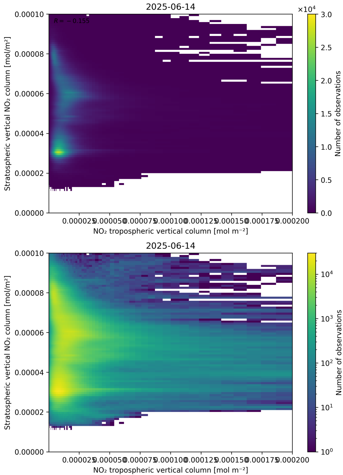
Figure 125: Scatter density plot of “NO 2 tropospheric vertical column” against “Stratospheric vertical NO 2 column” for 2025-06-13 to 2025-06-15.
