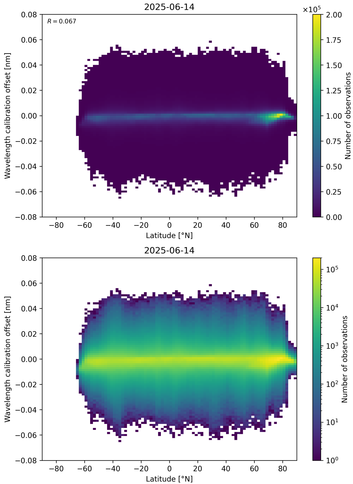
Figure 95: Scatter density plot of “Latitude” against “Wavelength calibration offset” for 2025-06-13 to 2025-06-15.
