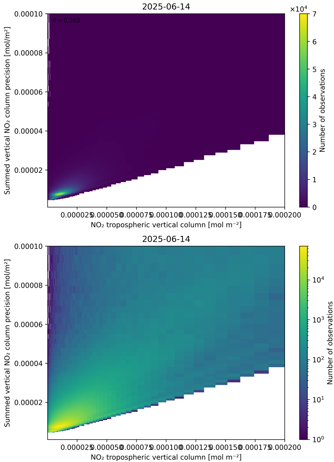
Figure 127: Scatter density plot of “NO 2 tropospheric vertical column” against “Summed vertical NO 2 column precision” for 2025-06-13 to 2025-06-15.
