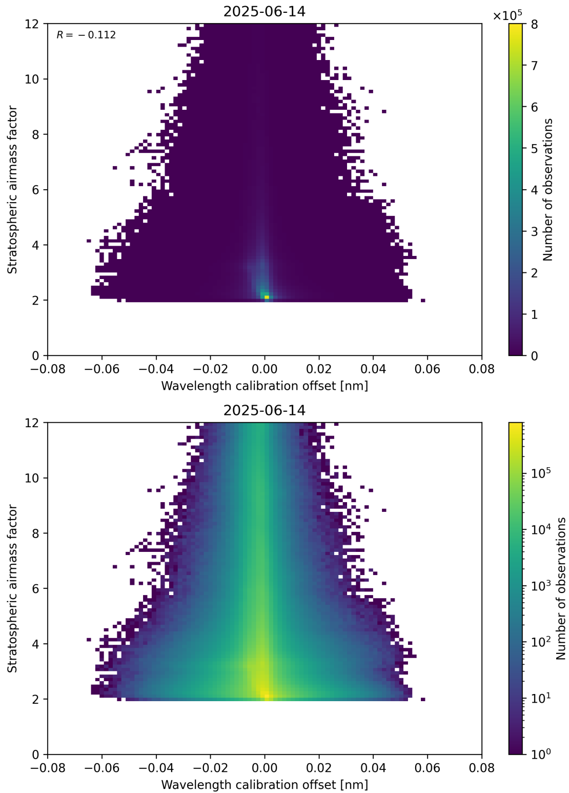
Figure 174: Scatter density plot of “Wavelength calibration offset” against “Stratospheric airmass factor” for 2025-06-13 to 2025-06-15.
