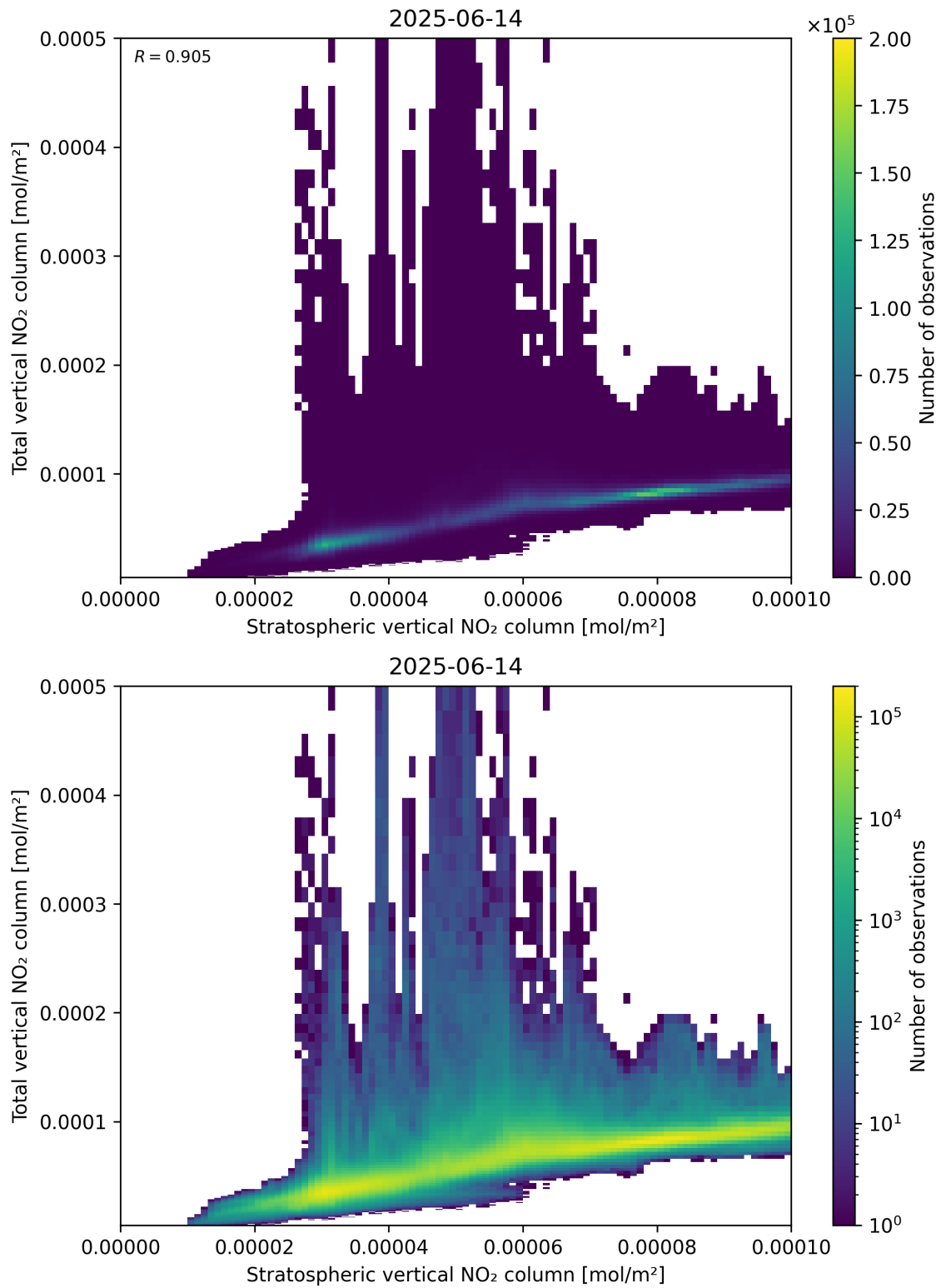
Figure 100: Scatter density plot of “Stratospheric vertical NO 2 column” against “Total vertical NO 2 column” for 2025-06-13 to 2025-06-15.
