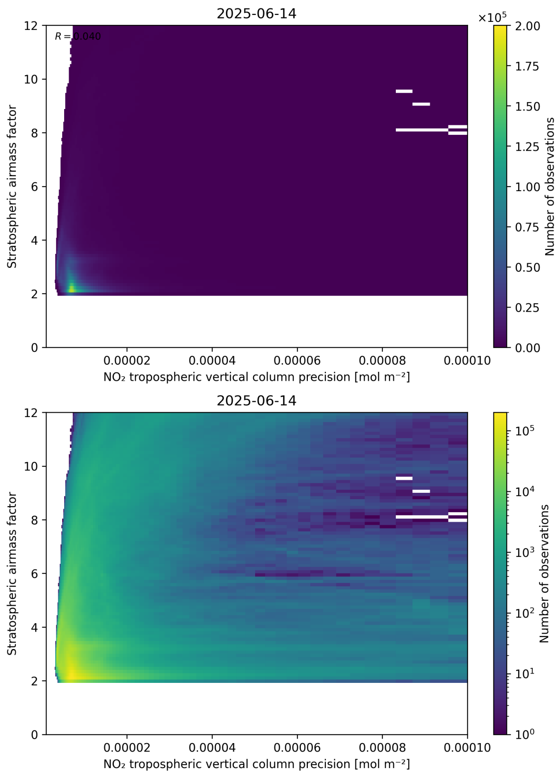
Figure 131: Scatter density plot of “NO 2 tropospheric vertical column precision” against “Stratospheric airmass factor” for 2025-06-13 to 2025-06-15.
