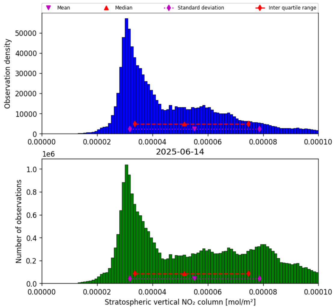
Figure 36: Histogram of “Stratospheric vertical NO 2 column” for 2025-06-13 to 2025-06-15
