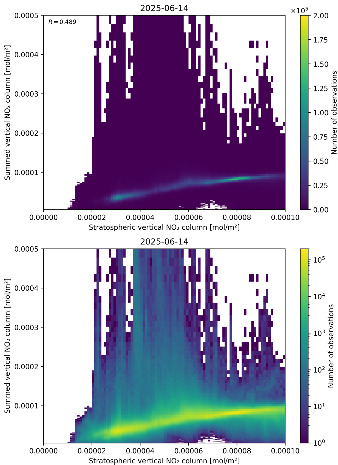
Figure 98: Scatter density plot of “Stratospheric vertical NO 2 column” against “Summed vertical NO 2 column” for 2025-06-13 to 2025-06-15.
