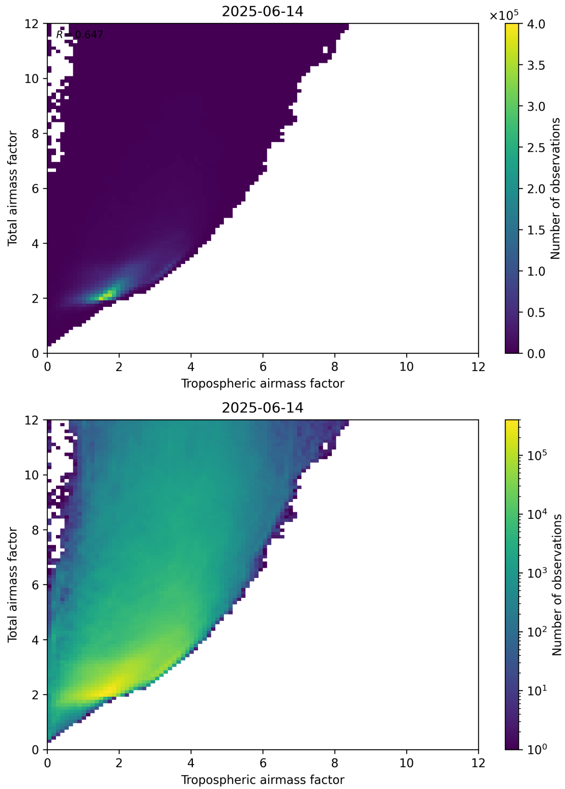
Figure 72: Scatter density plot of “Tropospheric airmass factor” against “Total airmass factor” for 2025-06-13 to 2025-06-15.
