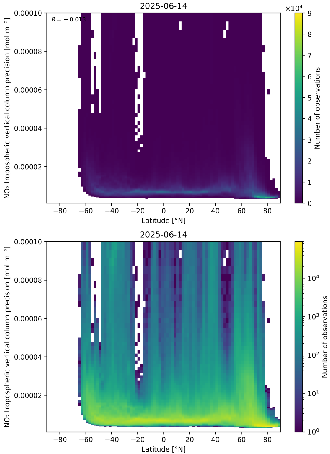
Figure 93: Scatter density plot of “Latitude” against “NO 2 tropospheric vertical column precision” for 2025-06-13 to 2025-06-15.
