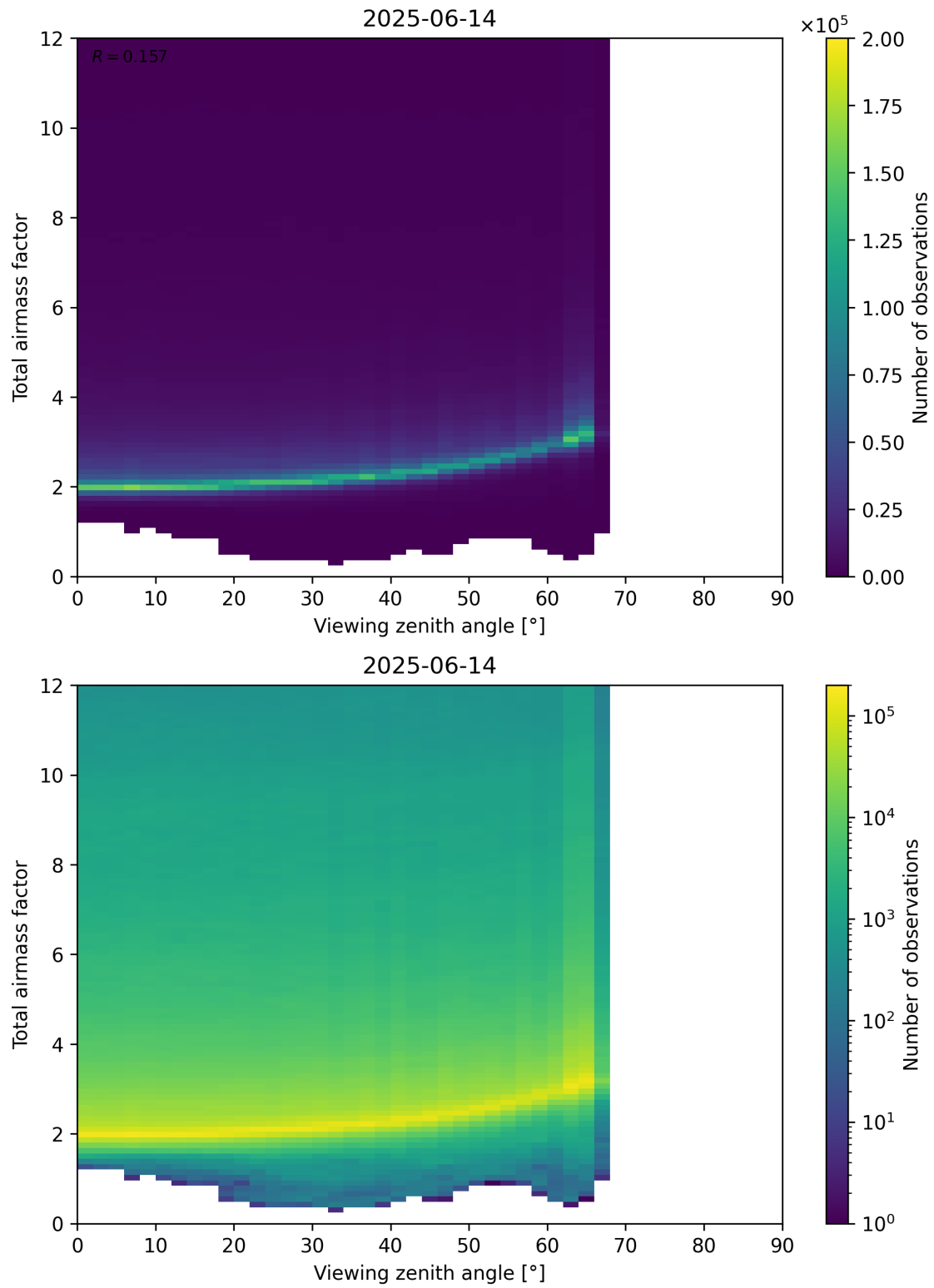
Figure 160: Scatter density plot of “Viewing zenith angle” against “Total airmass factor” for 2025-06-13 to 2025-06-15.
