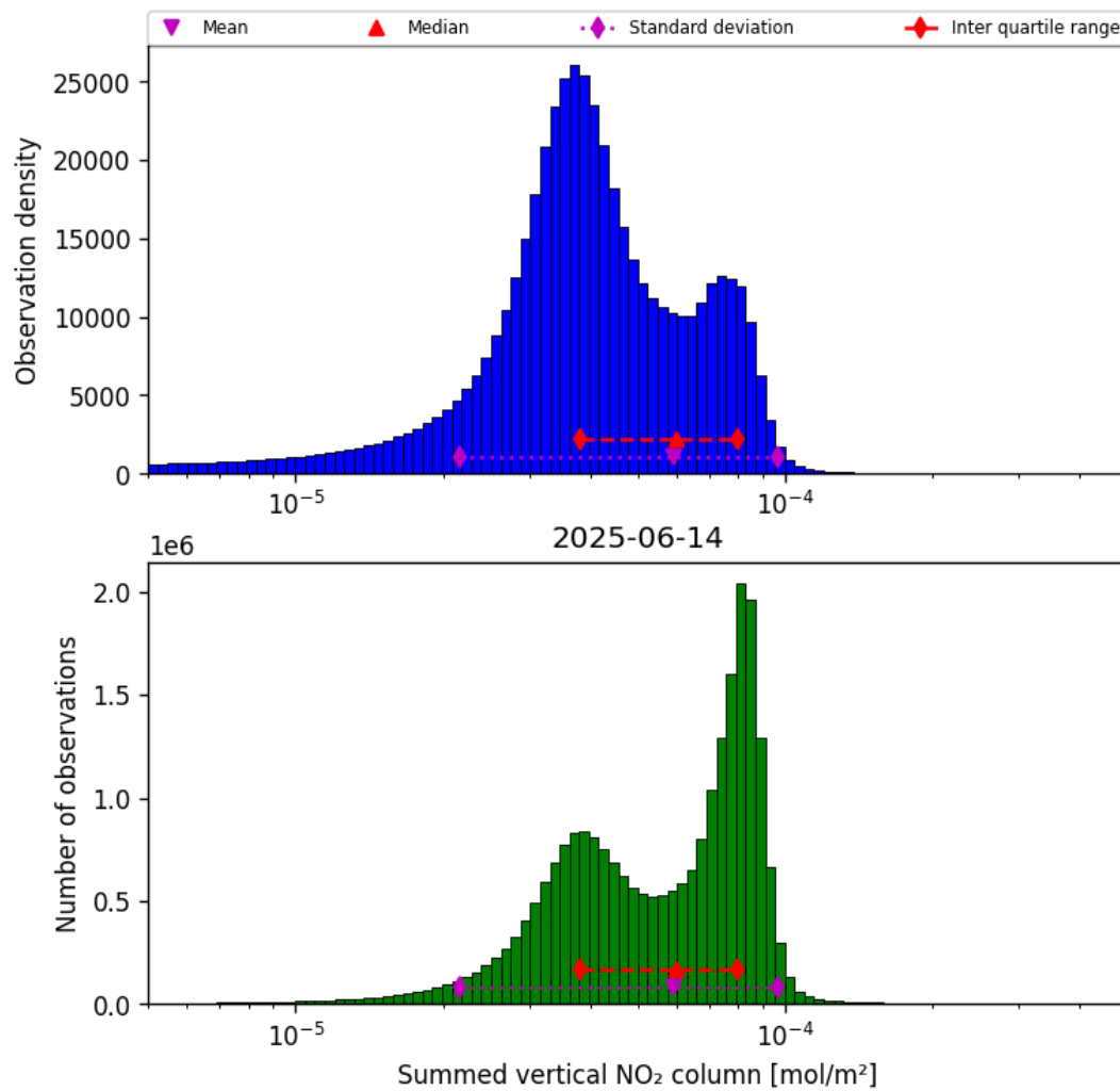
Figure 40: Histogram of “Summed vertical NO 2 column” for 2025-06-13 to 2025-06-15
