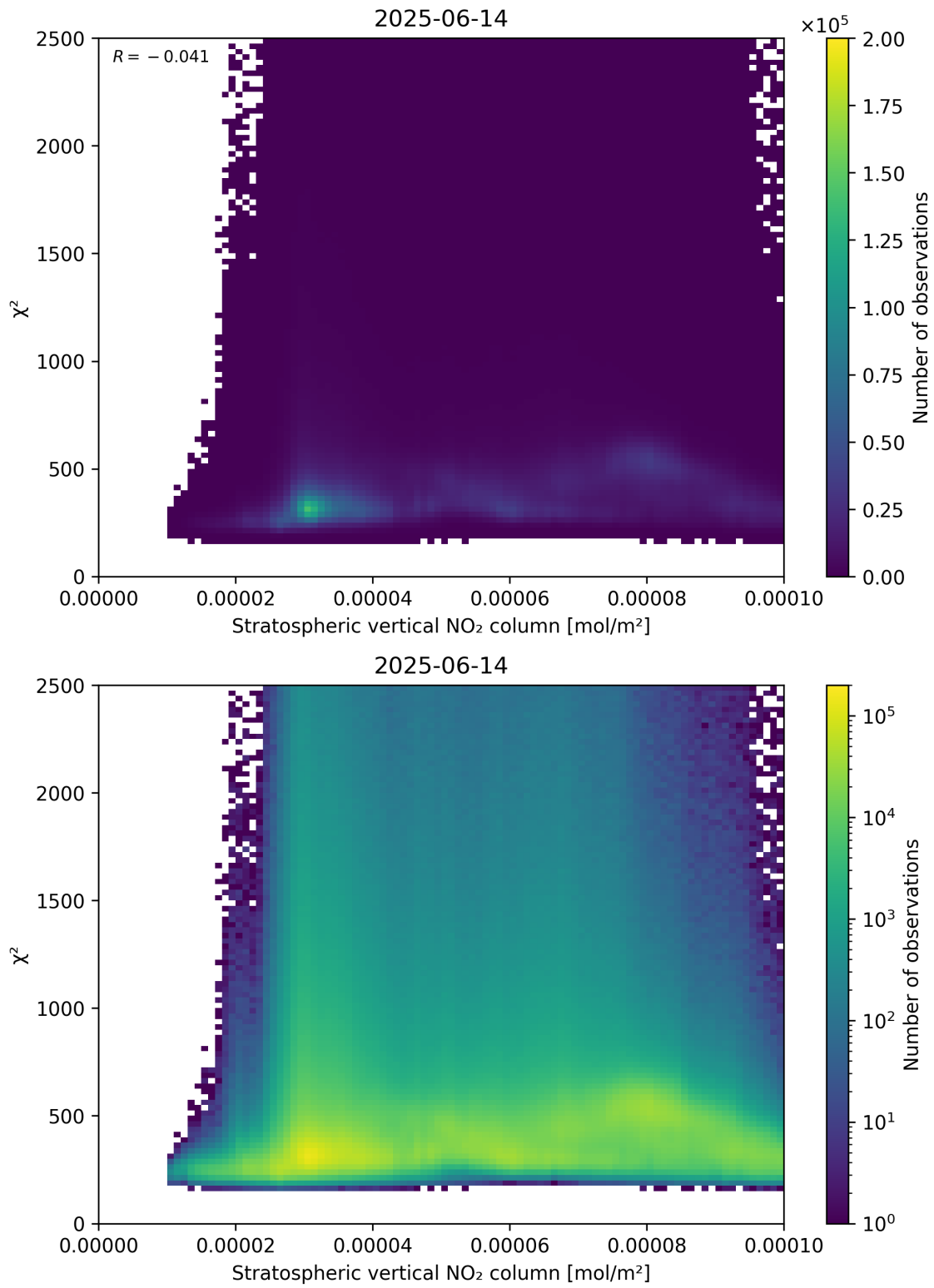
Figure 97: Scatter density plot of “Stratospheric vertical NO 2 column” against “ \chi^2 ” for 2025-06-13 to 2025-06-15.
