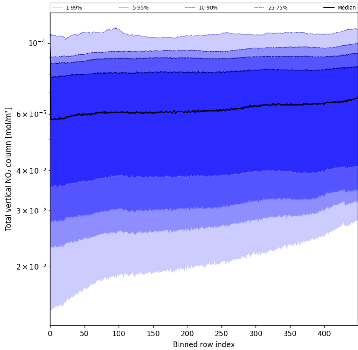
Figure 55: Along track statistics of “Total vertical NO 2 column” for 2025-06-13 to 2025-06-15
