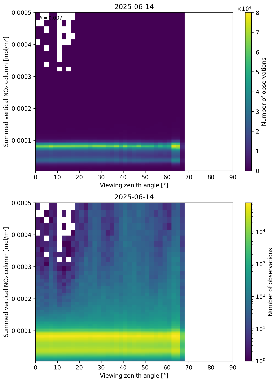
Figure 165: Scatter density plot of “Viewing zenith angle” against “Summed vertical NO 2 column” for 2025-06-13 to 2025-06-15.
