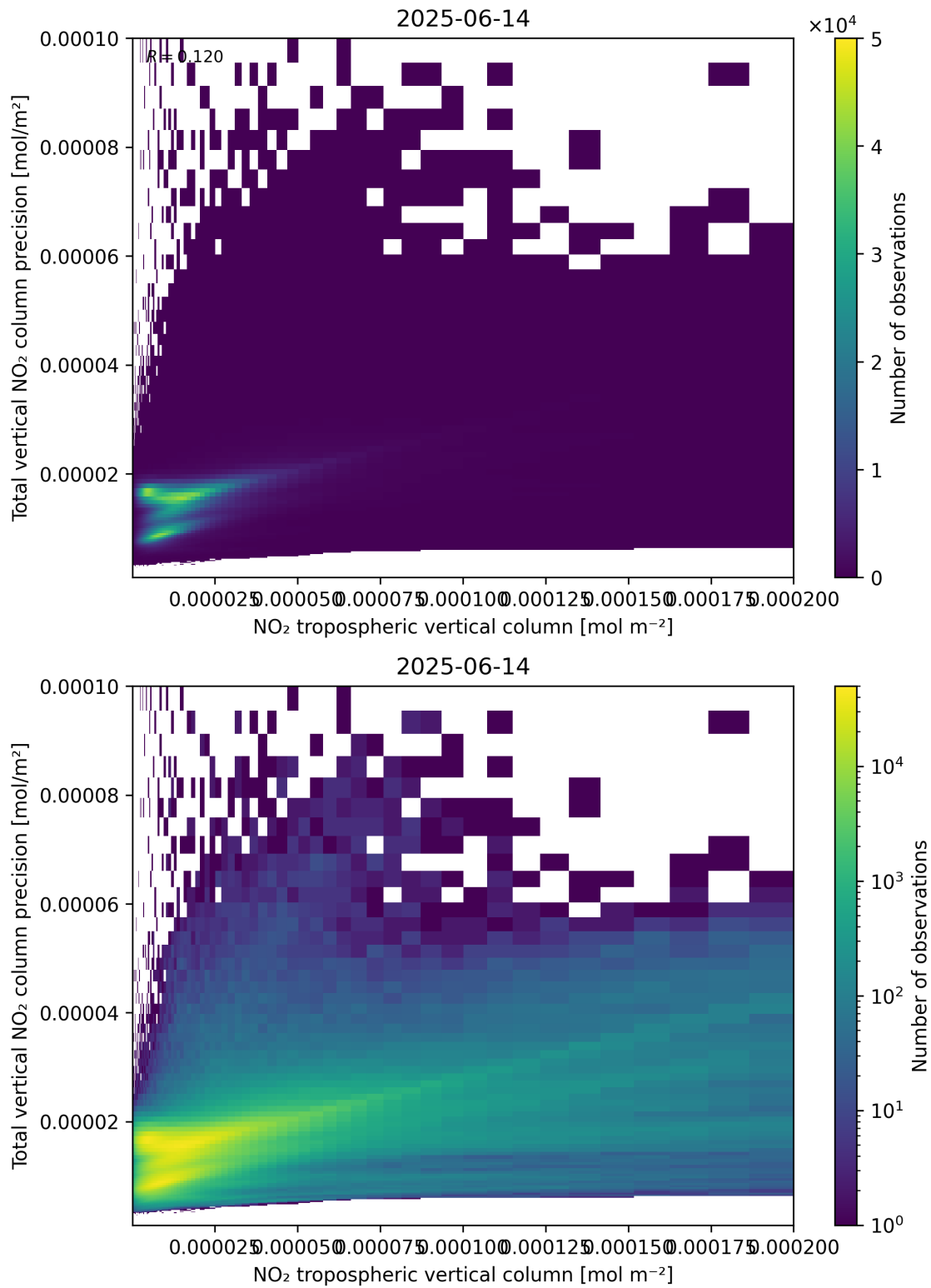
Figure 129: Scatter density plot of “NO 2 tropospheric vertical column” against “Total vertical NO 2 column precision” for 2025-06-13 to 2025-06-15.
