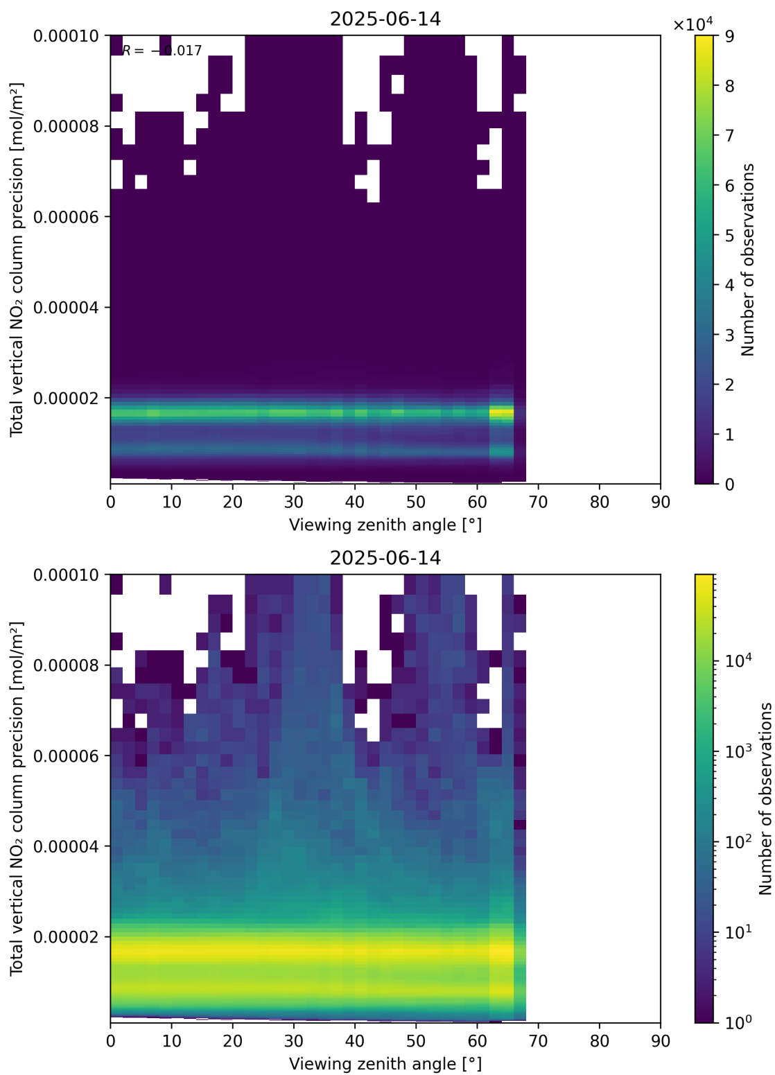
Figure 168: Scatter density plot of “Viewing zenith angle” against “Total vertical NO 2 column precision” for 2025-06-13 to 2025-06-15.
