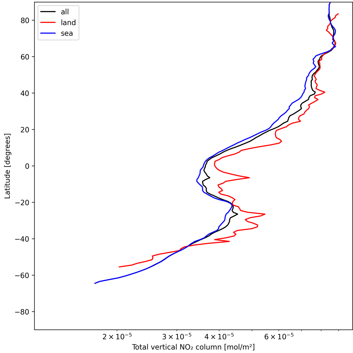
Figure 21: Zonal average of “Total vertical NO 2 column” for 2025-06-13 to 2025-06-15.
