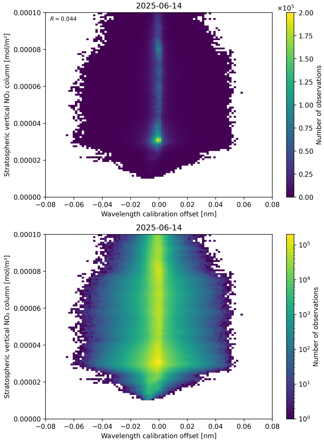
Figure 176: Scatter density plot of “Wavelength calibration offset” against “Stratospheric vertical NO 2 column” for 2025-06-13 to 2025-06-15.
