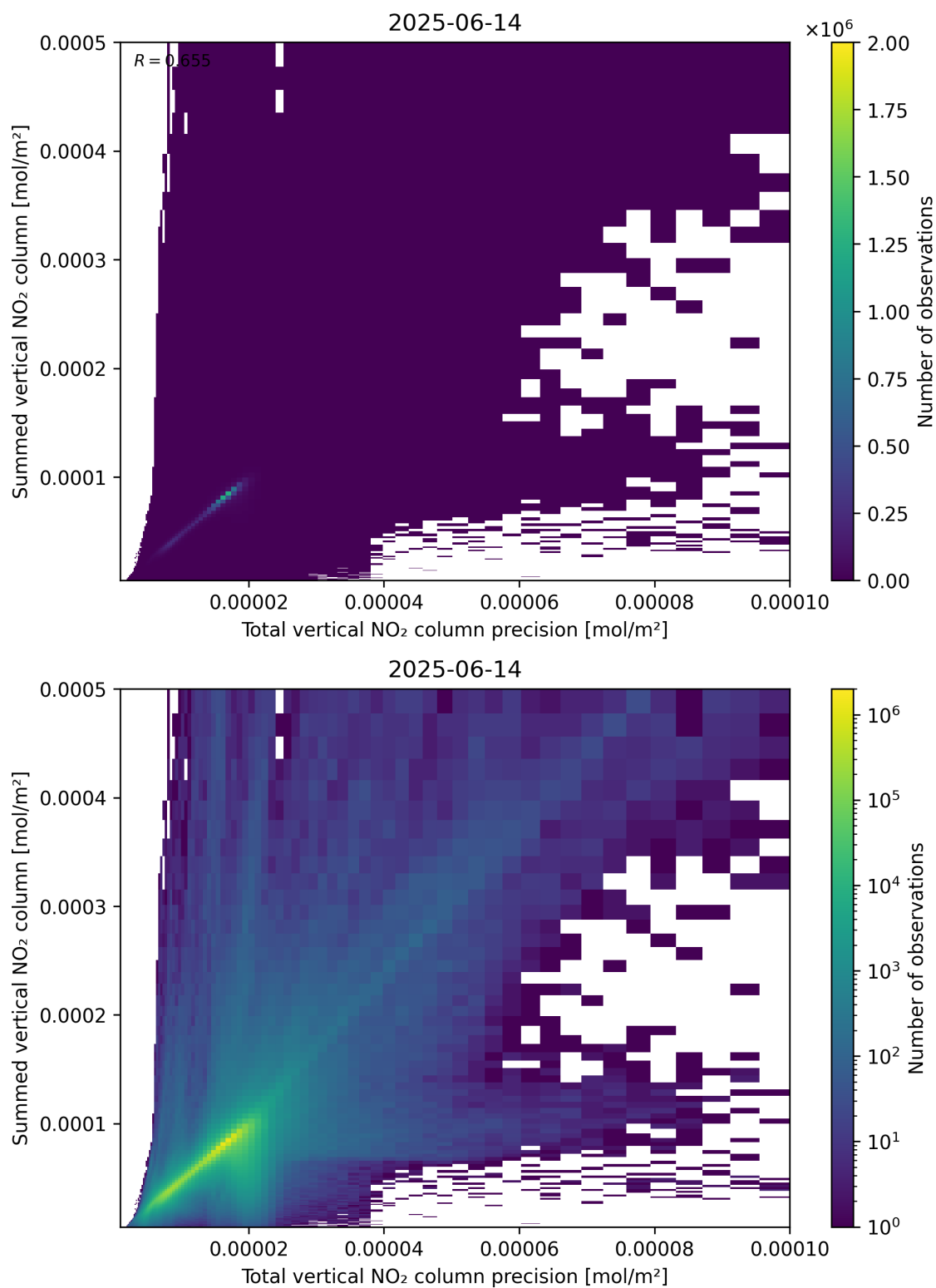
Figure 117: Scatter density plot of “Total vertical NO 2 column precision” against “Summed vertical NO 2 column” for 2025-06-13 to 2025-06-15.
