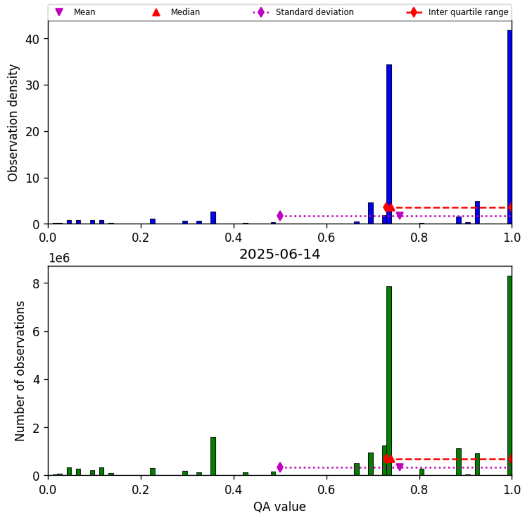
Figure 28: Histogram of “QA value” for 2025-06-13 to 2025-06-15
