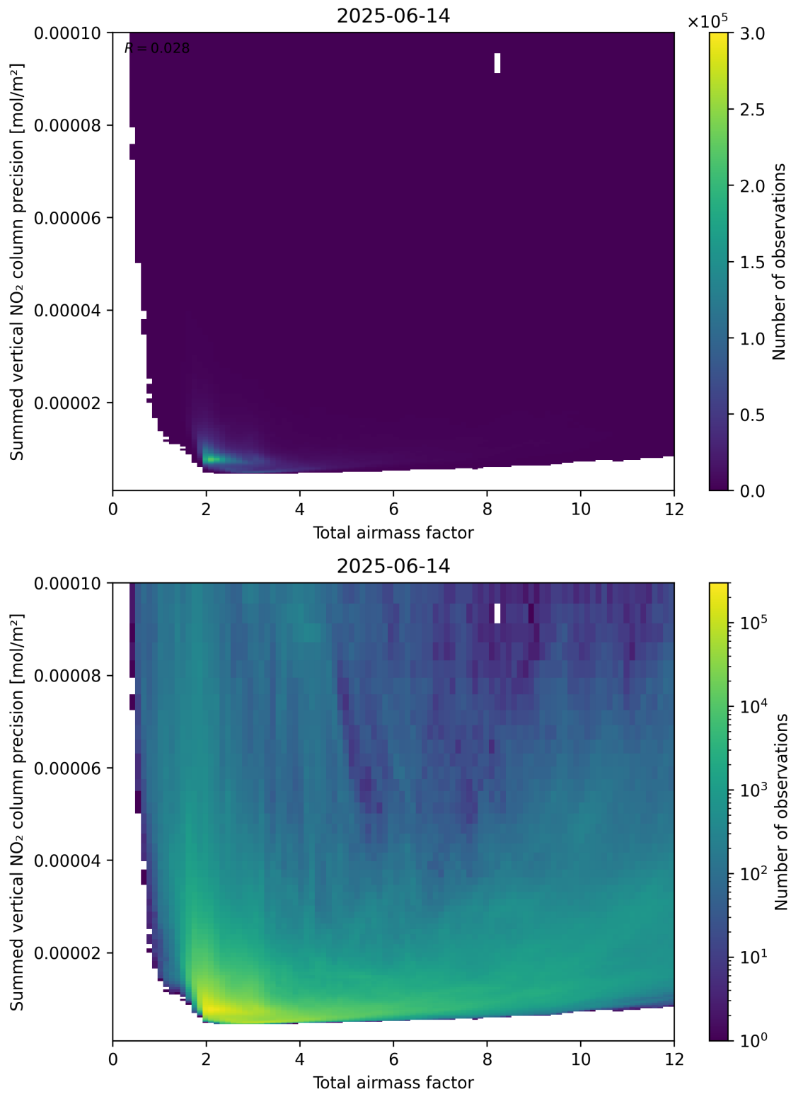
Figure 66: Scatter density plot of “Total airmass factor” against “Summed vertical NO 2 column precision” for 2025-06-13 to 2025-06-15.
