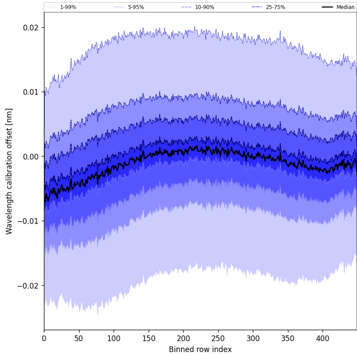
Figure 52: Along track statistics of “Wavelength calibration offset” for 2025-06-13 to 2025-06-15
