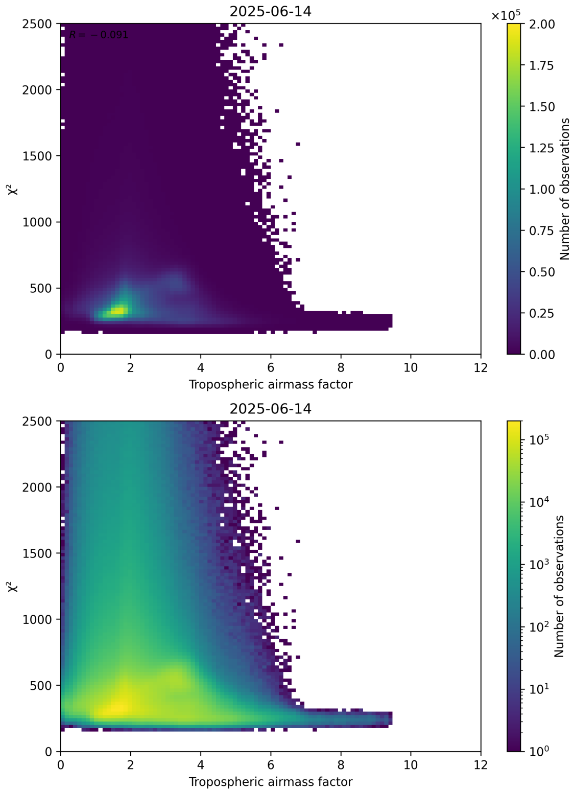
Figure 73: Scatter density plot of “Tropospheric airmass factor” against “ \chi^2 ” for 2025-06-13 to 2025-06-15.
