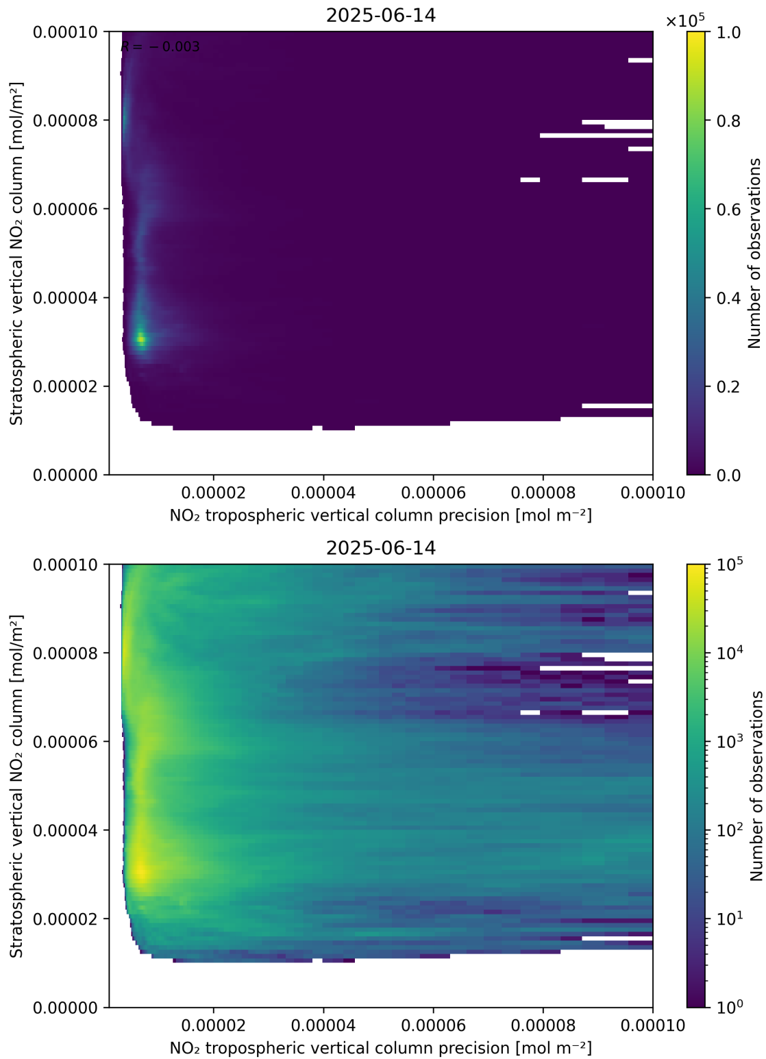
Figure 135: Scatter density plot of “NO 2 tropospheric vertical column precision” against “Stratospheric vertical NO 2 column” for 2025-06-13 to 2025-06-15.
