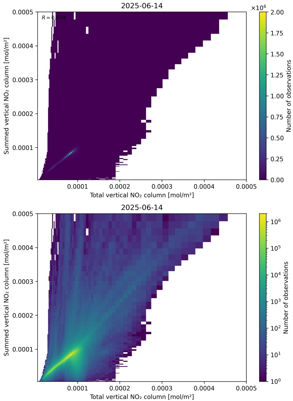
Figure 112: Scatter density plot of “Total vertical NO 2 column” against “Summed vertical NO 2 column” for 2025-06-13 to 2025-06-15.
