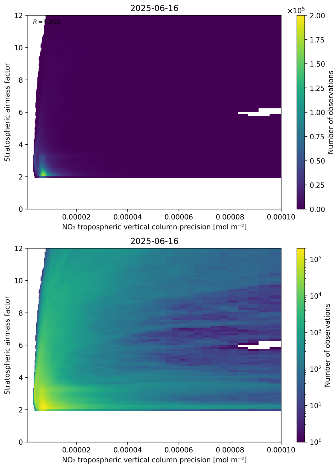
Figure 131: Scatter density plot of “NO 2 tropospheric vertical column precision” against “Stratospheric airmass factor” for 2025-06-16 to 2025-06-17.
