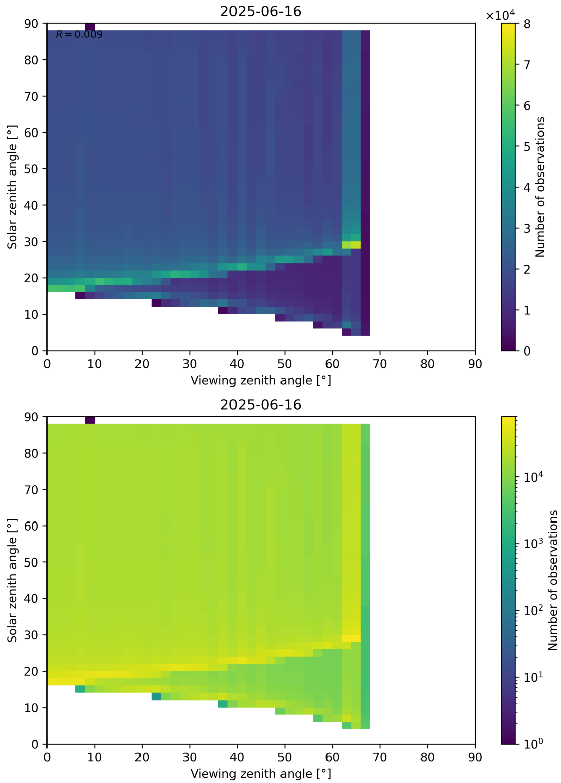
Figure 172: Scatter density plot of “Viewing zenith angle” against “Solar zenith angle” for 2025-06-16 to 2025-06-17.
