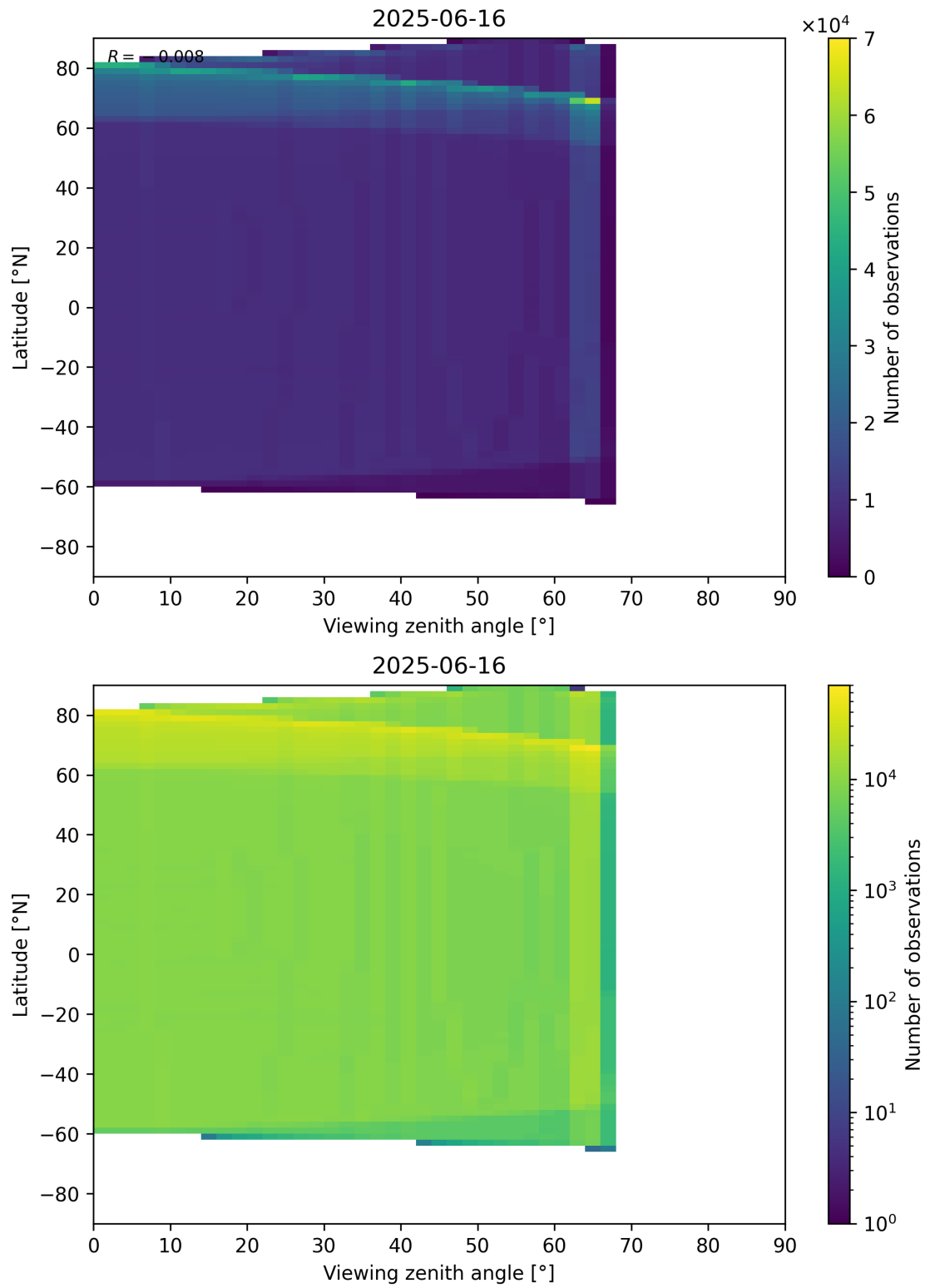
Figure 163: Scatter density plot of “Viewing zenith angle” against “Latitude” for 2025-06-16 to 2025-06-17.
