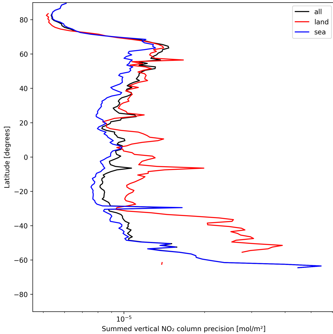
Figure 24: Zonal average of “Summed vertical NO 2 column precision” for 2025-06-16 to 2025-06-17.
