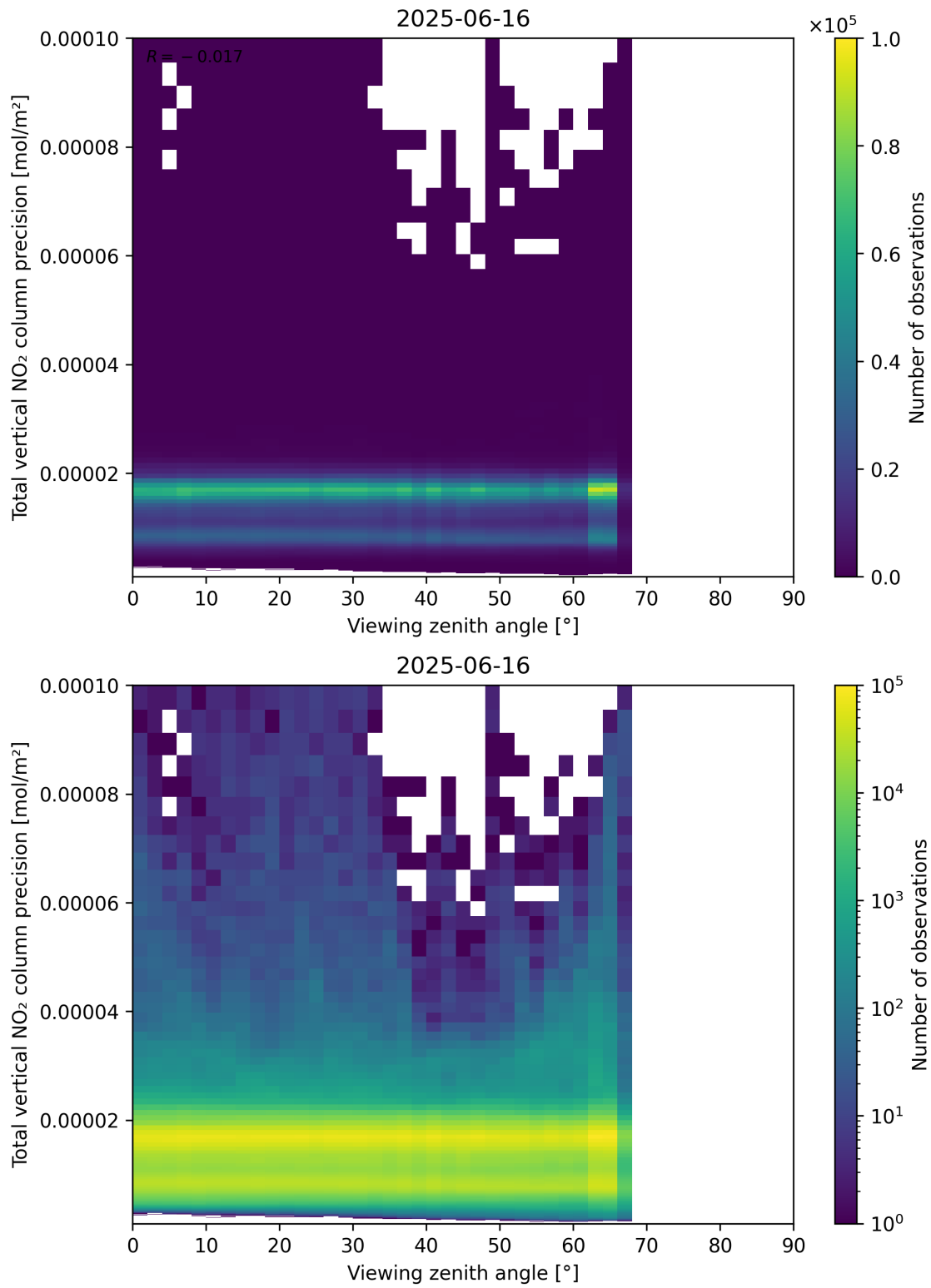
Figure 168: Scatter density plot of “Viewing zenith angle” against “Total vertical NO 2 column precision” for 2025-06-16 to 2025-06-17.
