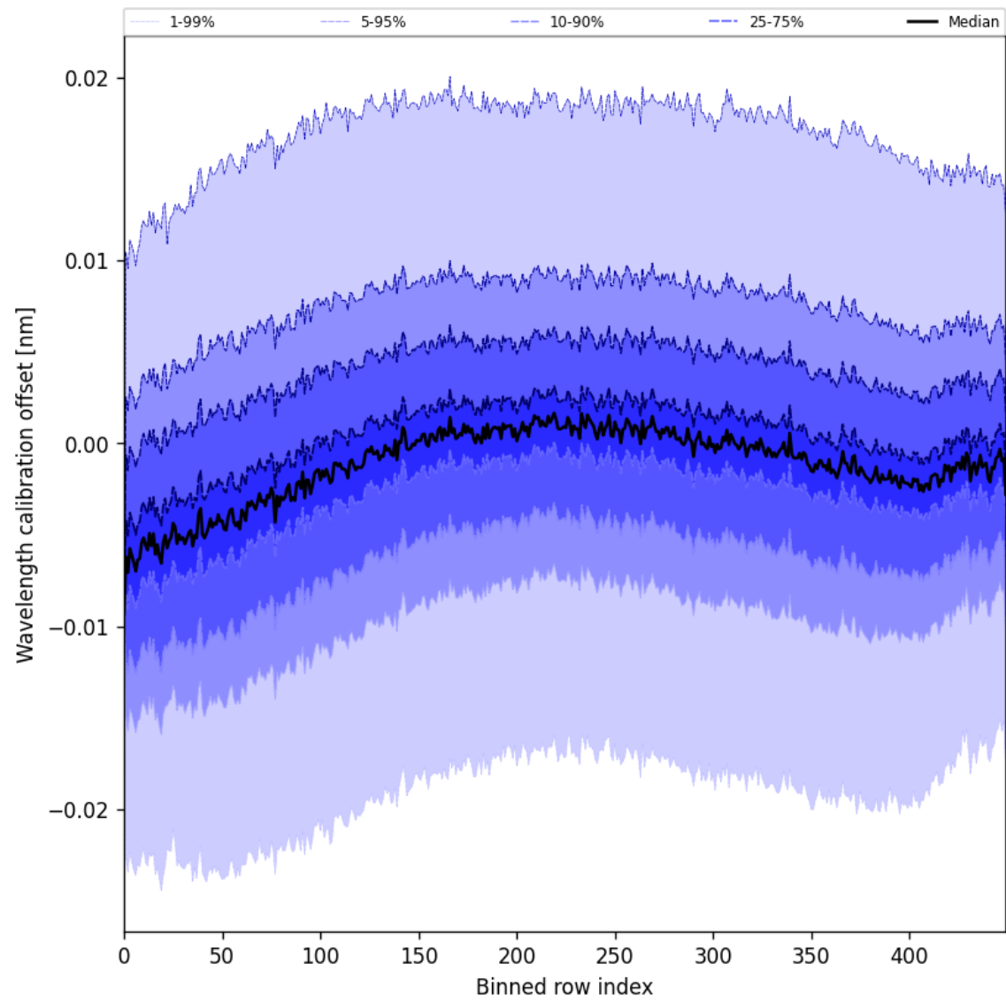
Figure 52: Along track statistics of “Wavelength calibration offset” for 2025-06-16 to 2025-06-17
