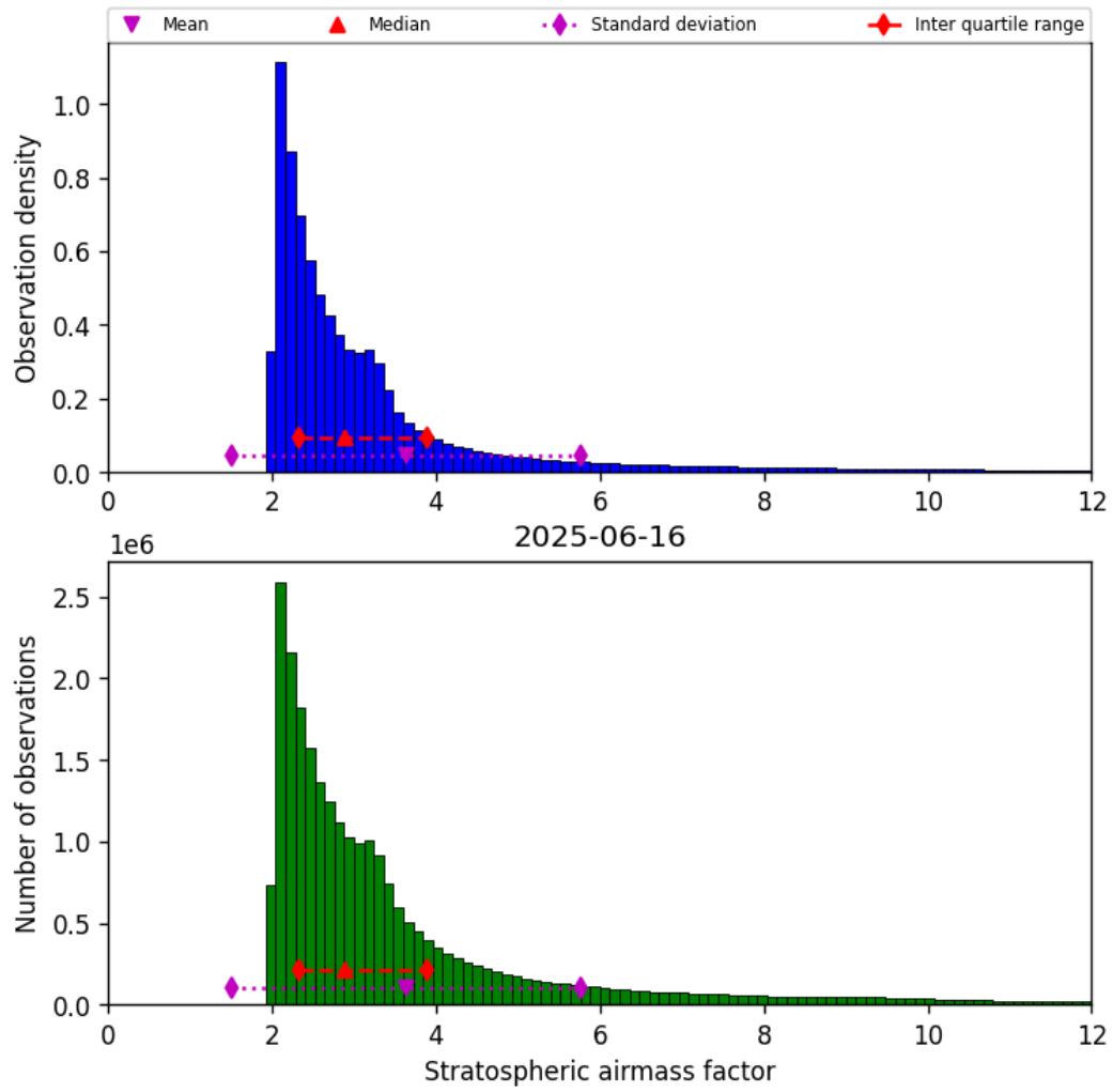
Figure 44: Histogram of “Stratospheric airmass factor” for 2025-06-16 to 2025-06-17
