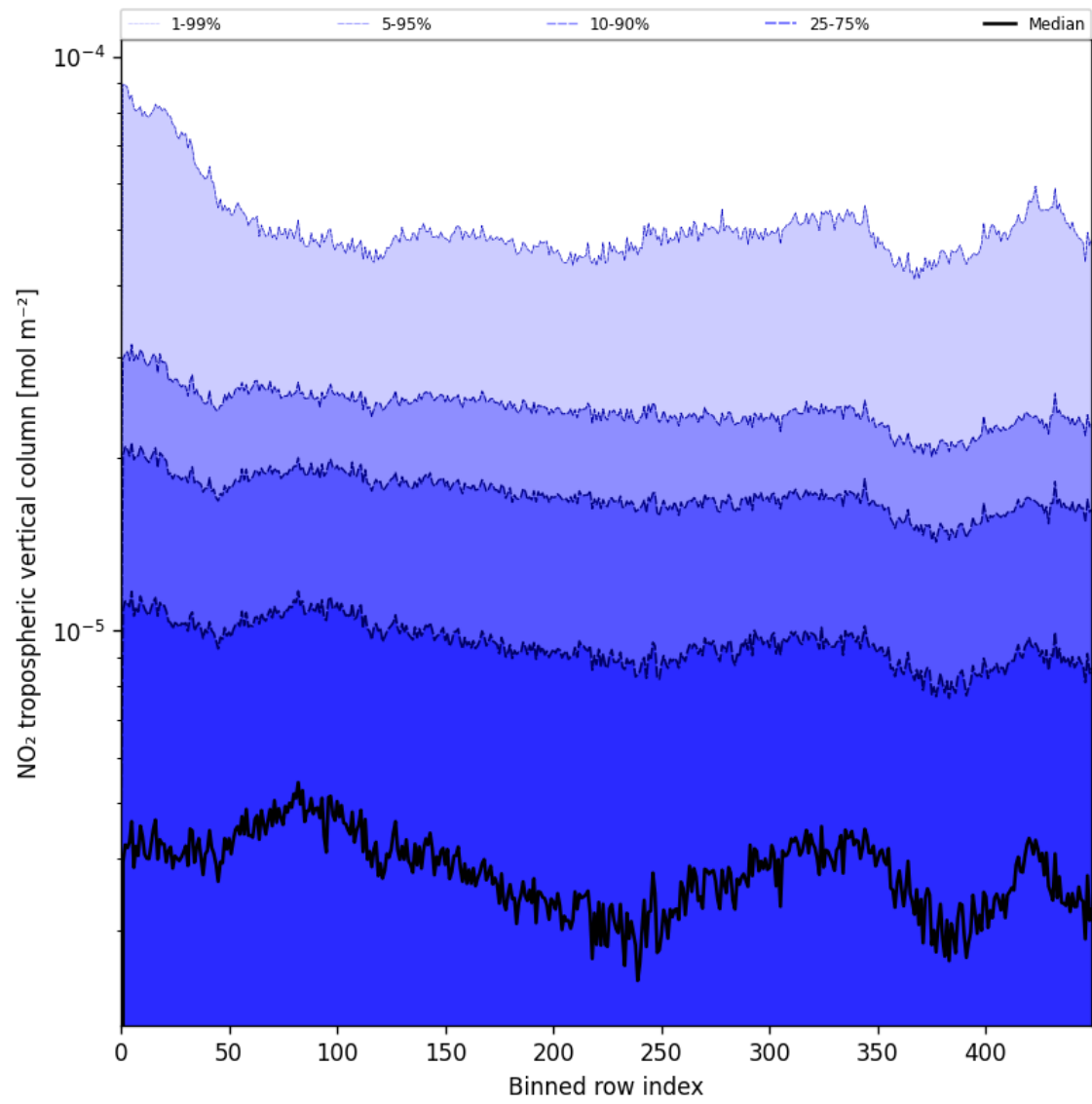
Figure 46: Along track statistics of “NO 2 tropospheric vertical column” for 2025-06-16 to 2025-06-17
