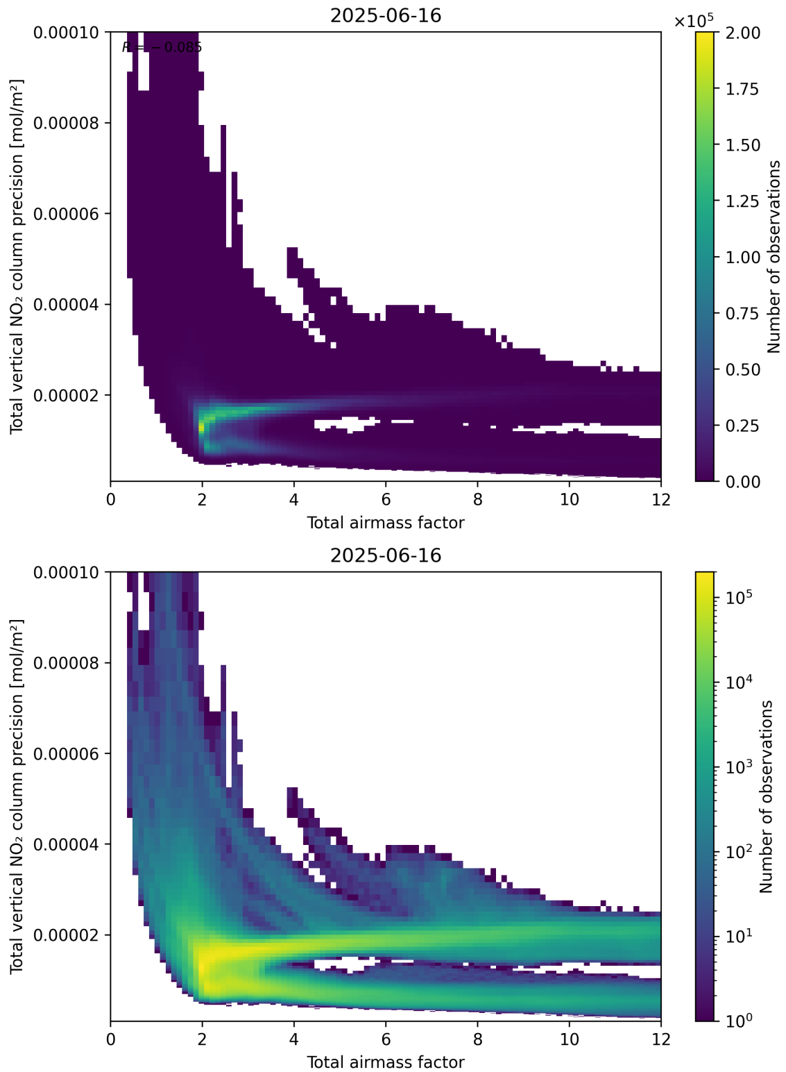
Figure 68: Scatter density plot of “Total airmass factor” against “Total vertical NO 2 column precision” for 2025-06-16 to 2025-06-17.
