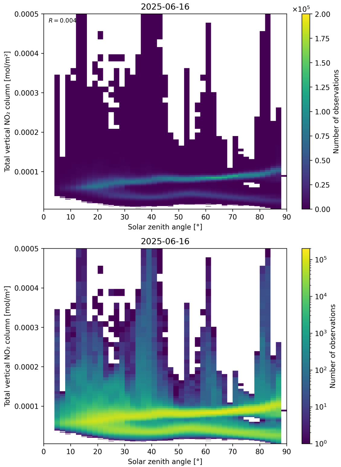
Figure 153: Scatter density plot of “Solar zenith angle” against “Total vertical NO 2 column” for 2025-06-16 to 2025-06-17.
