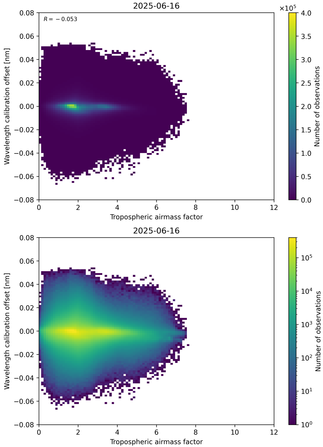
Figure 80: Scatter density plot of “Tropospheric airmass factor” against “Wavelength calibration offset” for 2025-06-16 to 2025-06-17.
