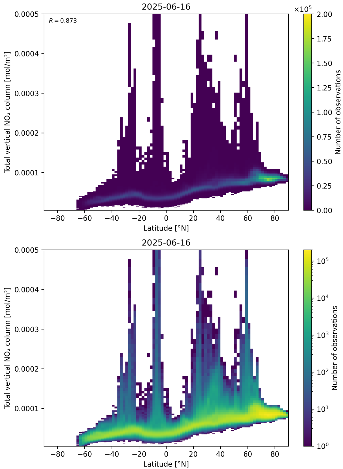
Figure 90: Scatter density plot of “Latitude” against “Total vertical NO 2 column” for 2025-06-16 to 2025-06-17.
