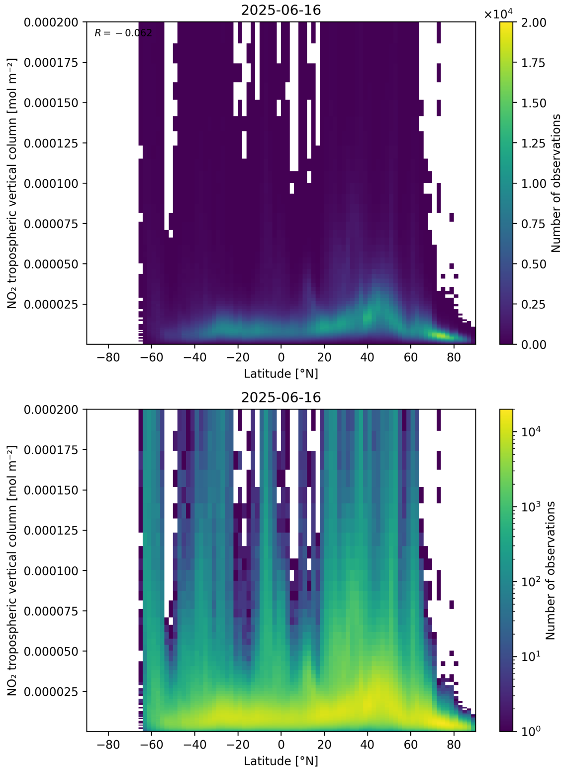
Figure 92: Scatter density plot of “Latitude” against “NO 2 tropospheric vertical column” for 2025-06-16 to 2025-06-17.
