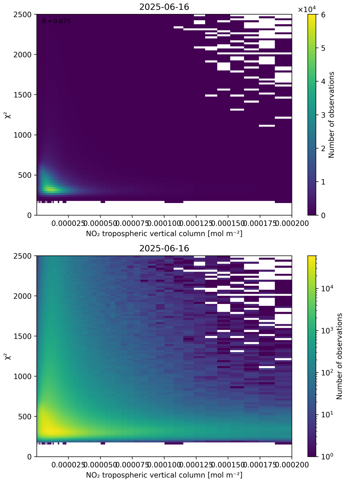
Figure 124: Scatter density plot of “NO 2 tropospheric vertical column” against “ \chi^2 ” for 2025-06-16 to 2025-06-17.
