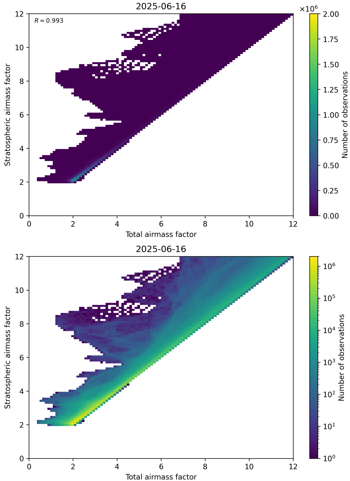
Figure 62: Scatter density plot of “Total airmass factor” against “Stratospheric airmass factor” for 2025-06-16 to 2025-06-17.
