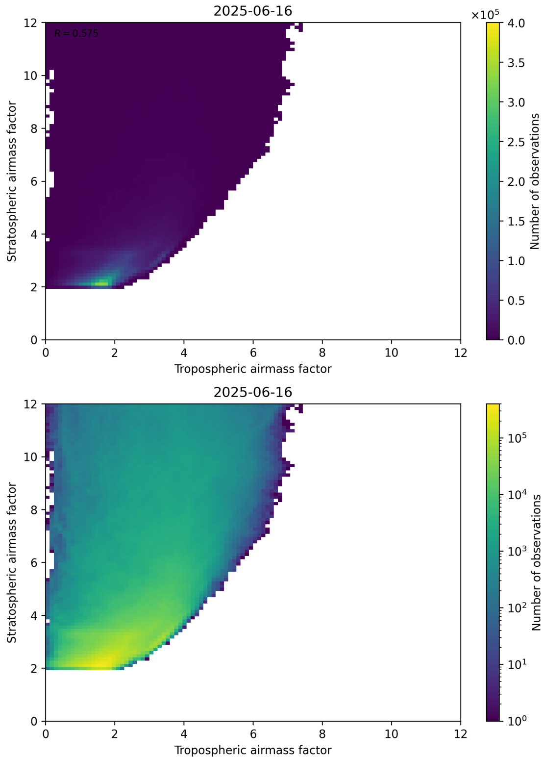
Figure 71: Scatter density plot of “Tropospheric airmass factor” against “Stratospheric airmass factor” for 2025-06-16 to 2025-06-17.
