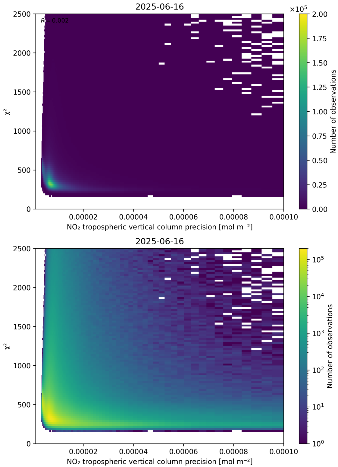
Figure 134: Scatter density plot of “NO 2 tropospheric vertical column precision” against “ \chi^2 ” for 2025-06-16 to 2025-06-17.
