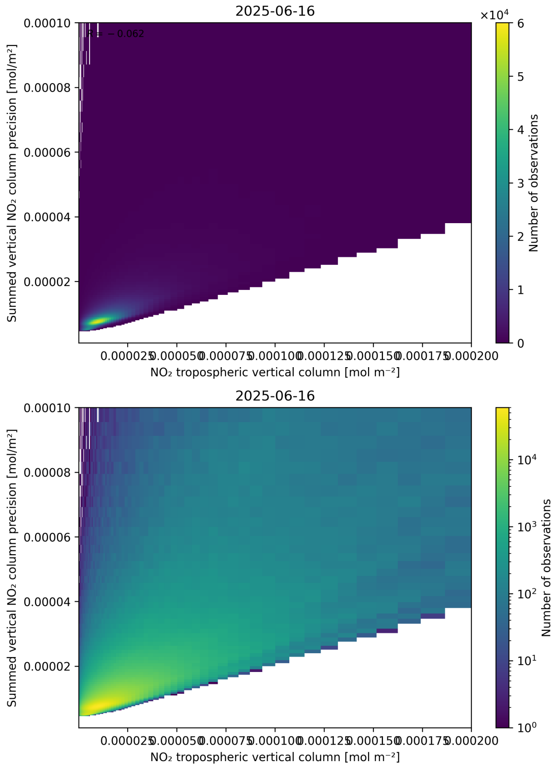
Figure 127: Scatter density plot of “NO 2 tropospheric vertical column” against “Summed vertical NO 2 column precision” for 2025-06-16 to 2025-06-17.
