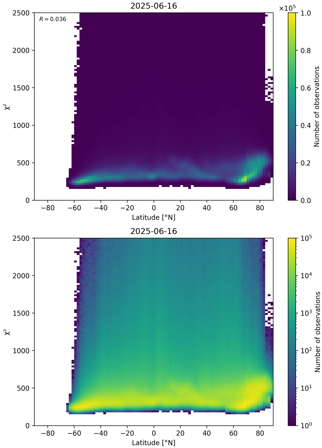
Figure 86: Scatter density plot of “Latitude” against “ \chi^2 ” for 2025-06-16 to 2025-06-17.
