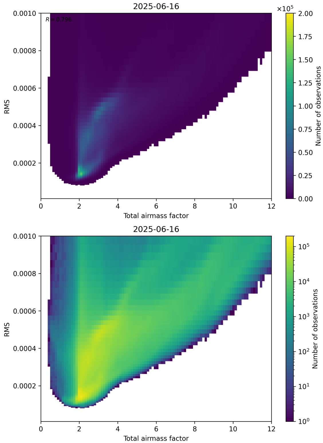
Figure 69: Scatter density plot of “Total airmass factor” against “RMS” for 2025-06-16 to 2025-06-17.
