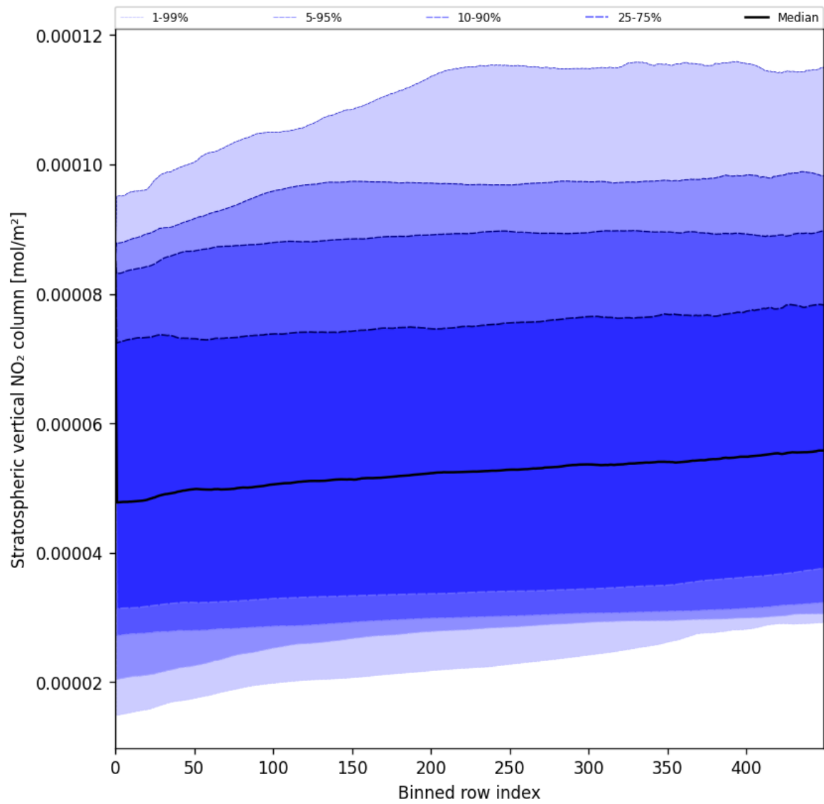
Figure 53: Along track statistics of “Stratospheric vertical NO 2 column” for 2025-06-16 to 2025-06-17
