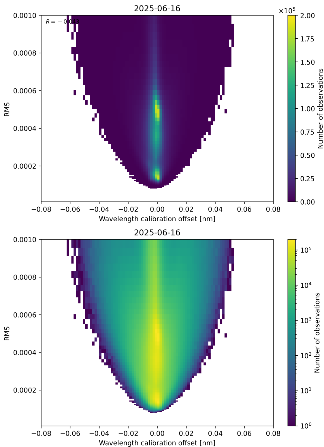
Figure 181: Scatter density plot of “Wavelength calibration offset” against “RMS” for 2025-06-16 to 2025-06-17.
