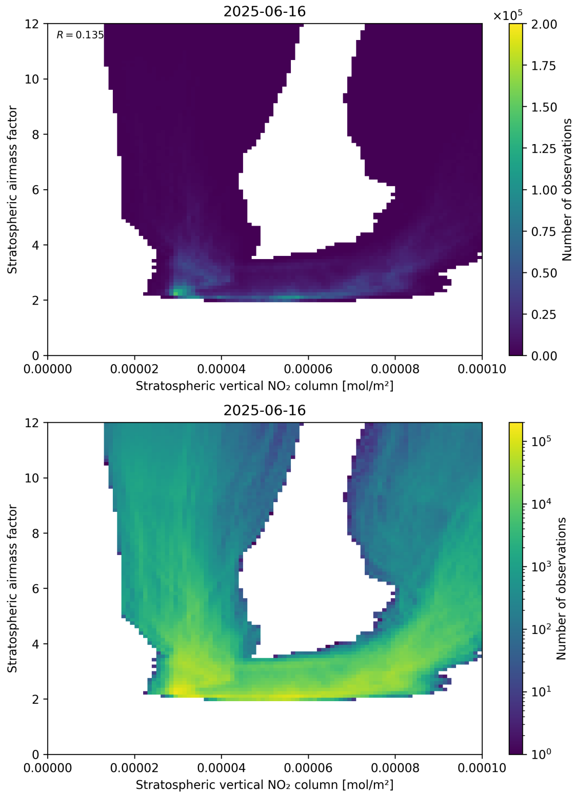
Figure 96: Scatter density plot of “Stratospheric vertical NO 2 column” against “Stratospheric airmass factor” for 2025-06-16 to 2025-06-17.
