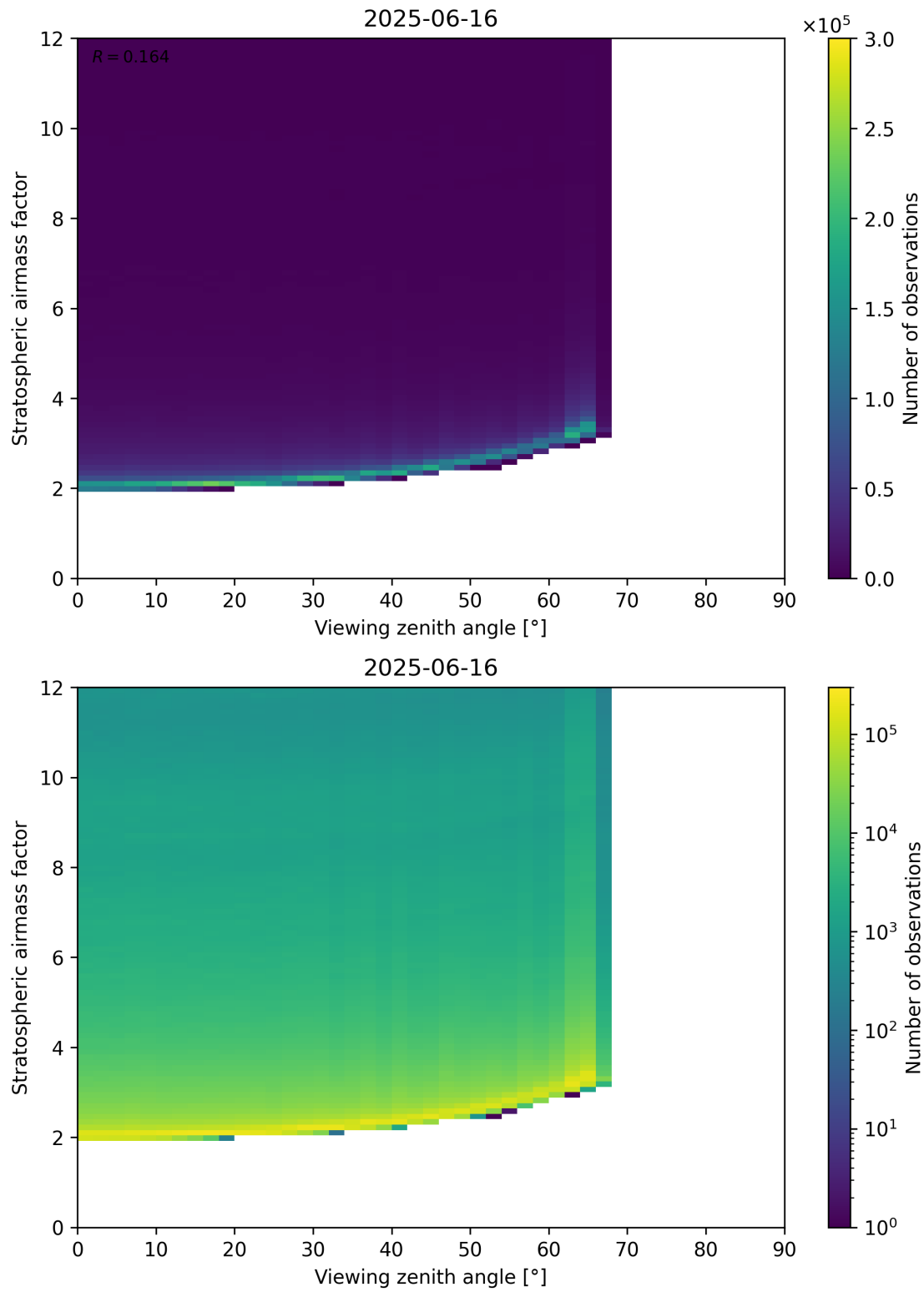
Figure 159: Scatter density plot of “Viewing zenith angle” against “Stratospheric airmass factor” for 2025-06-16 to 2025-06-17.
