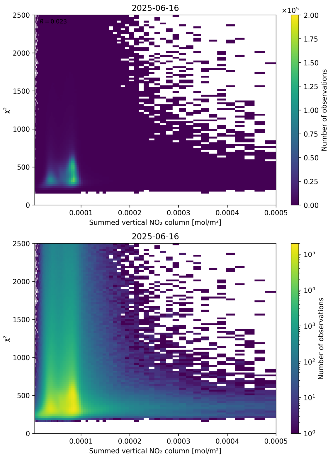
Figure 104: Scatter density plot of “Summed vertical NO 2 column” against “ \chi^2 ” for 2025-06-16 to 2025-06-17.
