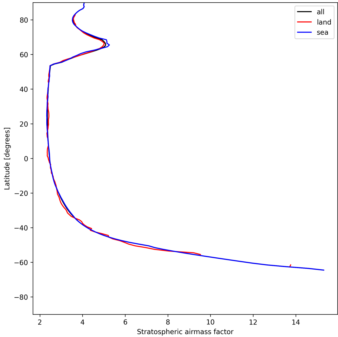
Figure 27: Zonal average of “Stratospheric airmass factor” for 2025-06-16 to 2025-06-17.
