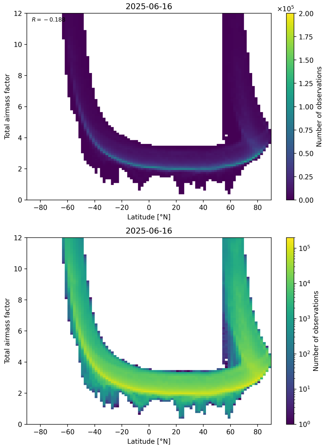
Figure 84: Scatter density plot of “Latitude” against “Total airmass factor” for 2025-06-16 to 2025-06-17.
