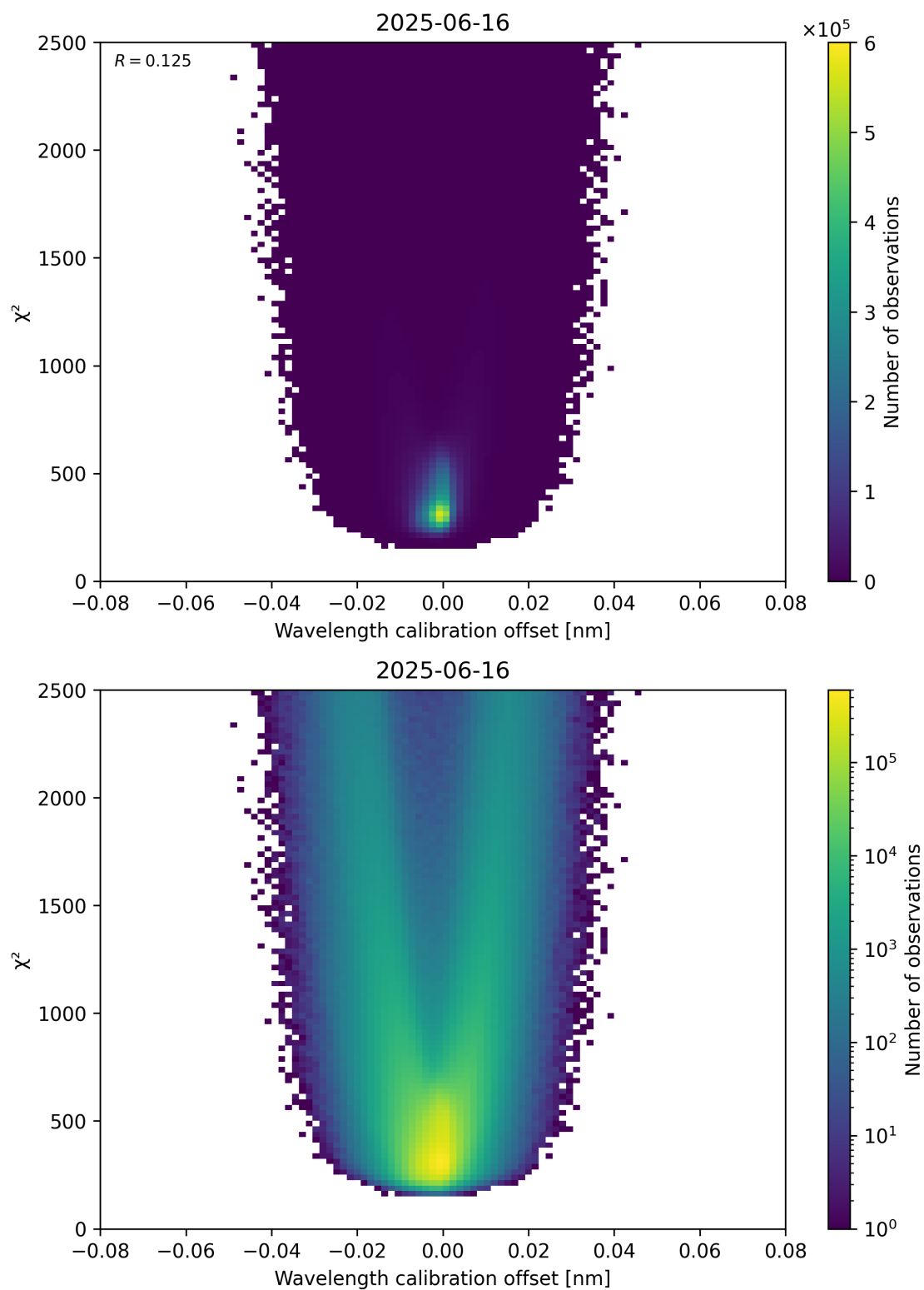
Figure 175: Scatter density plot of “Wavelength calibration offset” against “ \chi^2 ” for 2025-06-16 to 2025-06-17.
