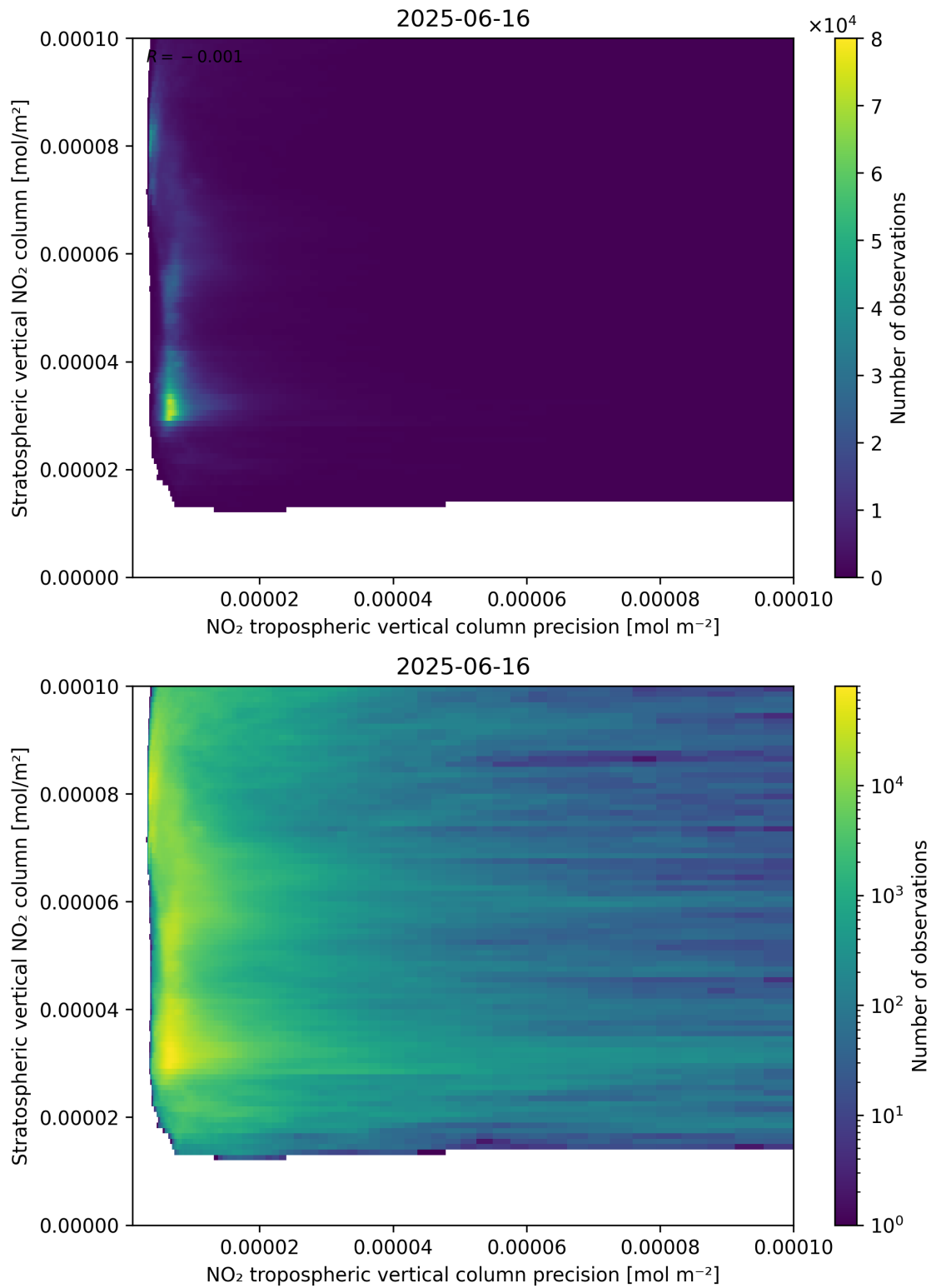
Figure 135: Scatter density plot of “NO 2 tropospheric vertical column precision” against “Stratospheric vertical NO 2 column” for 2025-06-16 to 2025-06-17.
