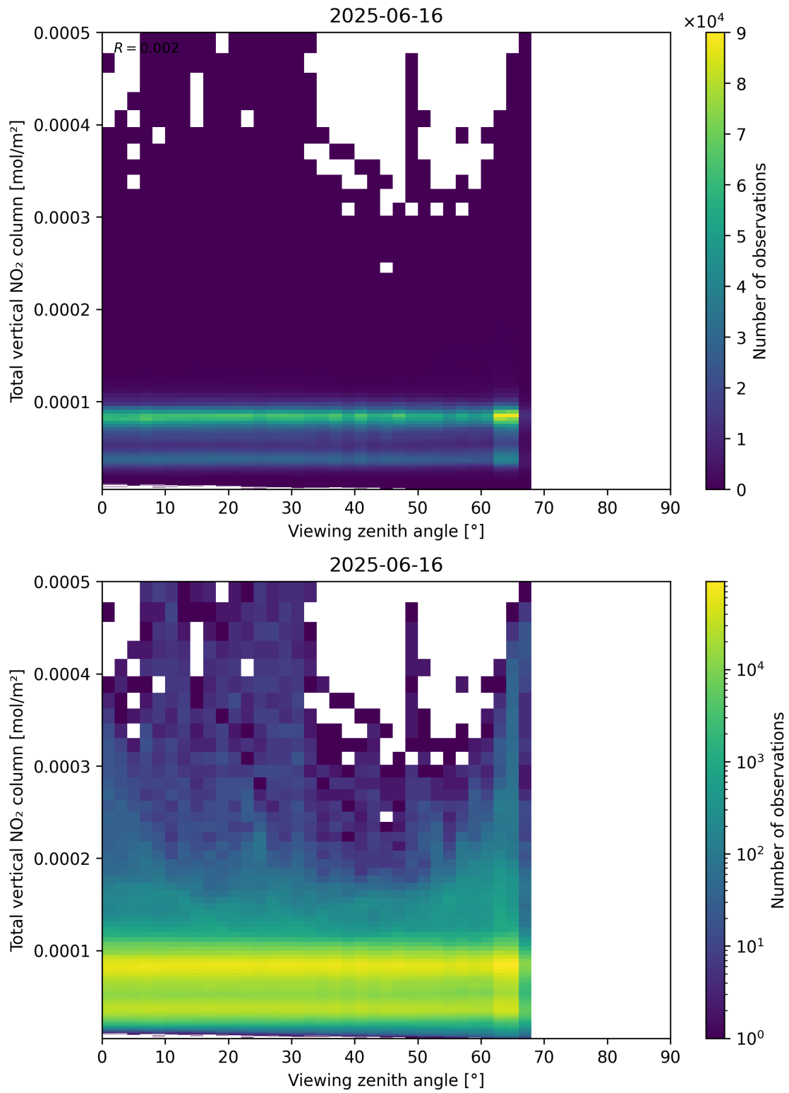
Figure 167: Scatter density plot of “Viewing zenith angle” against “Total vertical NO 2 column” for 2025-06-16 to 2025-06-17.
