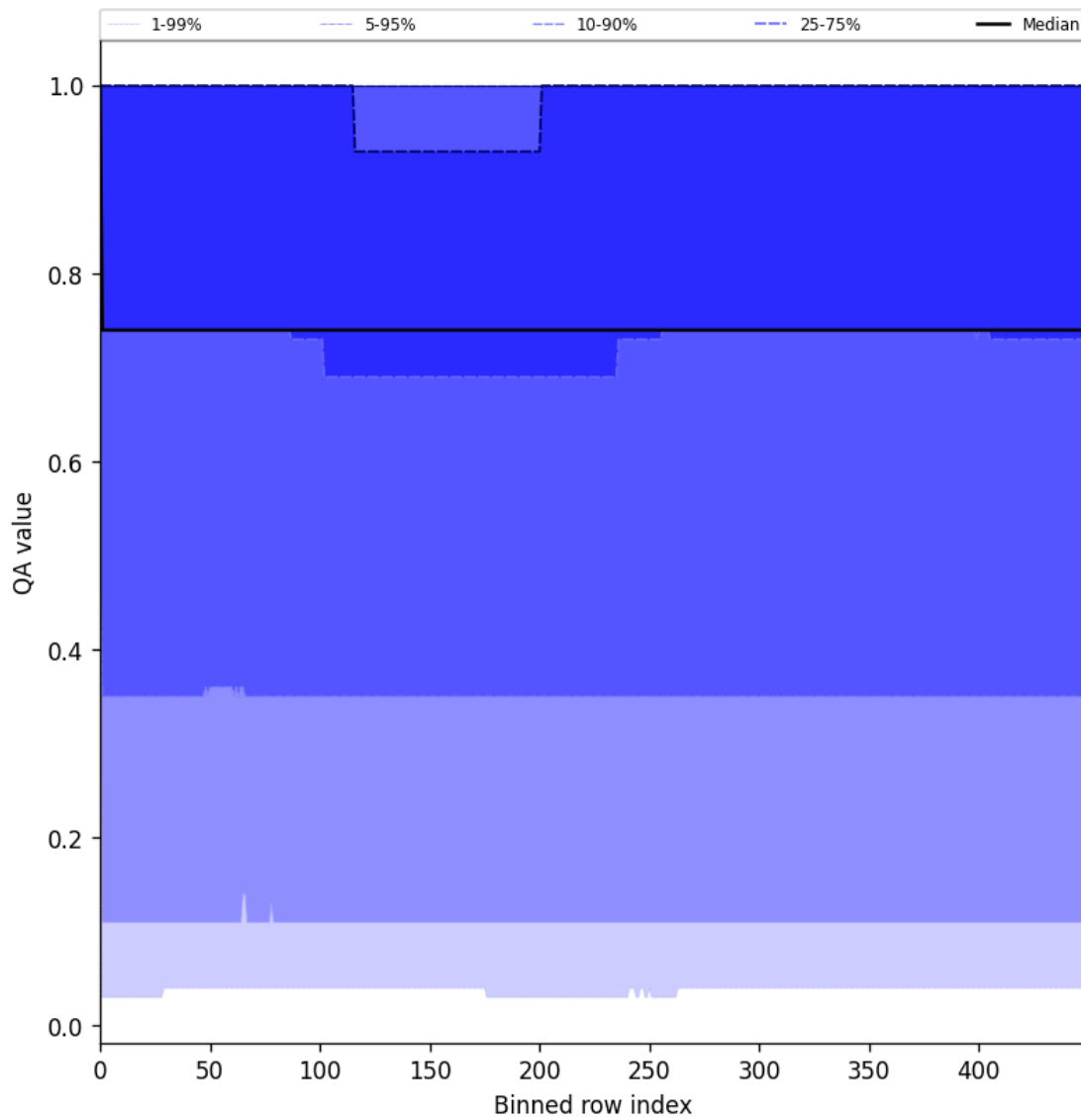
Figure 45: Along track statistics of “QA value” for 2025-06-16 to 2025-06-17
