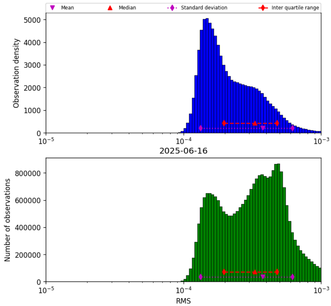
Figure 43: Histogram of “RMS” for 2025-06-16 to 2025-06-17
