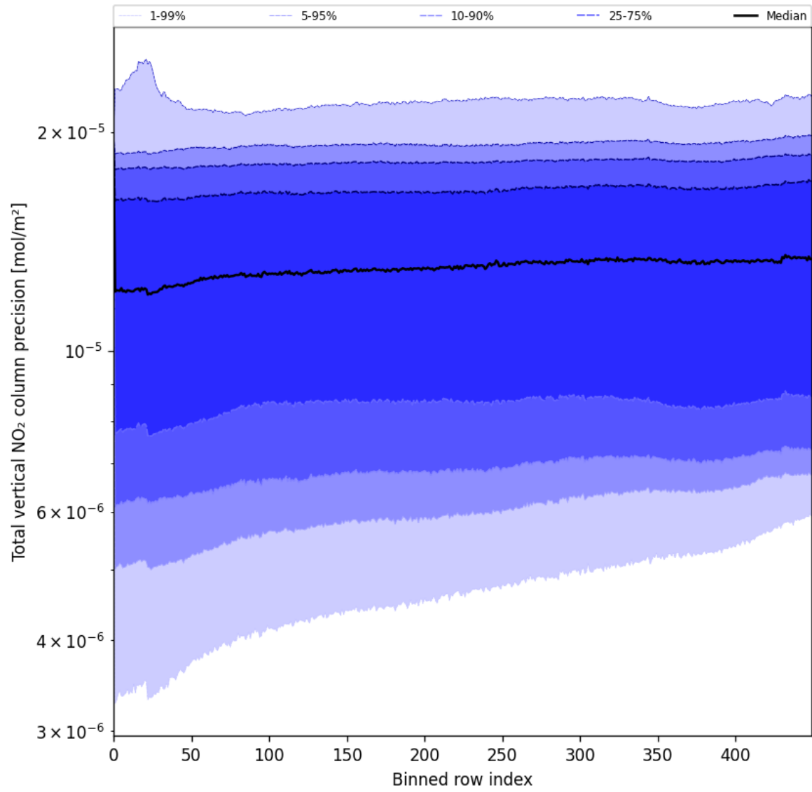
Figure 56: Along track statistics of “Total vertical NO 2 column precision” for 2025-06-16 to 2025-06-17
