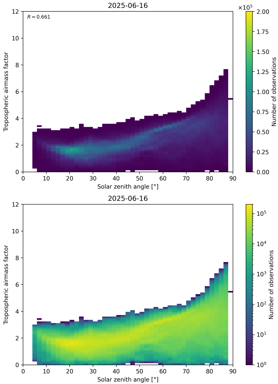
Figure 147: Scatter density plot of “Solar zenith angle” against “Tropospheric airmass factor” for 2025-06-16 to 2025-06-17.
