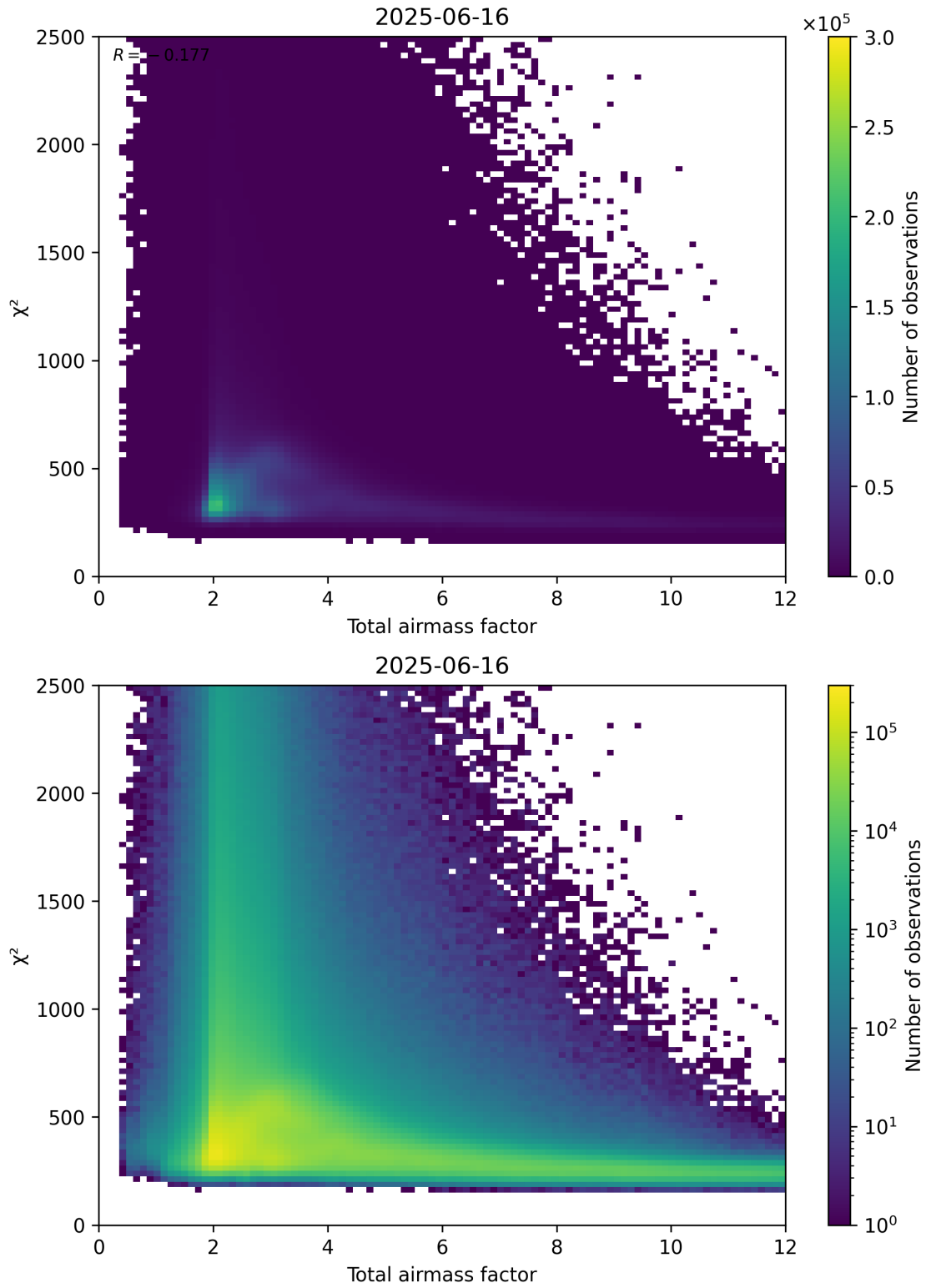
Figure 63: Scatter density plot of “Total airmass factor” against “ \chi^2 ” for 2025-06-16 to 2025-06-17.
