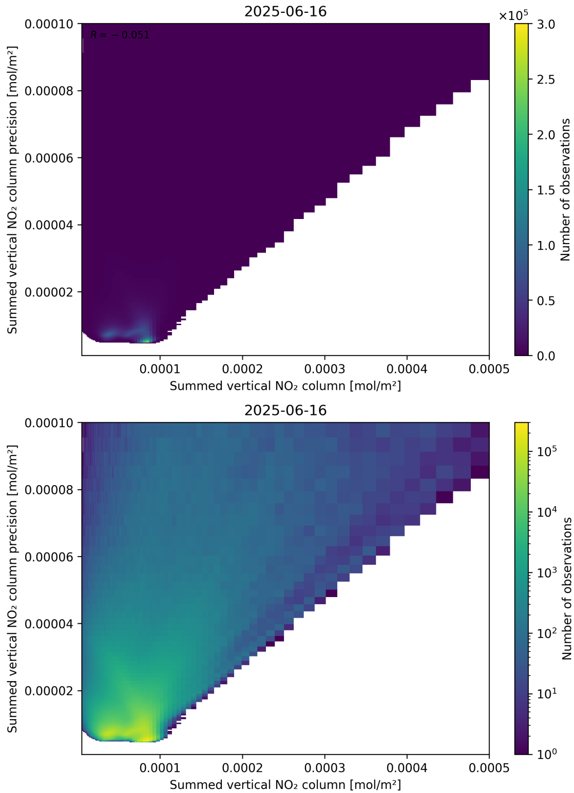
Figure 105: Scatter density plot of “Summed vertical NO 2 column” against “Summed vertical NO 2 column precision” for 2025-06-16 to 2025-06-17.
