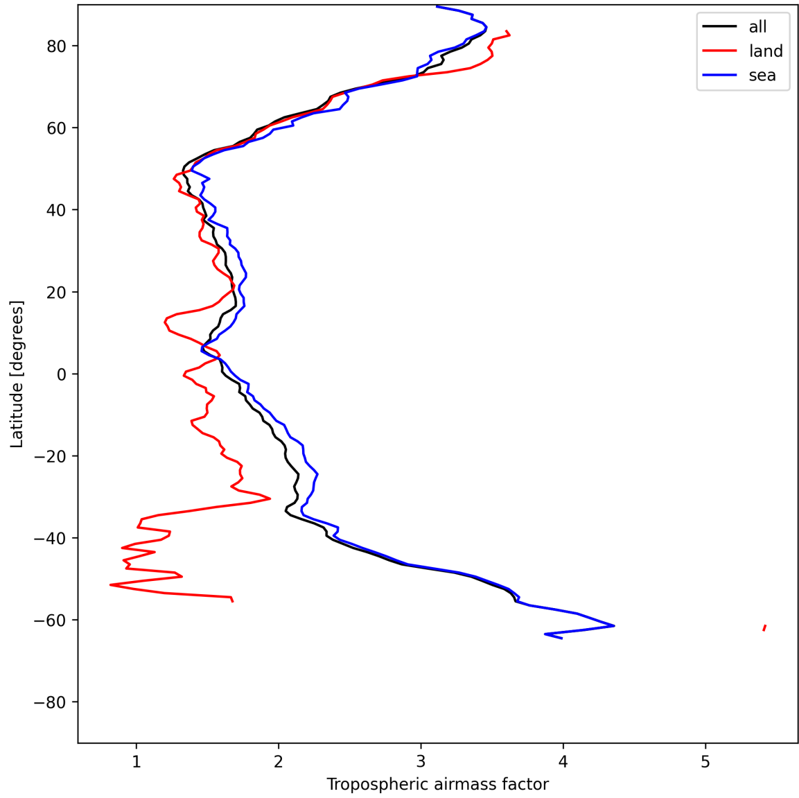
Figure 14: Zonal average of “Tropospheric airmass factor” for 2025-06-16 to 2025-06-17.
