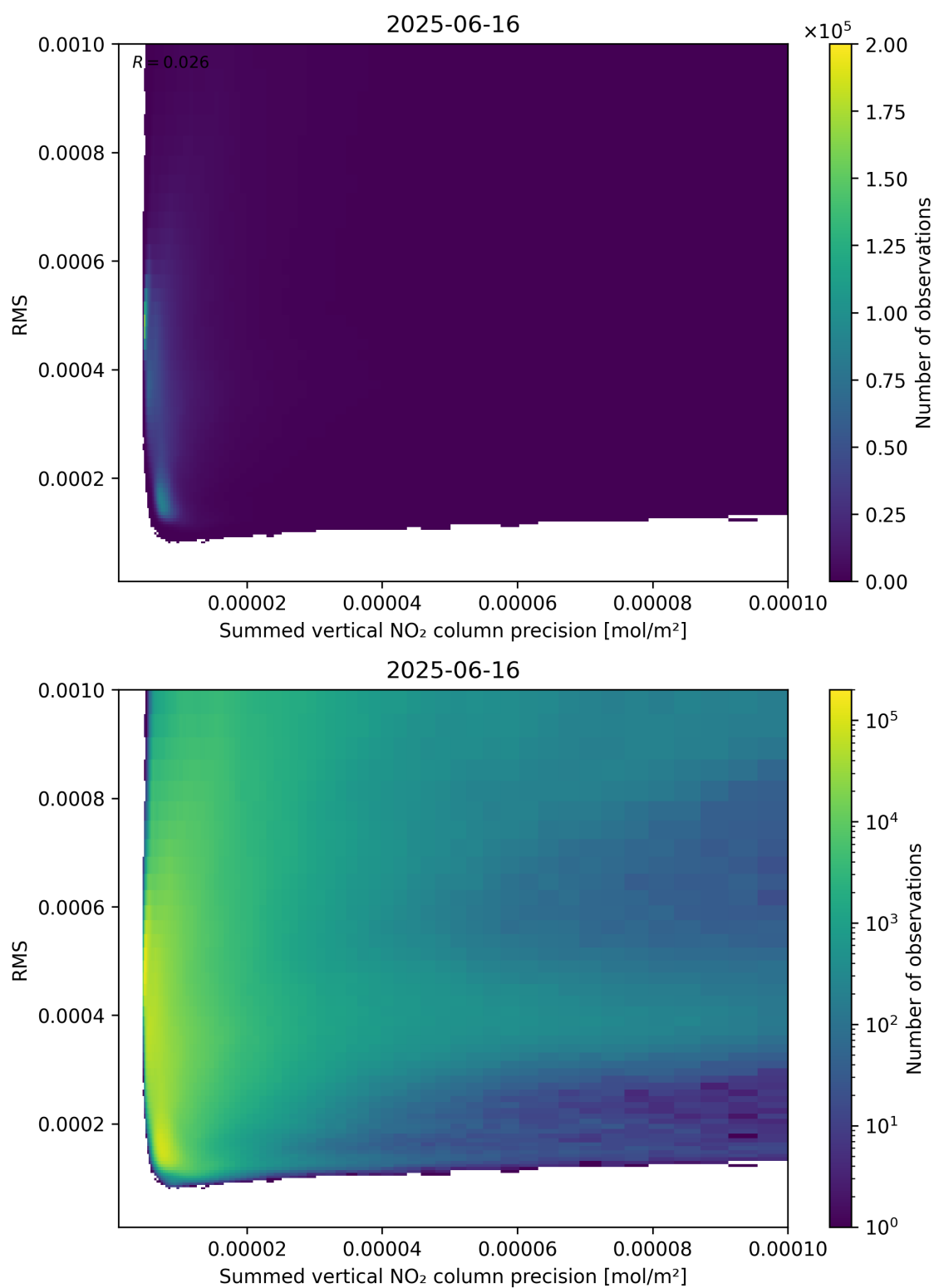
Figure 108: Scatter density plot of “Summed vertical NO 2 column precision” against “RMS” for 2025-06-16 to 2025-06-17.
