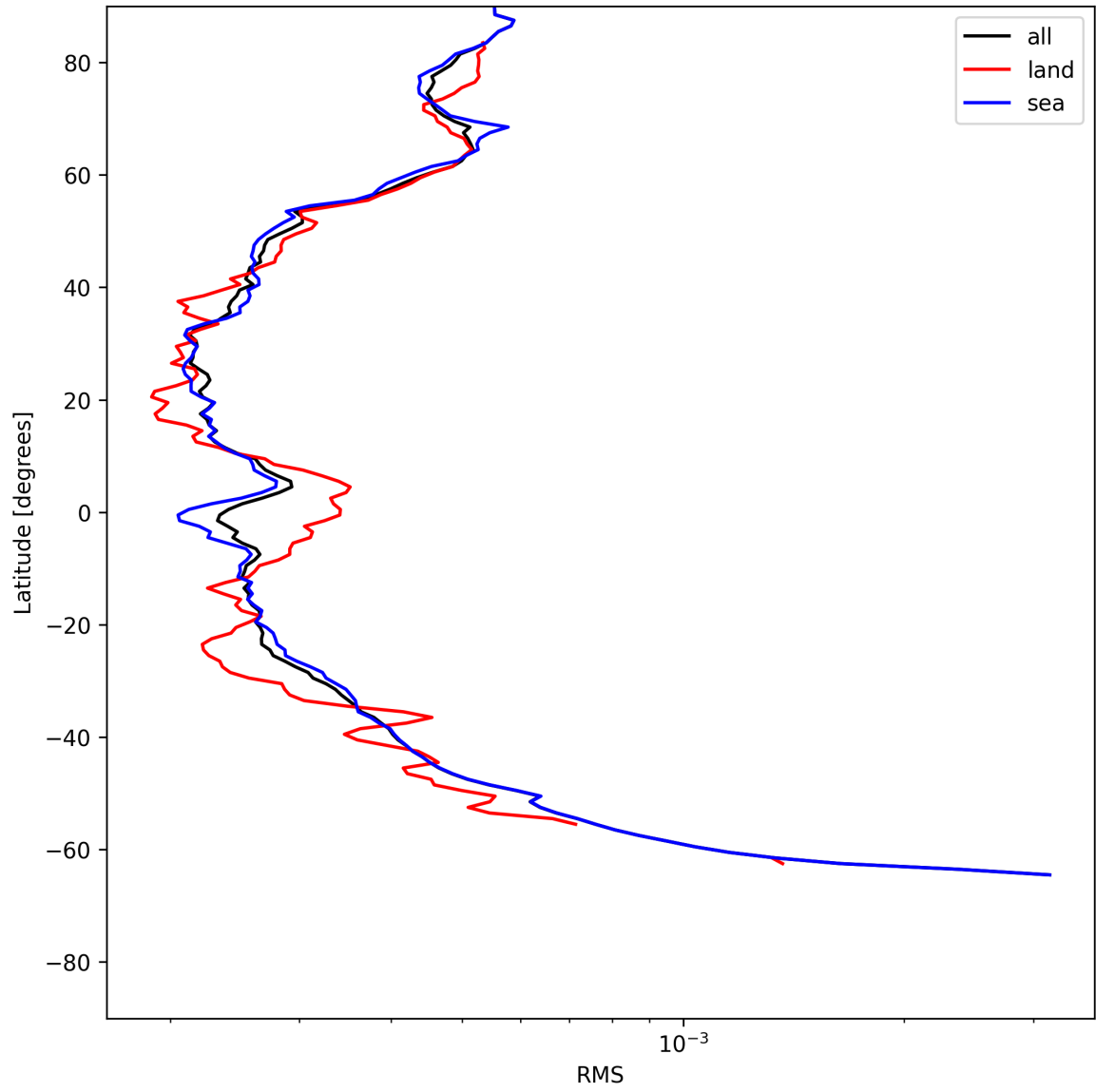
Figure 26: Zonal average of “RMS” for 2025-06-16 to 2025-06-17.
