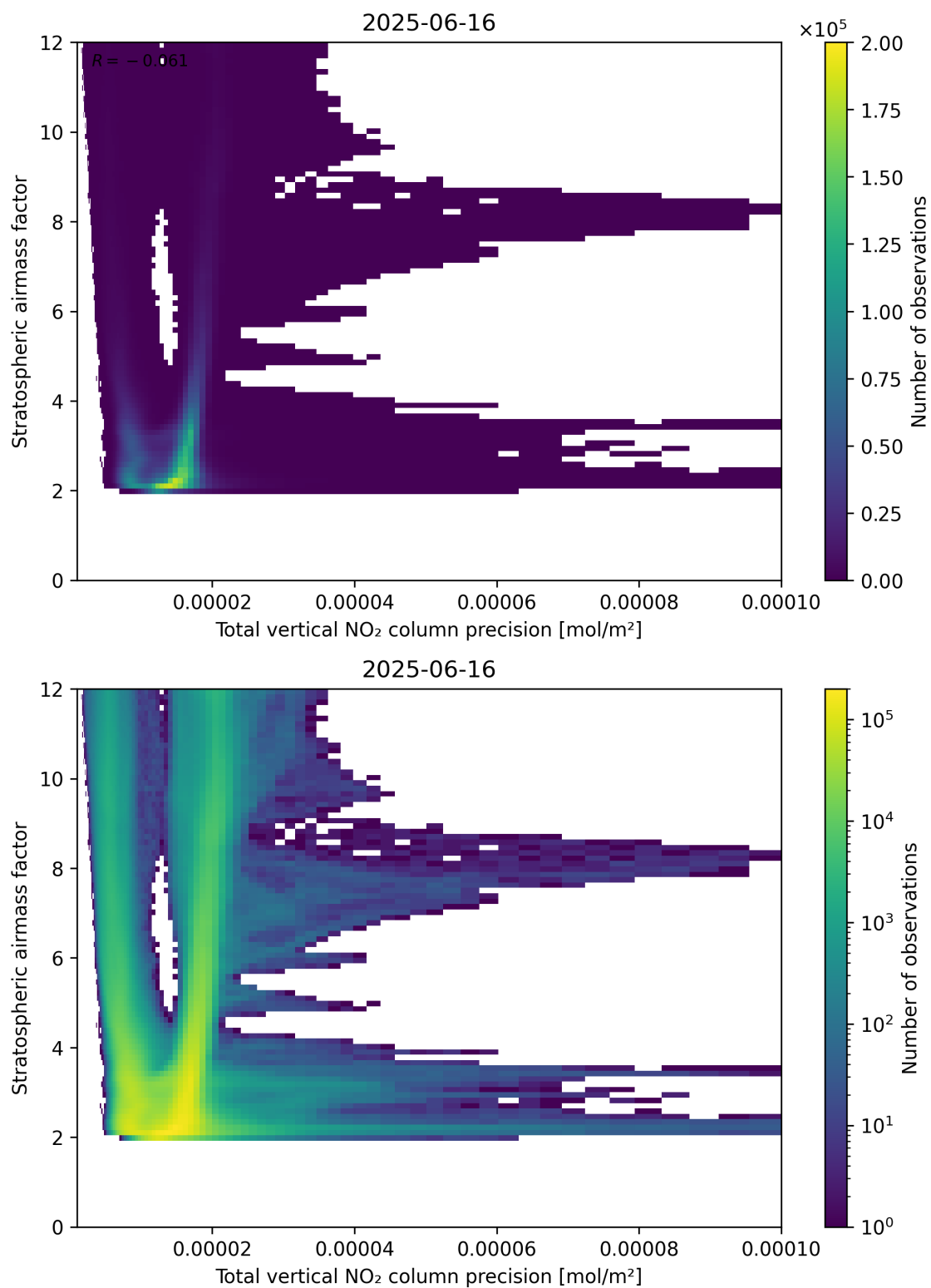
Figure 115: Scatter density plot of “Total vertical NO 2 column precision” against “Stratospheric air mass factor” for 2025-06-16 to 2025-06-17.
