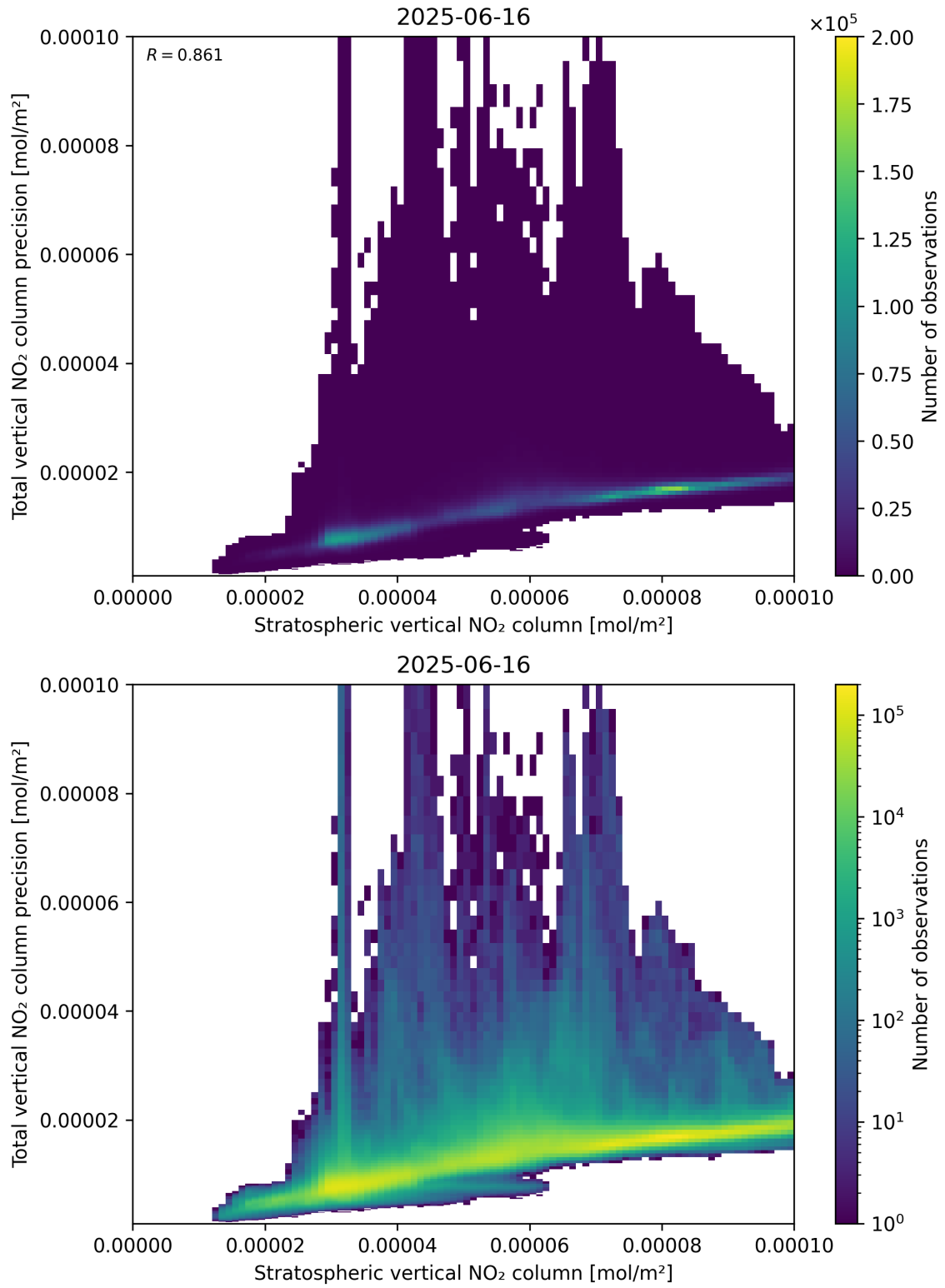
Figure 101: Scatter density plot of “Stratospheric vertical NO 2 column” against “Total vertical NO 2 column precision” for 2025-06-16 to 2025-06-17.
