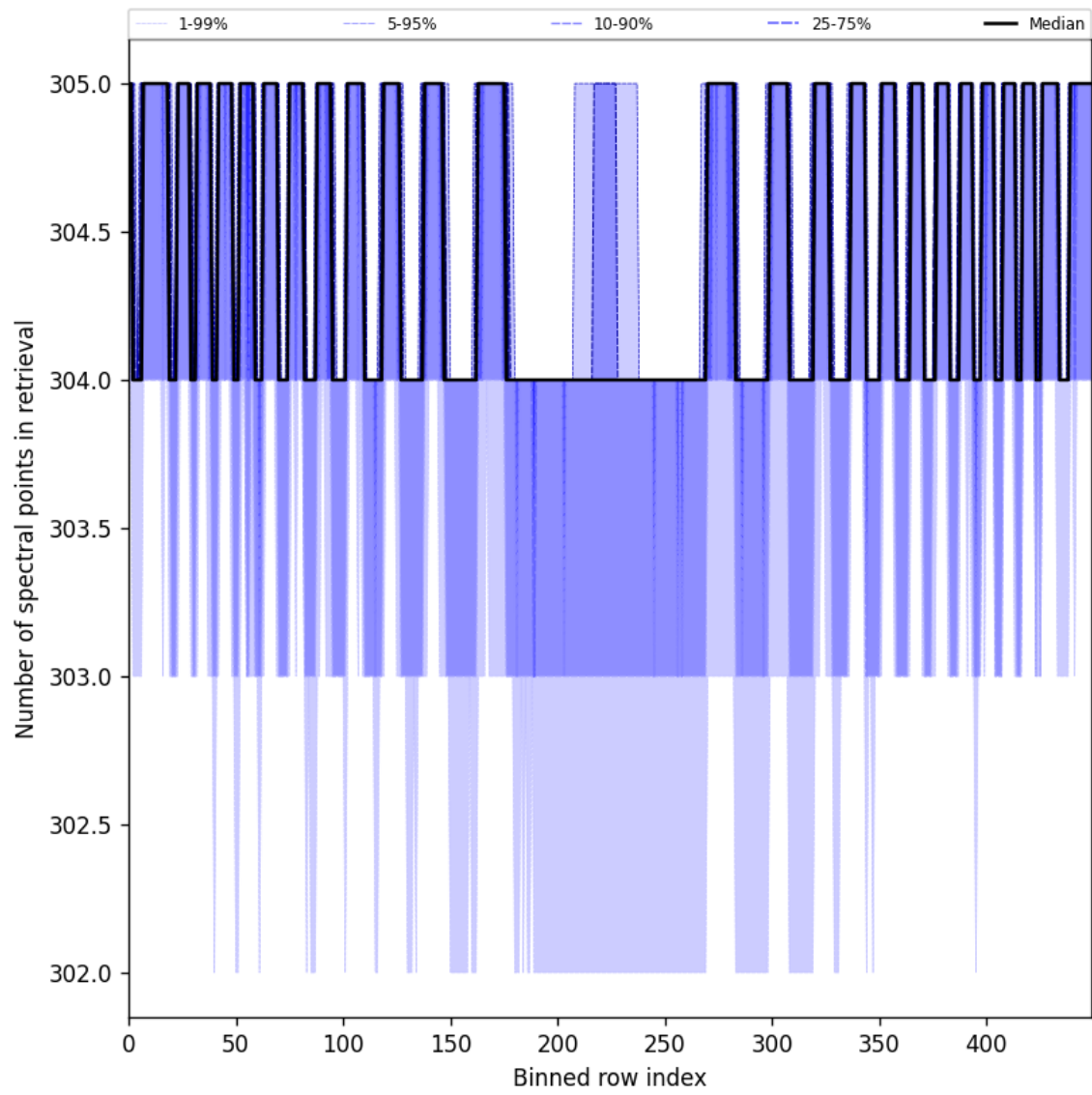
Figure 50: Along track statistics of “Number of spectral points in retrieval” for 2025-06-16 to 2025-06-17
