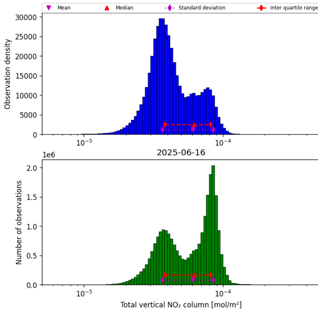
Figure 38: Histogram of “Total vertical NO 2 column” for 2025-06-16 to 2025-06-17
