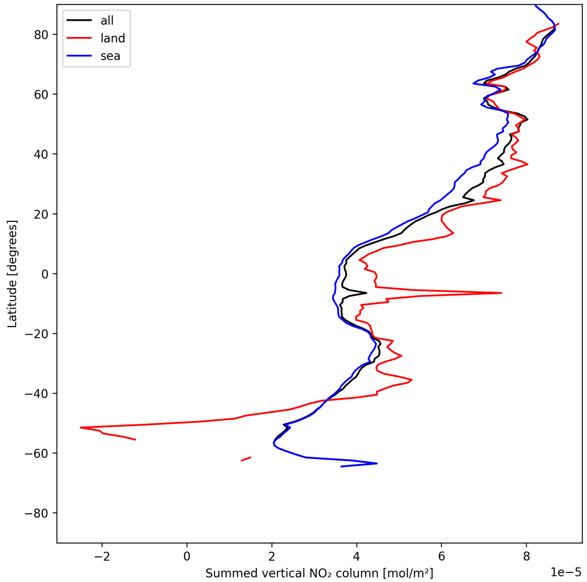
Figure 23: Zonal average of “Summed vertical NO 2 column” for 2025-06-16 to 2025-06-17.
