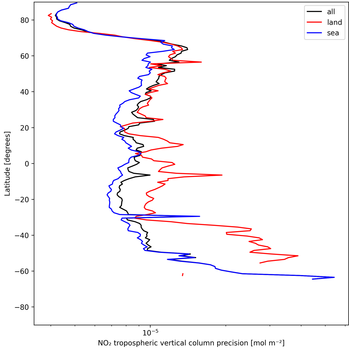
Figure 13: Zonal average of “NO 2 tropospheric vertical column precision” for 2025-06-16 to 2025-06-17.
