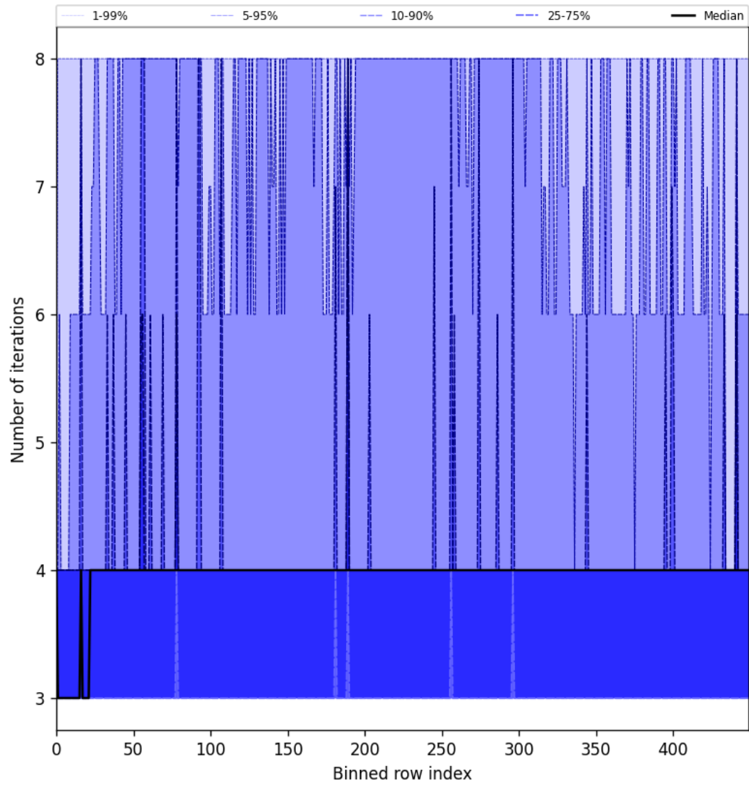
Figure 51: Along track statistics of “Number of iterations” for 2025-06-16 to 2025-06-17
