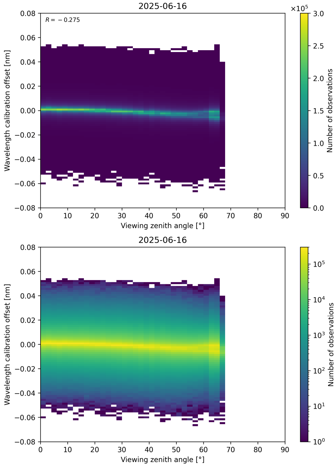
Figure 173: Scatter density plot of “Viewing zenith angle” against “Wavelength calibration offset” for 2025-06-16 to 2025-06-17.
