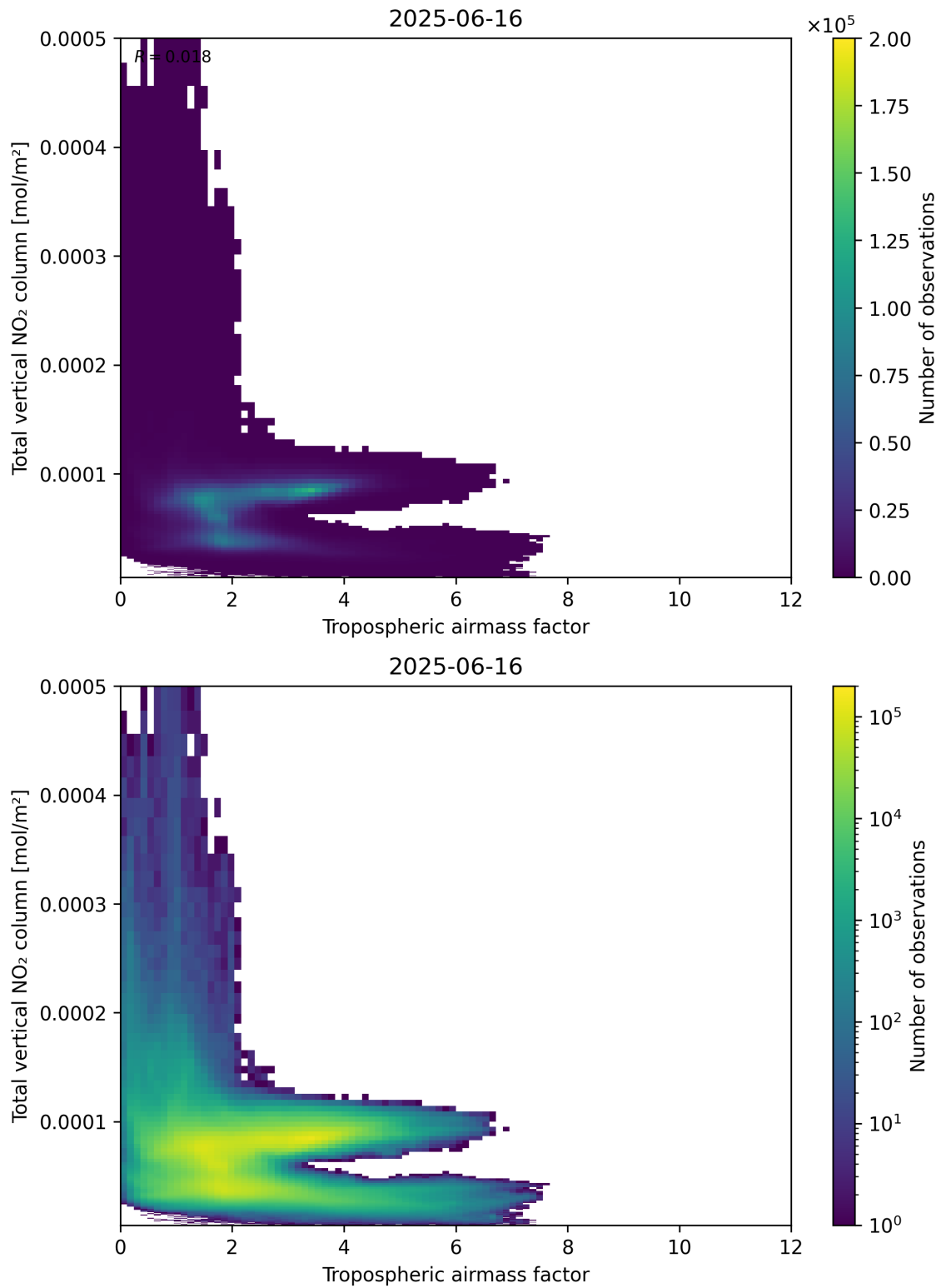
Figure 77: Scatter density plot of “Tropospheric airmass factor” against “Total vertical NO 2 column” for 2025-06-16 to 2025-06-17.
