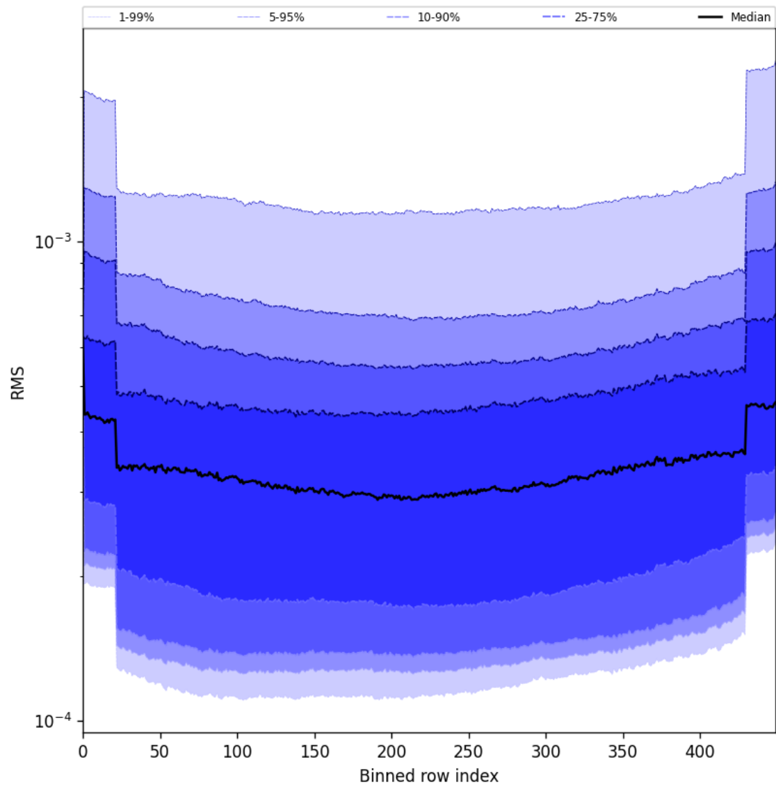
Figure 60: Along track statistics of “RMS” for 2025-06-16 to 2025-06-17
