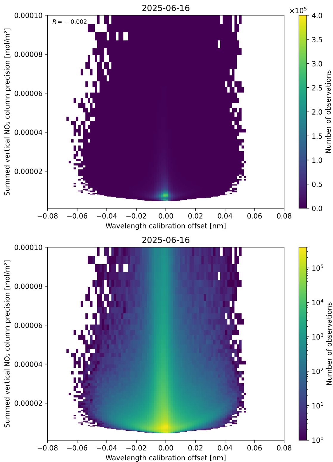
Figure 178: Scatter density plot of “Wavelength calibration offset” against “Summed vertical NO 2 column precision” for 2025-06-16 to 2025-06-17.
