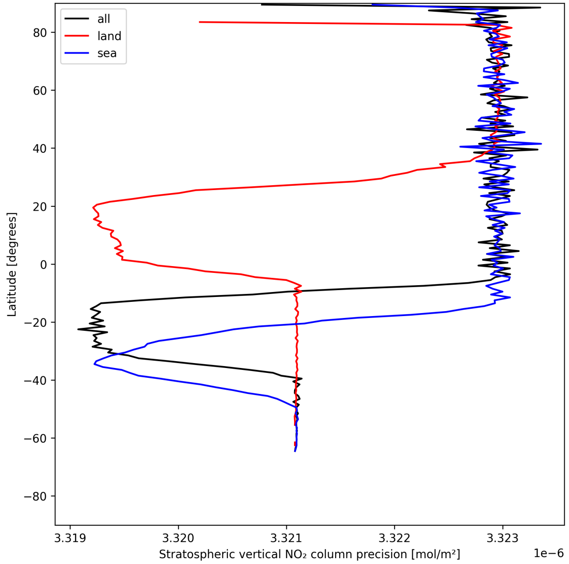
Figure 20: Zonal average of “Stratospheric vertical NO 2 column precision” for 2025-06-16 to 2025-06-17.
