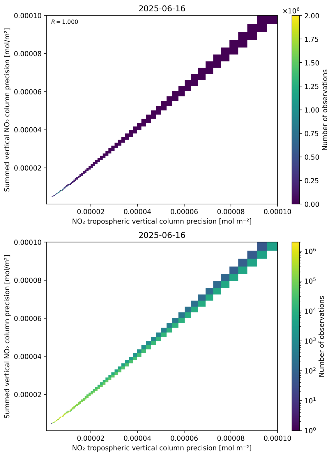
Figure 137: Scatter density plot of “NO 2 tropospheric vertical column precision” against “Summed vertical NO 2 column precision” for 2025-06-16 to 2025-06-17.
