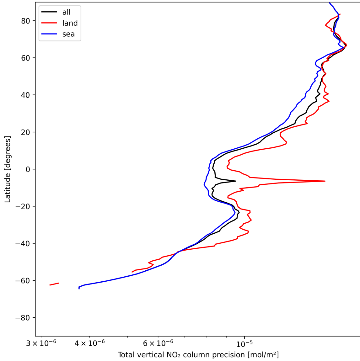
Figure 22: Zonal average of “Total vertical NO 2 column precision” for 2025-06-16 to 2025-06-17.
