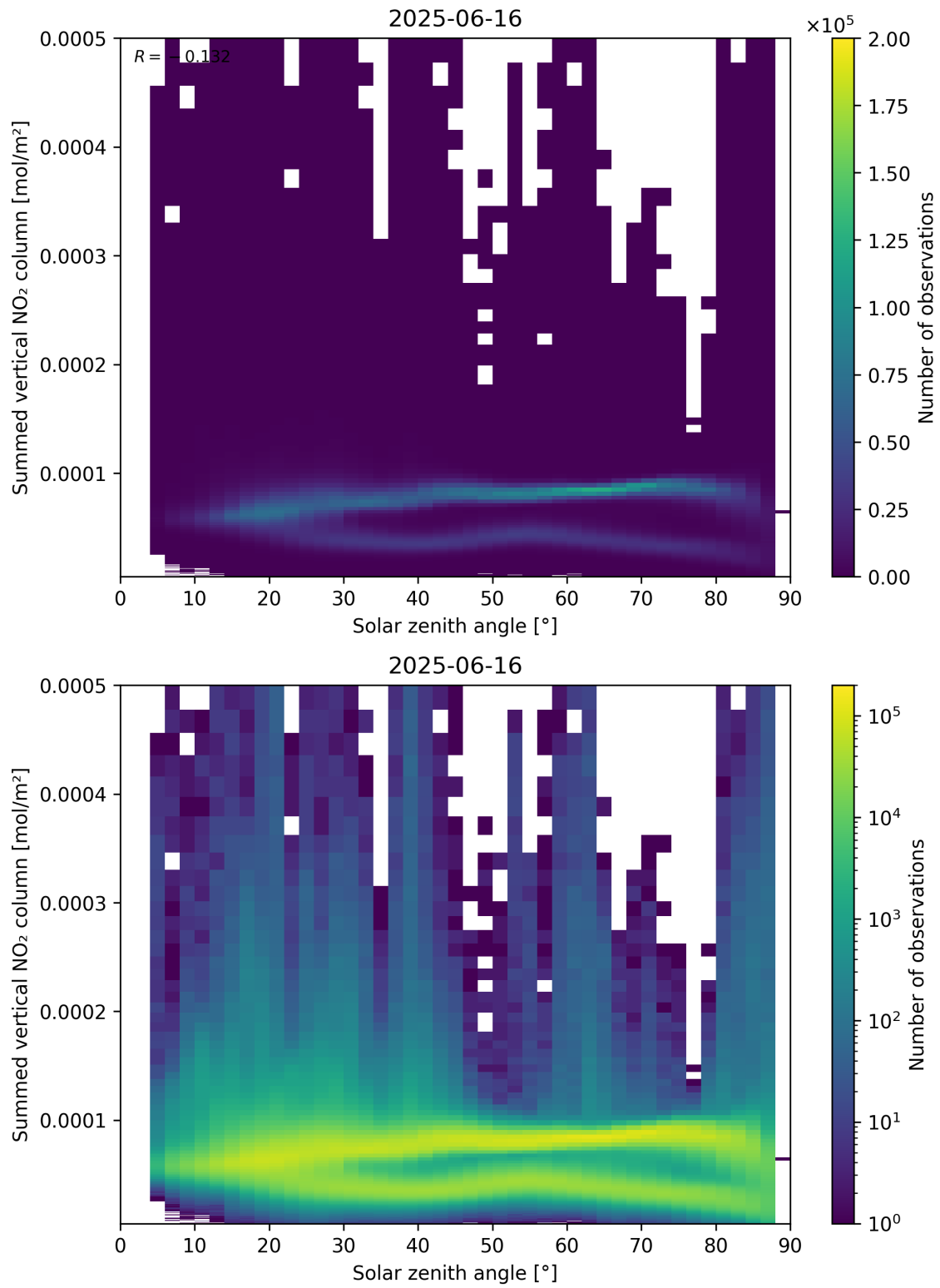
Figure 151: Scatter density plot of “Solar zenith angle” against “Summed vertical NO 2 column” for 2025-06-16 to 2025-06-17.
