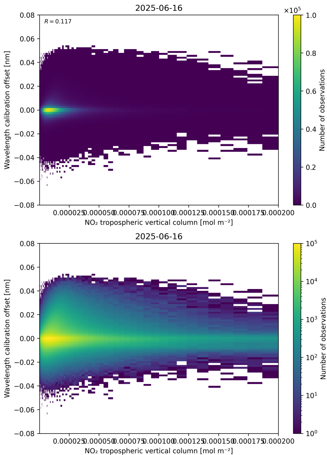
Figure 143: Scatter density plot of “NO 2 tropospheric vertical column” against “Wavelength calibration offset” for 2025-06-16 to 2025-06-17.
