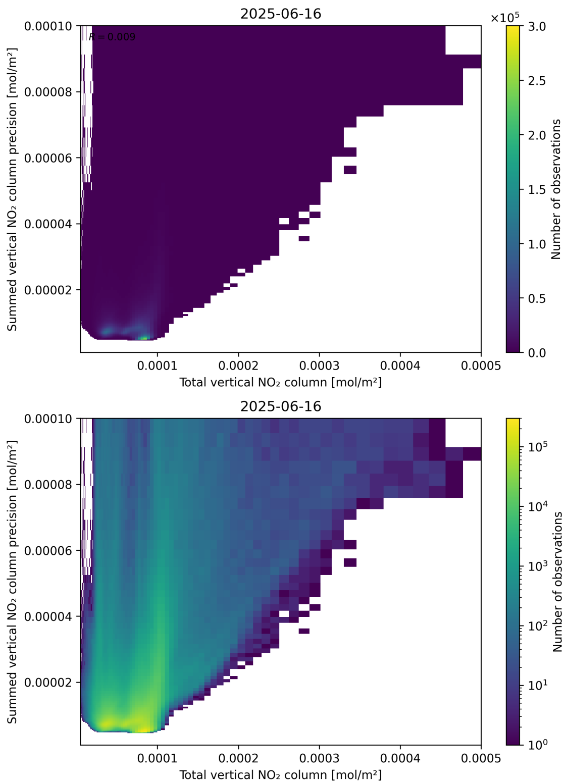
Figure 113: Scatter density plot of “Total vertical NO 2 column” against “Summed vertical NO 2 column precision” for 2025-06-16 to 2025-06-17.
