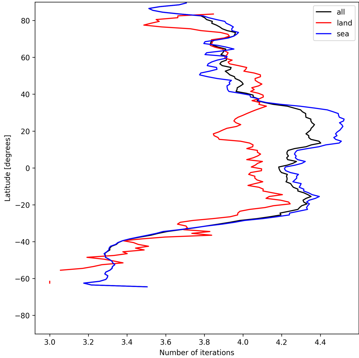
Figure 17: Zonal average of “Number of iterations” for 2025-06-16 to 2025-06-17.
