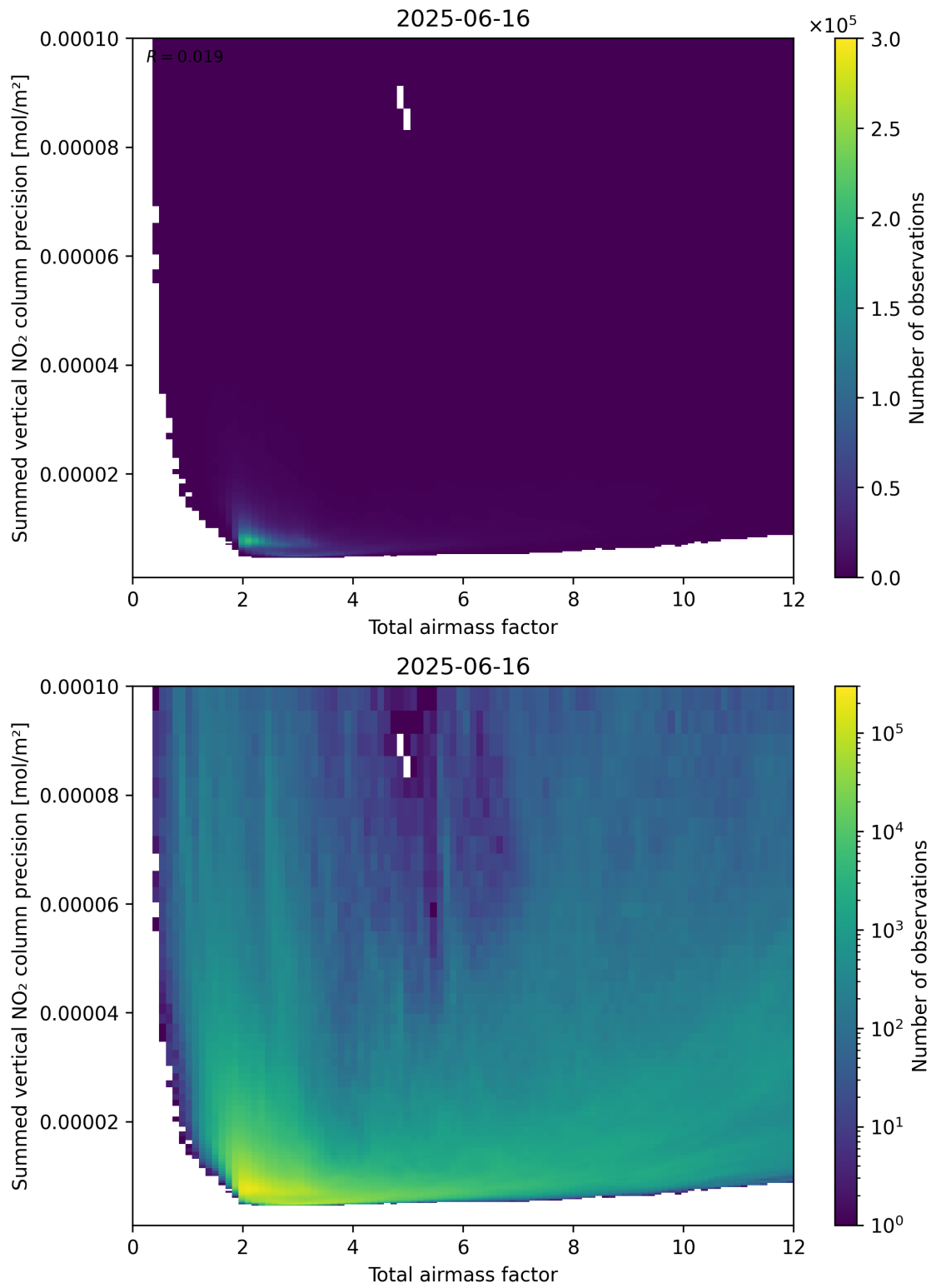
Figure 66: Scatter density plot of “Total airmass factor” against “Summed vertical NO 2 column precision” for 2025-06-16 to 2025-06-17.
