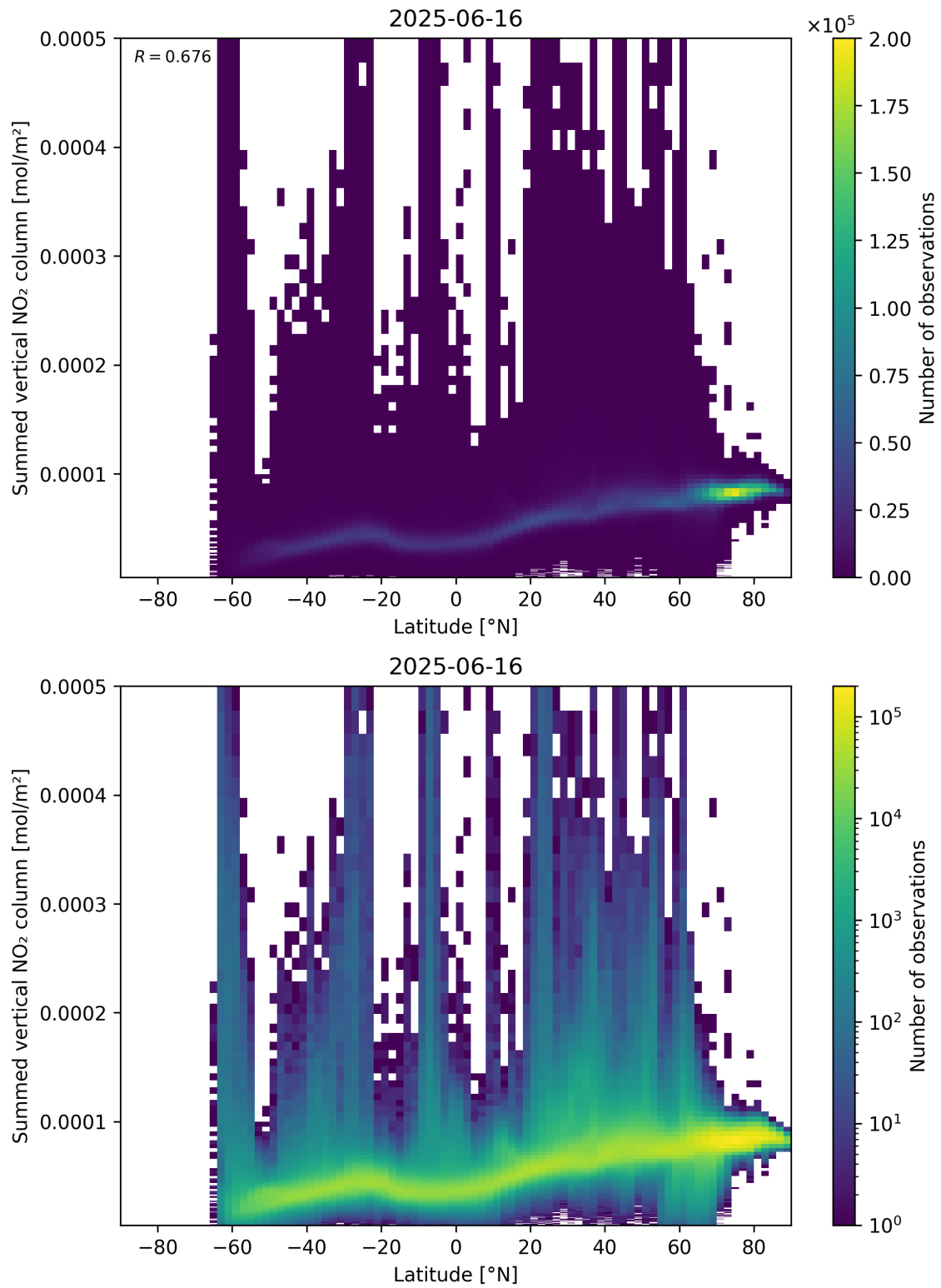
Figure 88: Scatter density plot of “Latitude” against “Summed vertical NO 2 column” for 2025-06-16 to 2025-06-17.
