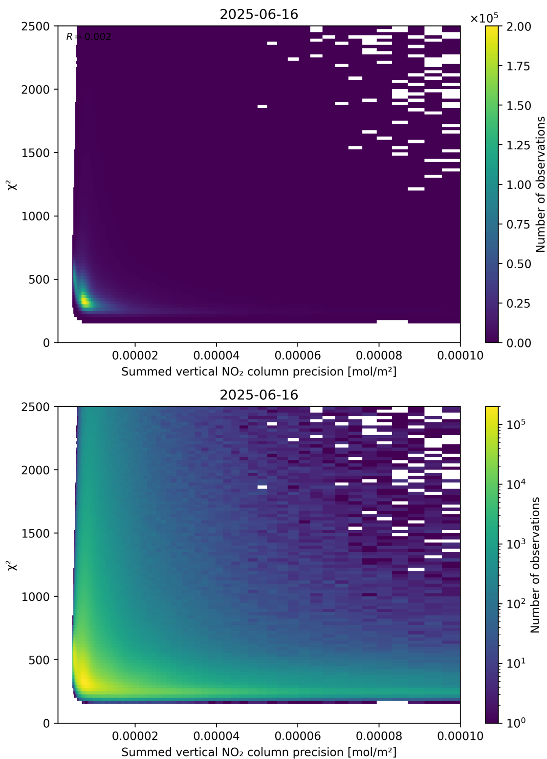
Figure 107: Scatter density plot of “Summed vertical NO 2 column precision” against “ \chi^2 ” for 2025-06-16 to 2025-06-17.
