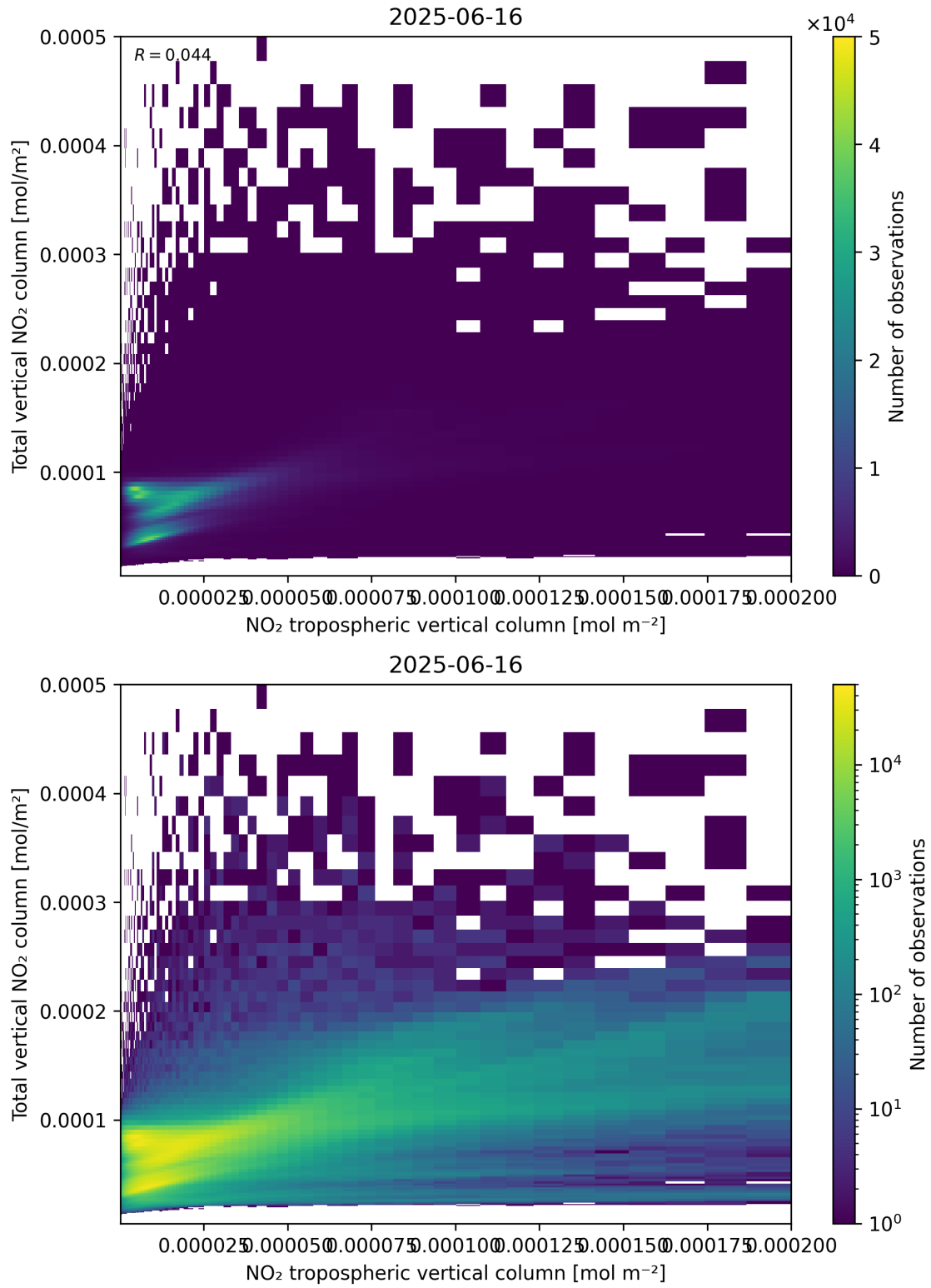
Figure 128: Scatter density plot of “NO 2 tropospheric vertical column” against “Total vertical NO 2 column” for 2025-06-16 to 2025-06-17.
