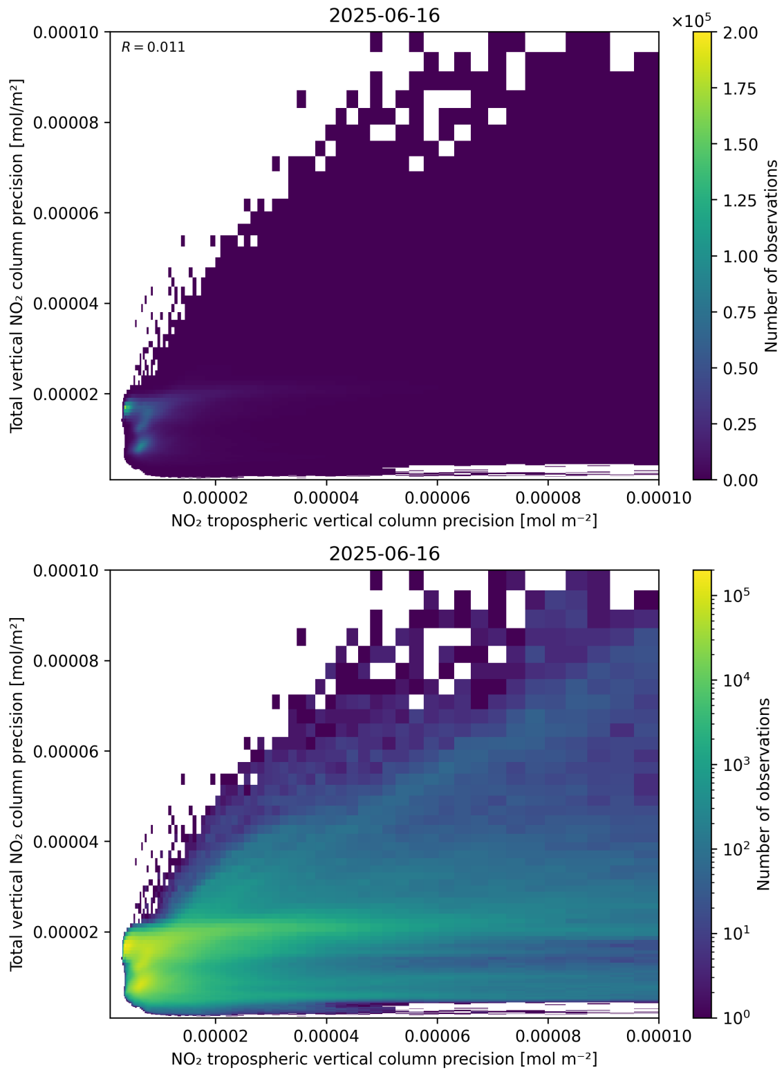
Figure 139: Scatter density plot of “NO 2 tropospheric vertical column precision” against “Total vertical NO 2 column precision” for 2025-06-16 to 2025-06-17.
