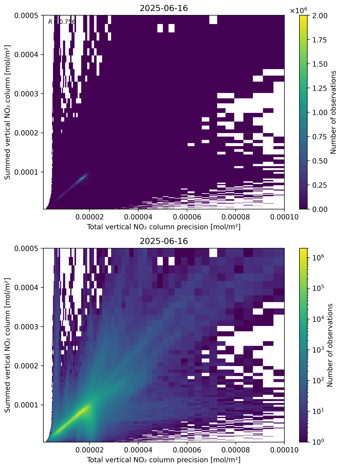
Figure 117: Scatter density plot of “Total vertical NO 2 column precision” against “Summed vertical NO 2 column” for 2025-06-16 to 2025-06-17.
