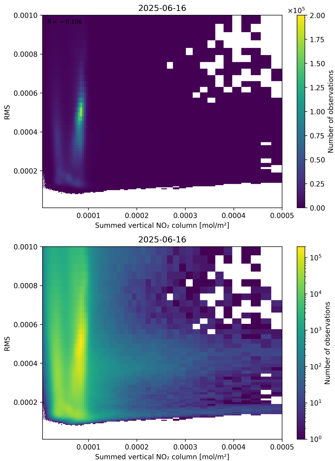
Figure 109: Scatter density plot of “Summed vertical NO 2 column” against “RMS” for 2025-06-16 to 2025-06-17.
