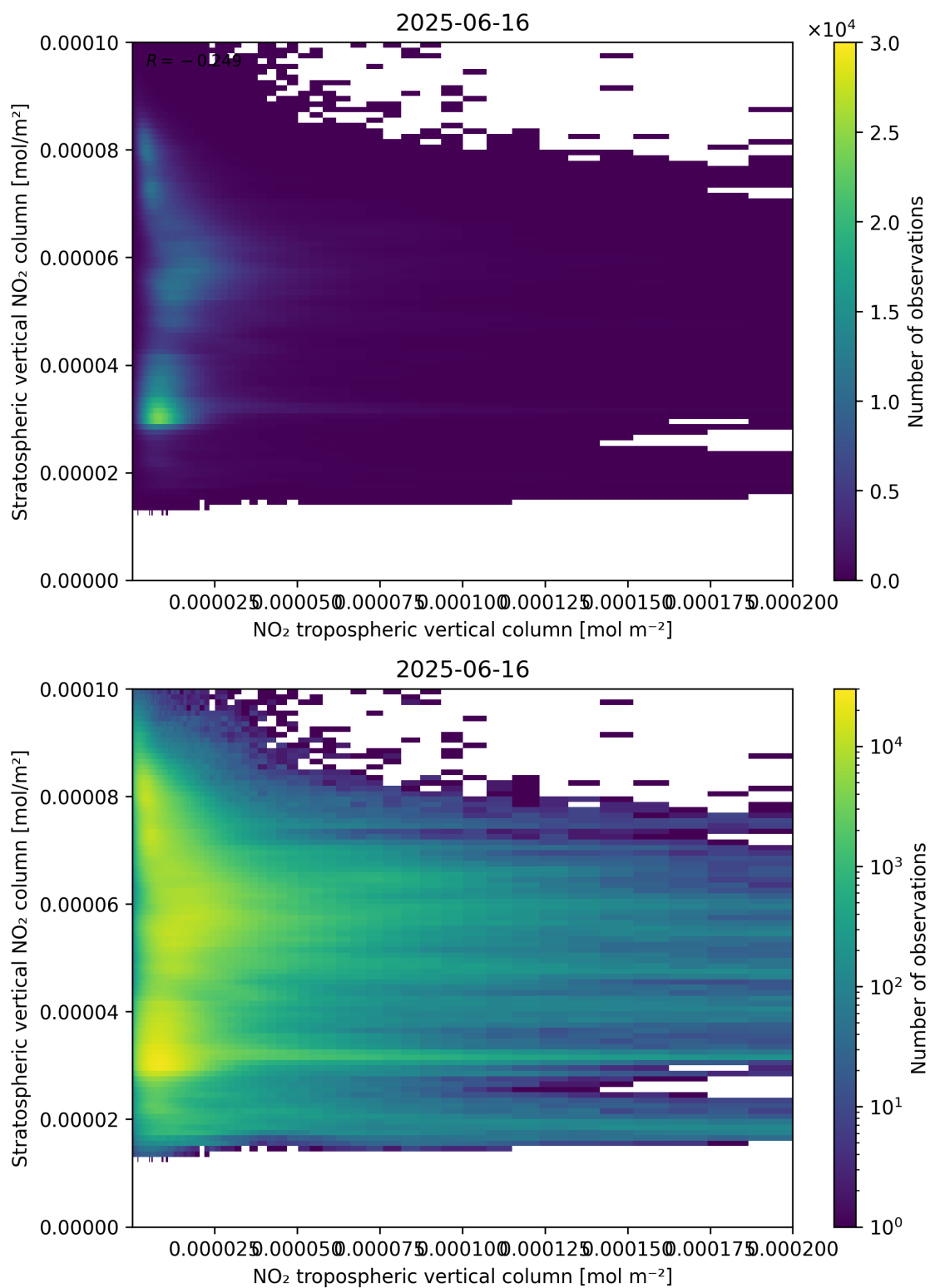
Figure 125: Scatter density plot of “NO 2 tropospheric vertical column” against “Stratospheric vertical NO 2 column” for 2025-06-16 to 2025-06-17.
