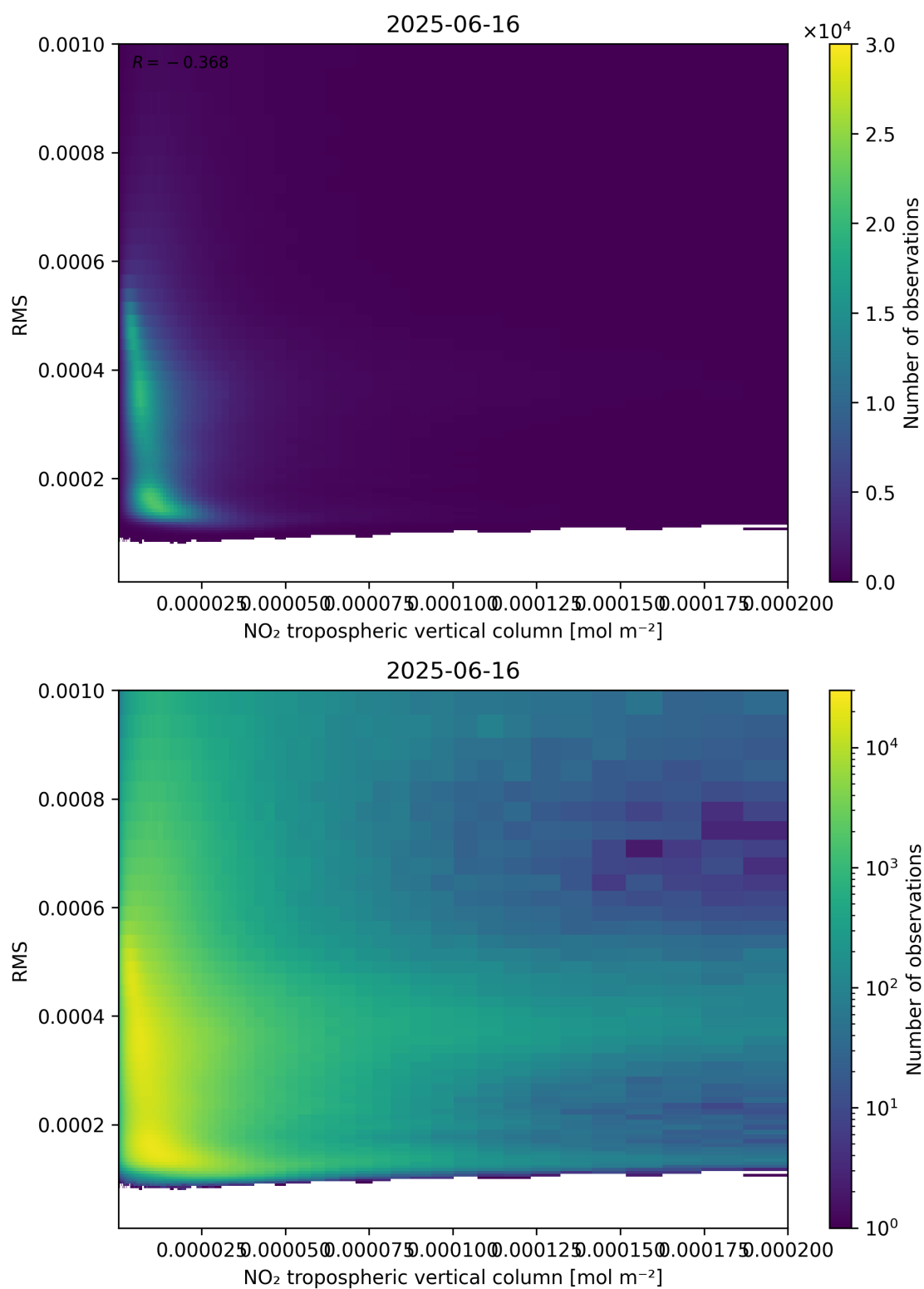
Figure 142: Scatter density plot of “NO 2 tropospheric vertical column” against “RMS” for 2025-06-16 to 2025-06-17.
