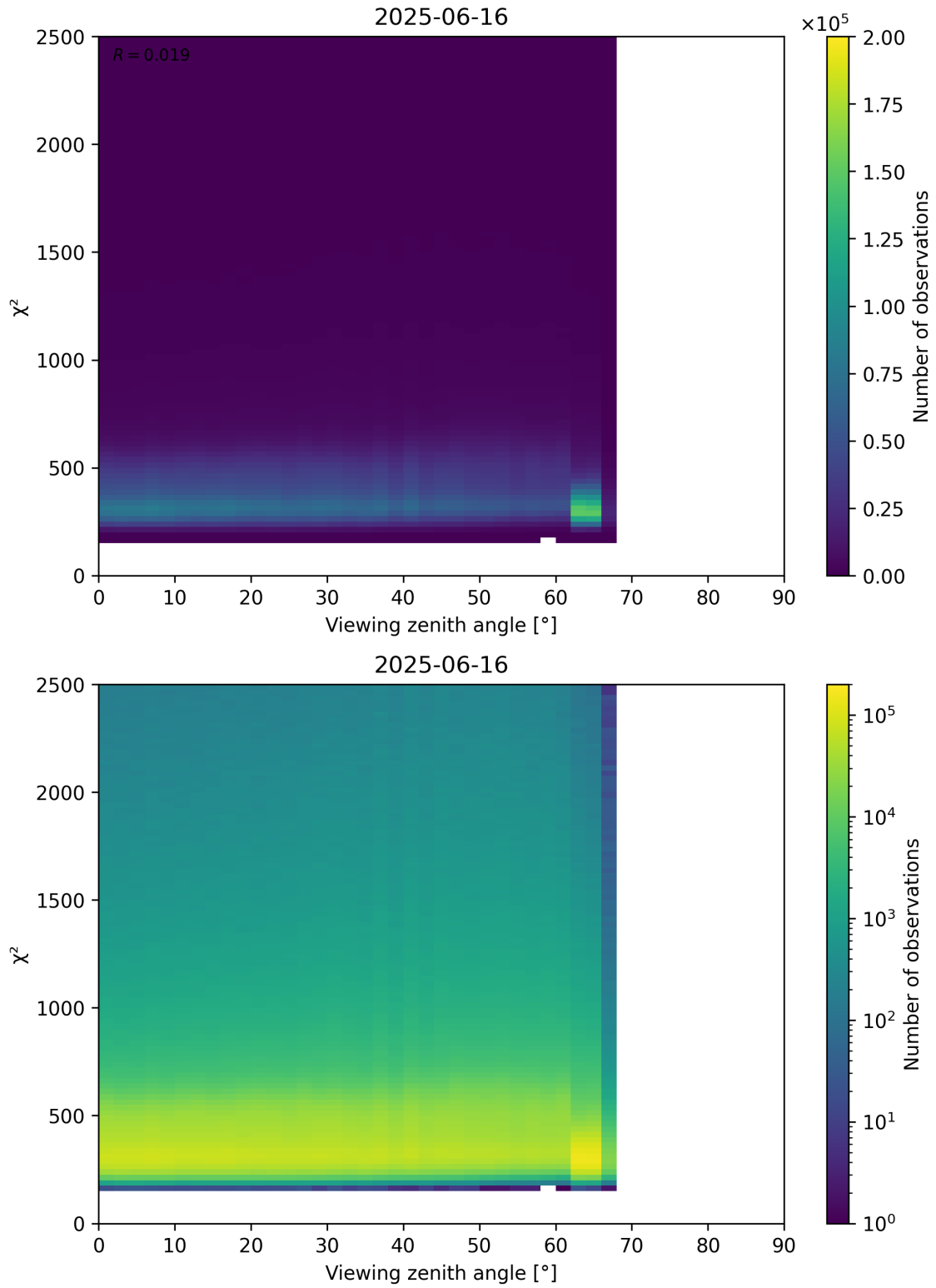
Figure 162: Scatter density plot of “Viewing zenith angle” against “ \chi^2 ” for 2025-06-16 to 2025-06-17.
