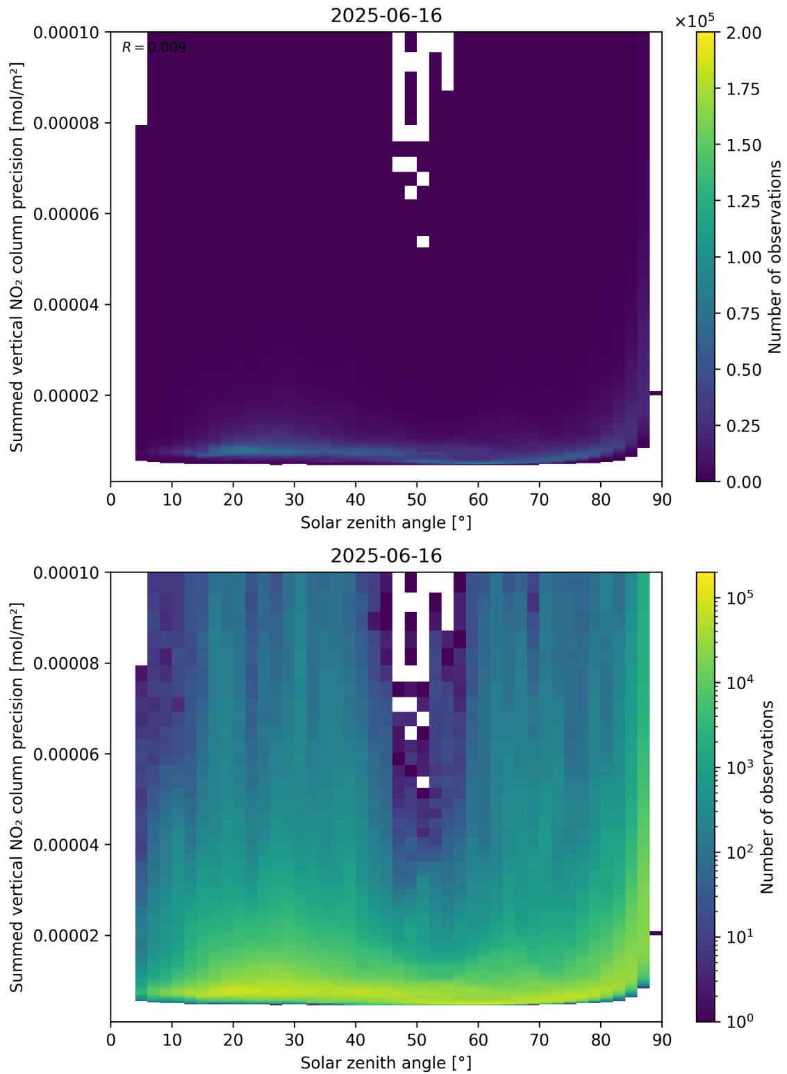
Figure 152: Scatter density plot of “Solar zenith angle” against “Summed vertical NO 2 column precision” for 2025-06-16 to 2025-06-17.
