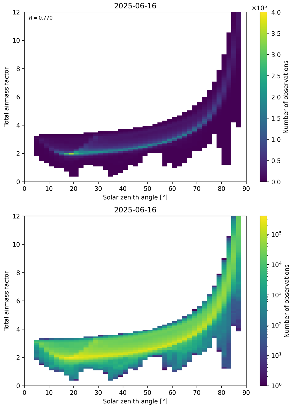
Figure 146: Scatter density plot of “Solar zenith angle” against “Total air mass factor” for 2025-06-16 to 2025-06-17.
