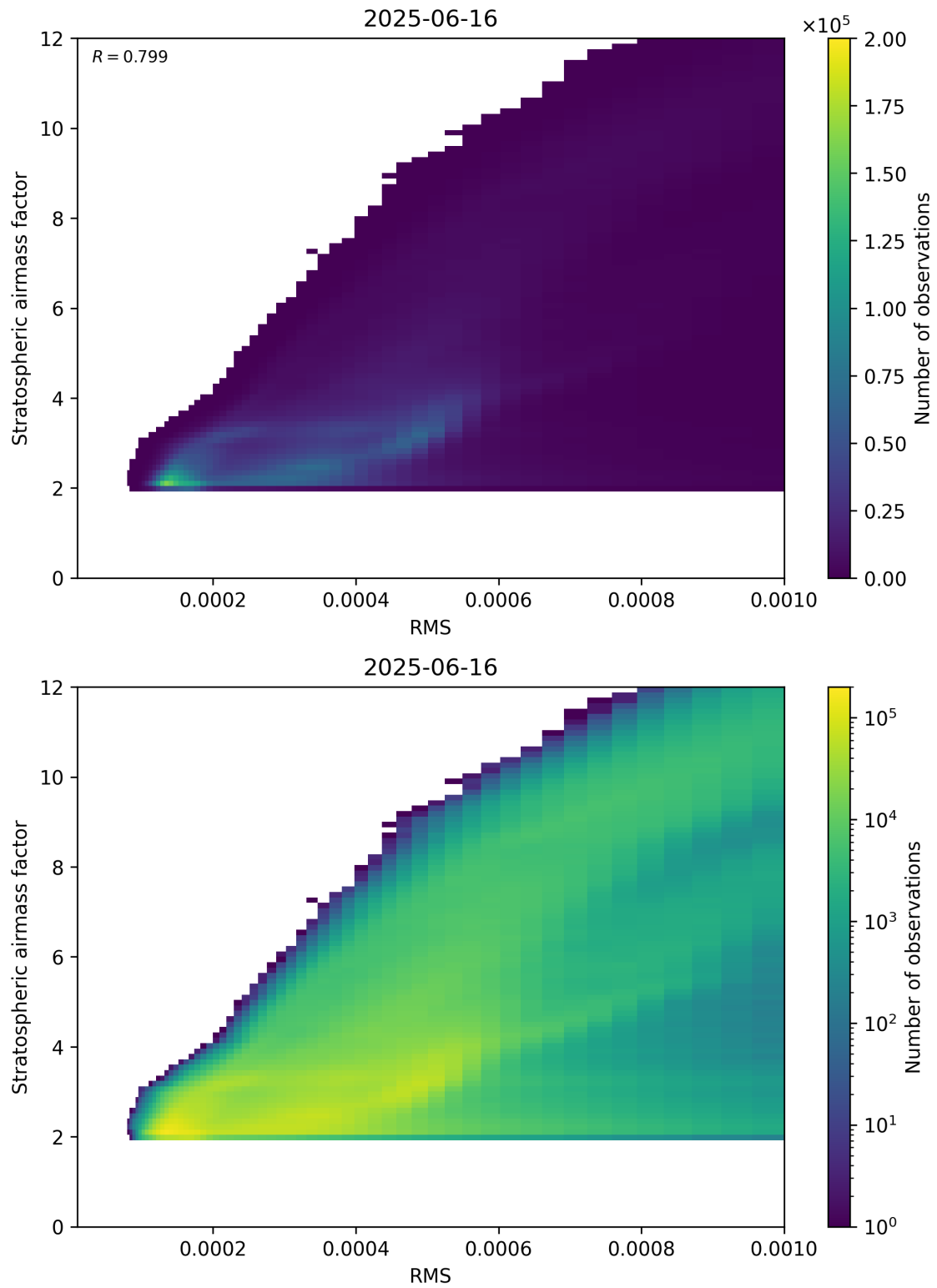
Figure 144: Scatter density plot of “RMS” against “Stratospheric airmass factor” for 2025-06-16 to 2025-06-17.
