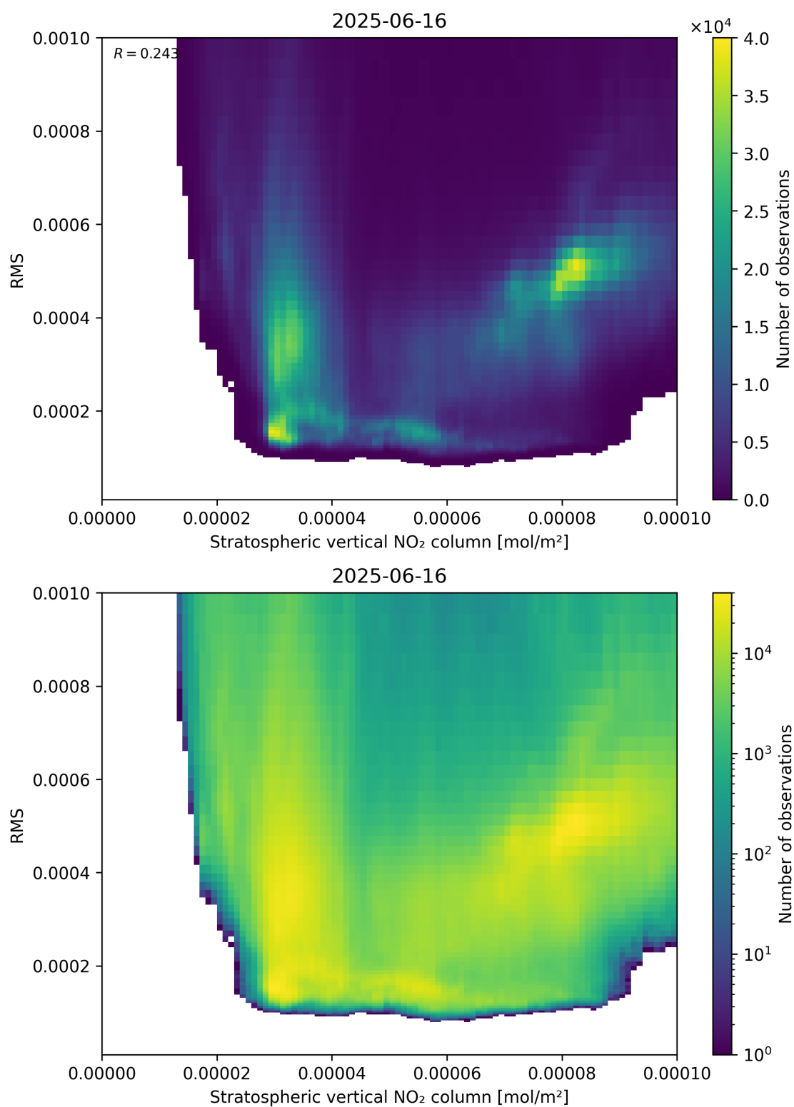
Figure 102: Scatter density plot of “Stratospheric vertical NO 2 column” against “RMS” for 2025-06-16 to 2025-06-17.
