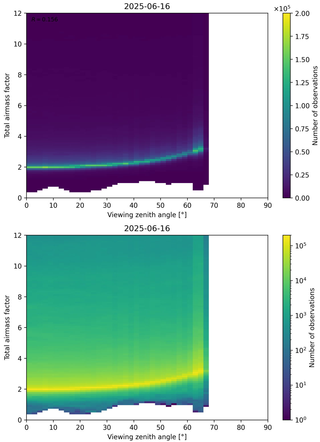
Figure 160: Scatter density plot of “Viewing zenith angle” against “Total airmass factor” for 2025-06-16 to 2025-06-17.
