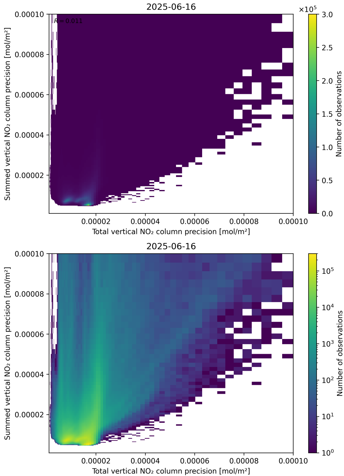
Figure 118: Scatter density plot of “Total vertical NO 2 column precision” against “Summed vertical NO 2 column precision” for 2025-06-16 to 2025-06-17.
