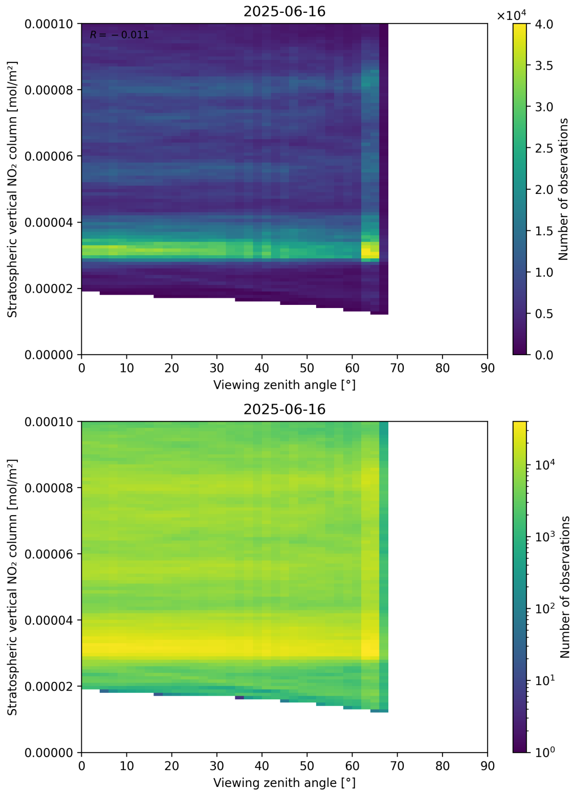
Figure 164: Scatter density plot of “Viewing zenith angle” against “Stratospheric vertical NO 2 column” for 2025-06-16 to 2025-06-17.
