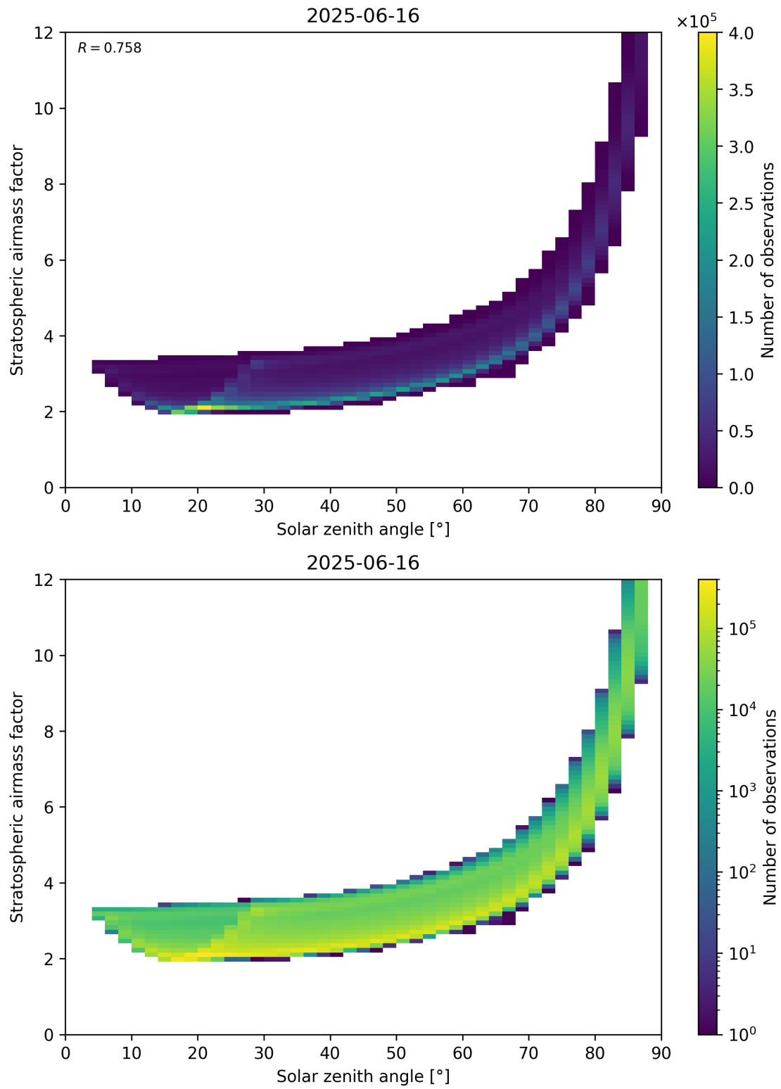
Figure 145: Scatter density plot of “Solar zenith angle” against “Stratospheric airmass factor” for 2025-06-16 to 2025-06-17.
