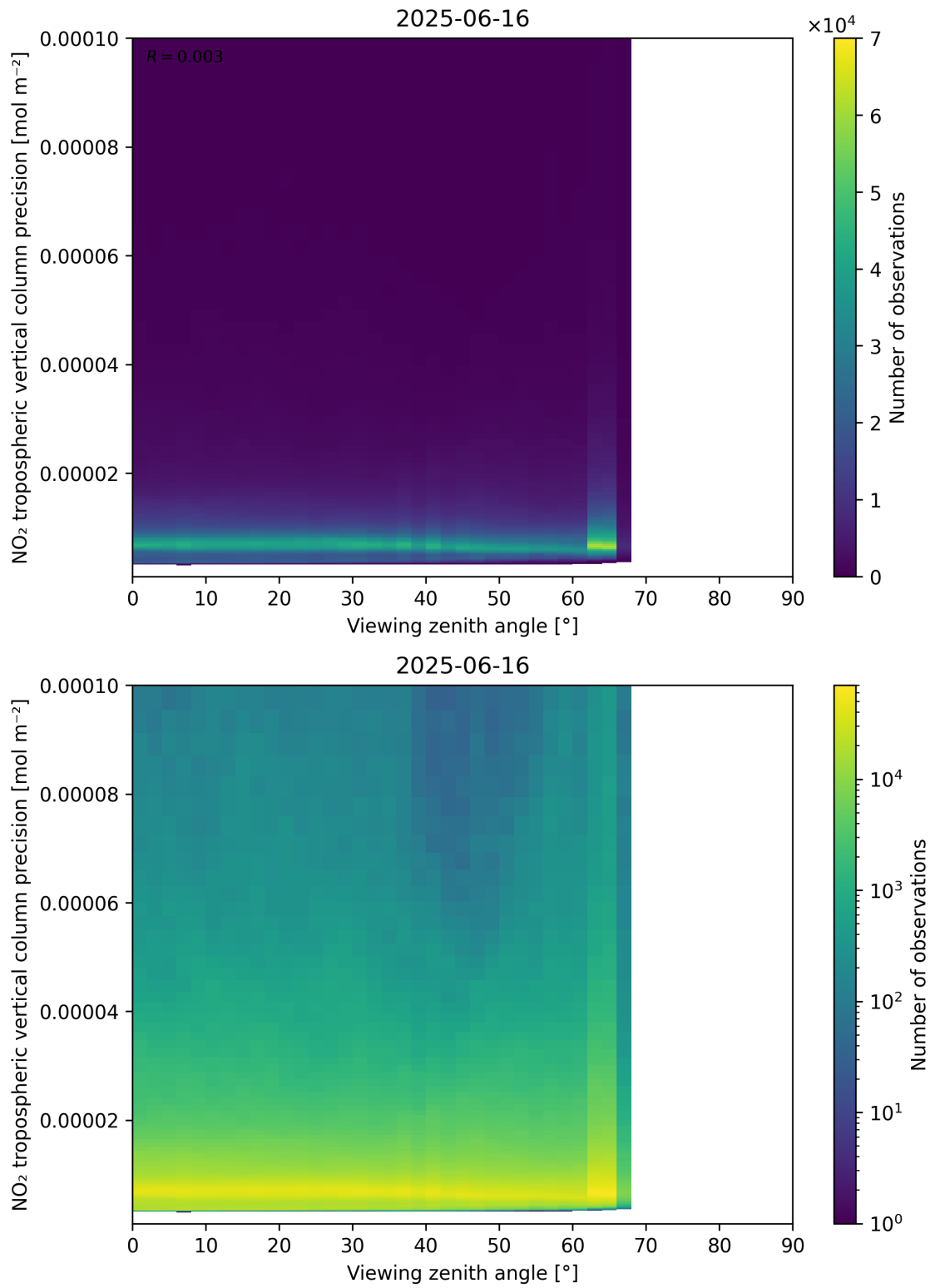
Figure 170: Scatter density plot of “Viewing zenith angle” against “NO 2 tropospheric vertical column precision” for 2025-06-16 to 2025-06-17.
