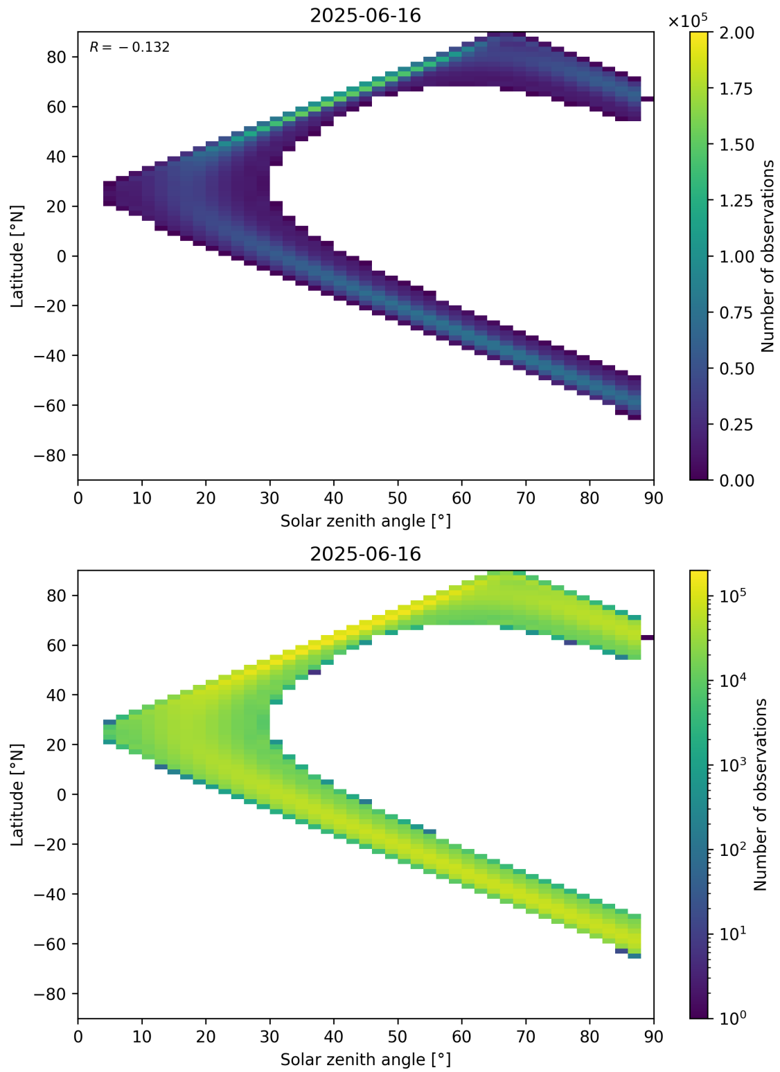
Figure 149: Scatter density plot of “Solar zenith angle” against “Latitude” for 2025-06-16 to 2025-06-17.
