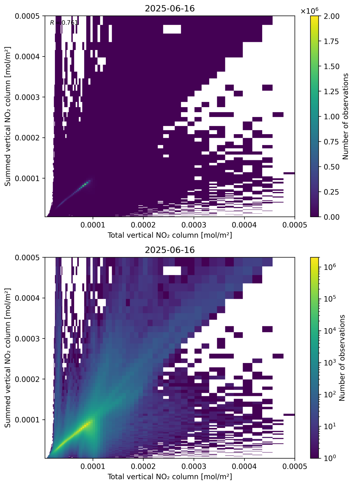
Figure 112: Scatter density plot of “Total vertical NO 2 column” against “Summed vertical NO 2 column” for 2025-06-16 to 2025-06-17.
