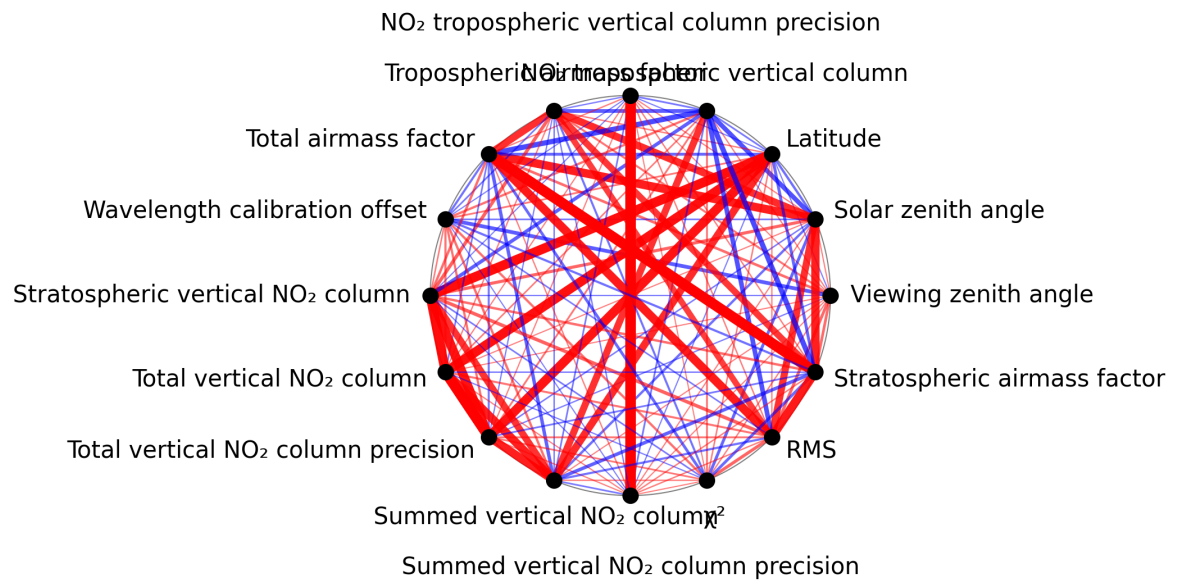
Figure 1: Map of correlation graph for 2025-06-16 to 2025-06-17.
