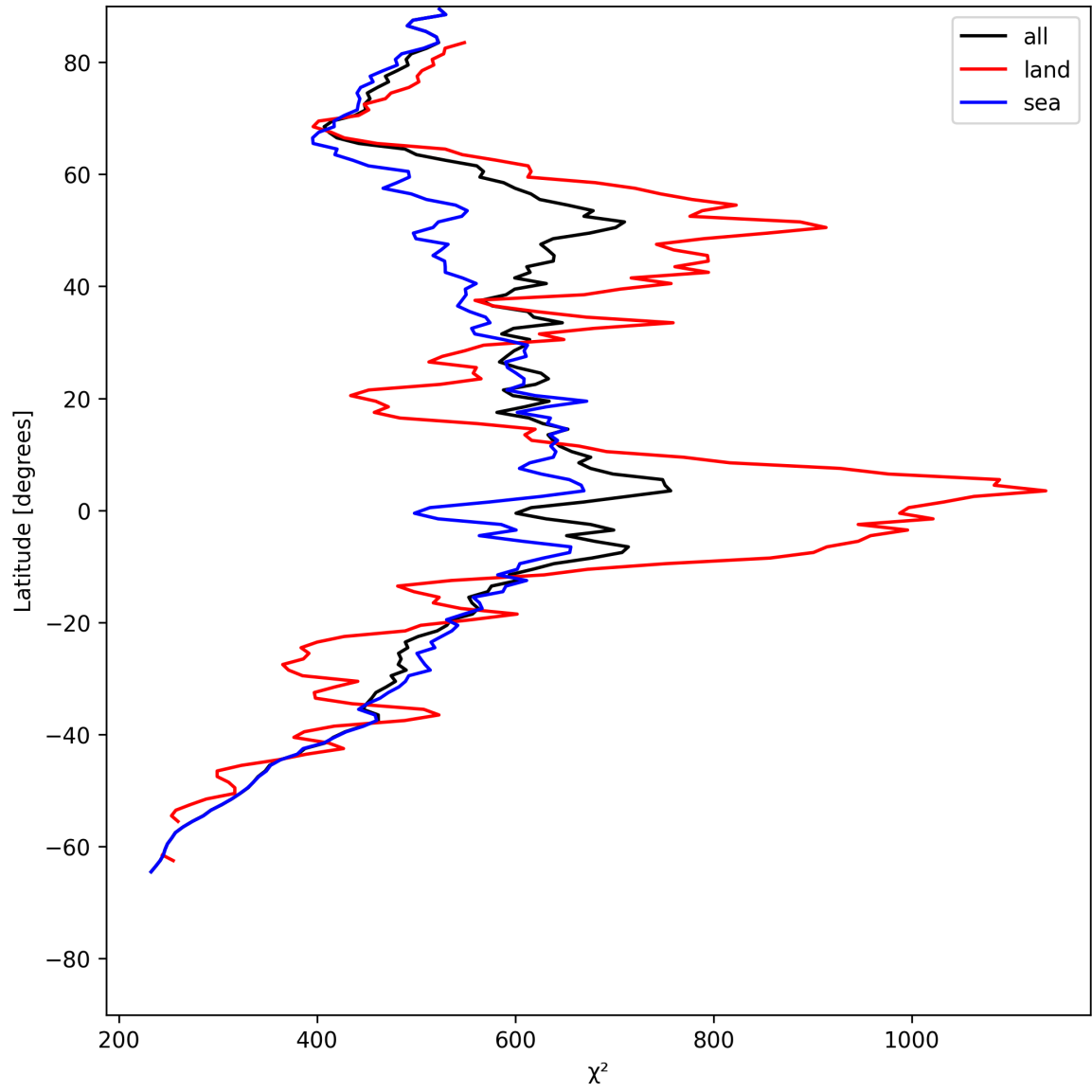
Figure 25: Zonal average of “ \chi^2 ” for 2025-06-16 to 2025-06-17.
