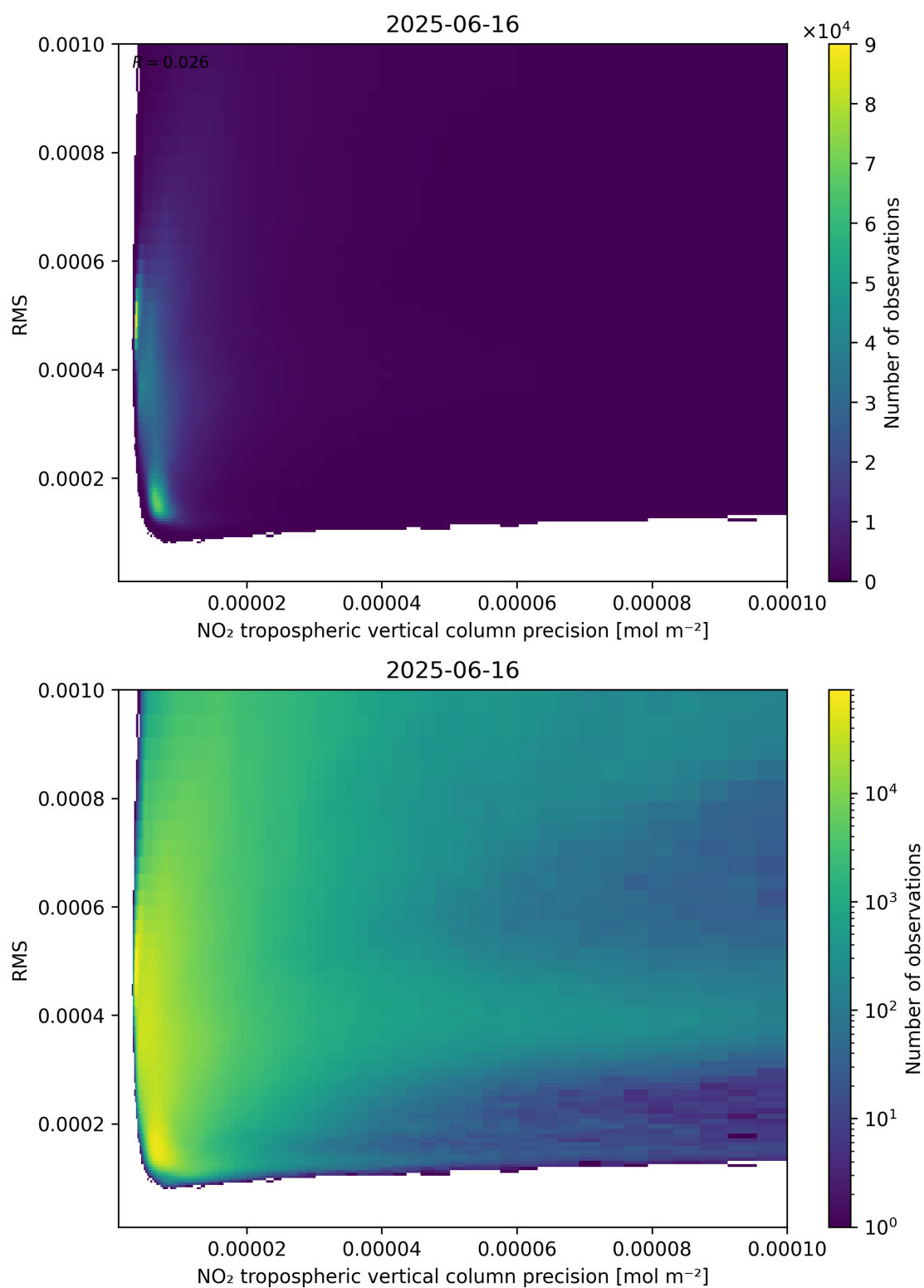
Figure 140: Scatter density plot of “NO 2 tropospheric vertical column precision” against “RMS” for 2025-06-16 to 2025-06-17.
