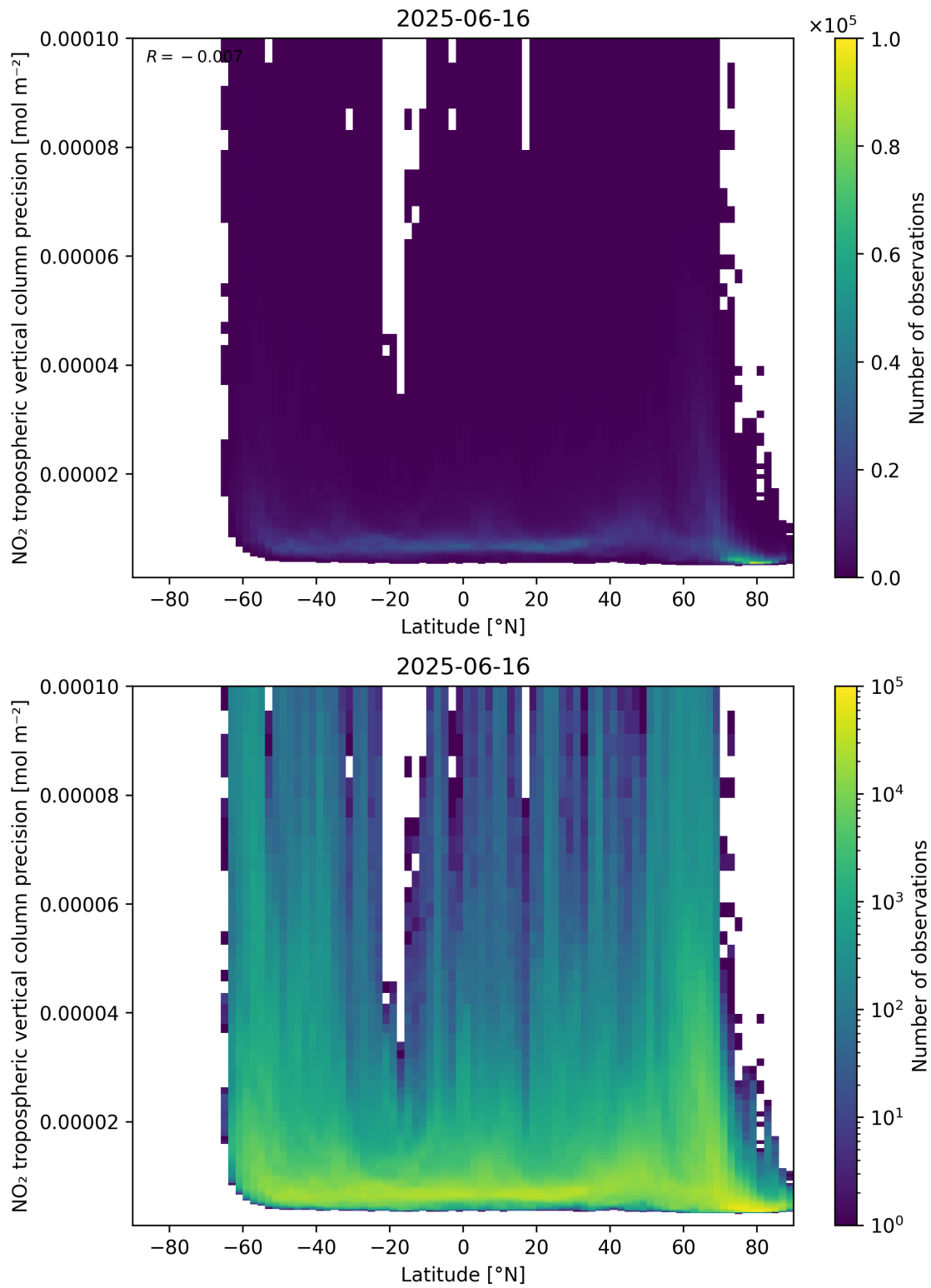
Figure 93: Scatter density plot of “Latitude” against “NO 2 tropospheric vertical column precision” for 2025-06-16 to 2025-06-17.
