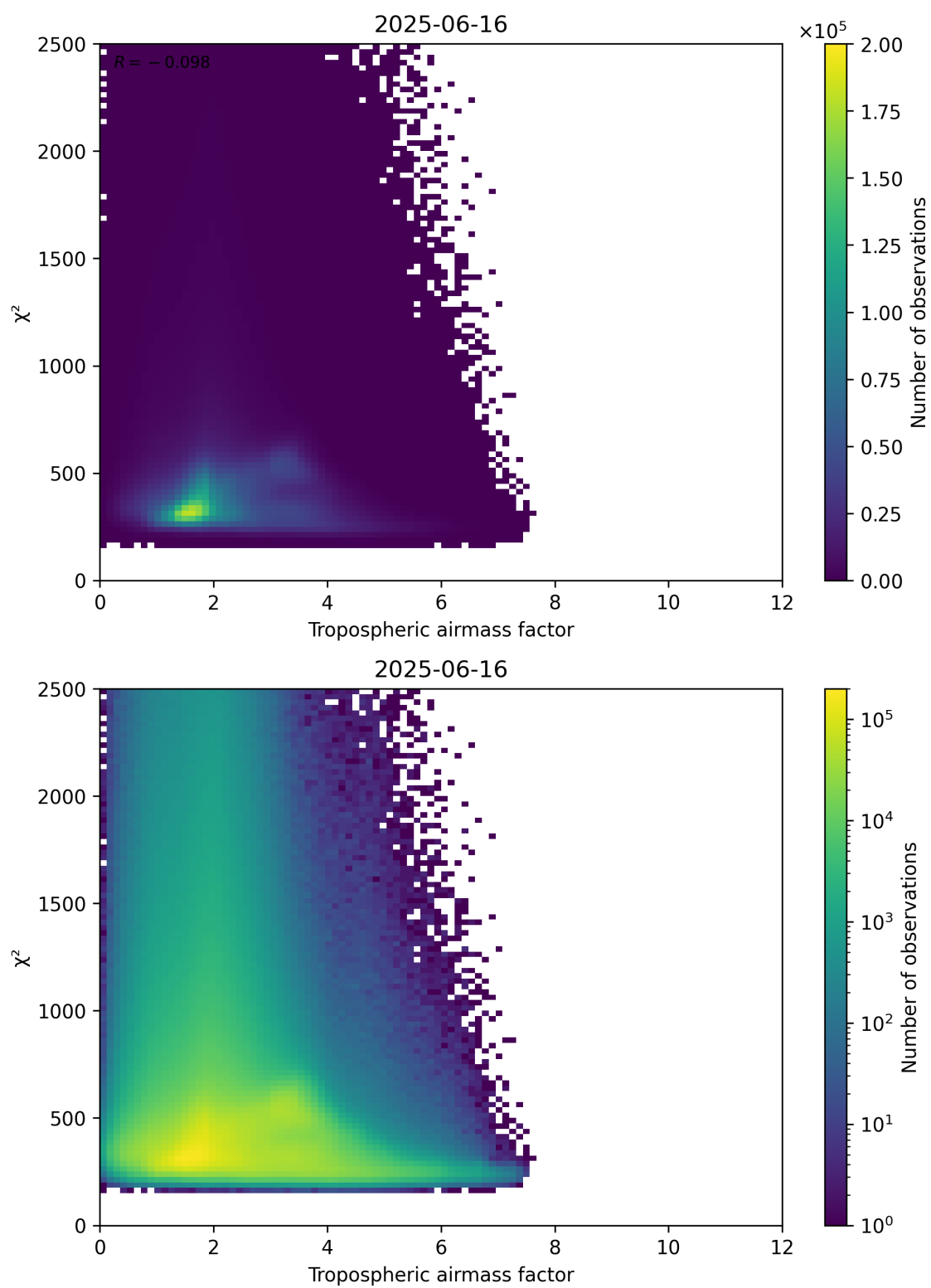
Figure 73: Scatter density plot of “Tropospheric airmass factor” against “ \chi^2 ” for 2025-06-16 to 2025-06-17.
