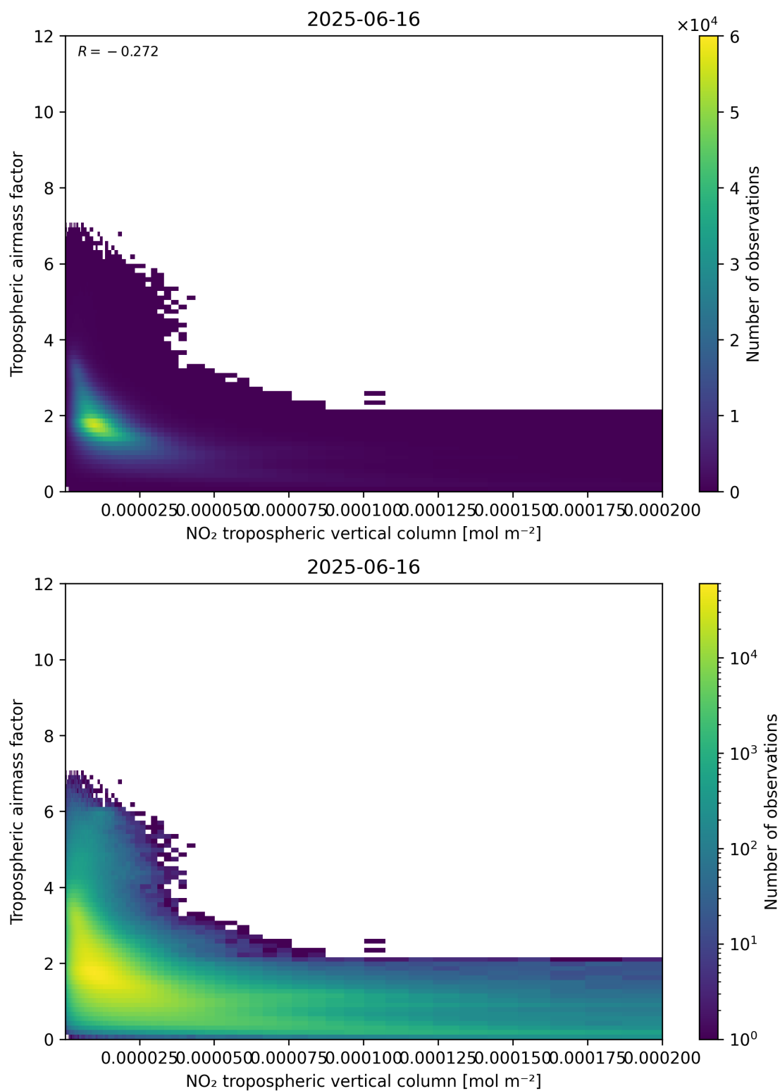
Figure 123: Scatter density plot of “NO 2 tropospheric vertical column” against “Tropospheric air mass factor” for 2025-06-16 to 2025-06-17.
