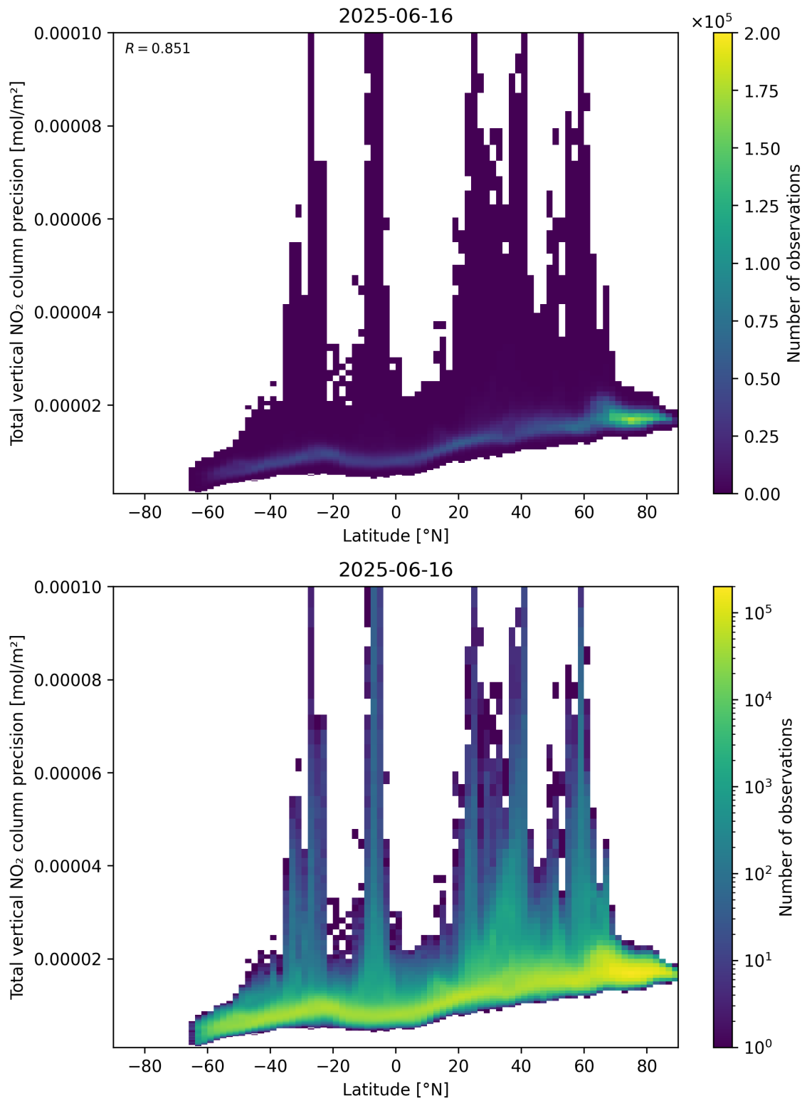
Figure 91: Scatter density plot of “Latitude” against “Total vertical NO 2 column precision” for 2025-06-16 to 2025-06-17.
