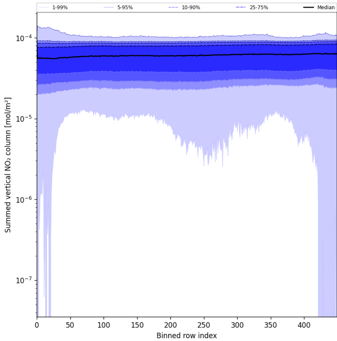
Figure 57: Along track statistics of “Summed vertical NO 2 column” for 2025-06-16 to 2025-06-17
