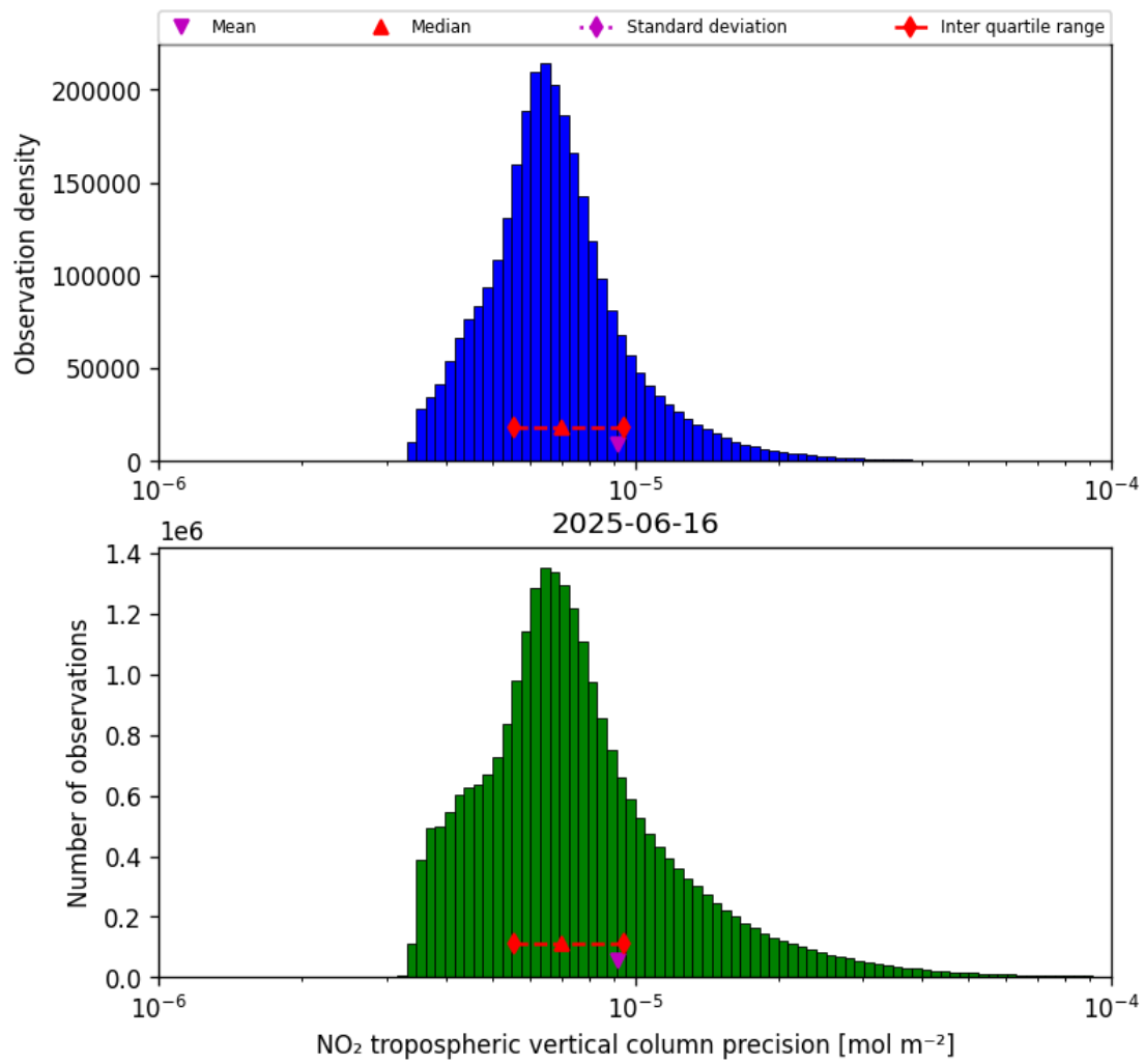
Figure 30: Histogram of “NO 2 tropospheric vertical column precision” for 2025-06-16 to 2025-06-17
