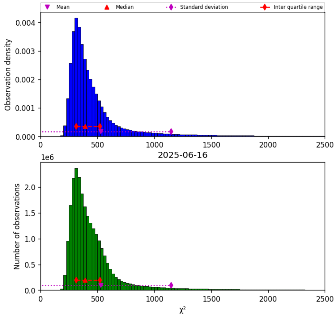
Figure 42: Histogram of “ \chi^2 ” for 2025-06-16 to 2025-06-17
