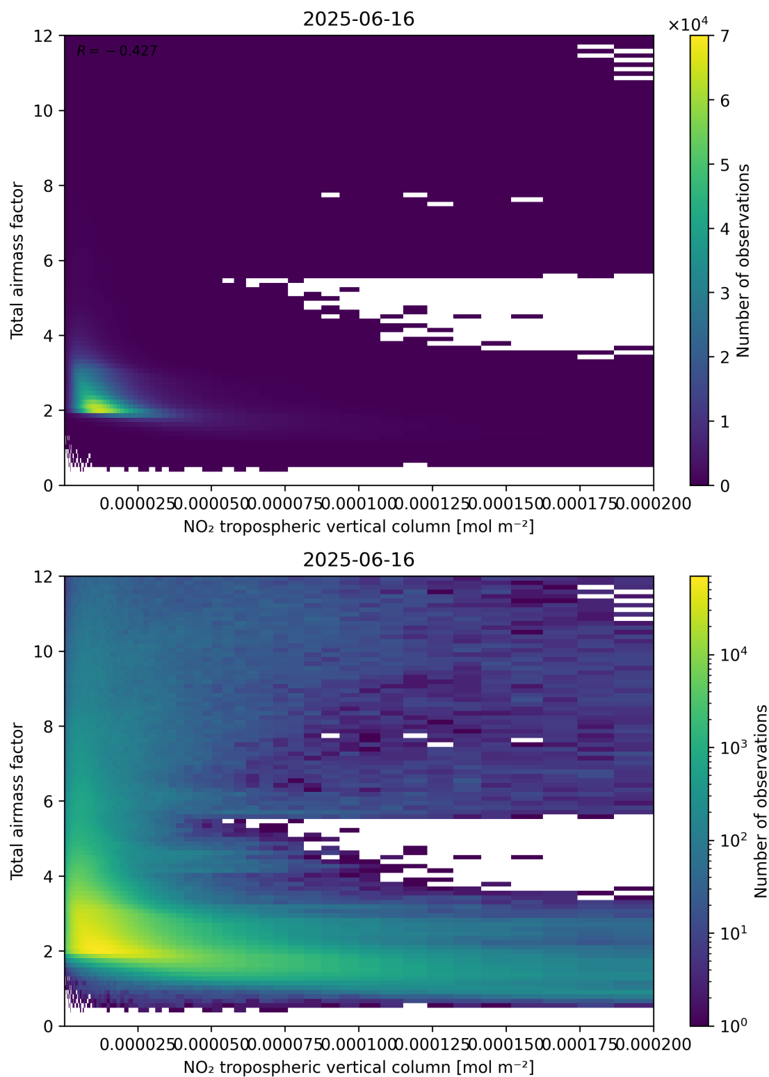
Figure 122: Scatter density plot of “NO 2 tropospheric vertical column” against “Total air mass factor” for 2025-06-16 to 2025-06-17.
