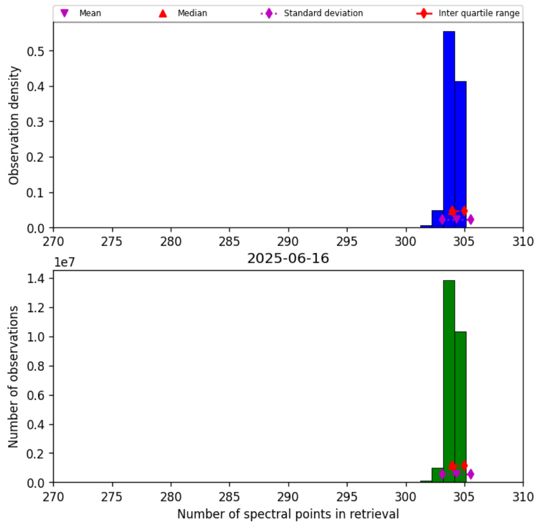
Figure 33: Histogram of “Number of spectral points in retrieval” for 2025-06-16 to 2025-06-17
