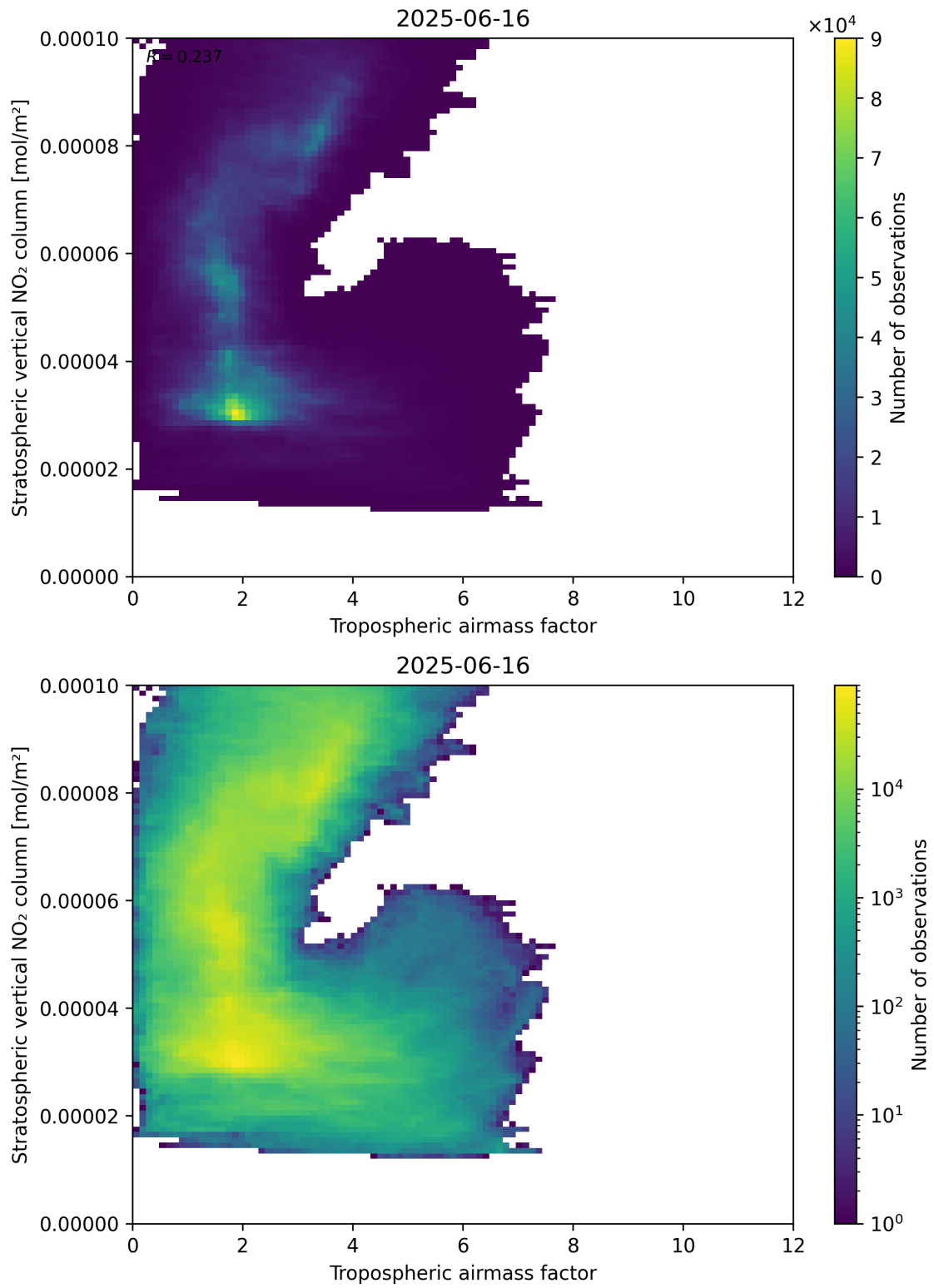
Figure 74: Scatter density plot of “Tropospheric air mass factor” against “Stratospheric vertical NO 2 column” for 2025-06-16 to 2025-06-17.
