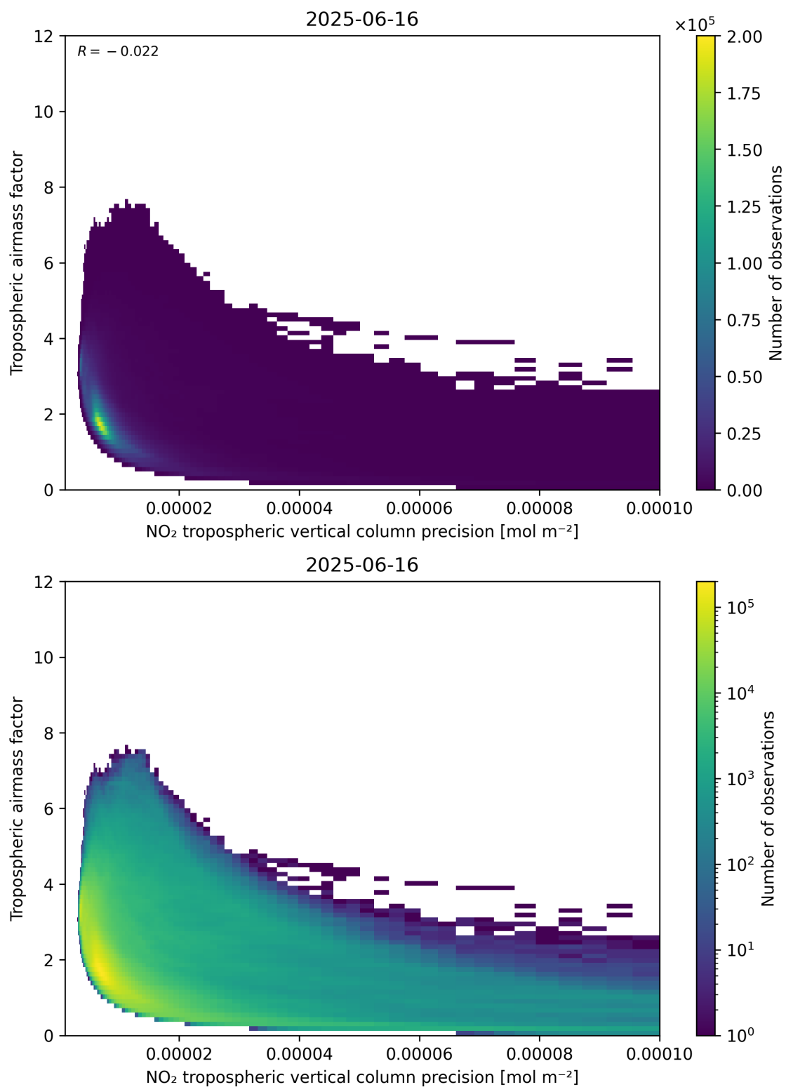
Figure 133: Scatter density plot of “NO 2 tropospheric vertical column precision” against “Tropospheric air mass factor” for 2025-06-16 to 2025-06-17.
