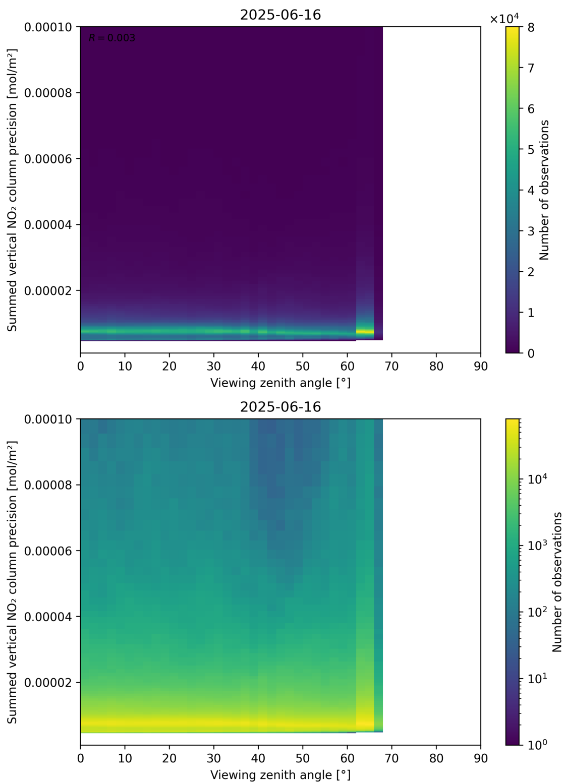
Figure 166: Scatter density plot of “Viewing zenith angle” against “Summed vertical NO 2 column precision” for 2025-06-16 to 2025-06-17.
