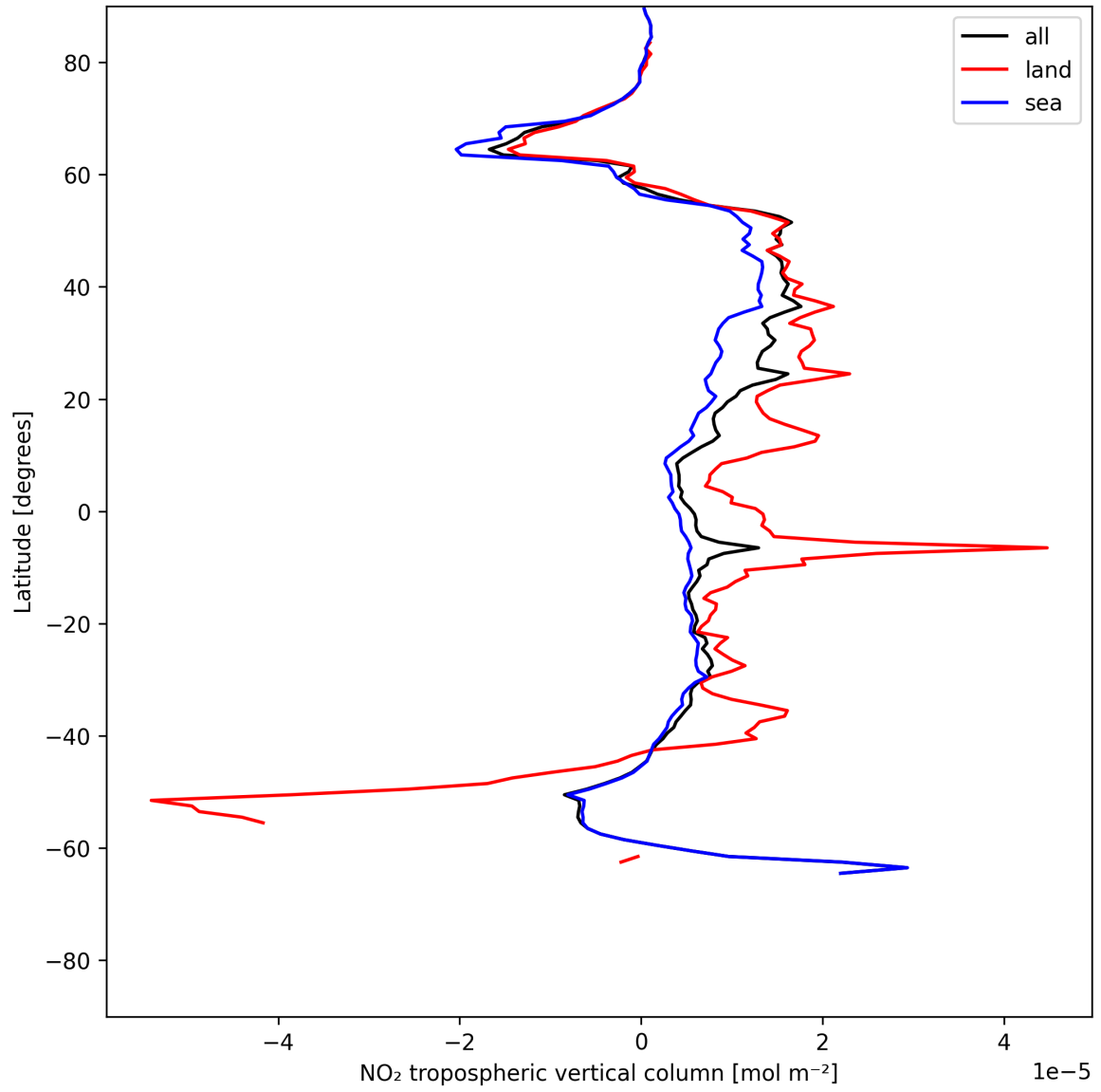
Figure 12: Zonal average of “NO 2 tropospheric vertical column” for 2025-06-16 to 2025-06-17.
