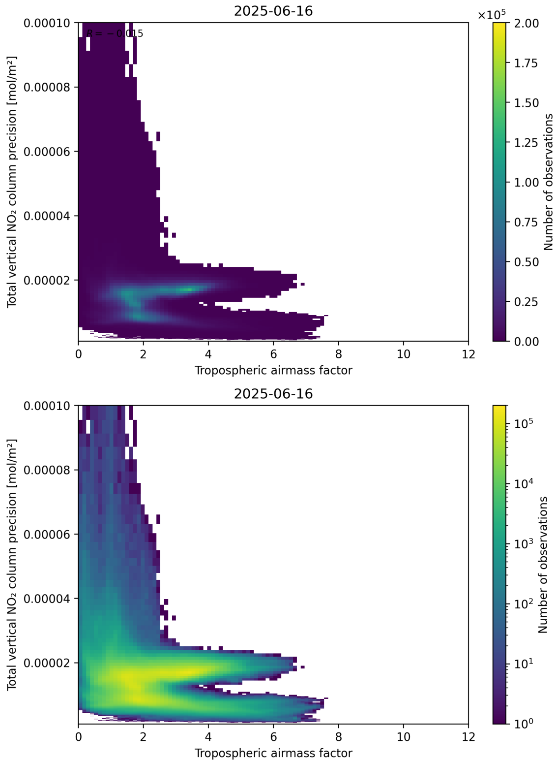
Figure 78: Scatter density plot of “Tropospheric air mass factor” against “Total vertical NO 2 column precision” for 2025-06-16 to 2025-06-17.
