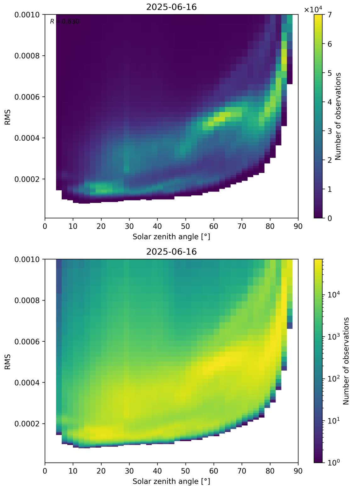
Figure 157: Scatter density plot of “Solar zenith angle” against “RMS” for 2025-06-16 to 2025-06-17.
