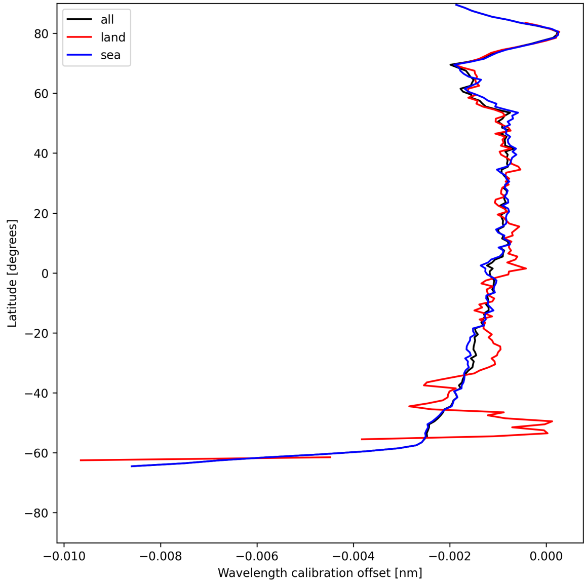
Figure 18: Zonal average of “Wavelength calibration offset” for 2025-06-16 to 2025-06-17.
