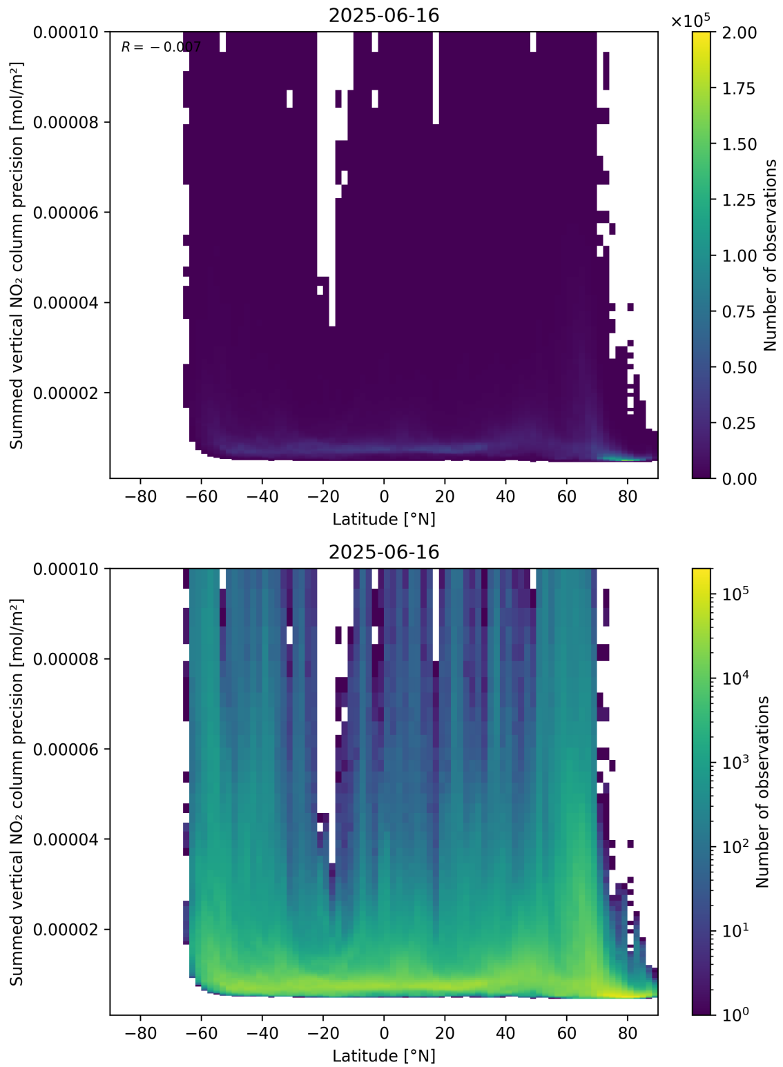
Figure 89: Scatter density plot of “Latitude” against “Summed vertical NO 2 column precision” for 2025-06-16 to 2025-06-17.
