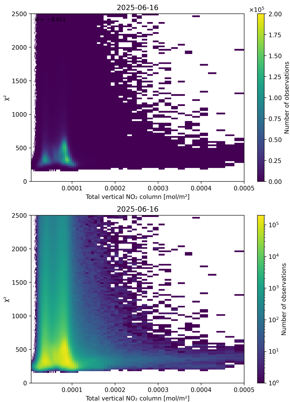
Figure 111: Scatter density plot of “Total vertical NO 2 column” against “ \chi^2 ” for 2025-06-16 to 2025-06-17.
