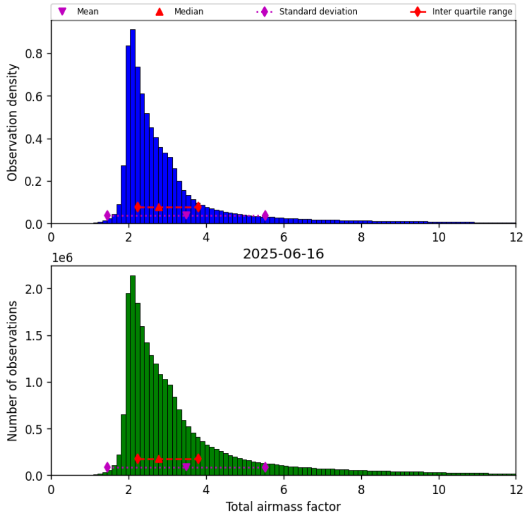
Figure 32: Histogram of “Total airmass factor” for 2025-06-16 to 2025-06-17
