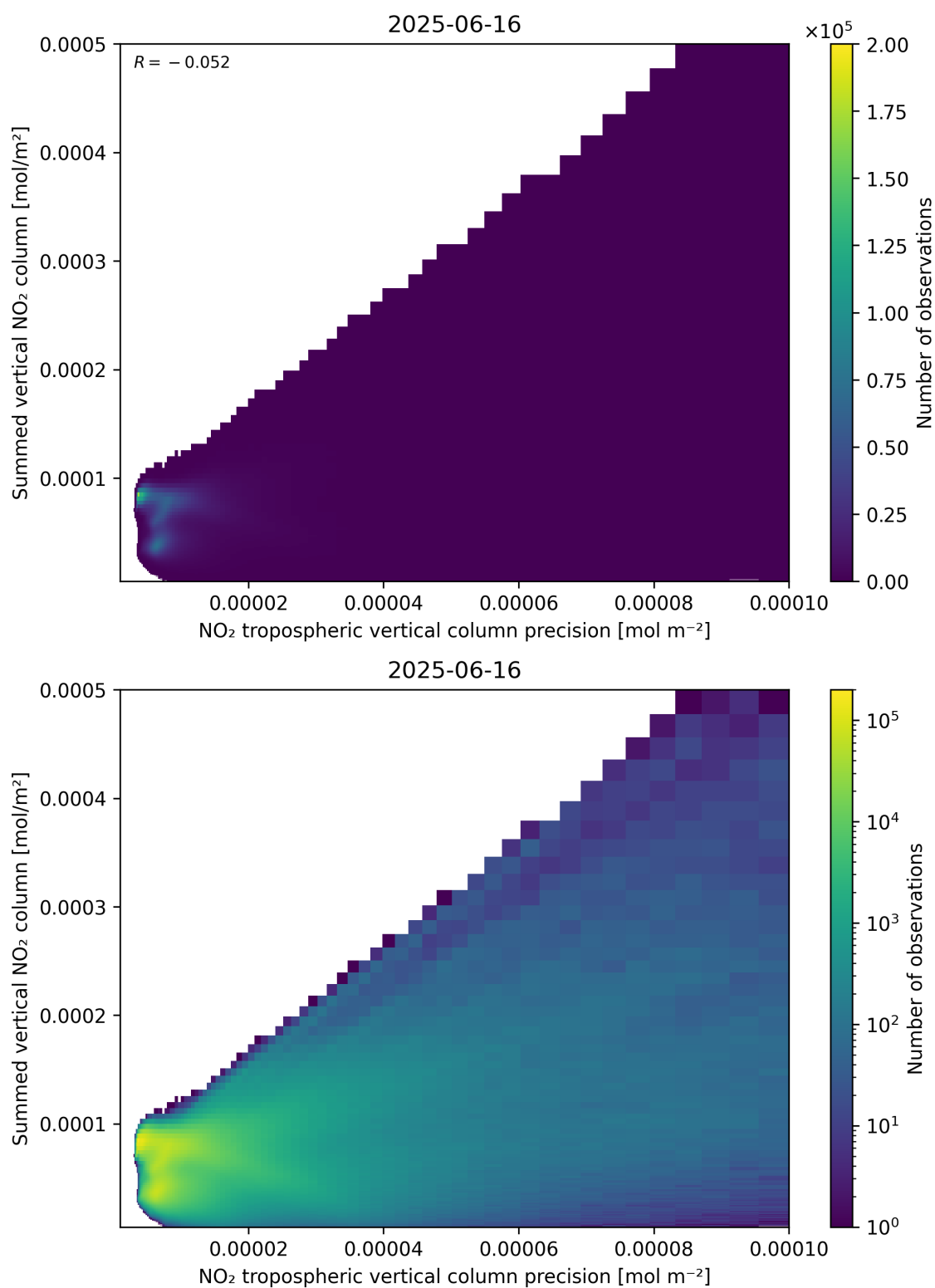
Figure 136: Scatter density plot of “NO 2 tropospheric vertical column precision” against “Summed vertical NO 2 column” for 2025-06-16 to 2025-06-17.
