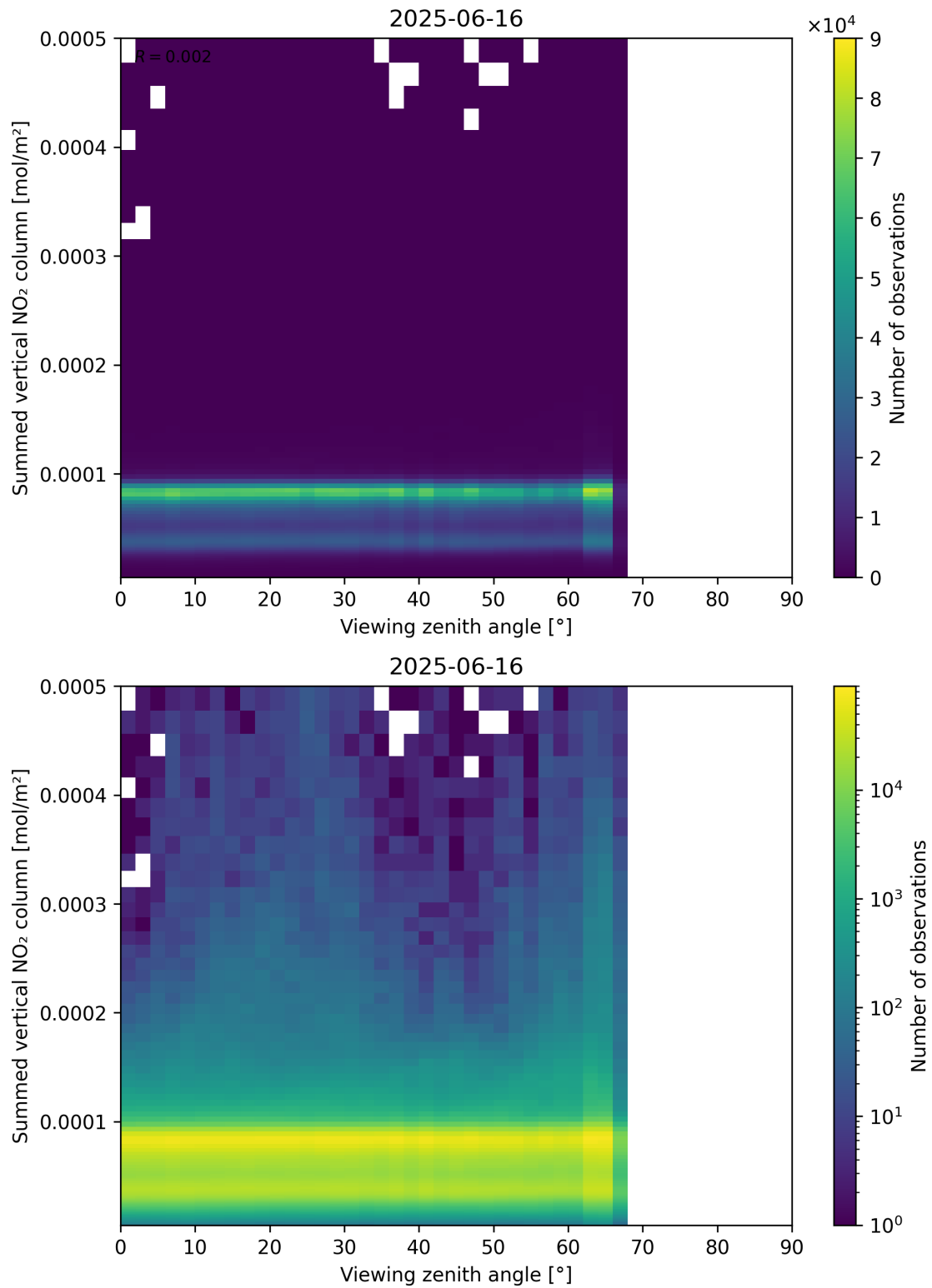
Figure 165: Scatter density plot of “Viewing zenith angle” against “Summed vertical NO 2 column” for 2025-06-16 to 2025-06-17.
