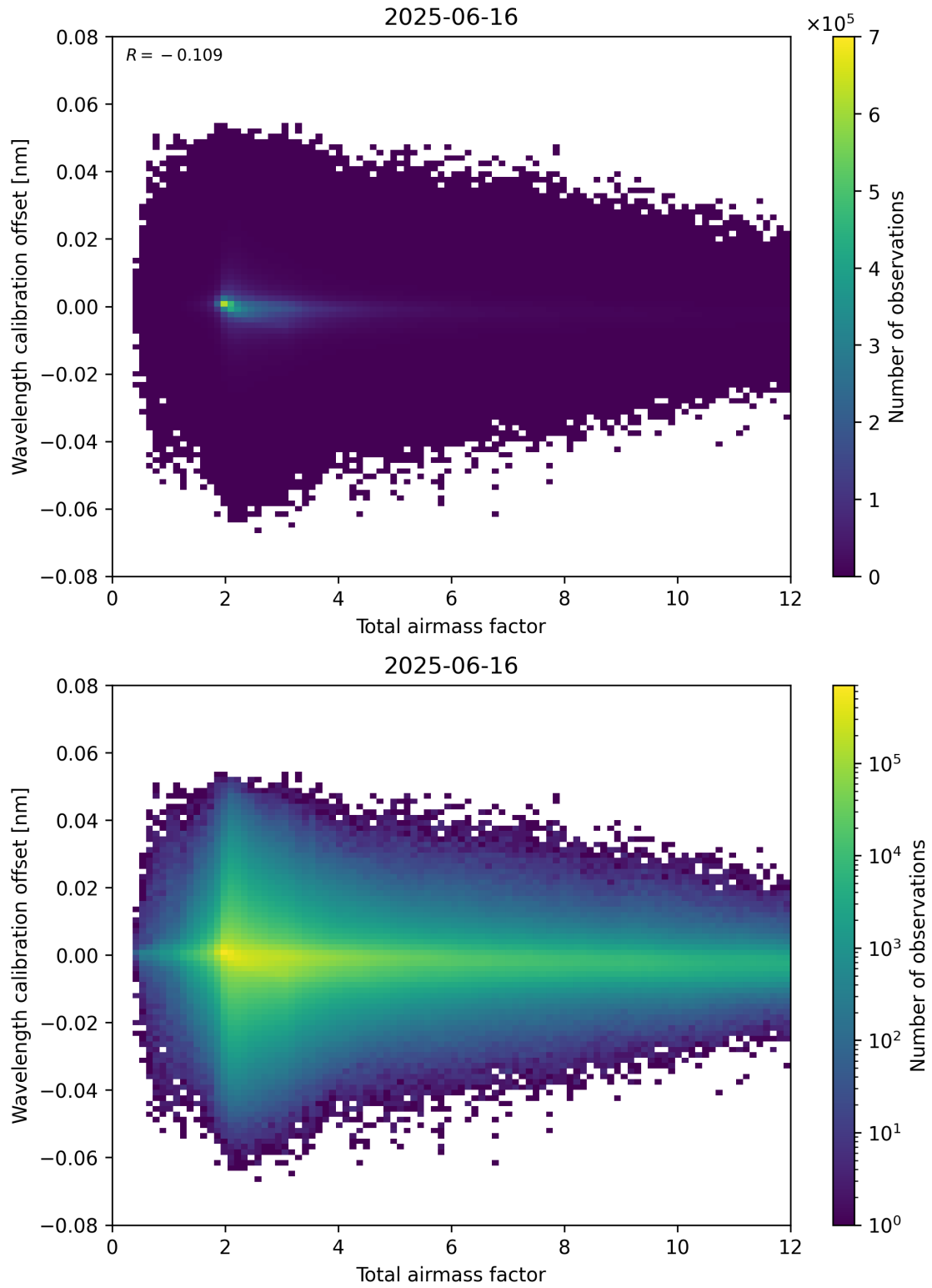
Figure 70: Scatter density plot of “Total airmass factor” against “Wavelength calibration offset” for 2025-06-16 to 2025-06-17.
