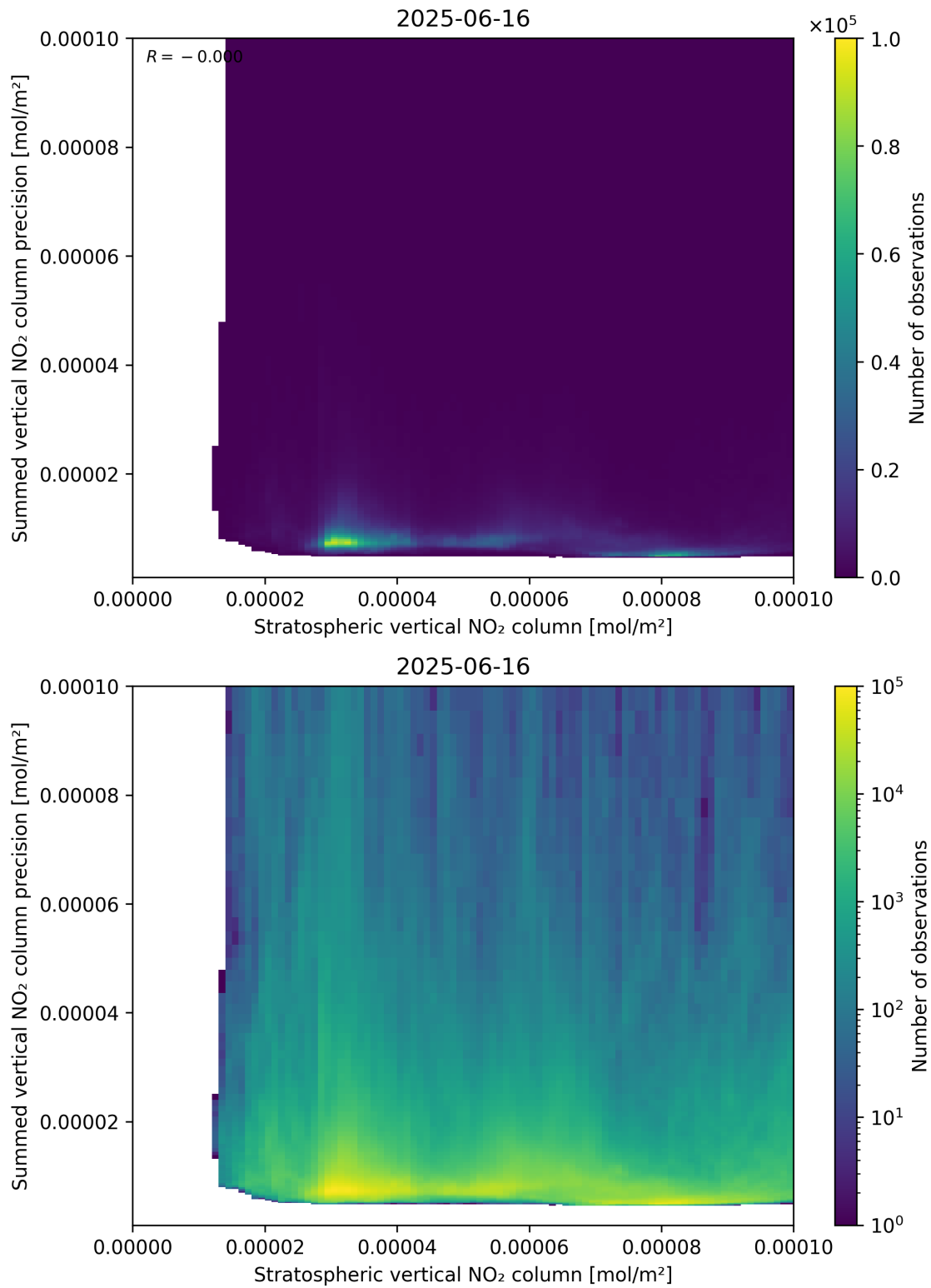
Figure 99: Scatter density plot of “Stratospheric vertical NO 2 column” against “Summed vertical NO 2 column precision” for 2025-06-16 to 2025-06-17.
