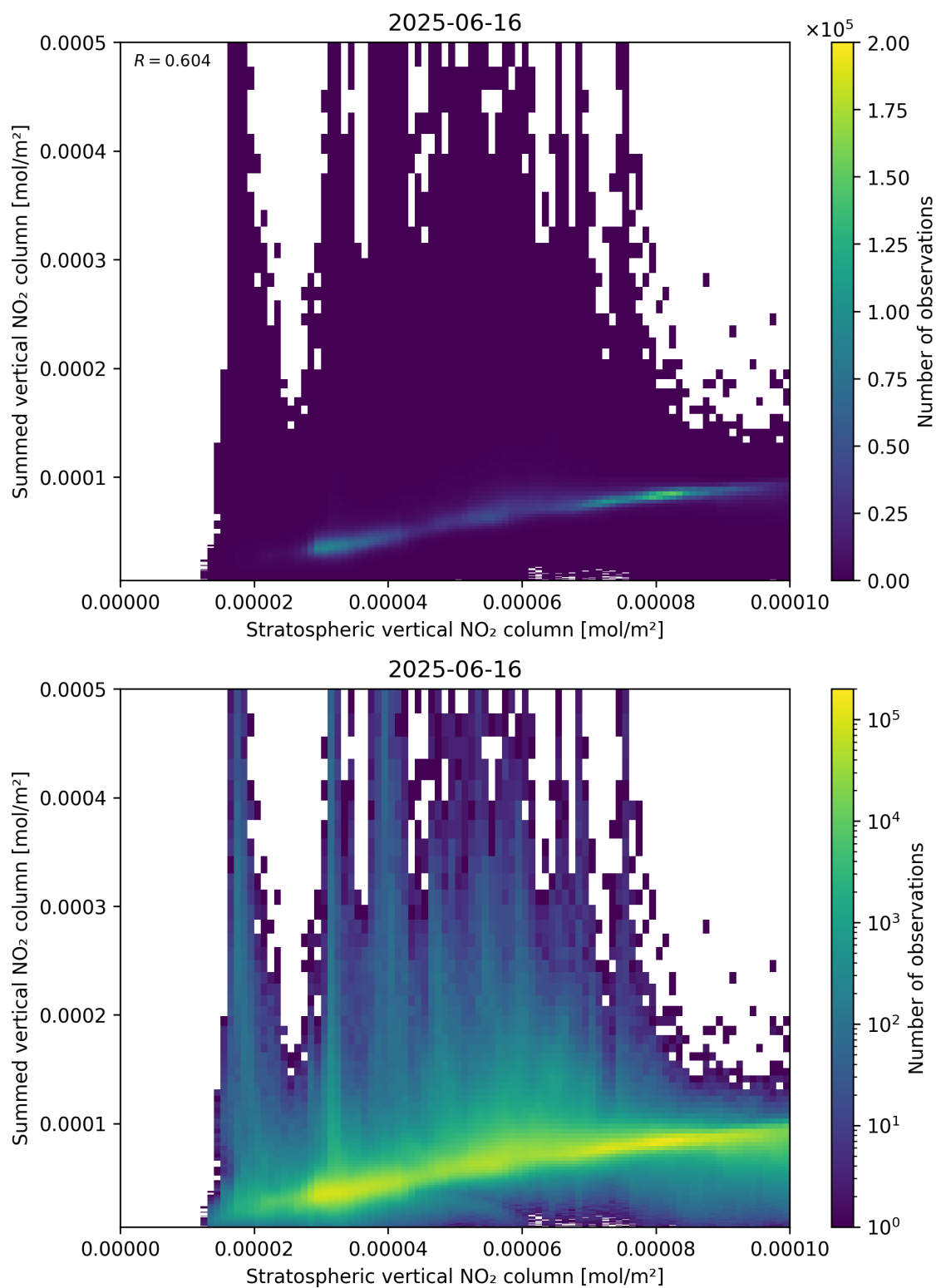
Figure 98: Scatter density plot of “Stratospheric vertical NO 2 column” against “Summed vertical NO 2 column” for 2025-06-16 to 2025-06-17.
