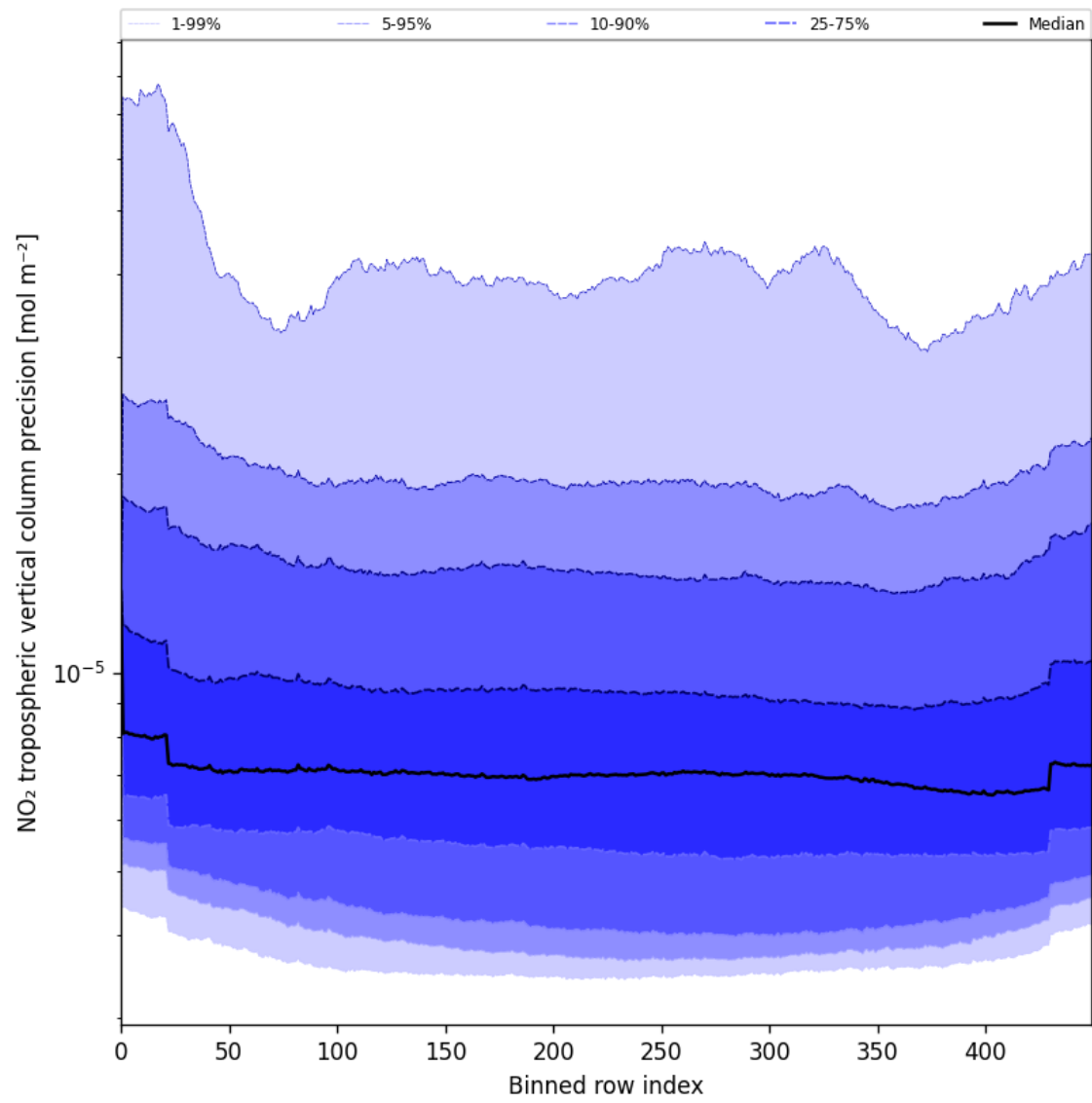
Figure 47: Along track statistics of “NO 2 tropospheric vertical column precision” for 2025-06-16 to 2025-06-17
