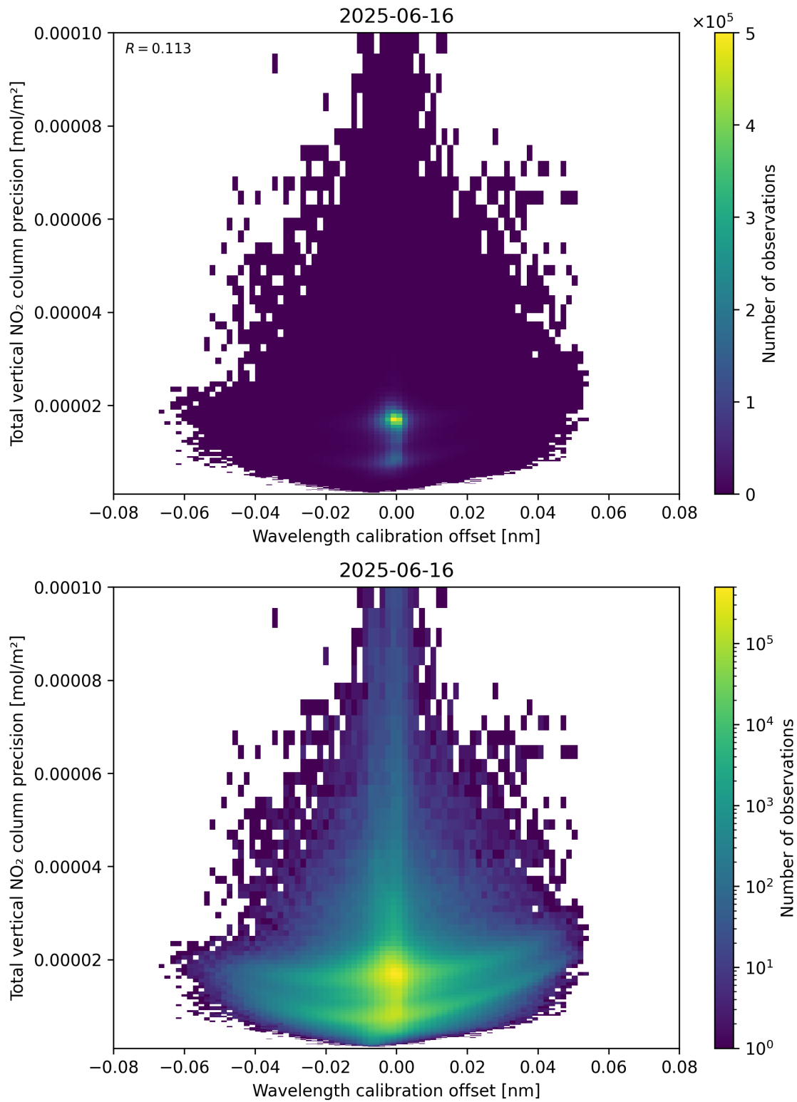
Figure 180: Scatter density plot of “Wavelength calibration offset” against “Total vertical NO 2 column precision” for 2025-06-16 to 2025-06-17.
