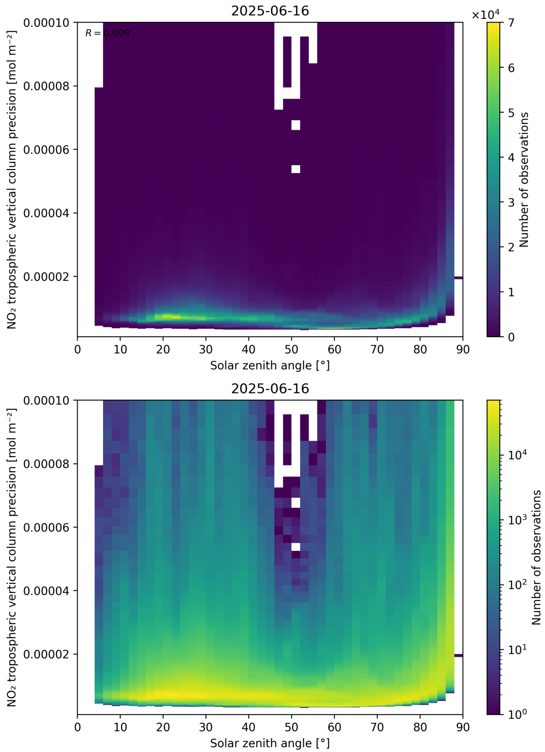
Figure 156: Scatter density plot of “Solar zenith angle” against “NO 2 tropospheric vertical column precision” for 2025-06-16 to 2025-06-17.
