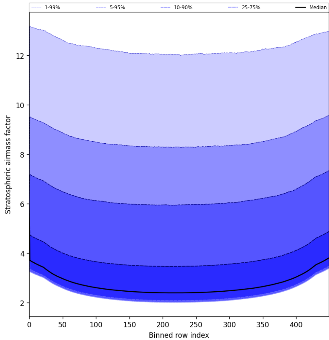
Figure 61: Along track statistics of “Stratospheric airmass factor” for 2025-06-16 to 2025-06-17
