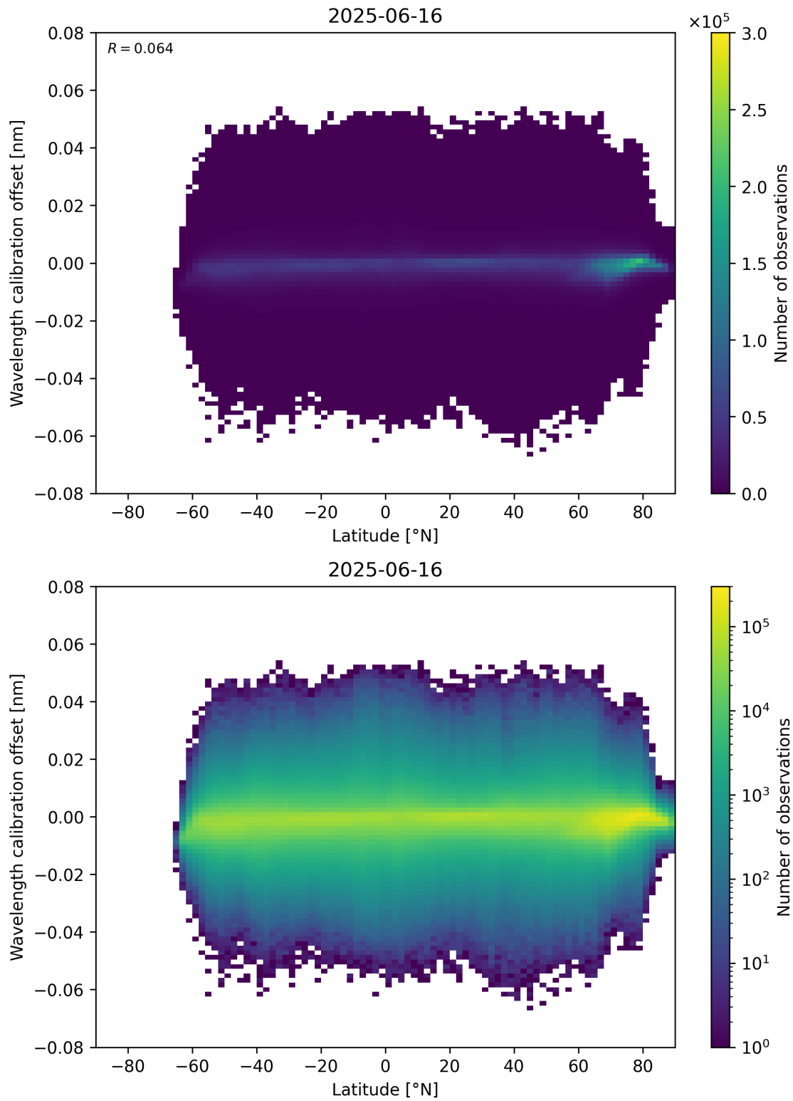
Figure 95: Scatter density plot of “Latitude” against “Wavelength calibration offset” for 2025-06-16 to 2025-06-17.
