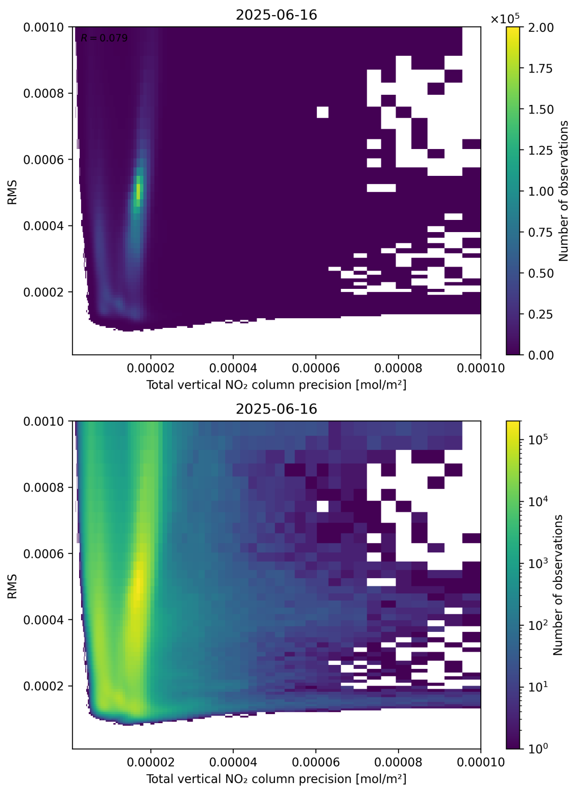
Figure 119: Scatter density plot of “Total vertical NO 2 column precision” against “RMS” for 2025-06-16 to 2025-06-17.
