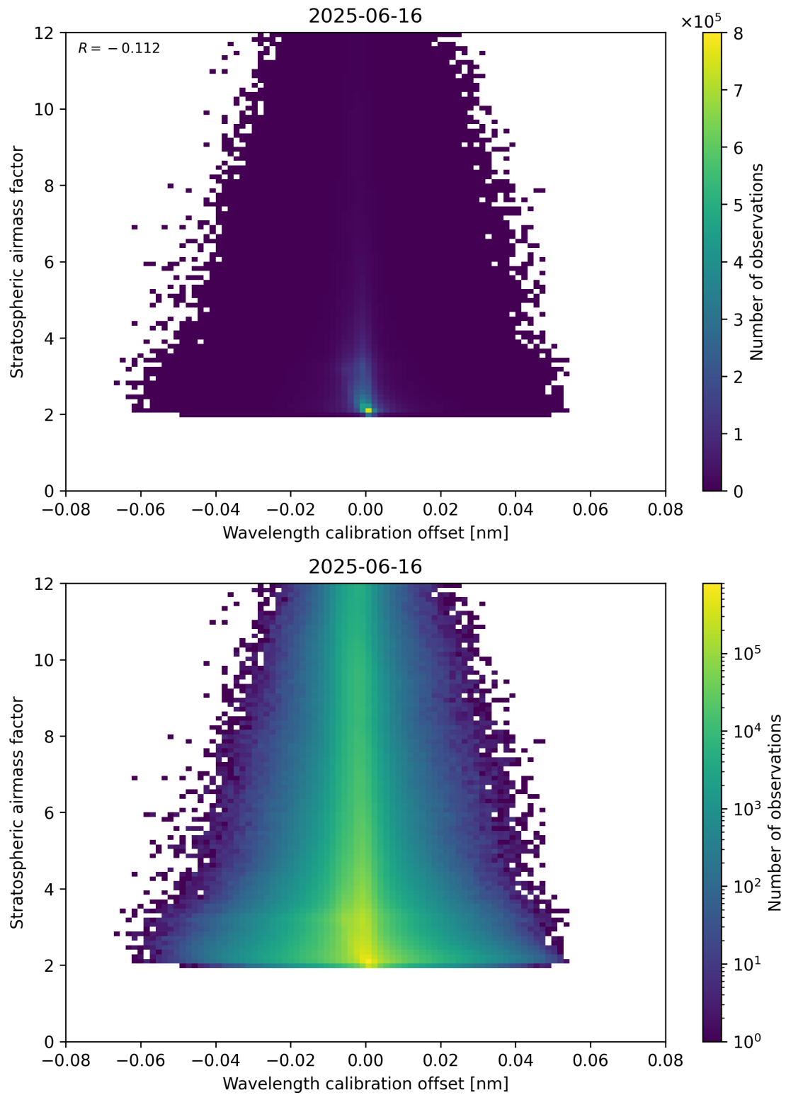
Figure 174: Scatter density plot of “Wavelength calibration offset” against “Stratospheric airmass factor” for 2025-06-16 to 2025-06-17.
