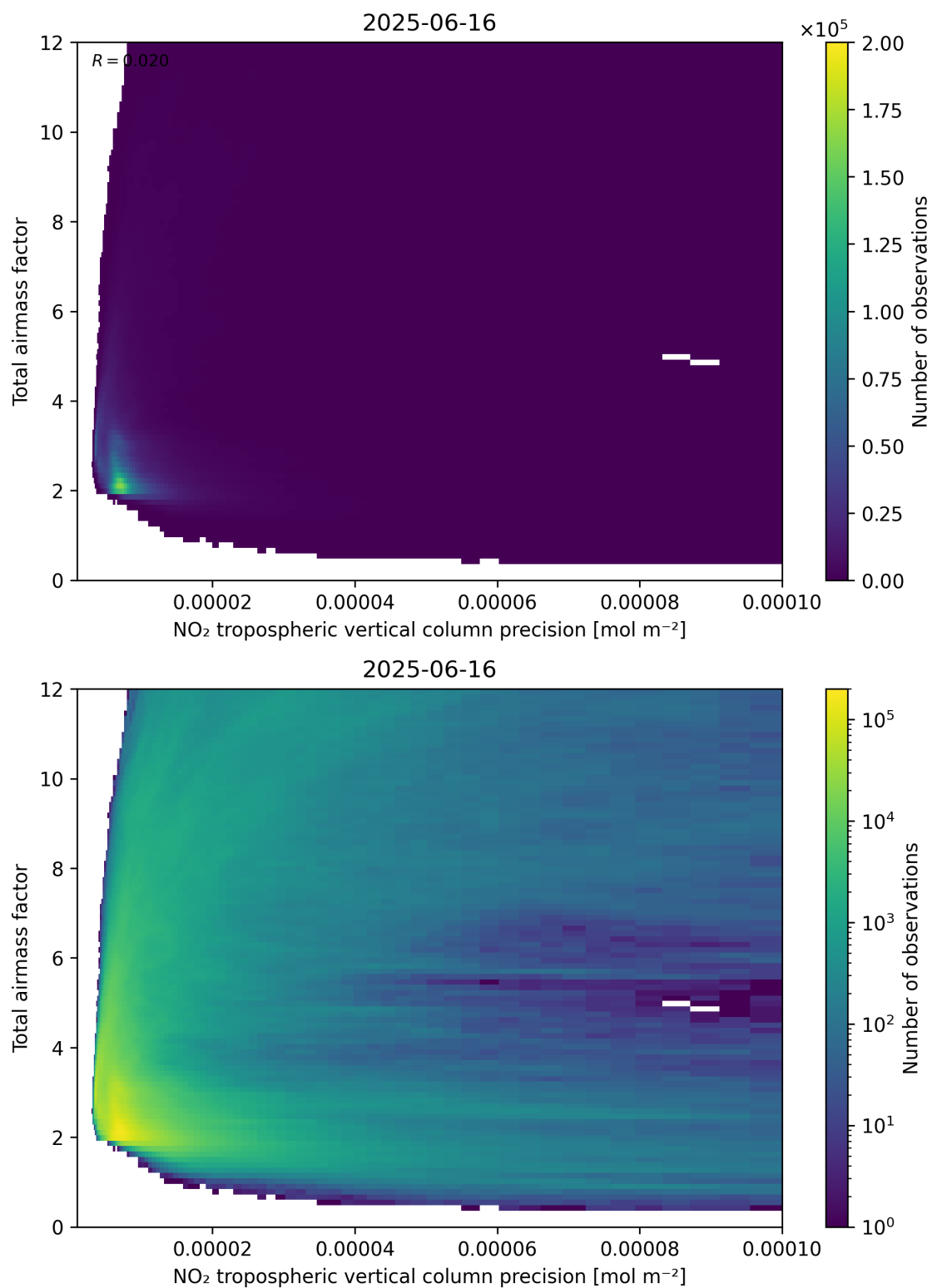
Figure 132: Scatter density plot of “NO 2 tropospheric vertical column precision” against “Total air mass factor” for 2025-06-16 to 2025-06-17.
