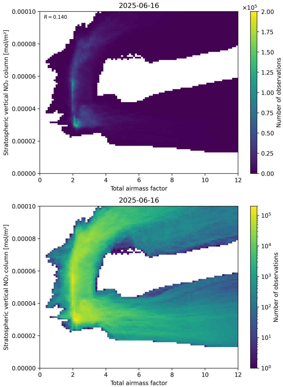
Figure 64: Scatter density plot of “Total airmass factor” against “Stratospheric vertical NO 2 column” for 2025-06-16 to 2025-06-17.
