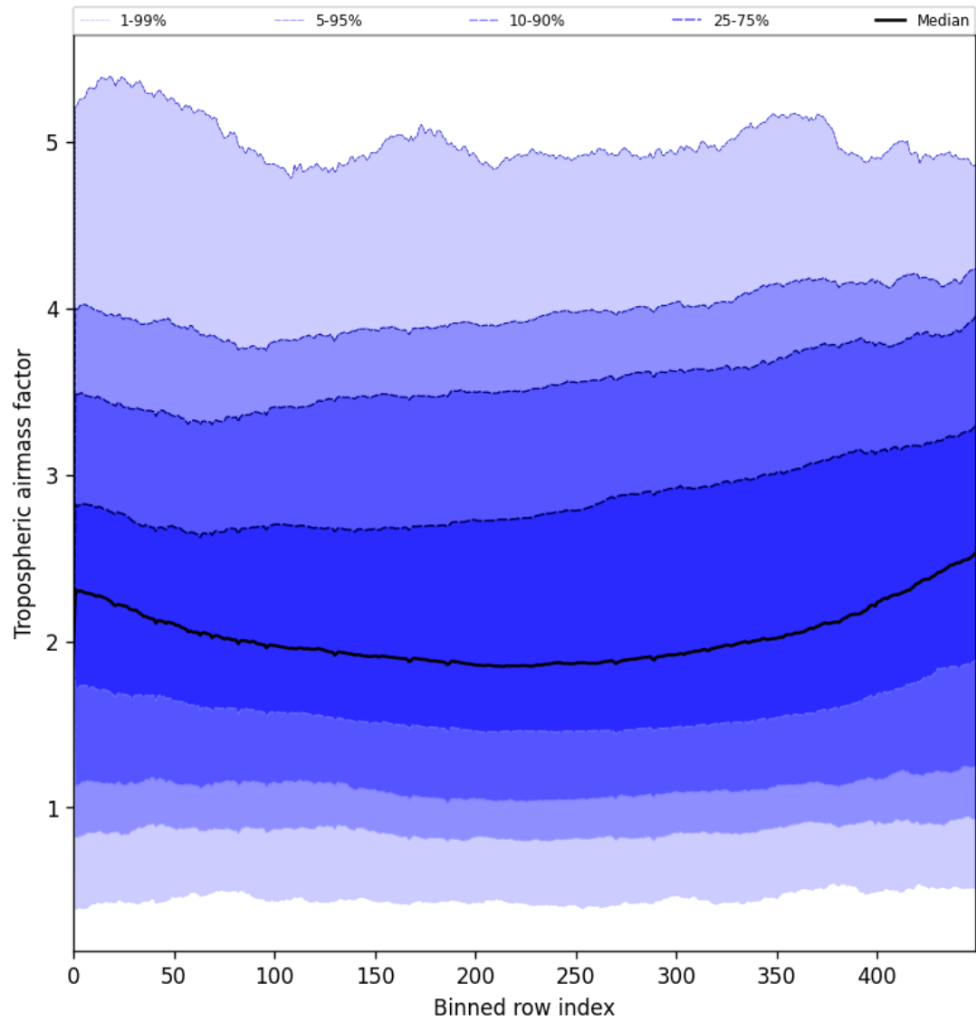
Figure 48: Along track statistics of “Tropospheric airmass factor” for 2025-06-16 to 2025-06-17
