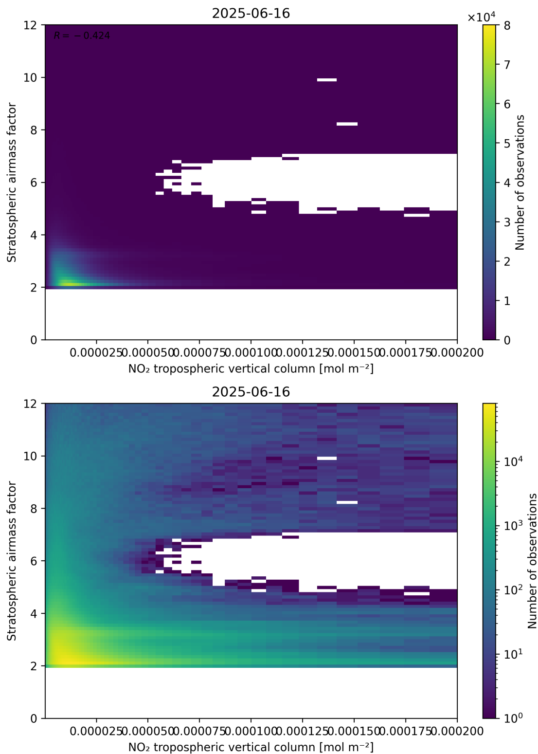
Figure 121: Scatter density plot of “NO 2 tropospheric vertical column” against “Stratospheric air mass factor” for 2025-06-16 to 2025-06-17.
