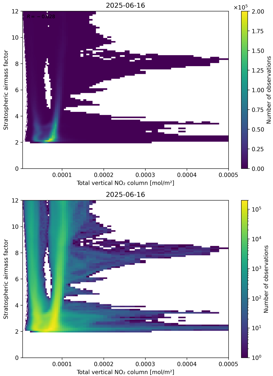
Figure 110: Scatter density plot of “Total vertical NO 2 column” against “Stratospheric air mass factor” for 2025-06-16 to 2025-06-17.
