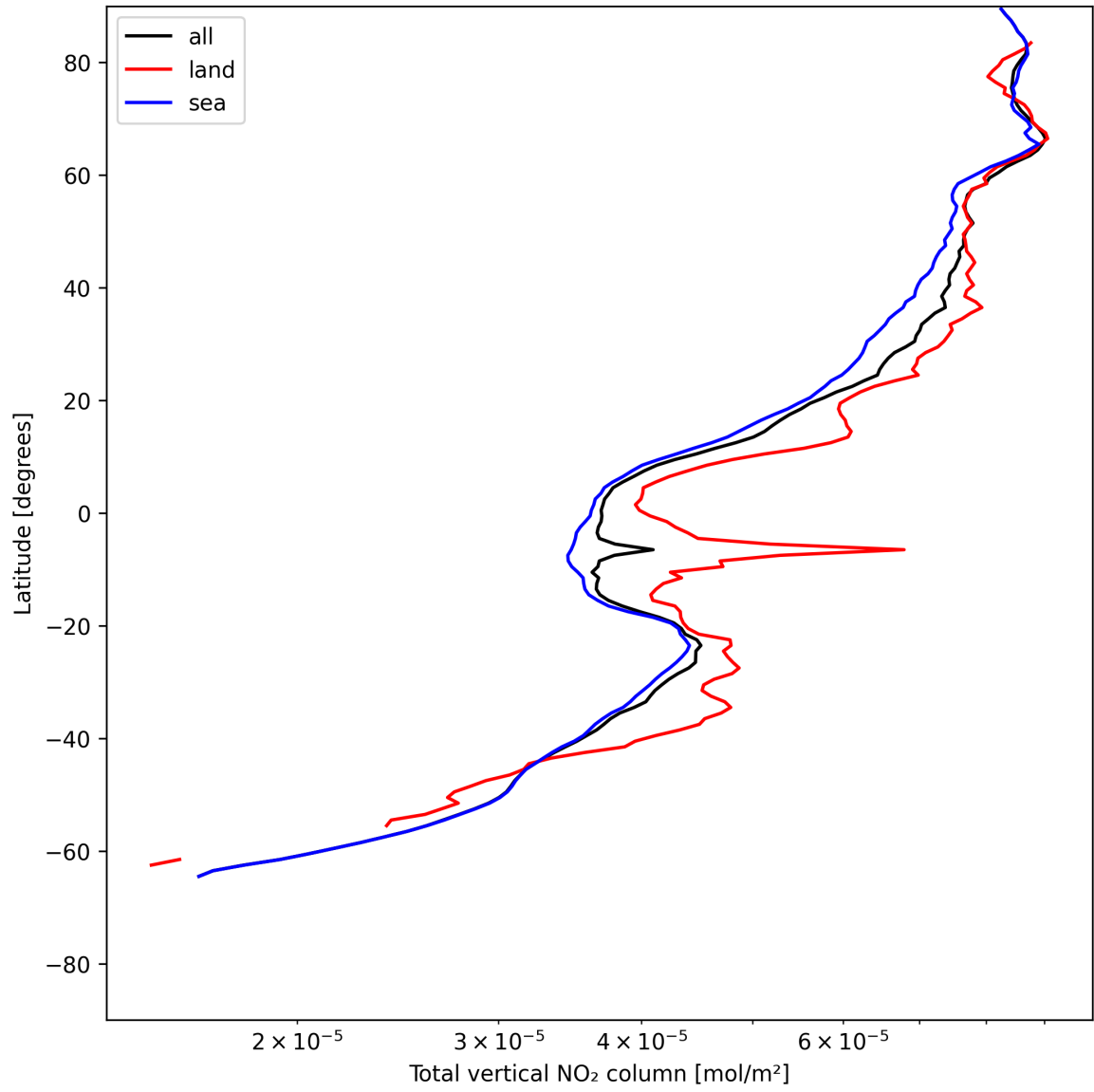
Figure 21: Zonal average of “Total vertical NO 2 column” for 2025-06-16 to 2025-06-17.
