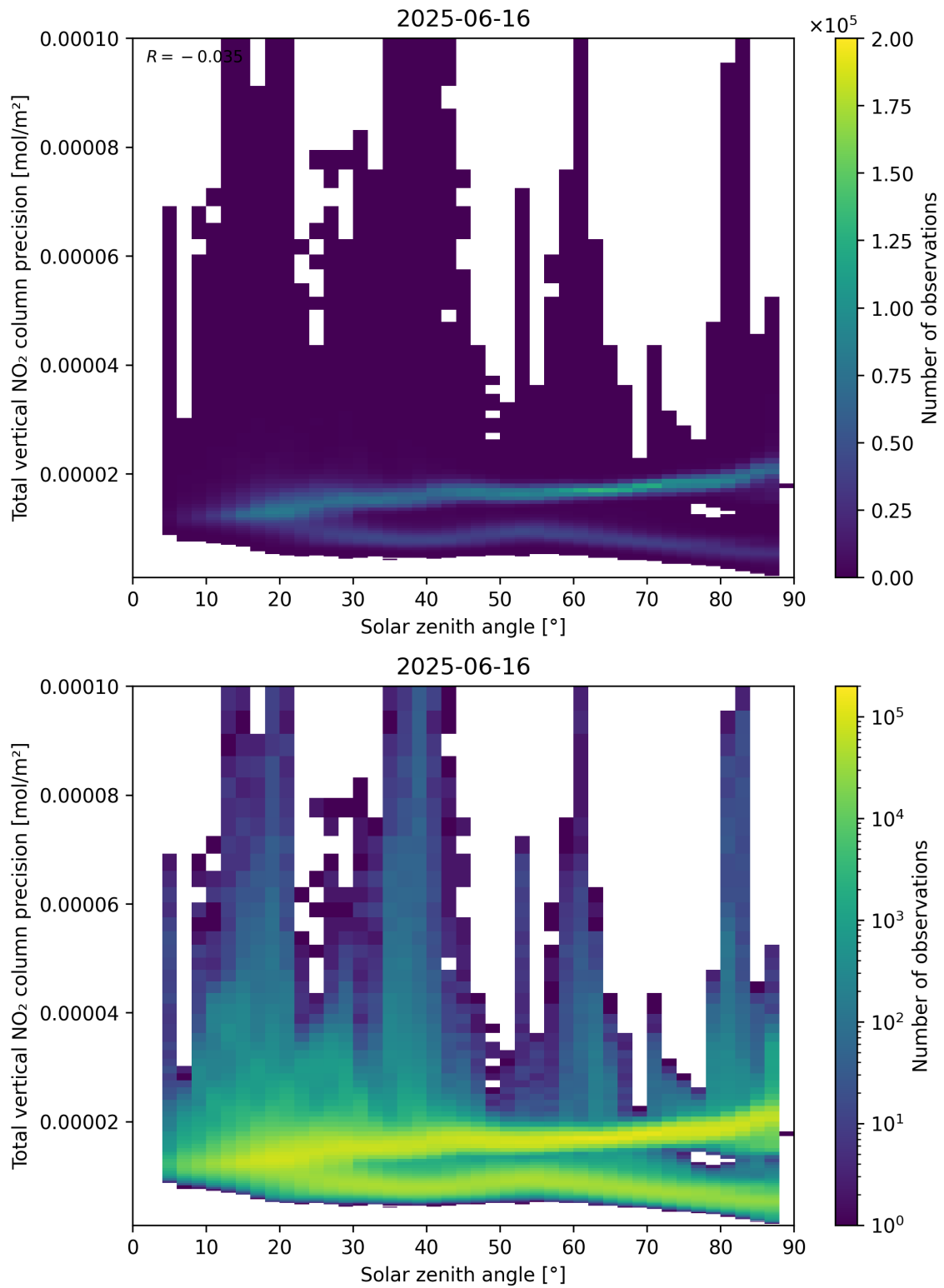
Figure 154: Scatter density plot of “Solar zenith angle” against “Total vertical NO 2 column precision” for 2025-06-16 to 2025-06-17.
