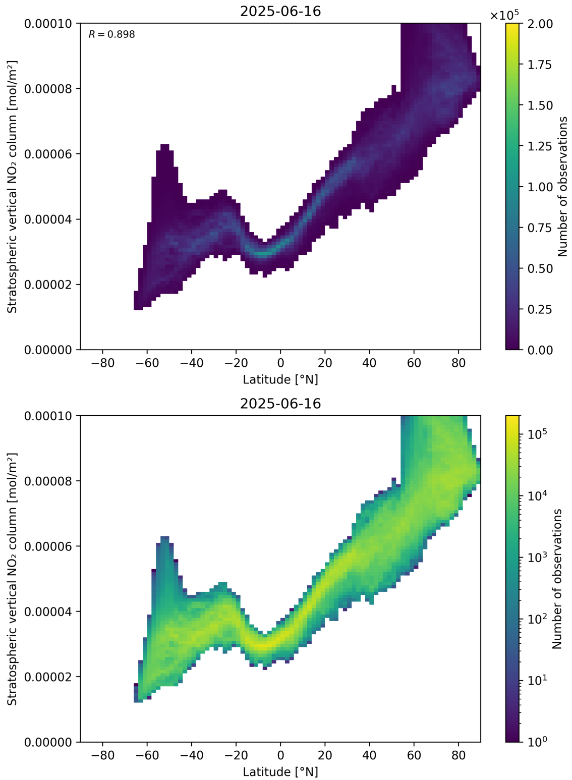
Figure 87: Scatter density plot of “Latitude” against “Stratospheric vertical NO 2 column” for 2025-06-16 to 2025-06-17.
