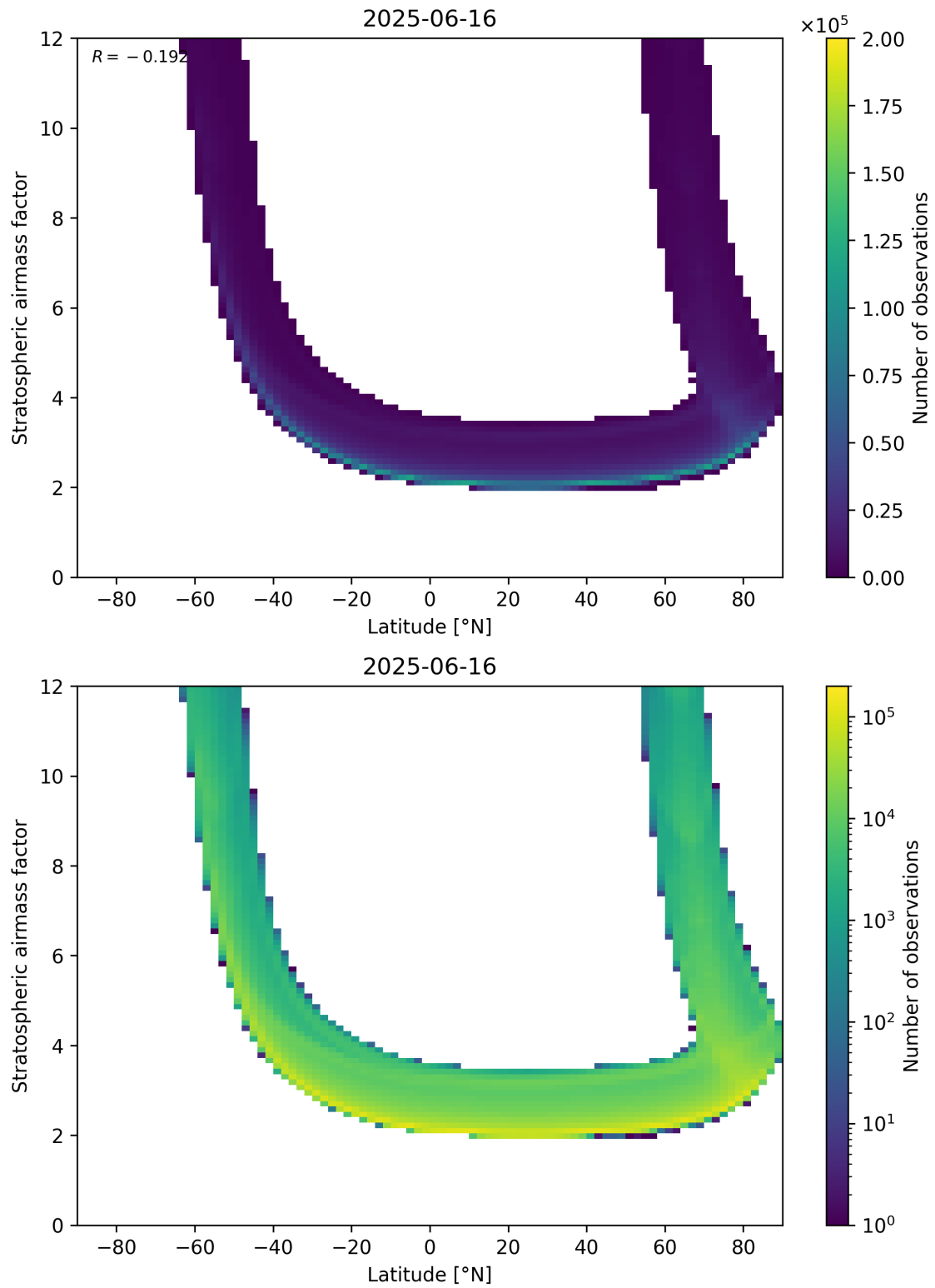
Figure 83: Scatter density plot of “Latitude” against “Stratospheric air mass factor” for 2025-06-16 to 2025-06-17.
