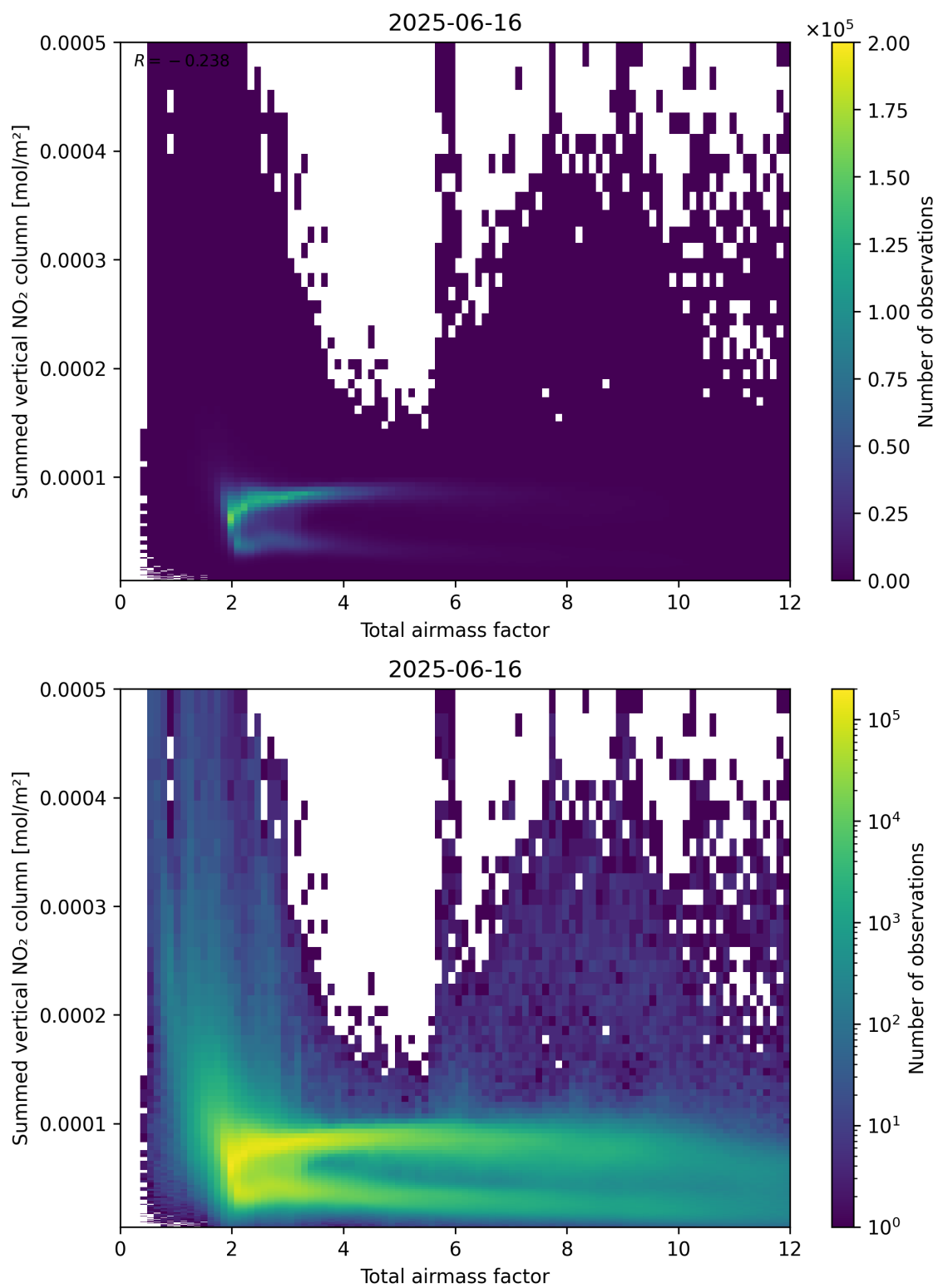
Figure 65: Scatter density plot of “Total airmass factor” against “Summed vertical NO 2 column” for 2025-06-16 to 2025-06-17.
