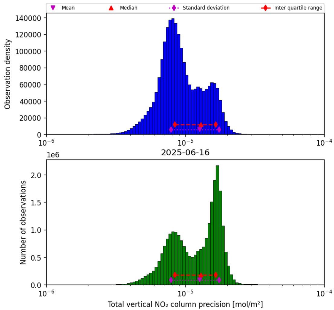
Figure 39: Histogram of “Total vertical NO 2 column precision” for 2025-06-16 to 2025-06-17
