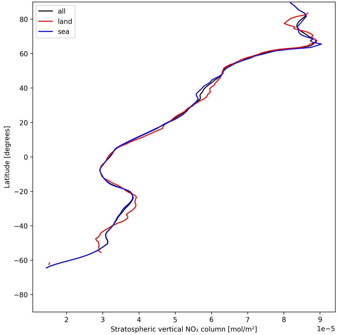
Figure 19: Zonal average of “Stratospheric vertical NO 2 column” for 2025-06-16 to 2025-06-17.
