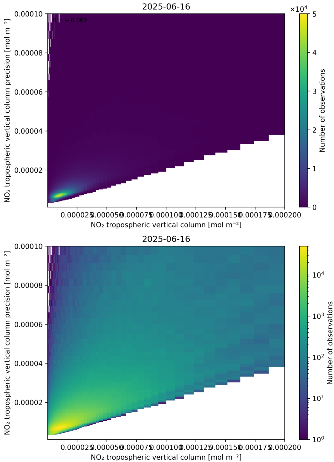
Figure 130: Scatter density plot of “NO 2 tropospheric vertical column” against “NO 2 tropospheric vertical column precision” for 2025-06-16 to 2025-06-17.
