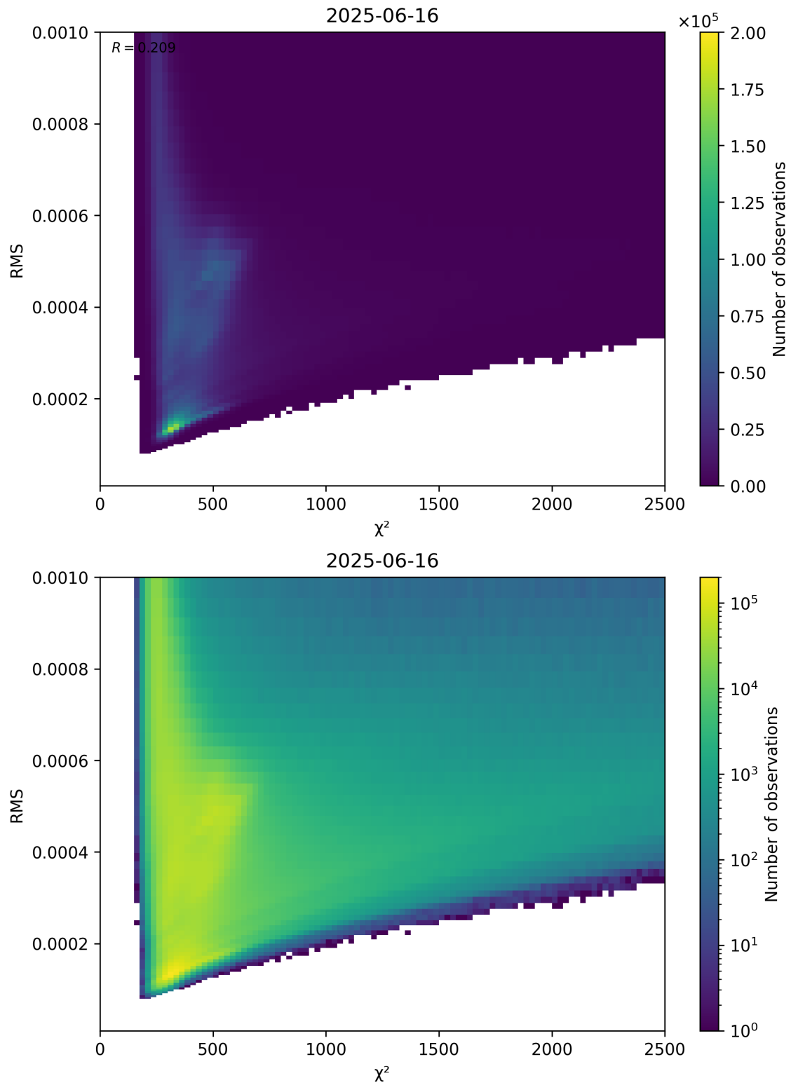
Figure 82: Scatter density plot of “ \chi^2 ” against “RMS” for 2025-06-16 to 2025-06-17.
