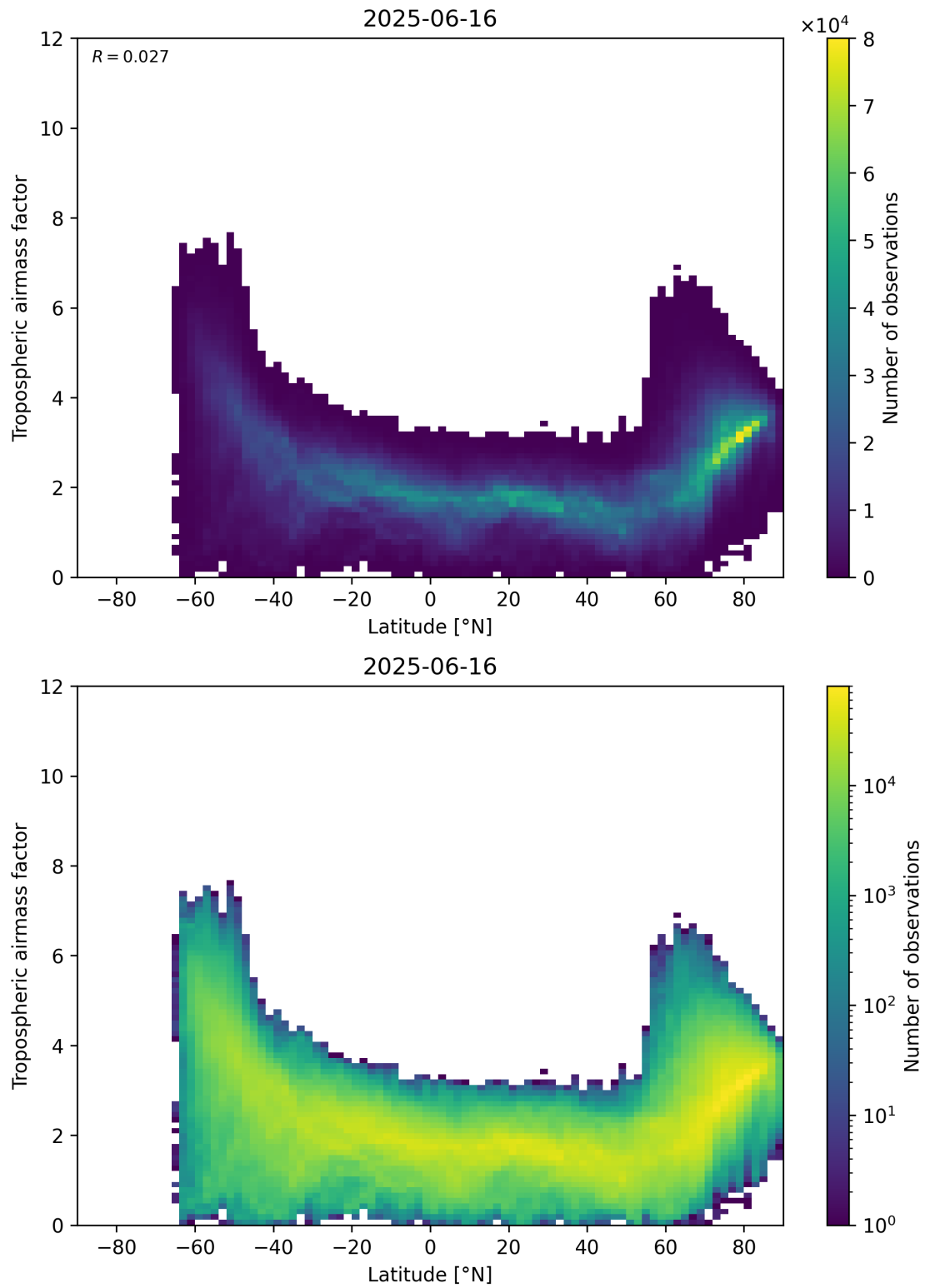
Figure 85: Scatter density plot of “Latitude” against “Tropospheric airmass factor” for 2025-06-16 to 2025-06-17.
