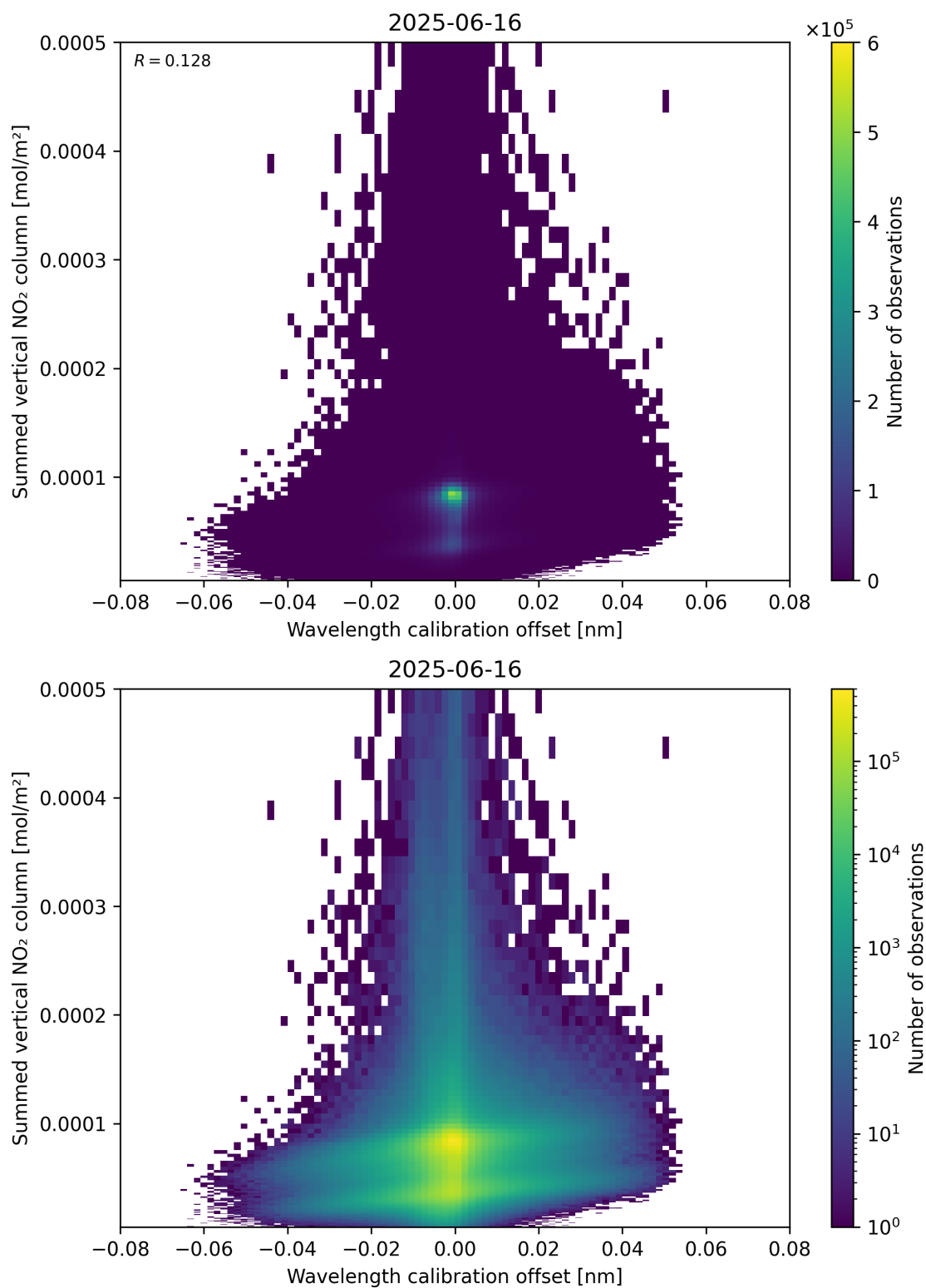
Figure 177: Scatter density plot of “Wavelength calibration offset” against “Summed vertical NO 2 column” for 2025-06-16 to 2025-06-17.
