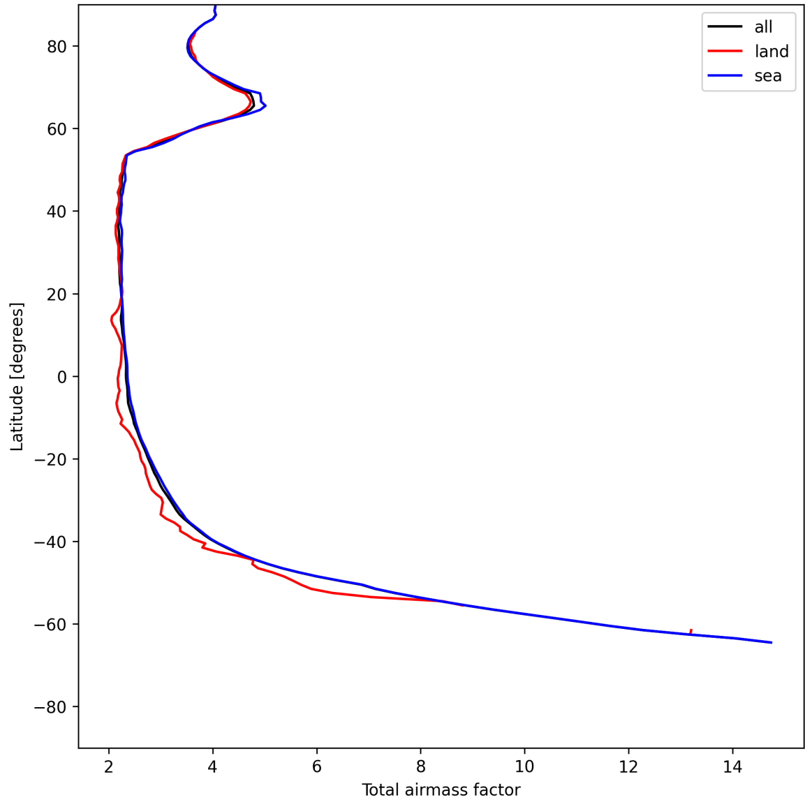
Figure 15: Zonal average of “Total airmass factor” for 2025-06-16 to 2025-06-17.
