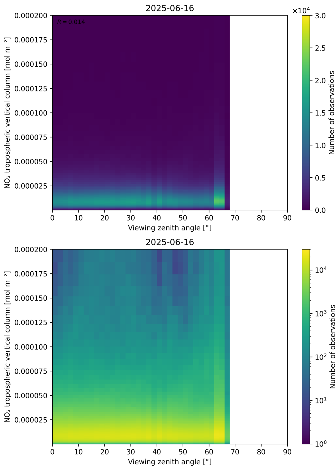
Figure 169: Scatter density plot of “Viewing zenith angle” against “NO 2 tropospheric vertical column” for 2025-06-16 to 2025-06-17.
