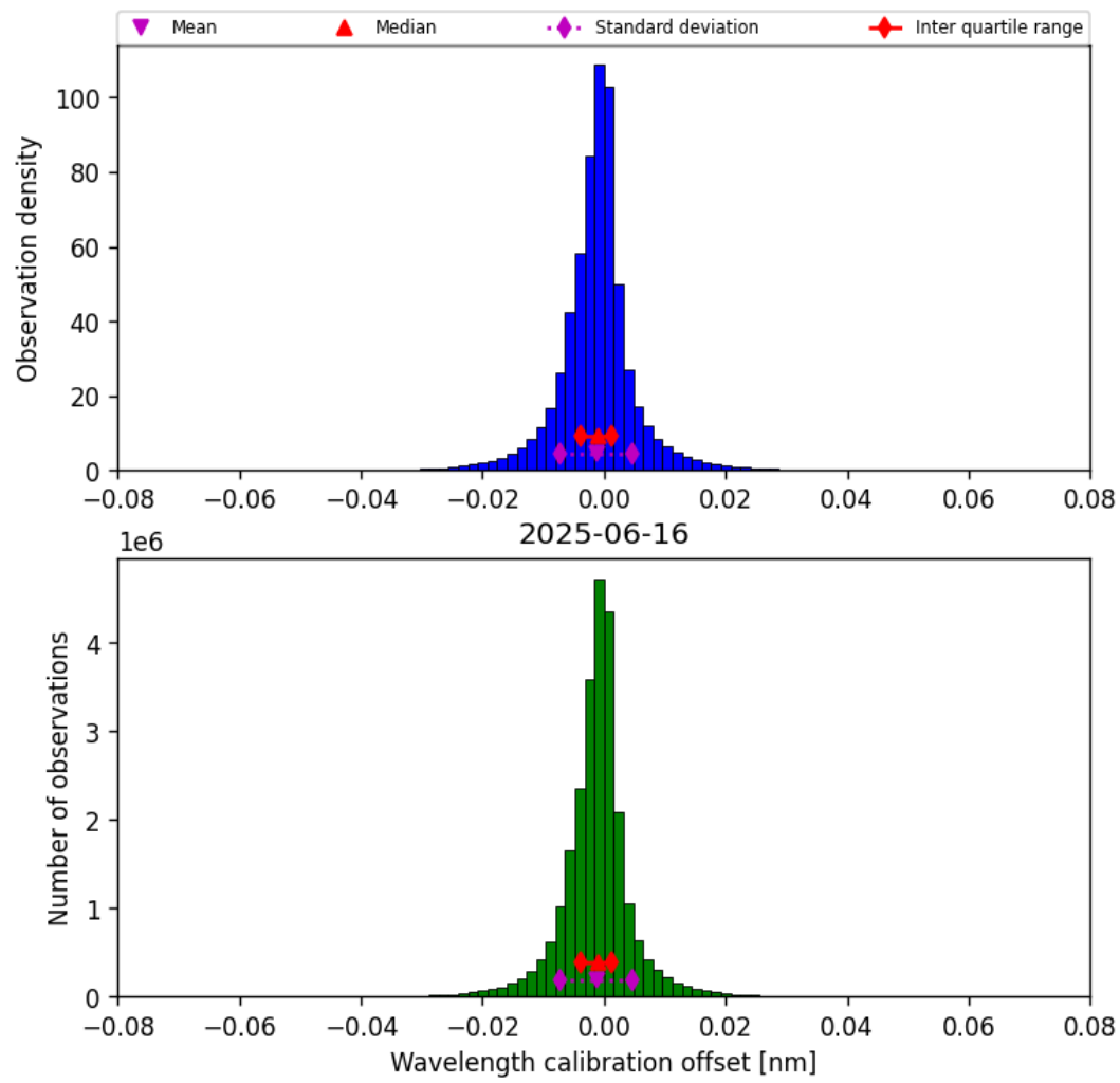
Figure 35: Histogram of “Wavelength calibration offset” for 2025-06-16 to 2025-06-17
