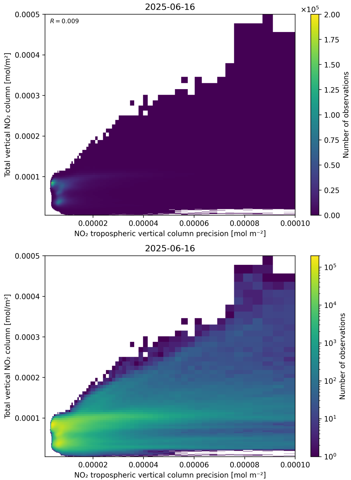
Figure 138: Scatter density plot of “NO 2 tropospheric vertical column precision” against “Total vertical NO 2 column” for 2025-06-16 to 2025-06-17.
