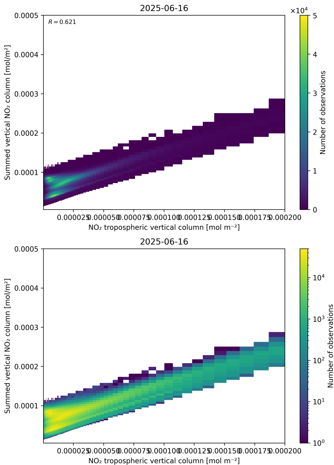
Figure 126: Scatter density plot of “NO 2 tropospheric vertical column” against “Summed vertical NO 2 column” for 2025-06-16 to 2025-06-17.
