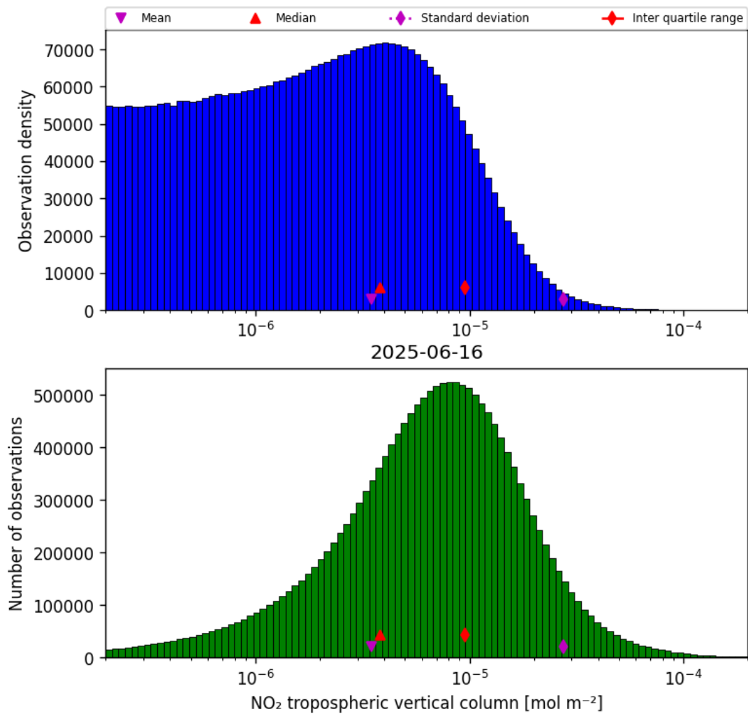
Figure 29: Histogram of “NO 2 tropospheric vertical column” for 2025-06-16 to 2025-06-17
