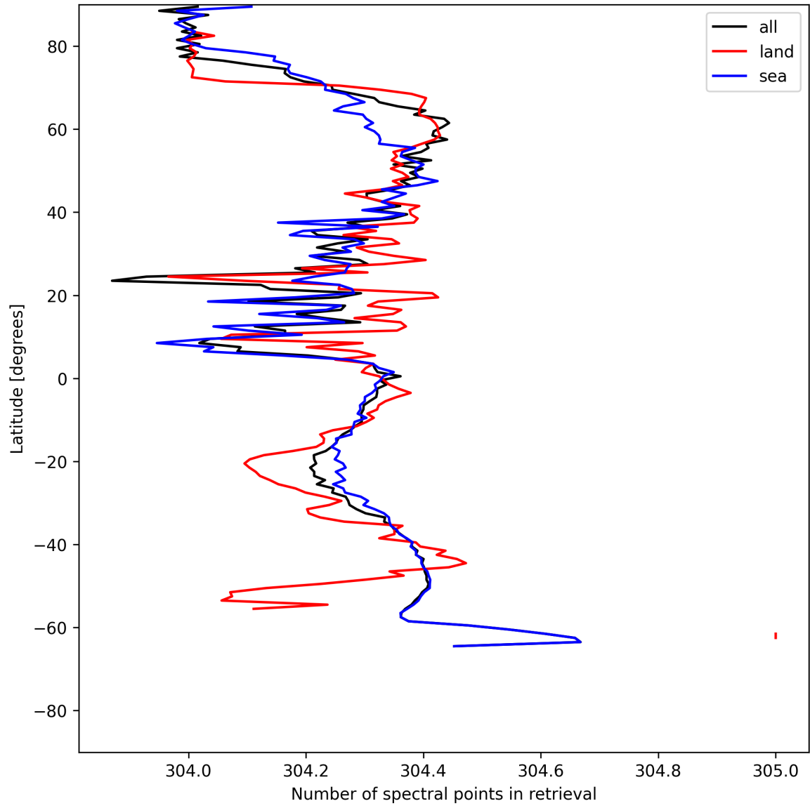
Figure 16: Zonal average of “Number of spectral points in retrieval” for 2025-06-16 to 2025-06-17.
