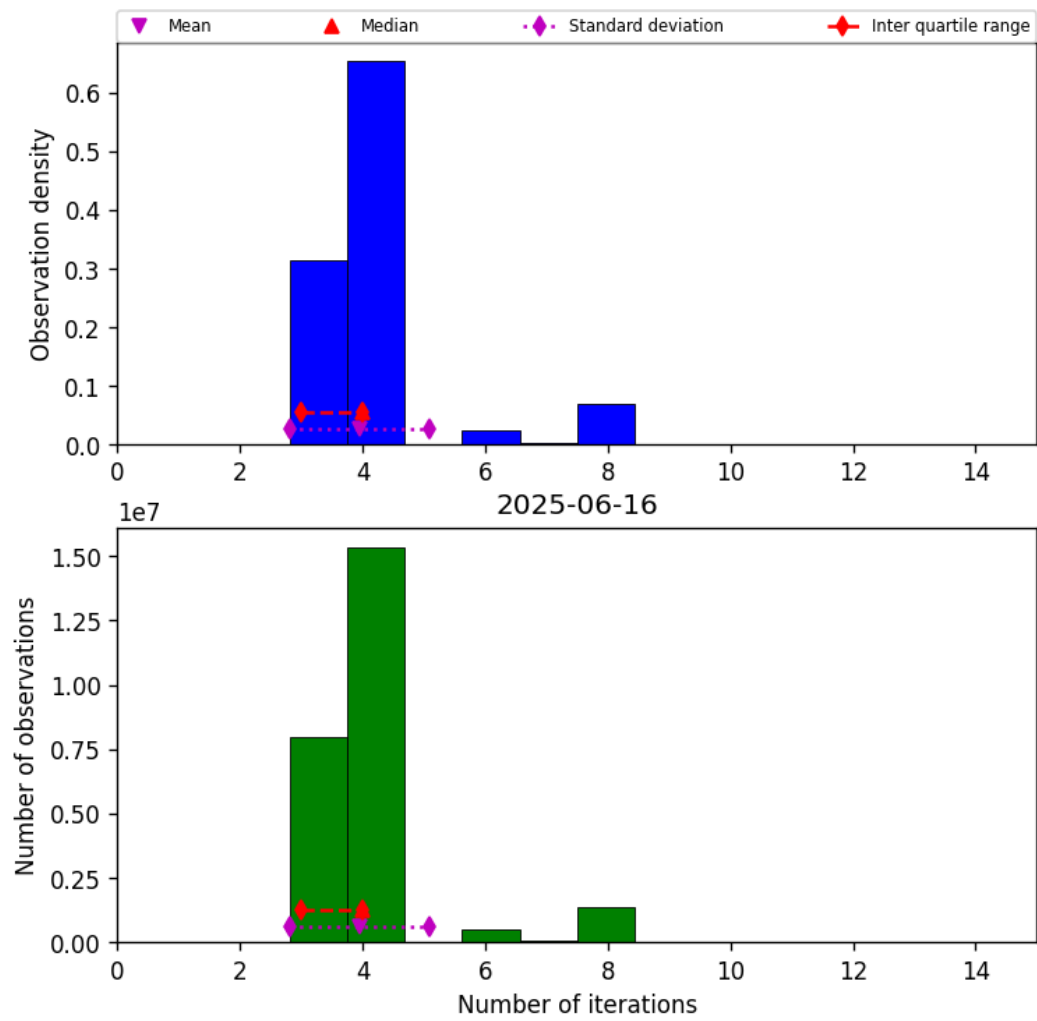
Figure 34: Histogram of “Number of iterations” for 2025-06-16 to 2025-06-17
