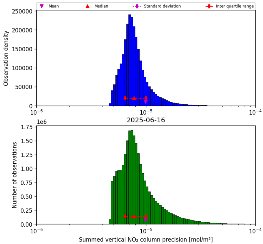
Figure 41: Histogram of "Summed vertical NO 2 column precision" for 2025-06-16 to 2025-06-17
