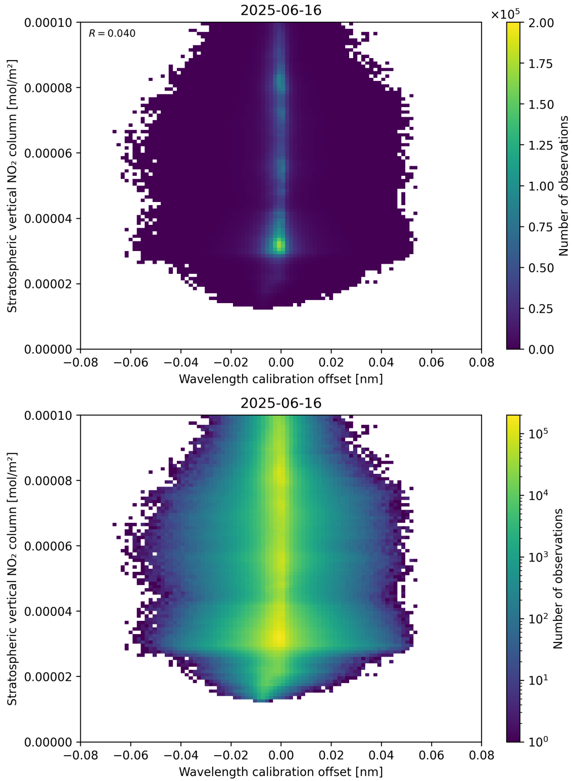
Figure 176: Scatter density plot of “Wavelength calibration offset” against “Stratospheric vertical NO 2 column” for 2025-06-16 to 2025-06-17.
