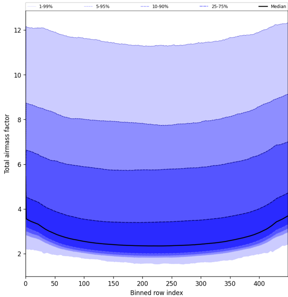
Figure 49: Along track statistics of “Total airmass factor” for 2025-06-16 to 2025-06-17
