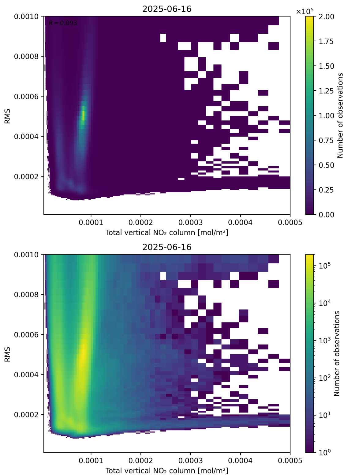
Figure 120: Scatter density plot of “Total vertical NO 2 column” against “RMS” for 2025-06-16 to 2025-06-17.
