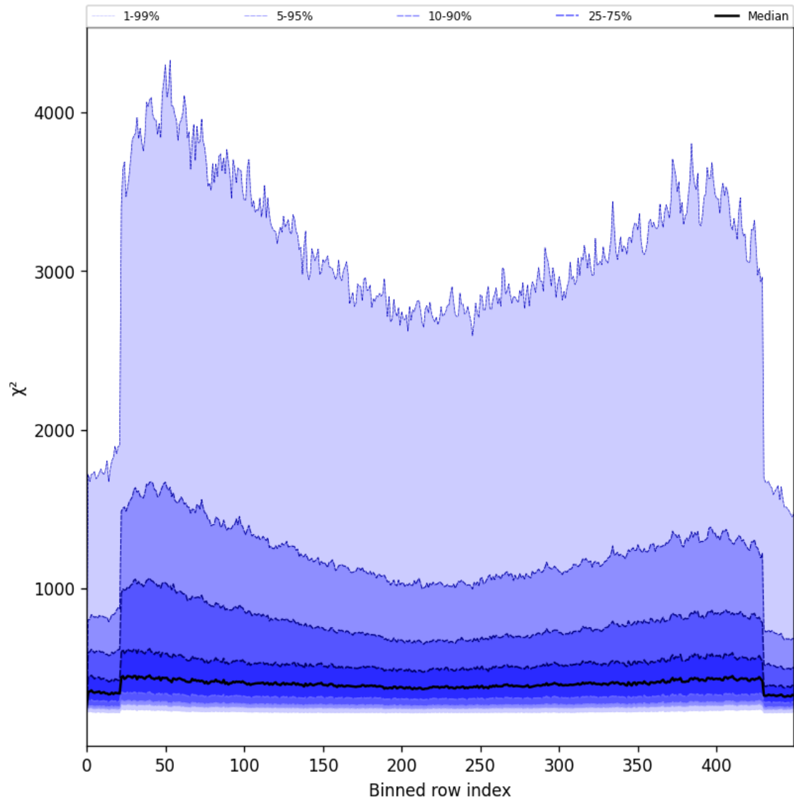
Figure 59: Along track statistics of “ \chi^2 ” for 2025-06-16 to 2025-06-17
