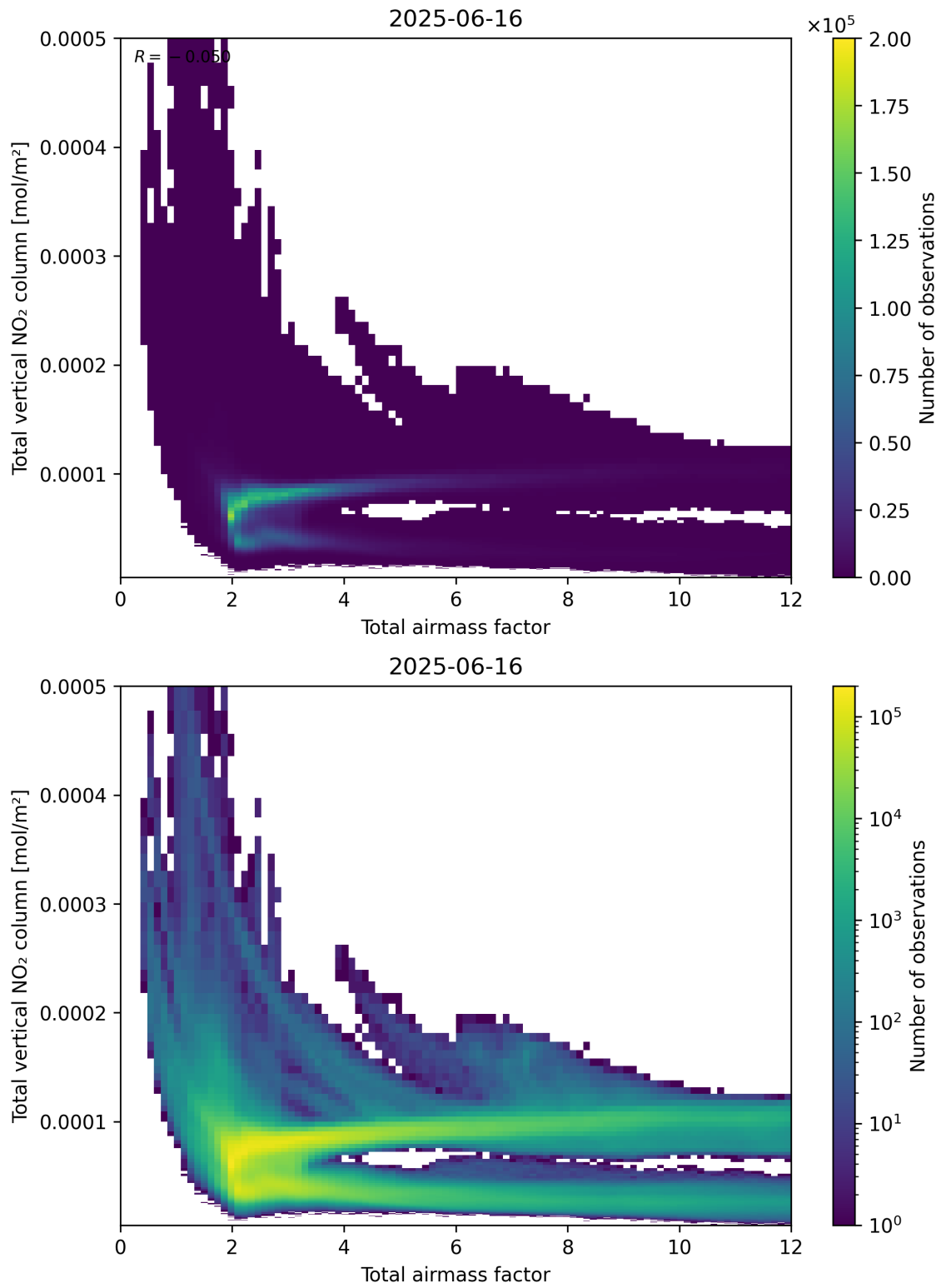
Figure 67: Scatter density plot of “Total airmass factor” against “Total vertical NO 2 column” for 2025-06-16 to 2025-06-17.
