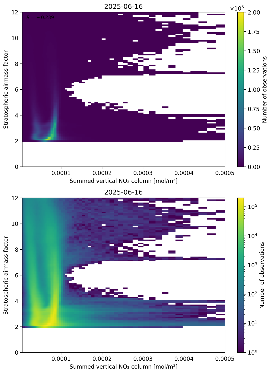
Figure 103: Scatter density plot of “Summed vertical NO 2 column” against “Stratospheric air mass factor” for 2025-06-16 to 2025-06-17.
