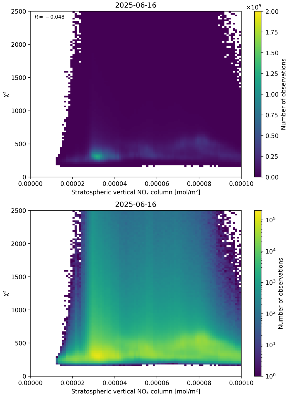
Figure 97: Scatter density plot of “Stratospheric vertical NO 2 column” against “ \chi^2 ” for 2025-06-16 to 2025-06-17.
