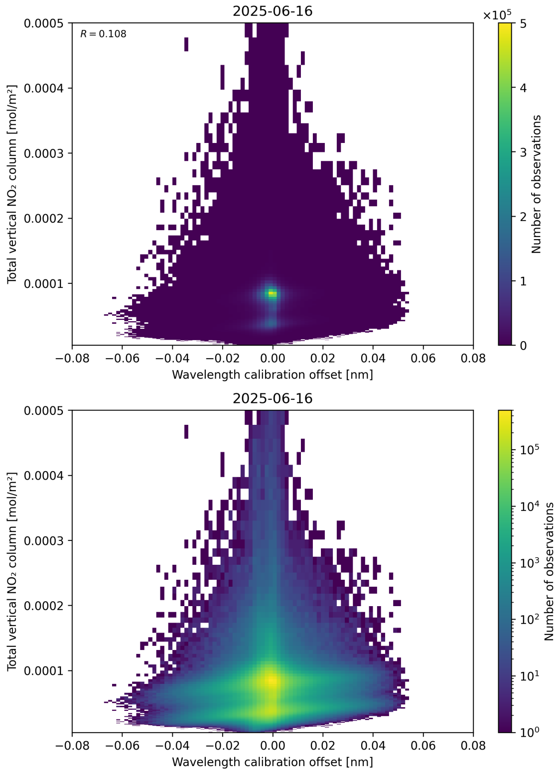
Figure 179: Scatter density plot of “Wavelength calibration offset” against “Total vertical NO 2 column” for 2025-06-16 to 2025-06-17.
