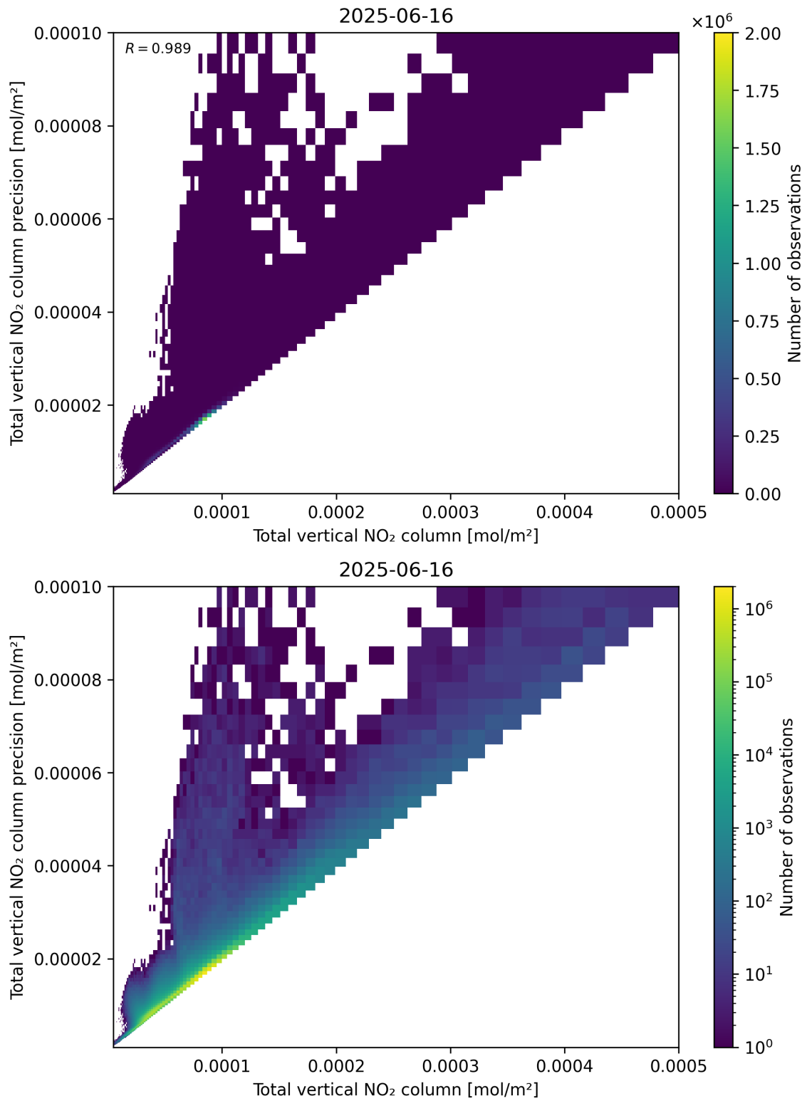
Figure 114: Scatter density plot of “Total vertical NO 2 column” against “Total vertical NO 2 column precision” for 2025-06-16 to 2025-06-17.
