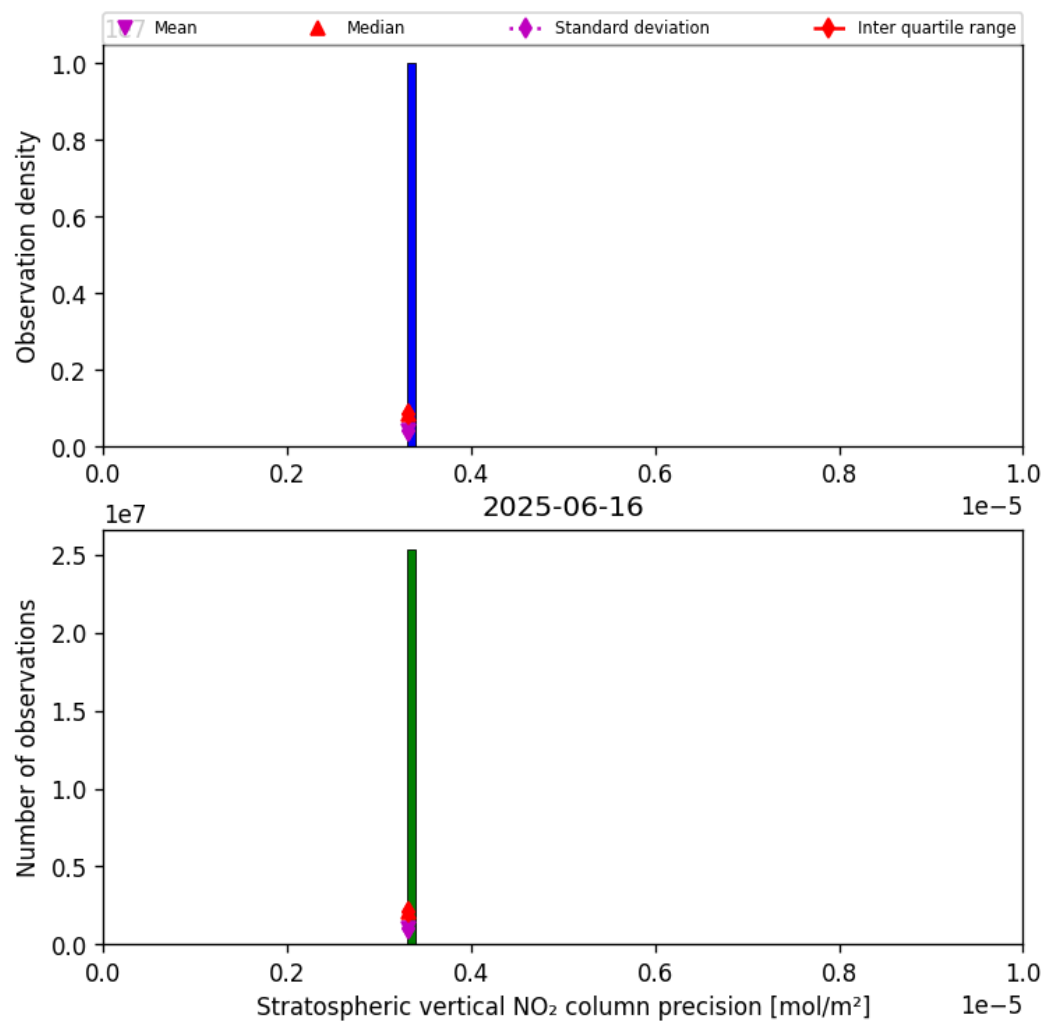
Figure 37: Histogram of “Stratospheric vertical NO 2 column precision” for 2025-06-16 to 2025-06-17
