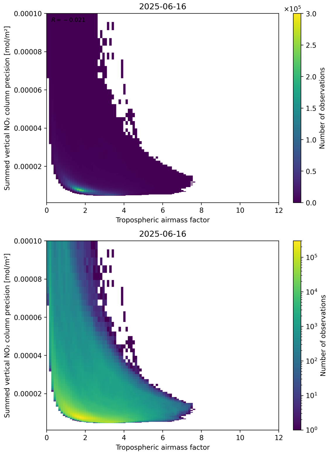
Figure 76: Scatter density plot of “Tropospheric air mass factor” against “Summed vertical NO 2 column precision” for 2025-06-16 to 2025-06-17.
