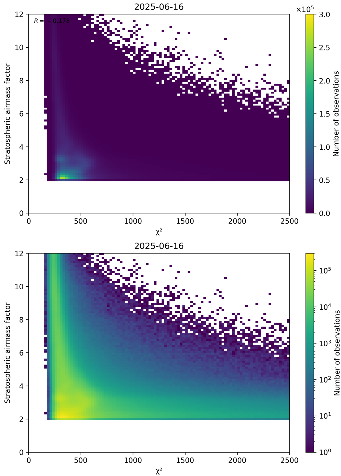
Figure 81: Scatter density plot of “ \chi^2 ” against “Stratospheric airmass factor” for 2025-06-16 to 2025-06-17.
