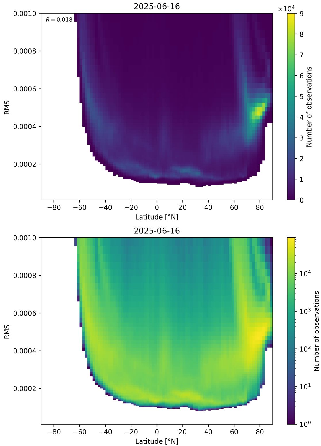
Figure 94: Scatter density plot of “Latitude” against “RMS” for 2025-06-16 to 2025-06-17.
