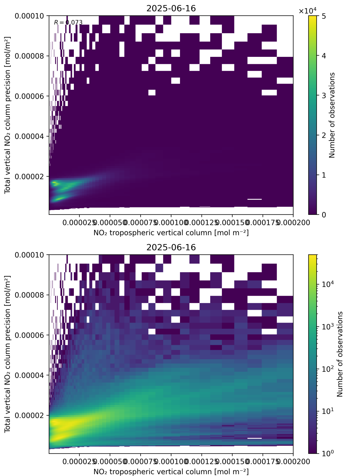
Figure 129: Scatter density plot of “NO 2 tropospheric vertical column” against “Total vertical NO 2 column precision” for 2025-06-16 to 2025-06-17.
