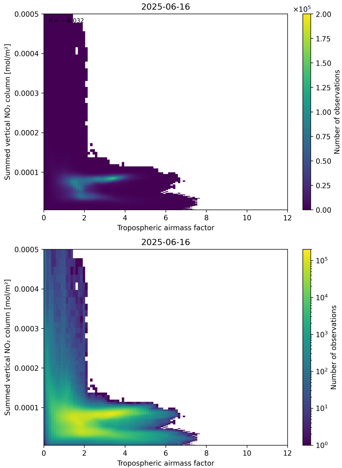
Figure 75: Scatter density plot of “Tropospheric airmass factor” against “Summed vertical NO 2 column” for 2025-06-16 to 2025-06-17.
