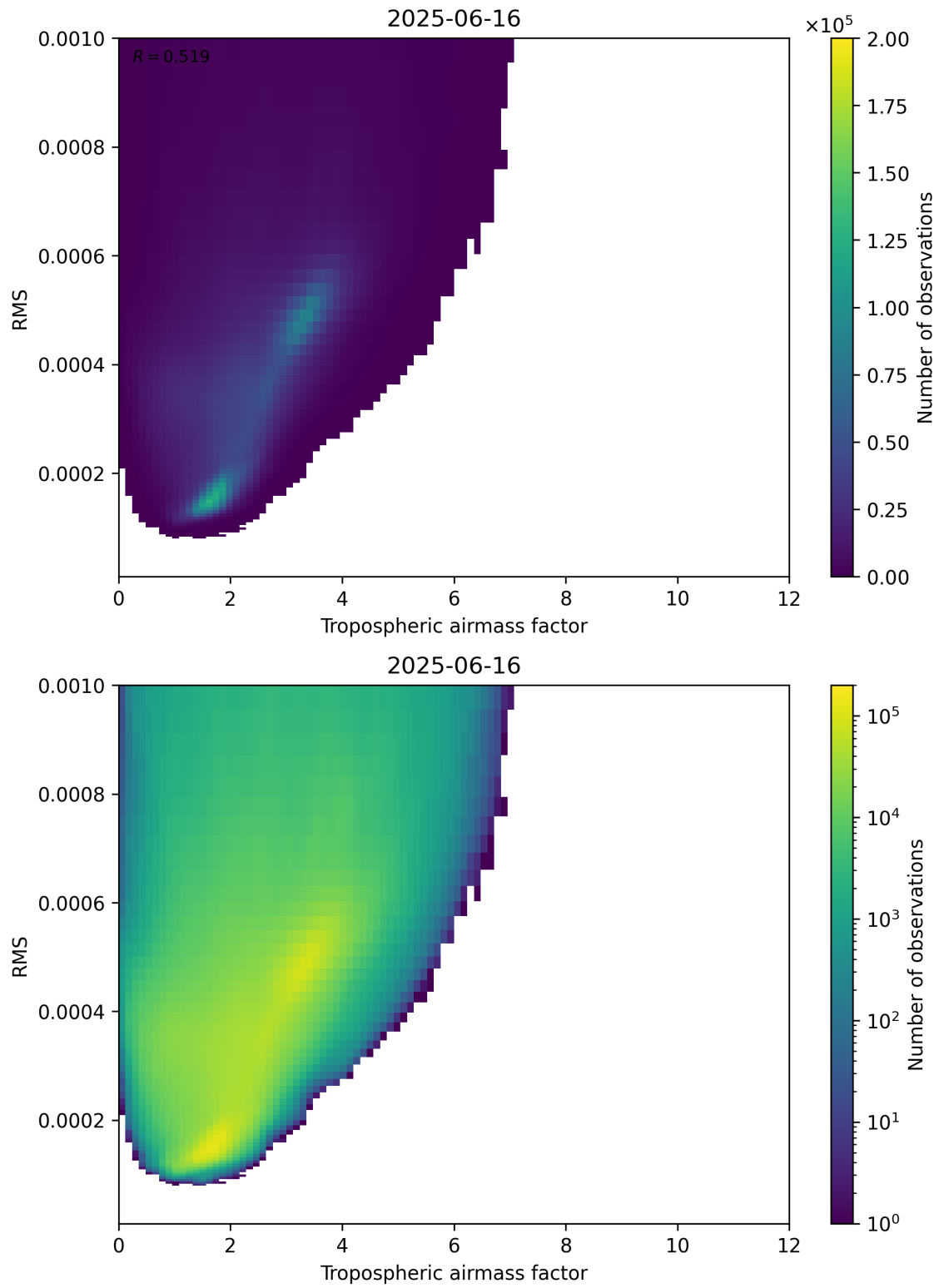
Figure 79: Scatter density plot of “Tropospheric airmass factor” against “RMS” for 2025-06-16 to 2025-06-17.
