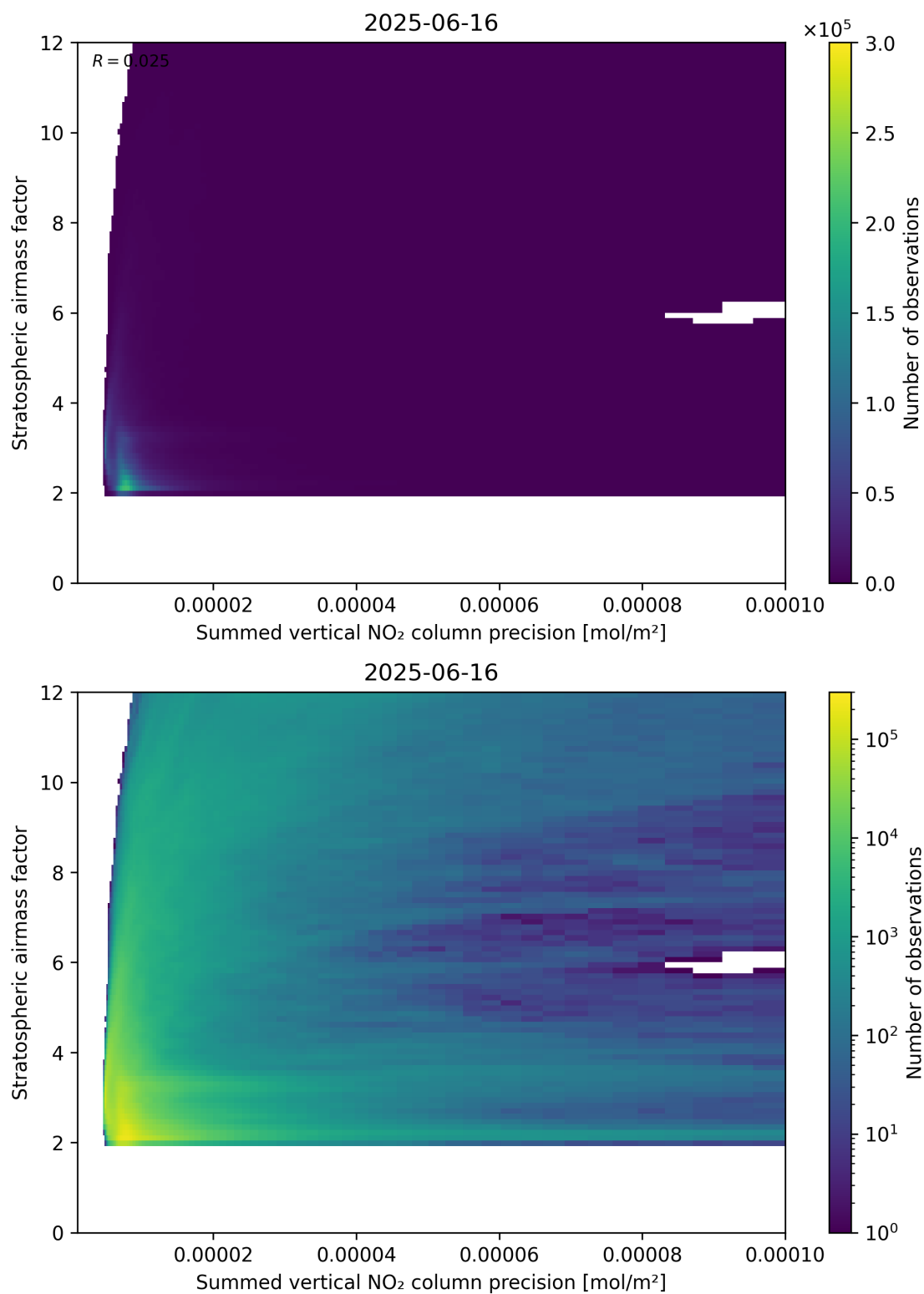
Figure 106: Scatter density plot of “Summed vertical NO 2 column precision” against “Stratospheric airmass factor” for 2025-06-16 to 2025-06-17.
