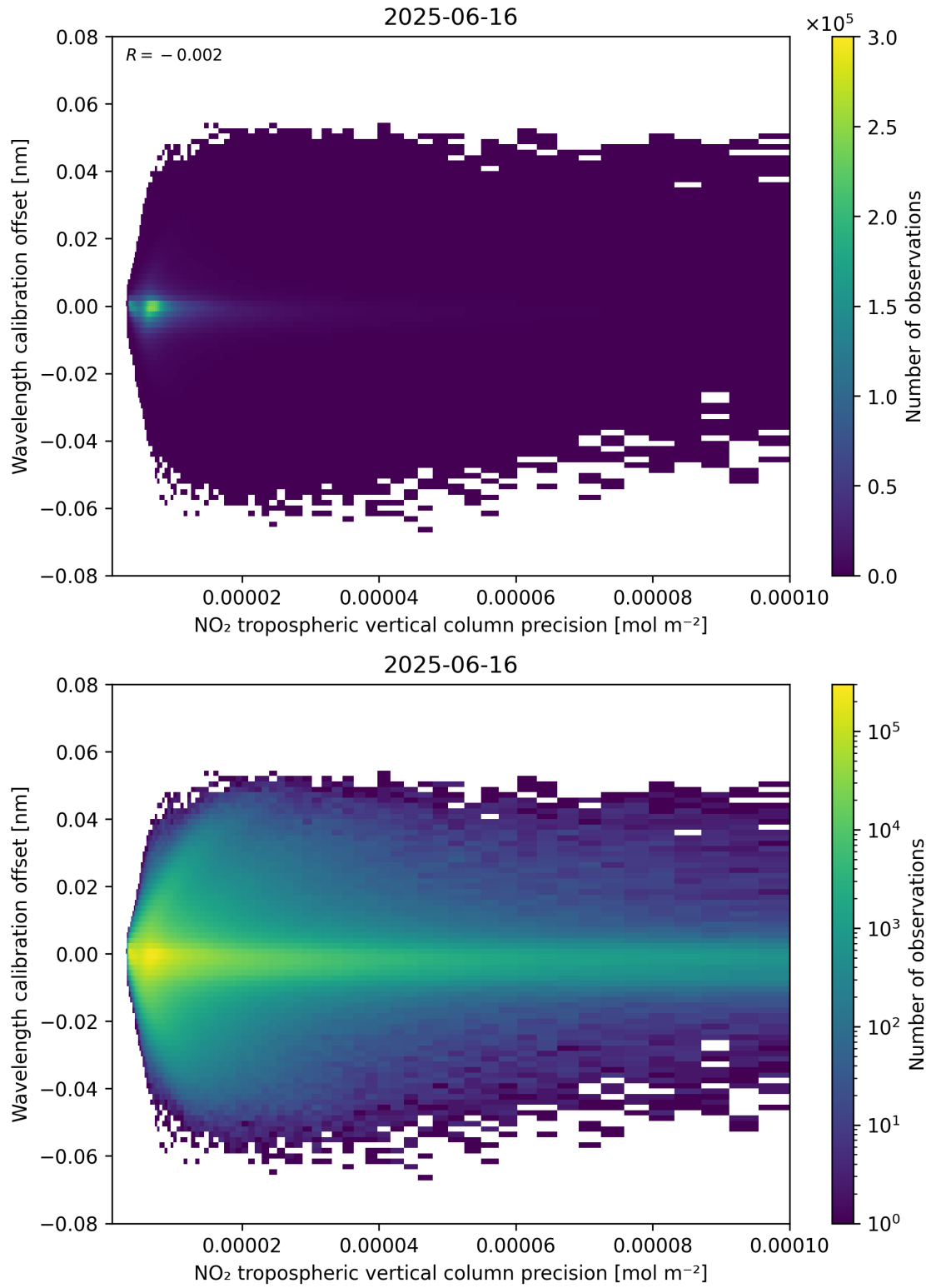
Figure 141: Scatter density plot of “NO 2 tropospheric vertical column precision” against “Wavelength calibration offset” for 2025-06-16 to 2025-06-17.
