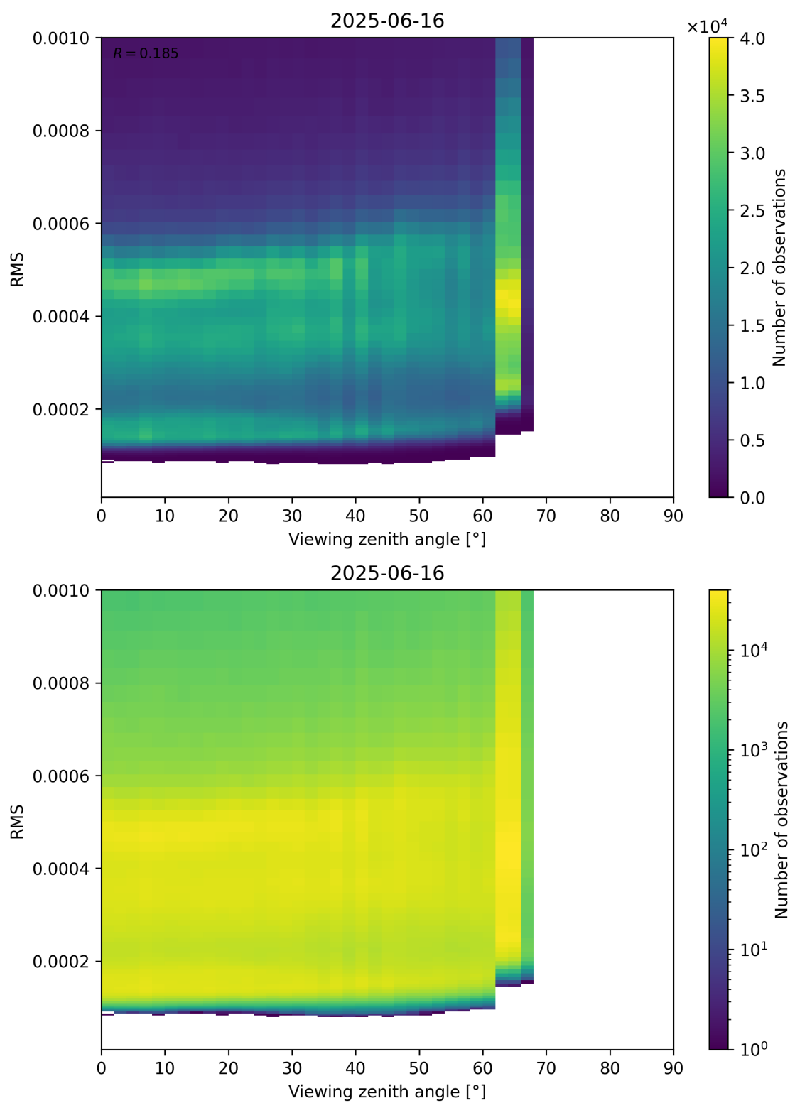
Figure 171: Scatter density plot of “Viewing zenith angle” against “RMS” for 2025-06-16 to 2025-06-17.
