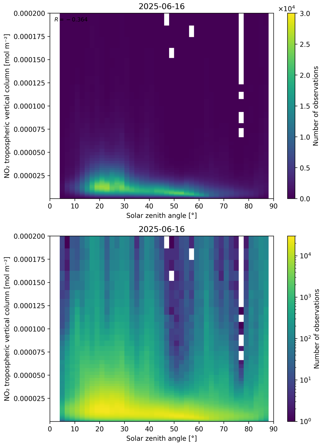
Figure 155: Scatter density plot of “Solar zenith angle” against “NO 2 tropospheric vertical column” for 2025-06-16 to 2025-06-17.
