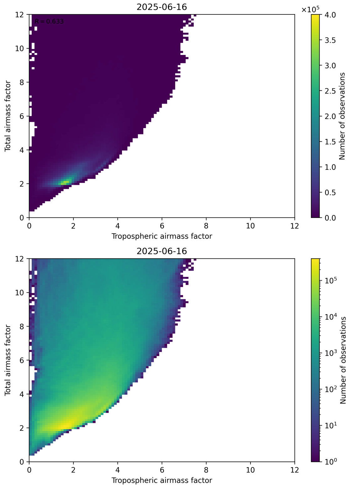
Figure 72: Scatter density plot of “Tropospheric airmass factor” against “Total airmass factor” for 2025-06-16 to 2025-06-17.
