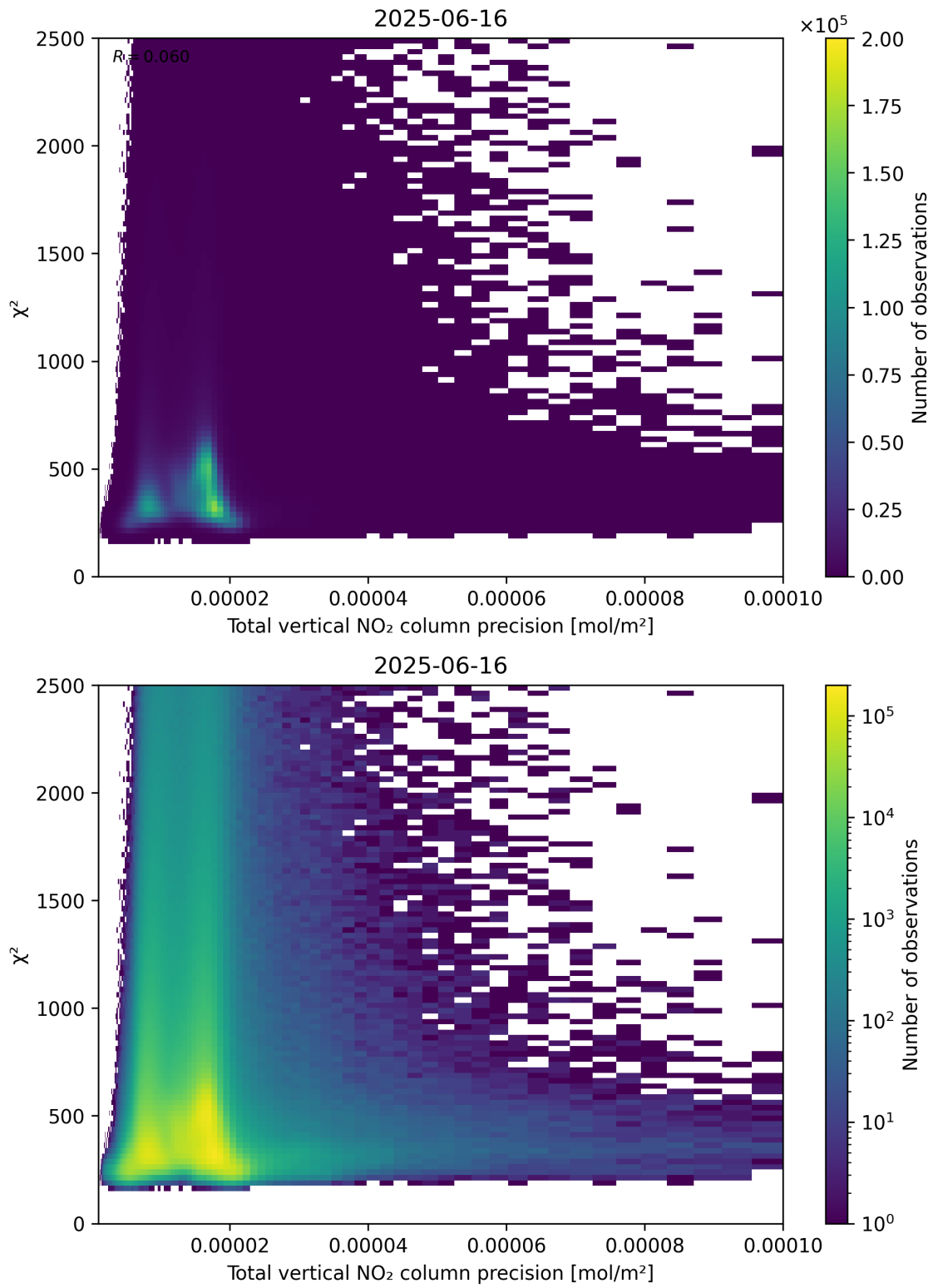
Figure 116: Scatter density plot of “Total vertical NO 2 column precision” against “ \chi^2 ” for 2025-06-16 to 2025-06-17.
