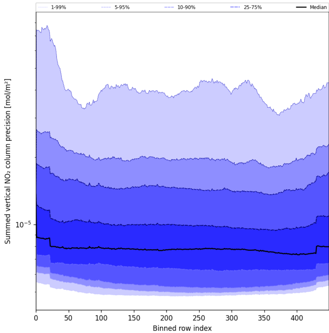
Figure 58: Along track statistics of “Summed vertical NO 2 column precision” for 2025-06-16 to 2025-06-17
