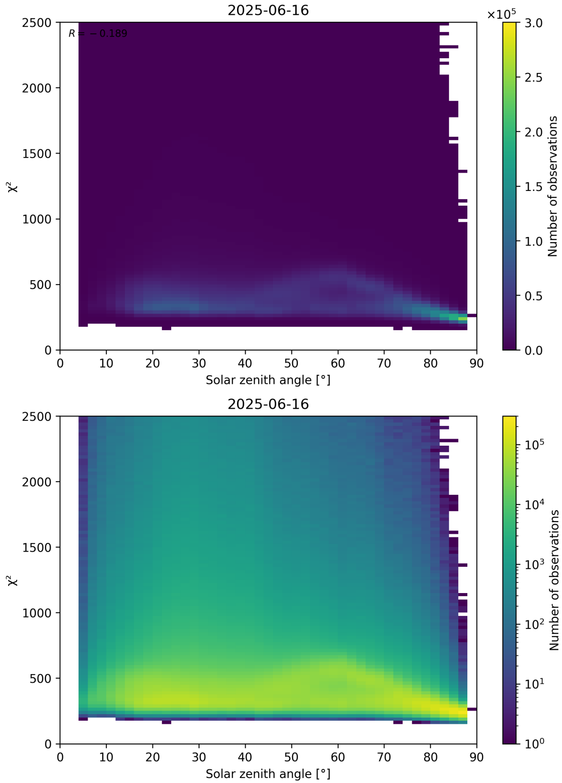
Figure 148: Scatter density plot of “Solar zenith angle” against “ \chi^2 ” for 2025-06-16 to 2025-06-17.
