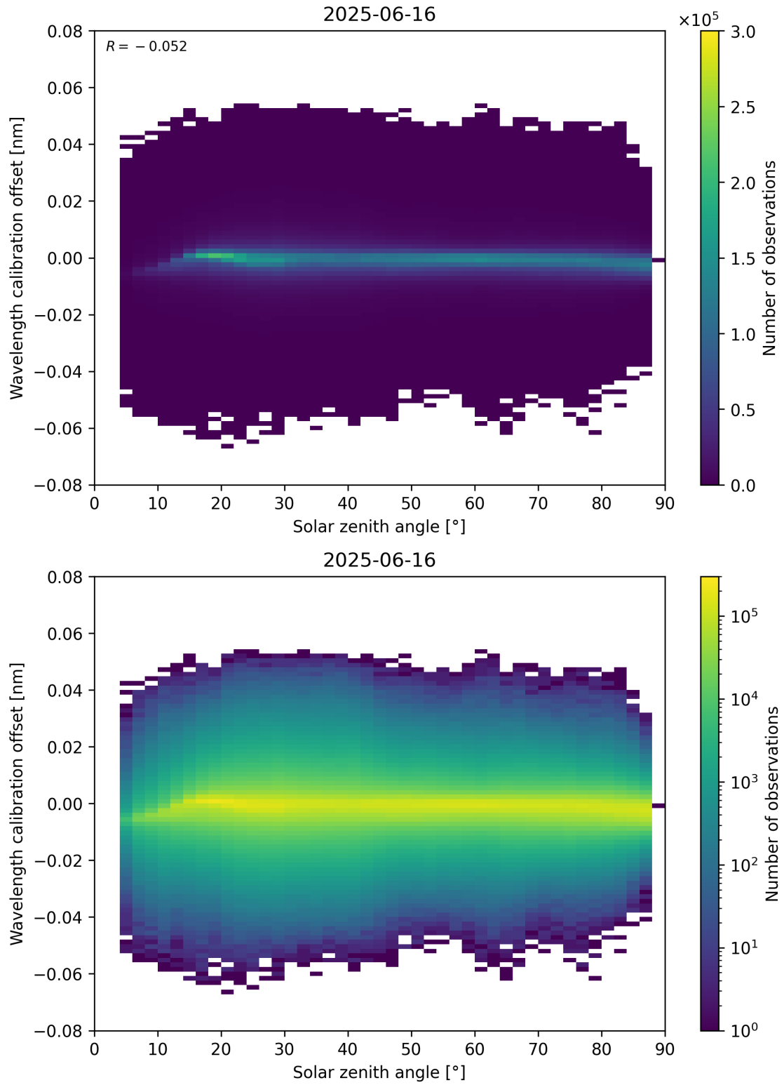
Figure 158: Scatter density plot of “Solar zenith angle” against “Wavelength calibration offset” for 2025-06-16 to 2025-06-17.
