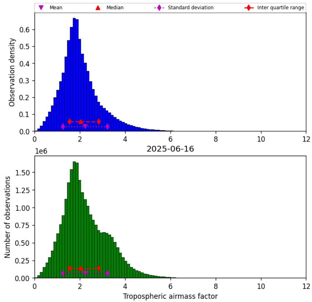
Figure 31: Histogram of “Tropospheric airmass factor” for 2025-06-16 to 2025-06-17
