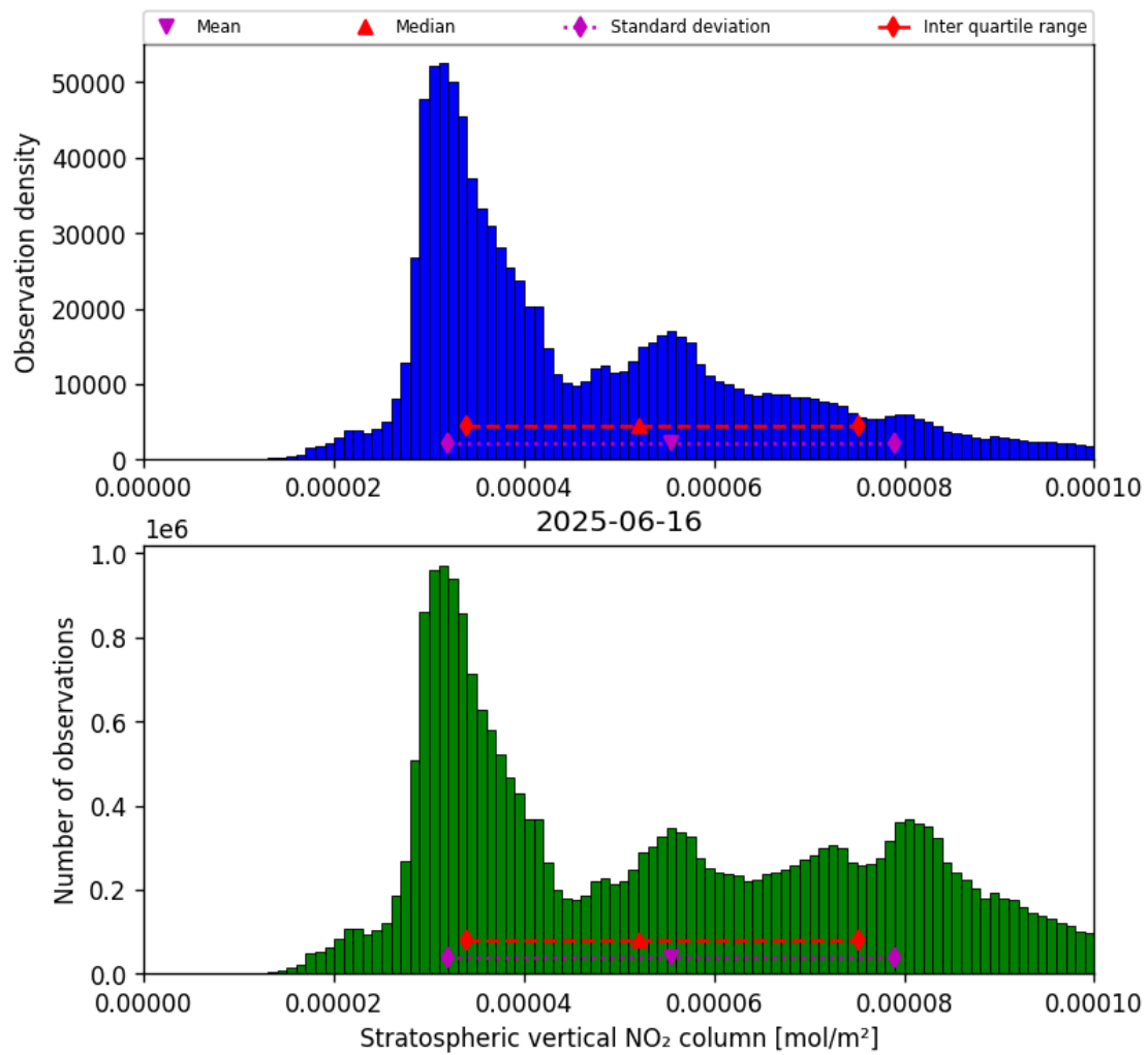
Figure 36: Histogram of “Stratospheric vertical NO 2 column” for 2025-06-16 to 2025-06-17
