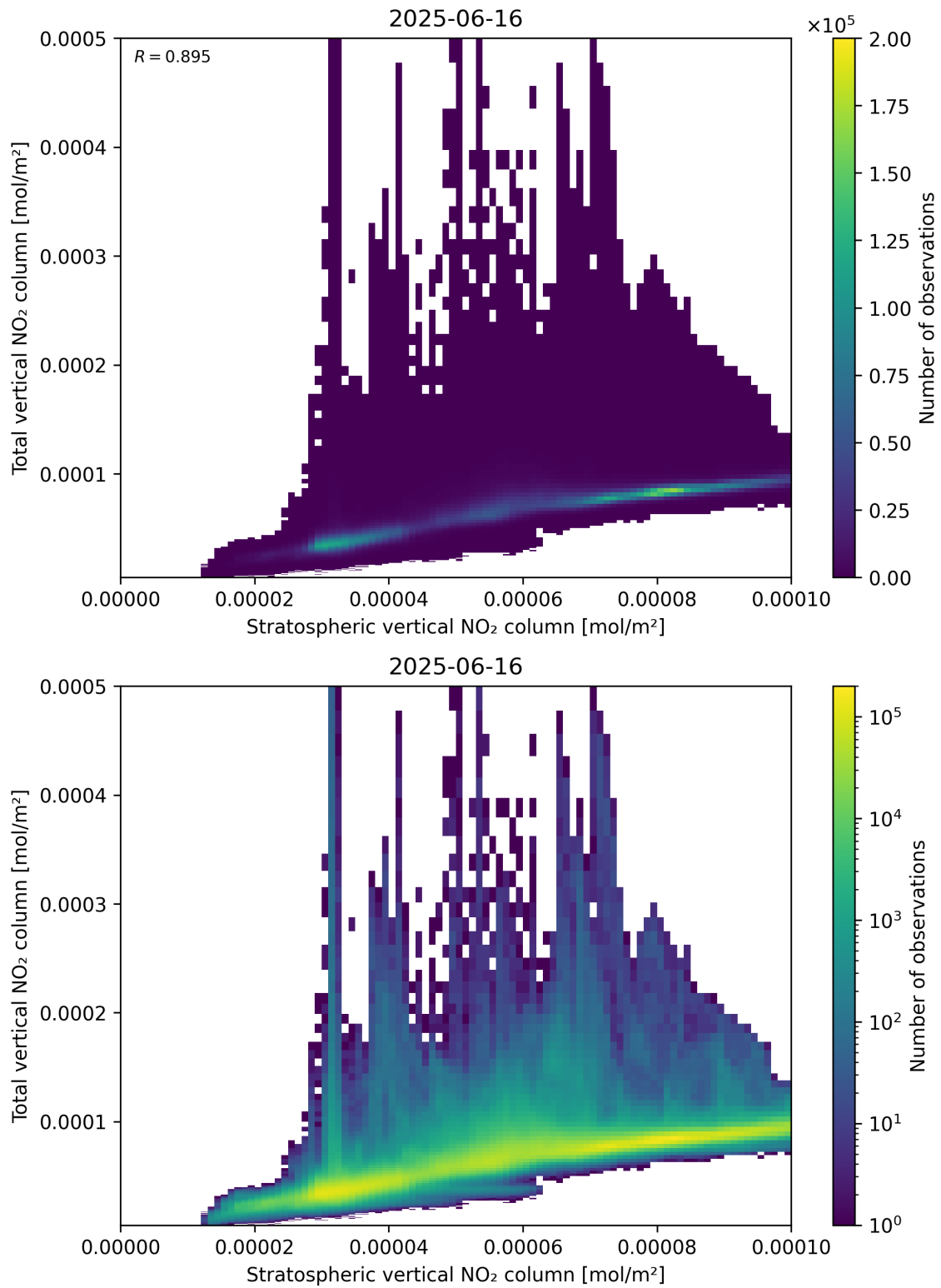
Figure 100: Scatter density plot of “Stratospheric vertical NO 2 column” against “Total vertical NO 2 column” for 2025-06-16 to 2025-06-17.
