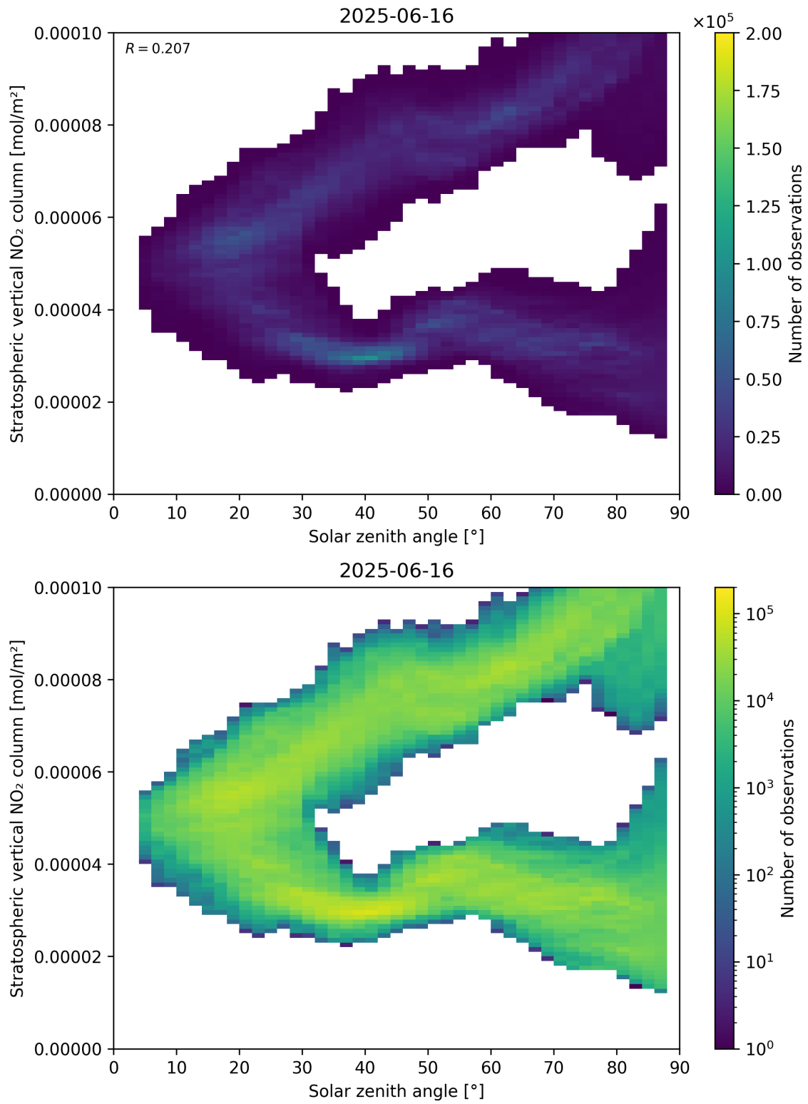
Figure 150: Scatter density plot of “Solar zenith angle” against “Stratospheric vertical NO 2 column” for 2025-06-16 to 2025-06-17.
