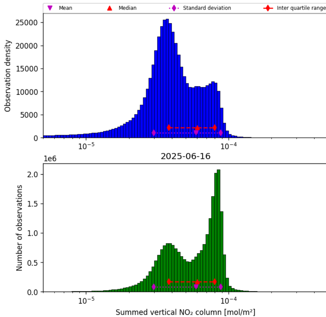
Figure 40: Histogram of “Summed vertical NO 2 column” for 2025-06-16 to 2025-06-17
