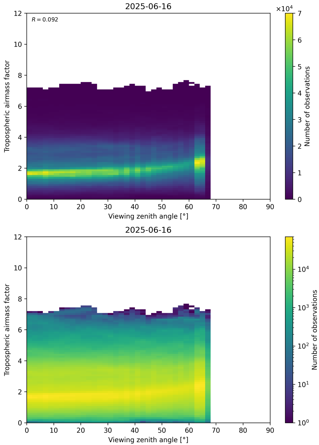
Figure 161: Scatter density plot of “Viewing zenith angle” against “Tropospheric airmass factor” for 2025-06-16 to 2025-06-17.
