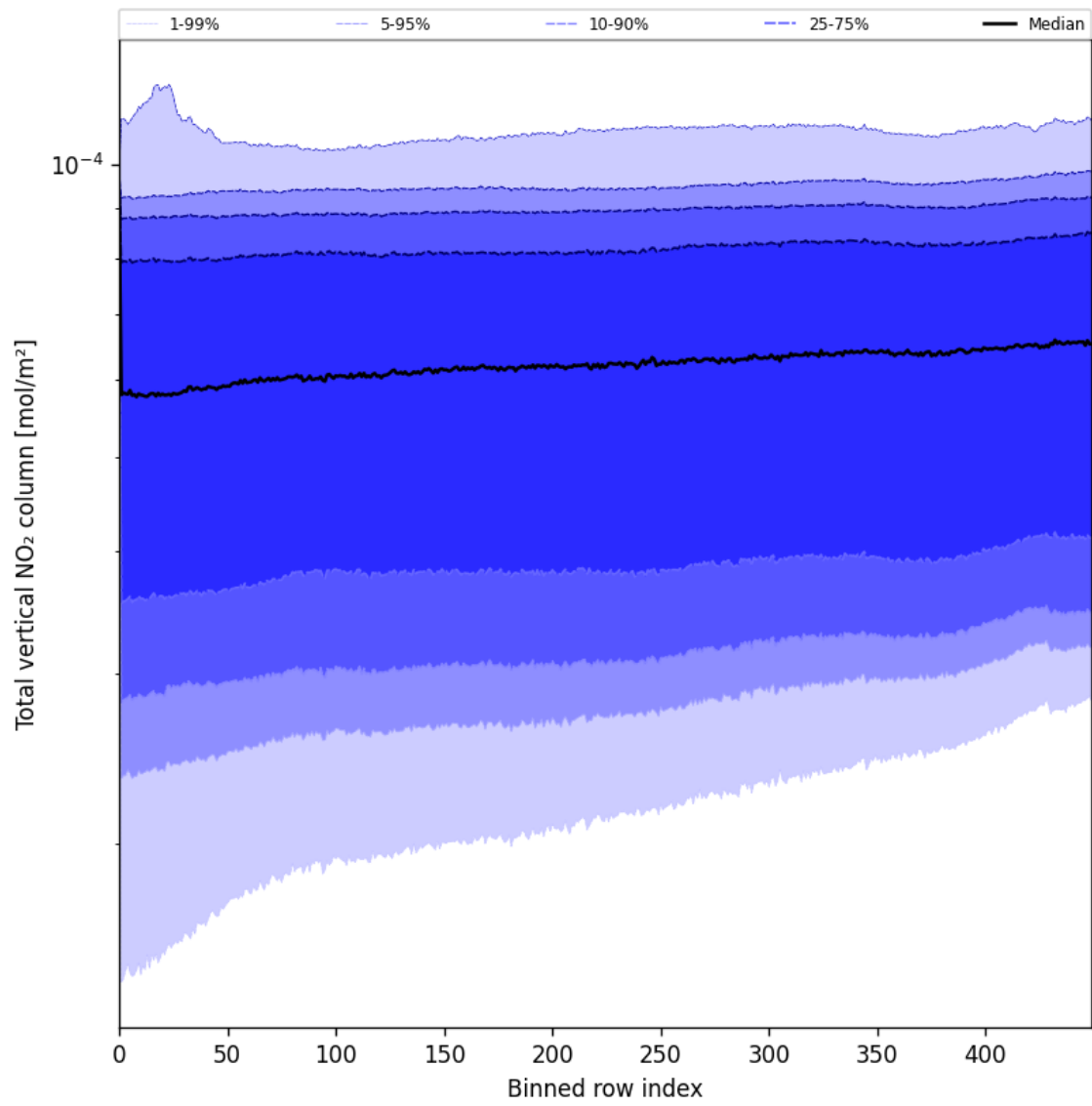
Figure 55: Along track statistics of “Total vertical NO 2 column” for 2025-06-16 to 2025-06-17
