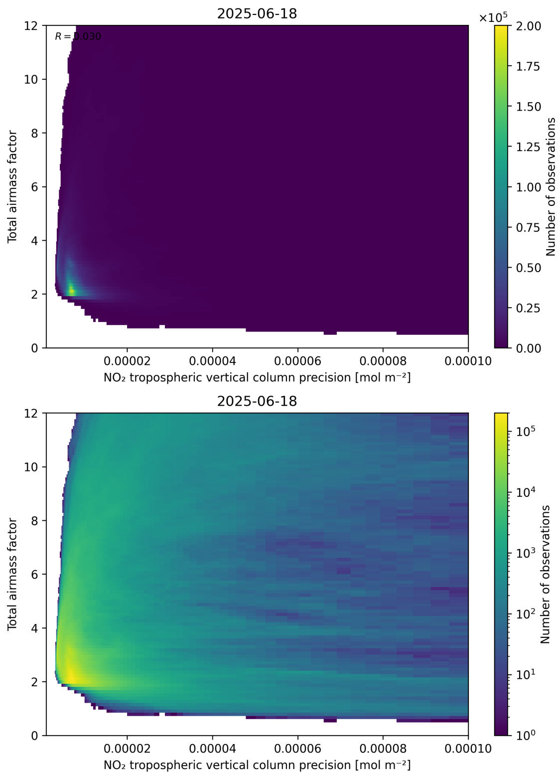
Figure 132: Scatter density plot of “NO 2 tropospheric vertical column precision” against “Total air mass factor” for 2025-06-17 to 2025-06-19.
