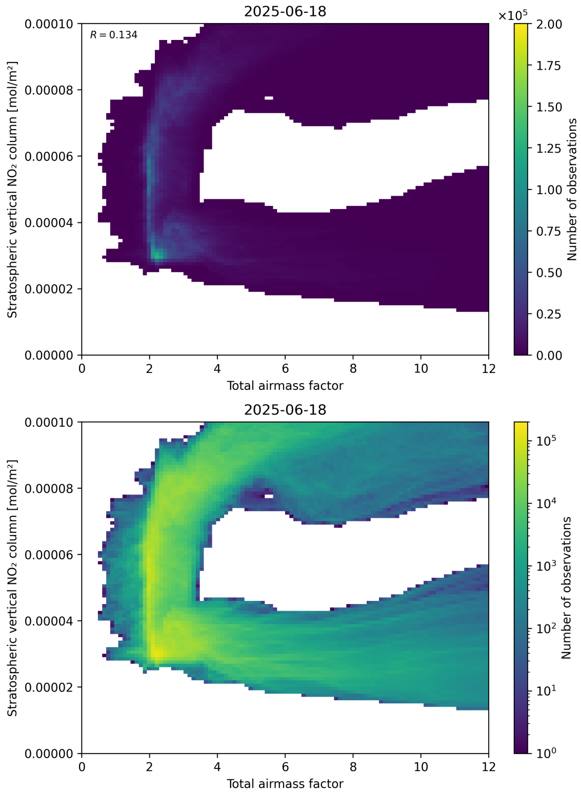
Figure 64: Scatter density plot of “Total airmass factor” against “Stratospheric vertical NO 2 column” for 2025-06-17 to 2025-06-19.
