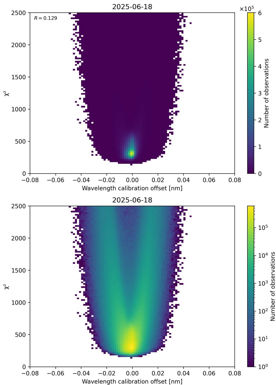
Figure 175: Scatter density plot of “Wavelength calibration offset” against “ \chi^2 ” for 2025-06-17 to 2025-06-19.
