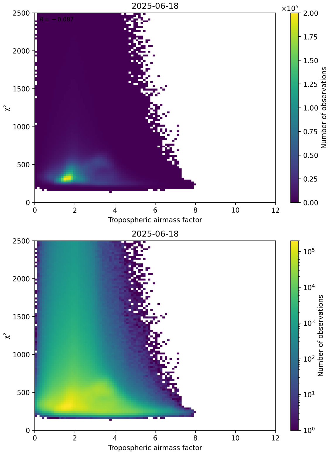
Figure 73: Scatter density plot of “Tropospheric airmass factor” against “ \chi^2 ” for 2025-06-17 to 2025-06-19.
