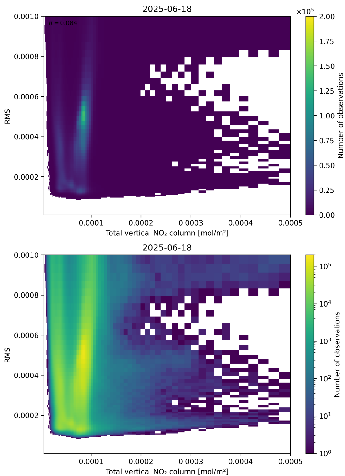
Figure 120: Scatter density plot of “Total vertical NO 2 column” against “RMS” for 2025-06-17 to 2025-06-19.
