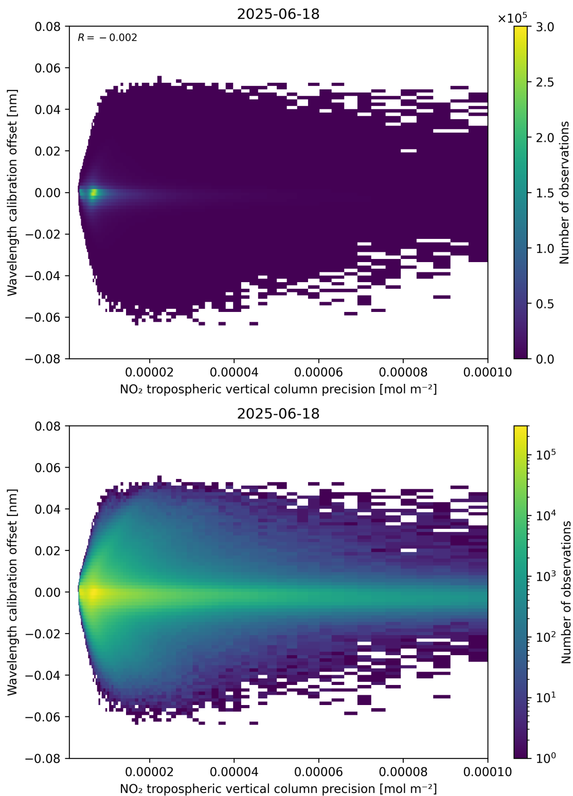
Figure 141: Scatter density plot of “NO 2 tropospheric vertical column precision” against “Wavelength calibration offset” for 2025-06-17 to 2025-06-19.
