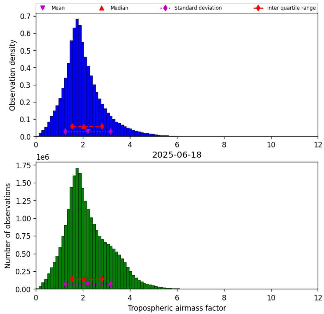
Figure 31: Histogram of “Tropospheric airmass factor” for 2025-06-17 to 2025-06-19
