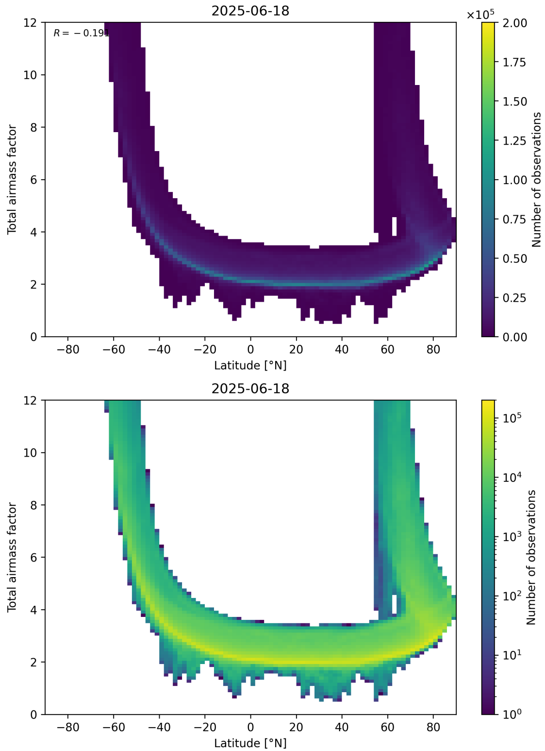
Figure 84: Scatter density plot of “Latitude” against “Total airmass factor” for 2025-06-17 to 2025-06-19.
