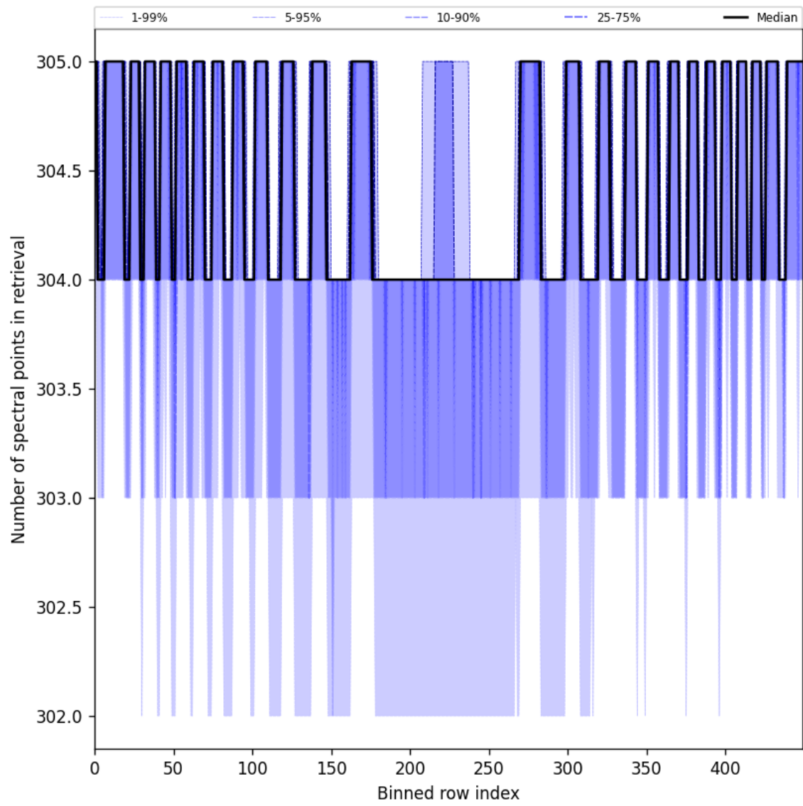
Figure 50: Along track statistics of “Number of spectral points in retrieval” for 2025-06-17 to 2025-06-19
