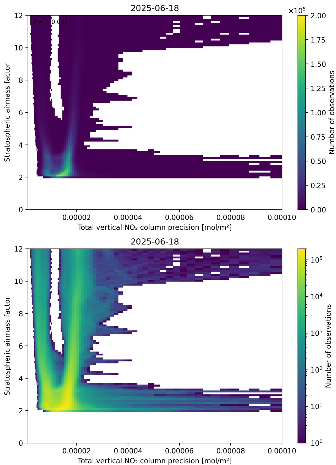
Figure 115: Scatter density plot of “Total vertical NO 2 column precision” against “Stratospheric air mass factor” for 2025-06-17 to 2025-06-19.
