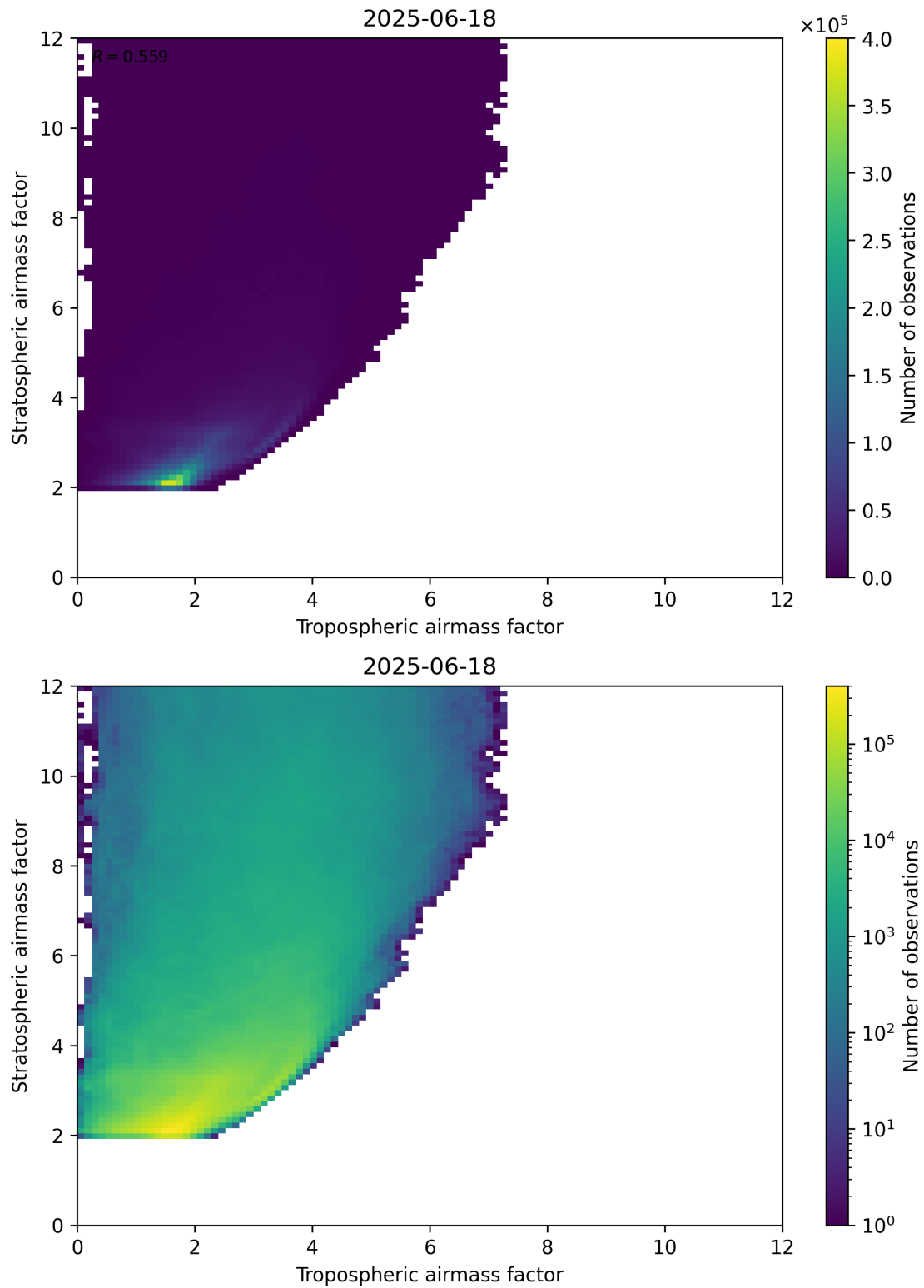
Figure 71: Scatter density plot of “Tropospheric airmass factor” against “Stratospheric airmass factor” for 2025-06-17 to 2025-06-19.
