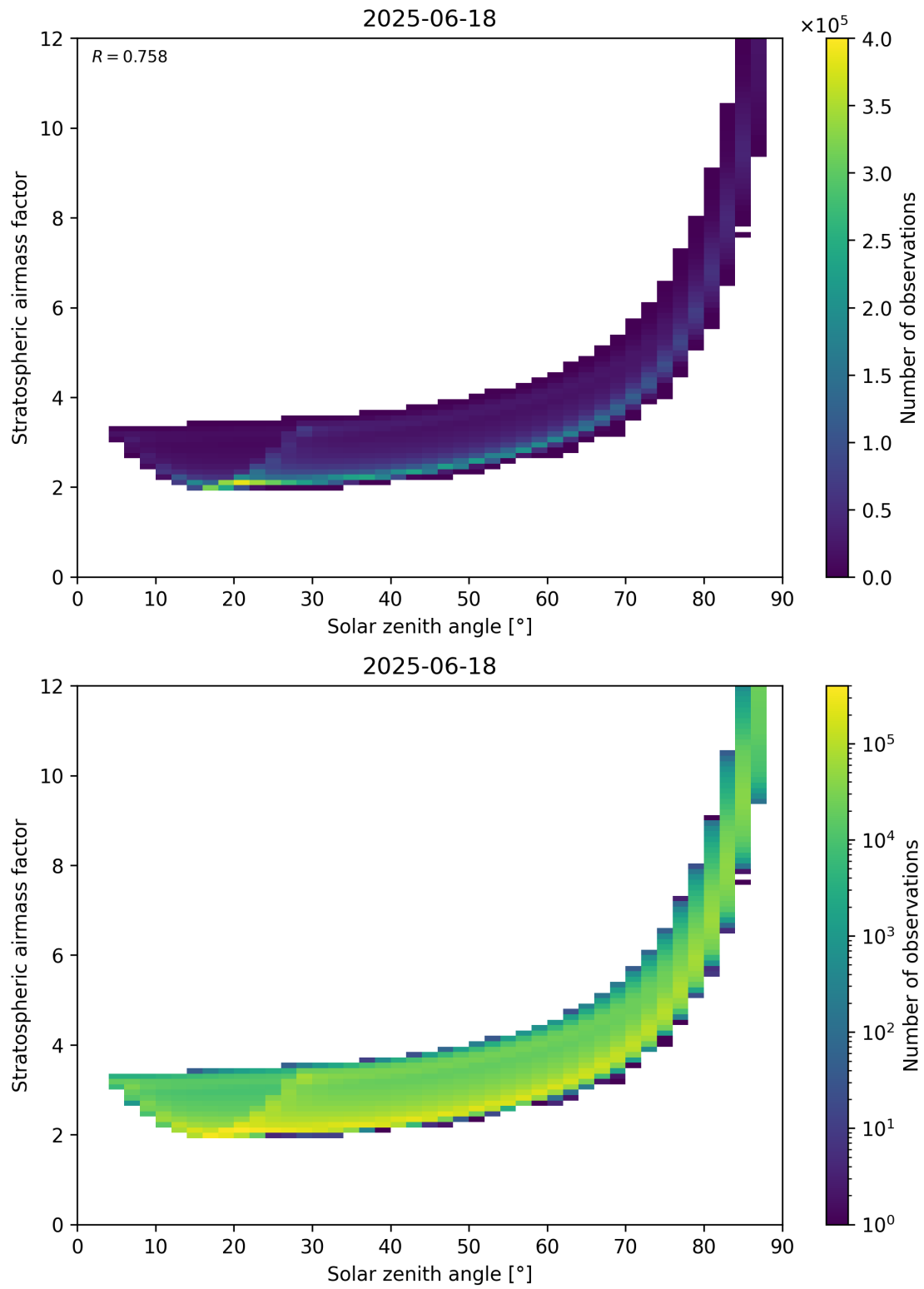
Figure 145: Scatter density plot of “Solar zenith angle” against “Stratospheric airmass factor” for 2025-06-17 to 2025-06-19.
