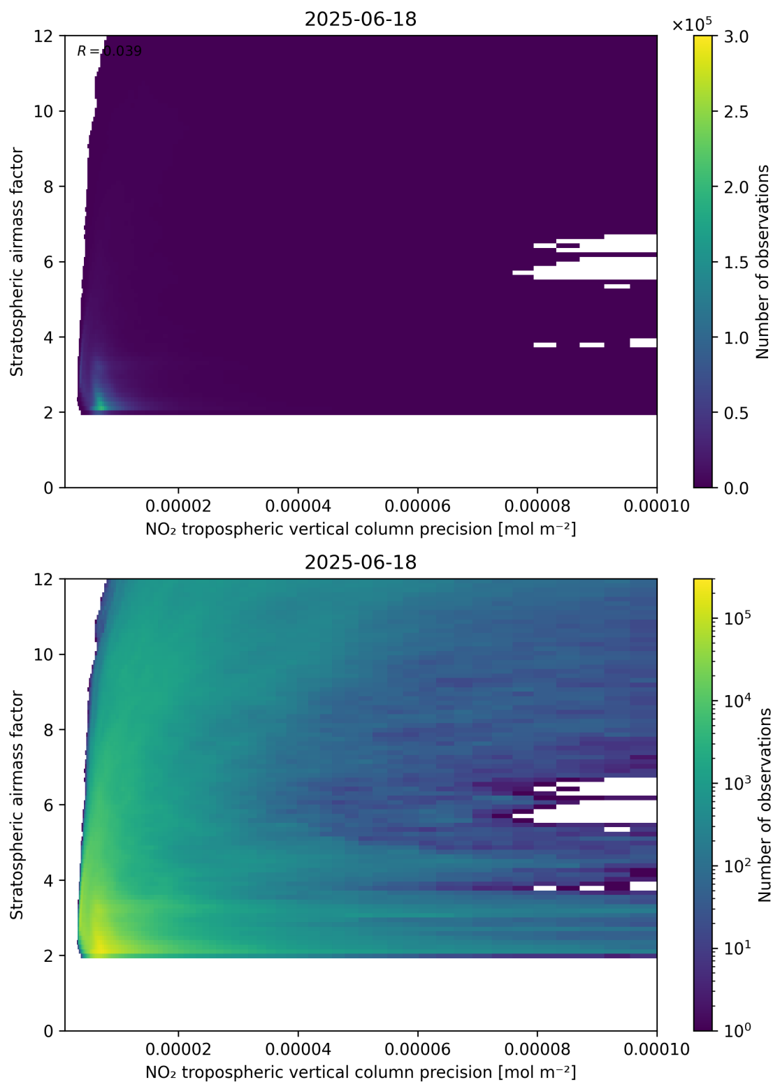
Figure 131: Scatter density plot of “NO 2 tropospheric vertical column precision” against “Stratospheric airmass factor” for 2025-06-17 to 2025-06-19.
