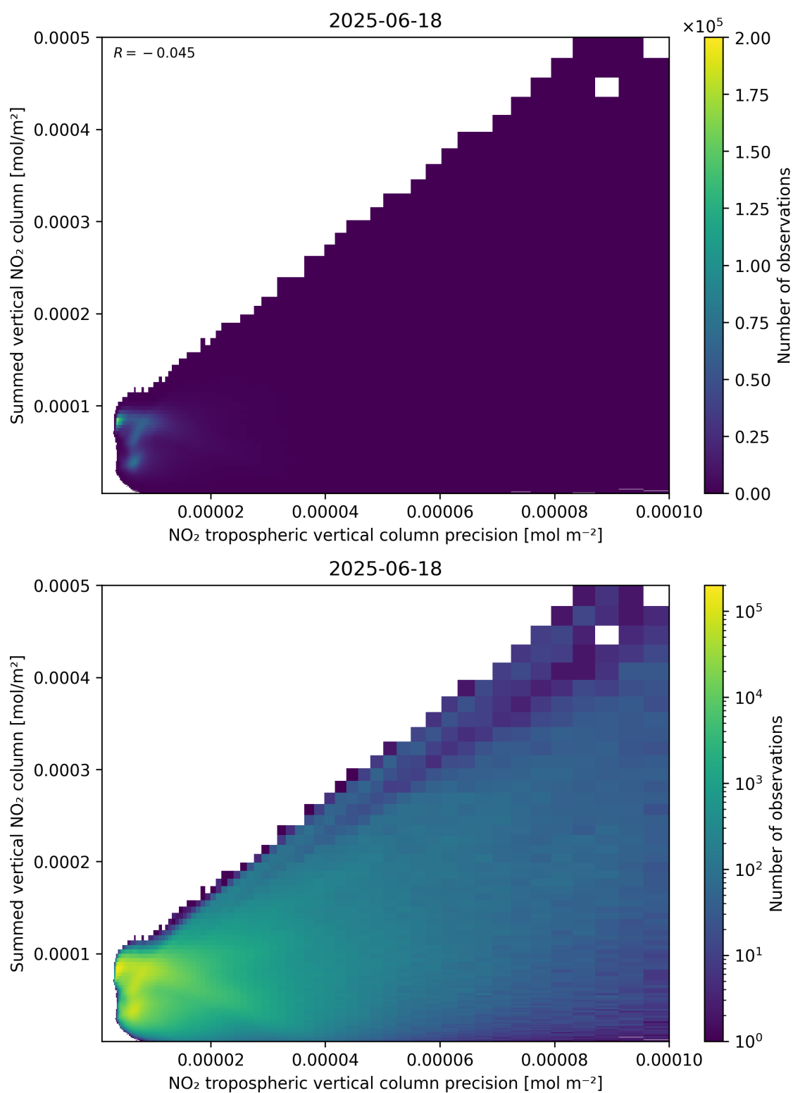
Figure 136: Scatter density plot of “NO 2 tropospheric vertical column precision” against “Summed vertical NO 2 column” for 2025-06-17 to 2025-06-19.
