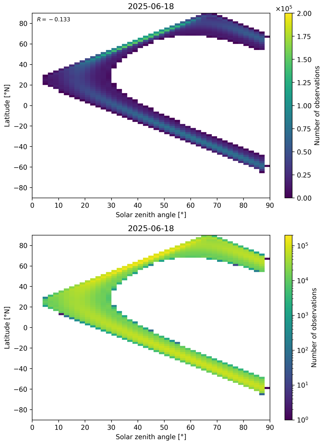
Figure 149: Scatter density plot of “Solar zenith angle” against “Latitude” for 2025-06-17 to 2025-06-19.
