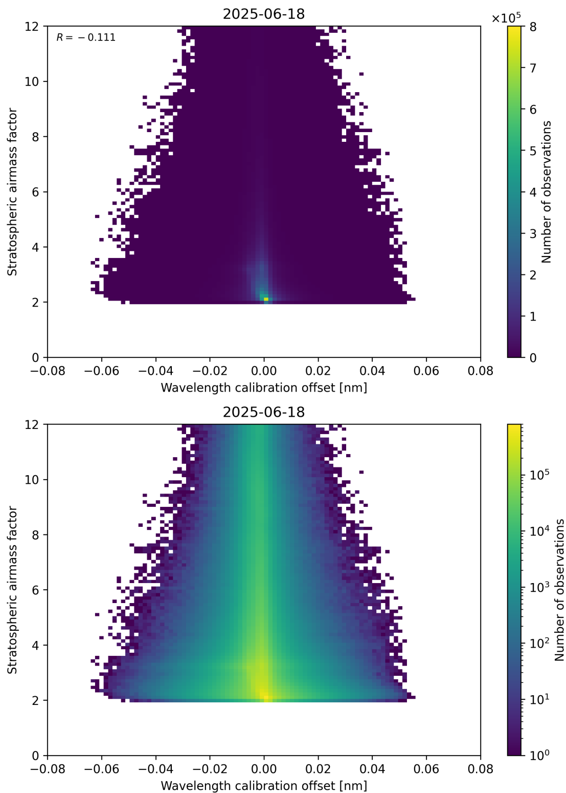
Figure 174: Scatter density plot of “Wavelength calibration offset” against “Stratospheric air mass factor” for 2025-06-17 to 2025-06-19.
