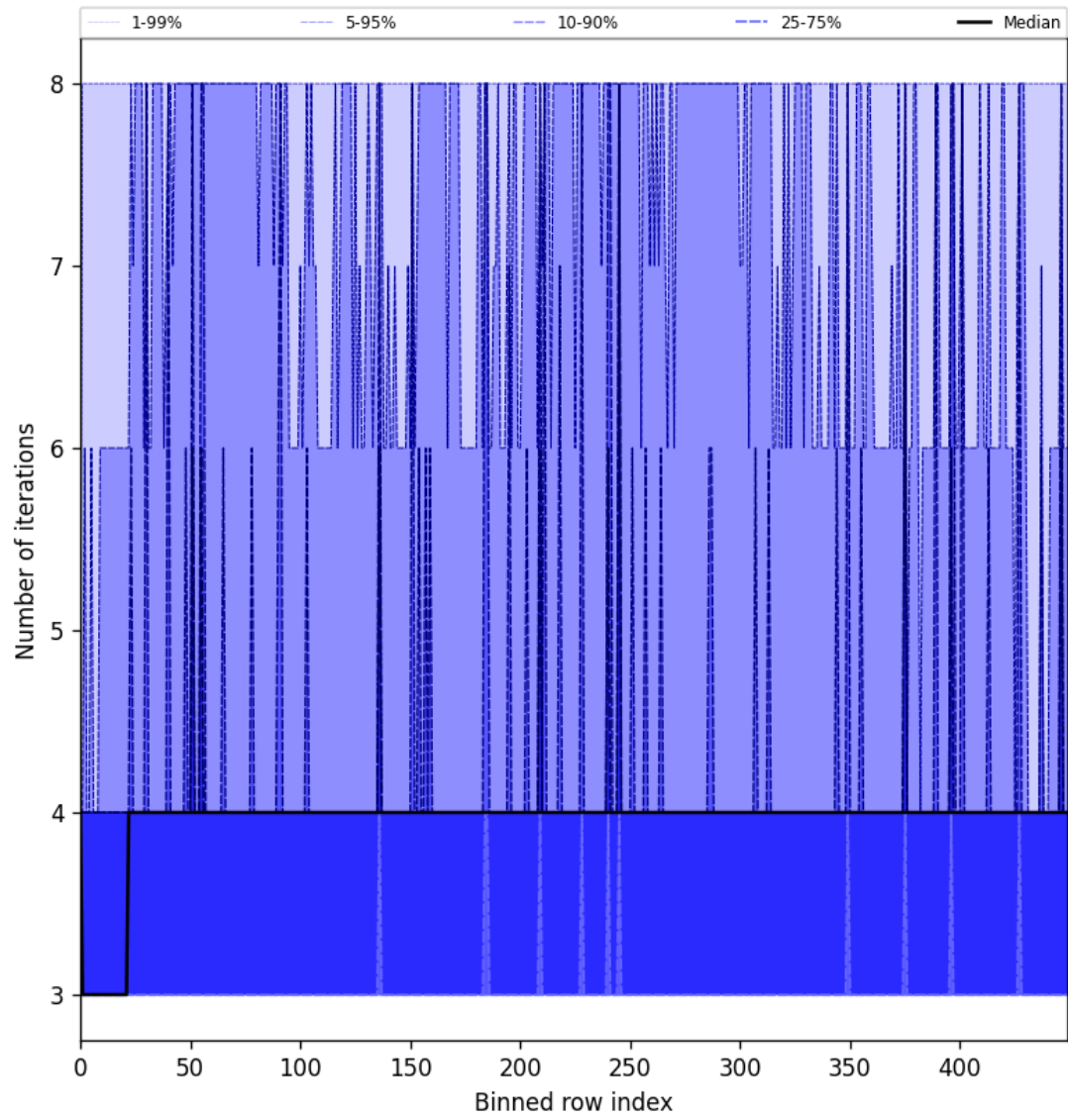
Figure 51: Along track statistics of “Number of iterations” for 2025-06-17 to 2025-06-19
