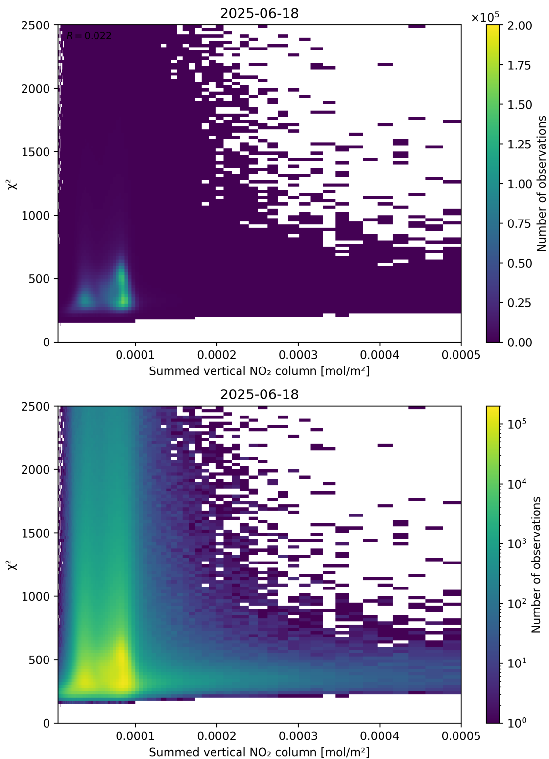
Figure 104: Scatter density plot of “Summed vertical NO 2 column” against “ \chi^2 ” for 2025-06-17 to 2025-06-19.
