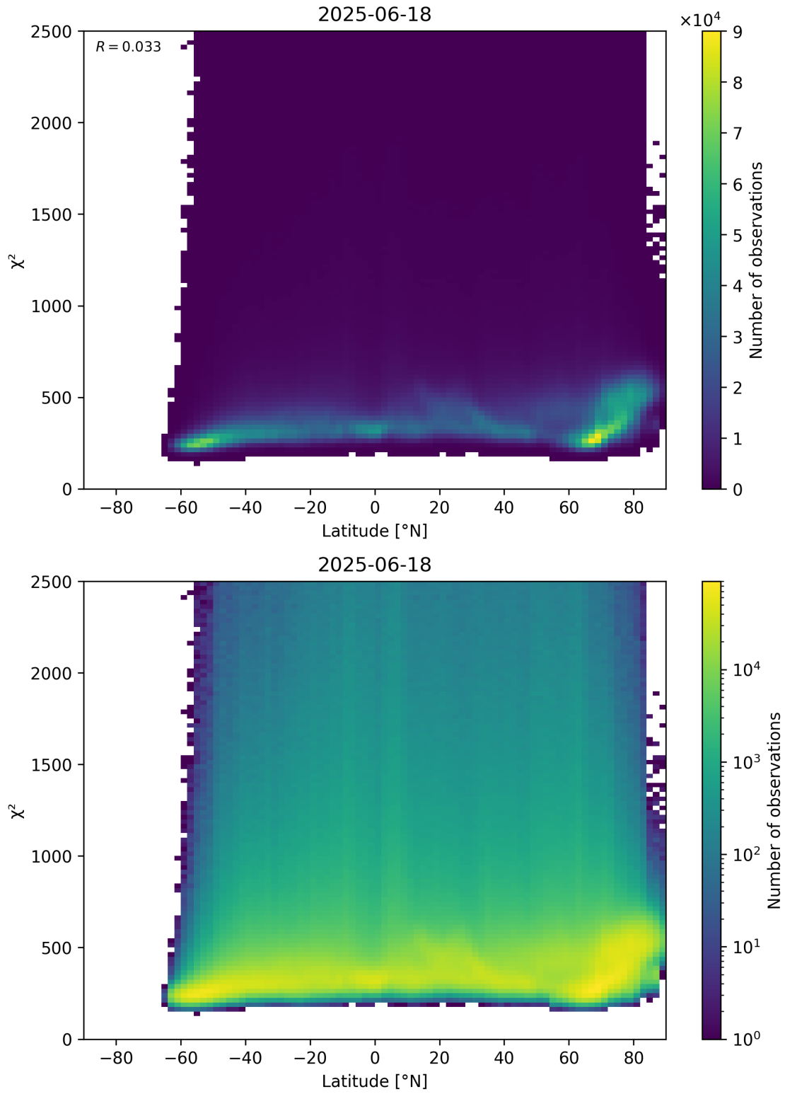
Figure 86: Scatter density plot of “Latitude” against “ \chi^2 ” for 2025-06-17 to 2025-06-19.
