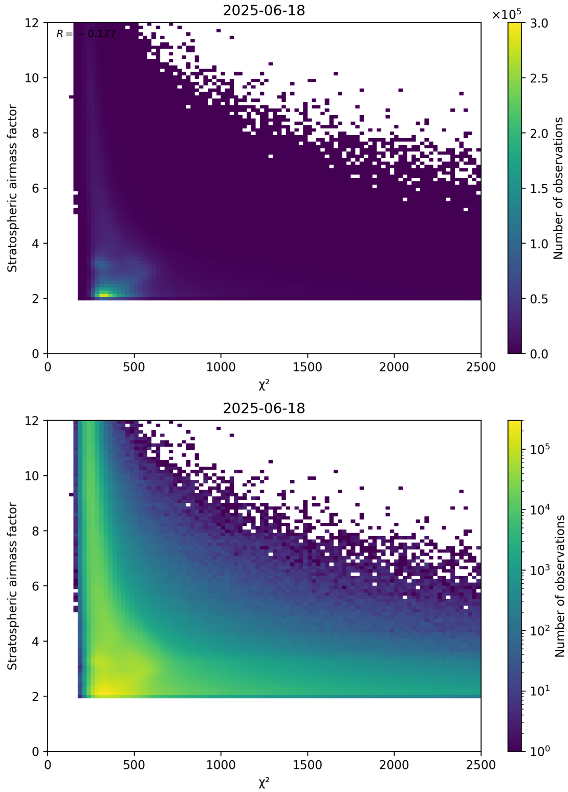
Figure 81: Scatter density plot of “ \chi^2 ” against “Stratospheric airmass factor” for 2025-06-17 to 2025-06-19.
