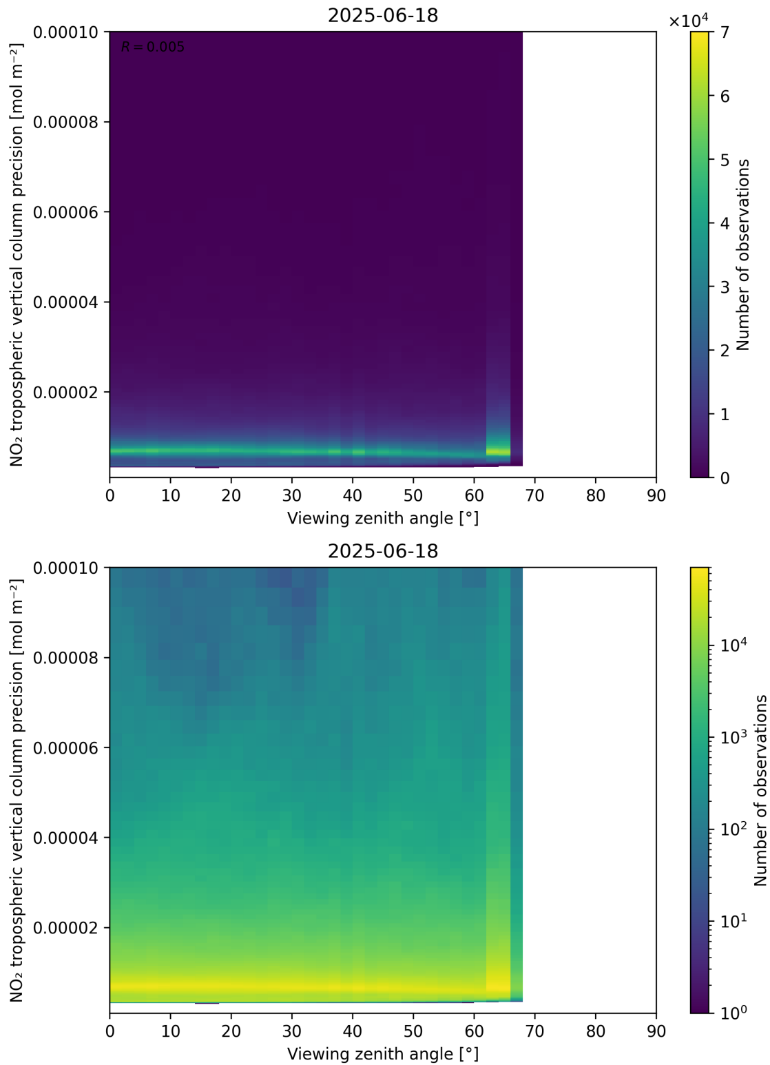
Figure 170: Scatter density plot of “Viewing zenith angle” against “NO 2 tropospheric vertical column precision” for 2025-06-17 to 2025-06-19.
