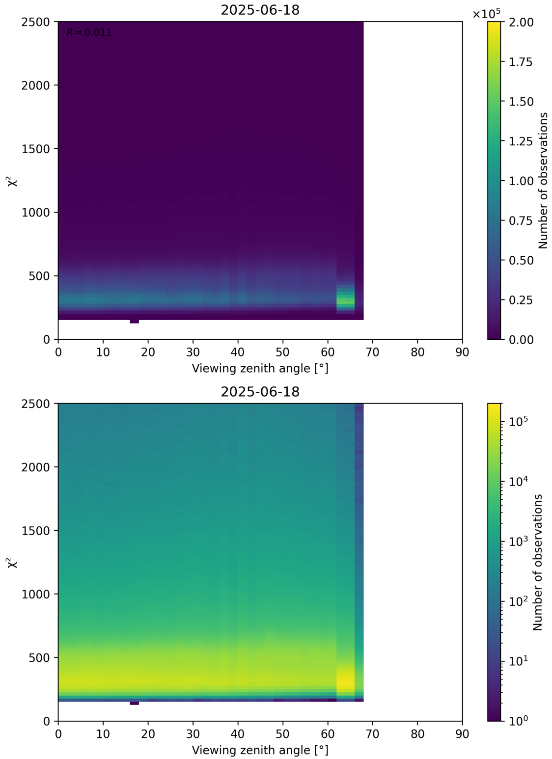
Figure 162: Scatter density plot of “Viewing zenith angle” against “ \chi^2 ” for 2025-06-17 to 2025-06-19.
