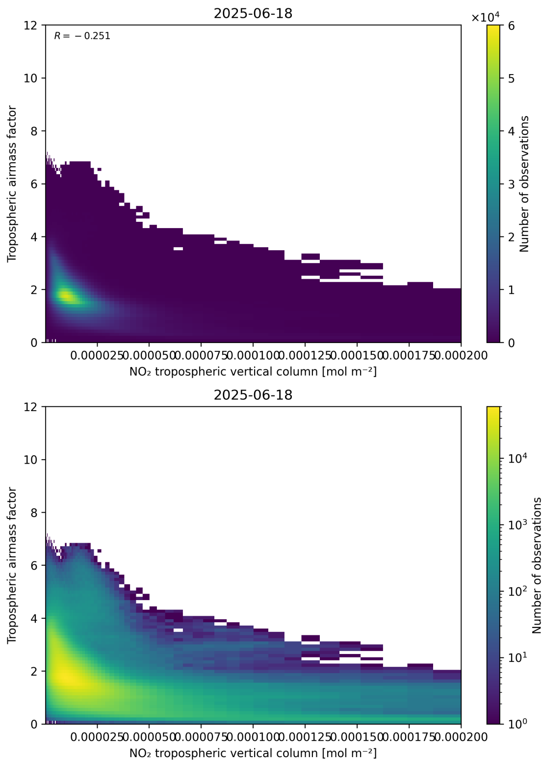
Figure 123: Scatter density plot of “NO 2 tropospheric vertical column” against “Tropospheric air mass factor” for 2025-06-17 to 2025-06-19.
