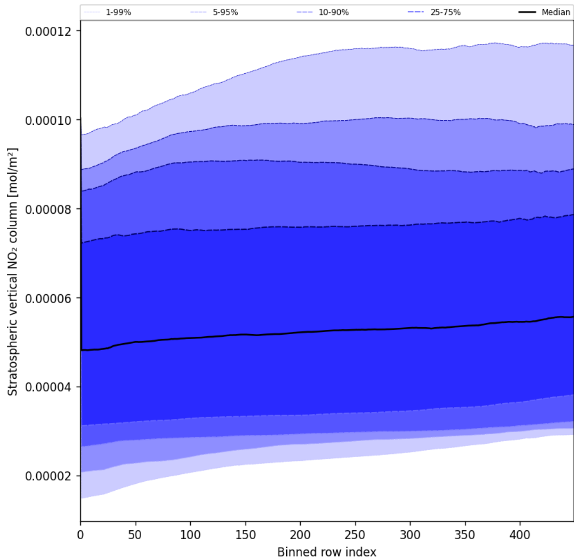
Figure 53: Along track statistics of “Stratospheric vertical NO 2 column” for 2025-06-17 to 2025-06-19
