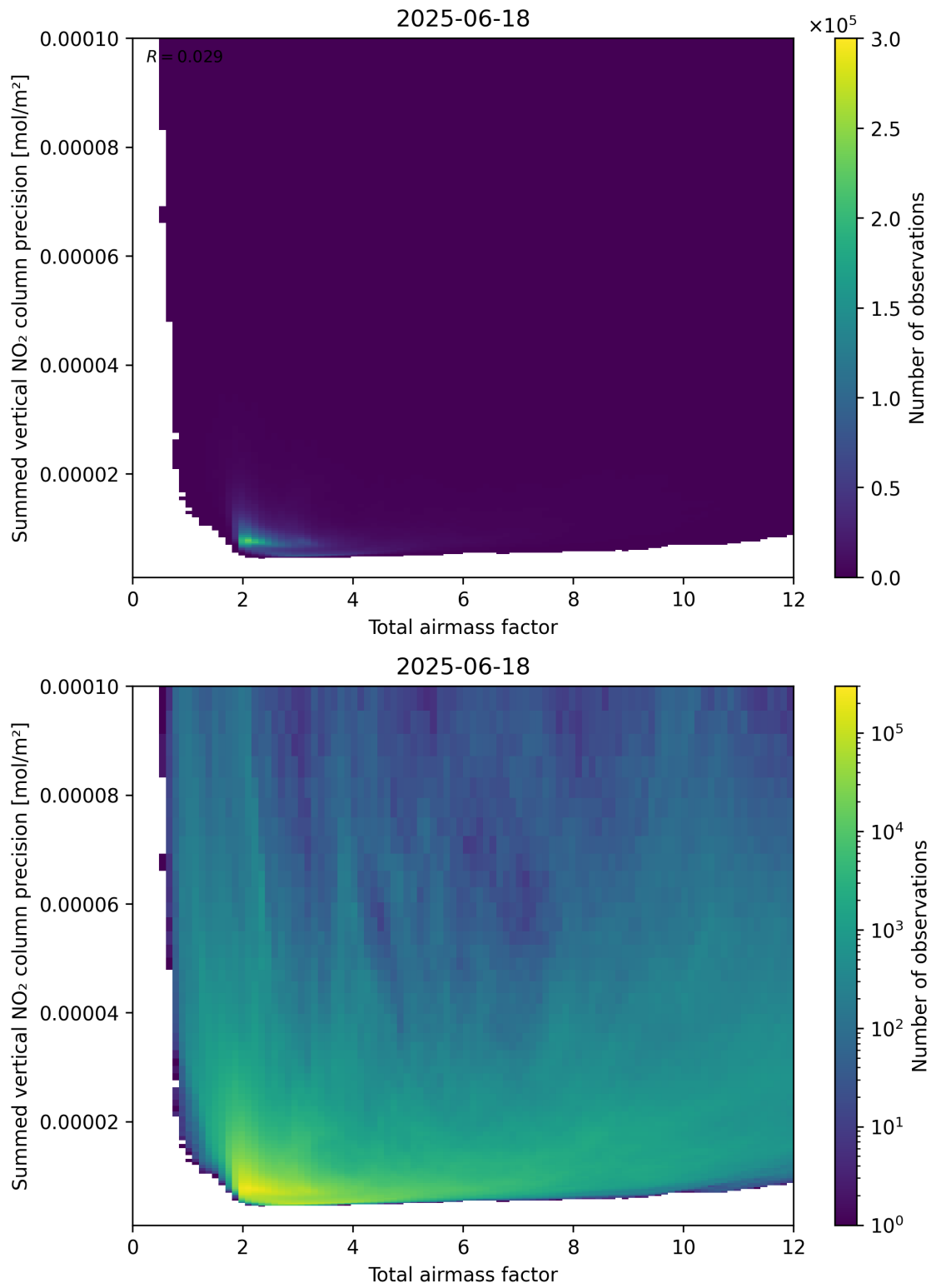
Figure 66: Scatter density plot of “Total airmass factor” against “Summed vertical NO 2 column precision” for 2025-06-17 to 2025-06-19.
