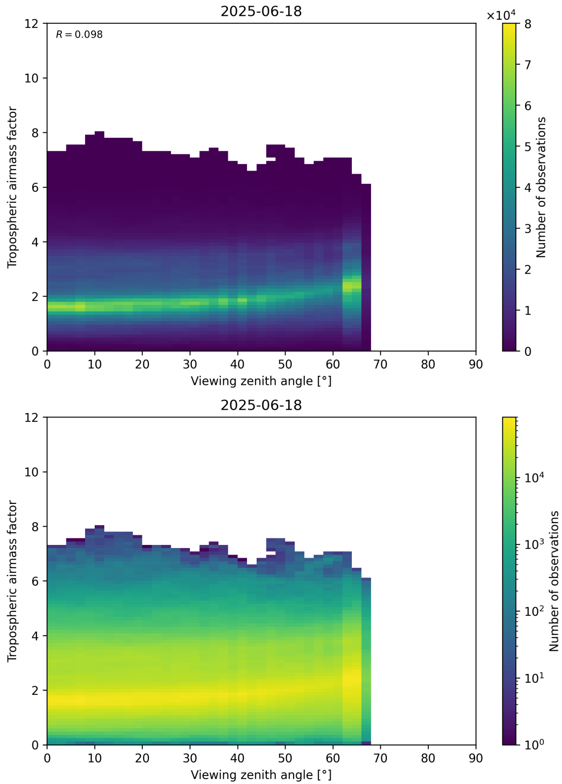
Figure 161: Scatter density plot of “Viewing zenith angle” against “Tropospheric airmass factor” for 2025-06-17 to 2025-06-19.
