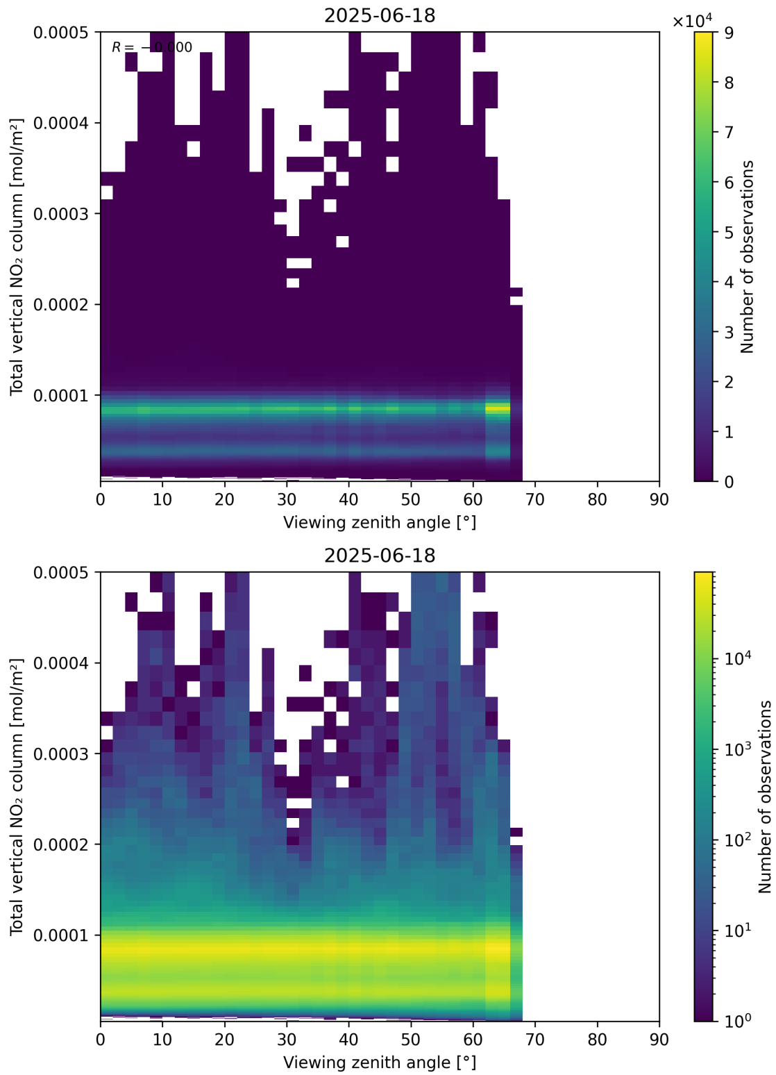
Figure 167: Scatter density plot of “Viewing zenith angle” against “Total vertical NO 2 column” for 2025-06-17 to 2025-06-19.
