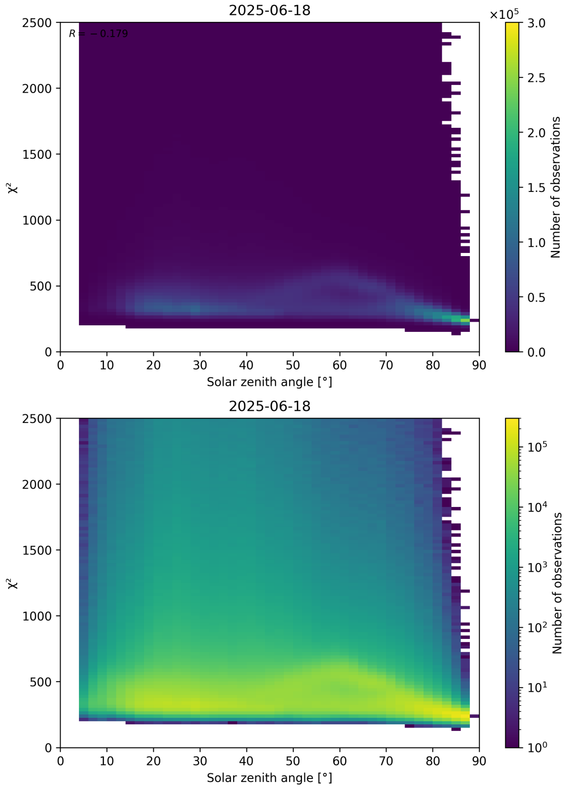
Figure 148: Scatter density plot of “Solar zenith angle” against “ \chi^2 ” for 2025-06-17 to 2025-06-19.
