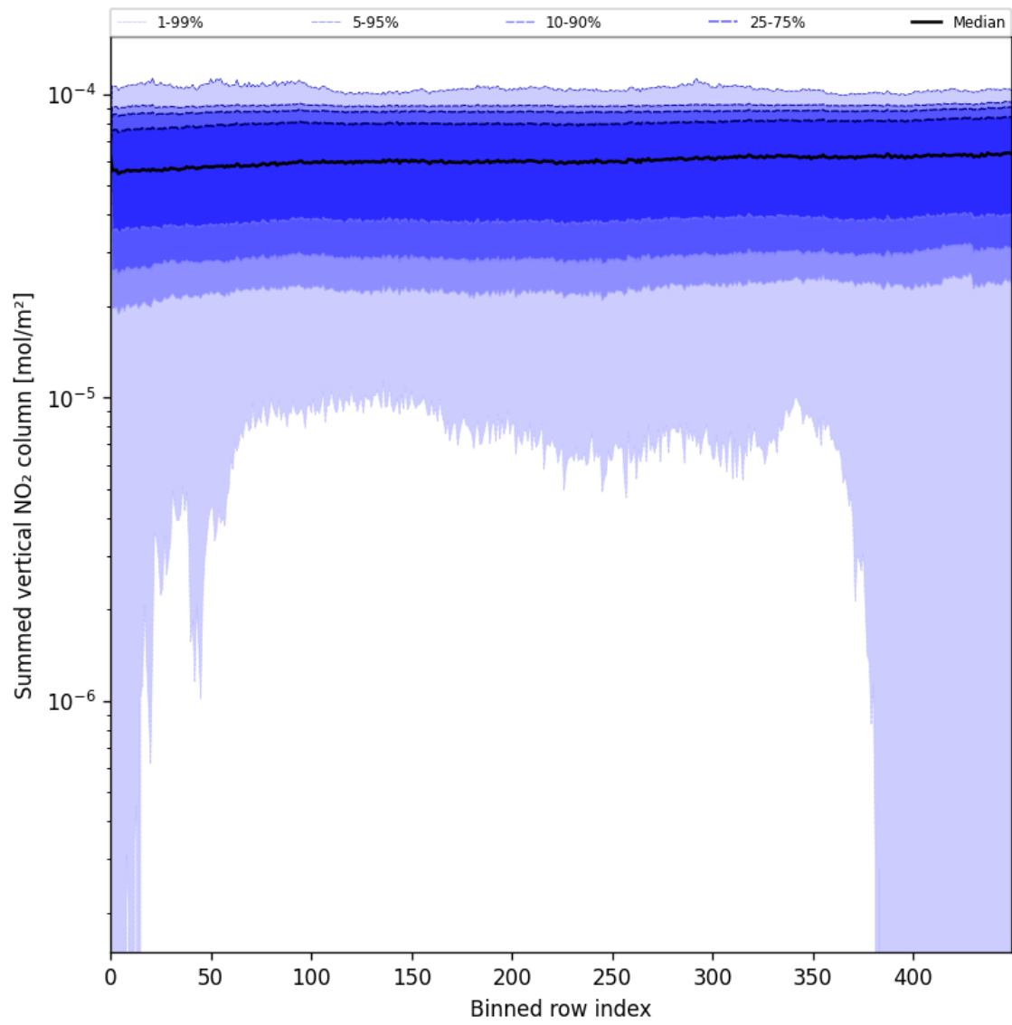
Figure 57: Along track statistics of “Summed vertical NO 2 column” for 2025-06-17 to 2025-06-19
