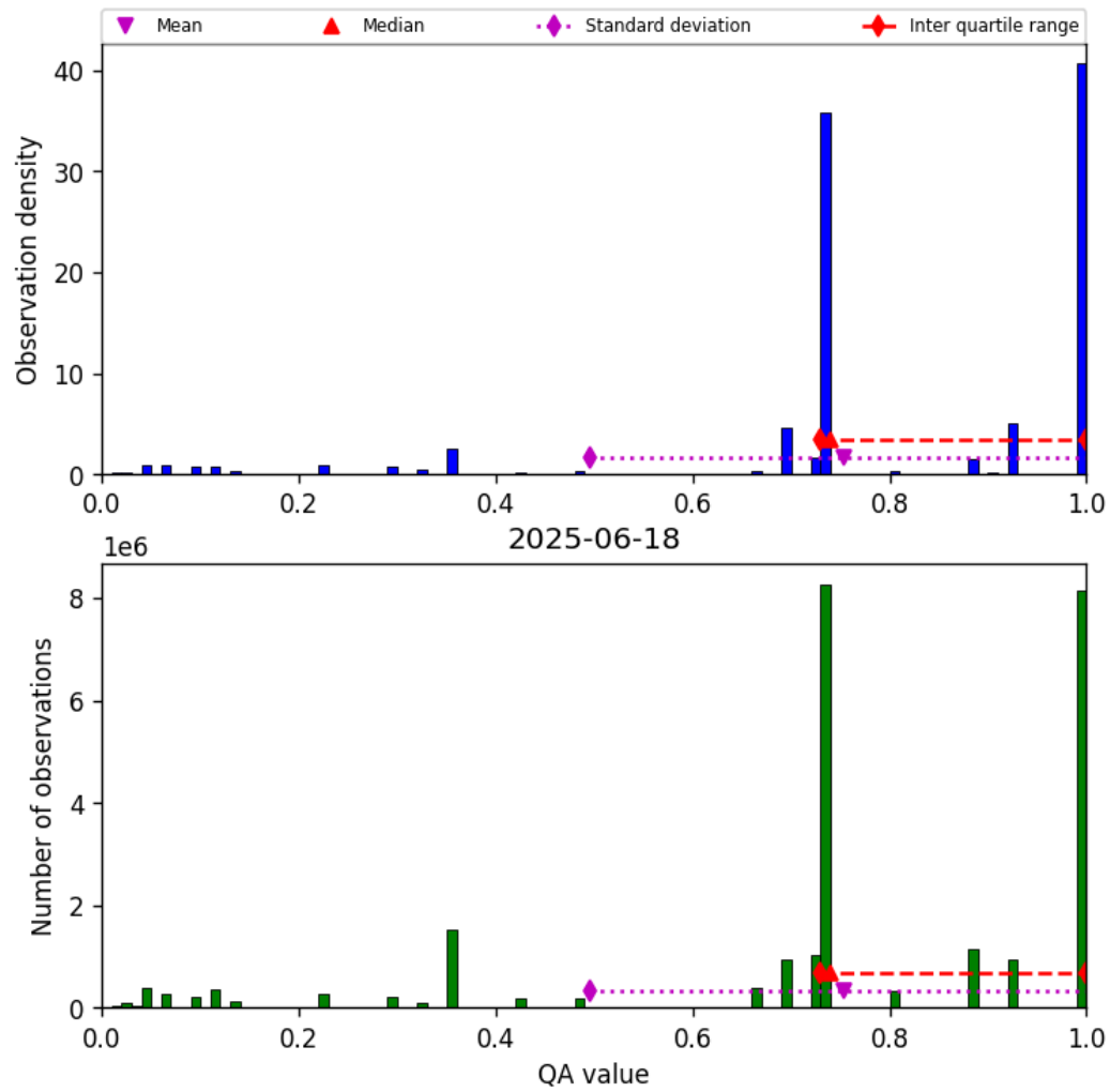
Figure 28: Histogram of “QA value” for 2025-06-17 to 2025-06-19
