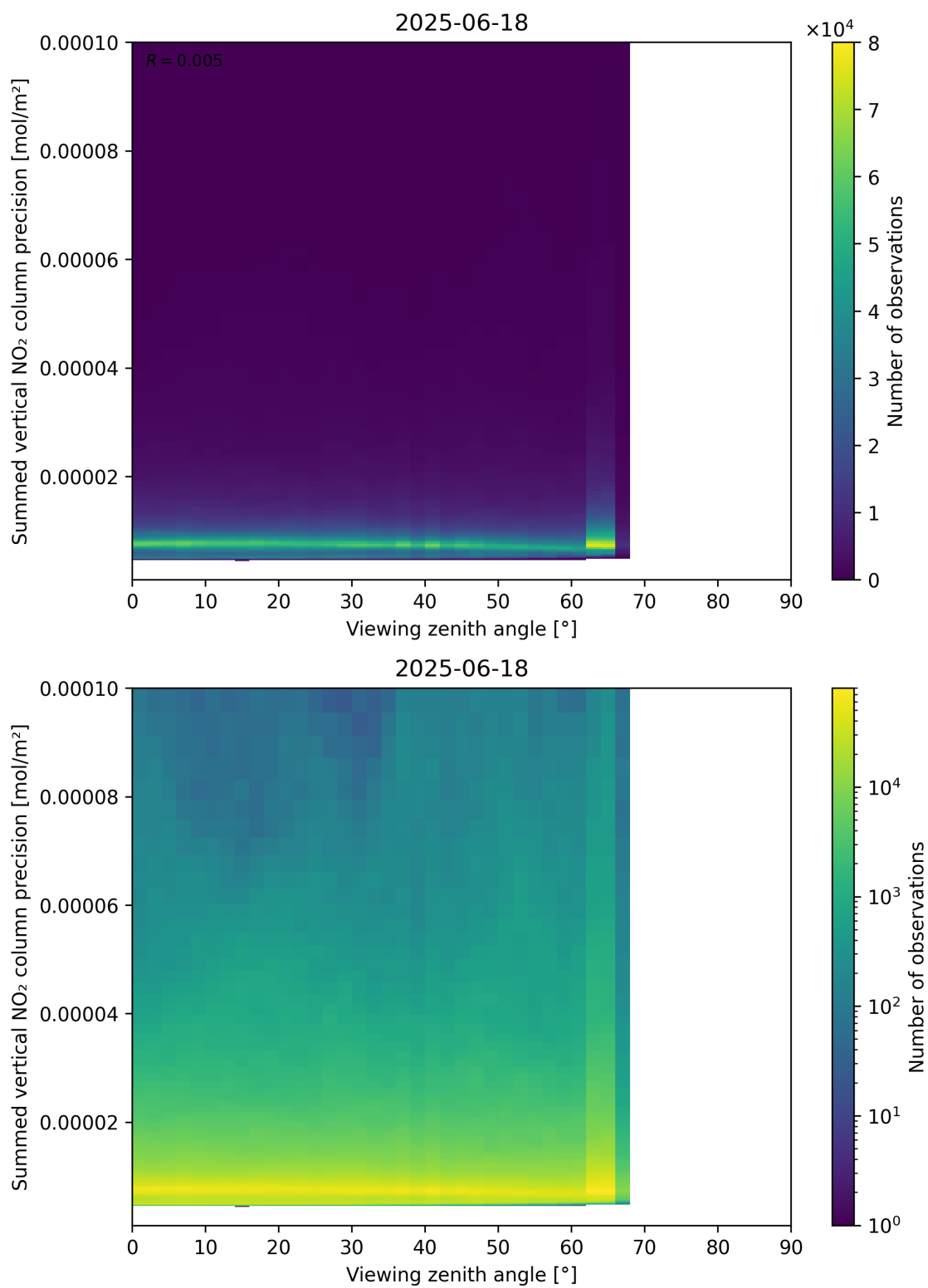
Figure 166: Scatter density plot of “Viewing zenith angle” against “Summed vertical NO 2 column precision” for 2025-06-17 to 2025-06-19.
