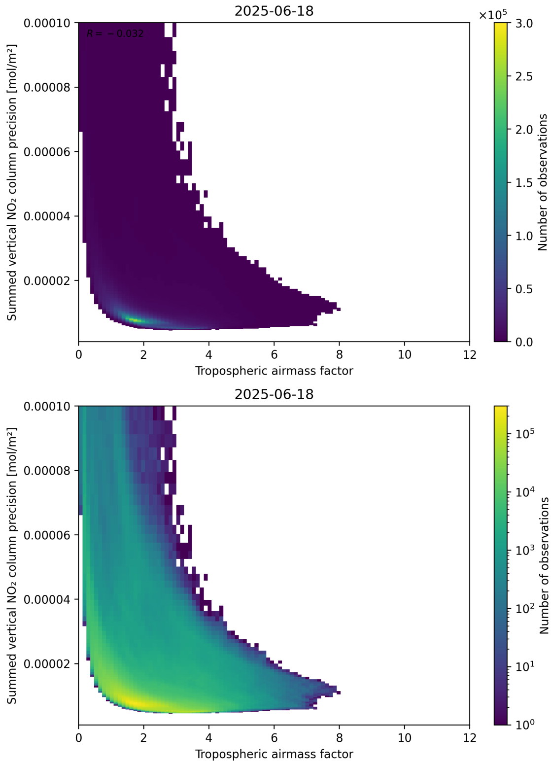
Figure 76: Scatter density plot of “Tropospheric air mass factor” against “Summed vertical NO 2 column precision” for 2025-06-17 to 2025-06-19.
