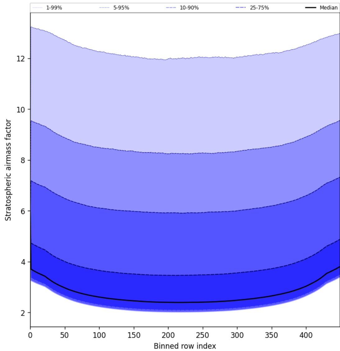
Figure 61: Along track statistics of “Stratospheric airmass factor” for 2025-06-17 to 2025-06-19
