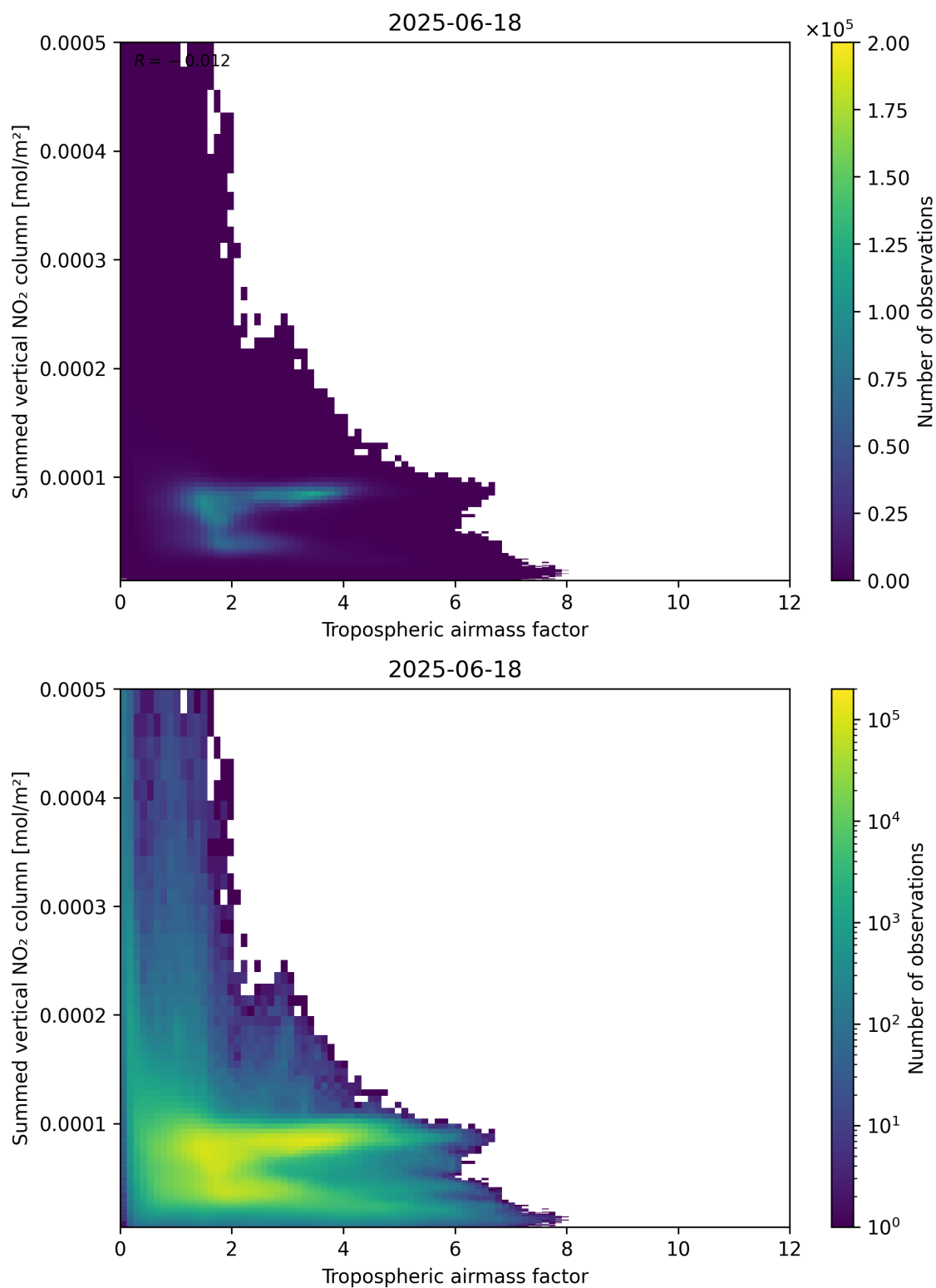
Figure 75: Scatter density plot of “Tropospheric air mass factor” against “Summed vertical NO 2 column” for 2025-06-17 to 2025-06-19.
