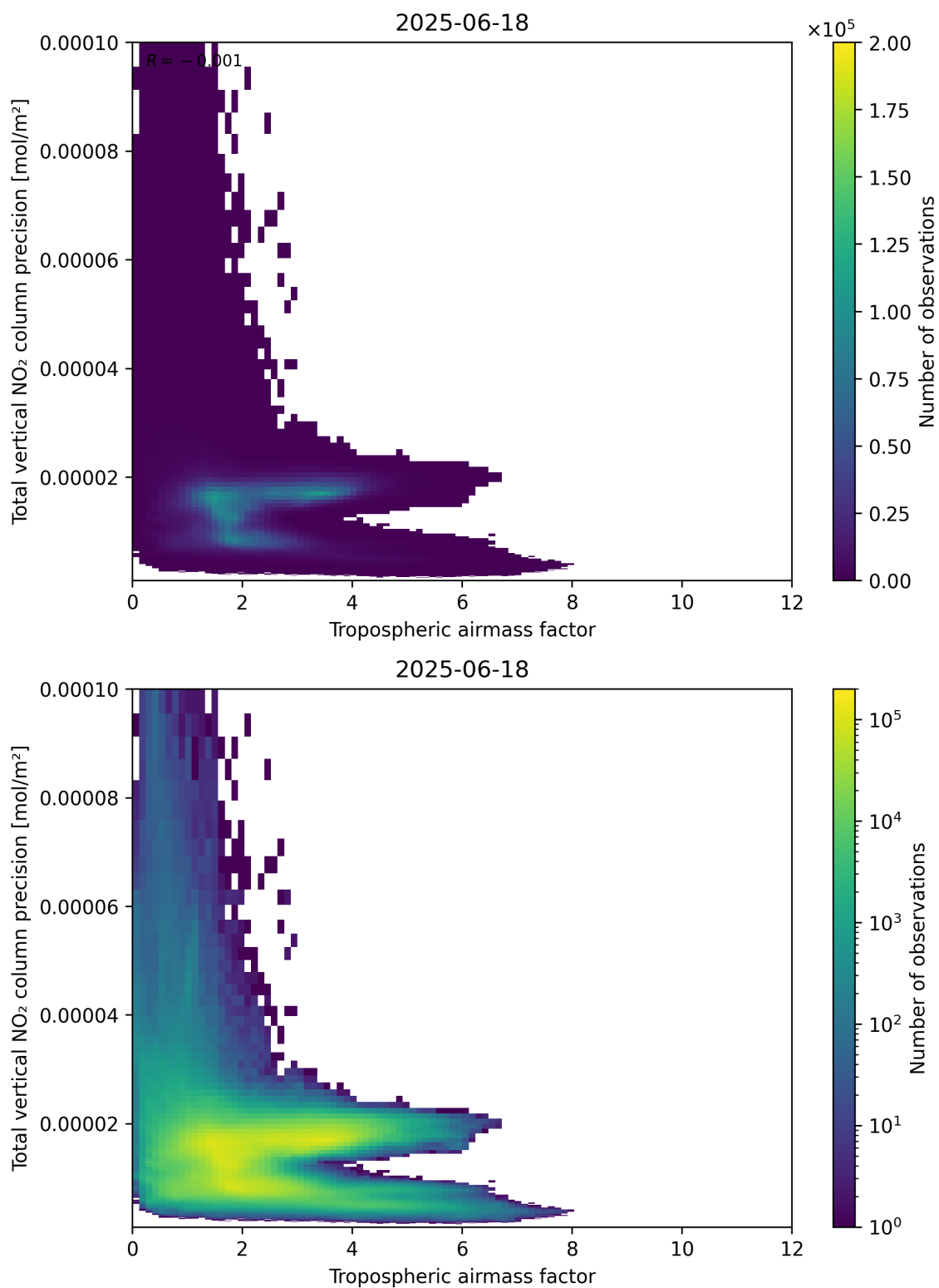
Figure 78: Scatter density plot of “Tropospheric airmass factor” against “Total vertical NO 2 column precision” for 2025-06-17 to 2025-06-19.
