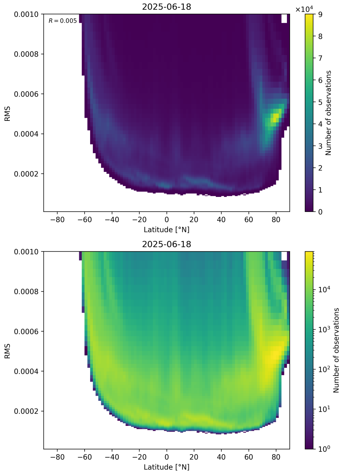
Figure 94: Scatter density plot of “Latitude” against “RMS” for 2025-06-17 to 2025-06-19.
