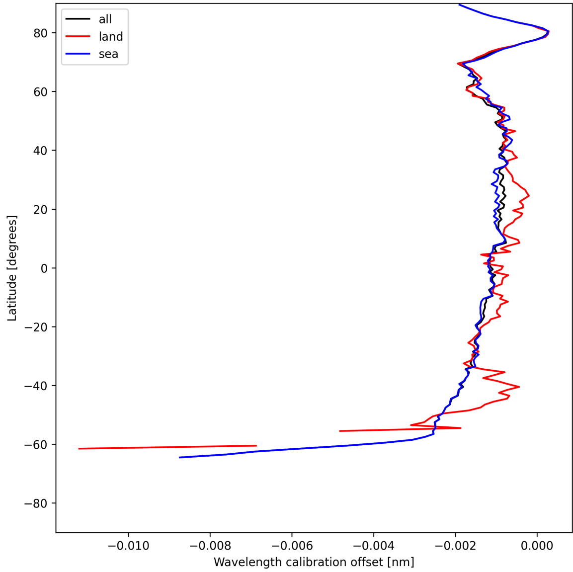
Figure 18: Zonal average of “Wavelength calibration offset” for 2025-06-17 to 2025-06-19.
