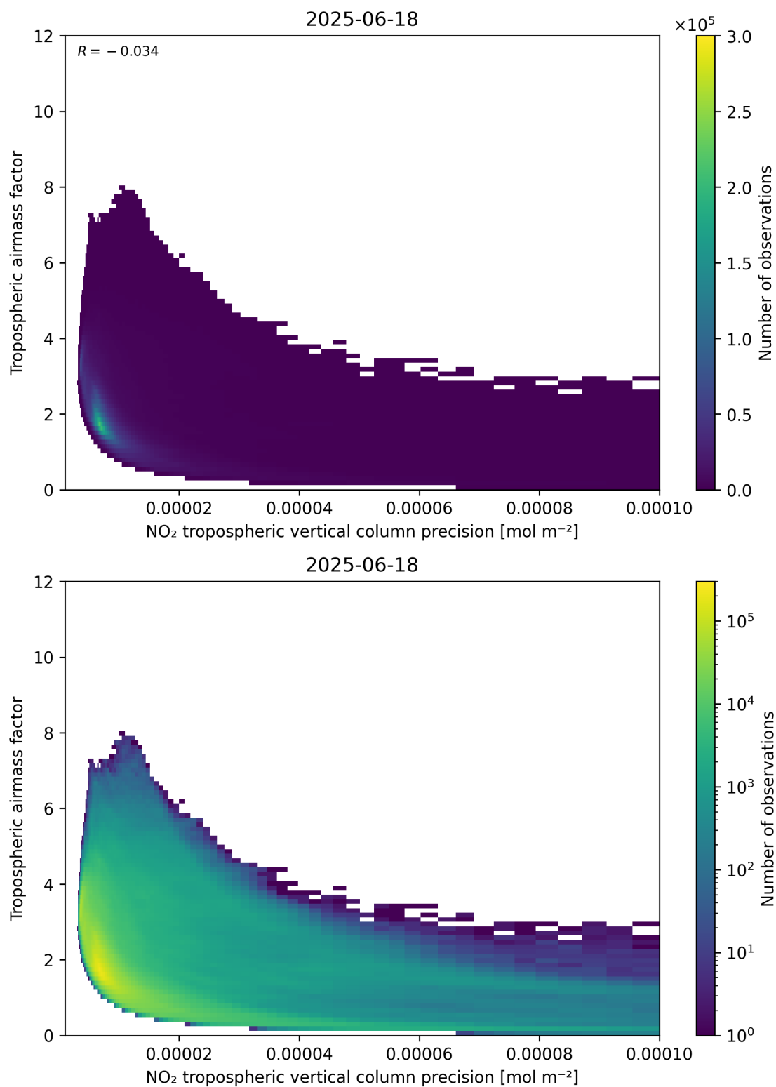
Figure 133: Scatter density plot of “NO 2 tropospheric vertical column precision” against “Tropospheric airmass factor” for 2025-06-17 to 2025-06-19.
