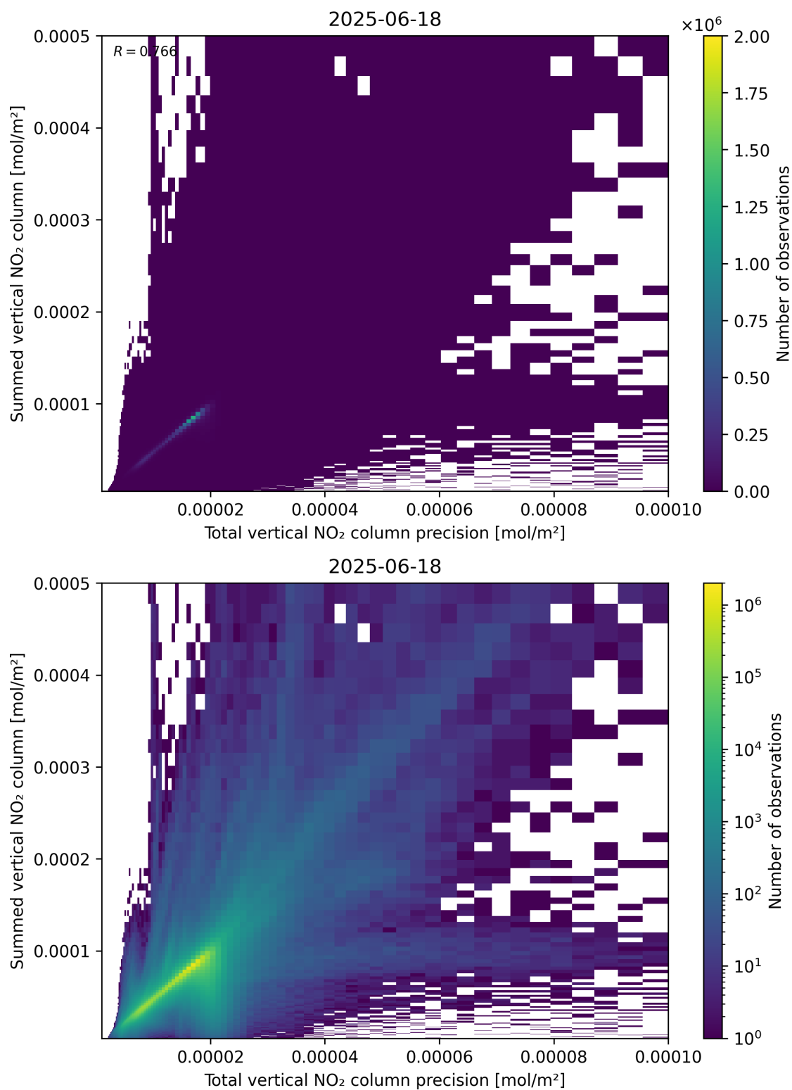
Figure 117: Scatter density plot of “Total vertical NO 2 column precision” against “Summed vertical NO 2 column” for 2025-06-17 to 2025-06-19.
