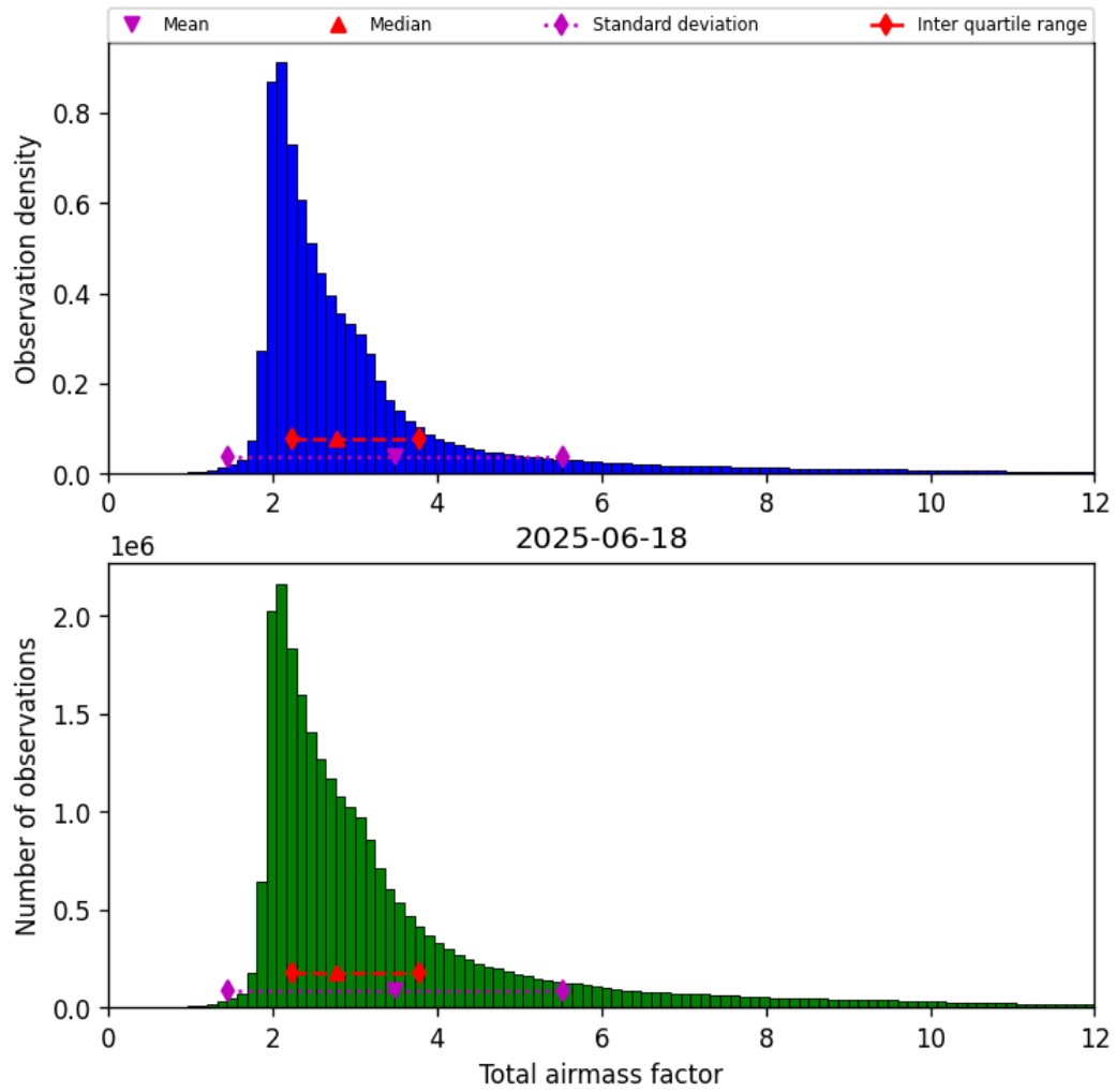
Figure 32: Histogram of “Total airmass factor” for 2025-06-17 to 2025-06-19
