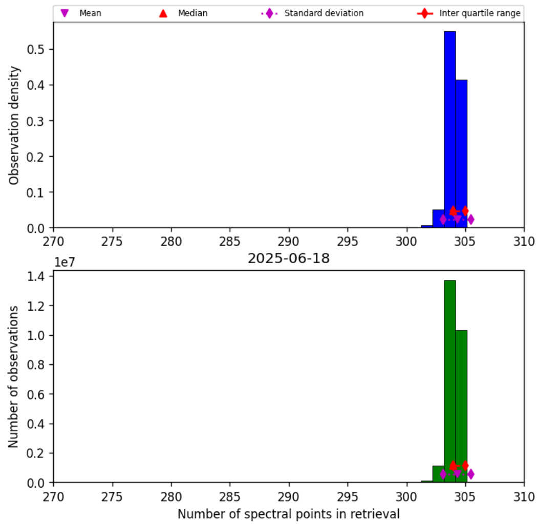
Figure 33: Histogram of “Number of spectral points in retrieval” for 2025-06-17 to 2025-06-19
