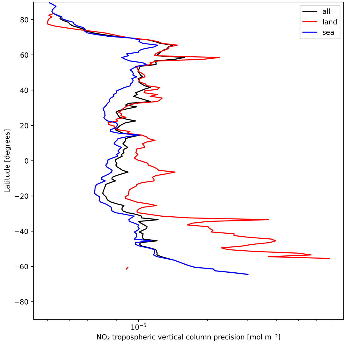
Figure 13: Zonal average of “NO 2 tropospheric vertical column precision” for 2025-06-17 to 2025-06-19.
