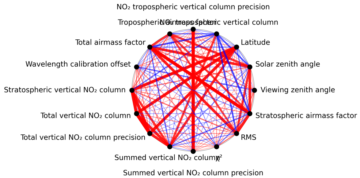
Figure 1: Map of correlation graph for 2025-06-17 to 2025-06-19.
