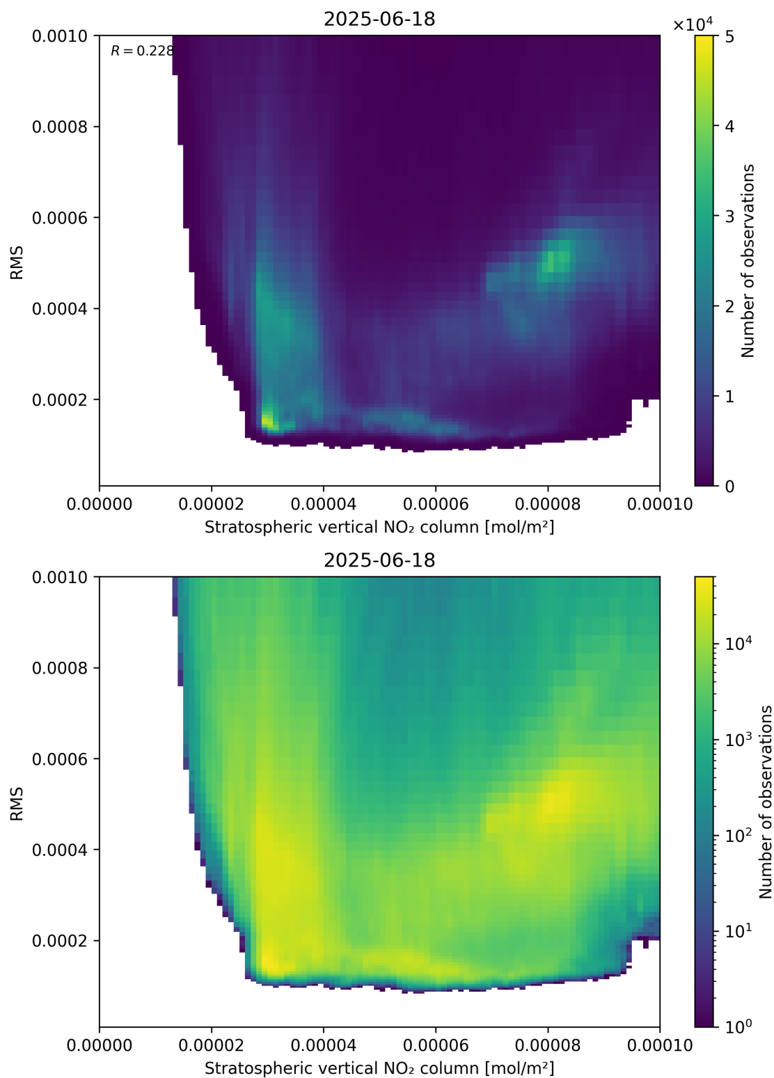
Figure 102: Scatter density plot of “Stratospheric vertical NO 2 column” against “RMS” for 2025-06-17 to 2025-06-19.
