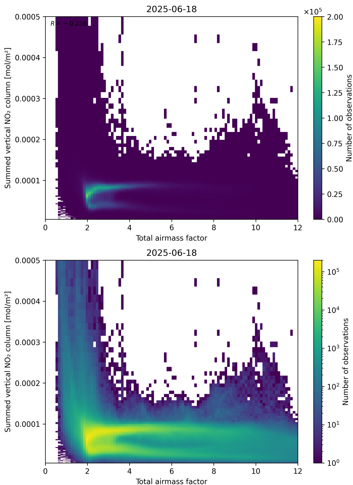
Figure 65: Scatter density plot of “Total airmass factor” against “Summed vertical NO 2 column” for 2025-06-17 to 2025-06-19.
