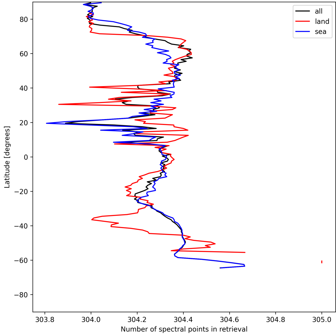
Figure 16: Zonal average of “Number of spectral points in retrieval” for 2025-06-17 to 2025-06-19.
