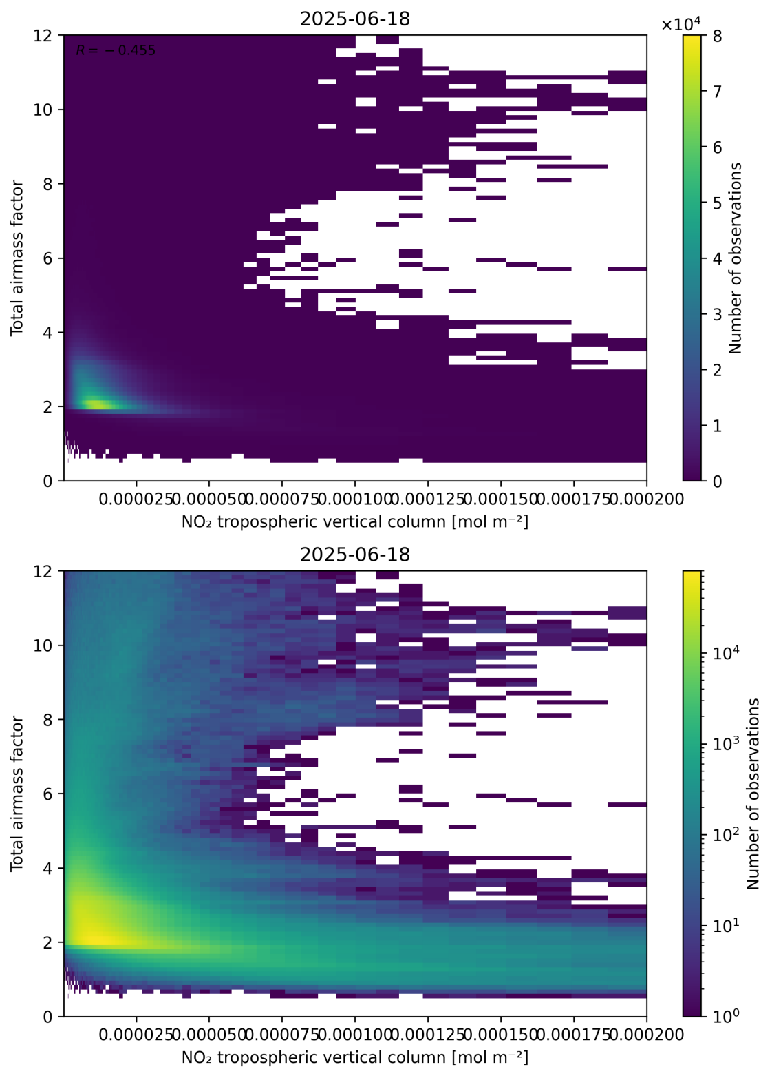
Figure 122: Scatter density plot of “NO 2 tropospheric vertical column” against “Total air mass factor” for 2025-06-17 to 2025-06-19.
