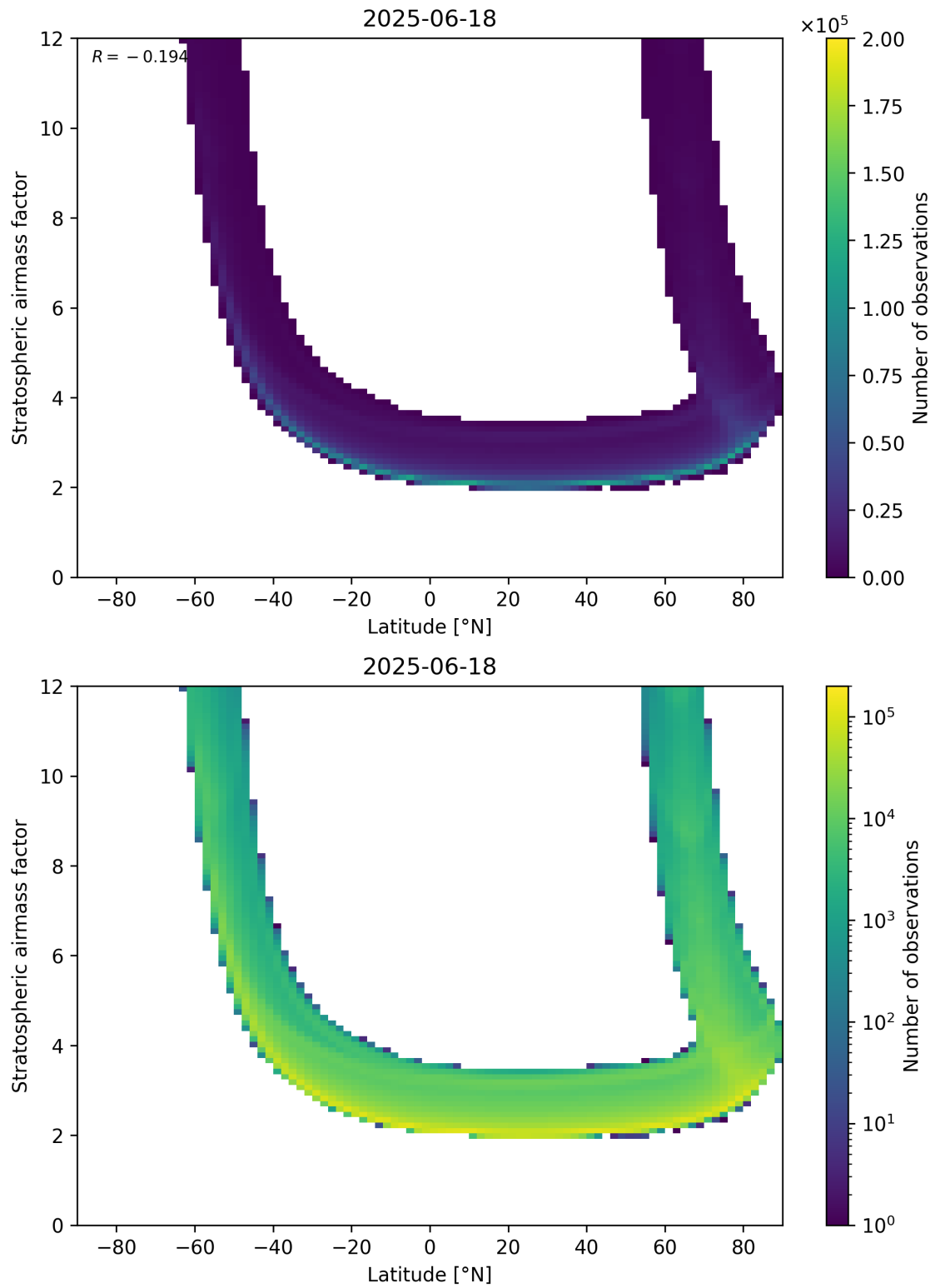
Figure 83: Scatter density plot of “Latitude” against “Stratospheric air mass factor” for 2025-06-17 to 2025-06-19.
