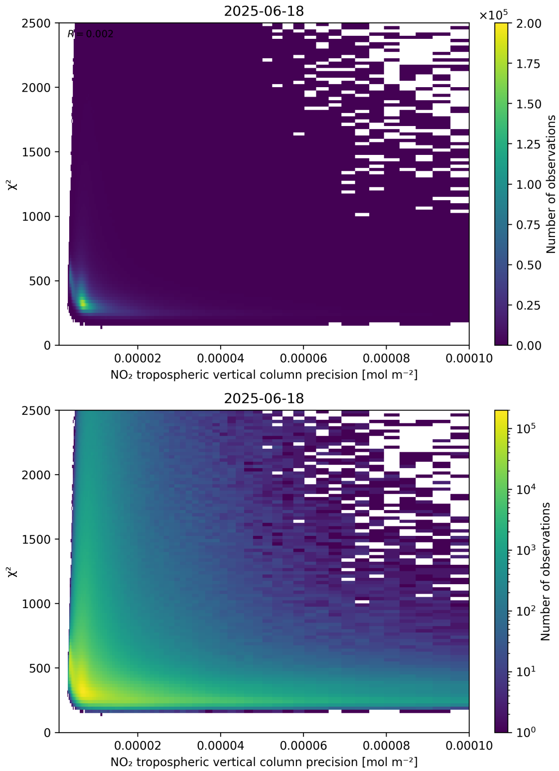
Figure 134: Scatter density plot of “NO 2 tropospheric vertical column precision” against “ \chi^2 ” for 2025-06-17 to 2025-06-19.
