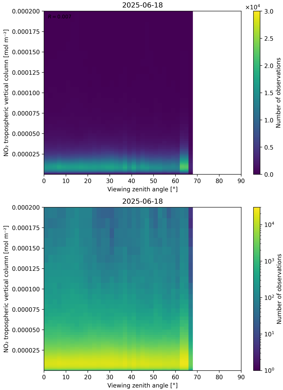
Figure 169: Scatter density plot of “Viewing zenith angle” against “NO 2 tropospheric vertical column” for 2025-06-17 to 2025-06-19.
