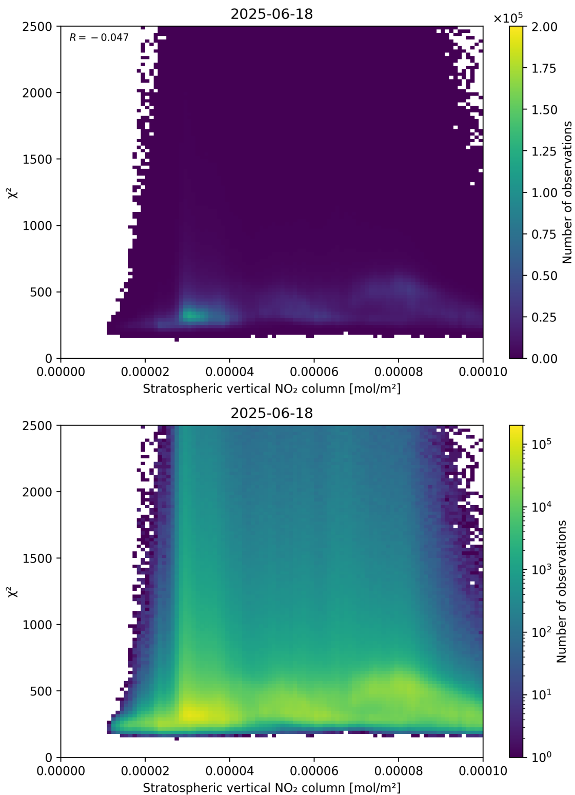
Figure 97: Scatter density plot of “Stratospheric vertical NO 2 column” against “ \chi^2 ” for 2025-06-17 to 2025-06-19.
