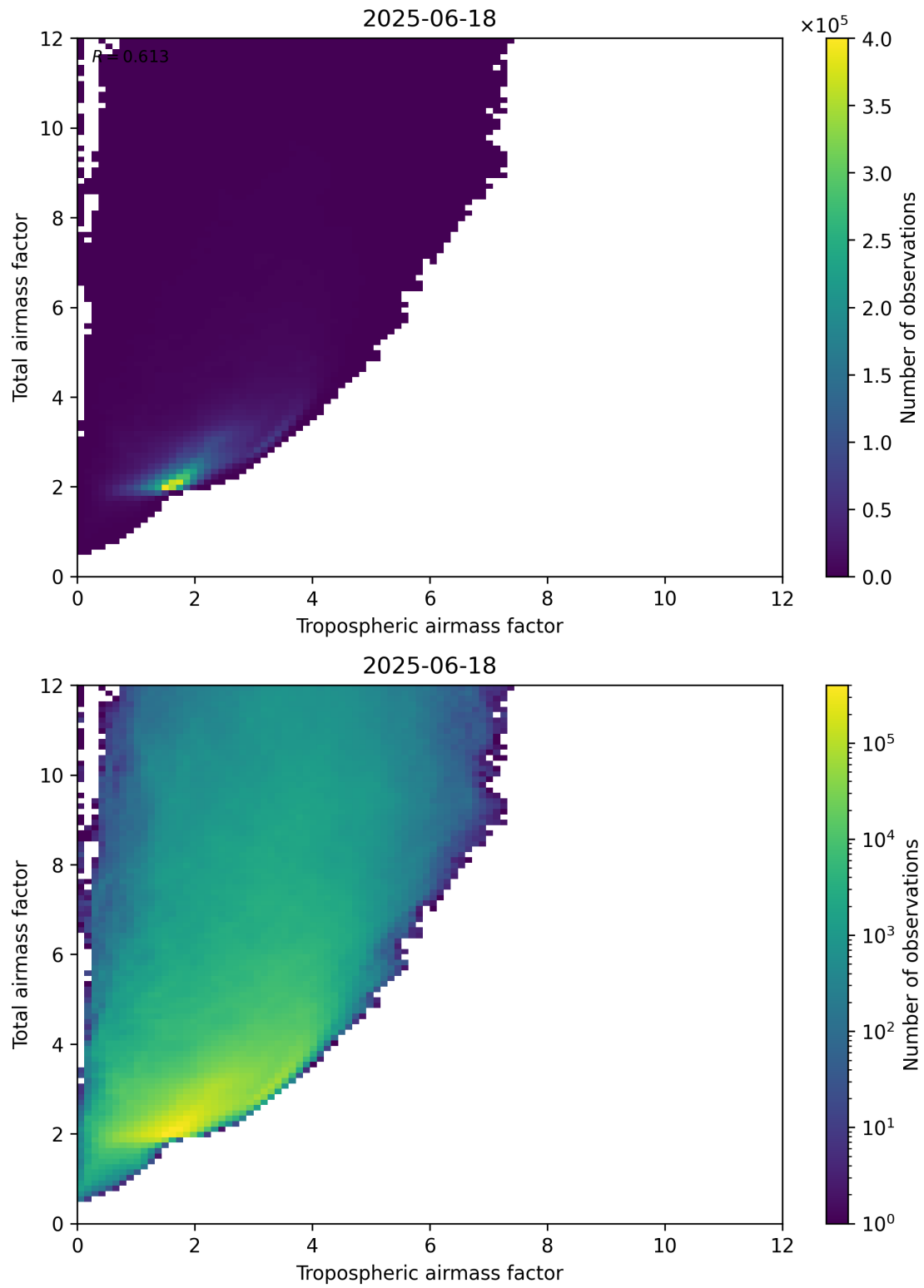
Figure 72: Scatter density plot of “Tropospheric airmass factor” against “Total airmass factor” for 2025-06-17 to 2025-06-19.
