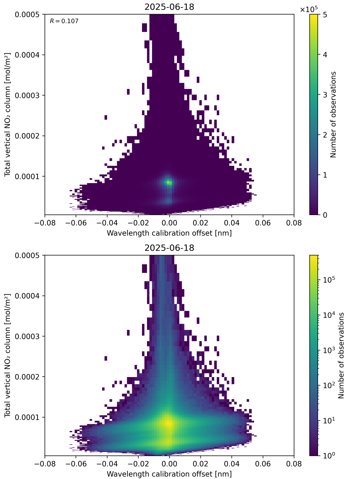
Figure 179: Scatter density plot of “Wavelength calibration offset” against “Total vertical NO 2 column” for 2025-06-17 to 2025-06-19.
