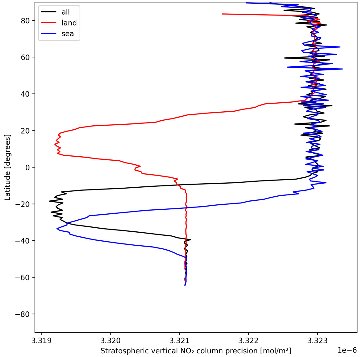
Figure 20: Zonal average of “Stratospheric vertical NO 2 column precision” for 2025-06-17 to 2025-06-19.
