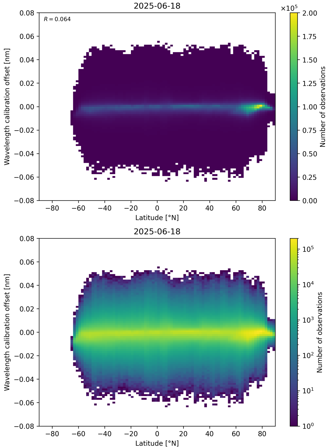
Figure 95: Scatter density plot of “Latitude” against “Wavelength calibration offset” for 2025-06-17 to 2025-06-19.
