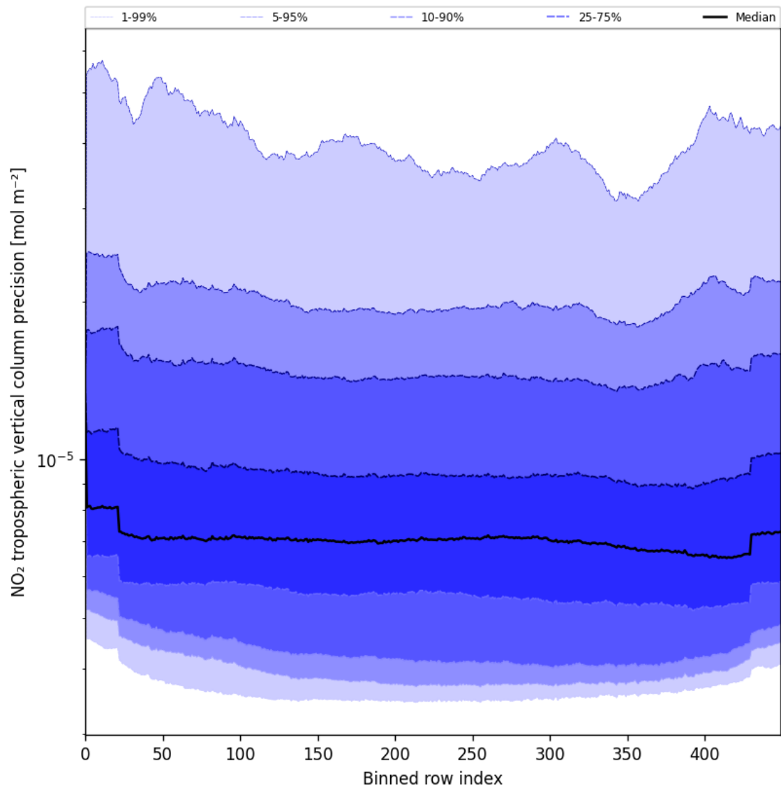
Figure 47: Along track statistics of “NO 2 tropospheric vertical column precision” for 2025-06-17 to 2025-06-19
