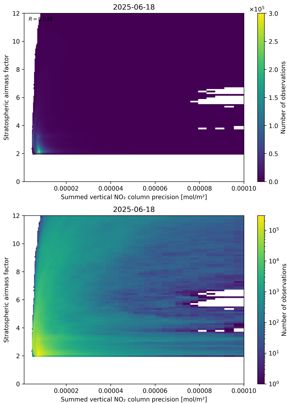
Figure 106: Scatter density plot of “Summed vertical NO 2 column precision” against “Stratospheric airmass factor” for 2025-06-17 to 2025-06-19.
