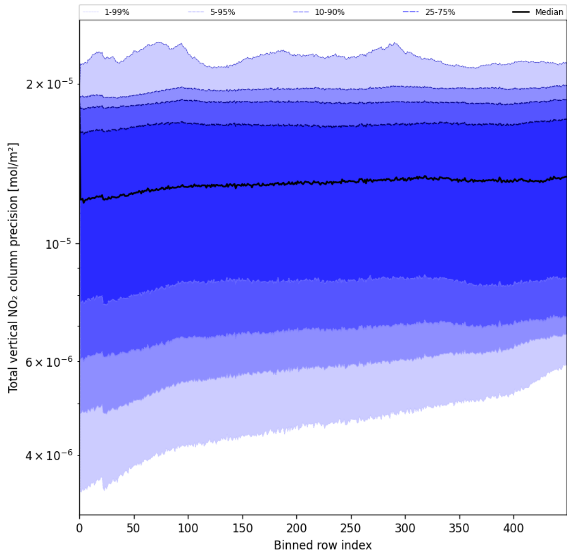
Figure 56: Along track statistics of "Total vertical NO 2 column precision" for 2025-06-17 to 2025-06-19
