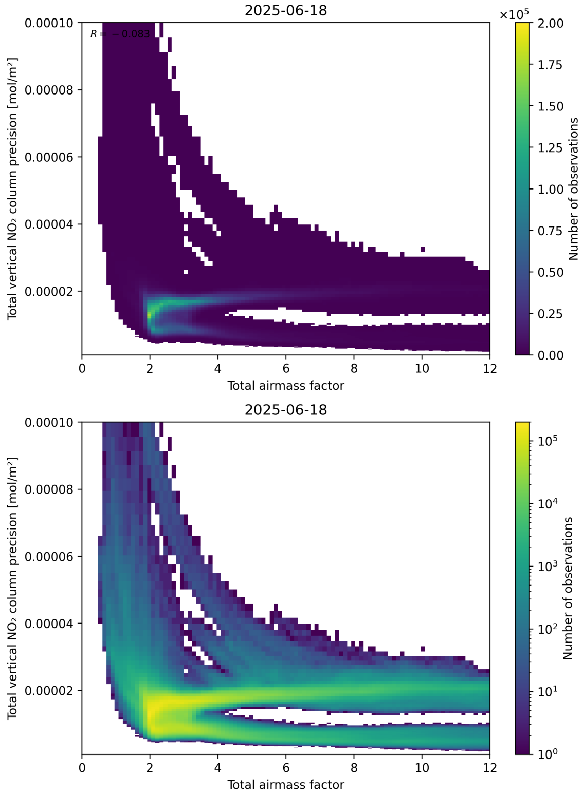
Figure 68: Scatter density plot of “Total airmass factor” against “Total vertical NO 2 column precision” for 2025-06-17 to 2025-06-19.
