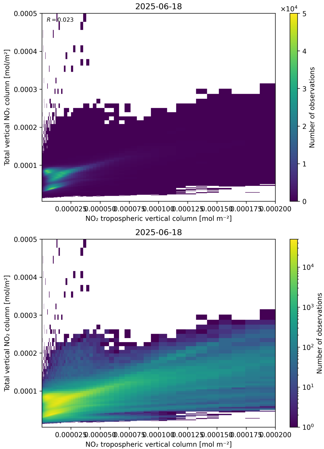
Figure 128: Scatter density plot of “NO 2 tropospheric vertical column” against “Total vertical NO 2 column” for 2025-06-17 to 2025-06-19.
