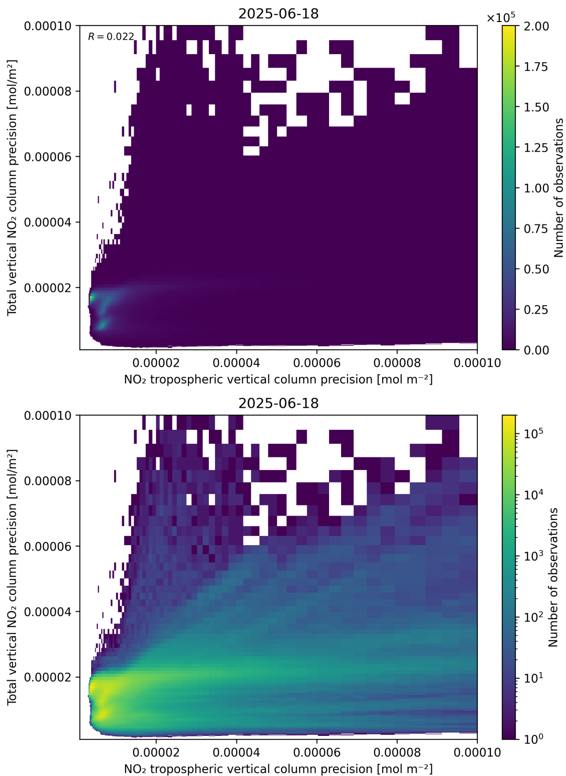
Figure 139: Scatter density plot of “NO 2 tropospheric vertical column precision” against “Total vertical NO 2 column precision” for 2025-06-17 to 2025-06-19.
