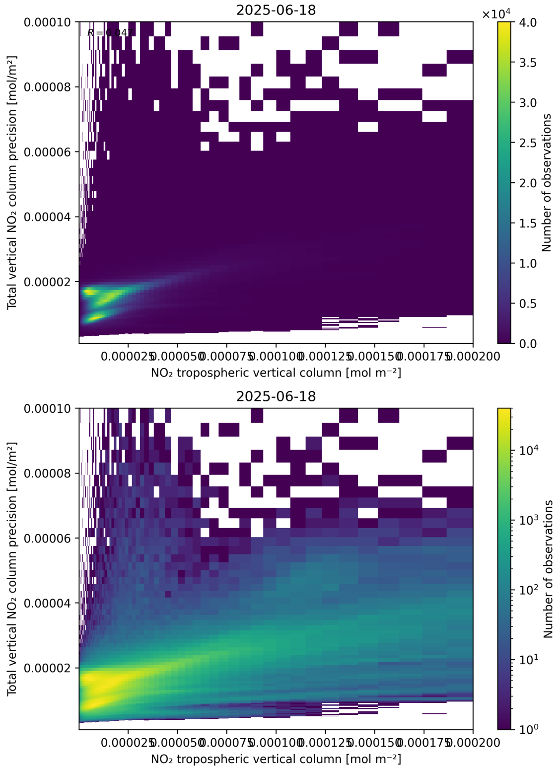
Figure 129: Scatter density plot of “NO 2 tropospheric vertical column” against “Total vertical NO 2 column precision” for 2025-06-17 to 2025-06-19.
