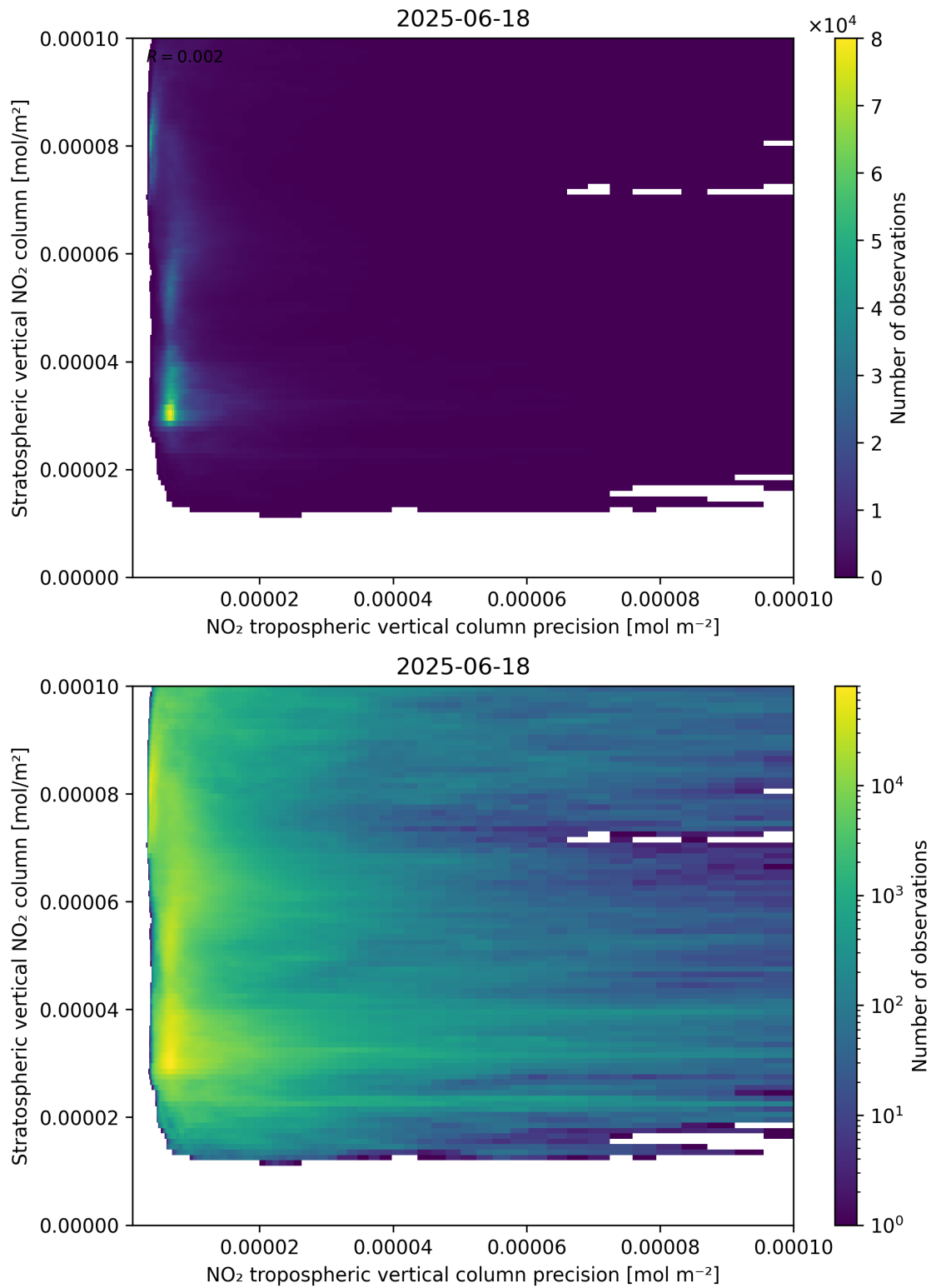
Figure 135: Scatter density plot of “NO 2 tropospheric vertical column precision” against “Stratospheric vertical NO 2 column” for 2025-06-17 to 2025-06-19.
