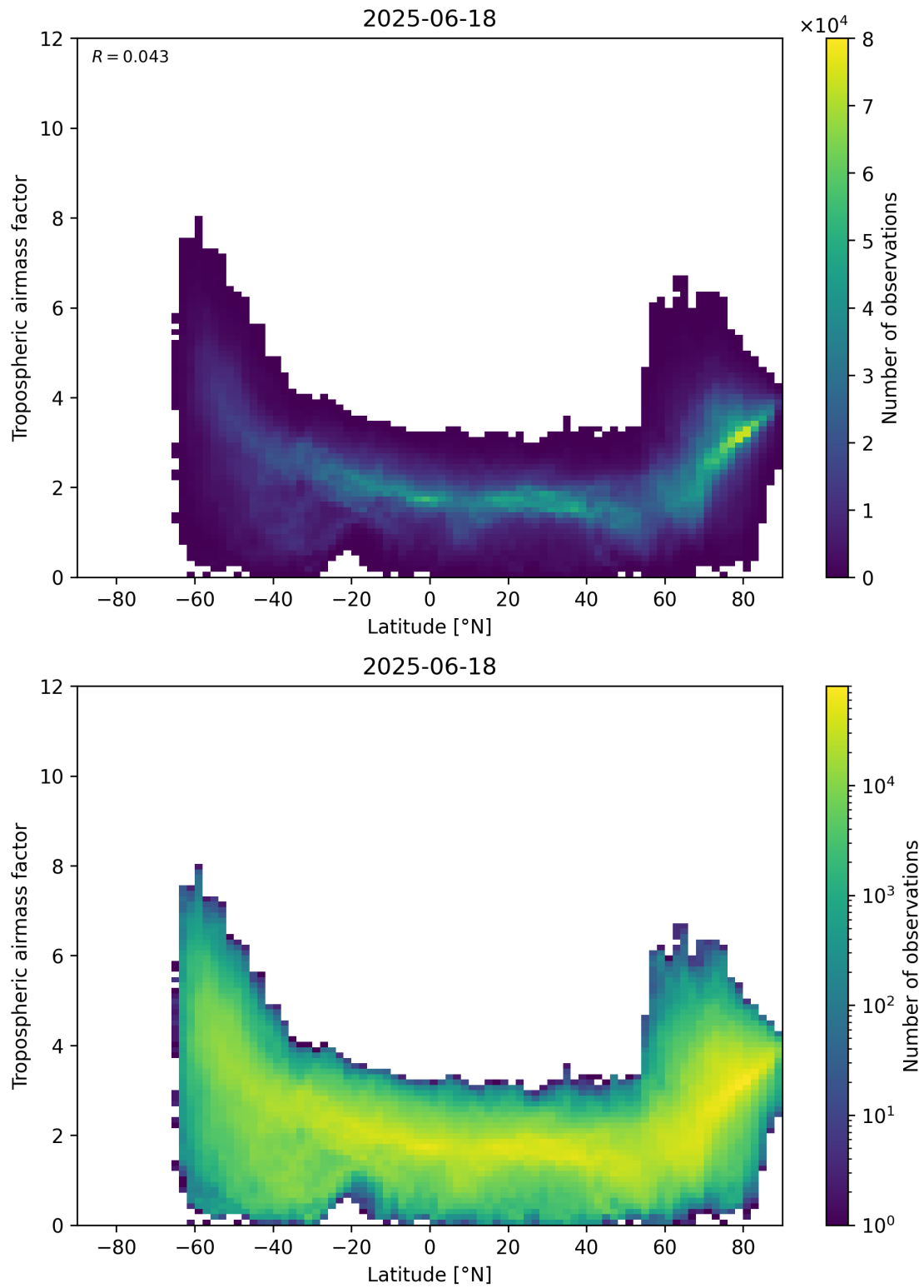
Figure 85: Scatter density plot of “Latitude” against “Tropospheric air mass factor” for 2025-06-17 to 2025-06-19.
