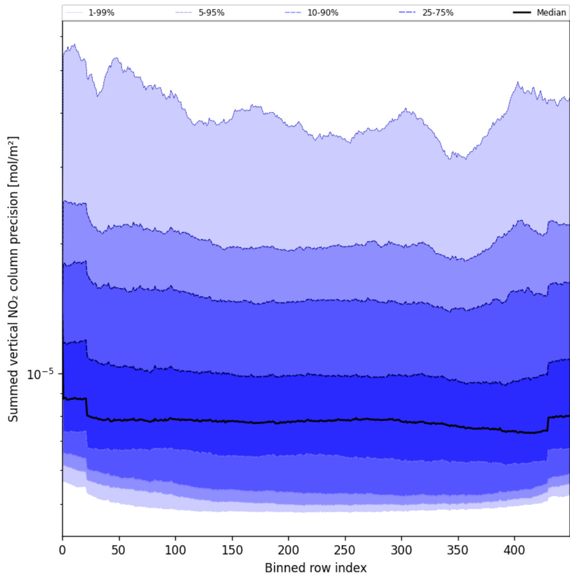
Figure 58: Along track statistics of “Summed vertical NO 2 column precision” for 2025-06-17 to 2025-06-19
