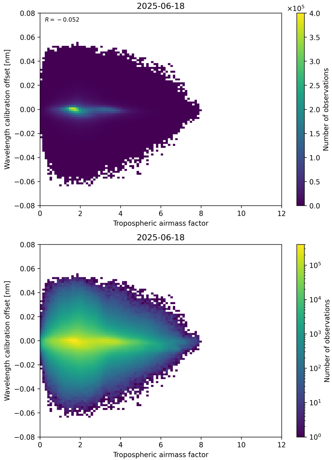
Figure 80: Scatter density plot of “Tropospheric airmass factor” against “Wavelength calibration offset” for 2025-06-17 to 2025-06-19.
