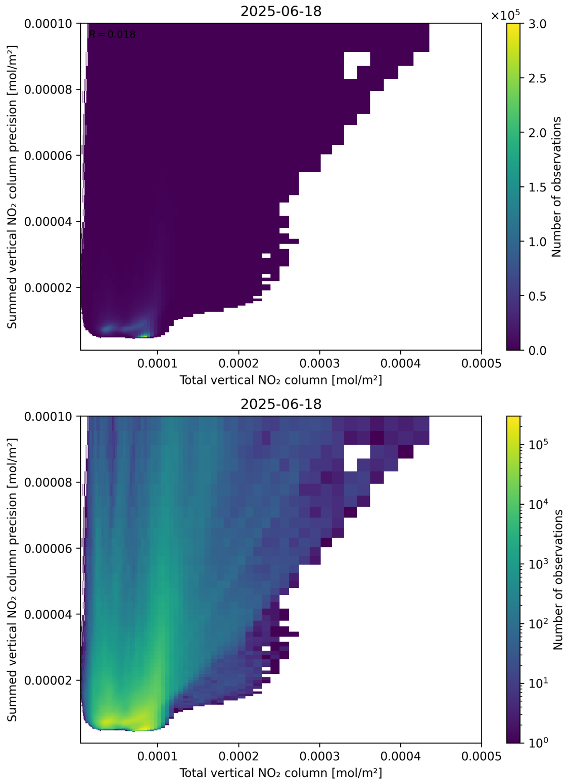
Figure 113: Scatter density plot of “Total vertical NO 2 column” against “Summed vertical NO 2 column precision” for 2025-06-17 to 2025-06-19.
