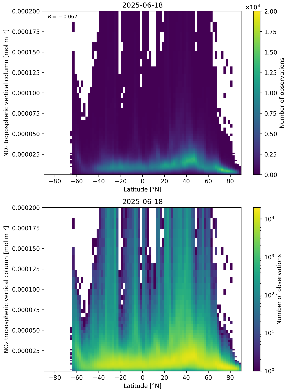
Figure 92: Scatter density plot of “Latitude” against “NO 2 tropospheric vertical column” for 2025-06-17 to 2025-06-19.
