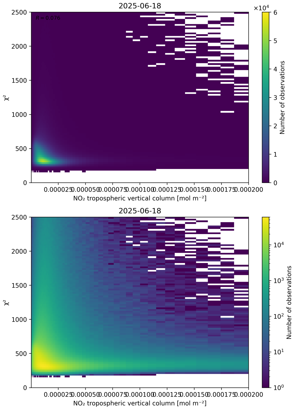
Figure 124: Scatter density plot of “NO 2 tropospheric vertical column” against “ \chi^2 ” for 2025-06-17 to 2025-06-19.
