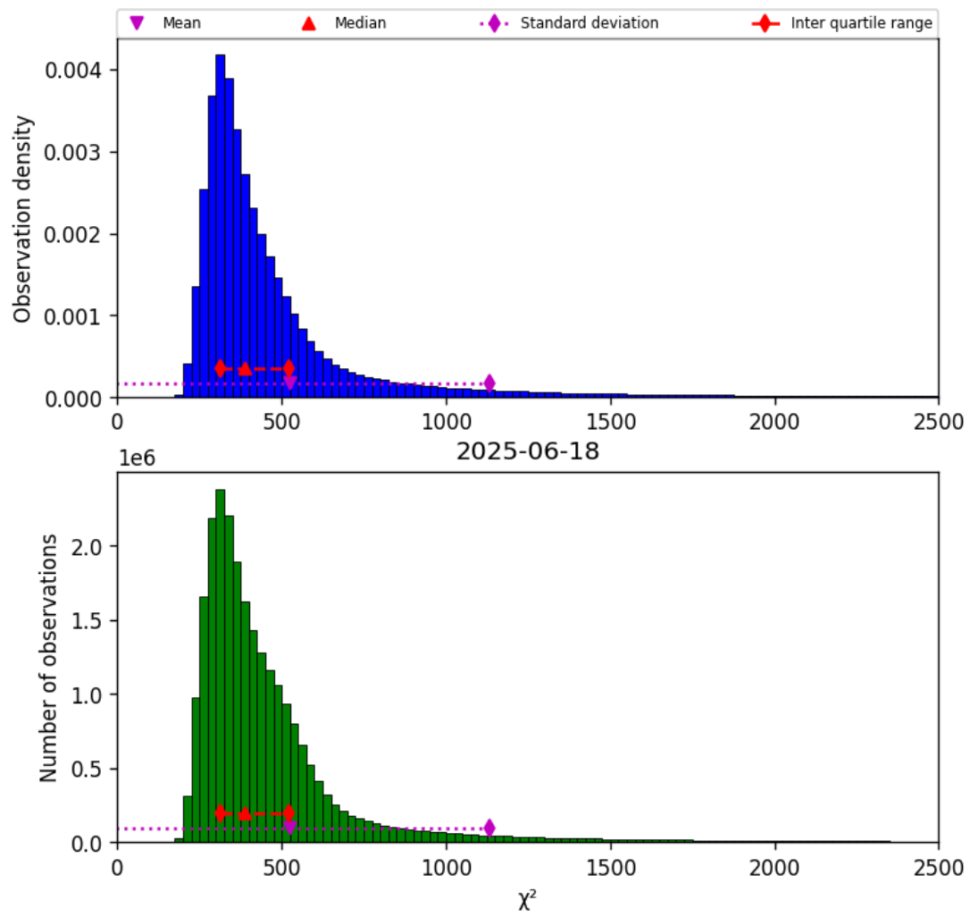
Figure 42: Histogram of “ \chi^2 ” for 2025-06-17 to 2025-06-19
