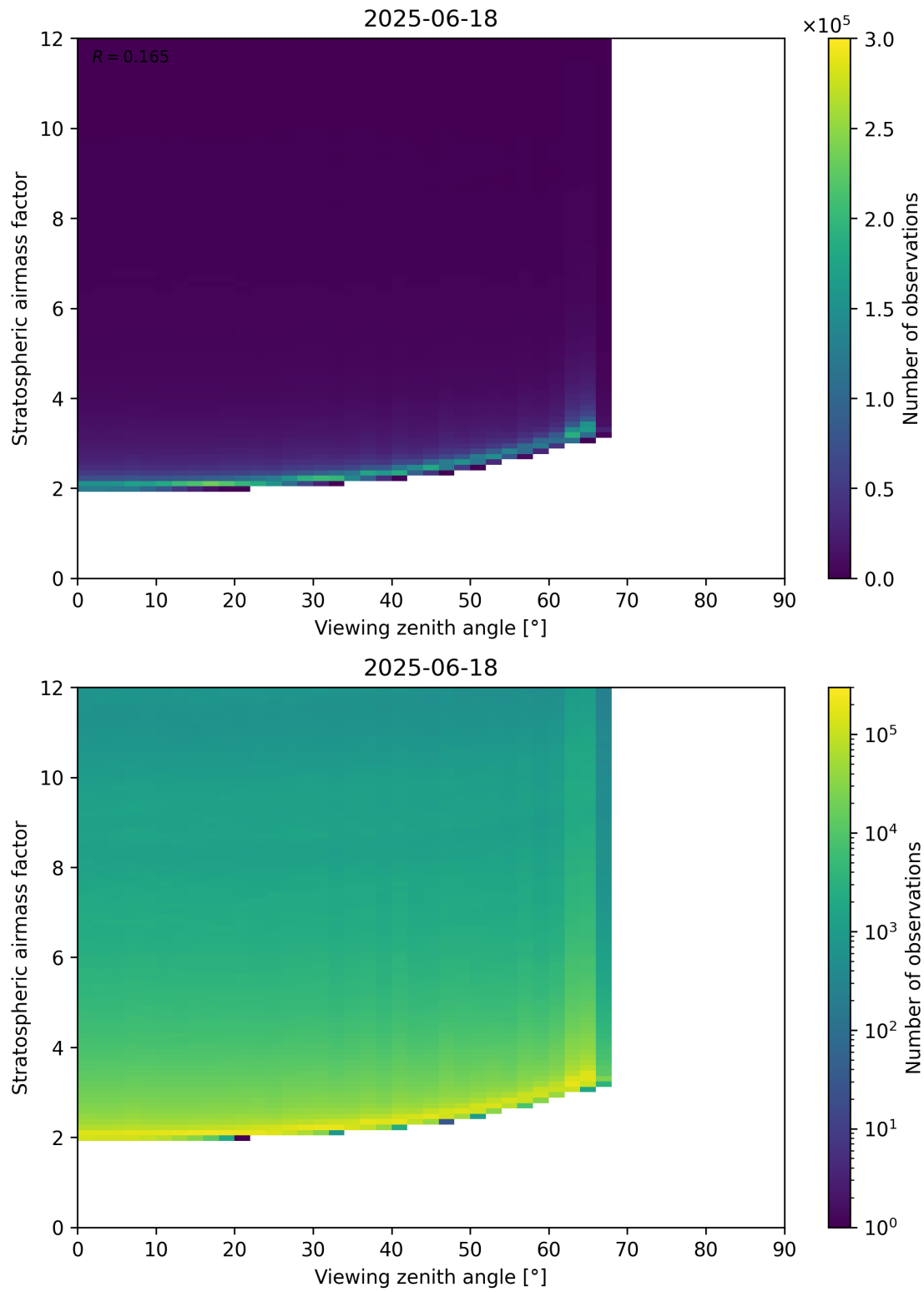
Figure 159: Scatter density plot of “Viewing zenith angle” against “Stratospheric airmass factor” for 2025-06-17 to 2025-06-19.
