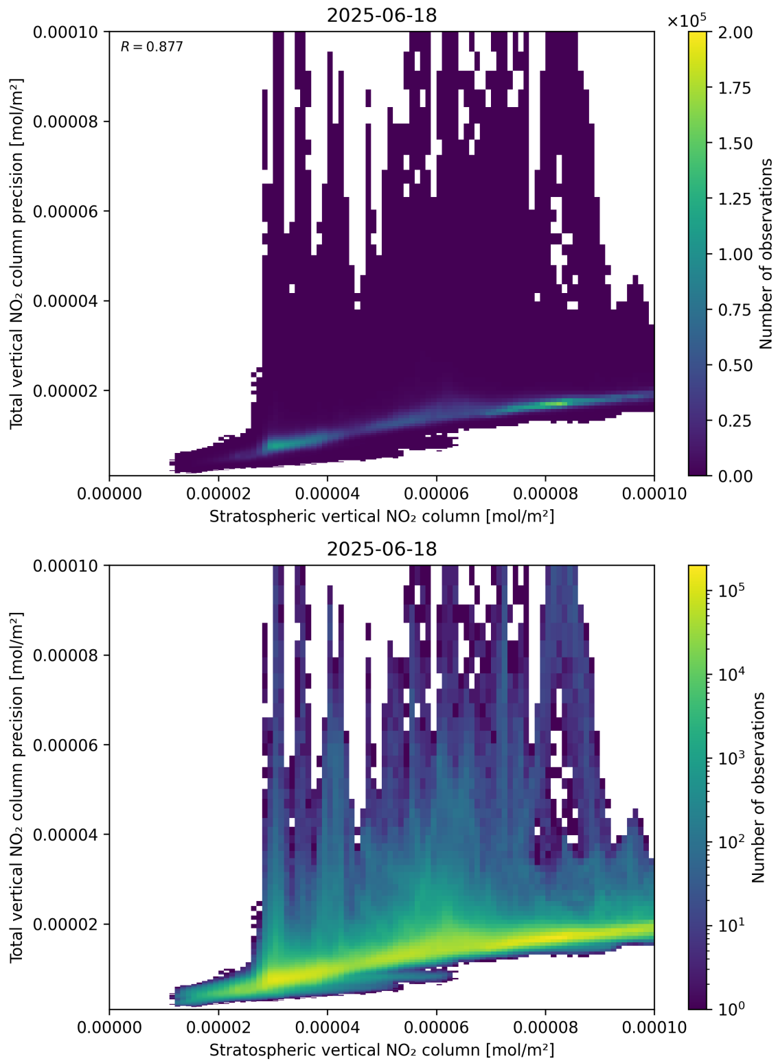
Figure 101: Scatter density plot of “Stratospheric vertical NO 2 column” against “Total vertical NO 2 column precision” for 2025-06-17 to 2025-06-19.
