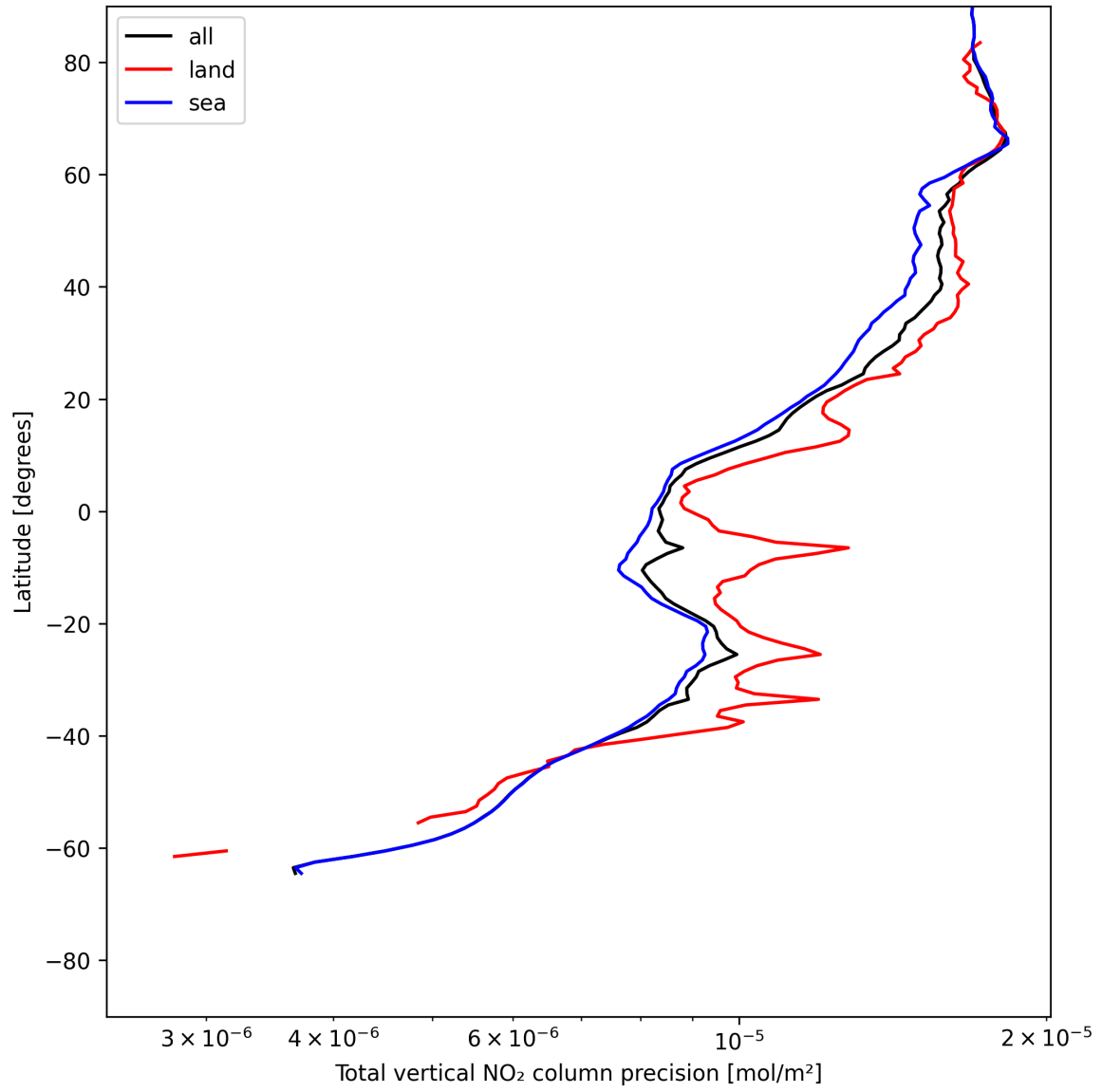
Figure 22: Zonal average of “Total vertical NO 2 column precision” for 2025-06-17 to 2025-06-19.
