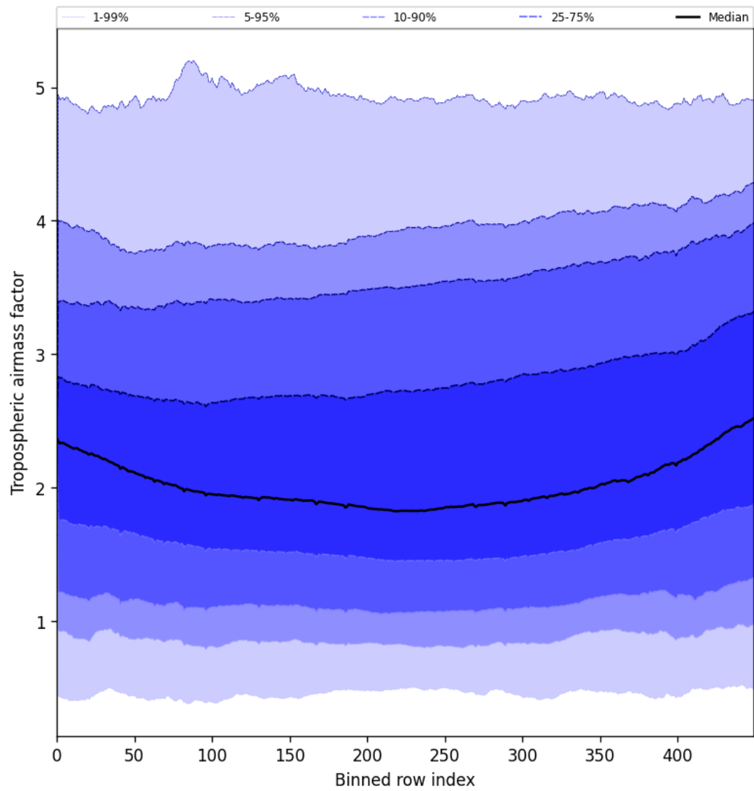
Figure 48: Along track statistics of “Tropospheric airmass factor” for 2025-06-17 to 2025-06-19
