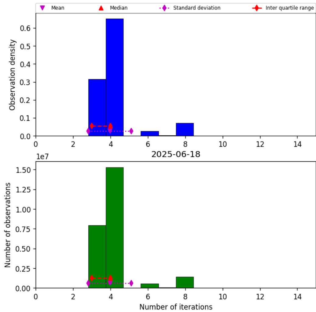
Figure 34: Histogram of “Number of iterations” for 2025-06-17 to 2025-06-19
