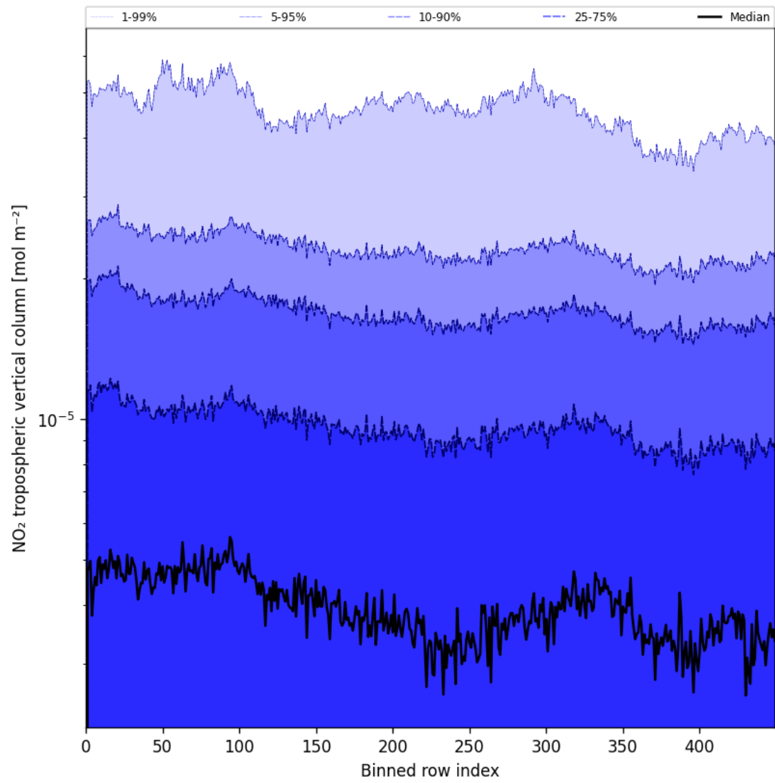
Figure 46: Along track statistics of “NO 2 tropospheric vertical column” for 2025-06-17 to 2025-06-19
