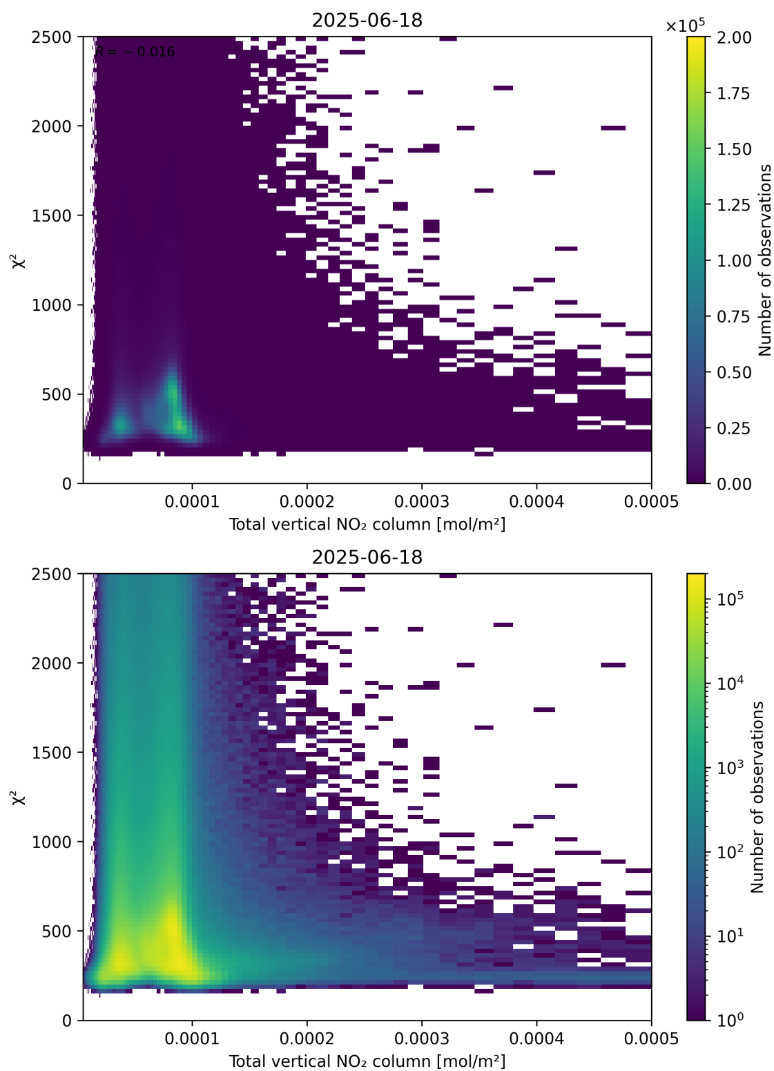
Figure 111: Scatter density plot of “Total vertical NO 2 column” against “ \chi^2 ” for 2025-06-17 to 2025-06-19.
