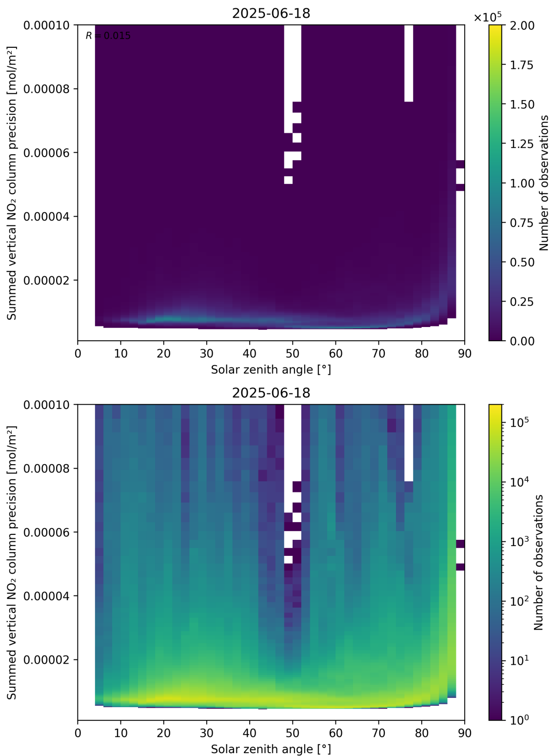
Figure 152: Scatter density plot of “Solar zenith angle” against “Summed vertical NO 2 column precision” for 2025-06-17 to 2025-06-19.
