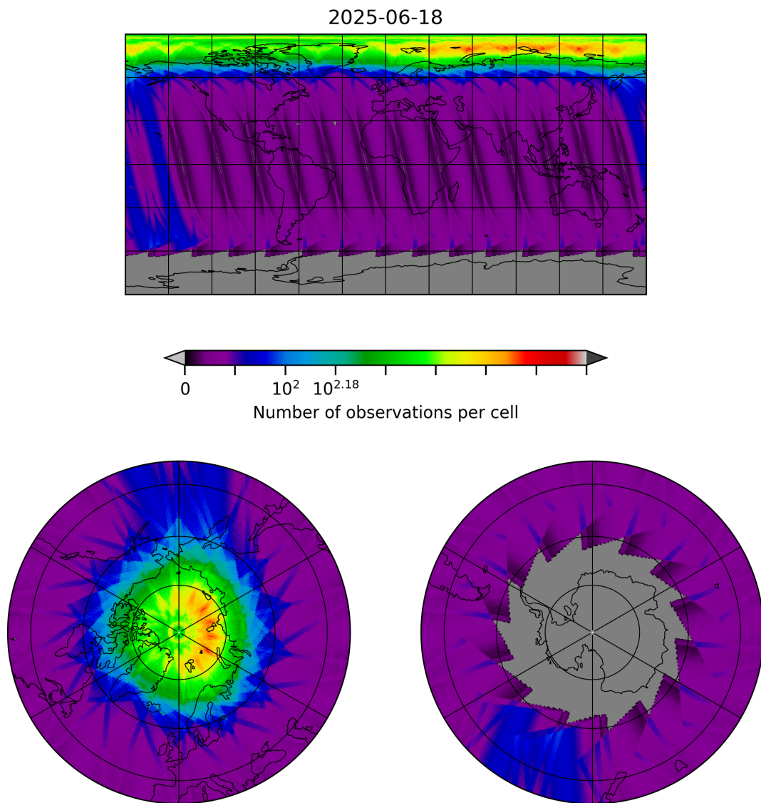
Figure 10: Map of the number of observations for 2025-06-17 to 2025-06-19
