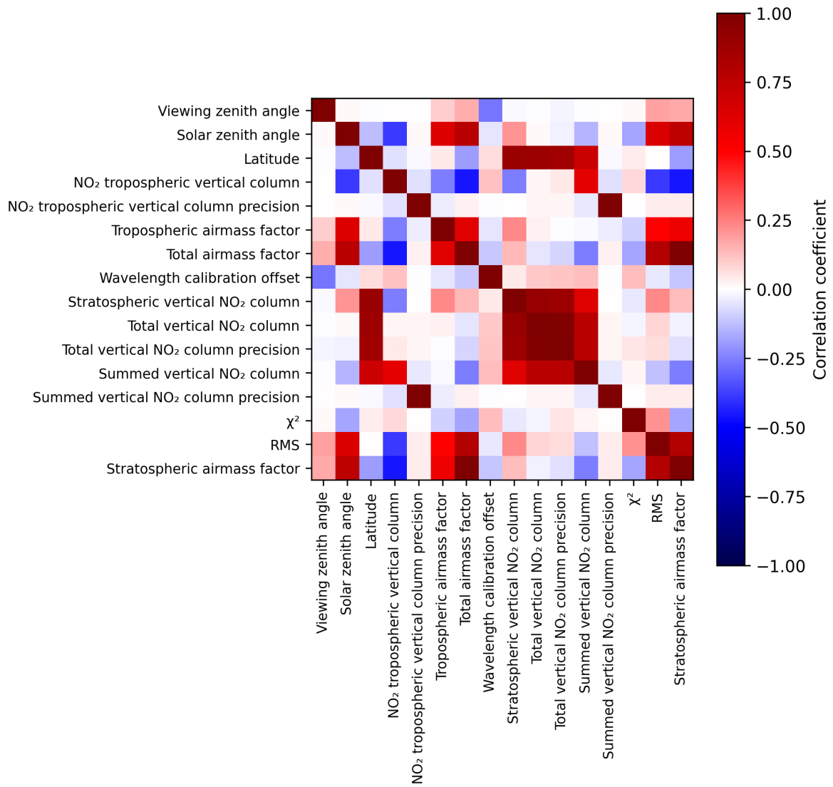
Figure 2: Map of correlation matrix for 2025-06-17 to 2025-06-19.
