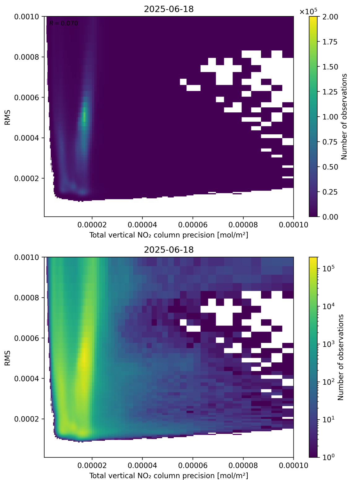
Figure 119: Scatter density plot of “Total vertical NO 2 column precision” against “RMS” for 2025-06-17 to 2025-06-19.
