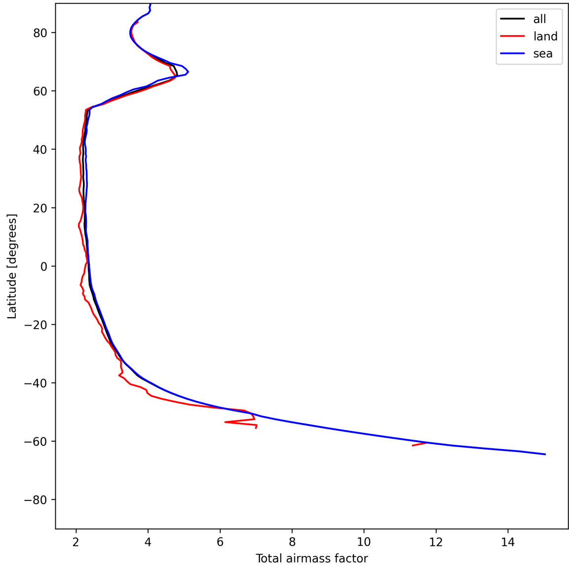
Figure 15: Zonal average of “Total airmass factor” for 2025-06-17 to 2025-06-19.
