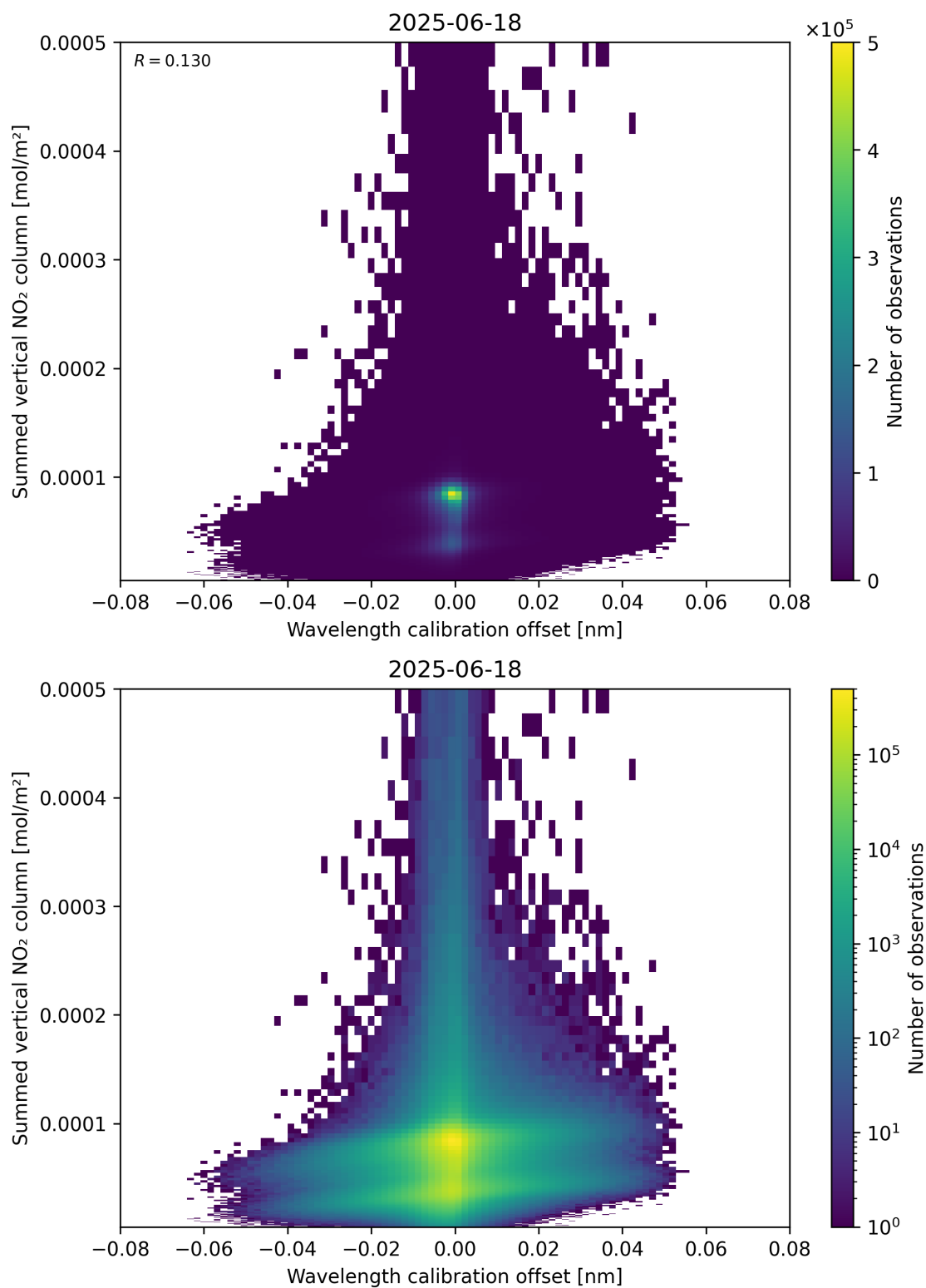
Figure 177: Scatter density plot of “Wavelength calibration offset” against “Summed vertical NO 2 column” for 2025-06-17 to 2025-06-19.
