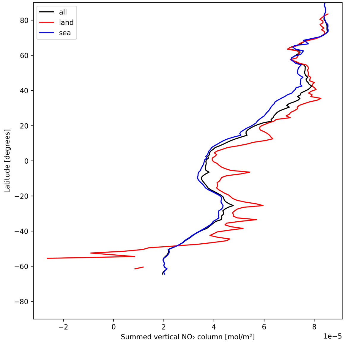
Figure 23: Zonal average of “Summed vertical NO 2 column” for 2025-06-17 to 2025-06-19.
