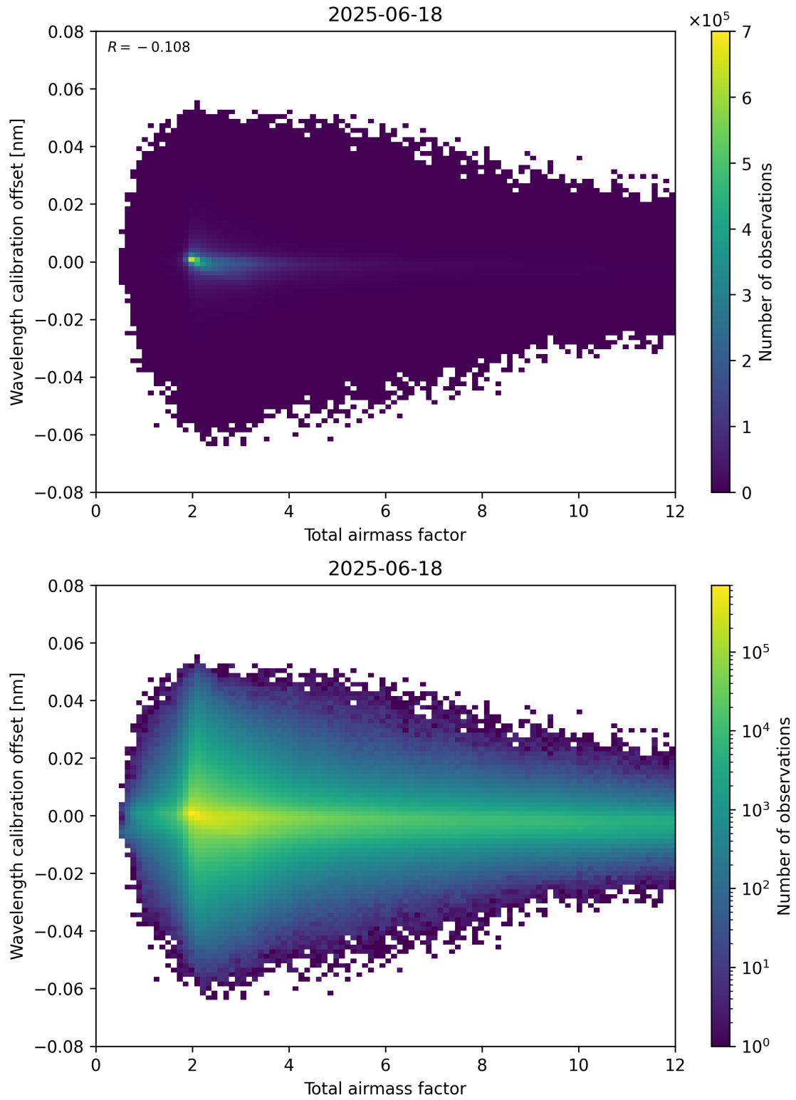
Figure 70: Scatter density plot of “Total airmass factor” against “Wavelength calibration offset” for 2025-06-17 to 2025-06-19.
