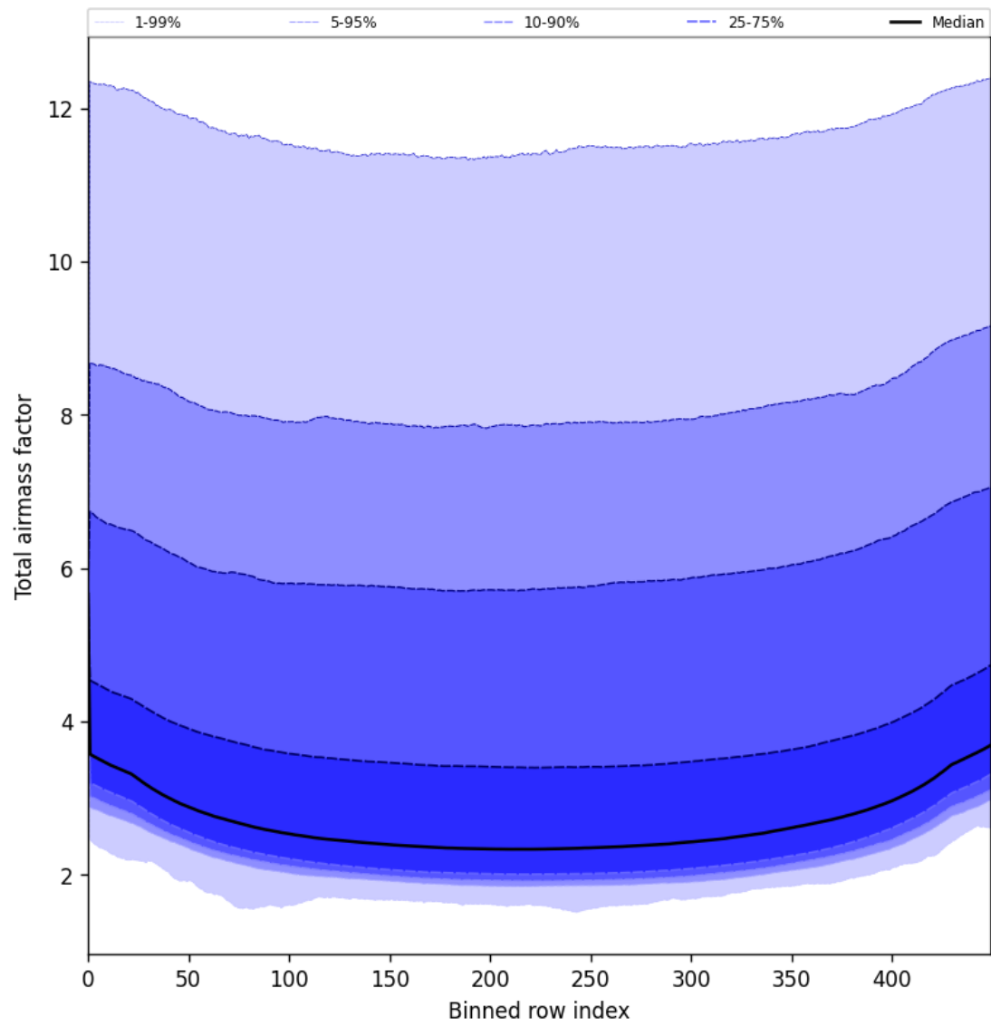
Figure 49: Along track statistics of “Total airmass factor” for 2025-06-17 to 2025-06-19
