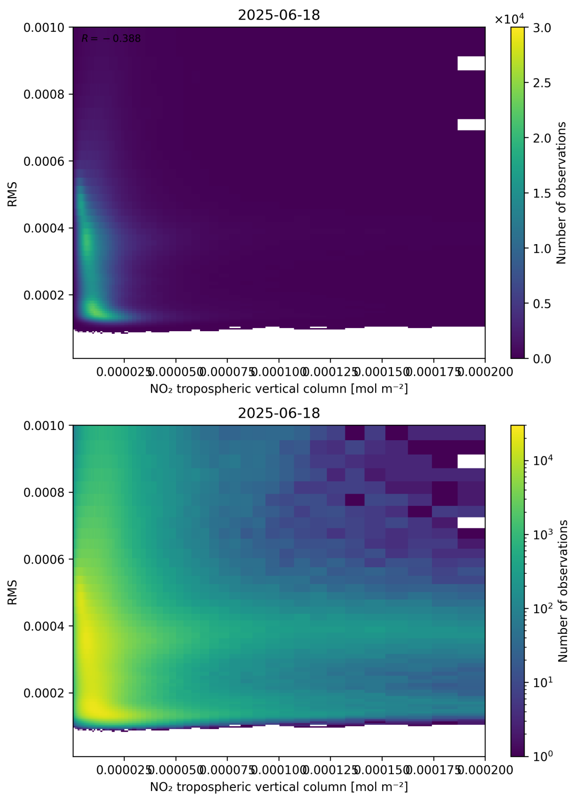
Figure 142: Scatter density plot of “NO 2 tropospheric vertical column” against “RMS” for 2025-06-17 to 2025-06-19.
