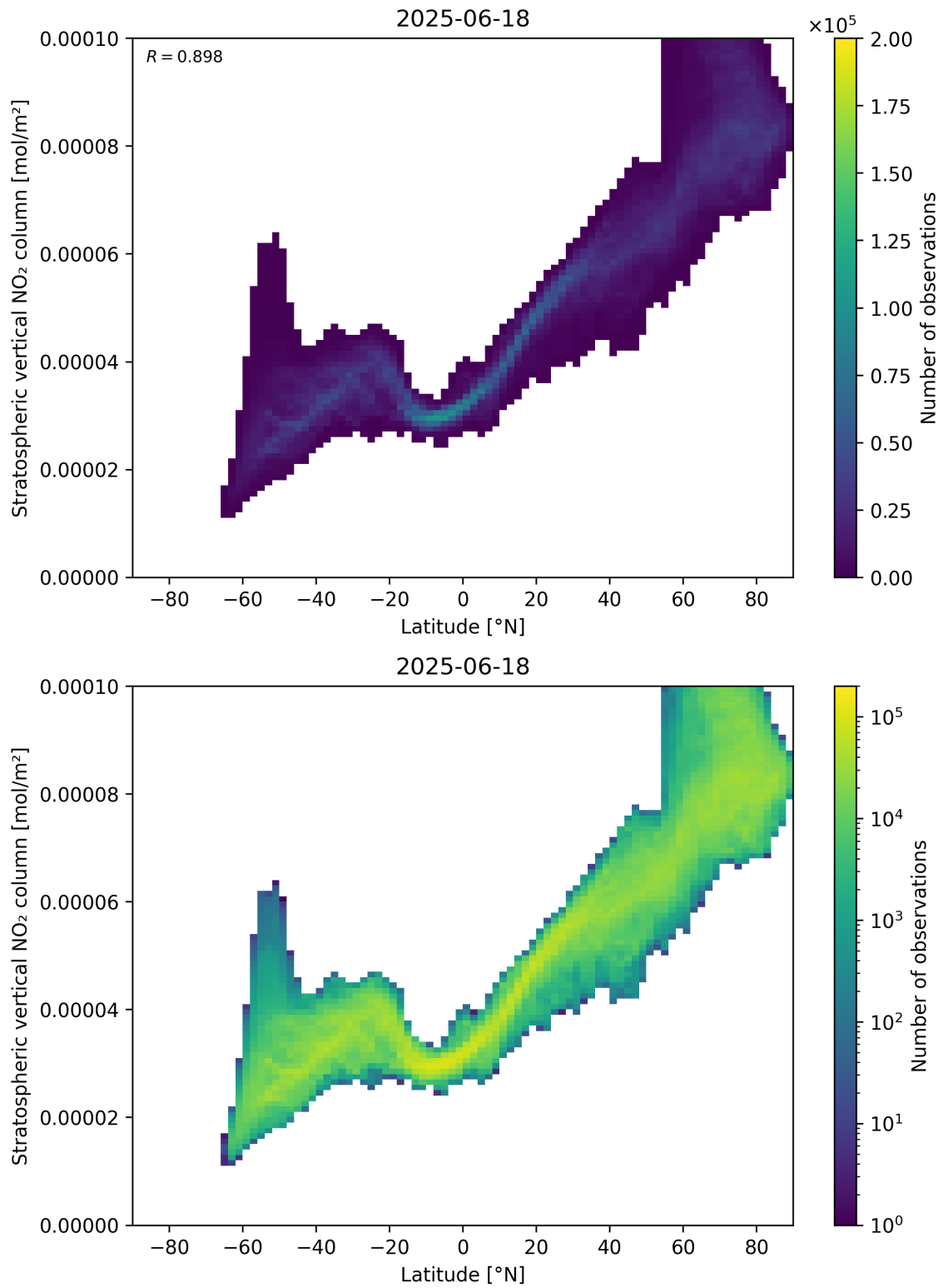
Figure 87: Scatter density plot of “Latitude” against “Stratospheric vertical NO 2 column” for 2025-06-17 to 2025-06-19.
