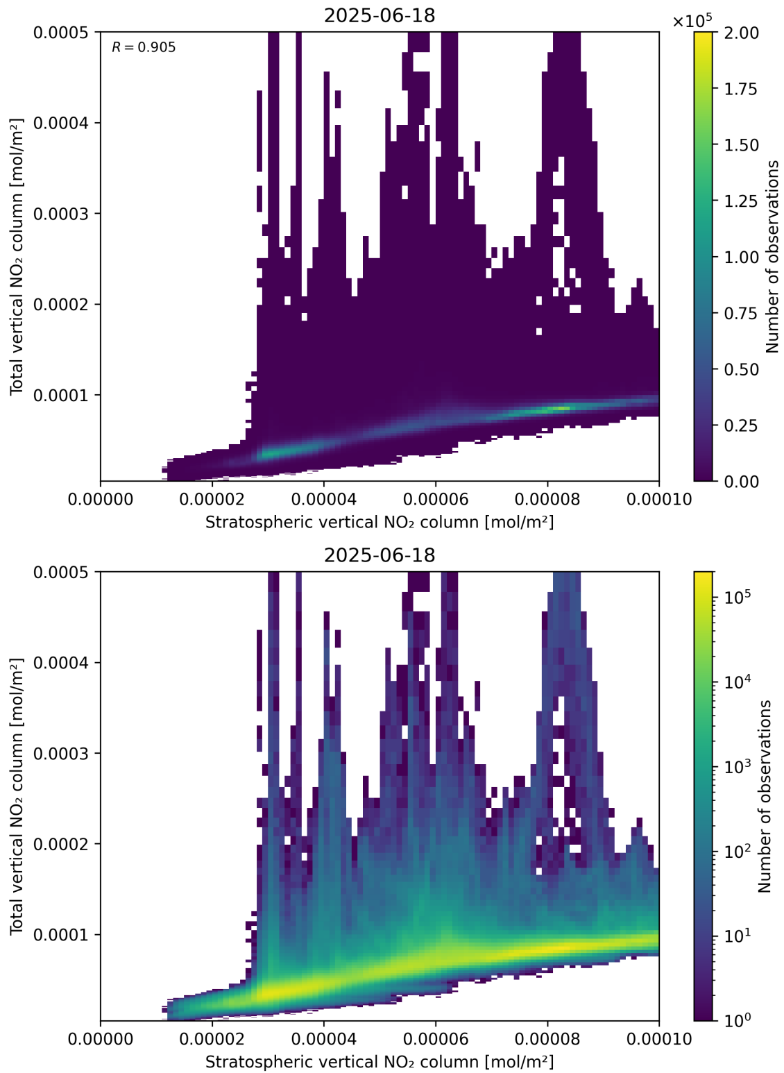
Figure 100: Scatter density plot of “Stratospheric vertical NO 2 column” against “Total vertical NO 2 column” for 2025-06-17 to 2025-06-19.
