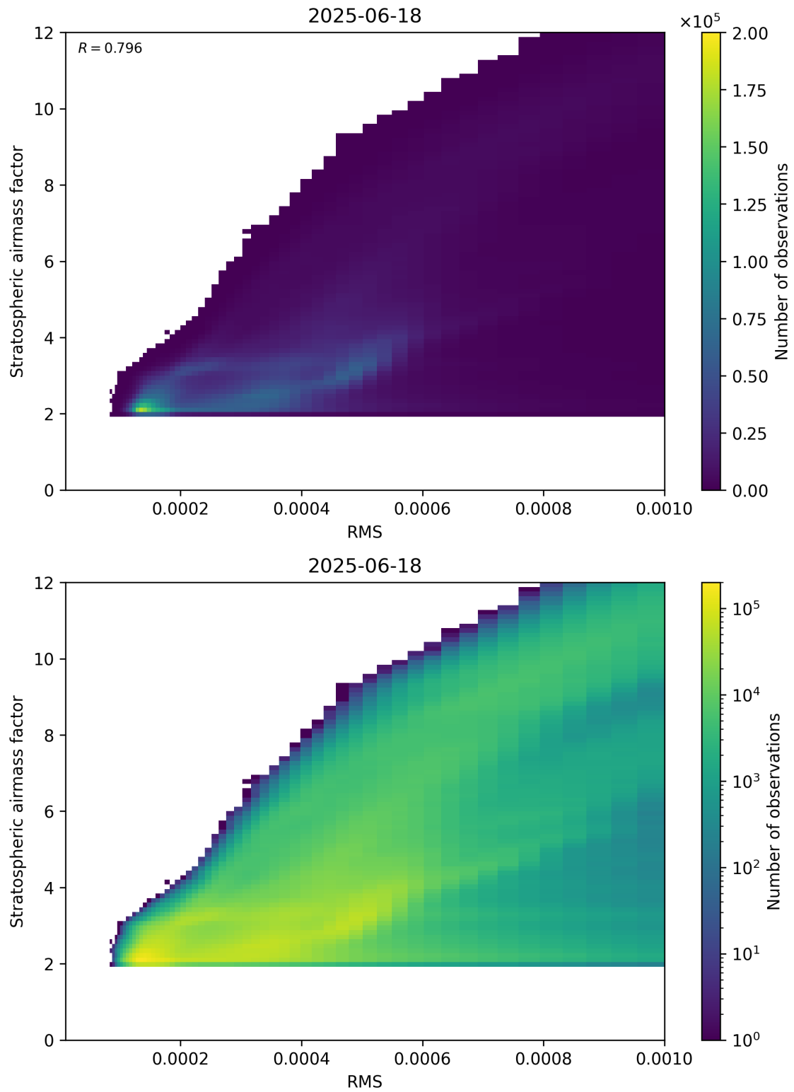
Figure 144: Scatter density plot of “RMS” against “Stratospheric airmass factor” for 2025-06-17 to 2025-06-19.
