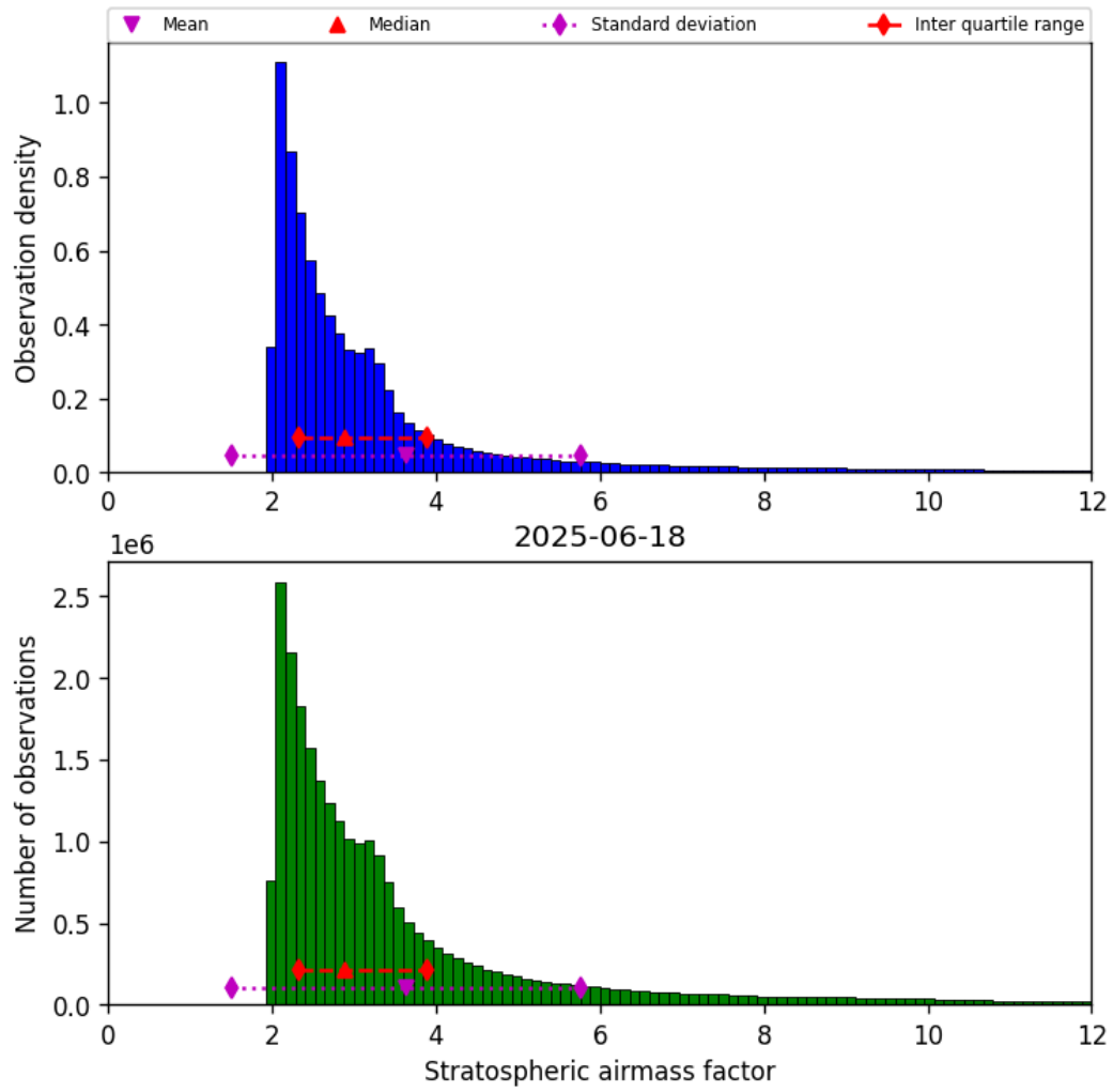
Figure 44: Histogram of “Stratospheric airmass factor” for 2025-06-17 to 2025-06-19
