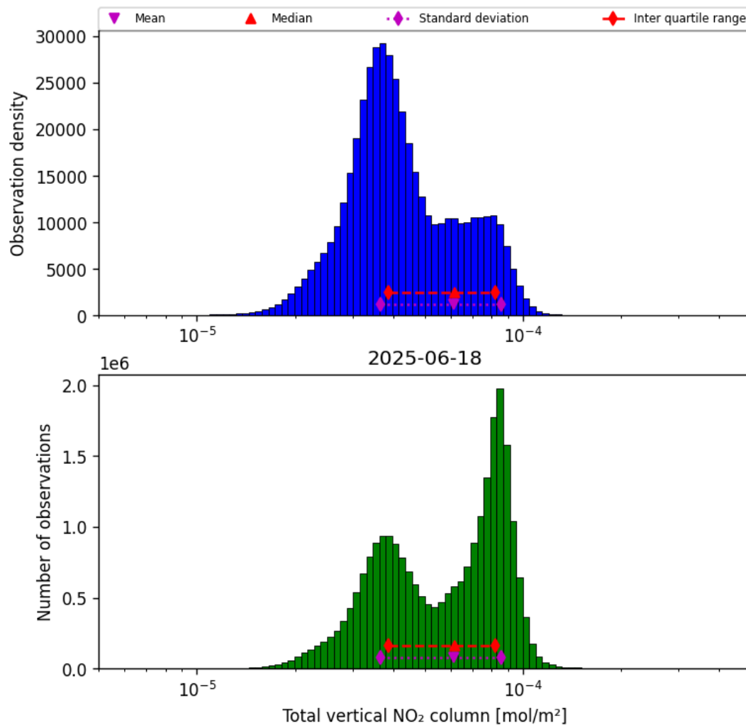
Figure 38: Histogram of “Total vertical NO 2 column” for 2025-06-17 to 2025-06-19
