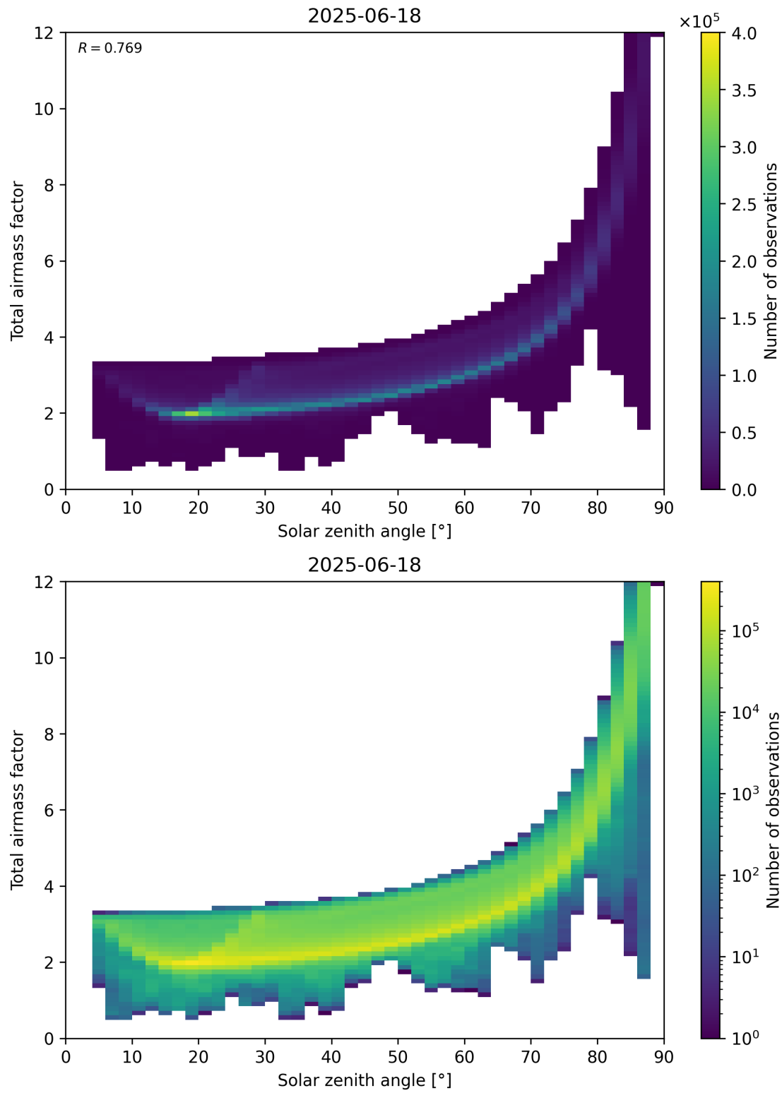
Figure 146: Scatter density plot of “Solar zenith angle” against “Total air mass factor” for 2025-06-17 to 2025-06-19.
