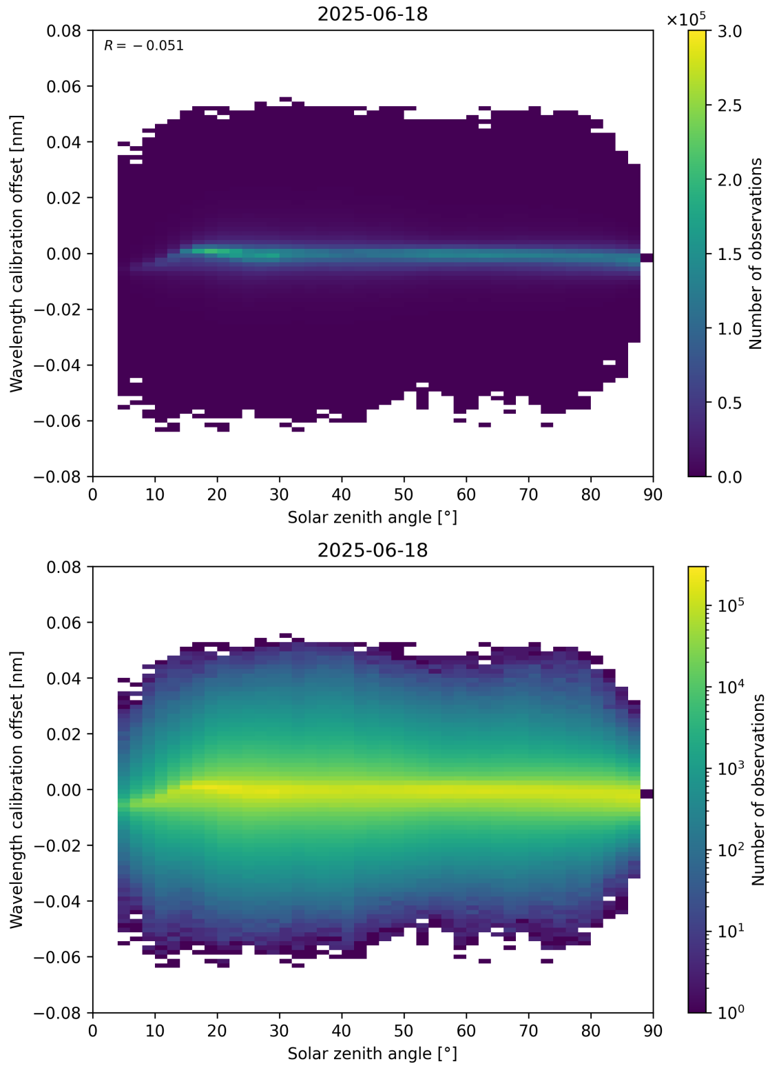
Figure 158: Scatter density plot of “Solar zenith angle” against “Wavelength calibration offset” for 2025-06-17 to 2025-06-19.
