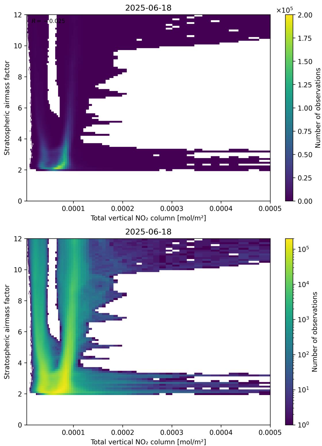
Figure 110: Scatter density plot of “Total vertical NO 2 column” against “Stratospheric airmass factor” for 2025-06-17 to 2025-06-19.
