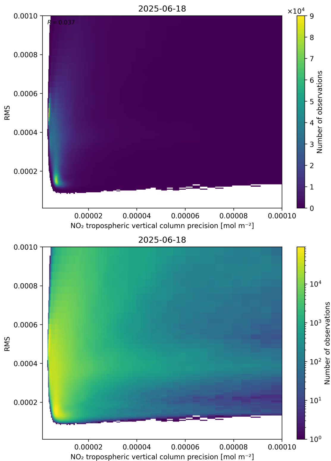
Figure 140: Scatter density plot of “NO 2 tropospheric vertical column precision” against “RMS” for 2025-06-17 to 2025-06-19.
