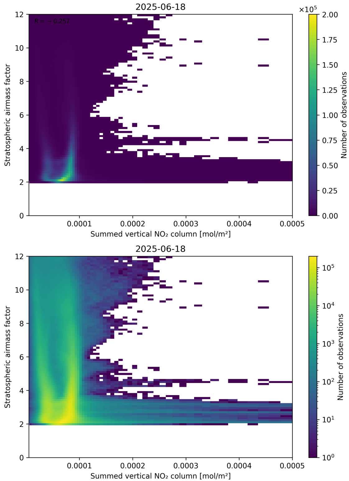
Figure 103: Scatter density plot of “Summed vertical NO 2 column” against “Stratospheric airmass factor” for 2025-06-17 to 2025-06-19.
