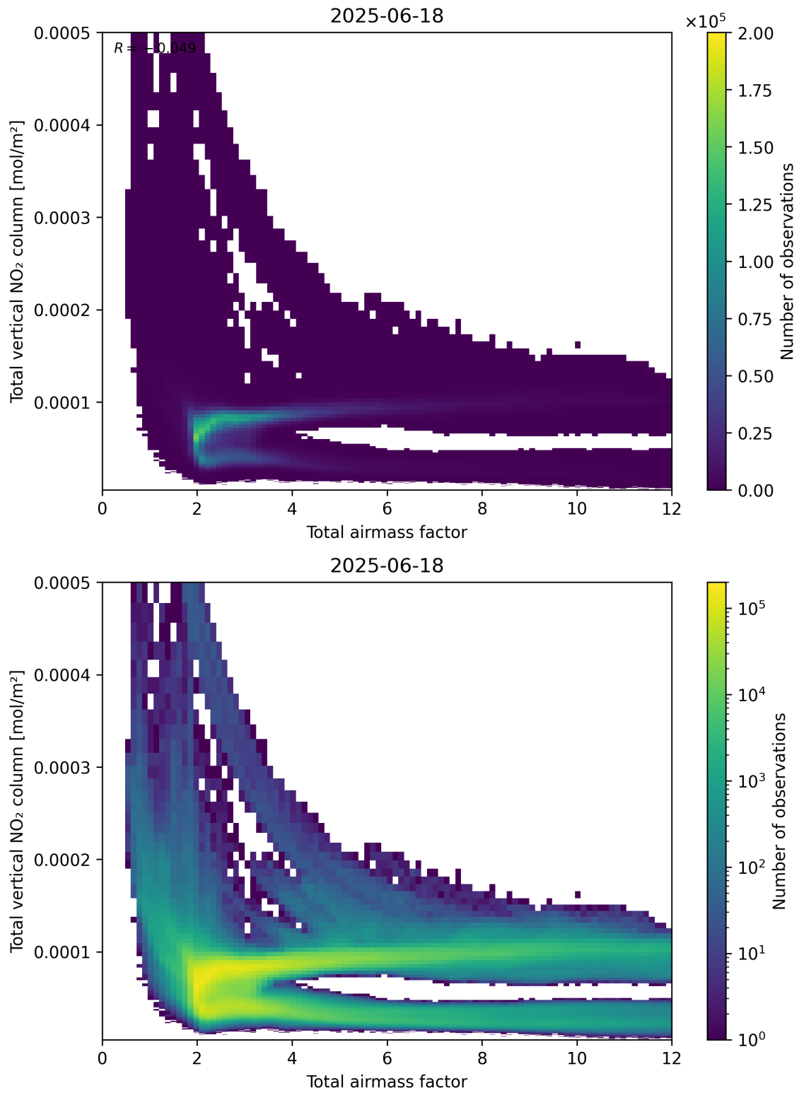
Figure 67: Scatter density plot of “Total airmass factor” against “Total vertical NO 2 column” for 2025-06-17 to 2025-06-19.
