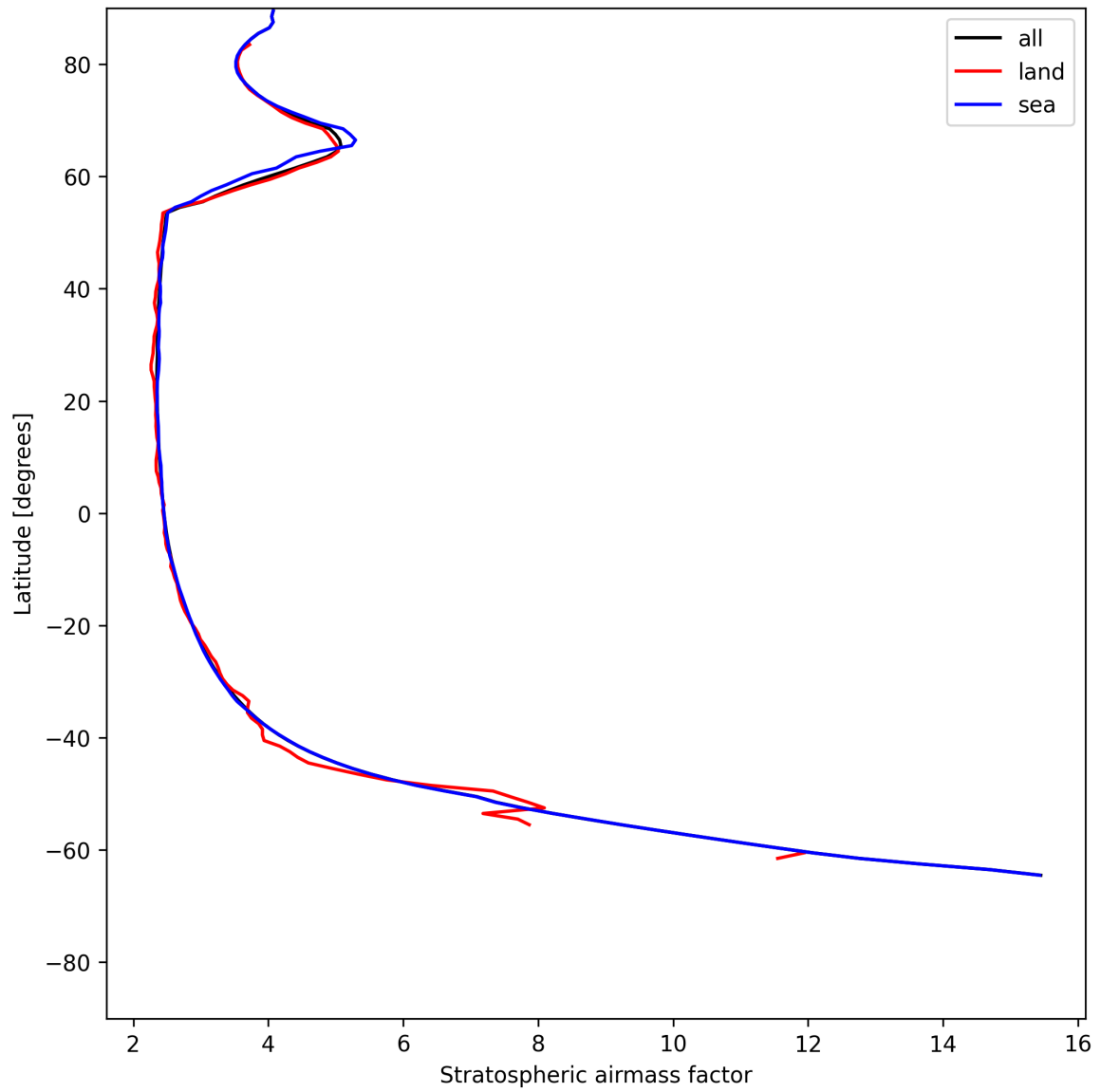
Figure 27: Zonal average of “Stratospheric airmass factor” for 2025-06-17 to 2025-06-19.
