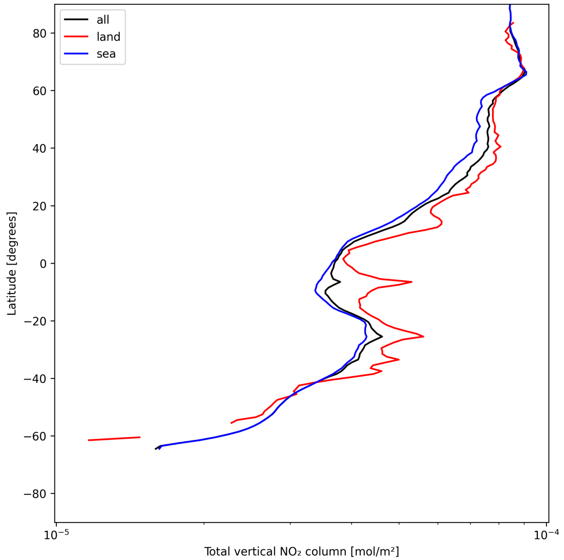
Figure 21: Zonal average of “Total vertical NO 2 column” for 2025-06-17 to 2025-06-19.
