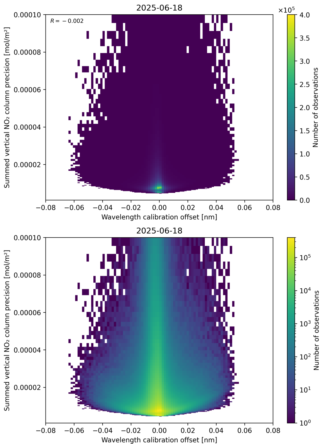
Figure 178: Scatter density plot of “Wavelength calibration offset” against “Summed vertical NO 2 column precision” for 2025-06-17 to 2025-06-19.
