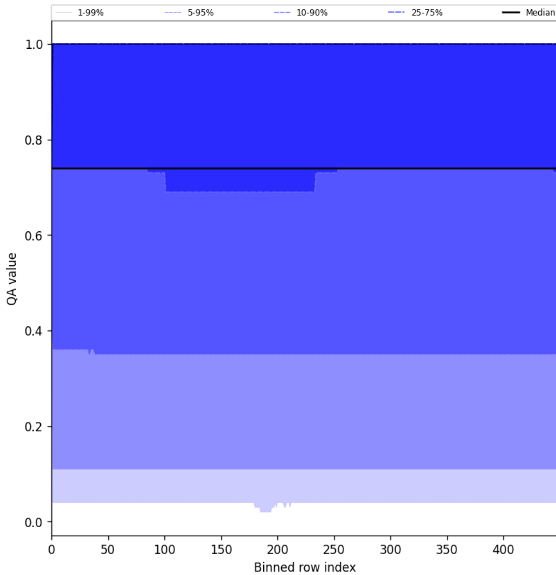
Figure 45: Along track statistics of “QA value” for 2025-06-17 to 2025-06-19
