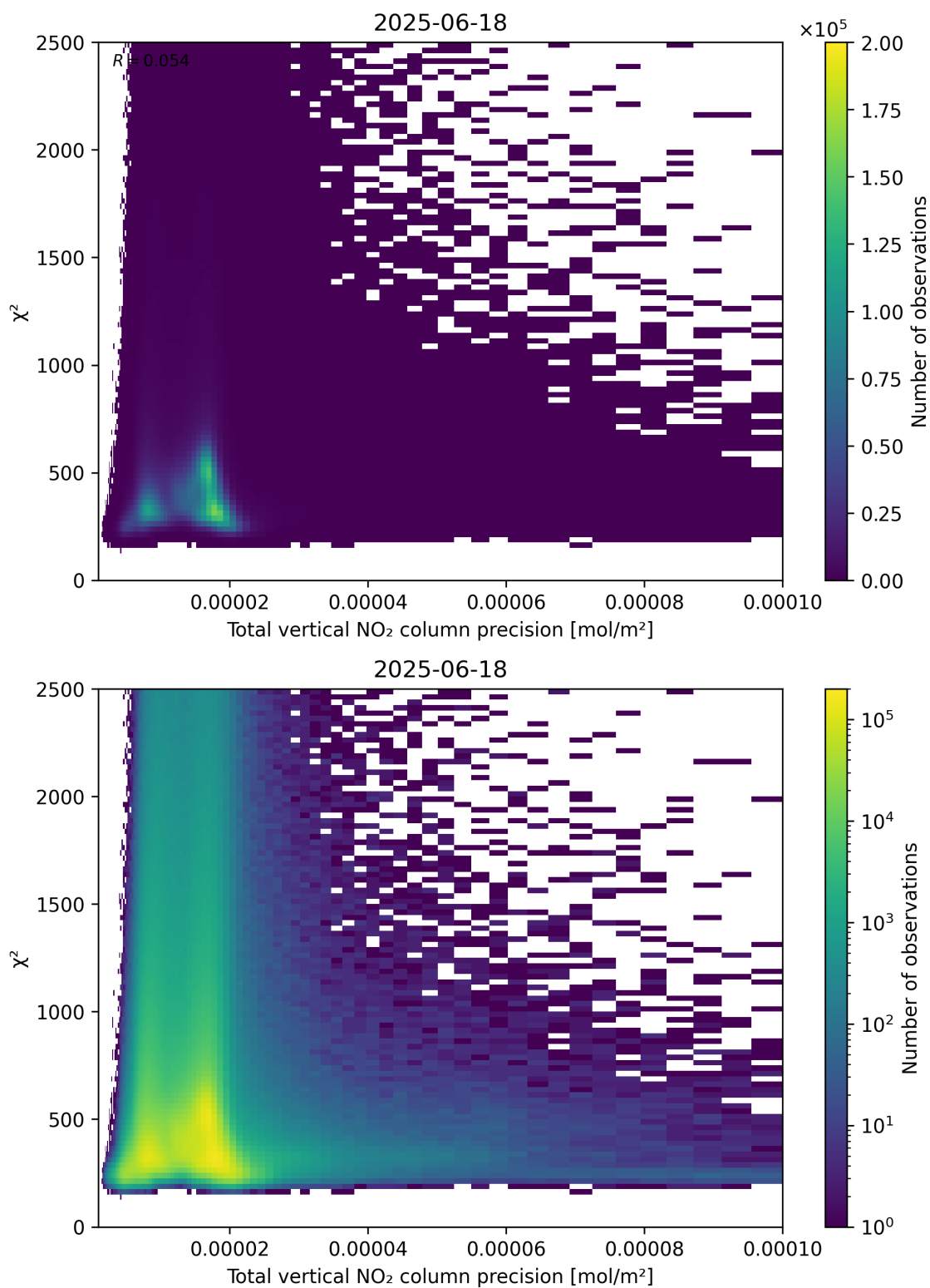
Figure 116: Scatter density plot of “Total vertical NO 2 column precision” against “ \chi^2 ” for 2025-06-17 to 2025-06-19.
