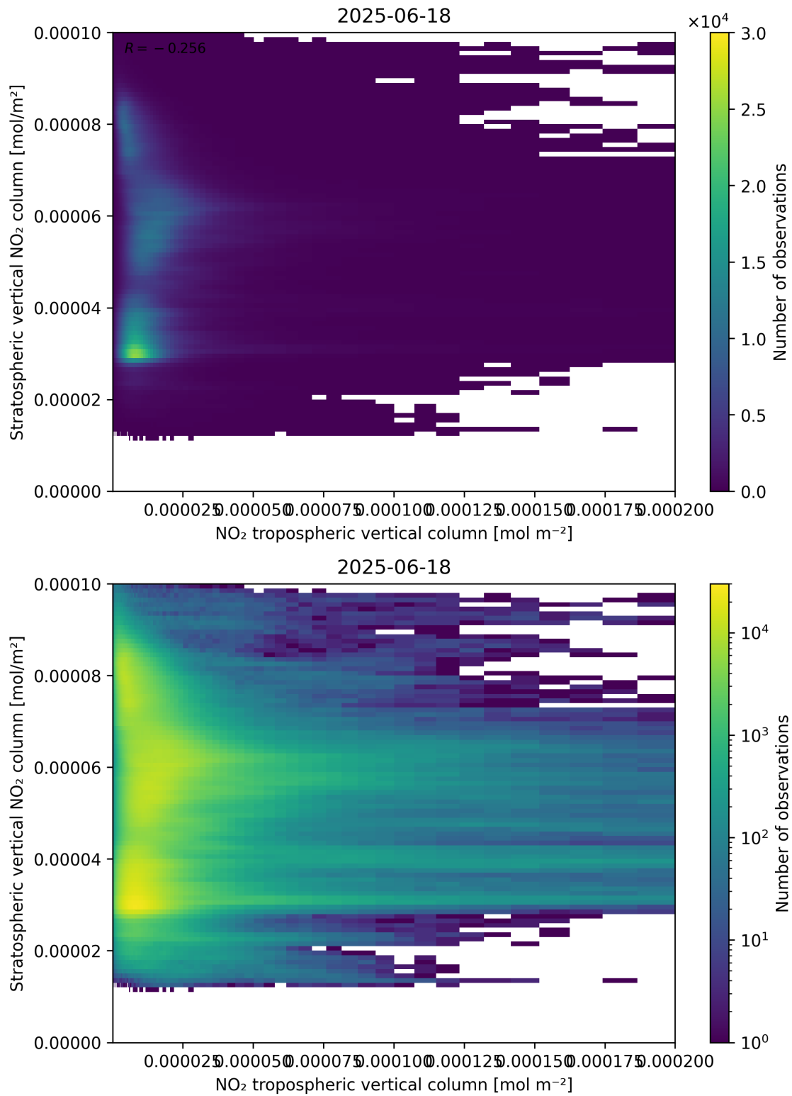
Figure 125: Scatter density plot of “NO 2 tropospheric vertical column” against “Stratospheric vertical NO 2 column” for 2025-06-17 to 2025-06-19.
