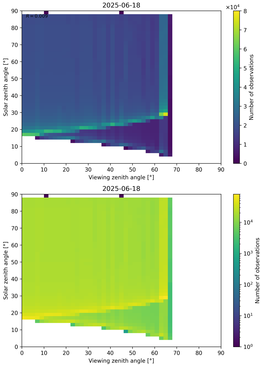
Figure 172: Scatter density plot of “Viewing zenith angle” against “Solar zenith angle” for 2025-06-17 to 2025-06-19.
