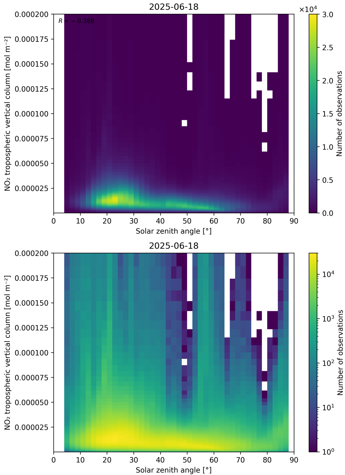
Figure 155: Scatter density plot of “Solar zenith angle” against “NO 2 tropospheric vertical column” for 2025-06-17 to 2025-06-19.
