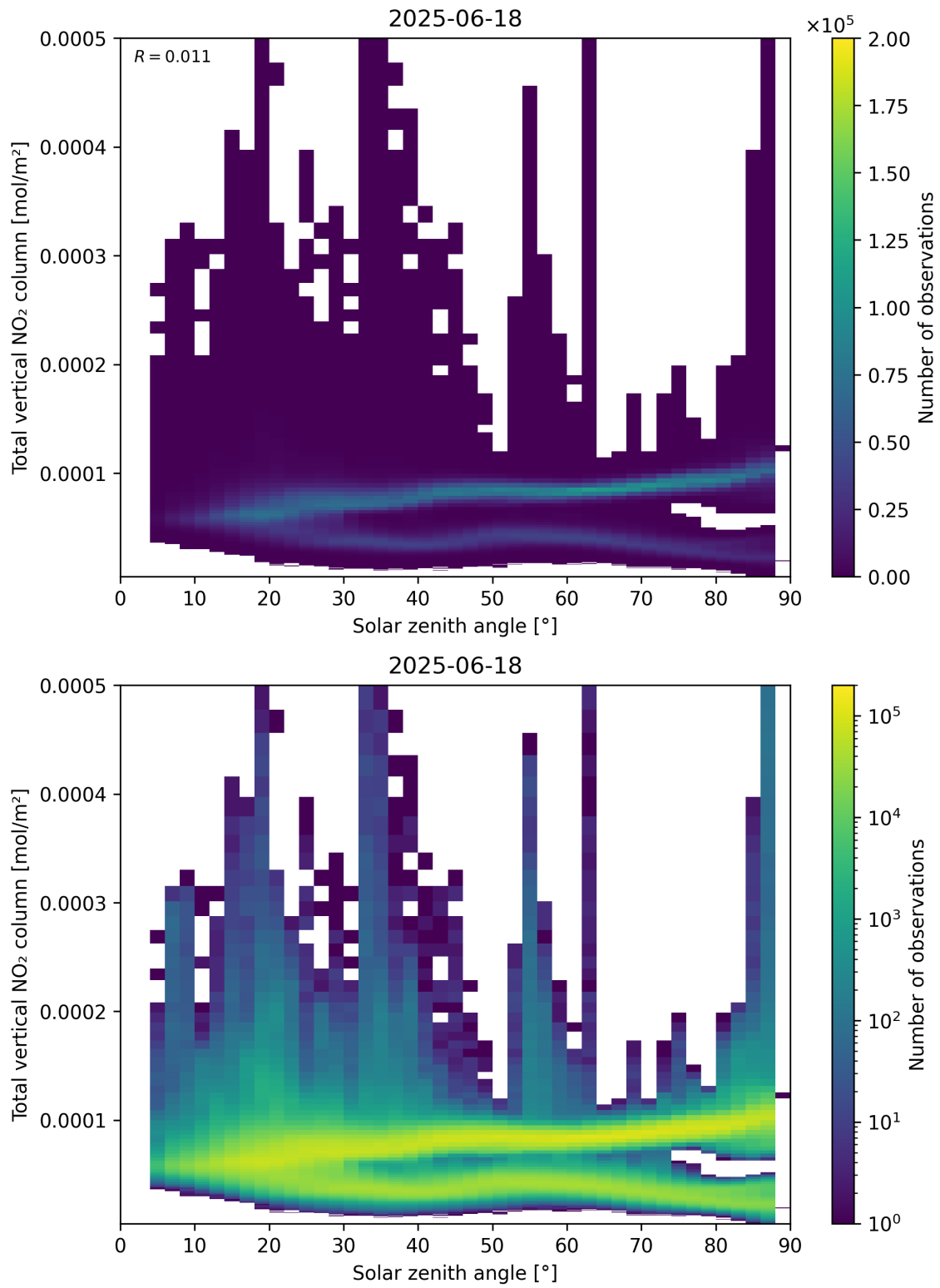
Figure 153: Scatter density plot of “Solar zenith angle” against “Total vertical NO 2 column” for 2025-06-17 to 2025-06-19.
