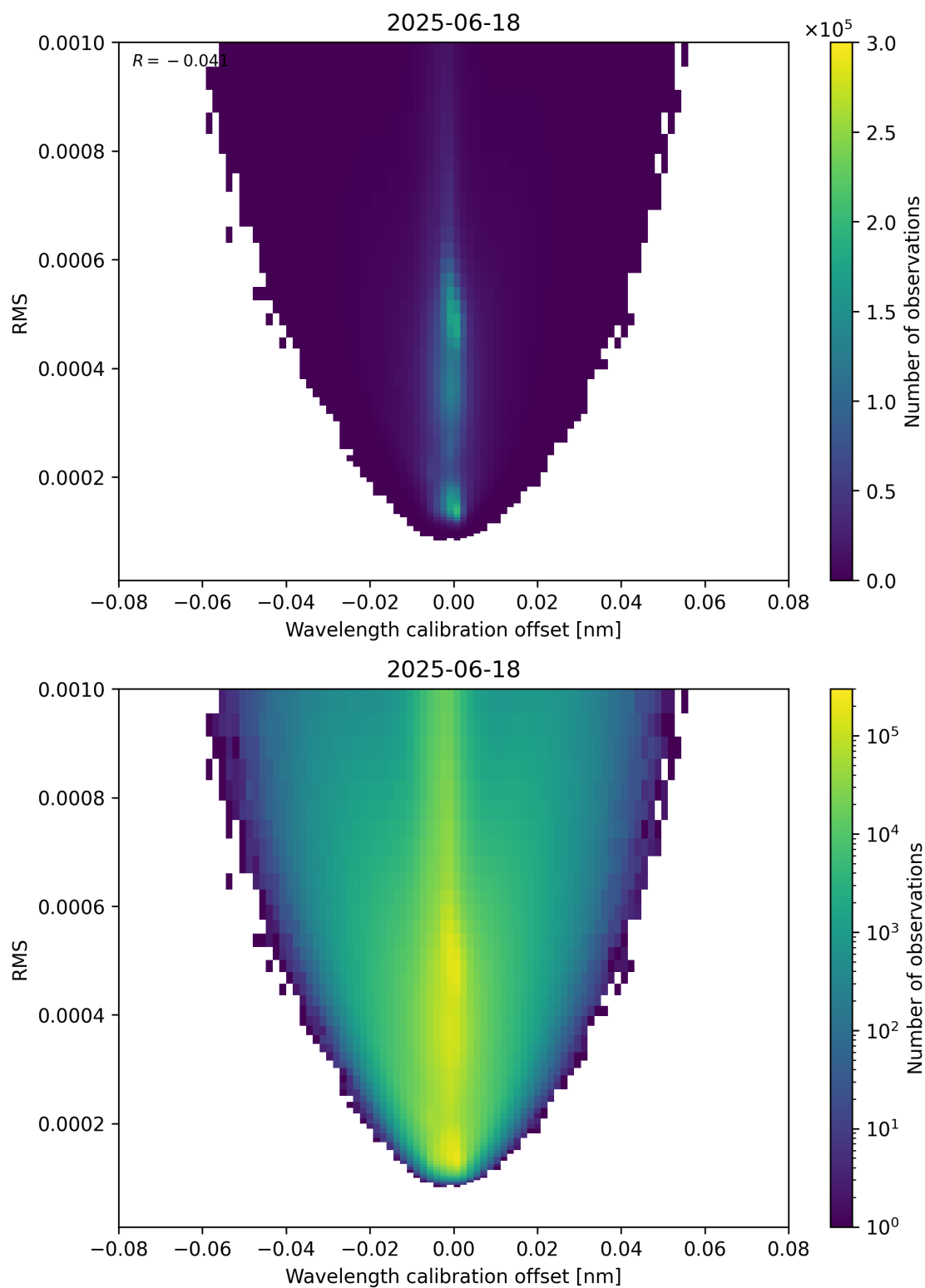
Figure 181: Scatter density plot of “Wavelength calibration offset” against “RMS” for 2025-06-17 to 2025-06-19.
