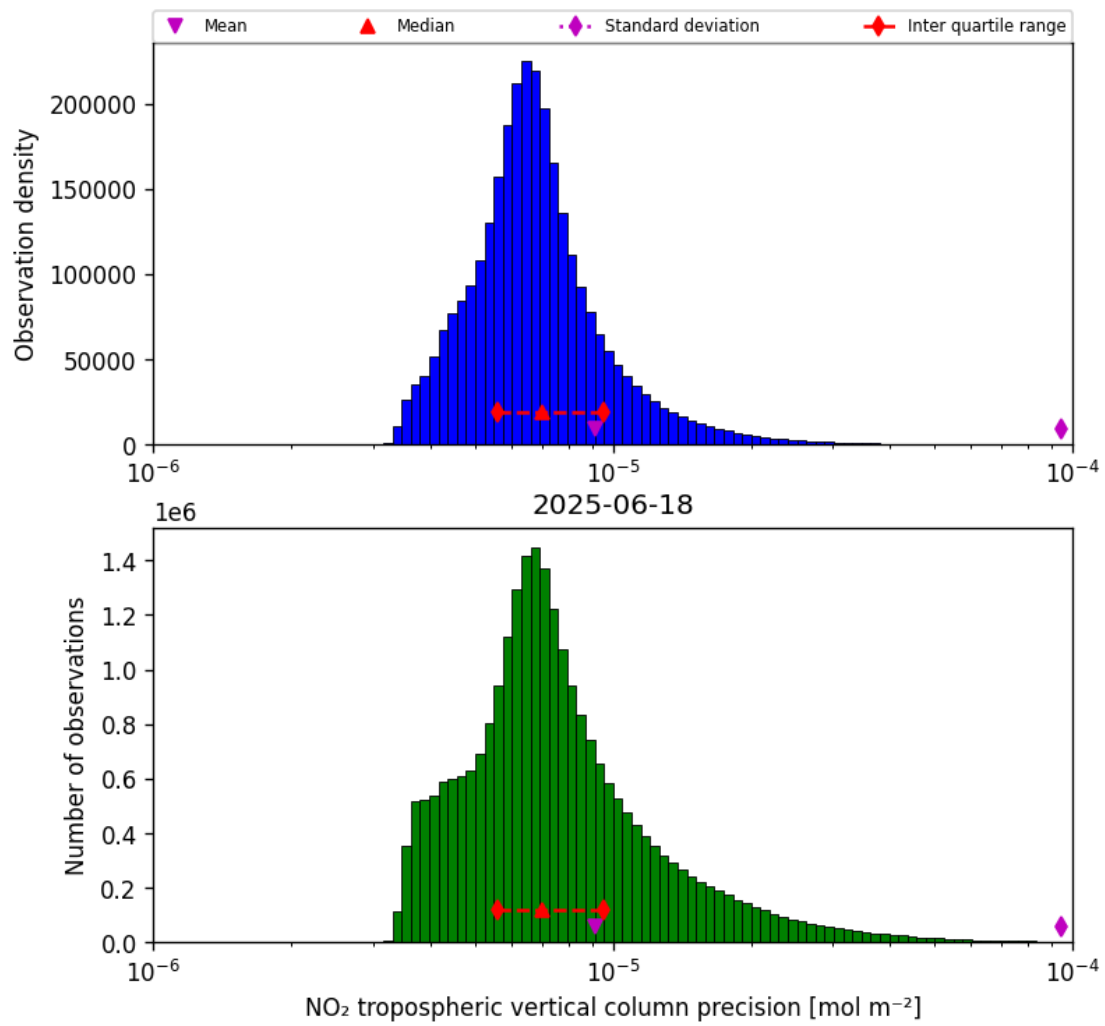
Figure 30: Histogram of “NO 2 tropospheric vertical column precision” for 2025-06-17 to 2025-06-19
