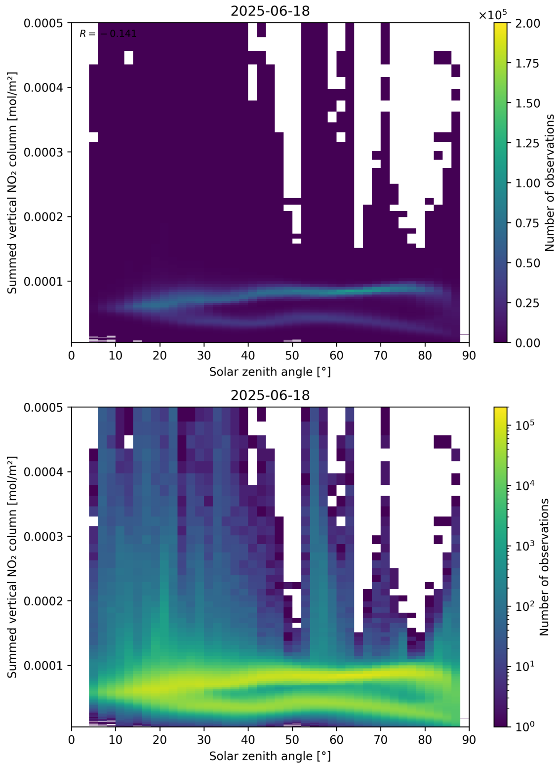
Figure 151: Scatter density plot of “Solar zenith angle” against “Summed vertical NO 2 column” for 2025-06-17 to 2025-06-19.
