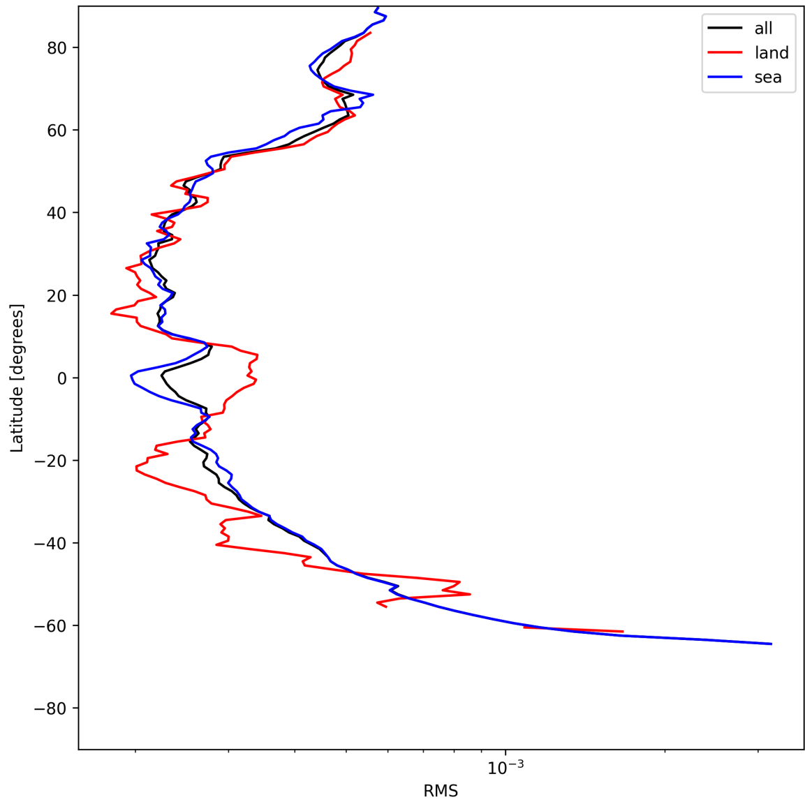
Figure 26: Zonal average of “RMS” for 2025-06-17 to 2025-06-19.
