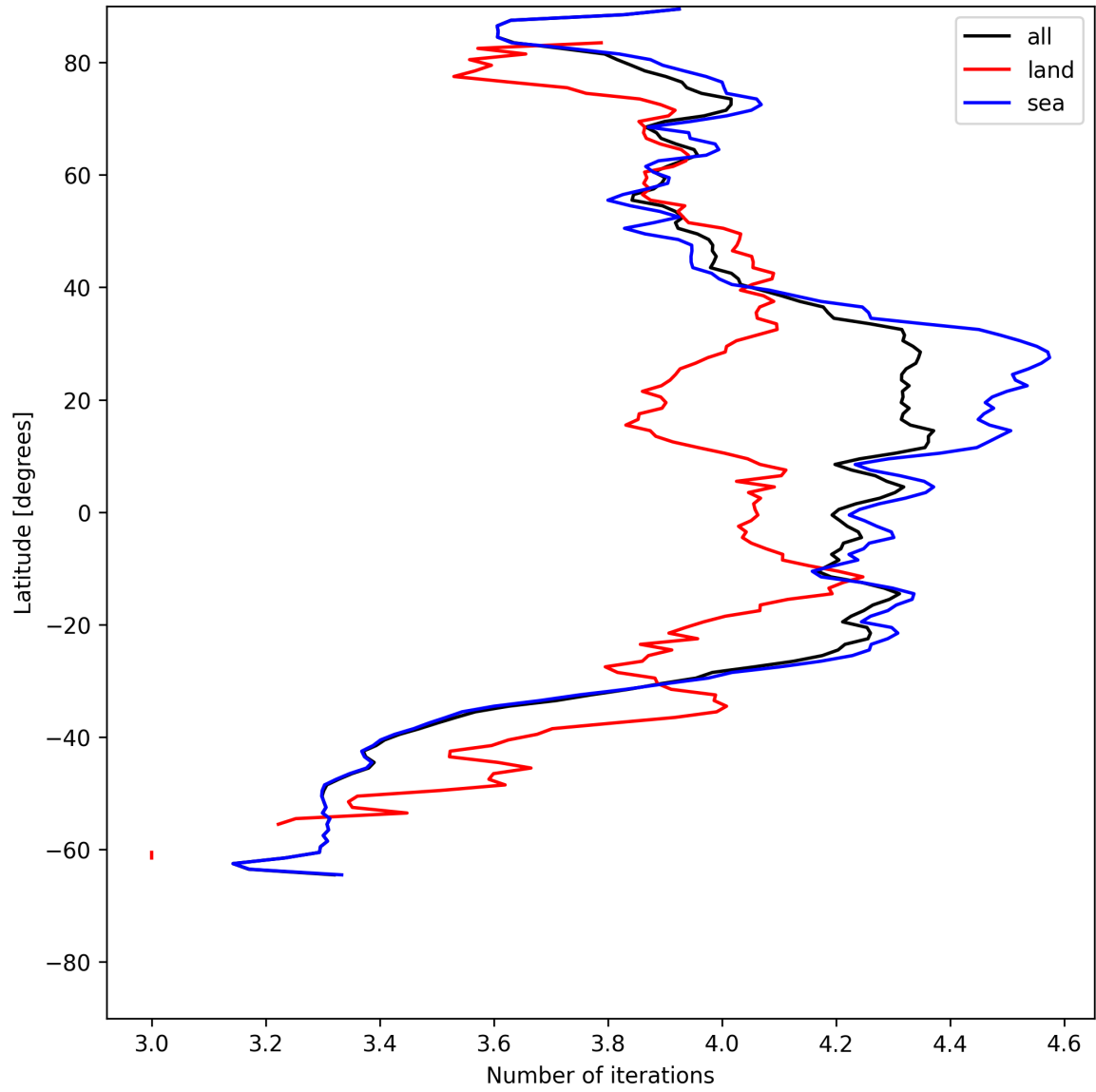
Figure 17: Zonal average of “Number of iterations” for 2025-06-17 to 2025-06-19.
