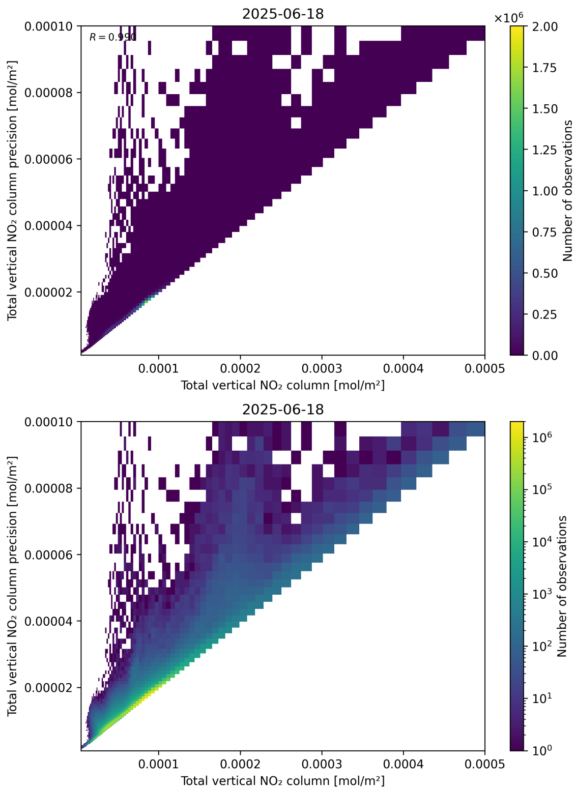
Figure 114: Scatter density plot of “Total vertical NO 2 column” against “Total vertical NO 2 column precision” for 2025-06-17 to 2025-06-19.
