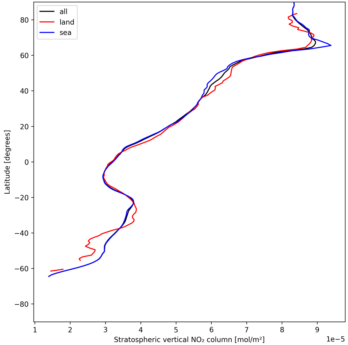
Figure 19: Zonal average of “Stratospheric vertical NO 2 column” for 2025-06-17 to 2025-06-19.
