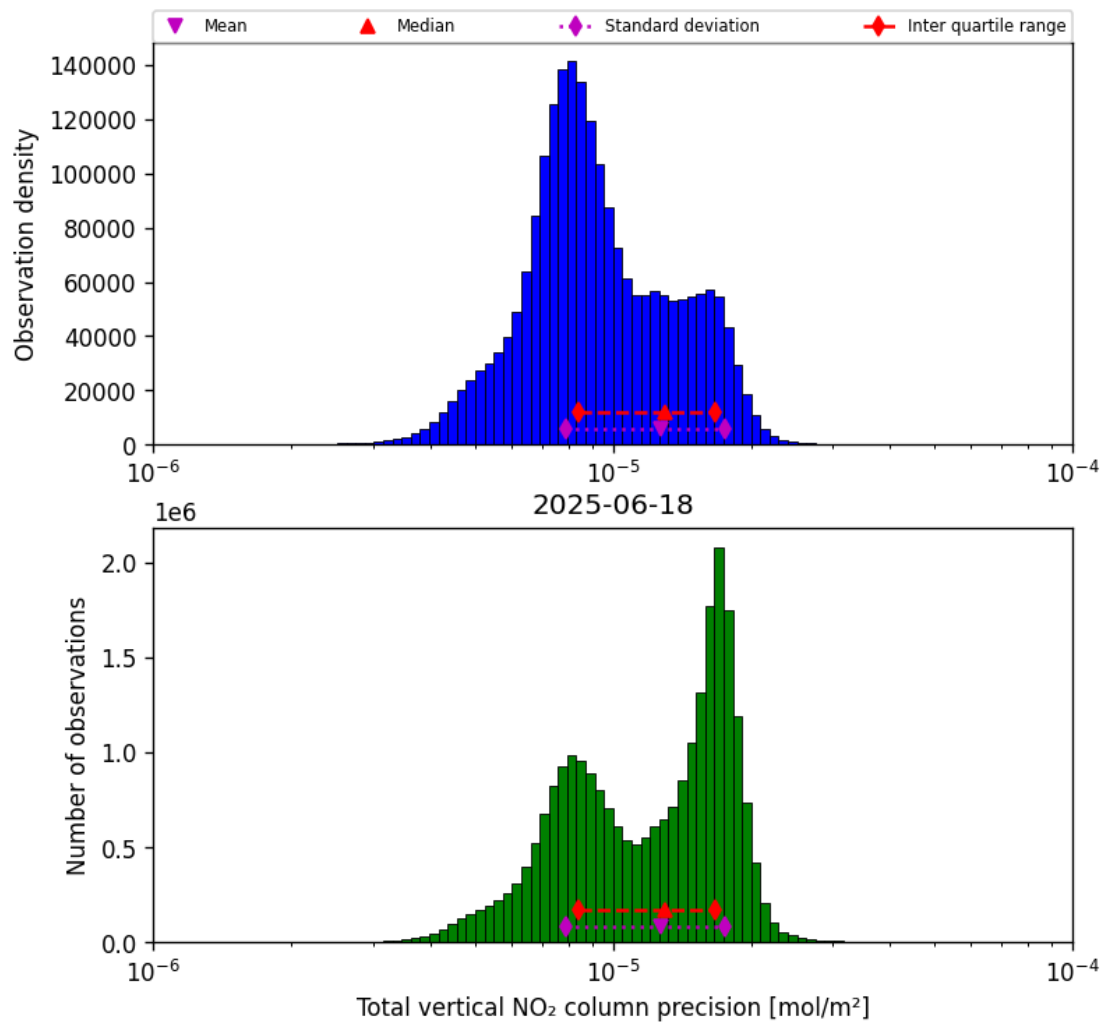
Figure 39: Histogram of “Total vertical NO 2 column precision” for 2025-06-17 to 2025-06-19
