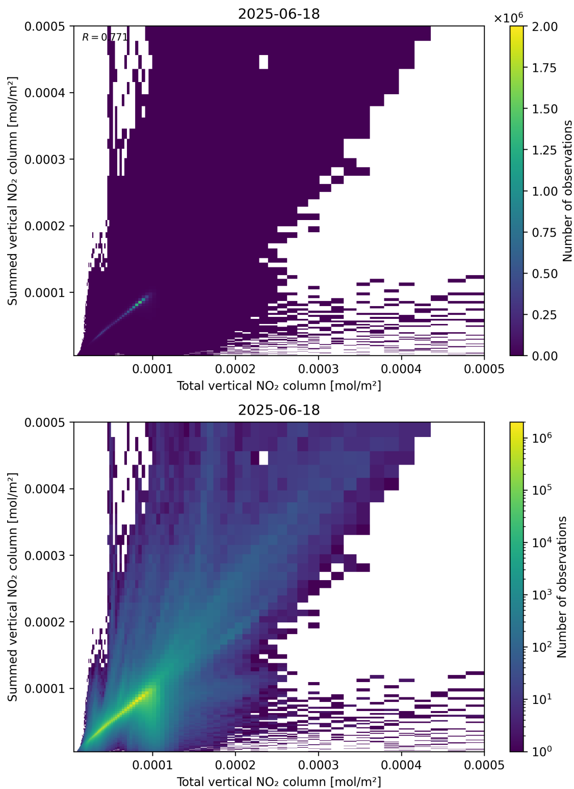
Figure 112: Scatter density plot of “Total vertical NO 2 column” against “Summed vertical NO 2 column” for 2025-06-17 to 2025-06-19.
