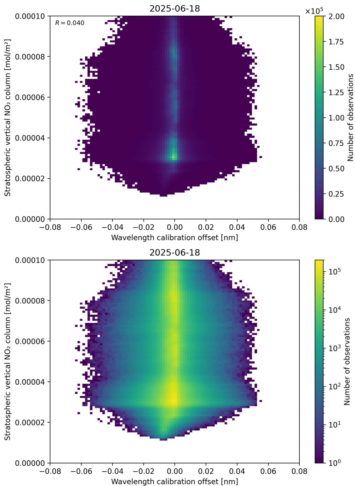
Figure 176: Scatter density plot of “Wavelength calibration offset” against “Stratospheric vertical NO 2 column” for 2025-06-17 to 2025-06-19.
