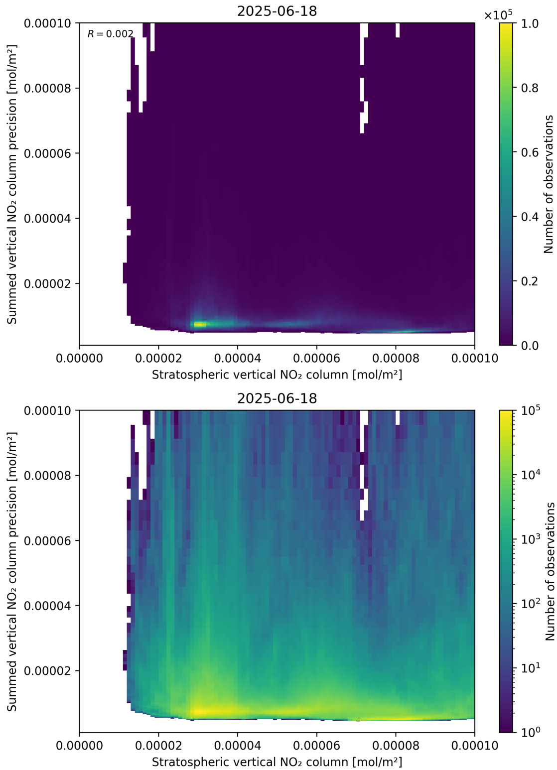
Figure 99: Scatter density plot of “Stratospheric vertical NO 2 column” against “Summed vertical NO 2 column precision” for 2025-06-17 to 2025-06-19.
