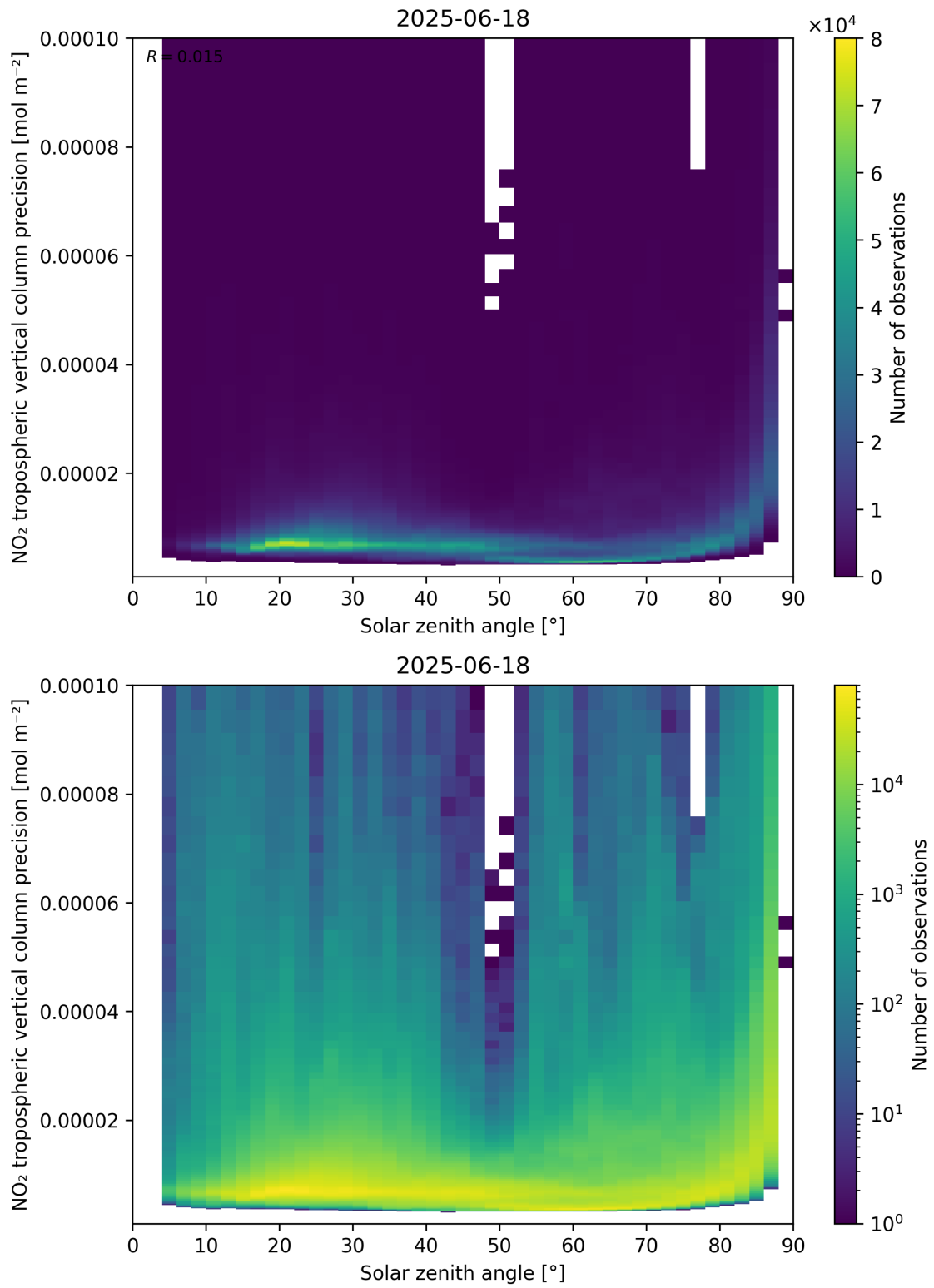
Figure 156: Scatter density plot of “Solar zenith angle” against “NO 2 tropospheric vertical column precision” for 2025-06-17 to 2025-06-19.
