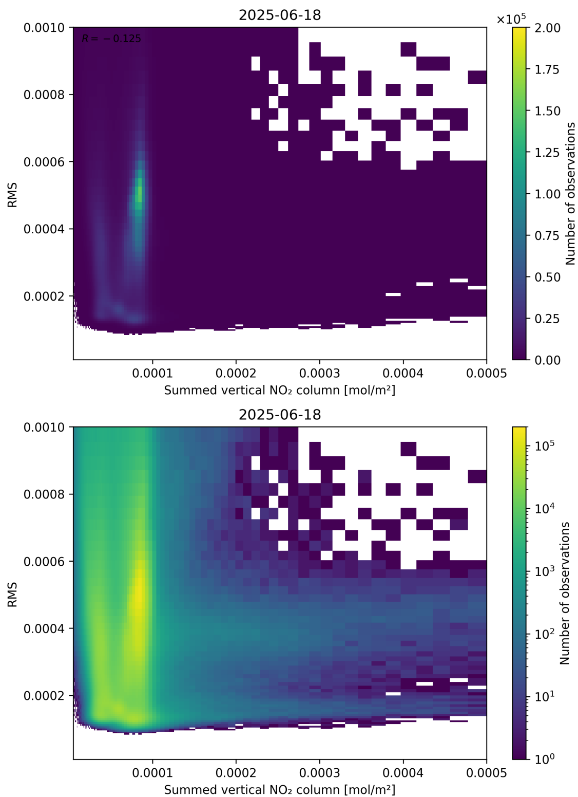
Figure 109: Scatter density plot of “Summed vertical NO 2 column” against “RMS” for 2025-06-17 to 2025-06-19.
