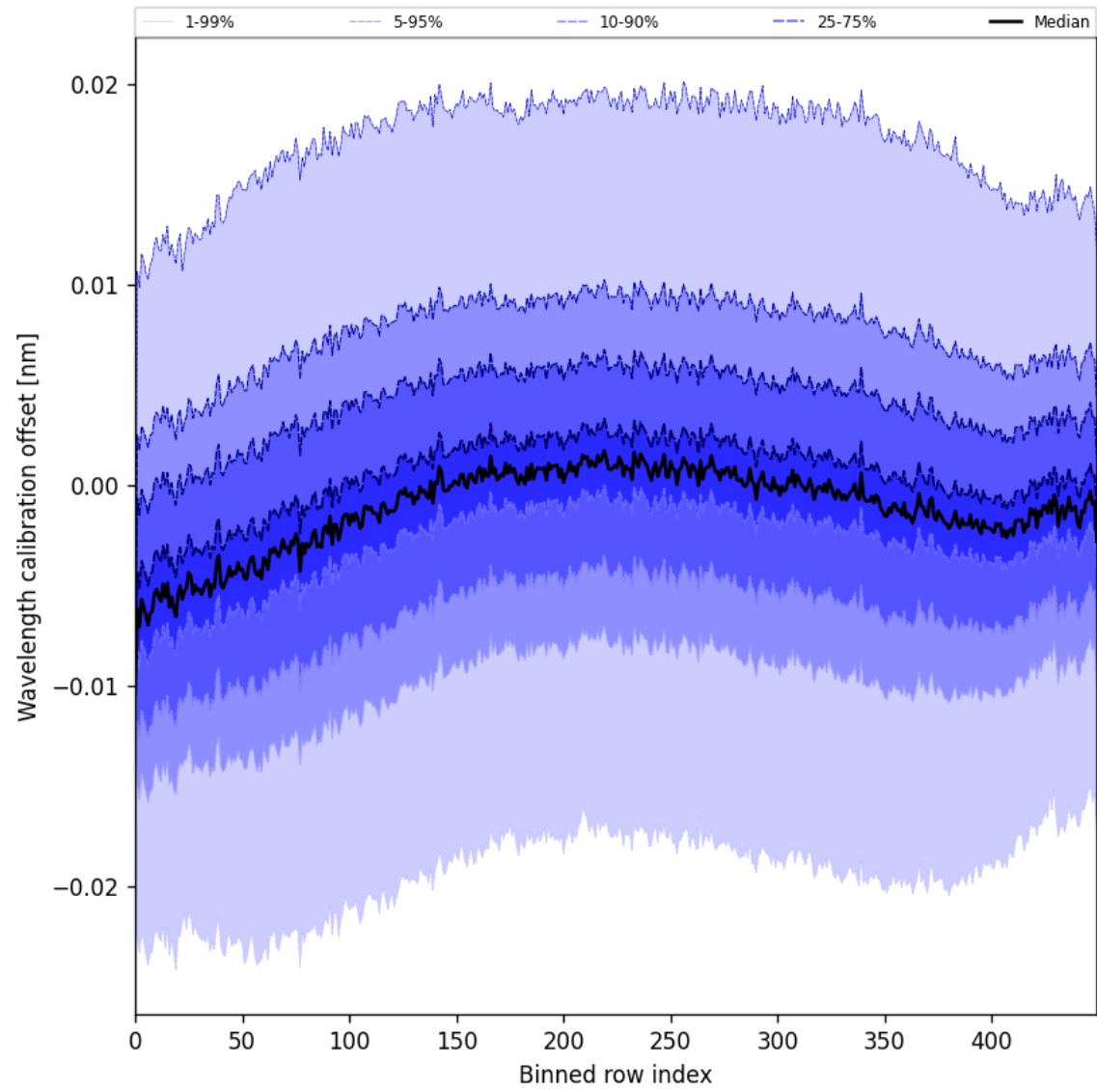
Figure 52: Along track statistics of “Wavelength calibration offset” for 2025-06-17 to 2025-06-19
