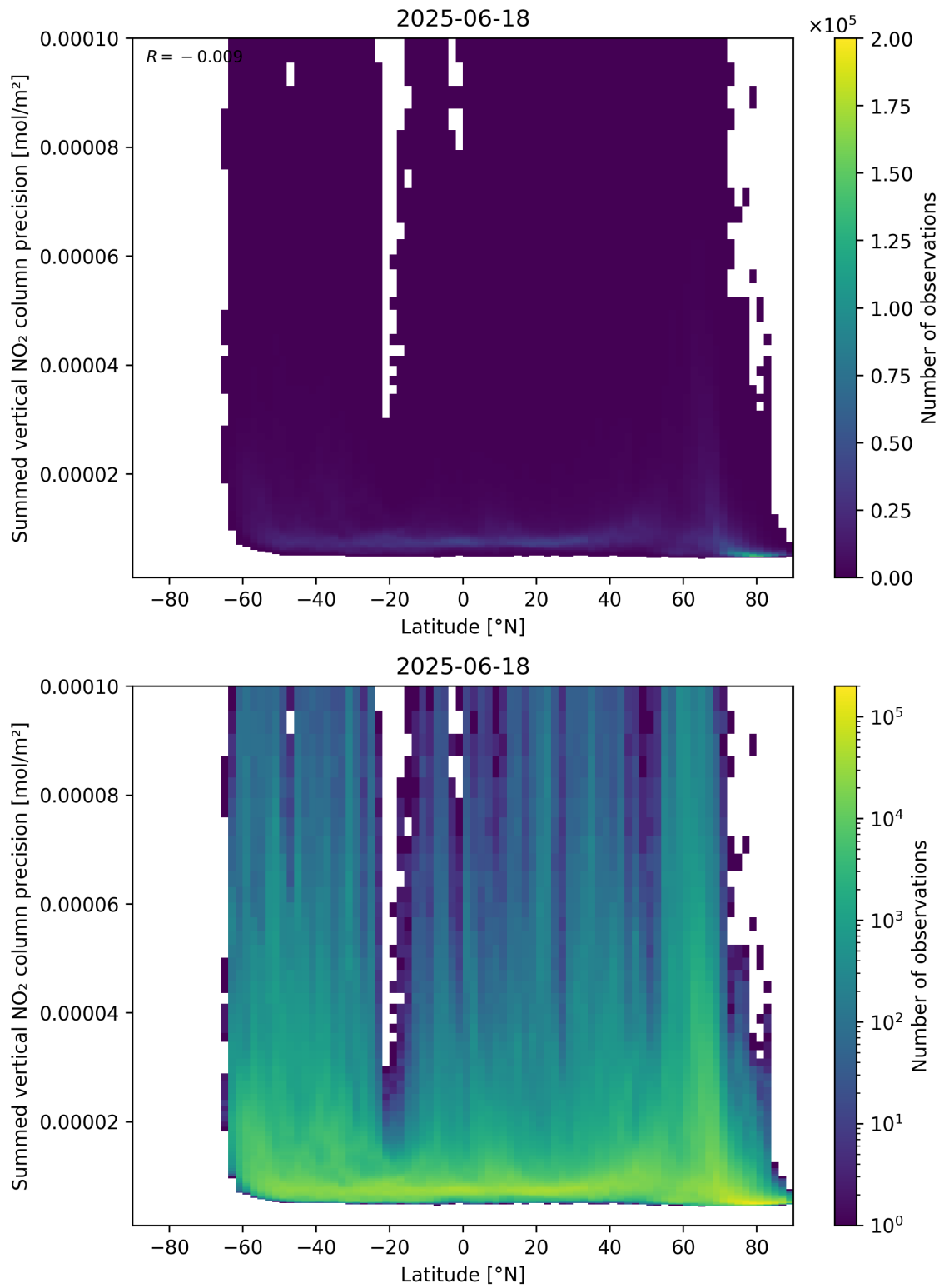
Figure 89: Scatter density plot of “Latitude” against “Summed vertical NO 2 column precision” for 2025-06-17 to 2025-06-19.
