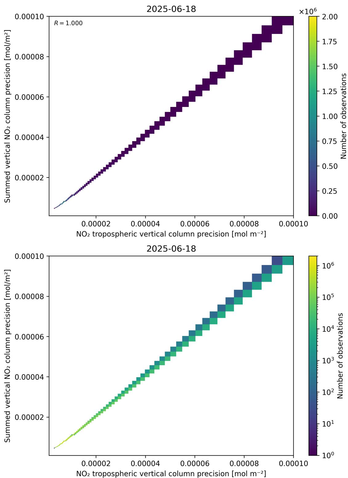
Figure 137: Scatter density plot of “NO 2 tropospheric vertical column precision” against “Summed vertical NO 2 column precision” for 2025-06-17 to 2025-06-19.
