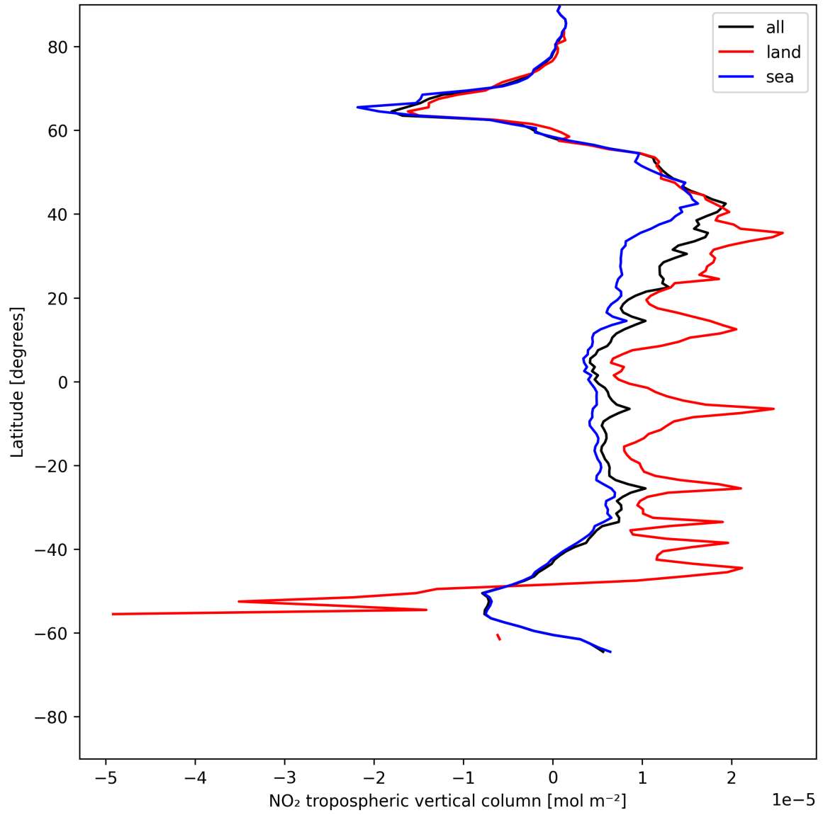
Figure 12: Zonal average of “NO 2 tropospheric vertical column” for 2025-06-17 to 2025-06-19.
