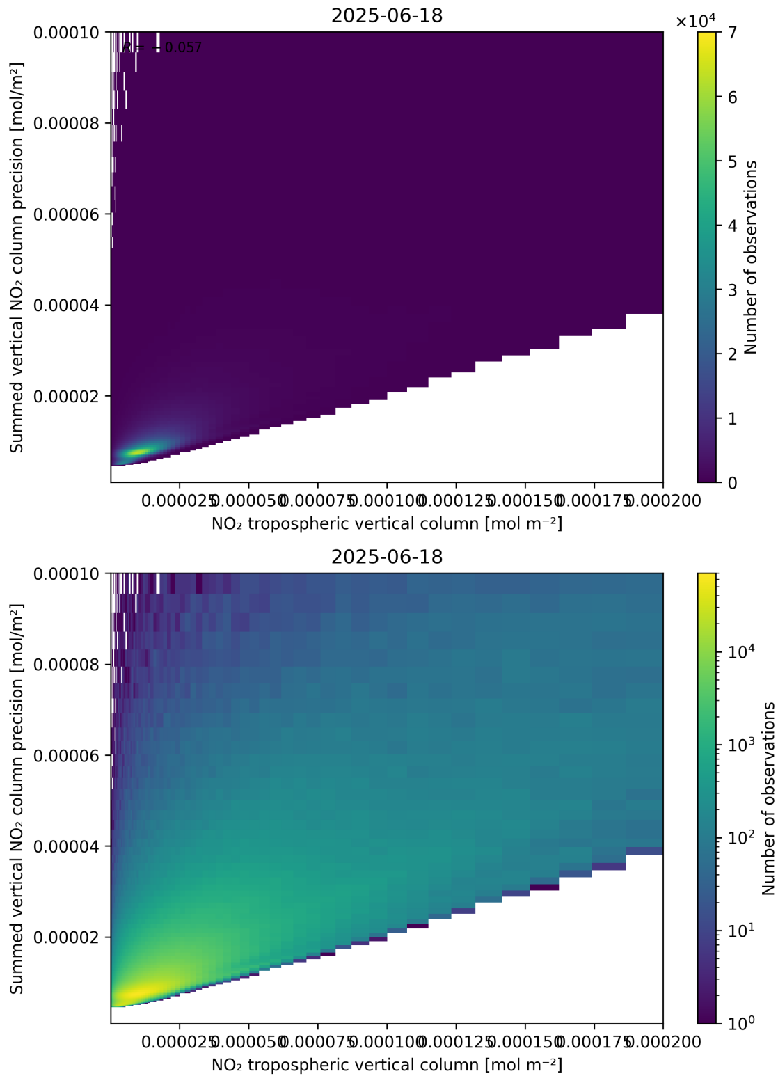
Figure 127: Scatter density plot of “NO 2 tropospheric vertical column” against “Summed vertical NO 2 column precision” for 2025-06-17 to 2025-06-19.
