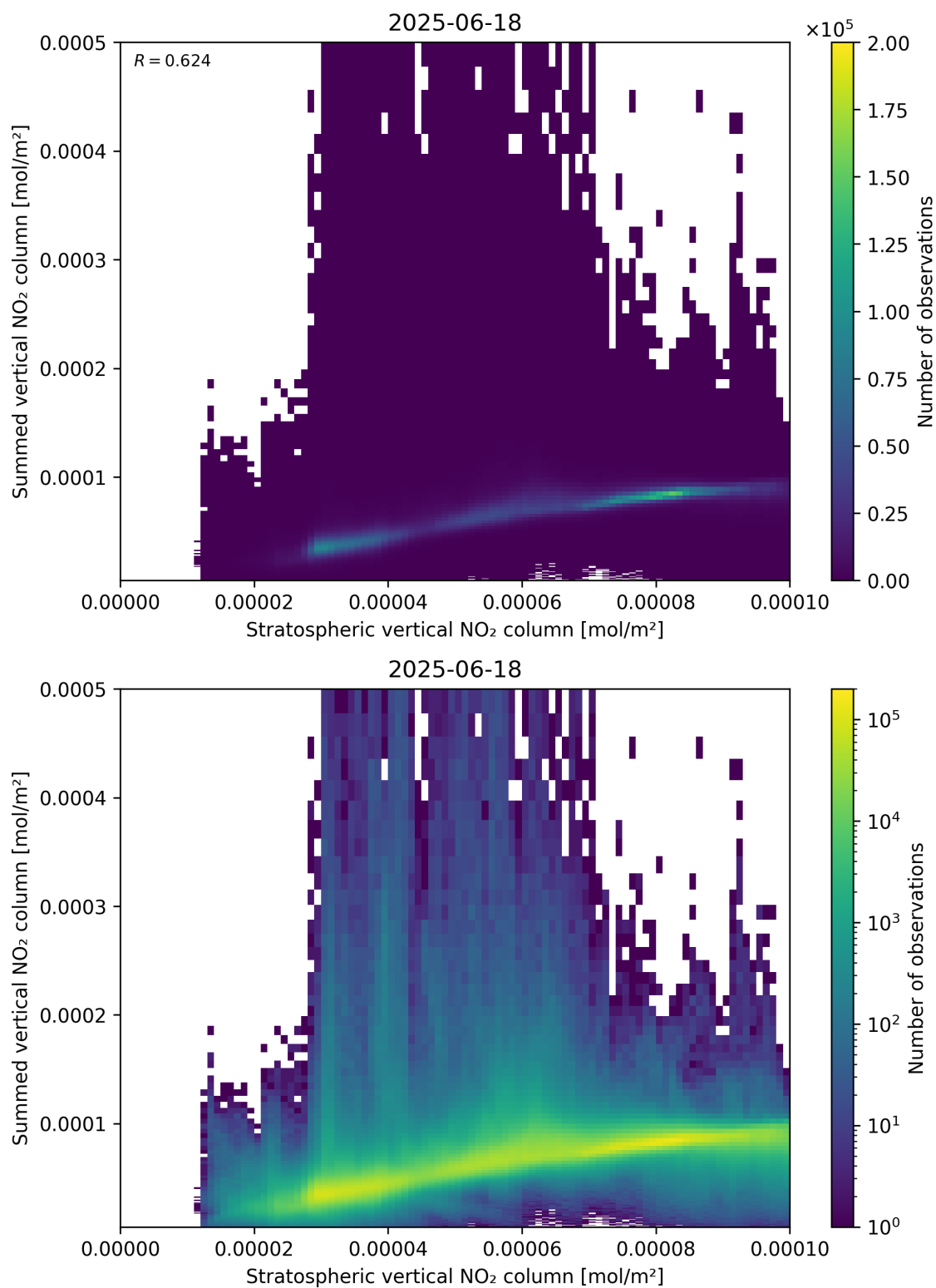
Figure 98: Scatter density plot of “Stratospheric vertical NO 2 column” against “Summed vertical NO 2 column” for 2025-06-17 to 2025-06-19.
