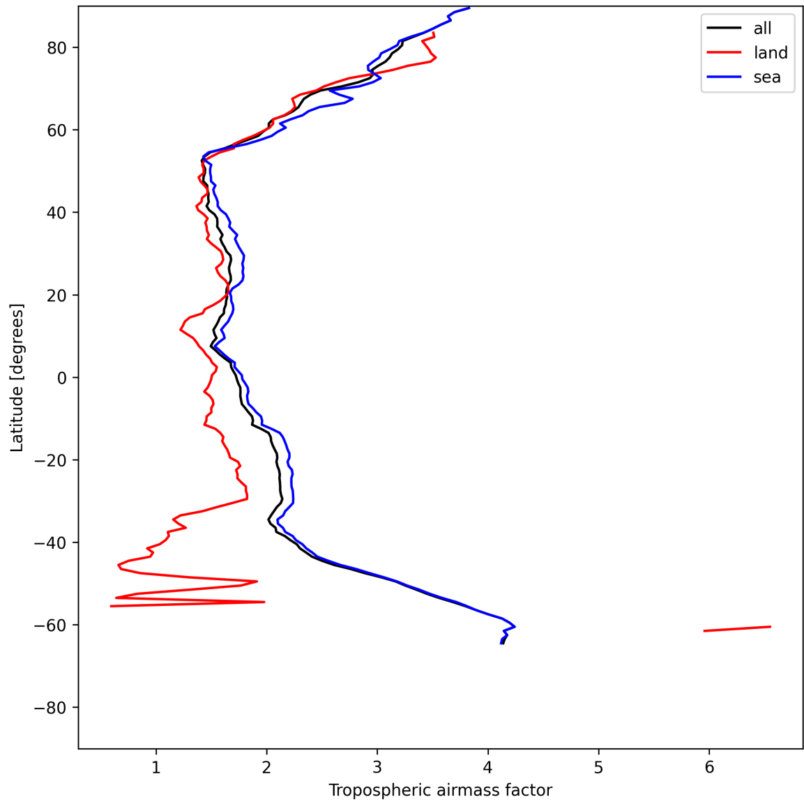
Figure 14: Zonal average of “Tropospheric air mass factor” for 2025-06-17 to 2025-06-19.
