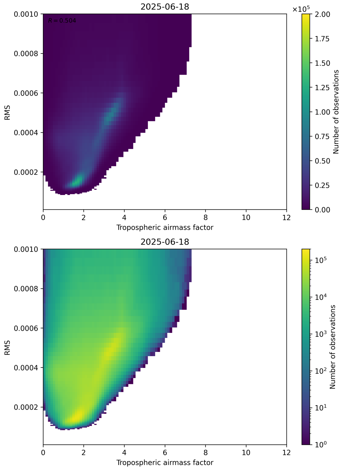
Figure 79: Scatter density plot of “Tropospheric airmass factor” against “RMS” for 2025-06-17 to 2025-06-19.
