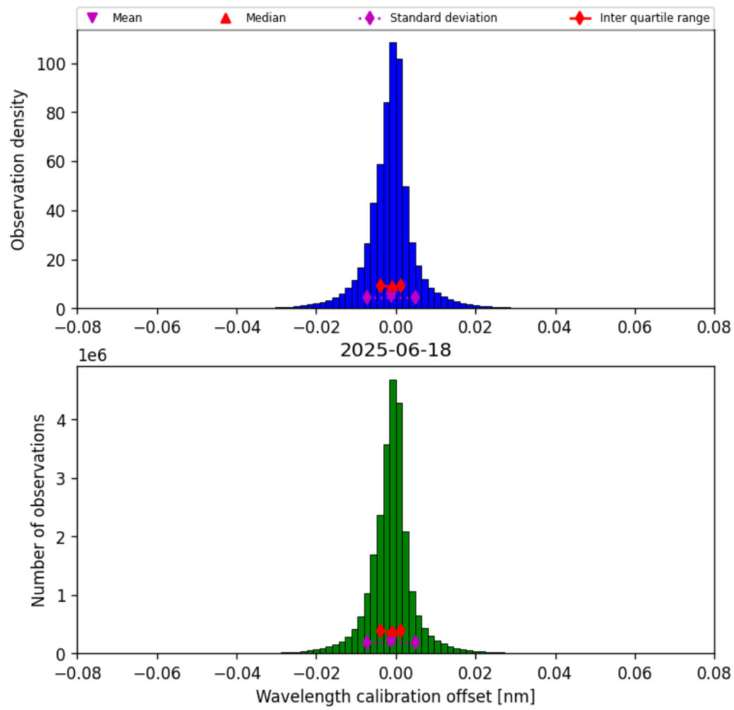
Figure 35: Histogram of “Wavelength calibration offset” for 2025-06-17 to 2025-06-19
