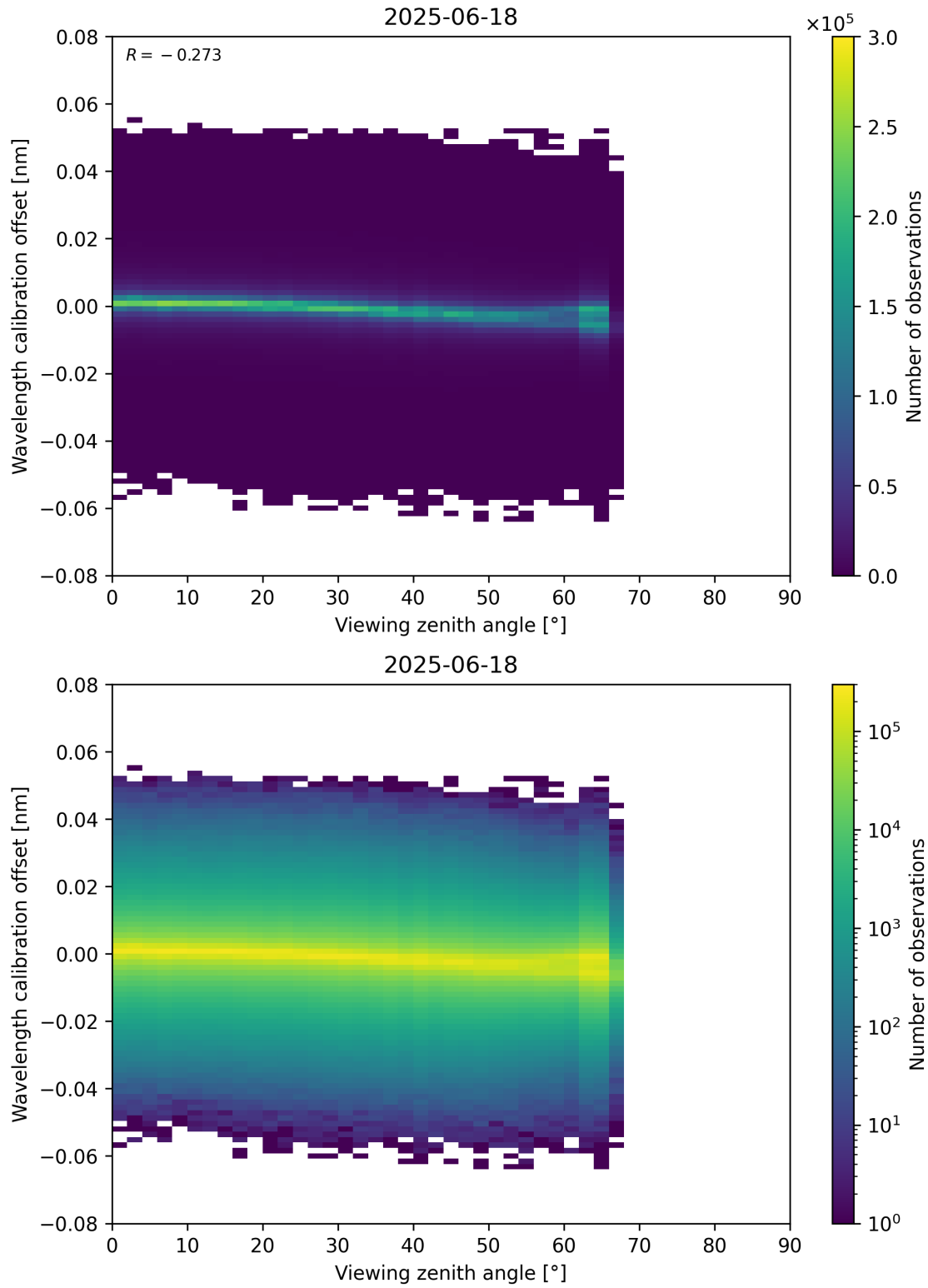
Figure 173: Scatter density plot of “Viewing zenith angle” against “Wavelength calibration offset” for 2025-06-17 to 2025-06-19.
