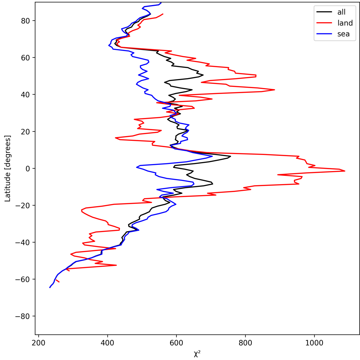
Figure 25: Zonal average of “ \chi^2 ” for 2025-06-17 to 2025-06-19.
