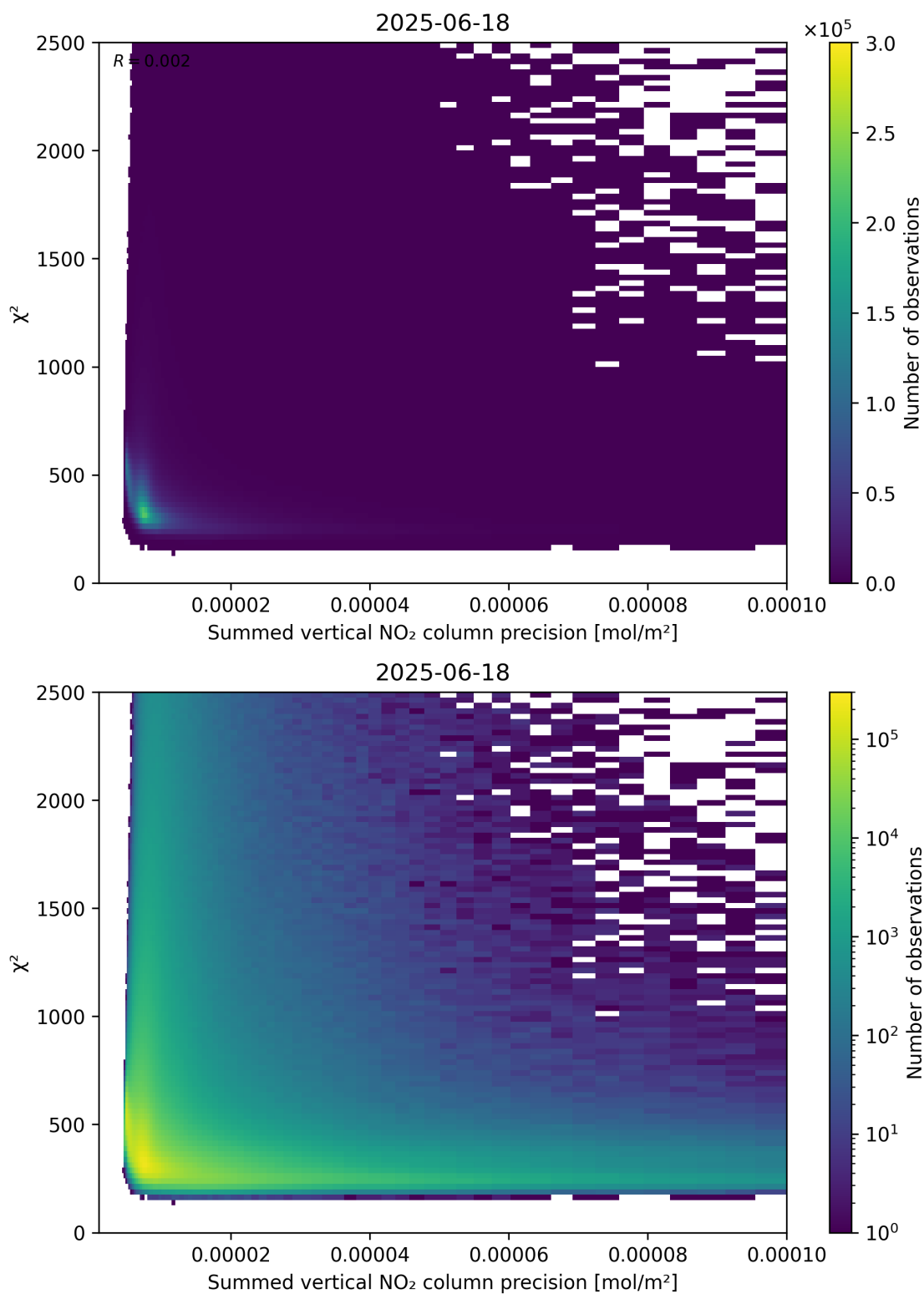
Figure 107: Scatter density plot of “Summed vertical NO 2 column precision” against “ \chi^2 ” for 2025-06-17 to 2025-06-19.
