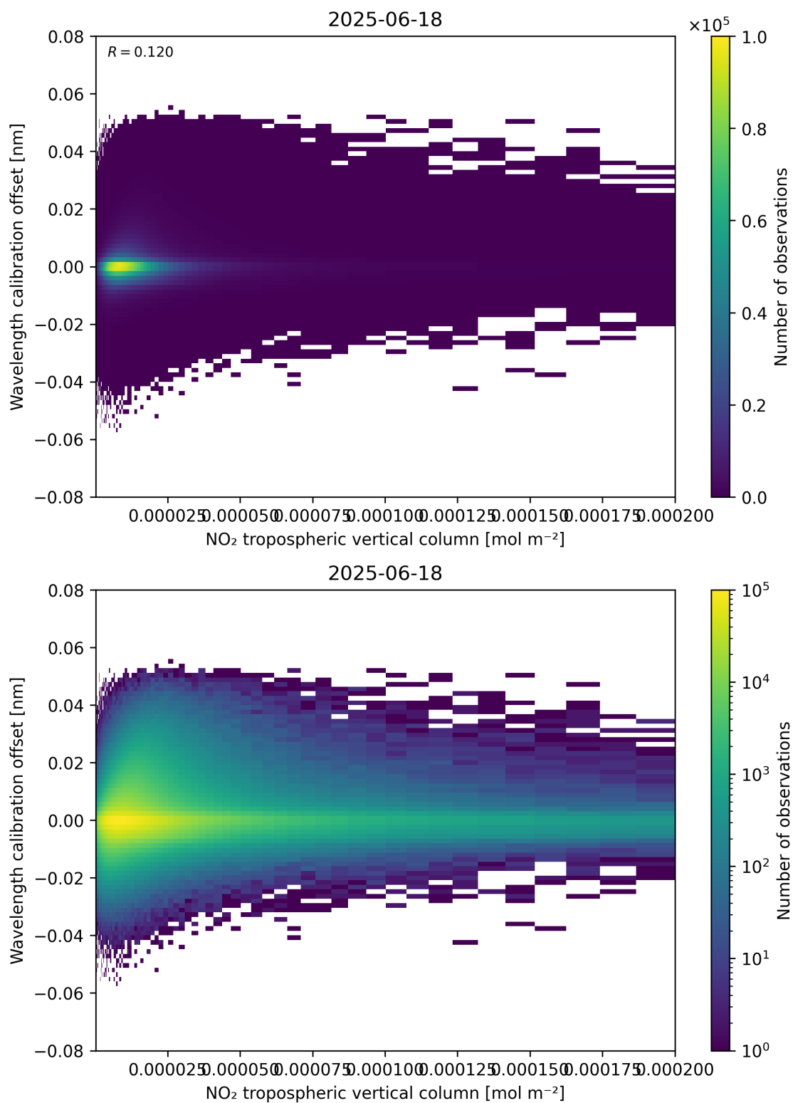
Figure 143: Scatter density plot of “NO 2 tropospheric vertical column” against “Wavelength calibration offset” for 2025-06-17 to 2025-06-19.
