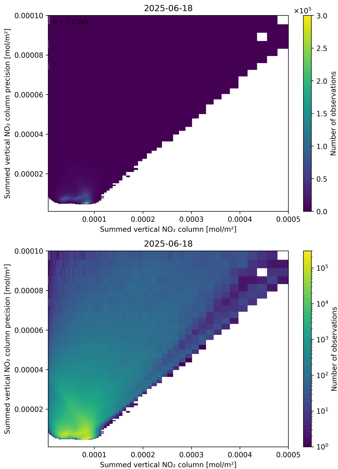
Figure 105: Scatter density plot of “Summed vertical NO 2 column” against “Summed vertical NO 2 column precision” for 2025-06-17 to 2025-06-19.
