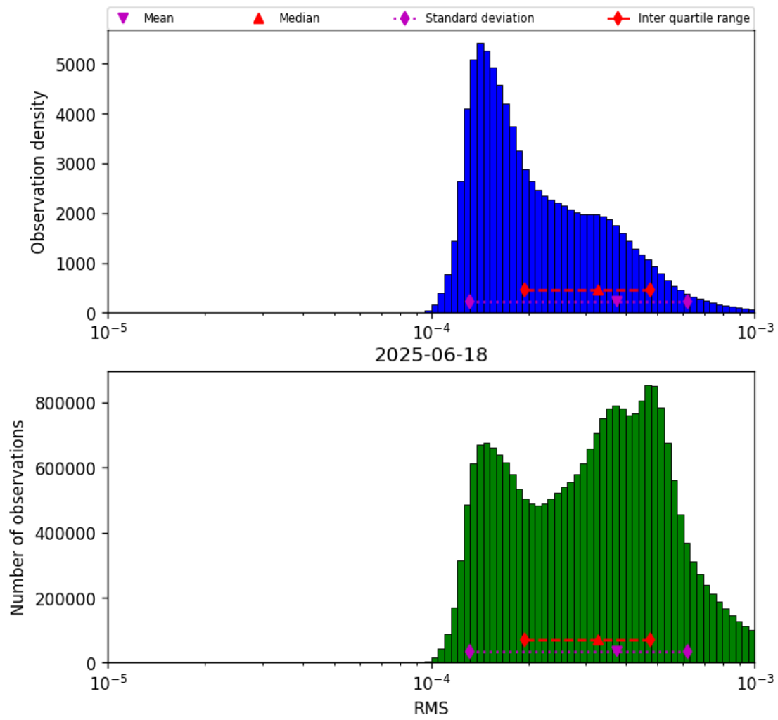
Figure 43: Histogram of “RMS” for 2025-06-17 to 2025-06-19
