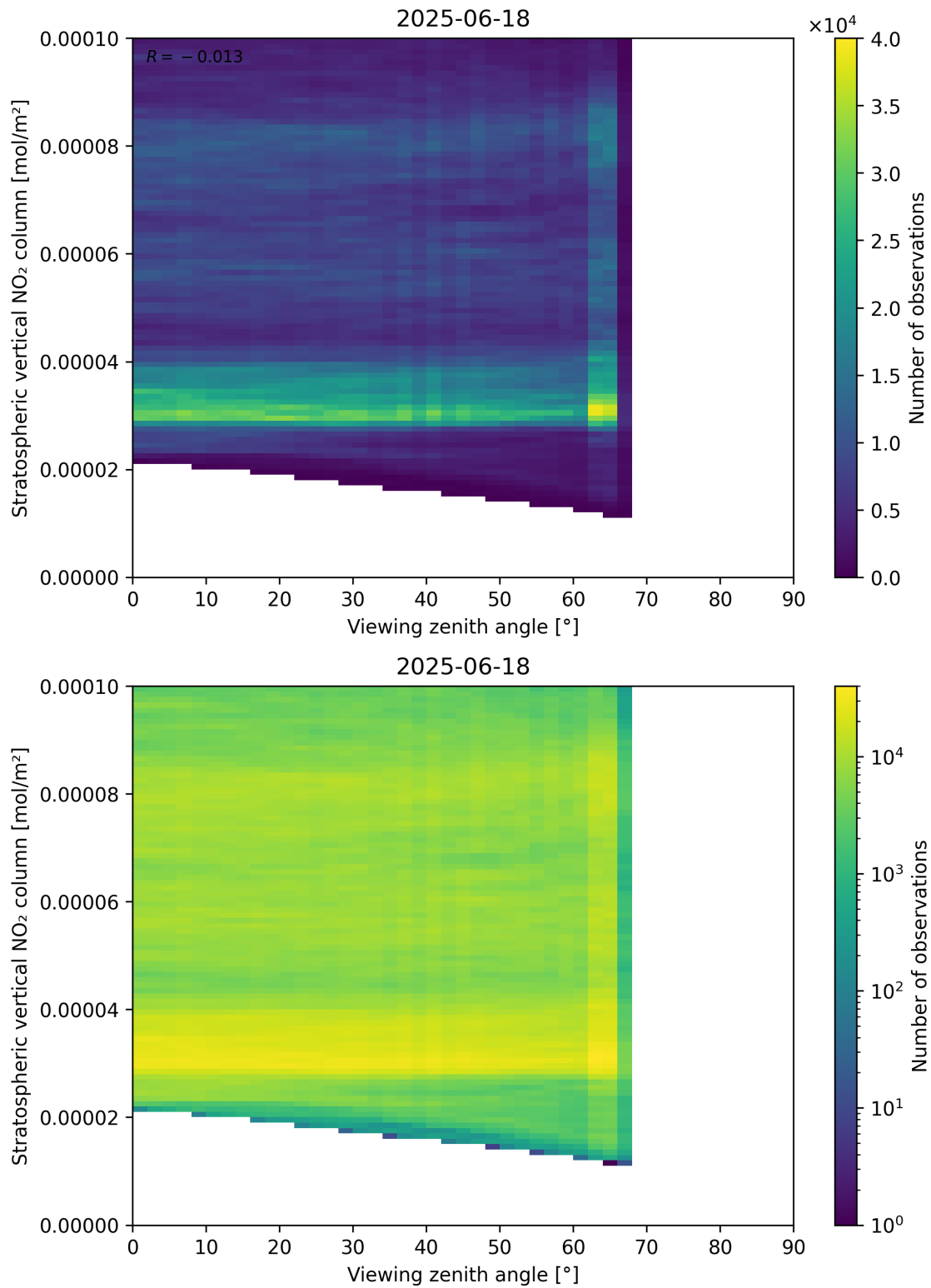
Figure 164: Scatter density plot of “Viewing zenith angle” against “Stratospheric vertical NO 2 column” for 2025-06-17 to 2025-06-19.
