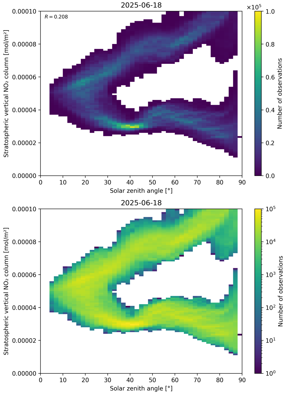
Figure 150: Scatter density plot of “Solar zenith angle” against “Stratospheric vertical NO 2 column” for 2025-06-17 to 2025-06-19.
