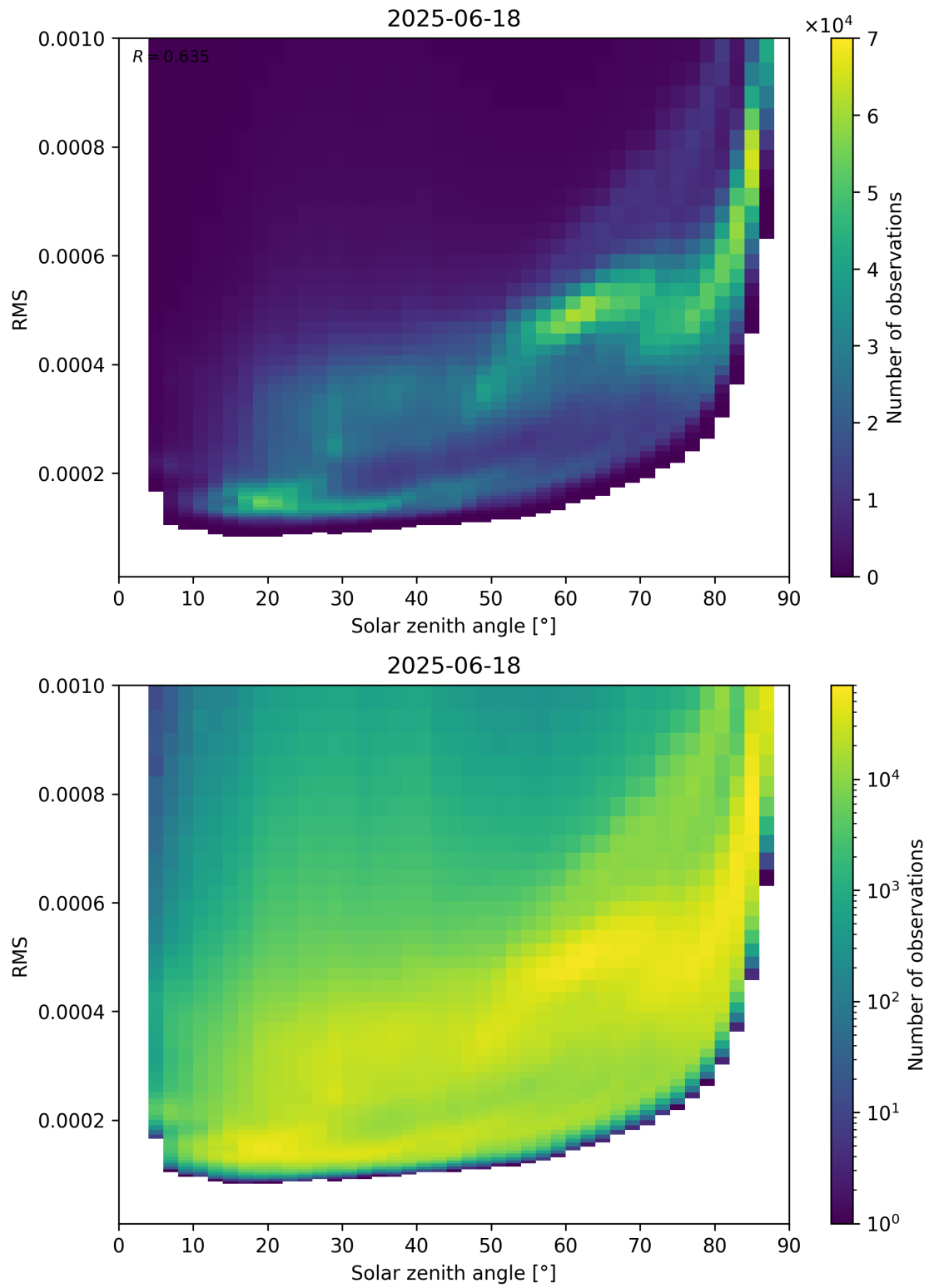
Figure 157: Scatter density plot of “Solar zenith angle” against “RMS” for 2025-06-17 to 2025-06-19.
