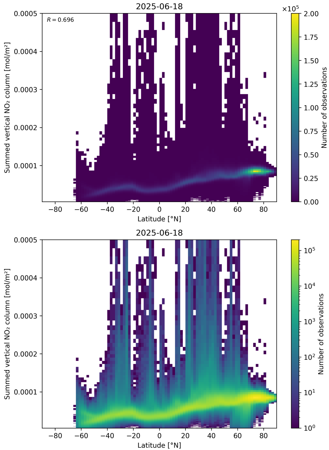
Figure 88: Scatter density plot of “Latitude” against “Summed vertical NO 2 column” for 2025-06-17 to 2025-06-19.
