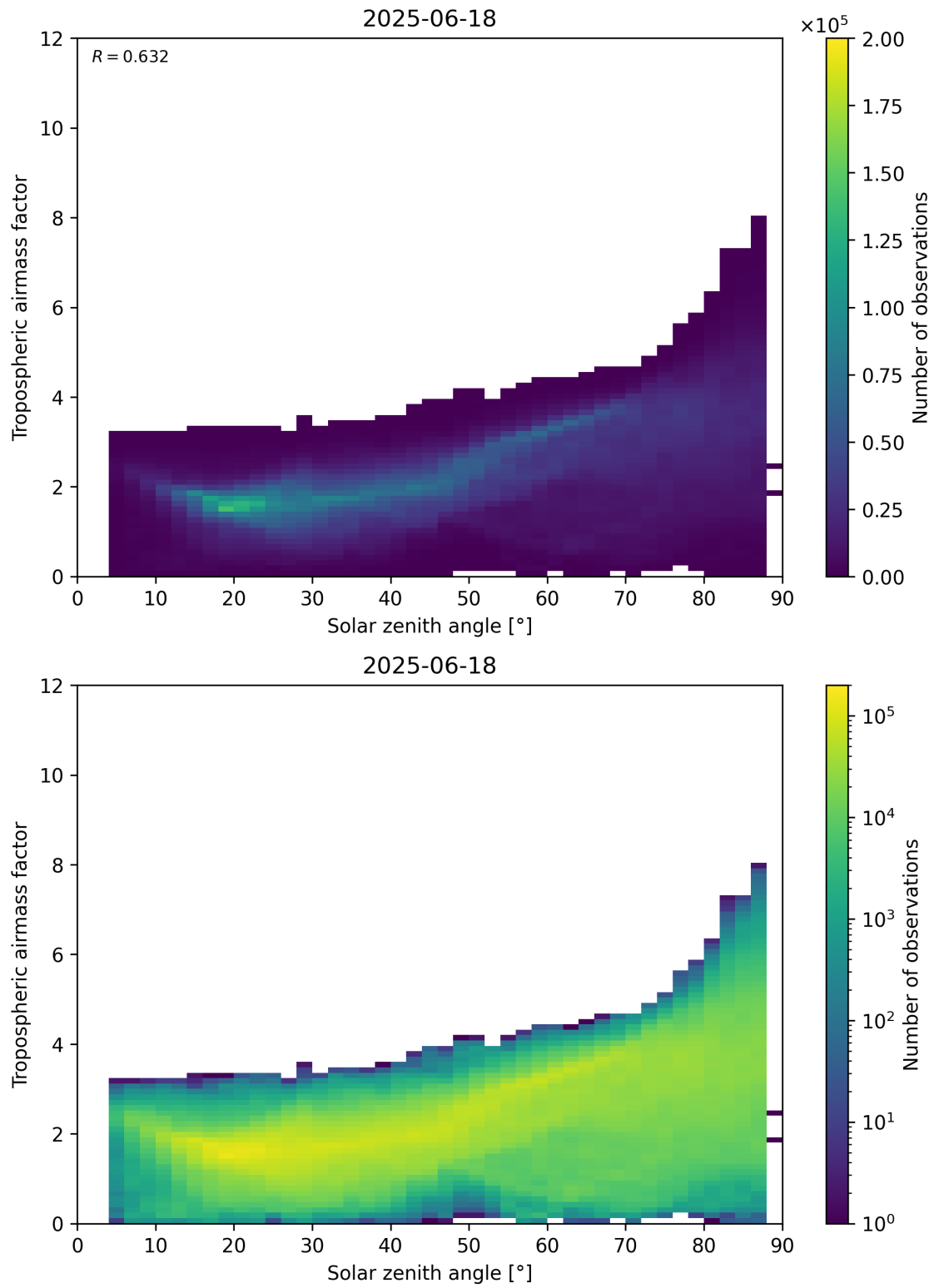
Figure 147: Scatter density plot of “Solar zenith angle” against “Tropospheric airmass factor” for 2025-06-17 to 2025-06-19.
