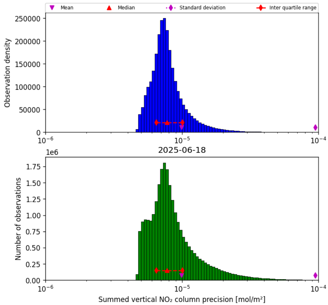
Figure 41: Histogram of "Summed vertical NO 2 column precision" for 2025-06-17 to 2025-06-19
