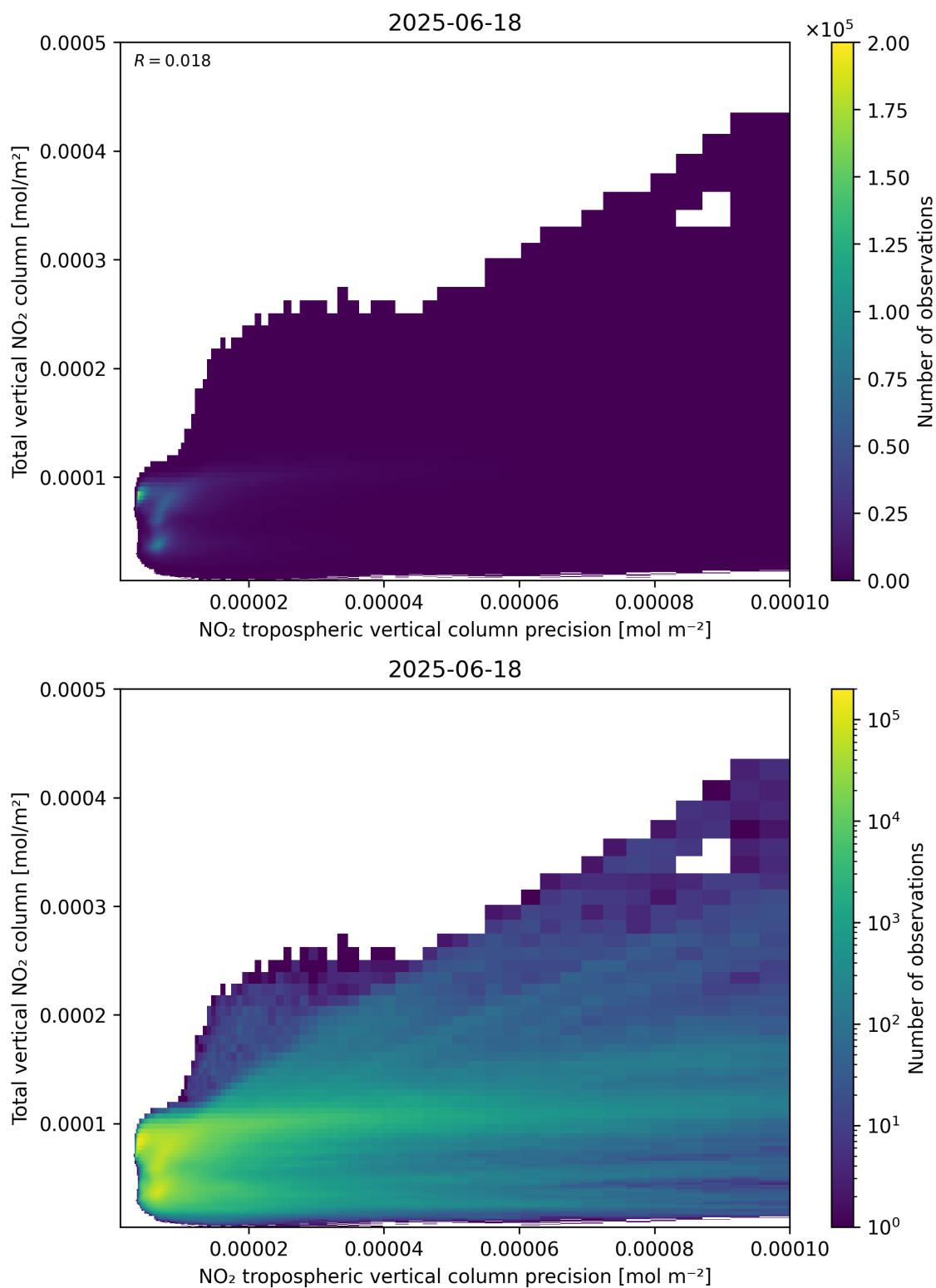
Figure 138: Scatter density plot of “NO 2 tropospheric vertical column precision” against “Total vertical NO 2 column” for 2025-06-17 to 2025-06-19.
