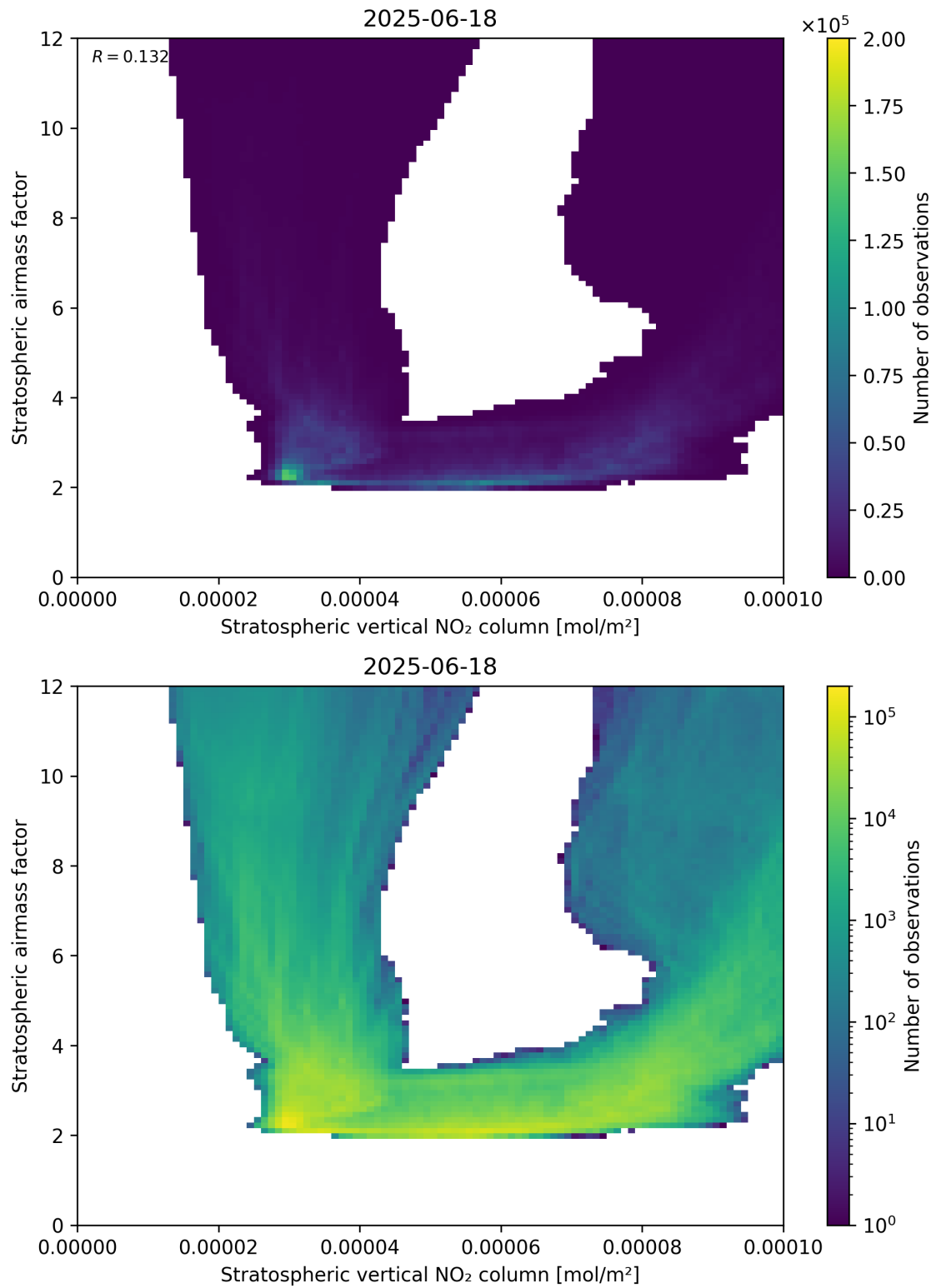
Figure 96: Scatter density plot of “Stratospheric vertical NO 2 column” against “Stratospheric airmass factor” for 2025-06-17 to 2025-06-19.
