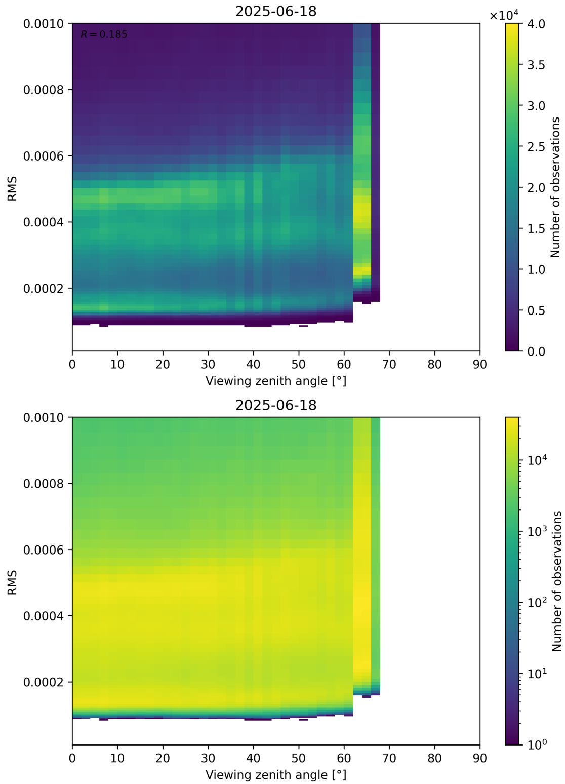
Figure 171: Scatter density plot of “Viewing zenith angle” against “RMS” for 2025-06-17 to 2025-06-19.
