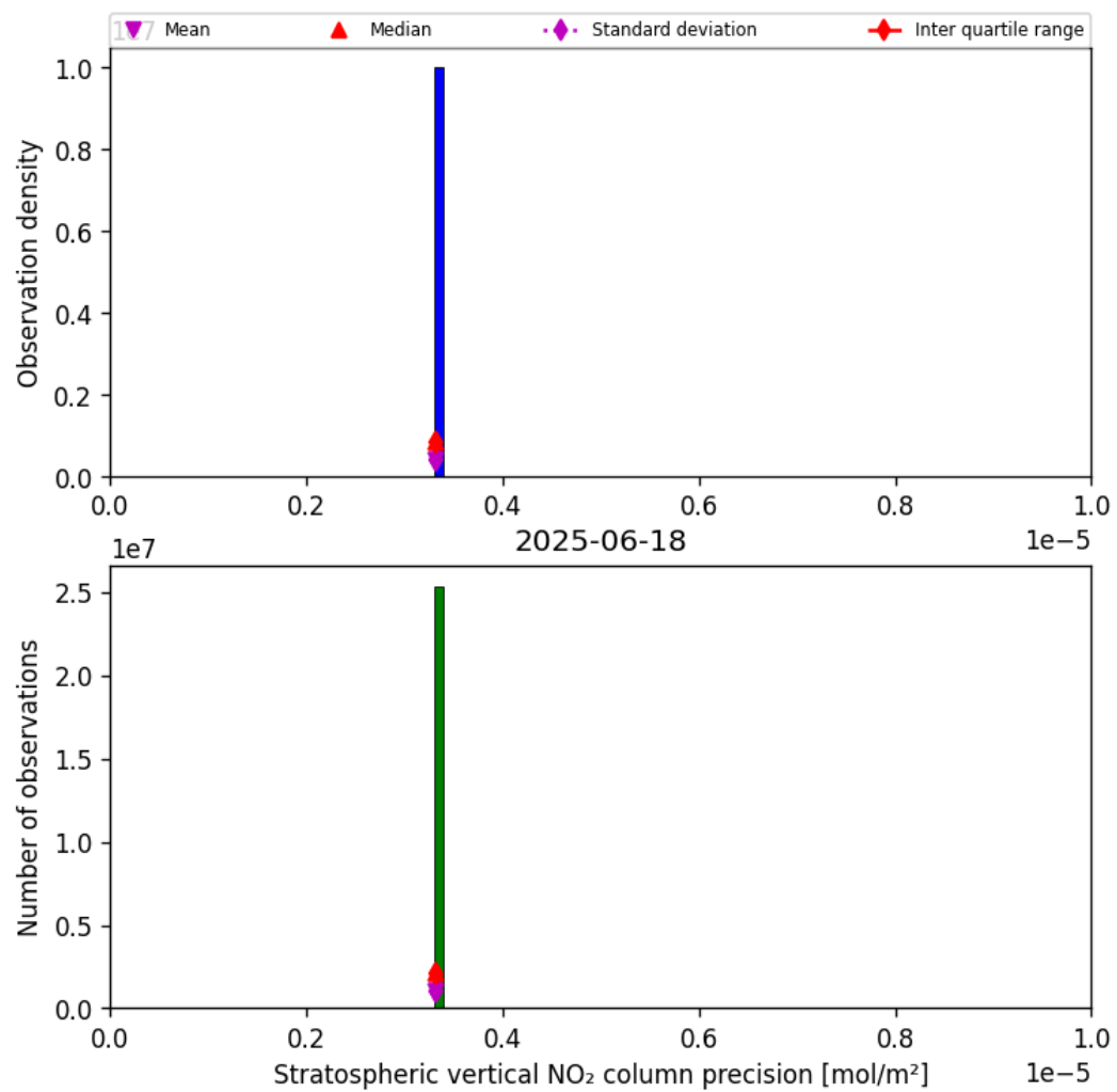
Figure 37: Histogram of “Stratospheric vertical NO 2 column precision” for 2025-06-17 to 2025-06-19
