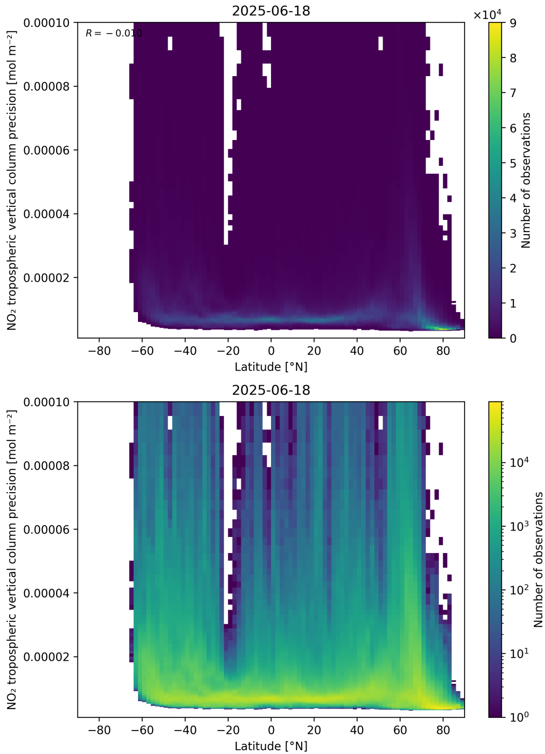
Figure 93: Scatter density plot of “Latitude” against “NO 2 tropospheric vertical column precision” for 2025-06-17 to 2025-06-19.
