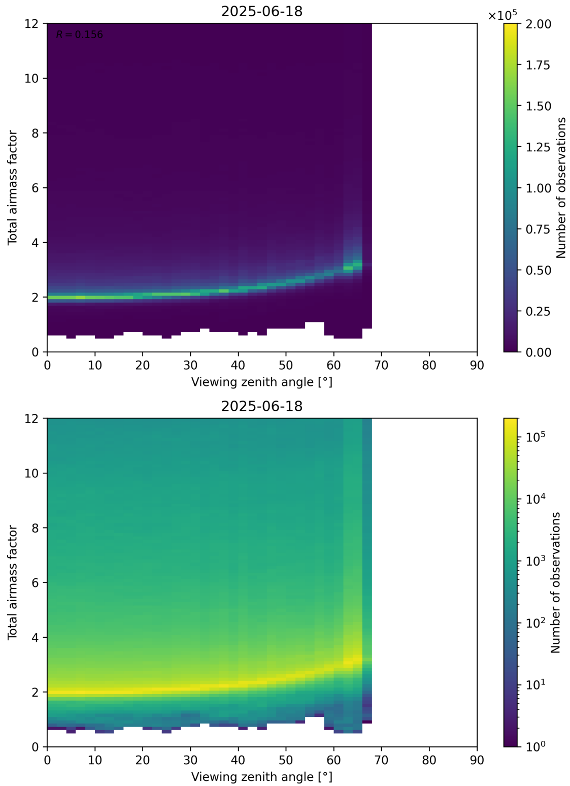
Figure 160: Scatter density plot of “Viewing zenith angle” against “Total airmass factor” for 2025-06-17 to 2025-06-19.
