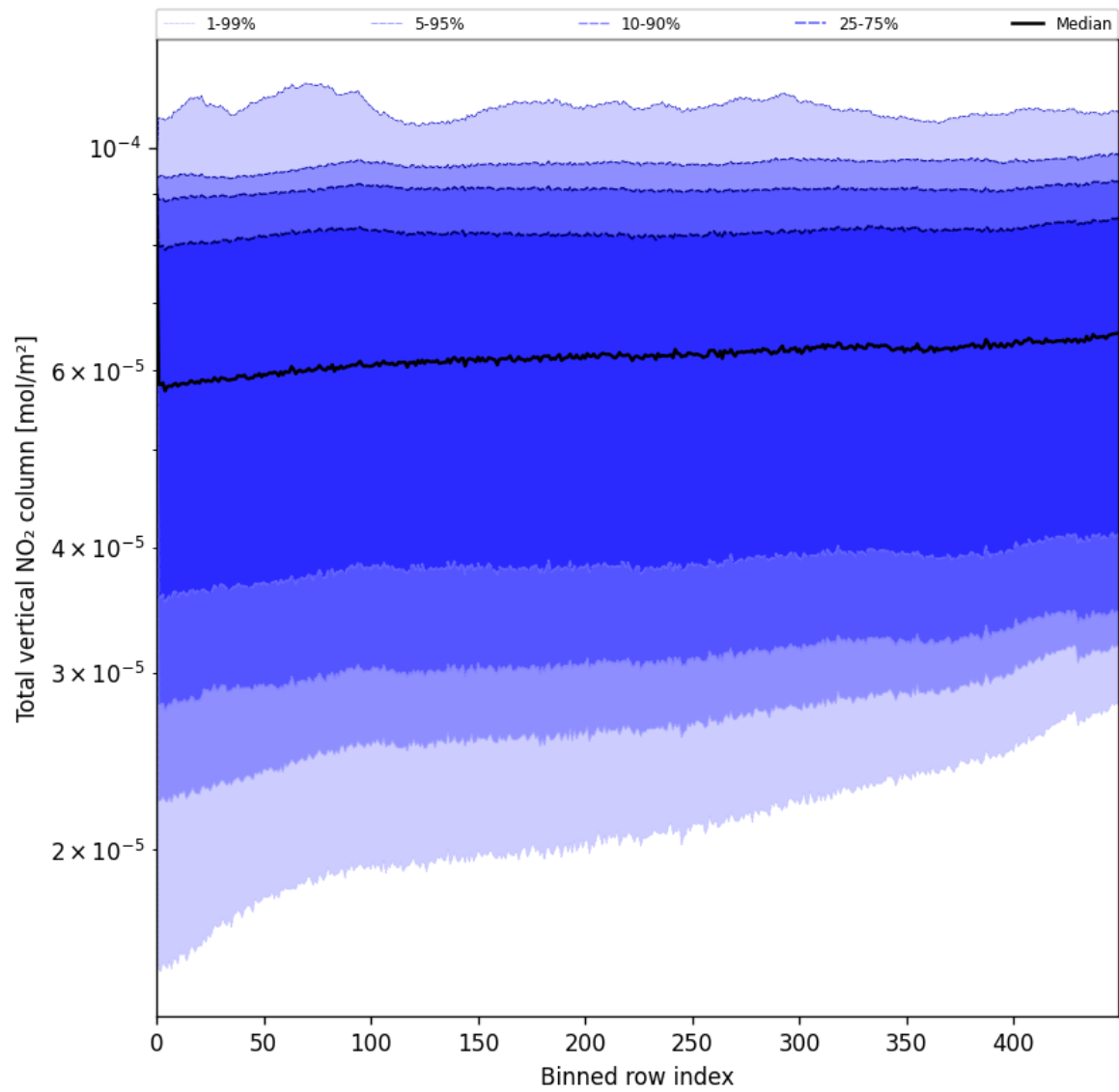
Figure 55: Along track statistics of “Total vertical NO 2 column” for 2025-06-17 to 2025-06-19
