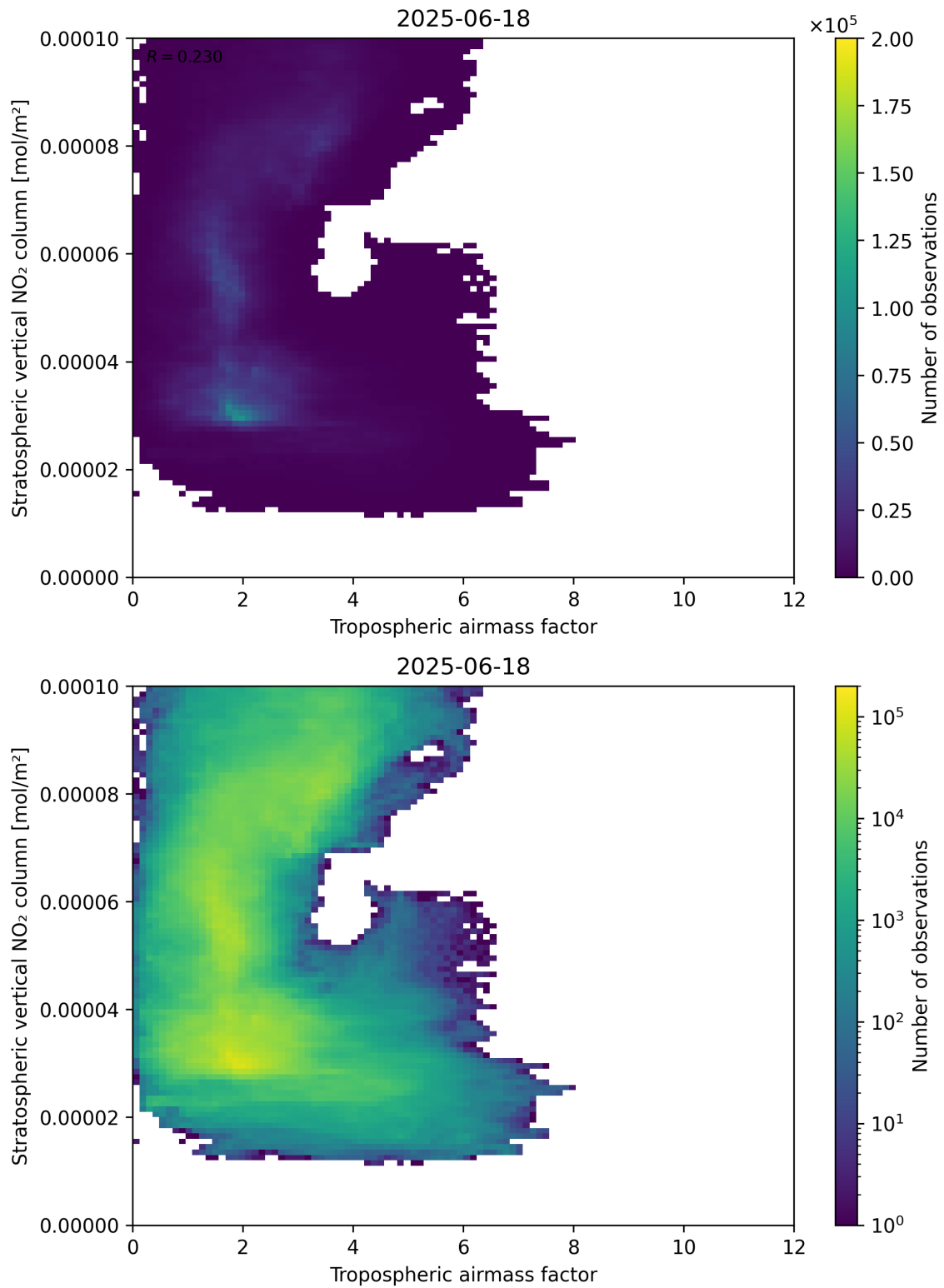
Figure 74: Scatter density plot of “Tropospheric air mass factor” against “Stratospheric vertical NO 2 column” for 2025-06-17 to 2025-06-19.
