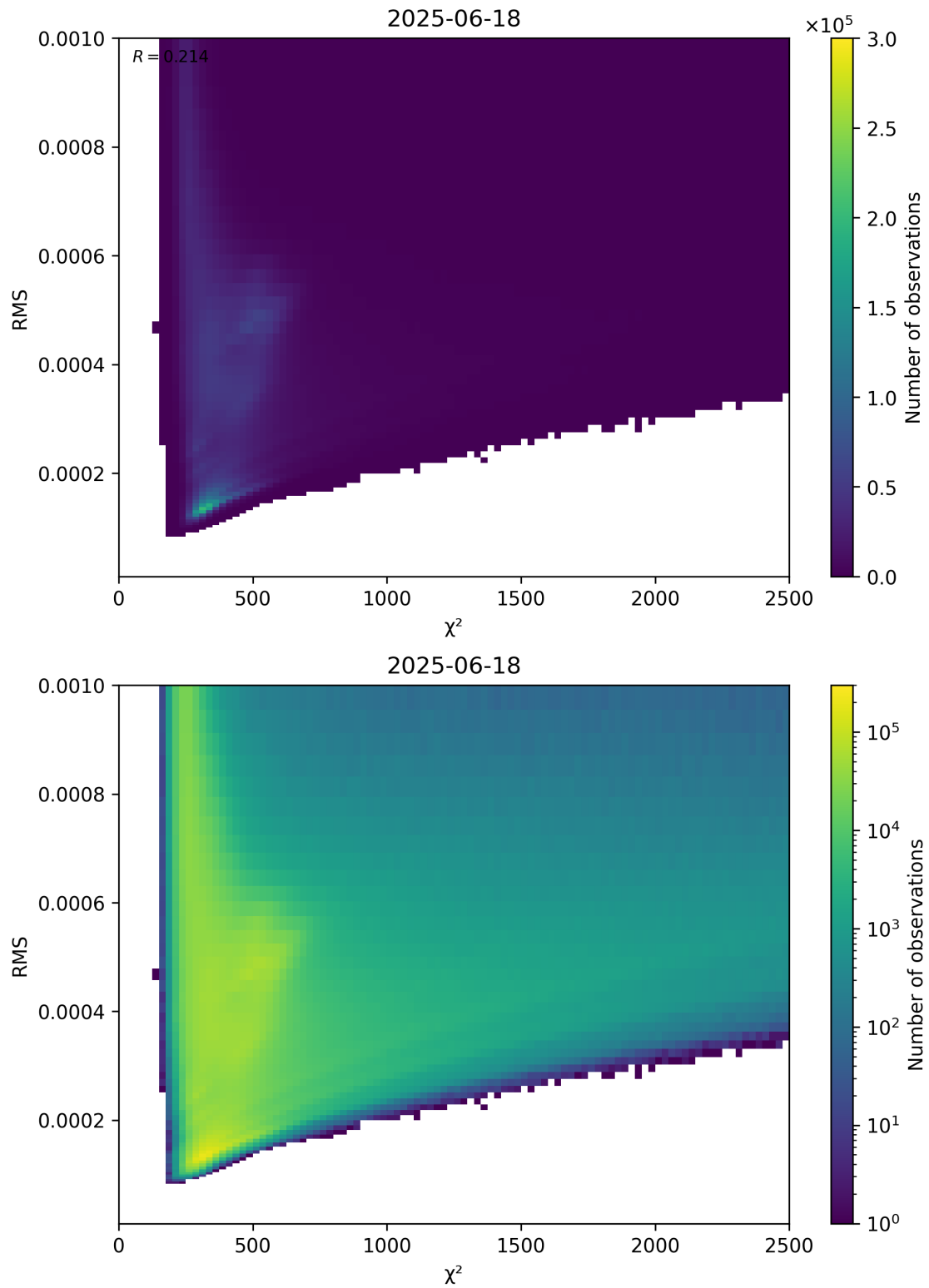
Figure 82: Scatter density plot of “ \chi^2 ” against “RMS” for 2025-06-17 to 2025-06-19.
