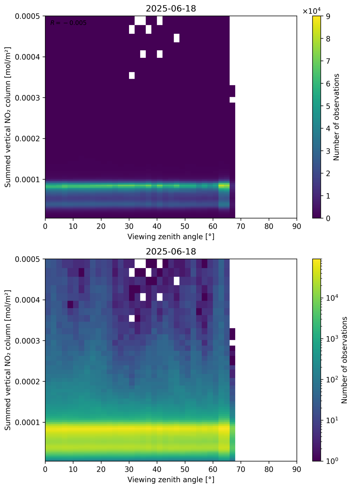
Figure 165: Scatter density plot of “Viewing zenith angle” against “Summed vertical NO 2 column” for 2025-06-17 to 2025-06-19.
