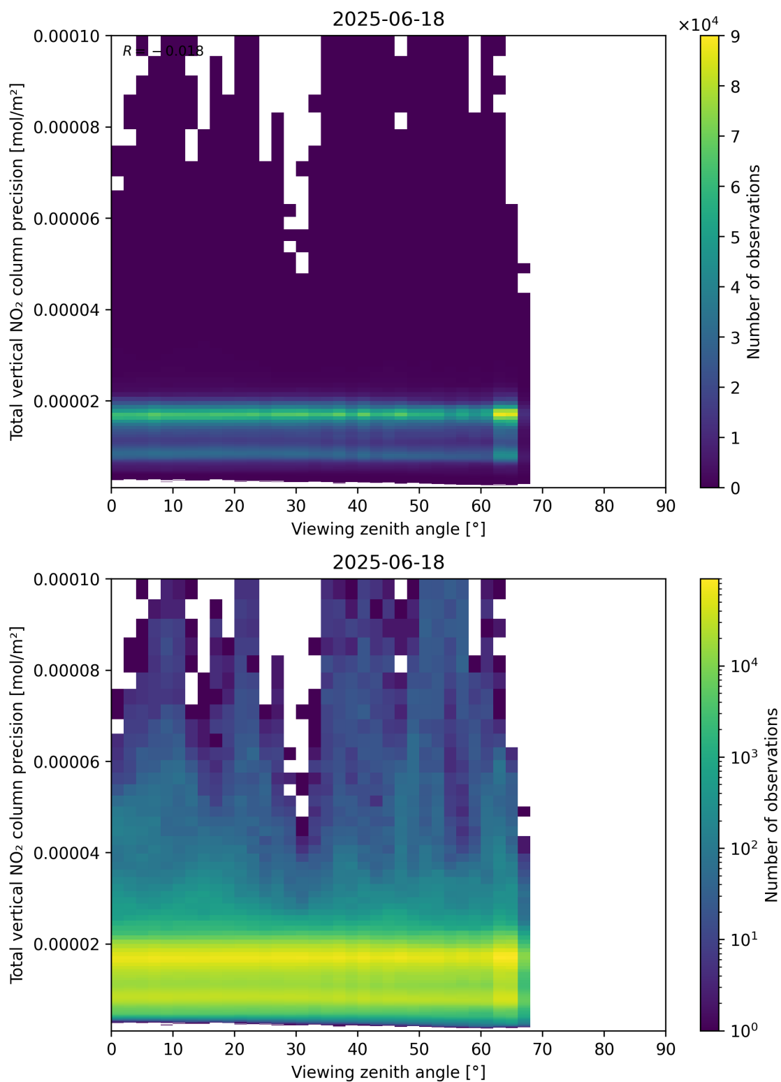
Figure 168: Scatter density plot of “Viewing zenith angle” against “Total vertical NO 2 column precision” for 2025-06-17 to 2025-06-19.
