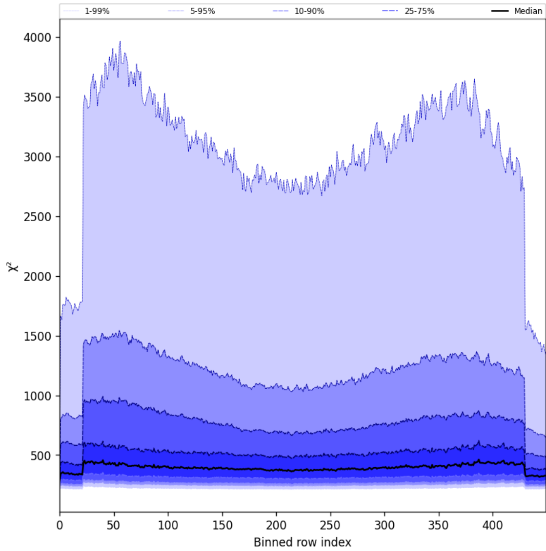
Figure 59: Along track statistics of “ \chi^2 ” for 2025-06-17 to 2025-06-19
