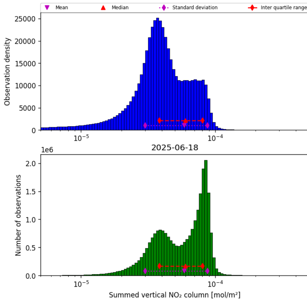
Figure 40: Histogram of “Summed vertical NO 2 column” for 2025-06-17 to 2025-06-19
