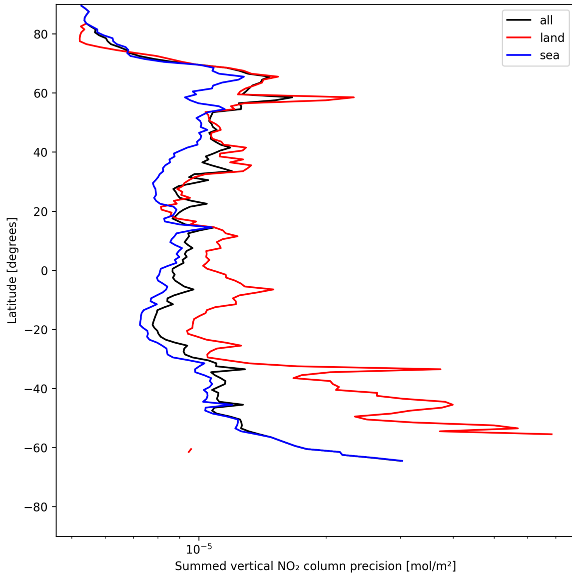
Figure 24: Zonal average of “Summed vertical NO 2 column precision” for 2025-06-17 to 2025-06-19.
