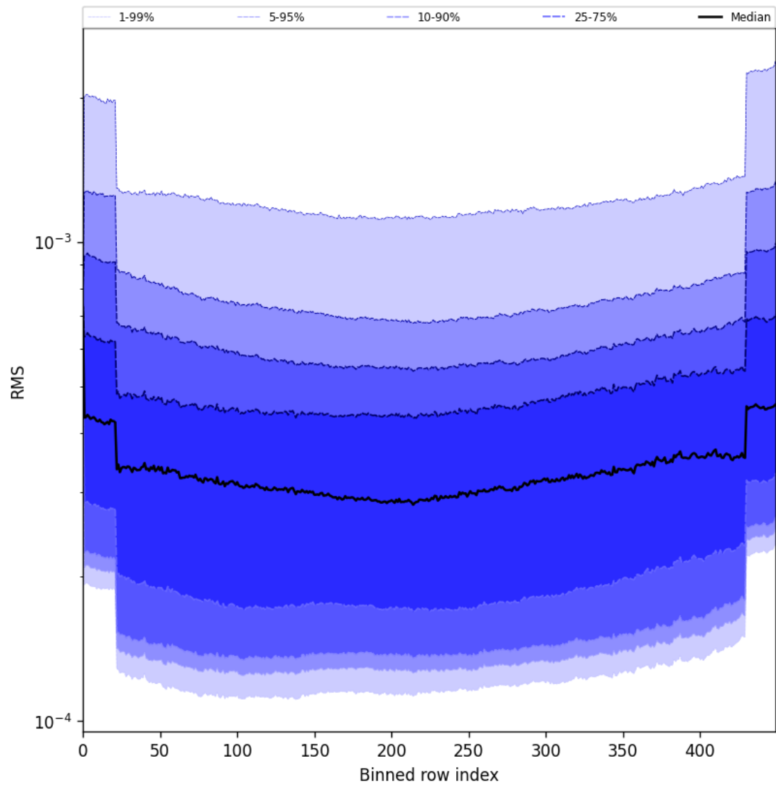
Figure 60: Along track statistics of “RMS” for 2025-06-17 to 2025-06-19
