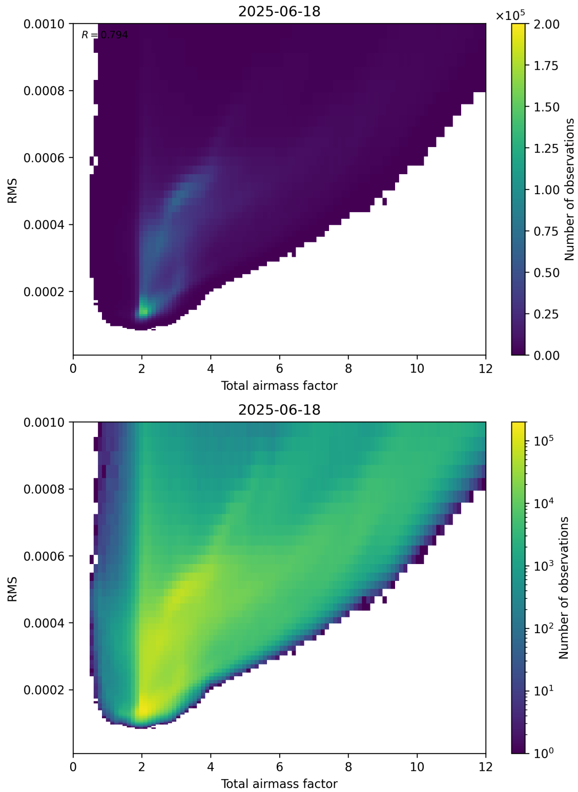
Figure 69: Scatter density plot of “Total airmass factor” against “RMS” for 2025-06-17 to 2025-06-19.
