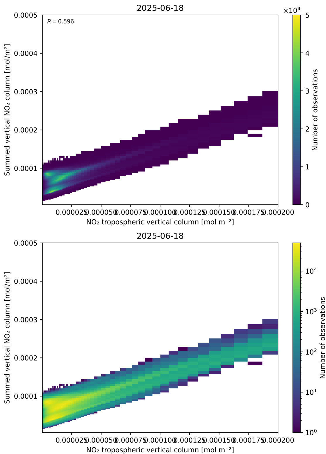
Figure 126: Scatter density plot of “NO 2 tropospheric vertical column” against “Summed vertical NO 2 column” for 2025-06-17 to 2025-06-19.
