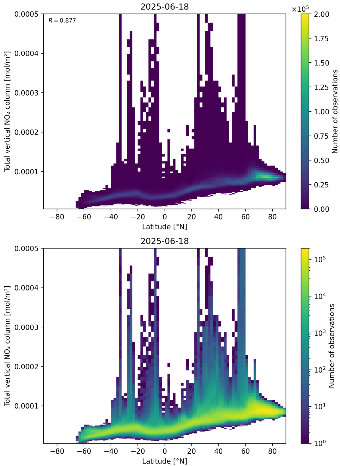
Figure 90: Scatter density plot of “Latitude” against “Total vertical NO 2 column” for 2025-06-17 to 2025-06-19.
