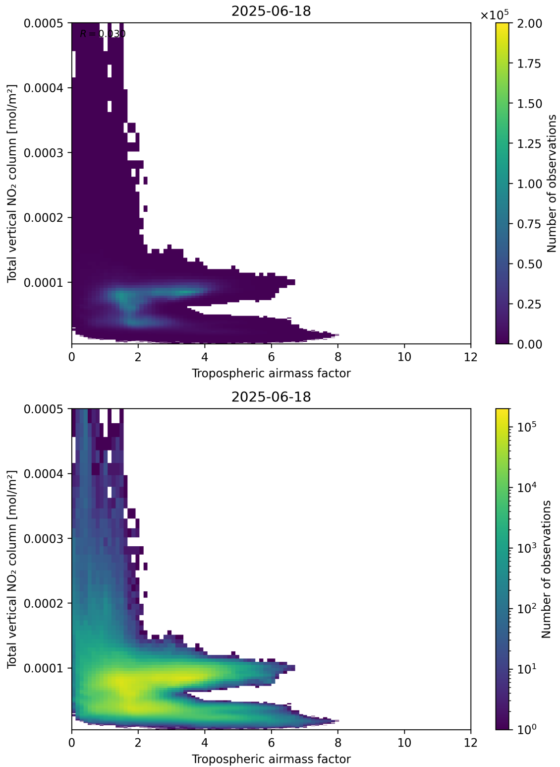
Figure 77: Scatter density plot of “Tropospheric airmass factor” against “Total vertical NO 2 column” for 2025-06-17 to 2025-06-19.
