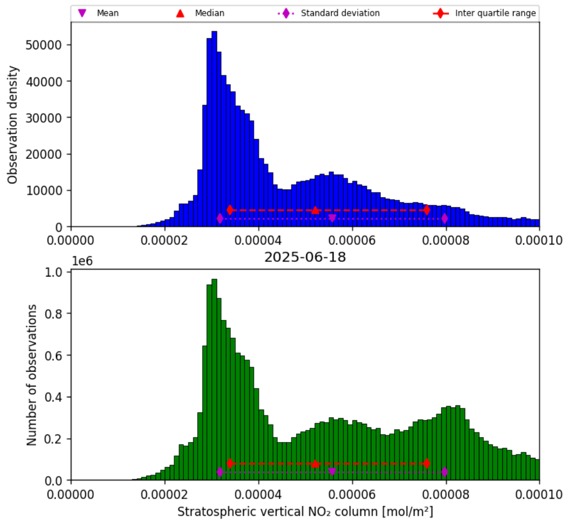
Figure 36: Histogram of “Stratospheric vertical NO 2 column” for 2025-06-17 to 2025-06-19
