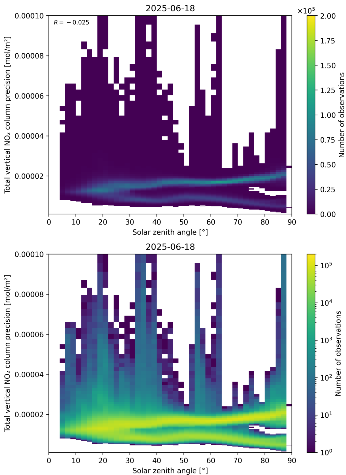
Figure 154: Scatter density plot of “Solar zenith angle” against “Total vertical NO 2 column precision” for 2025-06-17 to 2025-06-19.
