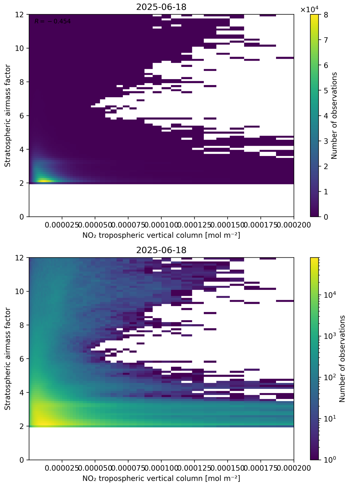
Figure 121: Scatter density plot of “NO 2 tropospheric vertical column” against “Stratospheric air mass factor” for 2025-06-17 to 2025-06-19.
