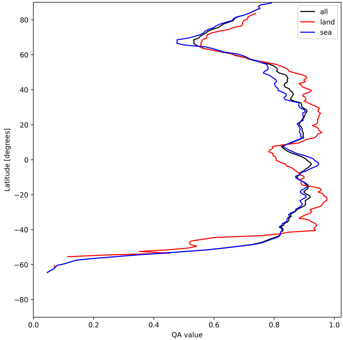
Figure 11: Zonal average of “QA value” for 2025-06-17 to 2025-06-19.
