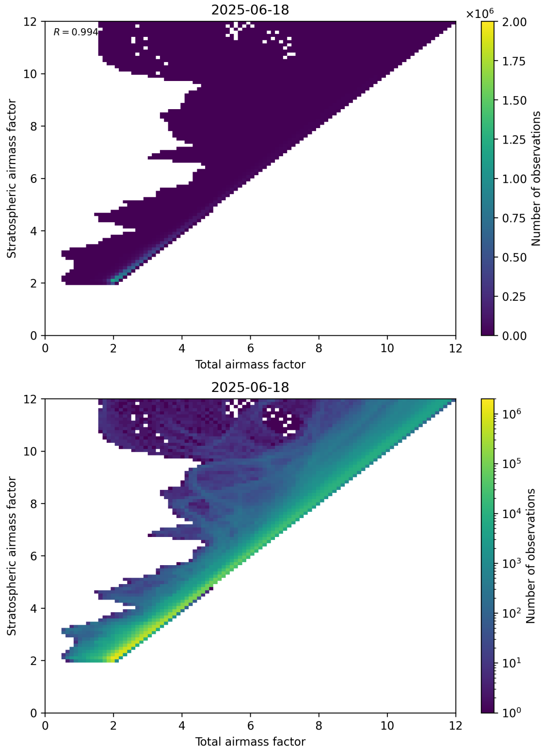
Figure 62: Scatter density plot of “Total airmass factor” against “Stratospheric airmass factor” for 2025-06-17 to 2025-06-19.
