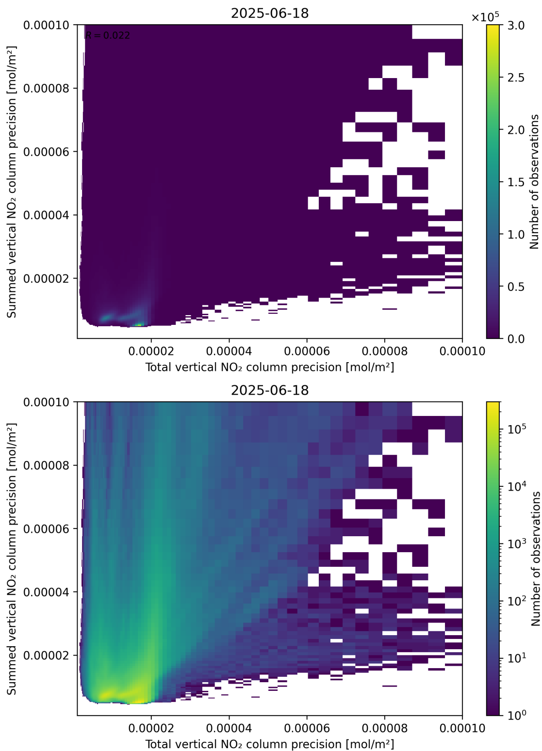
Figure 118: Scatter density plot of “Total vertical NO 2 column precision” against “Summed vertical NO 2 column precision” for 2025-06-17 to 2025-06-19.
