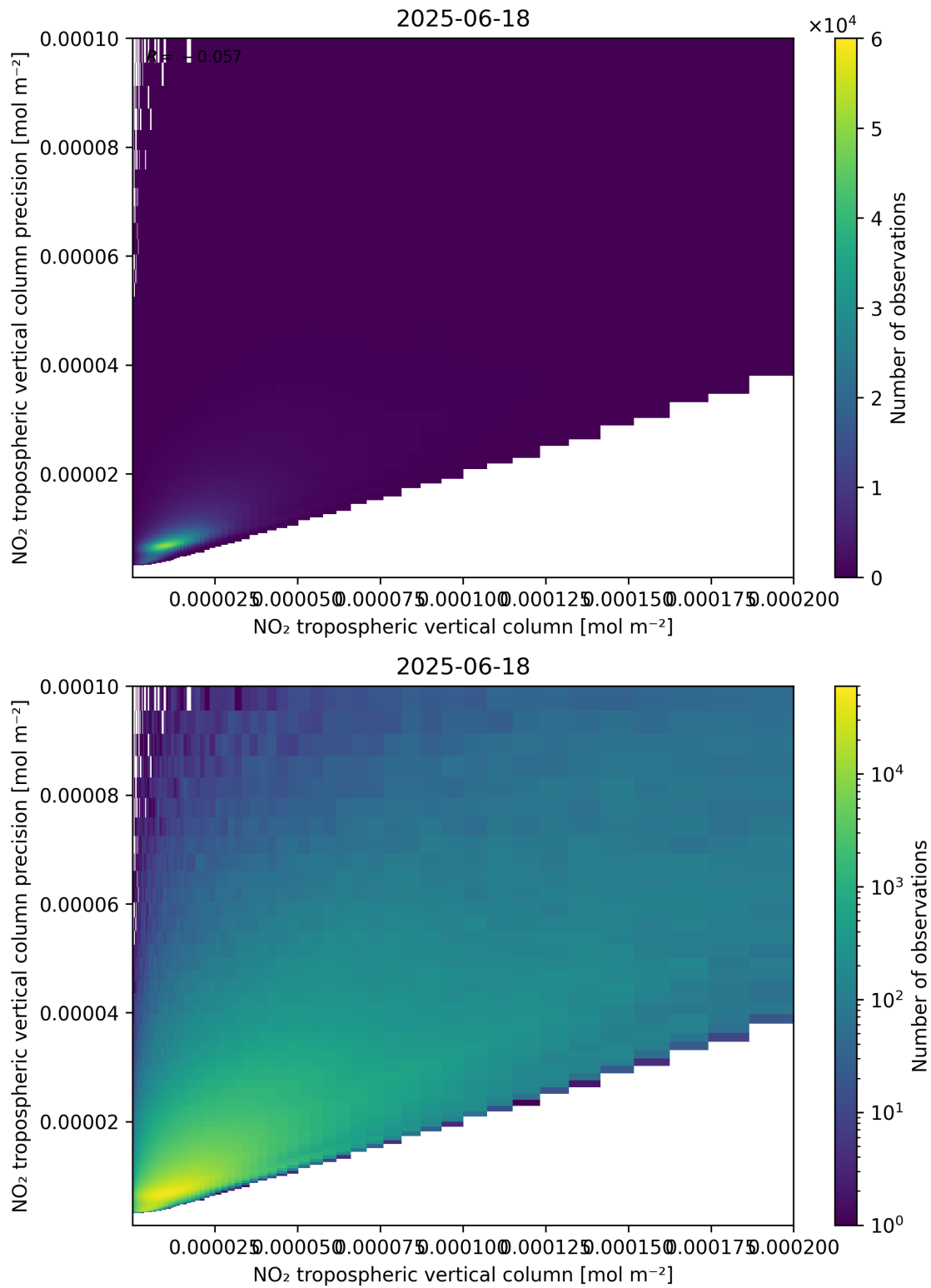
Figure 130: Scatter density plot of “NO 2 tropospheric vertical column” against “NO 2 tropospheric vertical column precision” for 2025-06-17 to 2025-06-19.
