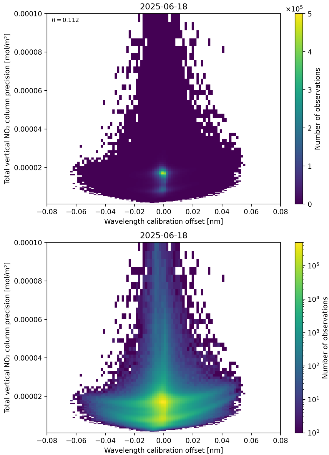
Figure 180: Scatter density plot of “Wavelength calibration offset” against “Total vertical NO 2 column precision” for 2025-06-17 to 2025-06-19.
