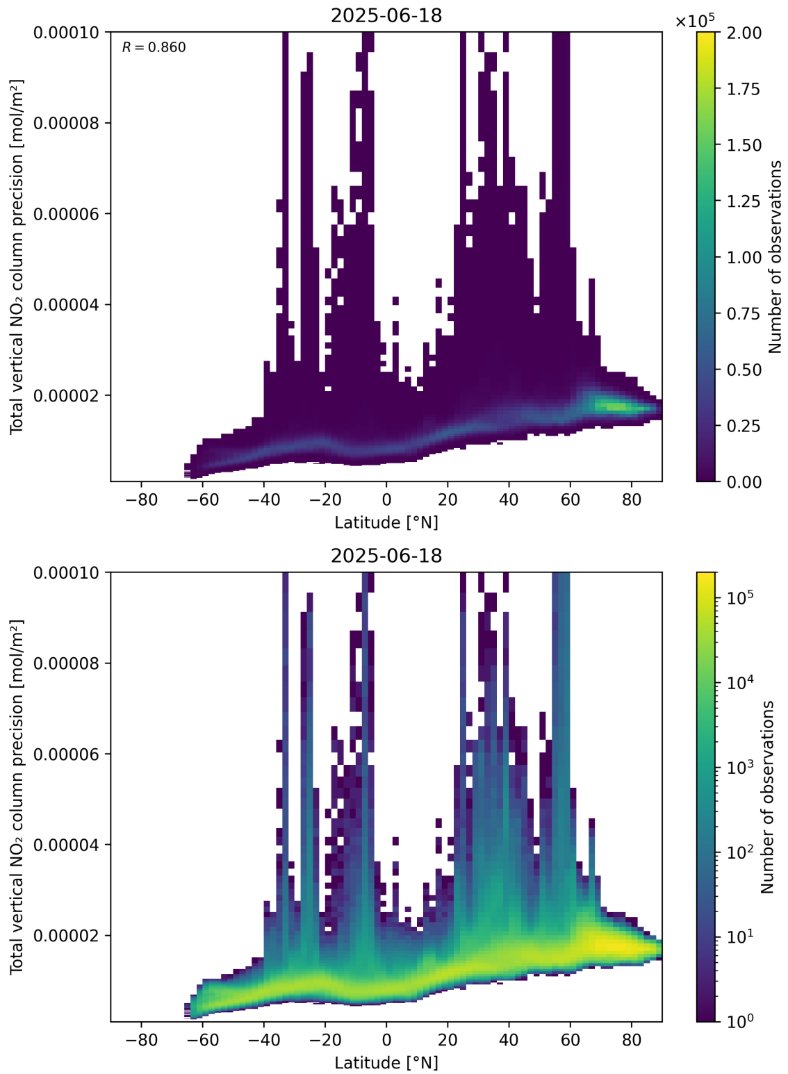
Figure 91: Scatter density plot of “Latitude” against “Total vertical NO 2 column precision” for 2025-06-17 to 2025-06-19.
