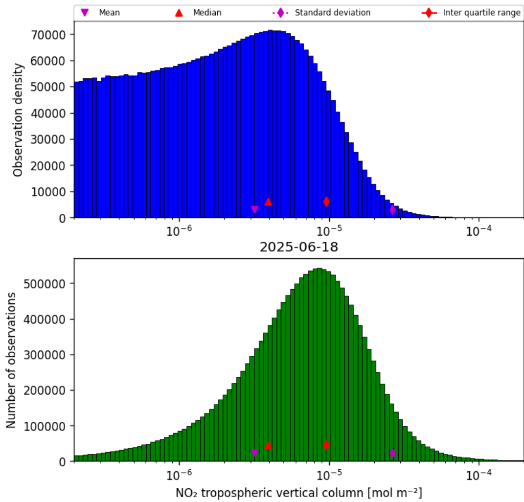
Figure 29: Histogram of “NO 2 tropospheric vertical column” for 2025-06-17 to 2025-06-19
