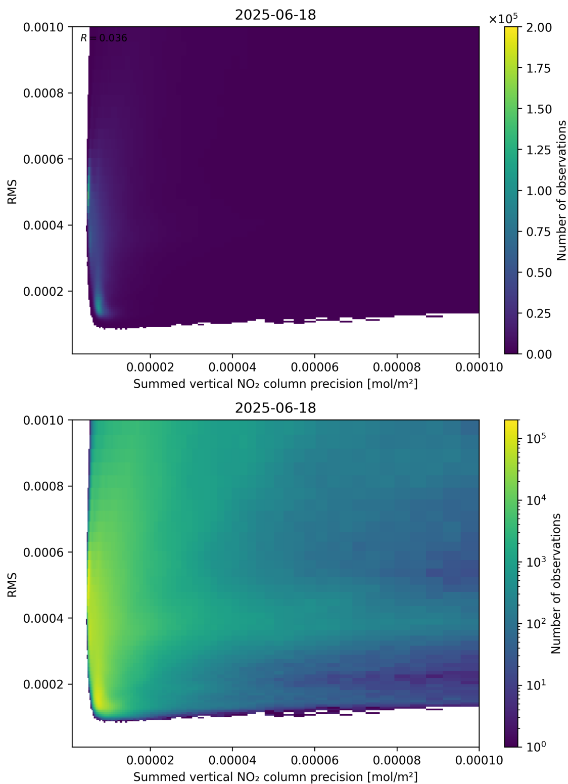
Figure 108: Scatter density plot of “Summed vertical NO 2 column precision” against “RMS” for 2025-06-17 to 2025-06-19.
