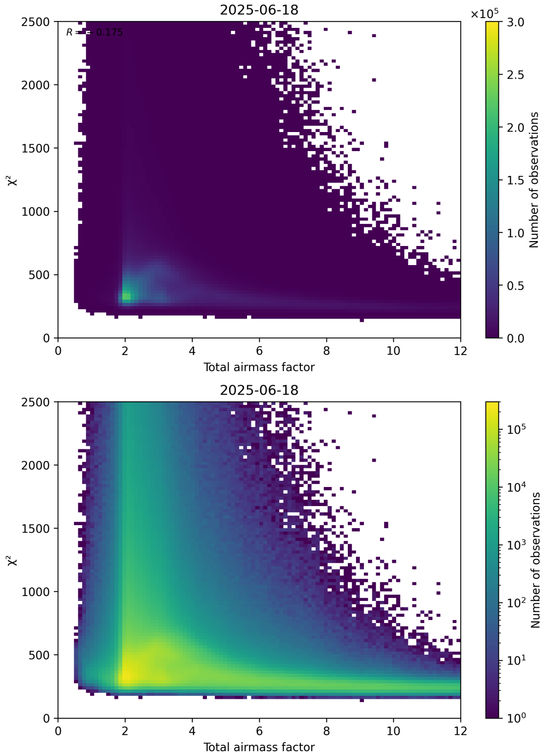
Figure 63: Scatter density plot of “Total airmass factor” against “ \chi^2 ” for 2025-06-17 to 2025-06-19.
