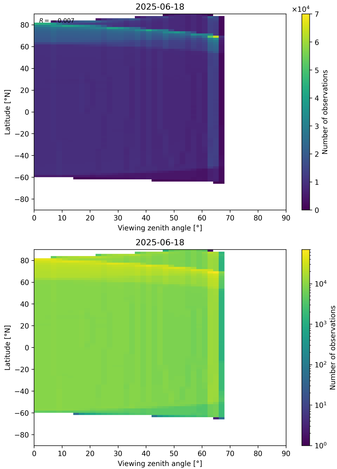
Figure 163: Scatter density plot of “Viewing zenith angle” against “Latitude” for 2025-06-17 to 2025-06-19.
