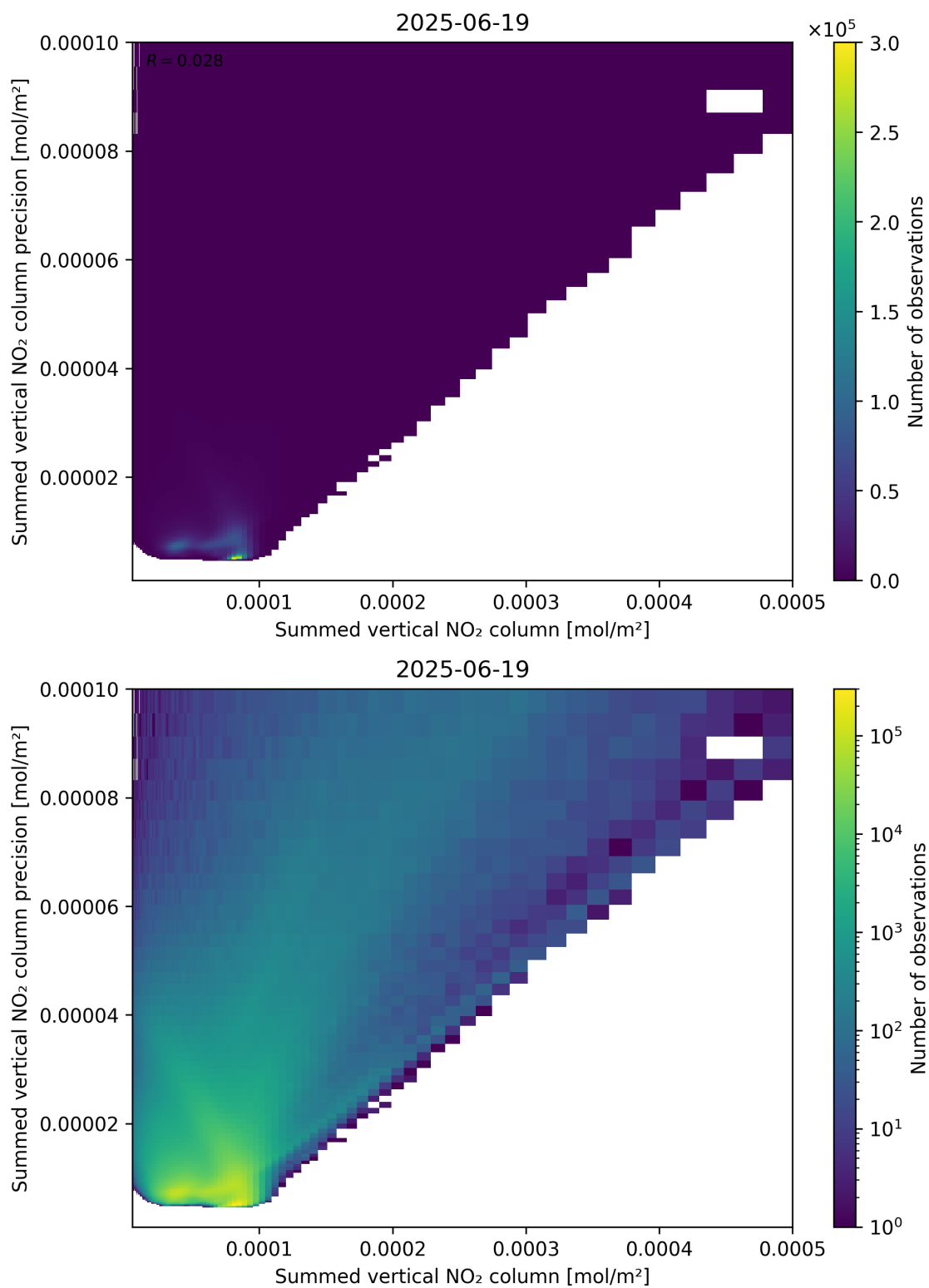
Figure 105: Scatter density plot of “Summed vertical NO 2 column” against “Summed vertical NO 2 column precision” for 2025-06-18 to 2025-06-20.
