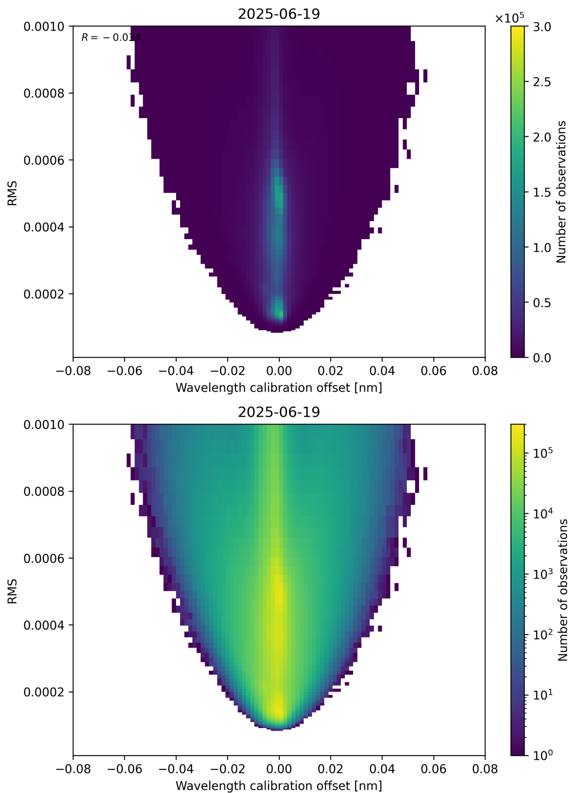
Figure 181: Scatter density plot of “Wavelength calibration offset” against “RMS” for 2025-06-18 to 2025-06-20.
