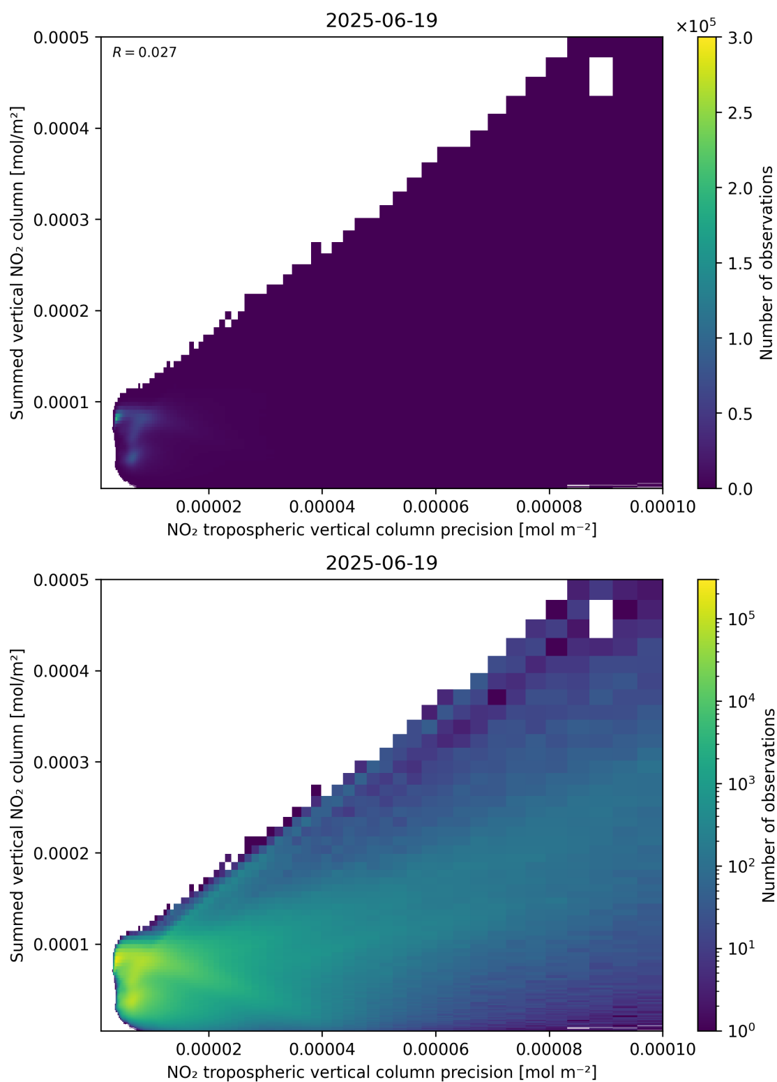
Figure 136: Scatter density plot of “NO 2 tropospheric vertical column precision” against “Summed vertical NO 2 column” for 2025-06-18 to 2025-06-20.
