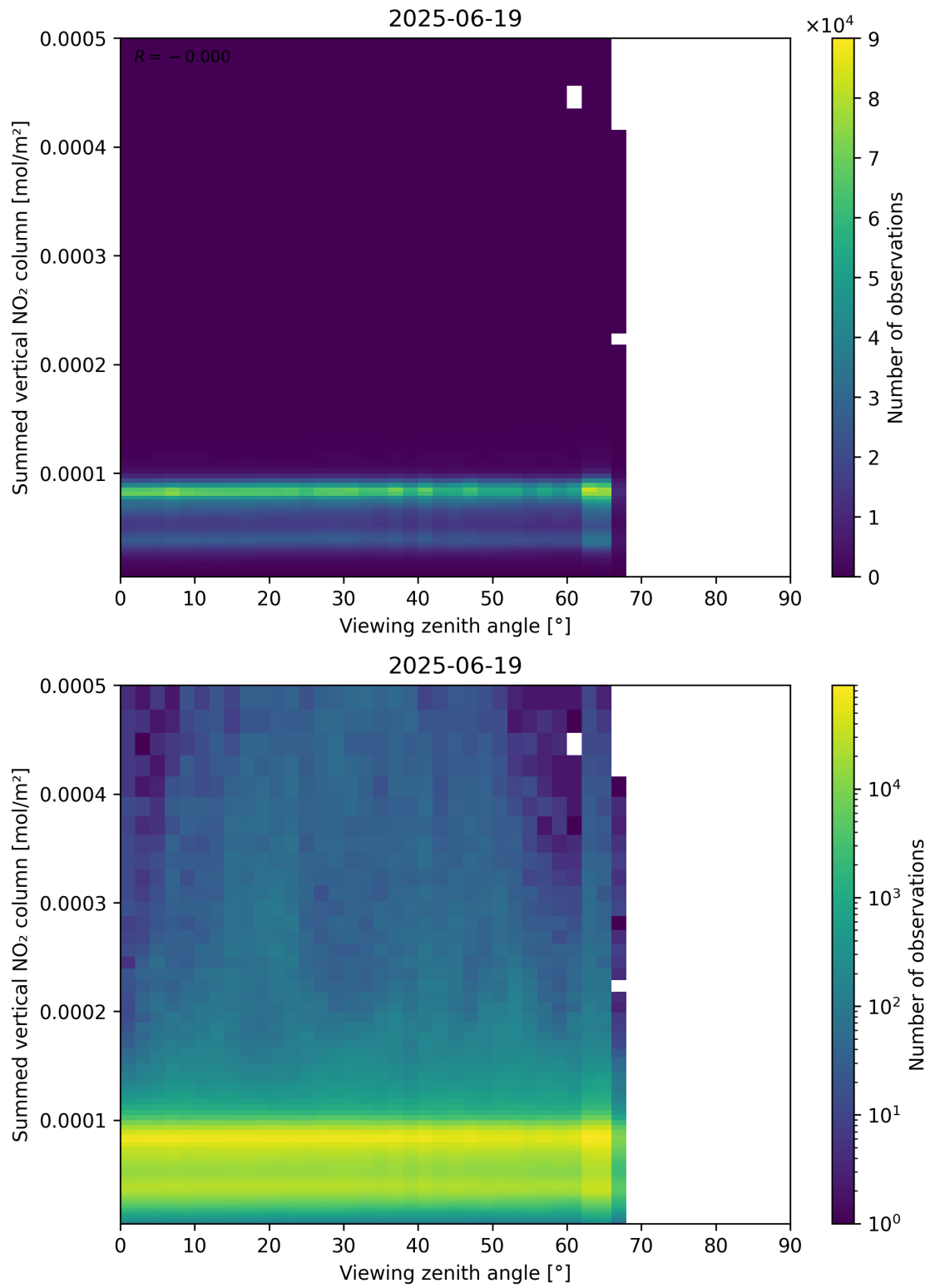
Figure 165: Scatter density plot of “Viewing zenith angle” against “Summed vertical NO 2 column” for 2025-06-18 to 2025-06-20.
