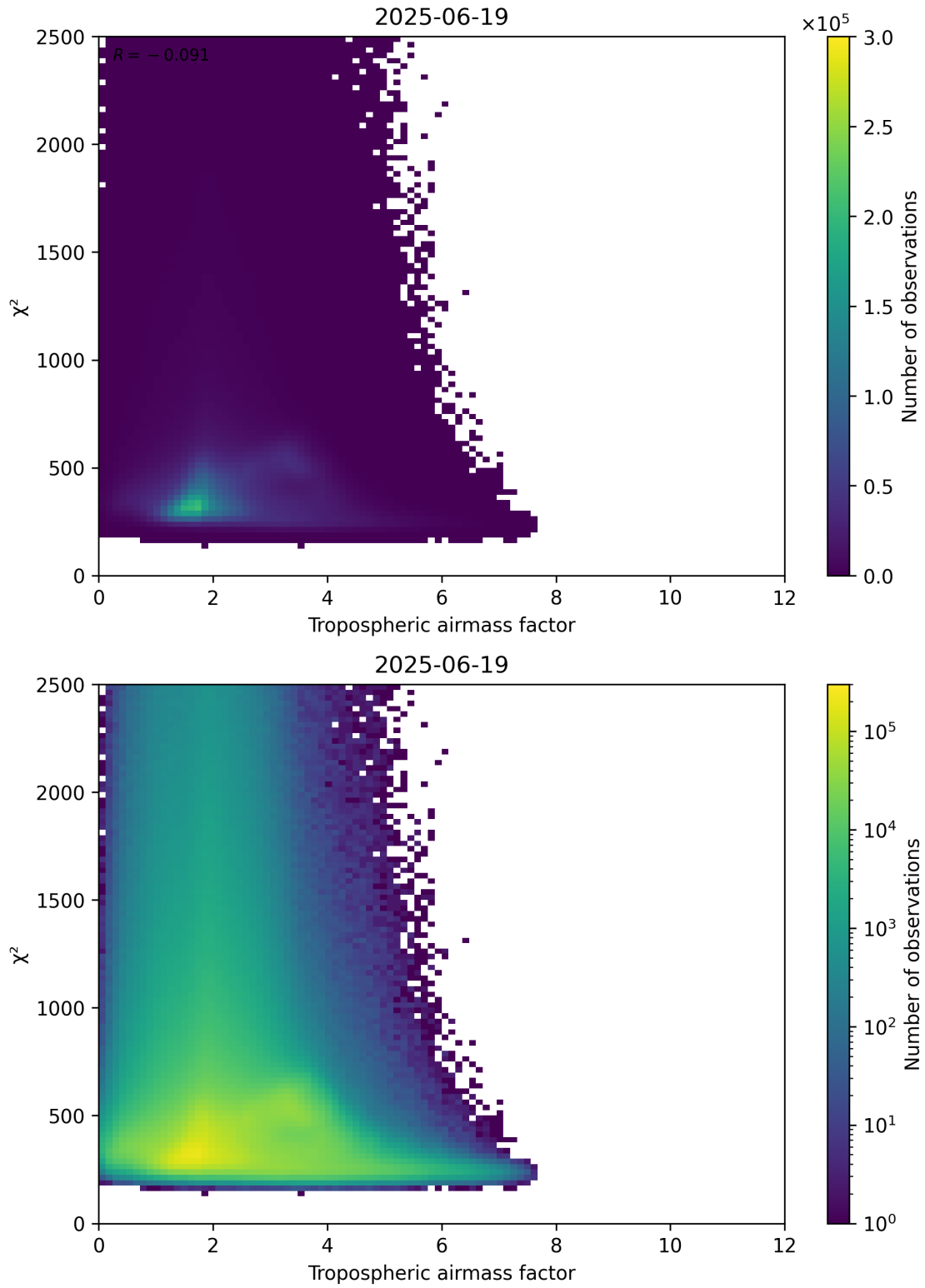
Figure 73: Scatter density plot of “Tropospheric airmass factor” against “ \chi^2 ” for 2025-06-18 to 2025-06-20.
