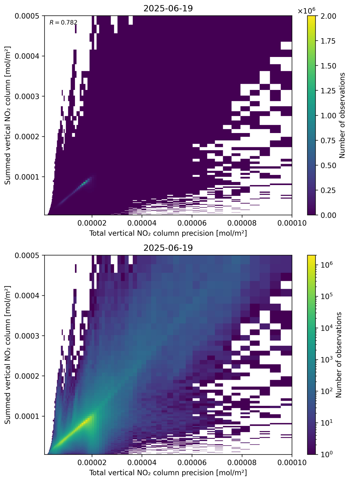
Figure 117: Scatter density plot of “Total vertical NO 2 column precision” against “Summed vertical NO 2 column” for 2025-06-18 to 2025-06-20.
