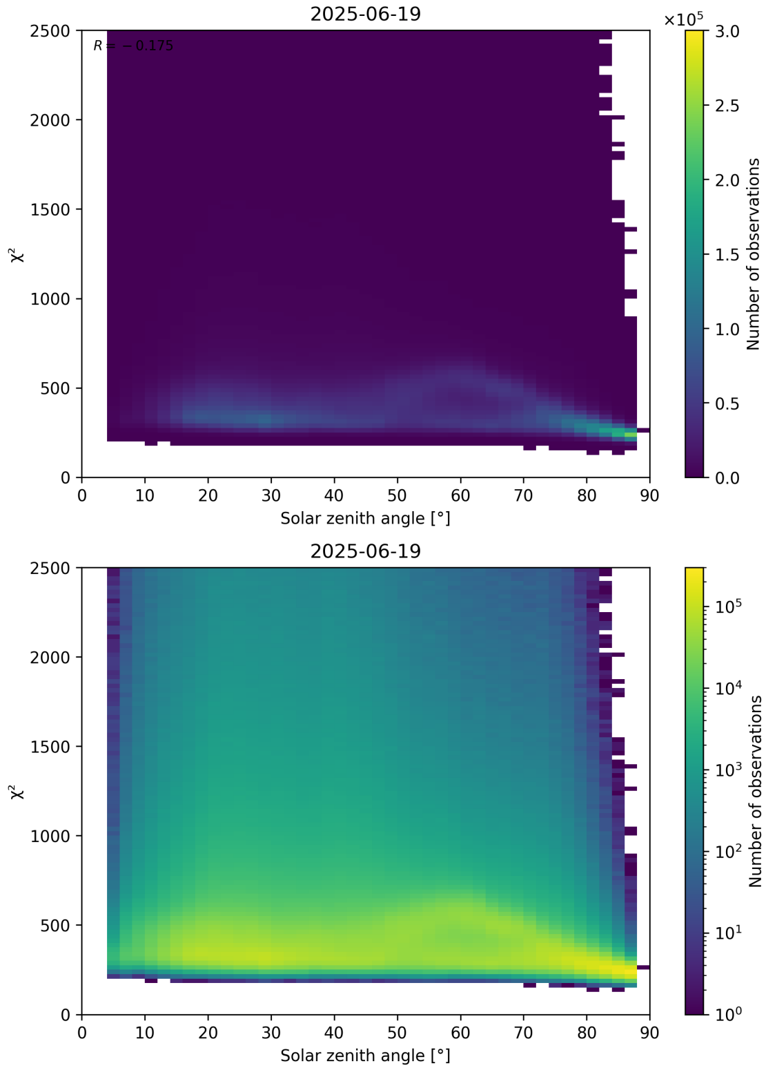
Figure 148: Scatter density plot of “Solar zenith angle” against “ \chi^2 ” for 2025-06-18 to 2025-06-20.
