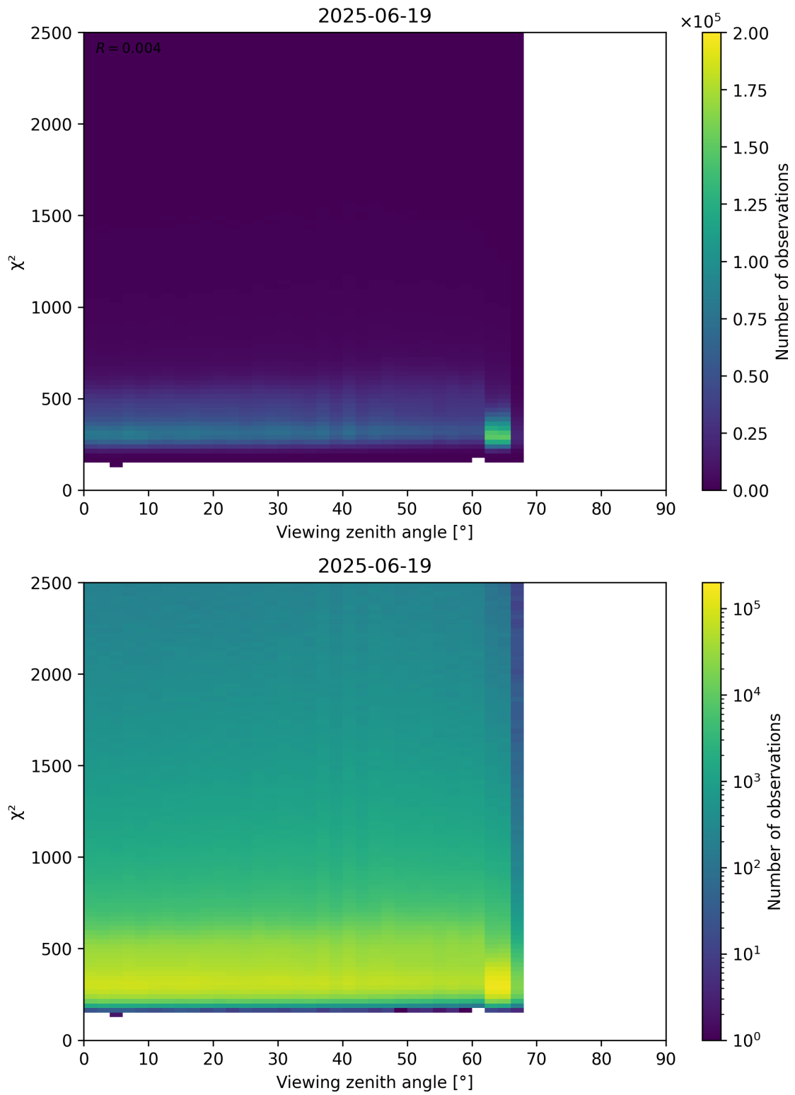
Figure 162: Scatter density plot of “Viewing zenith angle” against “ \chi^2 ” for 2025-06-18 to 2025-06-20.
