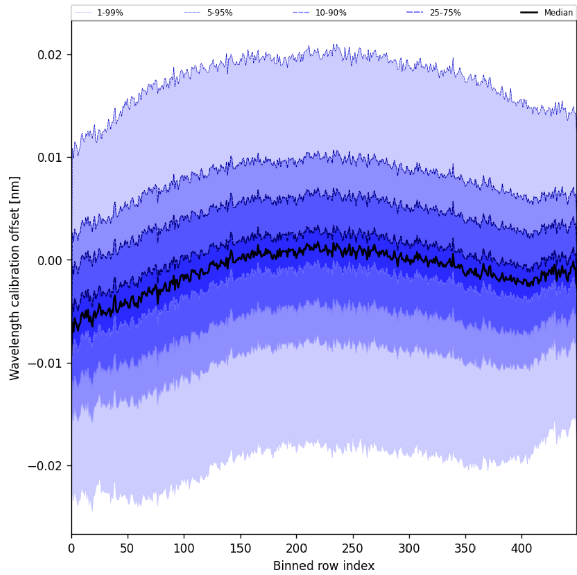
Figure 52: Along track statistics of “Wavelength calibration offset” for 2025-06-18 to 2025-06-20
