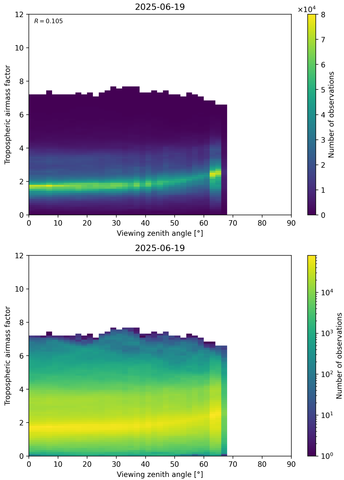
Figure 161: Scatter density plot of “Viewing zenith angle” against “Tropospheric airmass factor” for 2025-06-18 to 2025-06-20.
