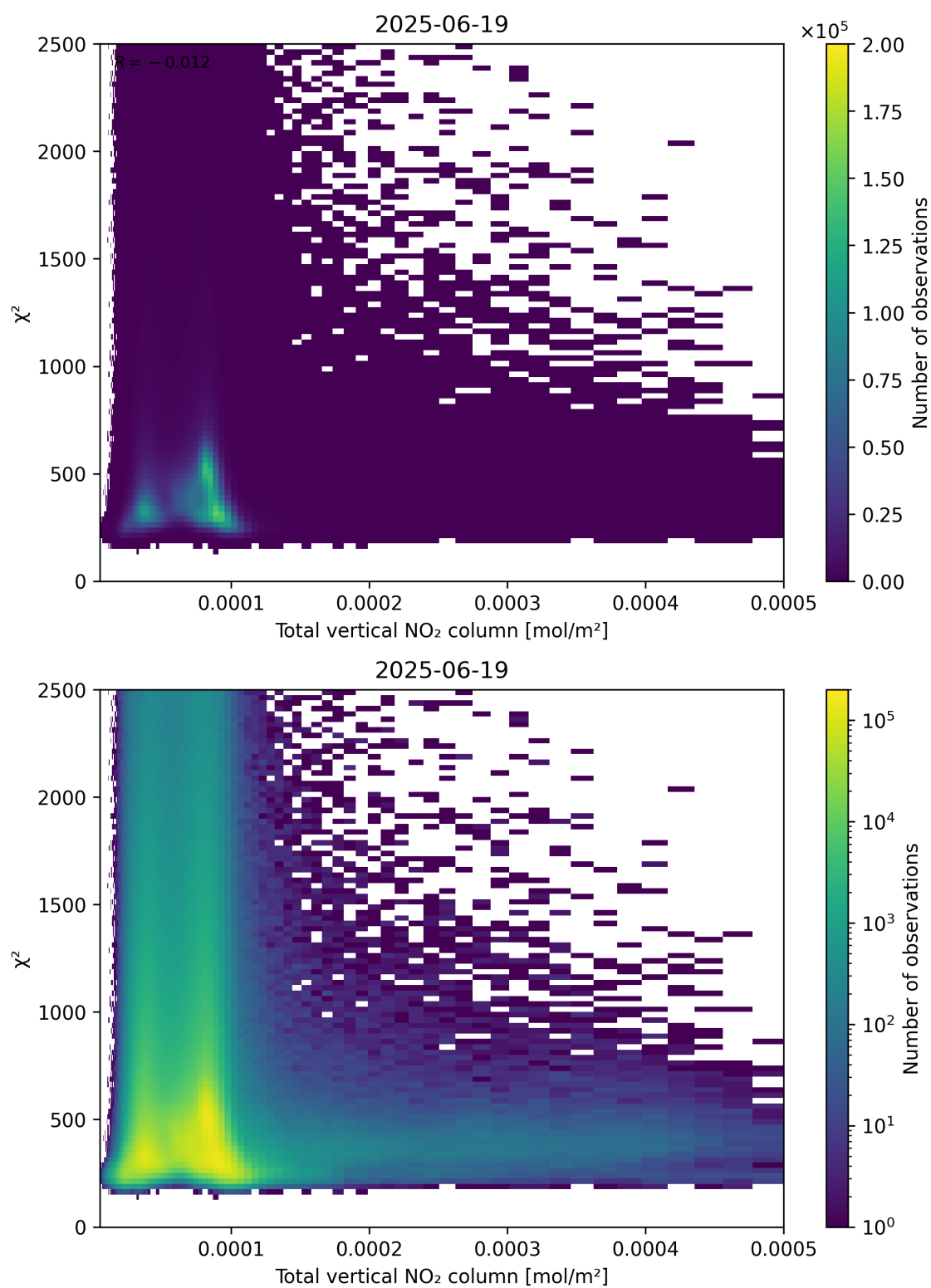
Figure 111: Scatter density plot of “Total vertical NO 2 column” against “ \chi^2 ” for 2025-06-18 to 2025-06-20.
