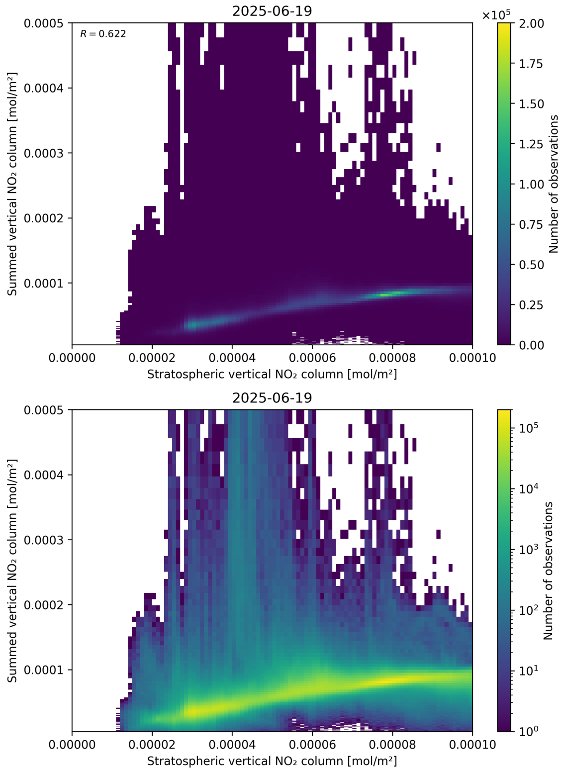
Figure 98: Scatter density plot of “Stratospheric vertical NO 2 column” against “Summed vertical NO 2 column” for 2025-06-18 to 2025-06-20.
