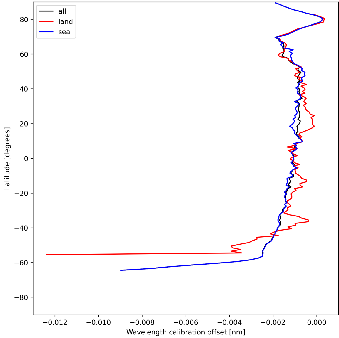
Figure 18: Zonal average of “Wavelength calibration offset” for 2025-06-18 to 2025-06-20.
