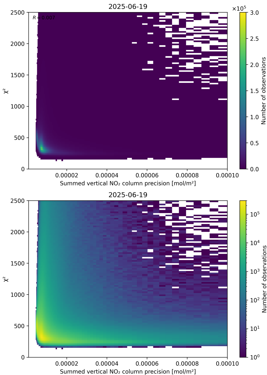
Figure 107: Scatter density plot of “Summed vertical NO 2 column precision” against “ \chi^2 ” for 2025-06-18 to 2025-06-20.
