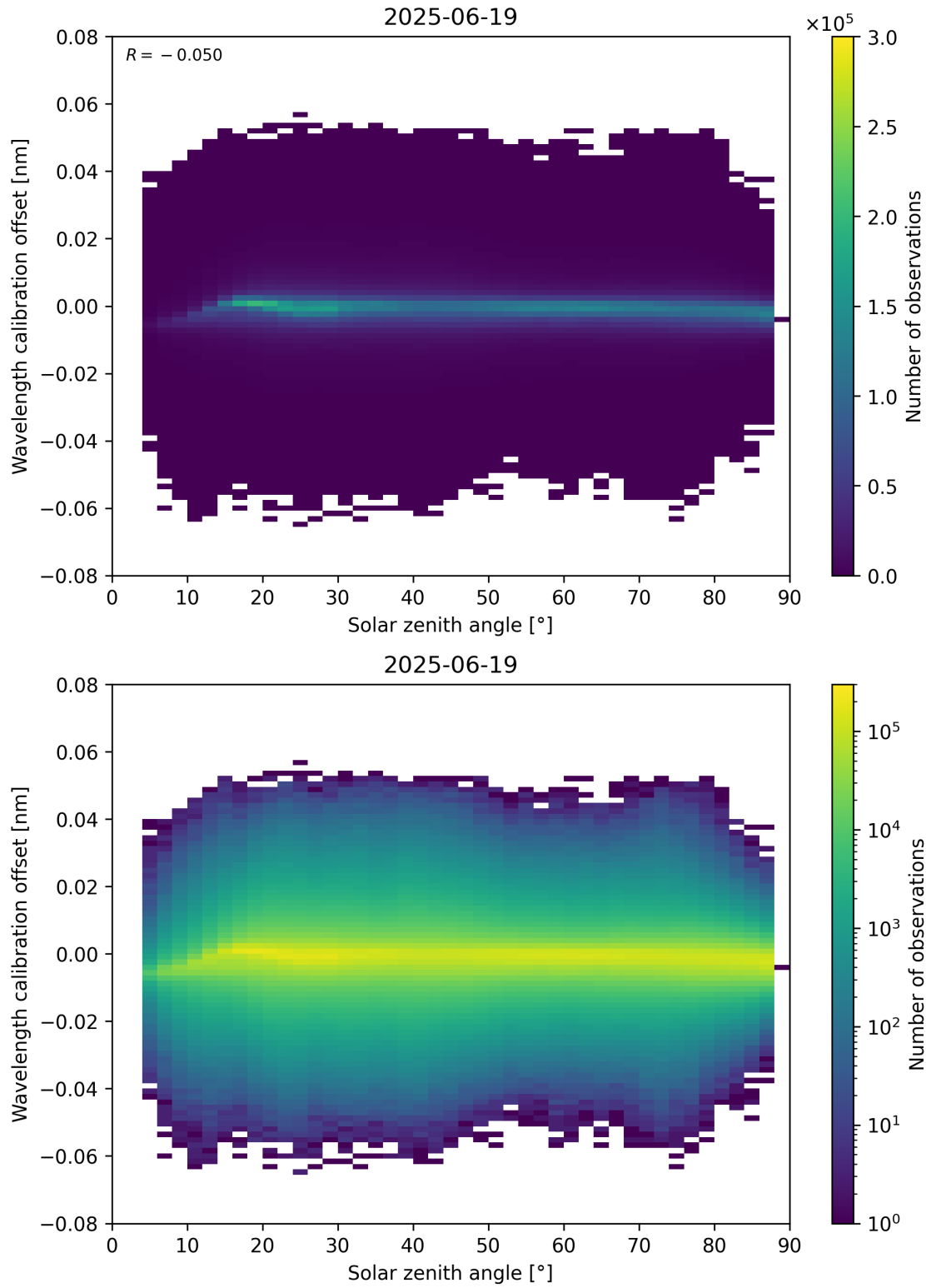
Figure 158: Scatter density plot of “Solar zenith angle” against “Wavelength calibration offset” for 2025-06-18 to 2025-06-20.
