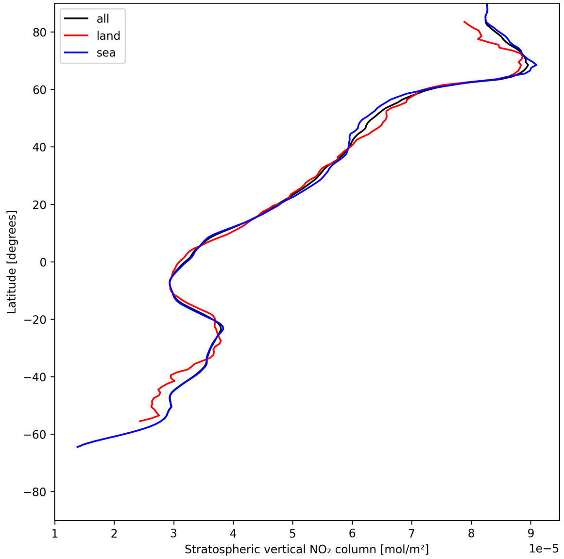
Figure 19: Zonal average of “Stratospheric vertical NO 2 column” for 2025-06-18 to 2025-06-20.
