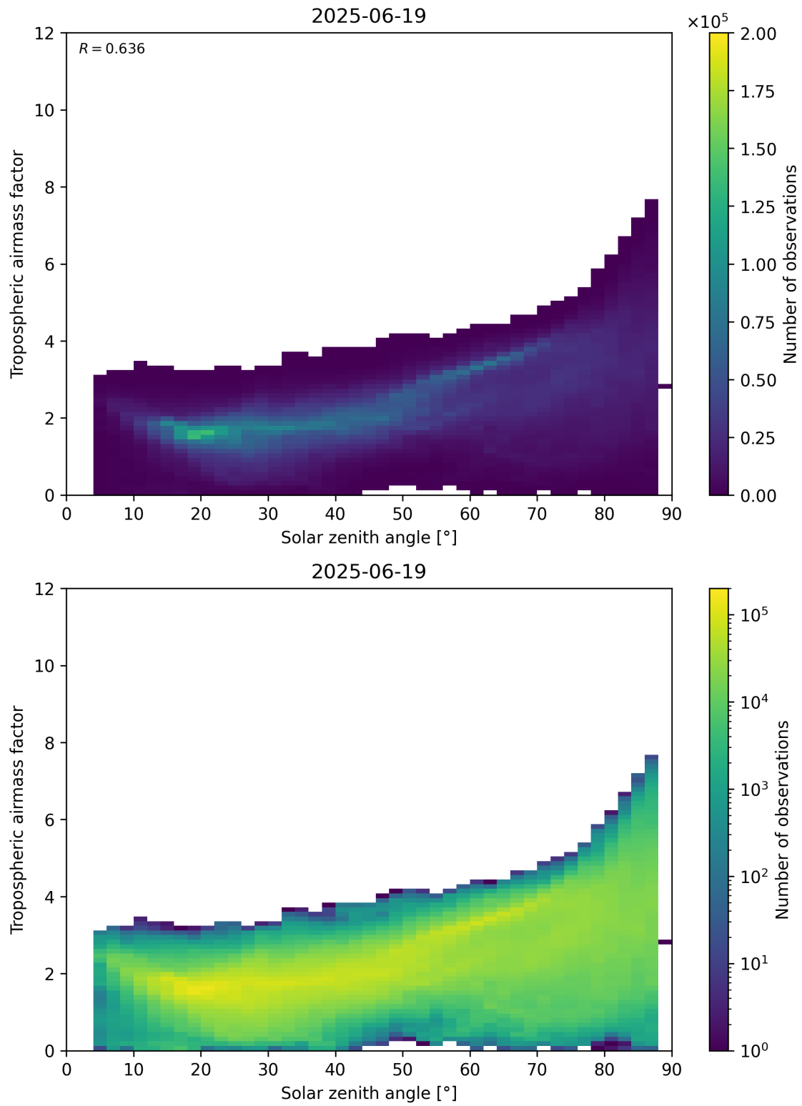
Figure 147: Scatter density plot of “Solar zenith angle” against “Tropospheric airmass factor” for 2025-06-18 to 2025-06-20.
