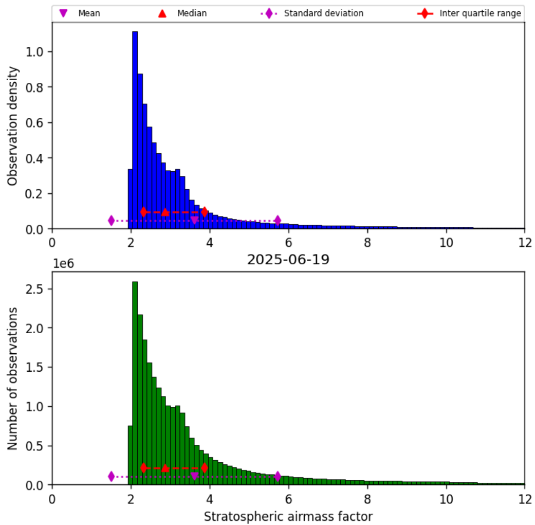
Figure 44: Histogram of “Stratospheric airmass factor” for 2025-06-18 to 2025-06-20
