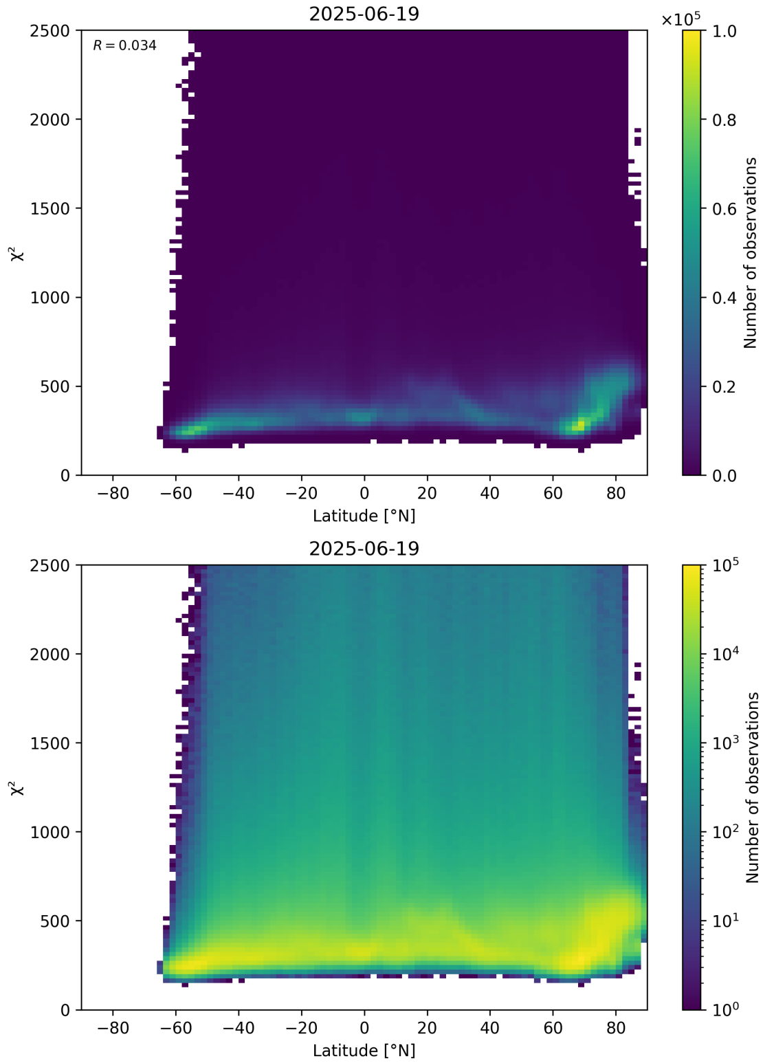
Figure 86: Scatter density plot of “Latitude” against “ \chi^2 ” for 2025-06-18 to 2025-06-20.
