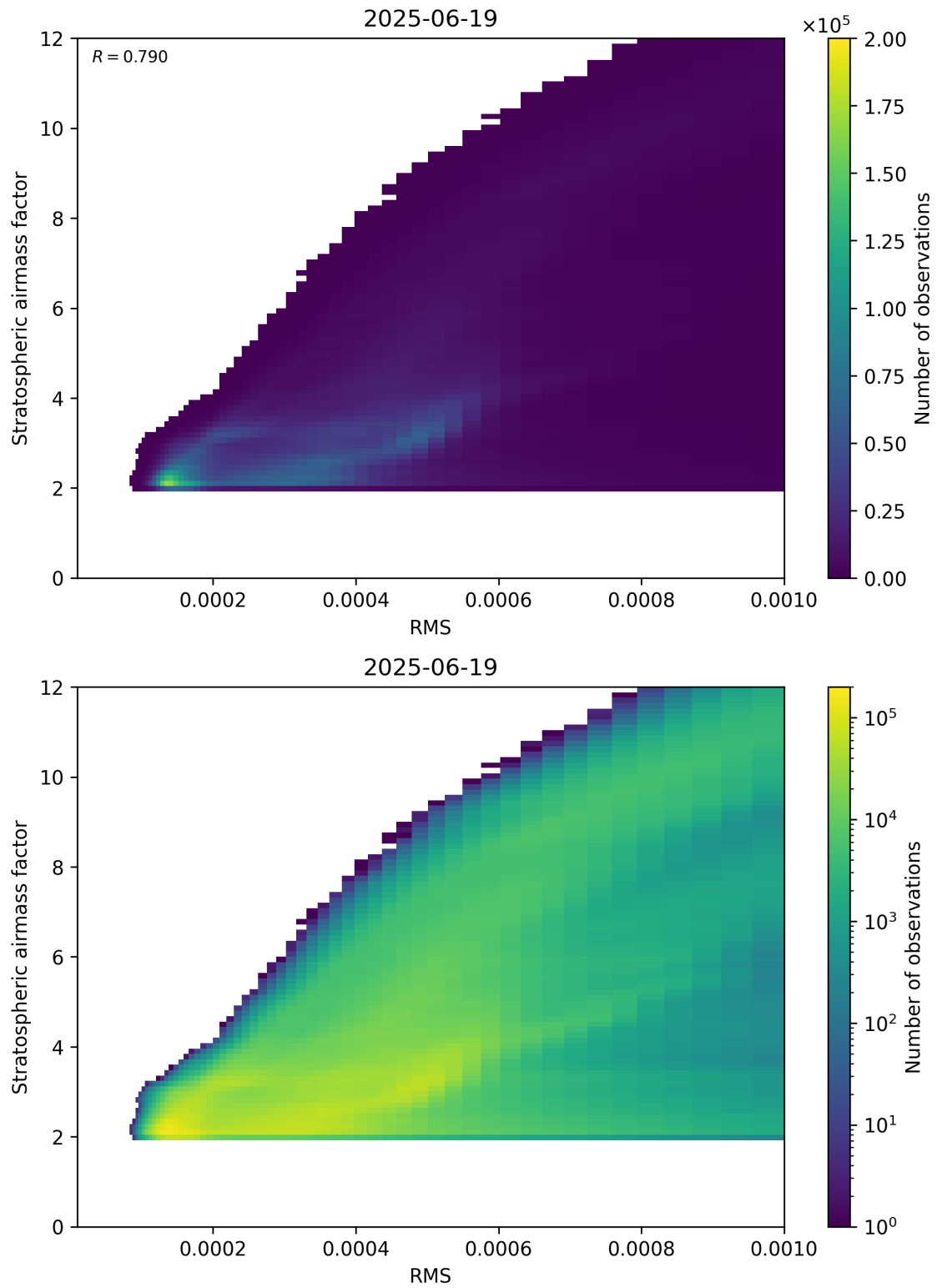
Figure 144: Scatter density plot of “RMS” against “Stratospheric airmass factor” for 2025-06-18 to 2025-06-20.
