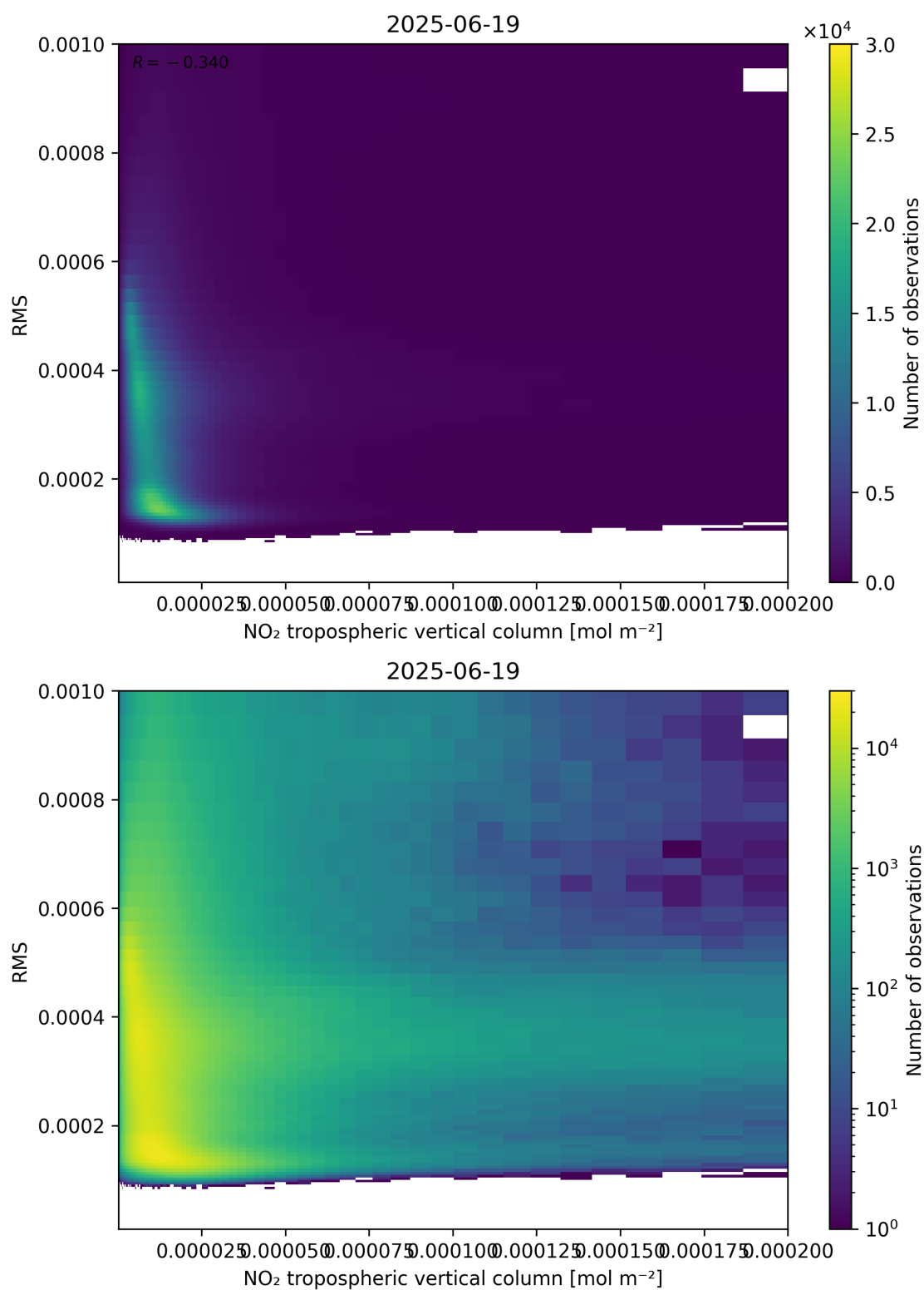
Figure 142: Scatter density plot of “NO 2 tropospheric vertical column” against “RMS” for 2025-06-18 to 2025-06-20.
