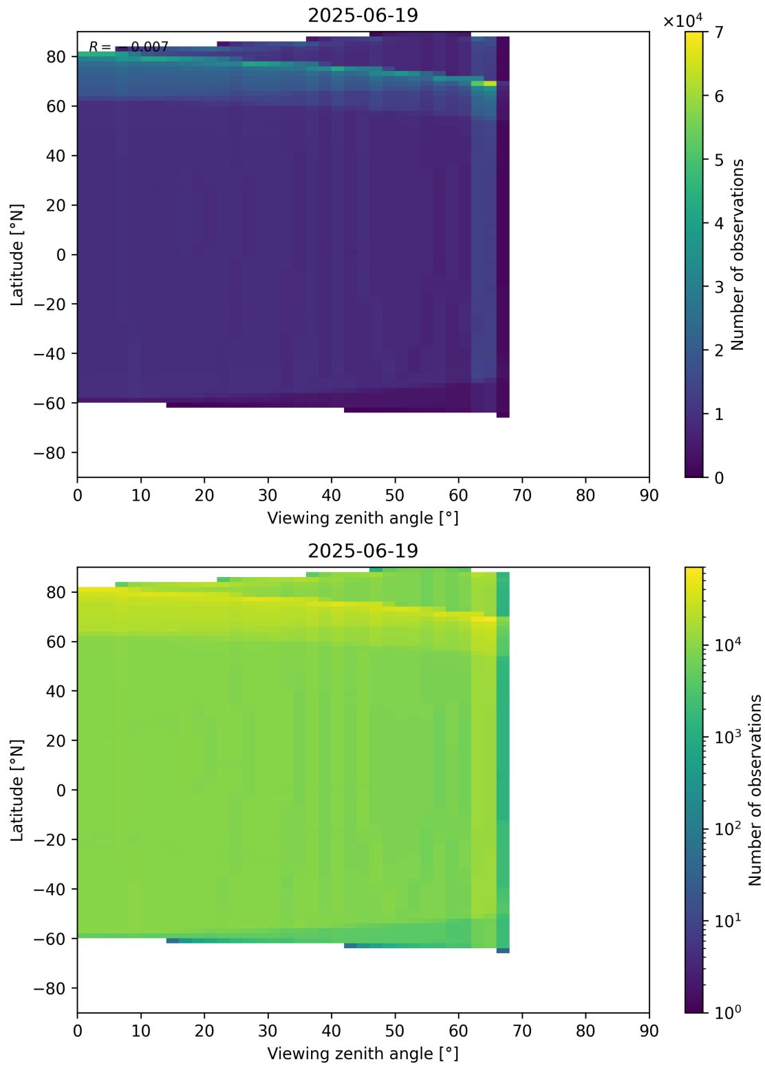
Figure 163: Scatter density plot of “Viewing zenith angle” against “Latitude” for 2025-06-18 to 2025-06-20.
