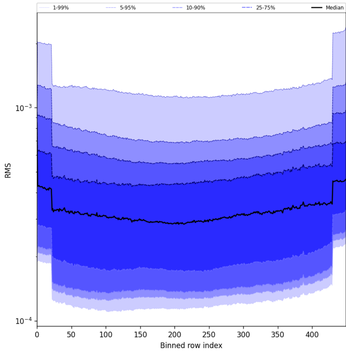
Figure 60: Along track statistics of “RMS” for 2025-06-18 to 2025-06-20
