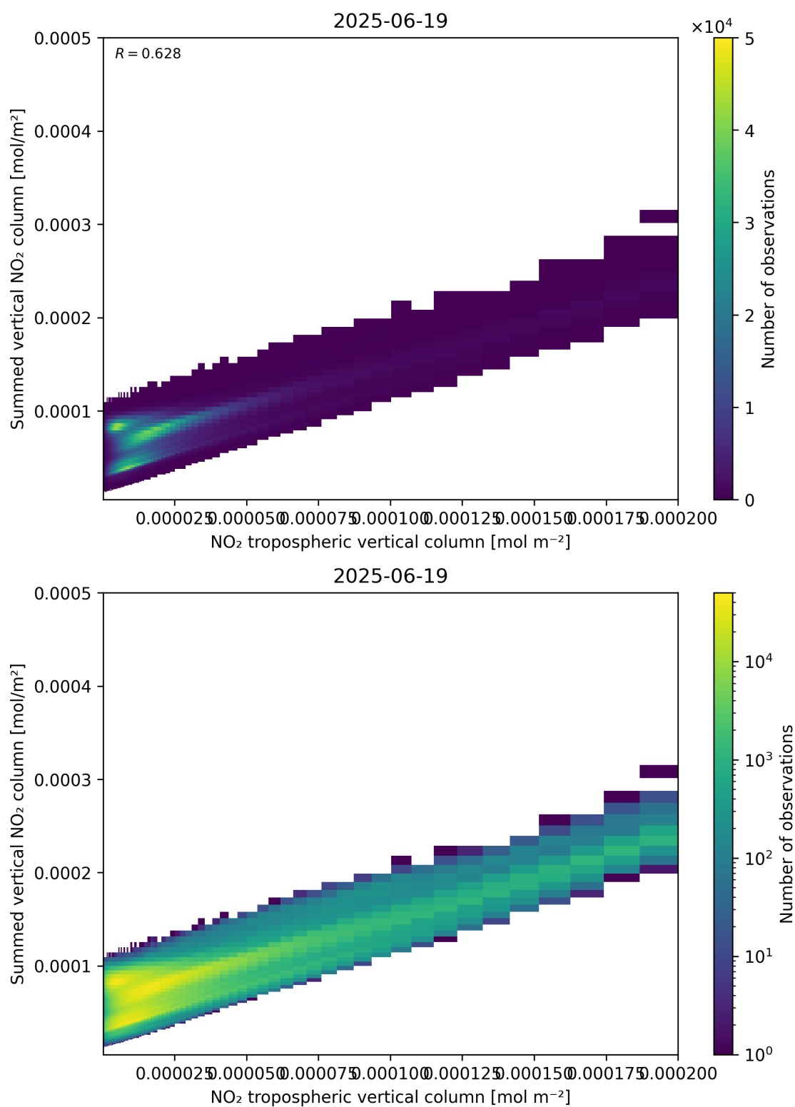
Figure 126: Scatter density plot of “NO 2 tropospheric vertical column” against “Summed vertical NO 2 column” for 2025-06-18 to 2025-06-20.
