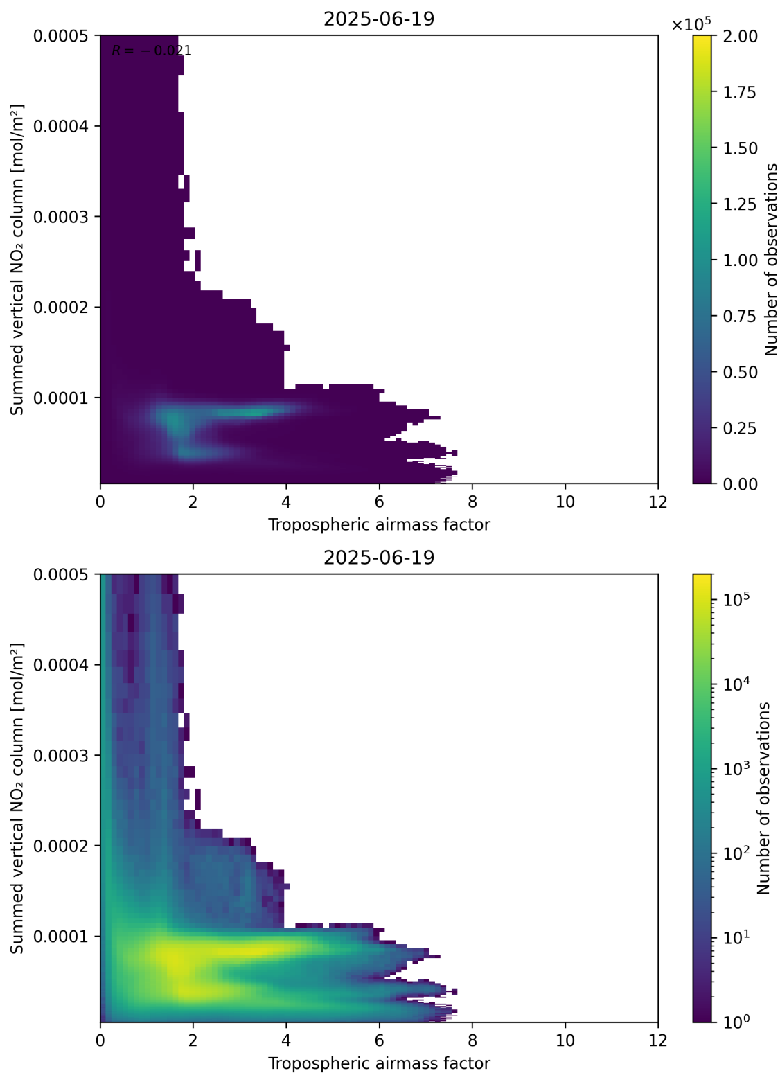
Figure 75: Scatter density plot of “Tropospheric airmass factor” against “Summed vertical NO 2 column” for 2025-06-18 to 2025-06-20.
