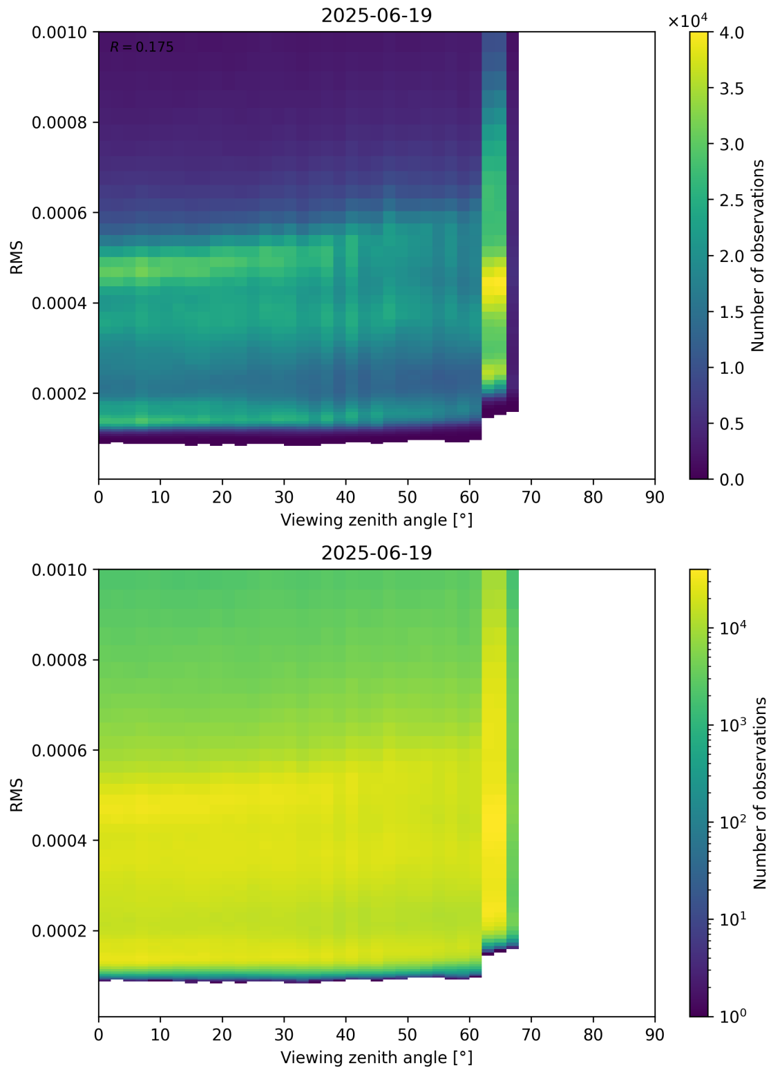
Figure 171: Scatter density plot of “Viewing zenith angle” against “RMS” for 2025-06-18 to 2025-06-20.
