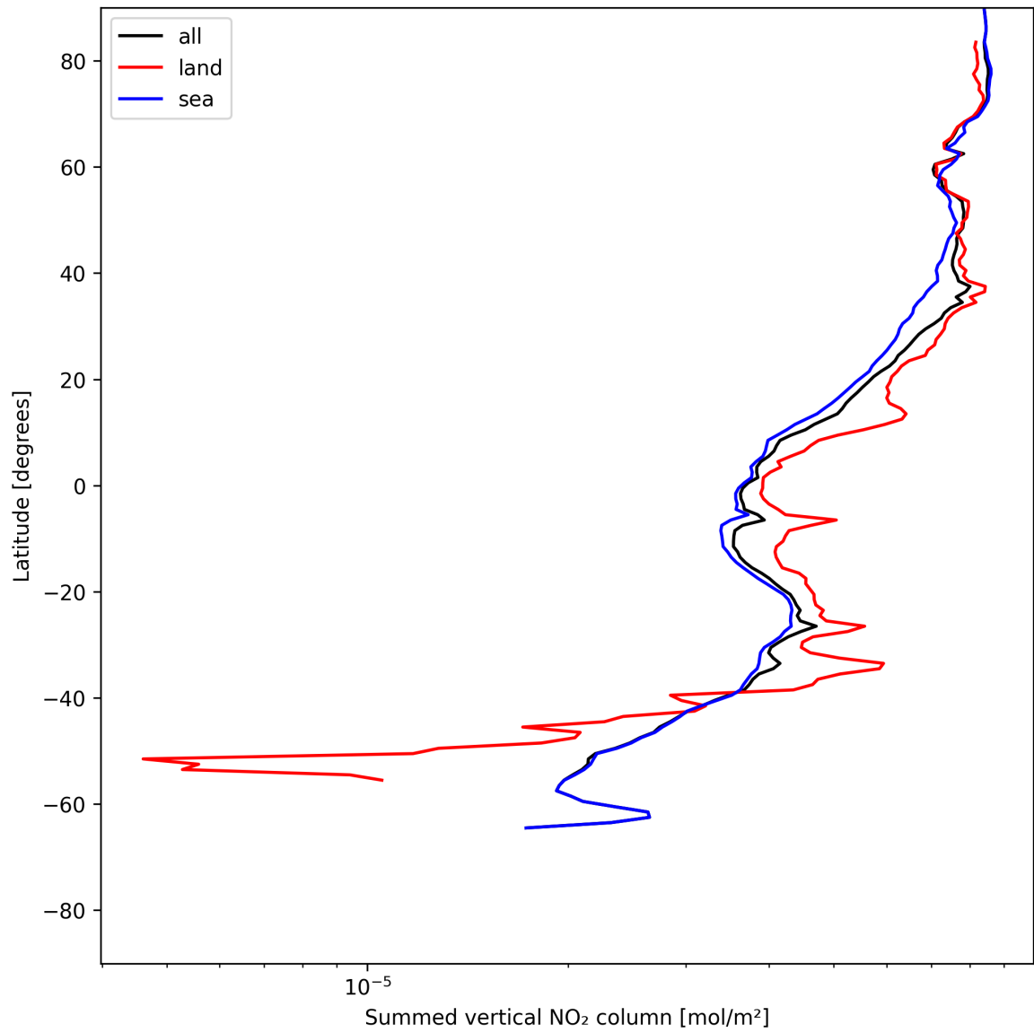
Figure 23: Zonal average of “Summed vertical NO 2 column” for 2025-06-18 to 2025-06-20.
