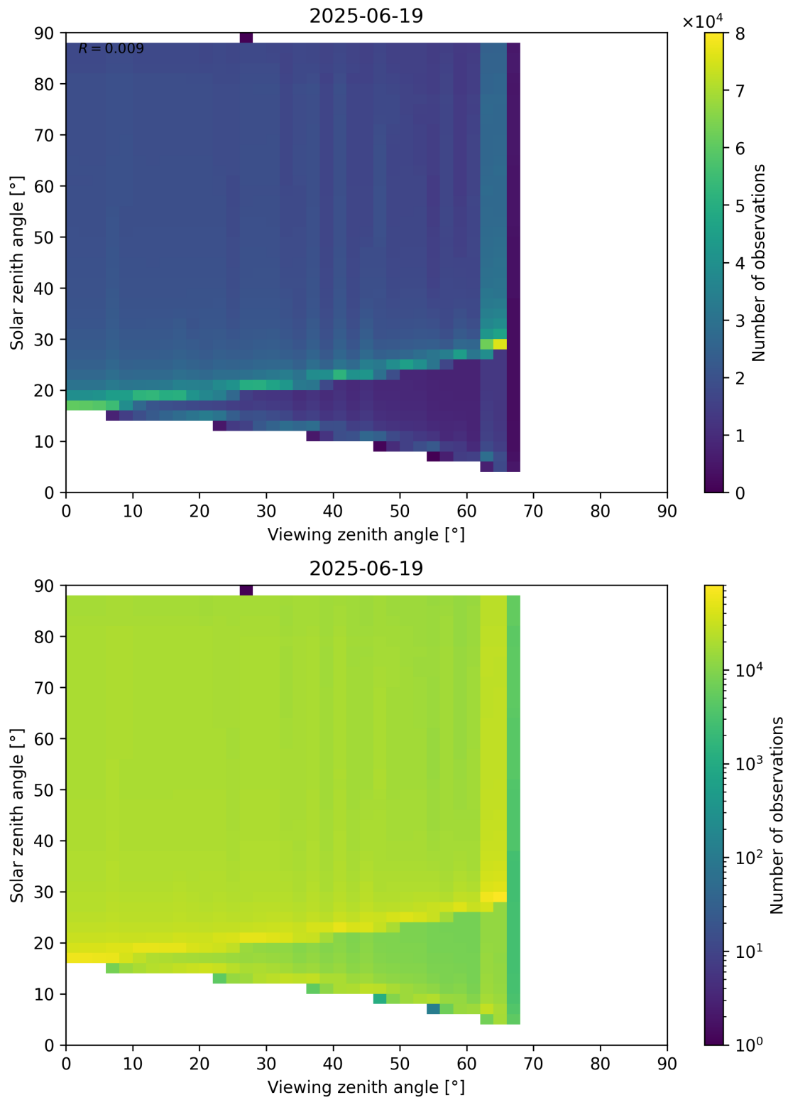
Figure 172: Scatter density plot of “Viewing zenith angle” against “Solar zenith angle” for 2025-06-18 to 2025-06-20.
