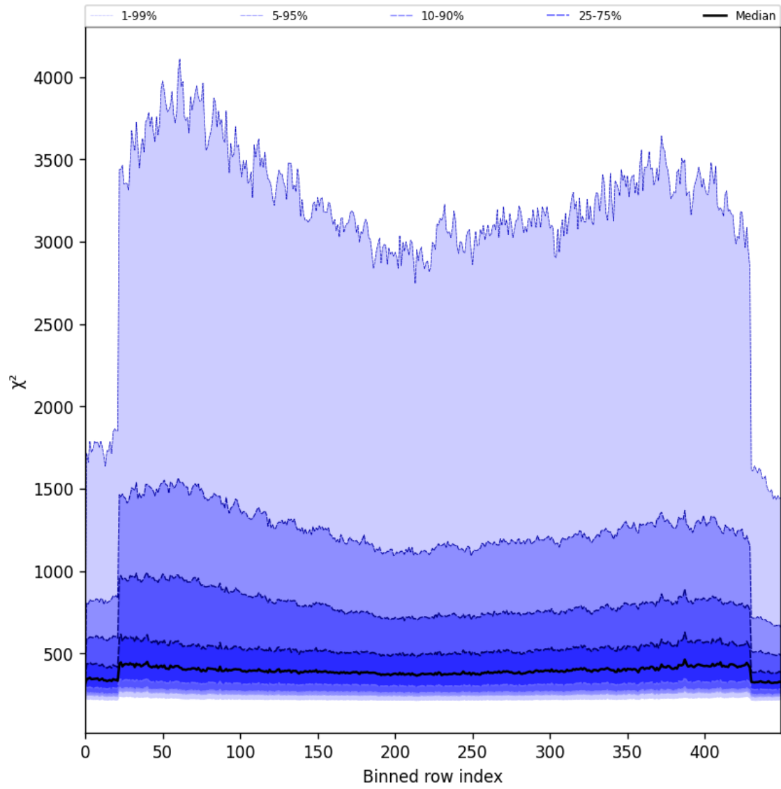
Figure 59: Along track statistics of “ \chi^2 ” for 2025-06-18 to 2025-06-20
