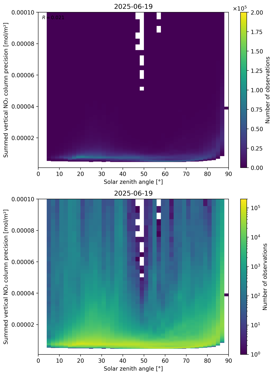
Figure 152: Scatter density plot of “Solar zenith angle” against “Summed vertical NO 2 column precision” for 2025-06-18 to 2025-06-20.
