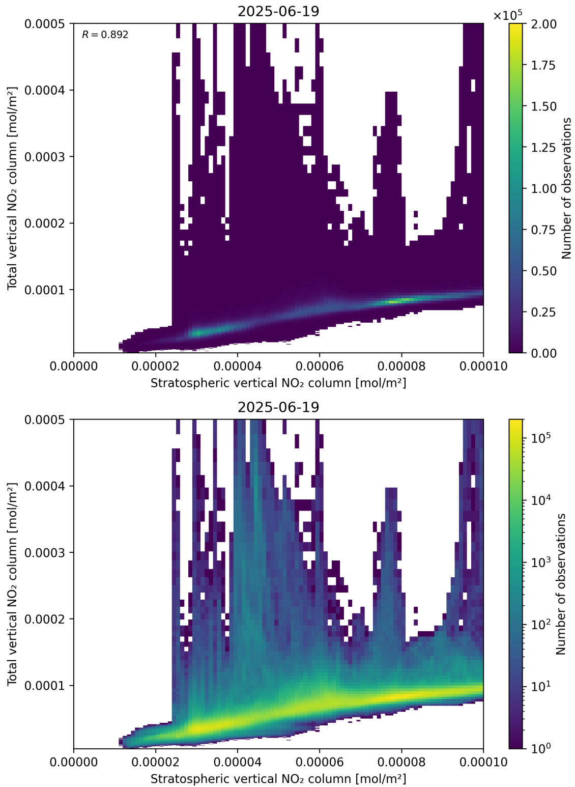
Figure 100: Scatter density plot of “Stratospheric vertical NO 2 column” against “Total vertical NO 2 column” for 2025-06-18 to 2025-06-20.
