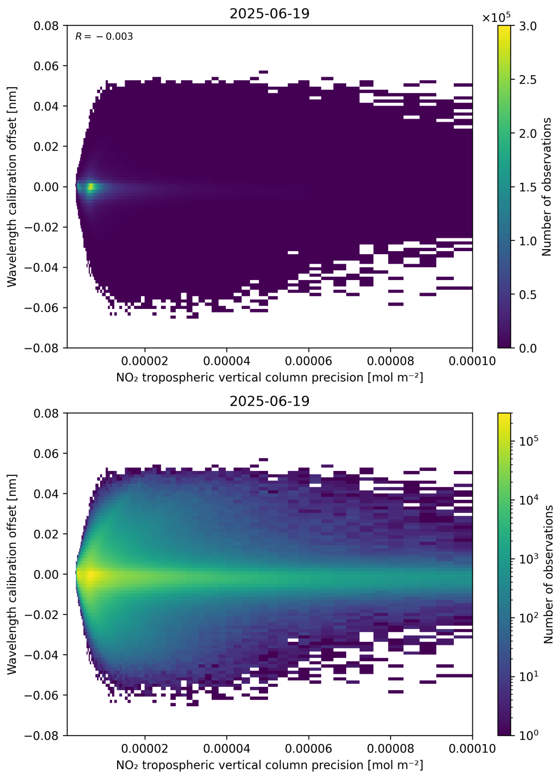
Figure 141: Scatter density plot of “NO 2 tropospheric vertical column precision” against “Wavelength calibration offset” for 2025-06-18 to 2025-06-20.
