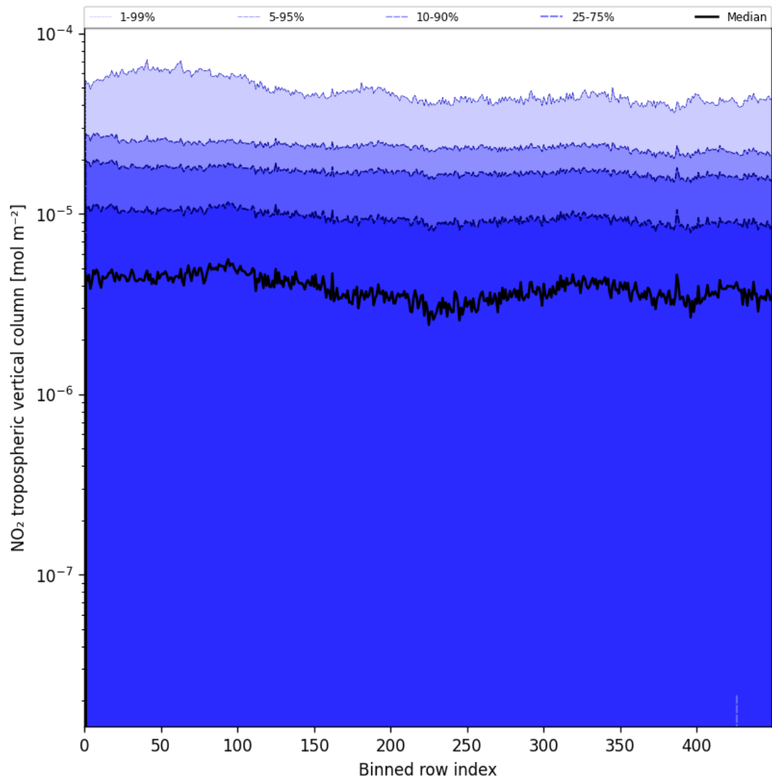
Figure 46: Along track statistics of “NO 2 tropospheric vertical column” for 2025-06-18 to 2025-06-20
