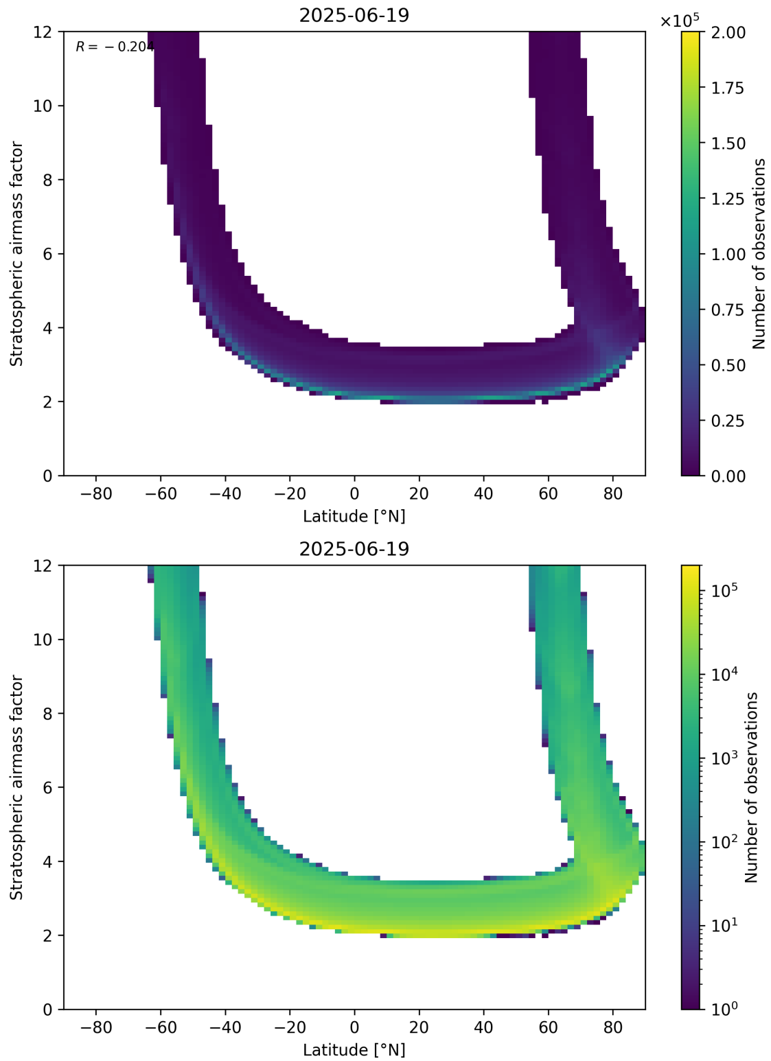
Figure 83: Scatter density plot of “Latitude” against “Stratospheric air mass factor” for 2025-06-18 to 2025-06-20.
