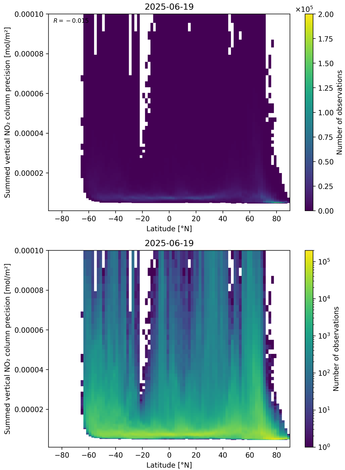
Figure 89: Scatter density plot of “Latitude” against “Summed vertical NO 2 column precision” for 2025-06-18 to 2025-06-20.
