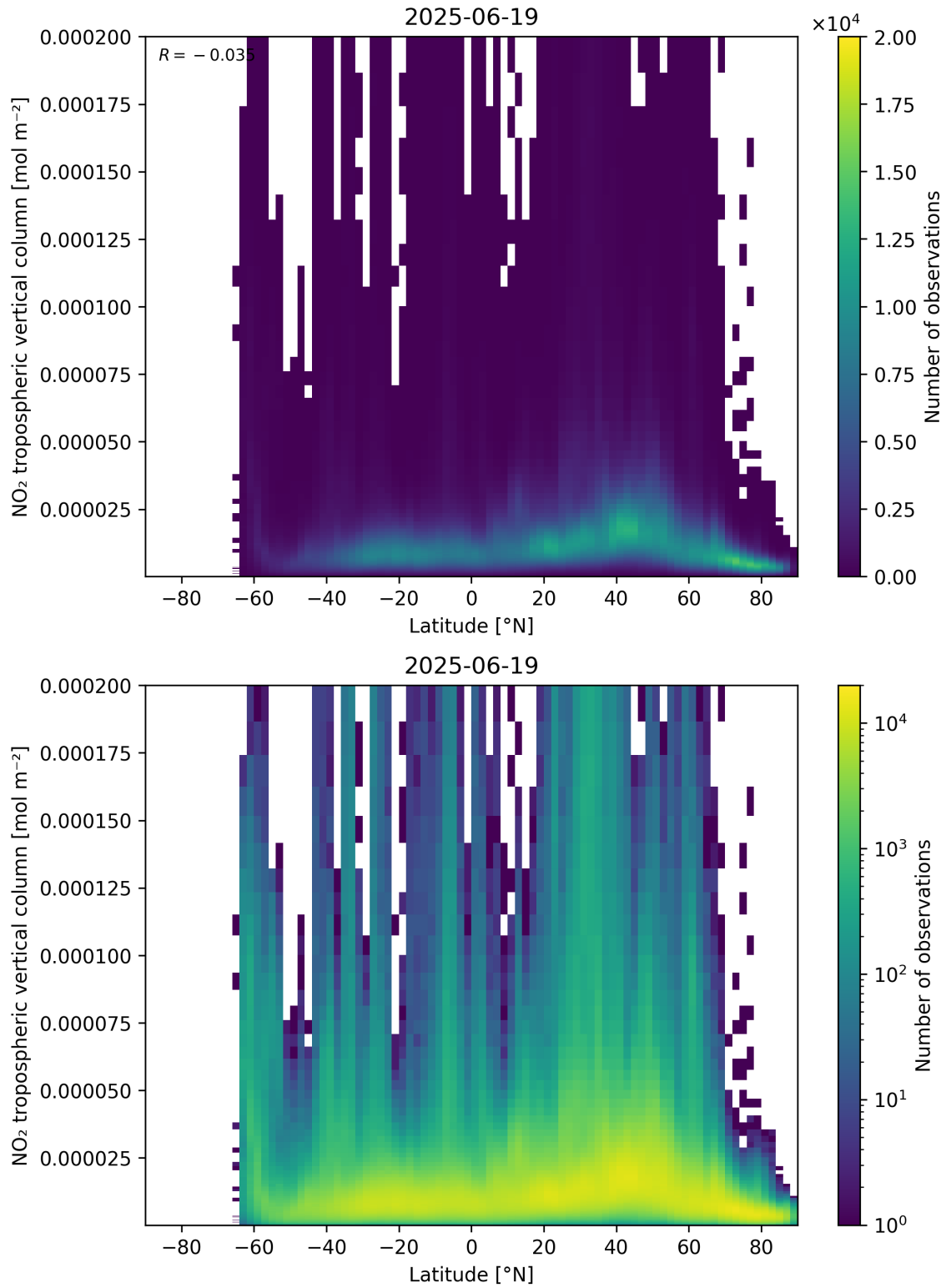
Figure 92: Scatter density plot of “Latitude” against “NO 2 tropospheric vertical column” for 2025-06-18 to 2025-06-20.
