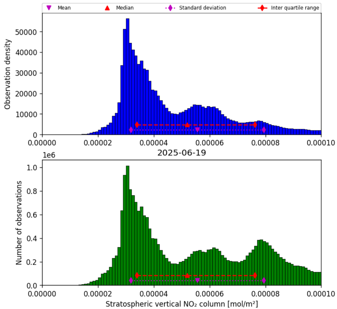
Figure 36: Histogram of “Stratospheric vertical NO 2 column” for 2025-06-18 to 2025-06-20
