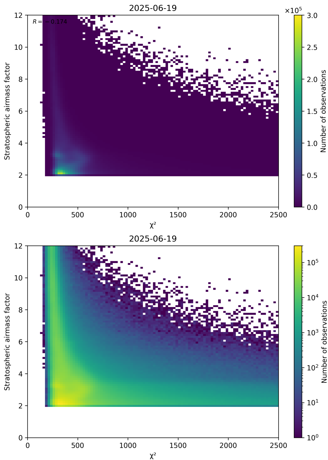
Figure 81: Scatter density plot of “ \chi^2 ” against “Stratospheric airmass factor” for 2025-06-18 to 2025-06-20.
