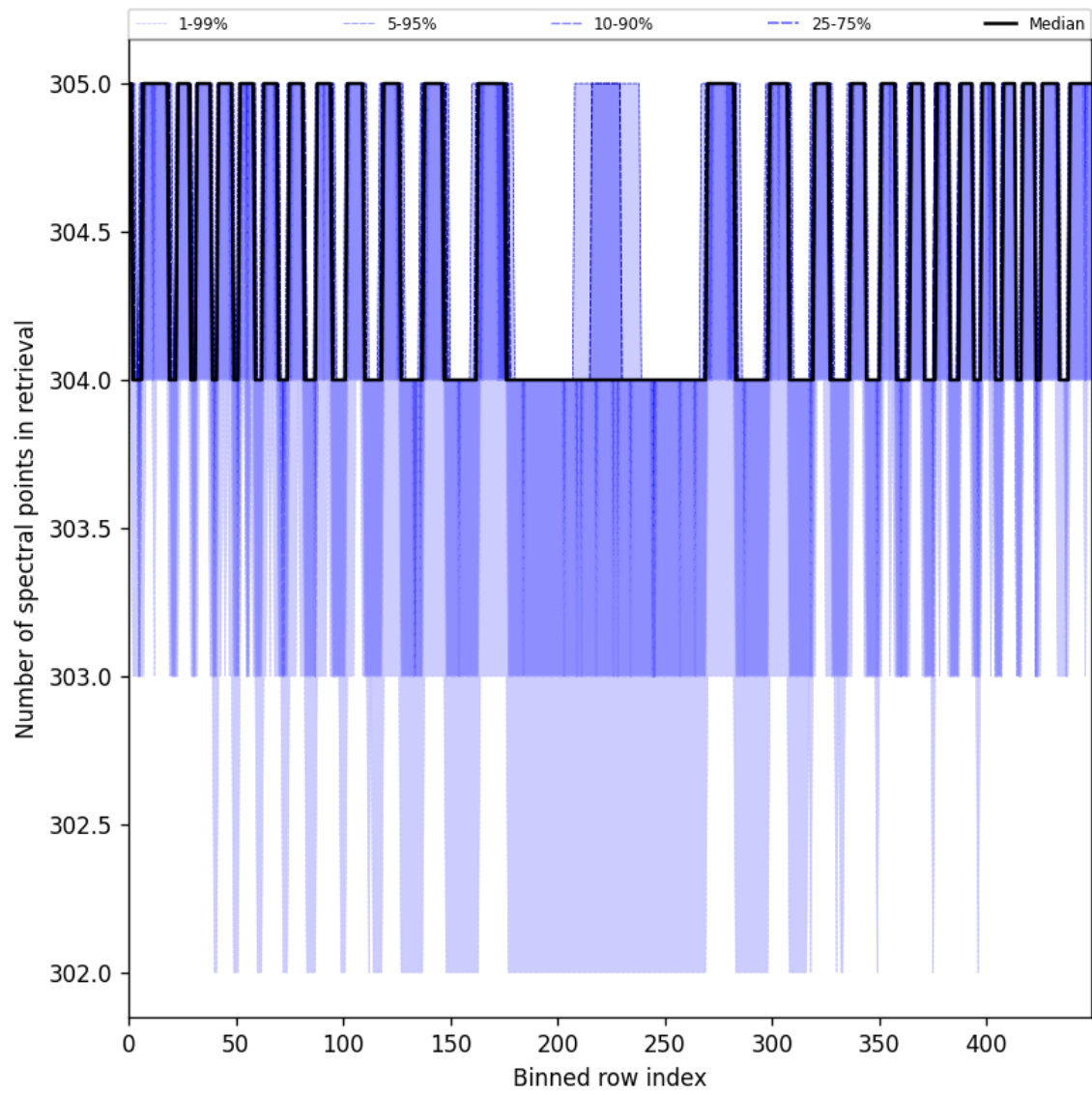
Figure 50: Along track statistics of “Number of spectral points in retrieval” for 2025-06-18 to 2025-06-20
