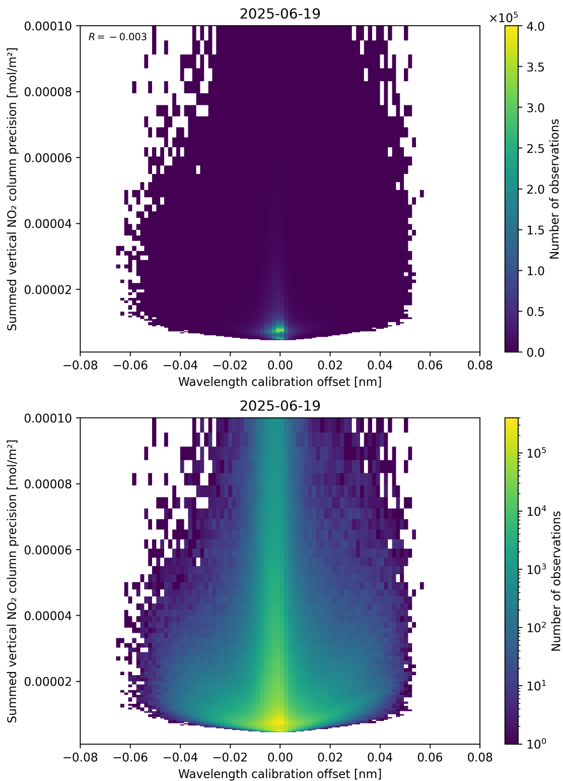
Figure 178: Scatter density plot of “Wavelength calibration offset” against “Summed vertical NO 2 column precision” for 2025-06-18 to 2025-06-20.
