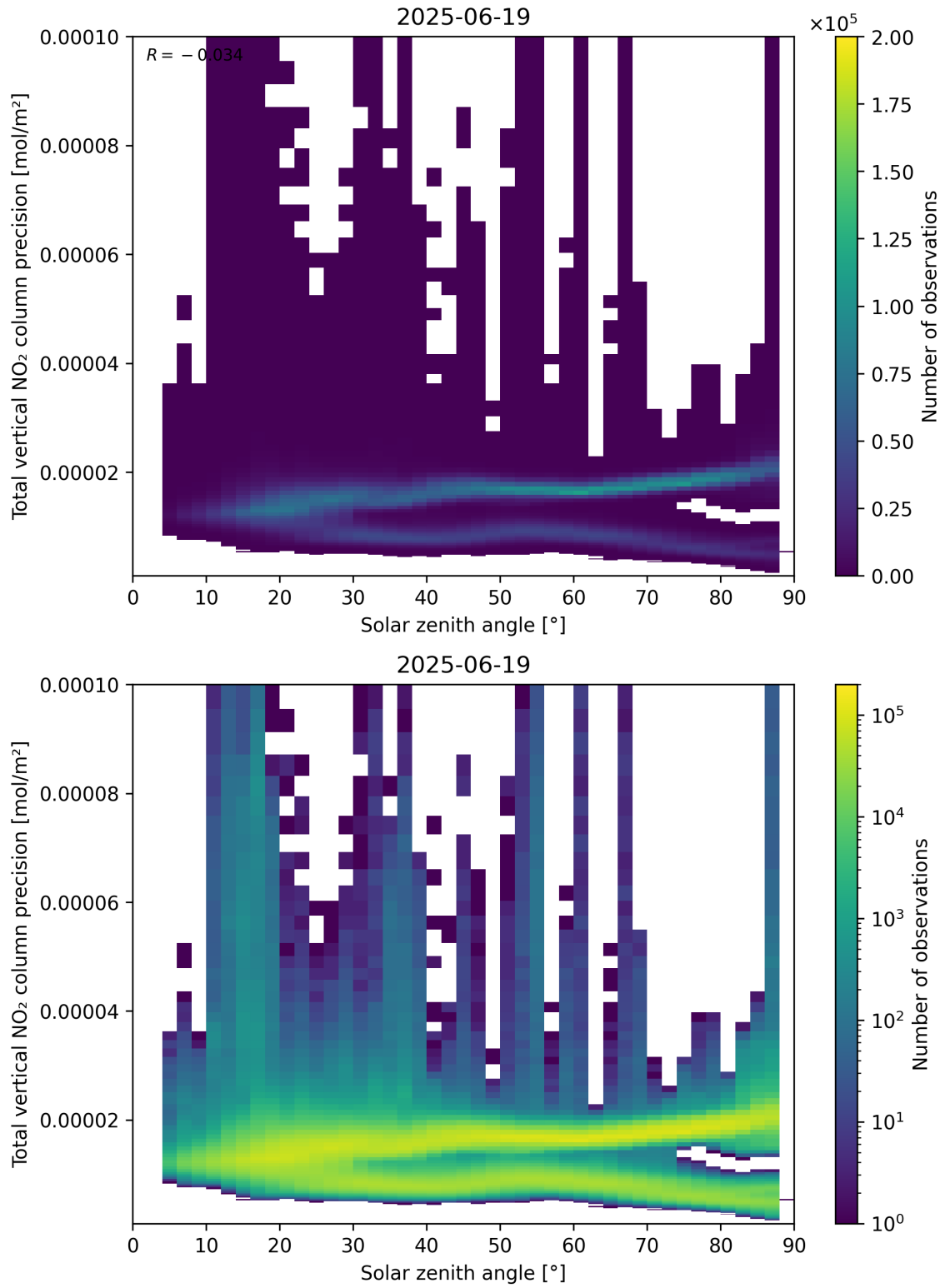
Figure 154: Scatter density plot of “Solar zenith angle” against “Total vertical NO 2 column precision” for 2025-06-18 to 2025-06-20.
