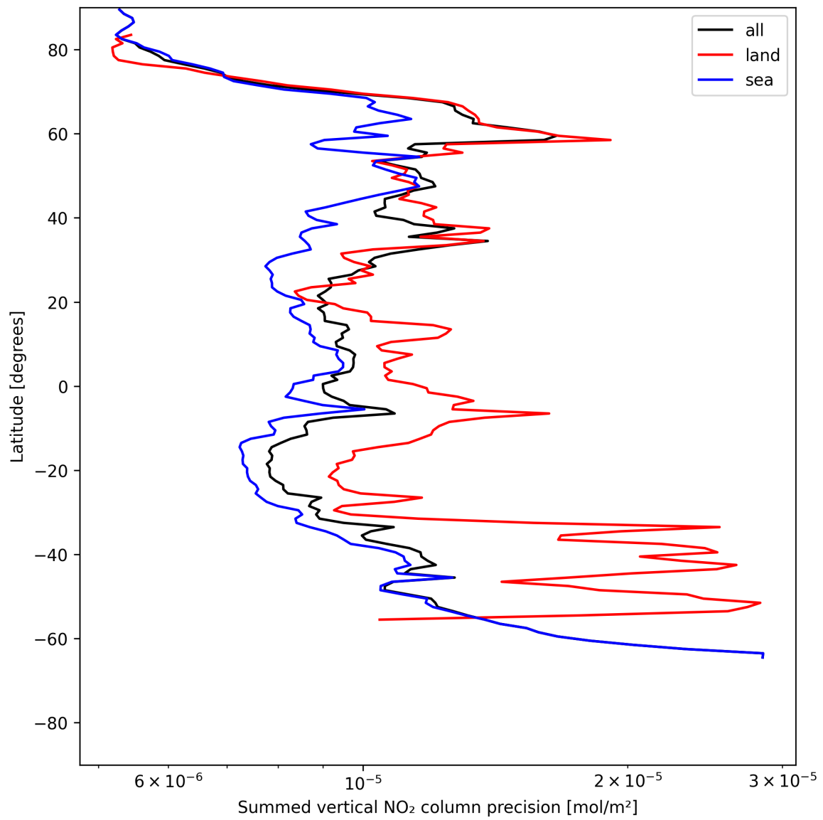
Figure 24: Zonal average of “Summed vertical NO 2 column precision” for 2025-06-18 to 2025-06-20.
