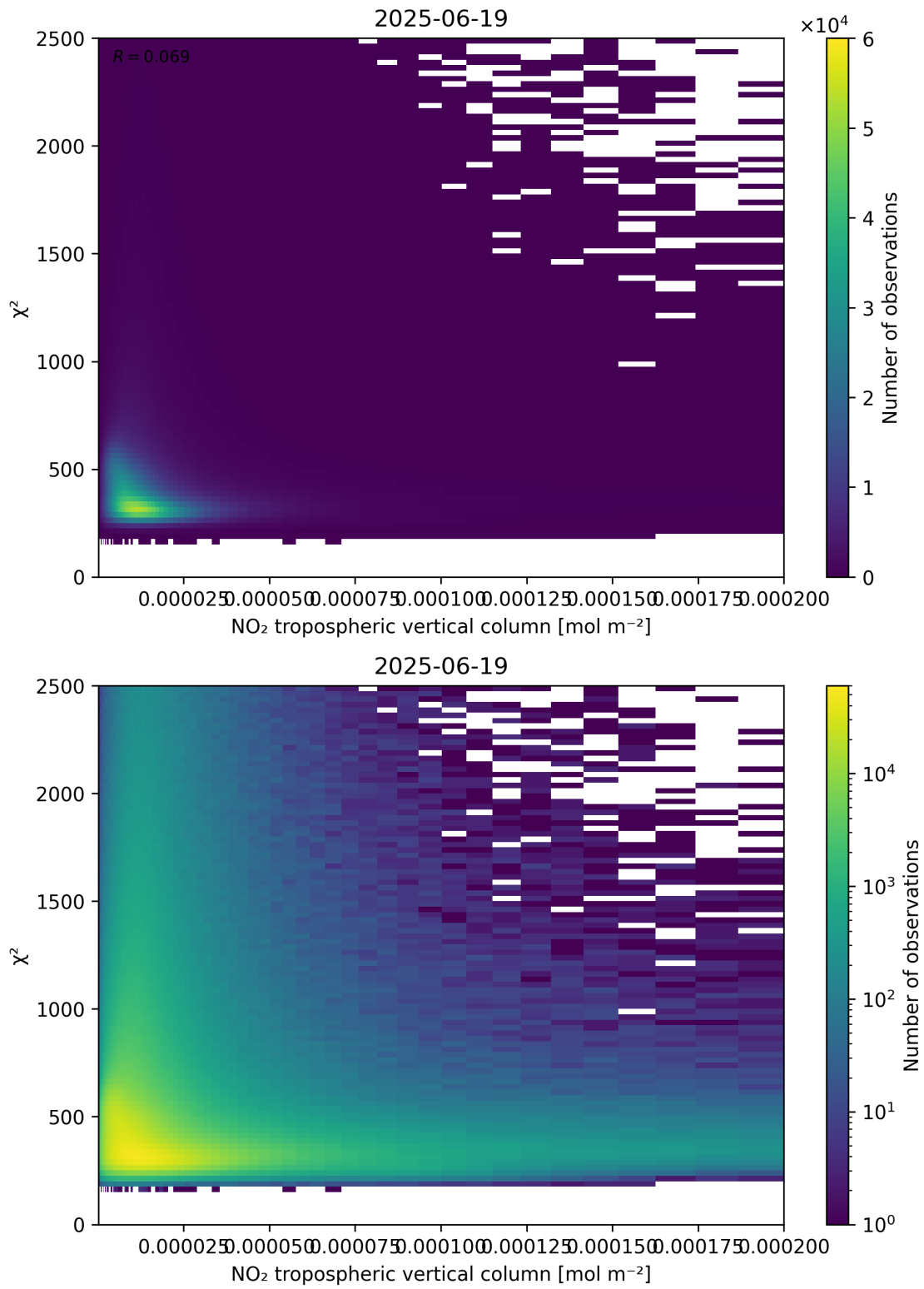
Figure 124: Scatter density plot of “NO 2 tropospheric vertical column” against “ \chi^2 ” for 2025-06-18 to 2025-06-20.
