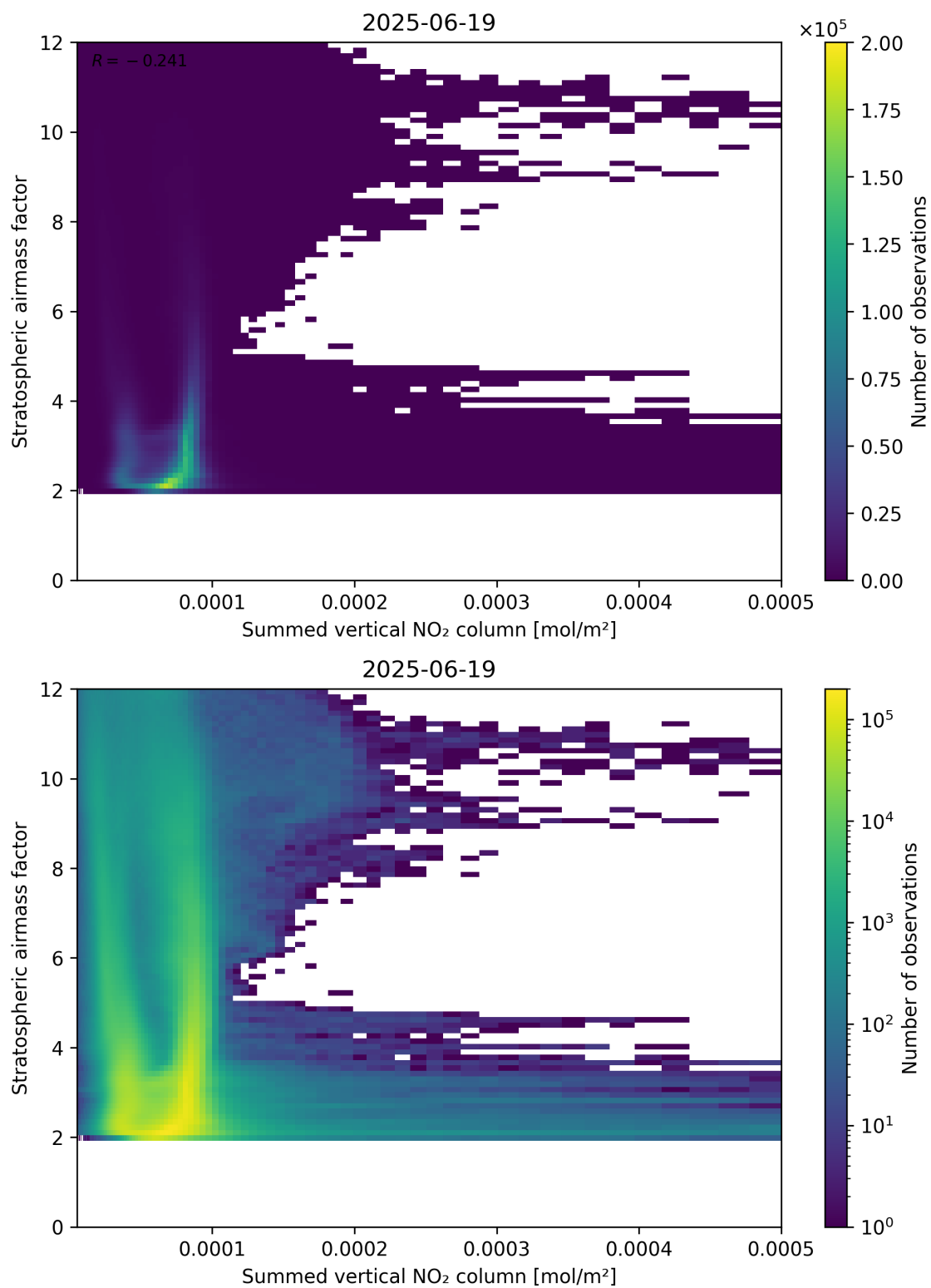
Figure 103: Scatter density plot of “Summed vertical NO 2 column” against “Stratospheric airmass factor” for 2025-06-18 to 2025-06-20.
