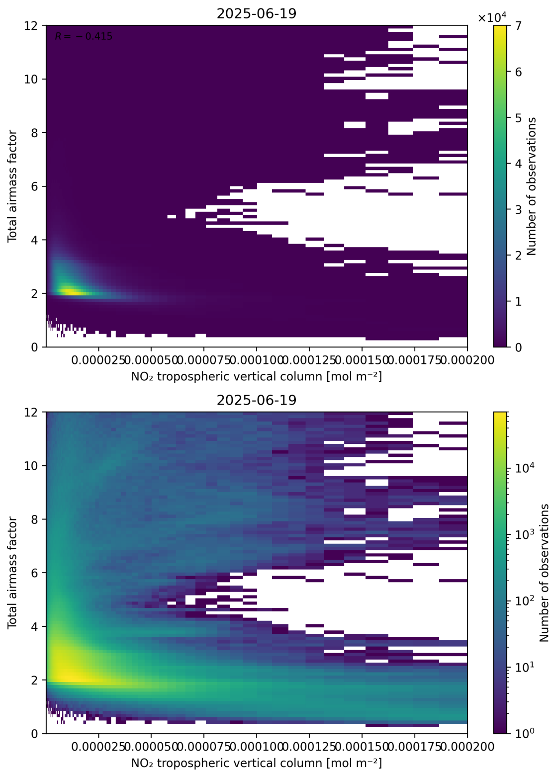
Figure 122: Scatter density plot of “NO 2 tropospheric vertical column” against “Total air mass factor” for 2025-06-18 to 2025-06-20.
