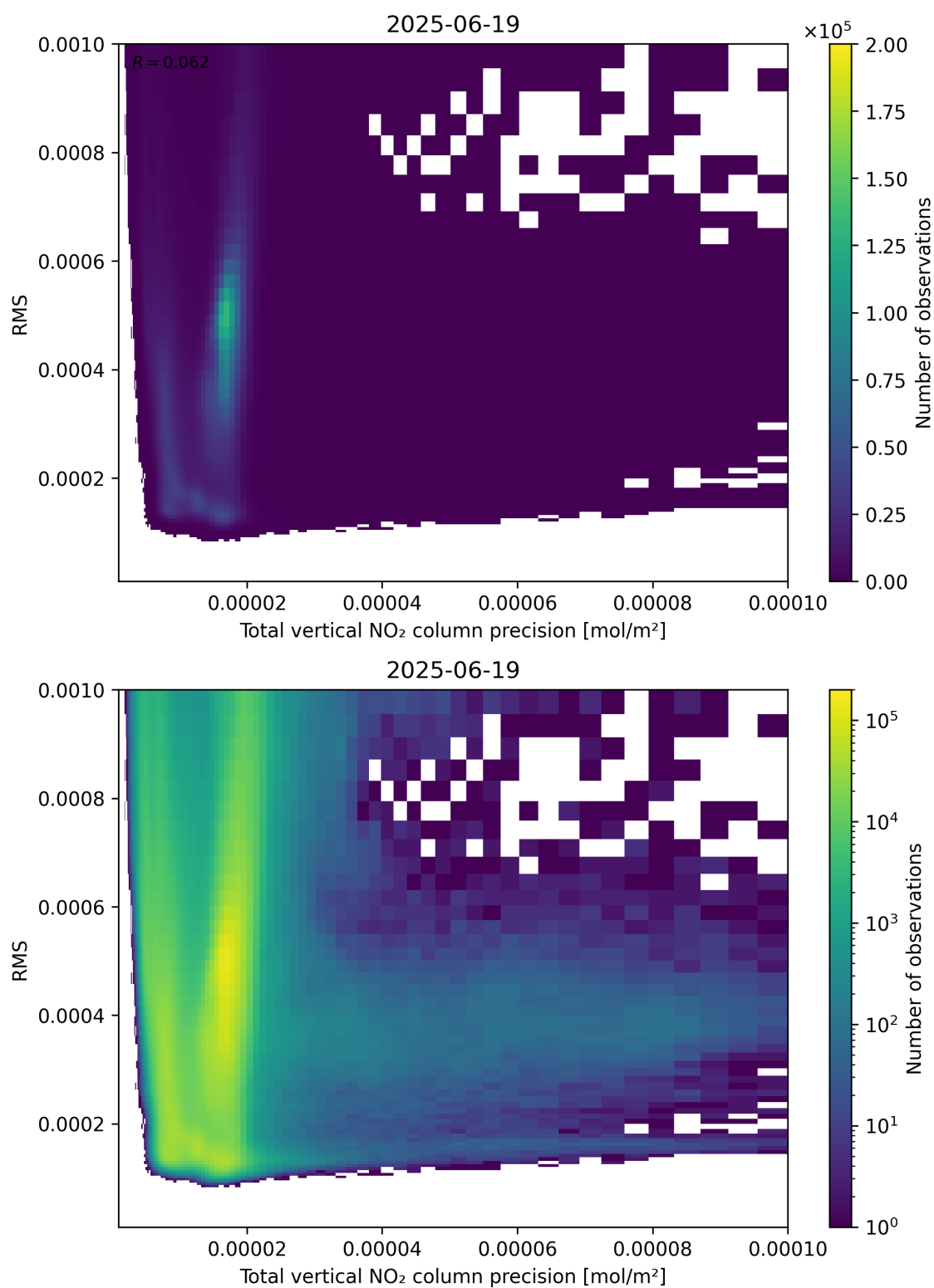
Figure 119: Scatter density plot of “Total vertical NO 2 column precision” against “RMS” for 2025-06-18 to 2025-06-20.
