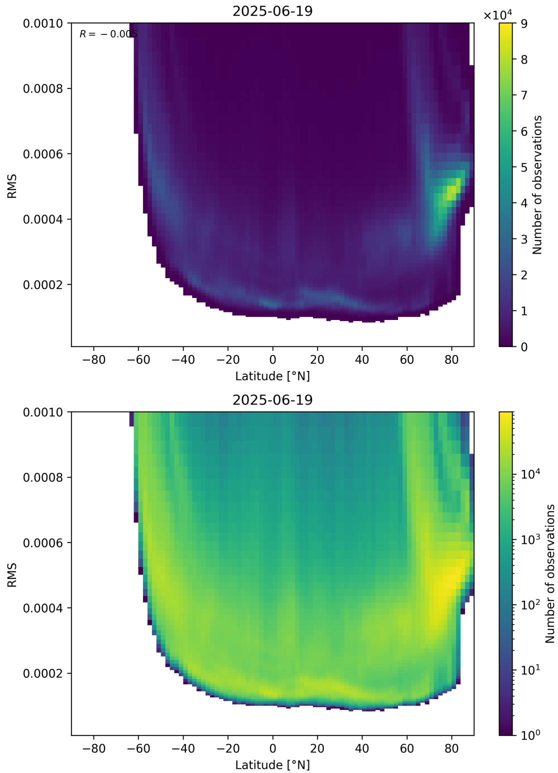
Figure 94: Scatter density plot of “Latitude” against “RMS” for 2025-06-18 to 2025-06-20.
