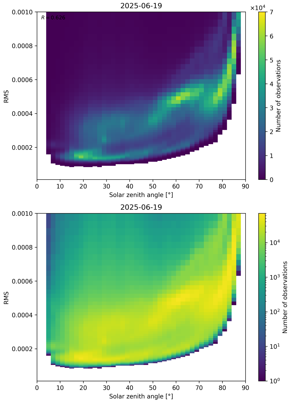
Figure 157: Scatter density plot of “Solar zenith angle” against “RMS” for 2025-06-18 to 2025-06-20.
