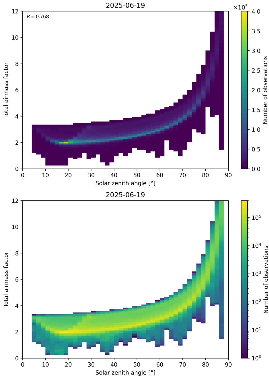
Figure 146: Scatter density plot of “Solar zenith angle” against “Total air mass factor” for 2025-06-18 to 2025-06-20.
