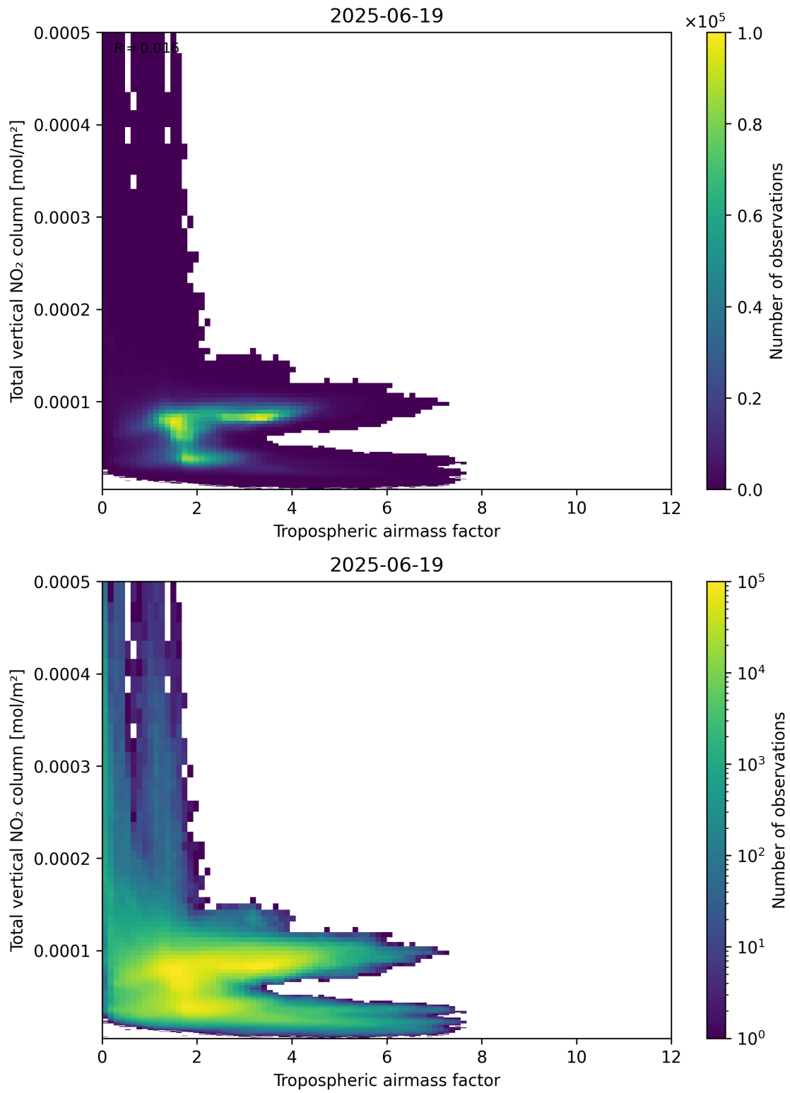
Figure 77: Scatter density plot of “Tropospheric airmass factor” against “Total vertical NO 2 column” for 2025-06-18 to 2025-06-20.
