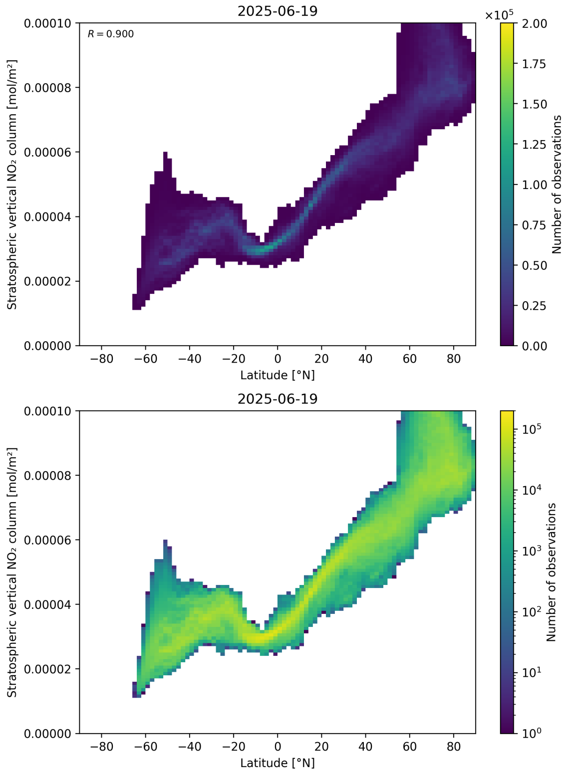
Figure 87: Scatter density plot of “Latitude” against “Stratospheric vertical NO 2 column” for 2025-06-18 to 2025-06-20.
