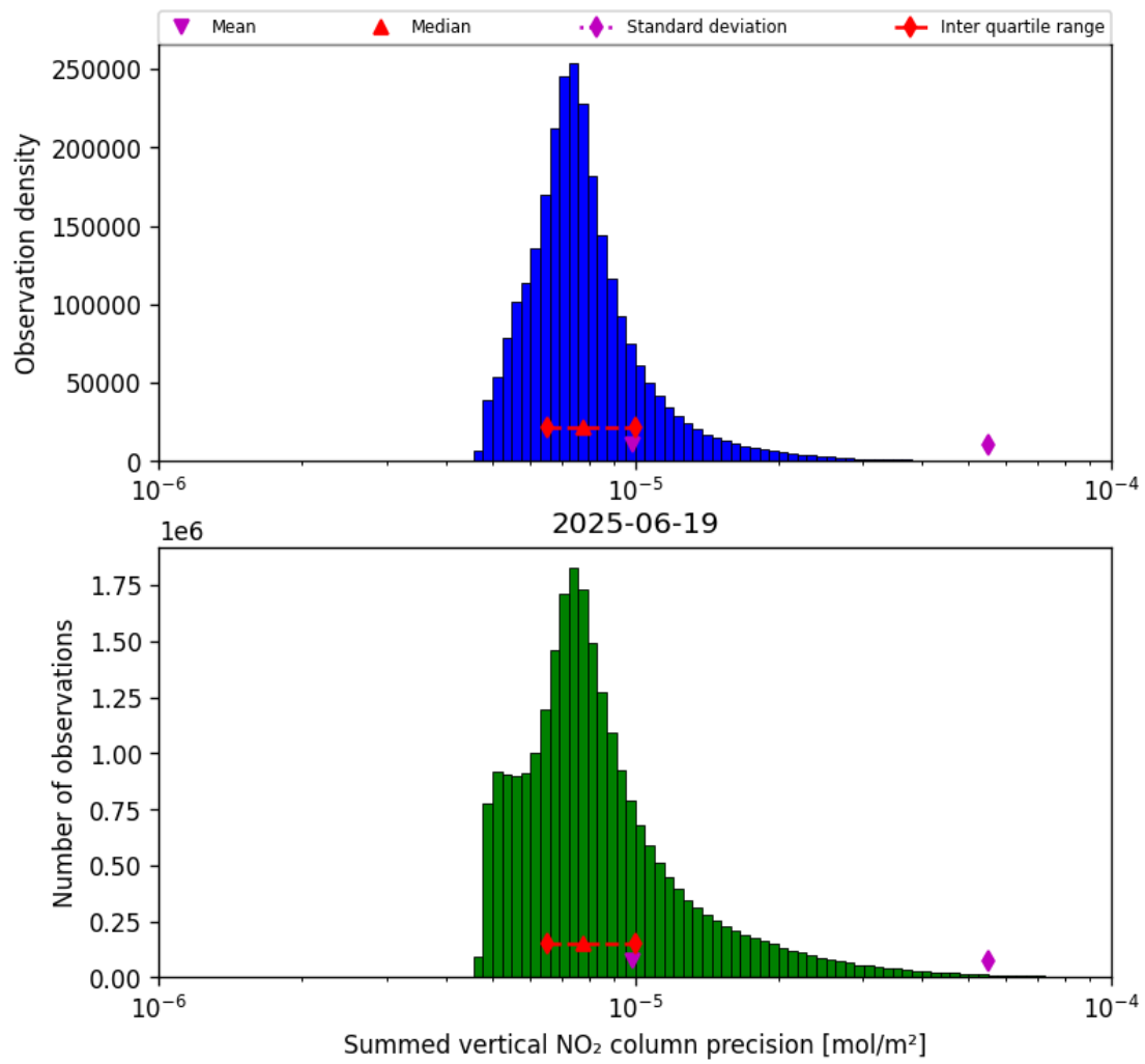
Figure 41: Histogram of "Summed vertical NO 2 column precision" for 2025-06-18 to 2025-06-20
