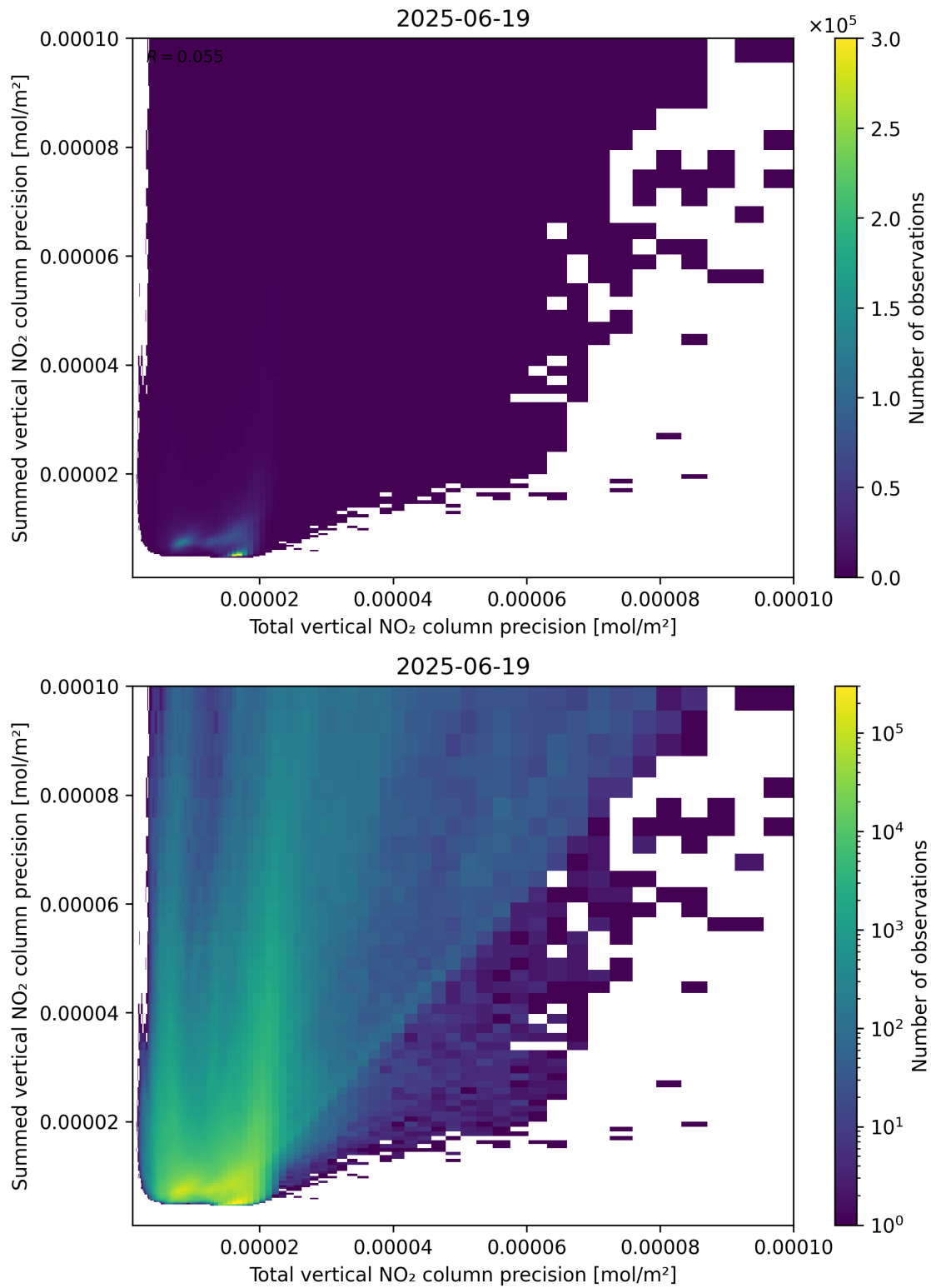
Figure 118: Scatter density plot of “Total vertical NO 2 column precision” against “Summed vertical NO 2 column precision” for 2025-06-18 to 2025-06-20.
