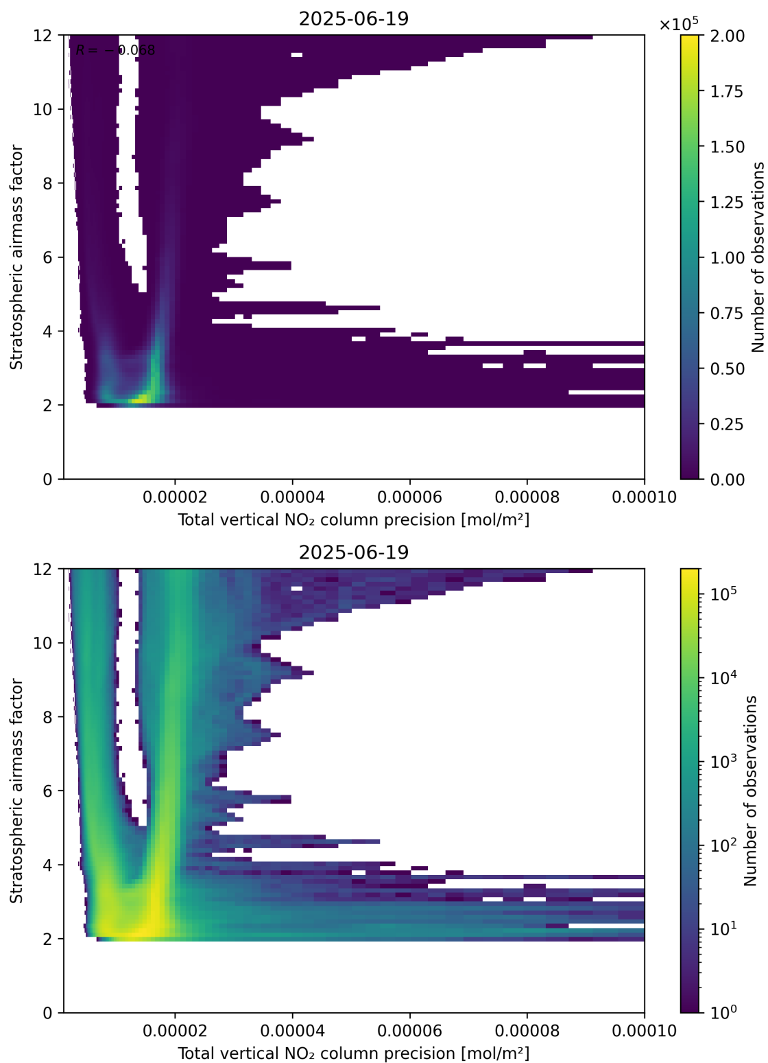
Figure 115: Scatter density plot of “Total vertical NO 2 column precision” against “Stratospheric air mass factor” for 2025-06-18 to 2025-06-20.
