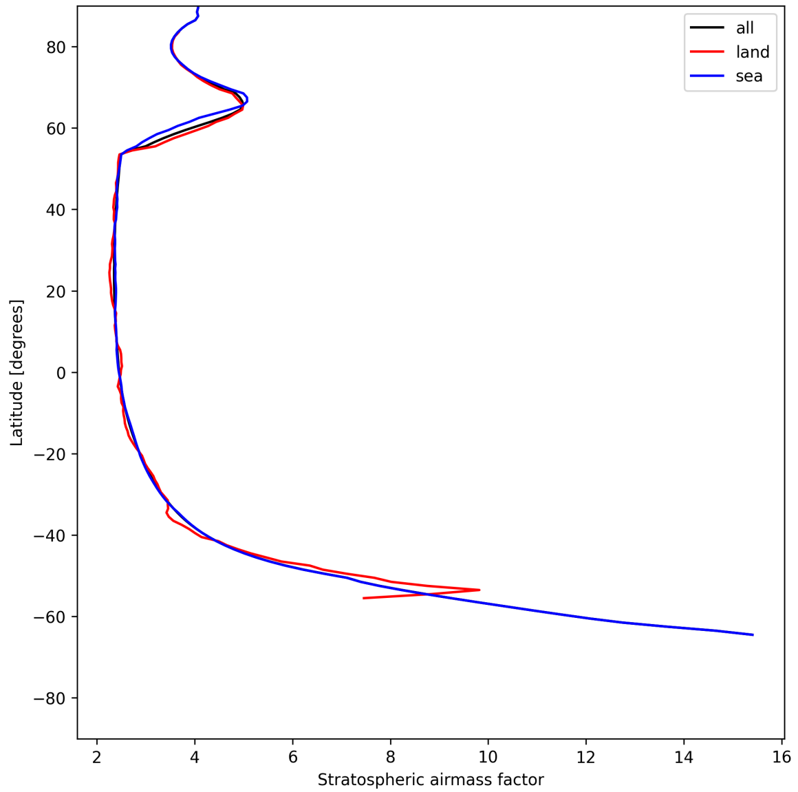
Figure 27: Zonal average of “Stratospheric airmass factor” for 2025-06-18 to 2025-06-20.
