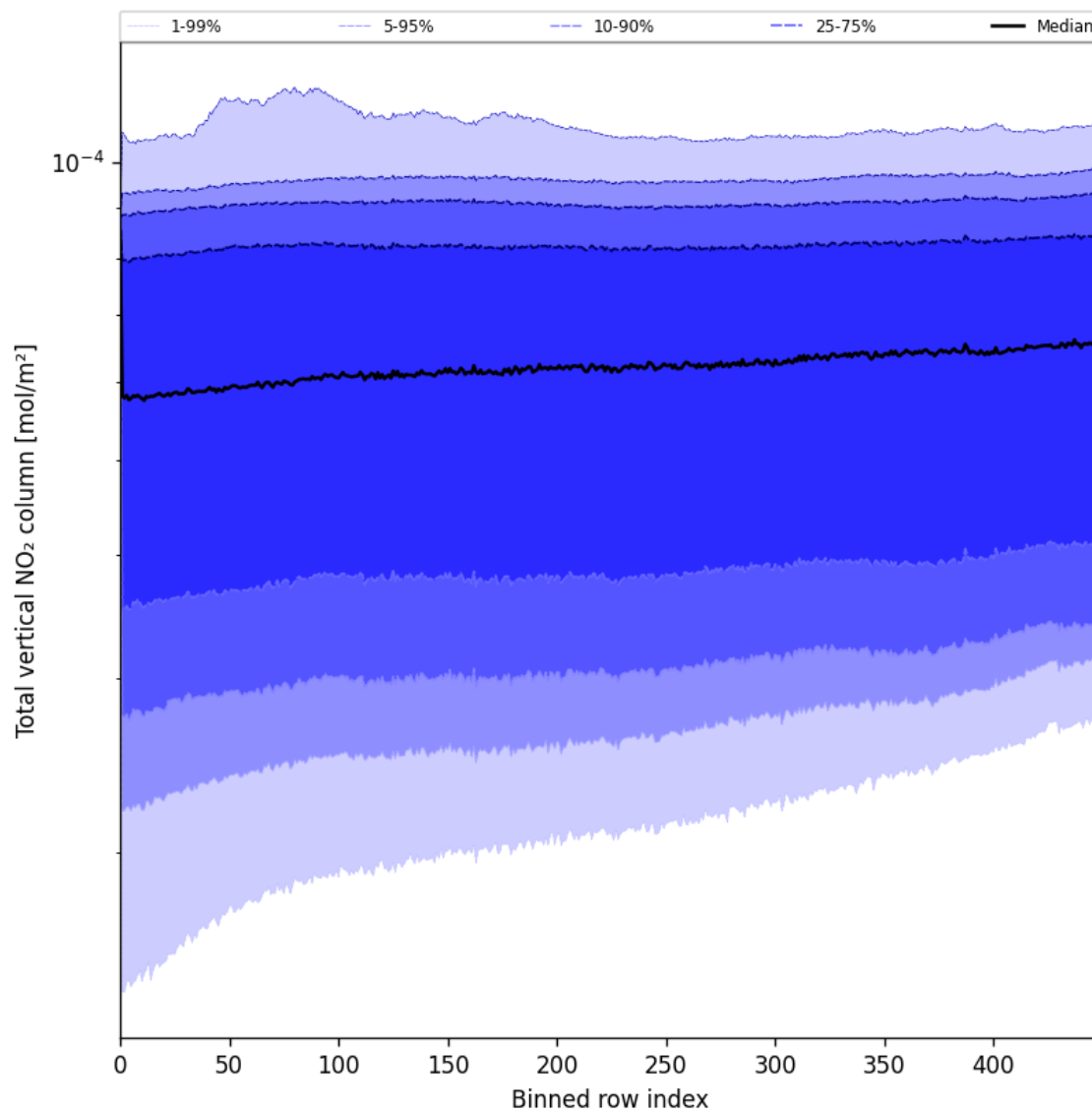
Figure 55: Along track statistics of “Total vertical NO 2 column” for 2025-06-18 to 2025-06-20
