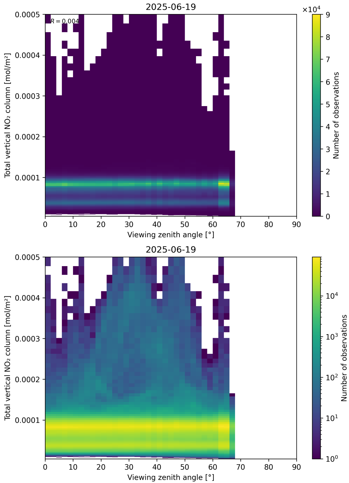
Figure 167: Scatter density plot of “Viewing zenith angle” against “Total vertical NO 2 column” for 2025-06-18 to 2025-06-20.
