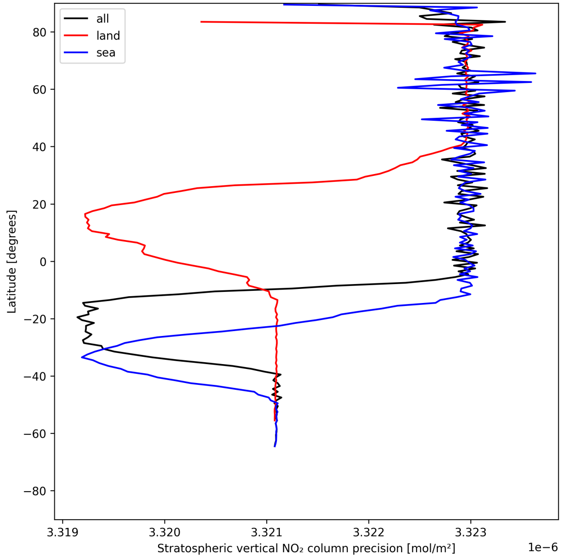
Figure 20: Zonal average of “Stratospheric vertical NO 2 column precision” for 2025-06-18 to 2025-06-20.
