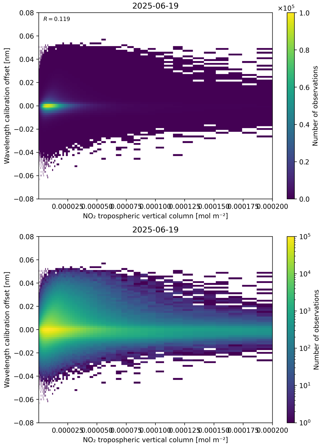
Figure 143: Scatter density plot of “NO 2 tropospheric vertical column” against “Wavelength calibration offset” for 2025-06-18 to 2025-06-20.
