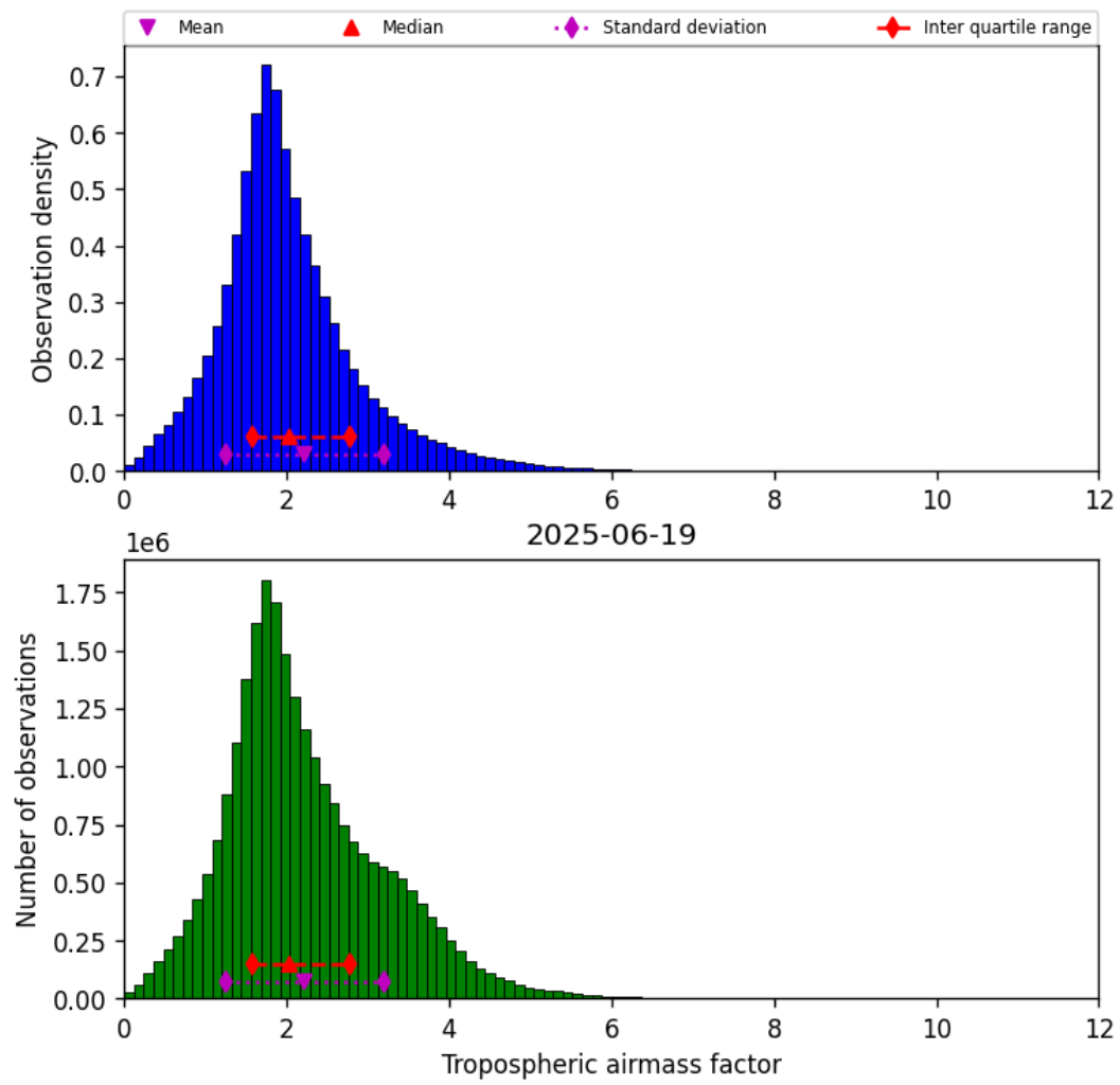
Figure 31: Histogram of “Tropospheric airmass factor” for 2025-06-18 to 2025-06-20
