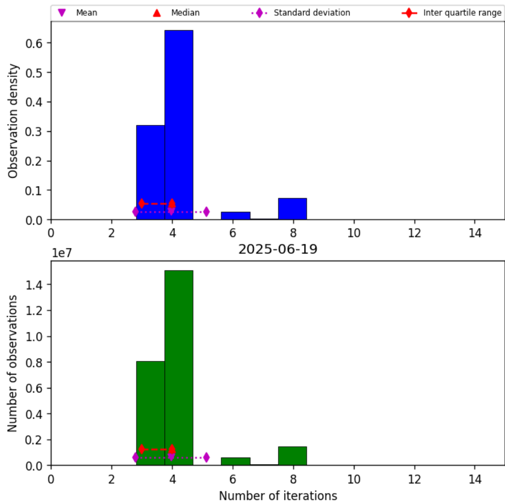
Figure 34: Histogram of “Number of iterations” for 2025-06-18 to 2025-06-20
