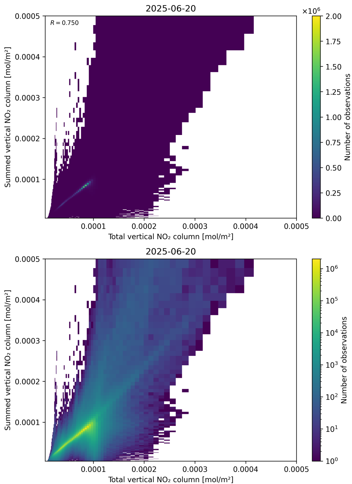
Figure 112: Scatter density plot of “Total vertical NO 2 column” against “Summed vertical NO 2 column” for 2025-06-19 to 2025-06-21.
