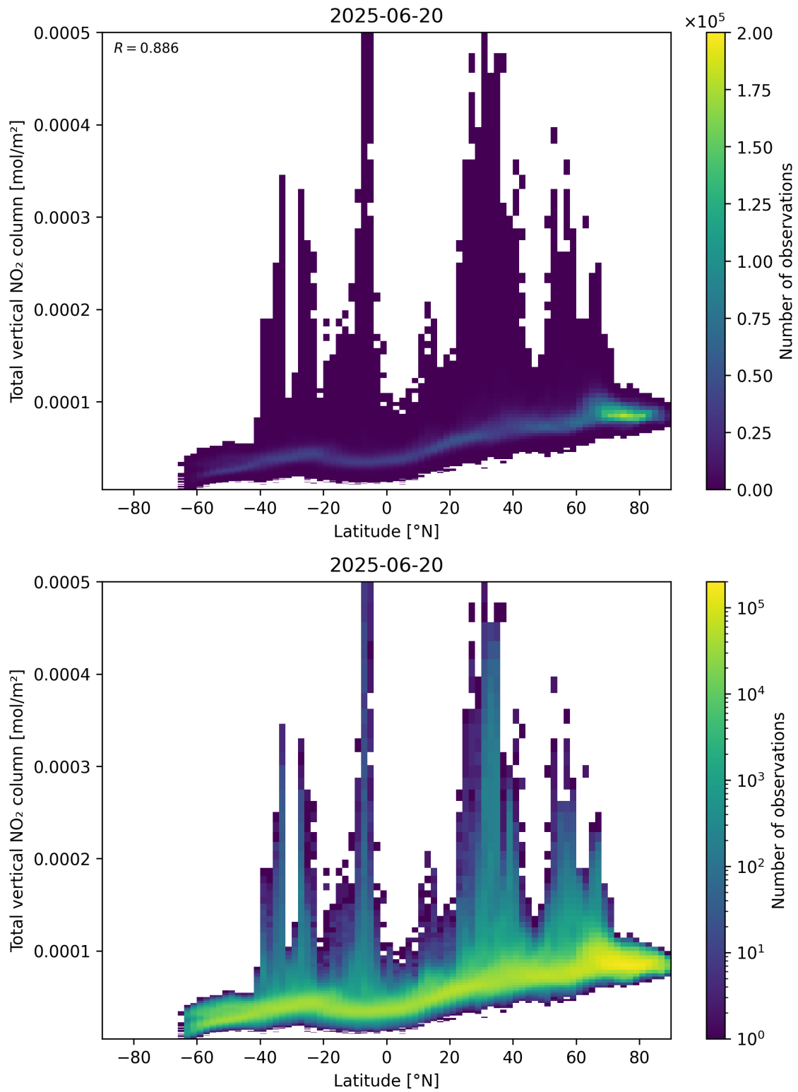
Figure 90: Scatter density plot of “Latitude” against “Total vertical NO 2 column” for 2025-06-19 to 2025-06-21.
