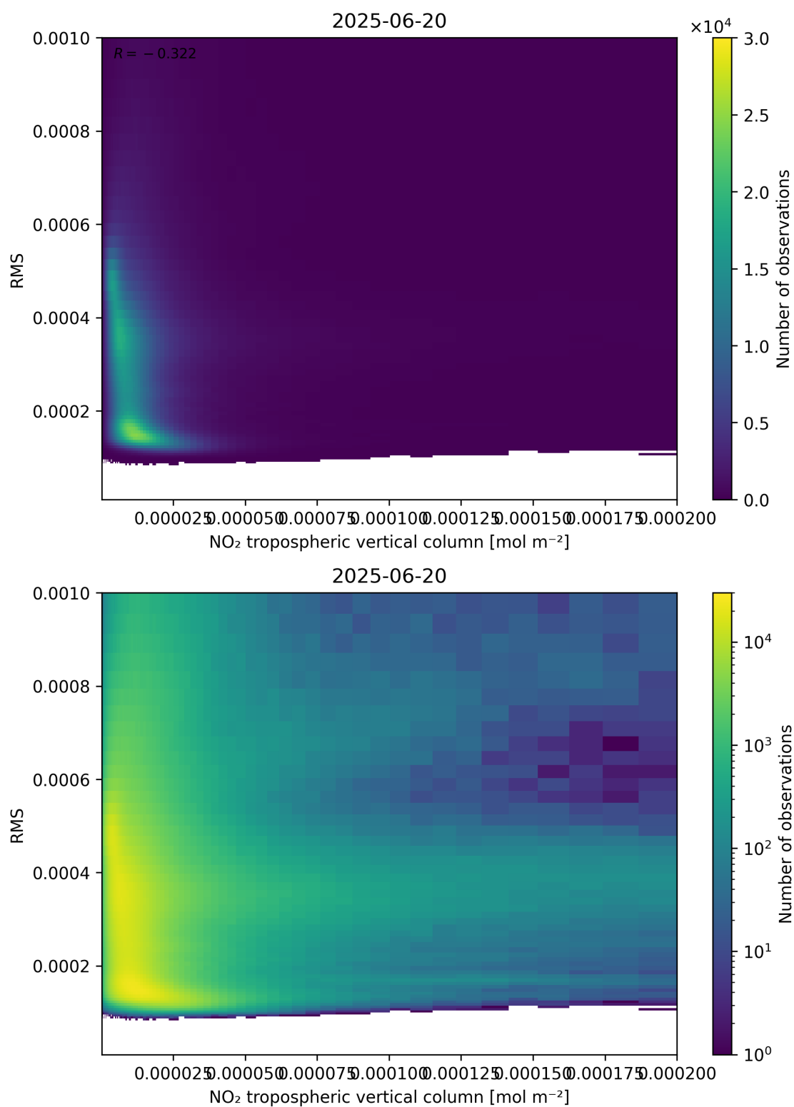
Figure 142: Scatter density plot of “NO 2 tropospheric vertical column” against “RMS” for 2025-06-19 to 2025-06-21.
