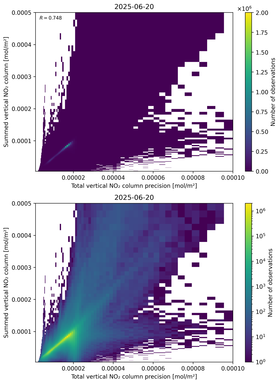
Figure 117: Scatter density plot of “Total vertical NO 2 column precision” against “Summed vertical NO 2 column” for 2025-06-19 to 2025-06-21.
