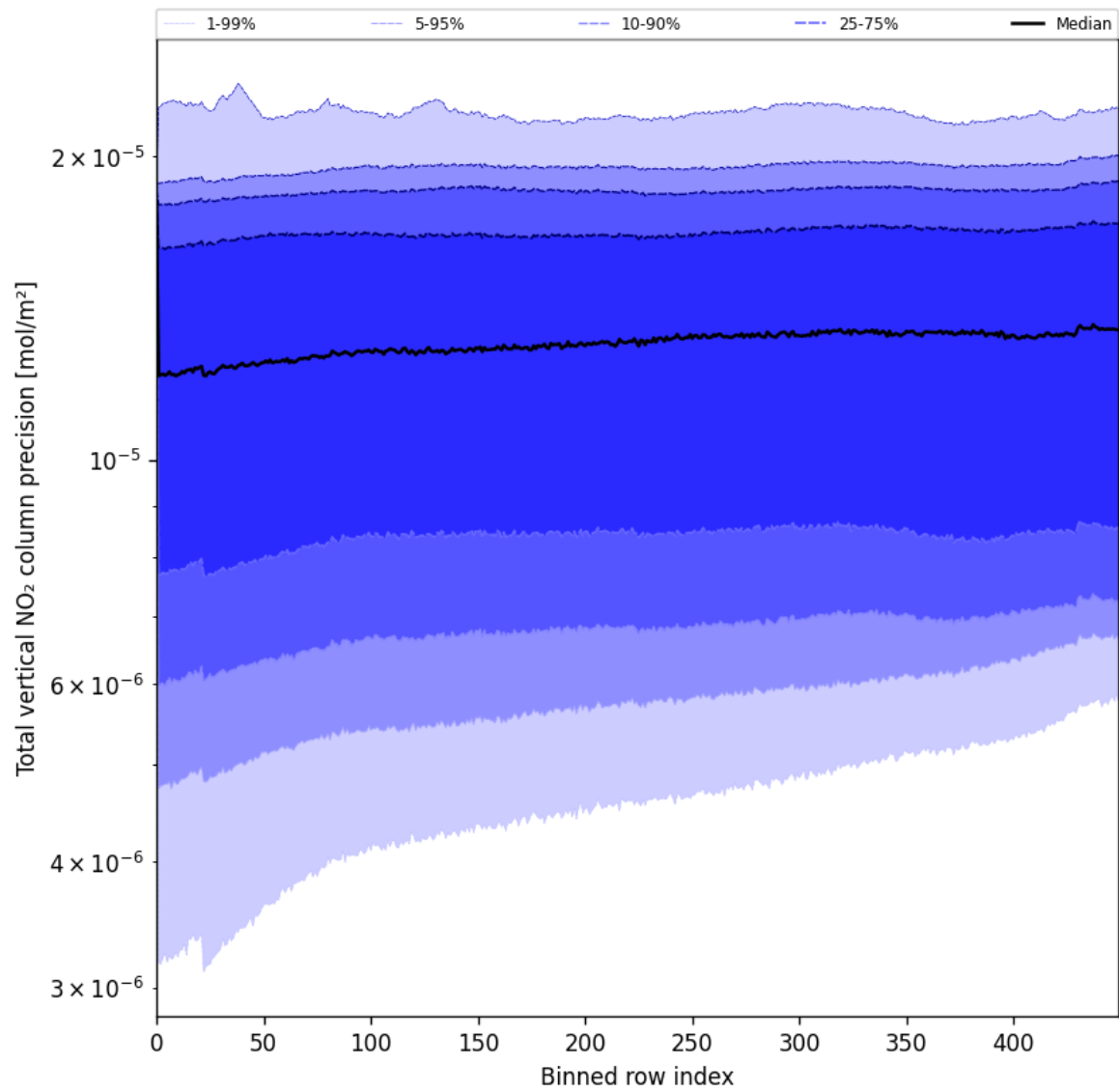
Figure 56: Along track statistics of “Total vertical NO 2 column precision” for 2025-06-19 to 2025-06-21
