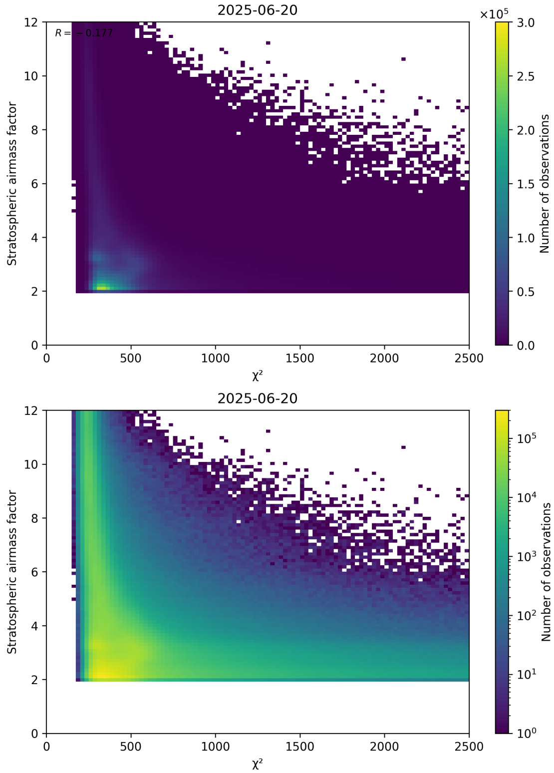
Figure 81: Scatter density plot of “ \chi^2 ” against “Stratospheric airmass factor” for 2025-06-19 to 2025-06-21.
