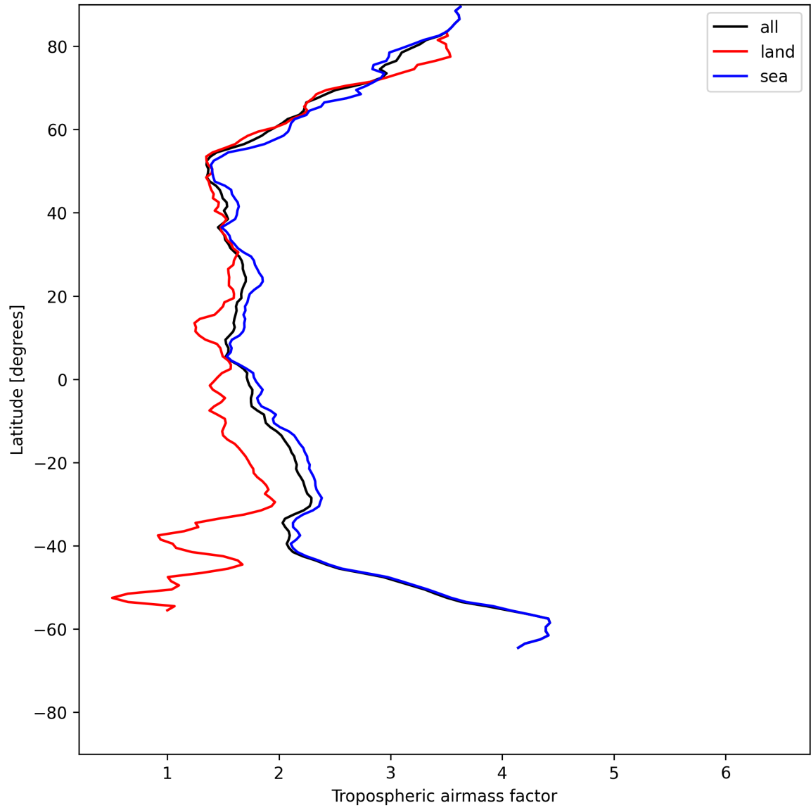
Figure 14: Zonal average of “Tropospheric air mass factor” for 2025-06-19 to 2025-06-21.
