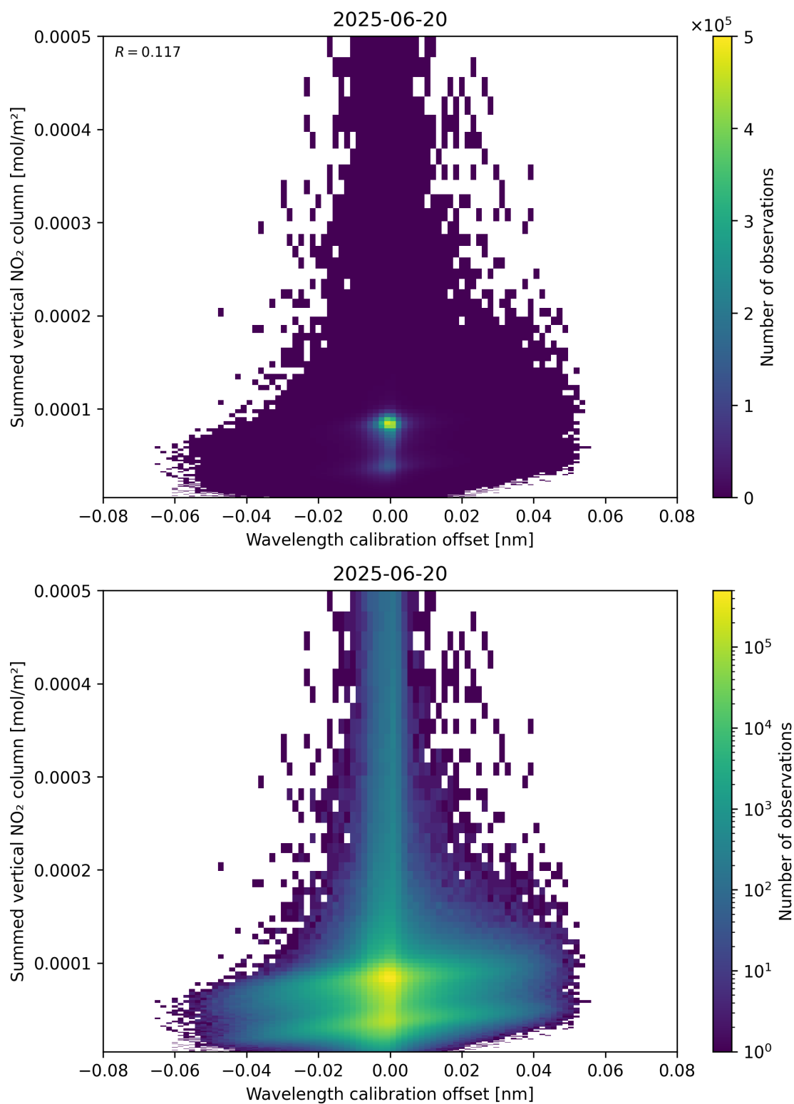
Figure 177: Scatter density plot of “Wavelength calibration offset” against “Summed vertical NO 2 column” for 2025-06-19 to 2025-06-21.
