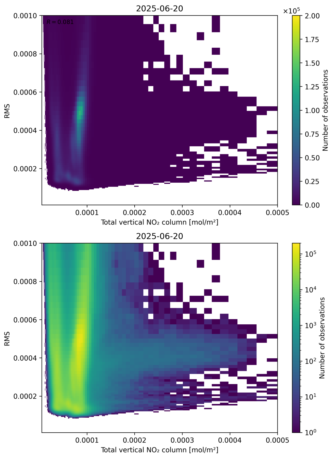
Figure 120: Scatter density plot of “Total vertical NO 2 column” against “RMS” for 2025-06-19 to 2025-06-21.
