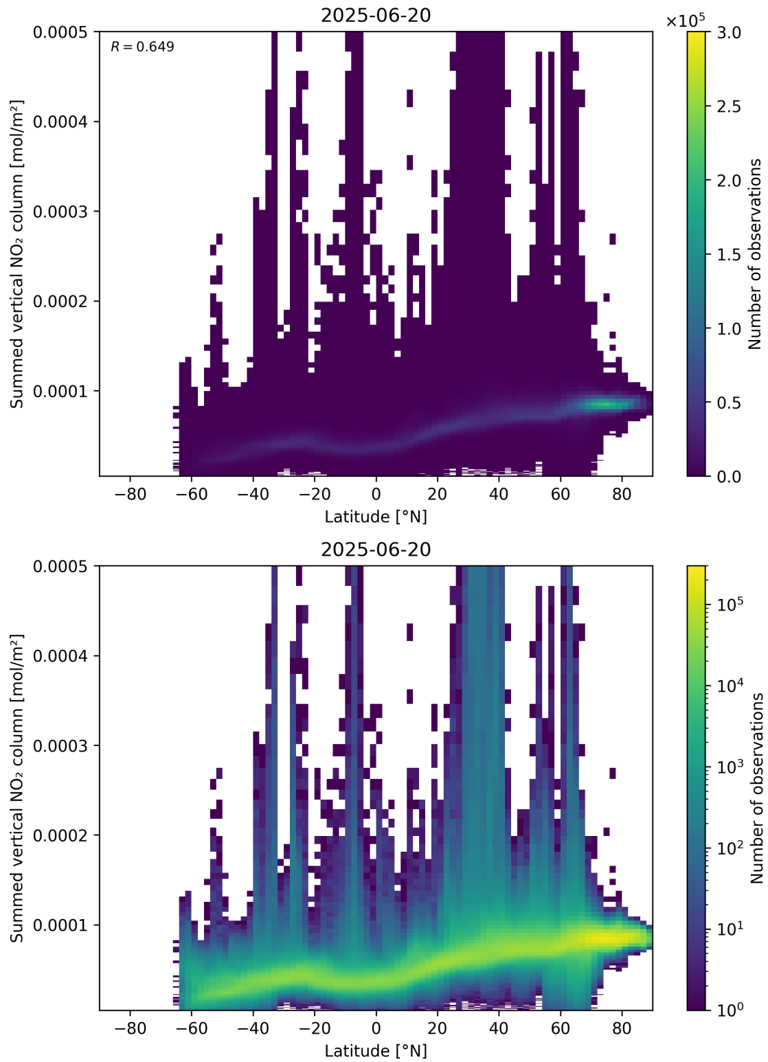
Figure 88: Scatter density plot of “Latitude” against “Summed vertical NO 2 column” for 2025-06-19 to 2025-06-21.
