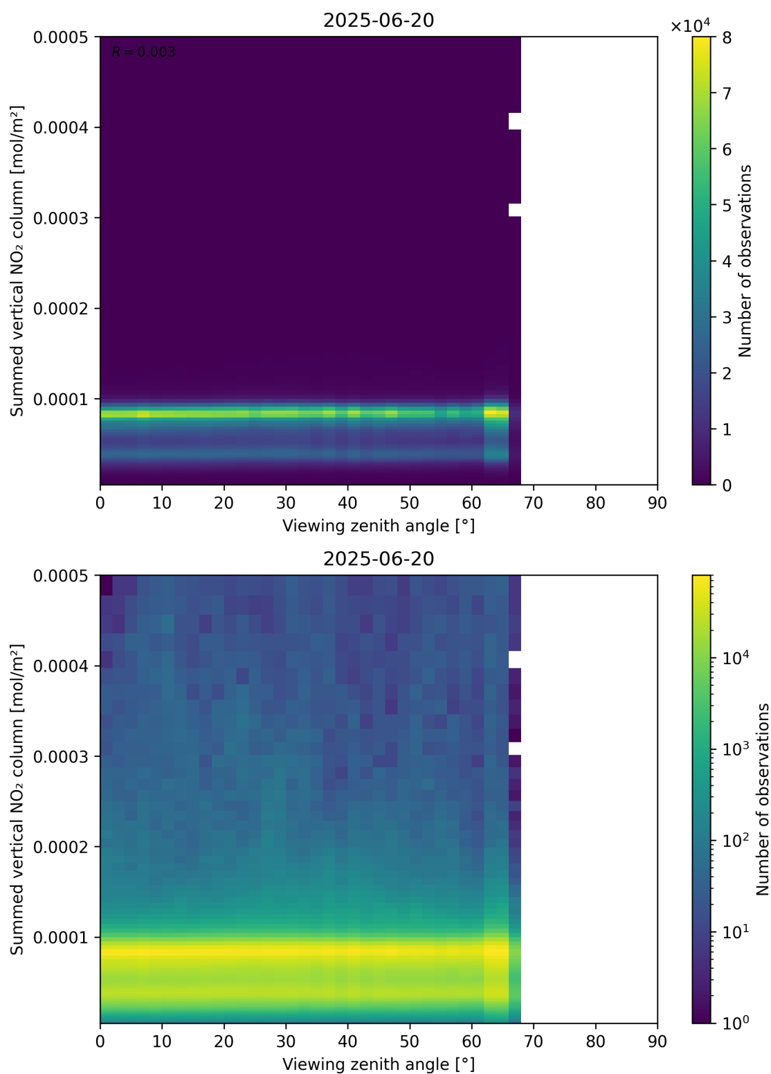
Figure 165: Scatter density plot of “Viewing zenith angle” against “Summed vertical NO 2 column” for 2025-06-19 to 2025-06-21.
