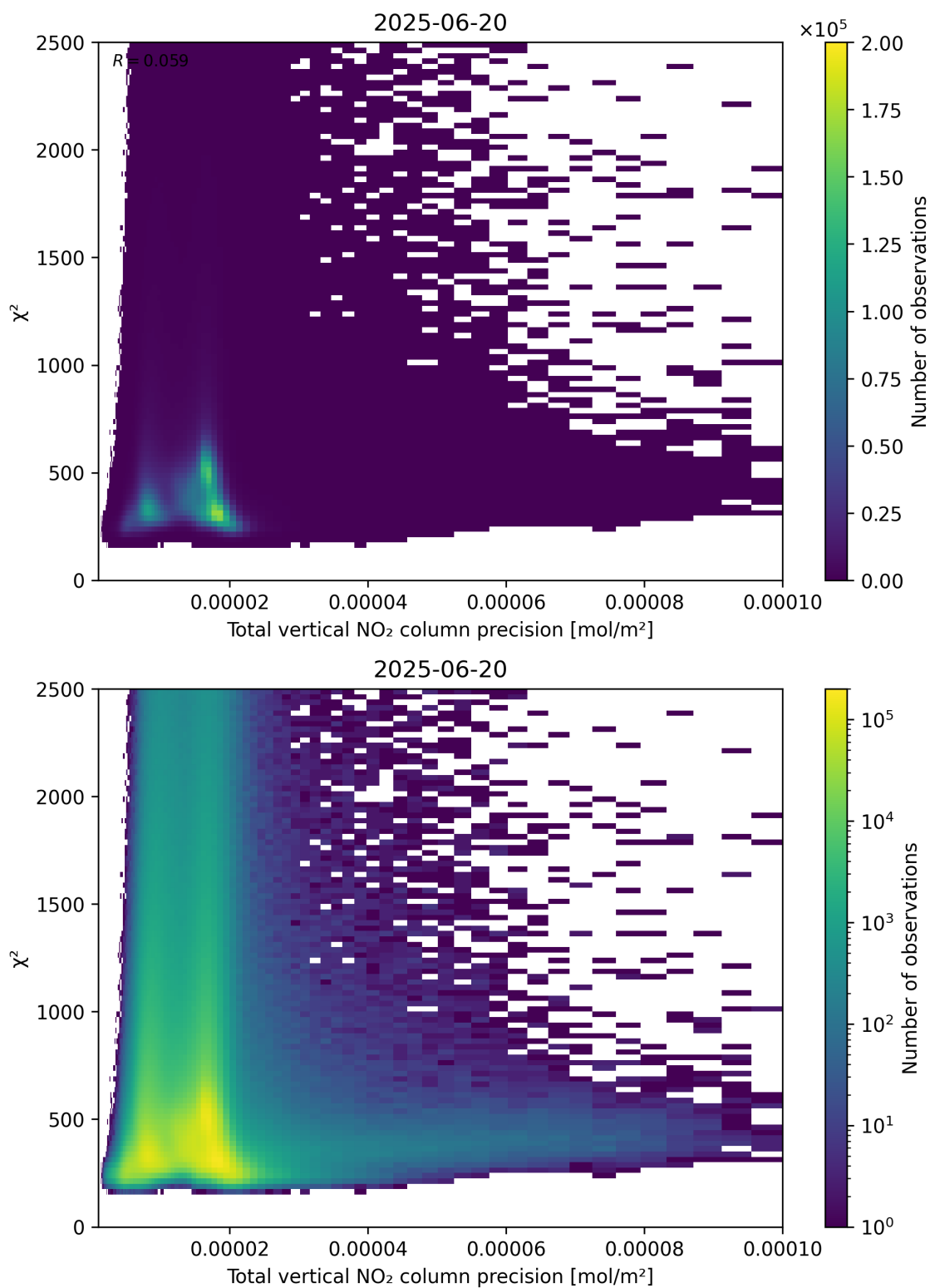
Figure 116: Scatter density plot of “Total vertical NO 2 column precision” against “ \chi^2 ” for 2025-06-19 to 2025-06-21.
