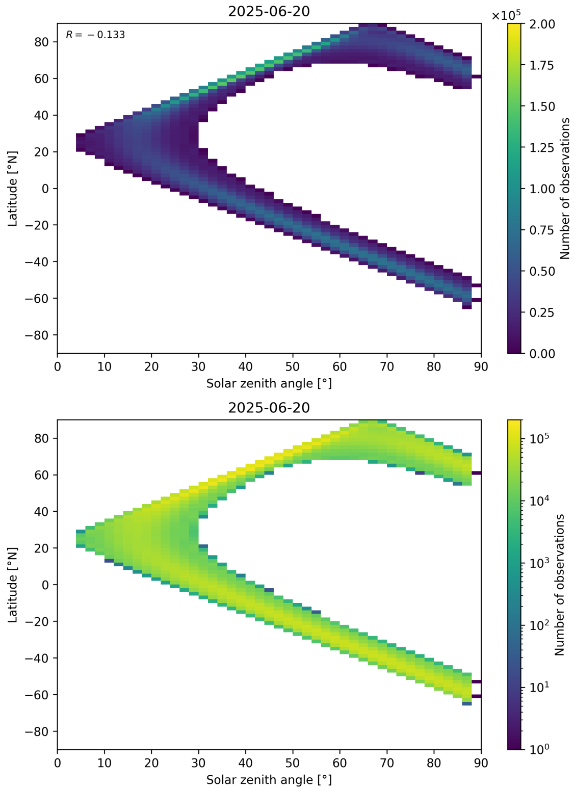
Figure 149: Scatter density plot of “Solar zenith angle” against “Latitude” for 2025-06-19 to 2025-06-21.
