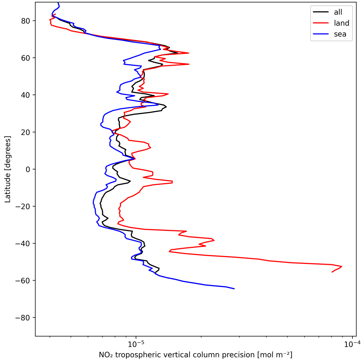
Figure 13: Zonal average of “NO 2 tropospheric vertical column precision” for 2025-06-19 to 2025-06-21.
