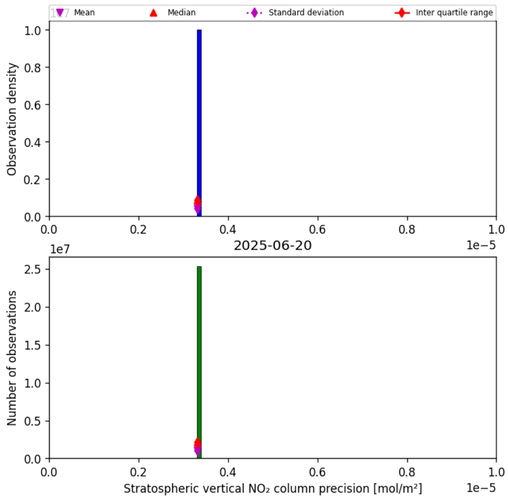
Figure 37: Histogram of “Stratospheric vertical NO 2 column precision” for 2025-06-19 to 2025-06-21
