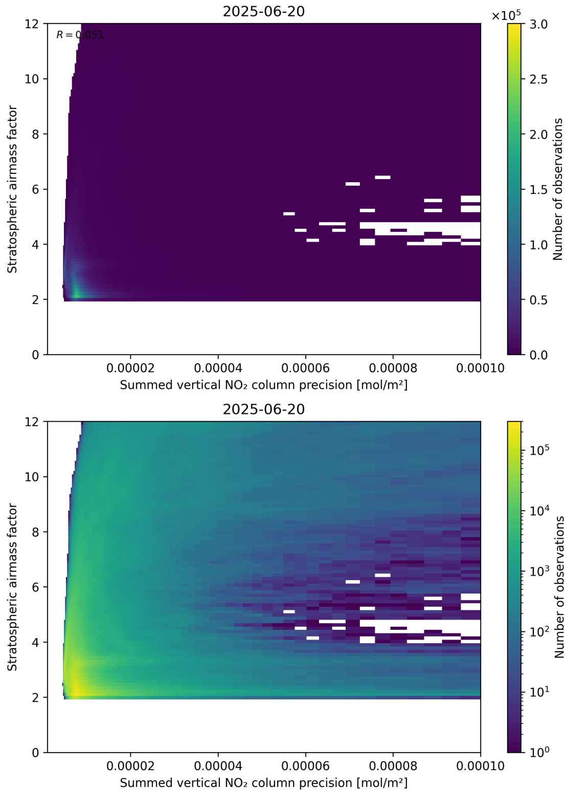
Figure 106: Scatter density plot of “Summed vertical NO 2 column precision” against “Stratospheric airmass factor” for 2025-06-19 to 2025-06-21.
