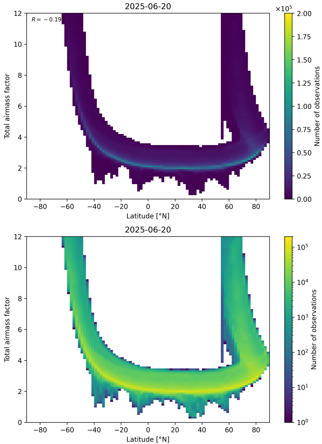
Figure 84: Scatter density plot of “Latitude” against “Total airmass factor” for 2025-06-19 to 2025-06-21.
