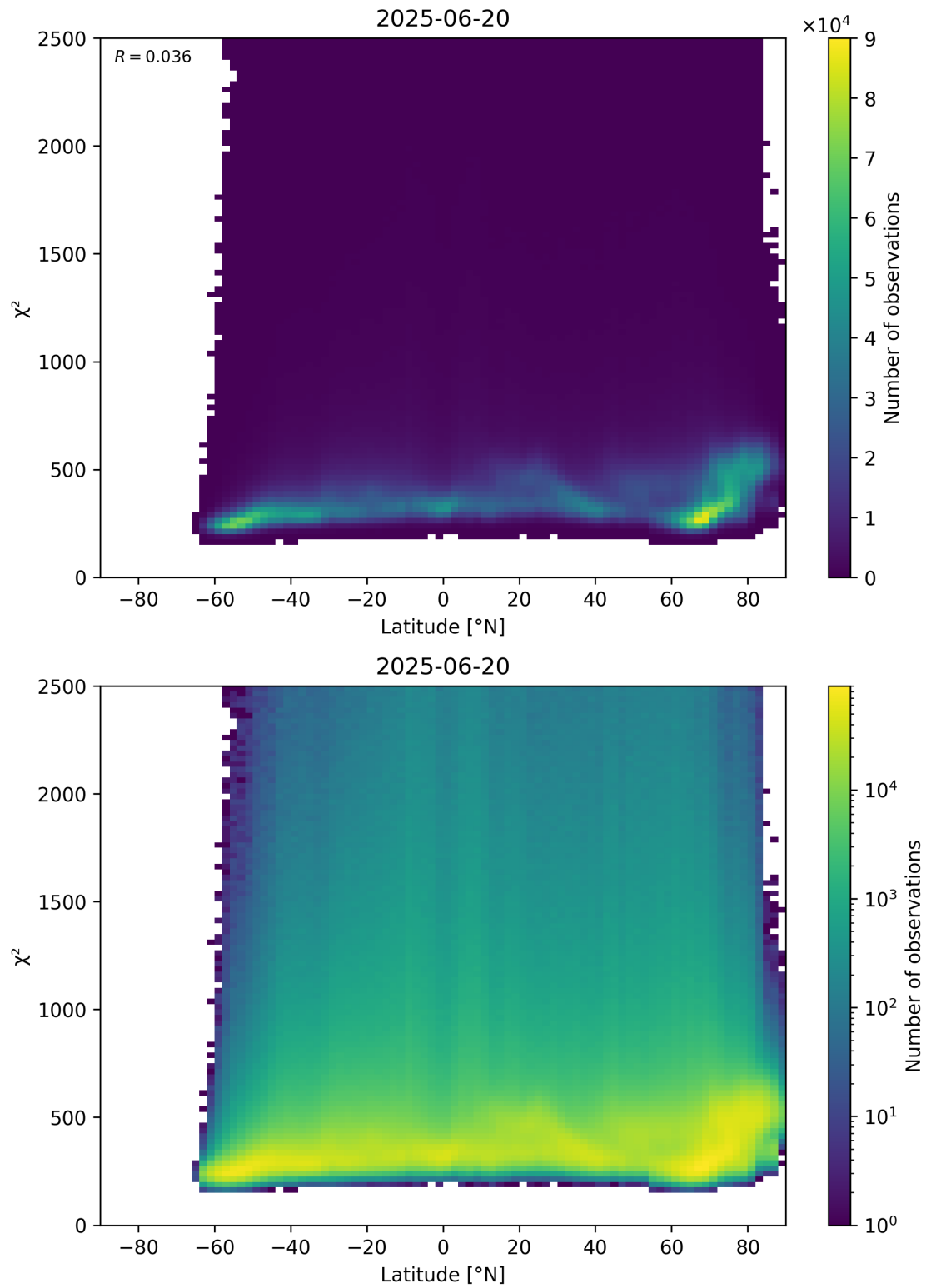
Figure 86: Scatter density plot of “Latitude” against “ \chi^2 ” for 2025-06-19 to 2025-06-21.
