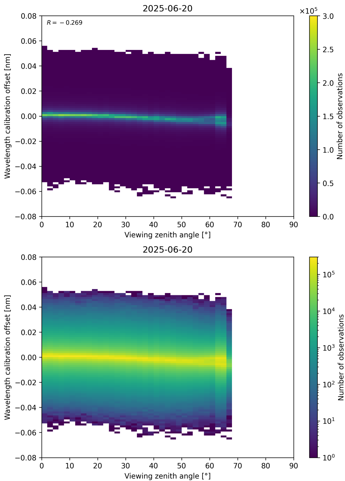
Figure 173: Scatter density plot of “Viewing zenith angle” against “Wavelength calibration offset” for 2025-06-19 to 2025-06-21.
