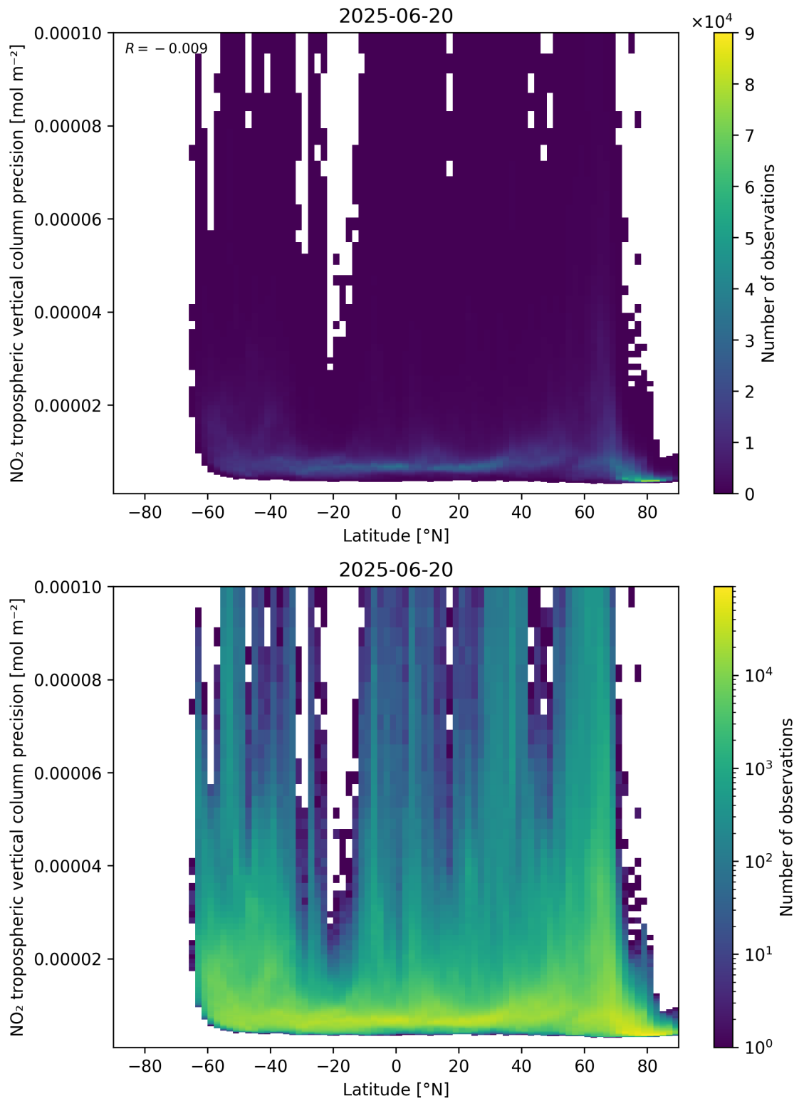
Figure 93: Scatter density plot of “Latitude” against “NO 2 tropospheric vertical column precision” for 2025-06-19 to 2025-06-21.
