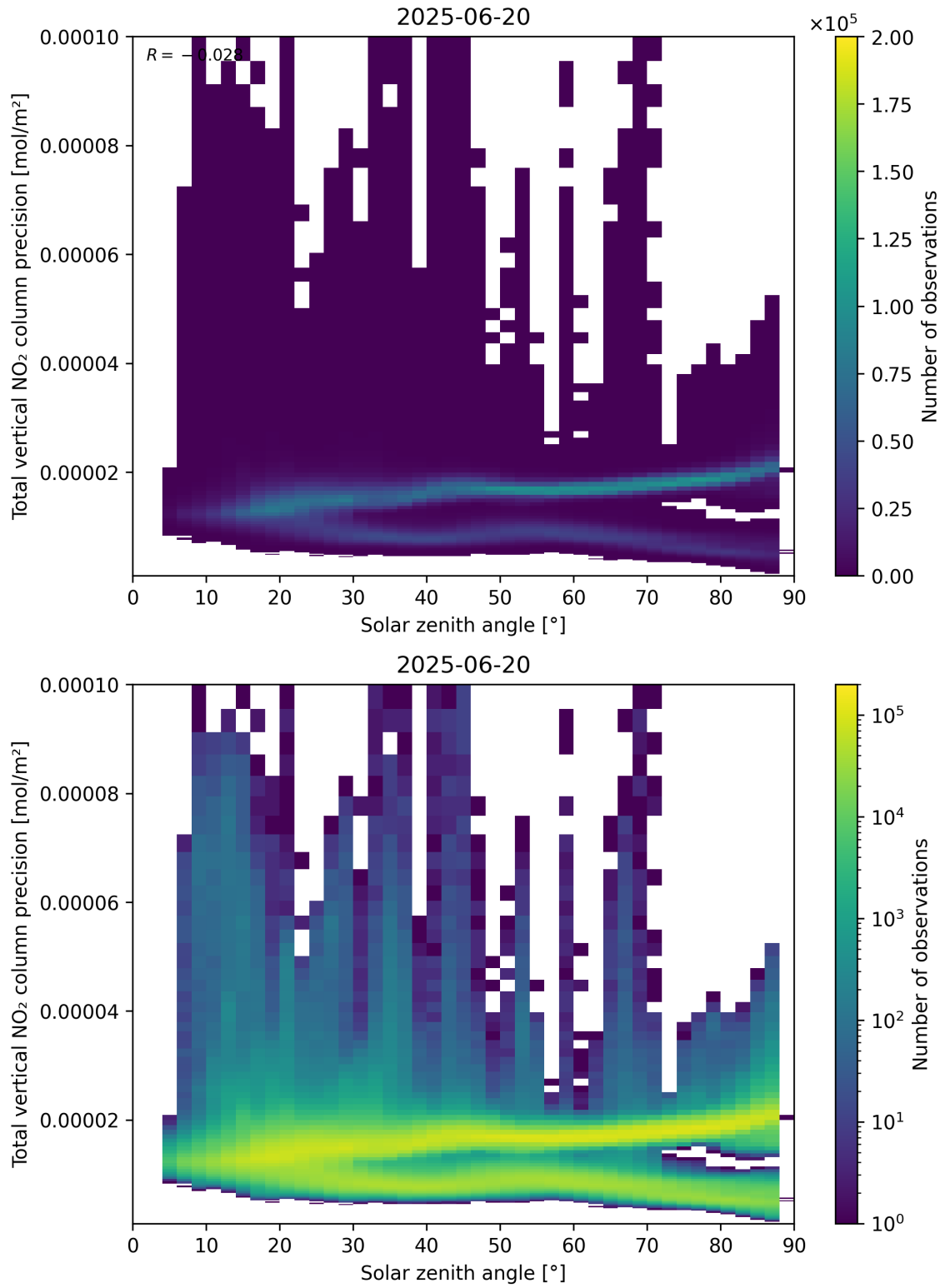
Figure 154: Scatter density plot of “Solar zenith angle” against “Total vertical NO 2 column precision” for 2025-06-19 to 2025-06-21.
