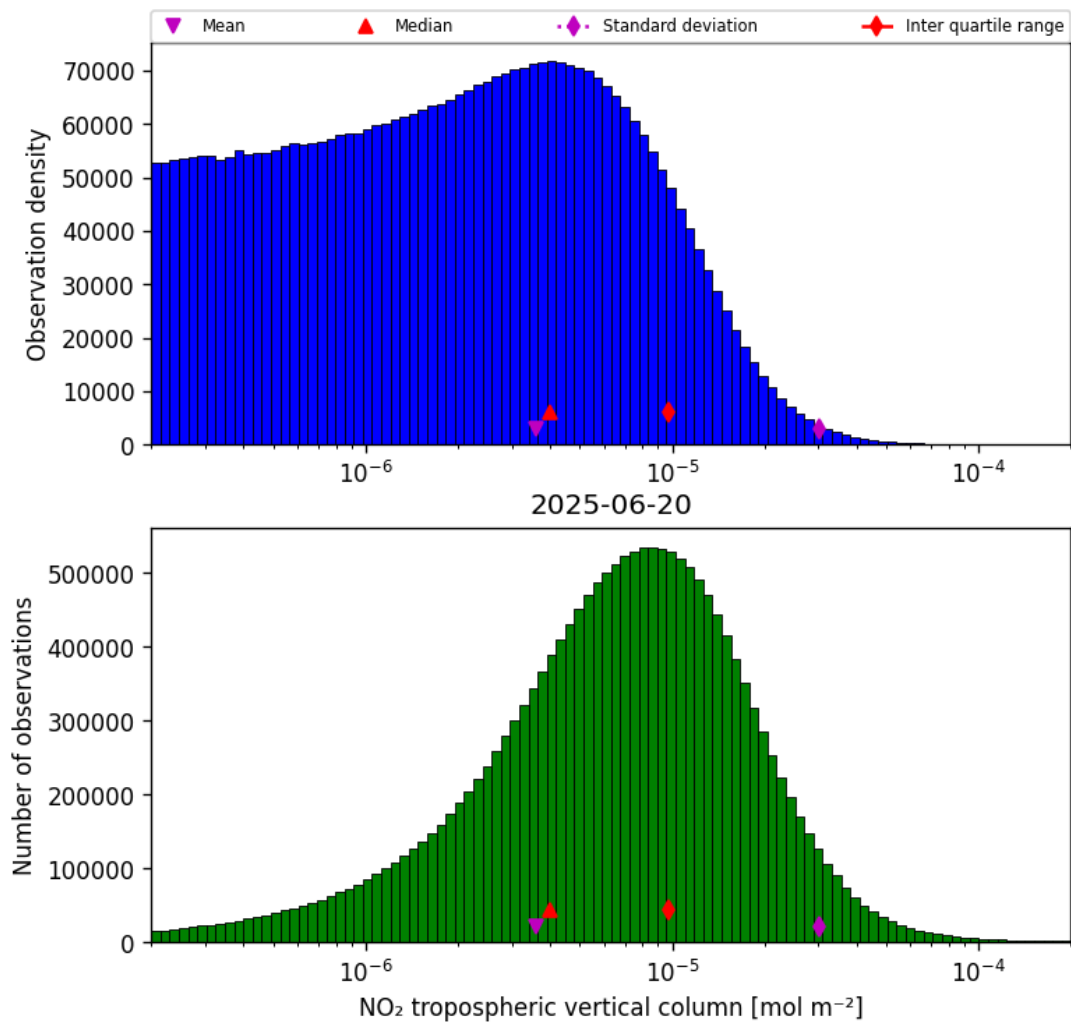
Figure 29: Histogram of “NO 2 tropospheric vertical column” for 2025-06-19 to 2025-06-21
