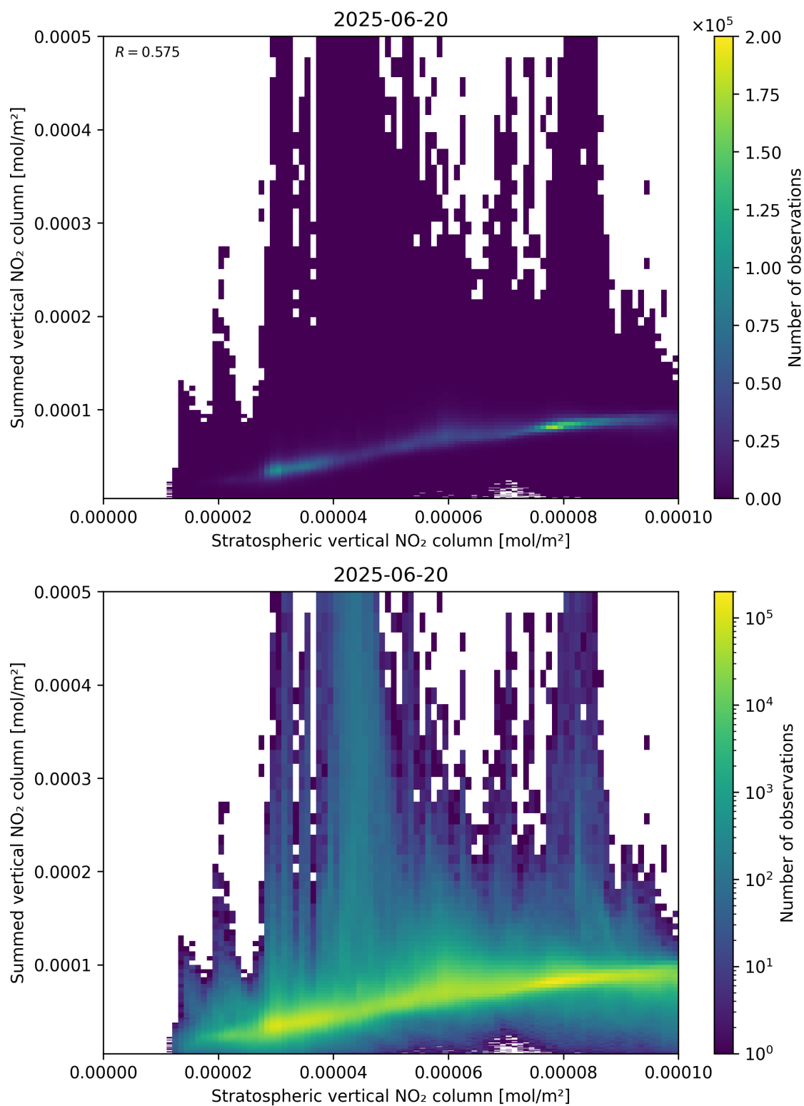
Figure 98: Scatter density plot of “Stratospheric vertical NO 2 column” against “Summed vertical NO 2 column” for 2025-06-19 to 2025-06-21.
