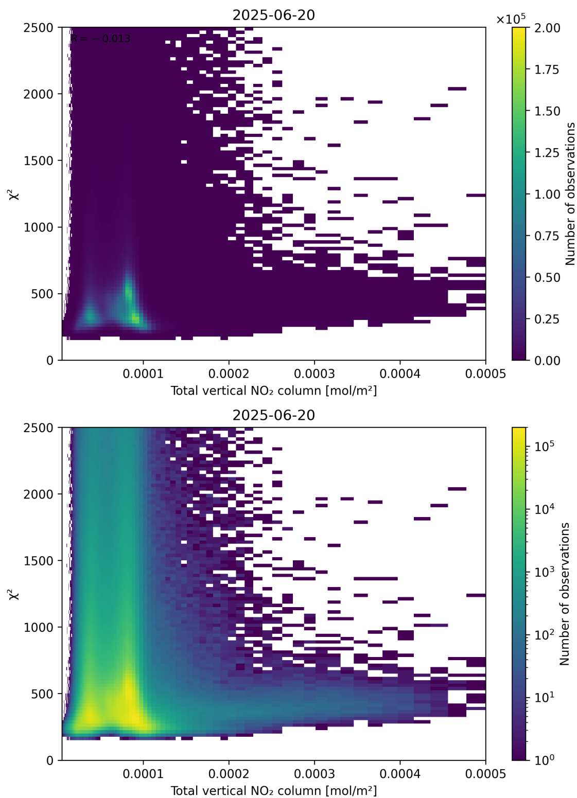
Figure 111: Scatter density plot of “Total vertical NO 2 column” against “ \chi^2 ” for 2025-06-19 to 2025-06-21.
