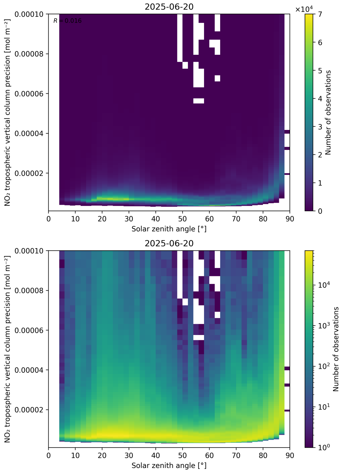
Figure 156: Scatter density plot of “Solar zenith angle” against “NO 2 tropospheric vertical column precision” for 2025-06-19 to 2025-06-21.
