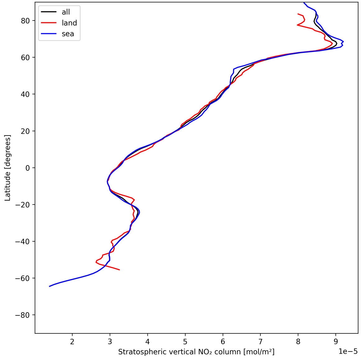
Figure 19: Zonal average of “Stratospheric vertical NO 2 column” for 2025-06-19 to 2025-06-21.
