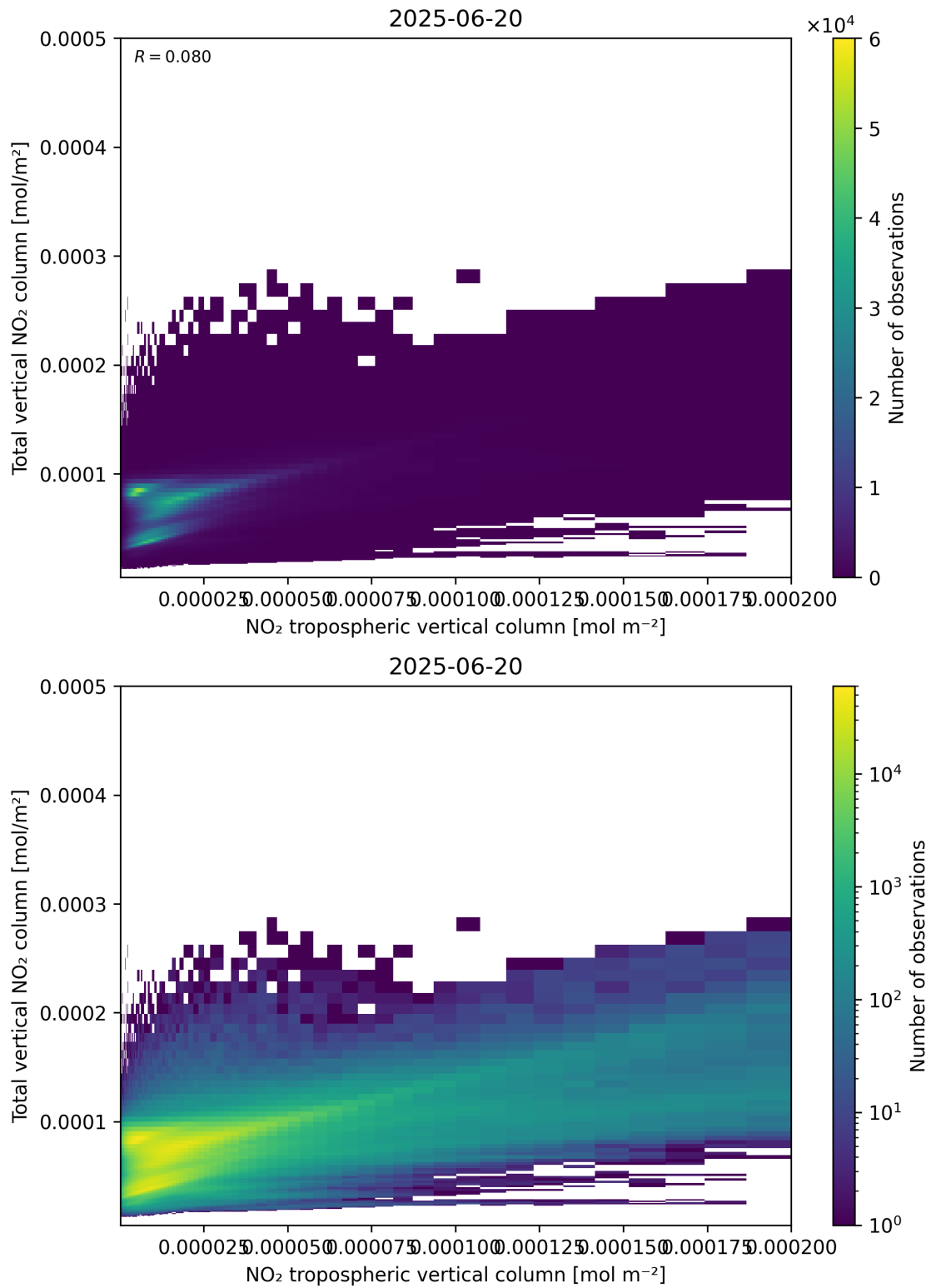
Figure 128: Scatter density plot of “NO 2 tropospheric vertical column” against “Total vertical NO 2 column” for 2025-06-19 to 2025-06-21.
