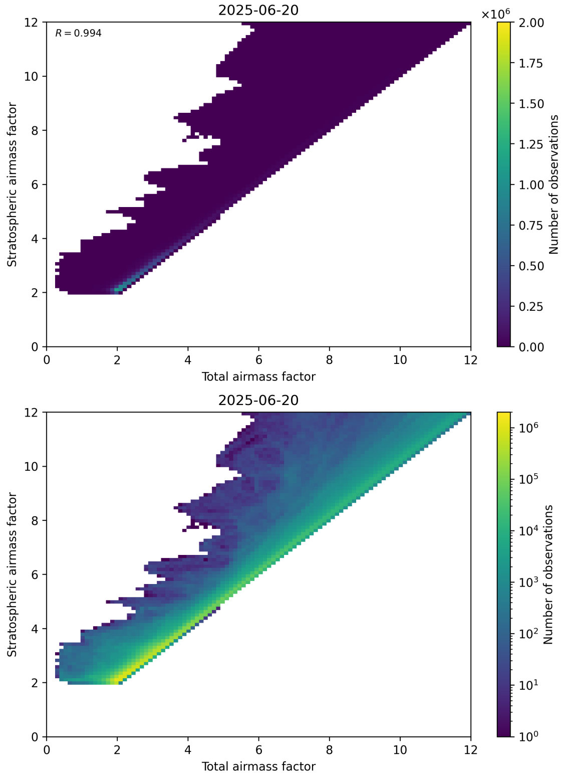
Figure 62: Scatter density plot of “Total airmass factor” against “Stratospheric airmass factor” for 2025-06-19 to 2025-06-21.
