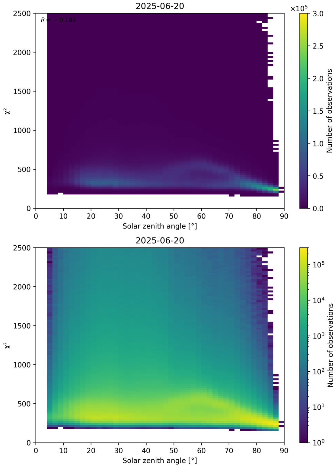
Figure 148: Scatter density plot of “Solar zenith angle” against “ \chi^2 ” for 2025-06-19 to 2025-06-21.
