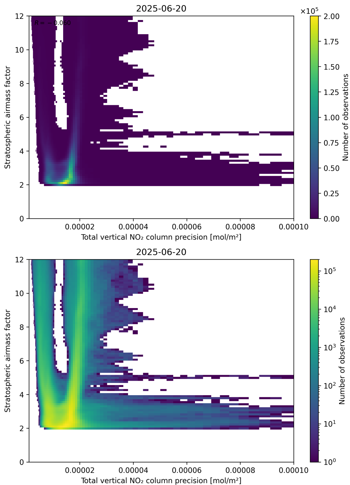
Figure 115: Scatter density plot of “Total vertical NO 2 column precision” against “Stratospheric air mass factor” for 2025-06-19 to 2025-06-21.
