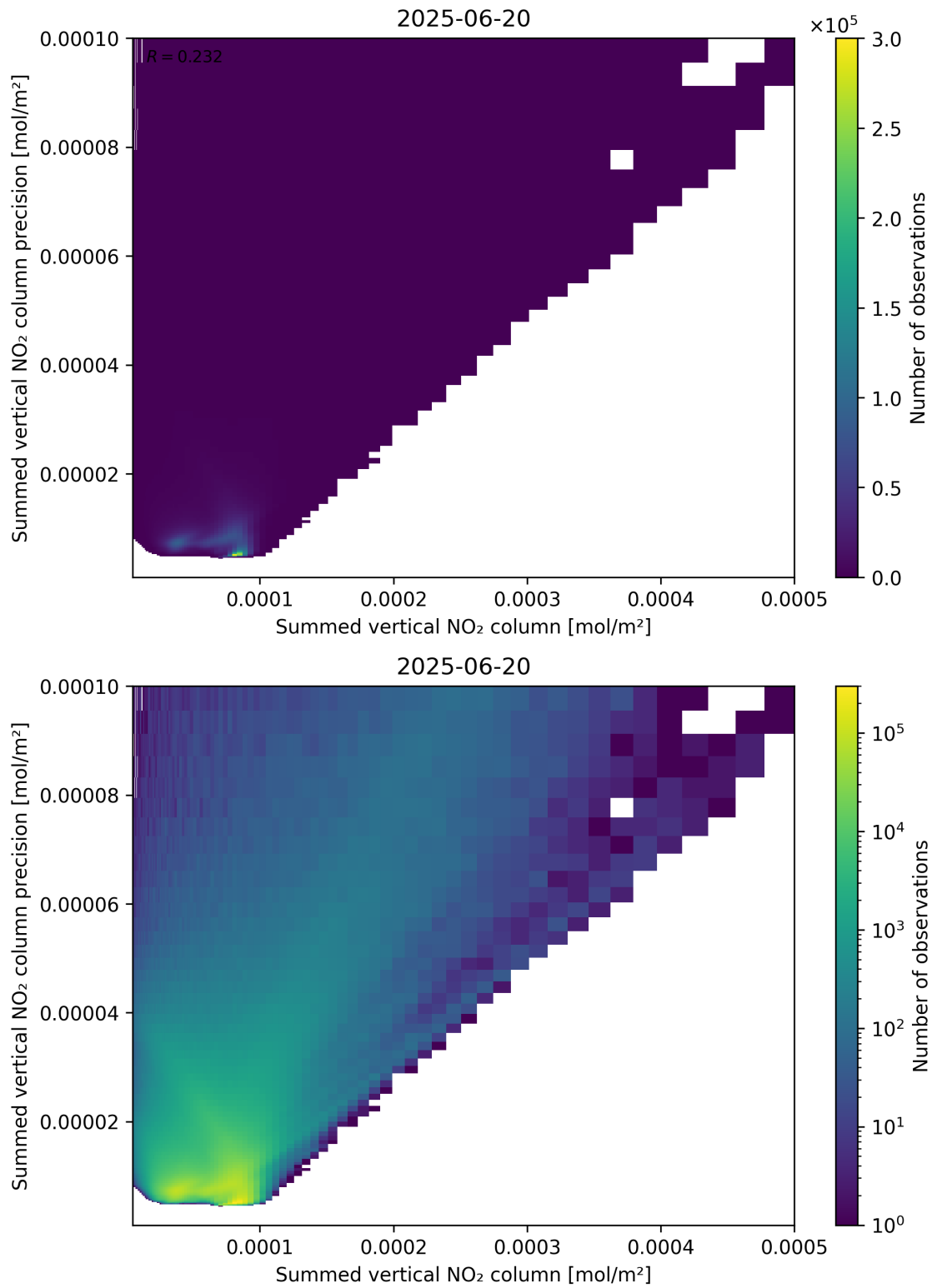
Figure 105: Scatter density plot of “Summed vertical NO 2 column” against “Summed vertical NO 2 column precision” for 2025-06-19 to 2025-06-21.
