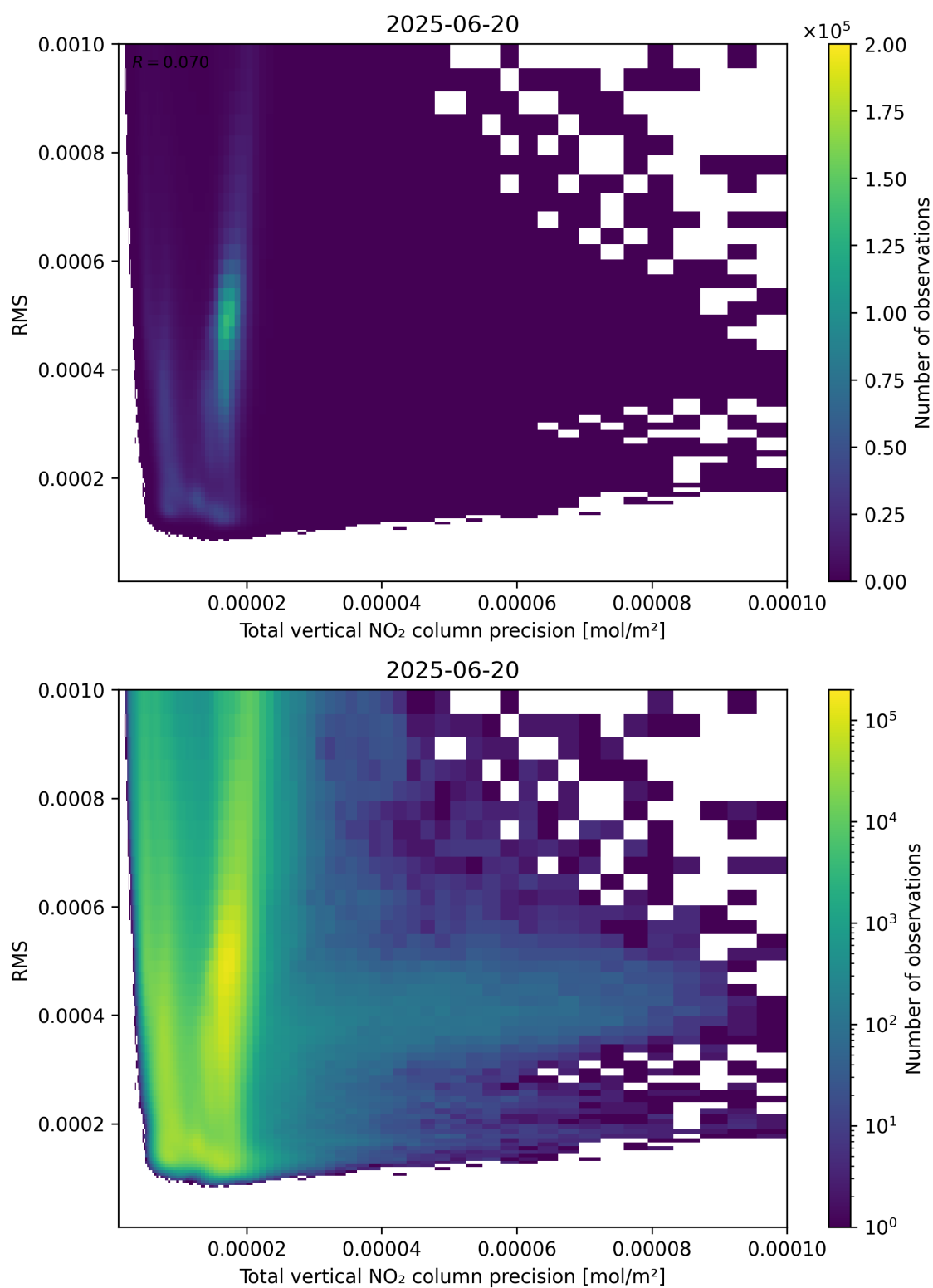
Figure 119: Scatter density plot of “Total vertical NO 2 column precision” against “RMS” for 2025-06-19 to 2025-06-21.
