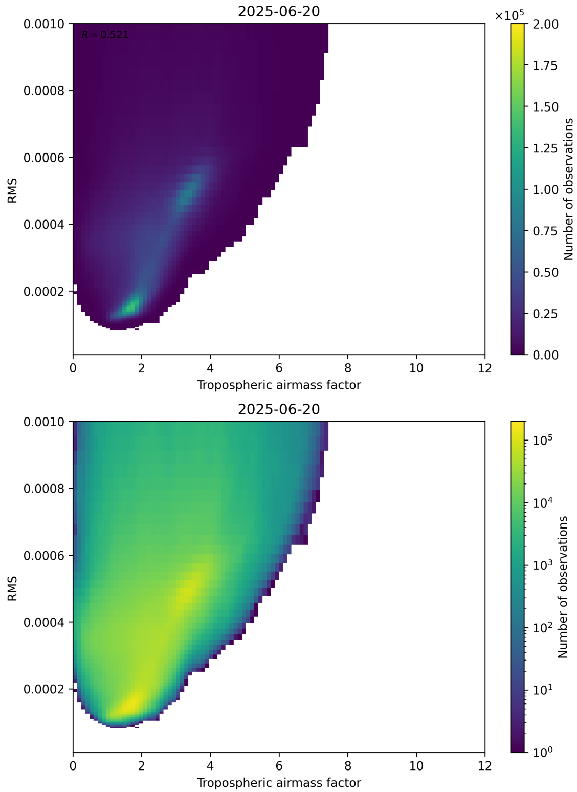
Figure 79: Scatter density plot of “Tropospheric airmass factor” against “RMS” for 2025-06-19 to 2025-06-21.
