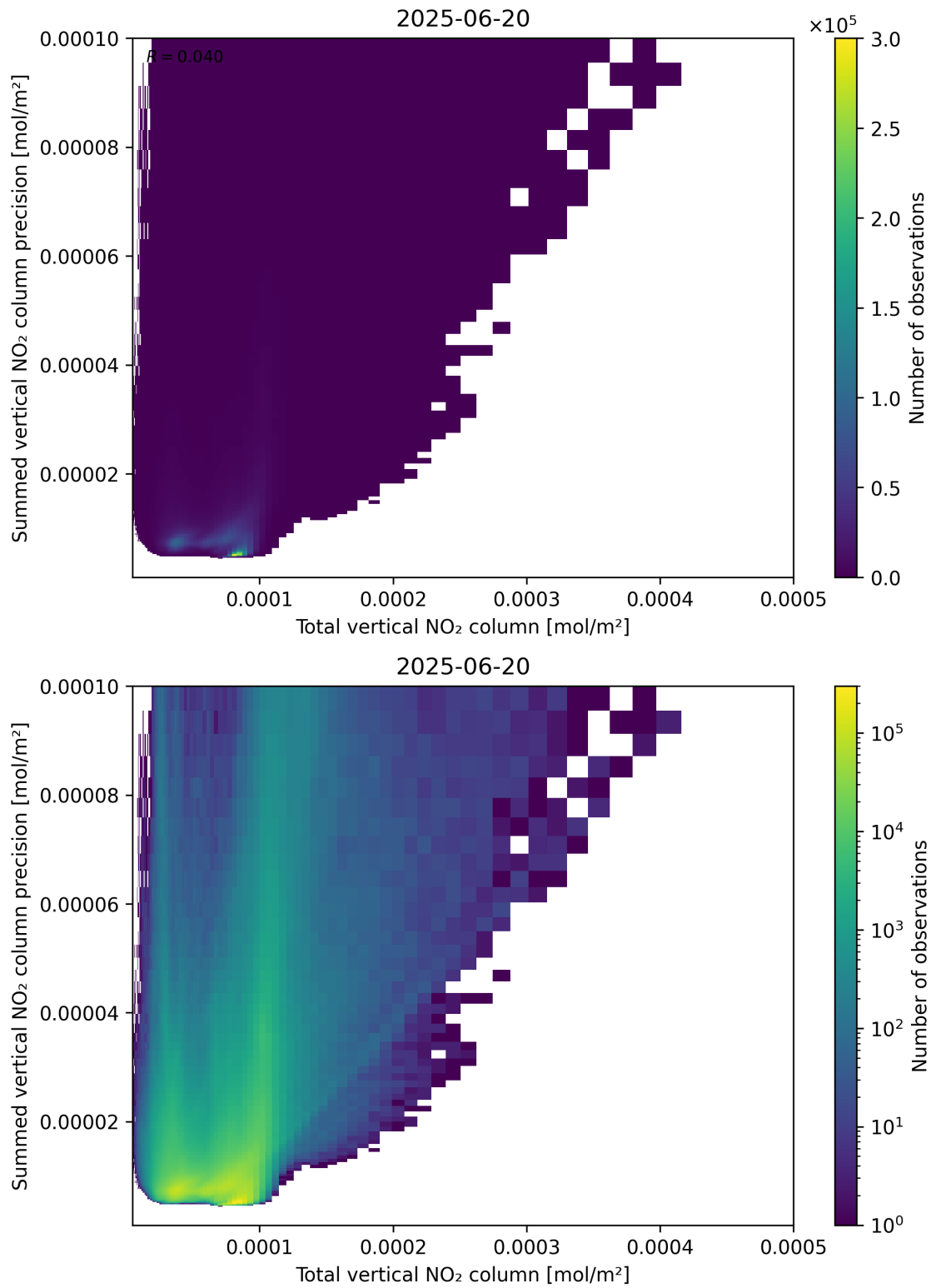
Figure 113: Scatter density plot of “Total vertical NO 2 column” against “Summed vertical NO 2 column precision” for 2025-06-19 to 2025-06-21.
