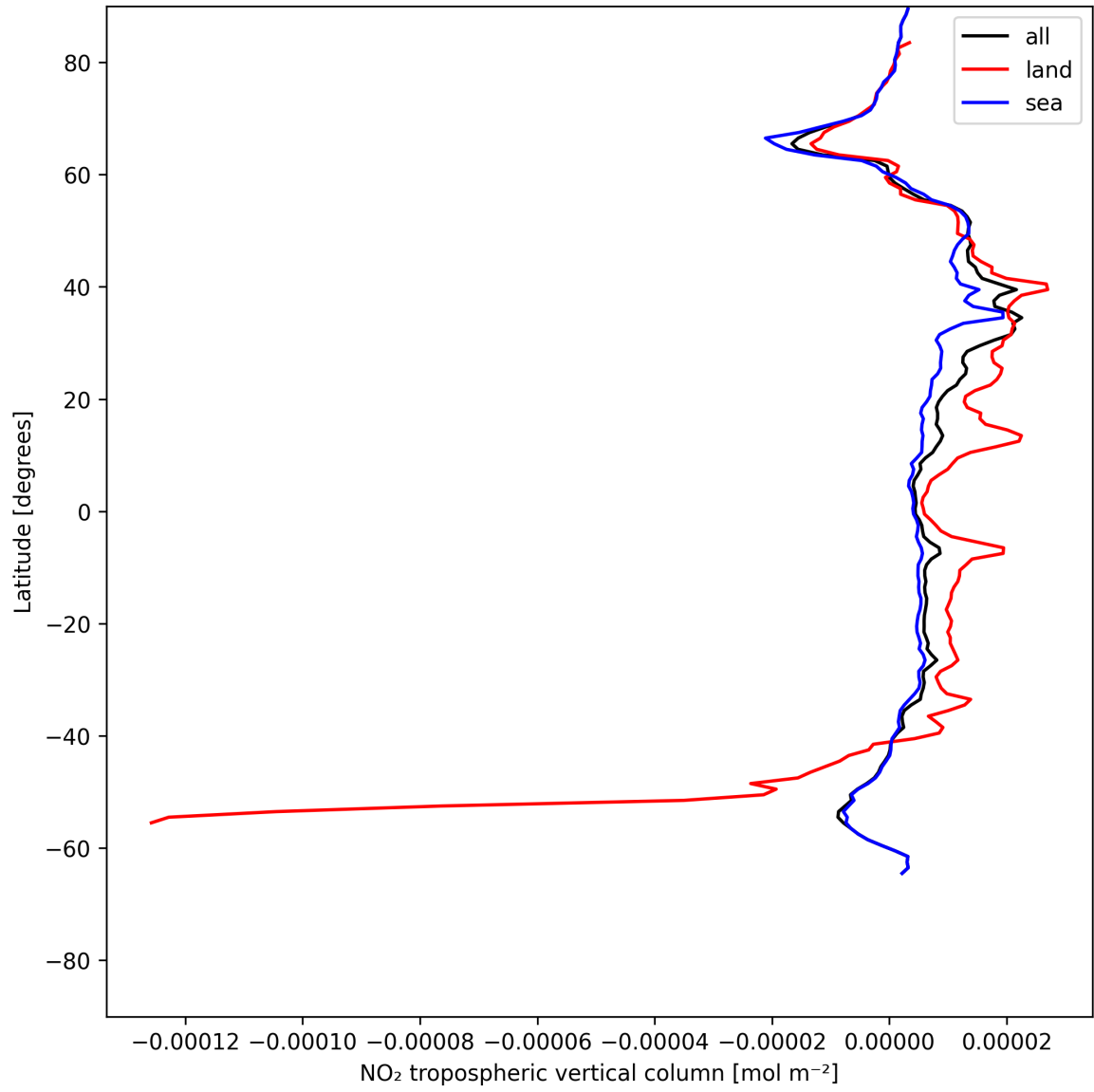
Figure 12: Zonal average of “NO 2 tropospheric vertical column” for 2025-06-19 to 2025-06-21.
