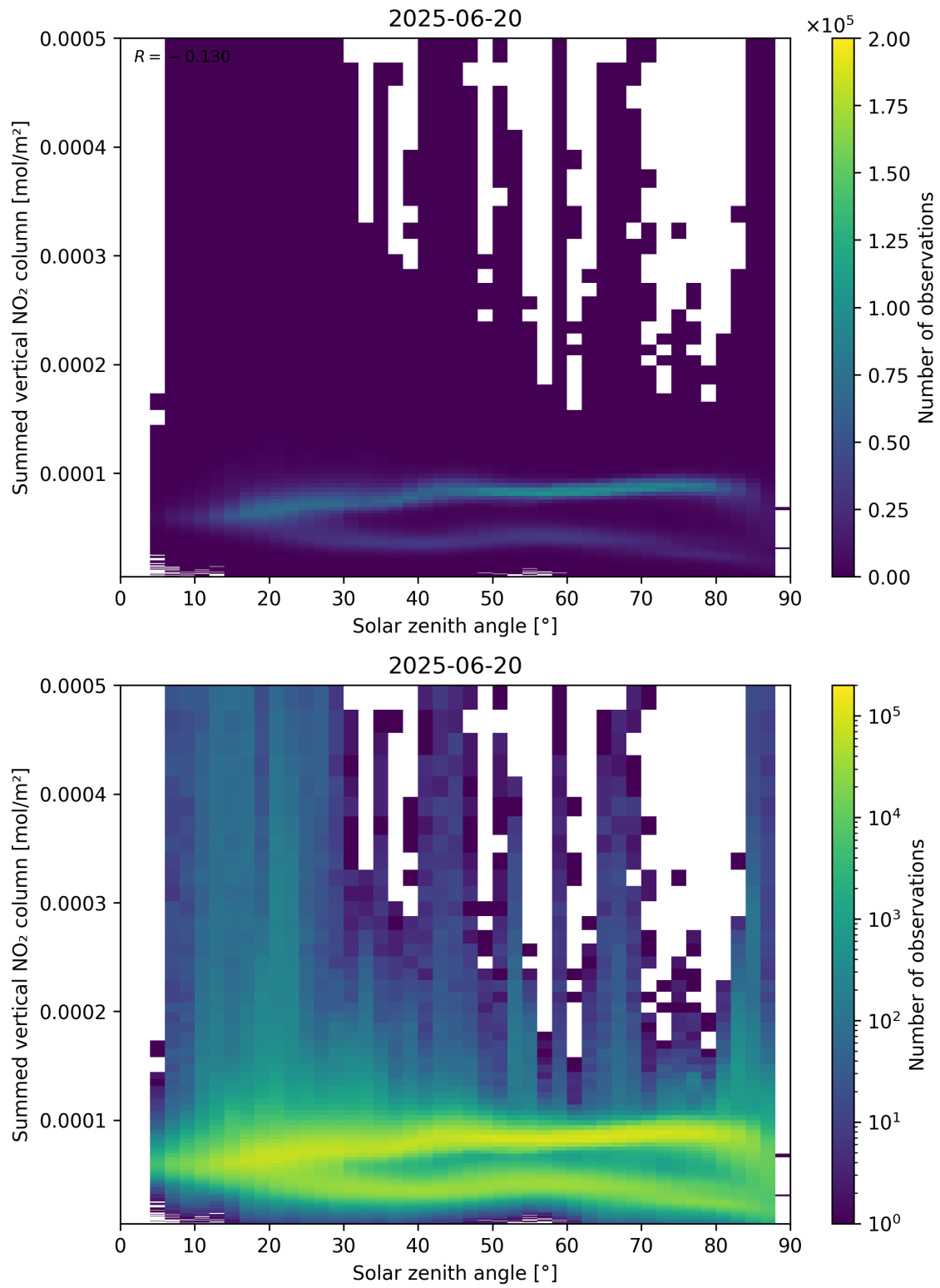
Figure 151: Scatter density plot of “Solar zenith angle” against “Summed vertical NO 2 column” for 2025-06-19 to 2025-06-21.
