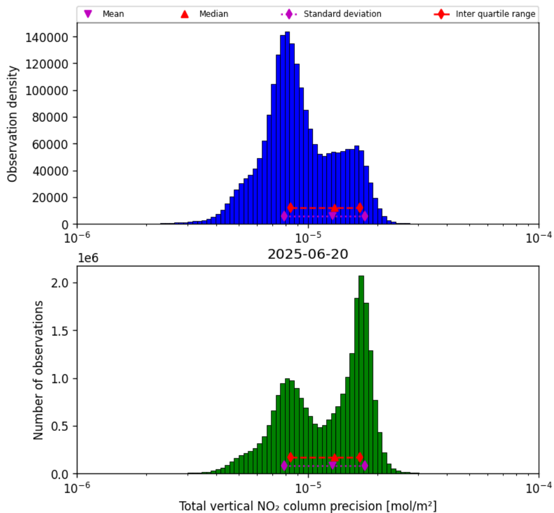
Figure 39: Histogram of “Total vertical NO 2 column precision” for 2025-06-19 to 2025-06-21
