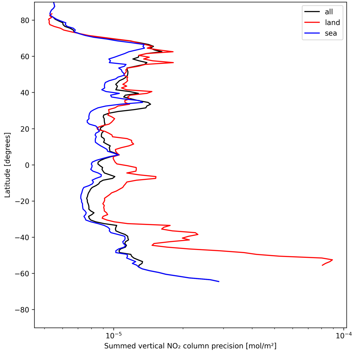
Figure 24: Zonal average of “Summed vertical NO 2 column precision” for 2025-06-19 to 2025-06-21.
