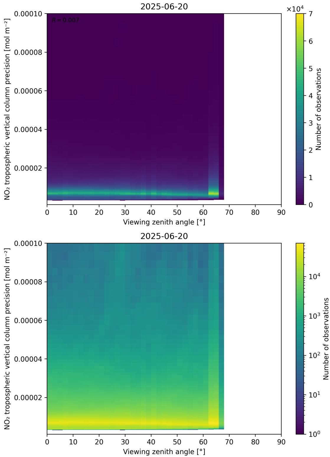
Figure 170: Scatter density plot of “Viewing zenith angle” against “NO 2 tropospheric vertical column precision” for 2025-06-19 to 2025-06-21.
