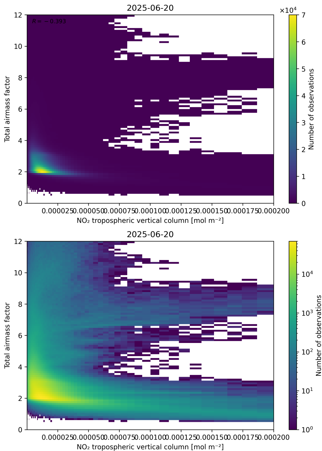
Figure 122: Scatter density plot of “NO 2 tropospheric vertical column” against “Total air mass factor” for 2025-06-19 to 2025-06-21.
