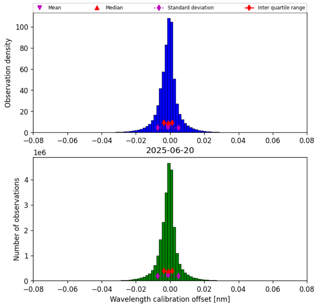
Figure 35: Histogram of “Wavelength calibration offset” for 2025-06-19 to 2025-06-21
