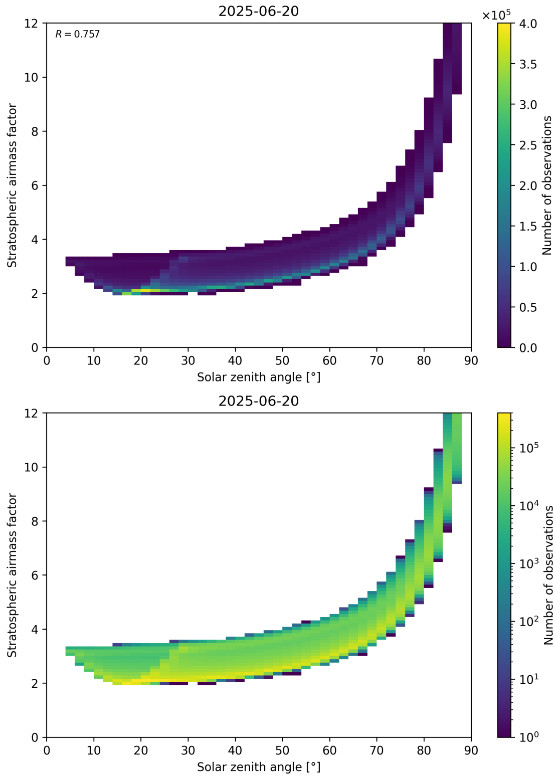
Figure 145: Scatter density plot of “Solar zenith angle” against “Stratospheric airmass factor” for 2025-06-19 to 2025-06-21.
