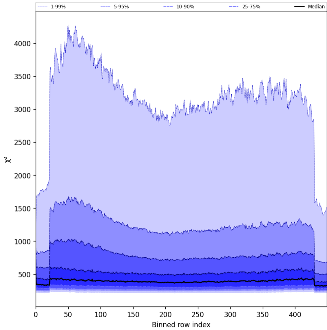
Figure 59: Along track statistics of “ \chi^2 ” for 2025-06-19 to 2025-06-21
