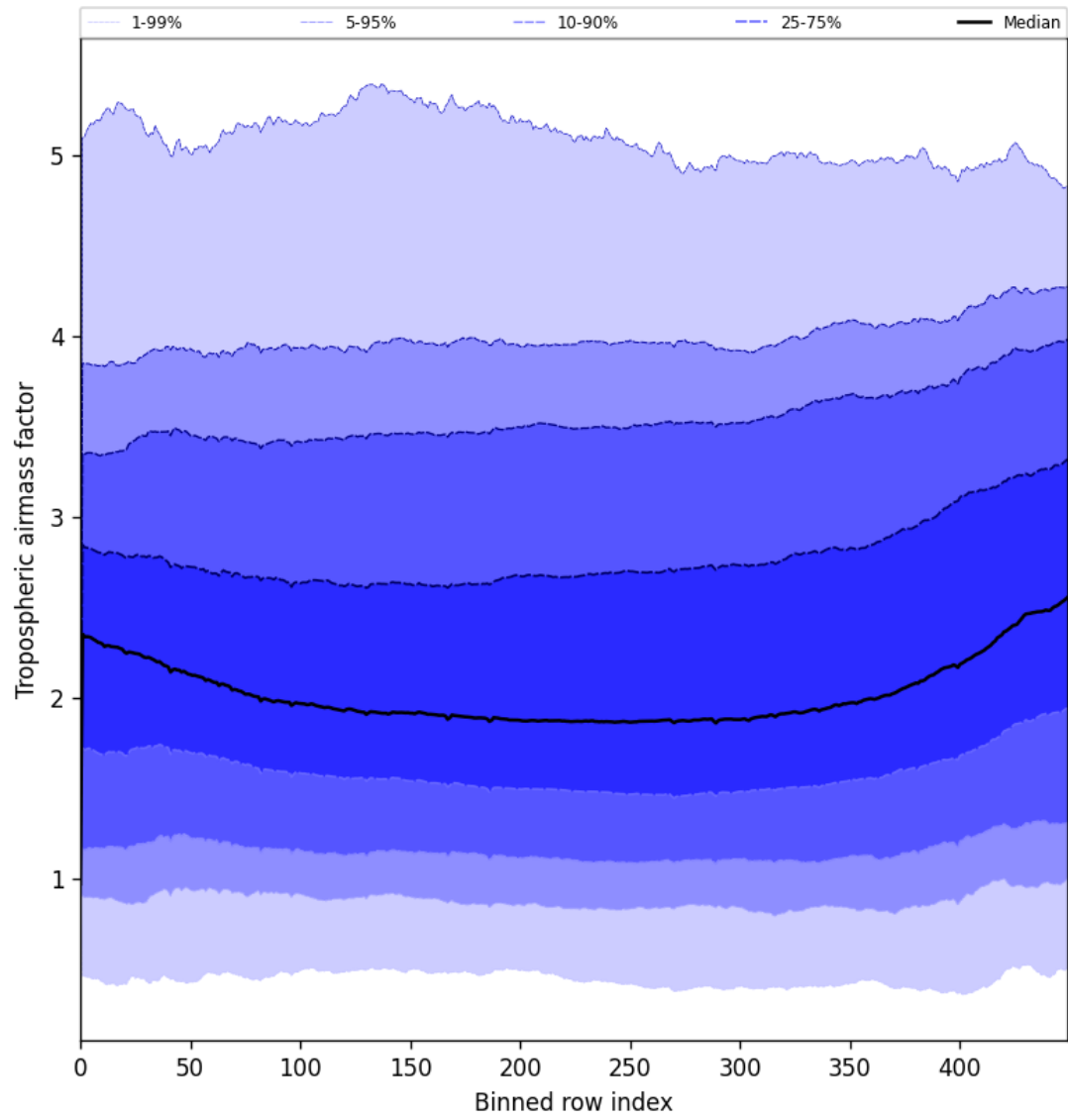
Figure 48: Along track statistics of “Tropospheric airmass factor” for 2025-06-19 to 2025-06-21
