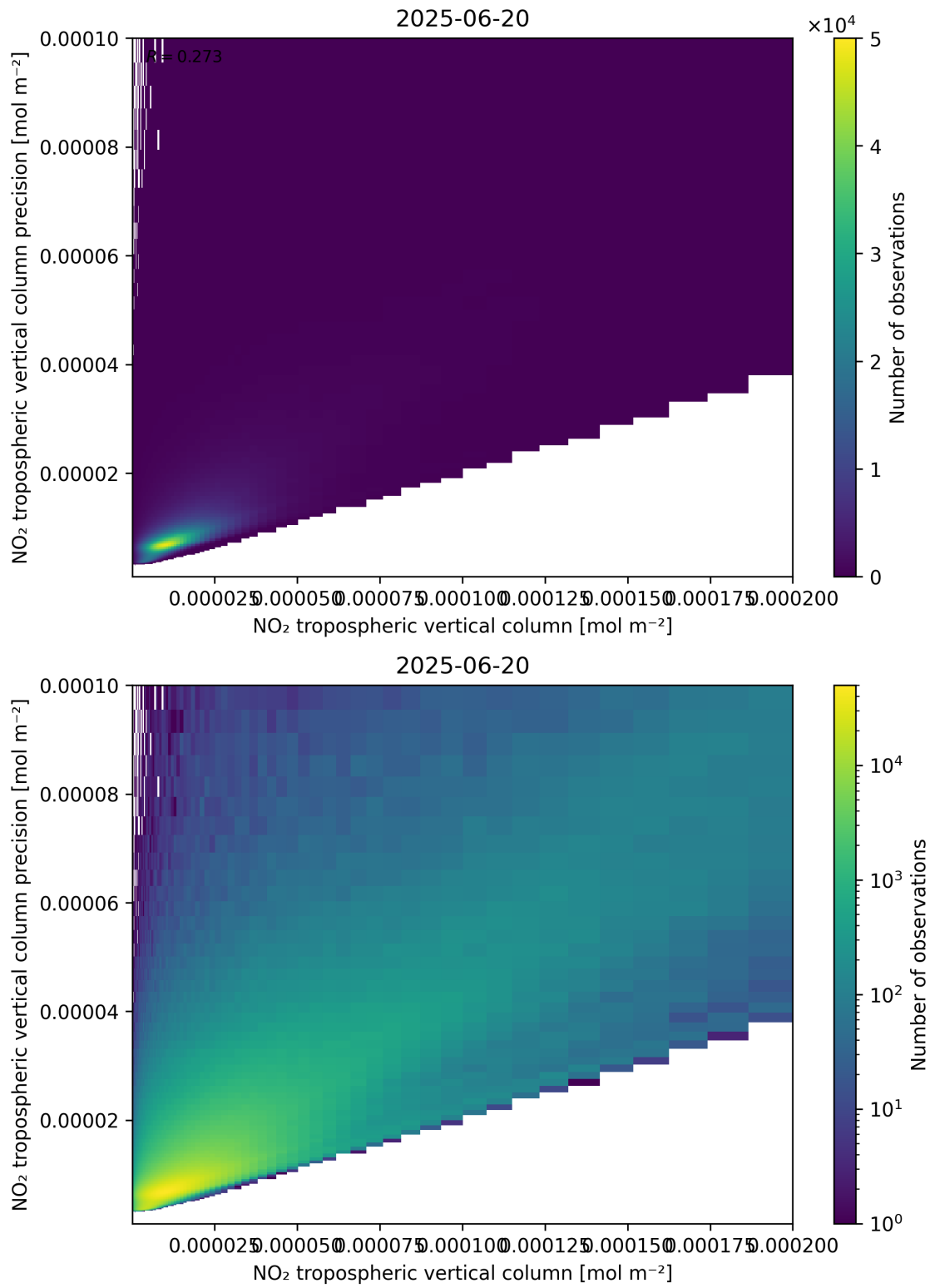
Figure 130: Scatter density plot of “NO 2 tropospheric vertical column” against “NO 2 tropospheric vertical column precision” for 2025-06-19 to 2025-06-21.
