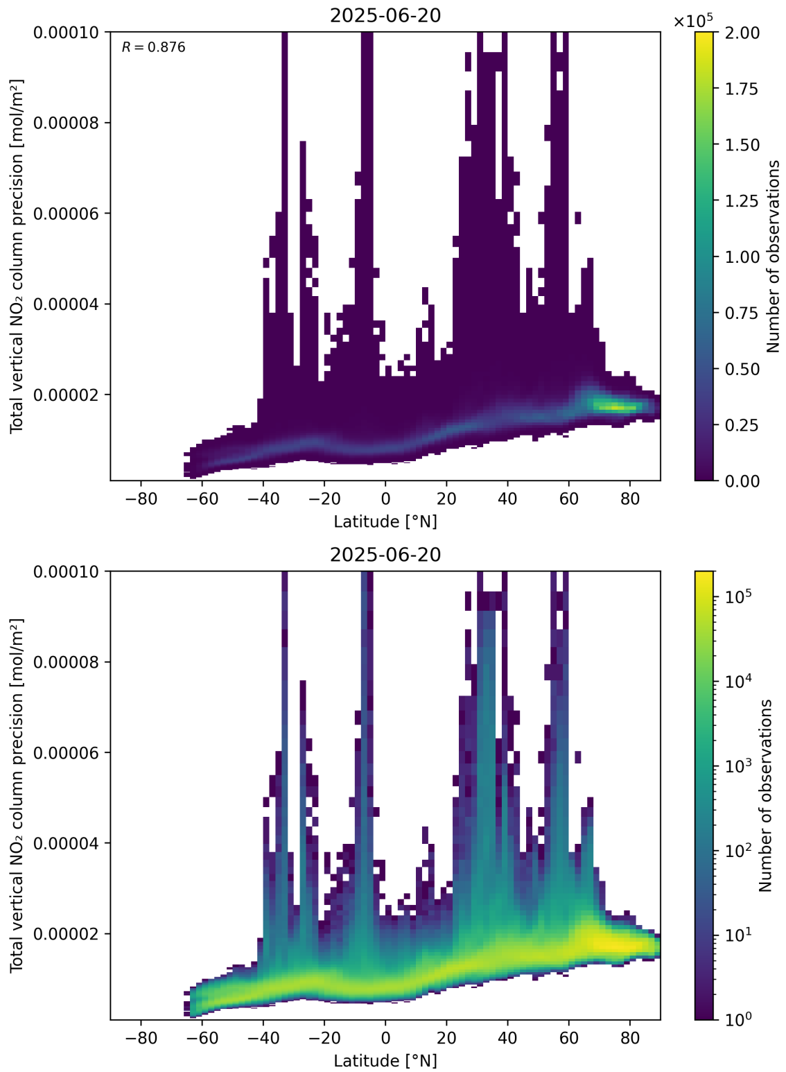
Figure 91: Scatter density plot of “Latitude” against “Total vertical NO 2 column precision” for 2025-06-19 to 2025-06-21.
