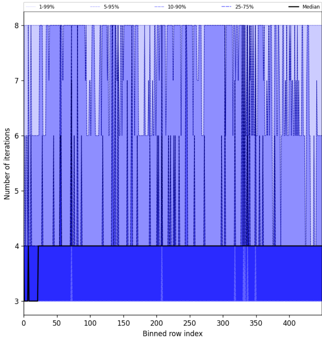
Figure 51: Along track statistics of “Number of iterations” for 2025-06-19 to 2025-06-21
