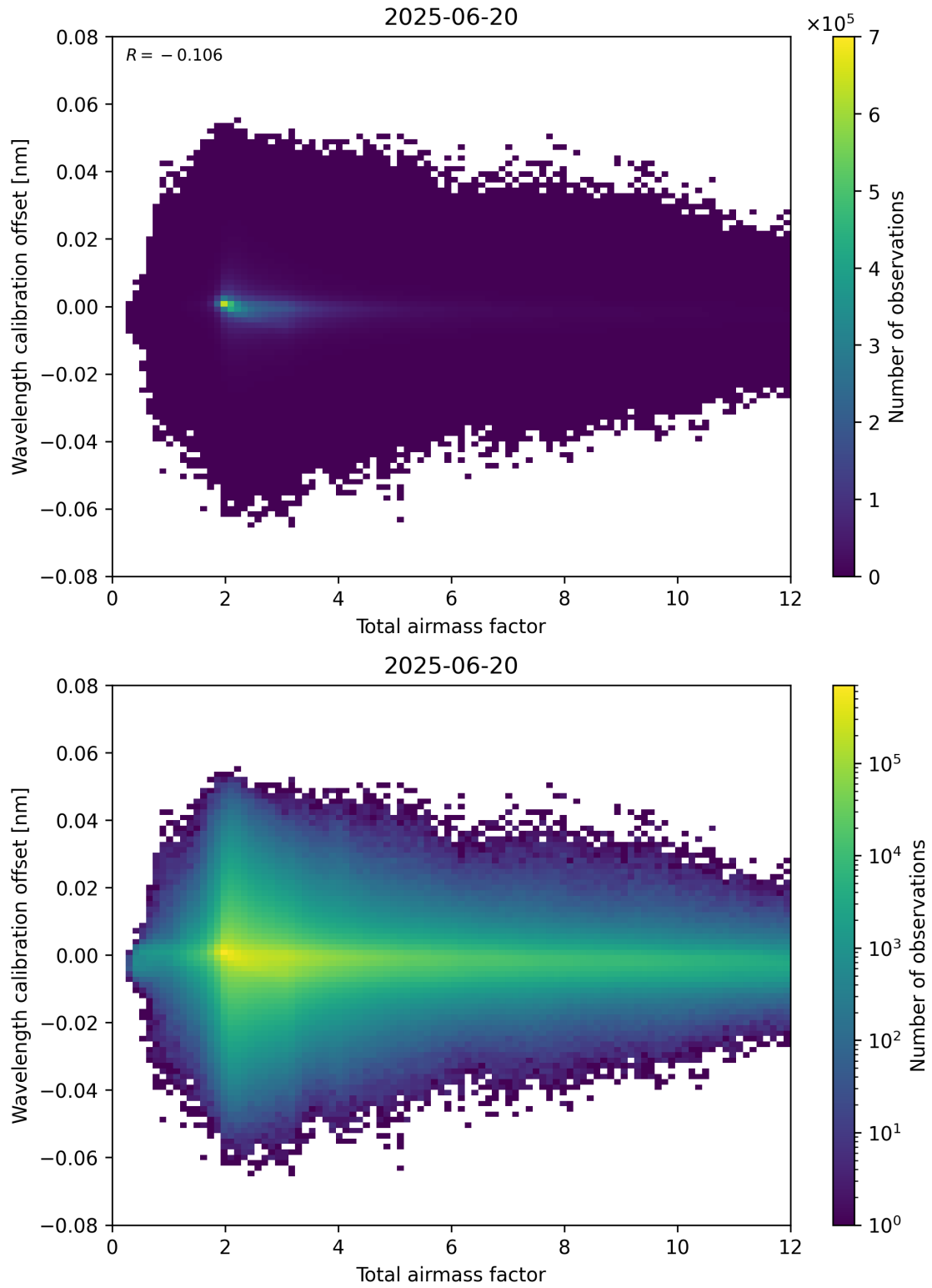
Figure 70: Scatter density plot of “Total airmass factor” against “Wavelength calibration offset” for 2025-06-19 to 2025-06-21.
