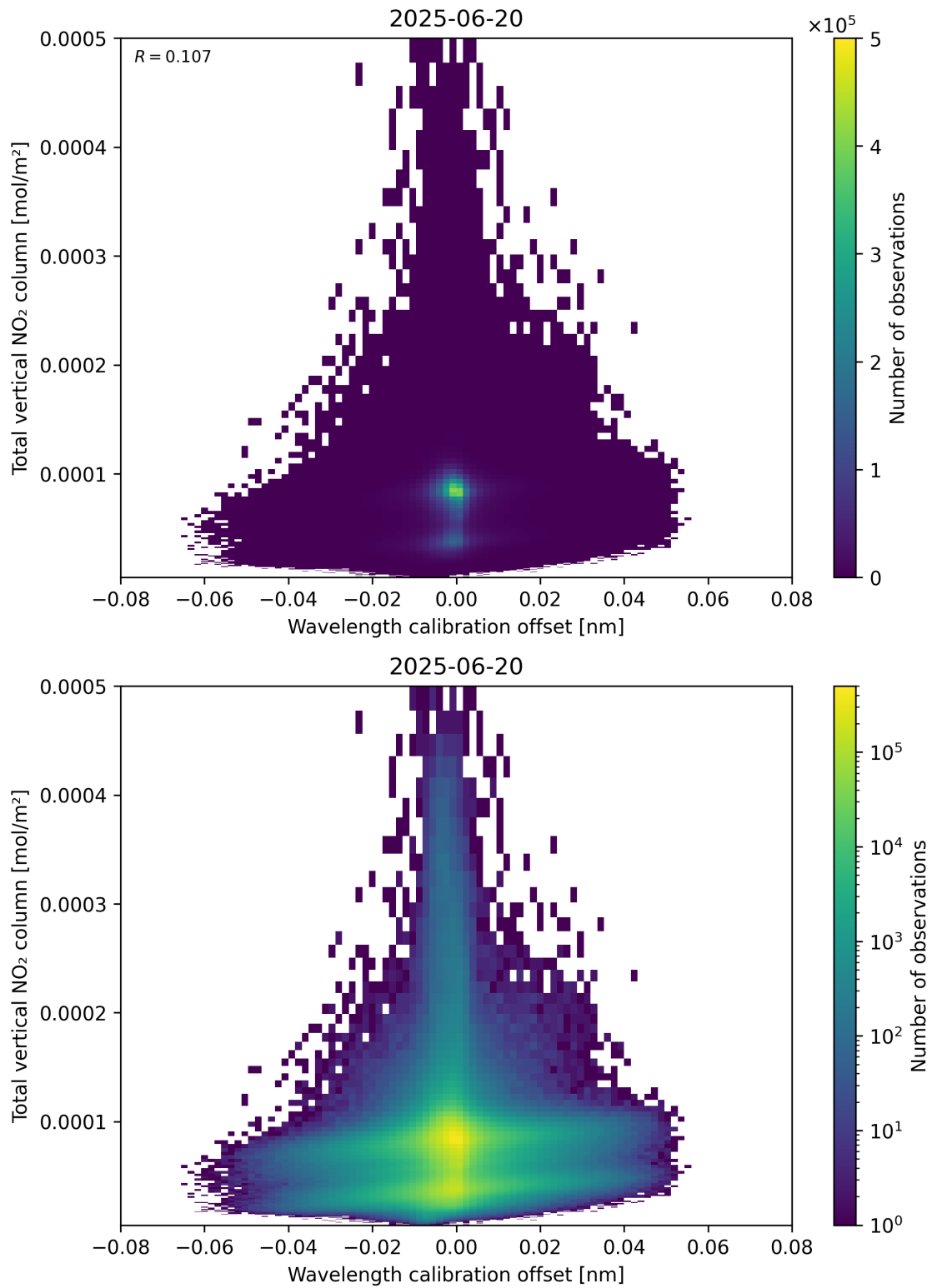
Figure 179: Scatter density plot of “Wavelength calibration offset” against “Total vertical NO 2 column” for 2025-06-19 to 2025-06-21.
