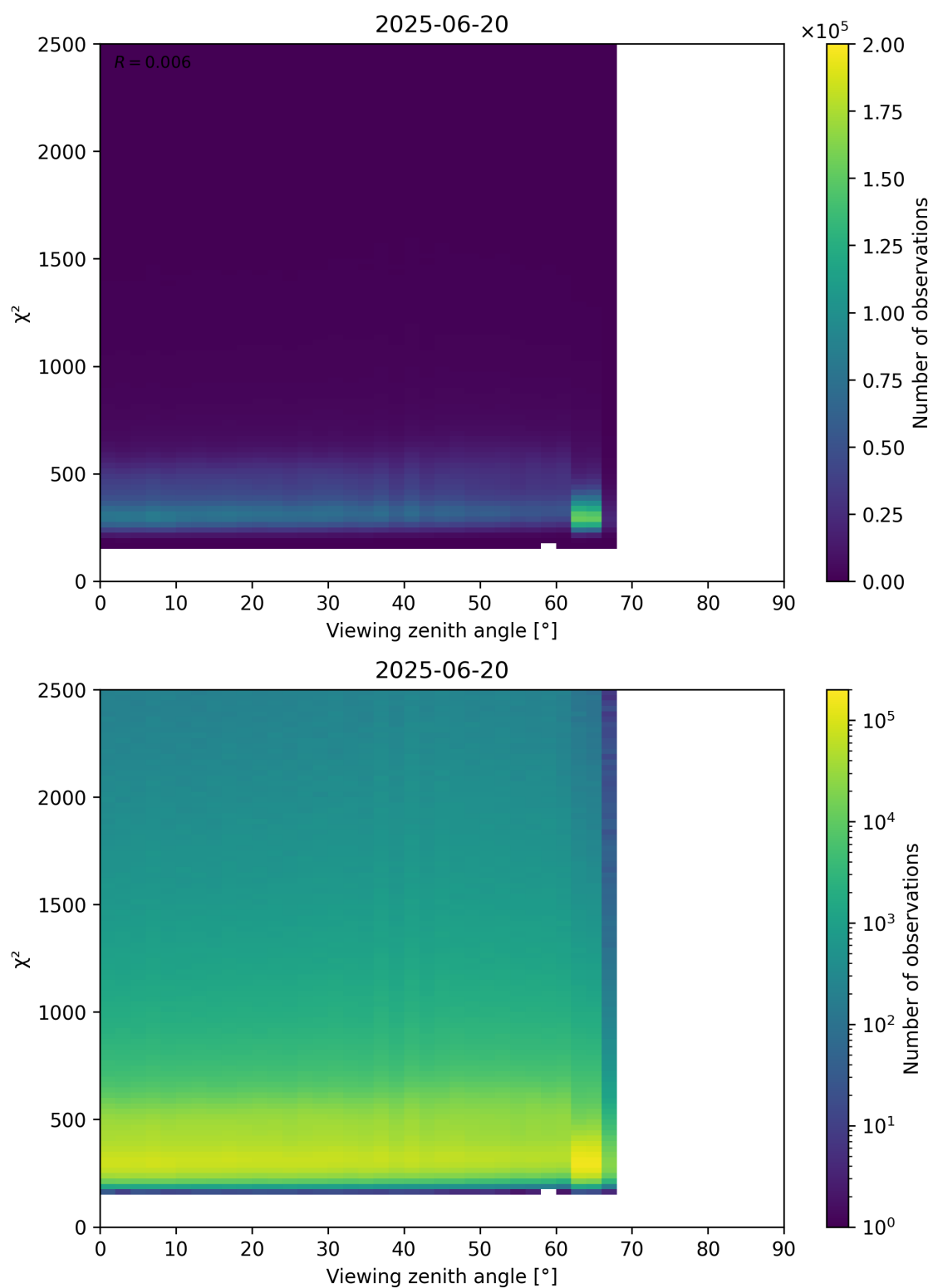
Figure 162: Scatter density plot of “Viewing zenith angle” against “ \chi^2 ” for 2025-06-19 to 2025-06-21.
