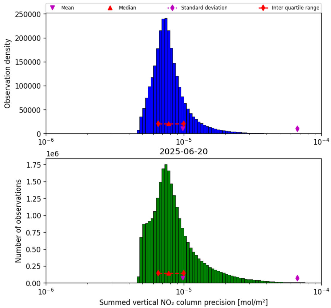
Figure 41: Histogram of "Summed vertical NO 2 column precision" for 2025-06-19 to 2025-06-21
