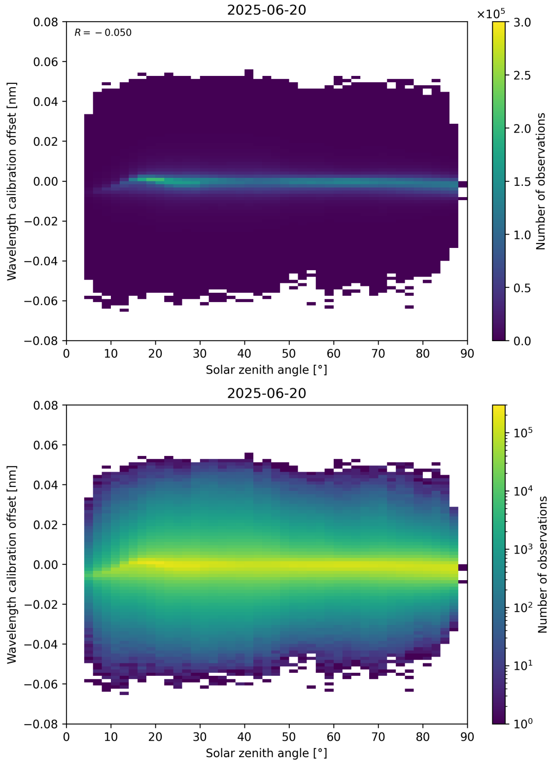
Figure 158: Scatter density plot of “Solar zenith angle” against “Wavelength calibration offset” for 2025-06-19 to 2025-06-21.
