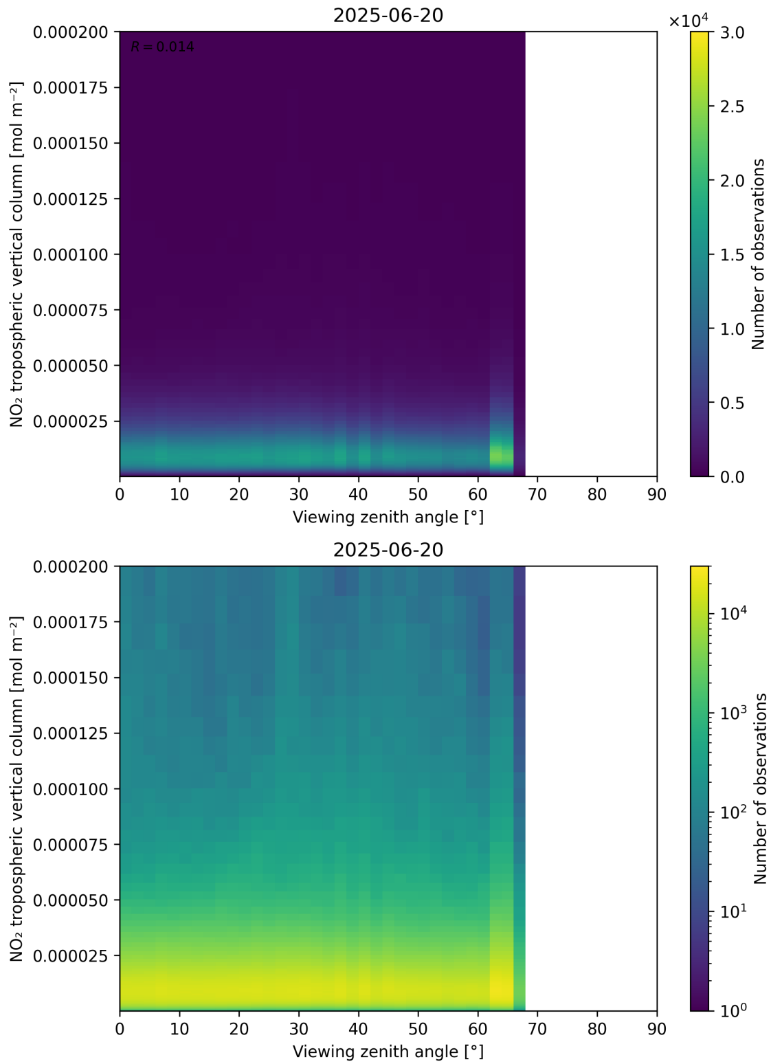
Figure 169: Scatter density plot of “Viewing zenith angle” against “NO 2 tropospheric vertical column” for 2025-06-19 to 2025-06-21.
