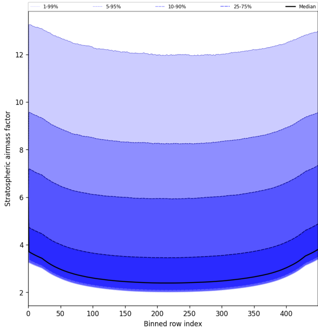
Figure 61: Along track statistics of “Stratospheric airmass factor” for 2025-06-19 to 2025-06-21
