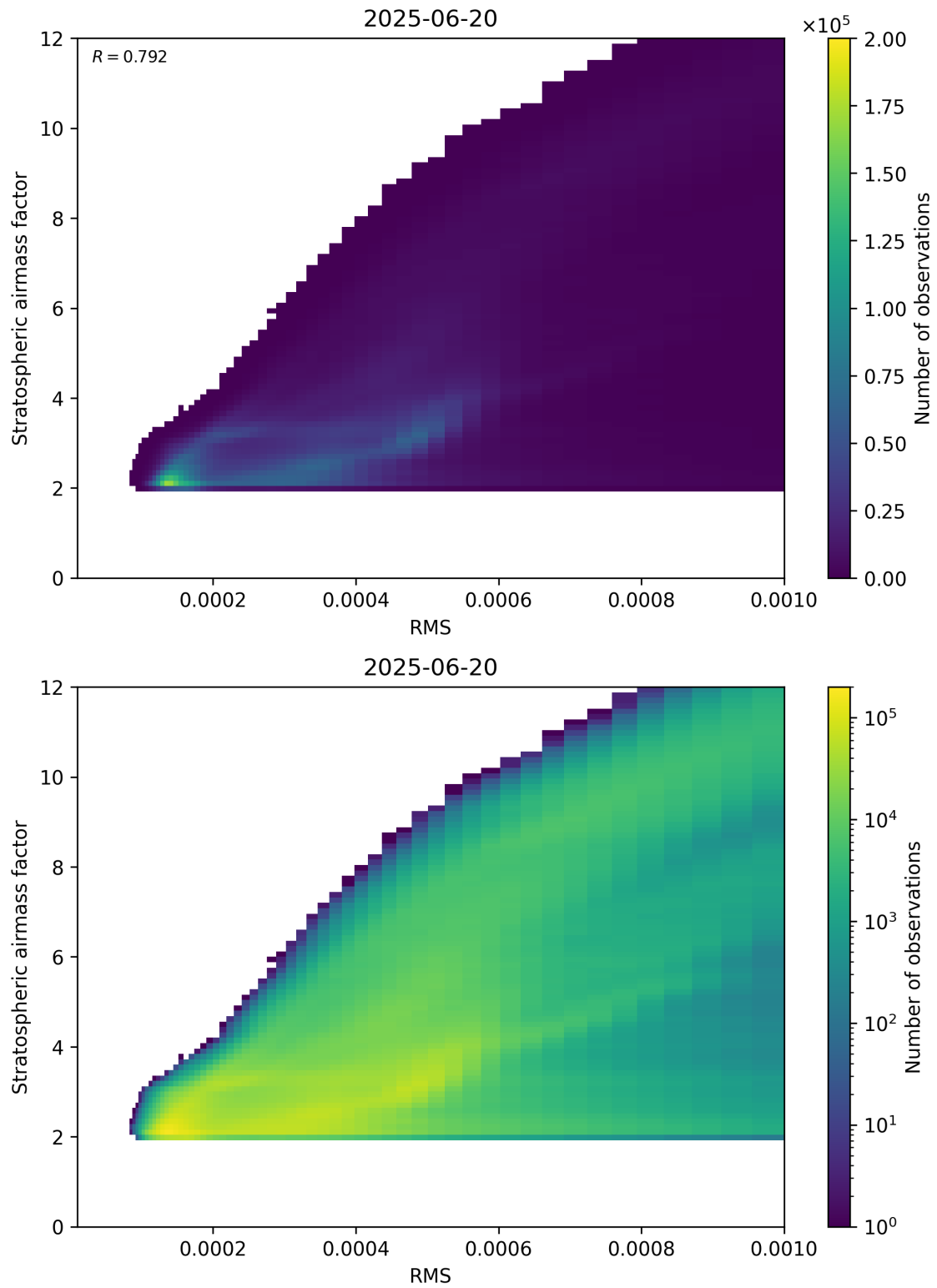
Figure 144: Scatter density plot of “RMS” against “Stratospheric airmass factor” for 2025-06-19 to 2025-06-21.
