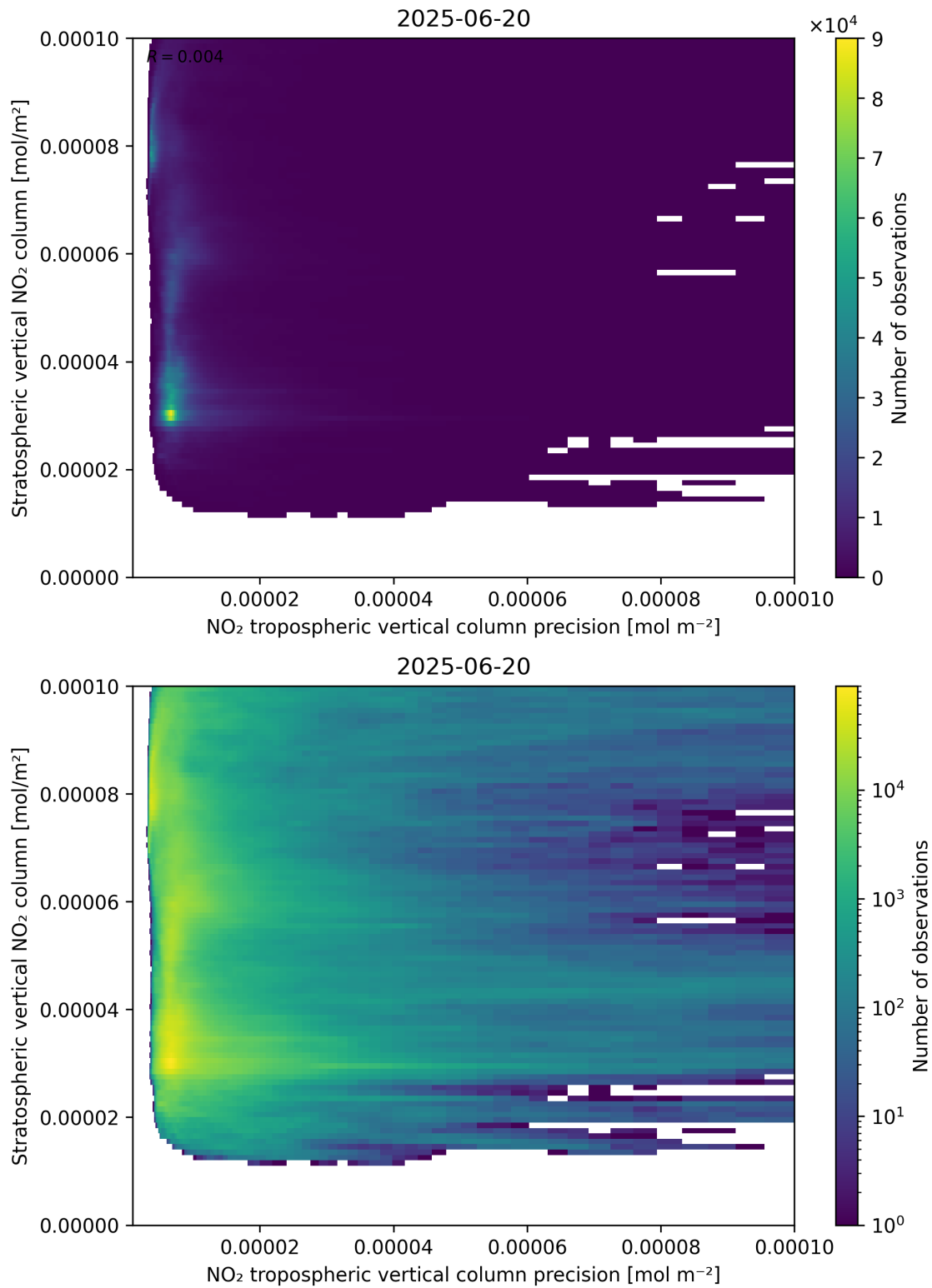
Figure 135: Scatter density plot of “NO 2 tropospheric vertical column precision” against “Stratospheric vertical NO 2 column” for 2025-06-19 to 2025-06-21.
