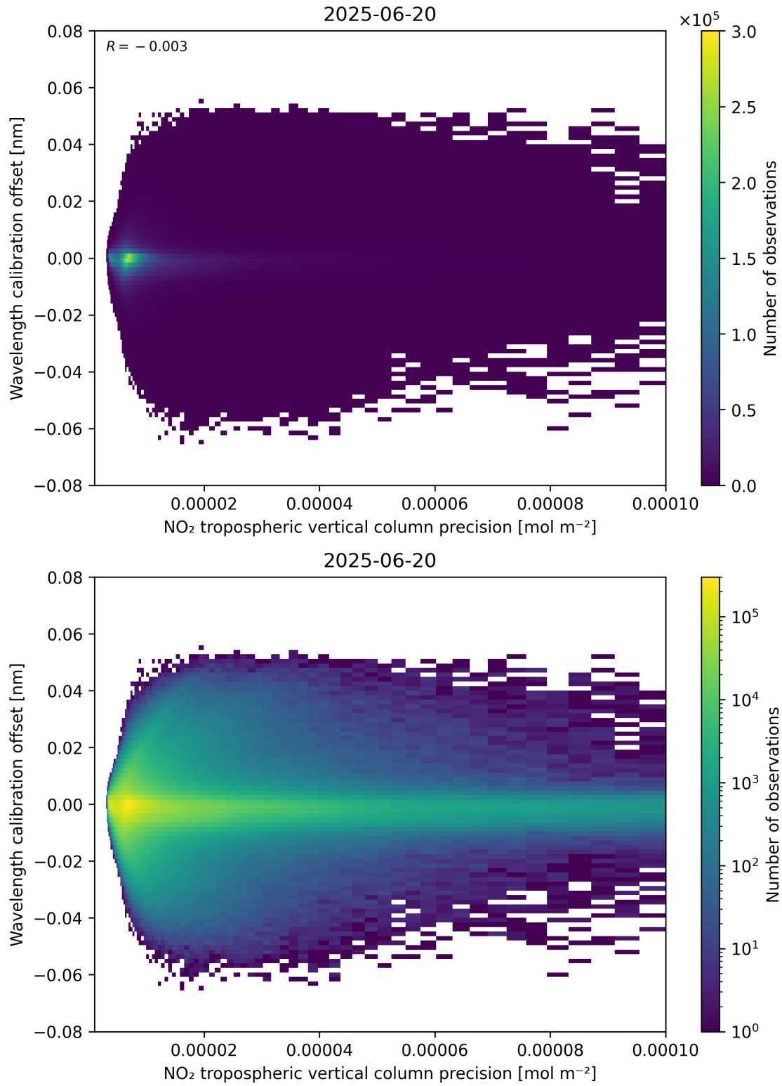
Figure 141: Scatter density plot of “NO 2 tropospheric vertical column precision” against “Wavelength calibration offset” for 2025-06-19 to 2025-06-21.
