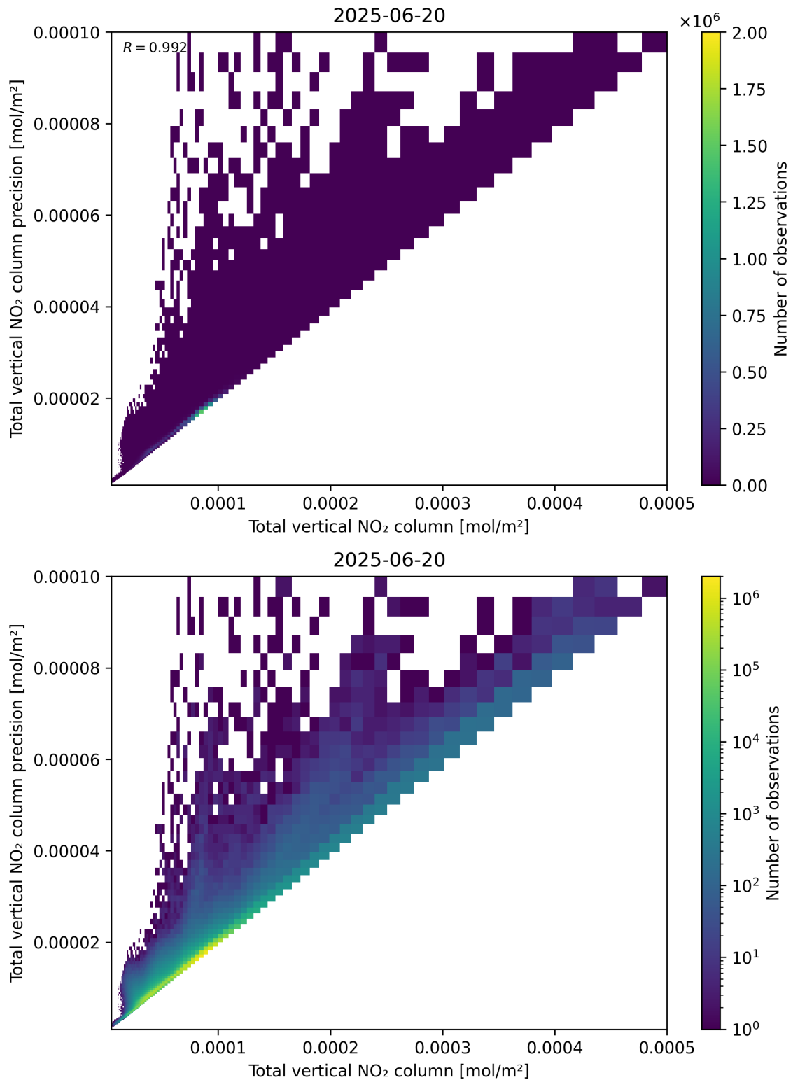
Figure 114: Scatter density plot of “Total vertical NO 2 column” against “Total vertical NO 2 column precision” for 2025-06-19 to 2025-06-21.
