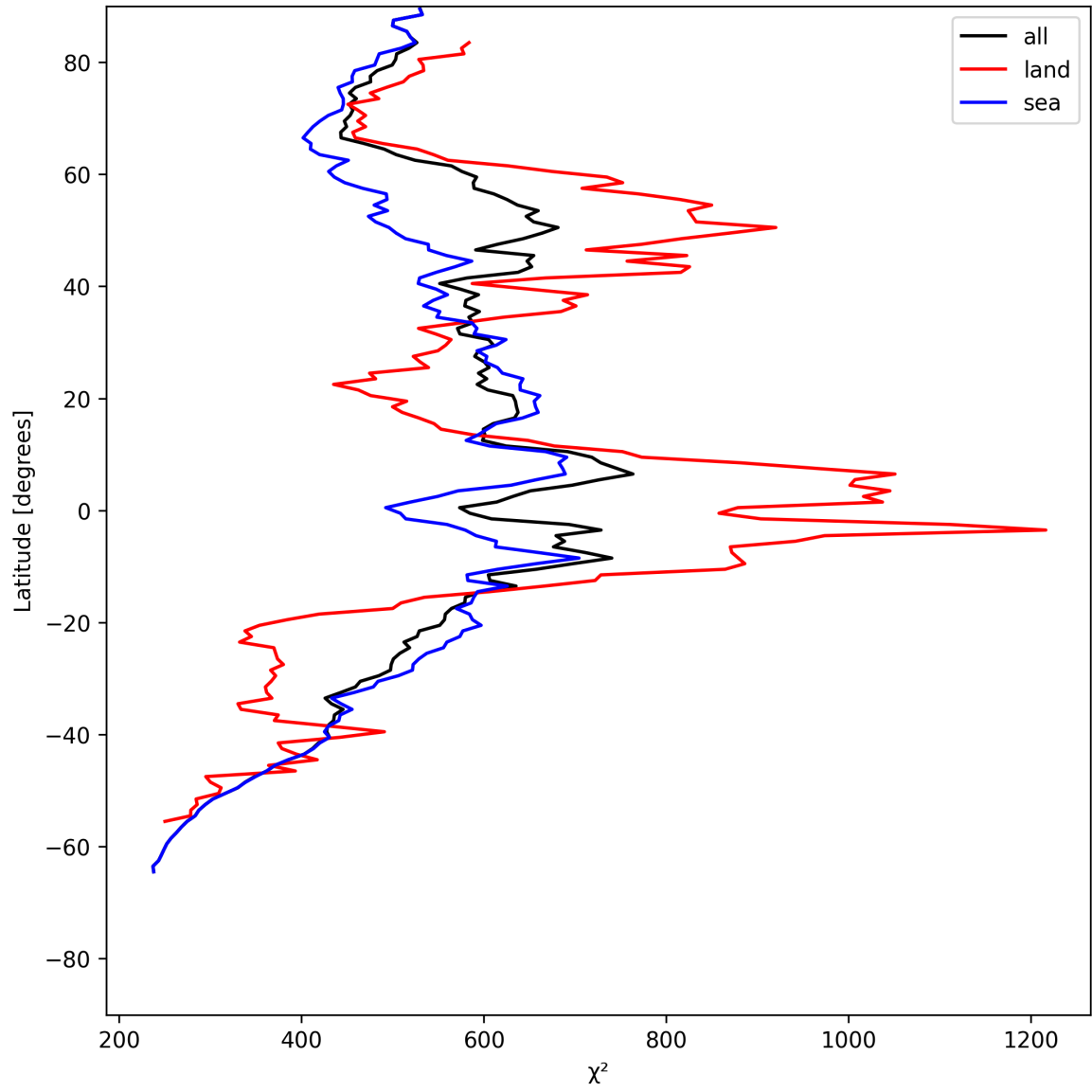
Figure 25: Zonal average of “ \chi^2 ” for 2025-06-19 to 2025-06-21.
