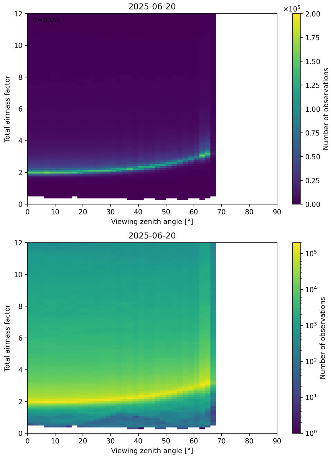
Figure 160: Scatter density plot of “Viewing zenith angle” against “Total airmass factor” for 2025-06-19 to 2025-06-21.
