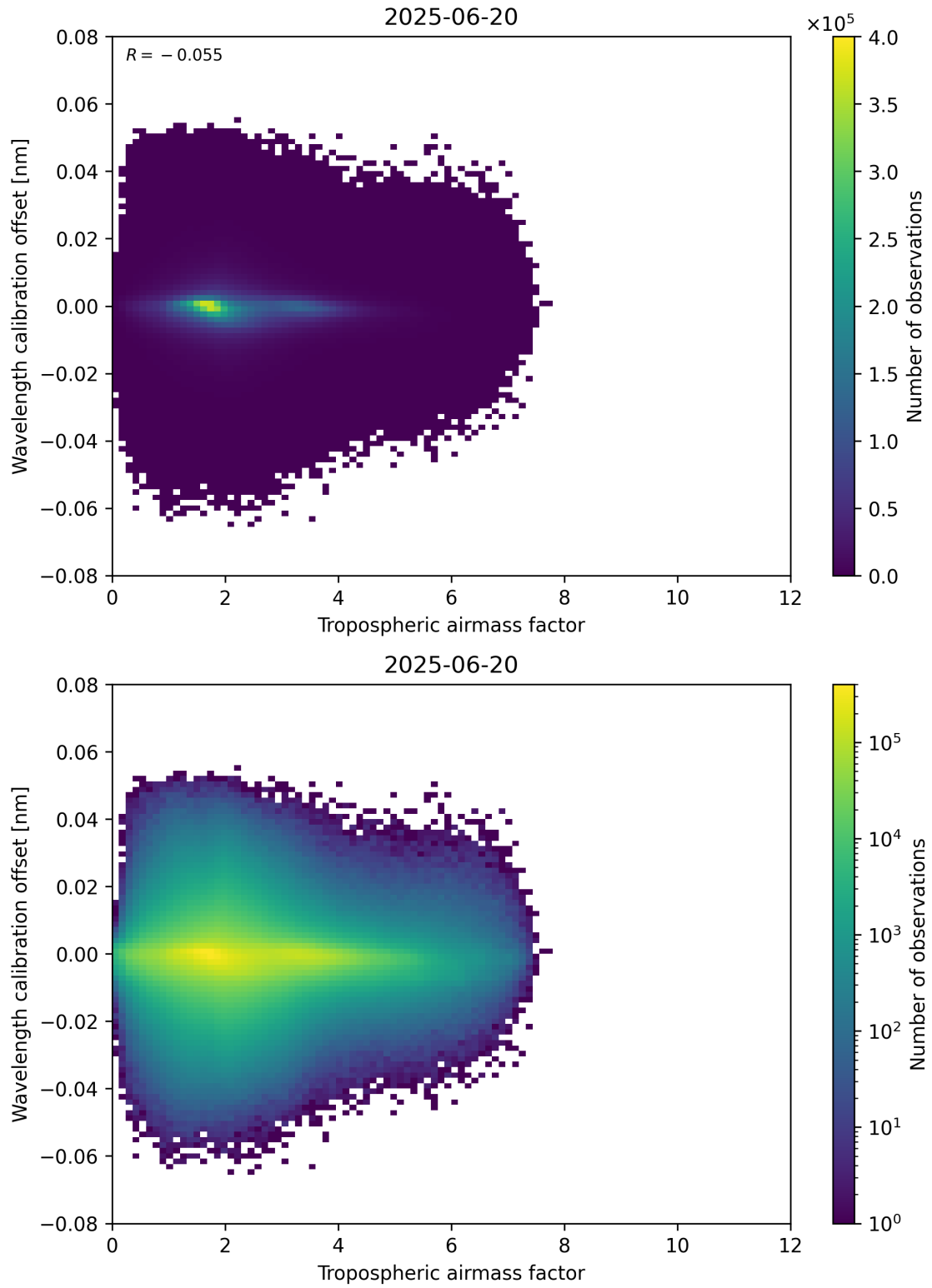
Figure 80: Scatter density plot of “Tropospheric airmass factor” against “Wavelength calibration offset” for 2025-06-19 to 2025-06-21.
