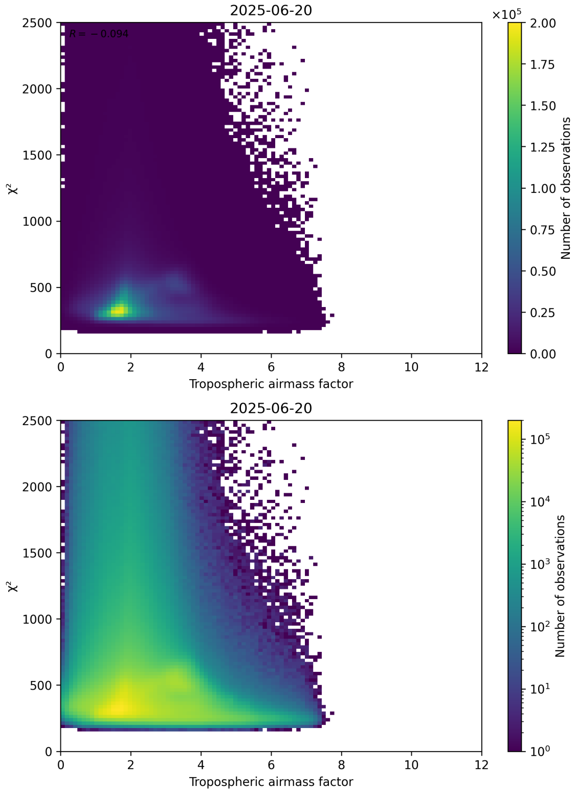
Figure 73: Scatter density plot of “Tropospheric airmass factor” against “ \chi^2 ” for 2025-06-19 to 2025-06-21.
