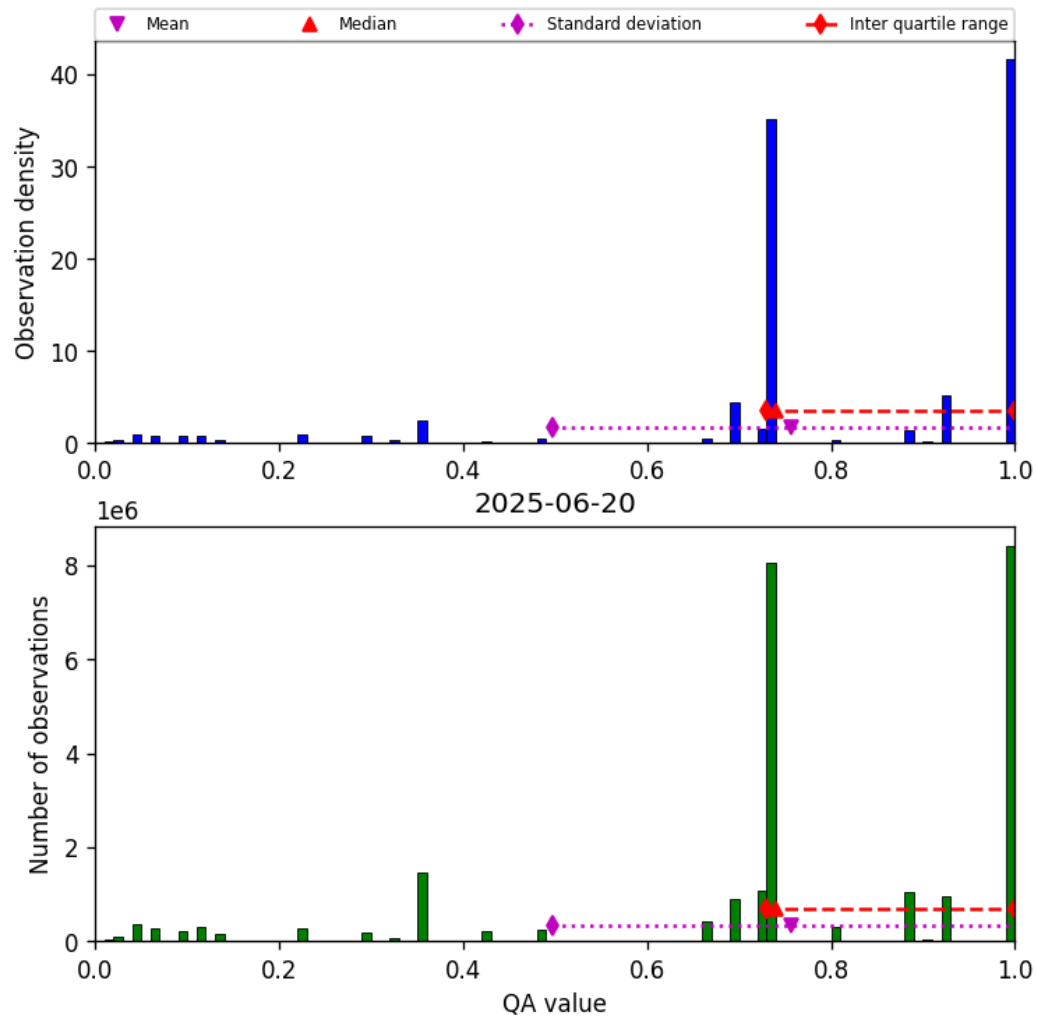
Figure 28: Histogram of “QA value” for 2025-06-19 to 2025-06-21
