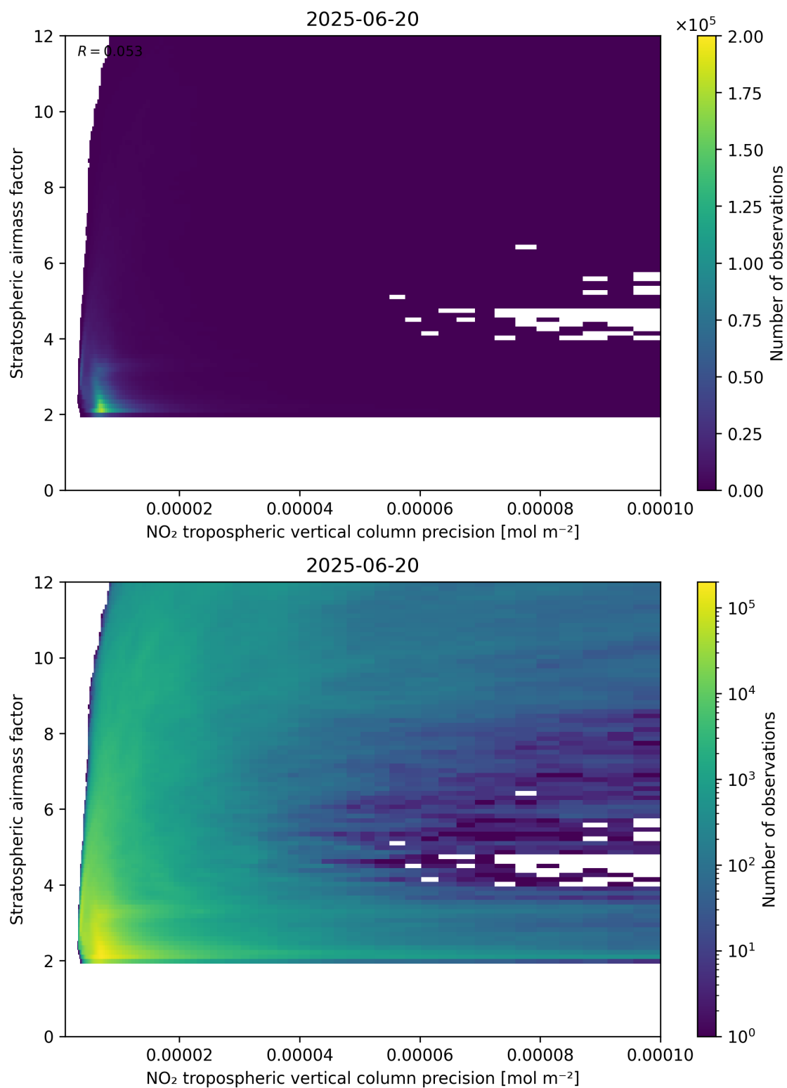
Figure 131: Scatter density plot of “NO 2 tropospheric vertical column precision” against “Stratospheric airmass factor” for 2025-06-19 to 2025-06-21.
