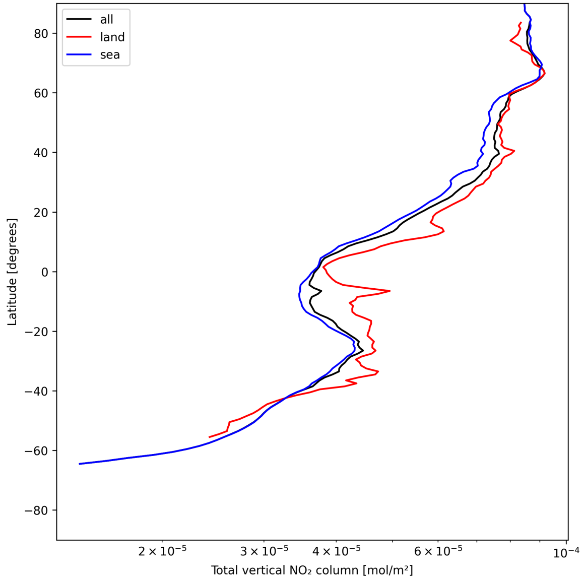
Figure 21: Zonal average of “Total vertical NO 2 column” for 2025-06-19 to 2025-06-21.
