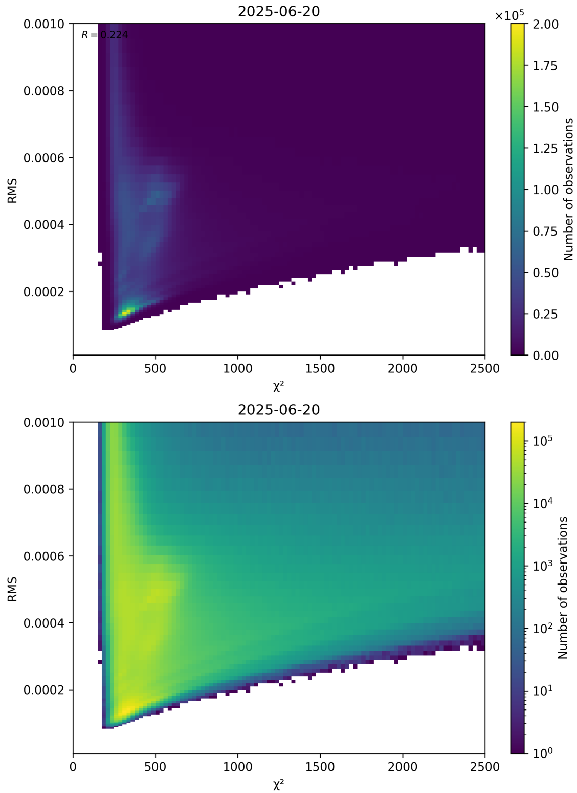
Figure 82: Scatter density plot of “ \chi^2 ” against “RMS” for 2025-06-19 to 2025-06-21.
