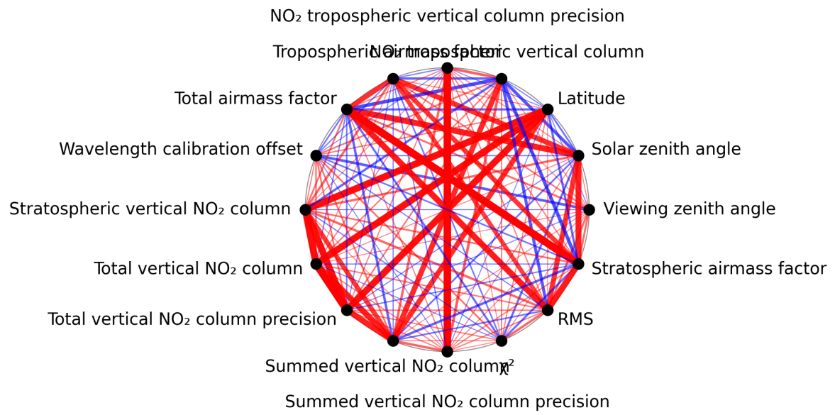
Figure 1: Map of correlation graph for 2025-06-19 to 2025-06-21.
