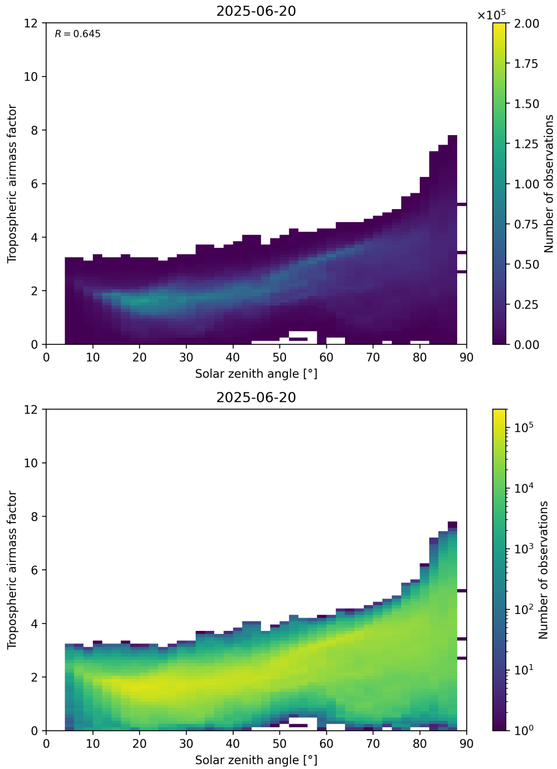
Figure 147: Scatter density plot of “Solar zenith angle” against “Tropospheric airmass factor” for 2025-06-19 to 2025-06-21.
