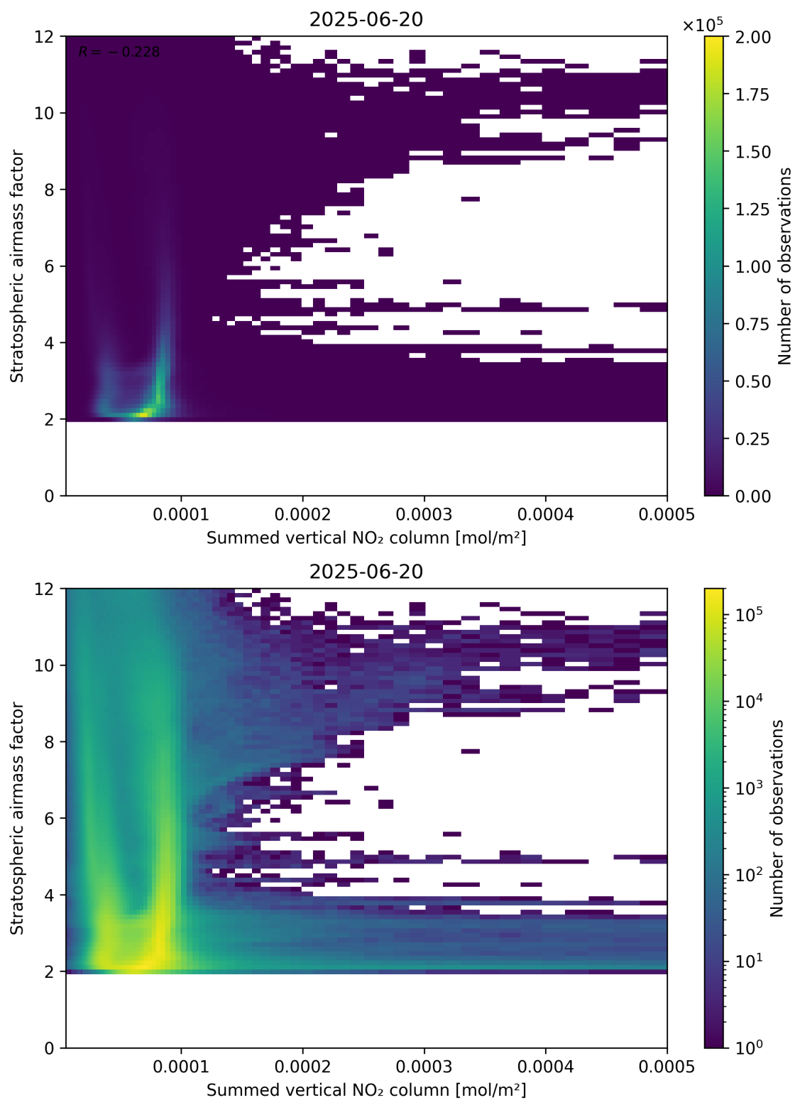
Figure 103: Scatter density plot of “Summed vertical NO 2 column” against “Stratospheric air mass factor” for 2025-06-19 to 2025-06-21.
