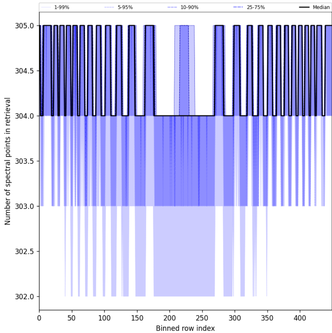
Figure 50: Along track statistics of “Number of spectral points in retrieval” for 2025-06-19 to 2025-06-21
