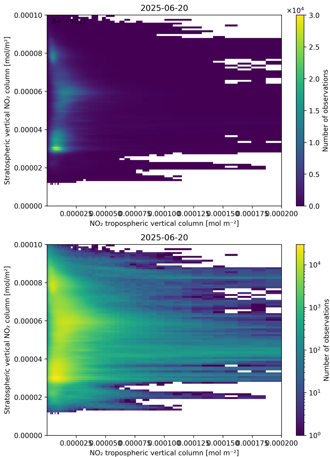
Figure 125: Scatter density plot of “NO 2 tropospheric vertical column” against “Stratospheric vertical NO 2 column” for 2025-06-19 to 2025-06-21.
