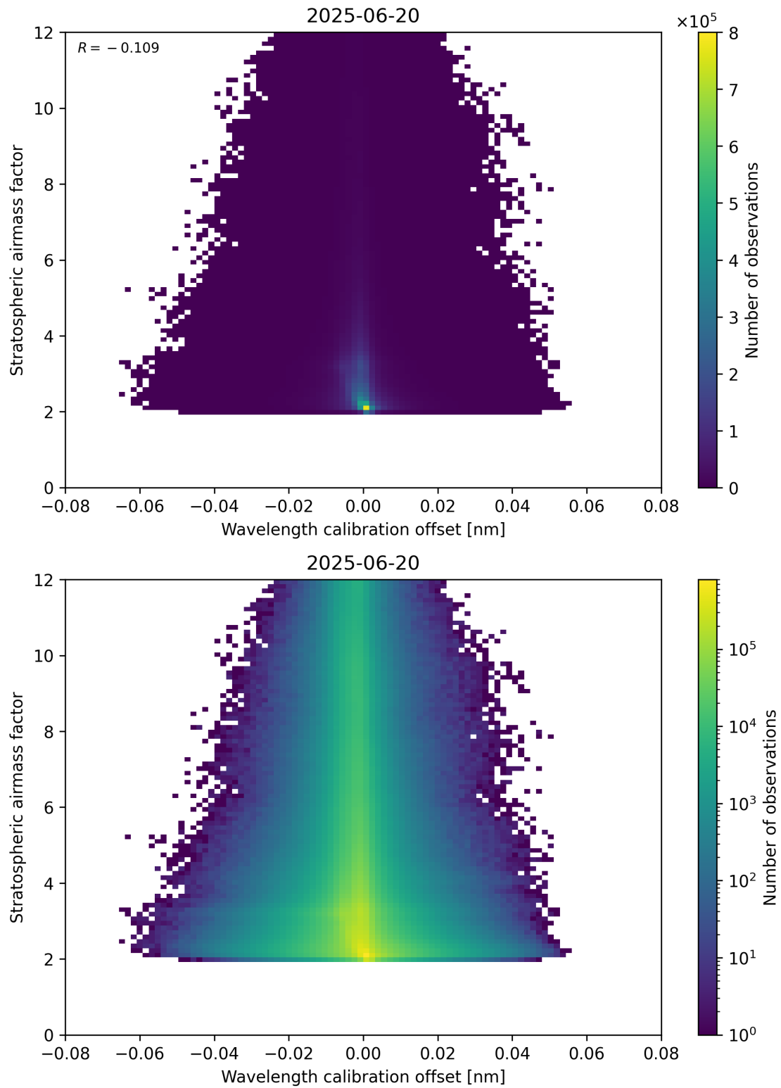
Figure 174: Scatter density plot of “Wavelength calibration offset” against “Stratospheric airmass factor” for 2025-06-19 to 2025-06-21.
