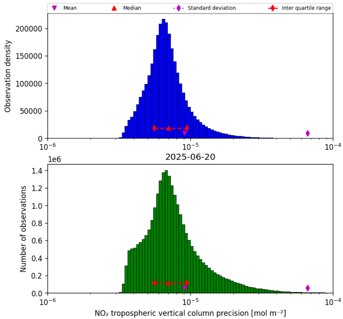
Figure 30: Histogram of “NO 2 tropospheric vertical column precision” for 2025-06-19 to 2025-06-21
