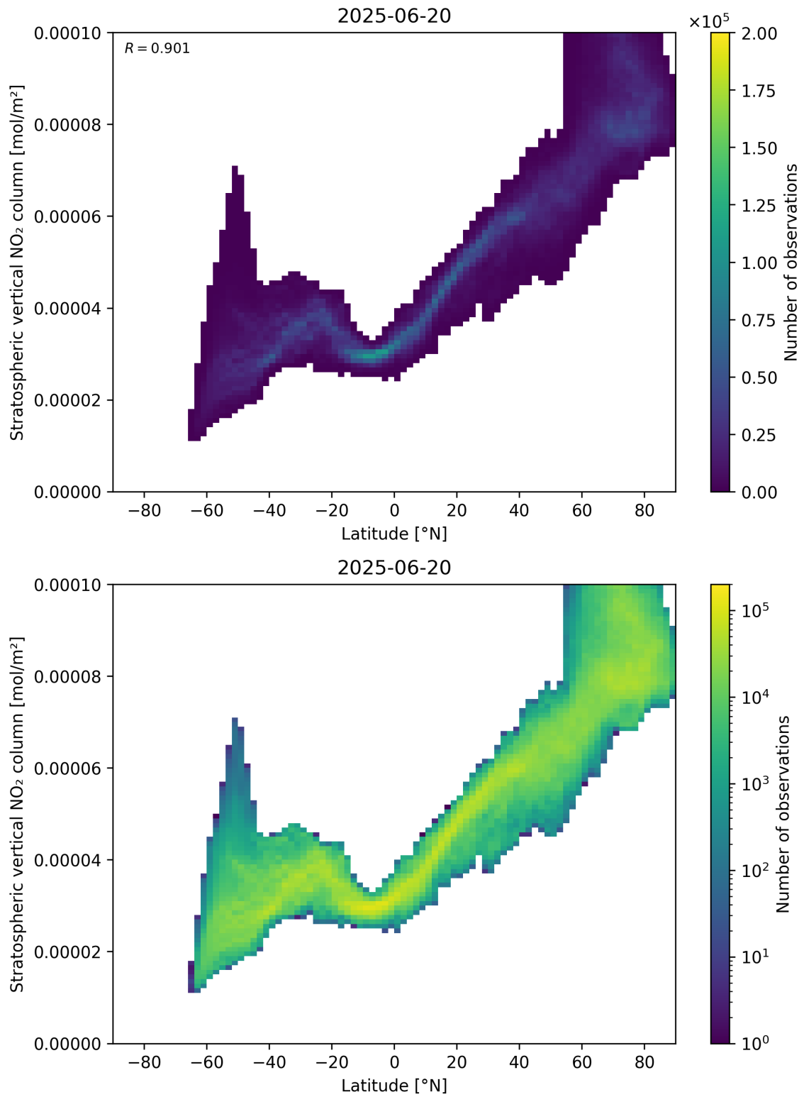
Figure 87: Scatter density plot of “Latitude” against “Stratospheric vertical NO 2 column” for 2025-06-19 to 2025-06-21.
