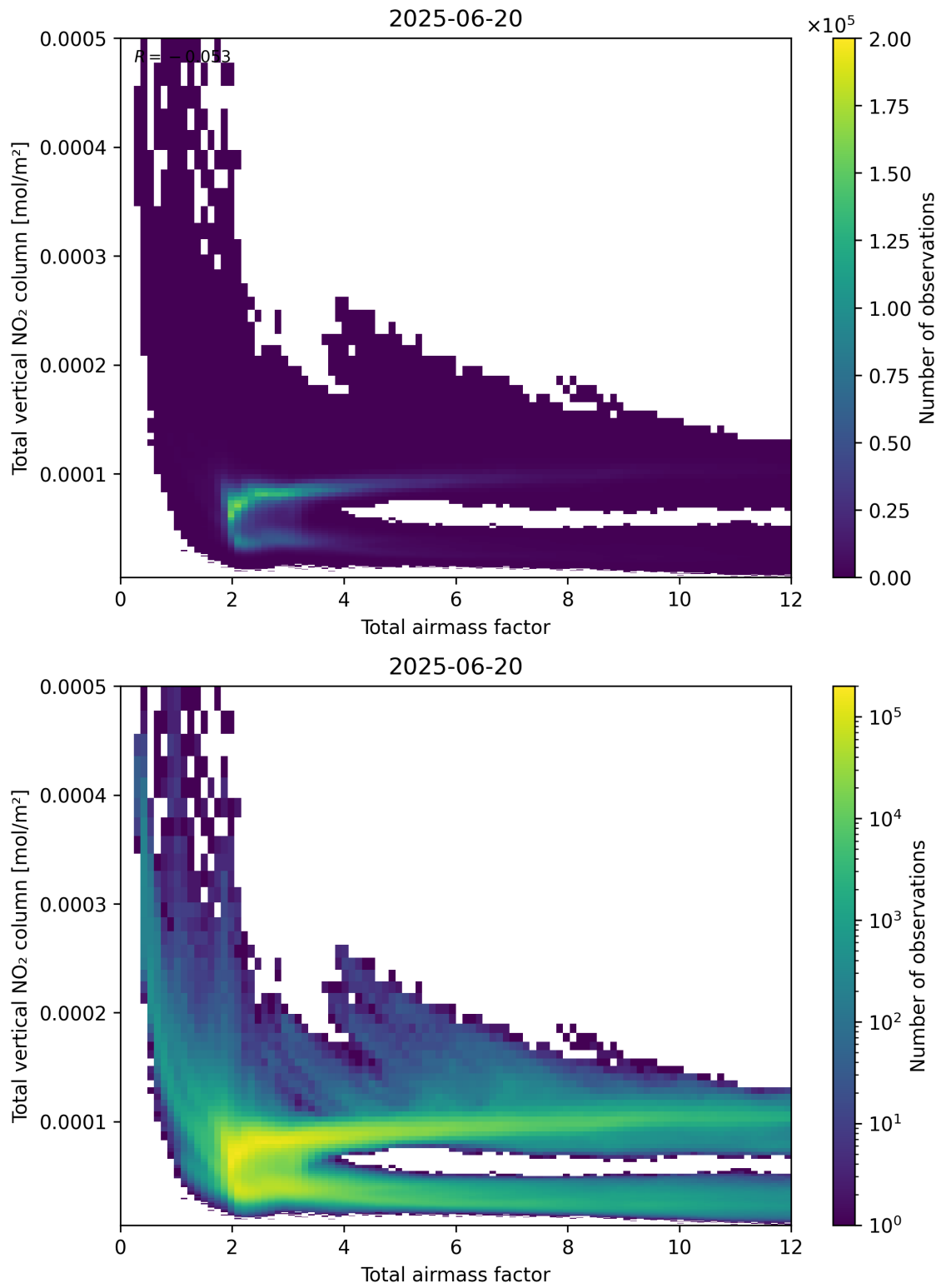
Figure 67: Scatter density plot of “Total airmass factor” against “Total vertical NO 2 column” for 2025-06-19 to 2025-06-21.
