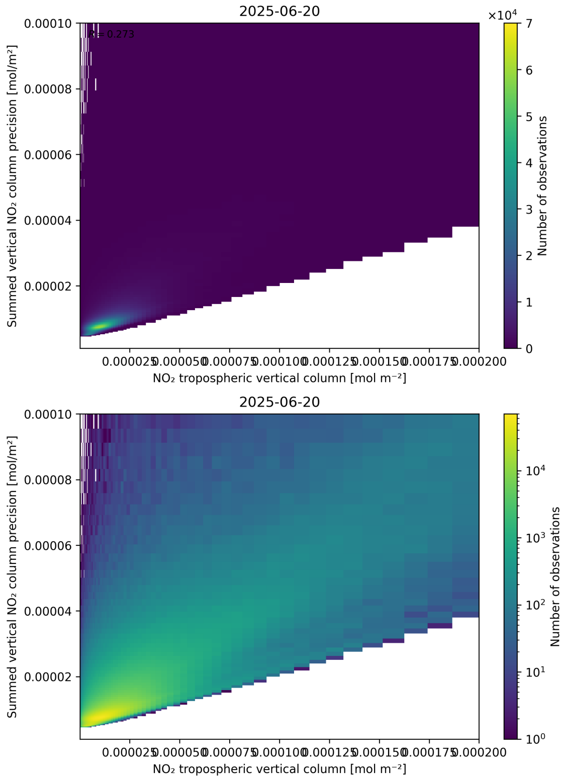
Figure 127: Scatter density plot of “NO 2 tropospheric vertical column” against “Summed vertical NO 2 column precision” for 2025-06-19 to 2025-06-21.
