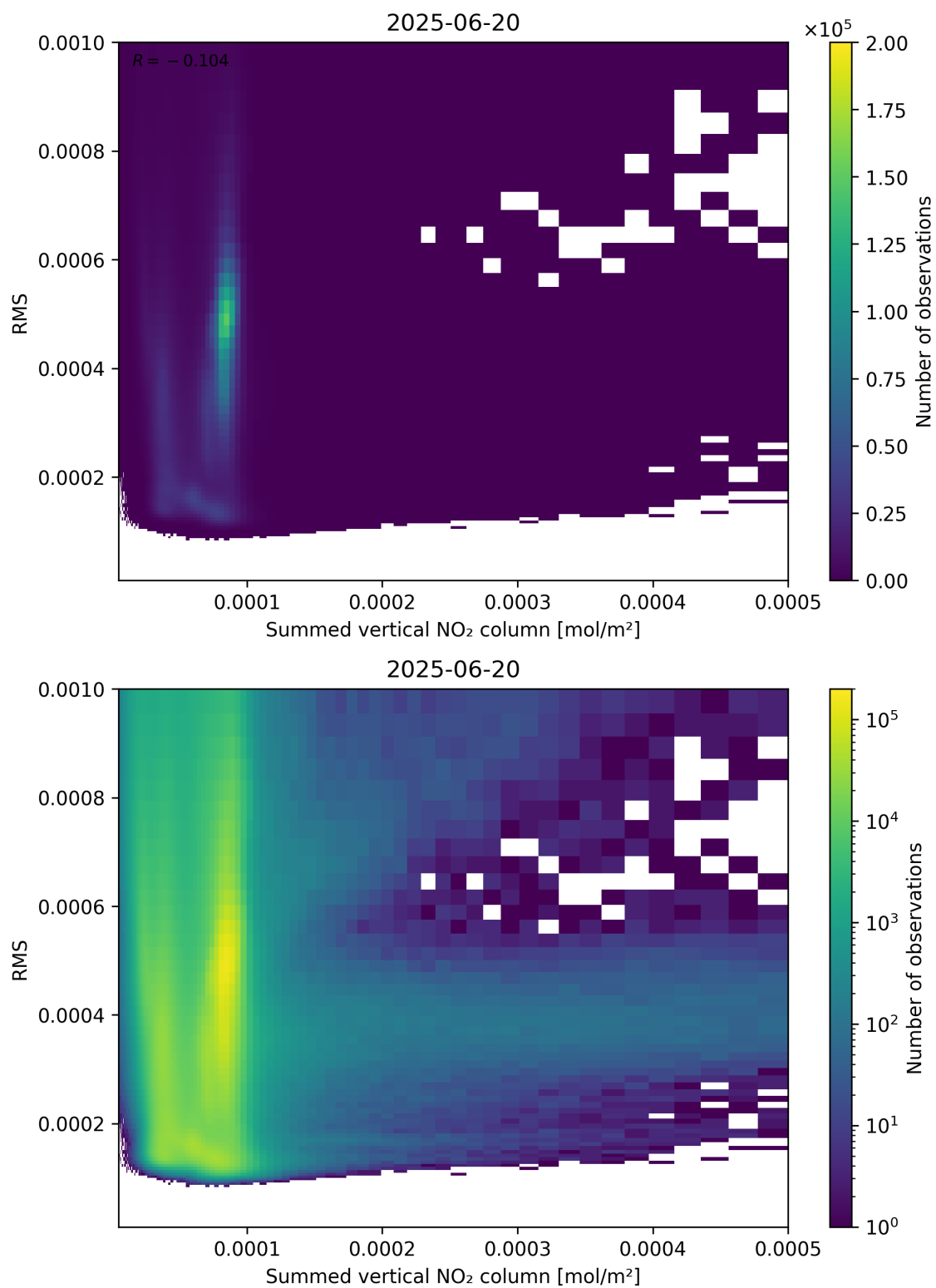
Figure 109: Scatter density plot of “Summed vertical NO 2 column” against “RMS” for 2025-06-19 to 2025-06-21.
