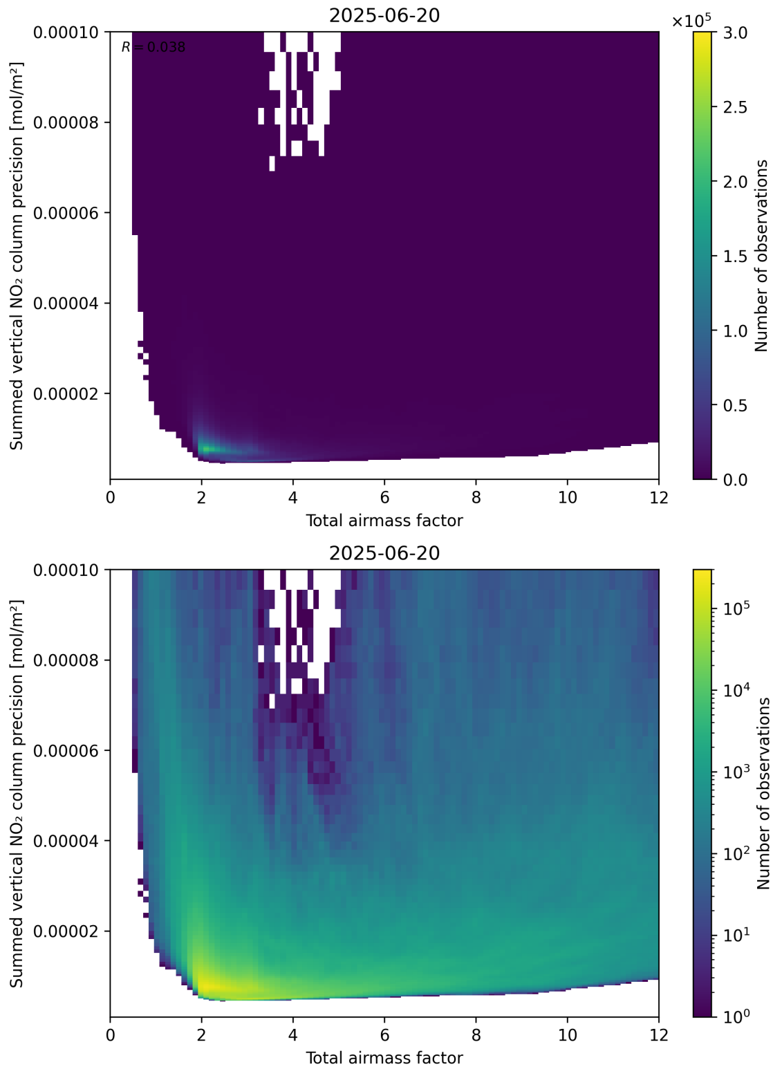
Figure 66: Scatter density plot of “Total airmass factor” against “Summed vertical NO 2 column precision” for 2025-06-19 to 2025-06-21.
