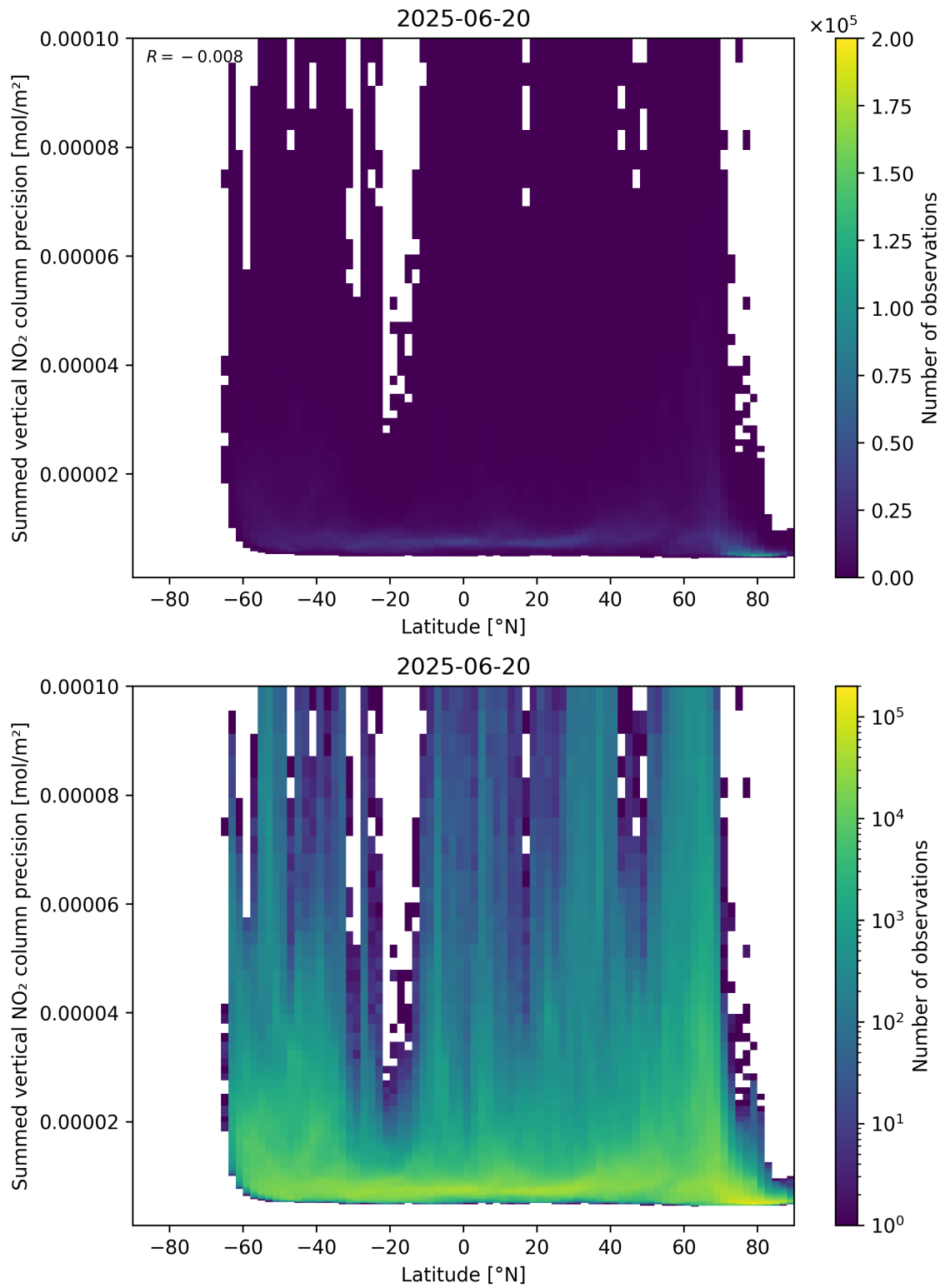
Figure 89: Scatter density plot of “Latitude” against “Summed vertical NO 2 column precision” for 2025-06-19 to 2025-06-21.
