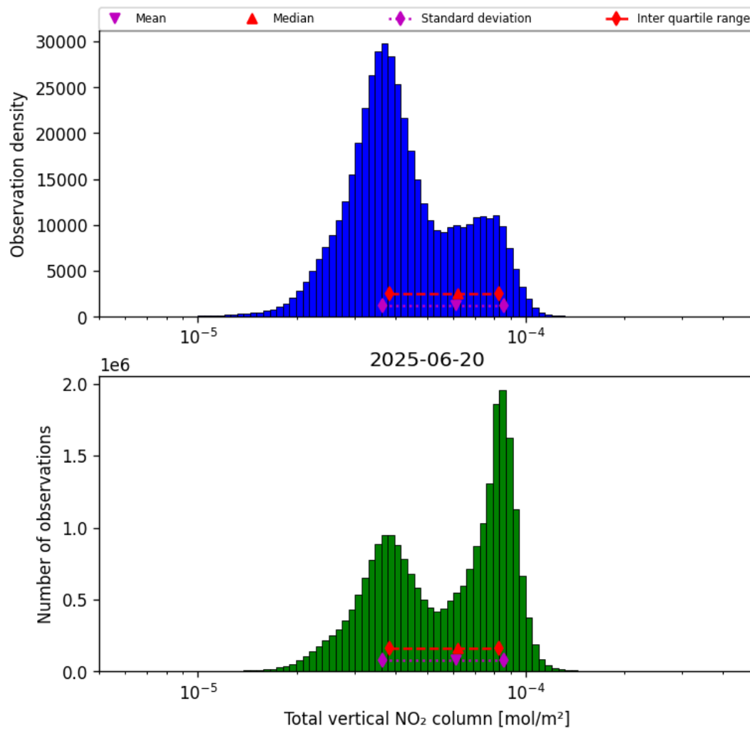
Figure 38: Histogram of “Total vertical NO 2 column” for 2025-06-19 to 2025-06-21
