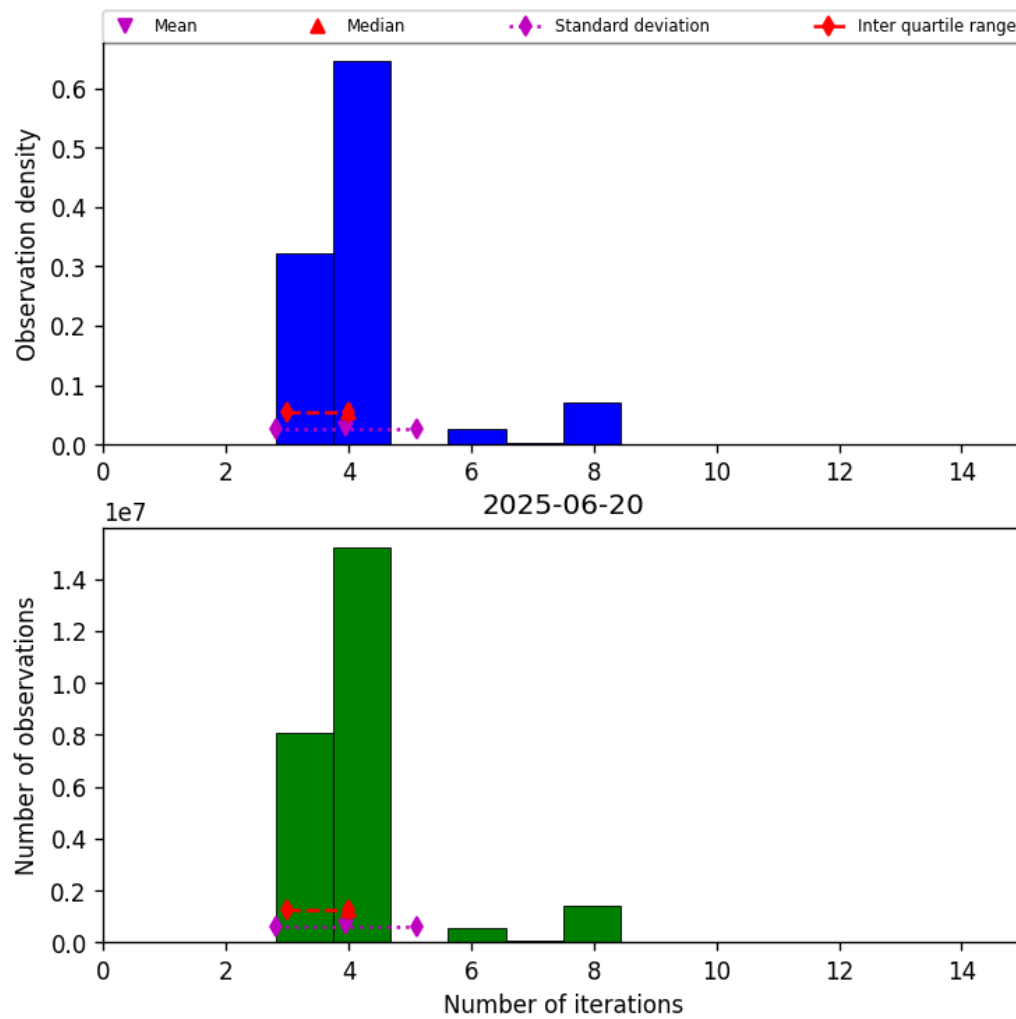
Figure 34: Histogram of “Number of iterations” for 2025-06-19 to 2025-06-21
