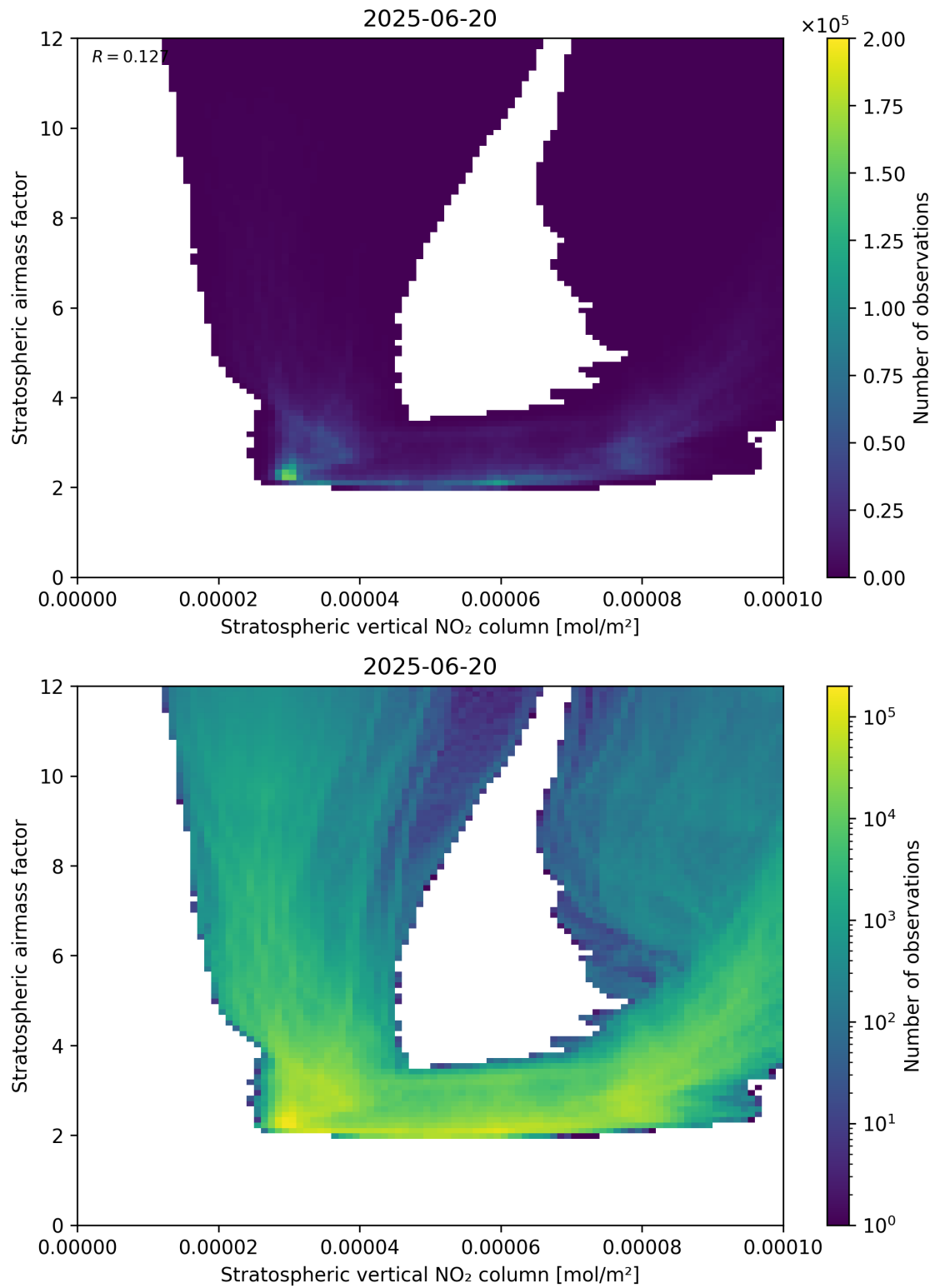
Figure 96: Scatter density plot of “Stratospheric vertical NO 2 column” against “Stratospheric airmass factor” for 2025-06-19 to 2025-06-21.
