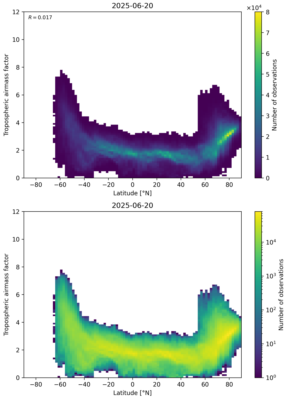
Figure 85: Scatter density plot of “Latitude” against “Tropospheric airmass factor” for 2025-06-19 to 2025-06-21.
