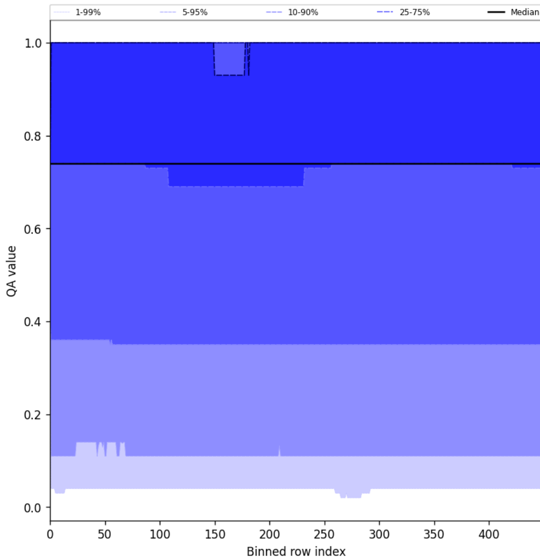
Figure 45: Along track statistics of “QA value” for 2025-06-19 to 2025-06-21
