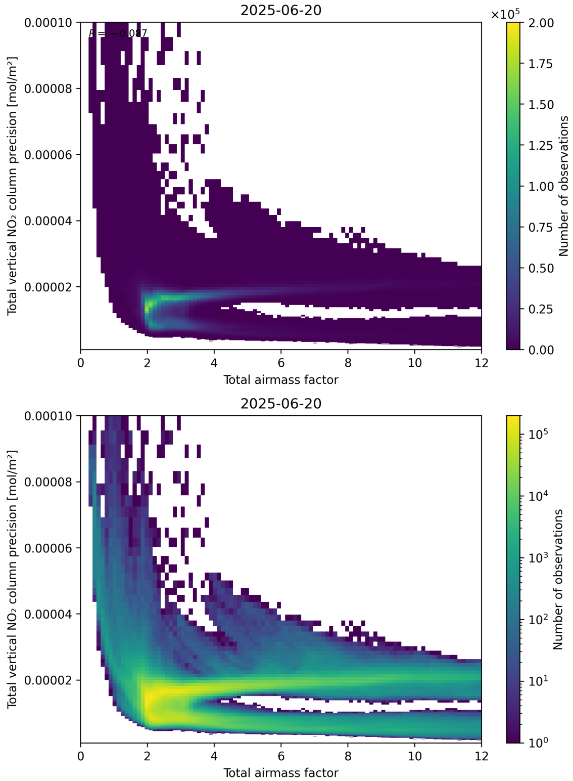
Figure 68: Scatter density plot of “Total airmass factor” against “Total vertical NO 2 column precision” for 2025-06-19 to 2025-06-21.
