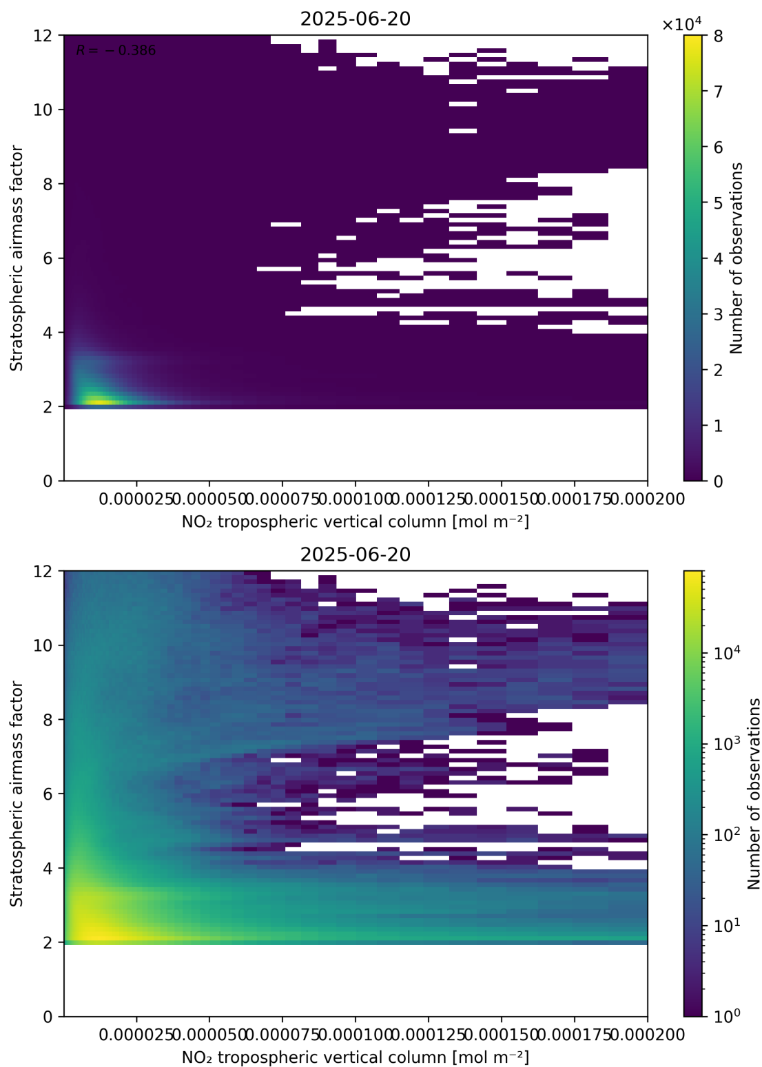
Figure 121: Scatter density plot of “NO 2 tropospheric vertical column” against “Stratospheric air mass factor” for 2025-06-19 to 2025-06-21.
