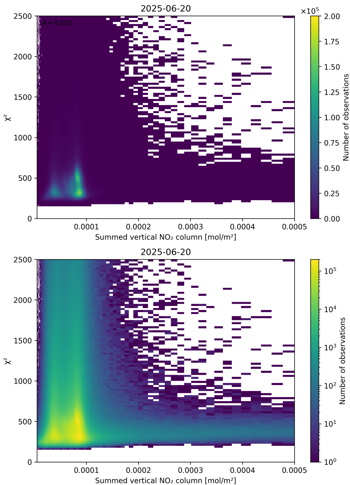
Figure 104: Scatter density plot of “Summed vertical NO 2 column” against “ \chi^2 ” for 2025-06-19 to 2025-06-21.
