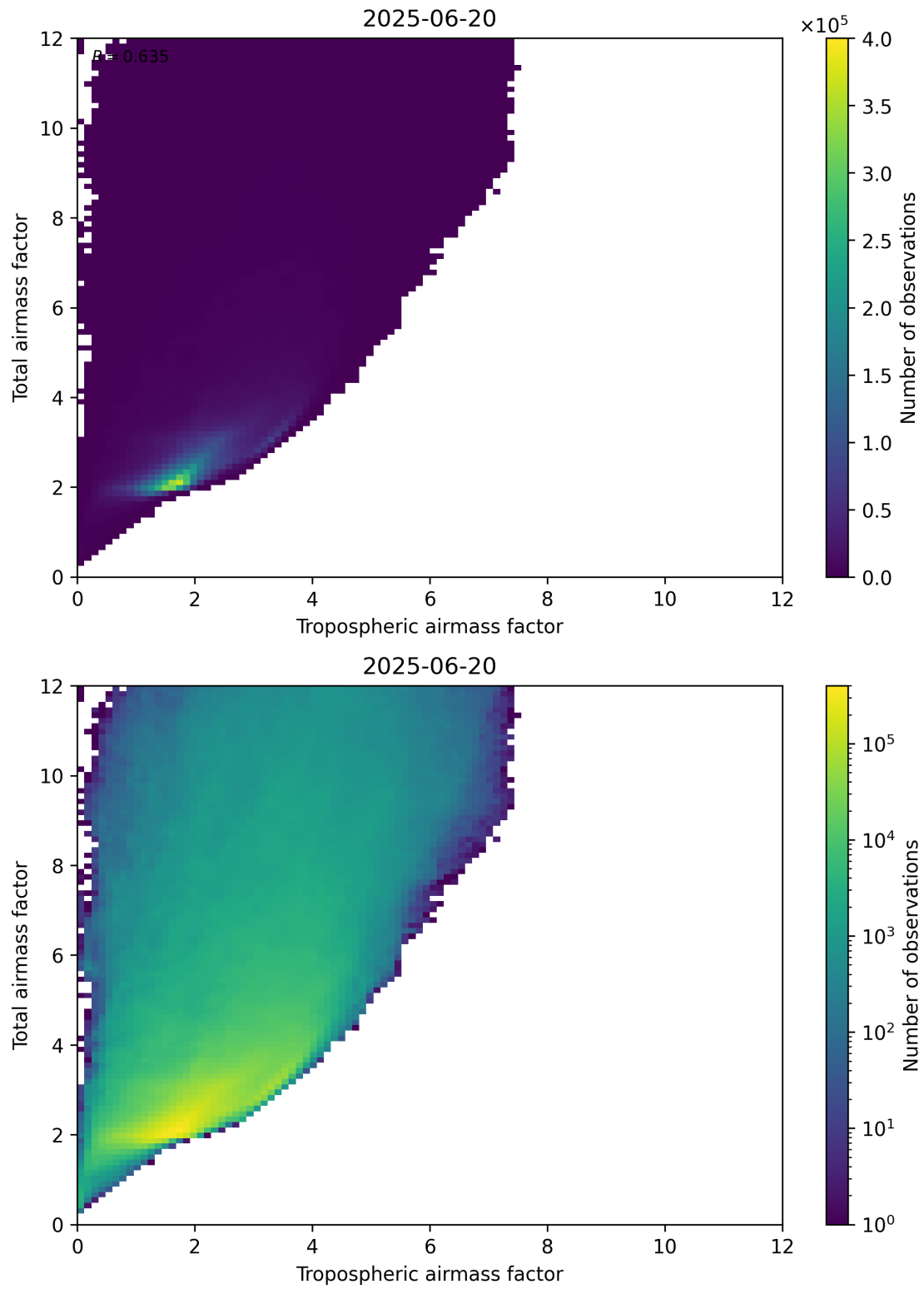
Figure 72: Scatter density plot of “Tropospheric airmass factor” against “Total airmass factor” for 2025-06-19 to 2025-06-21.
