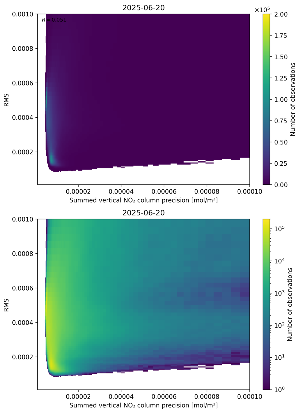
Figure 108: Scatter density plot of “Summed vertical NO 2 column precision” against “RMS” for 2025-06-19 to 2025-06-21.
