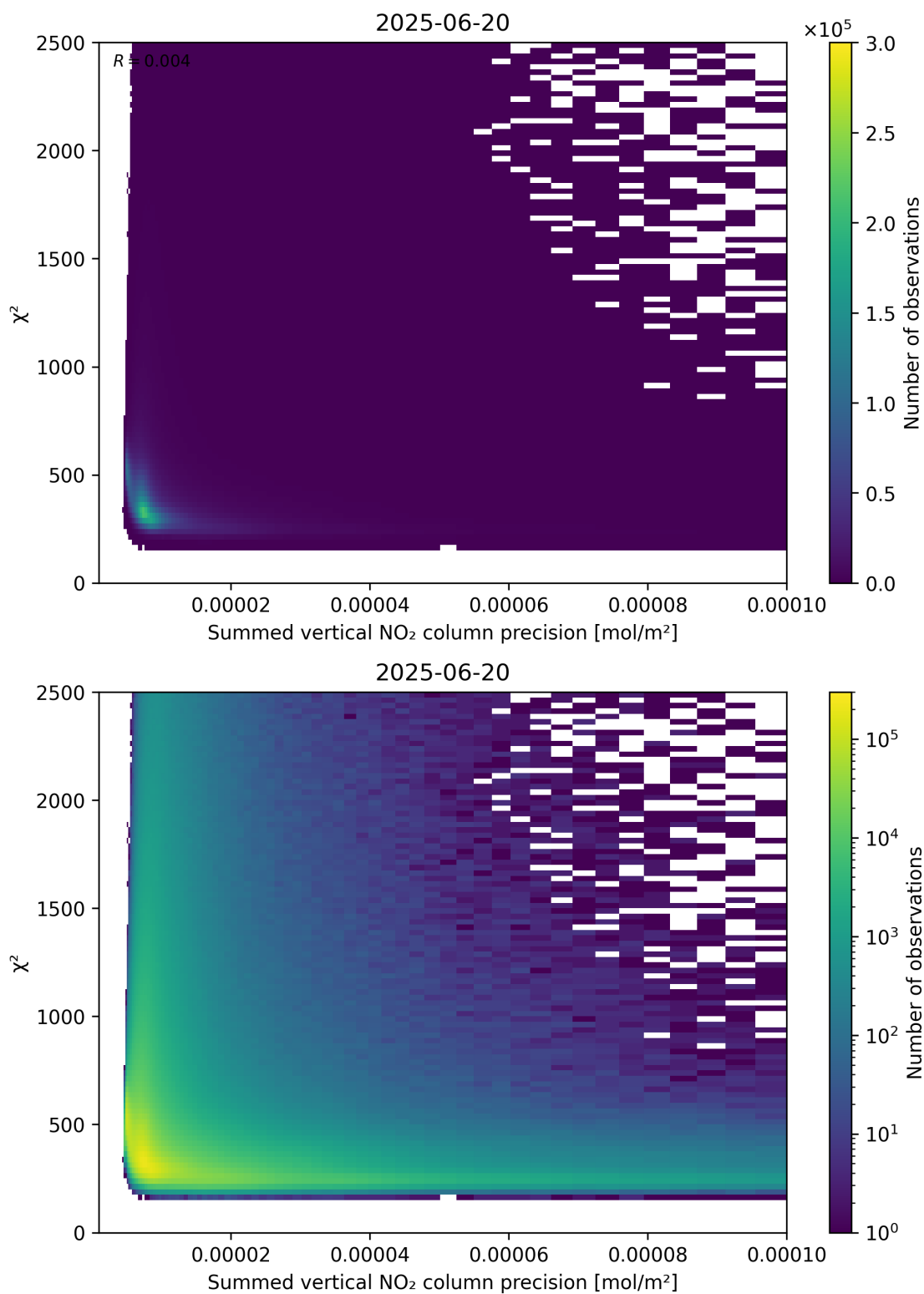
Figure 107: Scatter density plot of “Summed vertical NO 2 column precision” against “ \chi^2 ” for 2025-06-19 to 2025-06-21.
