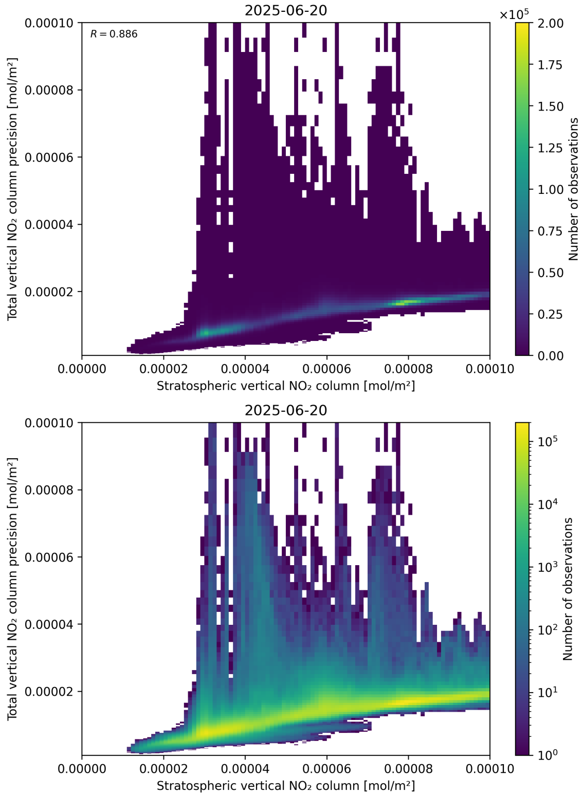
Figure 101: Scatter density plot of “Stratospheric vertical NO 2 column” against “Total vertical NO 2 column precision” for 2025-06-19 to 2025-06-21.
