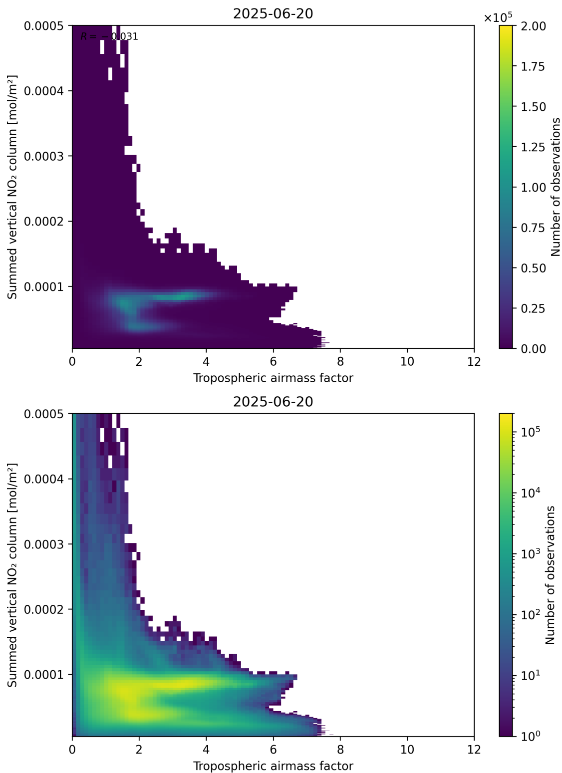
Figure 75: Scatter density plot of “Tropospheric airmass factor” against “Summed vertical NO 2 column” for 2025-06-19 to 2025-06-21.
