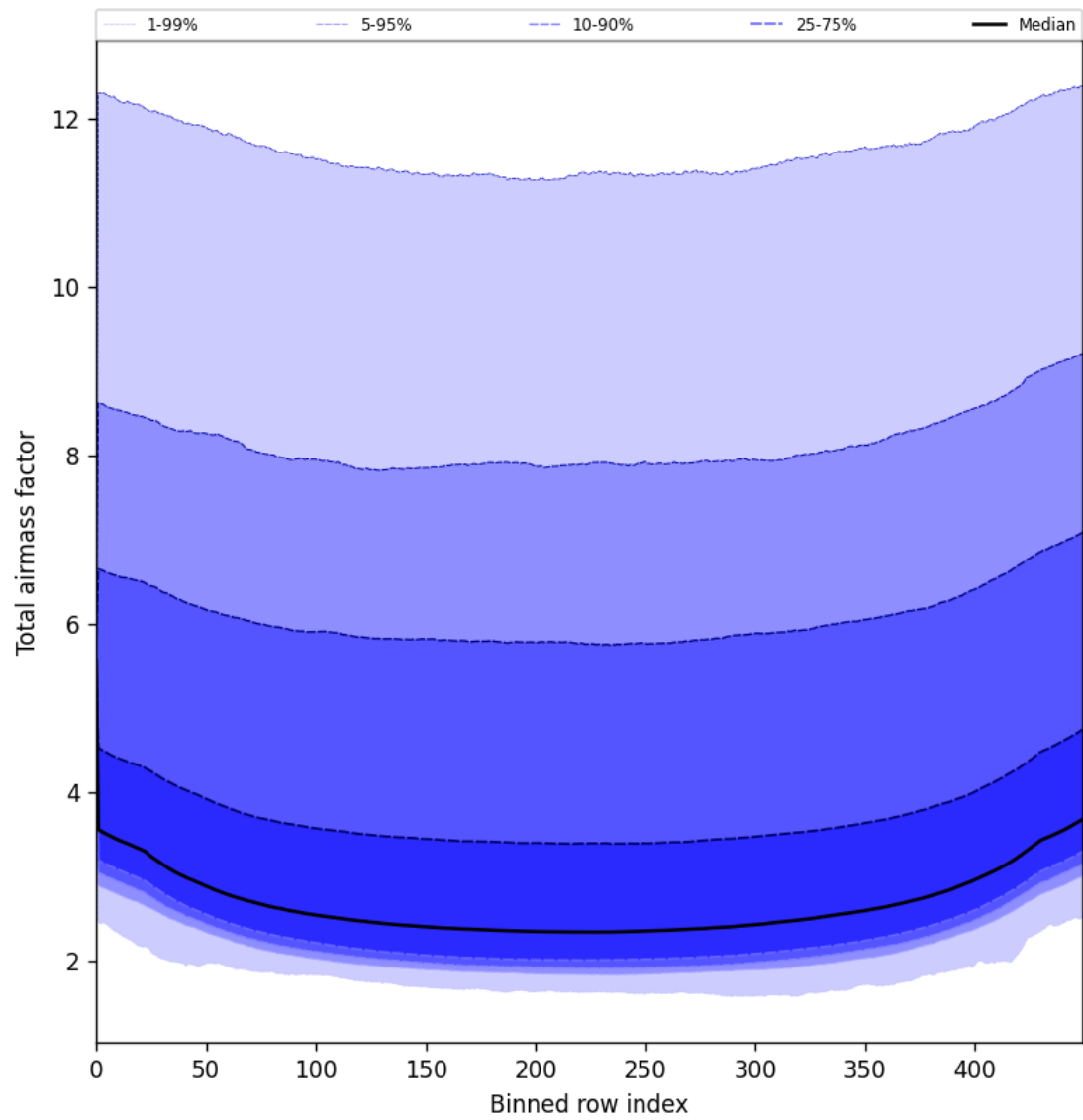
Figure 49: Along track statistics of “Total airmass factor” for 2025-06-19 to 2025-06-21
