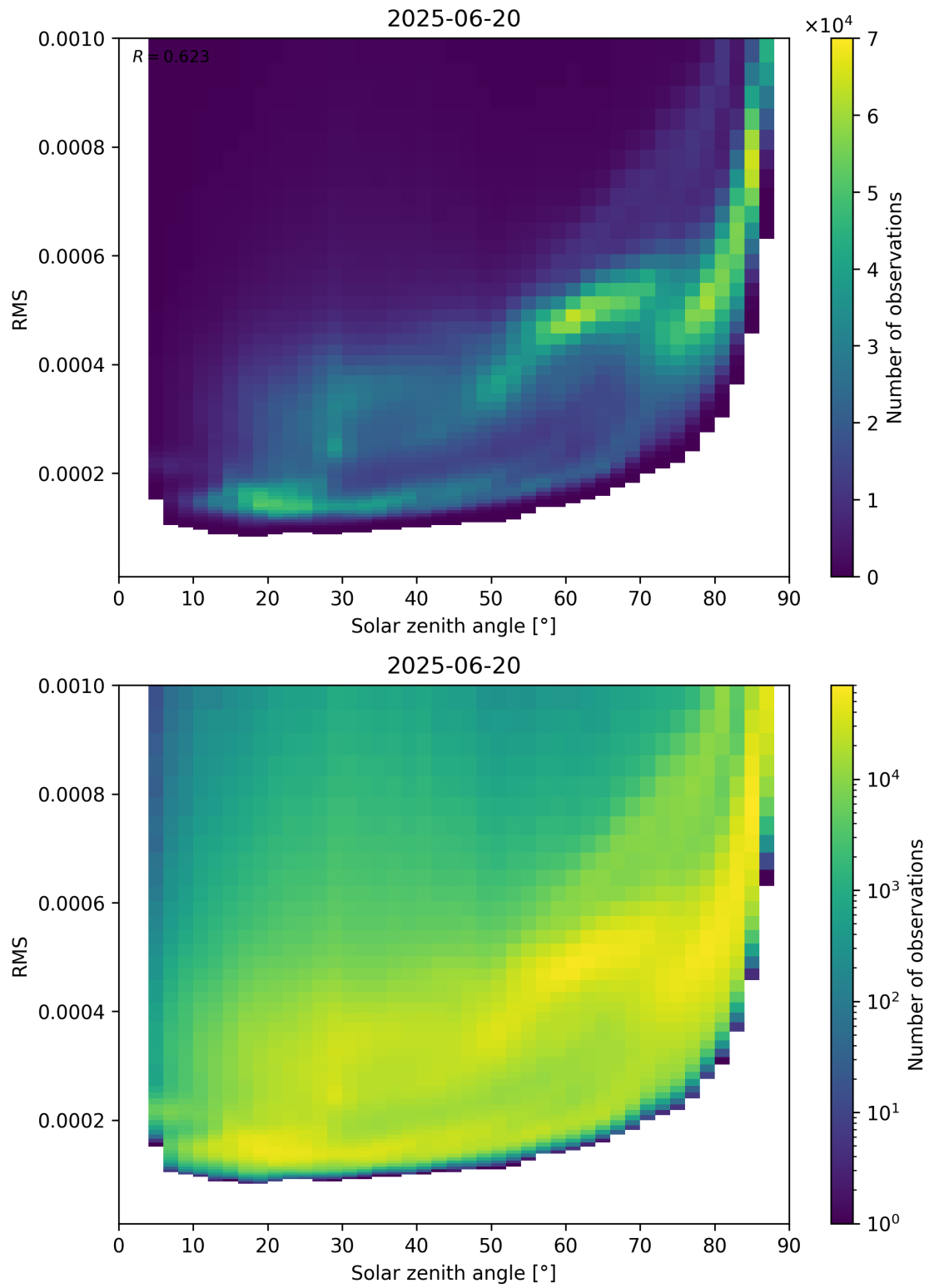
Figure 157: Scatter density plot of “Solar zenith angle” against “RMS” for 2025-06-19 to 2025-06-21.
