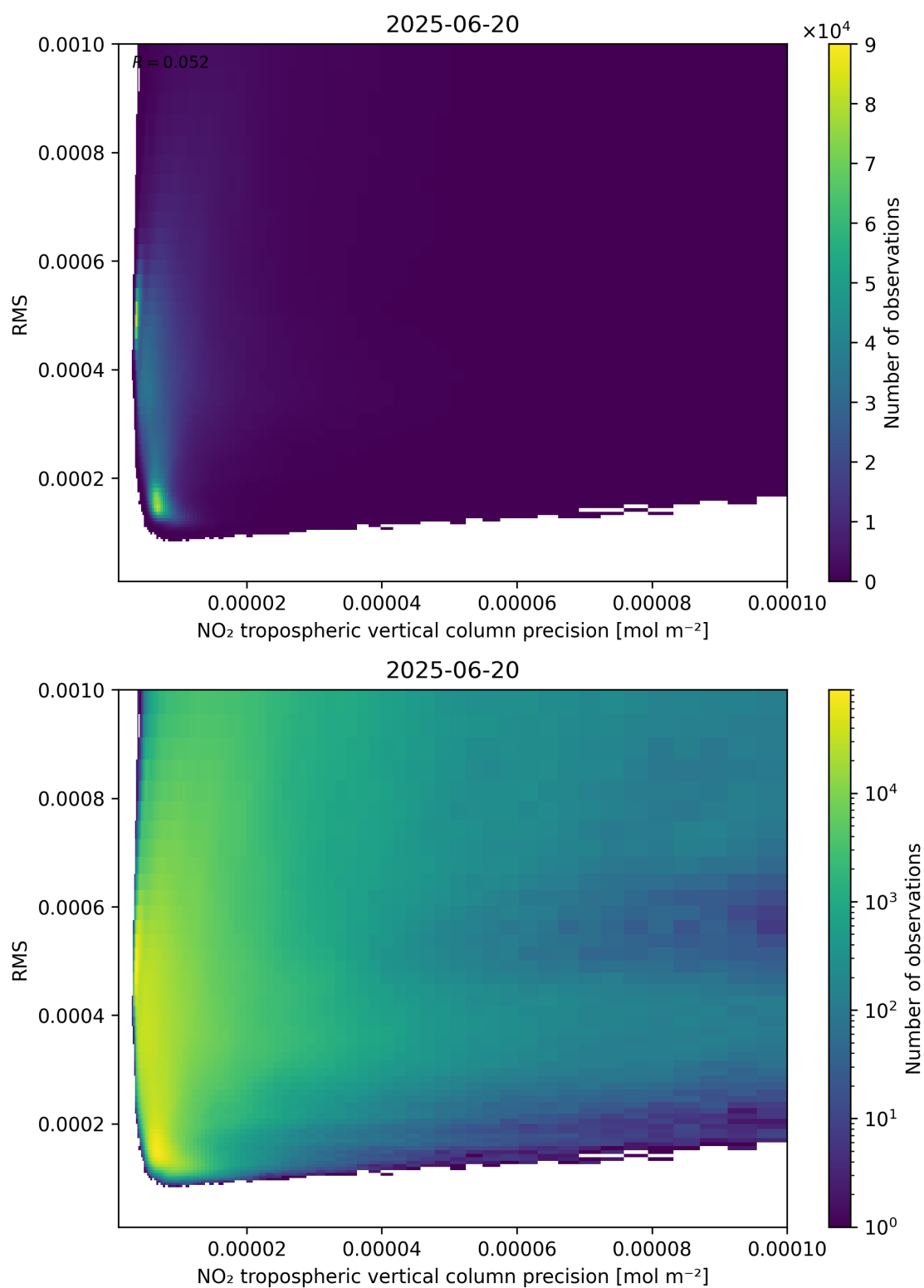
Figure 140: Scatter density plot of “NO 2 tropospheric vertical column precision” against “RMS” for 2025-06-19 to 2025-06-21.
