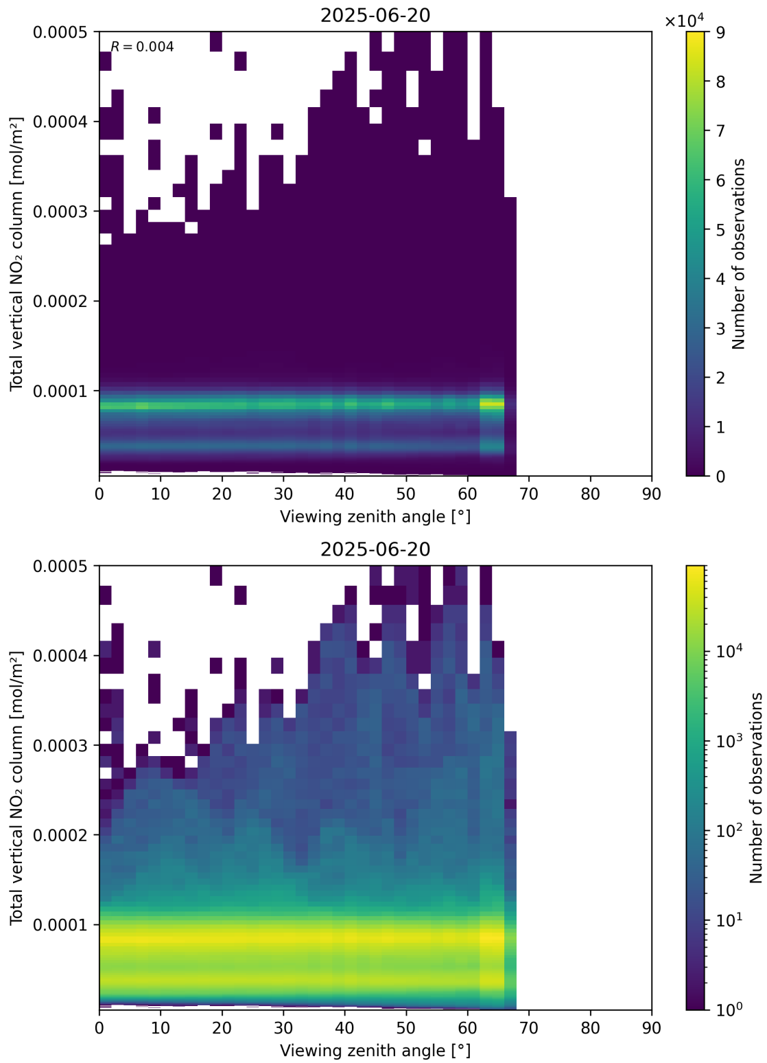
Figure 167: Scatter density plot of “Viewing zenith angle” against “Total vertical NO 2 column” for 2025-06-19 to 2025-06-21.
