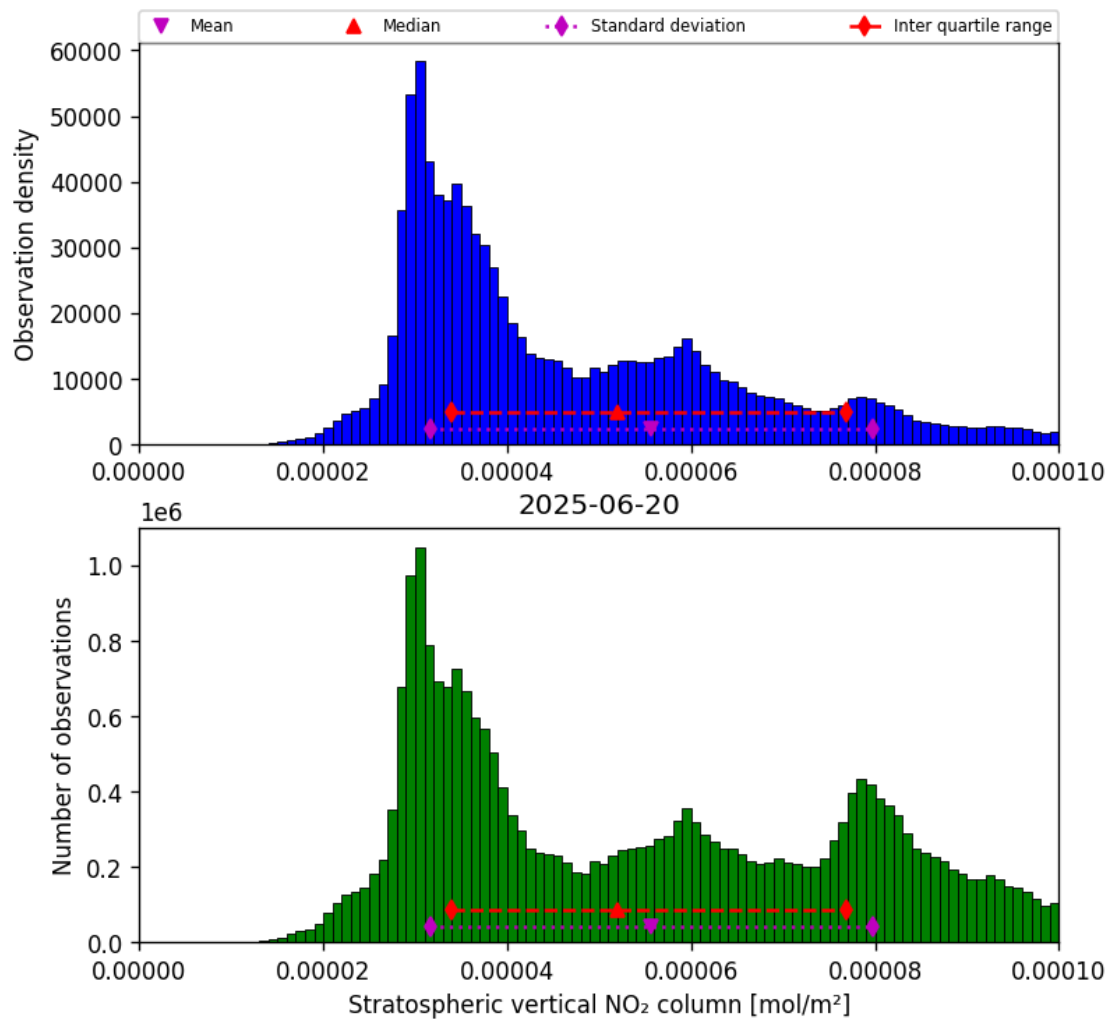
Figure 36: Histogram of “Stratospheric vertical NO 2 column” for 2025-06-19 to 2025-06-21
