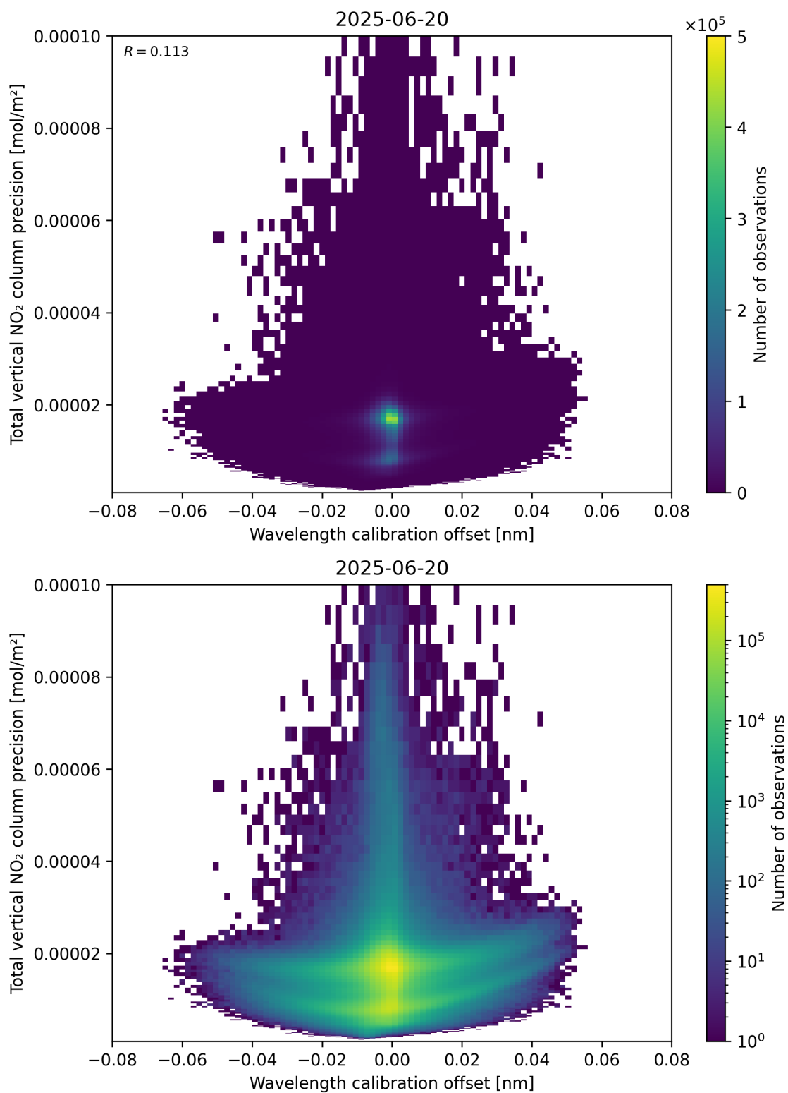
Figure 180: Scatter density plot of “Wavelength calibration offset” against “Total vertical NO 2 column precision” for 2025-06-19 to 2025-06-21.
