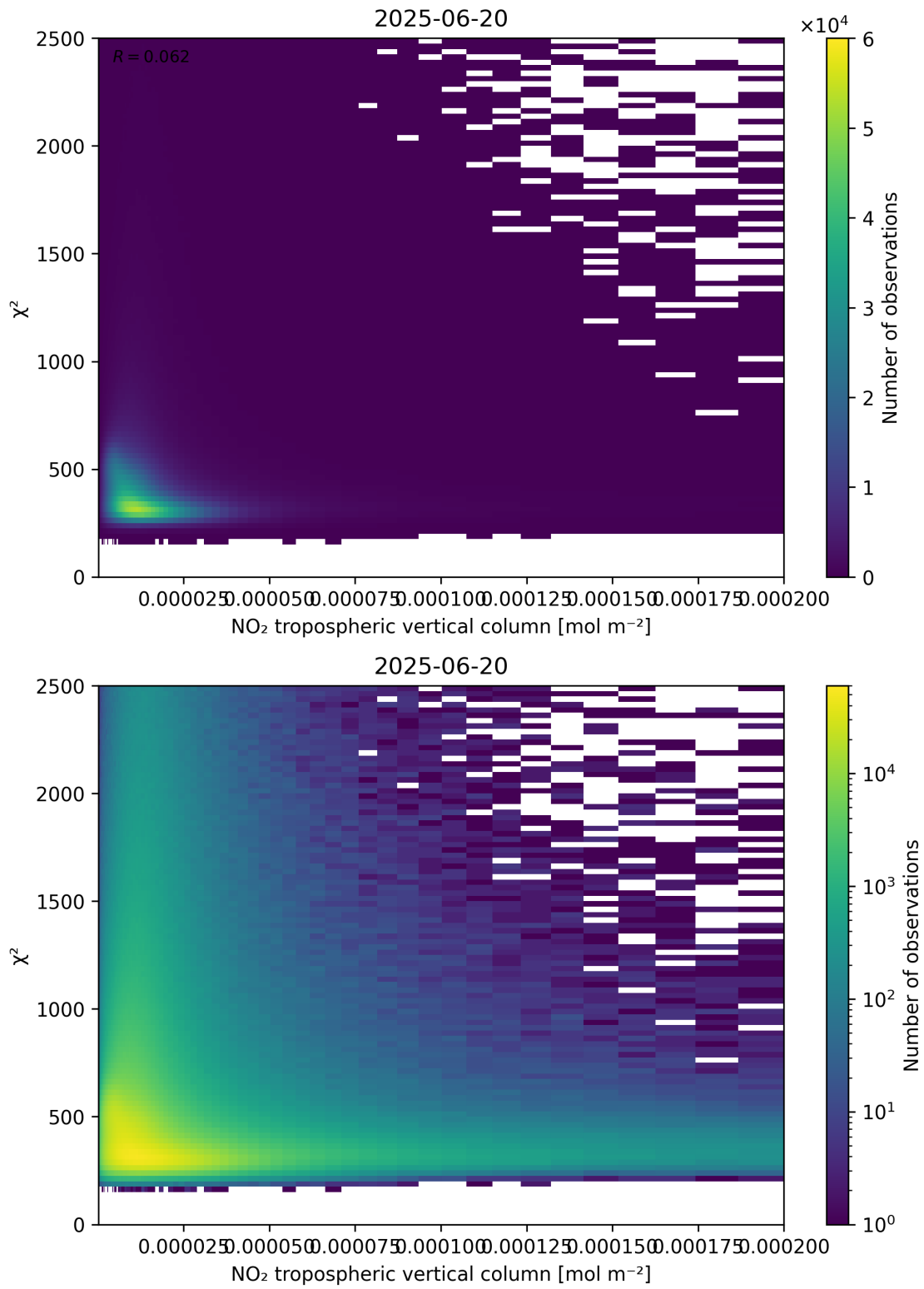
Figure 124: Scatter density plot of “NO 2 tropospheric vertical column” against “ \chi^2 ” for 2025-06-19 to 2025-06-21.
