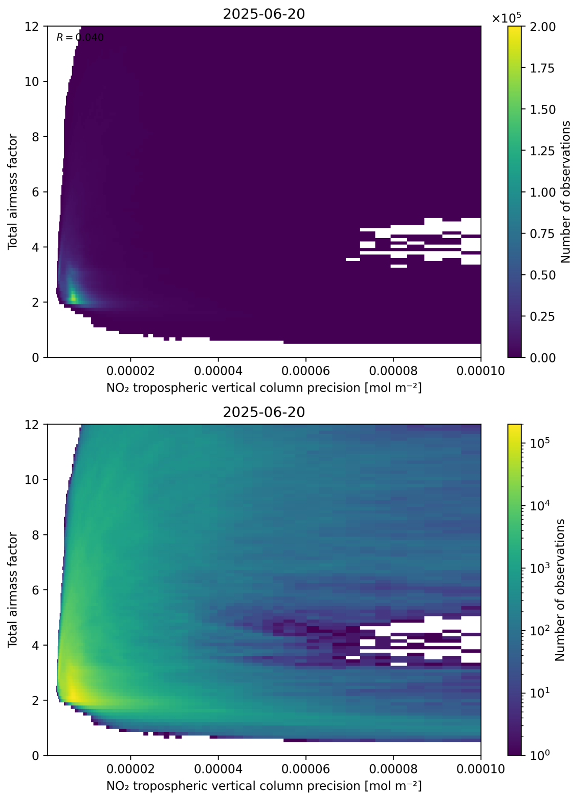
Figure 132: Scatter density plot of “NO 2 tropospheric vertical column precision” against “Total air mass factor” for 2025-06-19 to 2025-06-21.
