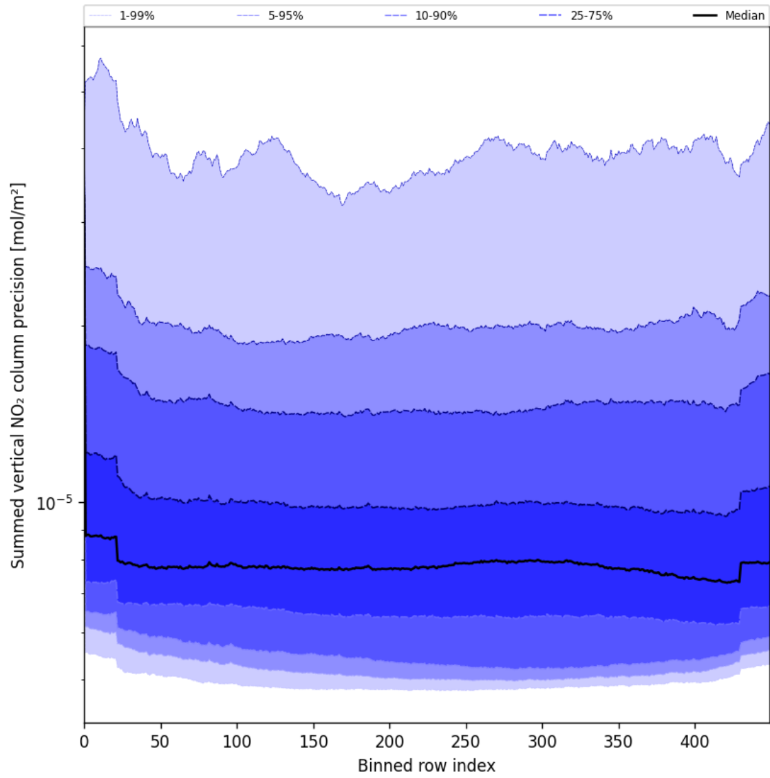
Figure 58: Along track statistics of “Summed vertical NO 2 column precision” for 2025-06-19 to 2025-06-21
