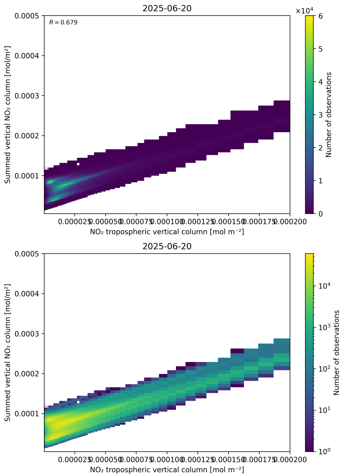
Figure 126: Scatter density plot of “NO 2 tropospheric vertical column” against “Summed vertical NO 2 column” for 2025-06-19 to 2025-06-21.
