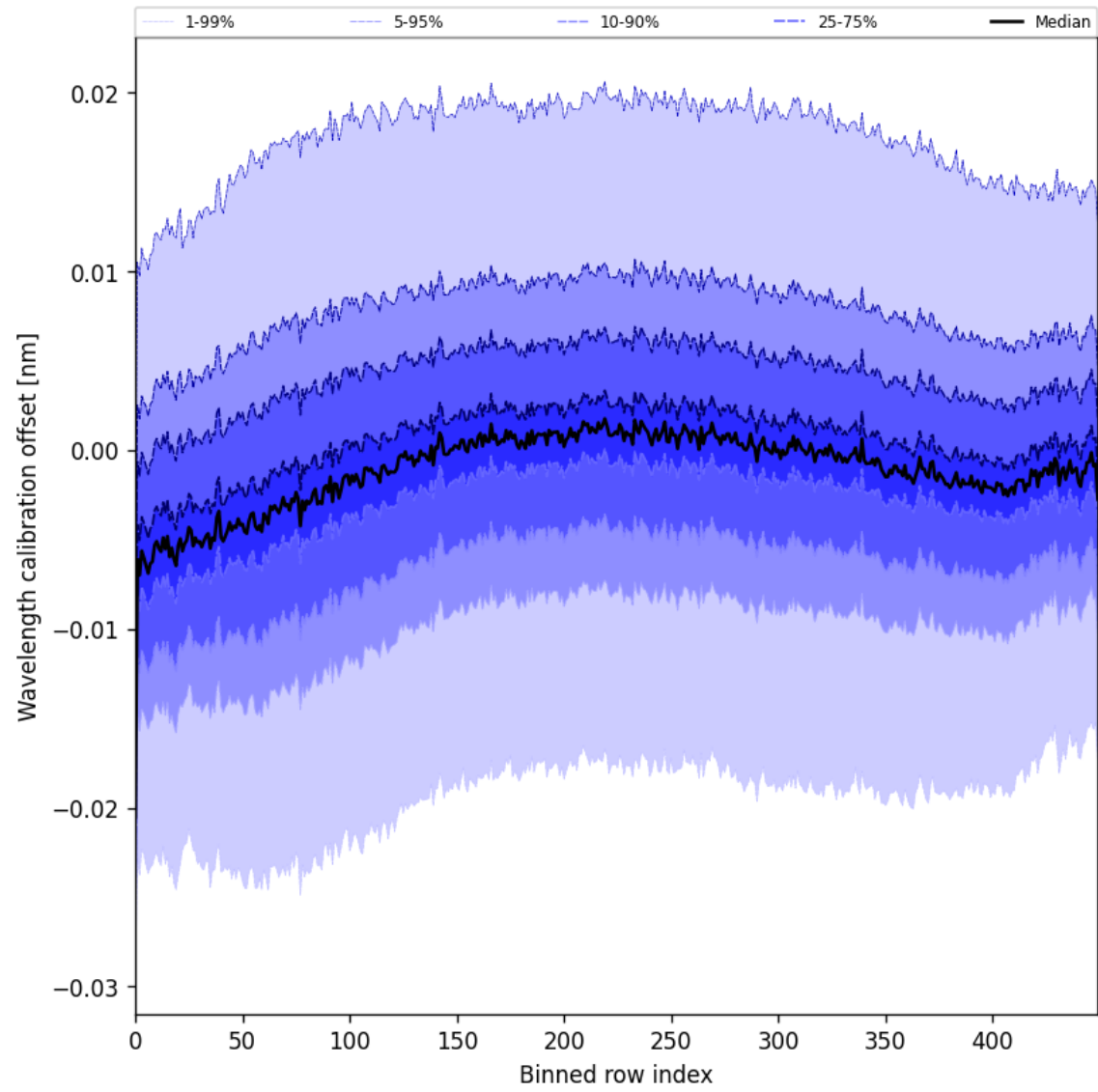
Figure 52: Along track statistics of “Wavelength calibration offset” for 2025-06-19 to 2025-06-21
