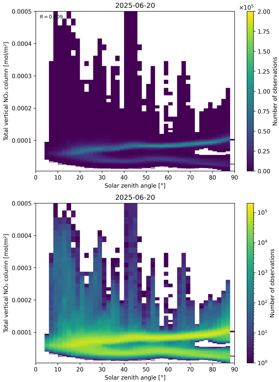
Figure 153: Scatter density plot of “Solar zenith angle” against “Total vertical NO 2 column” for 2025-06-19 to 2025-06-21.
