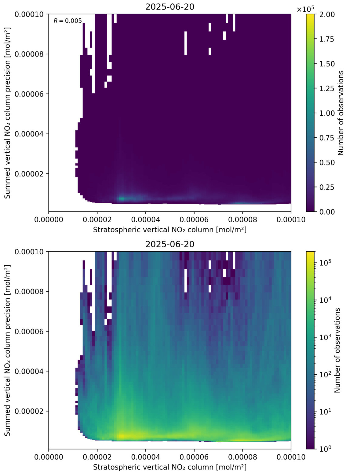
Figure 99: Scatter density plot of “Stratospheric vertical NO 2 column” against “Summed vertical NO 2 column precision” for 2025-06-19 to 2025-06-21.
