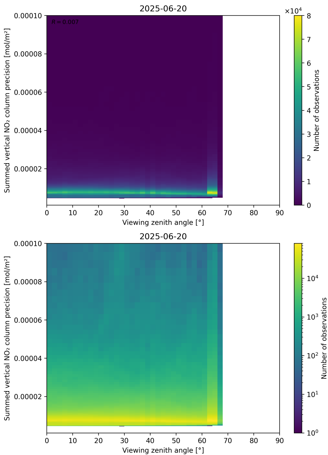
Figure 166: Scatter density plot of “Viewing zenith angle” against “Summed vertical NO 2 column precision” for 2025-06-19 to 2025-06-21.
