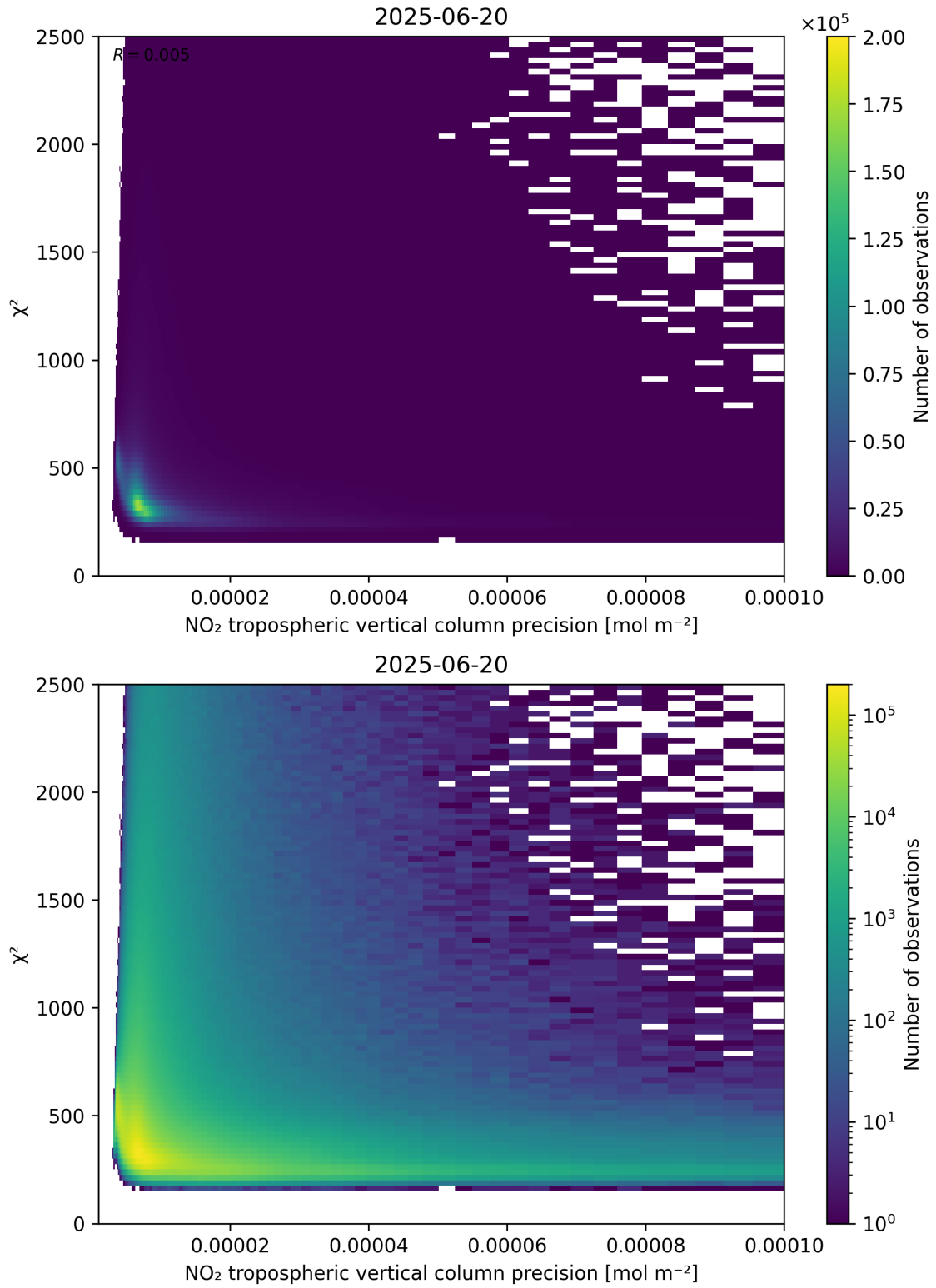
Figure 134: Scatter density plot of “NO 2 tropospheric vertical column precision” against “ \chi^2 ” for 2025-06-19 to 2025-06-21.
