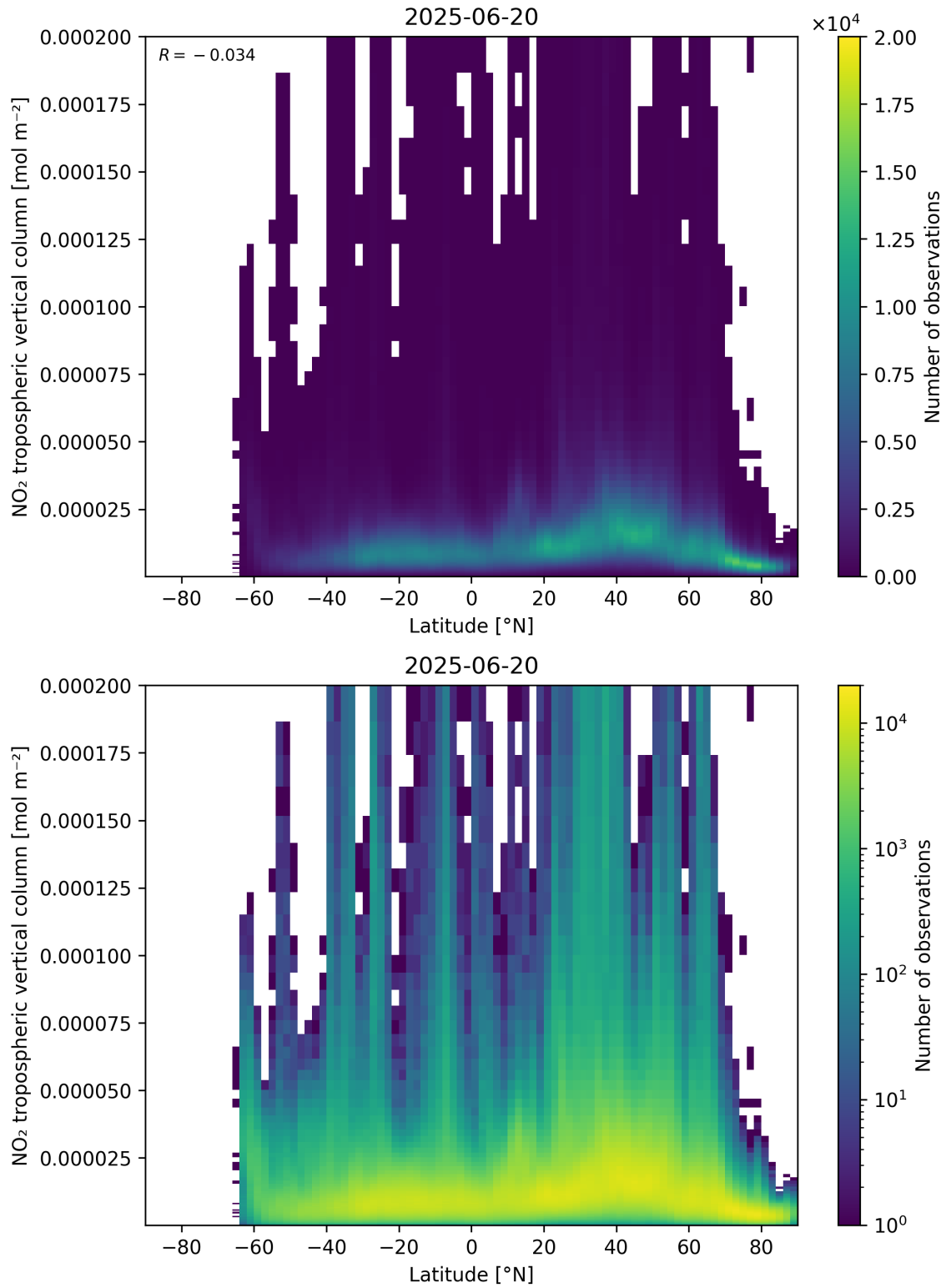
Figure 92: Scatter density plot of “Latitude” against “NO 2 tropospheric vertical column” for 2025-06-19 to 2025-06-21.
