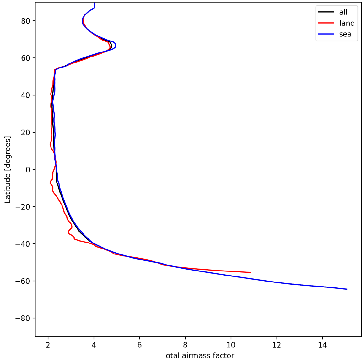
Figure 15: Zonal average of “Total airmass factor” for 2025-06-19 to 2025-06-21.
