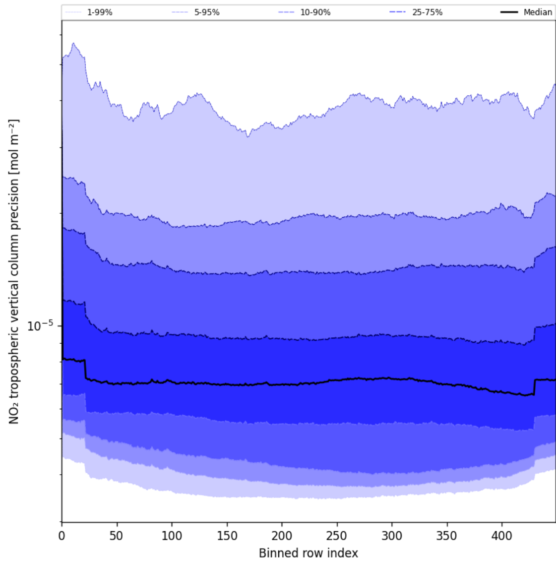
Figure 47: Along track statistics of “NO 2 tropospheric vertical column precision” for 2025-06-19 to 2025-06-21
