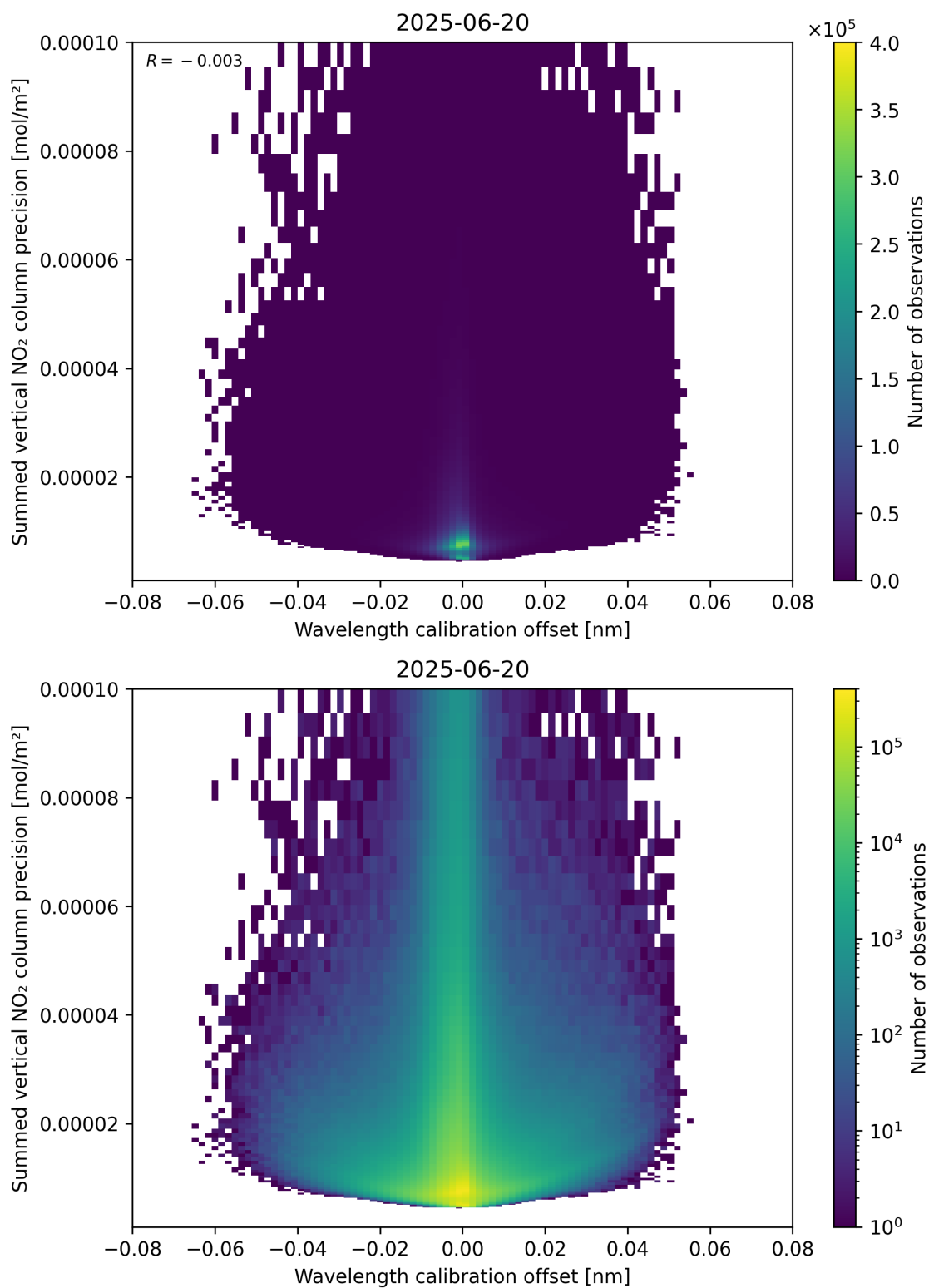
Figure 178: Scatter density plot of “Wavelength calibration offset” against “Summed vertical NO 2 column precision” for 2025-06-19 to 2025-06-21.
