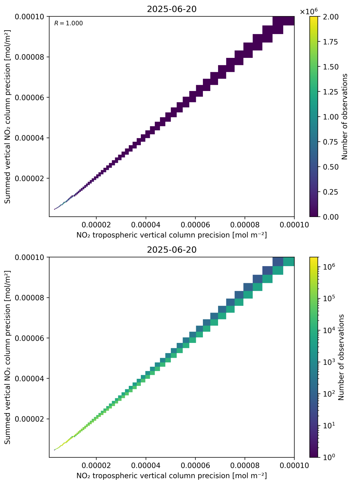
Figure 137: Scatter density plot of “NO 2 tropospheric vertical column precision” against “Summed vertical NO 2 column precision” for 2025-06-19 to 2025-06-21.
