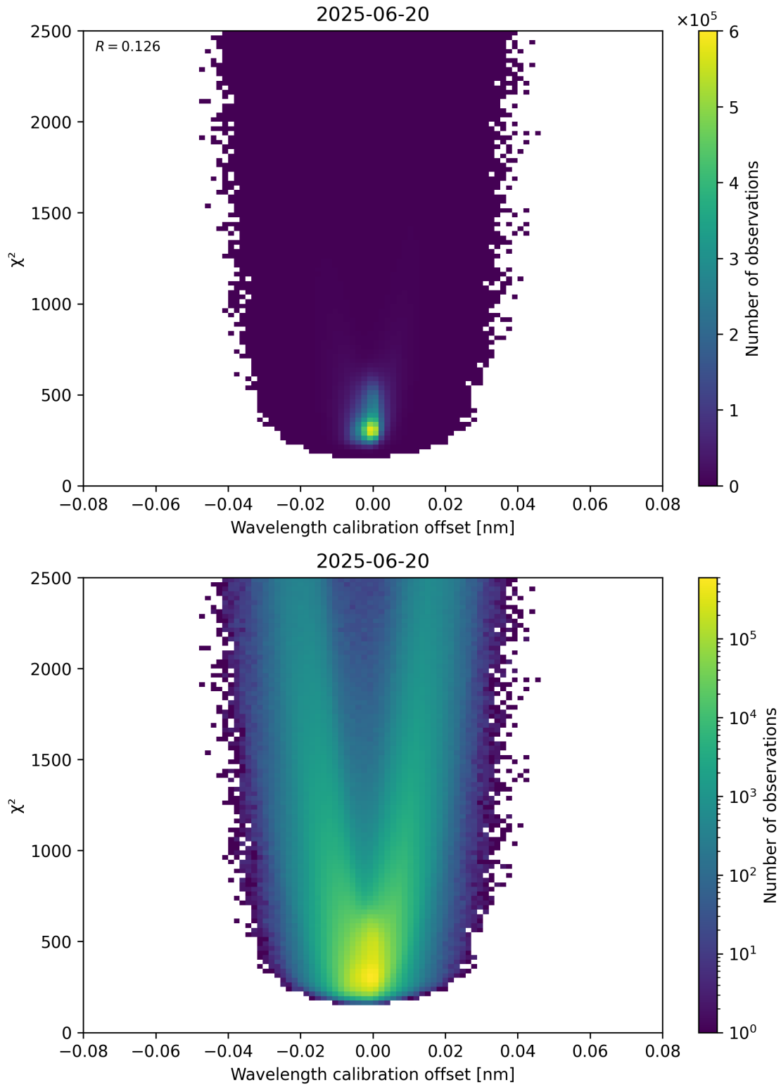
Figure 175: Scatter density plot of “Wavelength calibration offset” against “ \chi^2 ” for 2025-06-19 to 2025-06-21.
