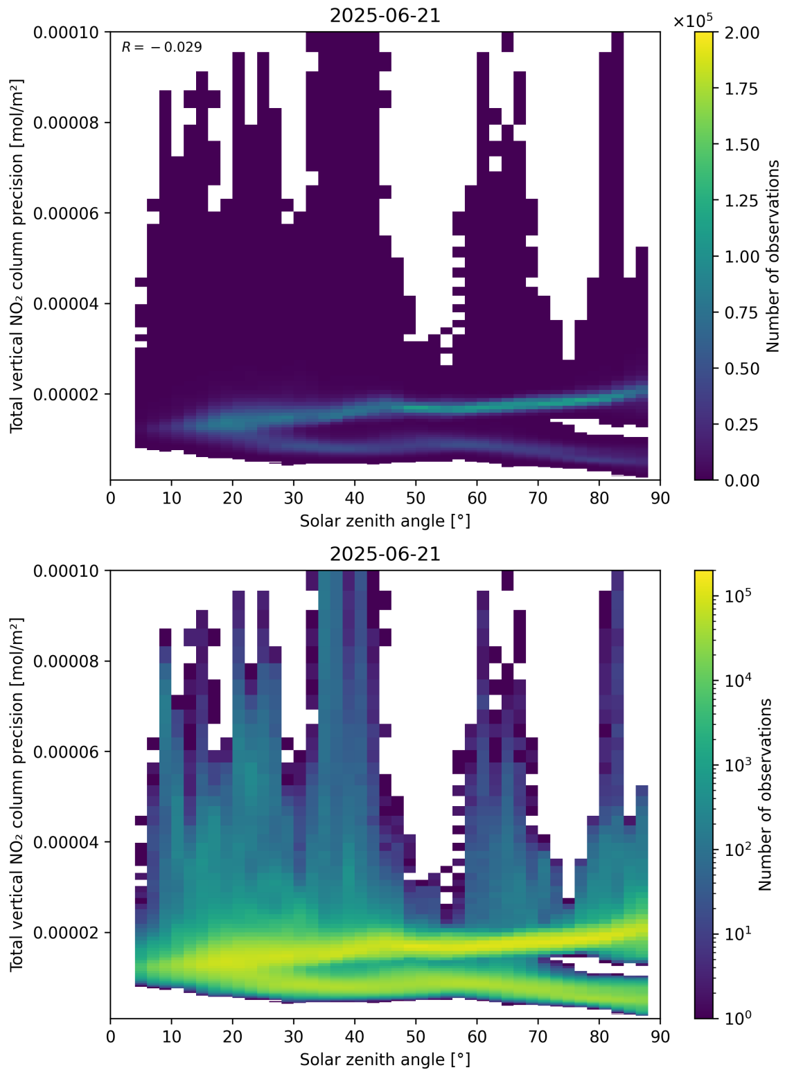
Figure 154: Scatter density plot of “Solar zenith angle” against “Total vertical NO 2 column precision” for 2025-06-20 to 2025-06-22.
