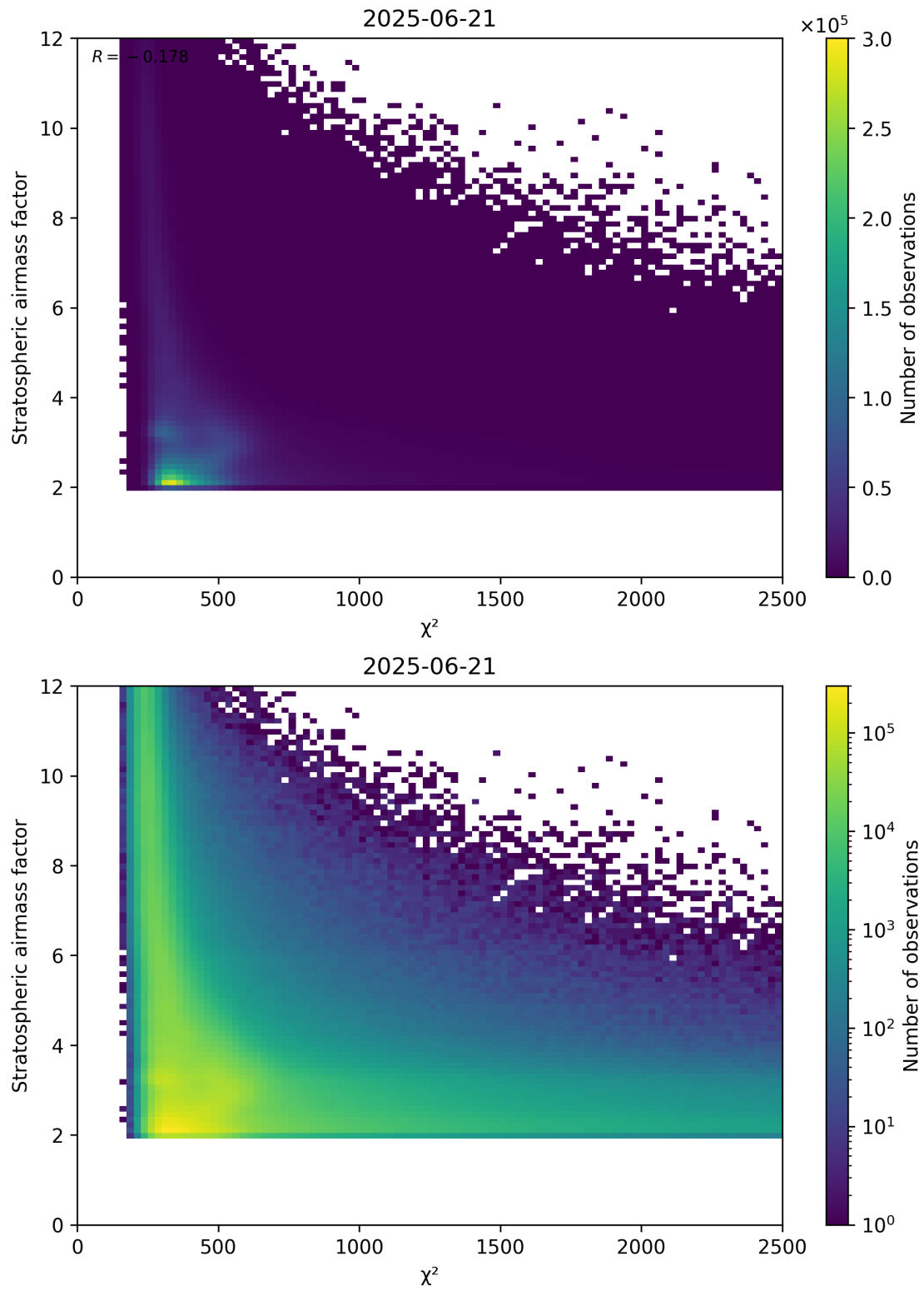
Figure 81: Scatter density plot of “ \chi^2 ” against “Stratospheric airmass factor” for 2025-06-20 to 2025-06-22.
