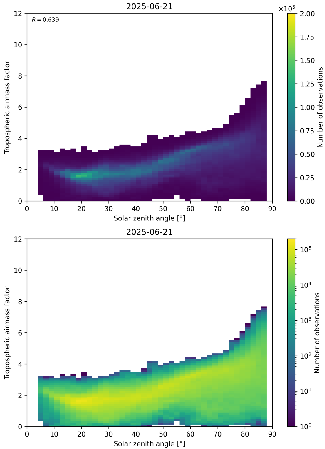
Figure 147: Scatter density plot of “Solar zenith angle” against “Tropospheric airmass factor” for 2025-06-20 to 2025-06-22.
