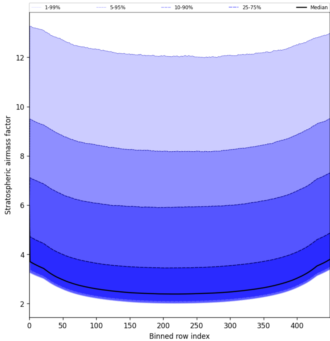
Figure 61: Along track statistics of “Stratospheric airmass factor” for 2025-06-20 to 2025-06-22
