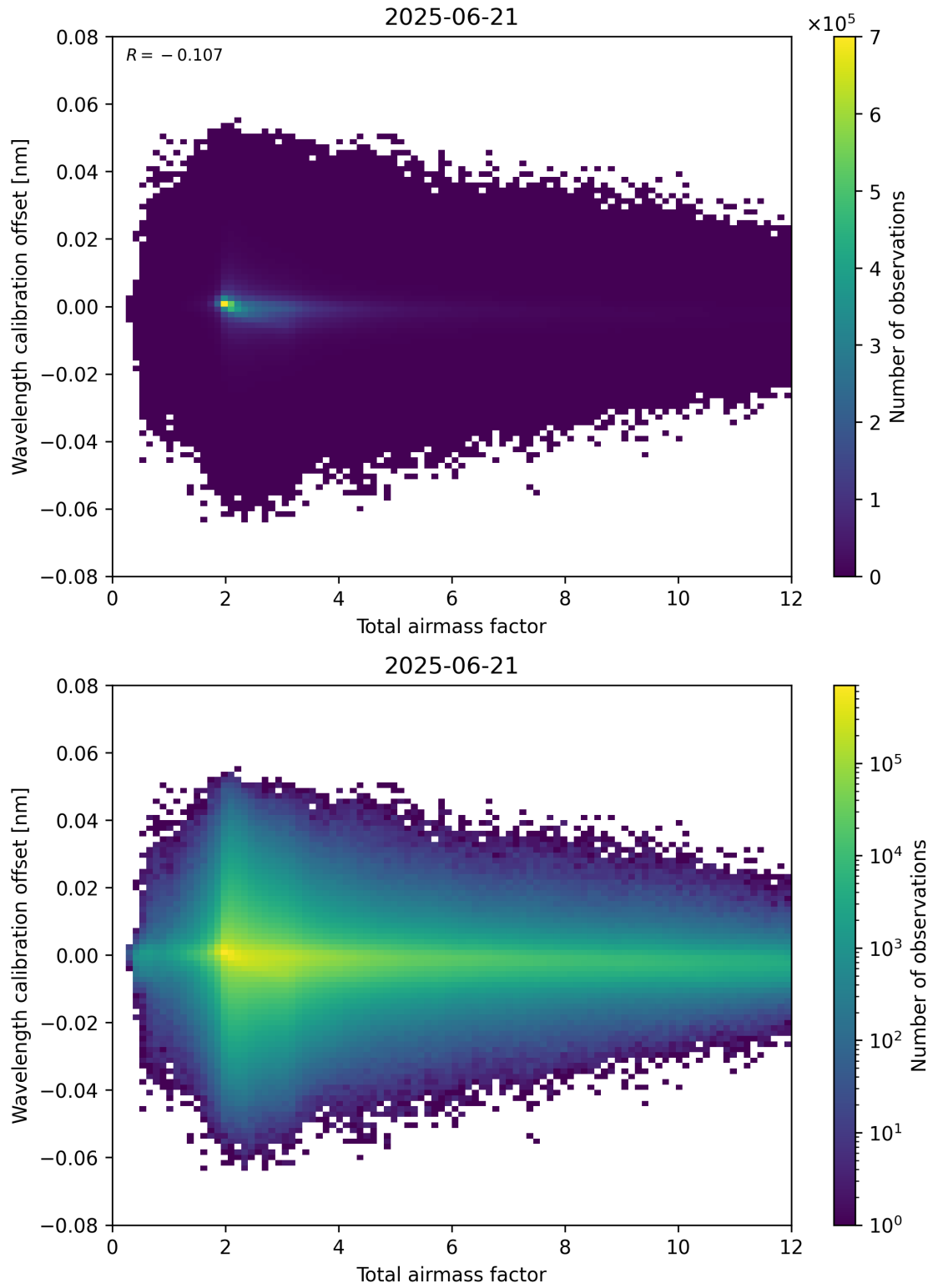
Figure 70: Scatter density plot of “Total airmass factor” against “Wavelength calibration offset” for 2025-06-20 to 2025-06-22.
