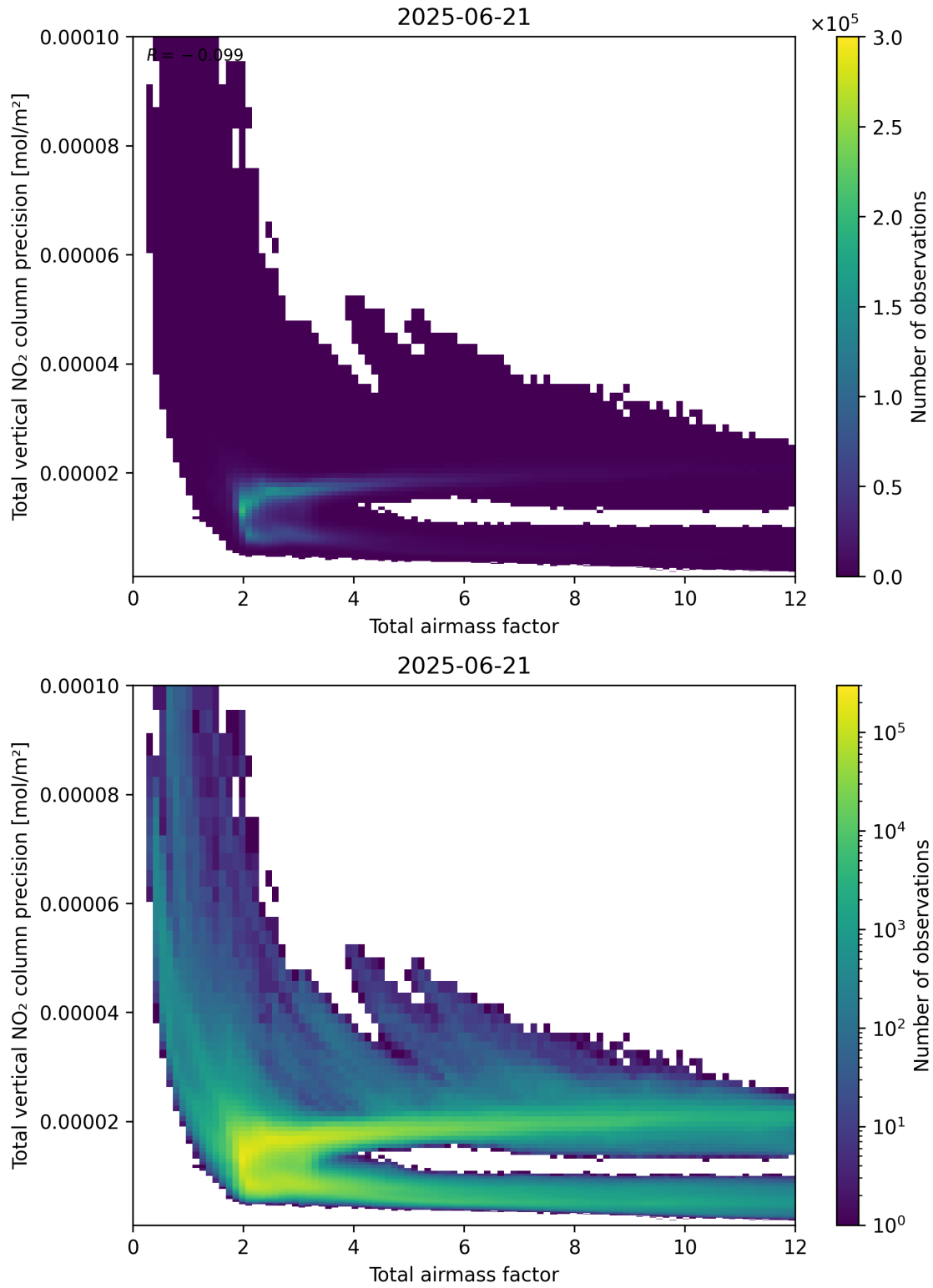
Figure 68: Scatter density plot of “Total airmass factor” against “Total vertical NO 2 column precision” for 2025-06-20 to 2025-06-22.
