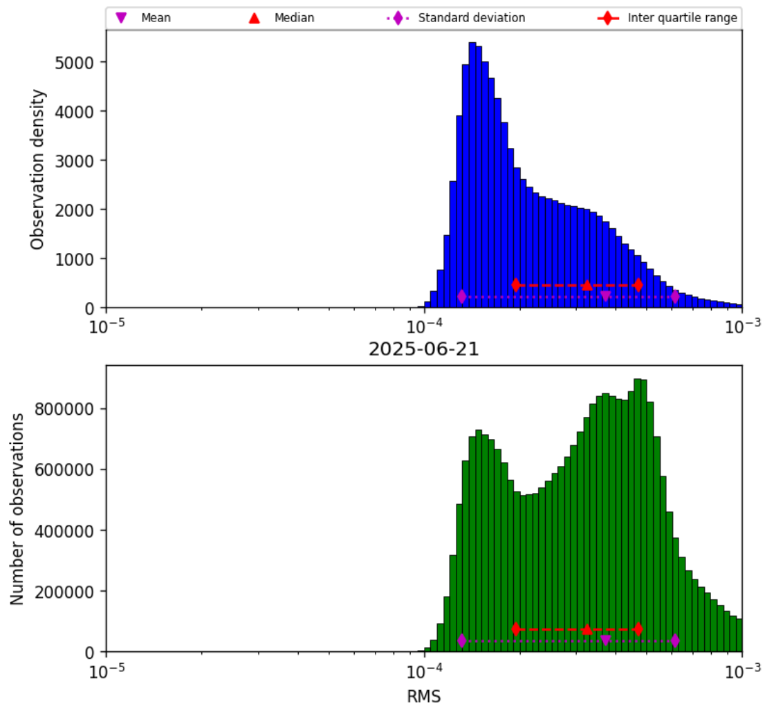
Figure 43: Histogram of “RMS” for 2025-06-20 to 2025-06-22
