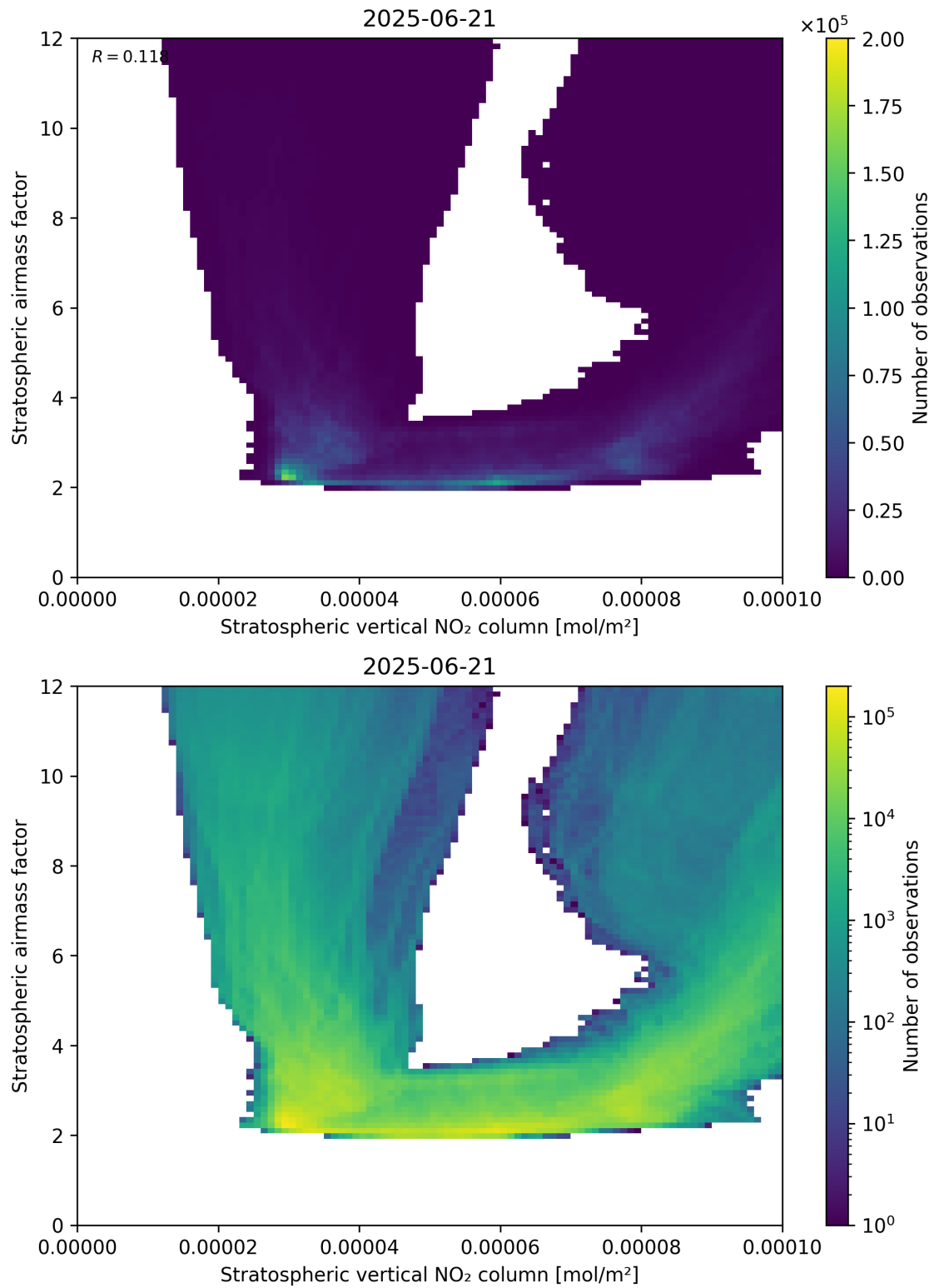
Figure 96: Scatter density plot of “Stratospheric vertical NO 2 column” against “Stratospheric airmass factor” for 2025-06-20 to 2025-06-22.
