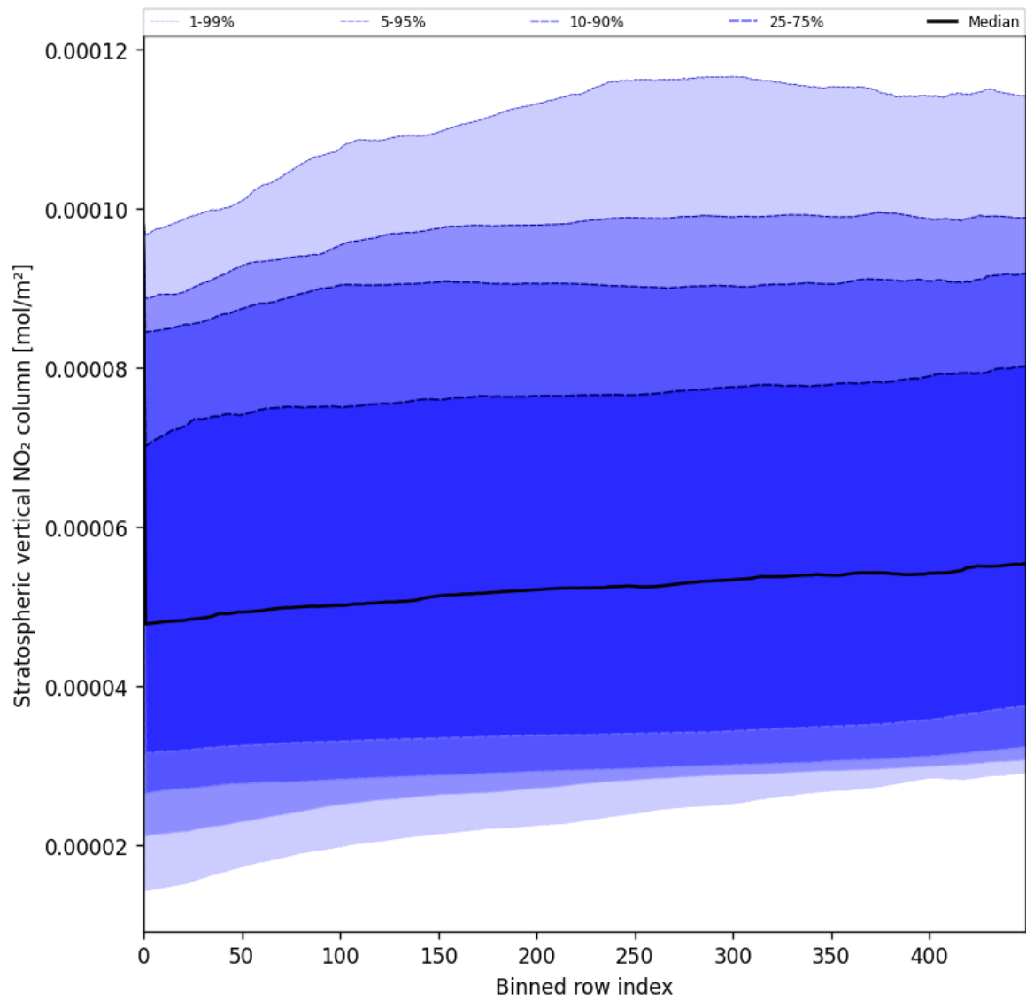
Figure 53: Along track statistics of “Stratospheric vertical NO 2 column” for 2025-06-20 to 2025-06-22
