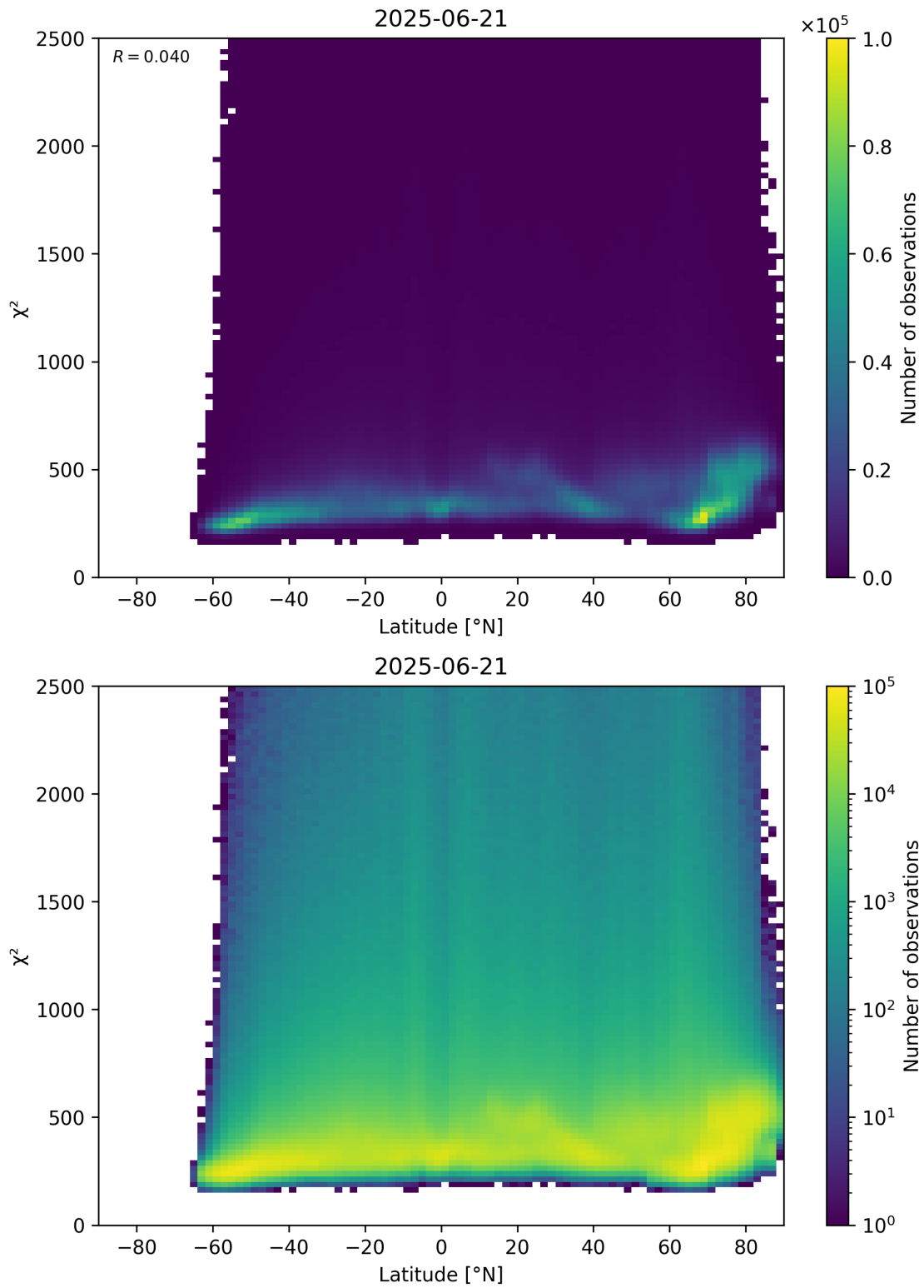
Figure 86: Scatter density plot of “Latitude” against “ \chi^2 ” for 2025-06-20 to 2025-06-22.
