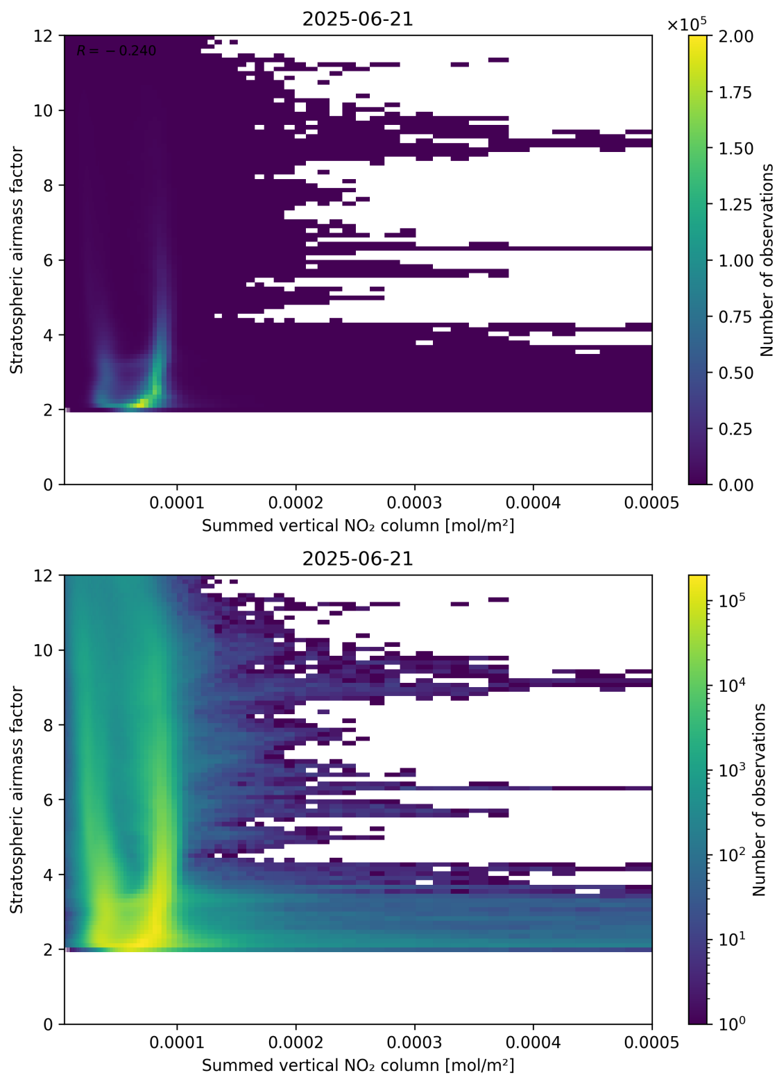
Figure 103: Scatter density plot of “Summed vertical NO 2 column” against “Stratospheric air mass factor” for 2025-06-20 to 2025-06-22.
