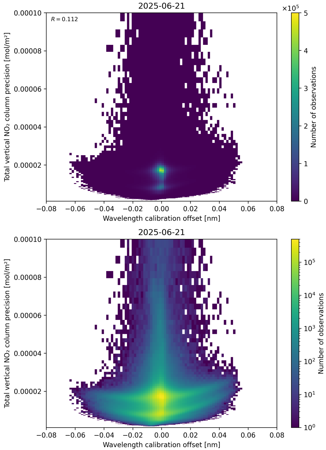
Figure 180: Scatter density plot of “Wavelength calibration offset” against “Total vertical NO 2 column precision” for 2025-06-20 to 2025-06-22.
