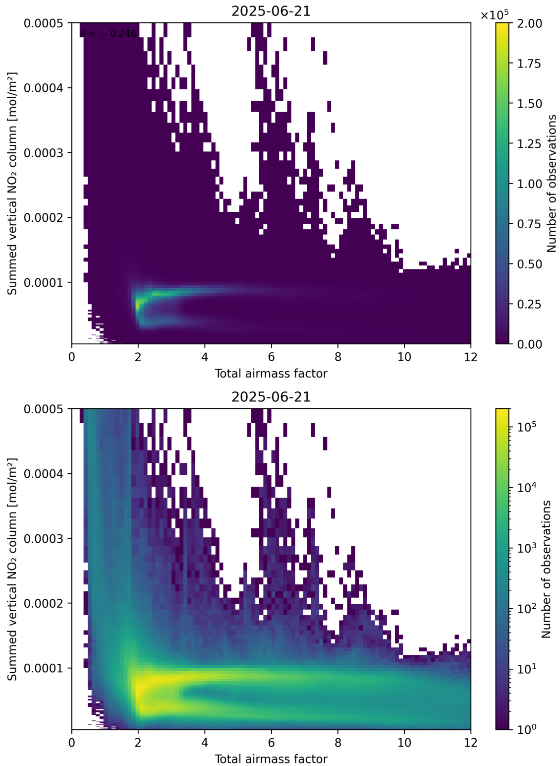
Figure 65: Scatter density plot of “Total airmass factor” against “Summed vertical NO 2 column” for 2025-06-20 to 2025-06-22.
