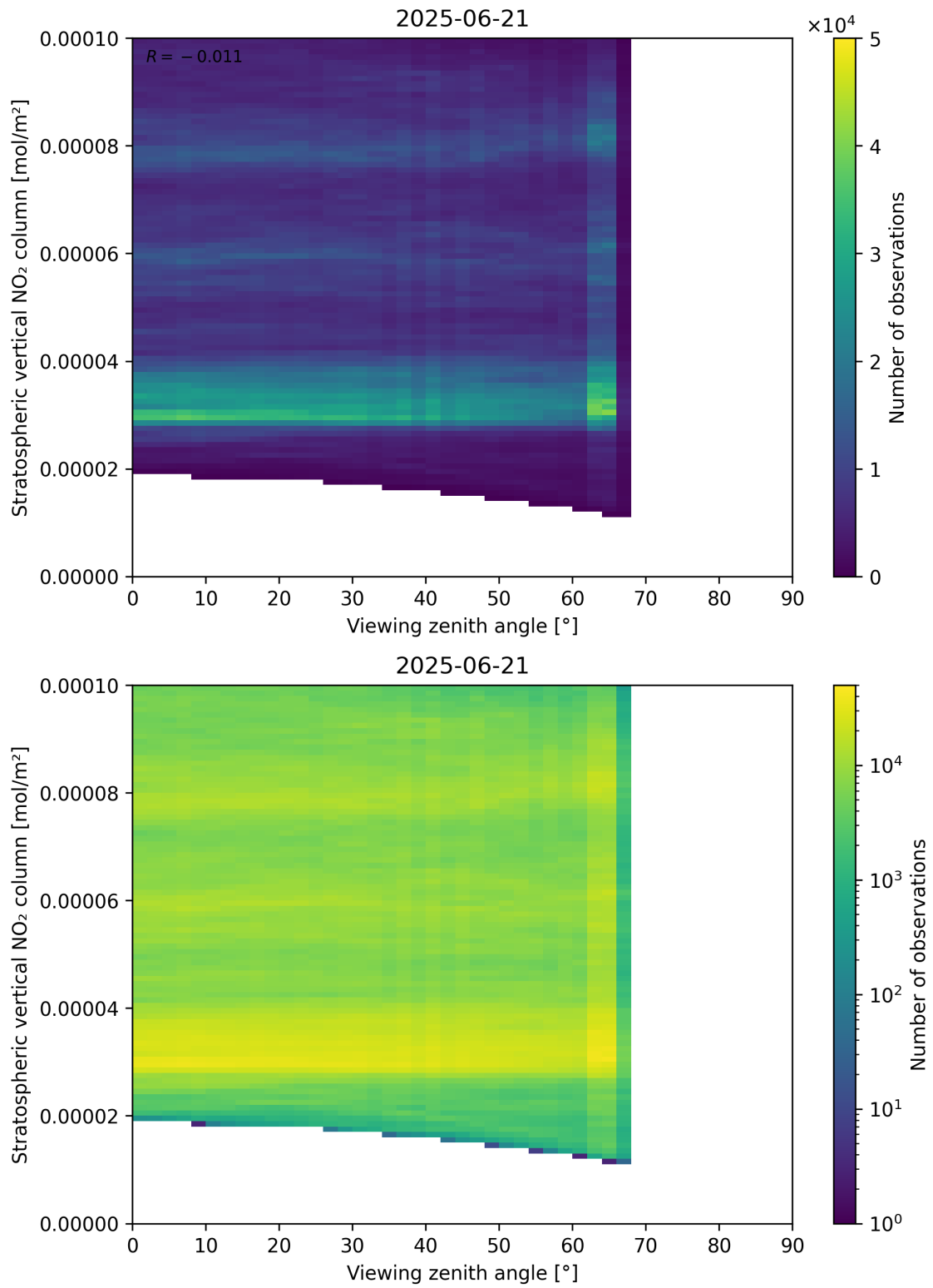
Figure 164: Scatter density plot of “Viewing zenith angle” against “Stratospheric vertical NO 2 column” for 2025-06-20 to 2025-06-22.
