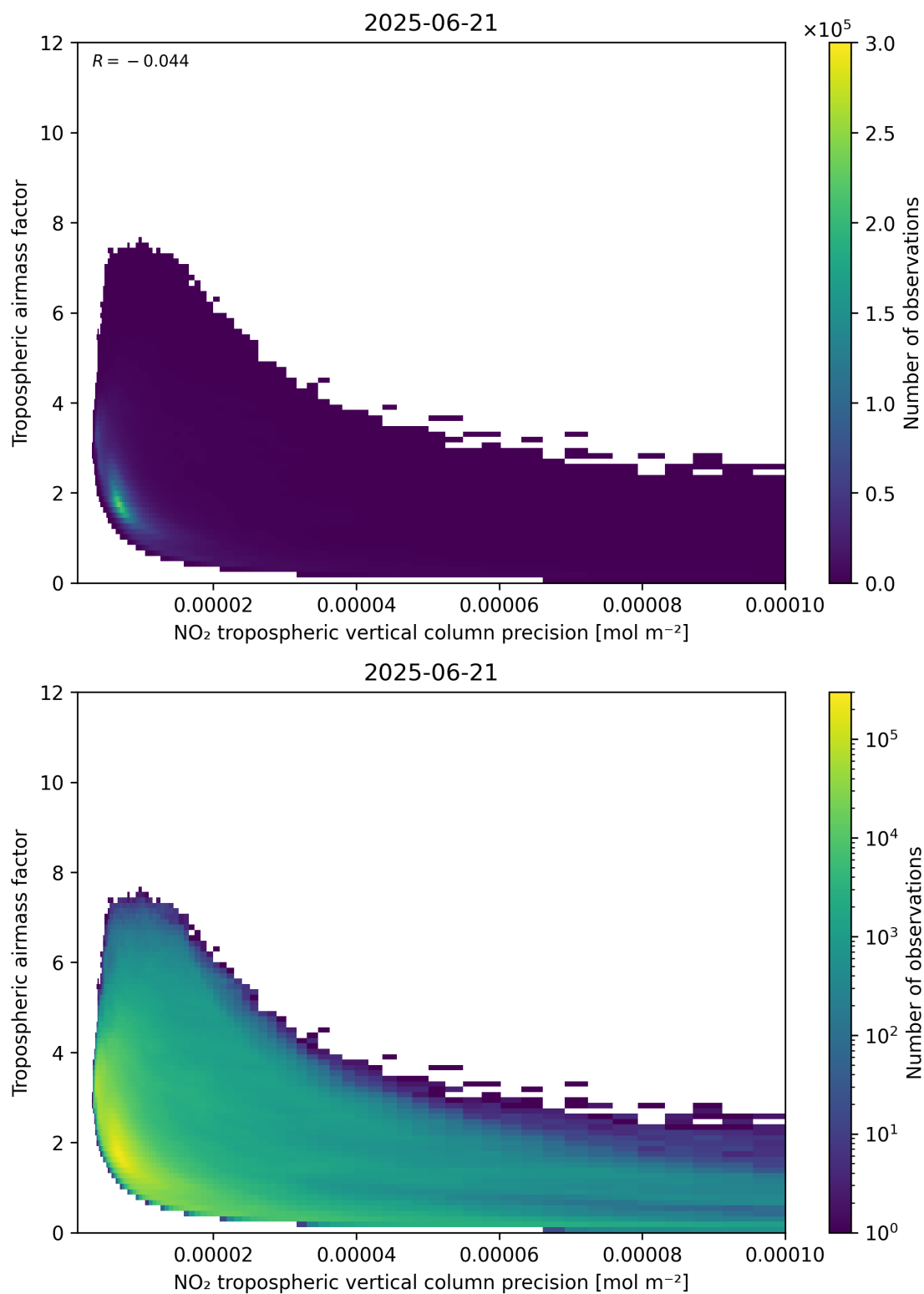
Figure 133: Scatter density plot of “NO 2 tropospheric vertical column precision” against “Tropospheric airmass factor” for 2025-06-20 to 2025-06-22.
