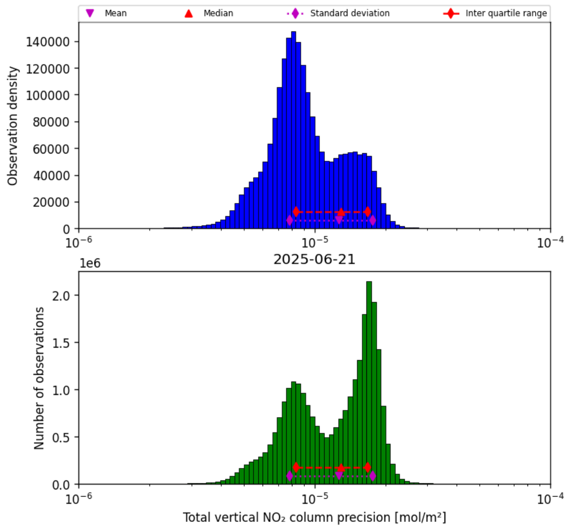
Figure 39: Histogram of “Total vertical NO 2 column precision” for 2025-06-20 to 2025-06-22
