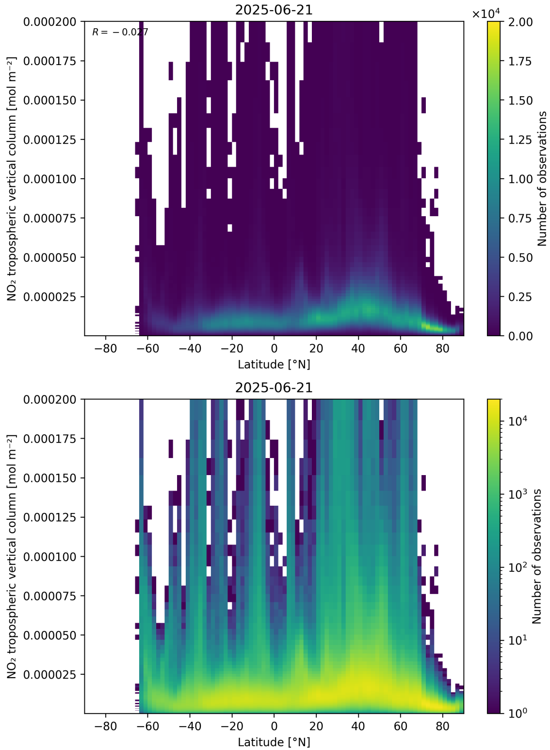
Figure 92: Scatter density plot of “Latitude” against “NO 2 tropospheric vertical column” for 2025-06-20 to 2025-06-22.
