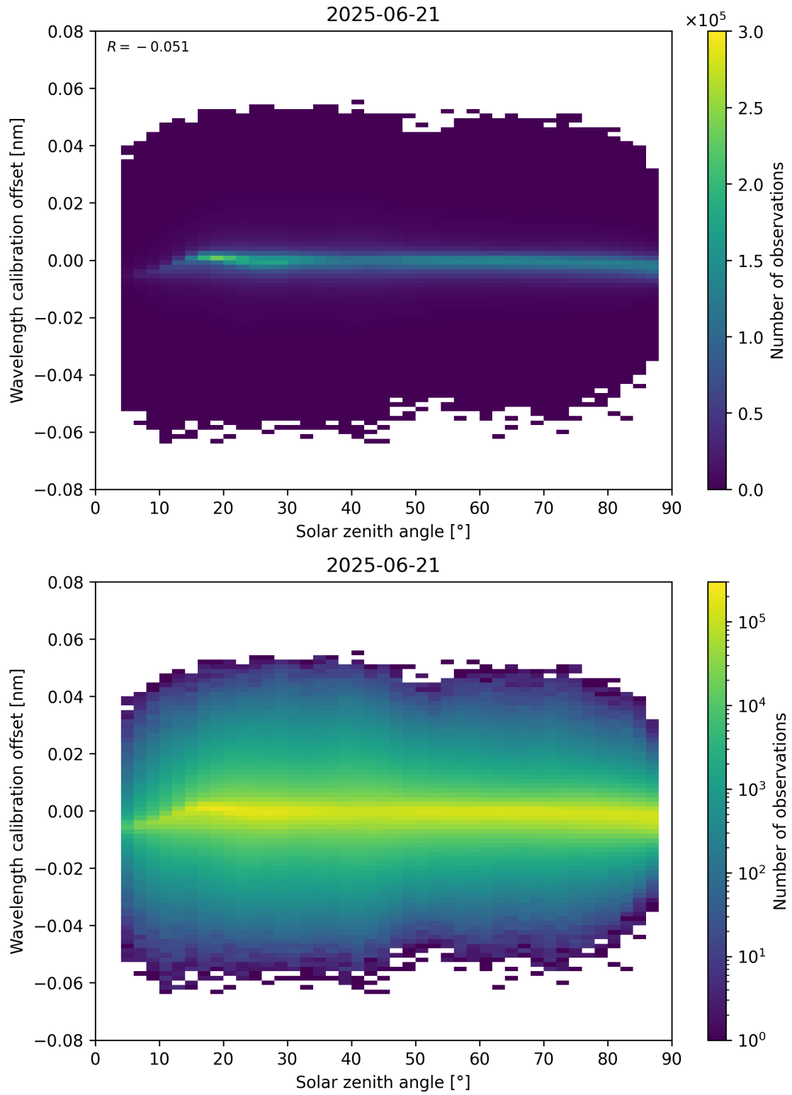
Figure 158: Scatter density plot of “Solar zenith angle” against “Wavelength calibration offset” for 2025-06-20 to 2025-06-22.
