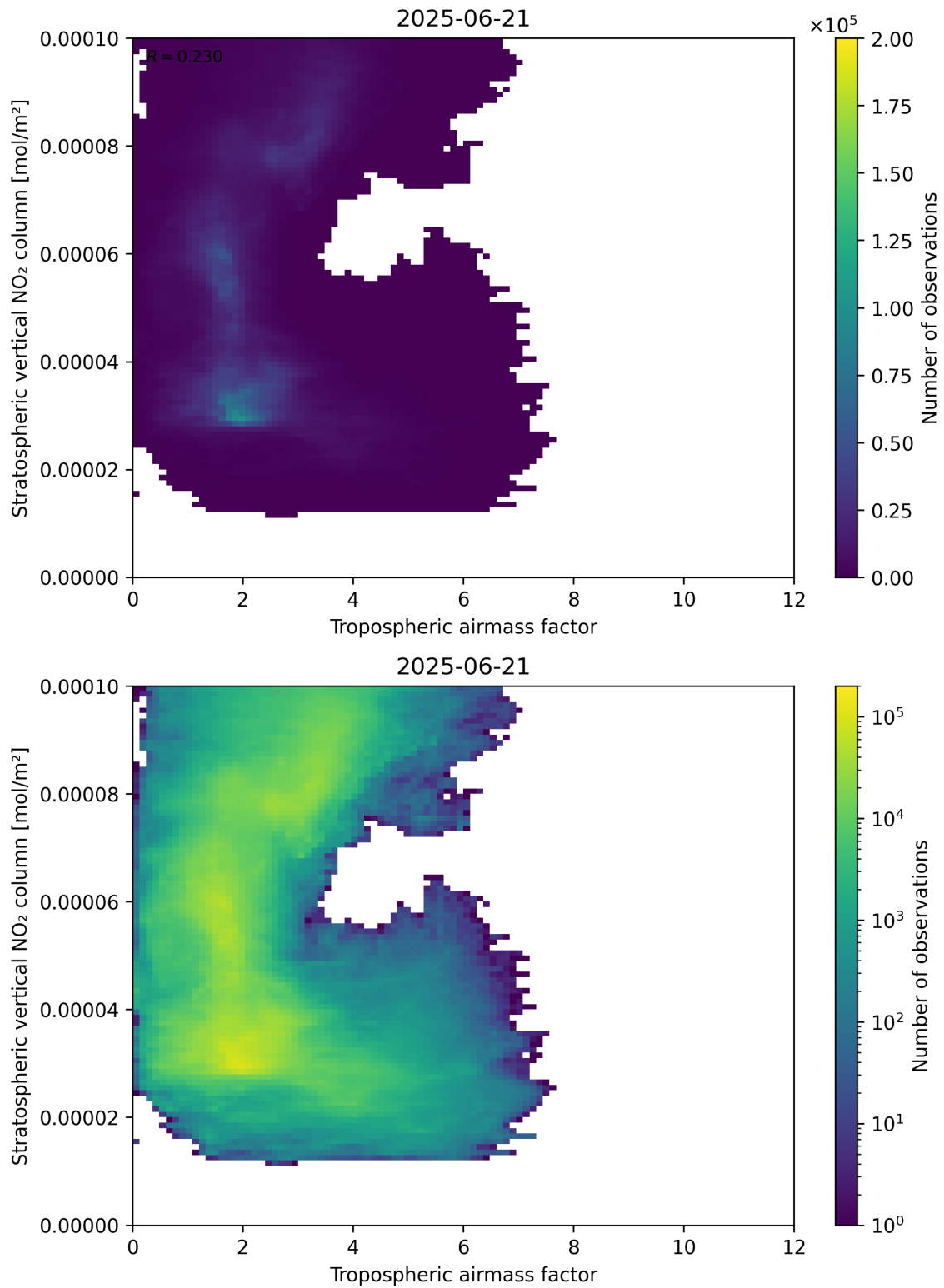
Figure 74: Scatter density plot of “Tropospheric airmass factor” against “Stratospheric vertical NO 2 column” for 2025-06-20 to 2025-06-22.
