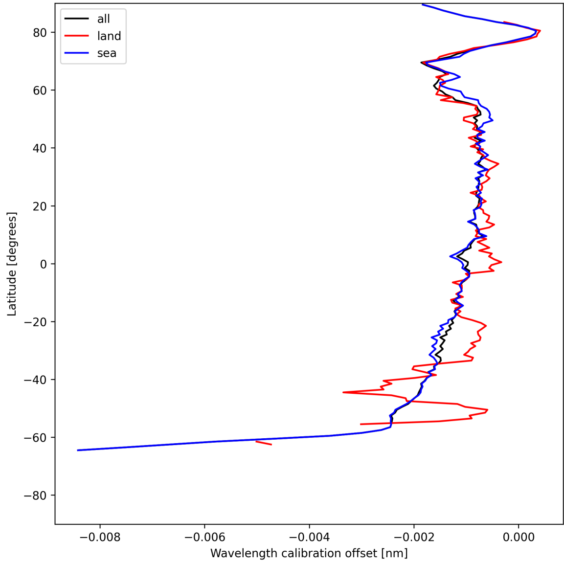
Figure 18: Zonal average of “Wavelength calibration offset” for 2025-06-20 to 2025-06-22.
