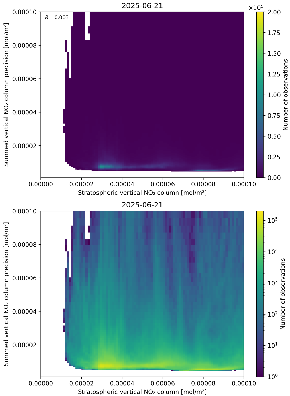
Figure 99: Scatter density plot of “Stratospheric vertical NO 2 column” against “Summed vertical NO 2 column precision” for 2025-06-20 to 2025-06-22.
