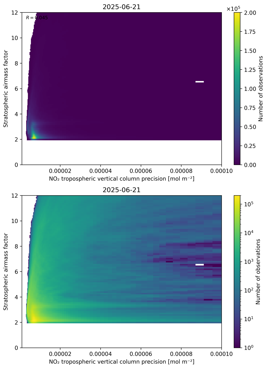
Figure 131: Scatter density plot of “NO 2 tropospheric vertical column precision” against “Stratospheric airmass factor” for 2025-06-20 to 2025-06-22.
