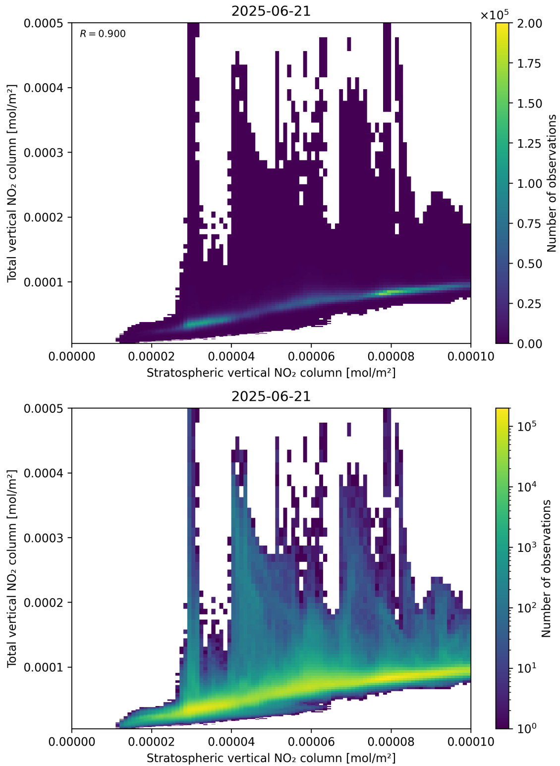
Figure 100: Scatter density plot of “Stratospheric vertical NO 2 column” against “Total vertical NO 2 column” for 2025-06-20 to 2025-06-22.
