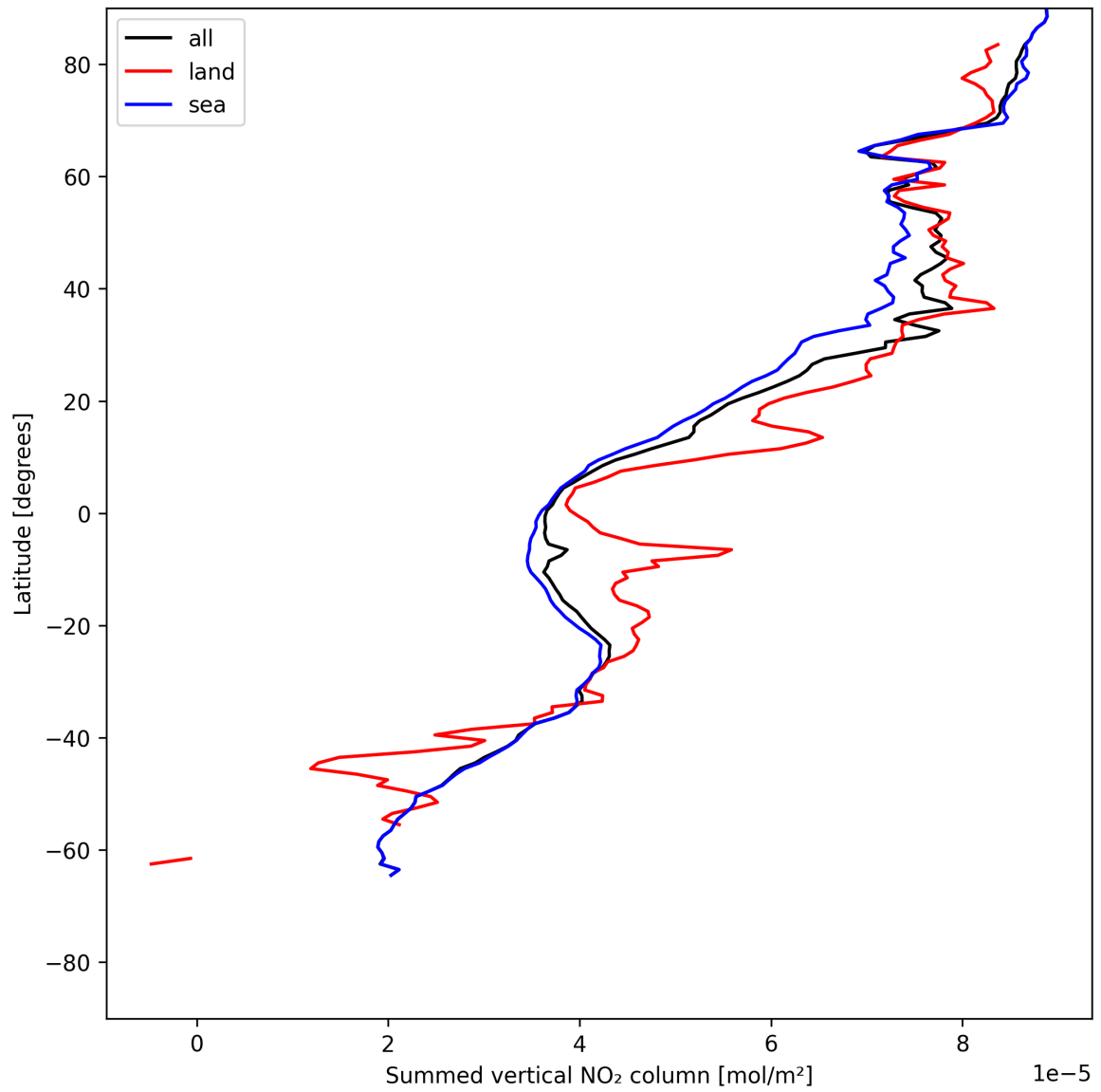
Figure 23: Zonal average of “Summed vertical NO 2 column” for 2025-06-20 to 2025-06-22.
