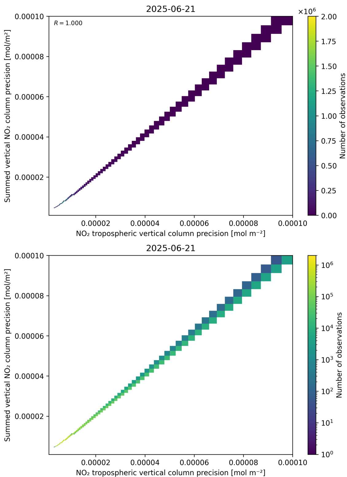
Figure 137: Scatter density plot of “NO 2 tropospheric vertical column precision” against “Summed vertical NO 2 column precision” for 2025-06-20 to 2025-06-22.
