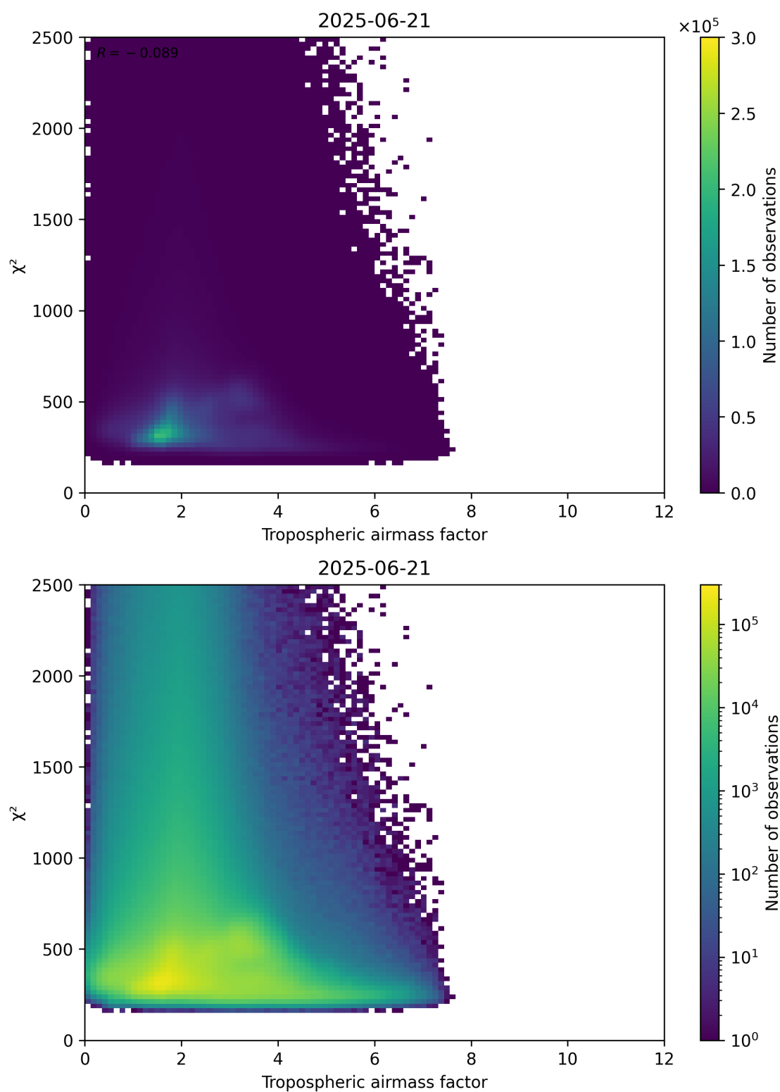
Figure 73: Scatter density plot of “Tropospheric airmass factor” against “ \chi^2 ” for 2025-06-20 to 2025-06-22.
