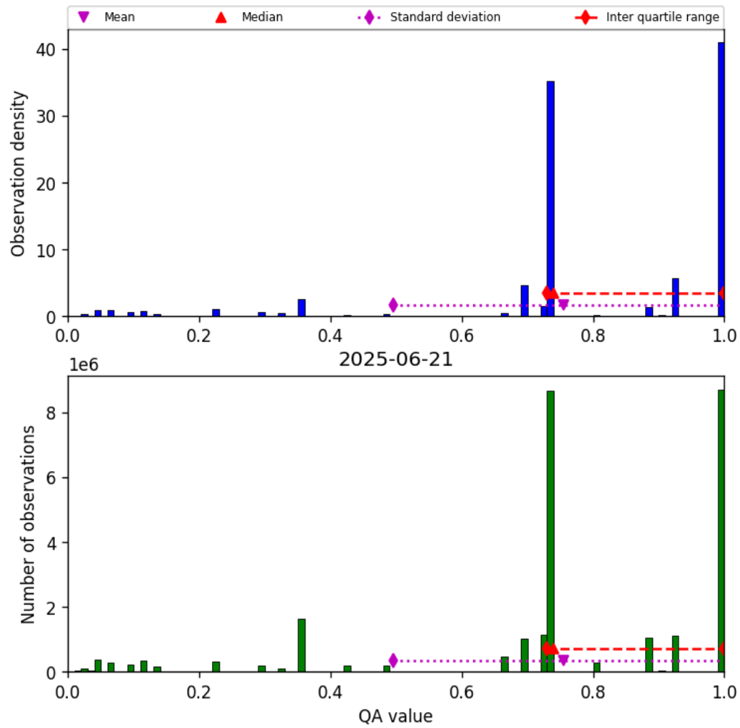
Figure 28: Histogram of “QA value” for 2025-06-20 to 2025-06-22
