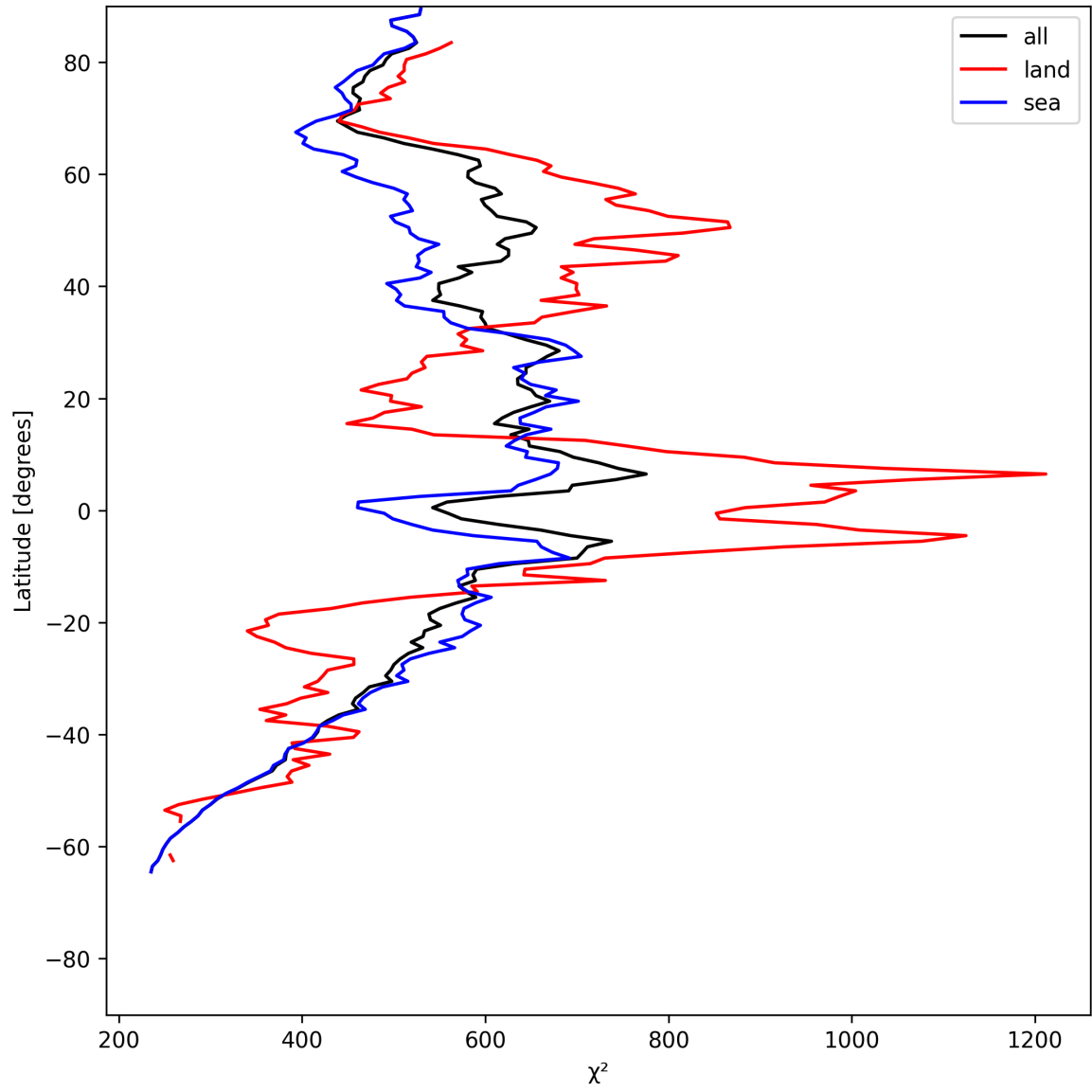
Figure 25: Zonal average of “ \chi^2 ” for 2025-06-20 to 2025-06-22.
