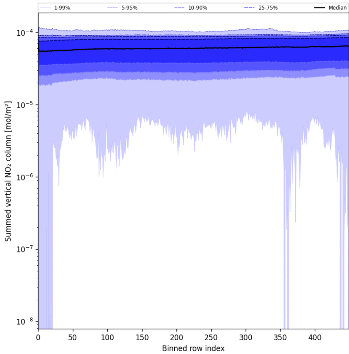
Figure 57: Along track statistics of “Summed vertical NO 2 column” for 2025-06-20 to 2025-06-22
