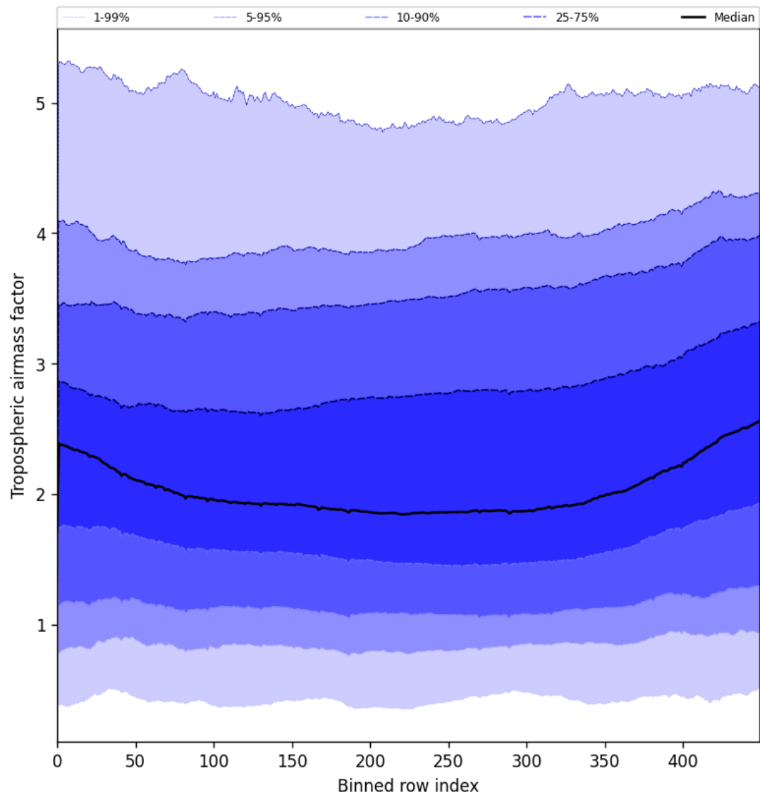
Figure 48: Along track statistics of “Tropospheric airmass factor” for 2025-06-20 to 2025-06-22
