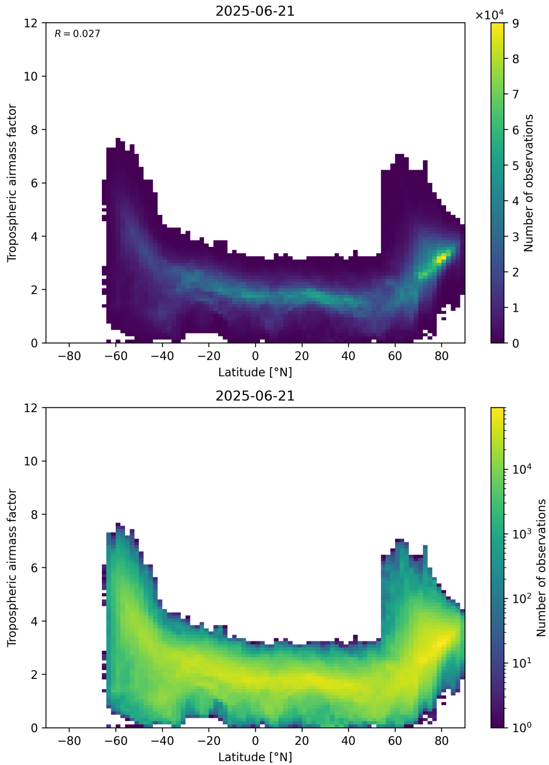
Figure 85: Scatter density plot of “Latitude” against “Tropospheric airmass factor” for 2025-06-20 to 2025-06-22.
