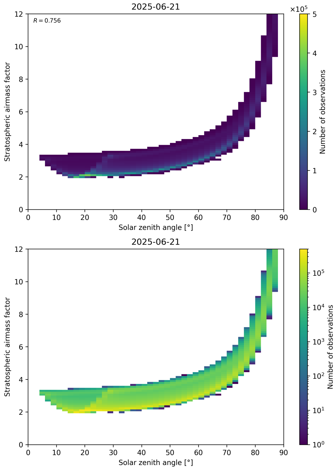
Figure 145: Scatter density plot of “Solar zenith angle” against “Stratospheric airmass factor” for 2025-06-20 to 2025-06-22.
