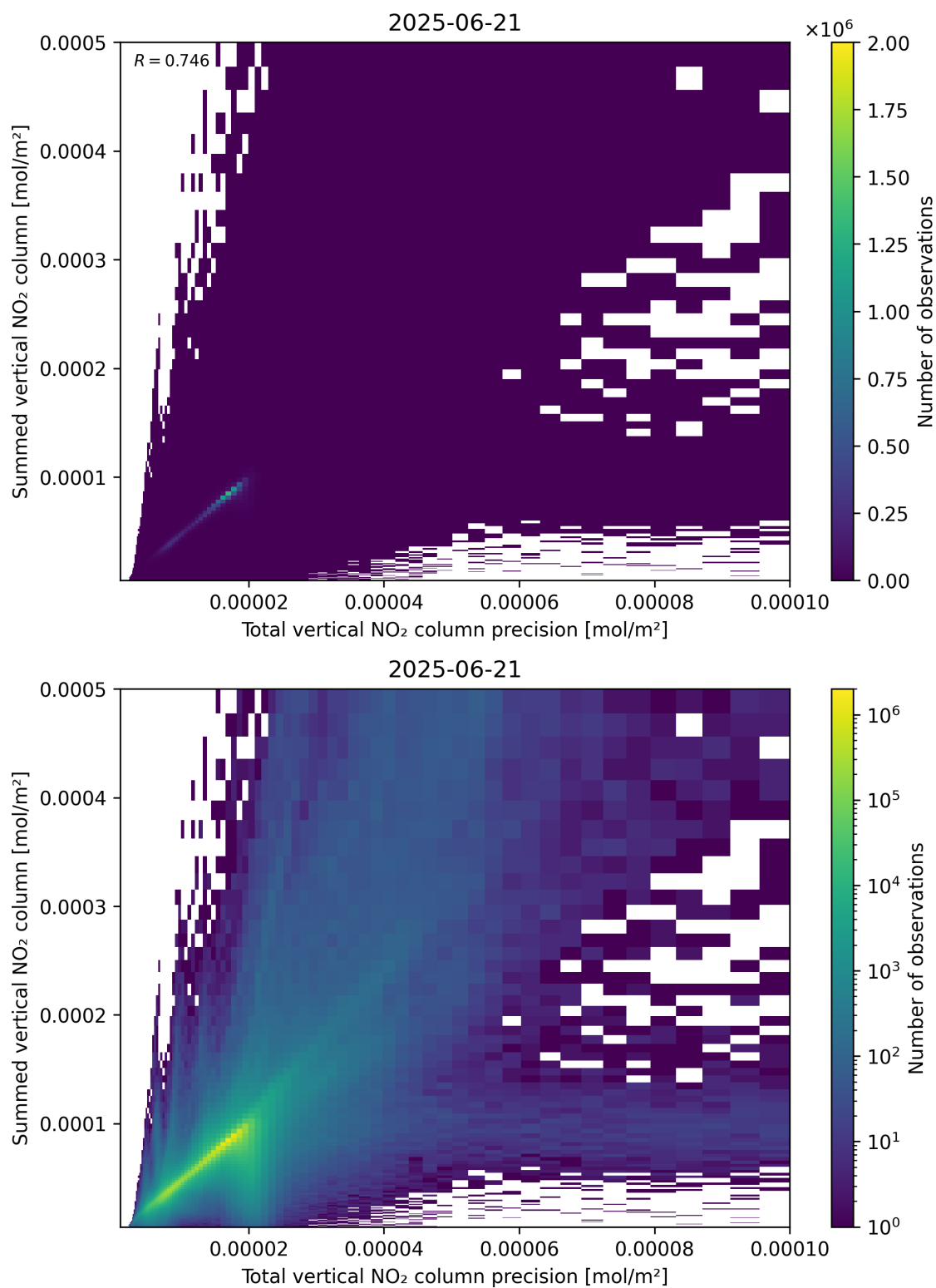
Figure 117: Scatter density plot of “Total vertical NO 2 column precision” against “Summed vertical NO 2 column” for 2025-06-20 to 2025-06-22.
