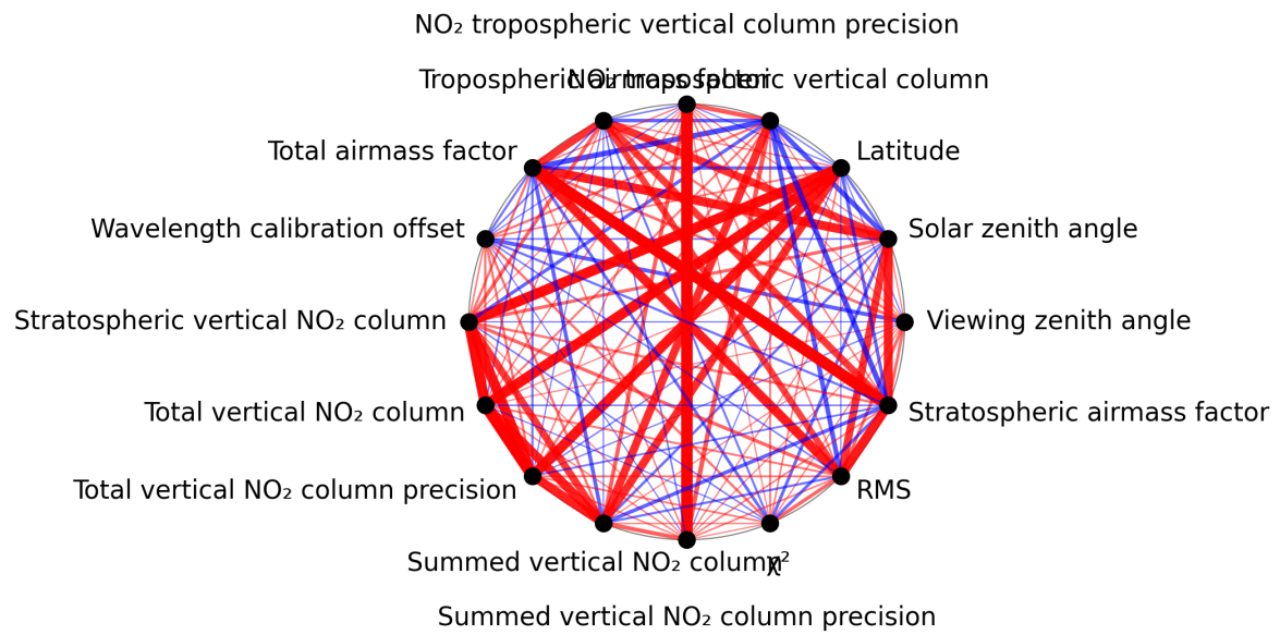
Figure 1: Map of correlation graph for 2025-06-20 to 2025-06-22.
