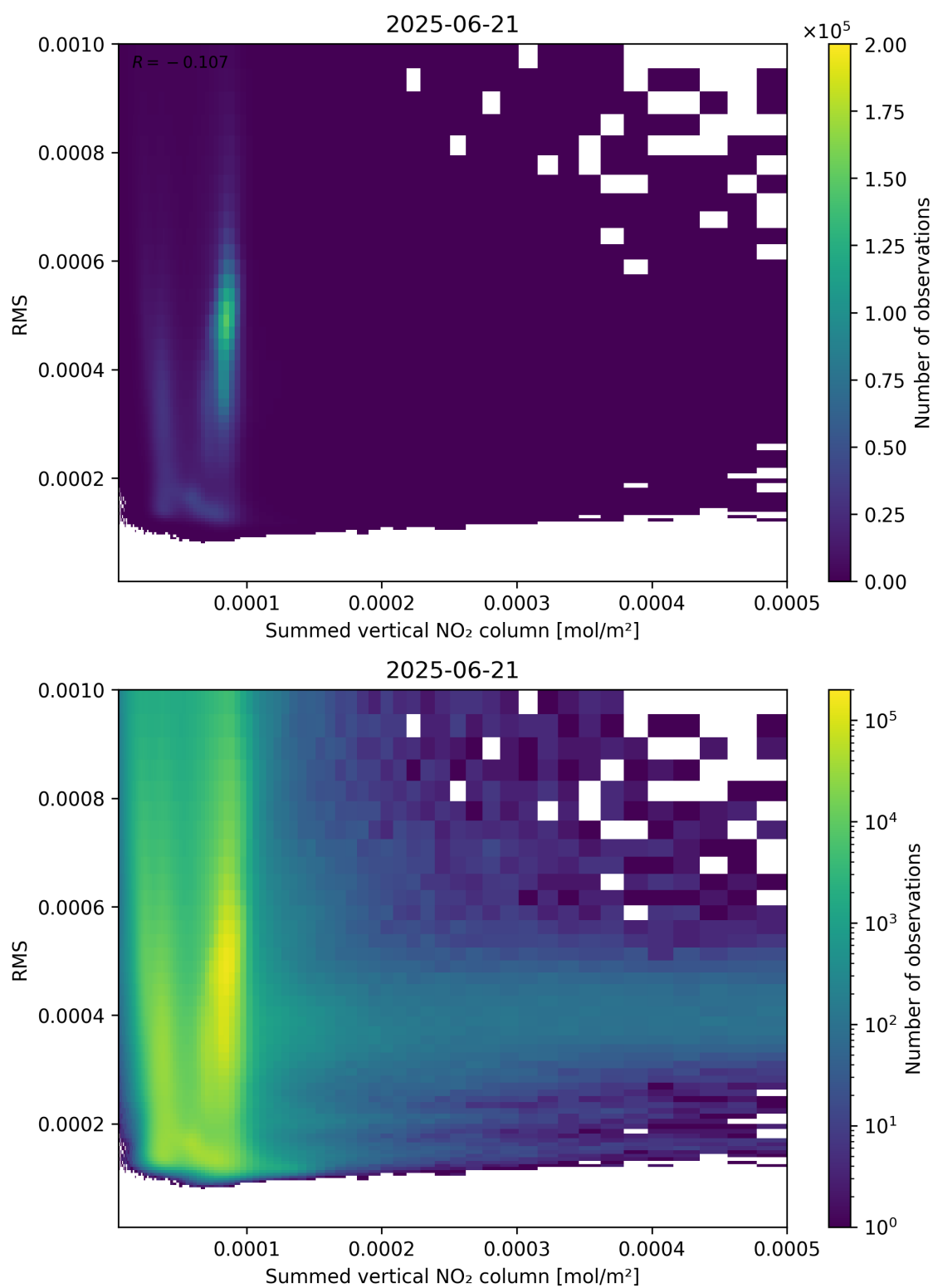
Figure 109: Scatter density plot of “Summed vertical NO 2 column” against “RMS” for 2025-06-20 to 2025-06-22.
