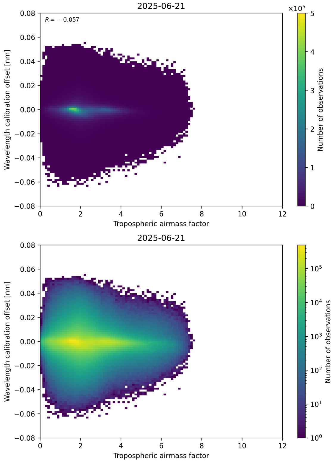
Figure 80: Scatter density plot of “Tropospheric airmass factor” against “Wavelength calibration offset” for 2025-06-20 to 2025-06-22.
