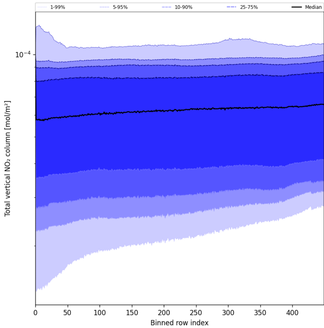
Figure 55: Along track statistics of “Total vertical NO 2 column” for 2025-06-20 to 2025-06-22
