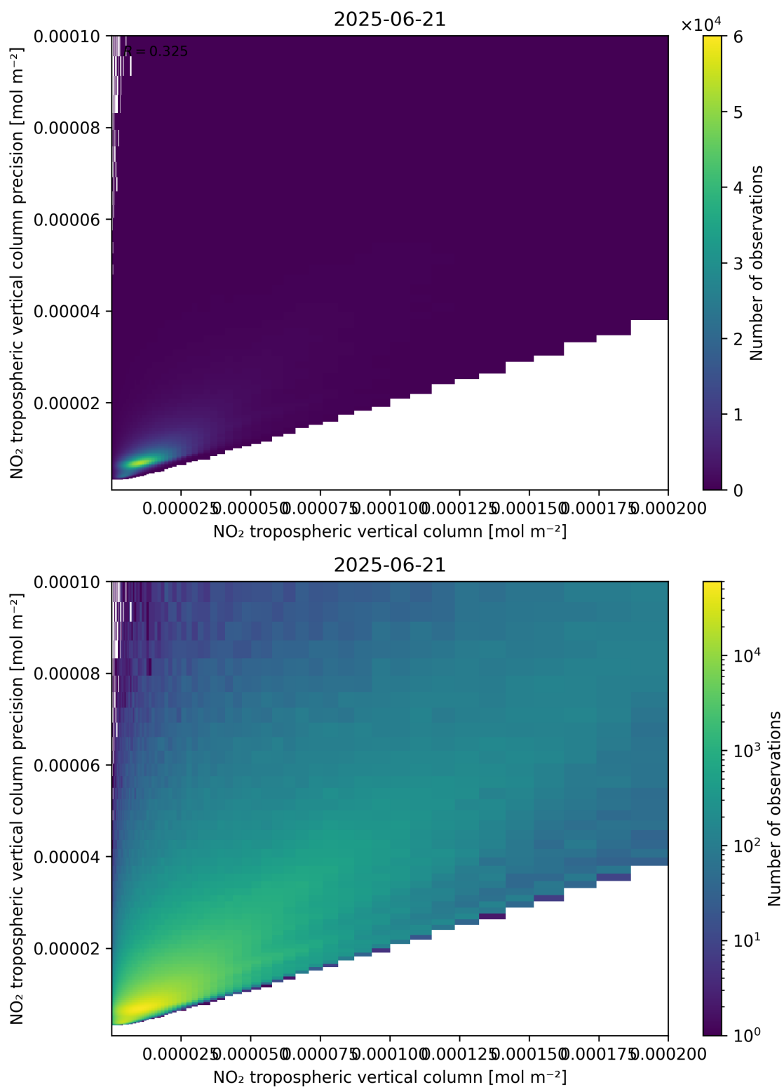
Figure 130: Scatter density plot of “NO 2 tropospheric vertical column” against “NO 2 tropospheric vertical column precision” for 2025-06-20 to 2025-06-22.
