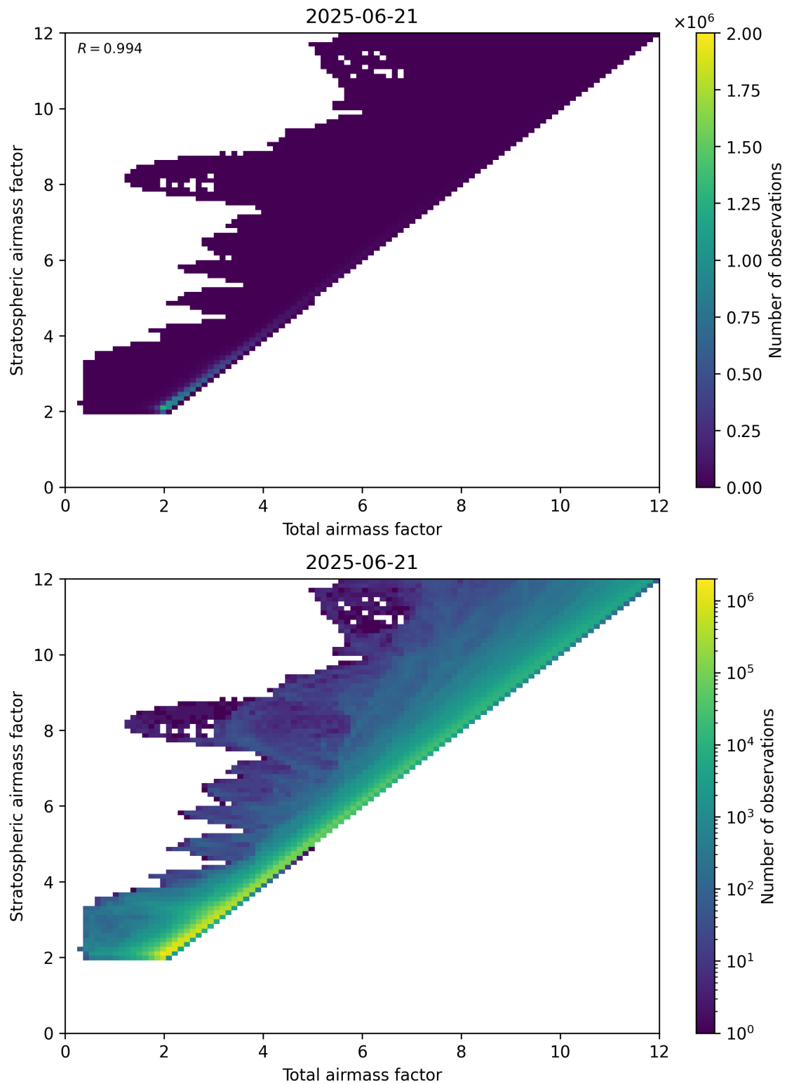
Figure 62: Scatter density plot of “Total airmass factor” against “Stratospheric airmass factor” for 2025-06-20 to 2025-06-22.
