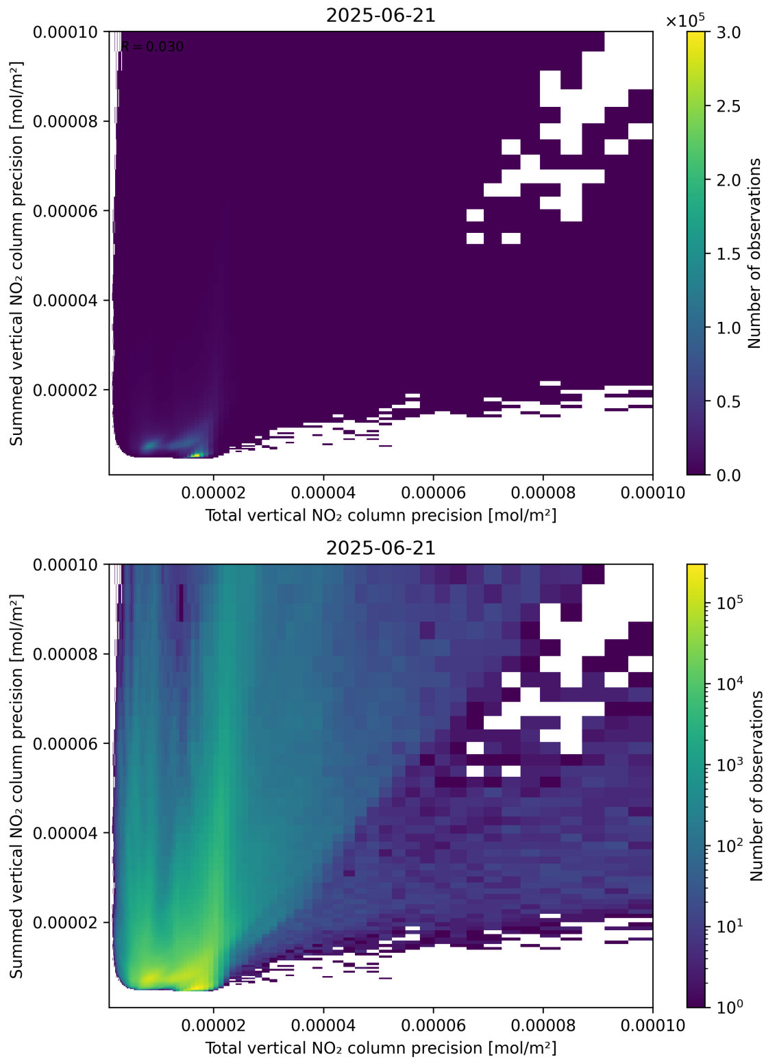
Figure 118: Scatter density plot of “Total vertical NO 2 column precision” against “Summed vertical NO 2 column precision” for 2025-06-20 to 2025-06-22.
