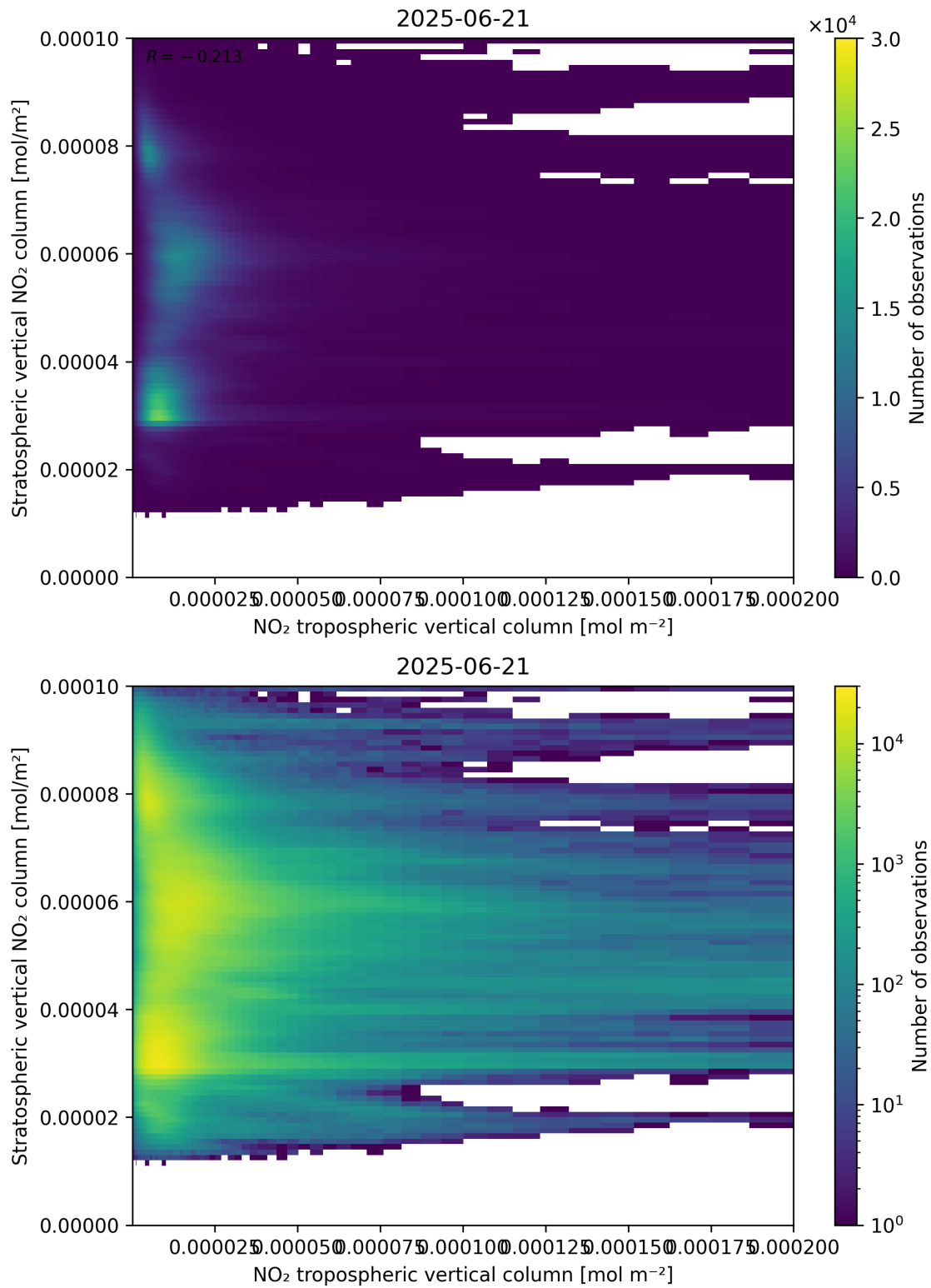
Figure 125: Scatter density plot of “NO 2 tropospheric vertical column” against “Stratospheric vertical NO 2 column” for 2025-06-20 to 2025-06-22.
