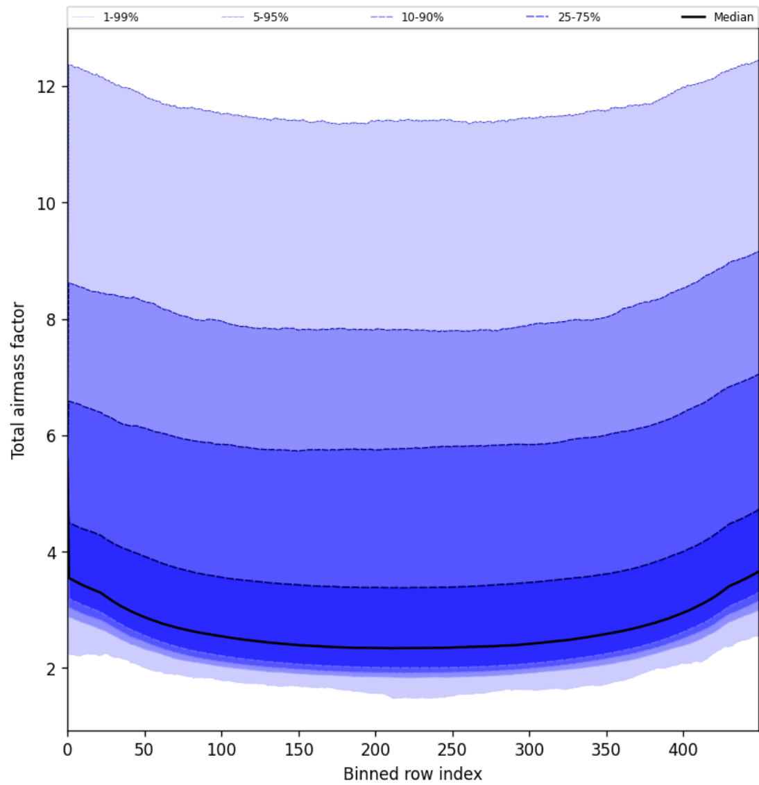
Figure 49: Along track statistics of “Total airmass factor” for 2025-06-20 to 2025-06-22
