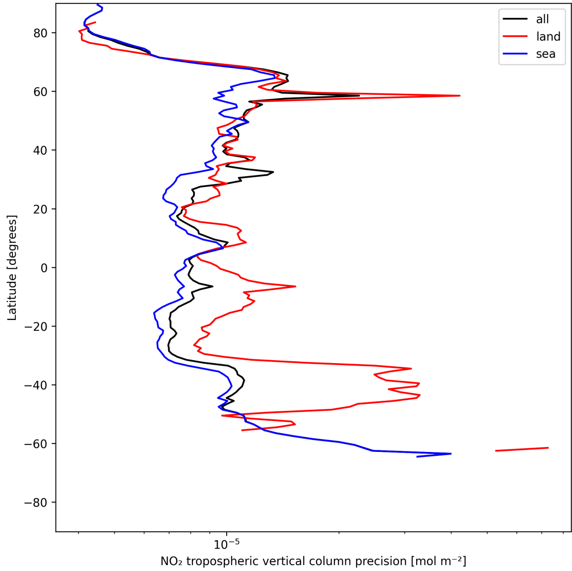
Figure 13: Zonal average of “NO 2 tropospheric vertical column precision” for 2025-06-20 to 2025-06-22.
