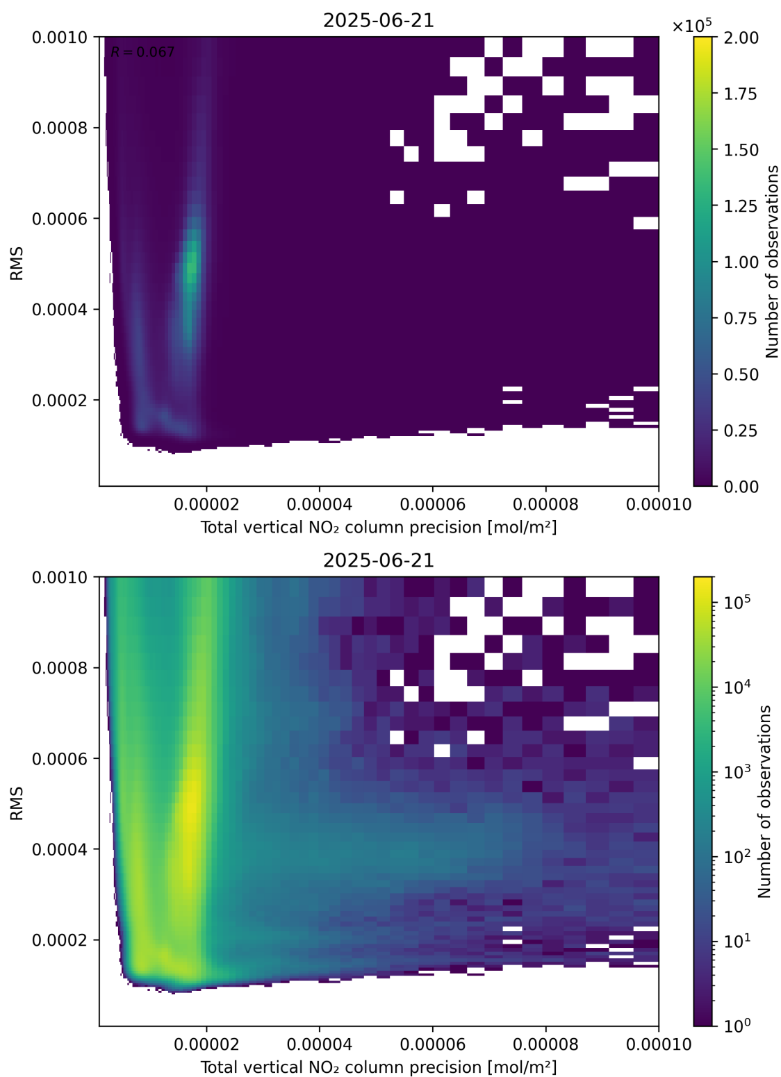
Figure 119: Scatter density plot of “Total vertical NO 2 column precision” against “RMS” for 2025-06-20 to 2025-06-22.
