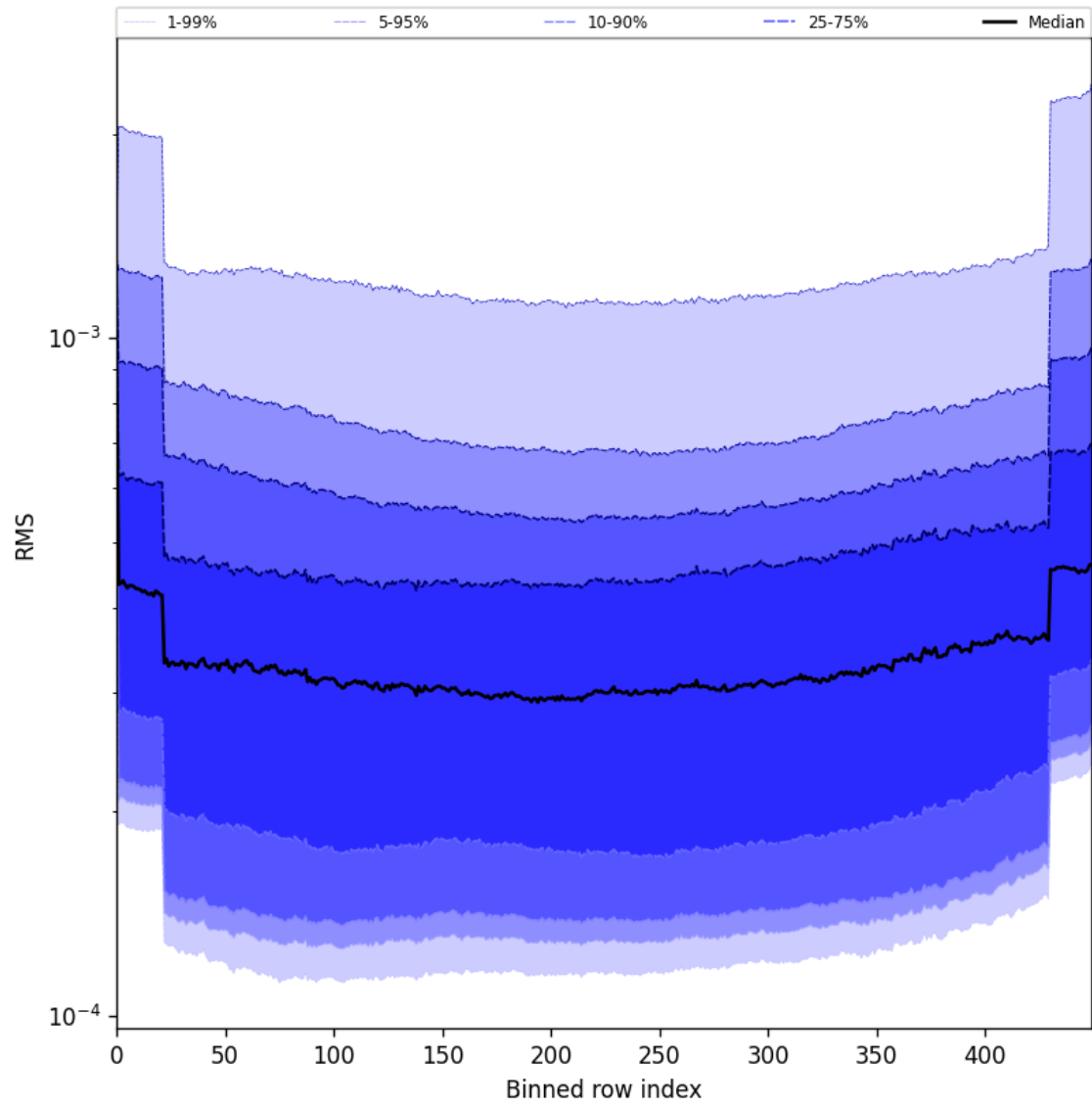
Figure 60: Along track statistics of “RMS” for 2025-06-20 to 2025-06-22
