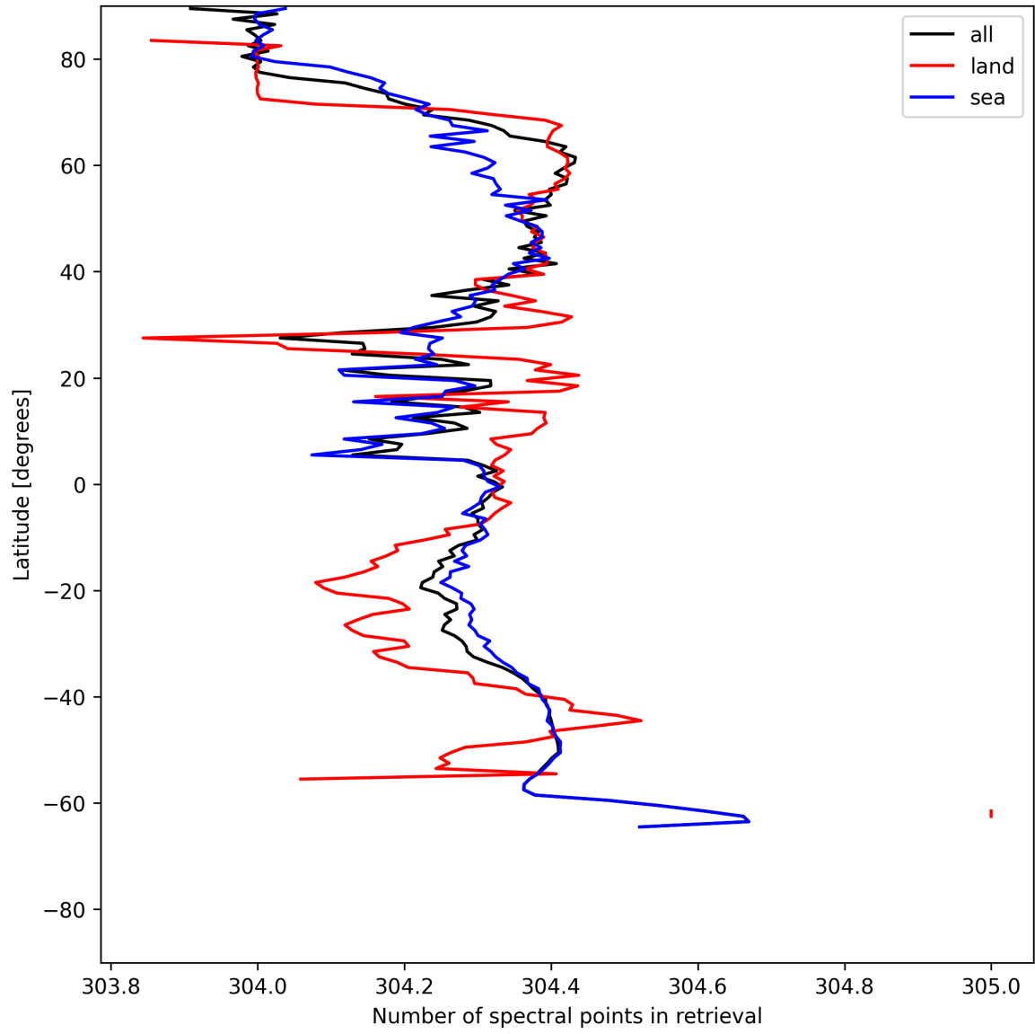
Figure 16: Zonal average of “Number of spectral points in retrieval” for 2025-06-20 to 2025-06-22.
