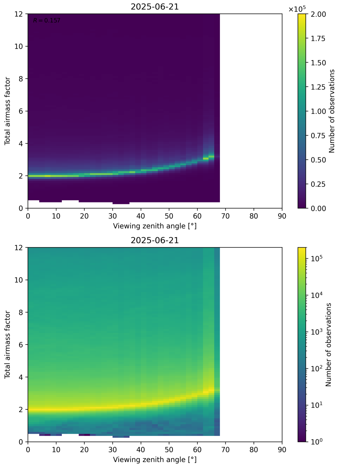
Figure 160: Scatter density plot of “Viewing zenith angle” against “Total airmass factor” for 2025-06-20 to 2025-06-22.
