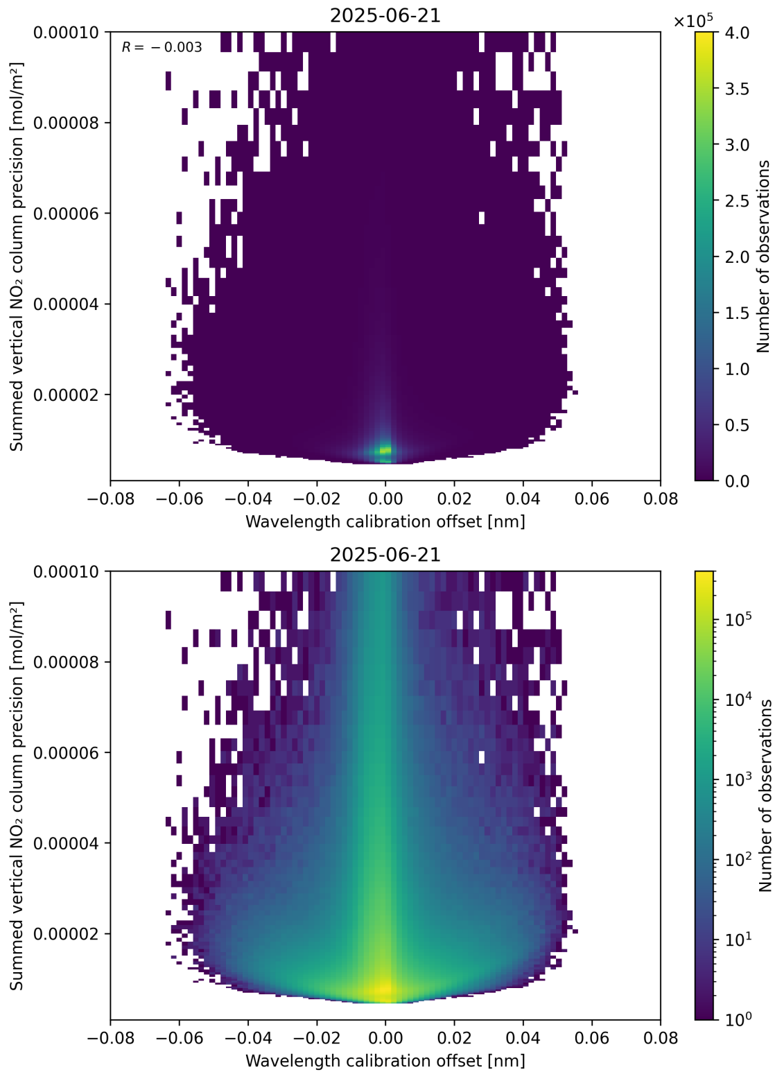
Figure 178: Scatter density plot of “Wavelength calibration offset” against “Summed vertical NO 2 column precision” for 2025-06-20 to 2025-06-22.
