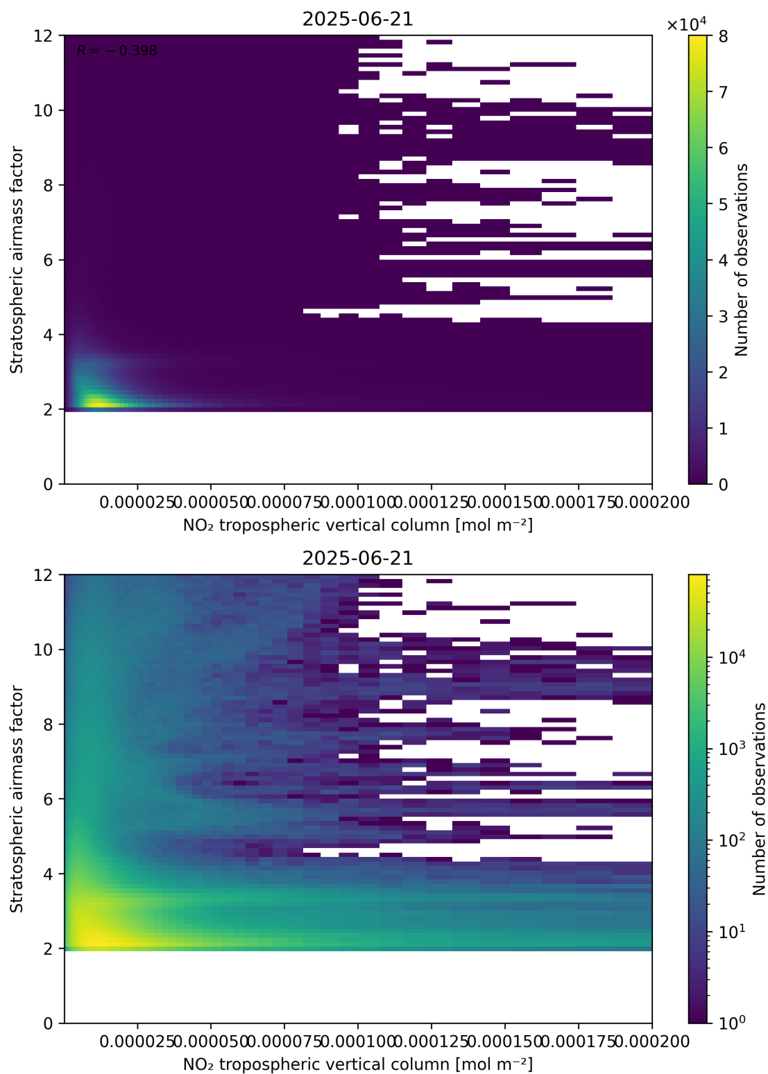
Figure 121: Scatter density plot of “NO 2 tropospheric vertical column” against “Stratospheric air mass factor” for 2025-06-20 to 2025-06-22.
