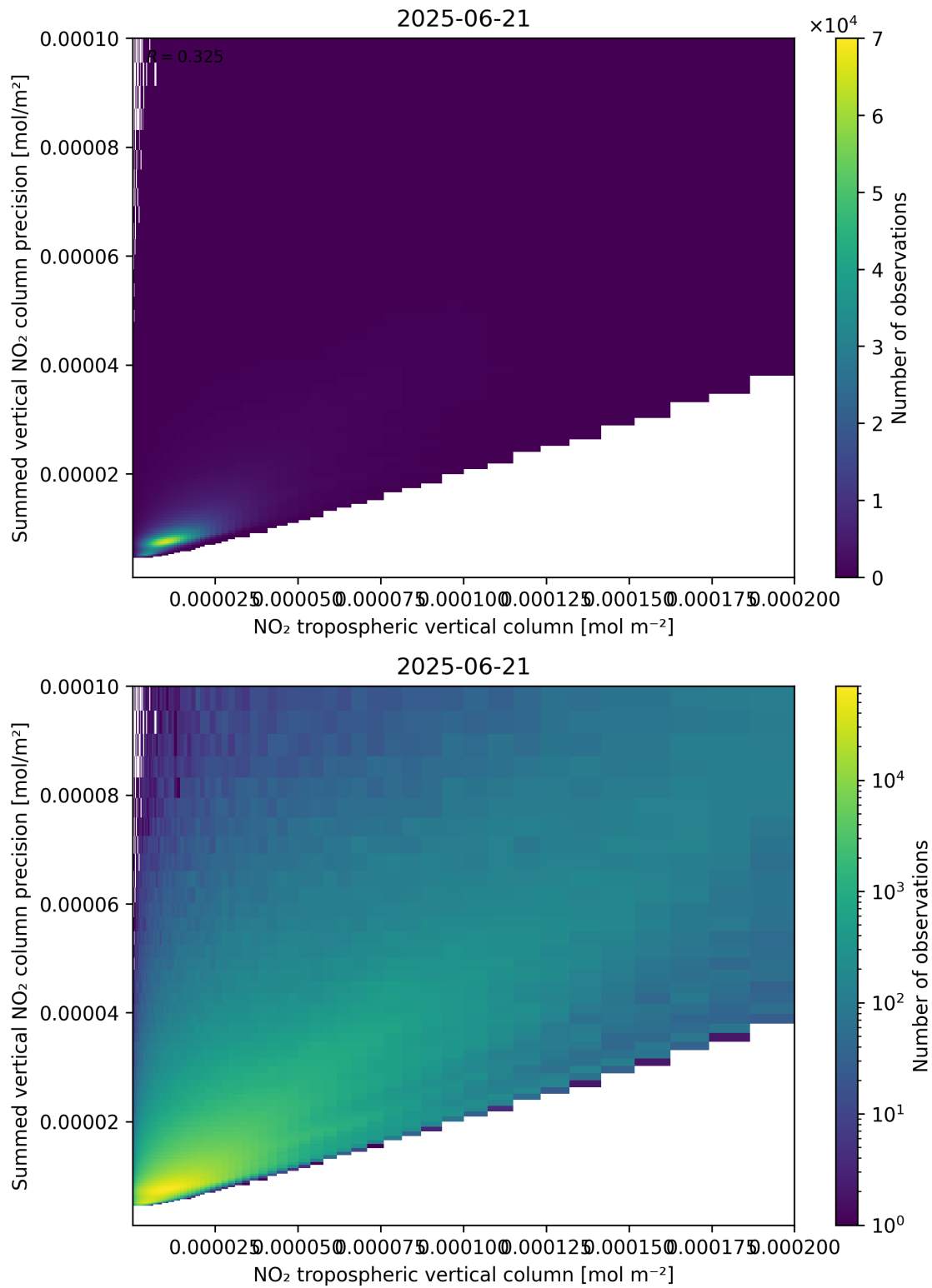
Figure 127: Scatter density plot of “NO 2 tropospheric vertical column” against “Summed vertical NO 2 column precision” for 2025-06-20 to 2025-06-22.
