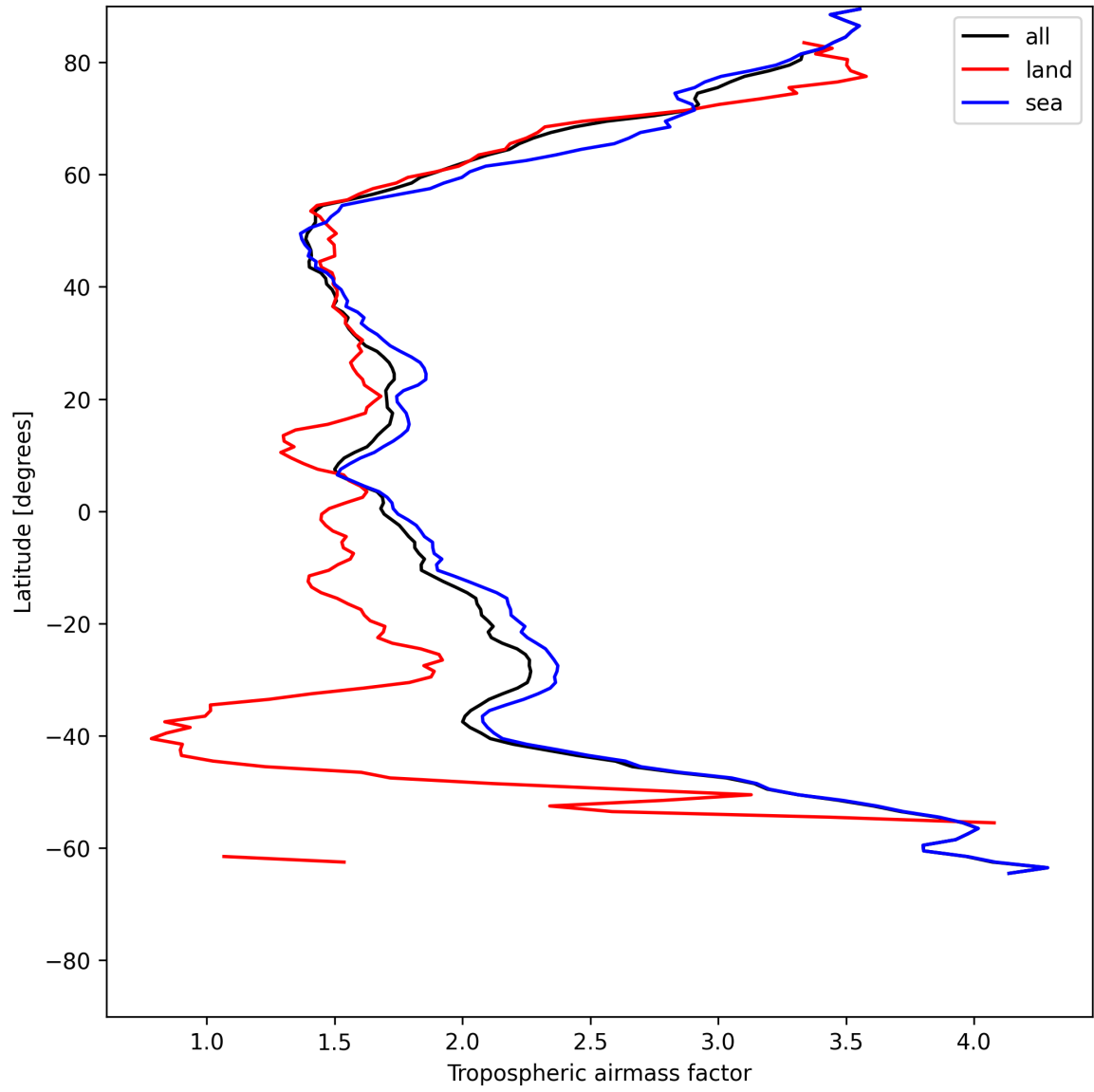
Figure 14: Zonal average of “Tropospheric air mass factor” for 2025-06-20 to 2025-06-22.
