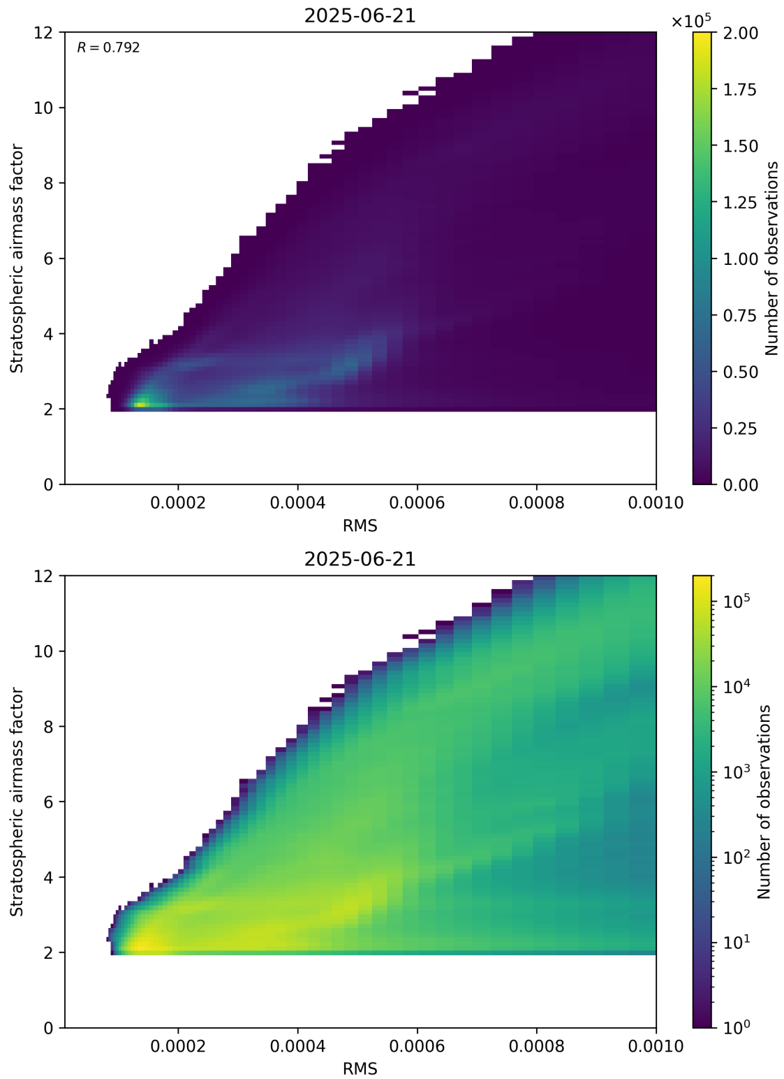
Figure 144: Scatter density plot of “RMS” against “Stratospheric airmass factor” for 2025-06-20 to 2025-06-22.
