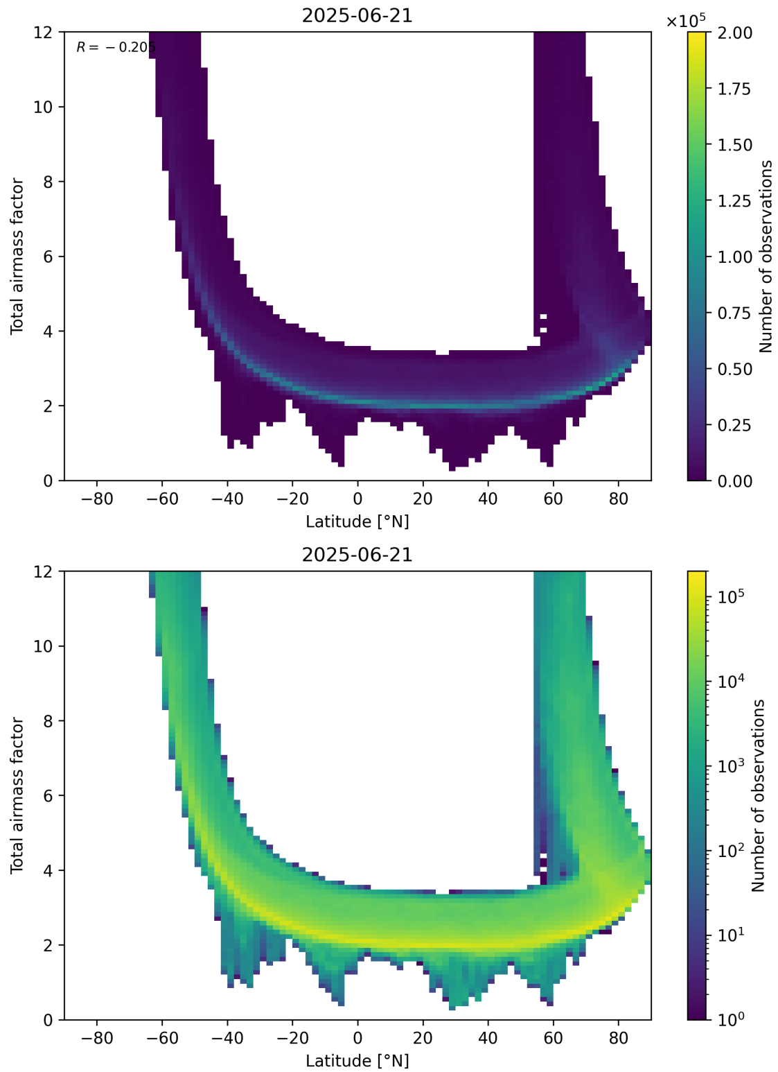
Figure 84: Scatter density plot of “Latitude” against “Total airmass factor” for 2025-06-20 to 2025-06-22.
