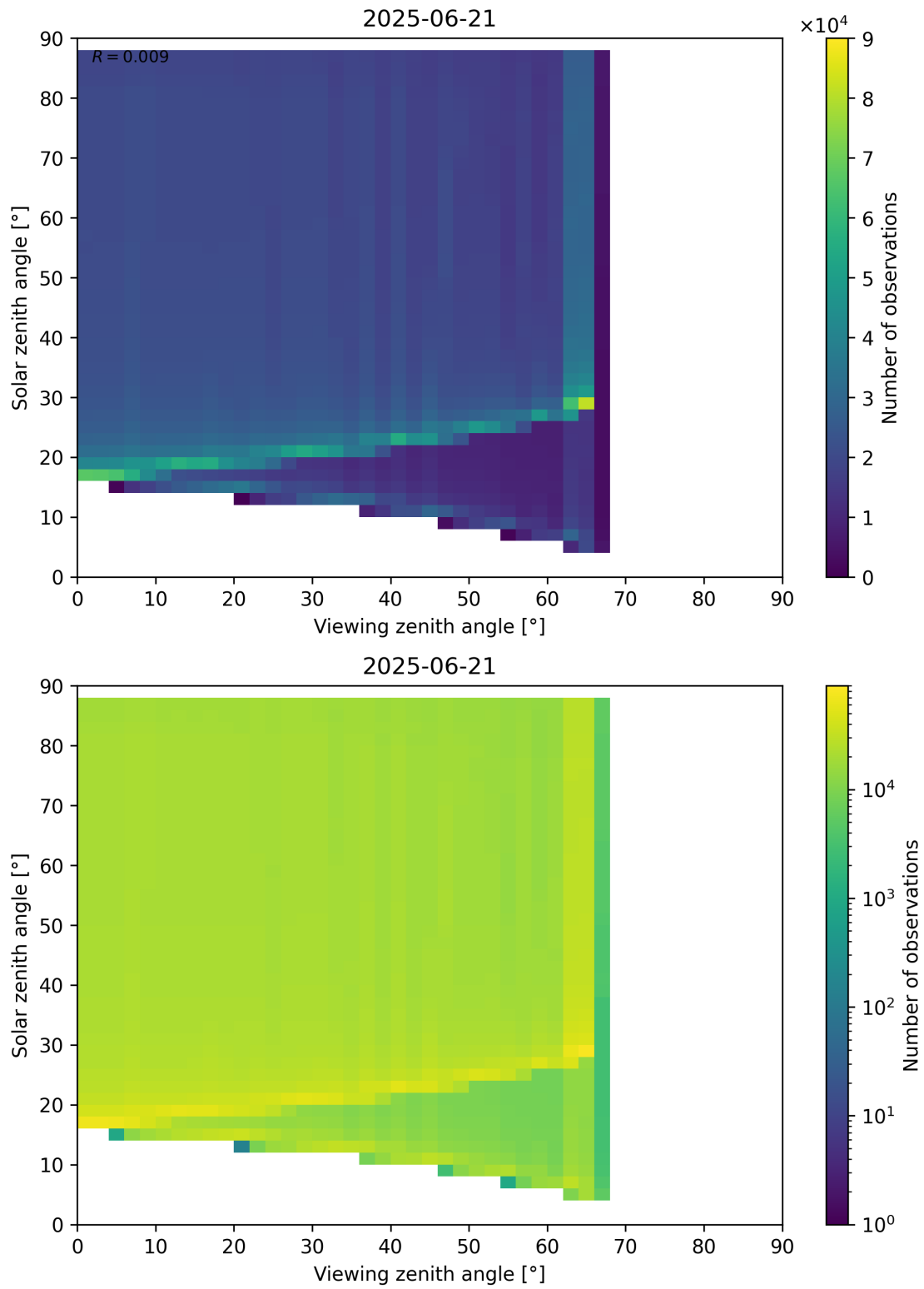
Figure 172: Scatter density plot of “Viewing zenith angle” against “Solar zenith angle” for 2025-06-20 to 2025-06-22.
