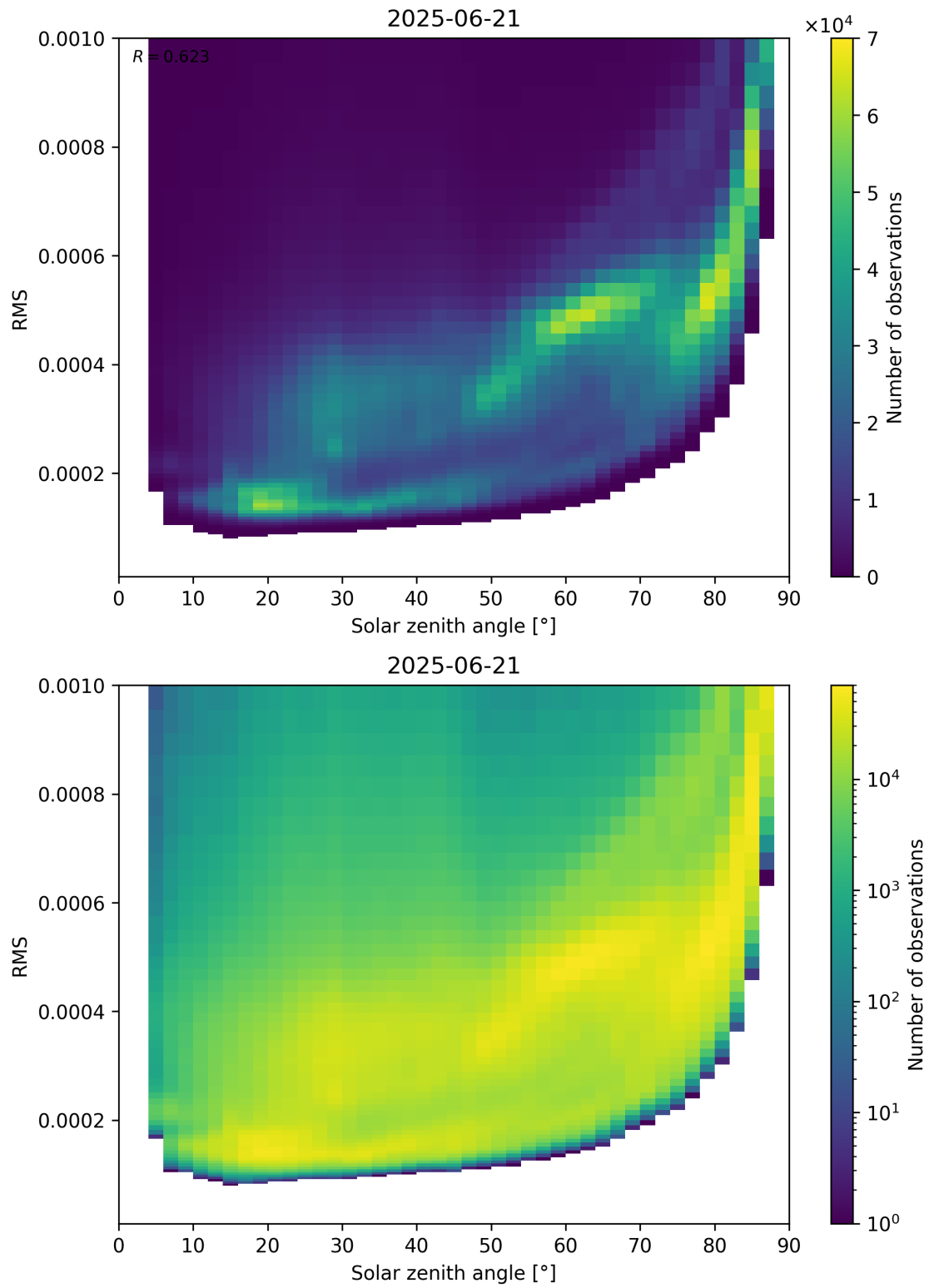
Figure 157: Scatter density plot of “Solar zenith angle” against “RMS” for 2025-06-20 to 2025-06-22.
