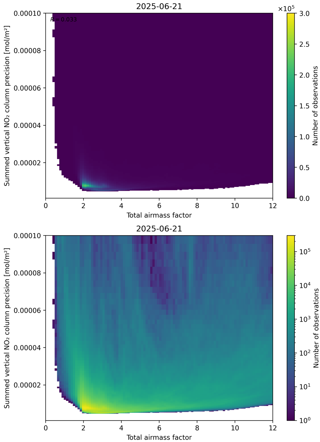
Figure 66: Scatter density plot of “Total airmass factor” against “Summed vertical NO 2 column precision” for 2025-06-20 to 2025-06-22.
