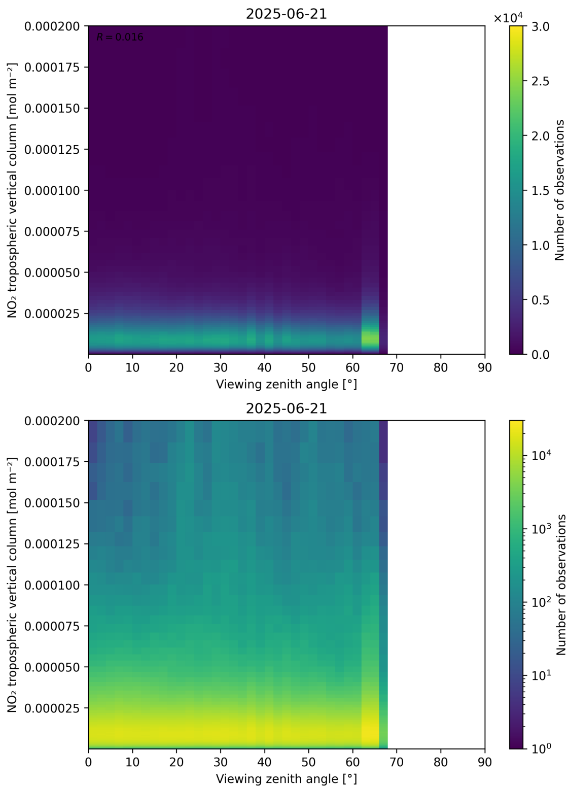
Figure 169: Scatter density plot of “Viewing zenith angle” against “NO 2 tropospheric vertical column” for 2025-06-20 to 2025-06-22.
