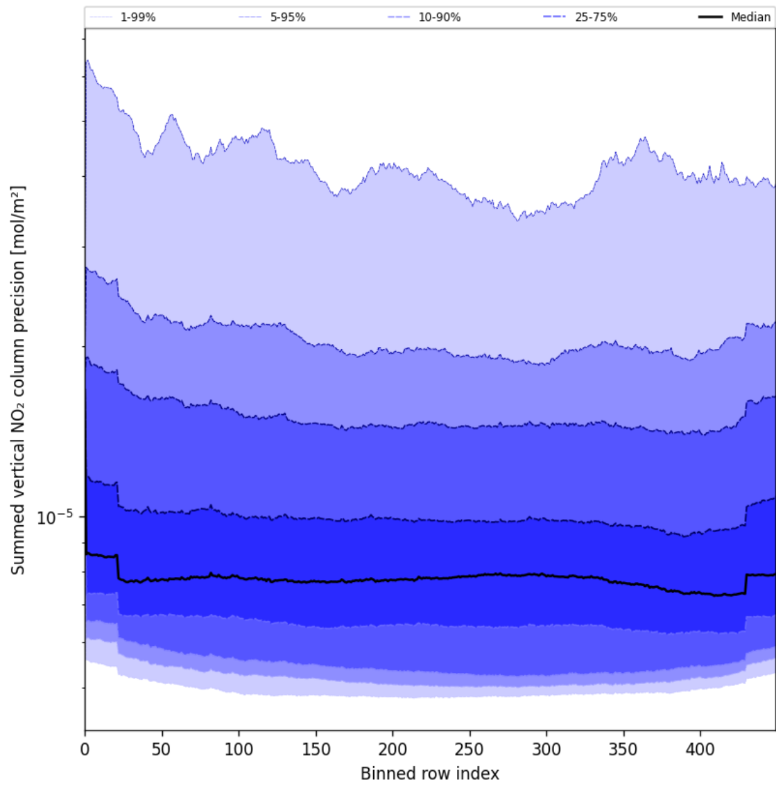
Figure 58: Along track statistics of “Summed vertical NO 2 column precision” for 2025-06-20 to 2025-06-22
