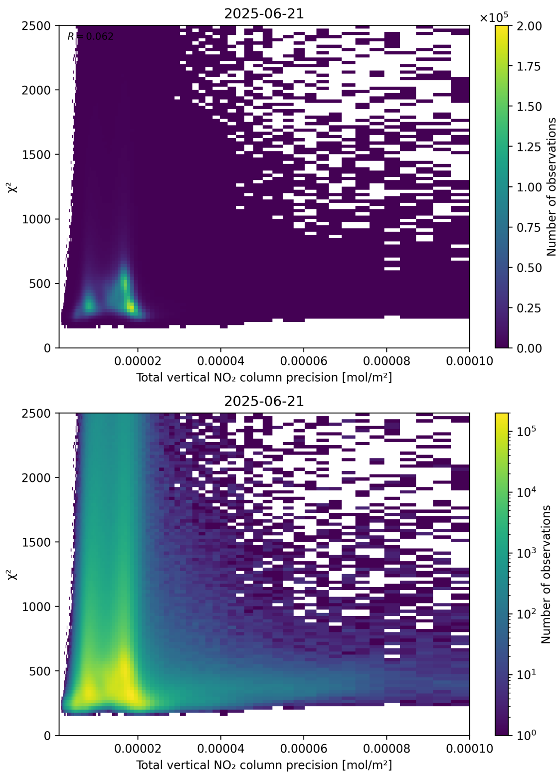
Figure 116: Scatter density plot of “Total vertical NO 2 column precision” against “ \chi^2 ” for 2025-06-20 to 2025-06-22.
