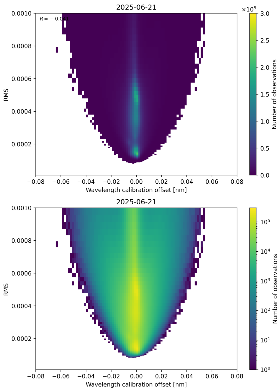
Figure 181: Scatter density plot of “Wavelength calibration offset” against “RMS” for 2025-06-20 to 2025-06-22.
