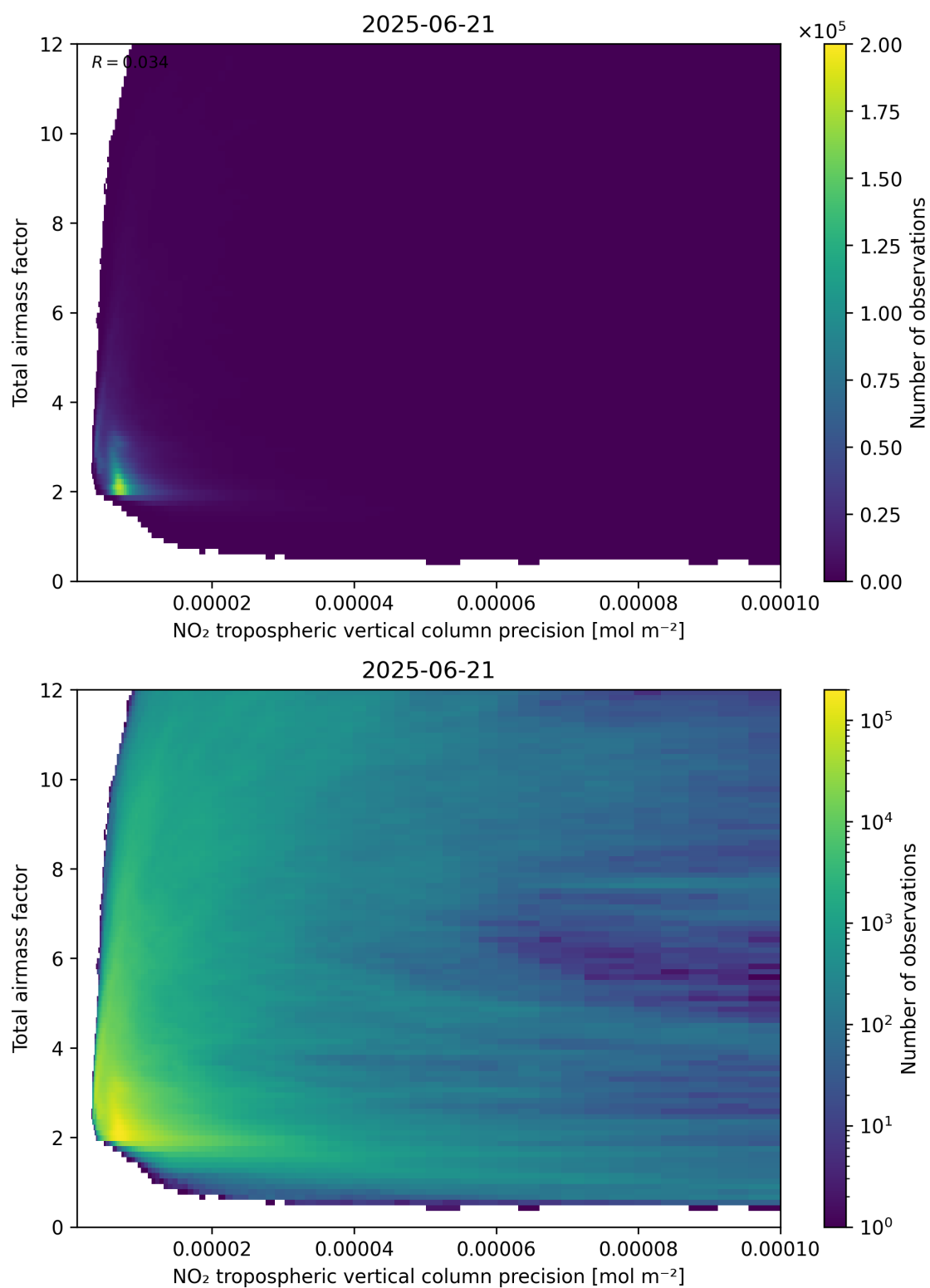
Figure 132: Scatter density plot of “NO 2 tropospheric vertical column precision” against “Total airmass factor” for 2025-06-20 to 2025-06-22.
