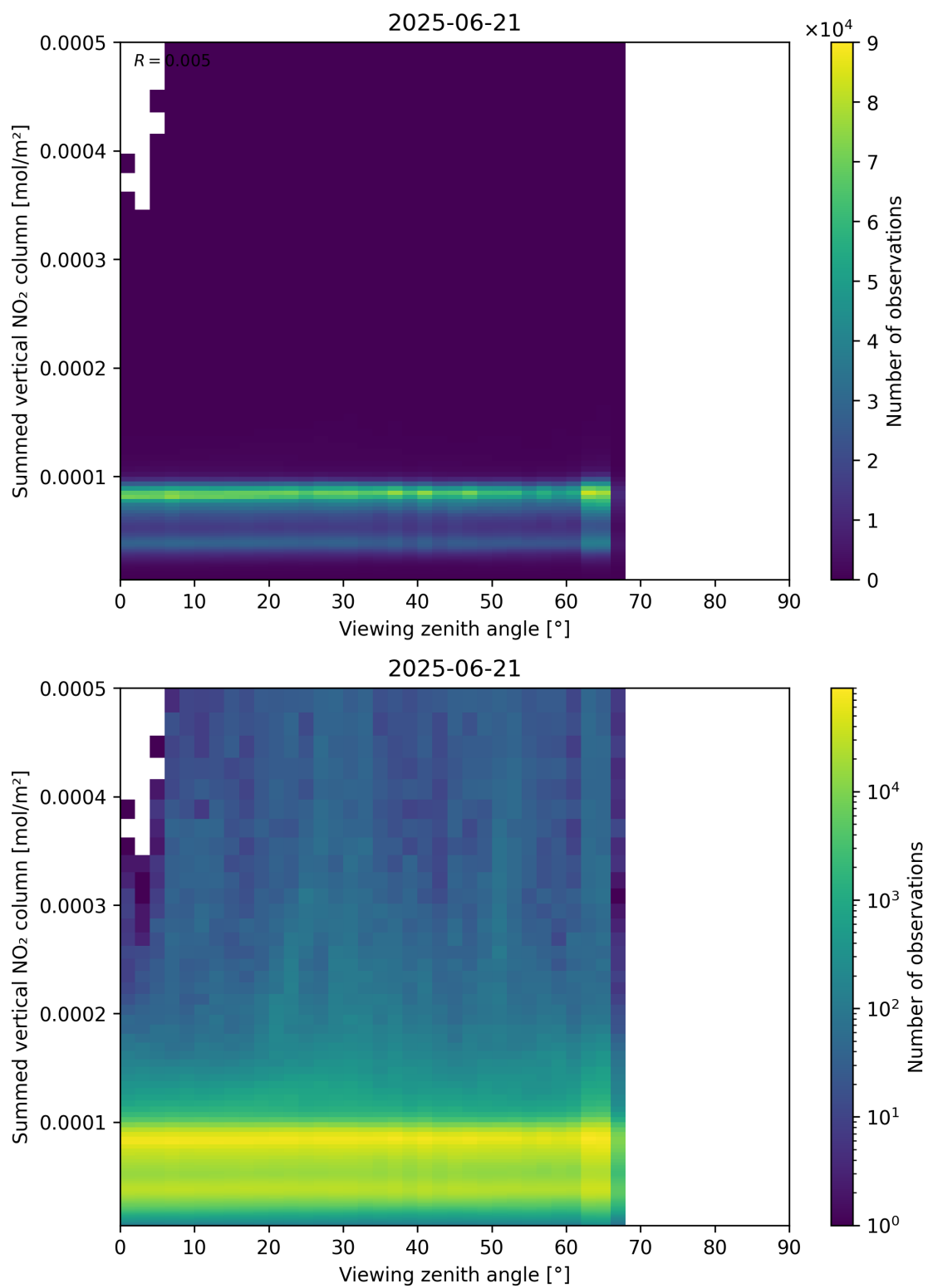
Figure 165: Scatter density plot of “Viewing zenith angle” against “Summed vertical NO 2 column” for 2025-06-20 to 2025-06-22.
