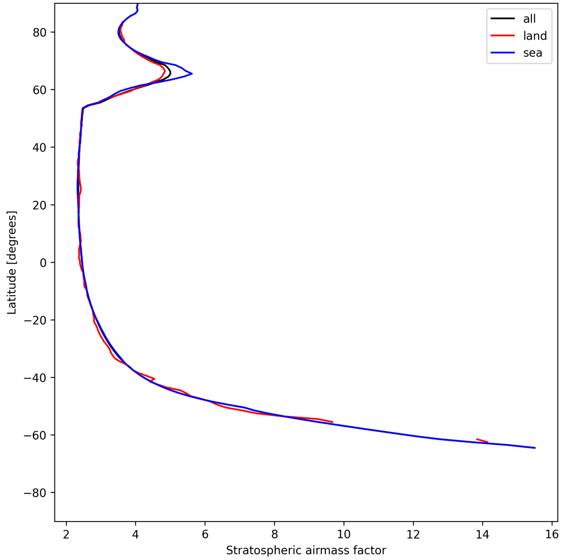
Figure 27: Zonal average of “Stratospheric airmass factor” for 2025-06-20 to 2025-06-22.
