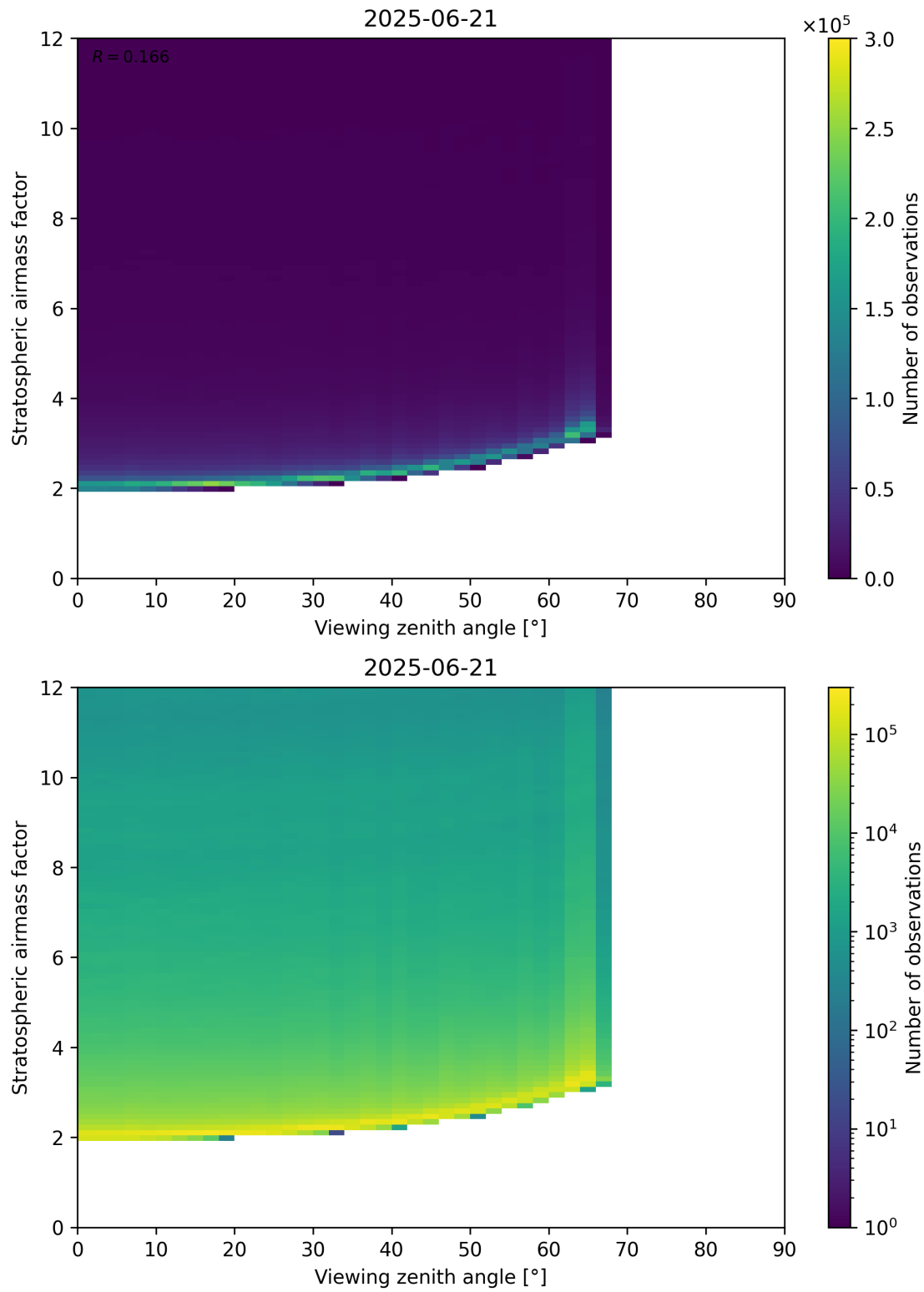
Figure 159: Scatter density plot of “Viewing zenith angle” against “Stratospheric airmass factor” for 2025-06-20 to 2025-06-22.
