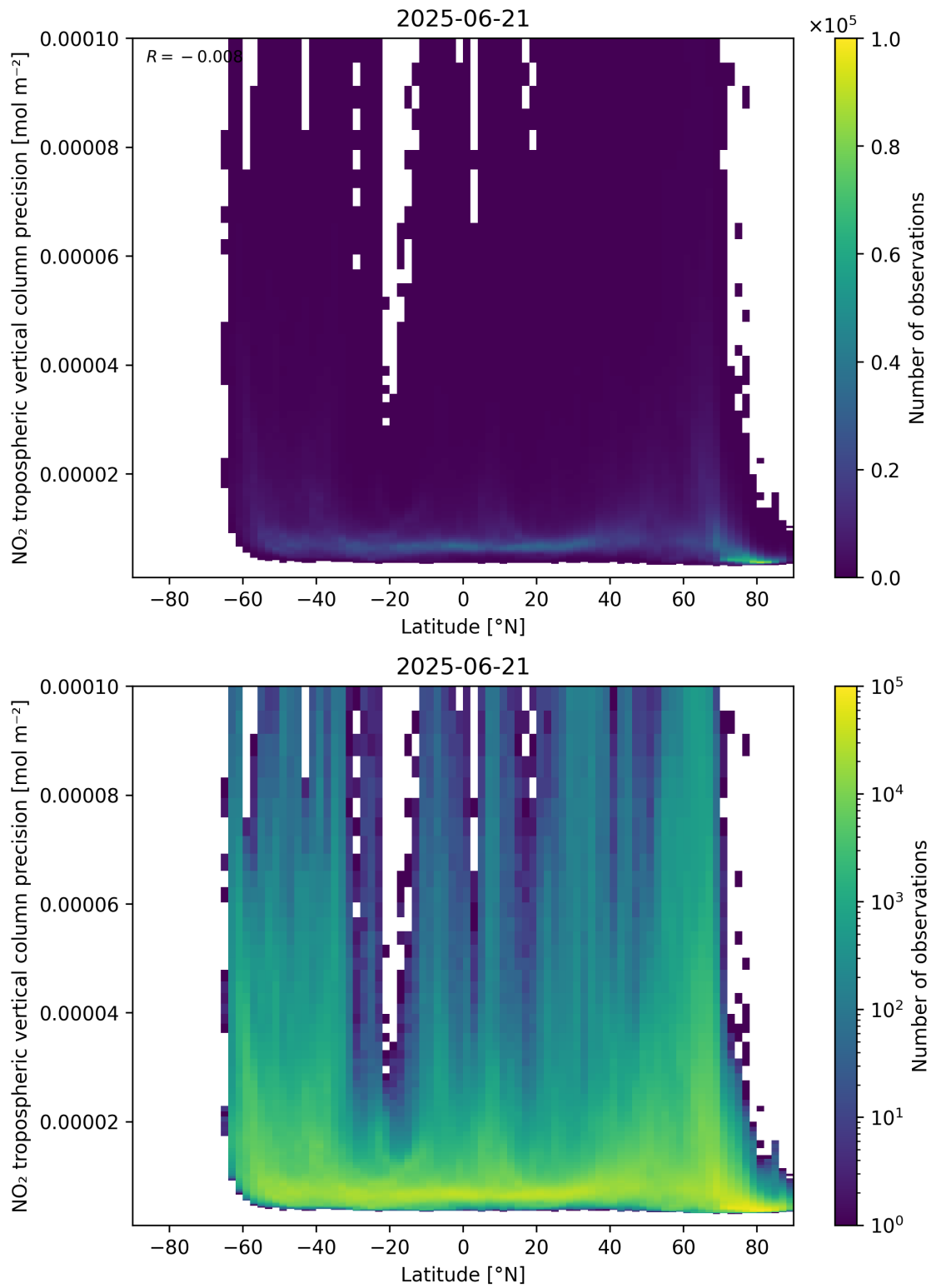
Figure 93: Scatter density plot of “Latitude” against “NO 2 tropospheric vertical column precision” for 2025-06-20 to 2025-06-22.
