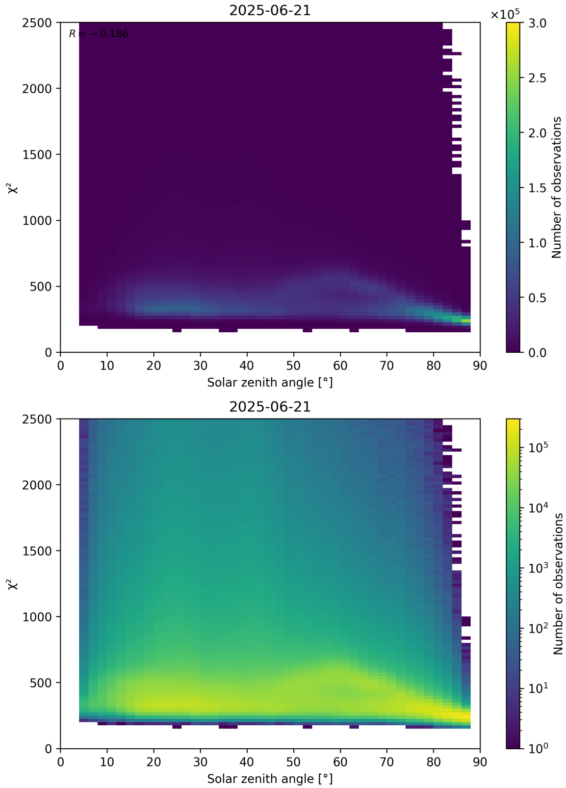
Figure 148: Scatter density plot of “Solar zenith angle” against “ \chi^2 ” for 2025-06-20 to 2025-06-22.
