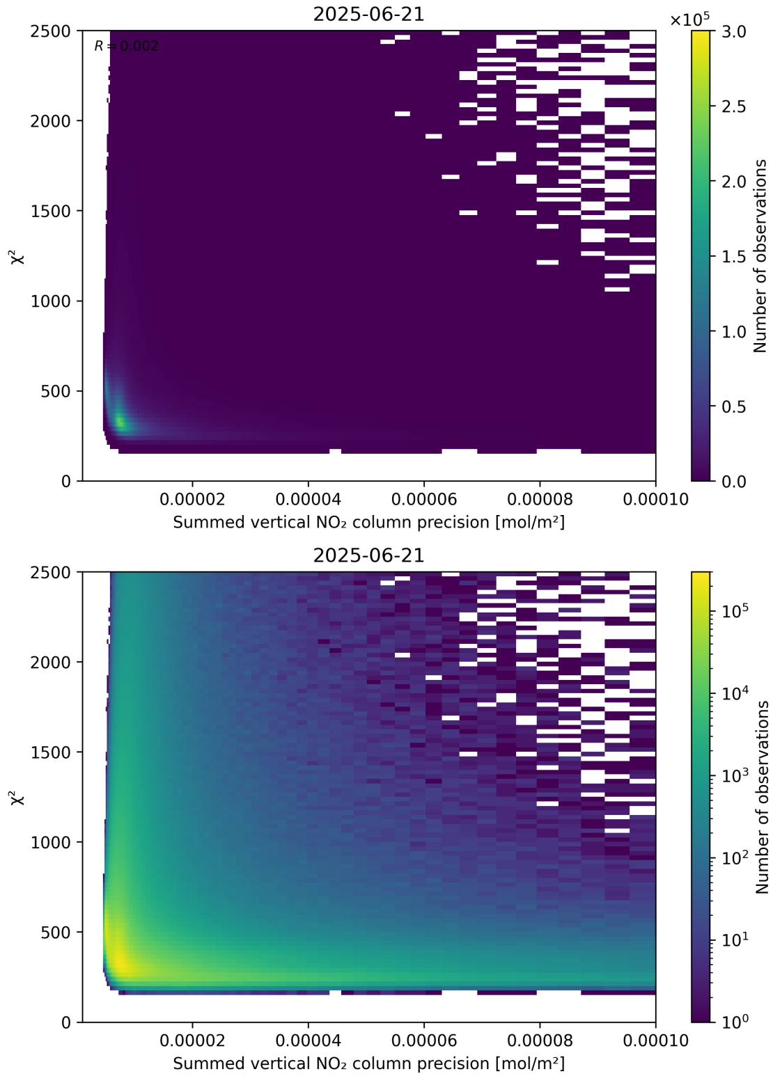
Figure 107: Scatter density plot of “Summed vertical NO 2 column precision” against “ \chi^2 ” for 2025-06-20 to 2025-06-22.
