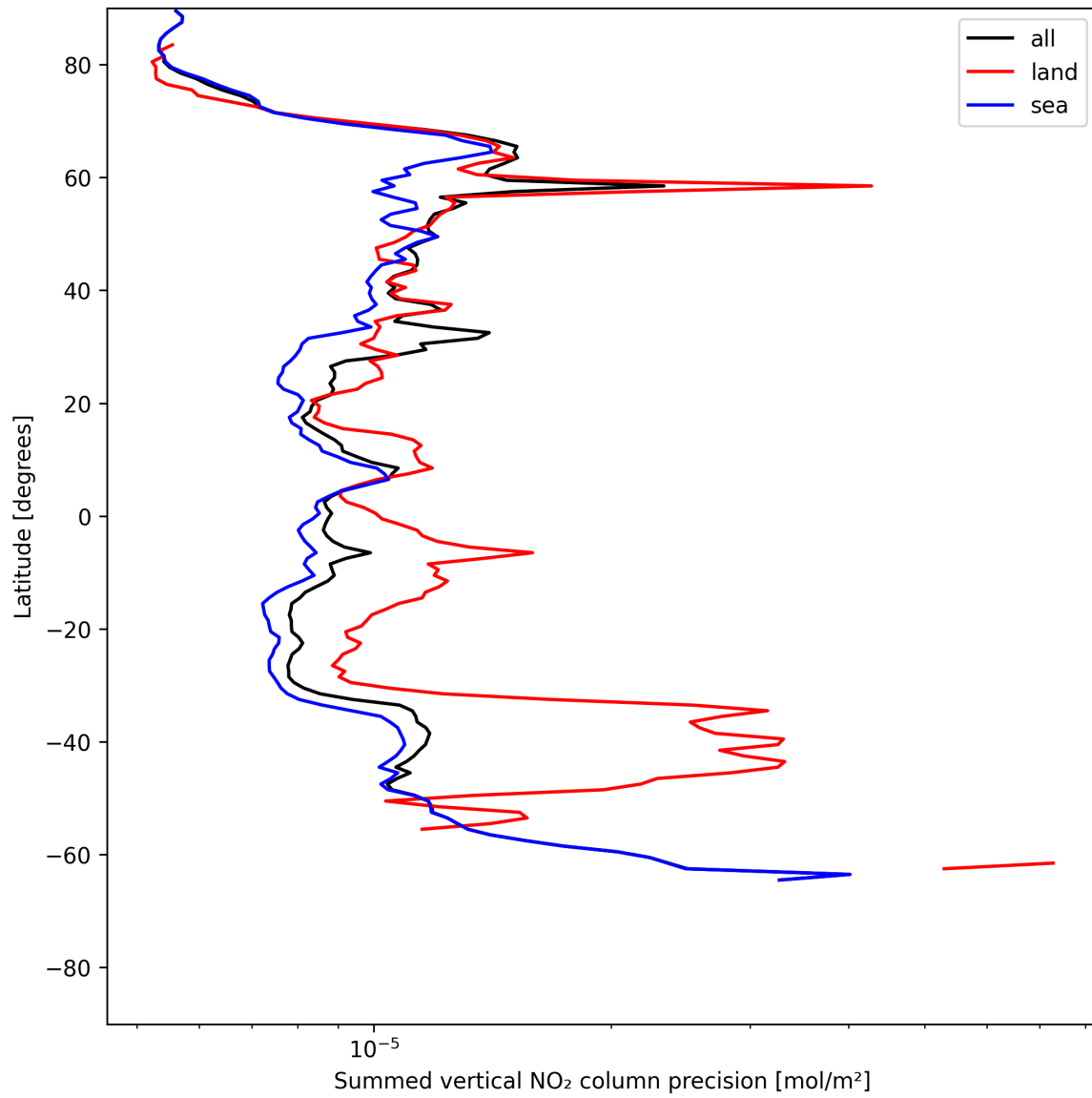
Figure 24: Zonal average of “Summed vertical NO 2 column precision” for 2025-06-20 to 2025-06-22.
