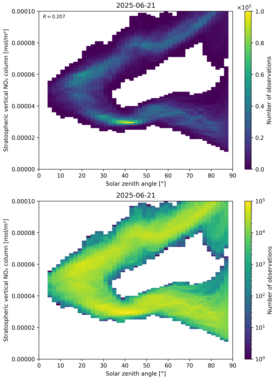
Figure 150: Scatter density plot of “Solar zenith angle” against “Stratospheric vertical NO 2 column” for 2025-06-20 to 2025-06-22.
