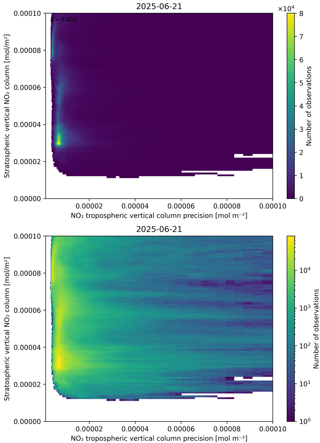
Figure 135: Scatter density plot of “NO 2 tropospheric vertical column precision” against “Stratospheric vertical NO 2 column” for 2025-06-20 to 2025-06-22.
