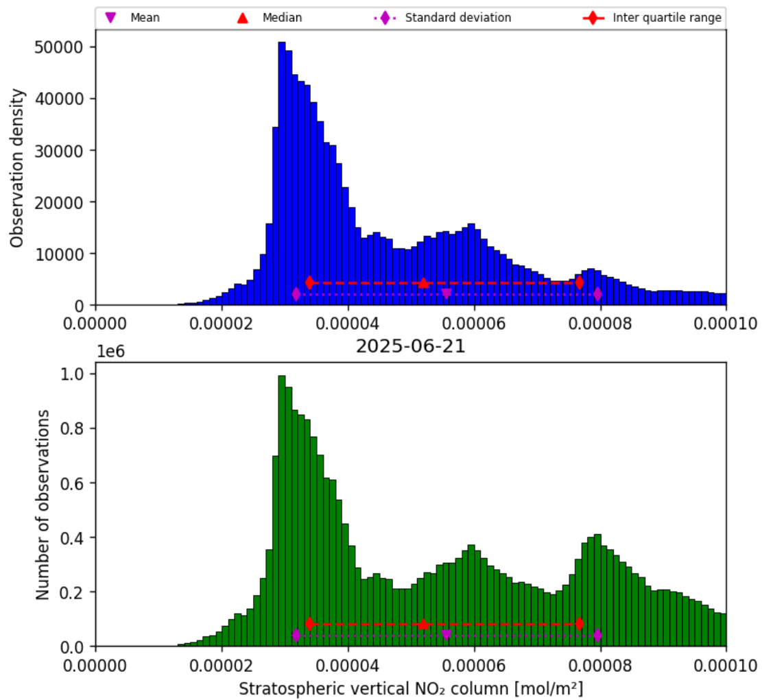
Figure 36: Histogram of “Stratospheric vertical NO 2 column” for 2025-06-20 to 2025-06-22
