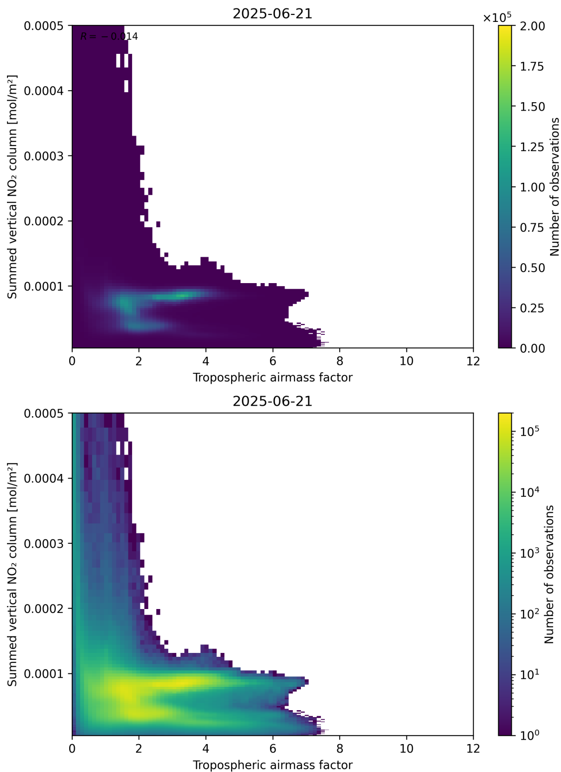
Figure 75: Scatter density plot of “Tropospheric air mass factor” against “Summed vertical NO 2 column” for 2025-06-20 to 2025-06-22.
