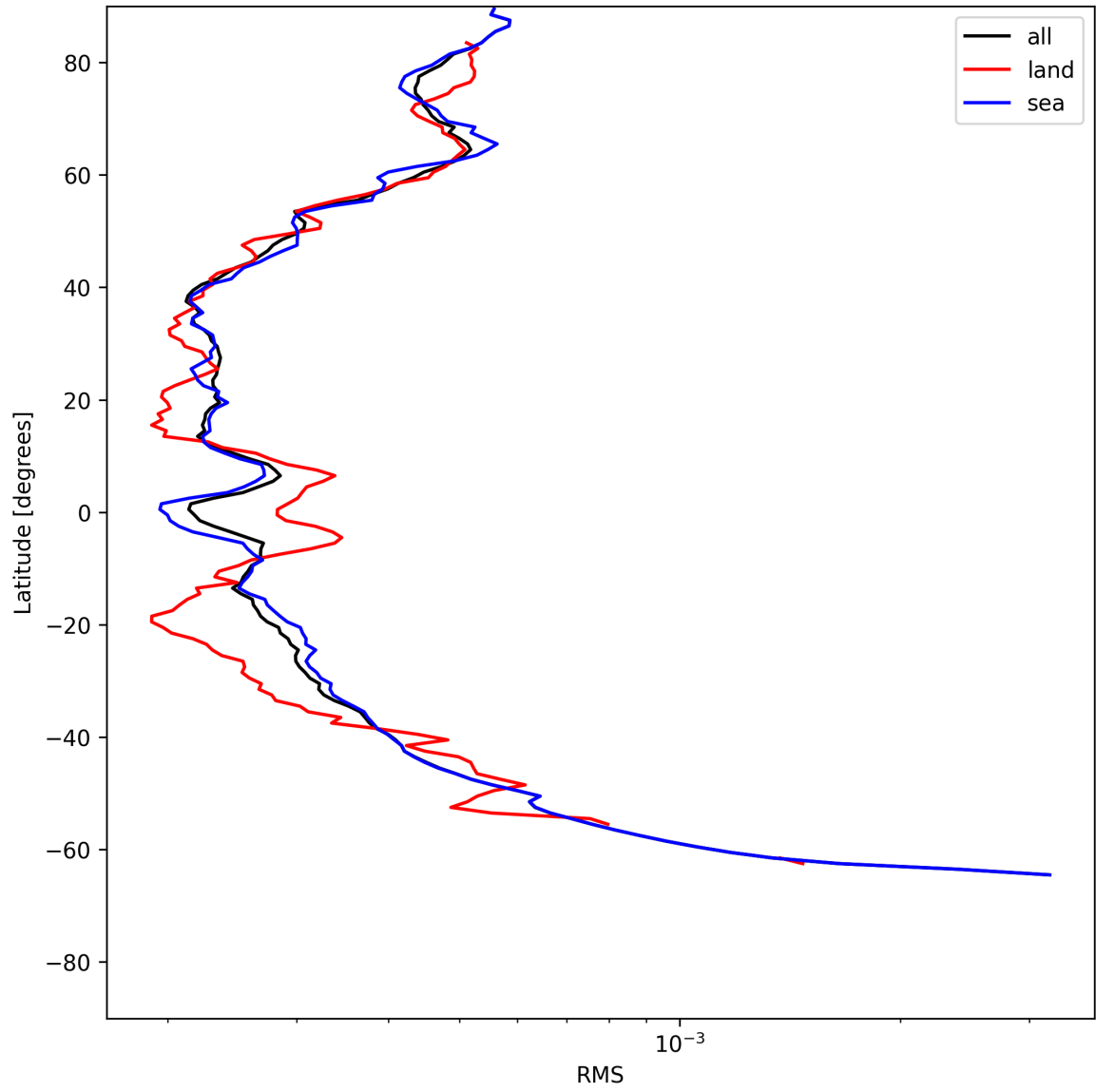
Figure 26: Zonal average of “RMS” for 2025-06-20 to 2025-06-22.
