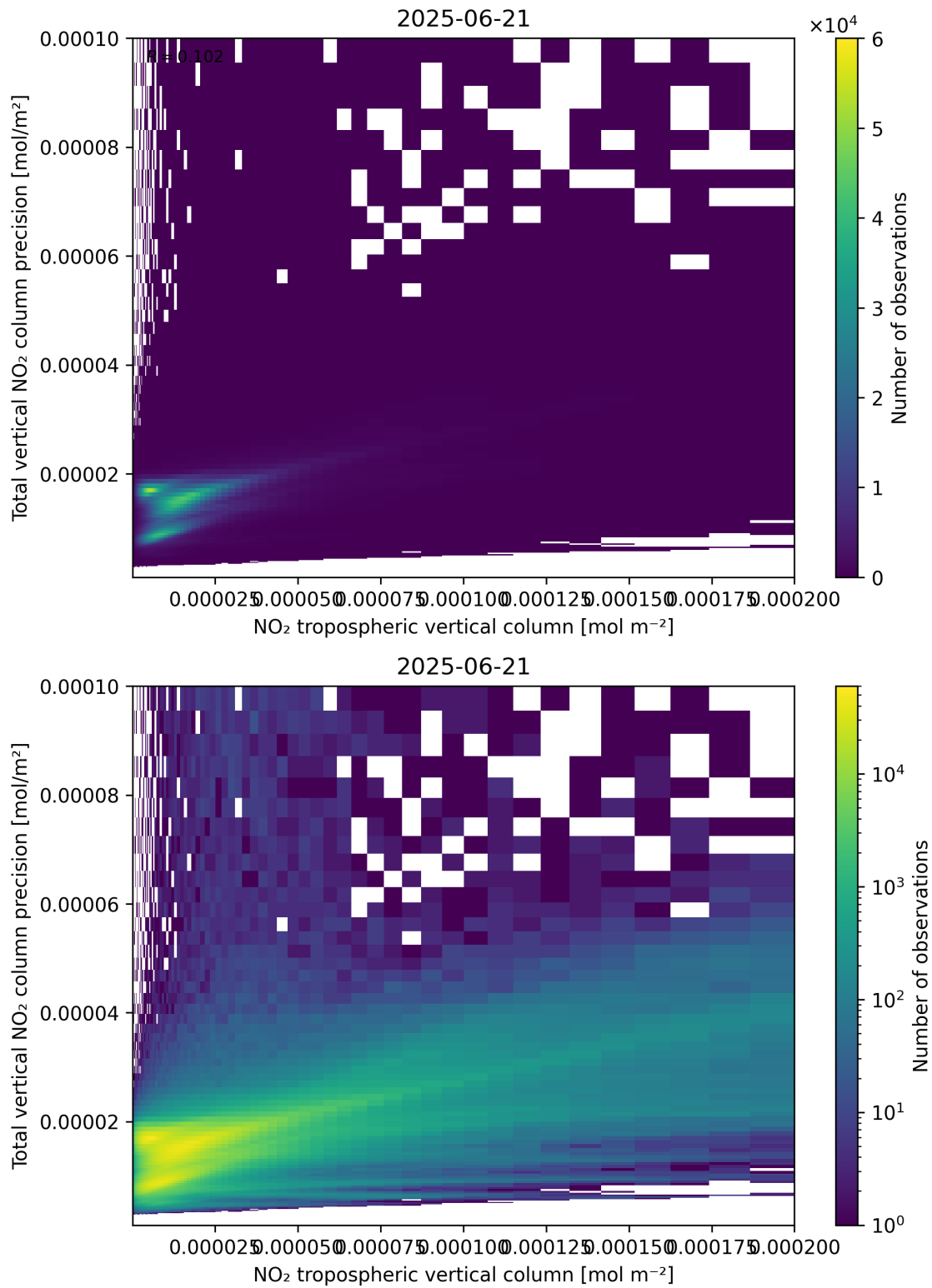
Figure 129: Scatter density plot of “NO 2 tropospheric vertical column” against “Total vertical NO 2 column precision” for 2025-06-20 to 2025-06-22.
