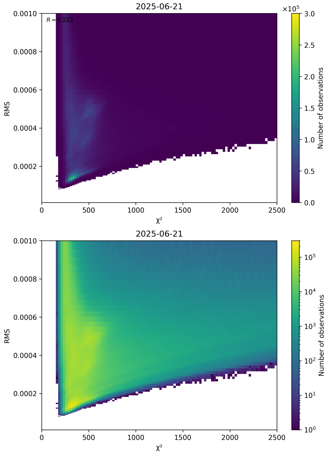
Figure 82: Scatter density plot of “ \chi^2 ” against “RMS” for 2025-06-20 to 2025-06-22.
