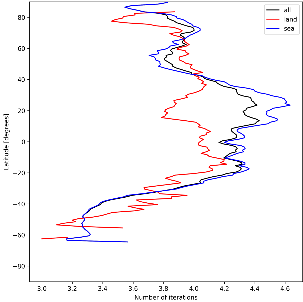
Figure 17: Zonal average of “Number of iterations” for 2025-06-20 to 2025-06-22.
