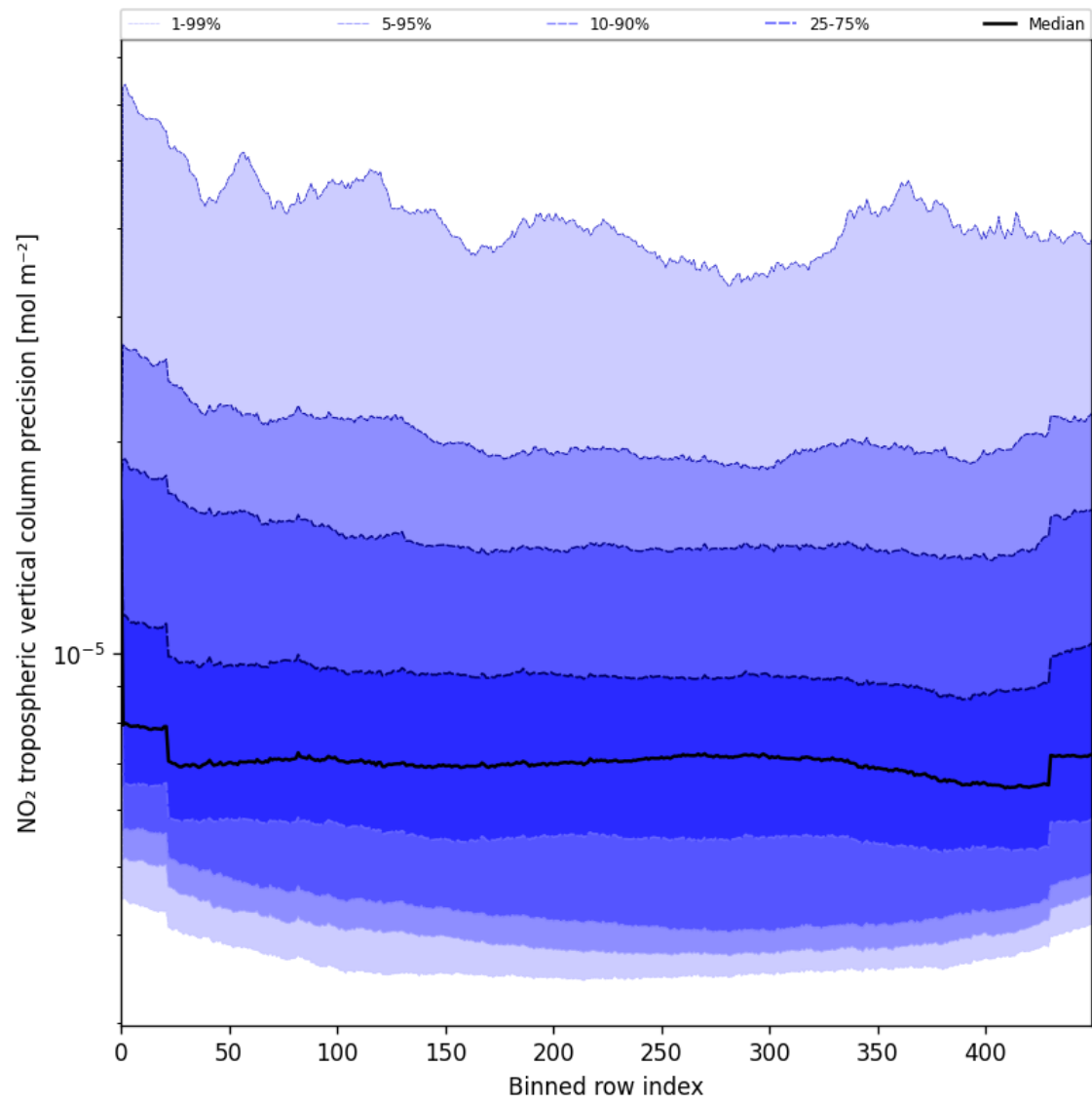
Figure 47: Along track statistics of “NO 2 tropospheric vertical column precision” for 2025-06-20 to 2025-06-22
