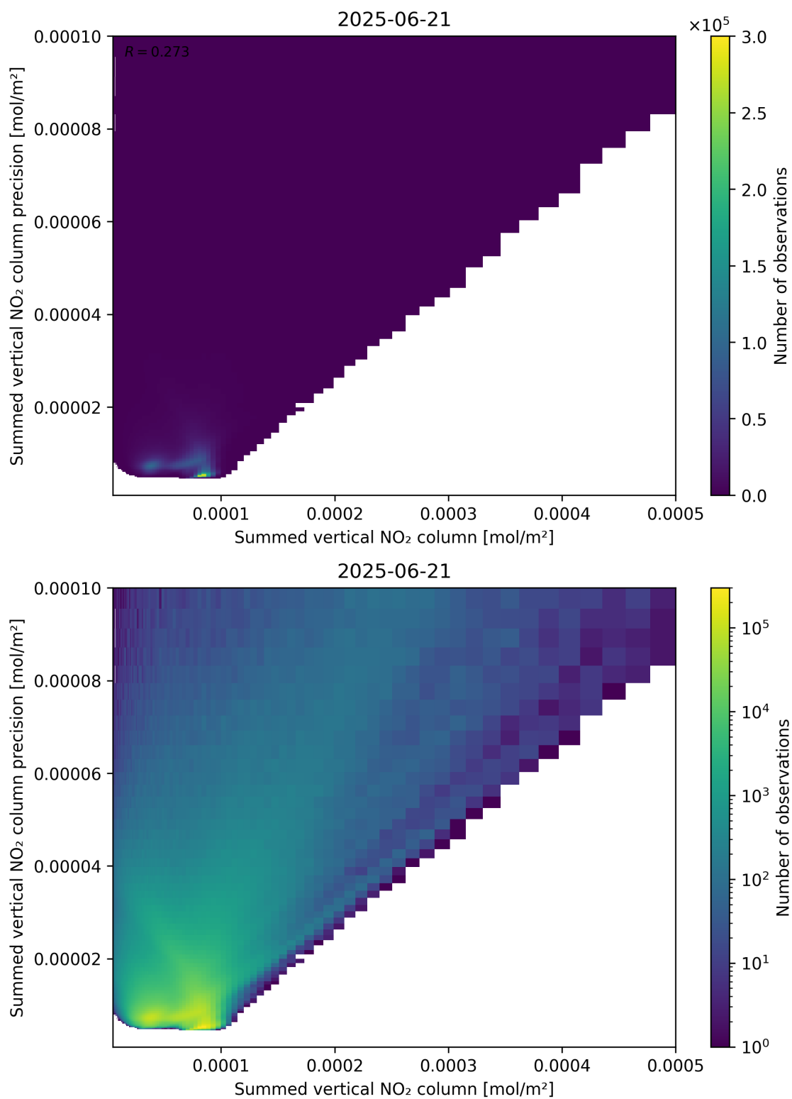
Figure 105: Scatter density plot of “Summed vertical NO 2 column” against “Summed vertical NO 2 column precision” for 2025-06-20 to 2025-06-22.
