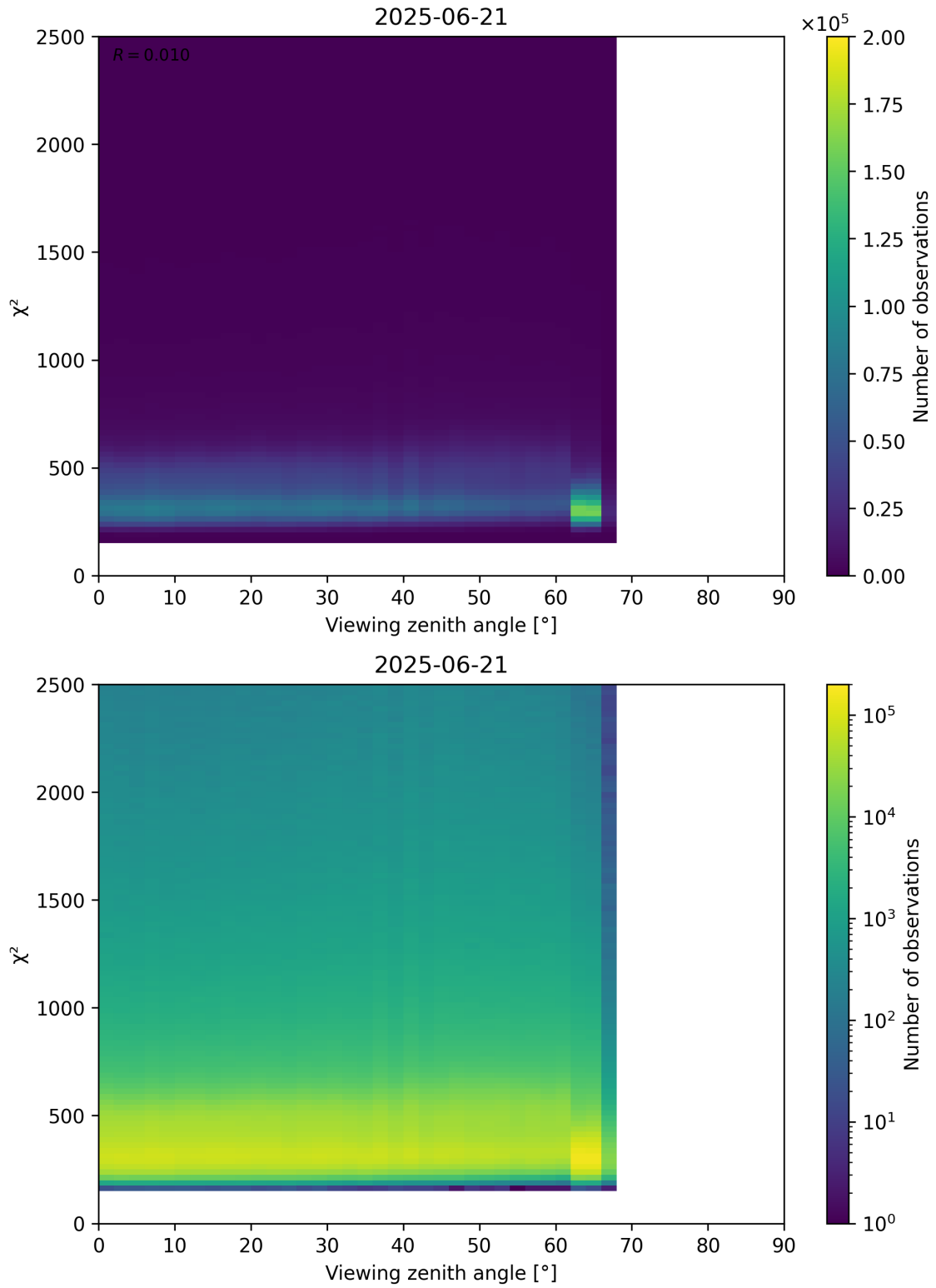
Figure 162: Scatter density plot of “Viewing zenith angle” against “ \chi^2 ” for 2025-06-20 to 2025-06-22.
