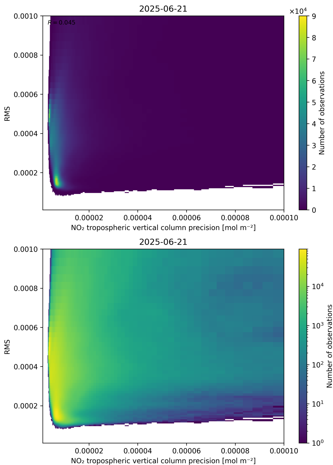
Figure 140: Scatter density plot of “NO 2 tropospheric vertical column precision” against “RMS” for 2025-06-20 to 2025-06-22.
