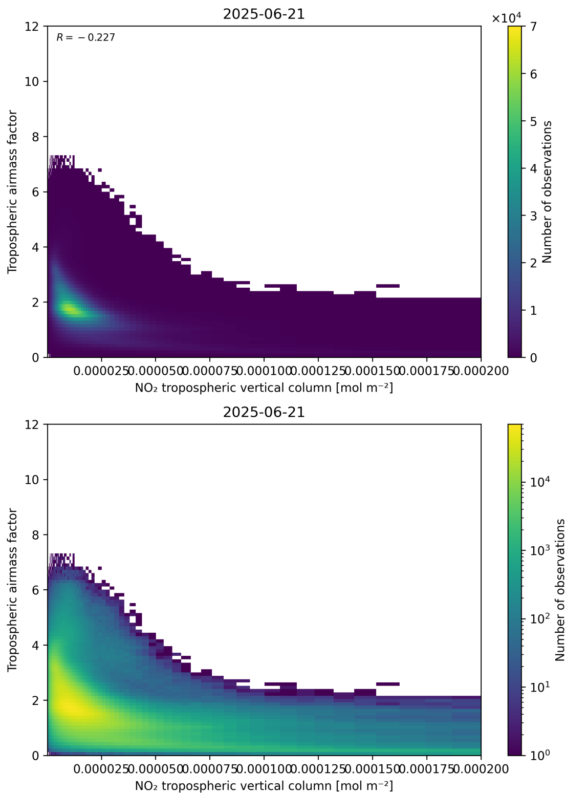
Figure 123: Scatter density plot of “NO 2 tropospheric vertical column” against “Tropospheric air mass factor” for 2025-06-20 to 2025-06-22.
