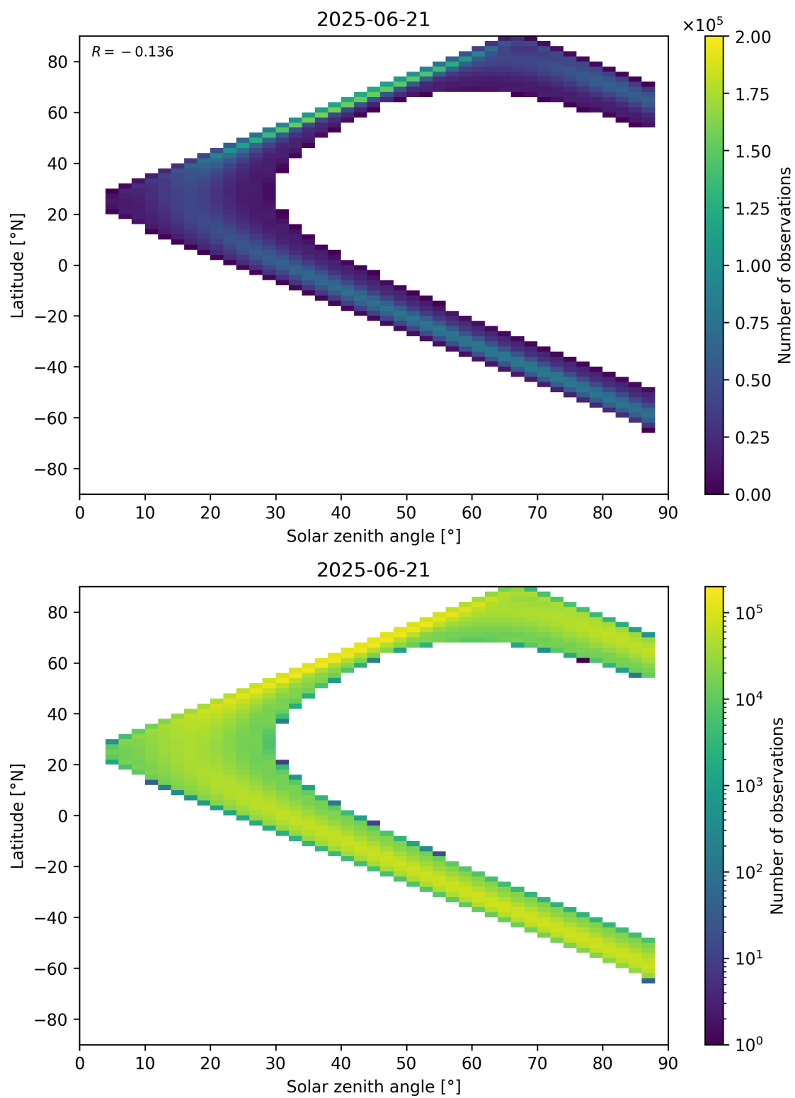
Figure 149: Scatter density plot of “Solar zenith angle” against “Latitude” for 2025-06-20 to 2025-06-22.
