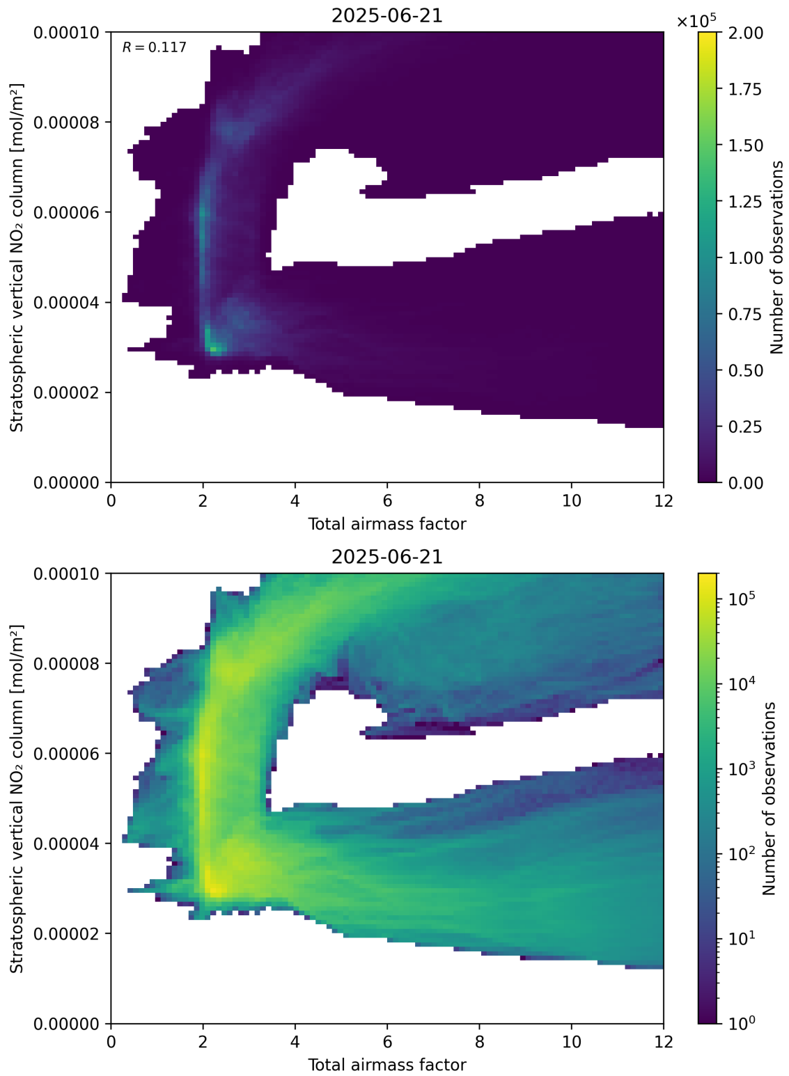
Figure 64: Scatter density plot of “Total airmass factor” against “Stratospheric vertical NO 2 column” for 2025-06-20 to 2025-06-22.
