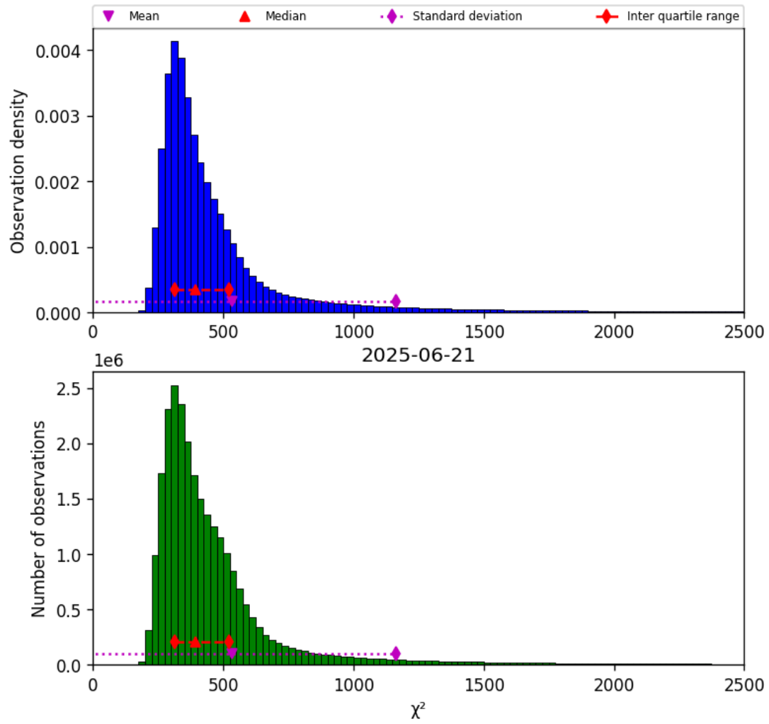
Figure 42: Histogram of “ \chi^2 ” for 2025-06-20 to 2025-06-22
