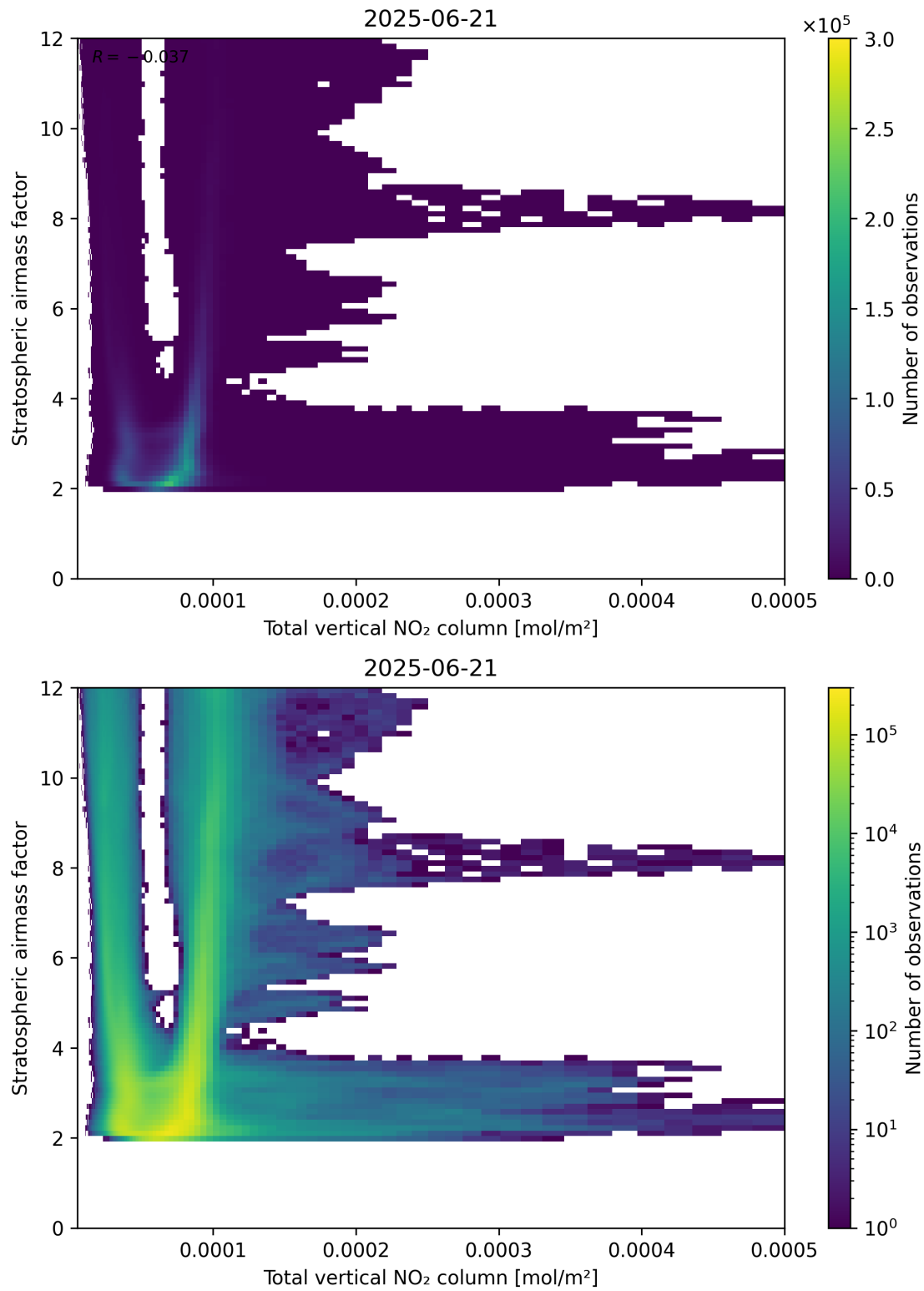
Figure 110: Scatter density plot of “Total vertical NO 2 column” against “Stratospheric air mass factor” for 2025-06-20 to 2025-06-22.
