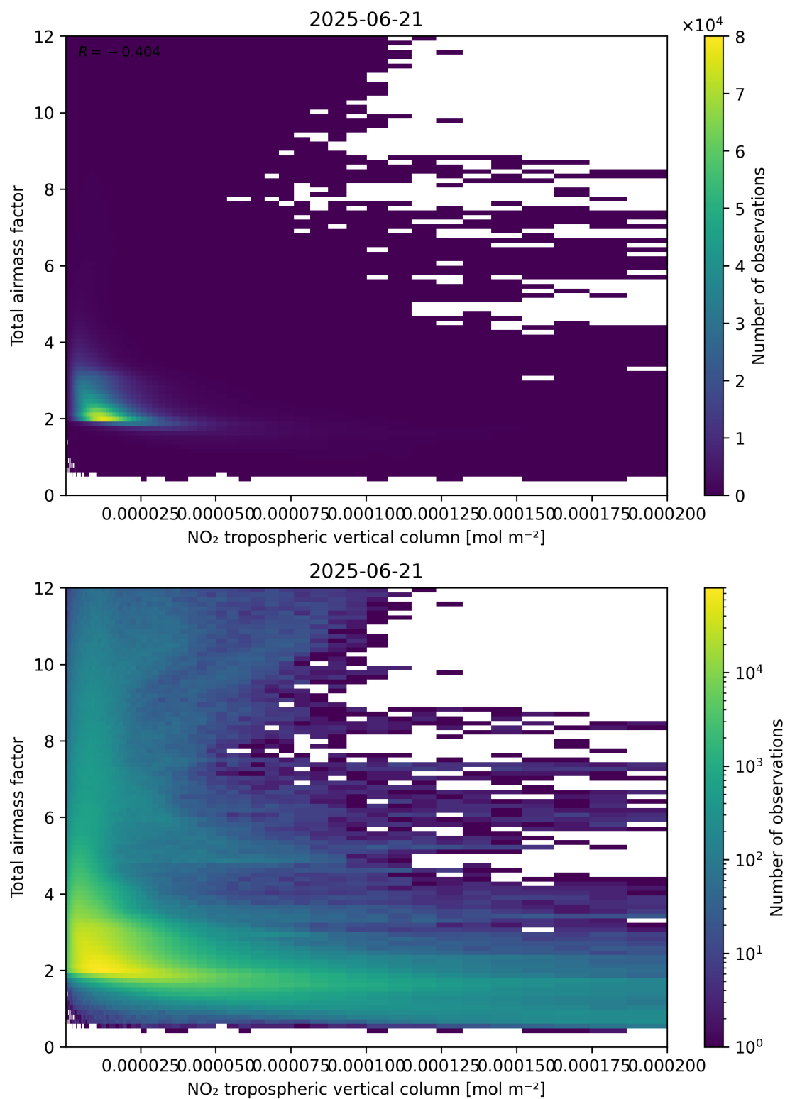
Figure 122: Scatter density plot of “NO 2 tropospheric vertical column” against “Total airmass factor” for 2025-06-20 to 2025-06-22.
