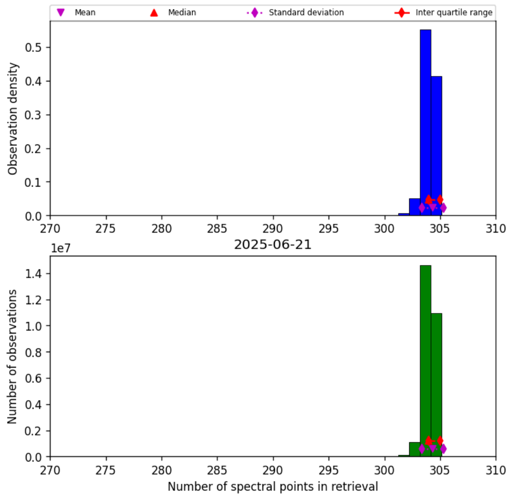
Figure 33: Histogram of “Number of spectral points in retrieval” for 2025-06-20 to 2025-06-22
