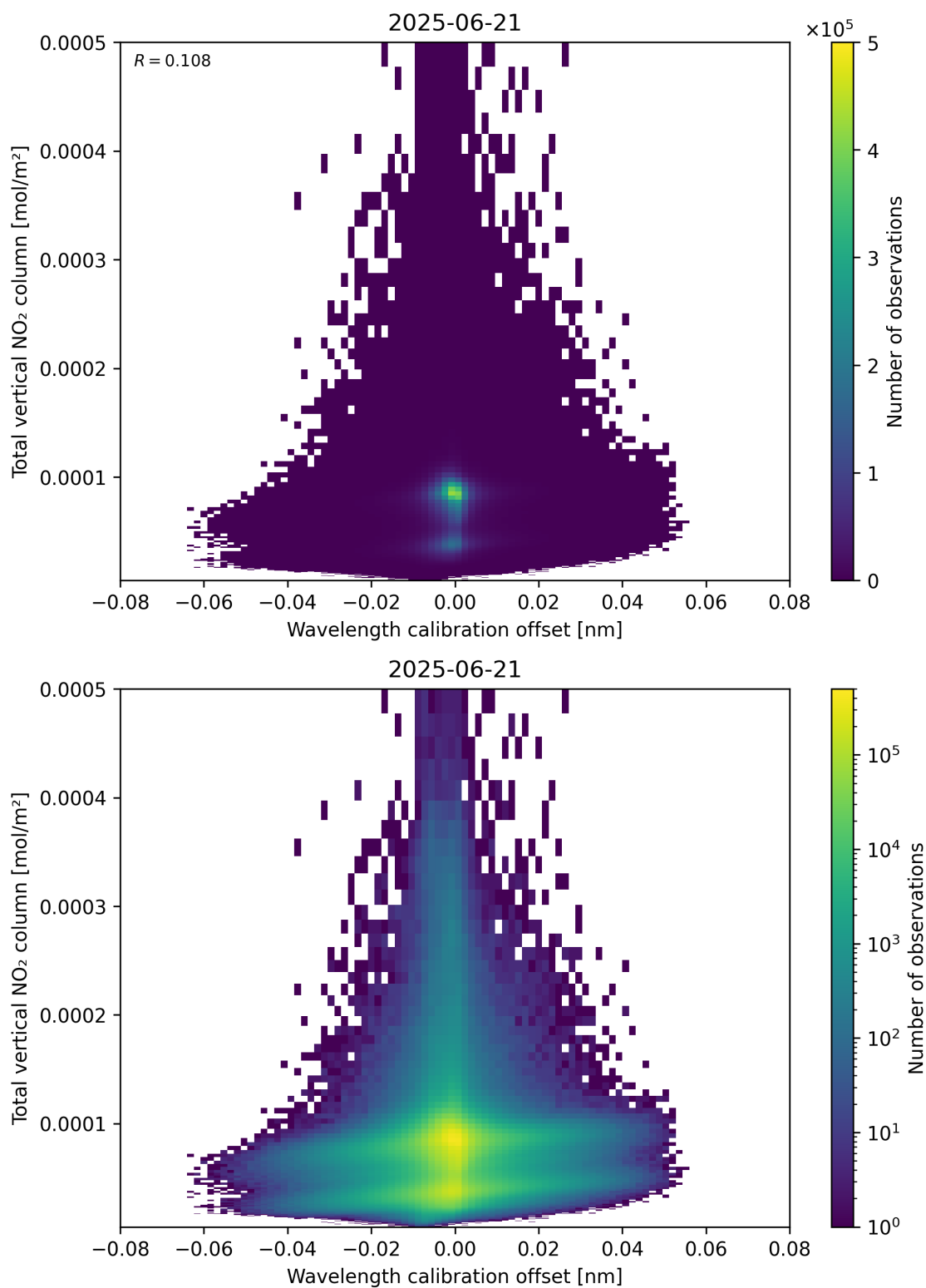
Figure 179: Scatter density plot of “Wavelength calibration offset” against “Total vertical NO 2 column” for 2025-06-20 to 2025-06-22.
