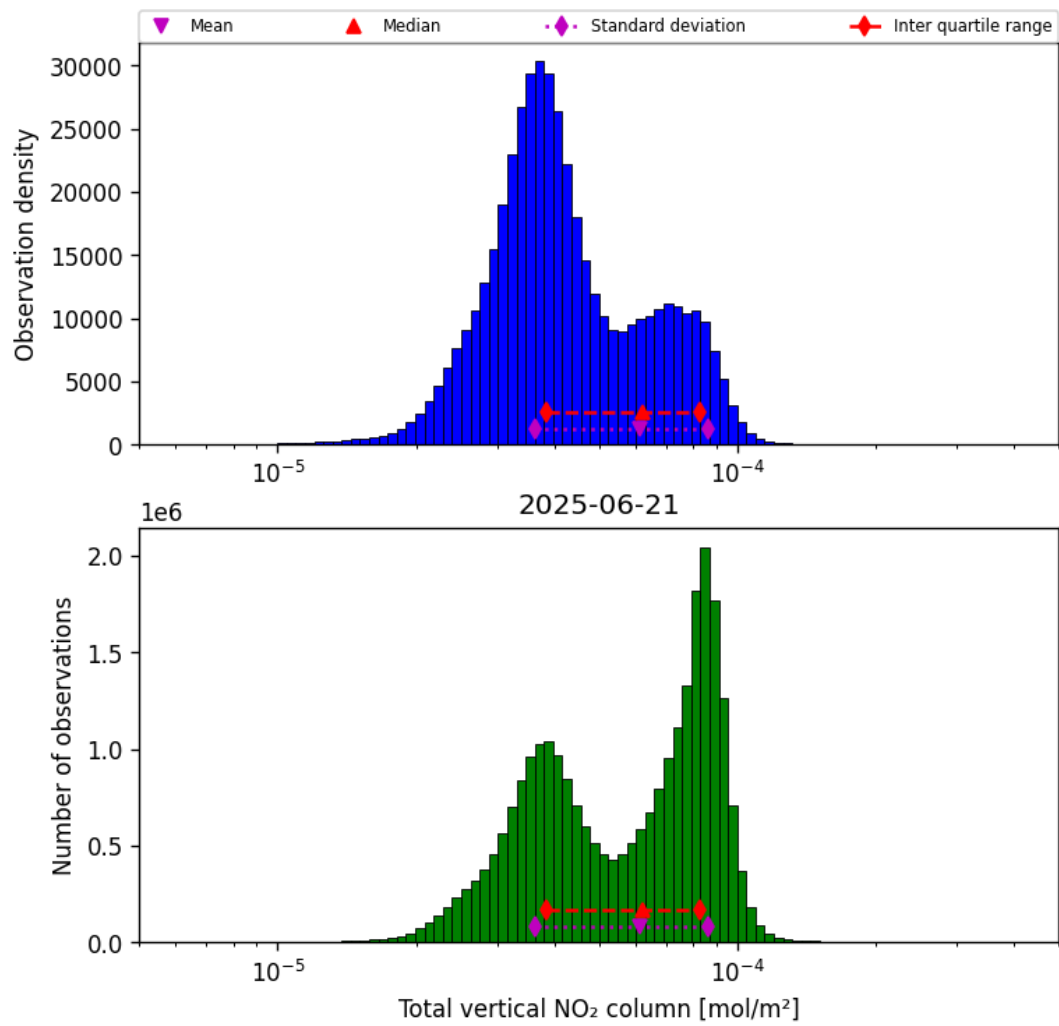
Figure 38: Histogram of “Total vertical NO 2 column” for 2025-06-20 to 2025-06-22
