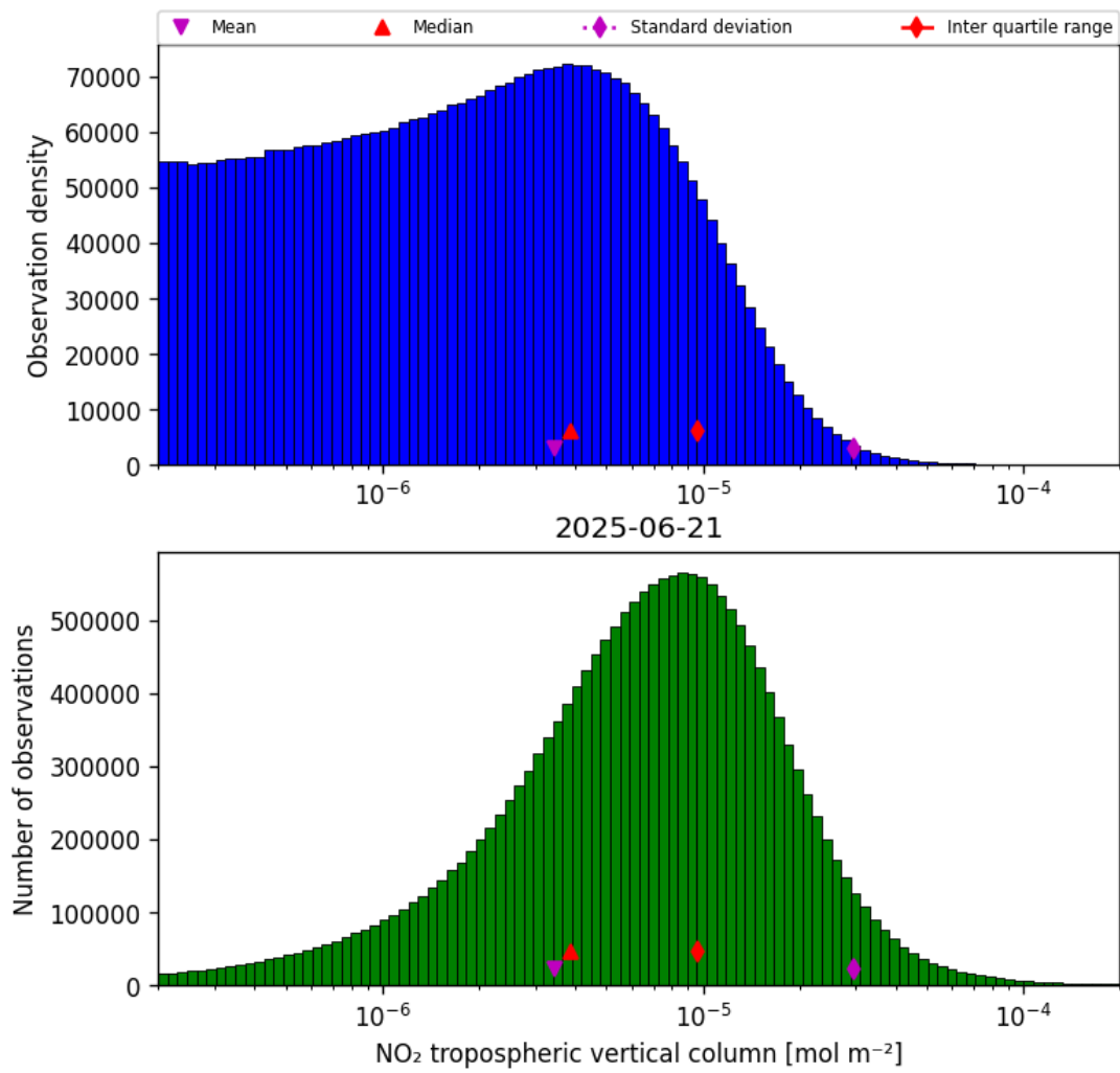
Figure 29: Histogram of “NO 2 tropospheric vertical column” for 2025-06-20 to 2025-06-22
