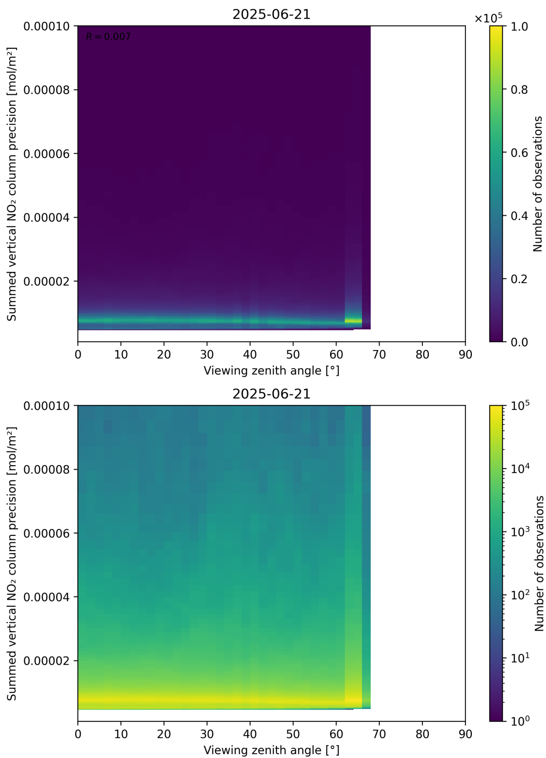
Figure 166: Scatter density plot of “Viewing zenith angle” against “Summed vertical NO 2 column precision” for 2025-06-20 to 2025-06-22.
