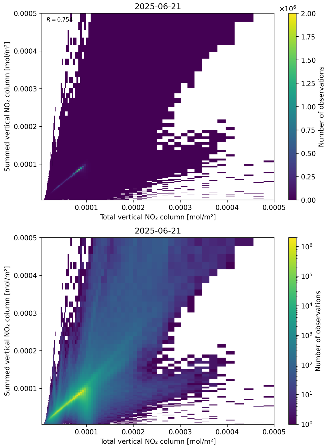
Figure 112: Scatter density plot of “Total vertical NO 2 column” against “Summed vertical NO 2 column” for 2025-06-20 to 2025-06-22.
