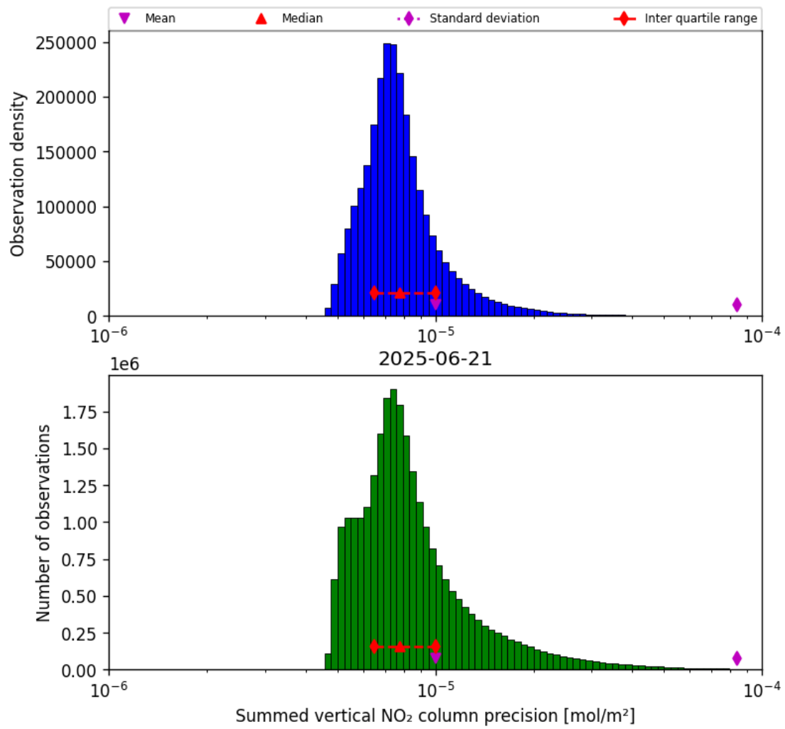
Figure 41: Histogram of “Summed vertical NO 2 column precision” for 2025-06-20 to 2025-06-22
