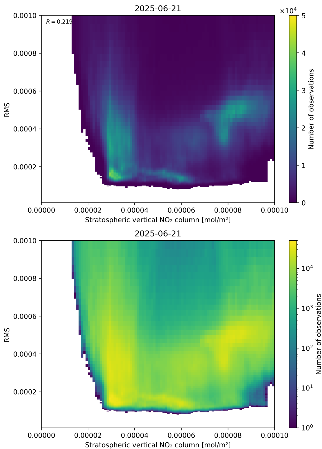
Figure 102: Scatter density plot of “Stratospheric vertical NO 2 column” against “RMS” for 2025-06-20 to 2025-06-22.
