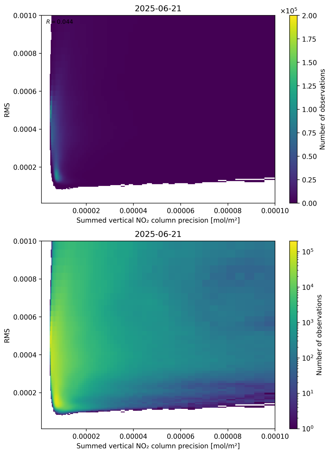
Figure 108: Scatter density plot of “Summed vertical NO 2 column precision” against “RMS” for 2025-06-20 to 2025-06-22.
