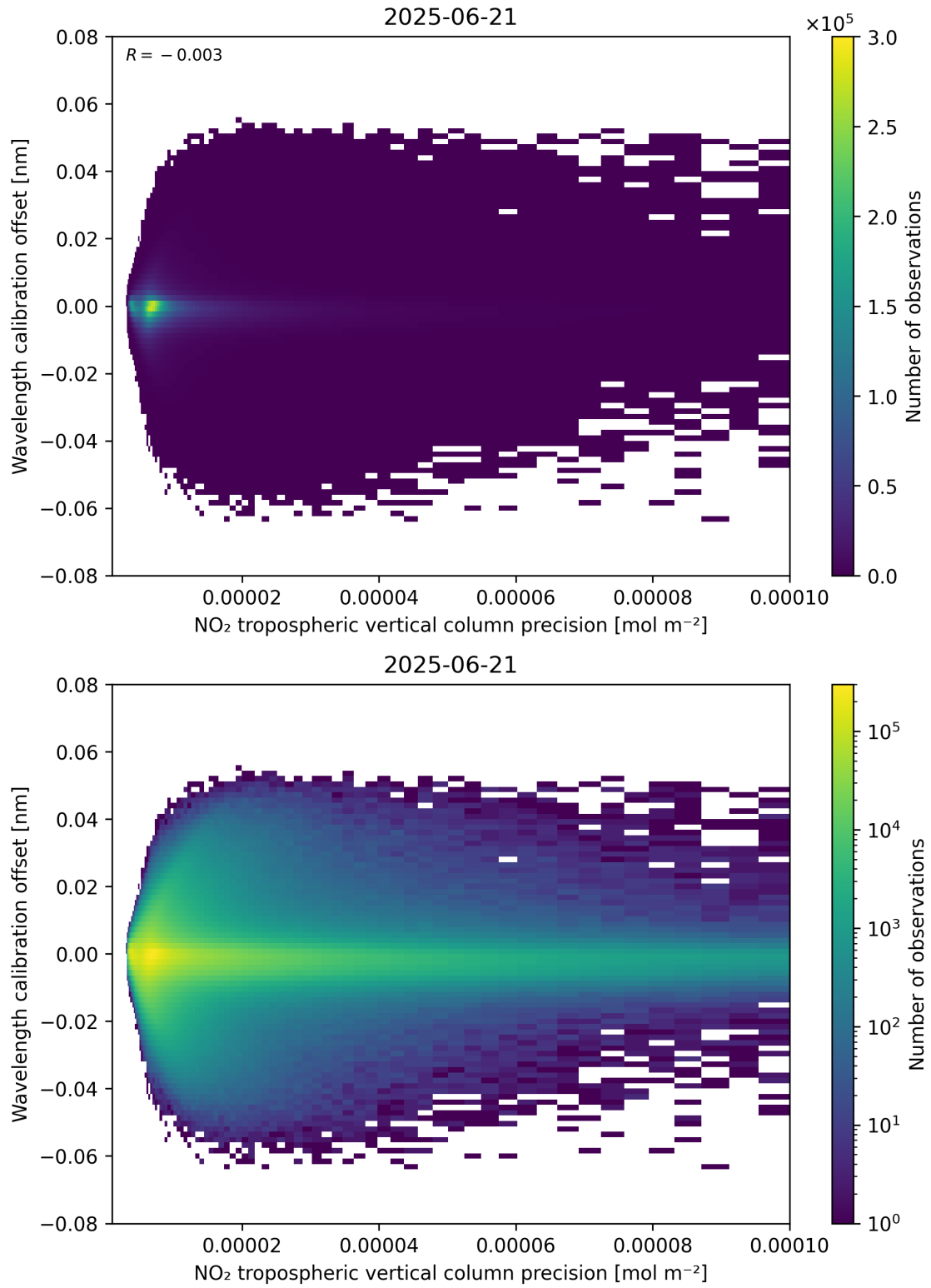
Figure 141: Scatter density plot of “NO 2 tropospheric vertical column precision” against “Wavelength calibration offset” for 2025-06-20 to 2025-06-22.
