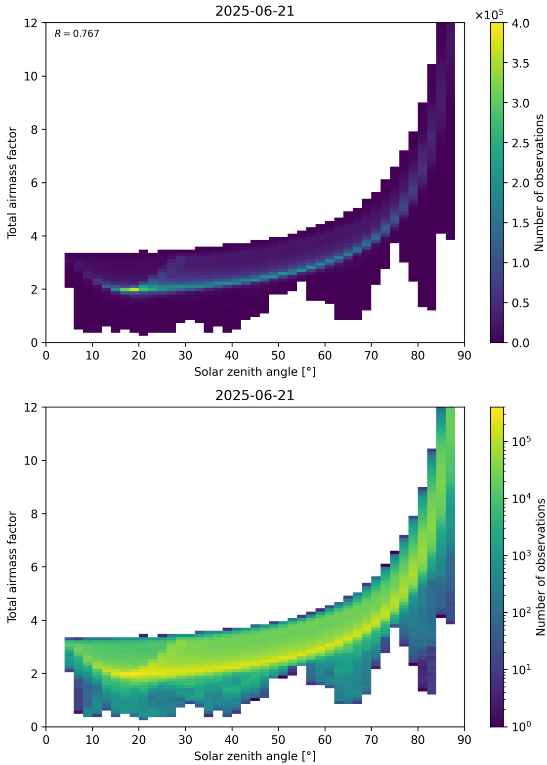
Figure 146: Scatter density plot of “Solar zenith angle” against “Total air mass factor” for 2025-06-20 to 2025-06-22.
