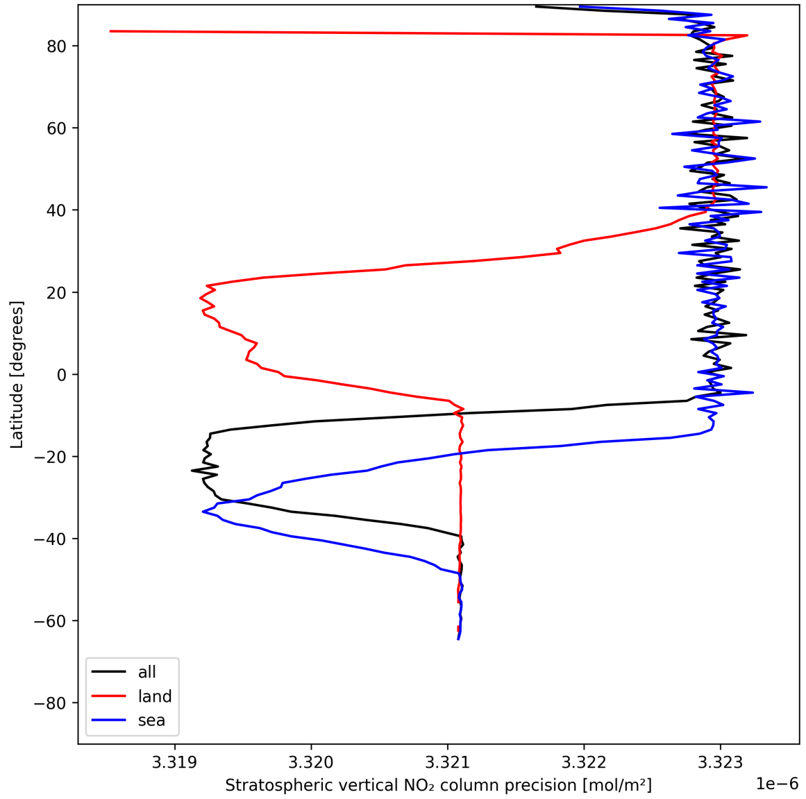
Figure 20: Zonal average of “Stratospheric vertical NO 2 column precision” for 2025-06-20 to 2025-06-22.
