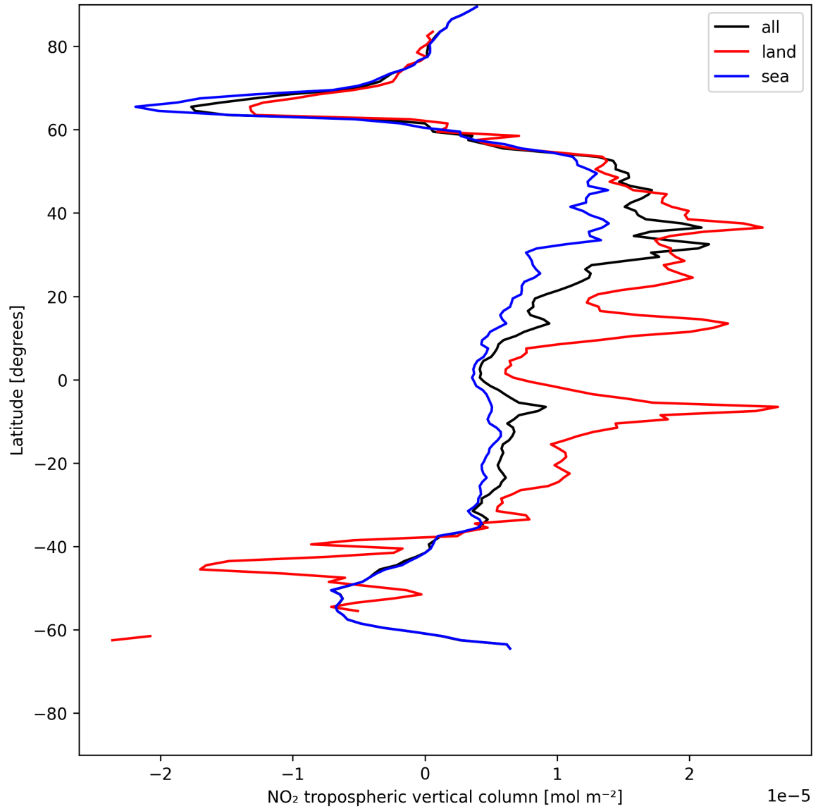
Figure 12: Zonal average of “NO 2 tropospheric vertical column” for 2025-06-20 to 2025-06-22.
