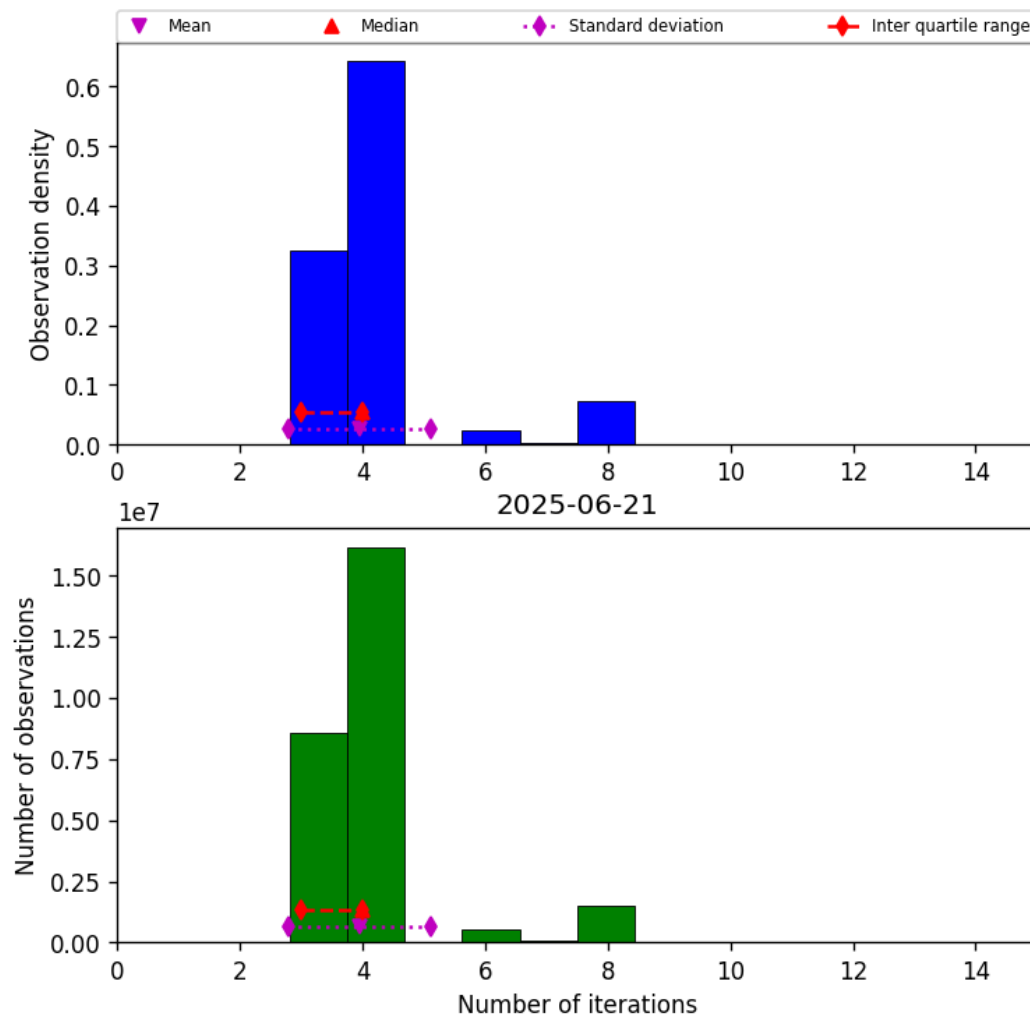
Figure 34: Histogram of “Number of iterations” for 2025-06-20 to 2025-06-22
