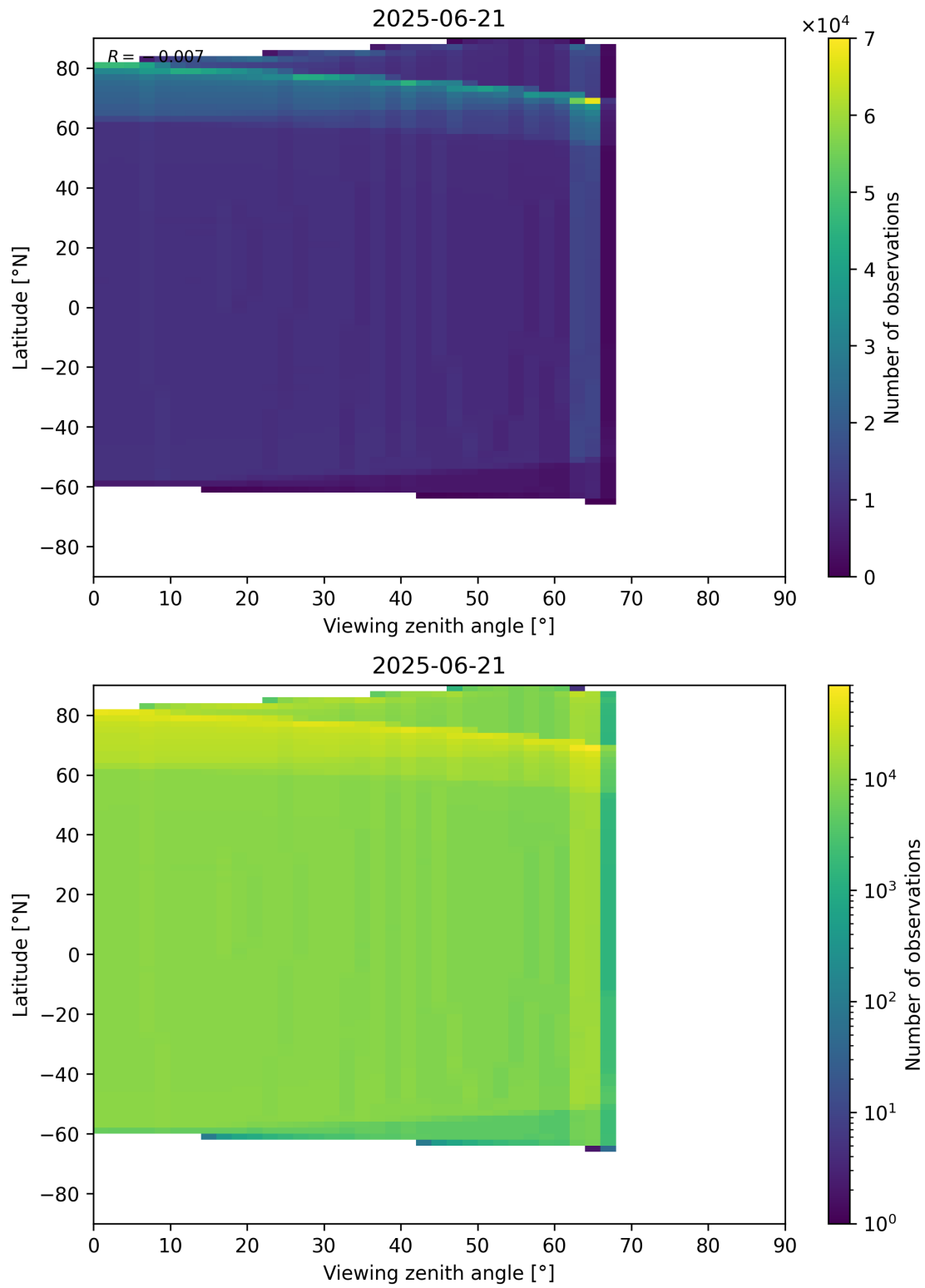
Figure 163: Scatter density plot of “Viewing zenith angle” against “Latitude” for 2025-06-20 to 2025-06-22.
