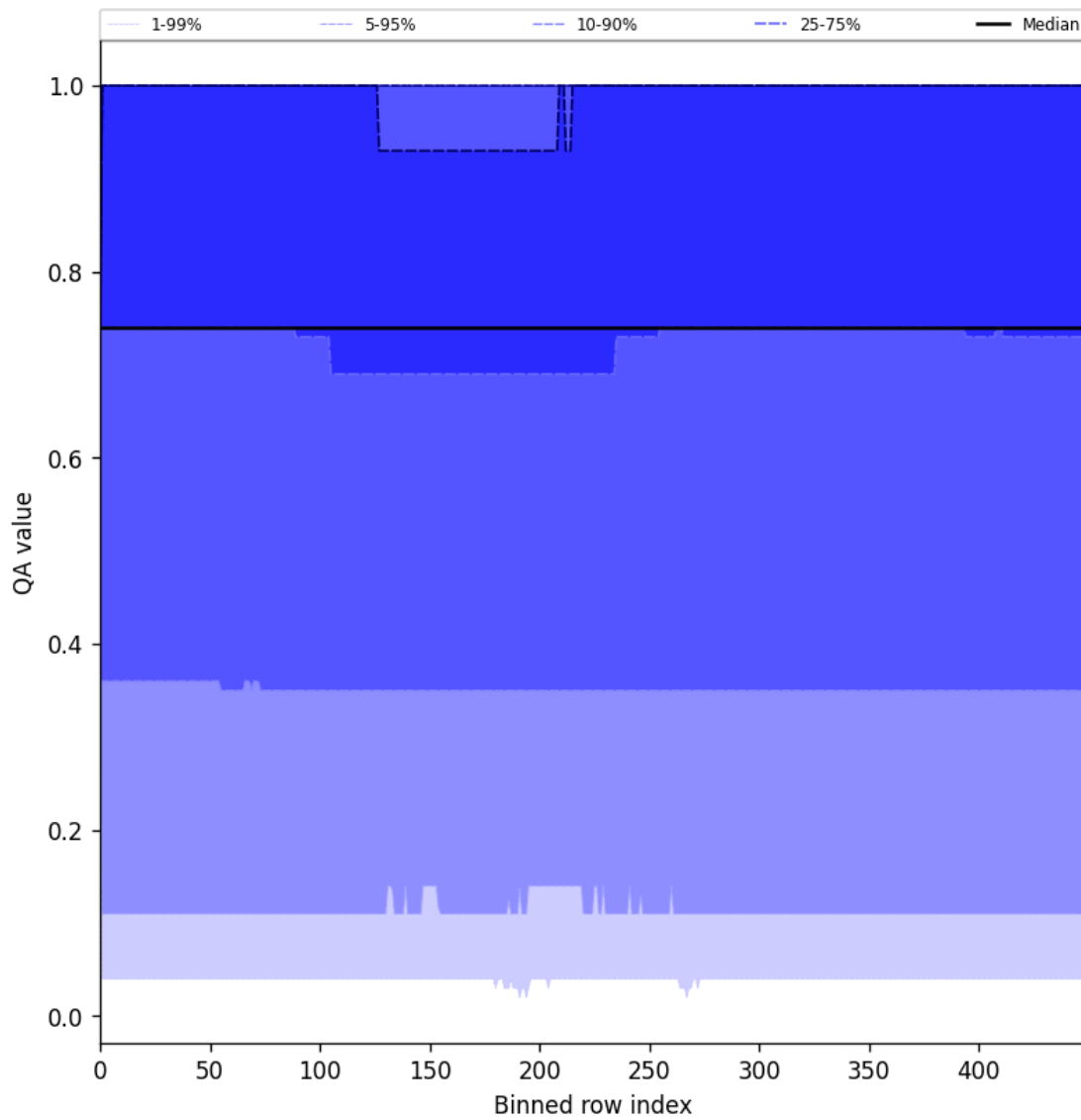
Figure 45: Along track statistics of “QA value” for 2025-06-20 to 2025-06-22
