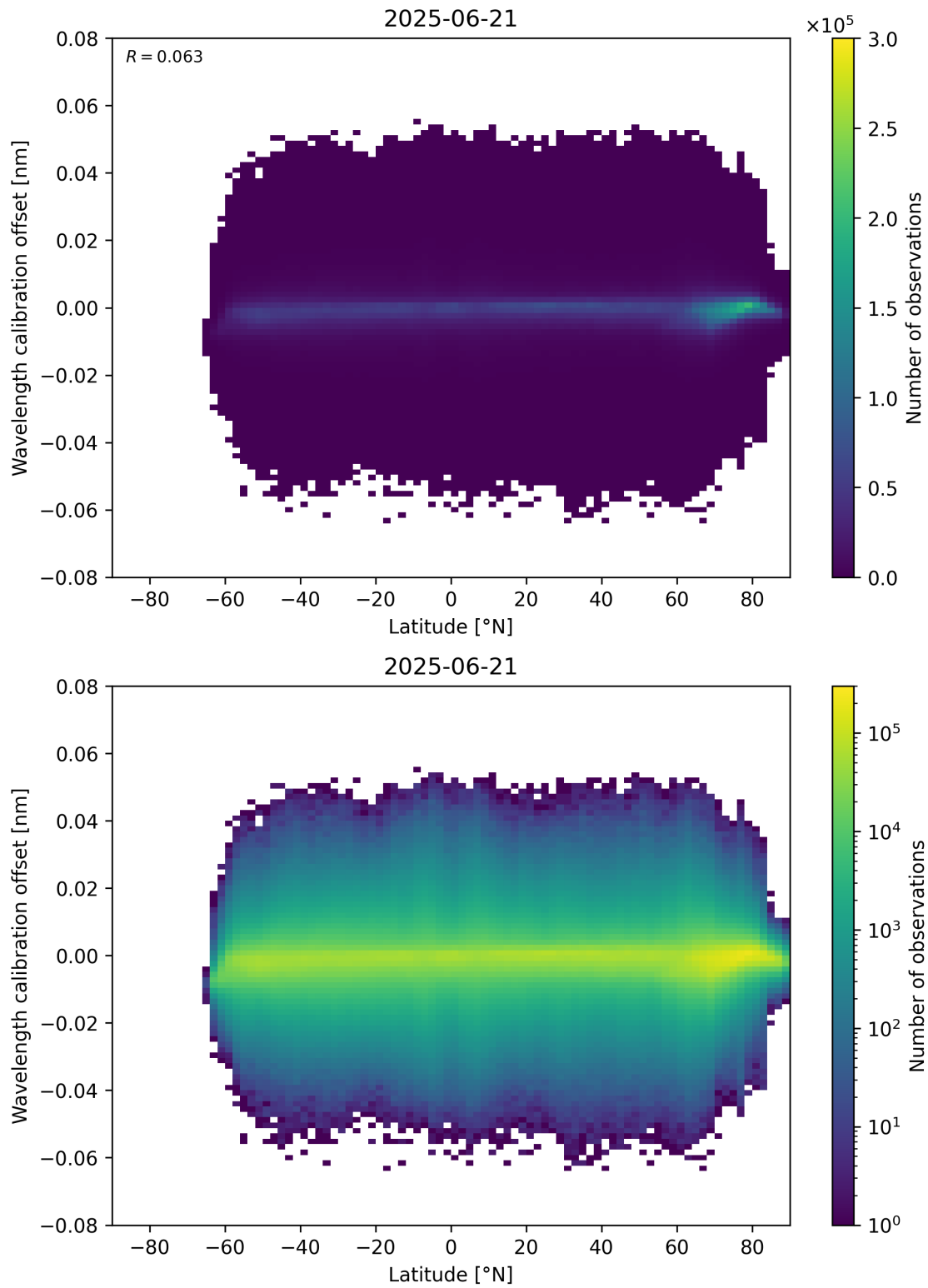
Figure 95: Scatter density plot of “Latitude” against “Wavelength calibration offset” for 2025-06-20 to 2025-06-22.
