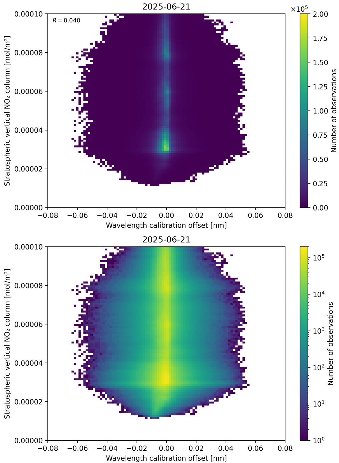
Figure 176: Scatter density plot of “Wavelength calibration offset” against “Stratospheric vertical NO 2 column” for 2025-06-20 to 2025-06-22.
