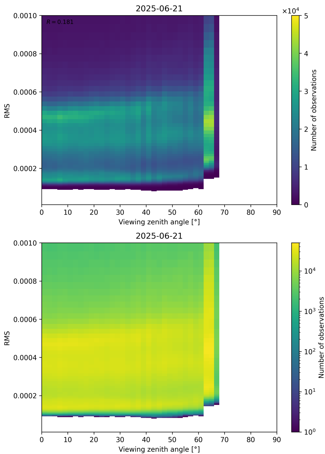
Figure 171: Scatter density plot of “Viewing zenith angle” against “RMS” for 2025-06-20 to 2025-06-22.
