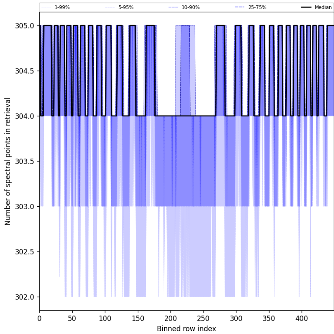
Figure 50: Along track statistics of “Number of spectral points in retrieval” for 2025-06-20 to 2025-06-22
