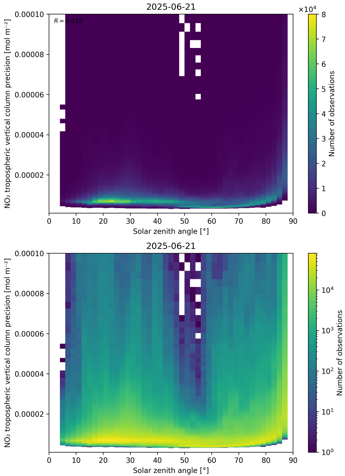
Figure 156: Scatter density plot of “Solar zenith angle” against “NO 2 tropospheric vertical column precision” for 2025-06-20 to 2025-06-22.
