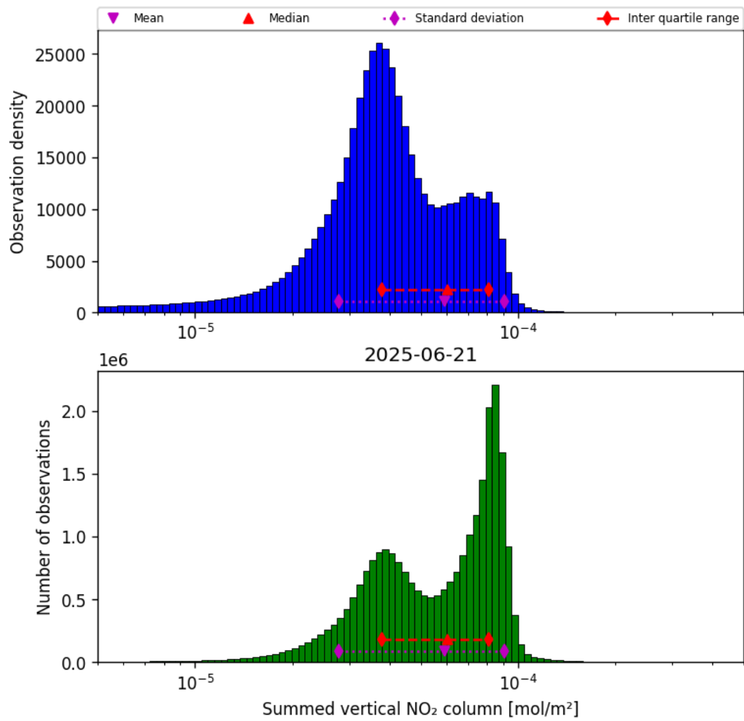
Figure 40: Histogram of “Summed vertical NO 2 column” for 2025-06-20 to 2025-06-22
