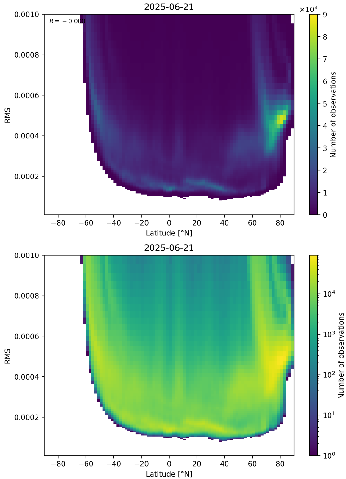
Figure 94: Scatter density plot of “Latitude” against “RMS” for 2025-06-20 to 2025-06-22.
