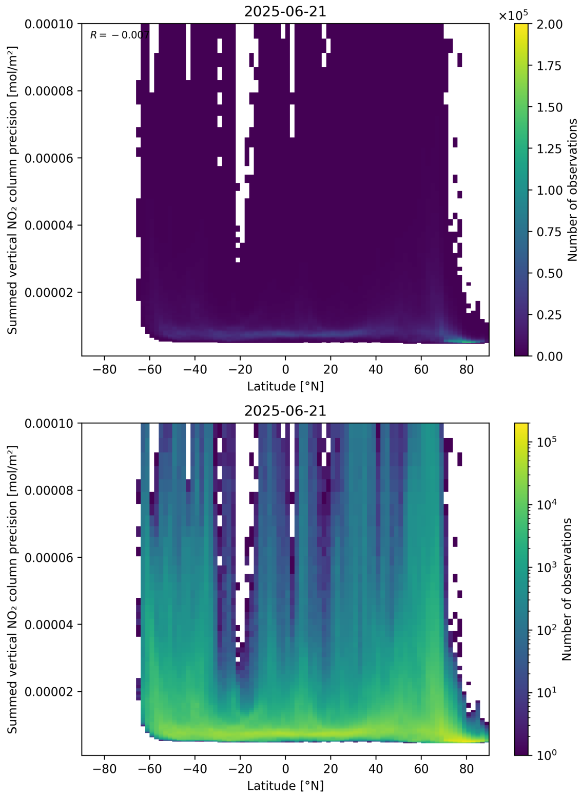
Figure 89: Scatter density plot of “Latitude” against “Summed vertical NO 2 column precision” for 2025-06-20 to 2025-06-22.
