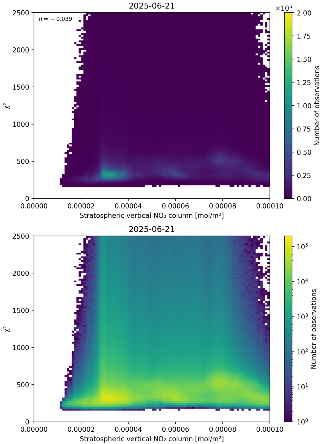
Figure 97: Scatter density plot of “Stratospheric vertical NO 2 column” against “ \chi^2 ” for 2025-06-20 to 2025-06-22.
