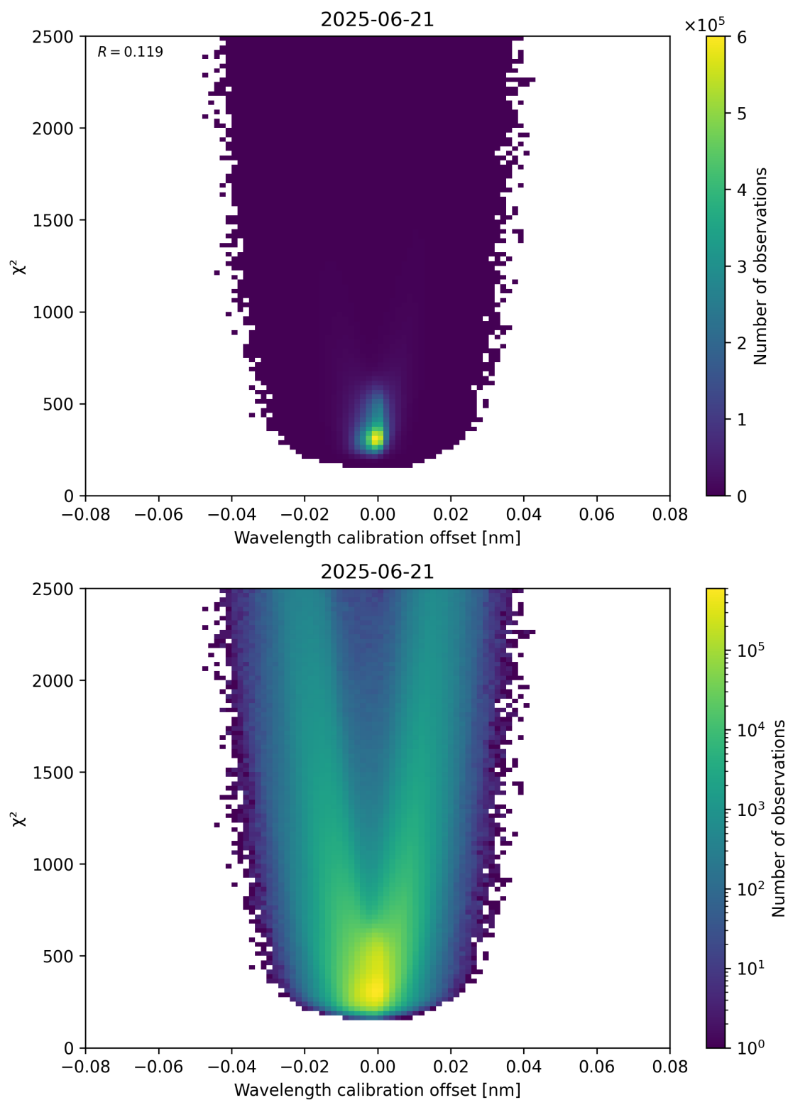
Figure 175: Scatter density plot of “Wavelength calibration offset” against “ \chi^2 ” for 2025-06-20 to 2025-06-22.
