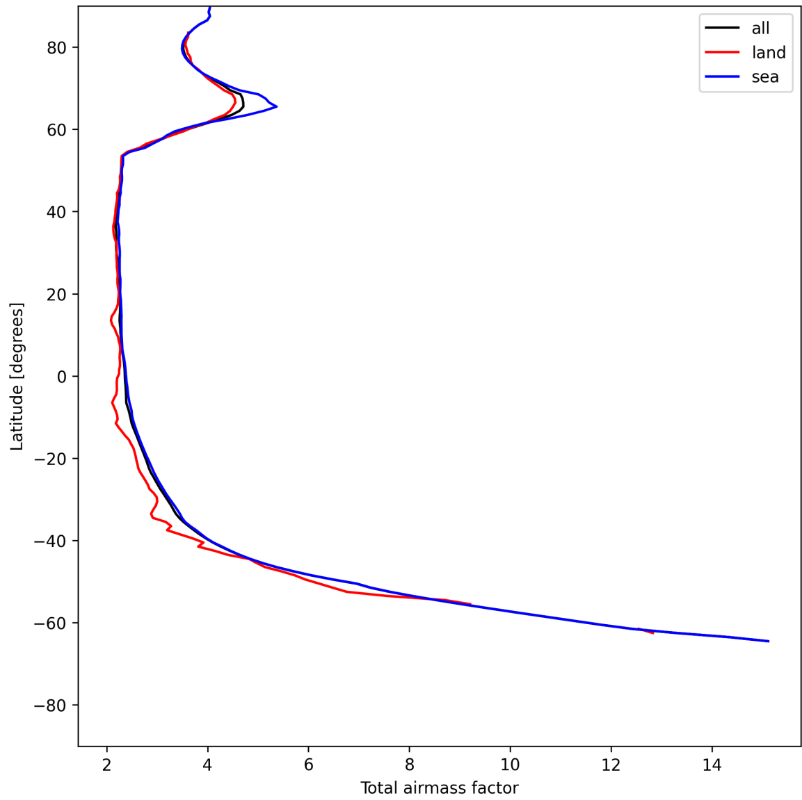
Figure 15: Zonal average of “Total airmass factor” for 2025-06-20 to 2025-06-22.
