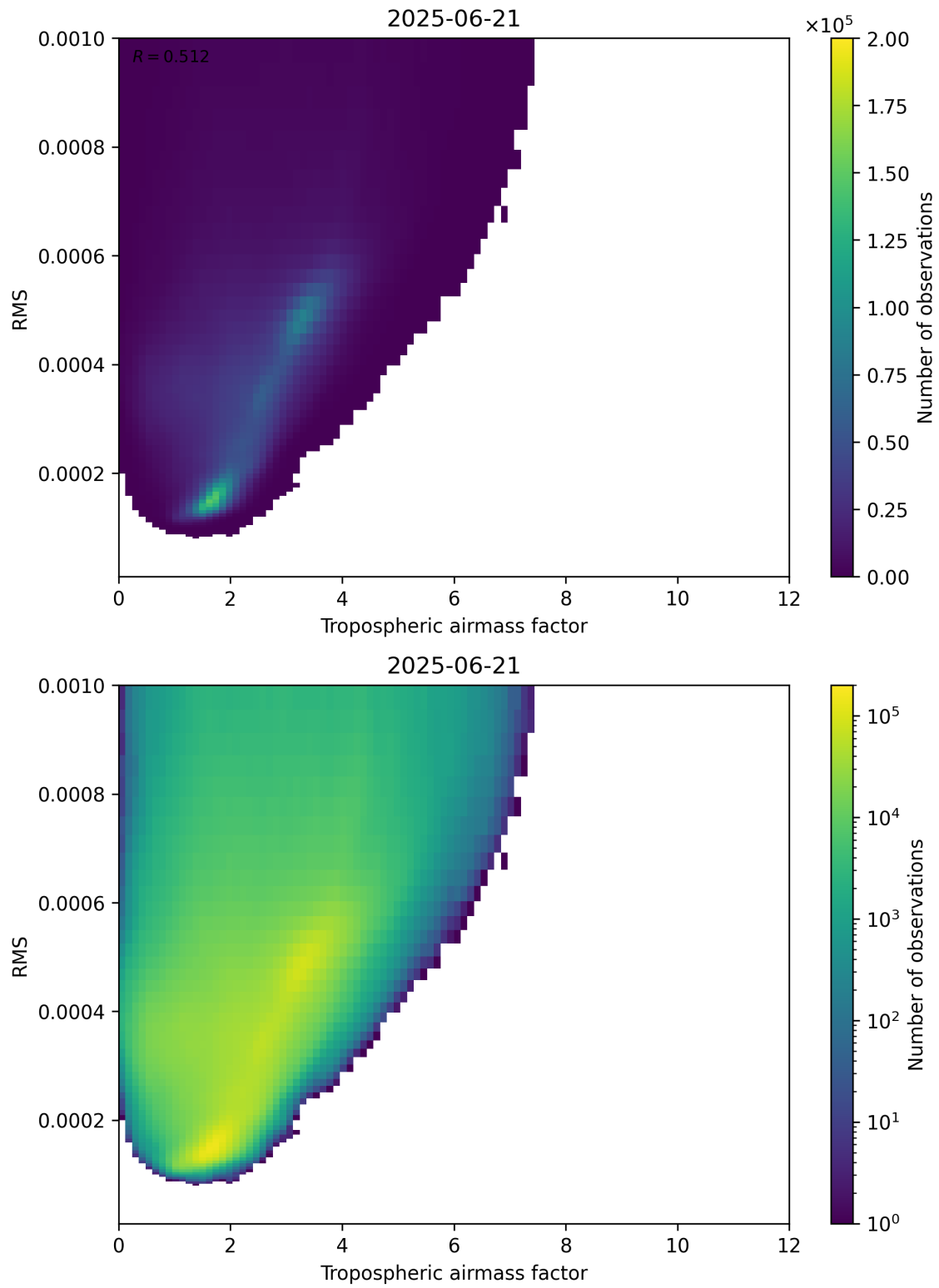
Figure 79: Scatter density plot of “Tropospheric airmass factor” against “RMS” for 2025-06-20 to 2025-06-22.
