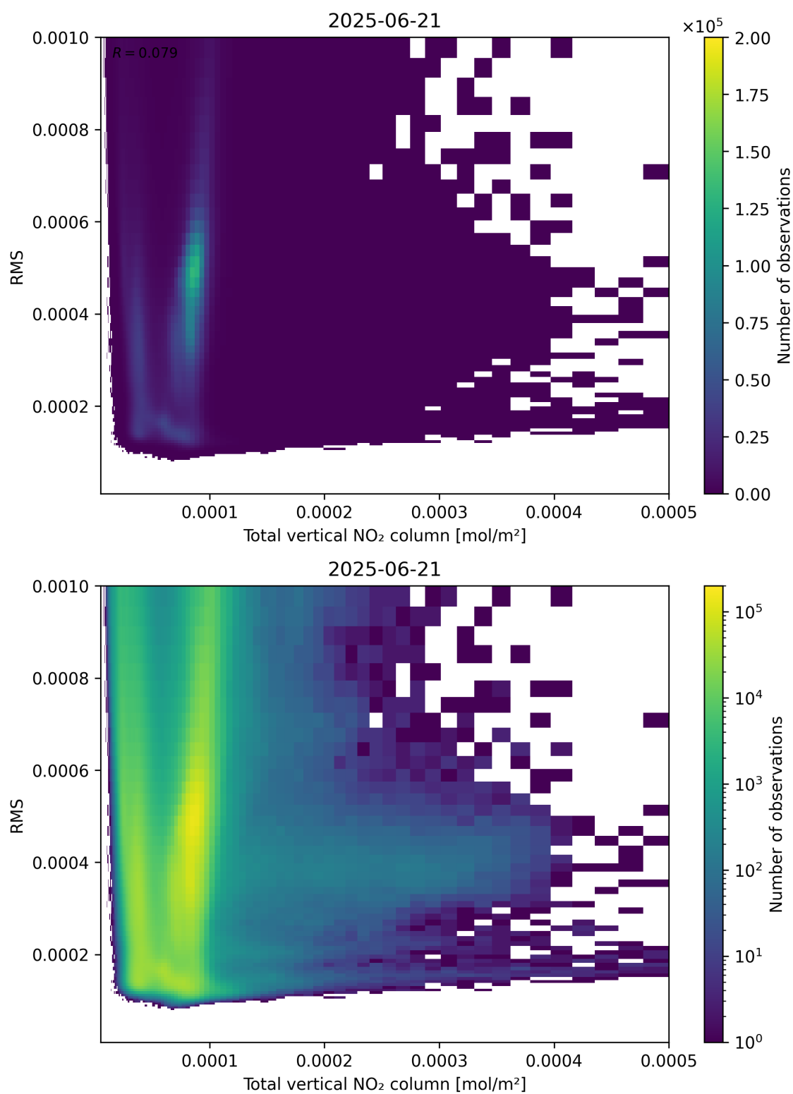
Figure 120: Scatter density plot of “Total vertical NO 2 column” against “RMS” for 2025-06-20 to 2025-06-22.
