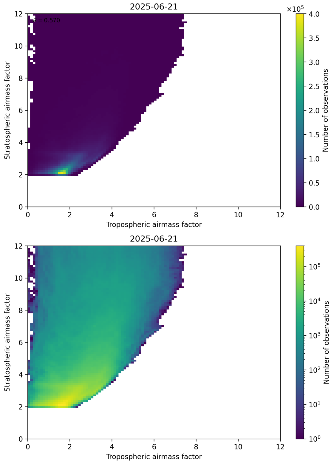
Figure 71: Scatter density plot of “Tropospheric airmass factor” against “Stratospheric airmass factor” for 2025-06-20 to 2025-06-22.
