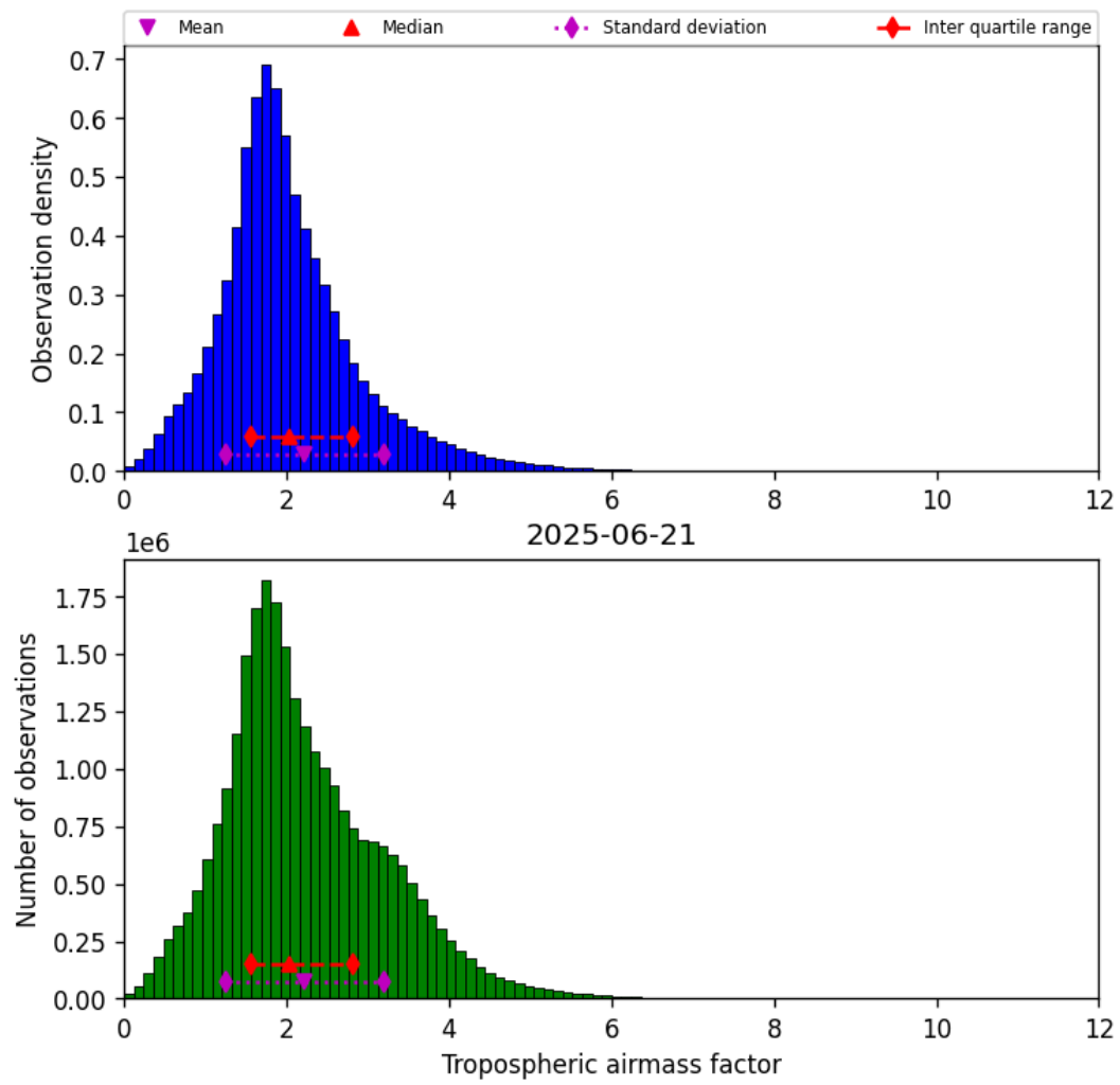
Figure 31: Histogram of “Tropospheric airmass factor” for 2025-06-20 to 2025-06-22
