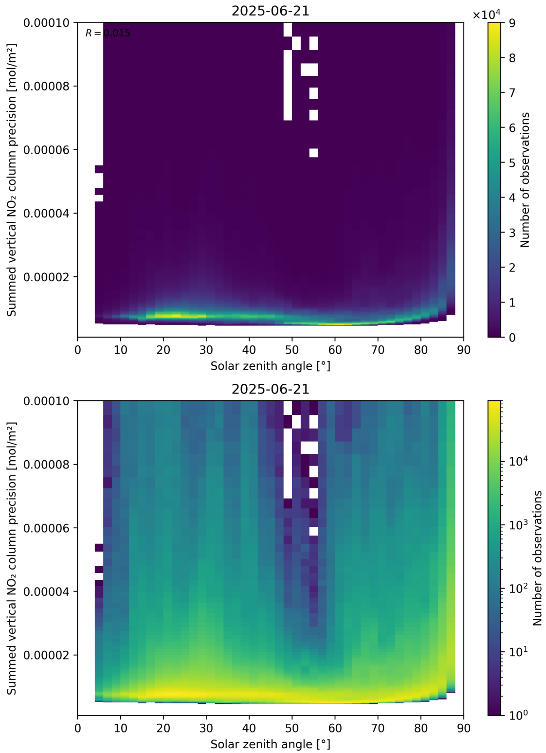
Figure 152: Scatter density plot of “Solar zenith angle” against “Summed vertical NO 2 column precision” for 2025-06-20 to 2025-06-22.
