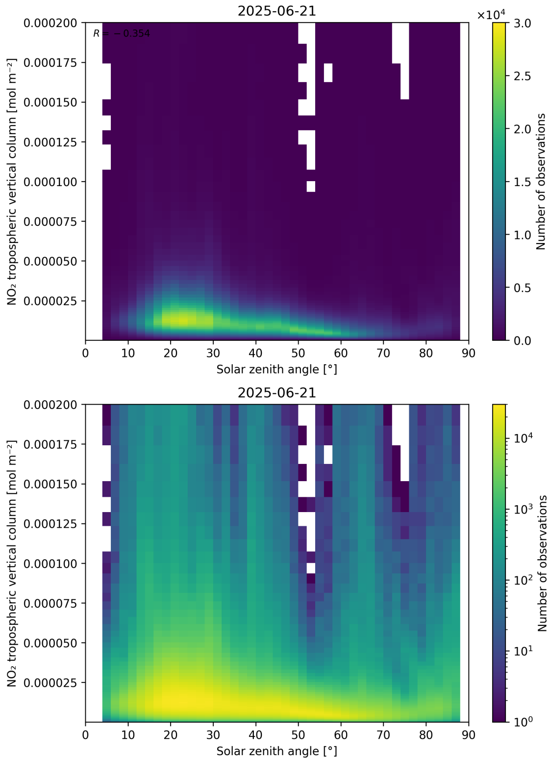
Figure 155: Scatter density plot of “Solar zenith angle” against “NO 2 tropospheric vertical column” for 2025-06-20 to 2025-06-22.
