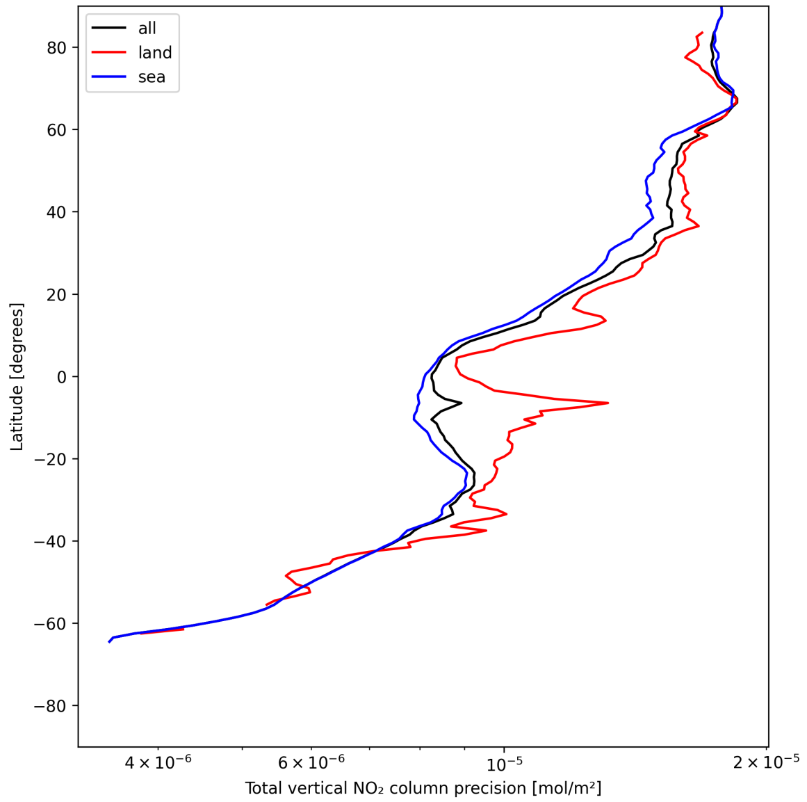
Figure 22: Zonal average of “Total vertical NO 2 column precision” for 2025-06-20 to 2025-06-22.
