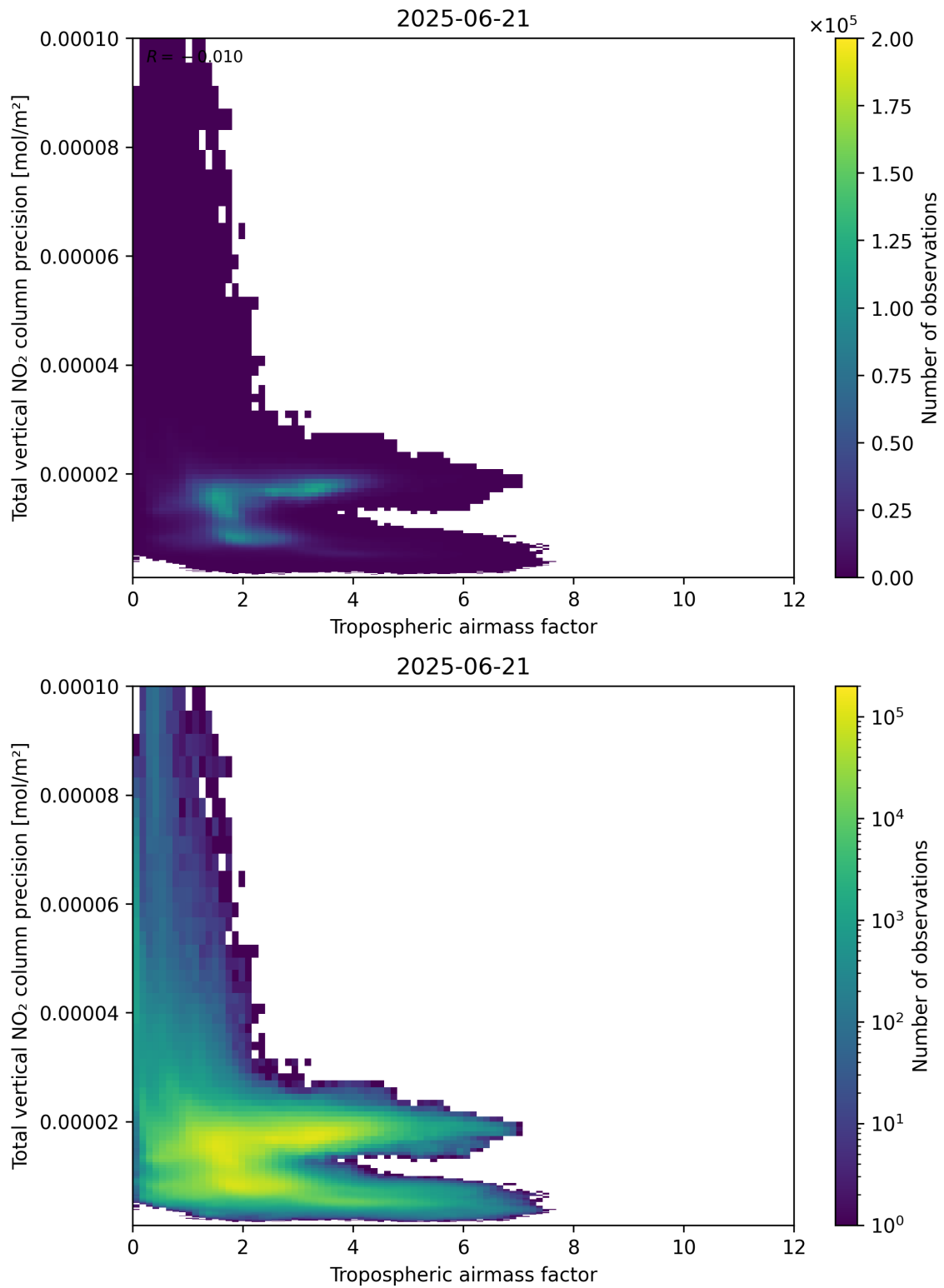
Figure 78: Scatter density plot of “Tropospheric air mass factor” against “Total vertical NO 2 column precision” for 2025-06-20 to 2025-06-22.
