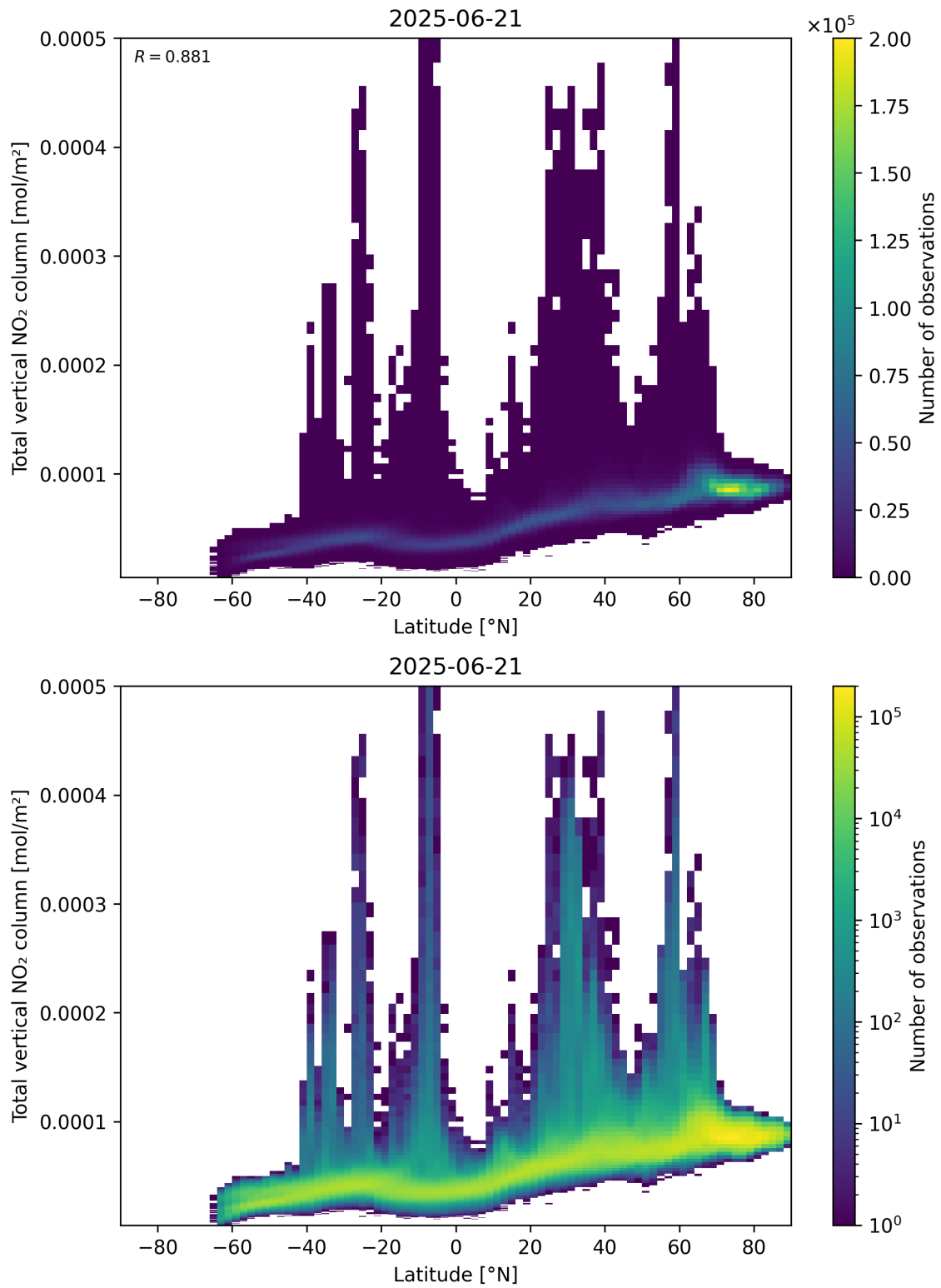
Figure 90: Scatter density plot of “Latitude” against “Total vertical NO 2 column” for 2025-06-20 to 2025-06-22.
