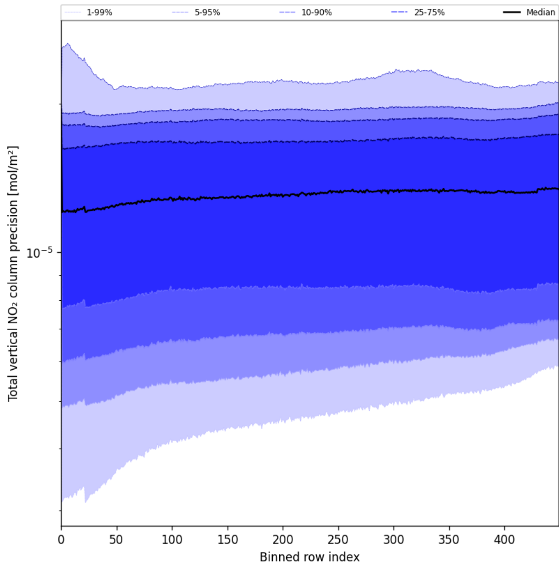
Figure 56: Along track statistics of “Total vertical NO 2 column precision” for 2025-06-20 to 2025-06-22
