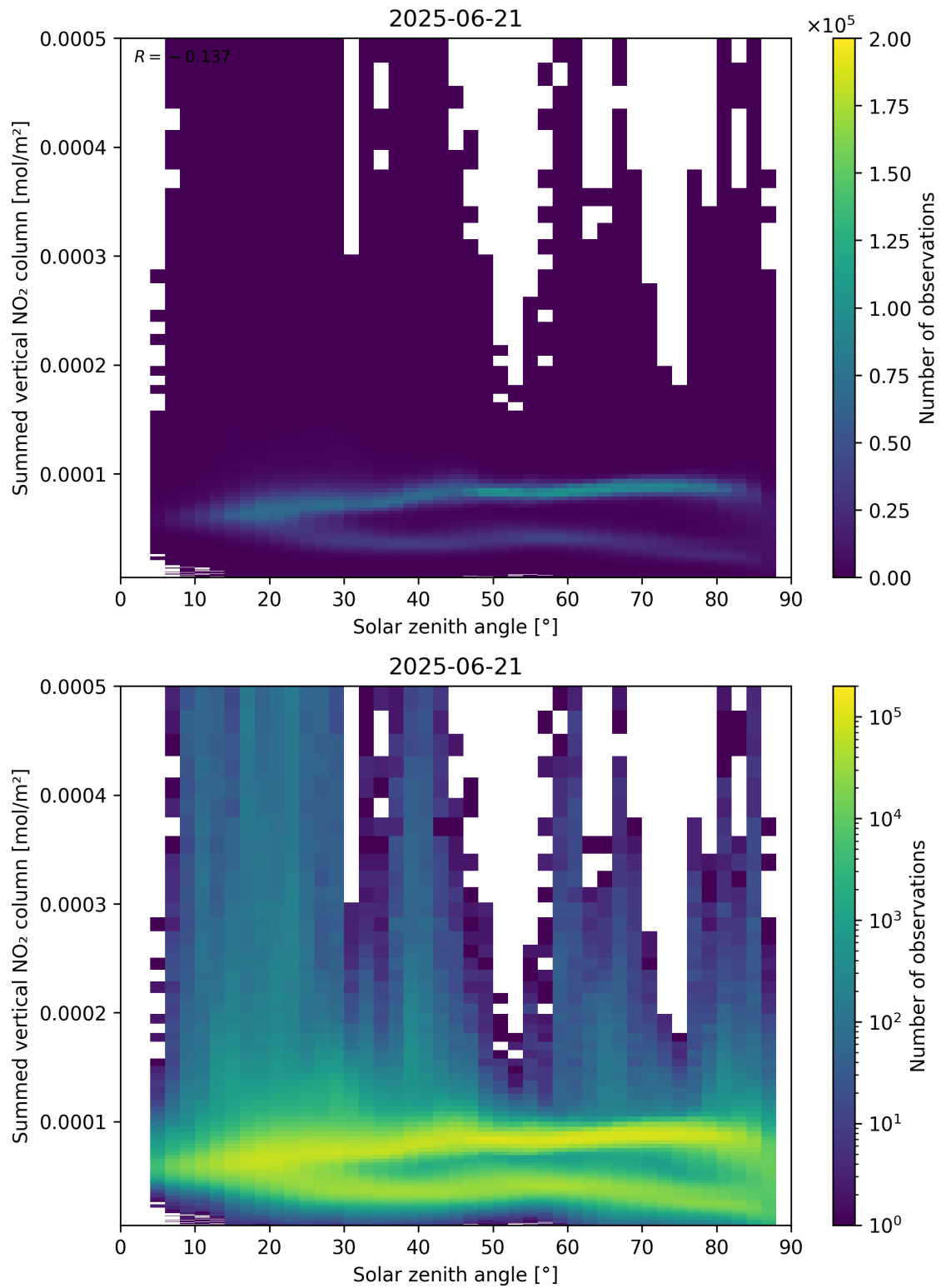
Figure 151: Scatter density plot of “Solar zenith angle” against “Summed vertical NO 2 column” for 2025-06-20 to 2025-06-22.
