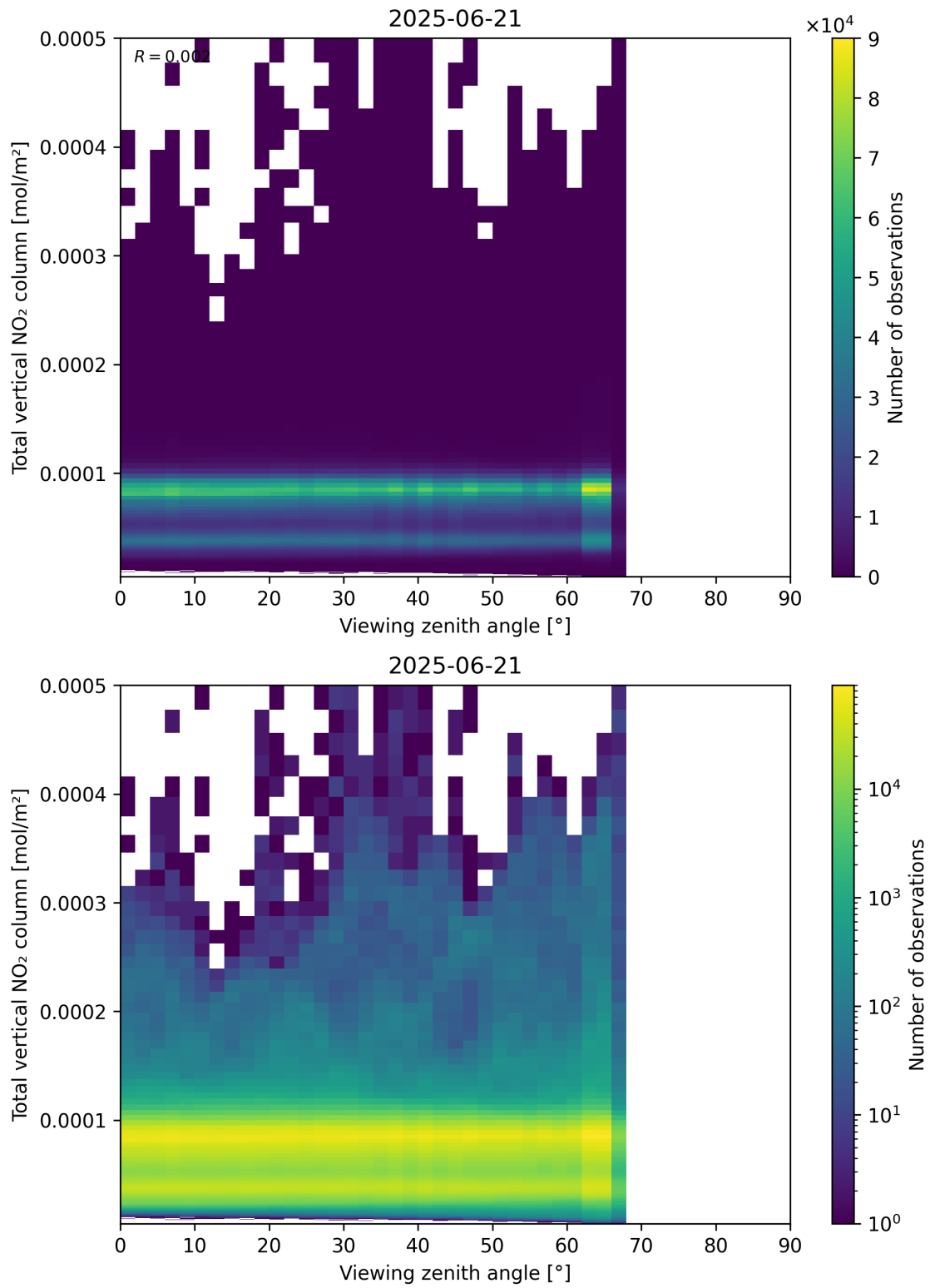
Figure 167: Scatter density plot of “Viewing zenith angle” against “Total vertical NO 2 column” for 2025-06-20 to 2025-06-22.
