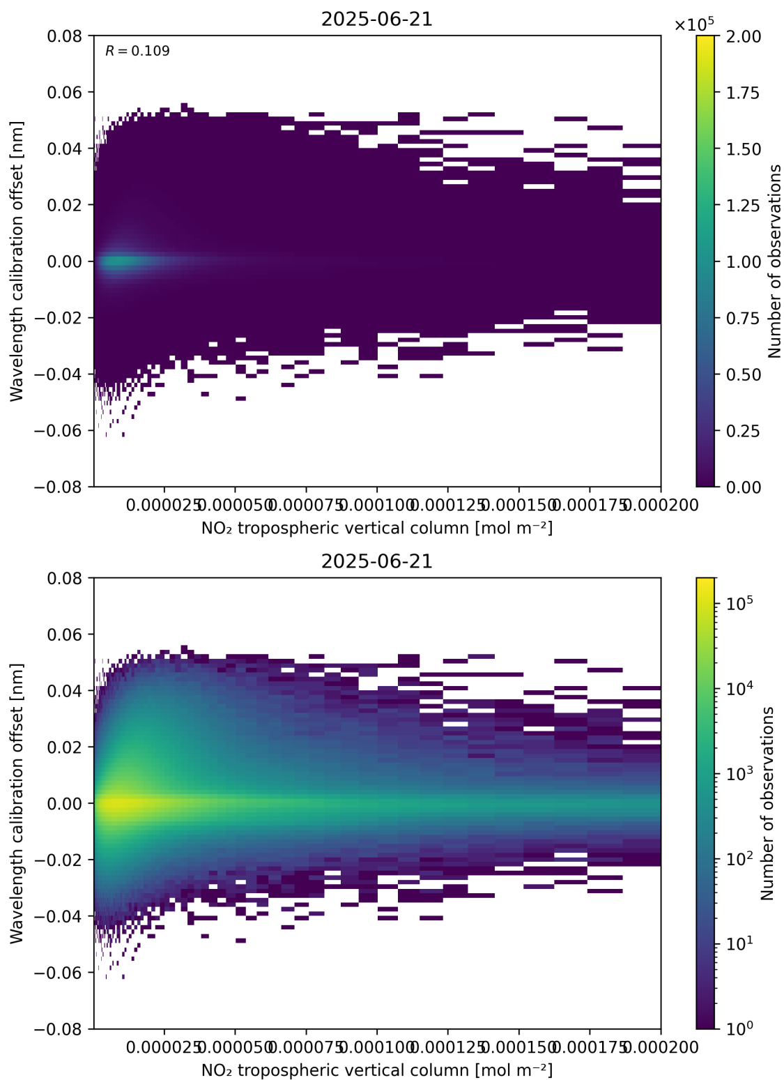
Figure 143: Scatter density plot of “NO 2 tropospheric vertical column” against “Wavelength calibration offset” for 2025-06-20 to 2025-06-22.
