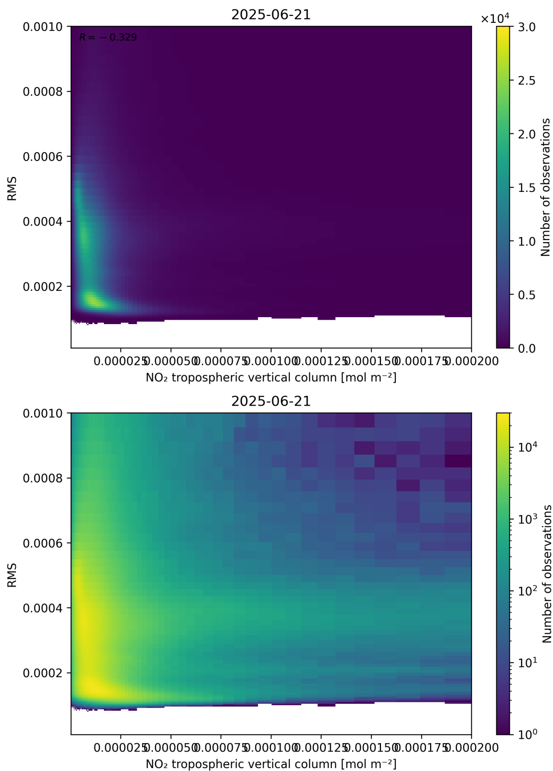
Figure 142: Scatter density plot of “NO 2 tropospheric vertical column” against “RMS” for 2025-06-20 to 2025-06-22.
