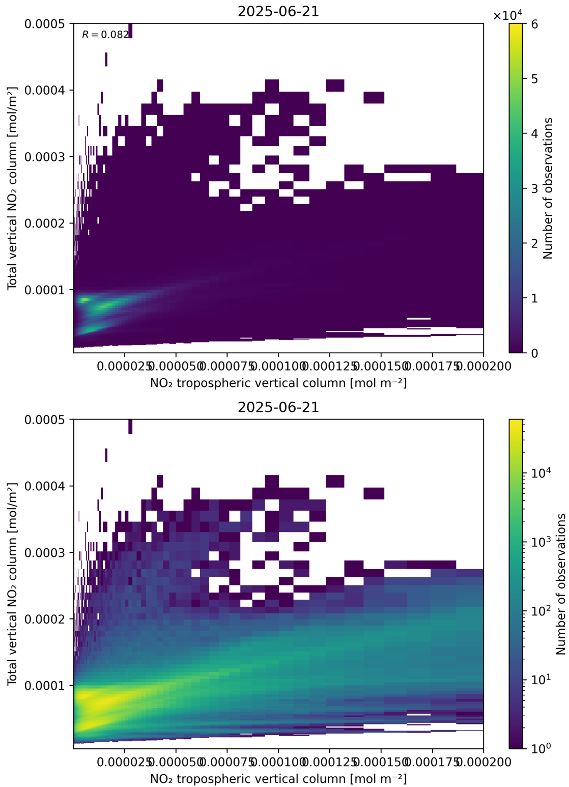
Figure 128: Scatter density plot of “NO 2 tropospheric vertical column” against “Total vertical NO 2 column” for 2025-06-20 to 2025-06-22.
