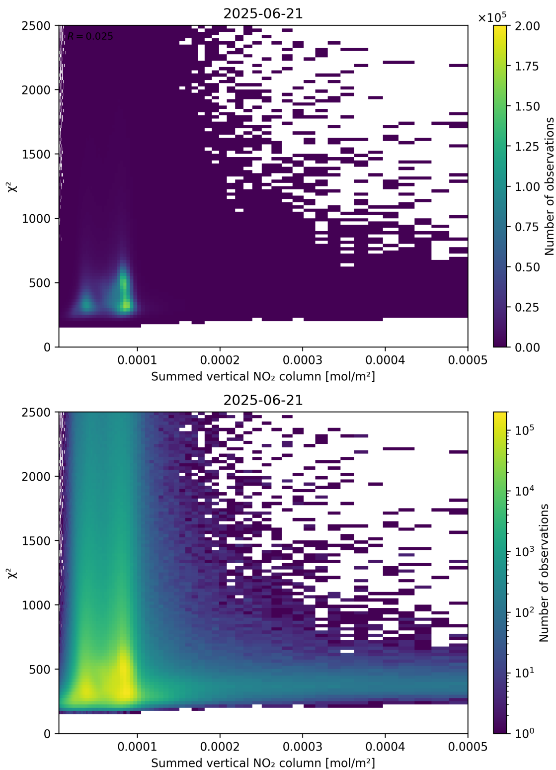
Figure 104: Scatter density plot of “Summed vertical NO 2 column” against “ \chi^2 ” for 2025-06-20 to 2025-06-22.
