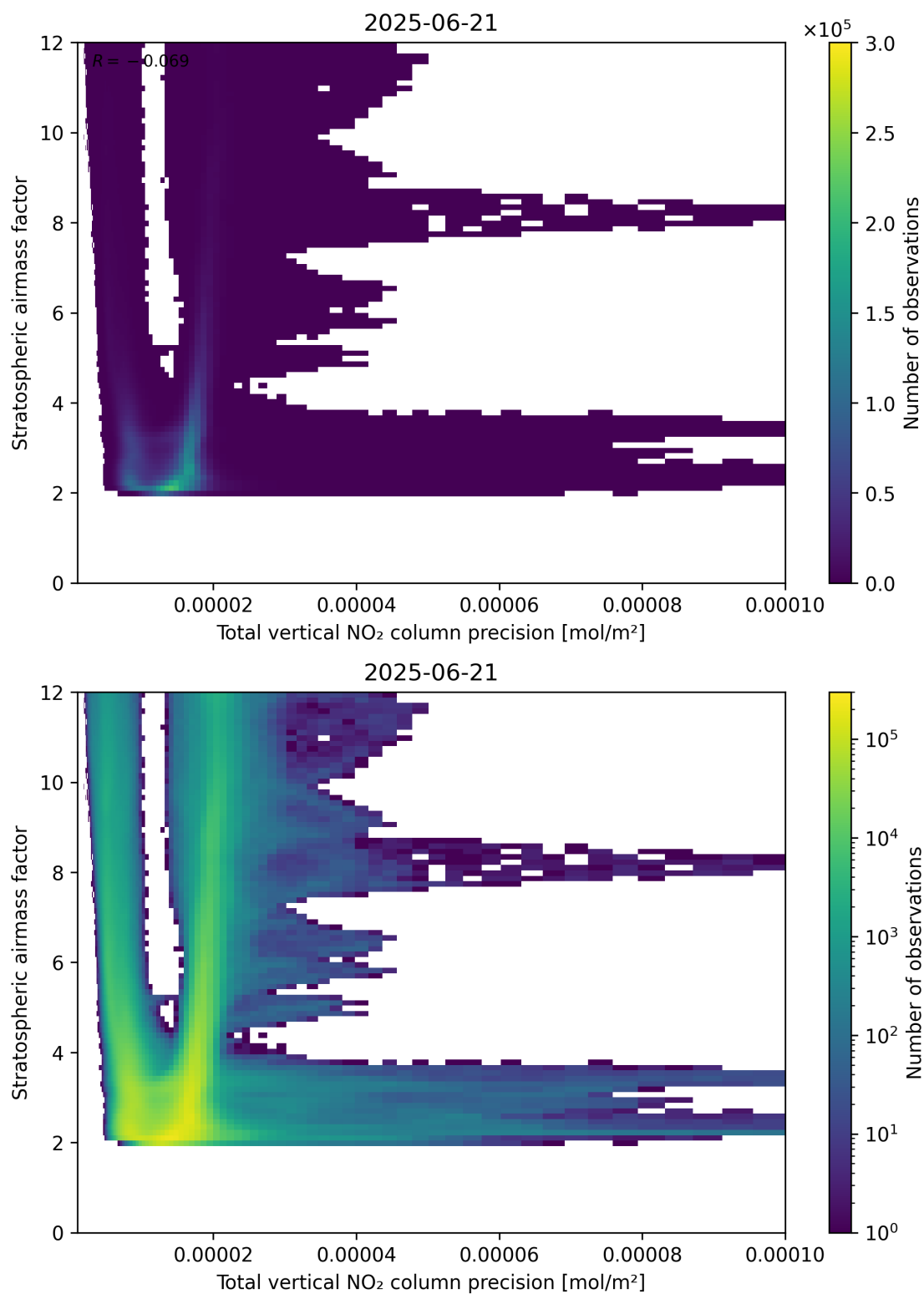
Figure 115: Scatter density plot of “Total vertical NO 2 column precision” against “Stratospheric air mass factor” for 2025-06-20 to 2025-06-22.
