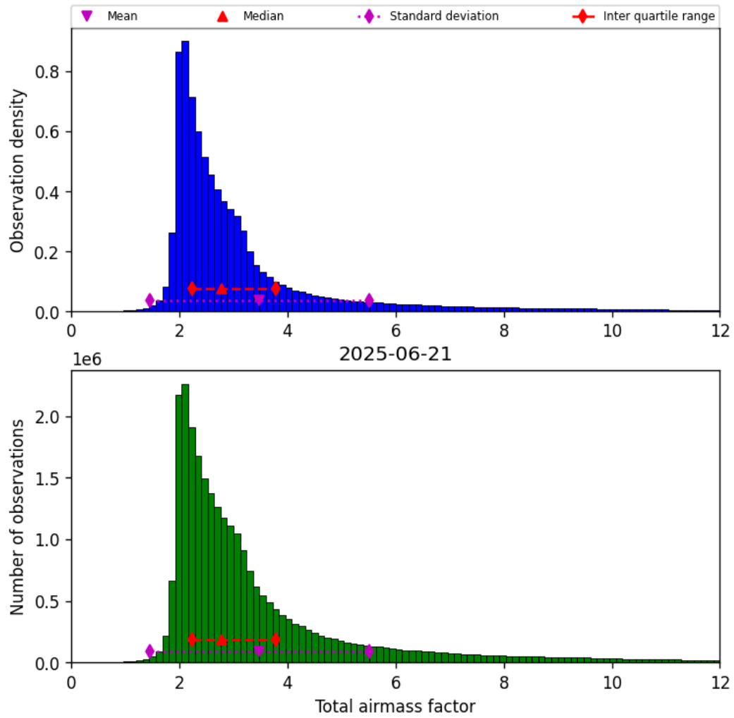
Figure 32: Histogram of “Total airmass factor” for 2025-06-20 to 2025-06-22
