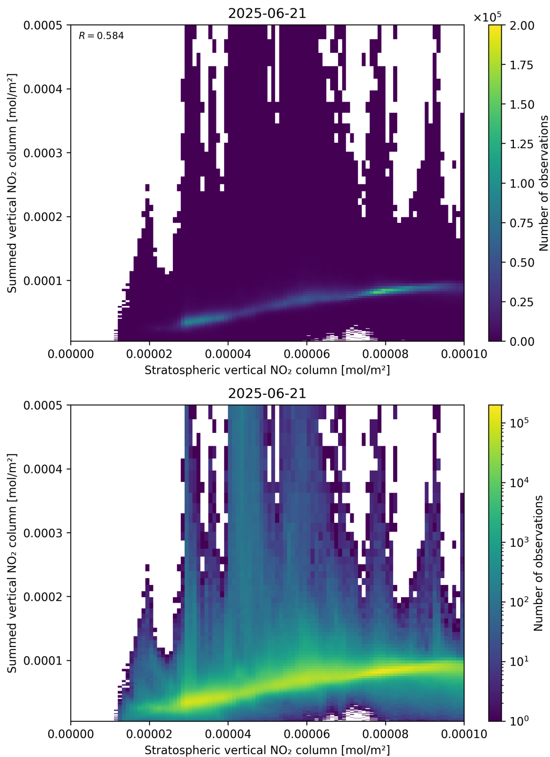
Figure 98: Scatter density plot of “Stratospheric vertical NO 2 column” against “Summed vertical NO 2 column” for 2025-06-20 to 2025-06-22.
