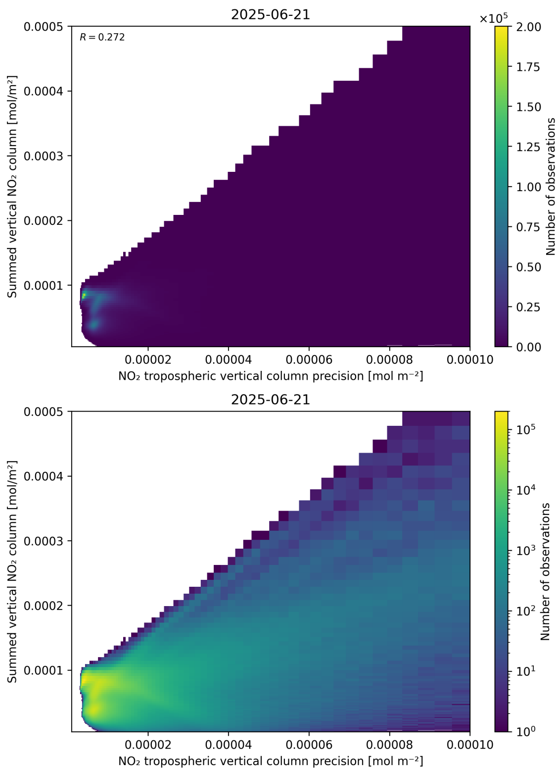
Figure 136: Scatter density plot of “NO 2 tropospheric vertical column precision” against “Summed vertical NO 2 column” for 2025-06-20 to 2025-06-22.
