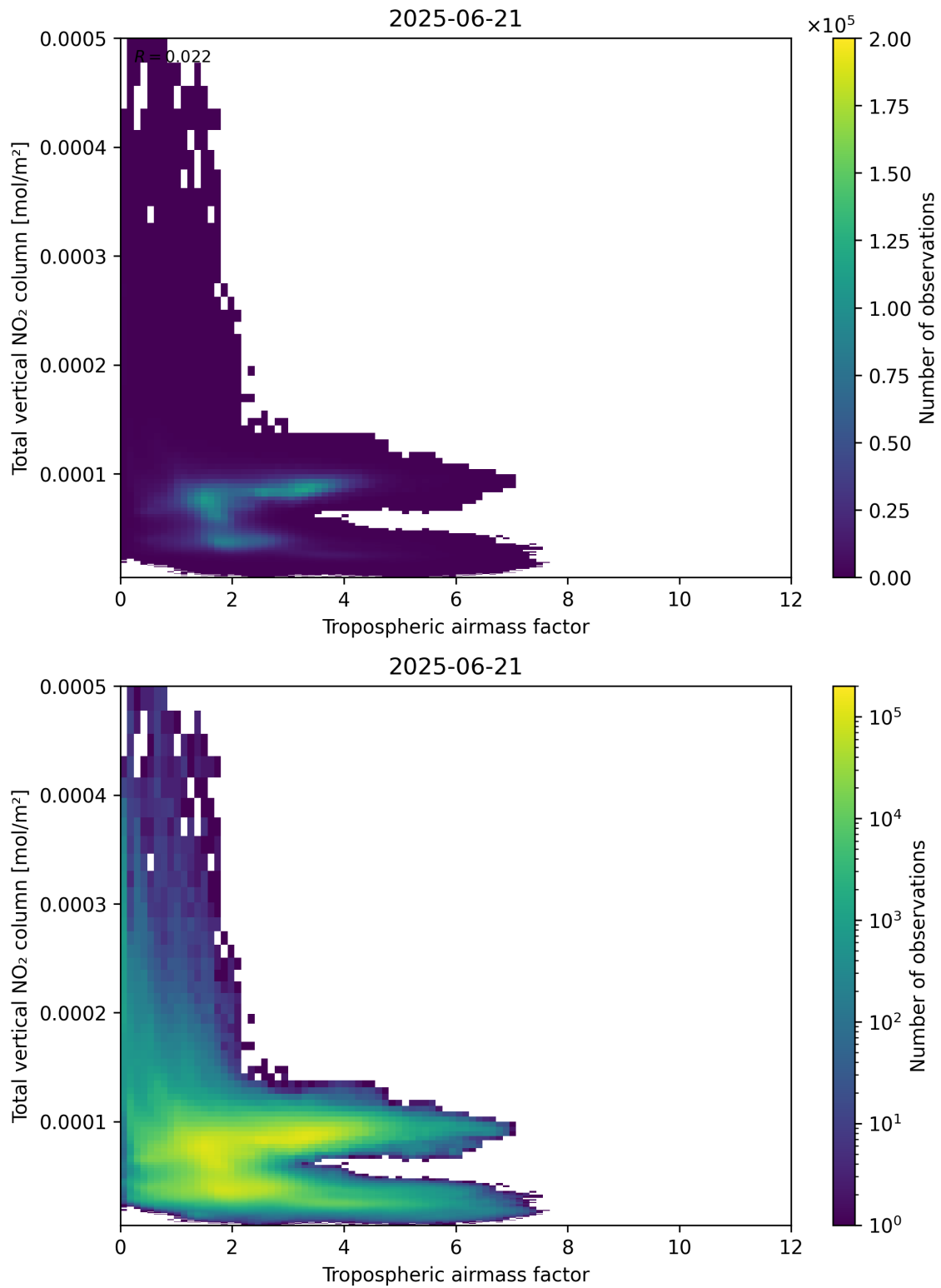
Figure 77: Scatter density plot of “Tropospheric airmass factor” against “Total vertical NO 2 column” for 2025-06-20 to 2025-06-22.
