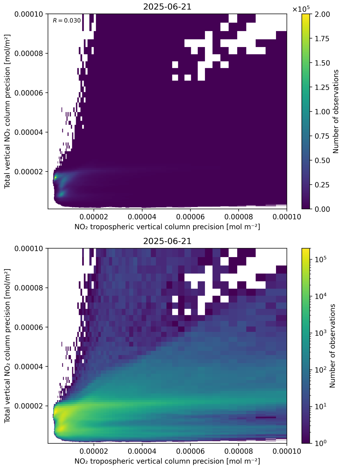
Figure 139: Scatter density plot of “NO 2 tropospheric vertical column precision” against “Total vertical NO 2 column precision” for 2025-06-20 to 2025-06-22.
