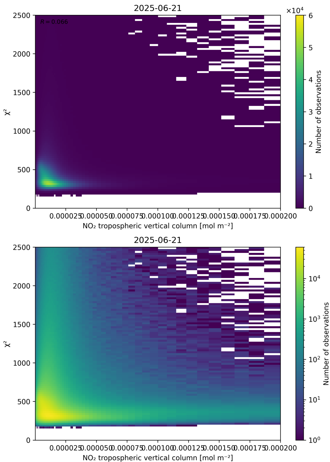
Figure 124: Scatter density plot of “NO 2 tropospheric vertical column” against “ \chi^2 ” for 2025-06-20 to 2025-06-22.
