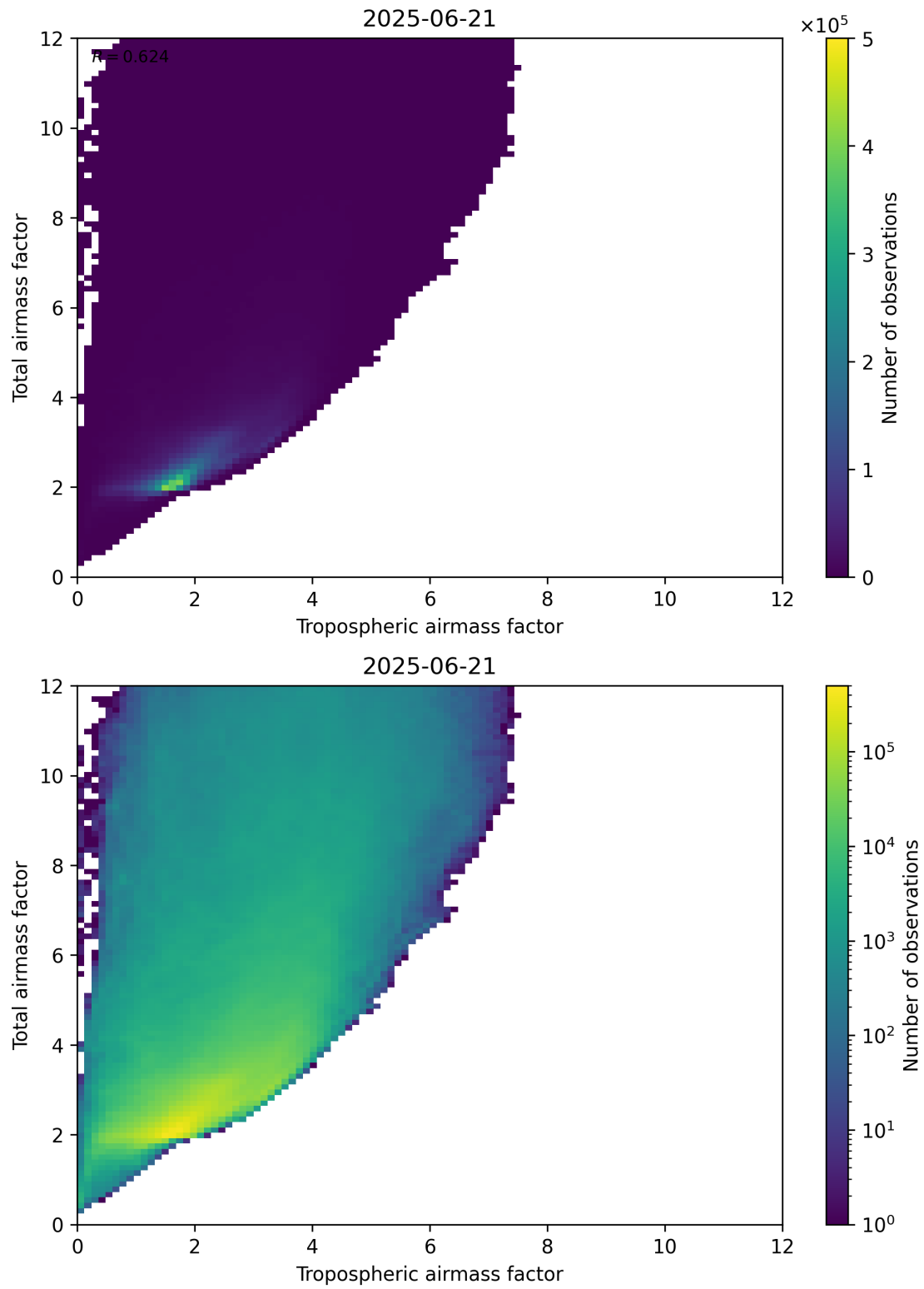
Figure 72: Scatter density plot of “Tropospheric airmass factor” against “Total airmass factor” for 2025-06-20 to 2025-06-22.
