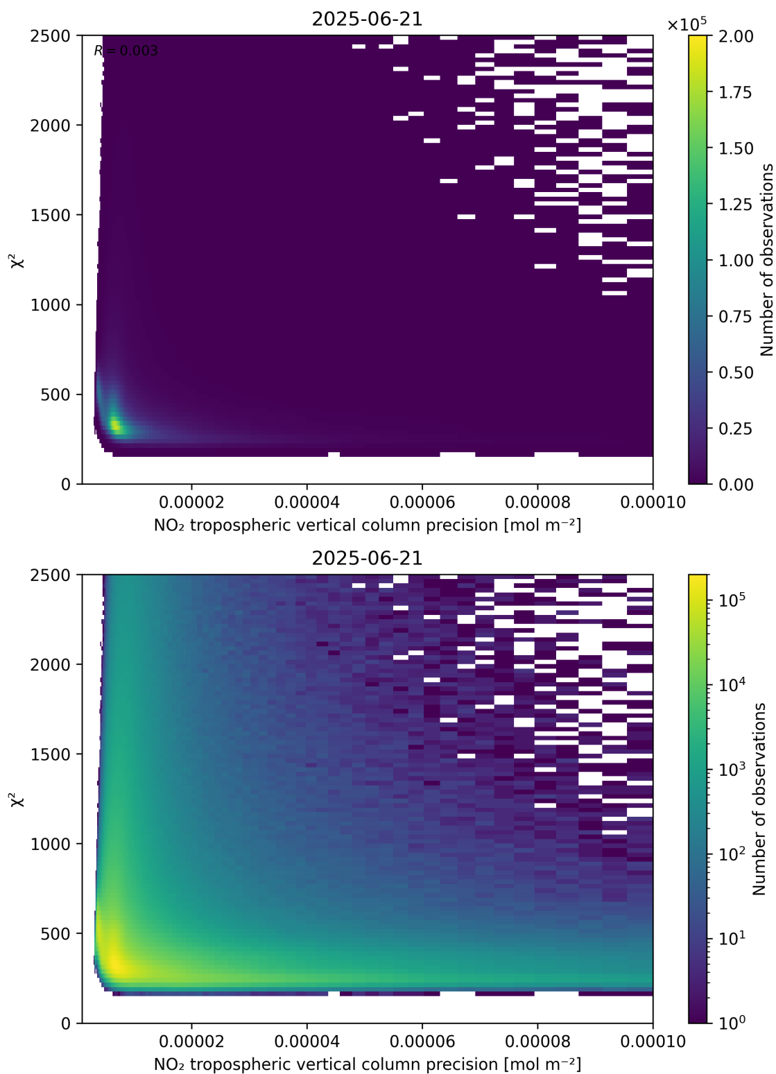
Figure 134: Scatter density plot of “NO 2 tropospheric vertical column precision” against “ \chi^2 ” for 2025-06-20 to 2025-06-22.
