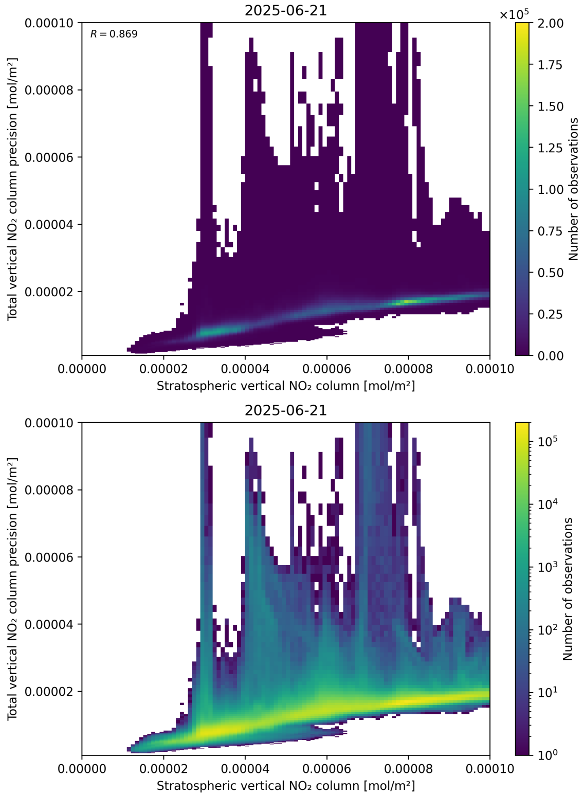
Figure 101: Scatter density plot of “Stratospheric vertical NO 2 column” against “Total vertical NO 2 column precision” for 2025-06-20 to 2025-06-22.
