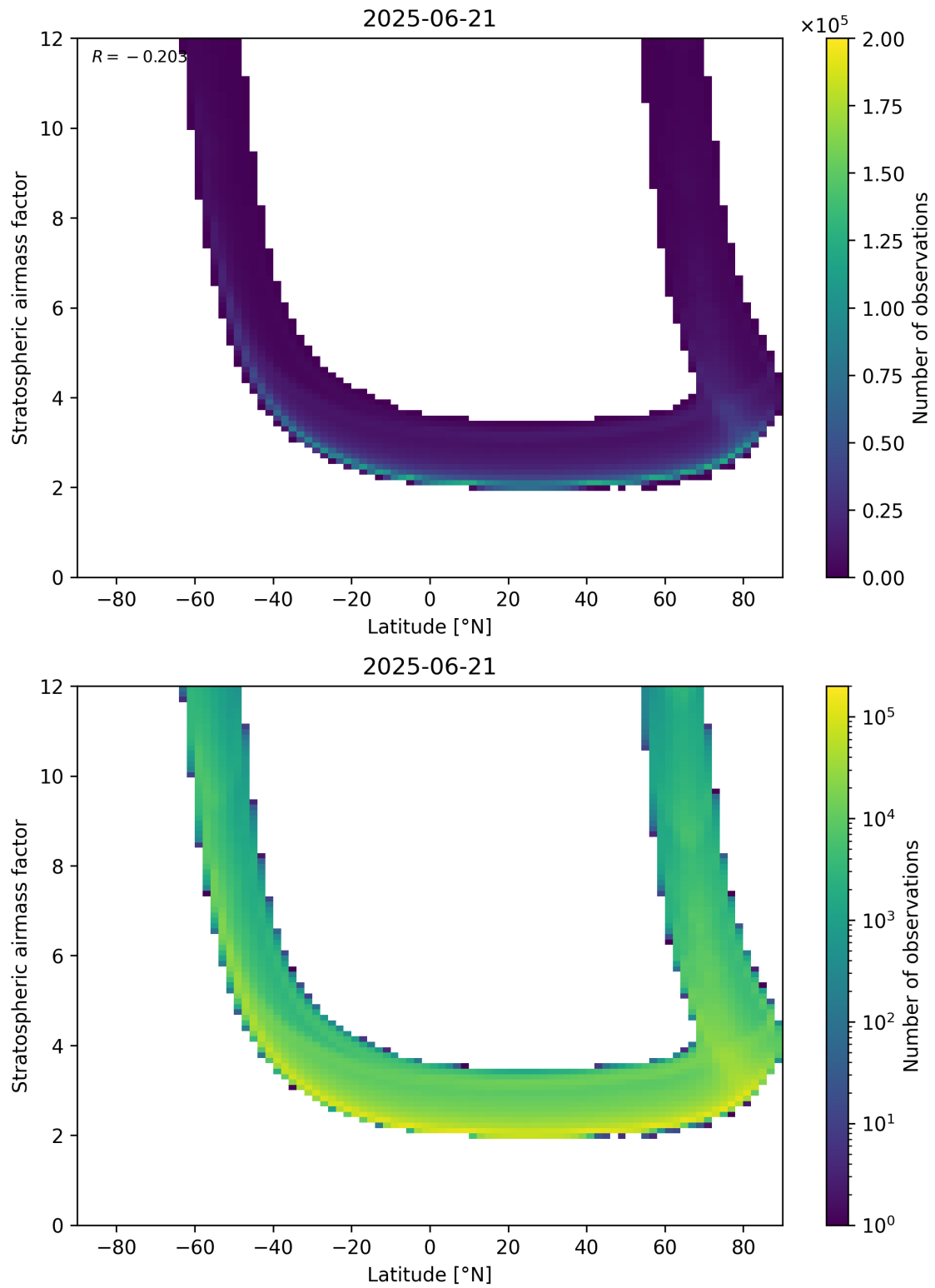
Figure 83: Scatter density plot of “Latitude” against “Stratospheric air mass factor” for 2025-06-20 to 2025-06-22.
