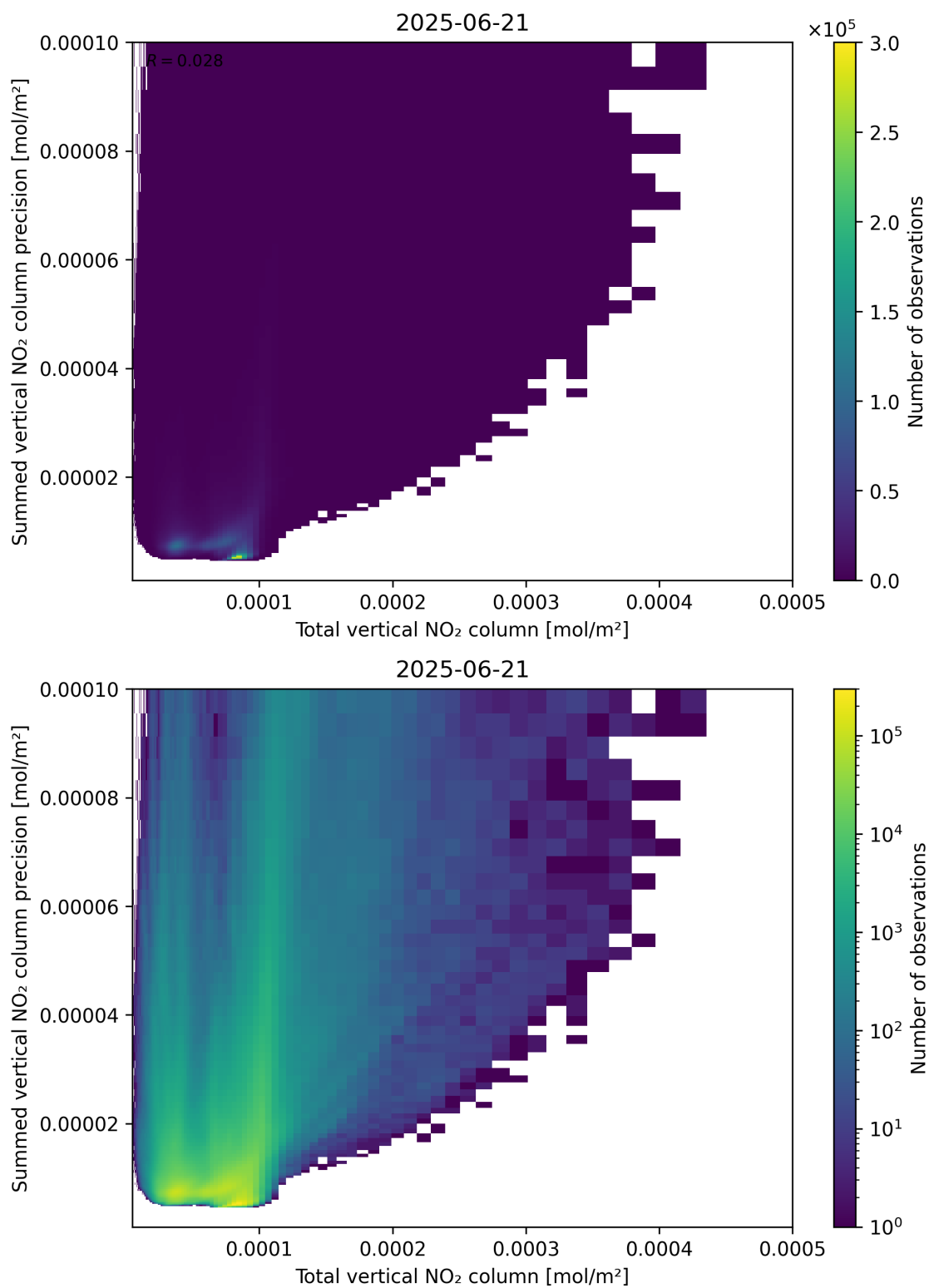
Figure 113: Scatter density plot of “Total vertical NO 2 column” against “Summed vertical NO 2 column precision” for 2025-06-20 to 2025-06-22.
