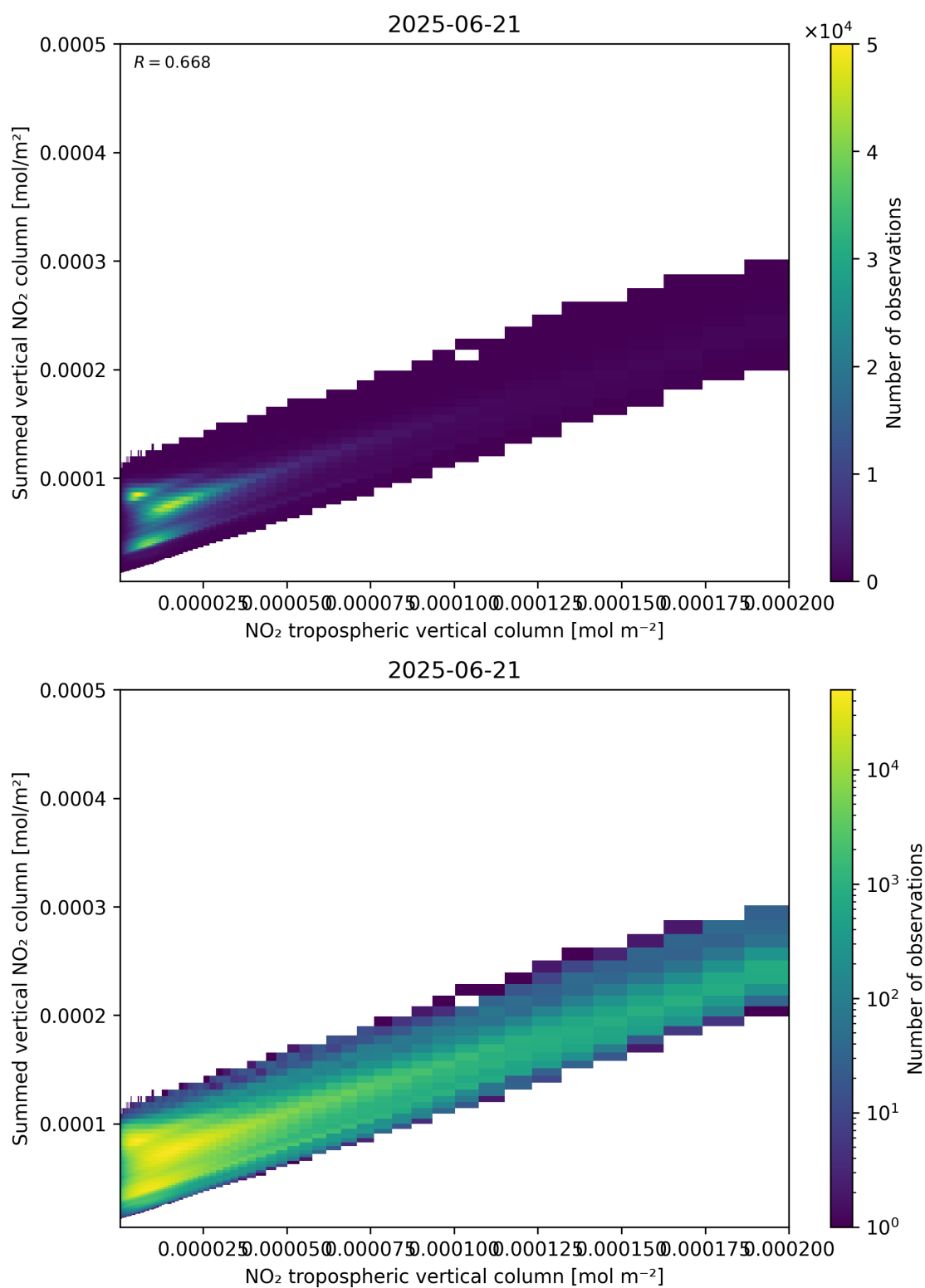
Figure 126: Scatter density plot of “NO 2 tropospheric vertical column” against “Summed vertical NO 2 column” for 2025-06-20 to 2025-06-22.
