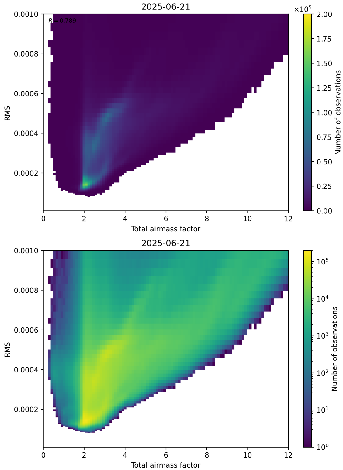
Figure 69: Scatter density plot of “Total airmass factor” against “RMS” for 2025-06-20 to 2025-06-22.
