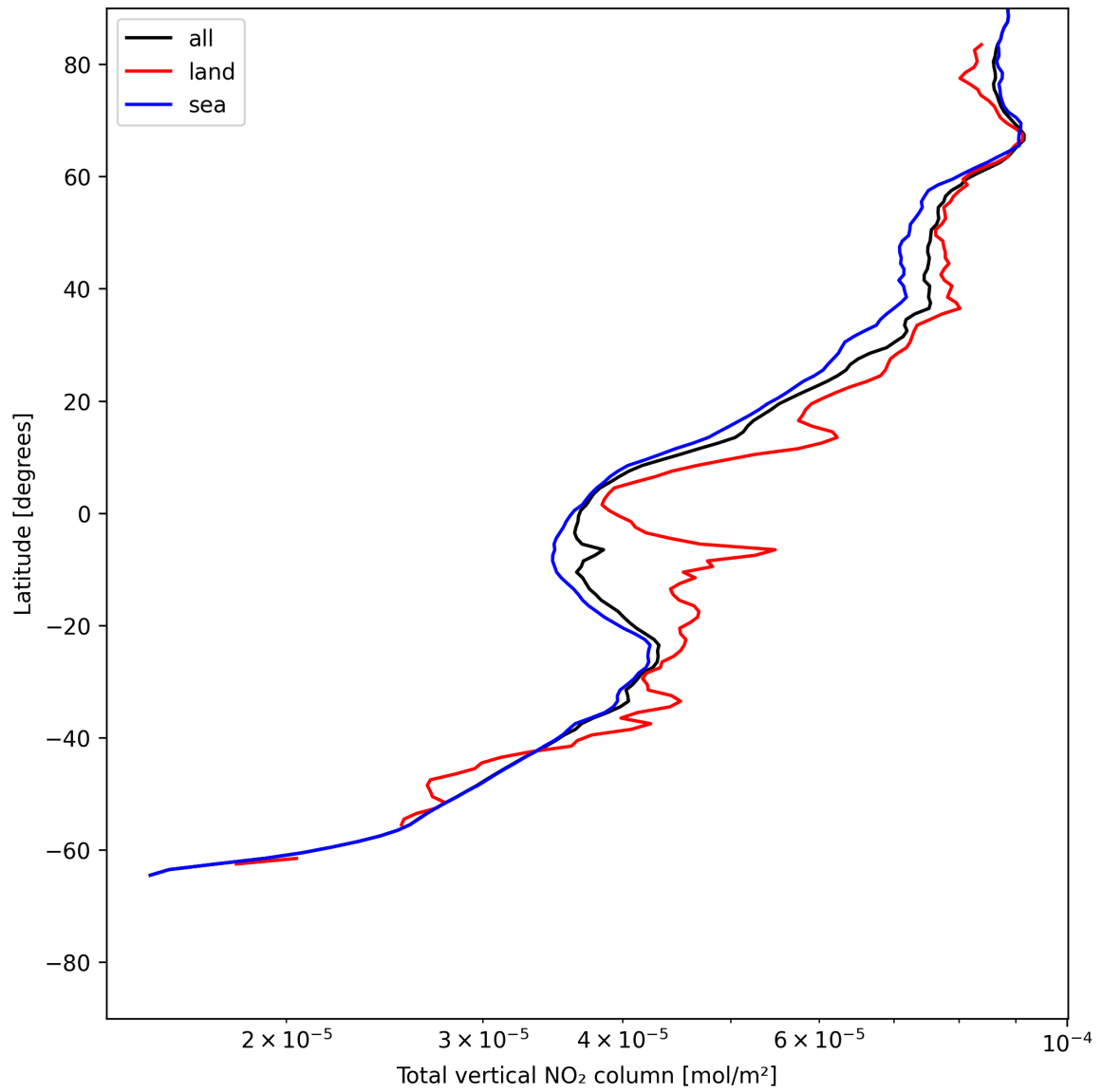
Figure 21: Zonal average of “Total vertical NO 2 column” for 2025-06-20 to 2025-06-22.
