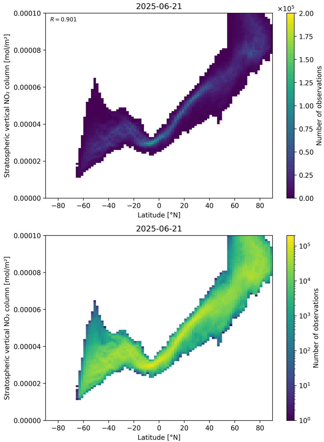
Figure 87: Scatter density plot of “Latitude” against “Stratospheric vertical \text{NO}_2 column” for 2025-06-20 to 2025-06-22.
