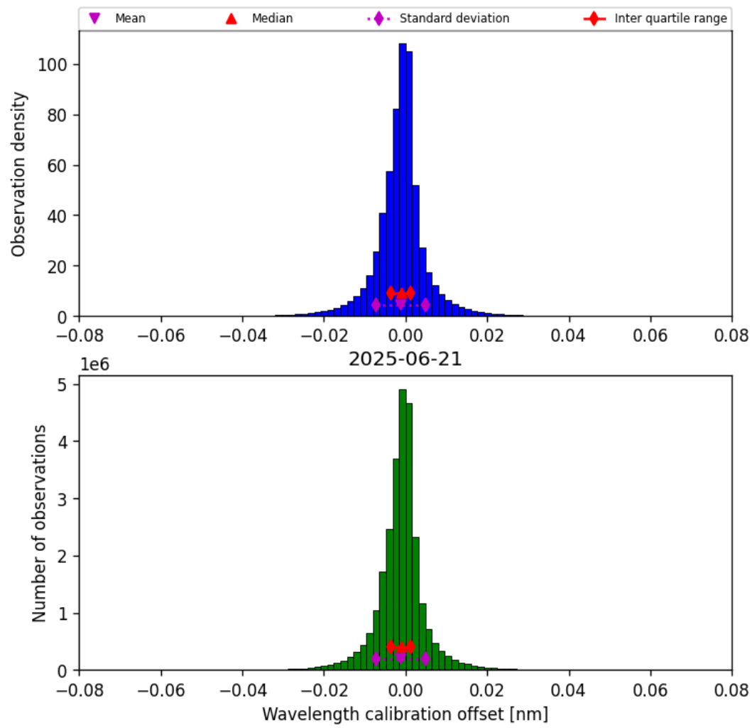
Figure 35: Histogram of “Wavelength calibration offset” for 2025-06-20 to 2025-06-22
