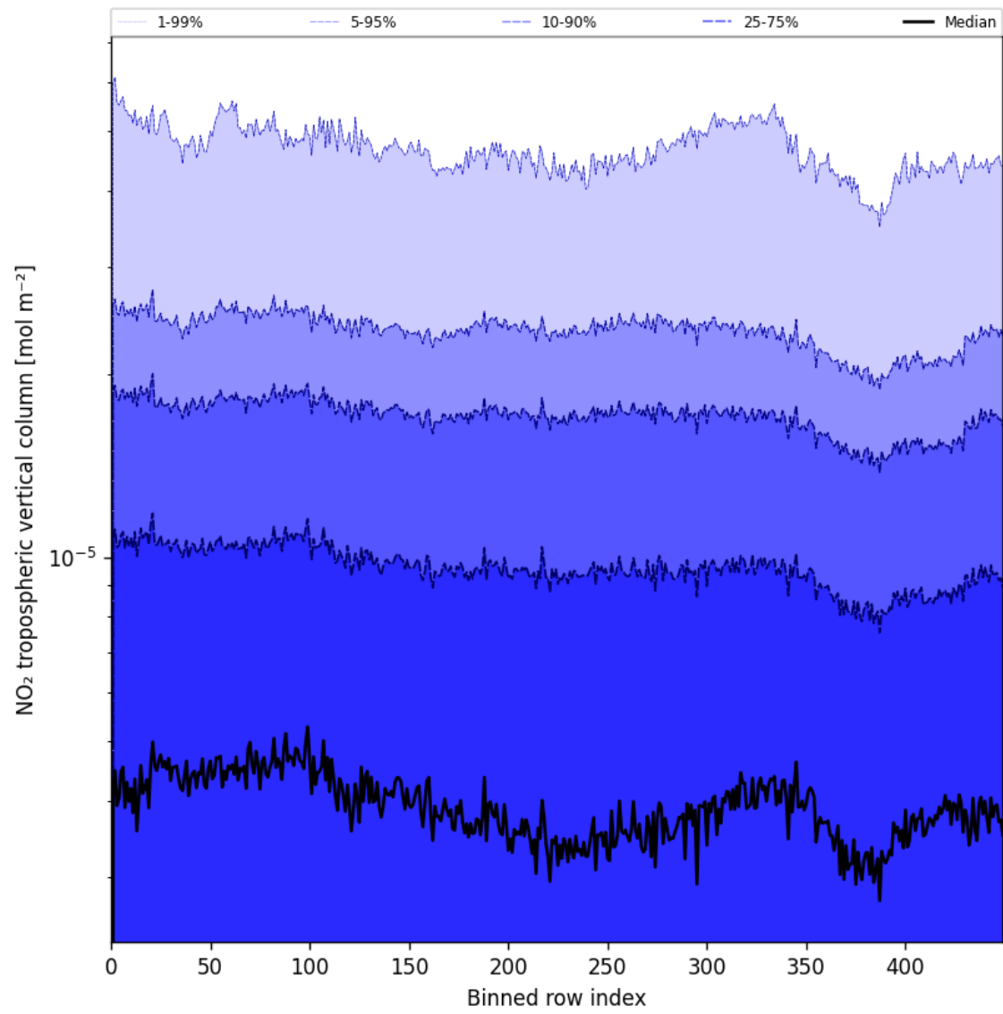
Figure 46: Along track statistics of “NO 2 tropospheric vertical column” for 2025-06-20 to 2025-06-22
