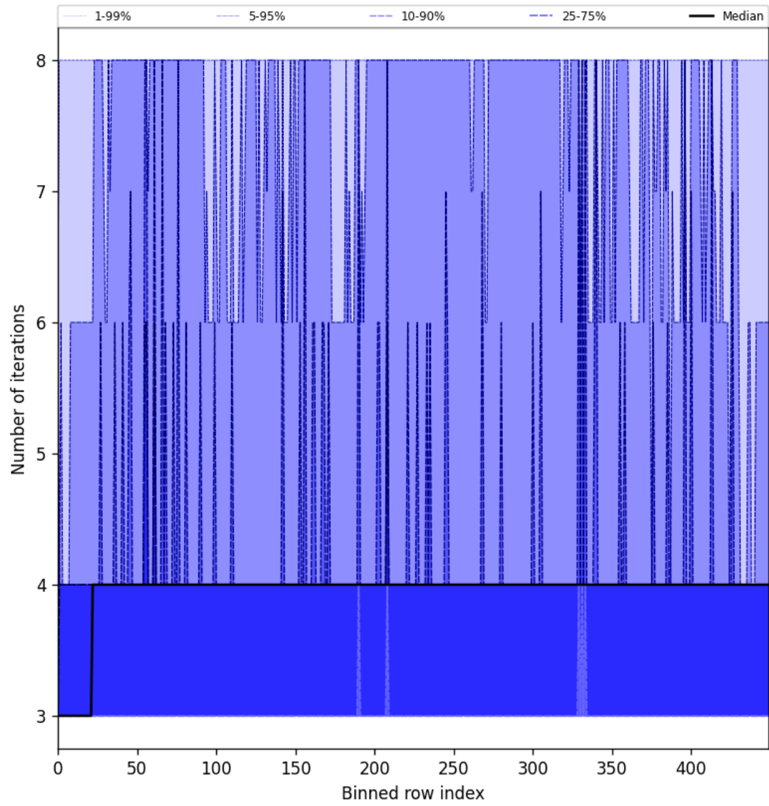
Figure 51: Along track statistics of “Number of iterations” for 2025-06-20 to 2025-06-22
