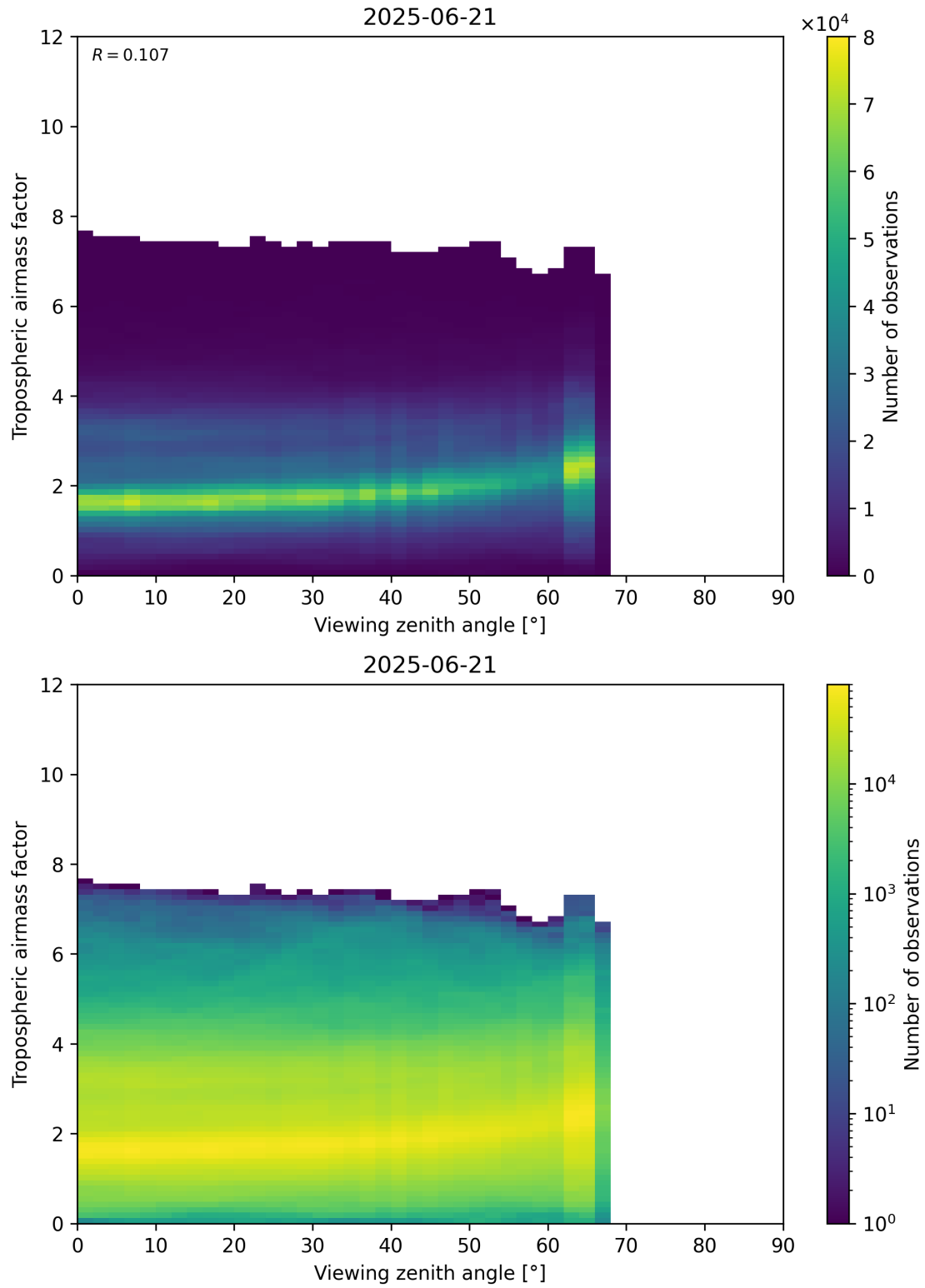
Figure 161: Scatter density plot of “Viewing zenith angle” against “Tropospheric airmass factor” for 2025-06-20 to 2025-06-22.
