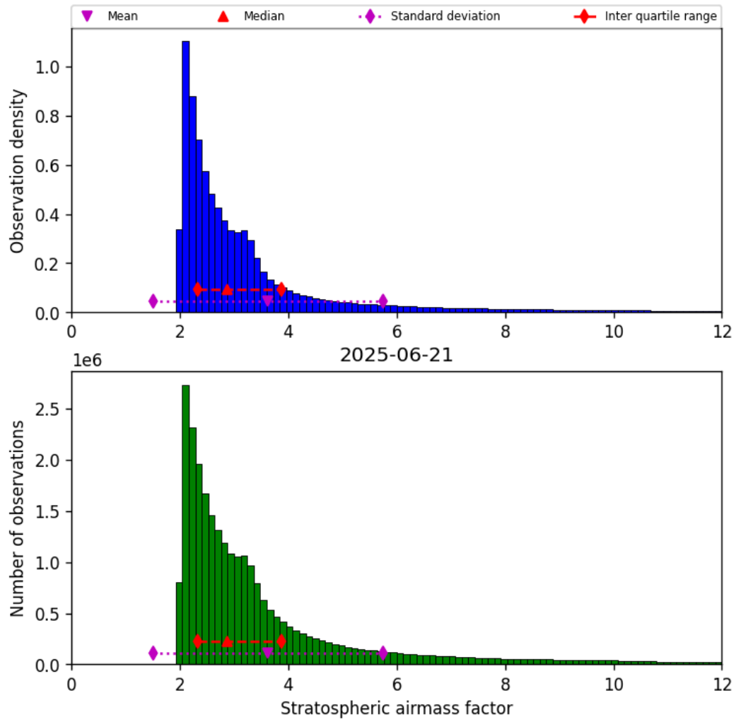
Figure 44: Histogram of “Stratospheric airmass factor” for 2025-06-20 to 2025-06-22
