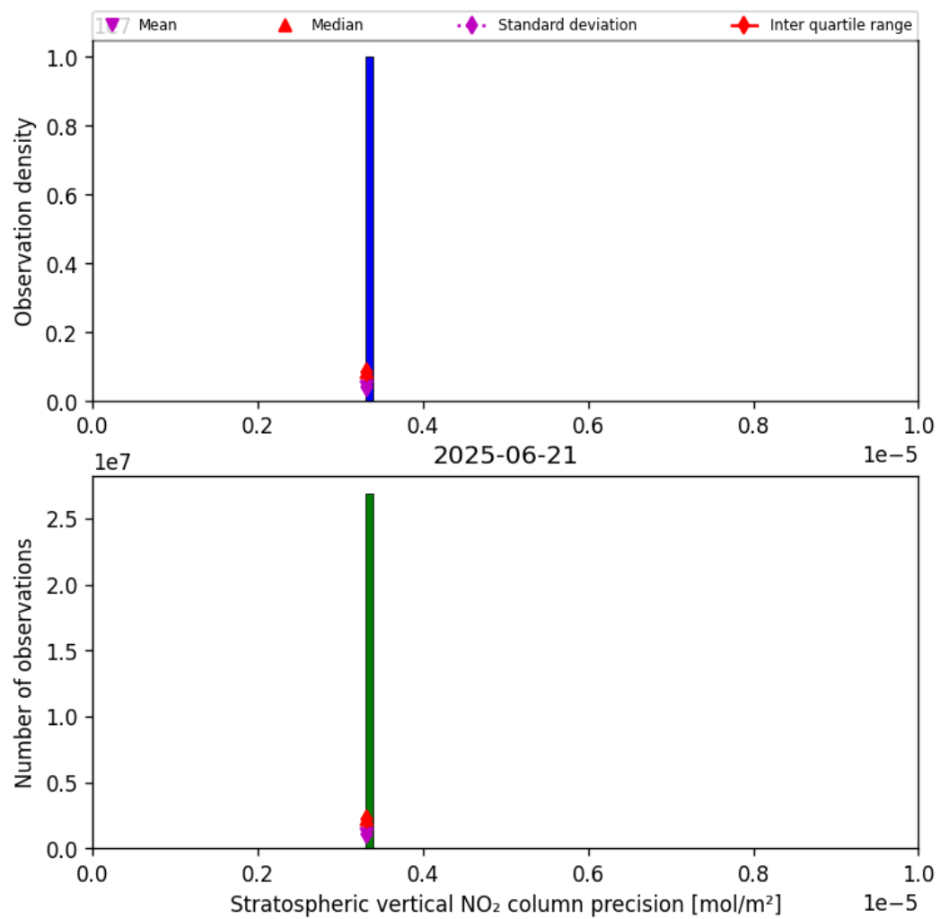
Figure 37: Histogram of “Stratospheric vertical NO 2 column precision” for 2025-06-20 to 2025-06-22
