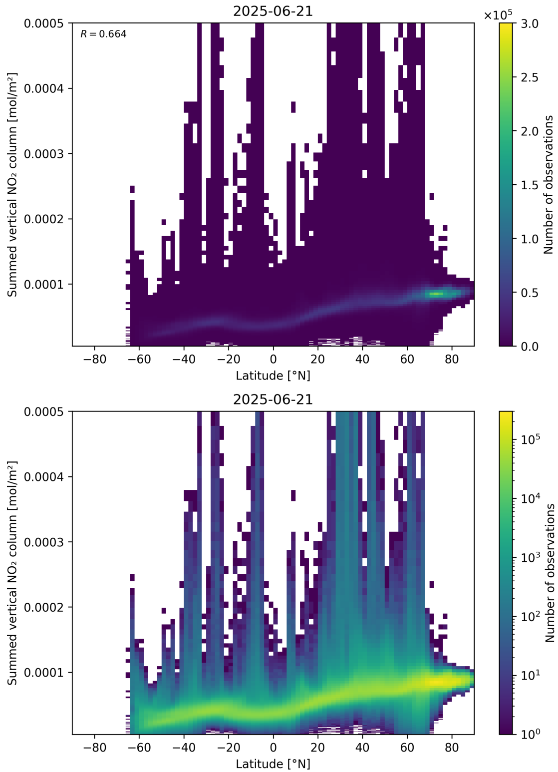
Figure 88: Scatter density plot of “Latitude” against “Summed vertical NO 2 column” for 2025-06-20 to 2025-06-22.
