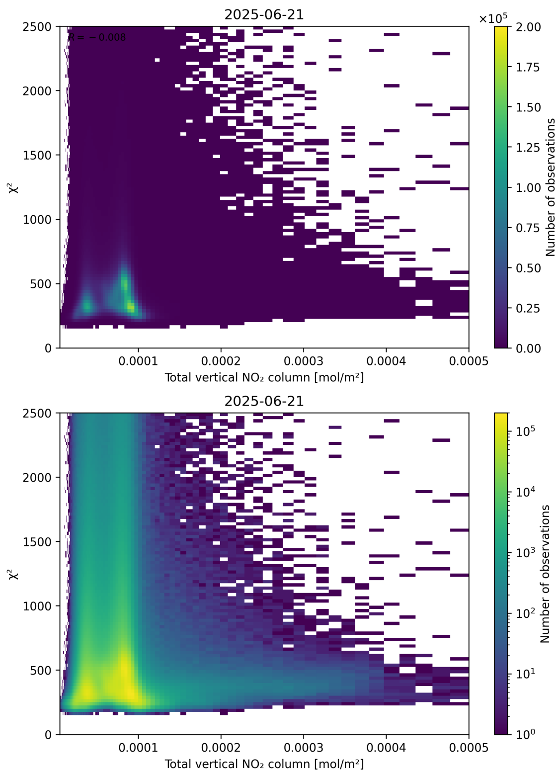
Figure 111: Scatter density plot of “Total vertical NO 2 column” against “ \chi^2 ” for 2025-06-20 to 2025-06-22.
