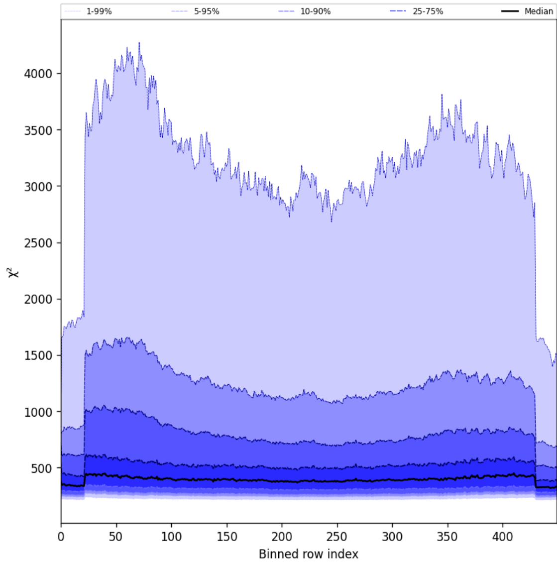
Figure 59: Along track statistics of “ \chi^2 ” for 2025-06-20 to 2025-06-22
