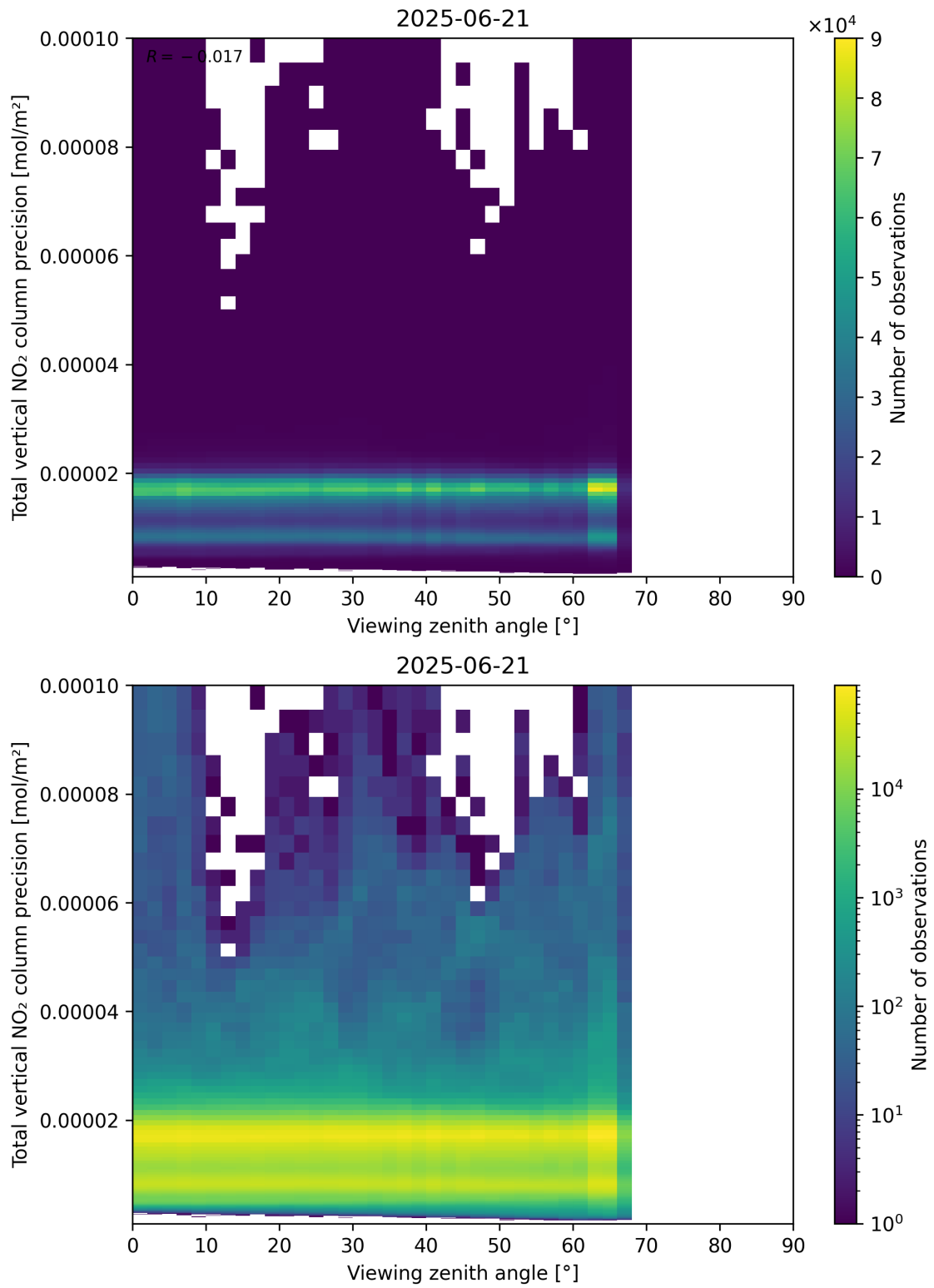
Figure 168: Scatter density plot of “Viewing zenith angle” against “Total vertical NO 2 column precision” for 2025-06-20 to 2025-06-22.
