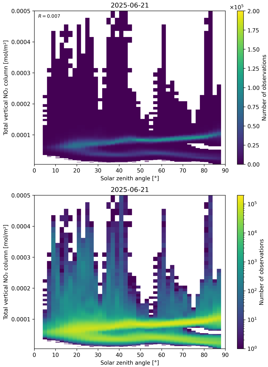
Figure 153: Scatter density plot of “Solar zenith angle” against “Total vertical NO 2 column” for 2025-06-20 to 2025-06-22.
