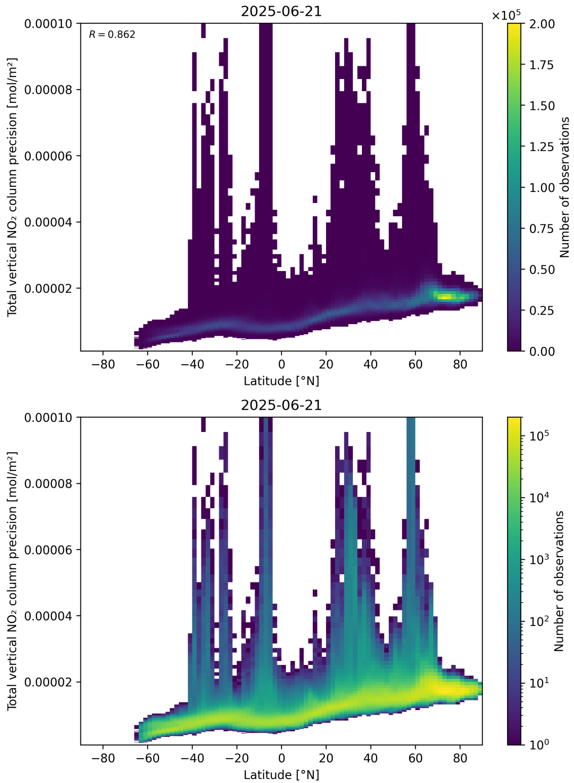
Figure 91: Scatter density plot of “Latitude” against “Total vertical NO 2 column precision” for 2025-06-20 to 2025-06-22.
