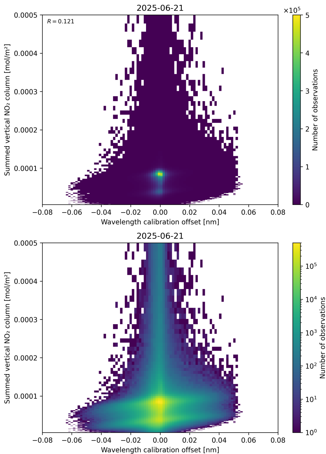
Figure 177: Scatter density plot of “Wavelength calibration offset” against “Summed vertical NO 2 column” for 2025-06-20 to 2025-06-22.
