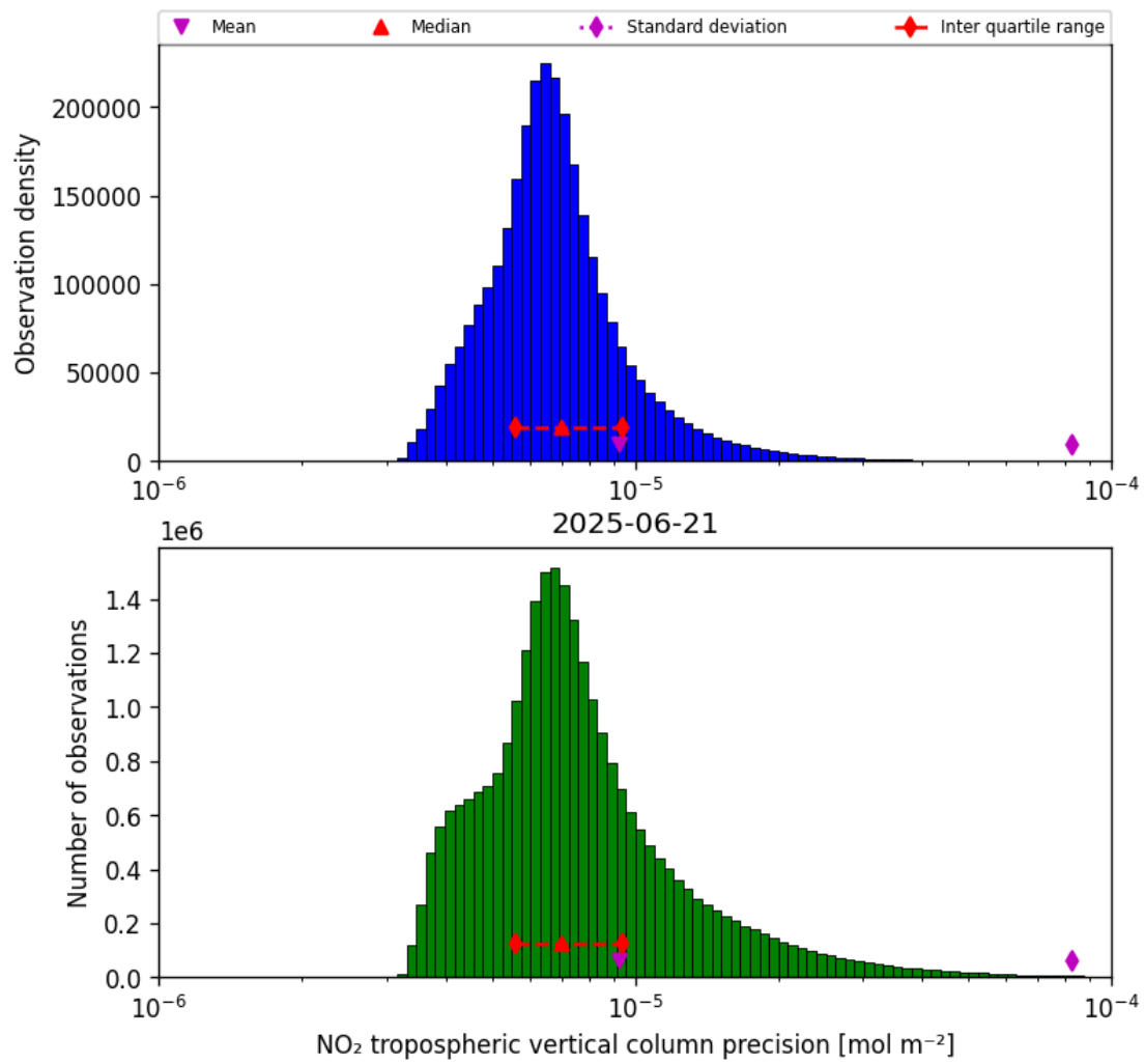
Figure 30: Histogram of “NO 2 tropospheric vertical column precision” for 2025-06-20 to 2025-06-22
