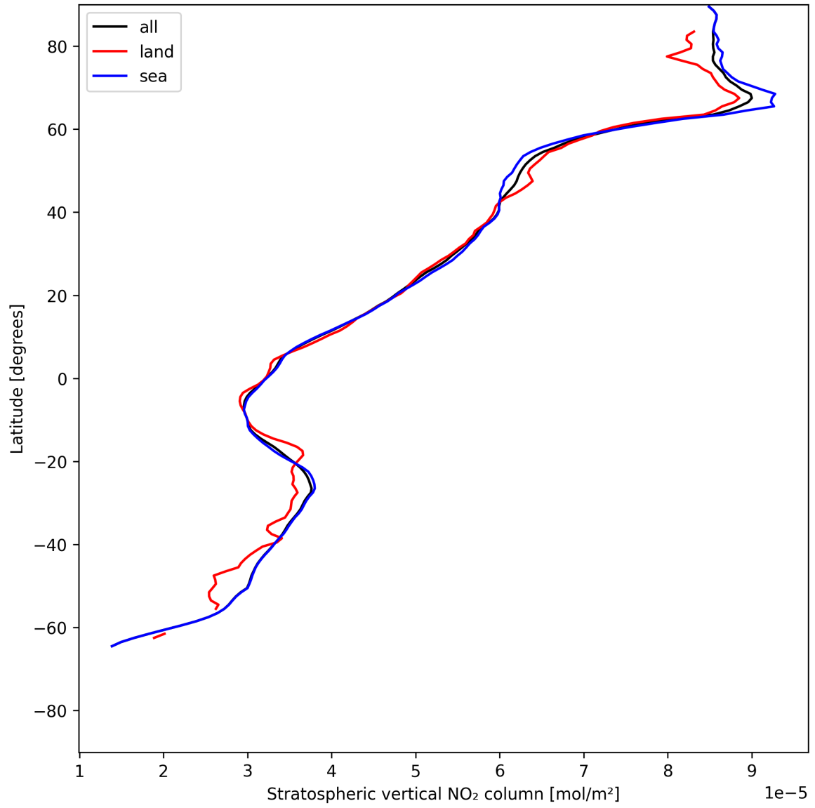
Figure 19: Zonal average of “Stratospheric vertical NO 2 column” for 2025-06-20 to 2025-06-22.
