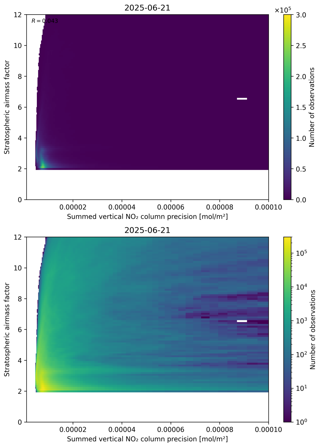
Figure 106: Scatter density plot of “Summed vertical NO 2 column precision” against “Stratospheric airmass factor” for 2025-06-20 to 2025-06-22.
