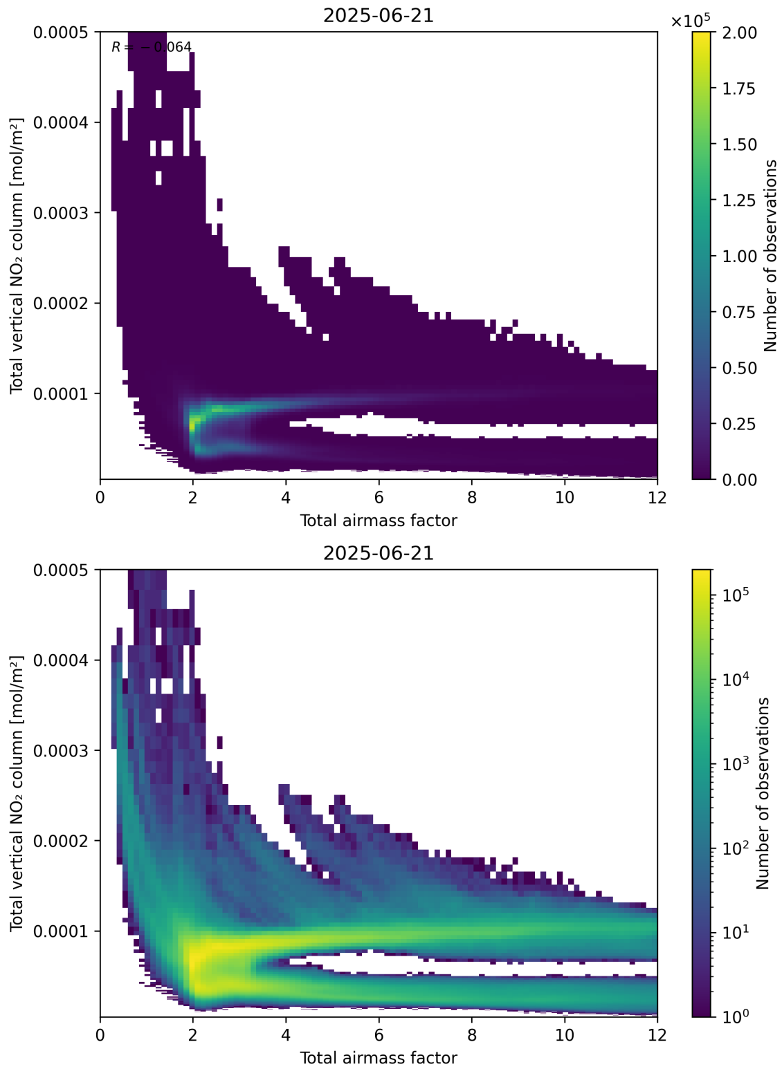
Figure 67: Scatter density plot of “Total airmass factor” against “Total vertical NO 2 column” for 2025-06-20 to 2025-06-22.
