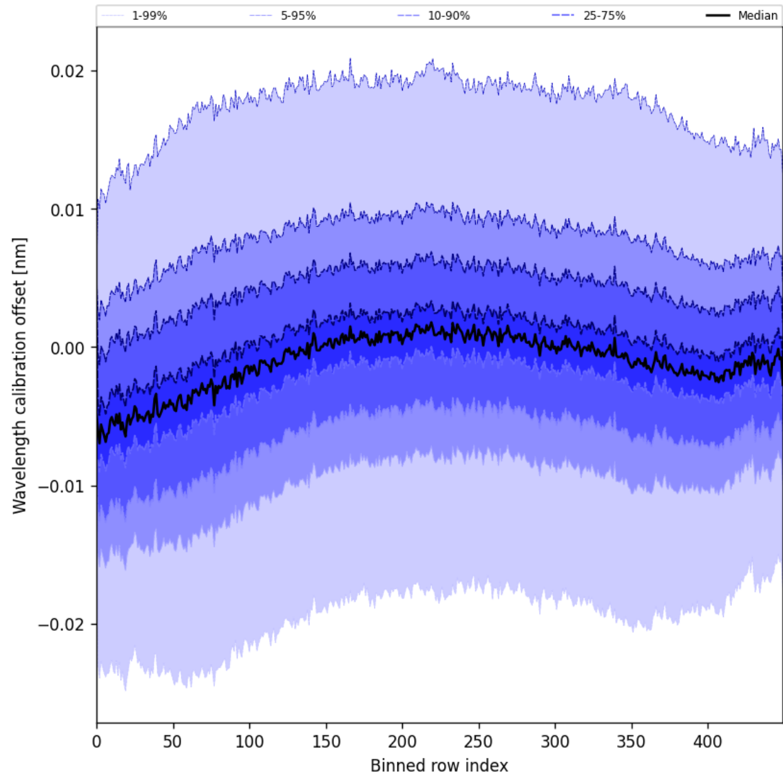
Figure 52: Along track statistics of “Wavelength calibration offset” for 2025-06-20 to 2025-06-22
