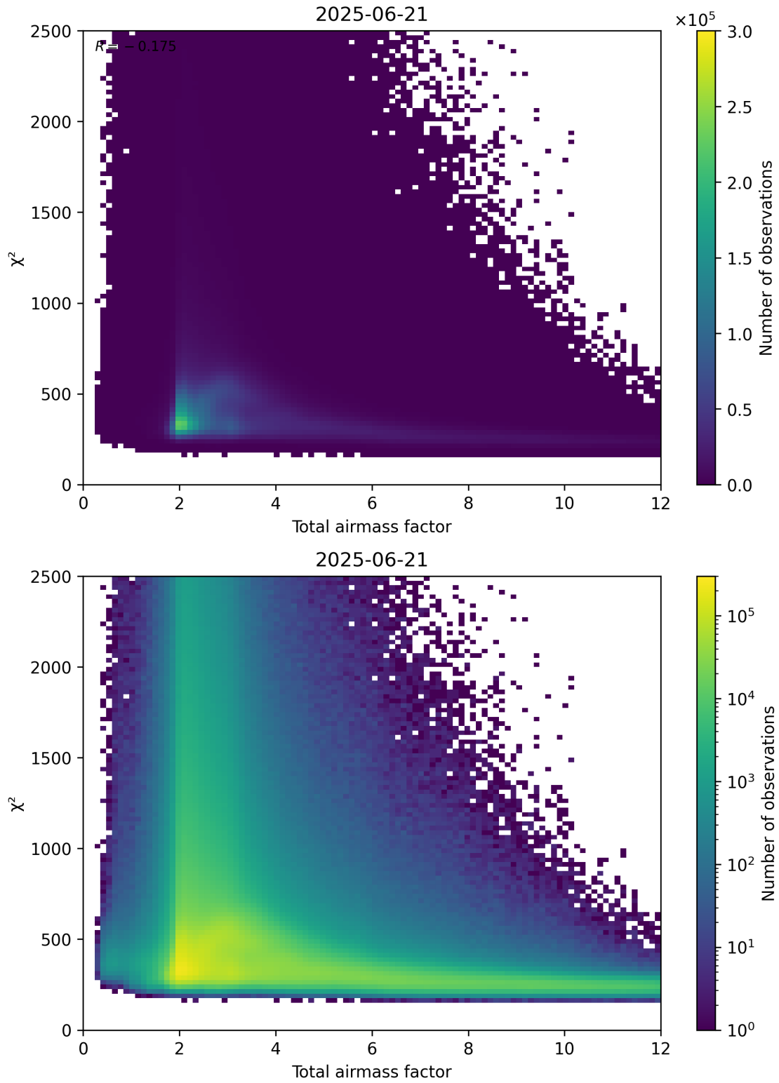
Figure 63: Scatter density plot of “Total airmass factor” against “ \chi^2 ” for 2025-06-20 to 2025-06-22.
