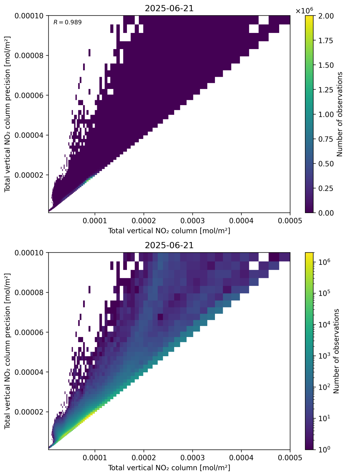
Figure 114: Scatter density plot of “Total vertical NO 2 column” against “Total vertical NO 2 column precision” for 2025-06-20 to 2025-06-22.
