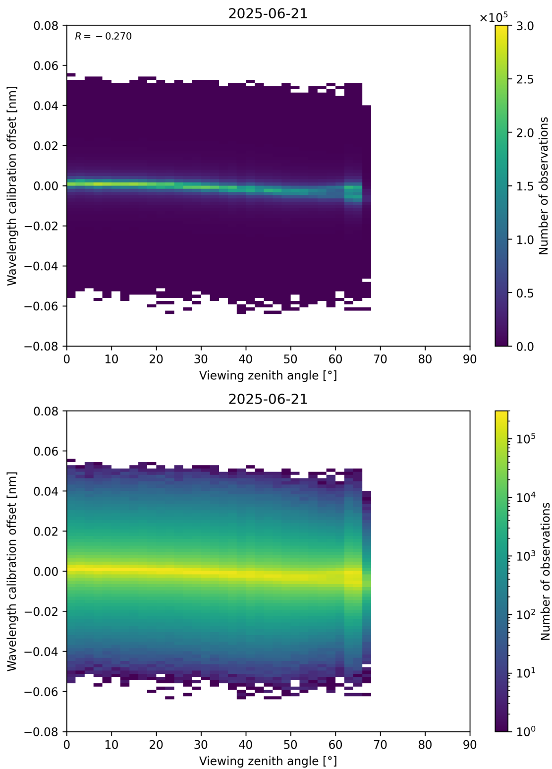
Figure 173: Scatter density plot of “Viewing zenith angle” against “Wavelength calibration offset” for 2025-06-20 to 2025-06-22.
