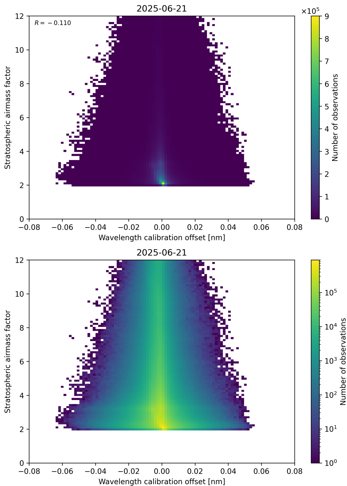
Figure 174: Scatter density plot of “Wavelength calibration offset” against “Stratospheric airmass factor” for 2025-06-20 to 2025-06-22.
