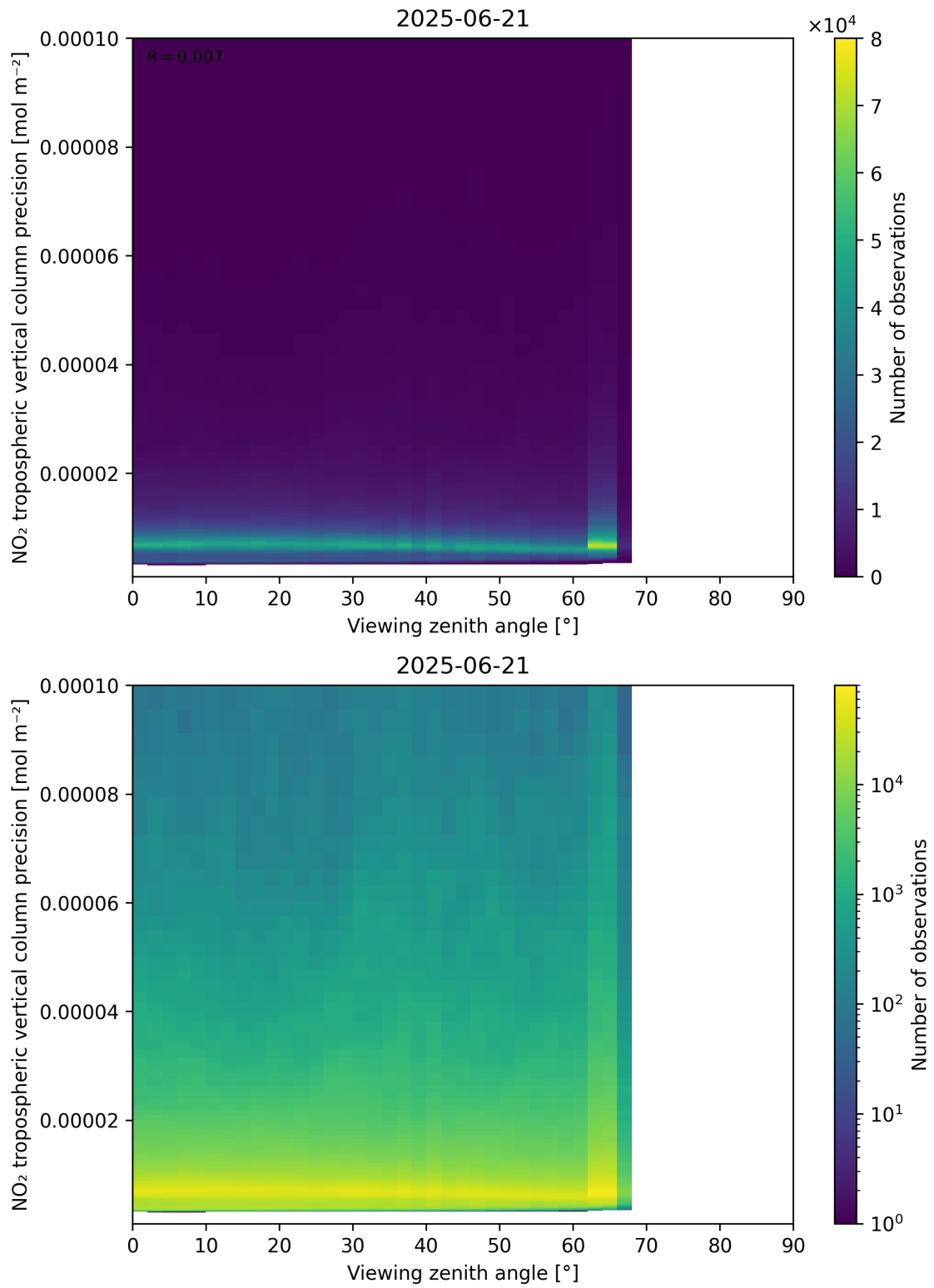
Figure 170: Scatter density plot of “Viewing zenith angle” against “NO 2 tropospheric vertical column precision” for 2025-06-20 to 2025-06-22.
