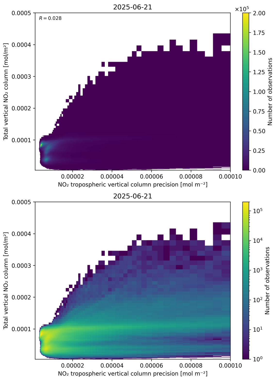
Figure 138: Scatter density plot of “NO 2 tropospheric vertical column precision” against “Total vertical NO 2 column” for 2025-06-20 to 2025-06-22.
