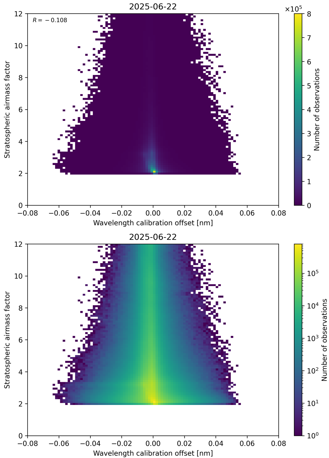
Figure 174: Scatter density plot of “Wavelength calibration offset” against “Stratospheric airmass factor” for 2025-06-22 to 2025-06-23.
