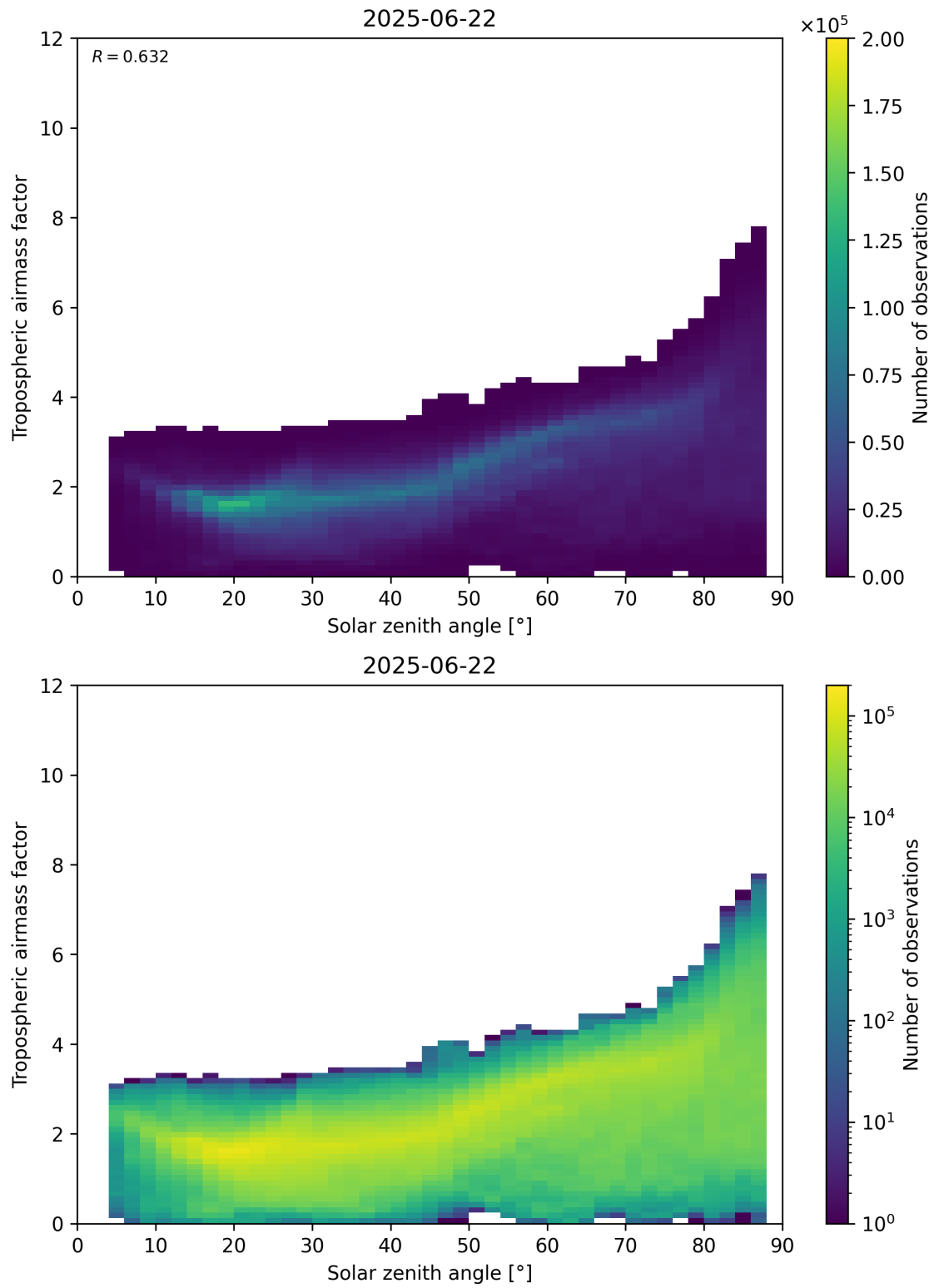
Figure 147: Scatter density plot of “Solar zenith angle” against “Tropospheric airmass factor” for 2025-06-22 to 2025-06-23.
