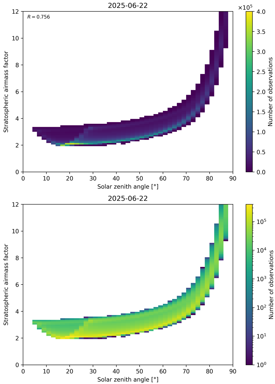
Figure 145: Scatter density plot of “Solar zenith angle” against “Stratospheric airmass factor” for 2025-06-22 to 2025-06-23.
