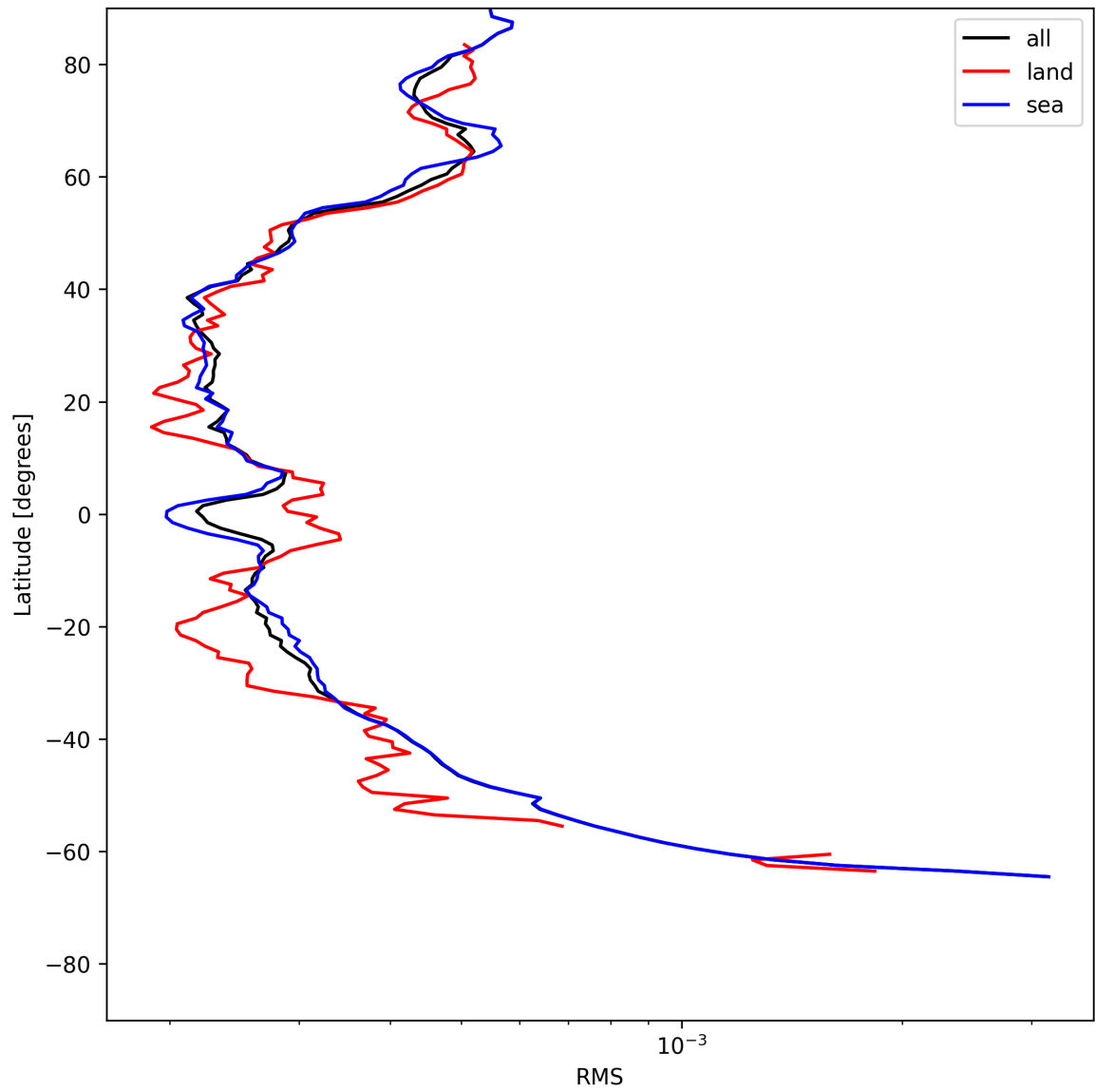
Figure 26: Zonal average of “RMS” for 2025-06-22 to 2025-06-23.
