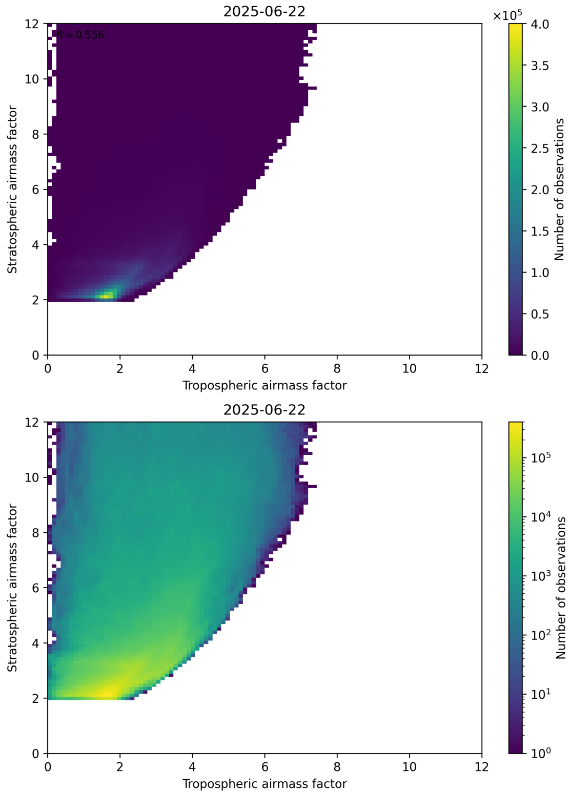
Figure 71: Scatter density plot of “Tropospheric airmass factor” against “Stratospheric airmass factor” for 2025-06-22 to 2025-06-23.
