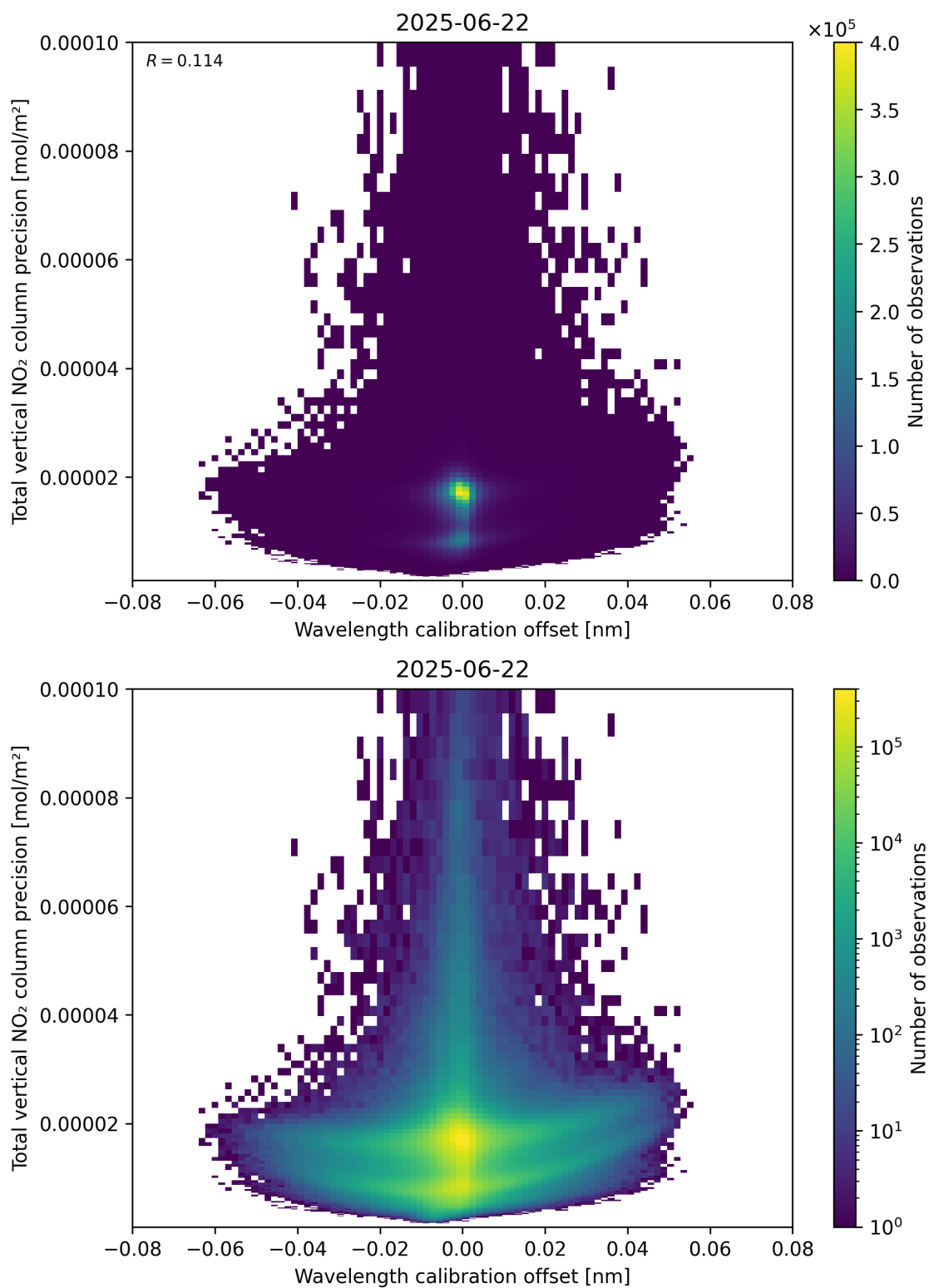
Figure 180: Scatter density plot of “Wavelength calibration offset” against “Total vertical NO 2 column precision” for 2025-06-22 to 2025-06-23.
