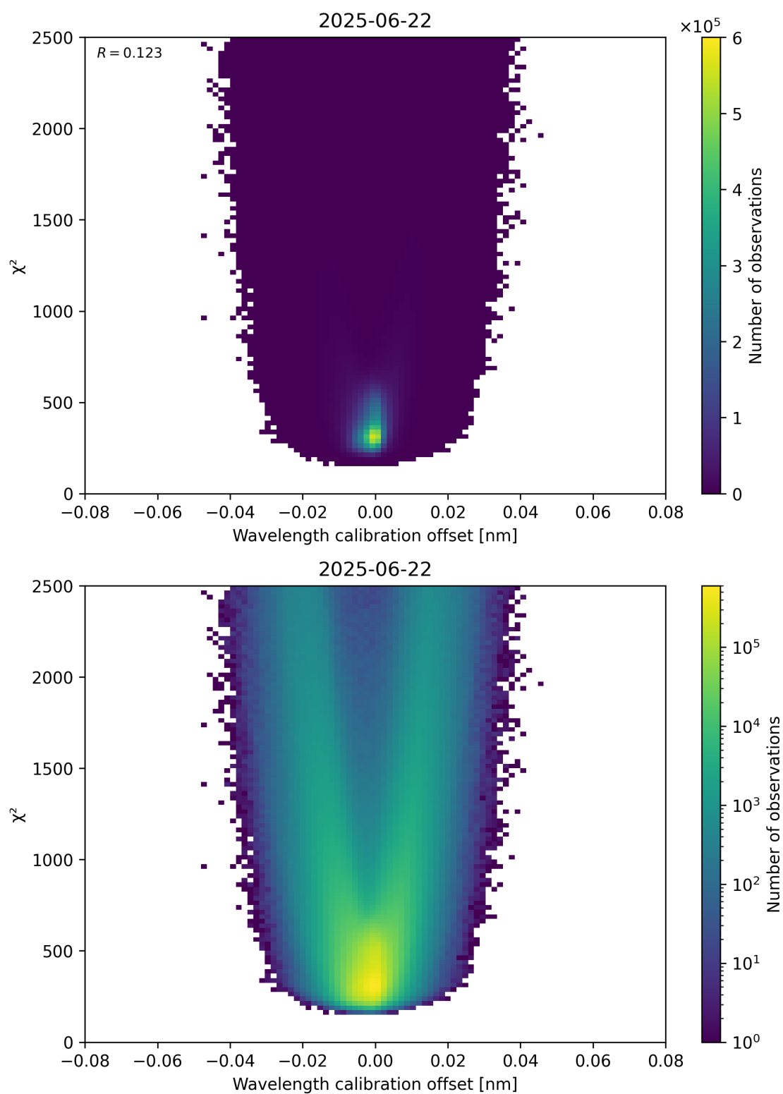
Figure 175: Scatter density plot of “Wavelength calibration offset” against “ \chi^2 ” for 2025-06-22 to 2025-06-23.
