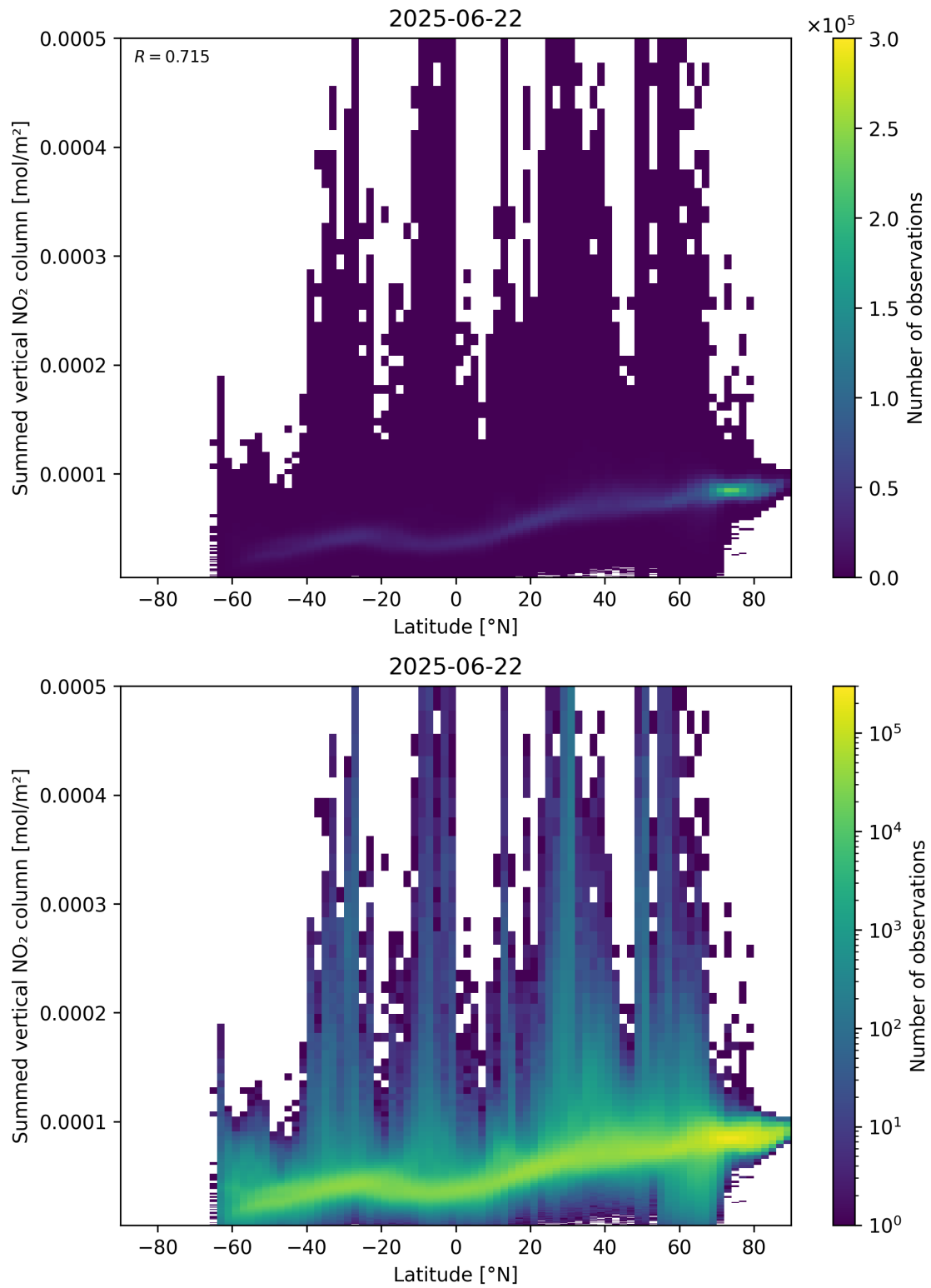
Figure 88: Scatter density plot of “Latitude” against “Summed vertical NO 2 column” for 2025-06-22 to 2025-06-23.
