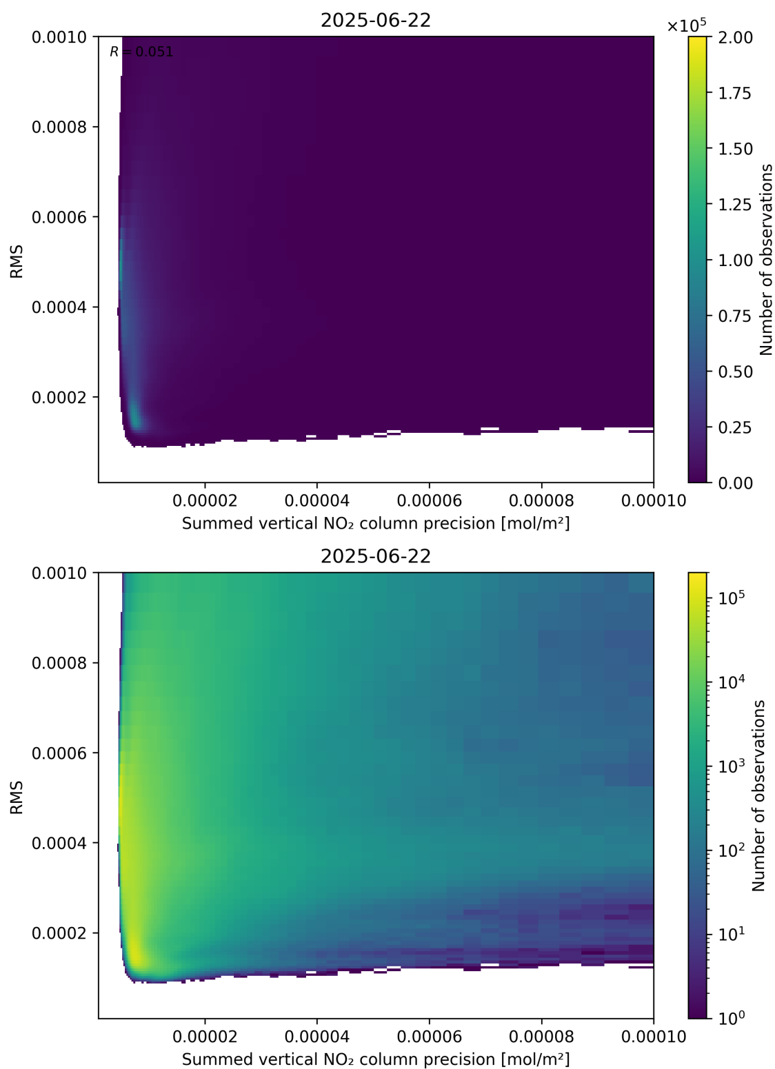
Figure 108: Scatter density plot of “Summed vertical NO 2 column precision” against “RMS” for 2025-06-22 to 2025-06-23.
