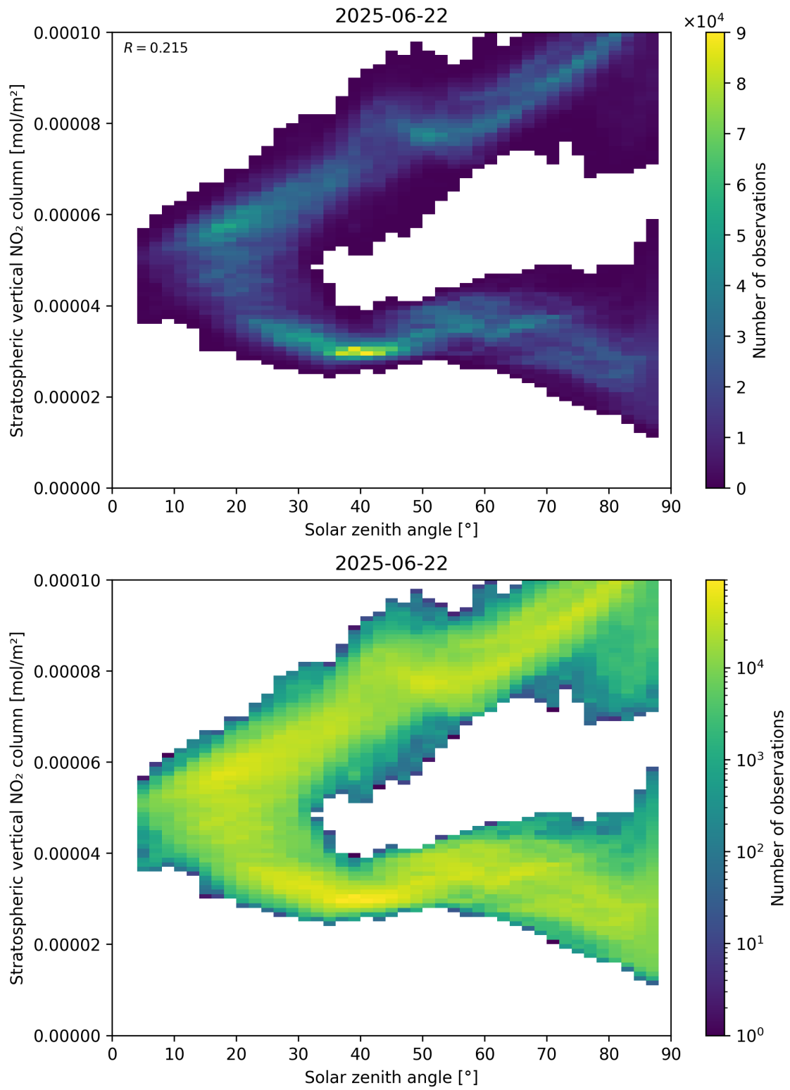
Figure 150: Scatter density plot of “Solar zenith angle” against “Stratospheric vertical NO 2 column” for 2025-06-22 to 2025-06-23.
