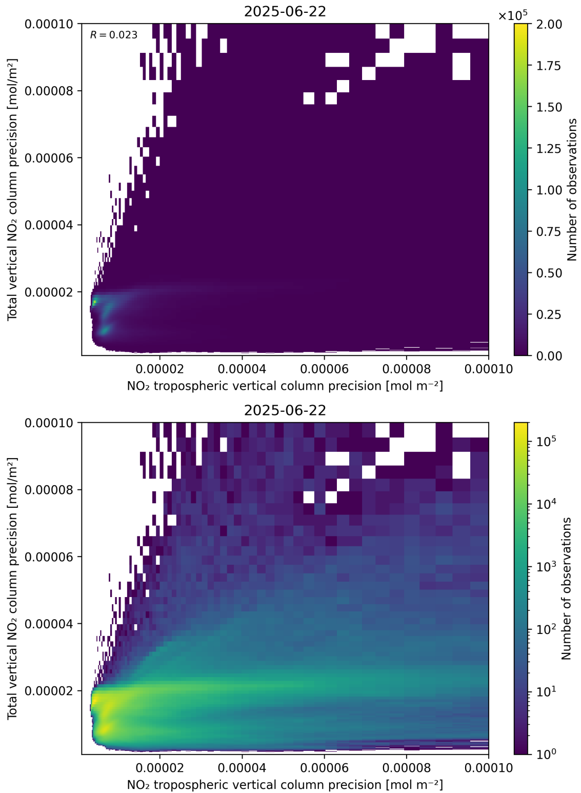
Figure 139: Scatter density plot of “NO 2 tropospheric vertical column precision” against “Total vertical NO 2 column precision” for 2025-06-22 to 2025-06-23.
