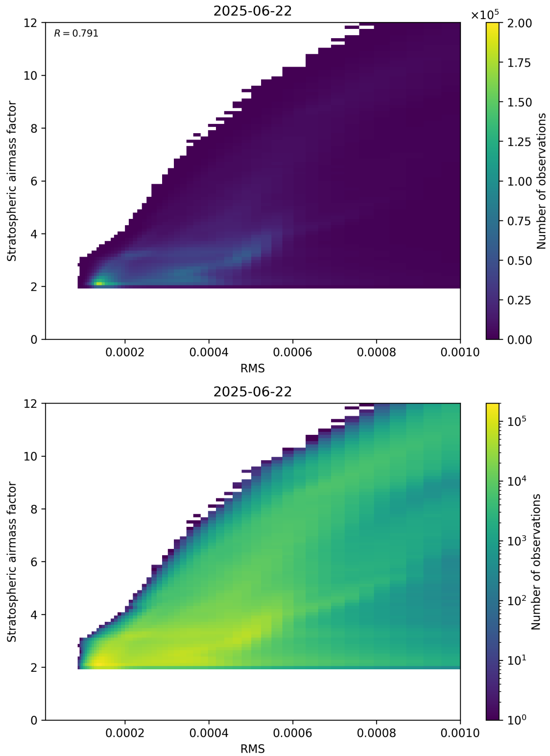
Figure 144: Scatter density plot of “RMS” against “Stratospheric airmass factor” for 2025-06-22 to 2025-06-23.
