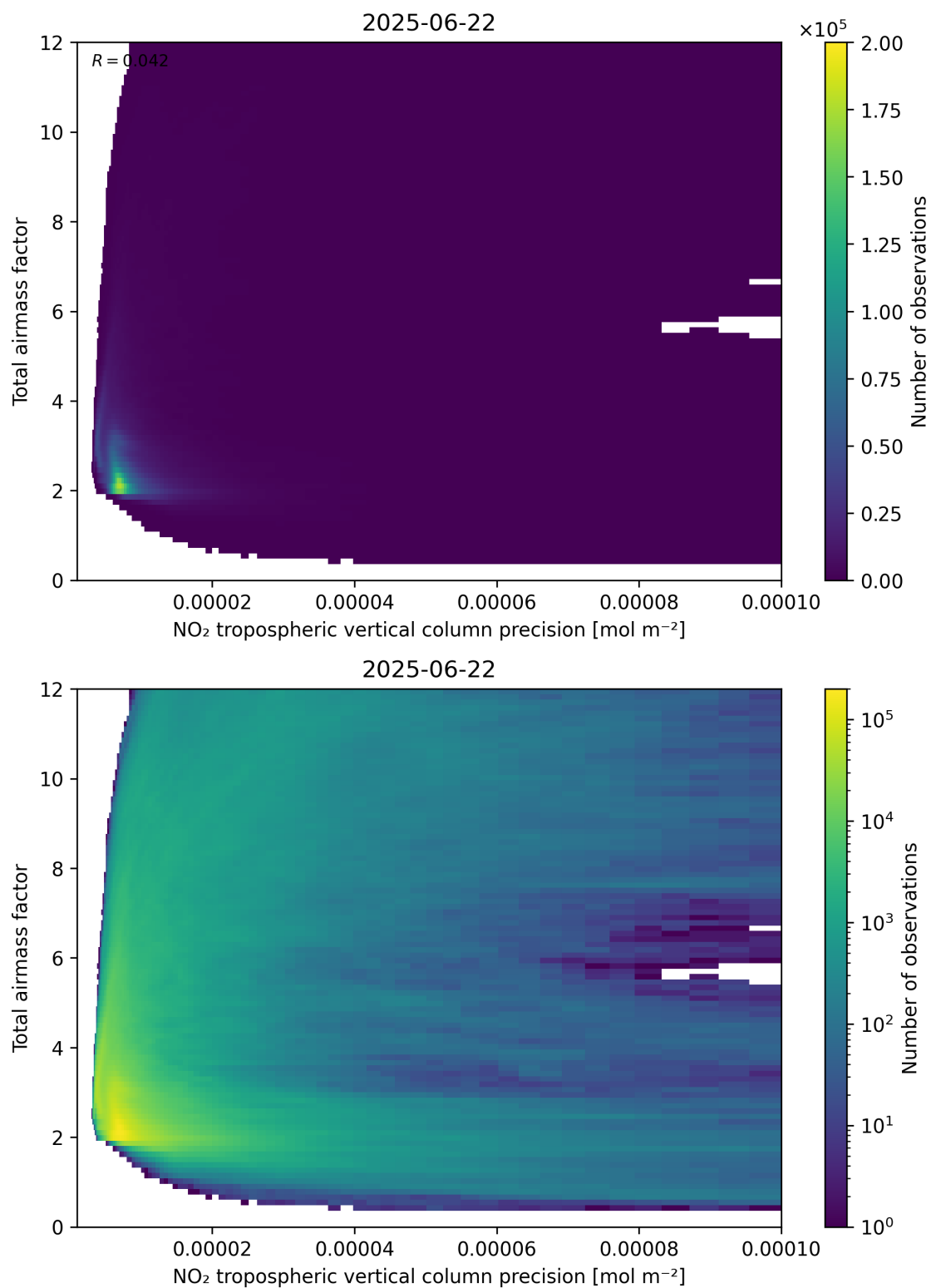
Figure 132: Scatter density plot of “NO 2 tropospheric vertical column precision” against “Total air mass factor” for 2025-06-22 to 2025-06-23.
