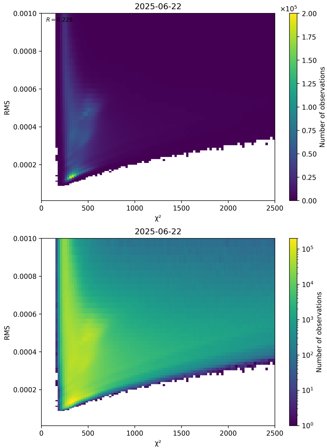
Figure 82: Scatter density plot of “ \chi^2 ” against “RMS” for 2025-06-22 to 2025-06-23.
