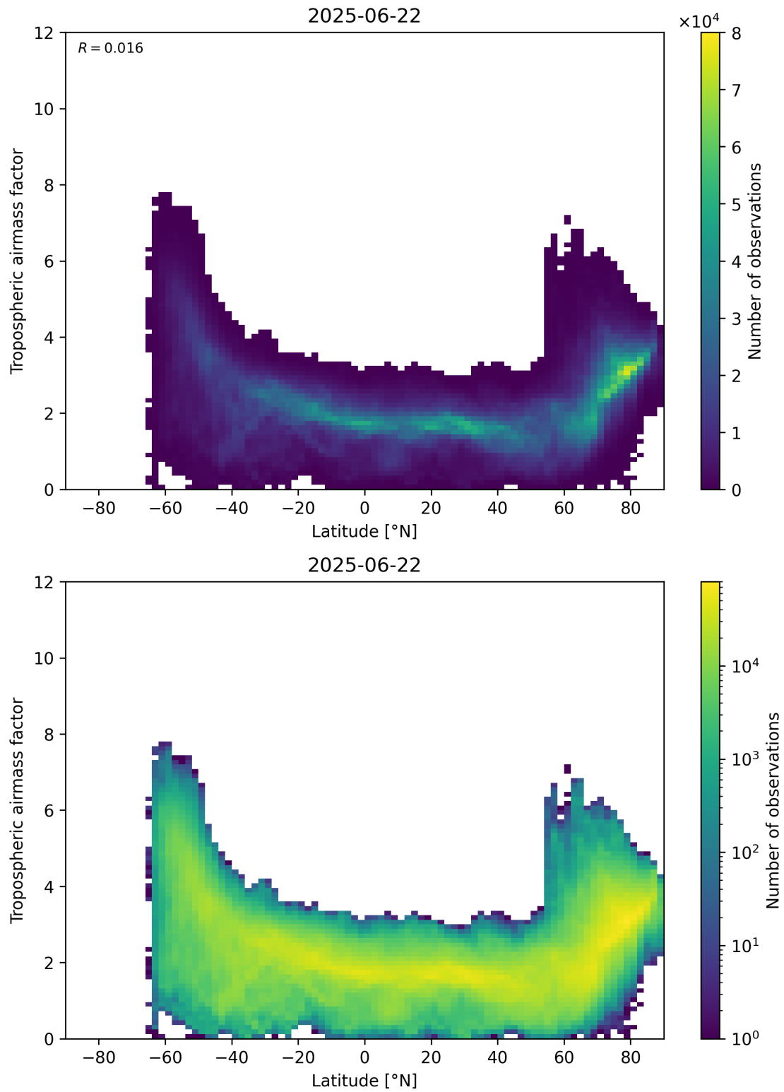
Figure 85: Scatter density plot of “Latitude” against “Tropospheric air mass factor” for 2025-06-22 to 2025-06-23.
