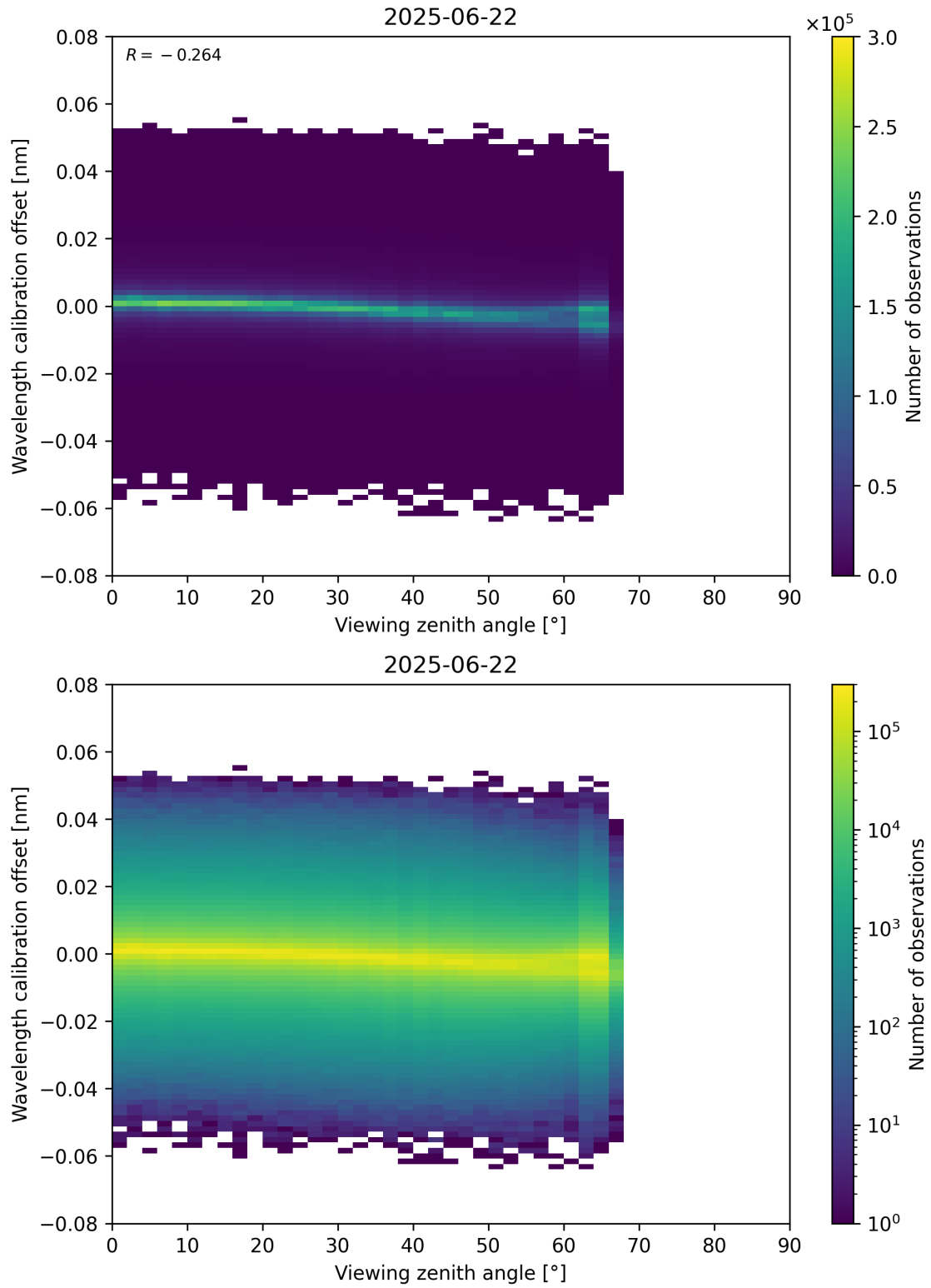
Figure 173: Scatter density plot of “Viewing zenith angle” against “Wavelength calibration offset” for 2025-06-22 to 2025-06-23.
