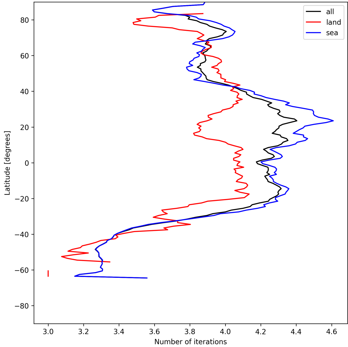
Figure 17: Zonal average of “Number of iterations” for 2025-06-22 to 2025-06-23.
