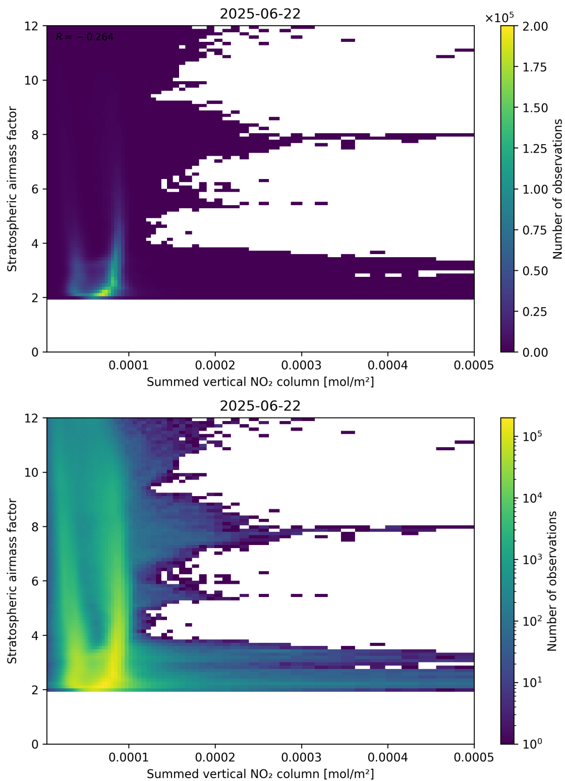
Figure 103: Scatter density plot of “Summed vertical NO 2 column” against “Stratospheric air mass factor” for 2025-06-22 to 2025-06-23.
