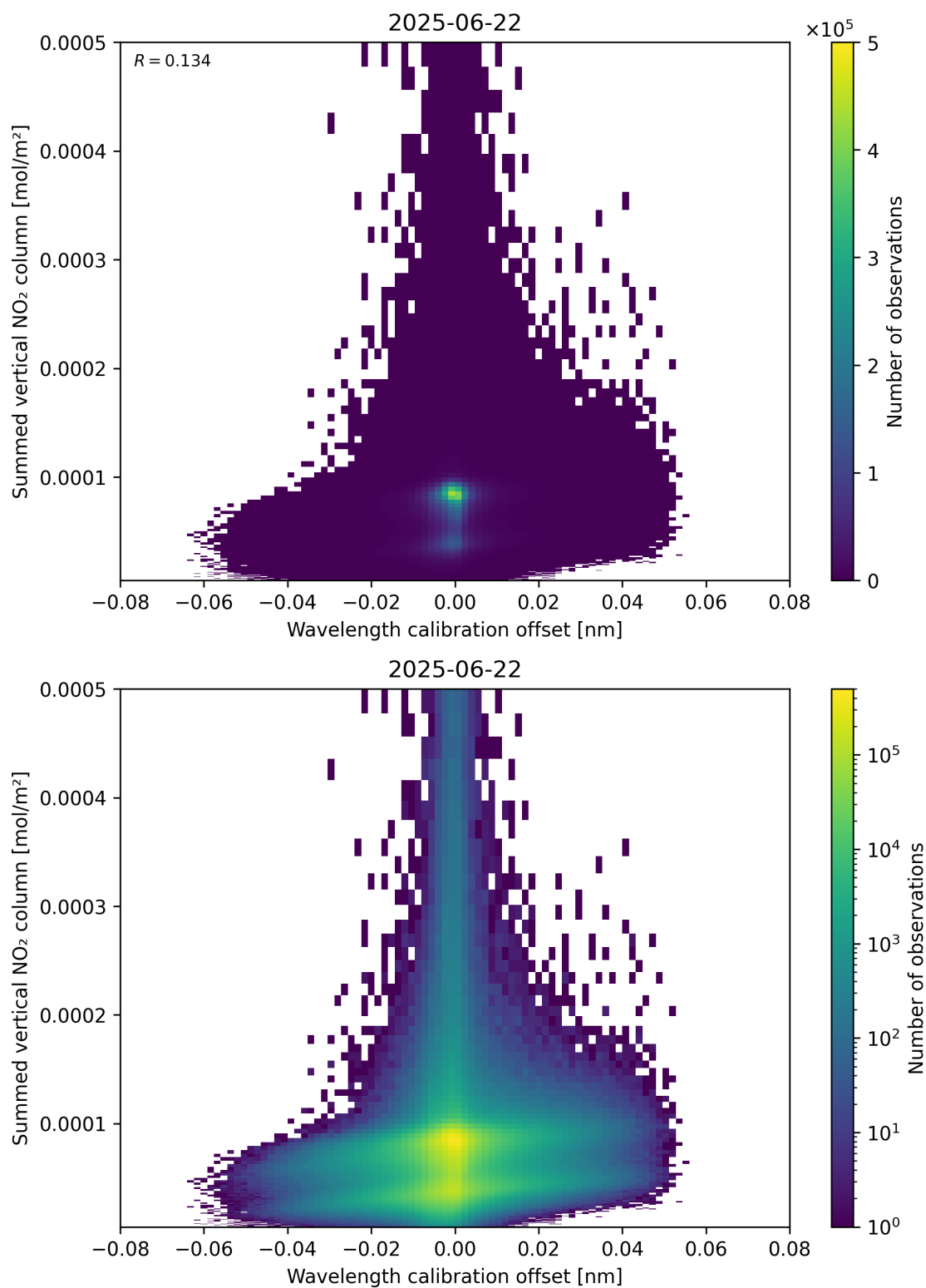
Figure 177: Scatter density plot of “Wavelength calibration offset” against “Summed vertical NO 2 column” for 2025-06-22 to 2025-06-23.
