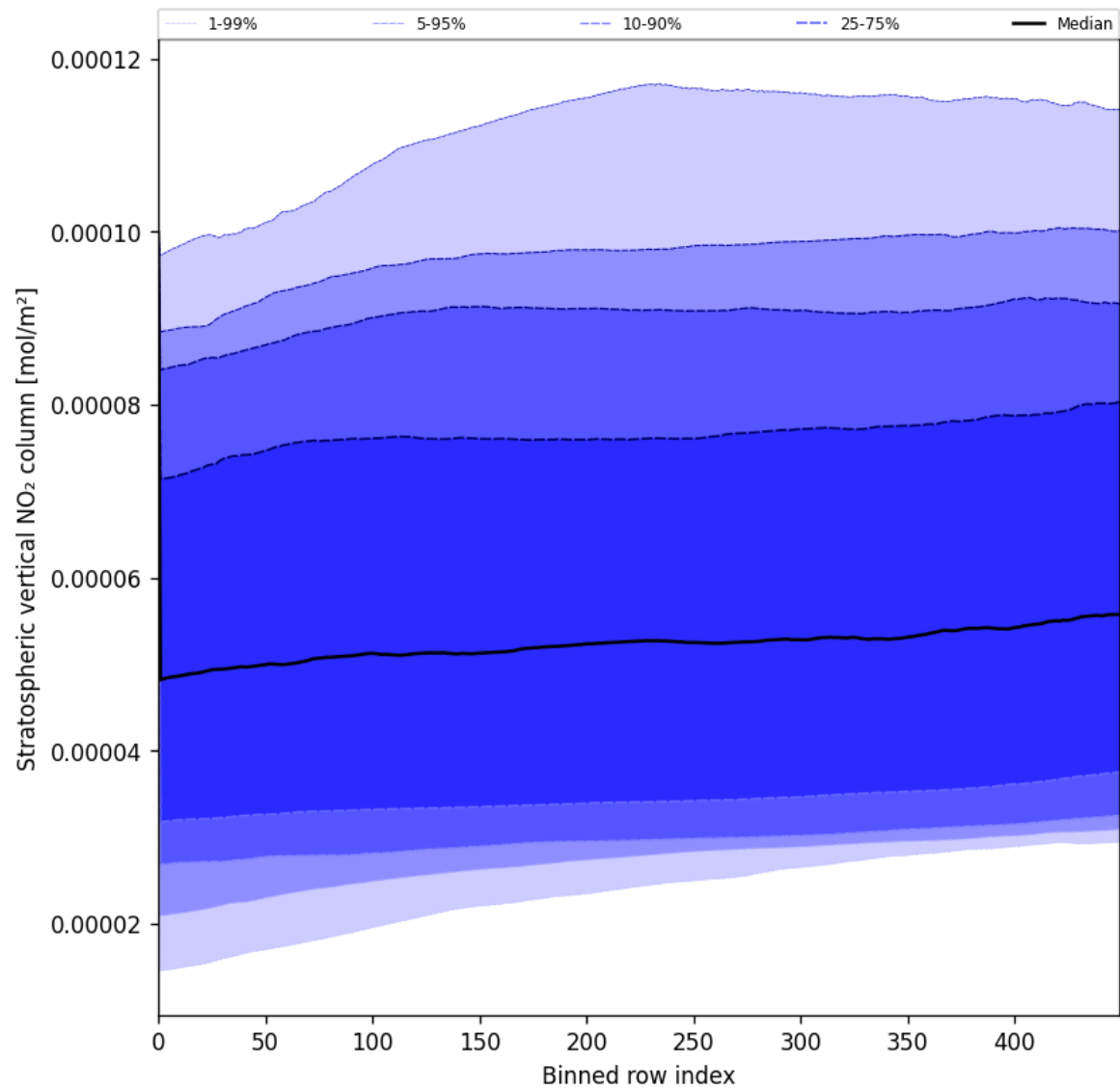
Figure 53: Along track statistics of “Stratospheric vertical NO 2 column” for 2025-06-22 to 2025-06-23
