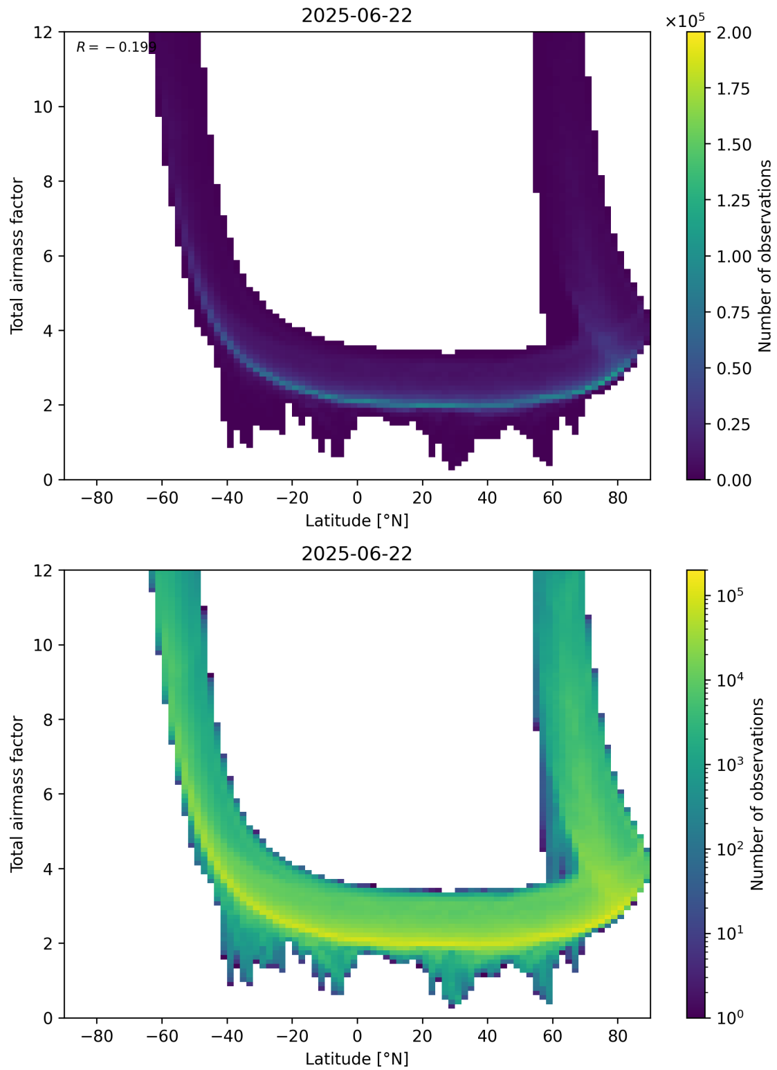
Figure 84: Scatter density plot of “Latitude” against “Total airmass factor” for 2025-06-22 to 2025-06-23.
