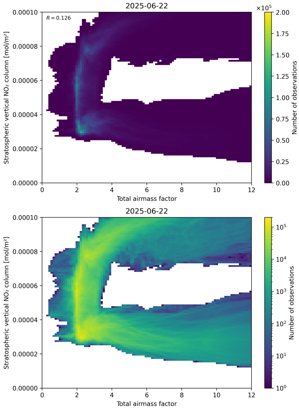
Figure 64: Scatter density plot of “Total airmass factor” against “Stratospheric vertical NO 2 column” for 2025-06-22 to 2025-06-23.
