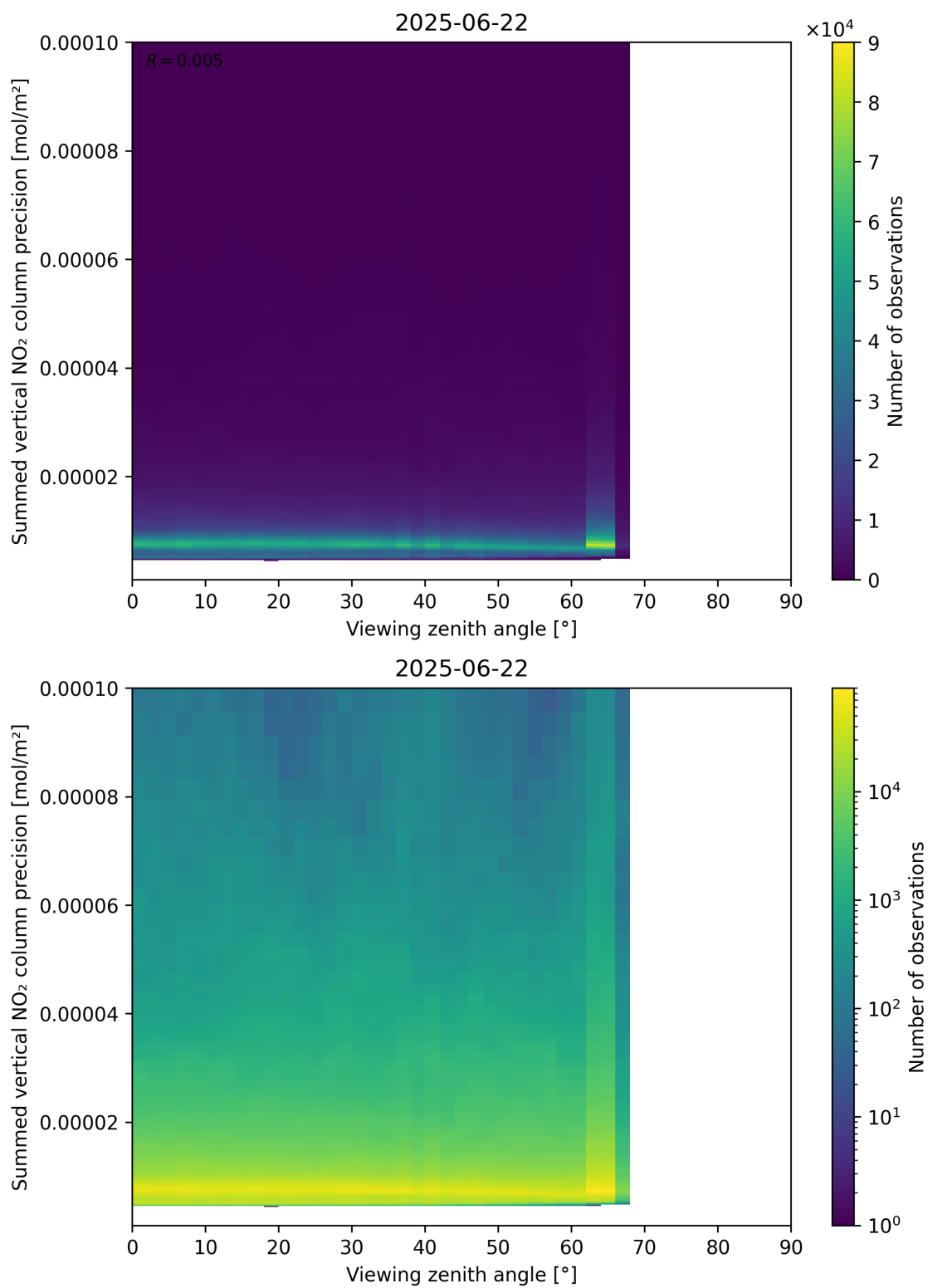
Figure 166: Scatter density plot of “Viewing zenith angle” against “Summed vertical NO 2 column precision” for 2025-06-22 to 2025-06-23.
