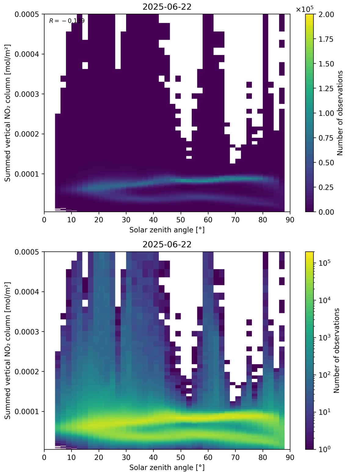
Figure 151: Scatter density plot of “Solar zenith angle” against “Summed vertical NO 2 column” for 2025-06-22 to 2025-06-23.
