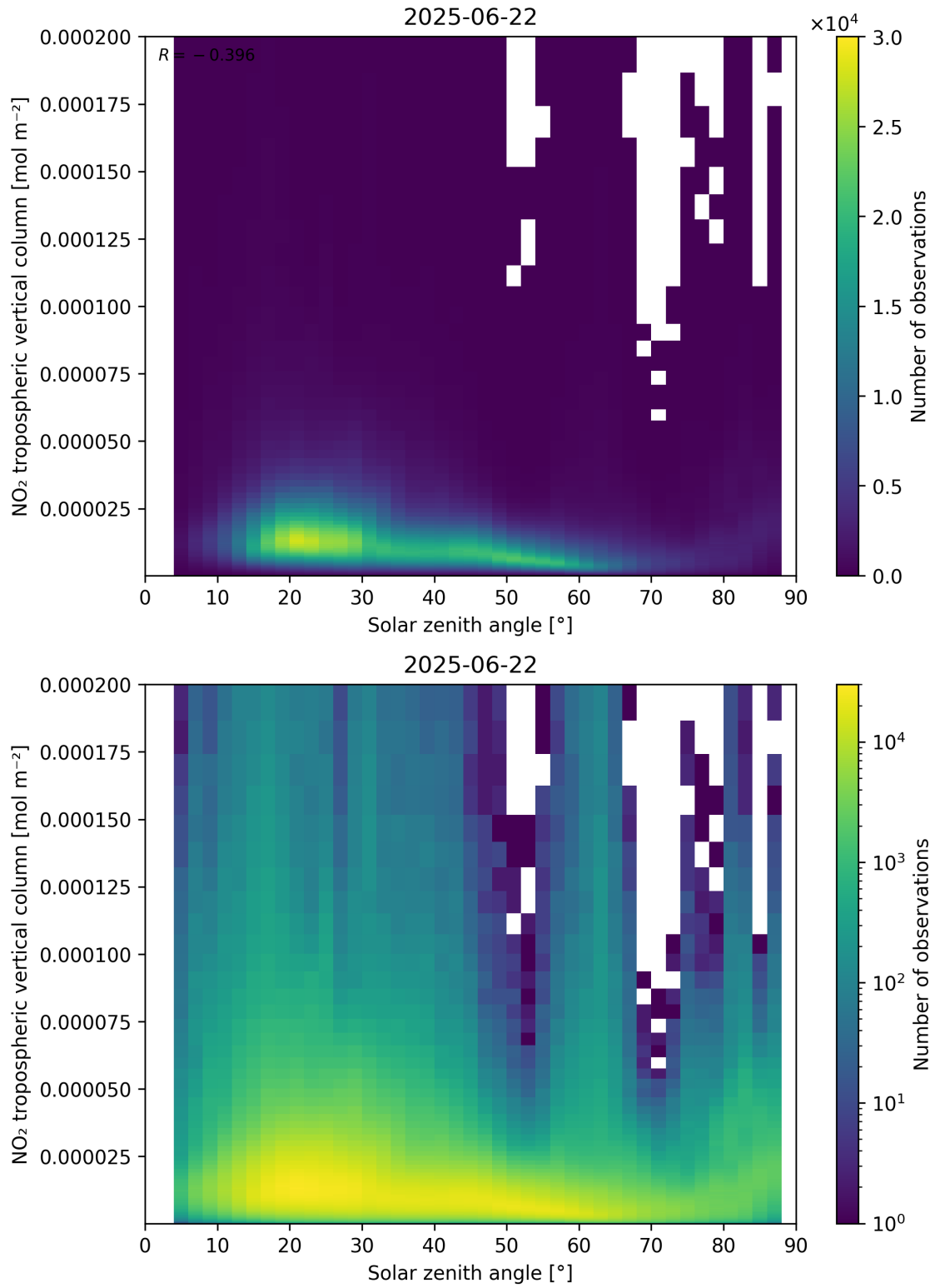
Figure 155: Scatter density plot of “Solar zenith angle” against “NO 2 tropospheric vertical column” for 2025-06-22 to 2025-06-23.
