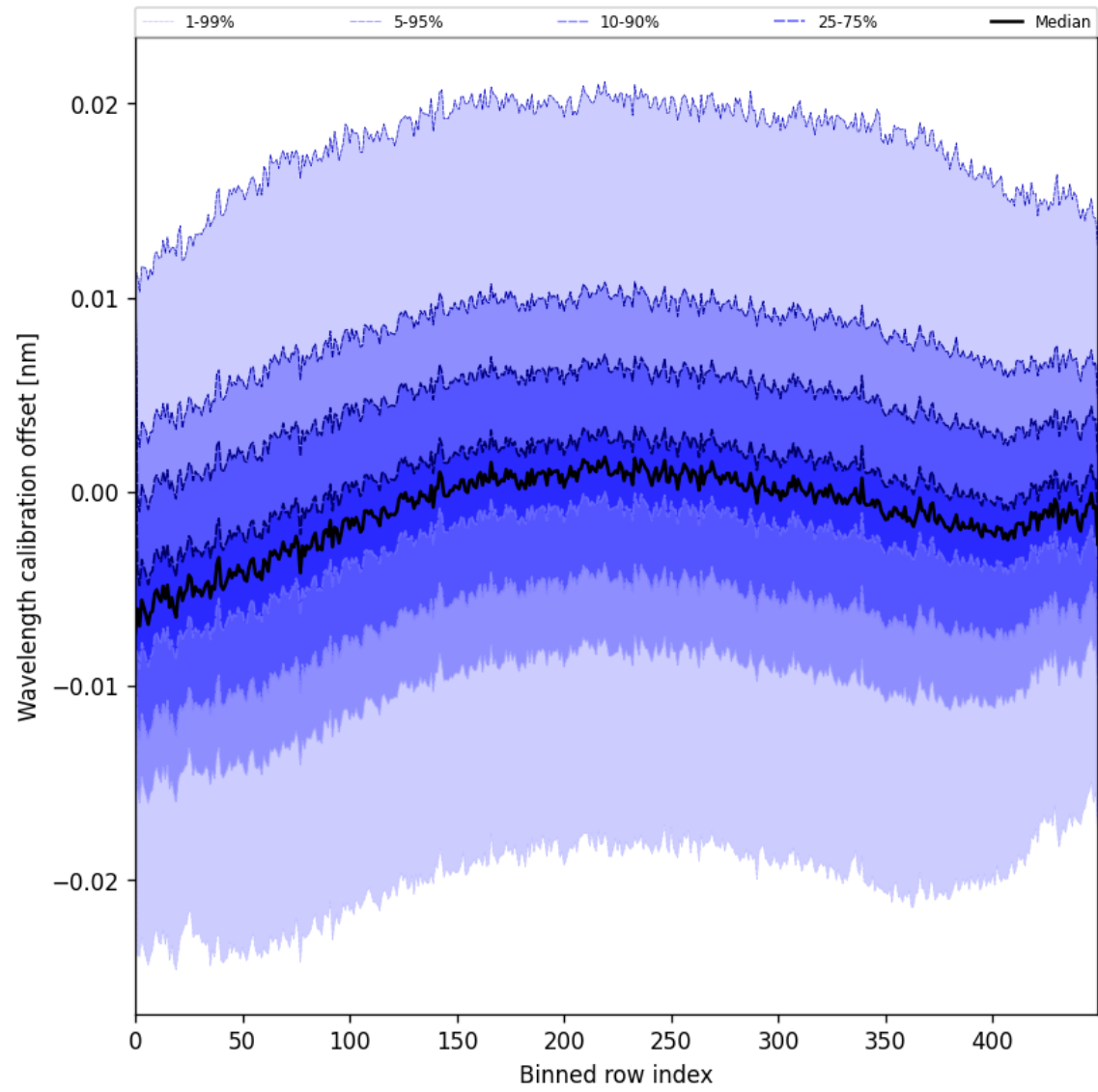
Figure 52: Along track statistics of “Wavelength calibration offset” for 2025-06-22 to 2025-06-23
