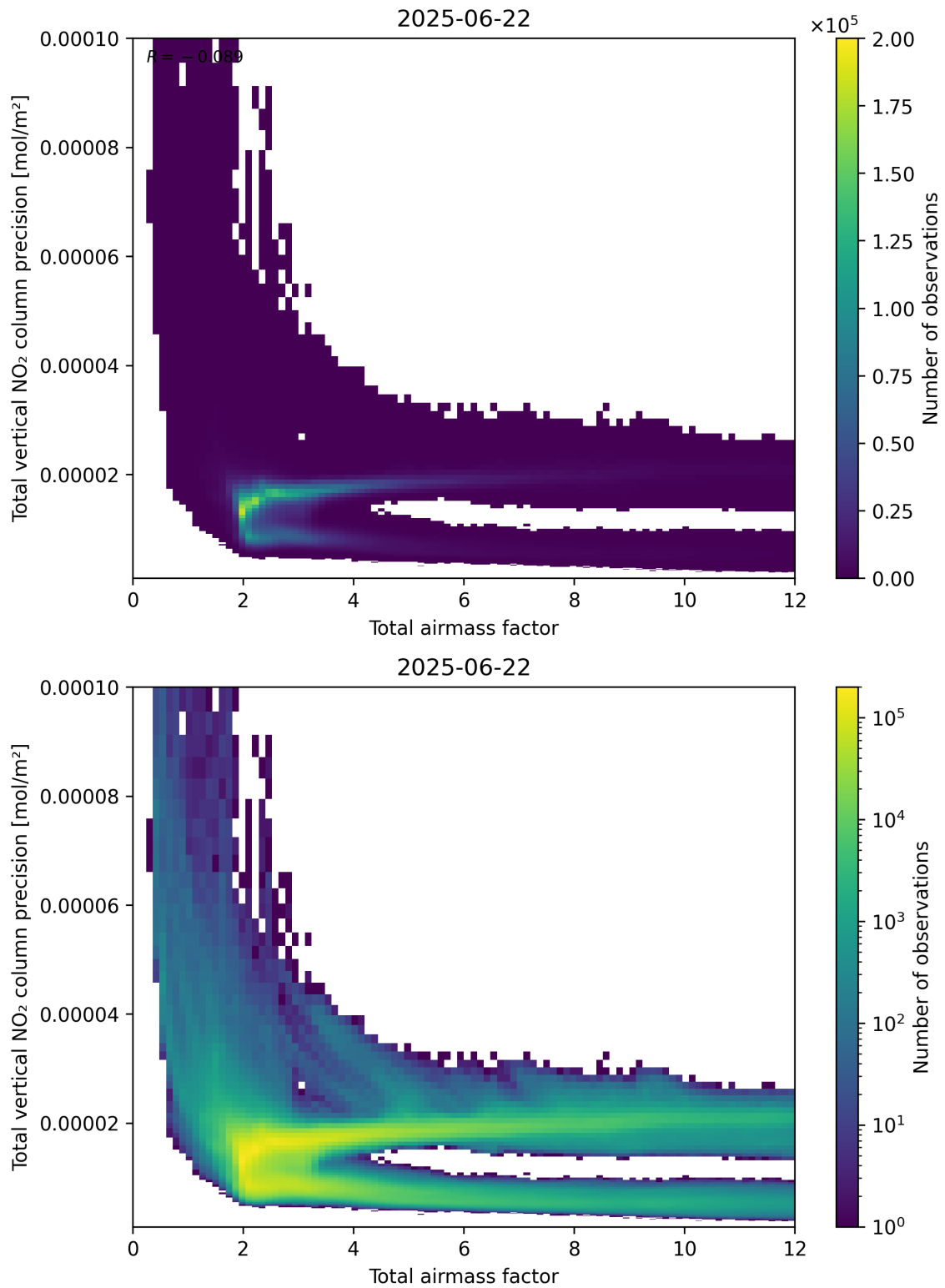
Figure 68: Scatter density plot of “Total airmass factor” against “Total vertical NO 2 column precision” for 2025-06-22 to 2025-06-23.
