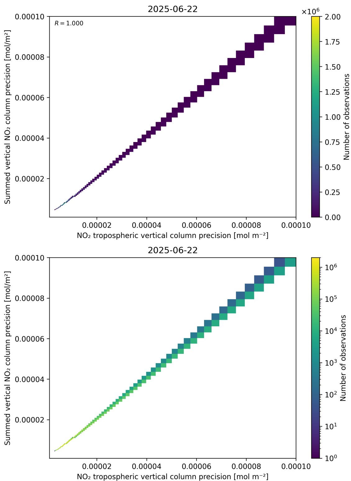
Figure 137: Scatter density plot of “NO 2 tropospheric vertical column precision” against “Summed vertical NO 2 column precision” for 2025-06-22 to 2025-06-23.
