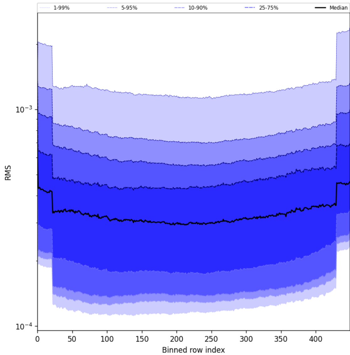
Figure 60: Along track statistics of “RMS” for 2025-06-22 to 2025-06-23
