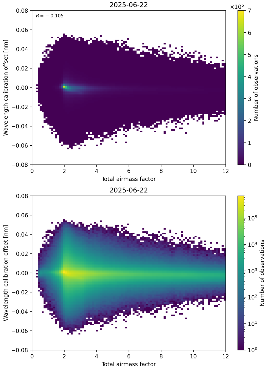
Figure 70: Scatter density plot of “Total airmass factor” against “Wavelength calibration offset” for 2025-06-22 to 2025-06-23.
