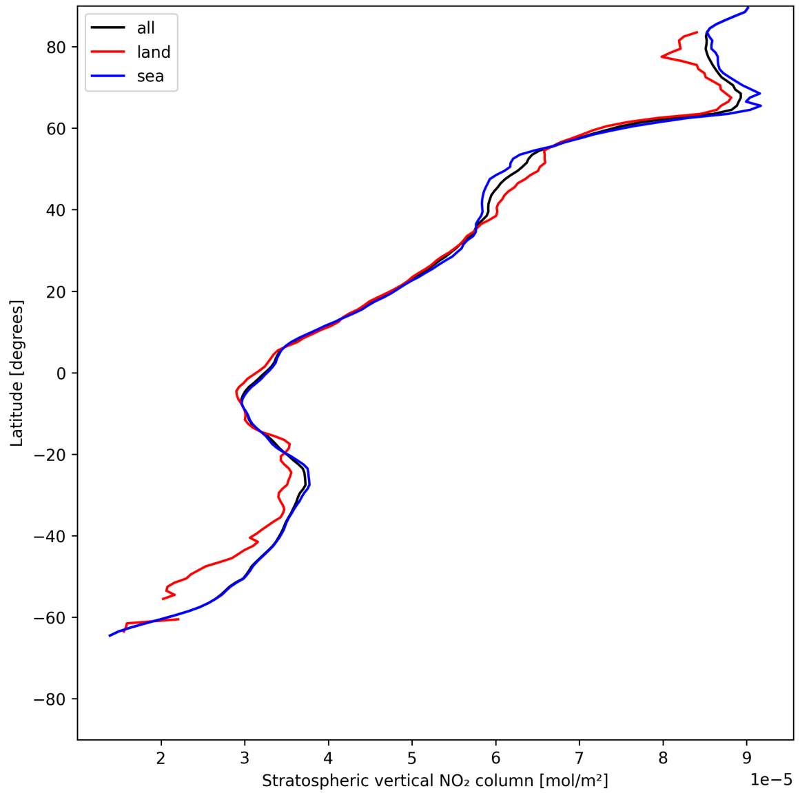
Figure 19: Zonal average of “Stratospheric vertical NO 2 column” for 2025-06-22 to 2025-06-23.
