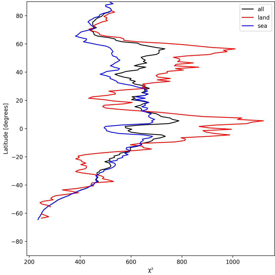
Figure 25: Zonal average of “ \chi^2 ” for 2025-06-22 to 2025-06-23.
