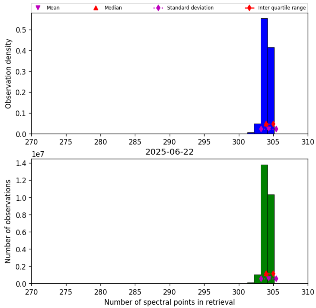
Figure 33: Histogram of “Number of spectral points in retrieval” for 2025-06-22 to 2025-06-23
