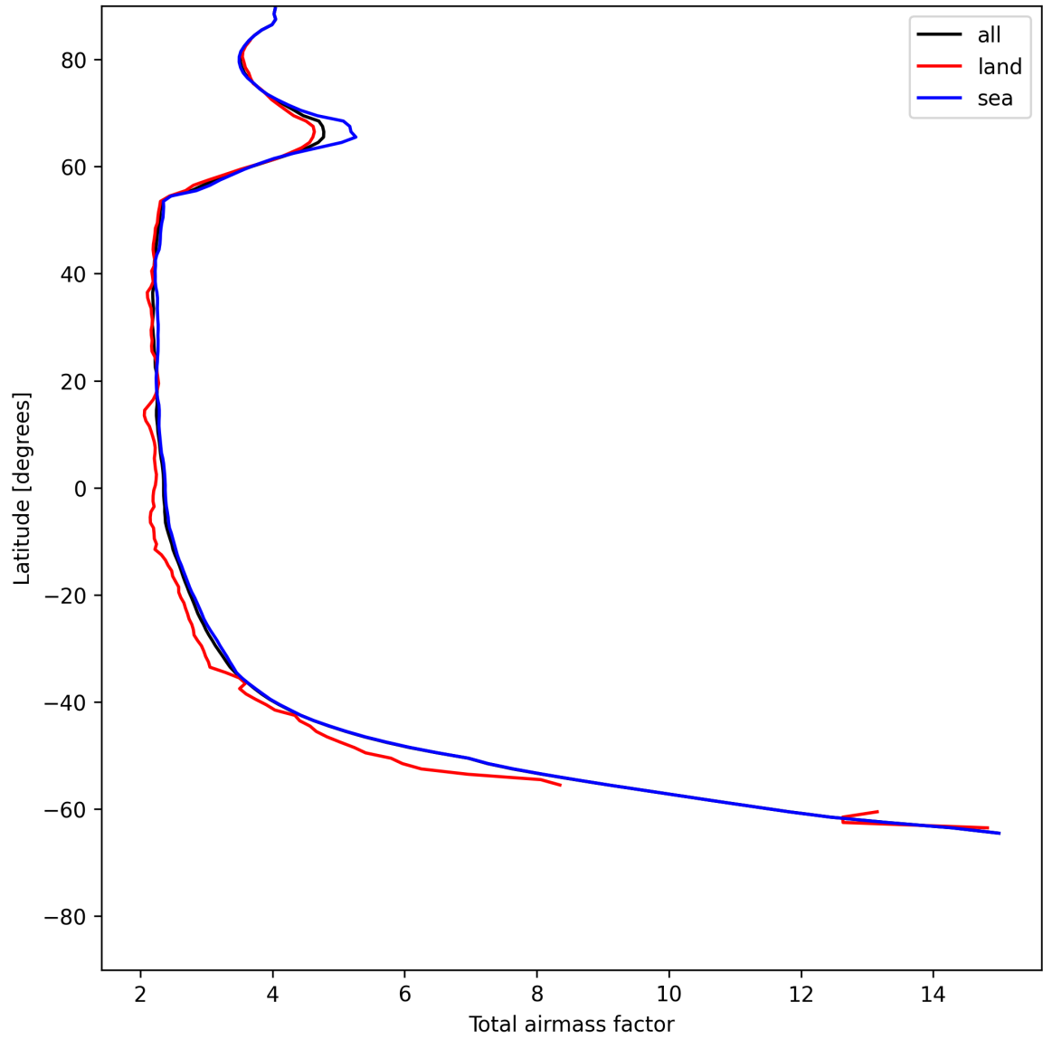
Figure 15: Zonal average of “Total airmass factor” for 2025-06-22 to 2025-06-23.
