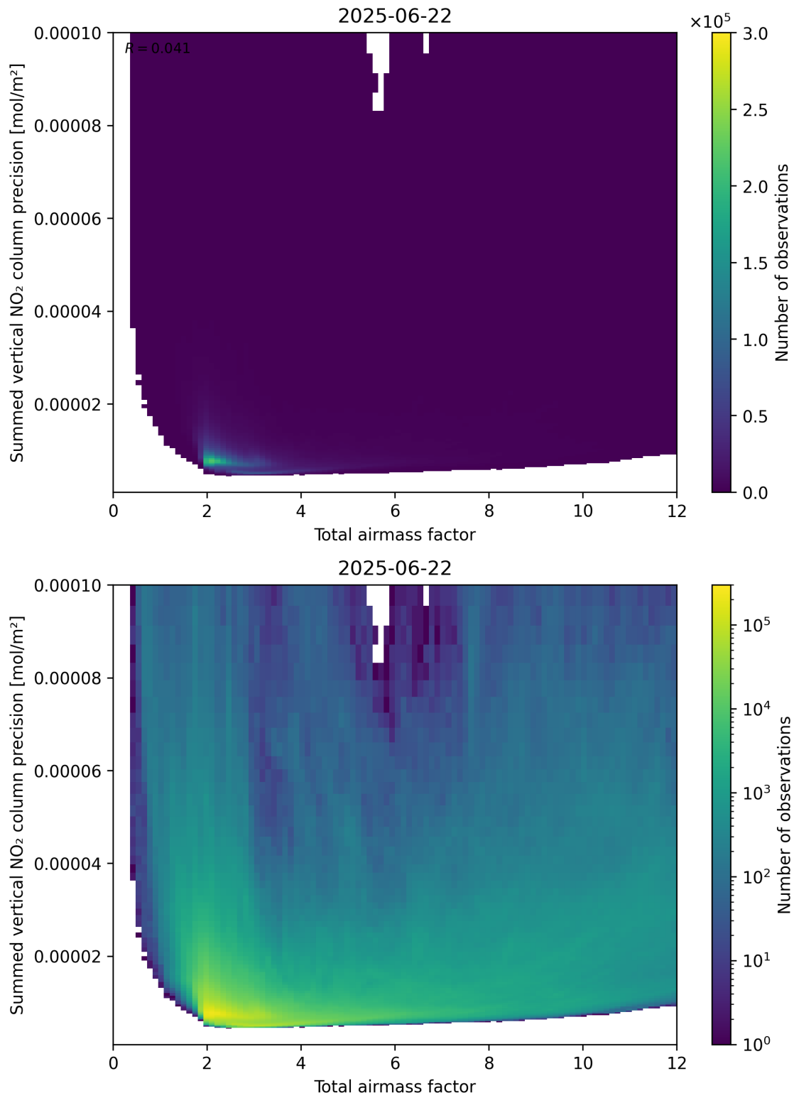
Figure 66: Scatter density plot of “Total airmass factor” against “Summed vertical NO 2 column precision” for 2025-06-22 to 2025-06-23.
