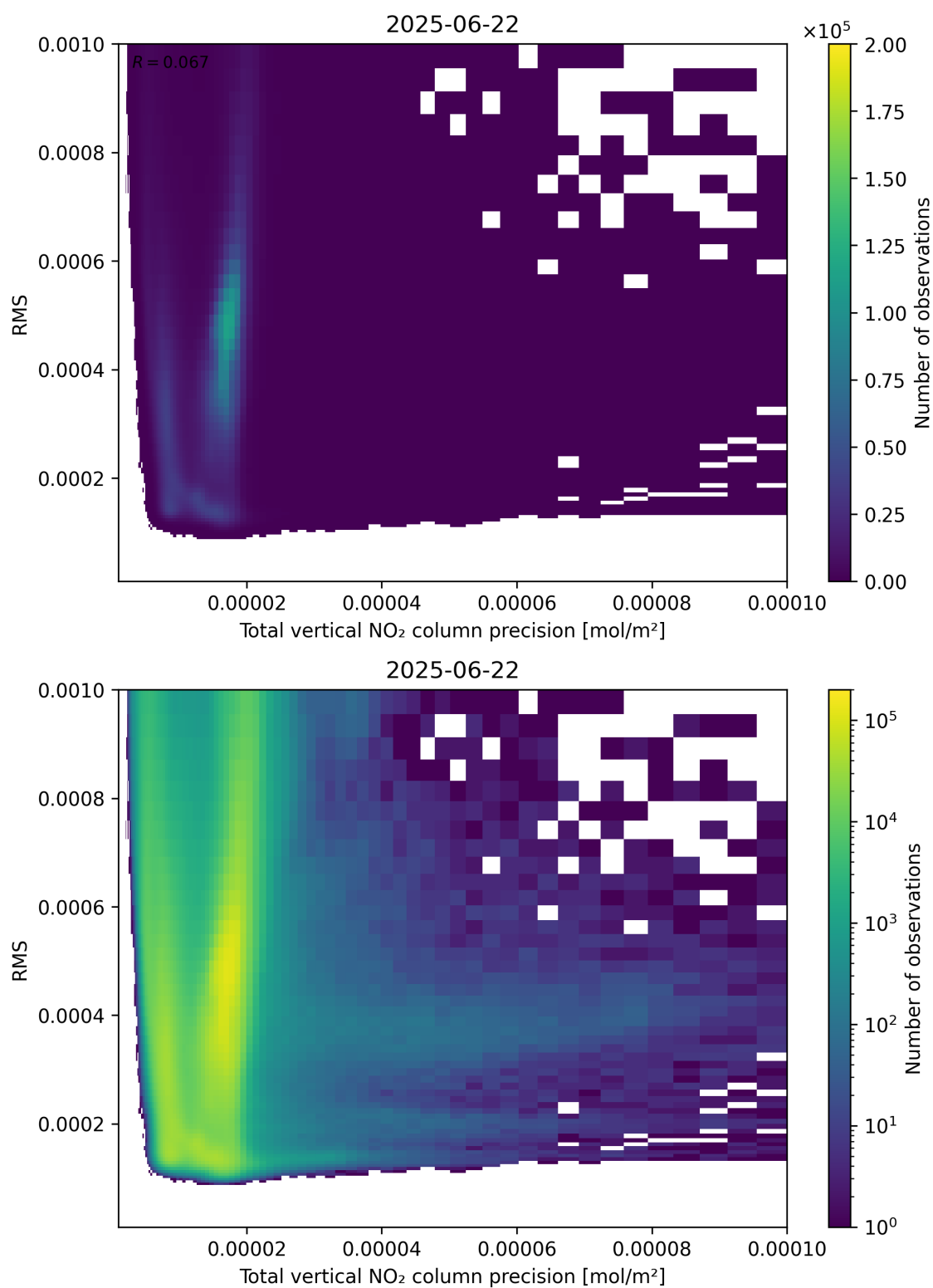
Figure 119: Scatter density plot of “Total vertical NO 2 column precision” against “RMS” for 2025-06-22 to 2025-06-23.
