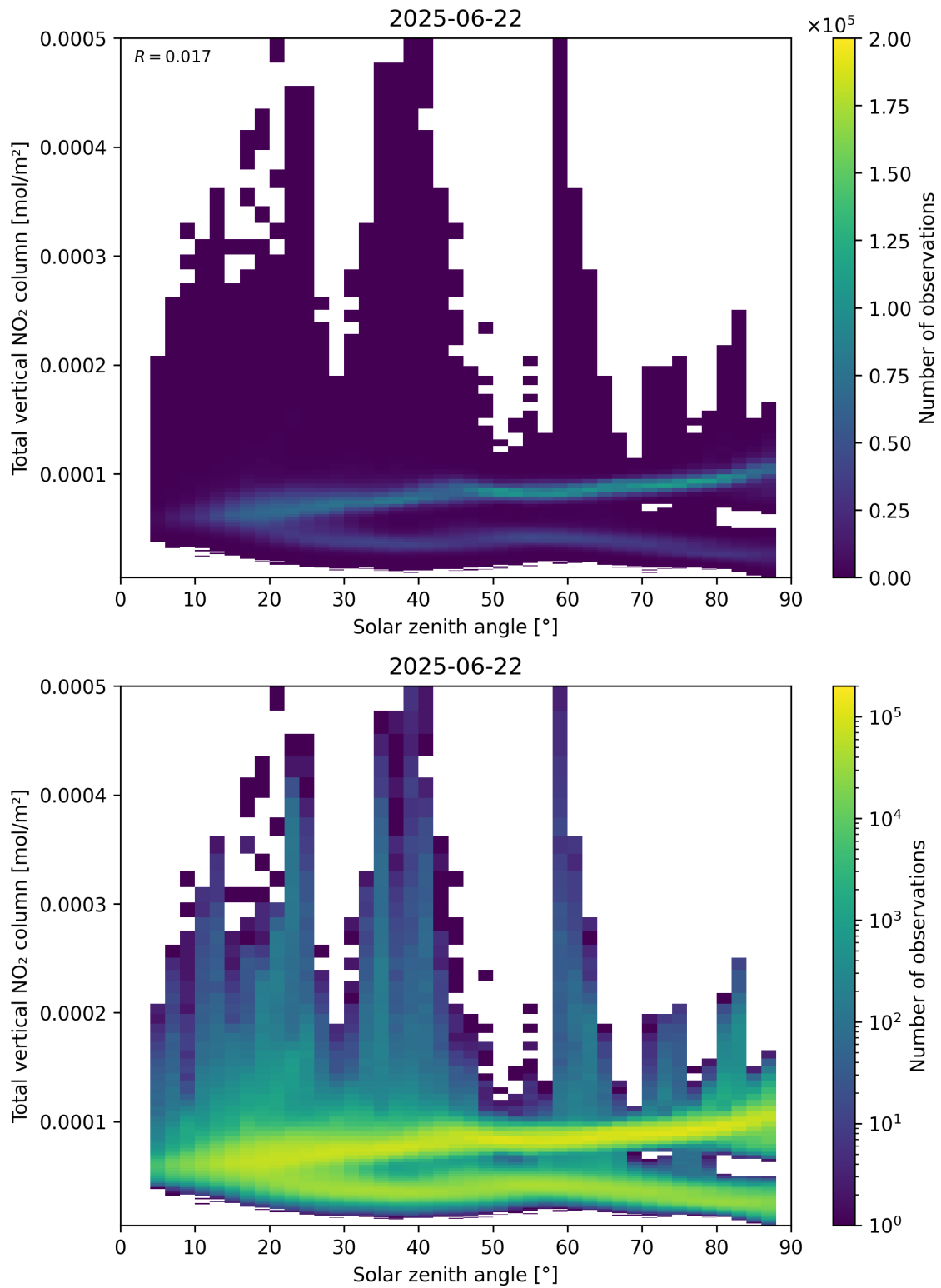
Figure 153: Scatter density plot of “Solar zenith angle” against “Total vertical NO 2 column” for 2025-06-22 to 2025-06-23.
