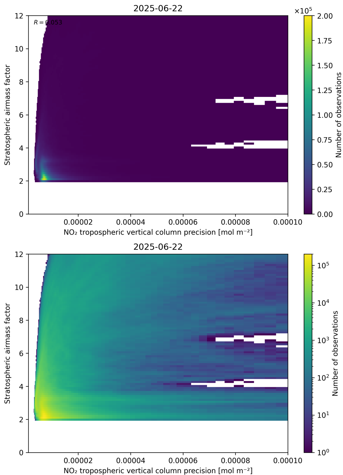
Figure 131: Scatter density plot of “NO 2 tropospheric vertical column precision” against “Stratospheric airmass factor” for 2025-06-22 to 2025-06-23.
