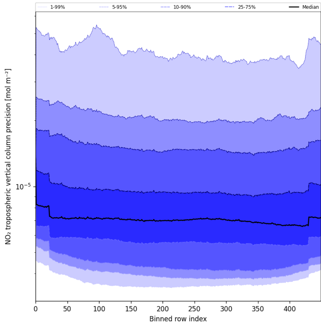
Figure 47: Along track statistics of “NO 2 tropospheric vertical column precision” for 2025-06-22 to 2025-06-23
