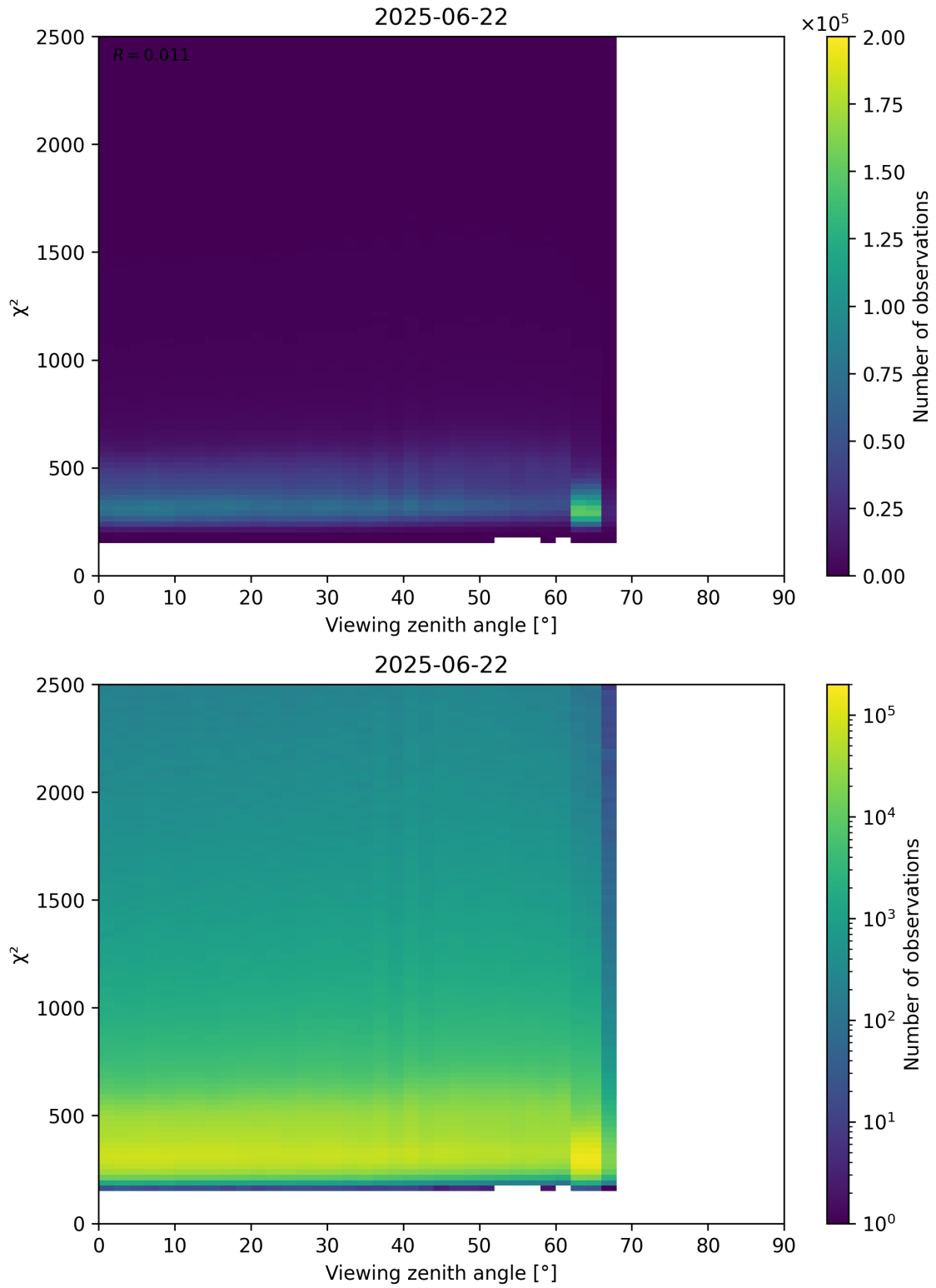
Figure 162: Scatter density plot of “Viewing zenith angle” against “ \chi^2 ” for 2025-06-22 to 2025-06-23.
