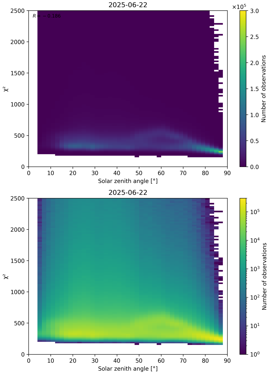
Figure 148: Scatter density plot of “Solar zenith angle” against “ \chi^2 ” for 2025-06-22 to 2025-06-23.
