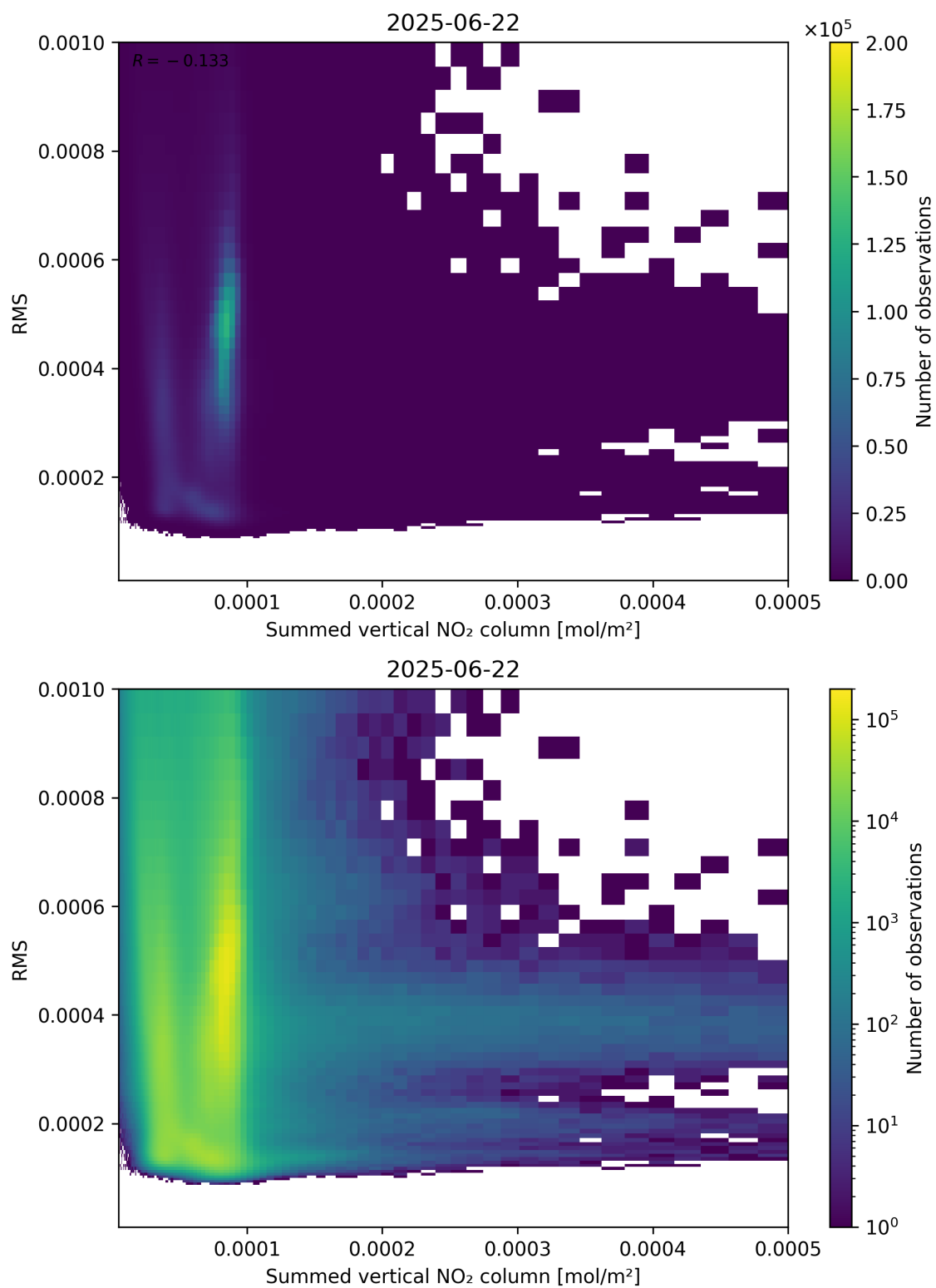
Figure 109: Scatter density plot of “Summed vertical NO 2 column” against “RMS” for 2025-06-22 to 2025-06-23.
