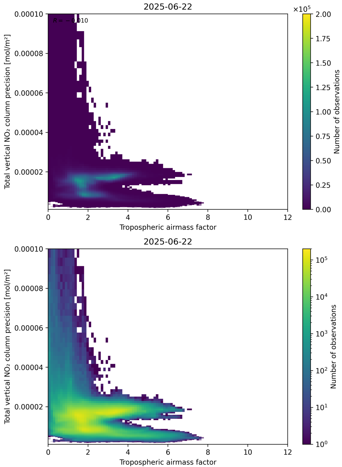
Figure 78: Scatter density plot of “Tropospheric air mass factor” against “Total vertical NO 2 column precision” for 2025-06-22 to 2025-06-23.
