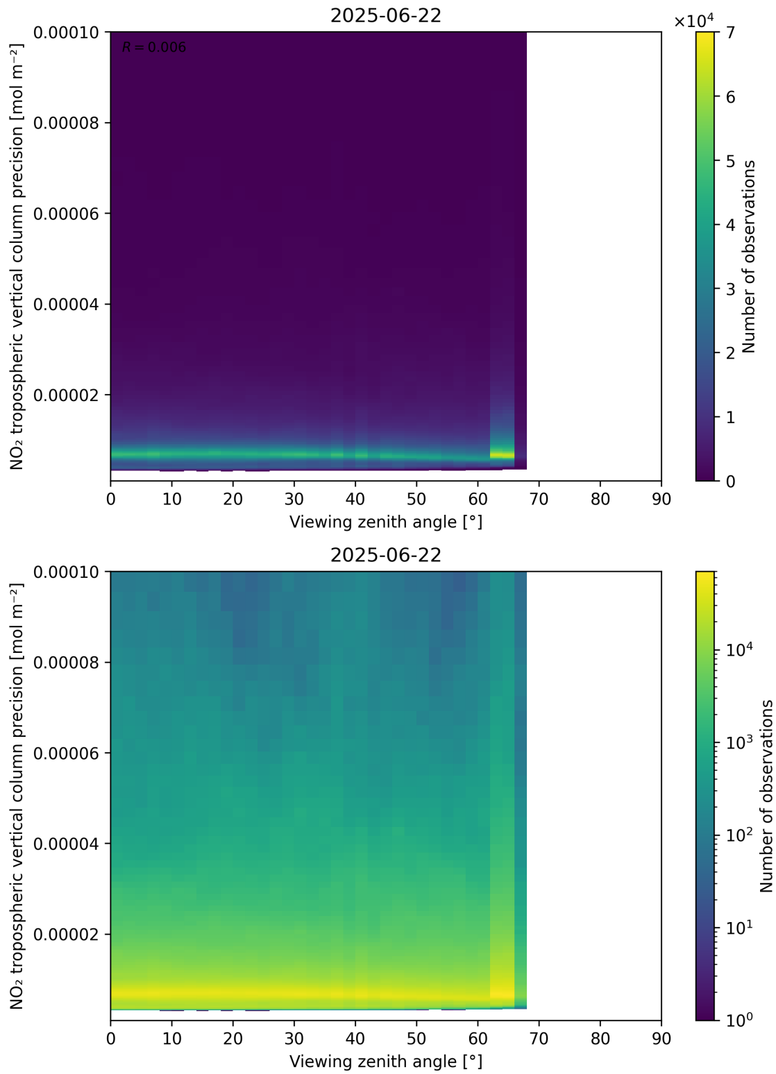
Figure 170: Scatter density plot of “Viewing zenith angle” against “NO 2 tropospheric vertical column precision” for 2025-06-22 to 2025-06-23.
