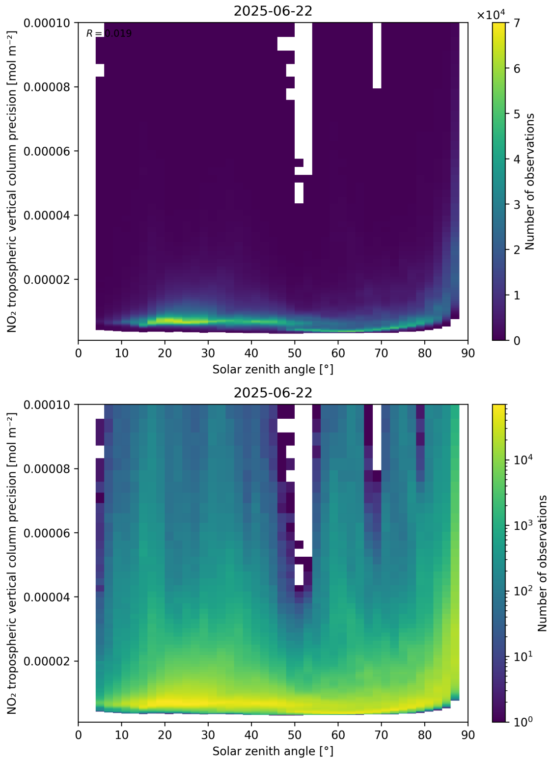
Figure 156: Scatter density plot of “Solar zenith angle” against “NO 2 tropospheric vertical column precision” for 2025-06-22 to 2025-06-23.
