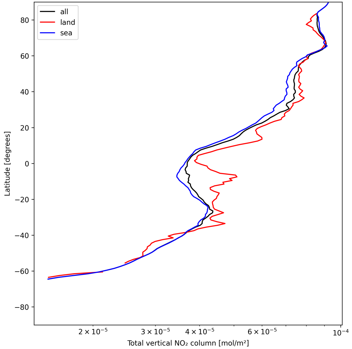
Figure 21: Zonal average of “Total vertical NO 2 column” for 2025-06-22 to 2025-06-23.
