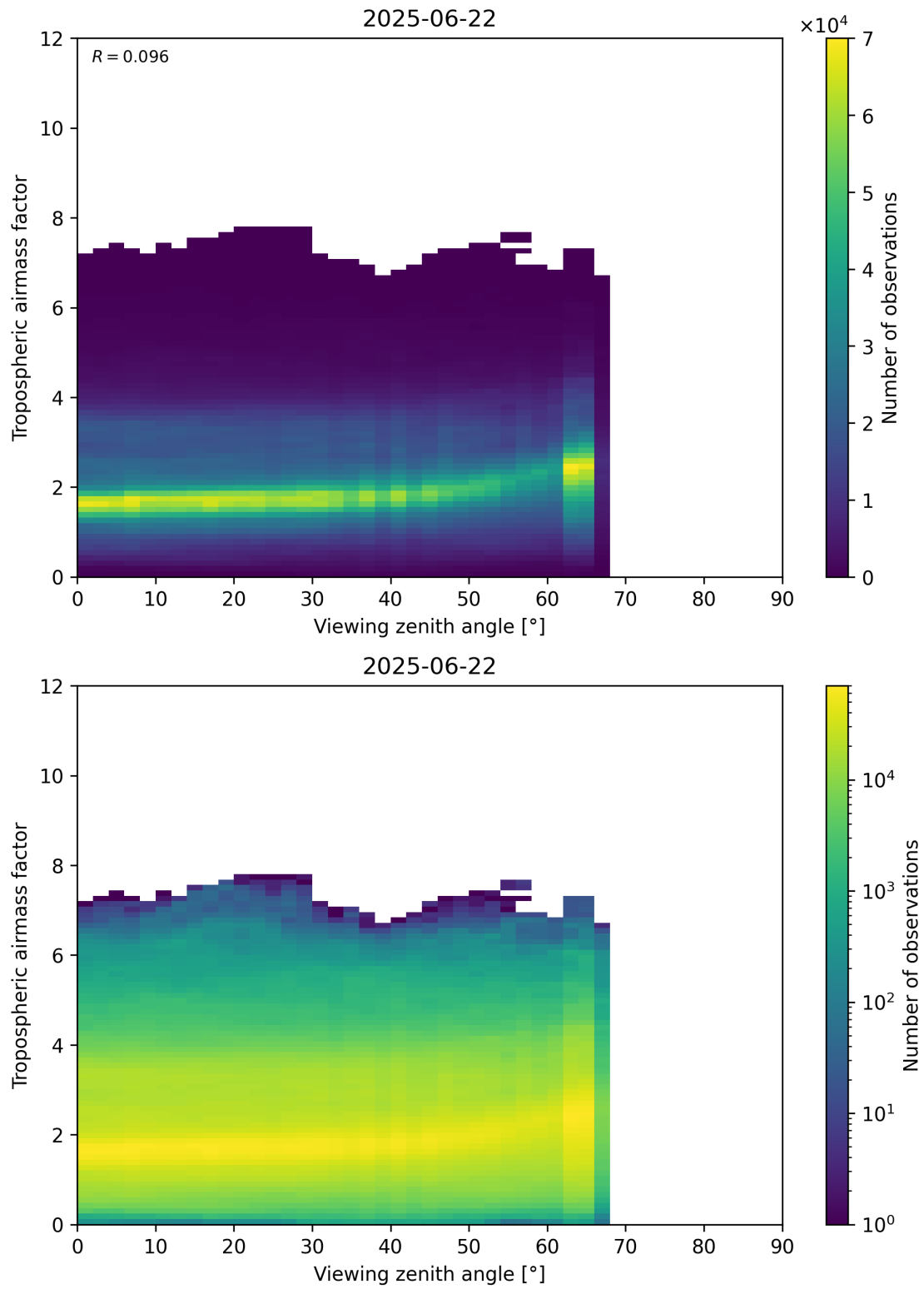
Figure 161: Scatter density plot of “Viewing zenith angle” against “Tropospheric airmass factor” for 2025-06-22 to 2025-06-23.
