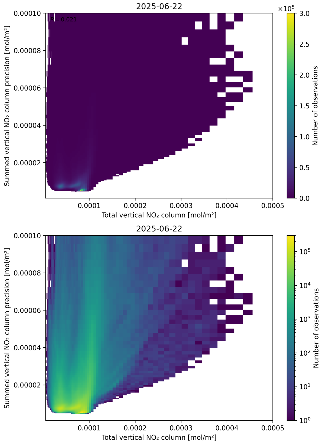
Figure 113: Scatter density plot of “Total vertical NO 2 column” against “Summed vertical NO 2 column precision” for 2025-06-22 to 2025-06-23.
