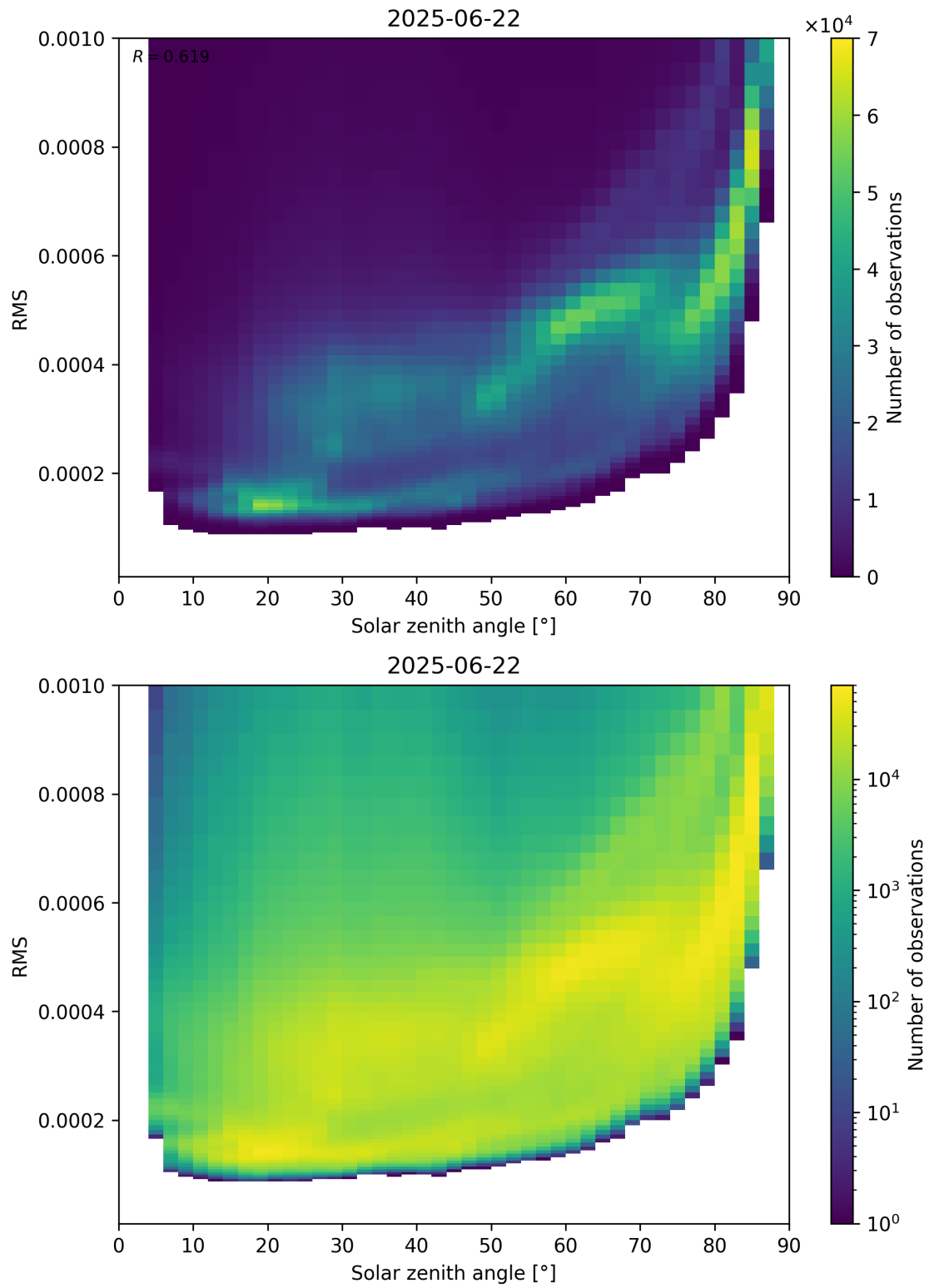
Figure 157: Scatter density plot of “Solar zenith angle” against “RMS” for 2025-06-22 to 2025-06-23.
