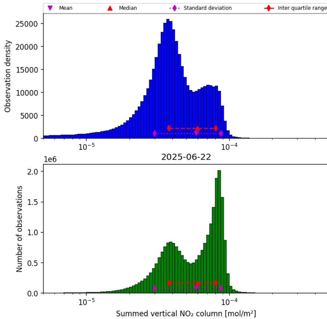
Figure 40: Histogram of "Summed vertical NO 2 column" for 2025-06-22 to 2025-06-23
