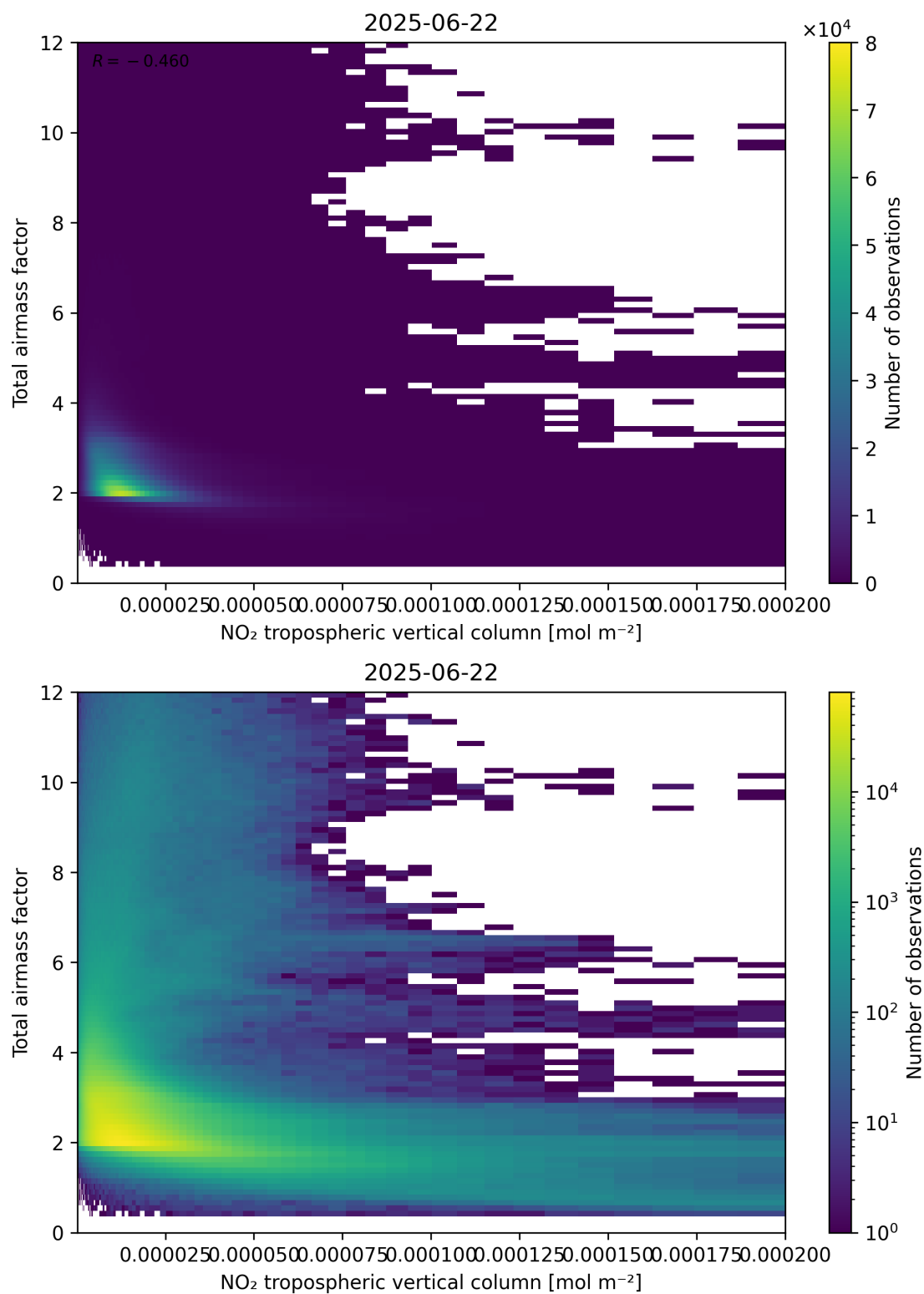
Figure 122: Scatter density plot of “NO 2 tropospheric vertical column” against “Total air mass factor” for 2025-06-22 to 2025-06-23.
