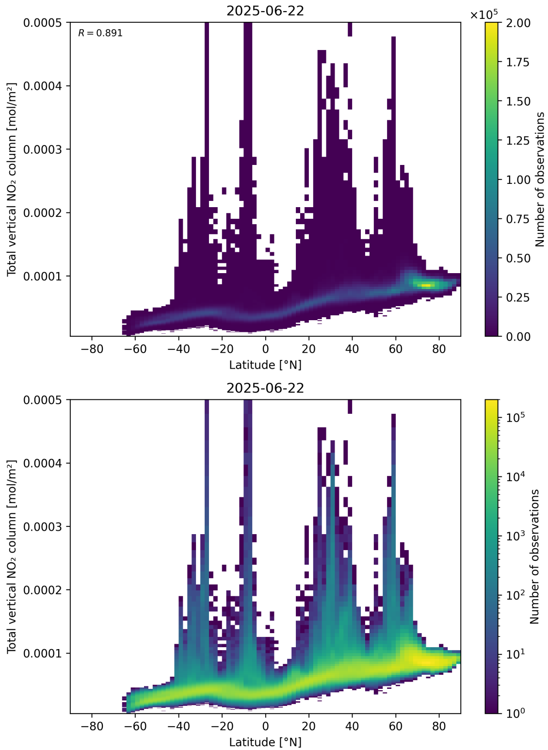
Figure 90: Scatter density plot of “Latitude” against “Total vertical NO 2 column” for 2025-06-22 to 2025-06-23.
