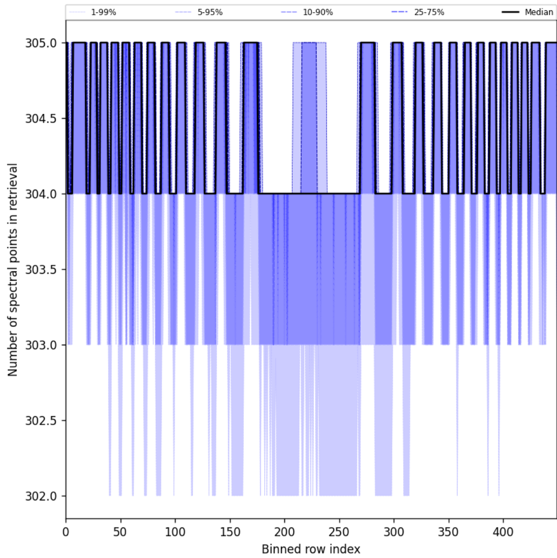
Figure 50: Along track statistics of “Number of spectral points in retrieval” for 2025-06-22 to 2025-06-23
