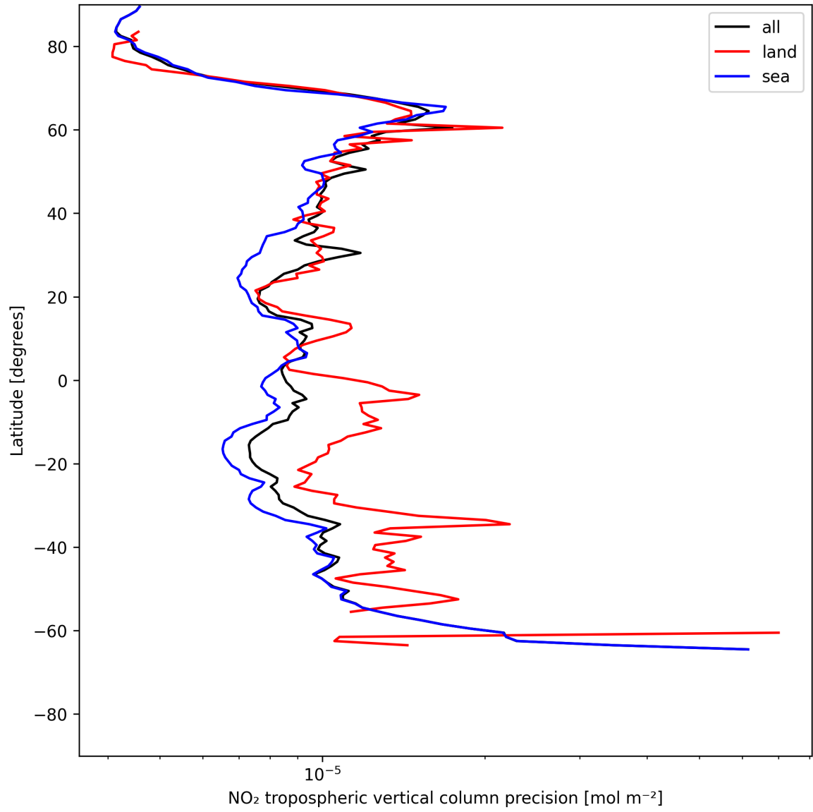
Figure 13: Zonal average of “NO 2 tropospheric vertical column precision” for 2025-06-22 to 2025-06-23.
