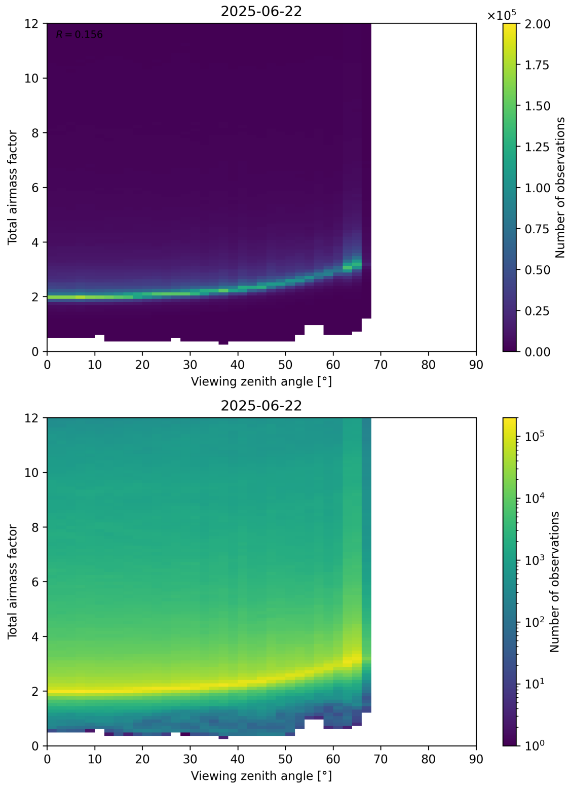
Figure 160: Scatter density plot of “Viewing zenith angle” against “Total airmass factor” for 2025-06-22 to 2025-06-23.
