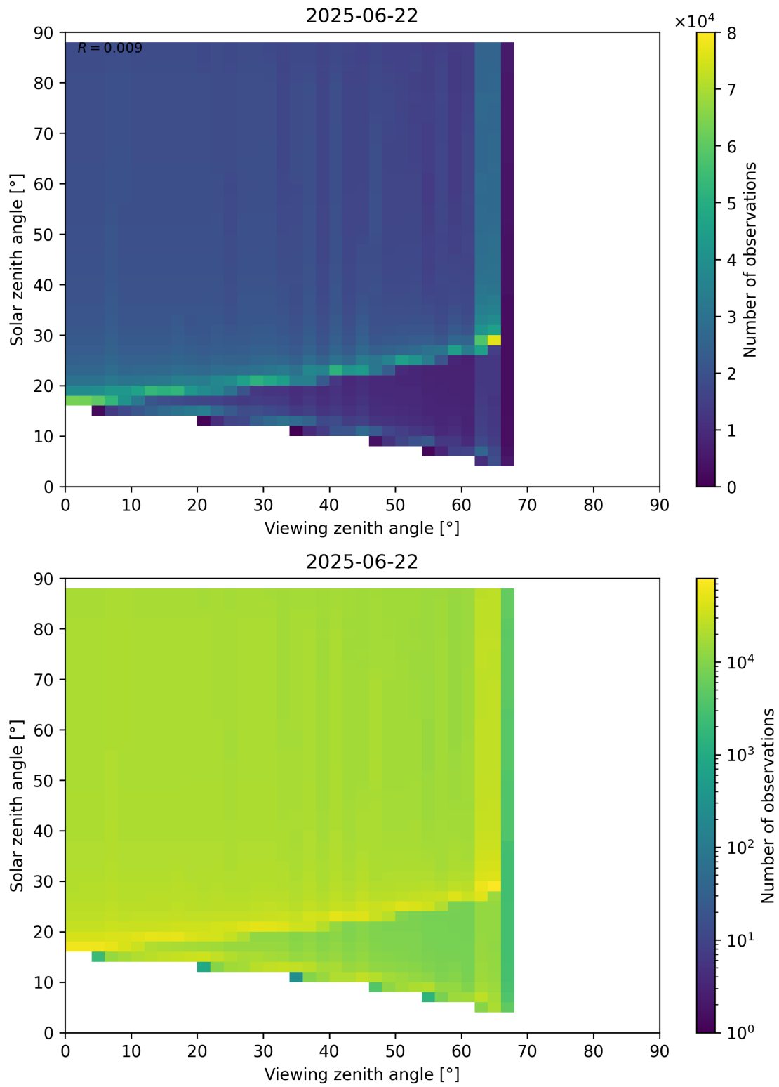
Figure 172: Scatter density plot of “Viewing zenith angle” against “Solar zenith angle” for 2025-06-22 to 2025-06-23.
