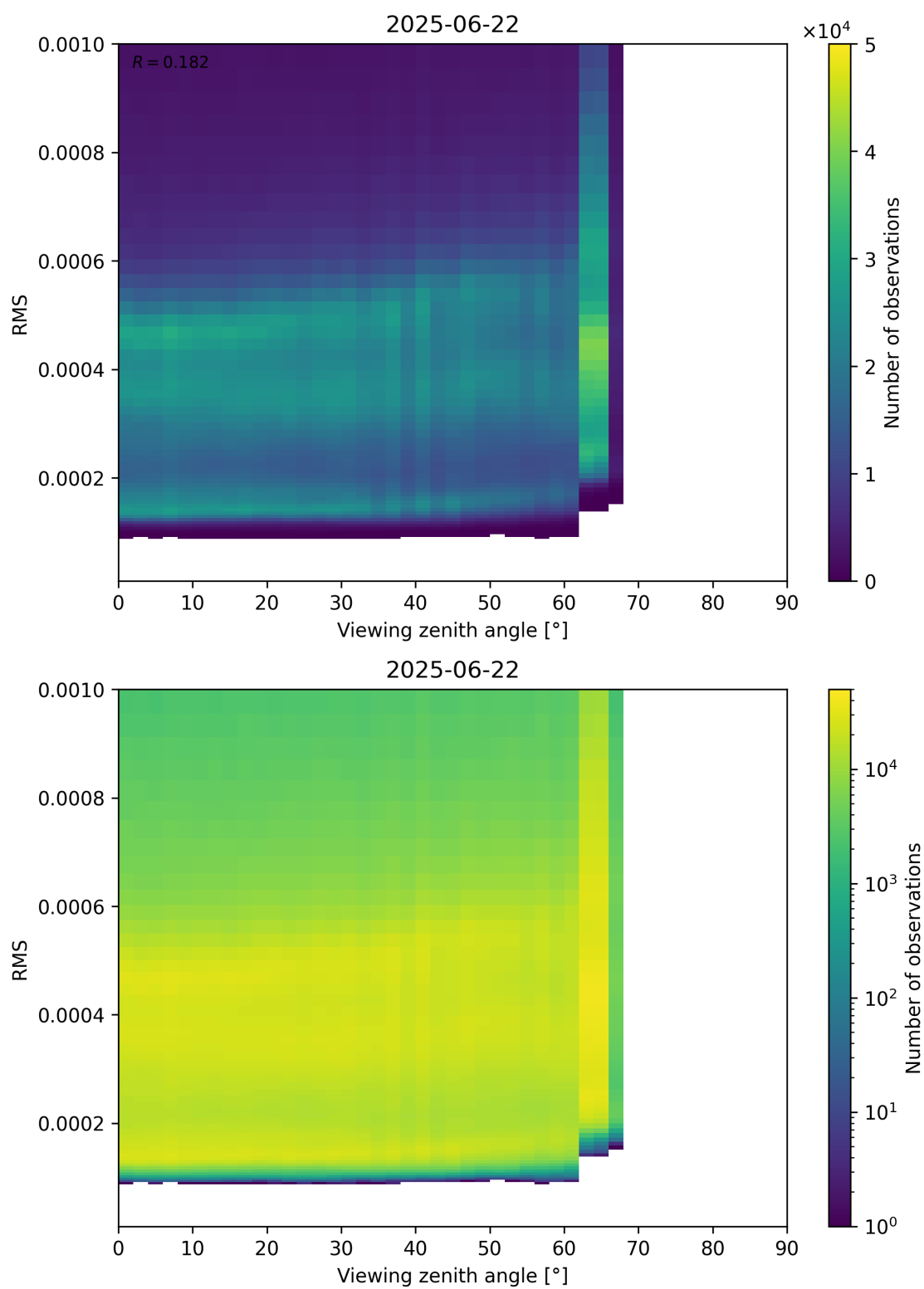
Figure 171: Scatter density plot of “Viewing zenith angle” against “RMS” for 2025-06-22 to 2025-06-23.
