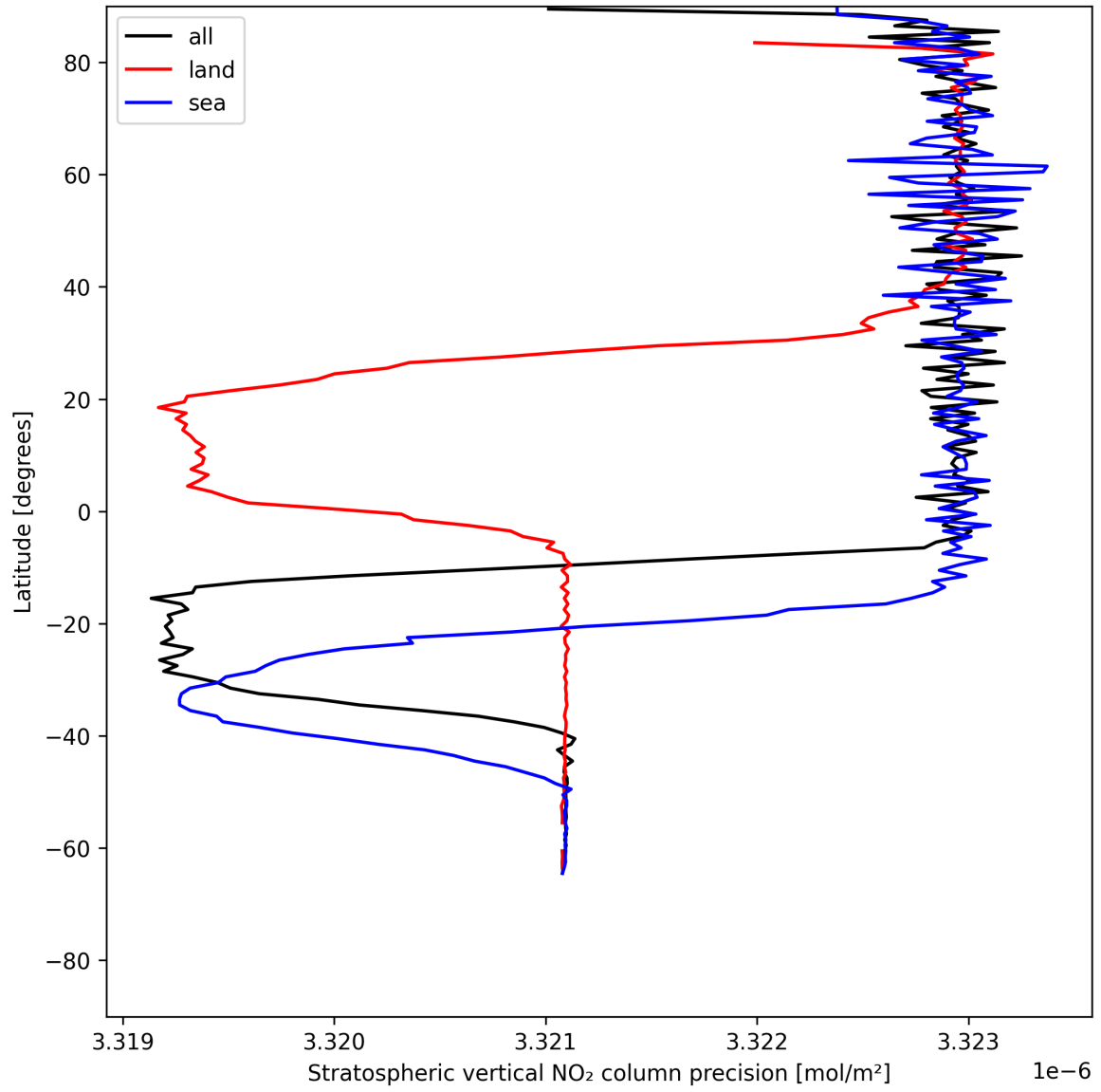
Figure 20: Zonal average of “Stratospheric vertical NO 2 column precision” for 2025-06-22 to 2025-06-23.
