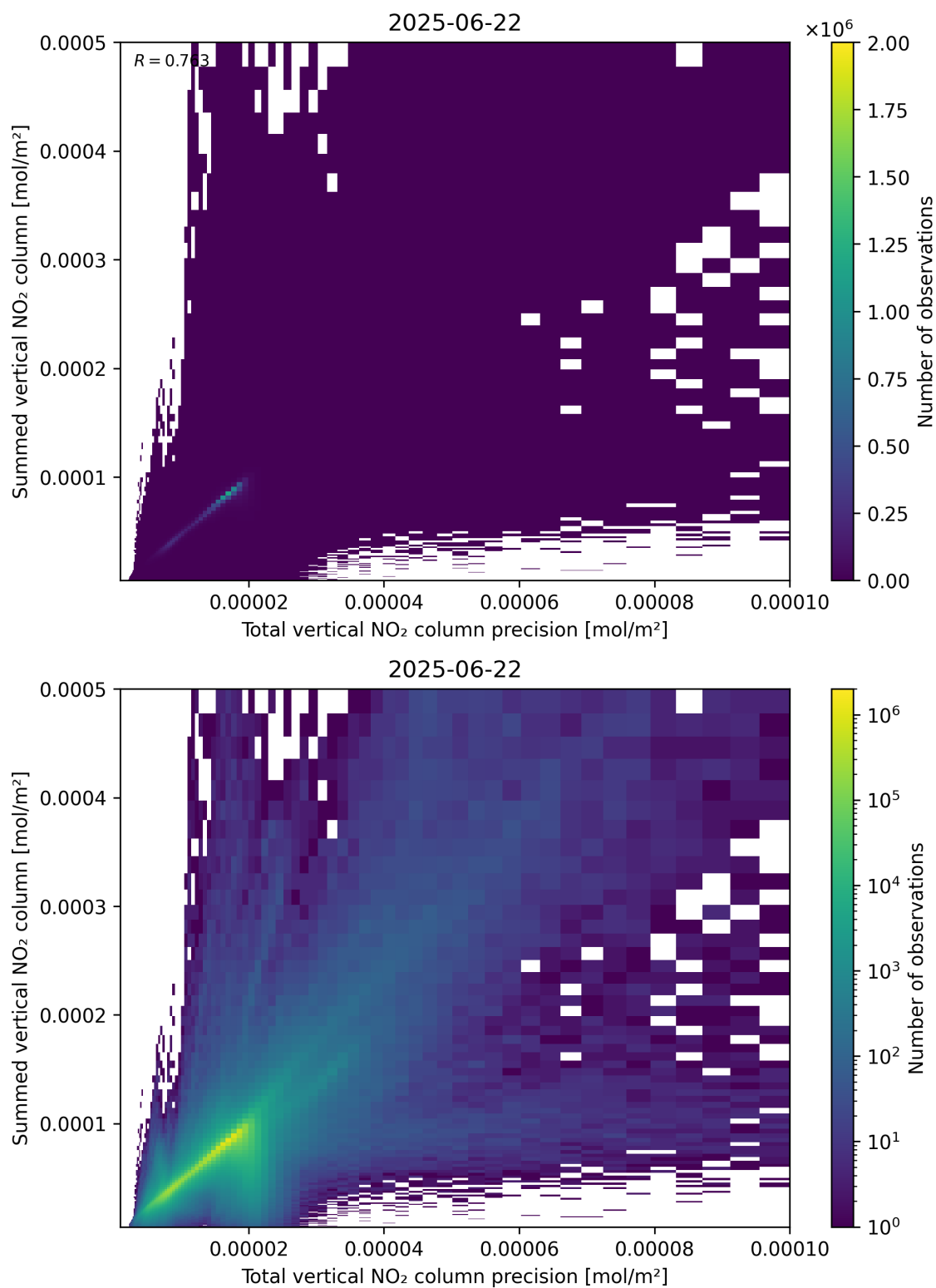
Figure 117: Scatter density plot of “Total vertical NO 2 column precision” against “Summed vertical NO 2 column” for 2025-06-22 to 2025-06-23.
