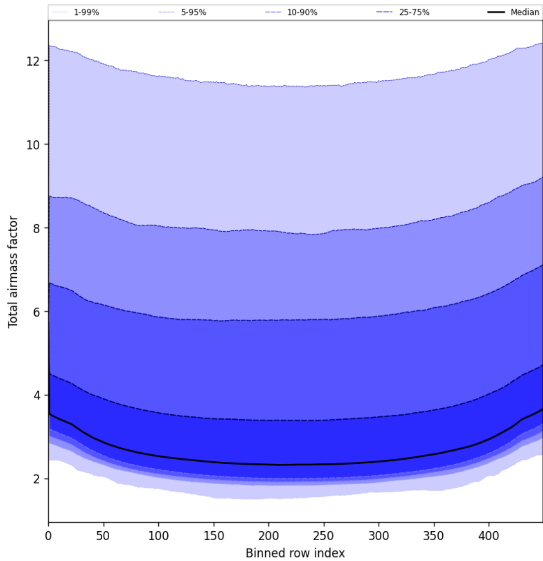
Figure 49: Along track statistics of “Total airmass factor” for 2025-06-22 to 2025-06-23
