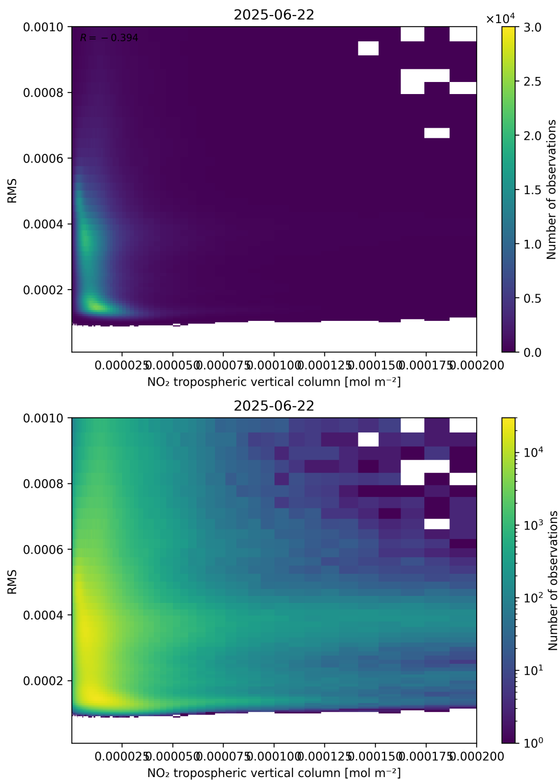
Figure 142: Scatter density plot of “NO 2 tropospheric vertical column” against “RMS” for 2025-06-22 to 2025-06-23.
