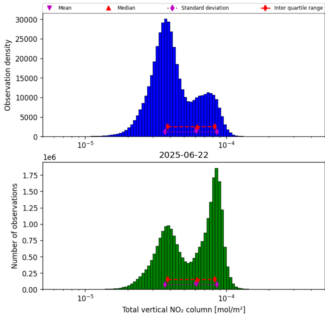
Figure 38: Histogram of “Total vertical NO 2 column” for 2025-06-22 to 2025-06-23
