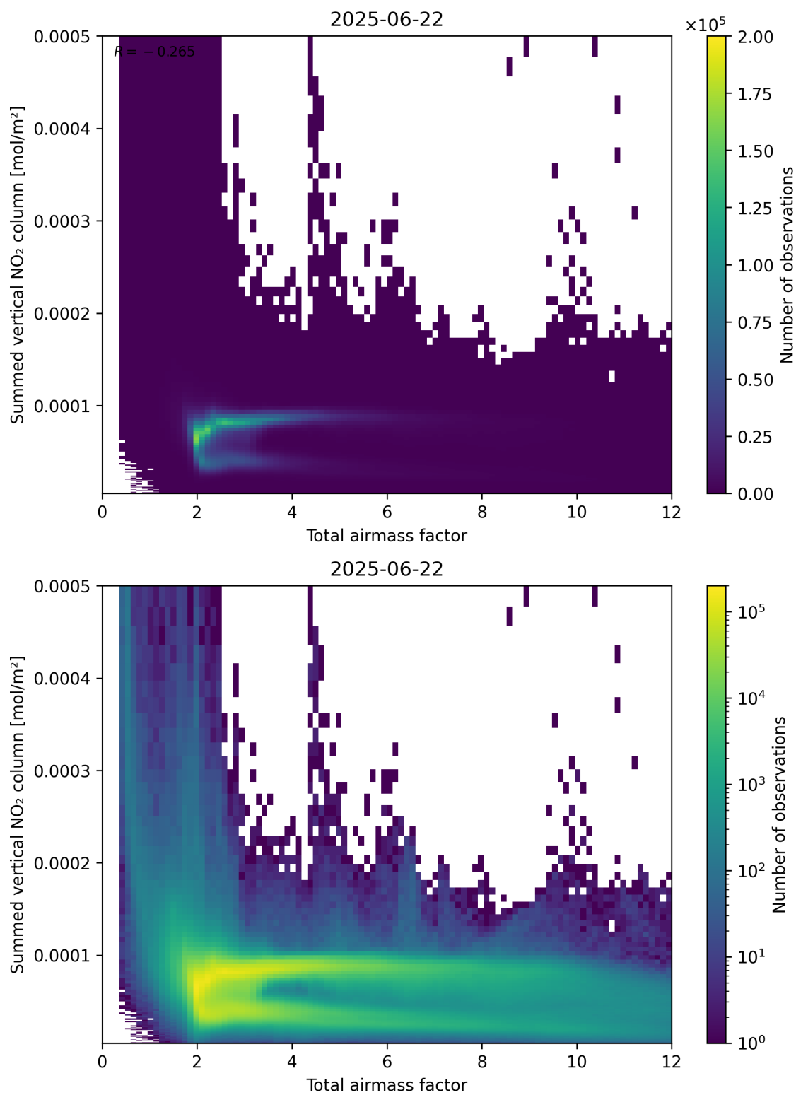
Figure 65: Scatter density plot of “Total airmass factor” against “Summed vertical NO 2 column” for 2025-06-22 to 2025-06-23.
