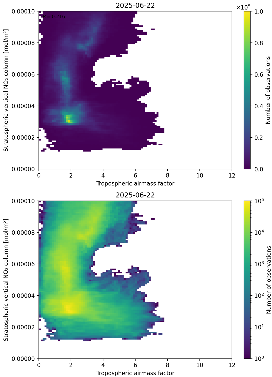
Figure 74: Scatter density plot of “Tropospheric airmass factor” against “Stratospheric vertical NO 2 column” for 2025-06-22 to 2025-06-23.
