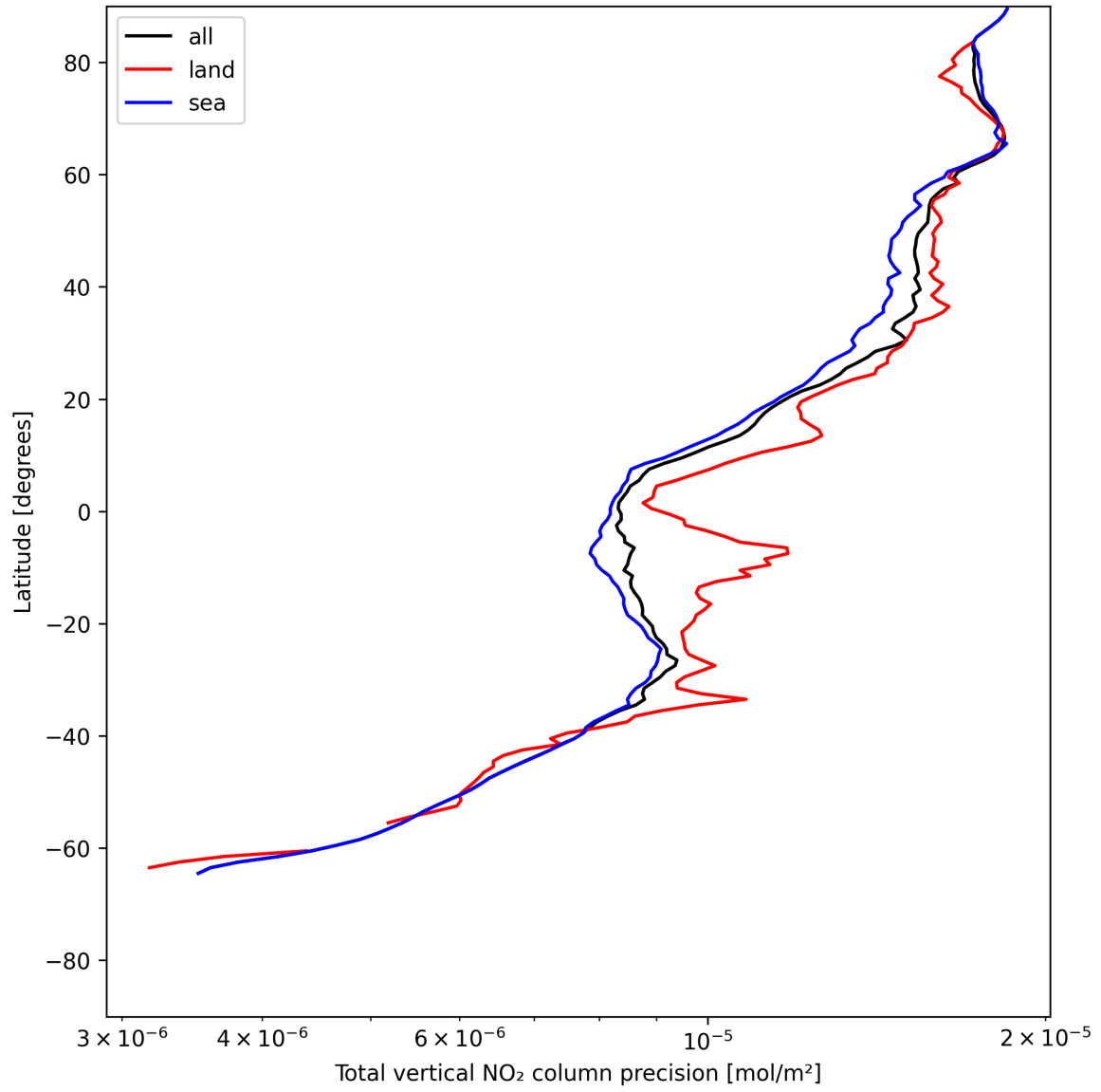
Figure 22: Zonal average of “Total vertical NO 2 column precision” for 2025-06-22 to 2025-06-23.
