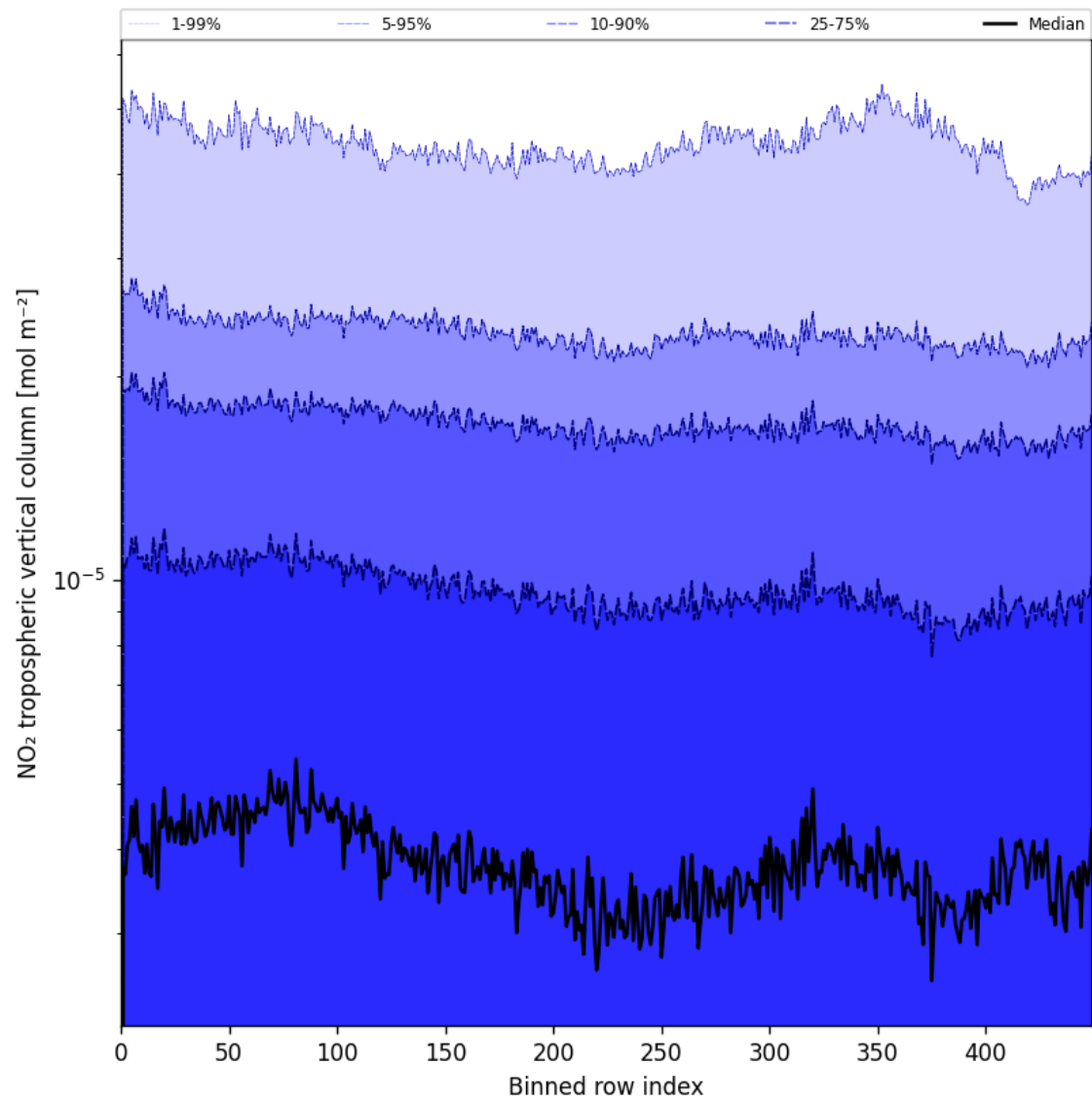
Figure 46: Along track statistics of “NO 2 tropospheric vertical column” for 2025-06-22 to 2025-06-23
