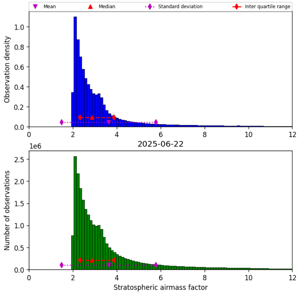
Figure 44: Histogram of “Stratospheric airmass factor” for 2025-06-22 to 2025-06-23
