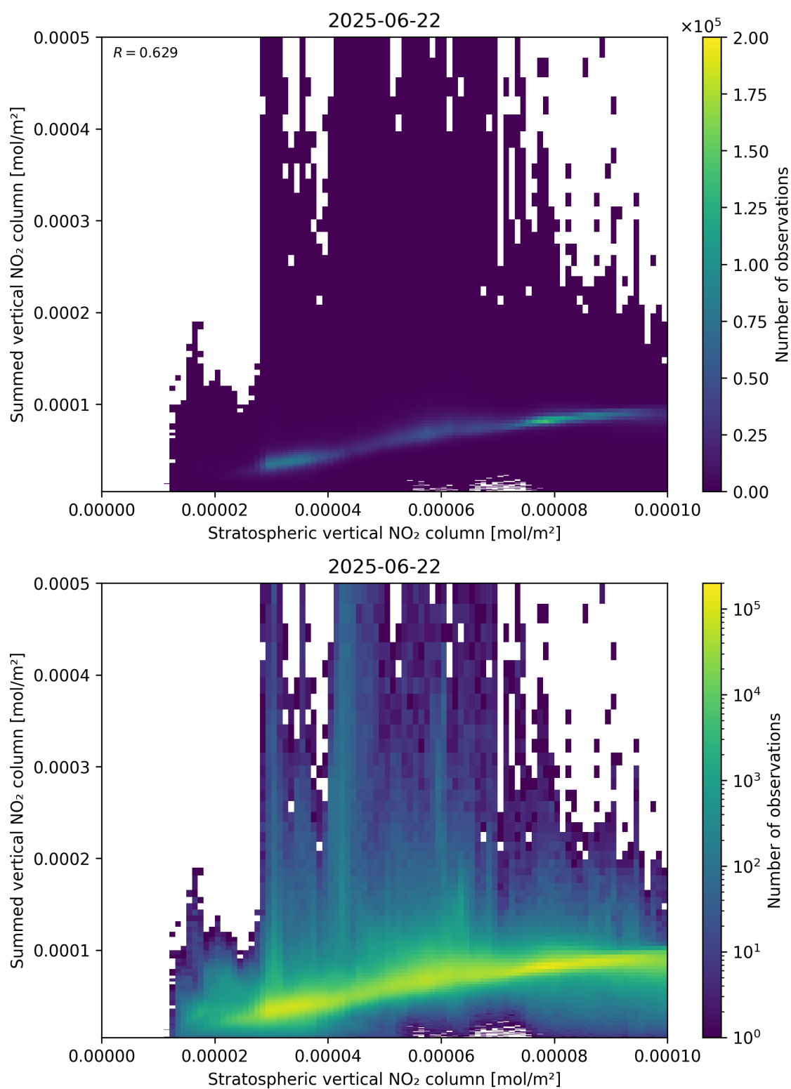
Figure 98: Scatter density plot of “Stratospheric vertical NO 2 column” against “Summed vertical NO 2 column” for 2025-06-22 to 2025-06-23.
