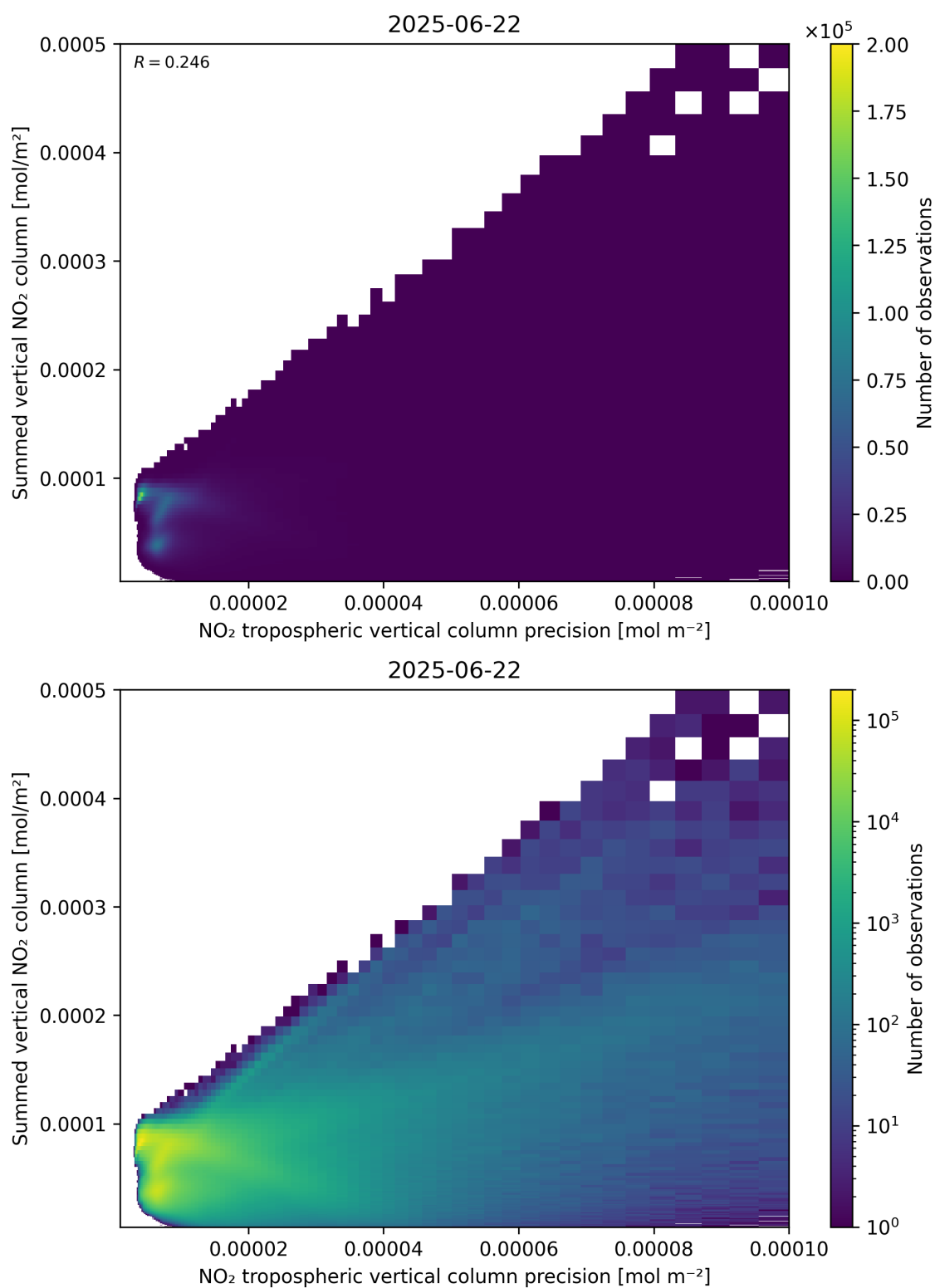
Figure 136: Scatter density plot of “NO 2 tropospheric vertical column precision” against “Summed vertical NO 2 column” for 2025-06-22 to 2025-06-23.
