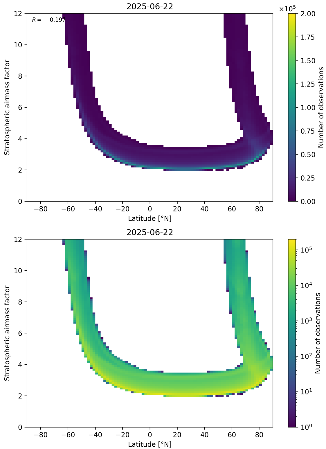
Figure 83: Scatter density plot of “Latitude” against “Stratospheric air mass factor” for 2025-06-22 to 2025-06-23.
