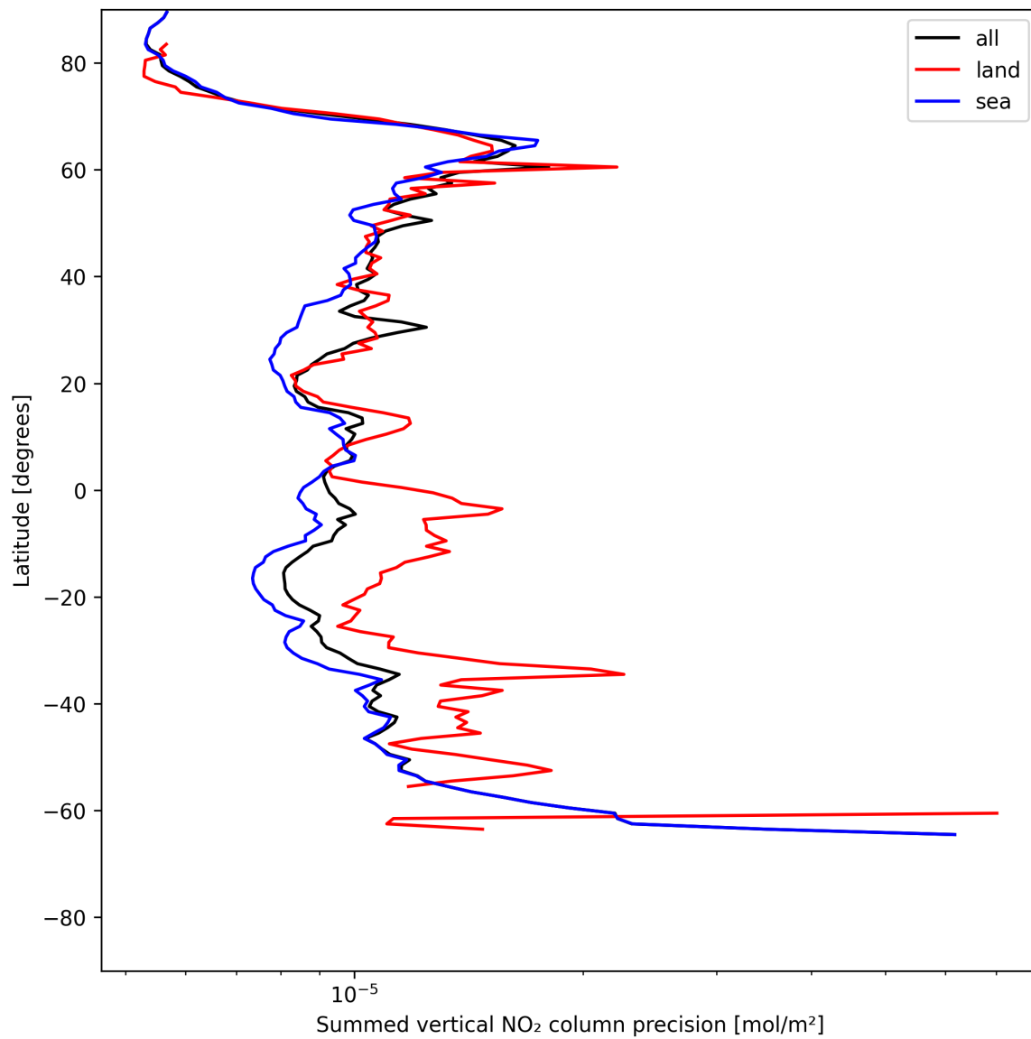
Figure 24: Zonal average of “Summed vertical NO 2 column precision” for 2025-06-22 to 2025-06-23.
