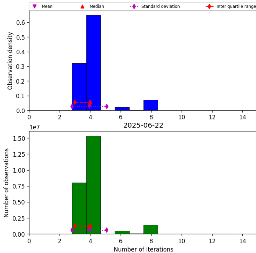
Figure 34: Histogram of “Number of iterations” for 2025-06-22 to 2025-06-23
