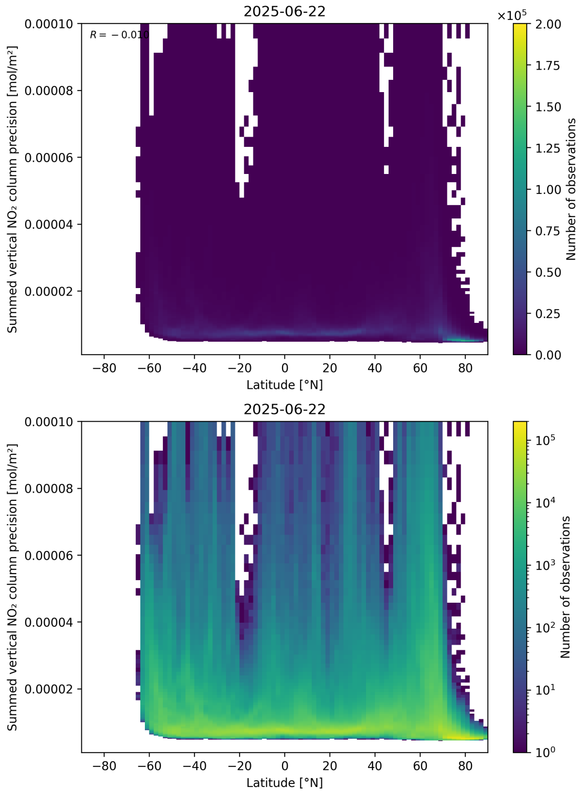
Figure 89: Scatter density plot of “Latitude” against “Summed vertical NO 2 column precision” for 2025-06-22 to 2025-06-23.
