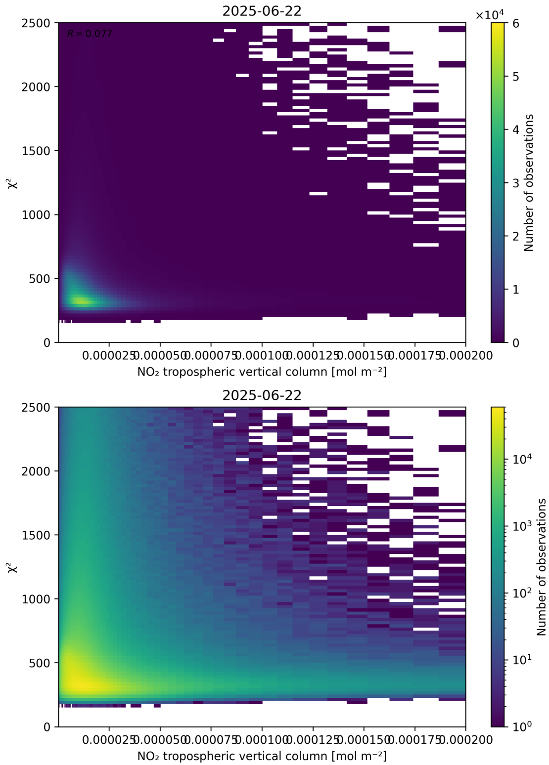
Figure 124: Scatter density plot of “NO 2 tropospheric vertical column” against “ \chi^2 ” for 2025-06-22 to 2025-06-23.
