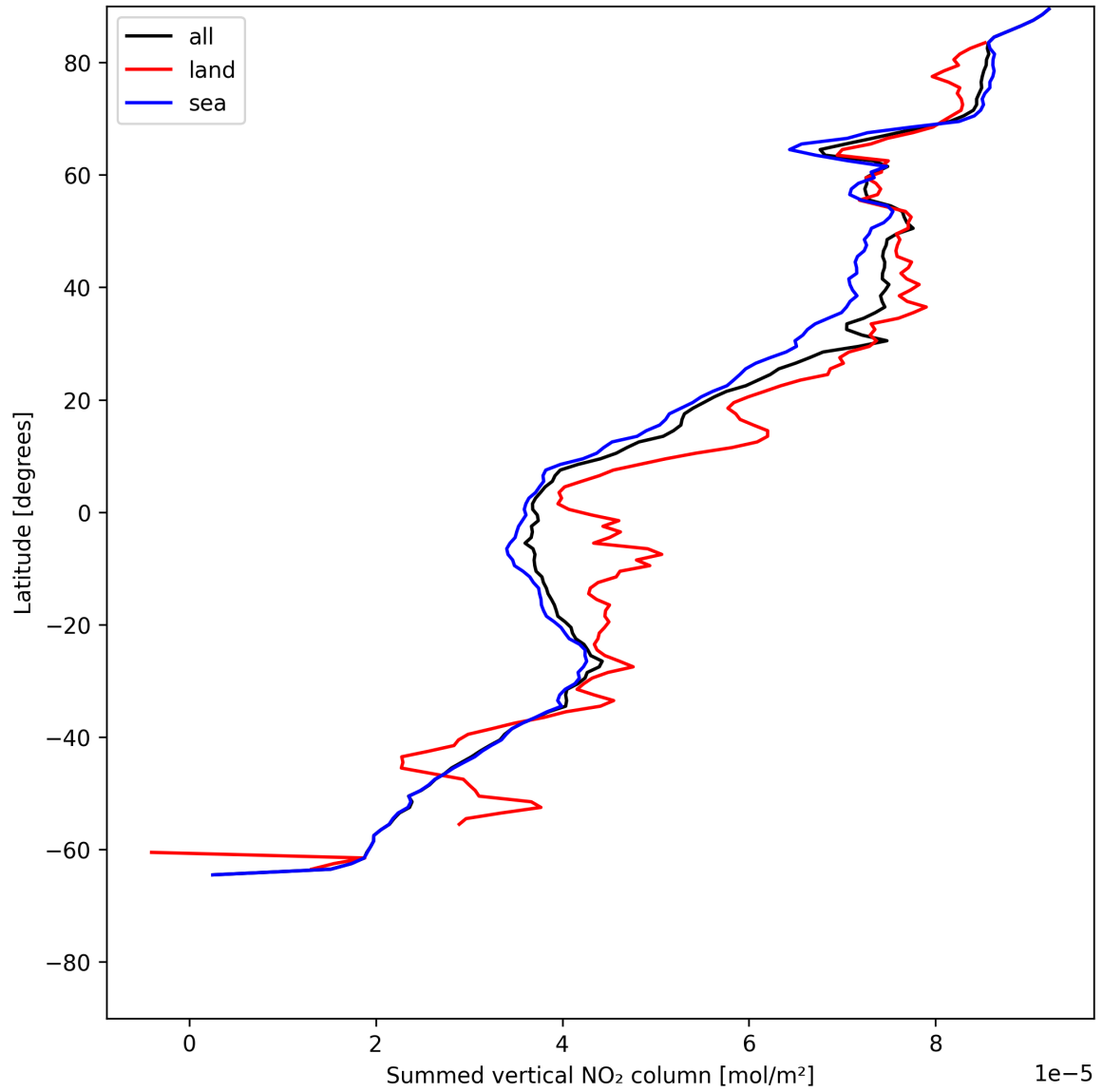
Figure 23: Zonal average of “Summed vertical NO 2 column” for 2025-06-22 to 2025-06-23.
