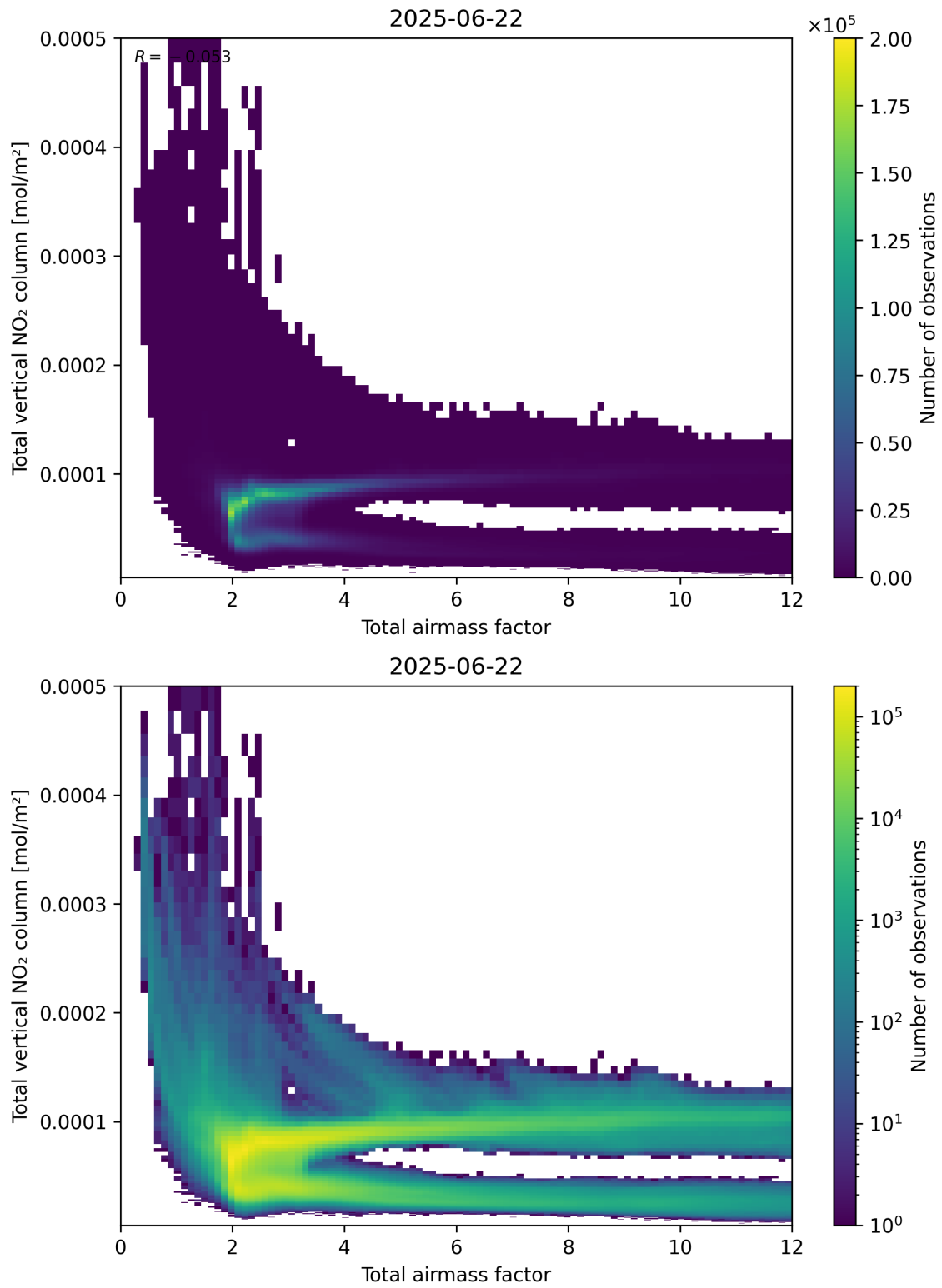
Figure 67: Scatter density plot of “Total airmass factor” against “Total vertical NO 2 column” for 2025-06-22 to 2025-06-23.
