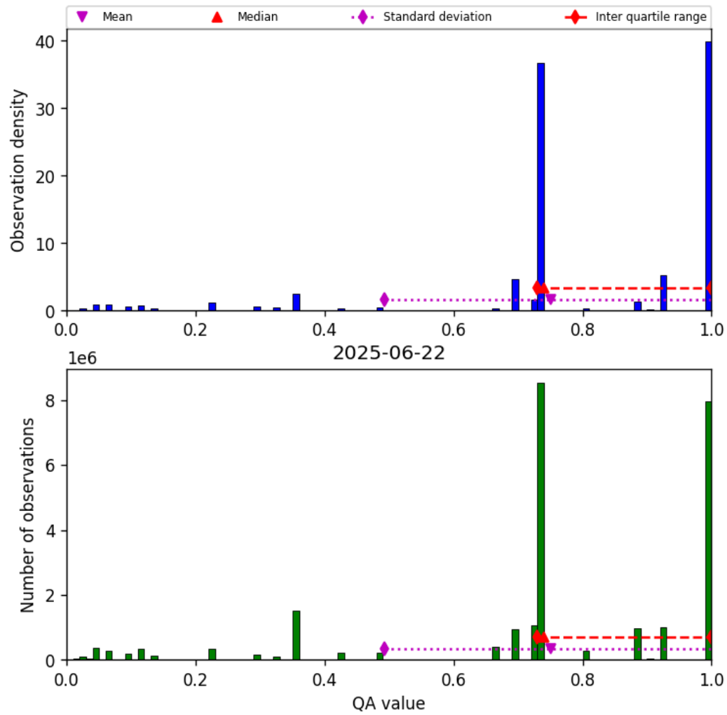
Figure 28: Histogram of “QA value” for 2025-06-22 to 2025-06-23
