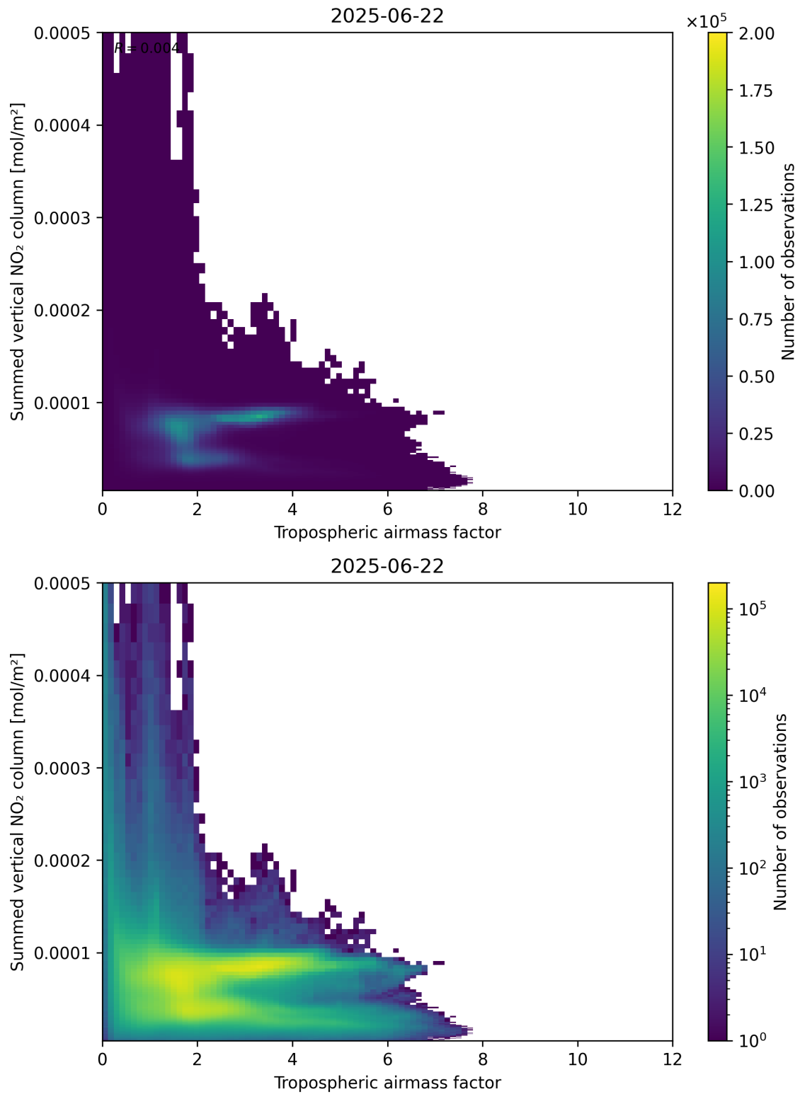
Figure 75: Scatter density plot of “Tropospheric airmass factor” against “Summed vertical NO 2 column” for 2025-06-22 to 2025-06-23.
