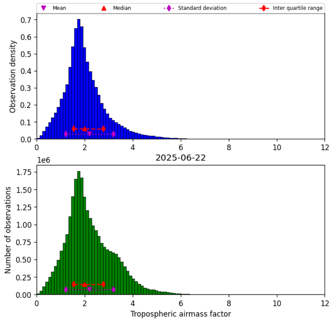
Figure 31: Histogram of “Tropospheric airmass factor” for 2025-06-22 to 2025-06-23
