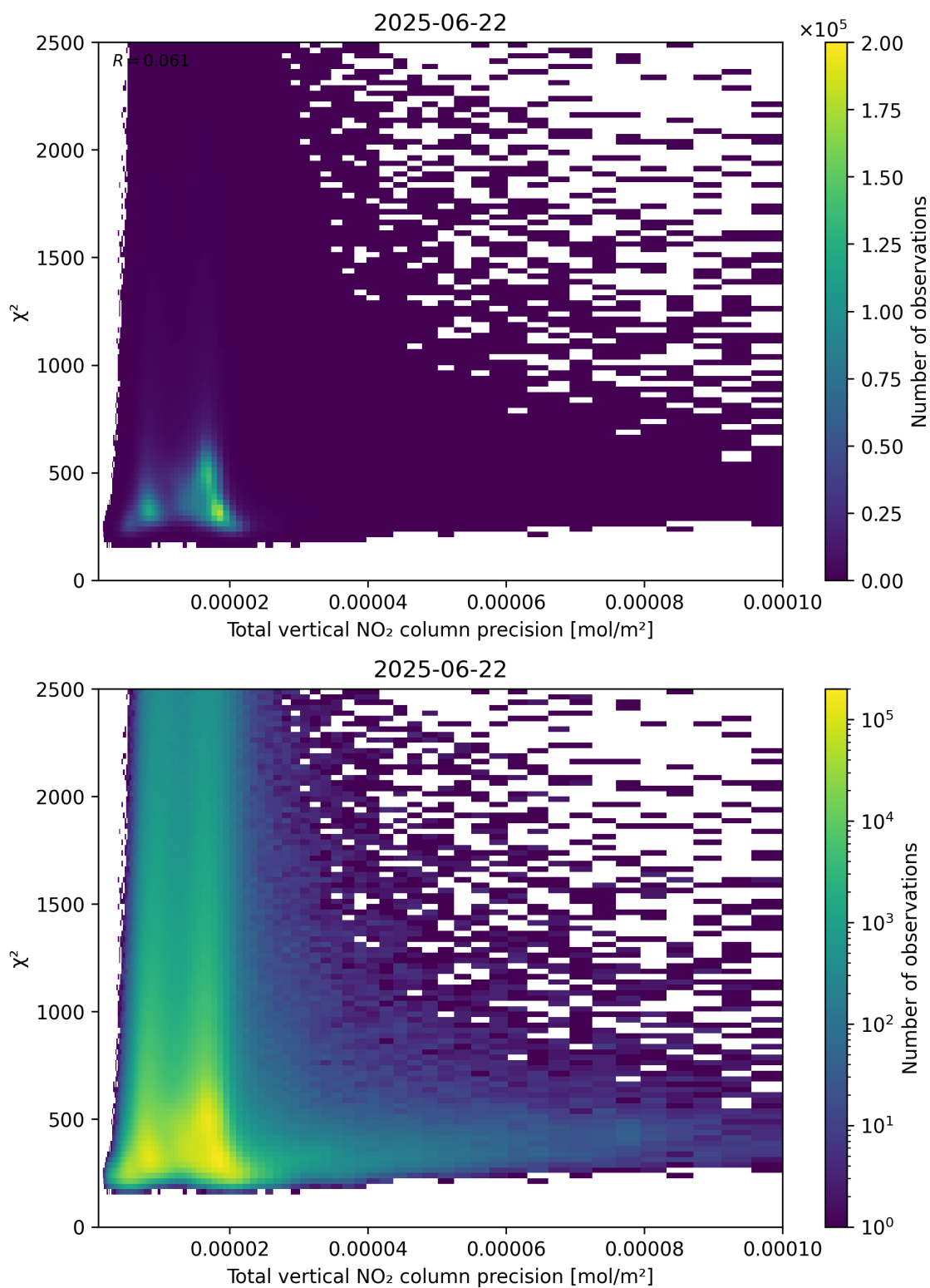
Figure 116: Scatter density plot of “Total vertical NO 2 column precision” against “ \chi^2 ” for 2025-06-22 to 2025-06-23.
