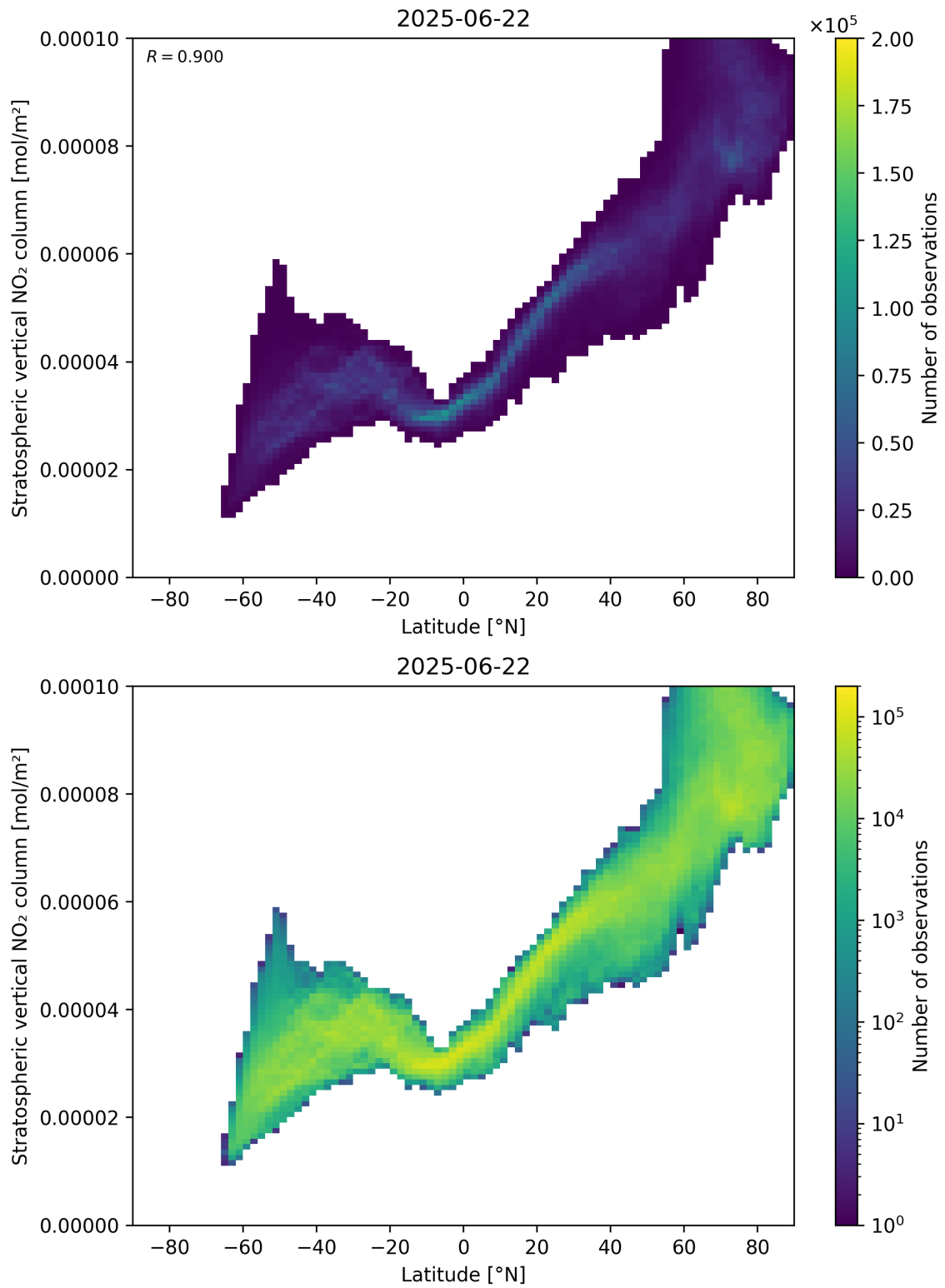
Figure 87: Scatter density plot of “Latitude” against “Stratospheric vertical \text{NO}_2 column” for 2025-06-22 to 2025-06-23.
