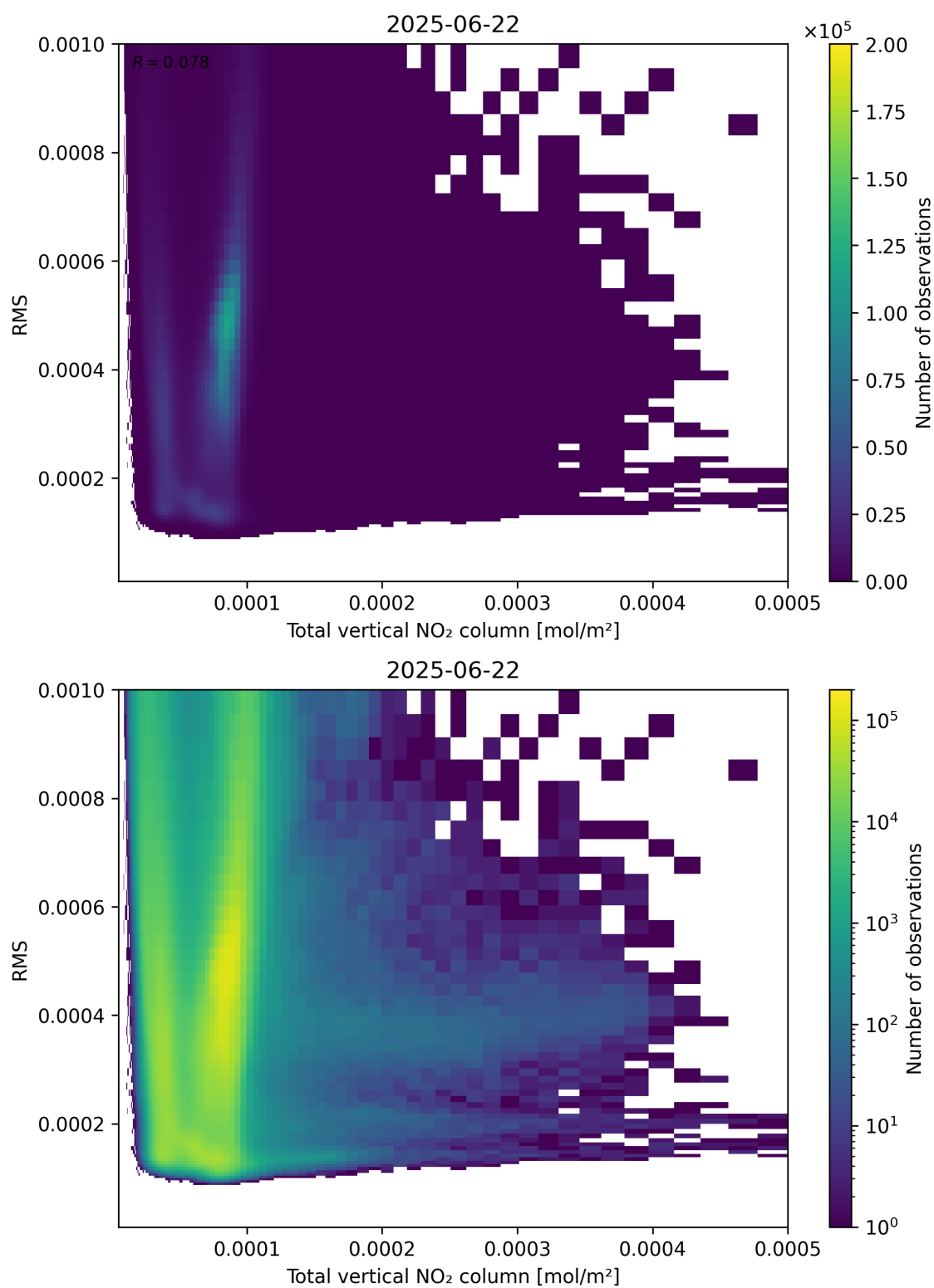
Figure 120: Scatter density plot of “Total vertical NO 2 column” against “RMS” for 2025-06-22 to 2025-06-23.
