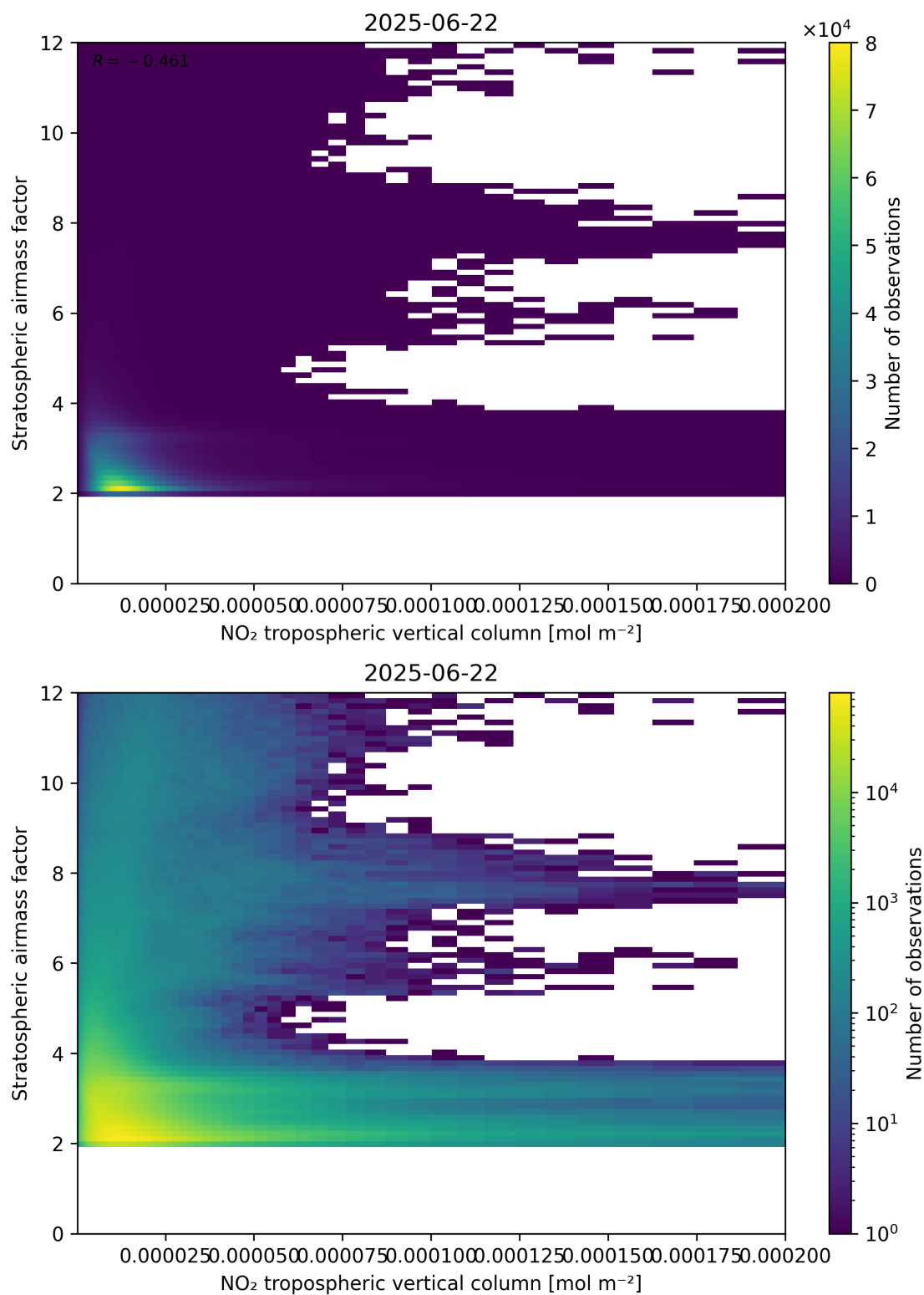
Figure 121: Scatter density plot of “NO 2 tropospheric vertical column” against “Stratospheric air mass factor” for 2025-06-22 to 2025-06-23.
