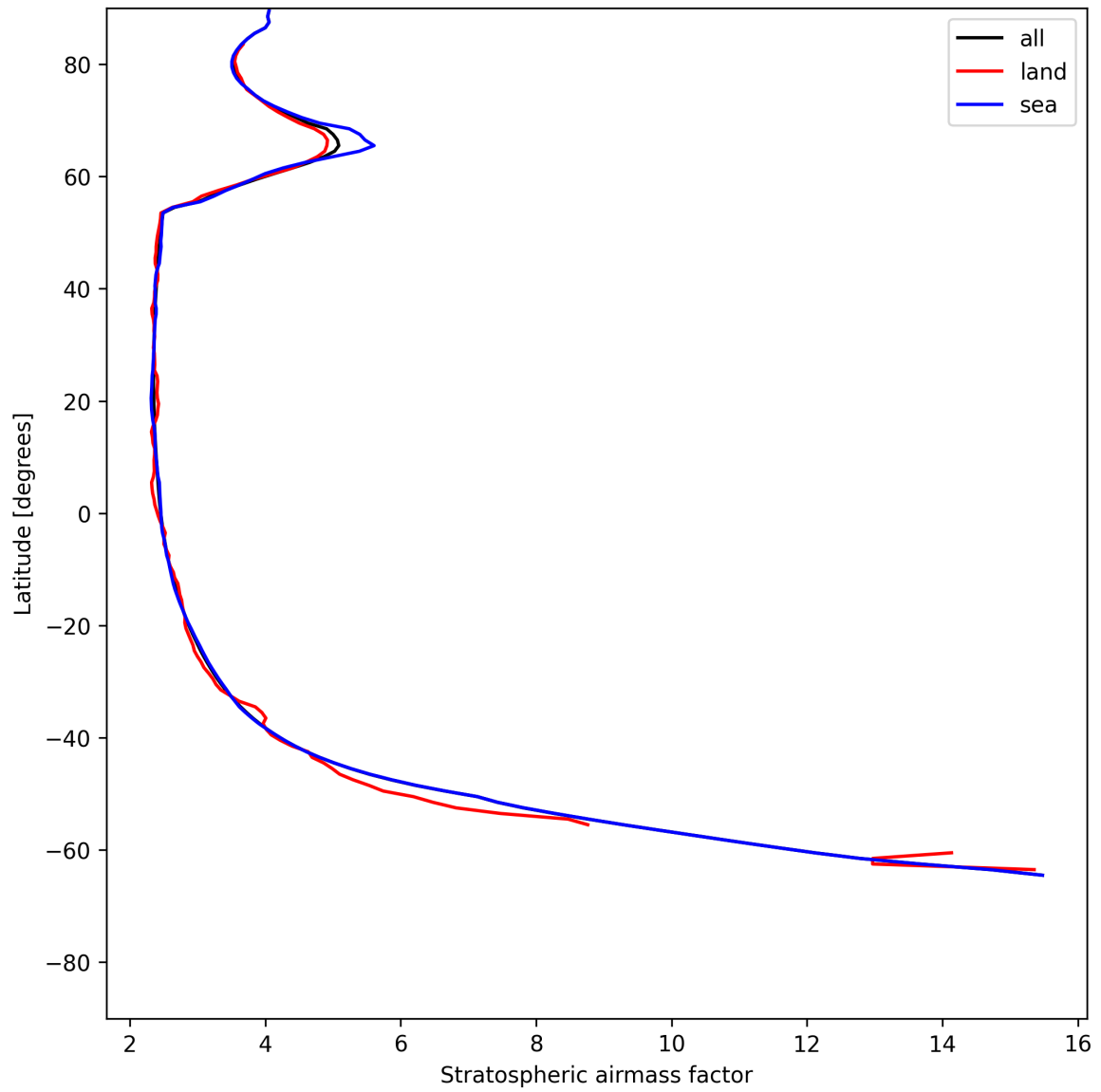
Figure 27: Zonal average of “Stratospheric airmass factor” for 2025-06-22 to 2025-06-23.
