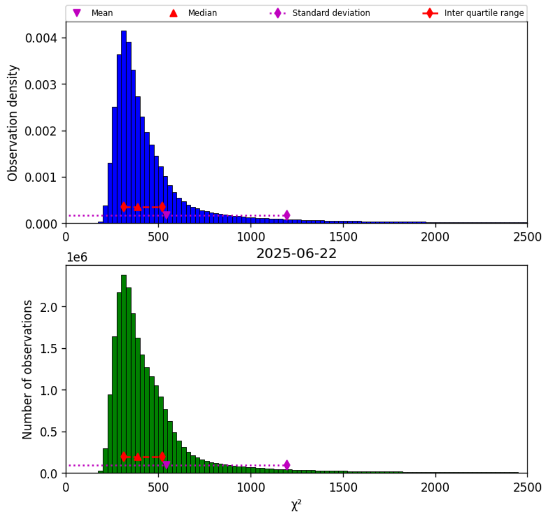
Figure 42: Histogram of “ \chi^2 ” for 2025-06-22 to 2025-06-23
