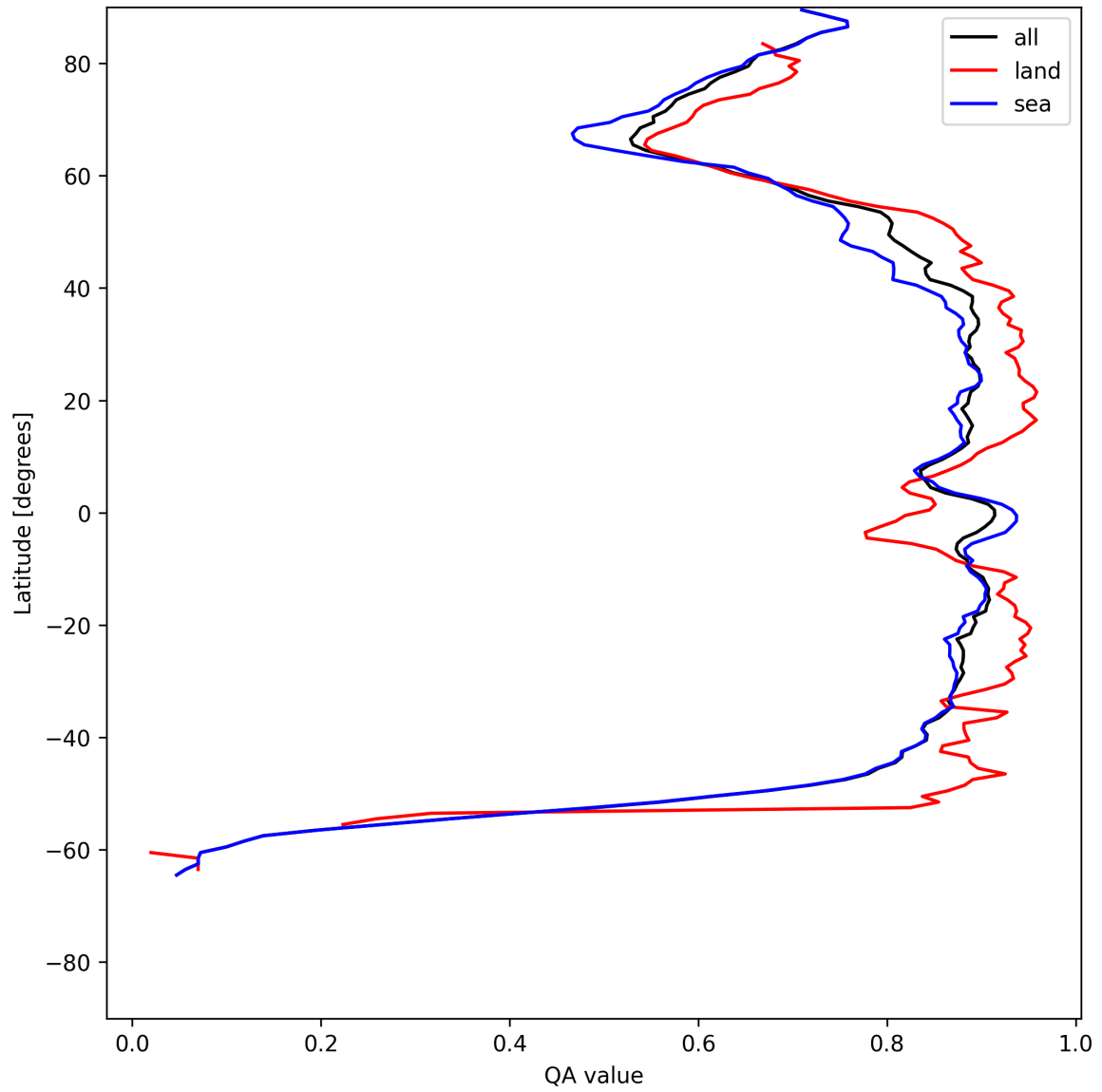
Figure 11: Zonal average of “QA value” for 2025-06-22 to 2025-06-23.
