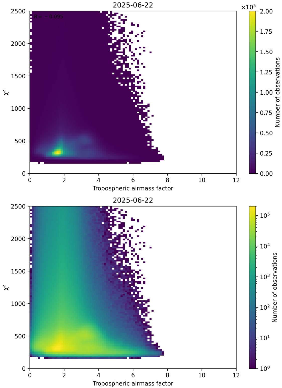
Figure 73: Scatter density plot of “Tropospheric airmass factor” against “ \chi^2 ” for 2025-06-22 to 2025-06-23.
