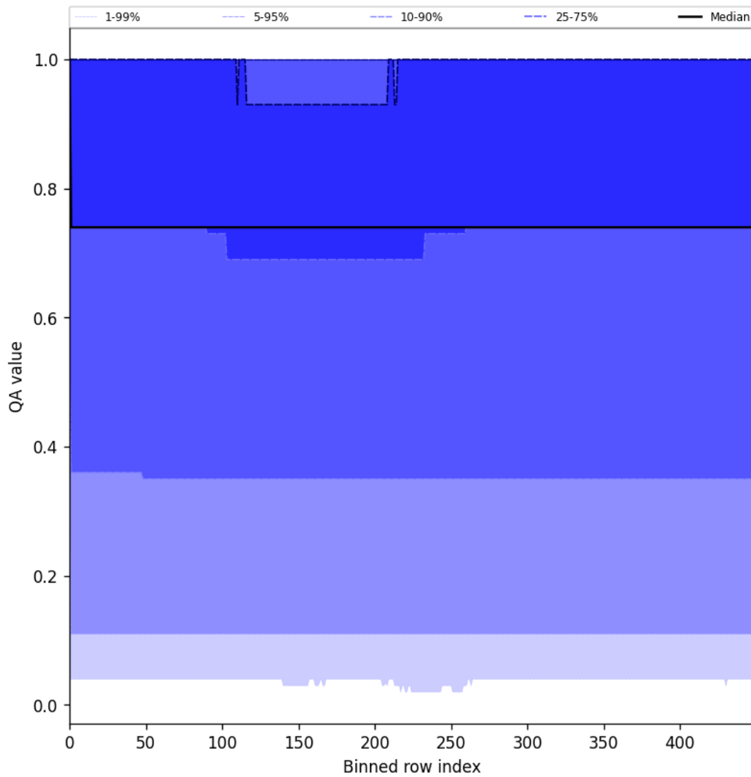
Figure 45: Along track statistics of “QA value” for 2025-06-22 to 2025-06-23
