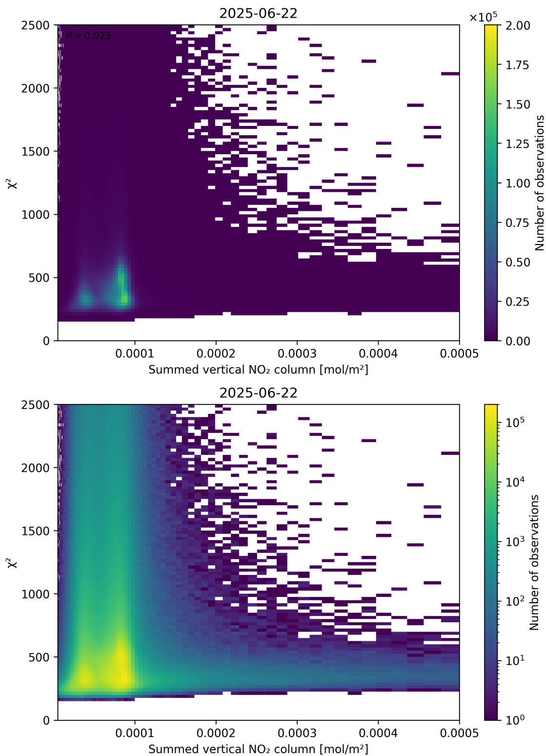
Figure 104: Scatter density plot of “Summed vertical NO 2 column” against “ \chi^2 ” for 2025-06-22 to 2025-06-23.
