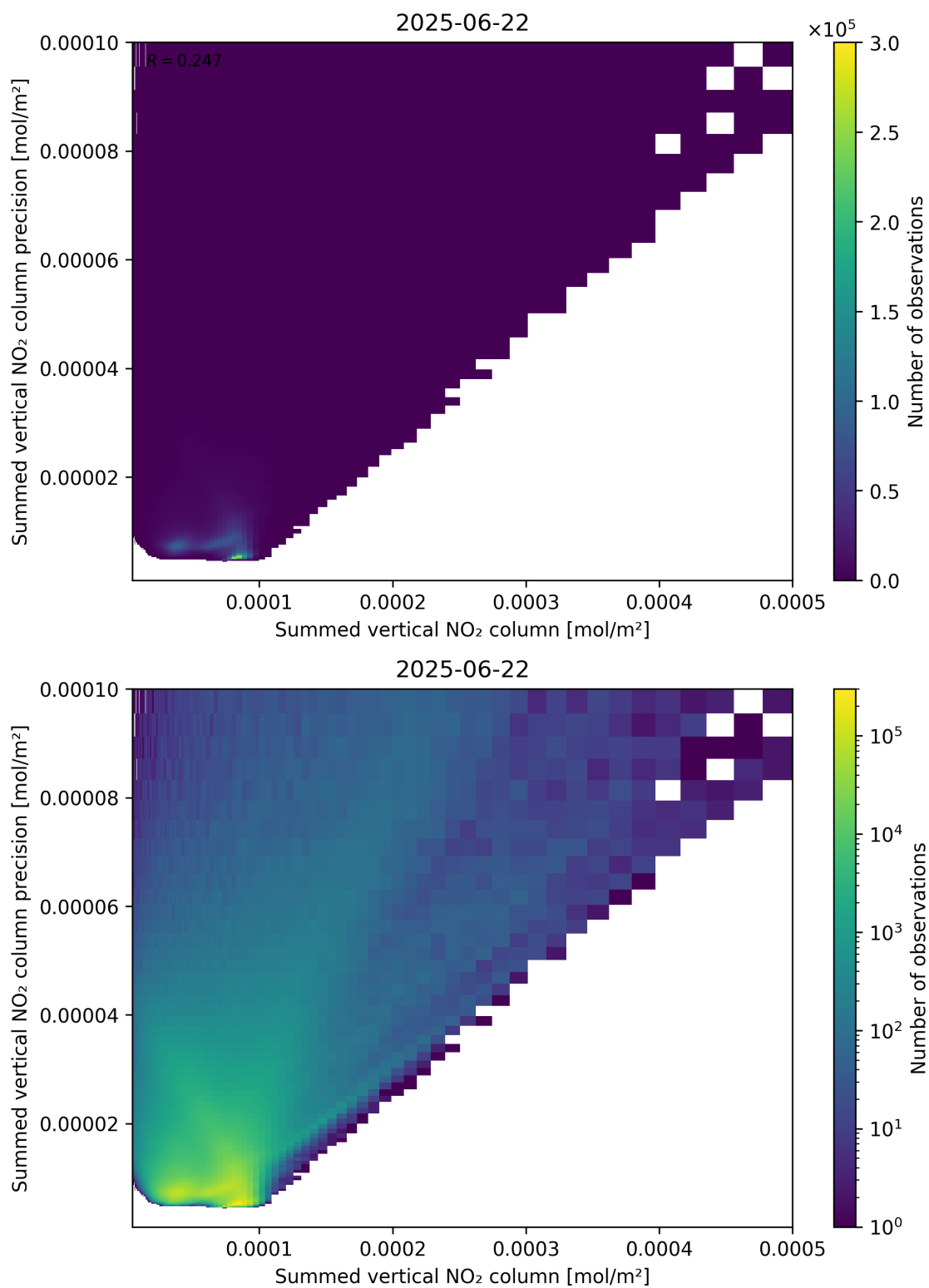
Figure 105: Scatter density plot of “Summed vertical NO 2 column” against “Summed vertical NO 2 column precision” for 2025-06-22 to 2025-06-23.
