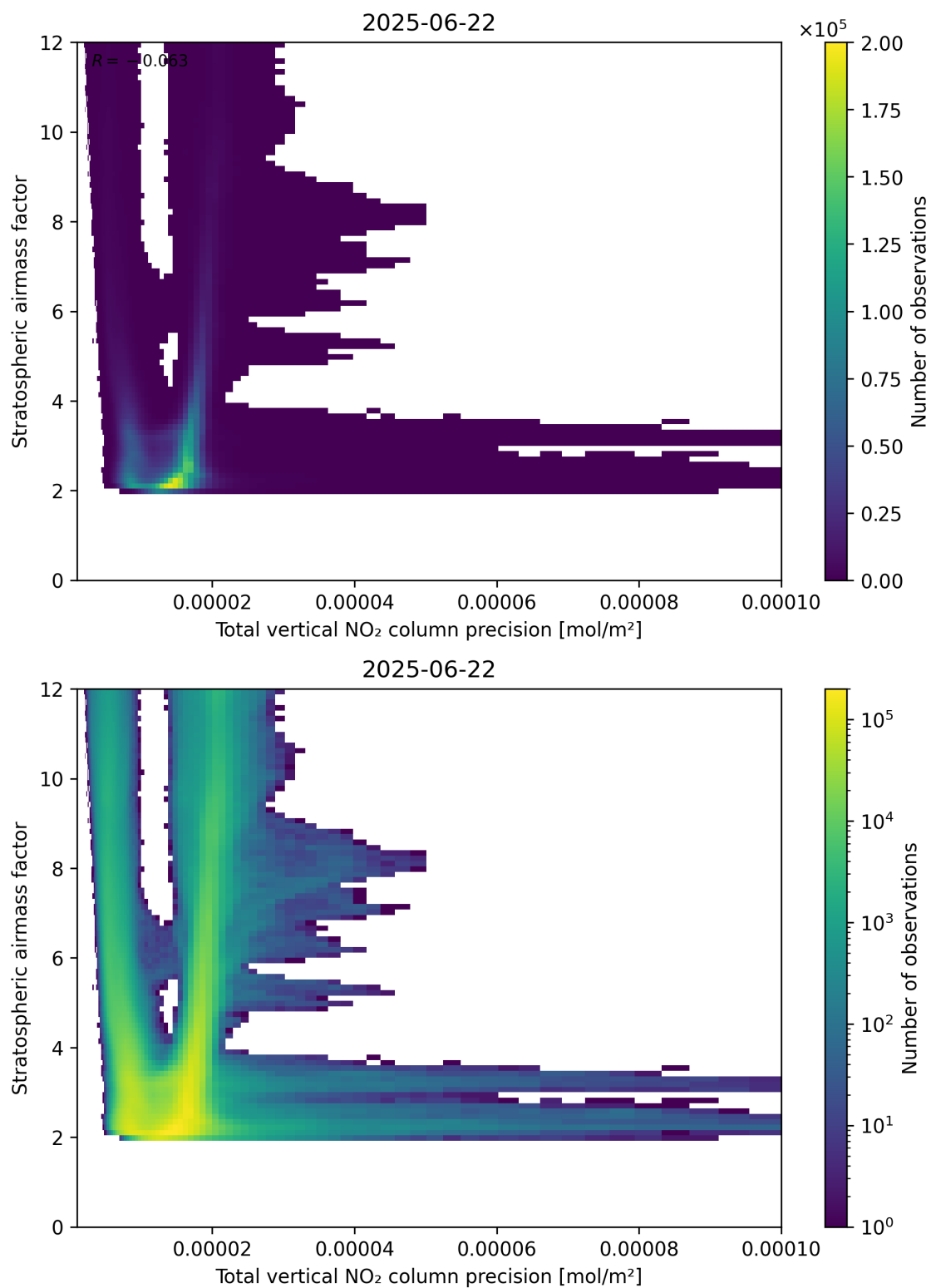
Figure 115: Scatter density plot of “Total vertical NO 2 column precision” against “Stratospheric air mass factor” for 2025-06-22 to 2025-06-23.
