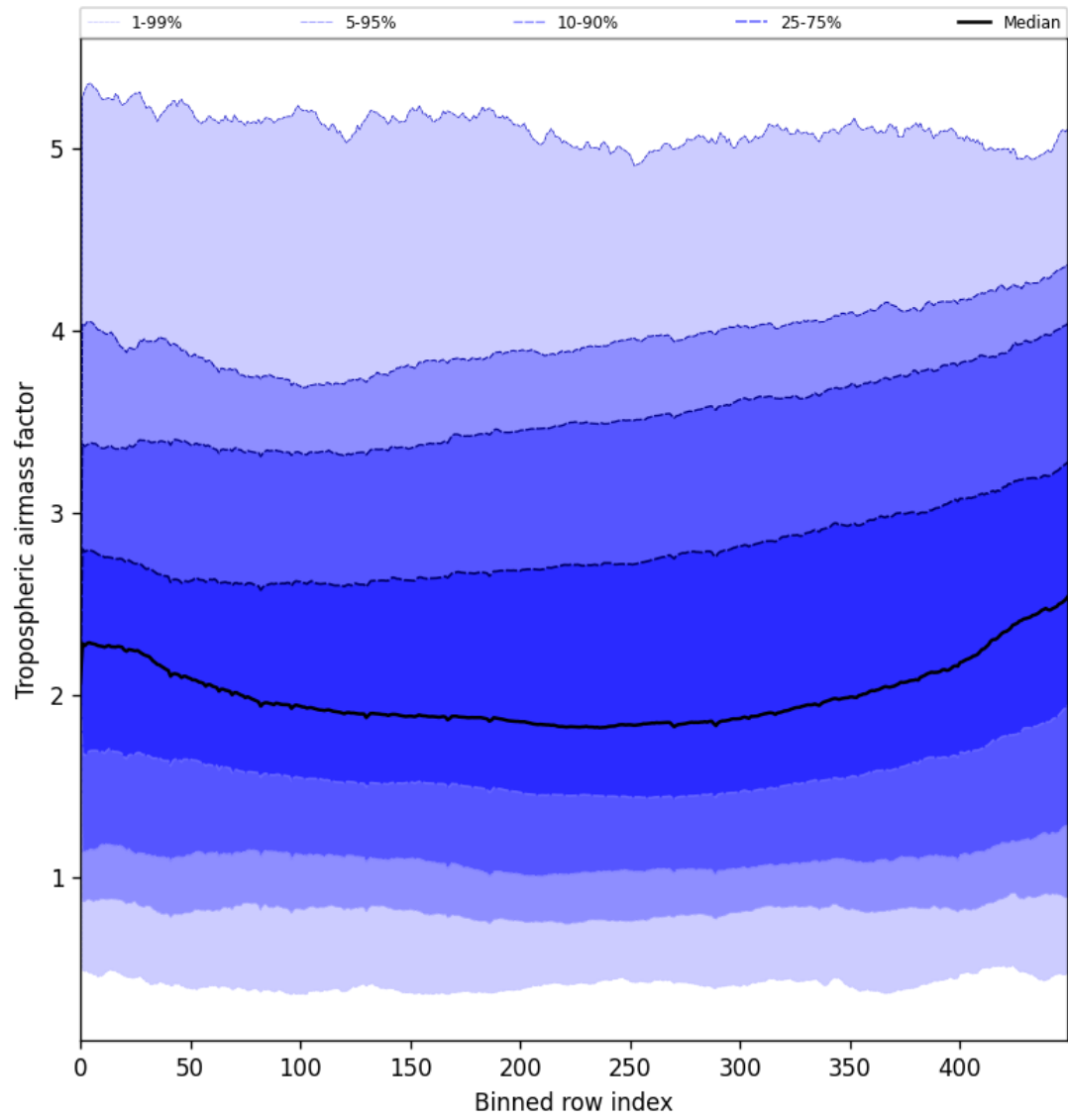
Figure 48: Along track statistics of “Tropospheric airmass factor” for 2025-06-22 to 2025-06-23
