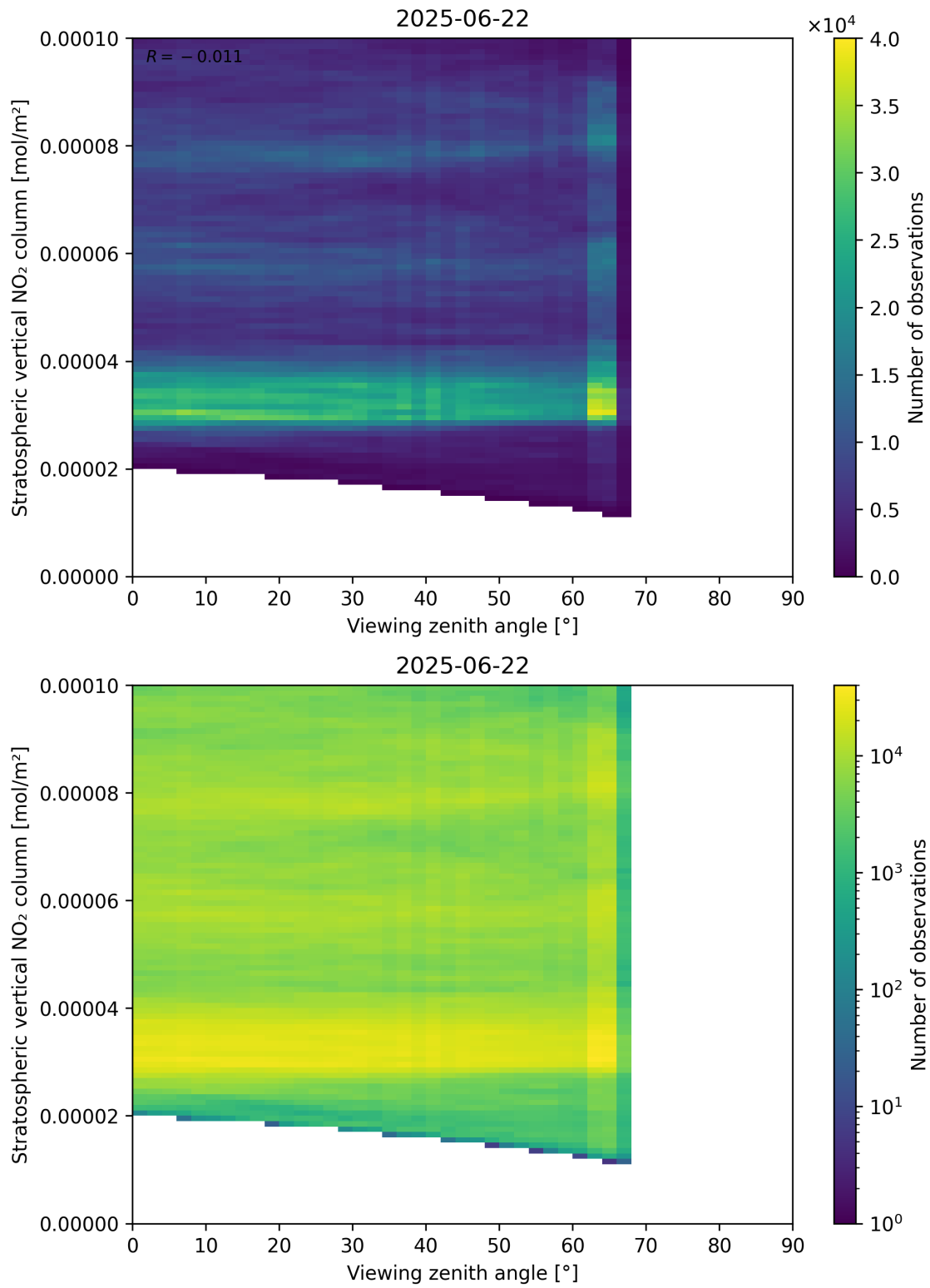
Figure 164: Scatter density plot of “Viewing zenith angle” against “Stratospheric vertical NO 2 column” for 2025-06-22 to 2025-06-23.
