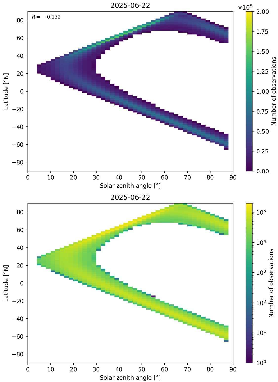
Figure 149: Scatter density plot of “Solar zenith angle” against “Latitude” for 2025-06-22 to 2025-06-23.
