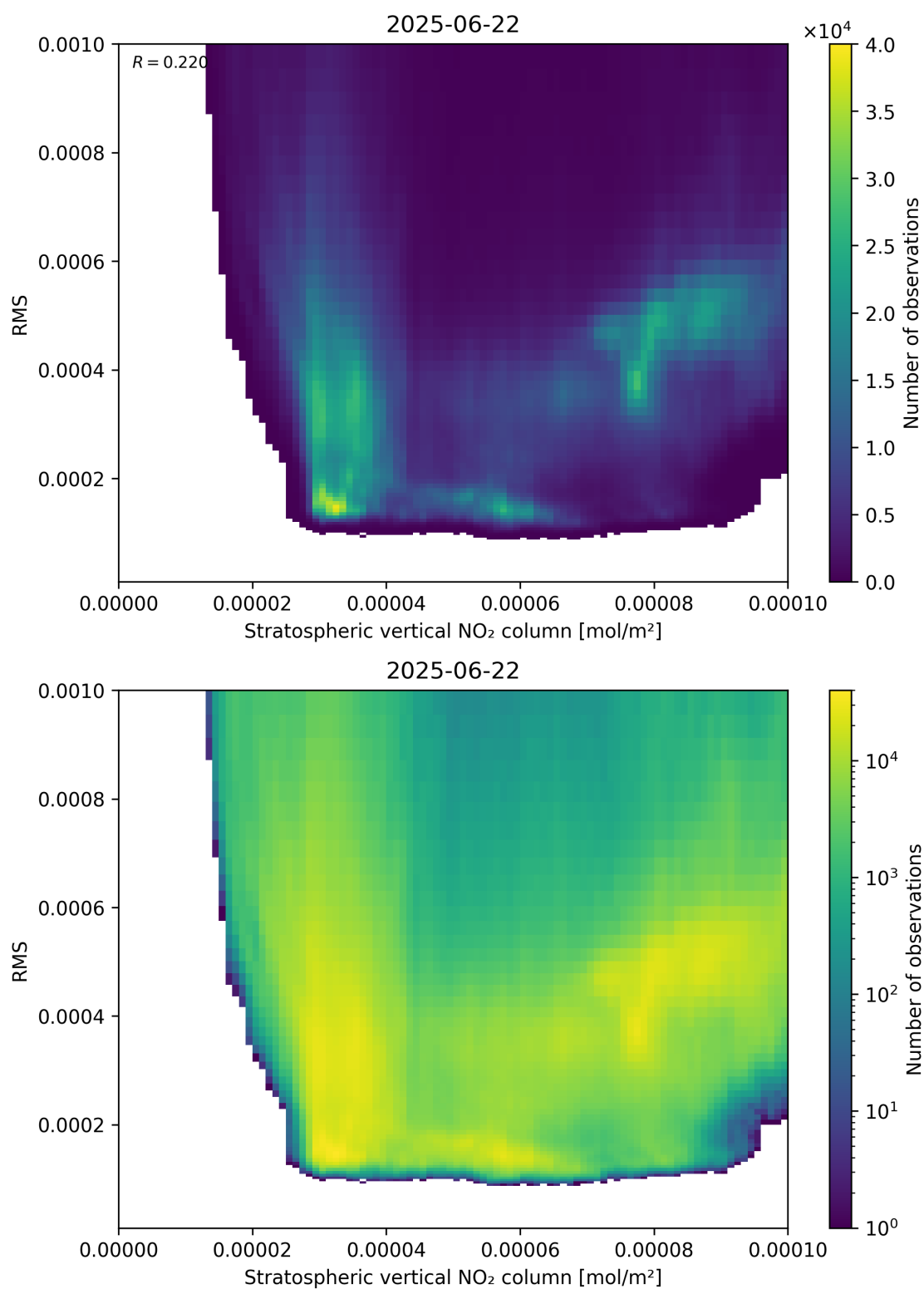
Figure 102: Scatter density plot of “Stratospheric vertical NO 2 column” against “RMS” for 2025-06-22 to 2025-06-23.
