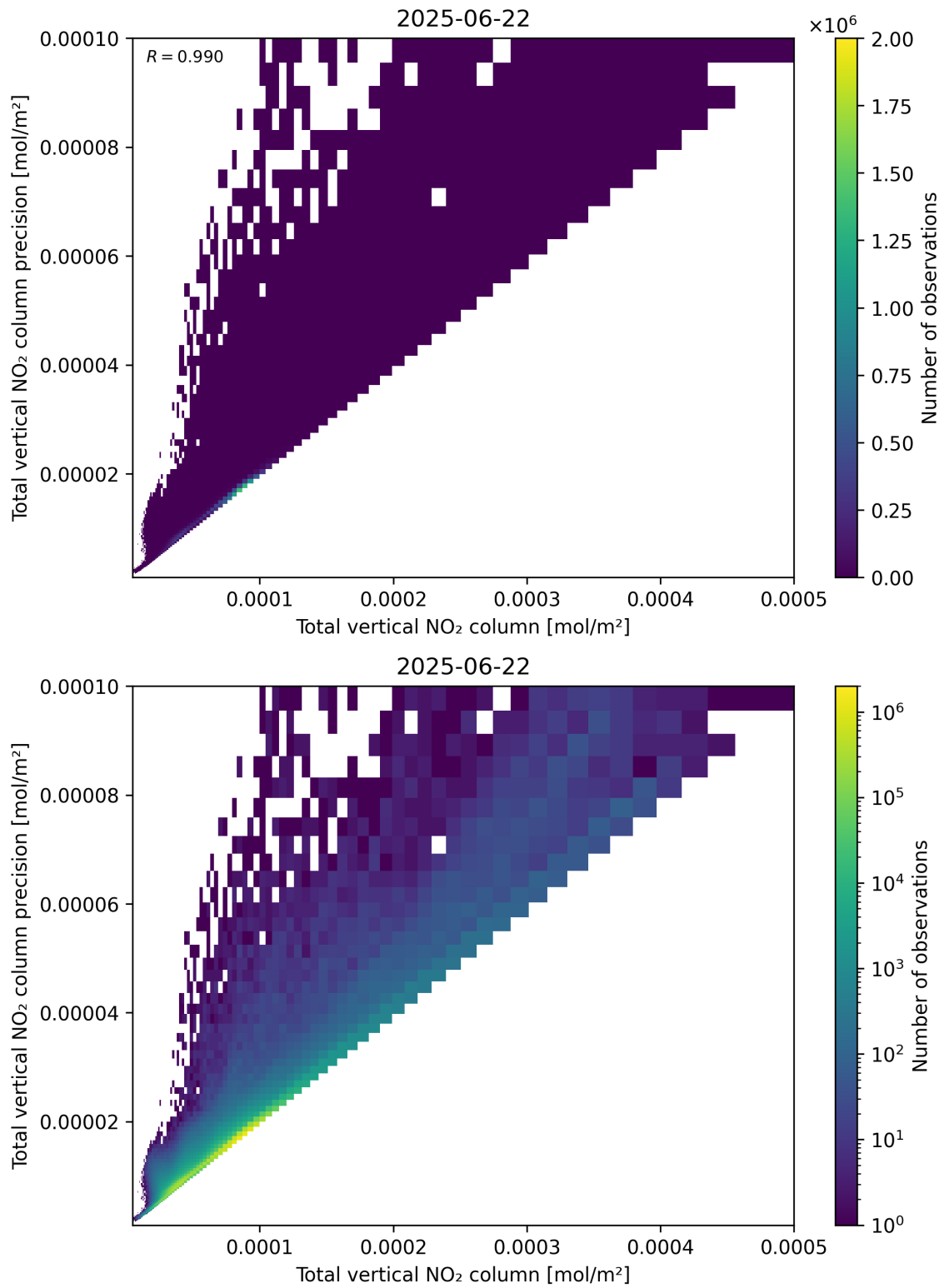
Figure 114: Scatter density plot of “Total vertical NO 2 column” against “Total vertical NO 2 column precision” for 2025-06-22 to 2025-06-23.
