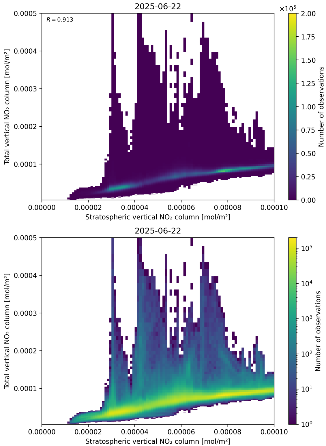
Figure 100: Scatter density plot of “Stratospheric vertical NO 2 column” against “Total vertical NO 2 column” for 2025-06-22 to 2025-06-23.
