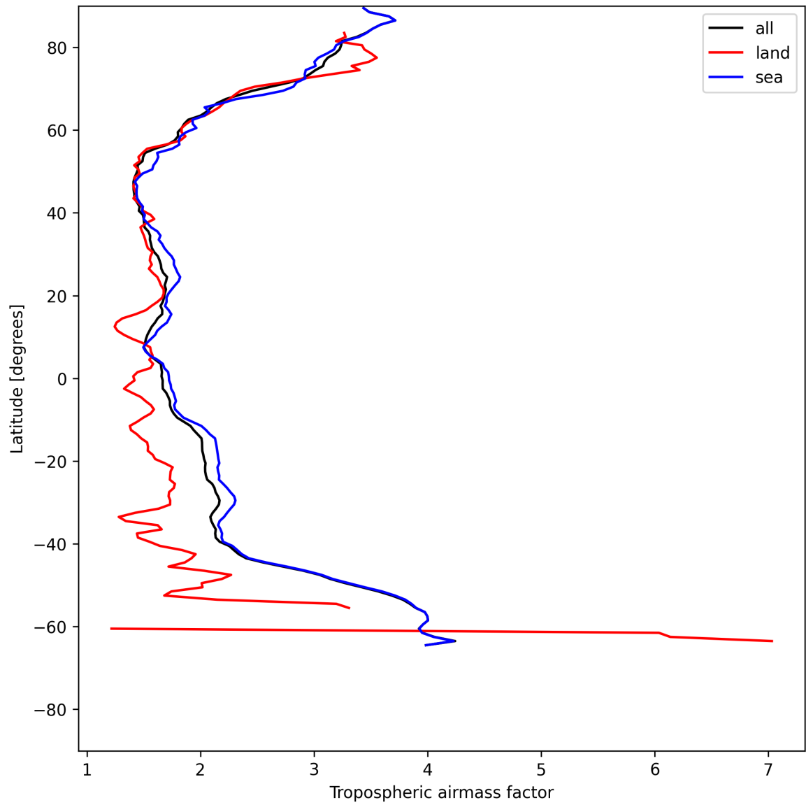
Figure 14: Zonal average of “Tropospheric airmass factor” for 2025-06-22 to 2025-06-23.
