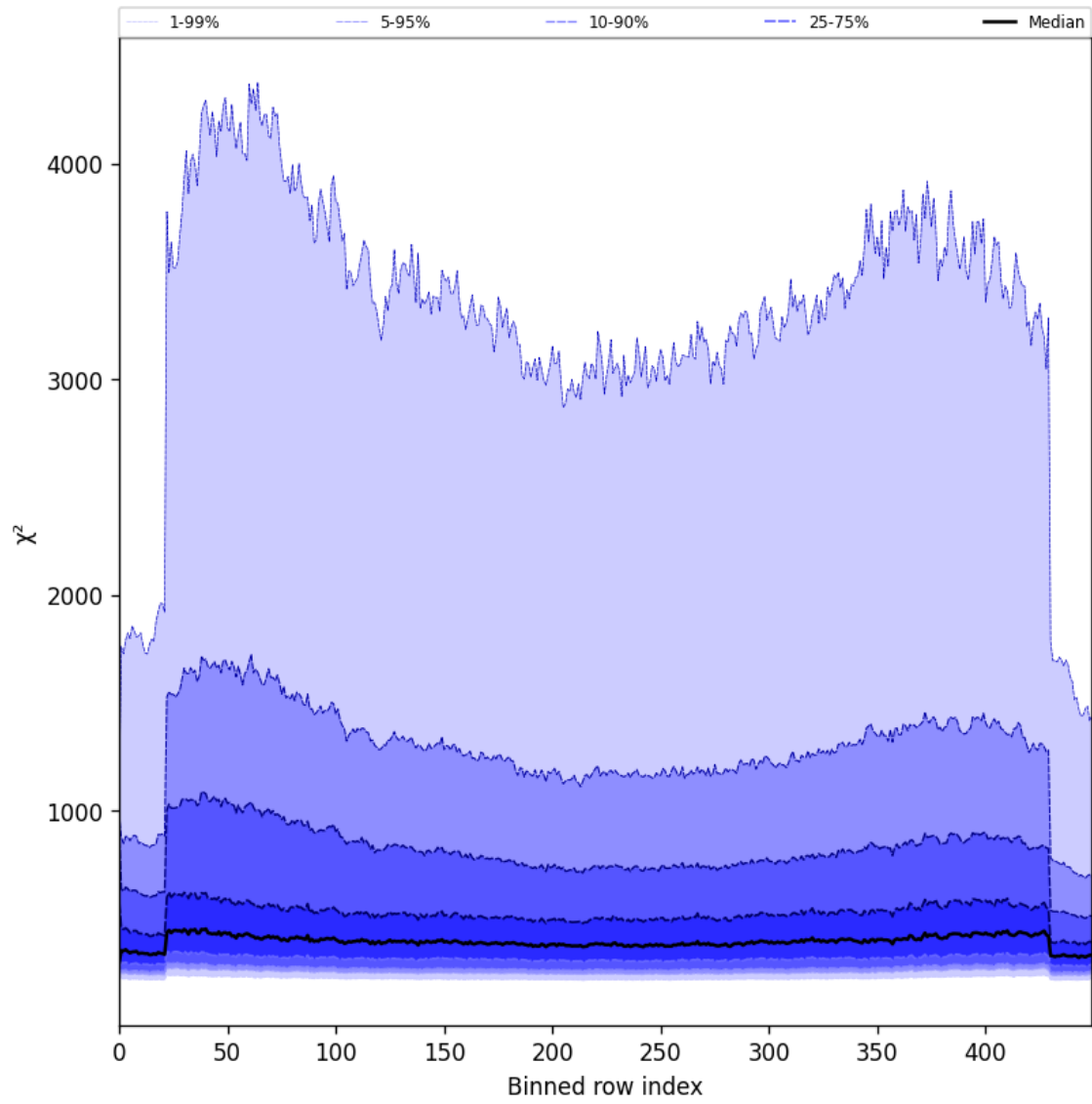
Figure 59: Along track statistics of “ \chi^2 ” for 2025-06-22 to 2025-06-23
