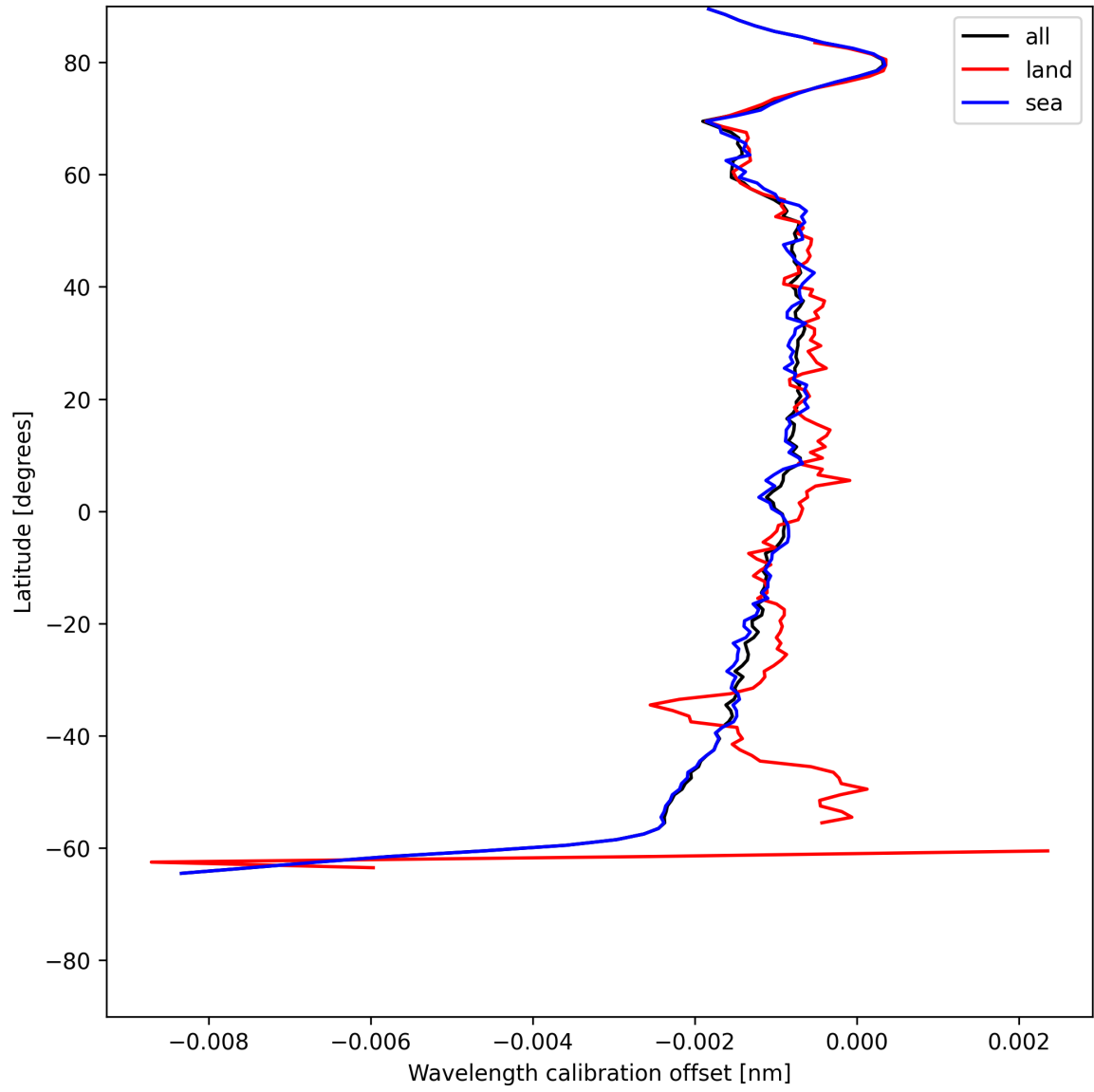
Figure 18: Zonal average of “Wavelength calibration offset” for 2025-06-22 to 2025-06-23.
