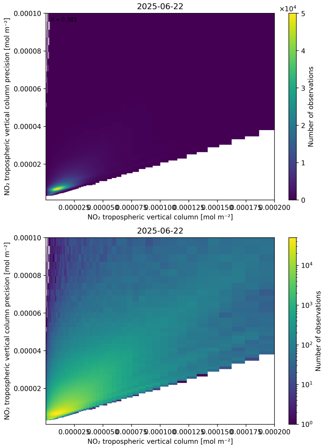
Figure 130: Scatter density plot of “NO 2 tropospheric vertical column” against “NO 2 tropospheric vertical column precision” for 2025-06-22 to 2025-06-23.
