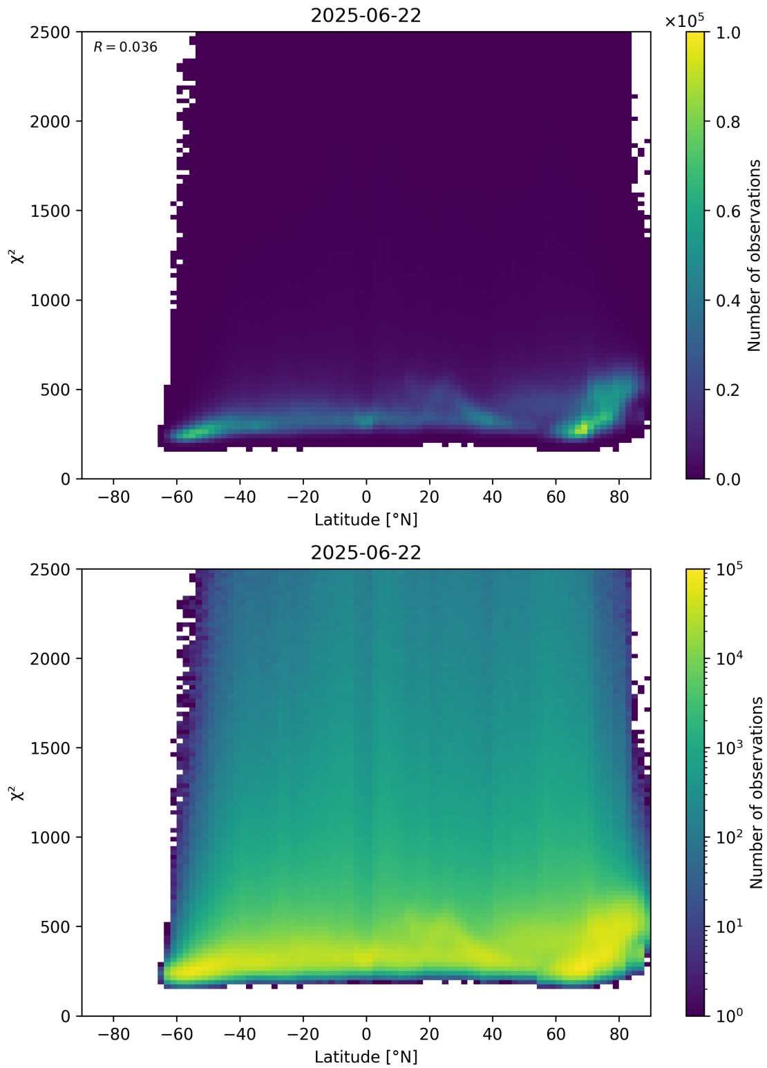
Figure 86: Scatter density plot of “Latitude” against “ \chi^2 ” for 2025-06-22 to 2025-06-23.
