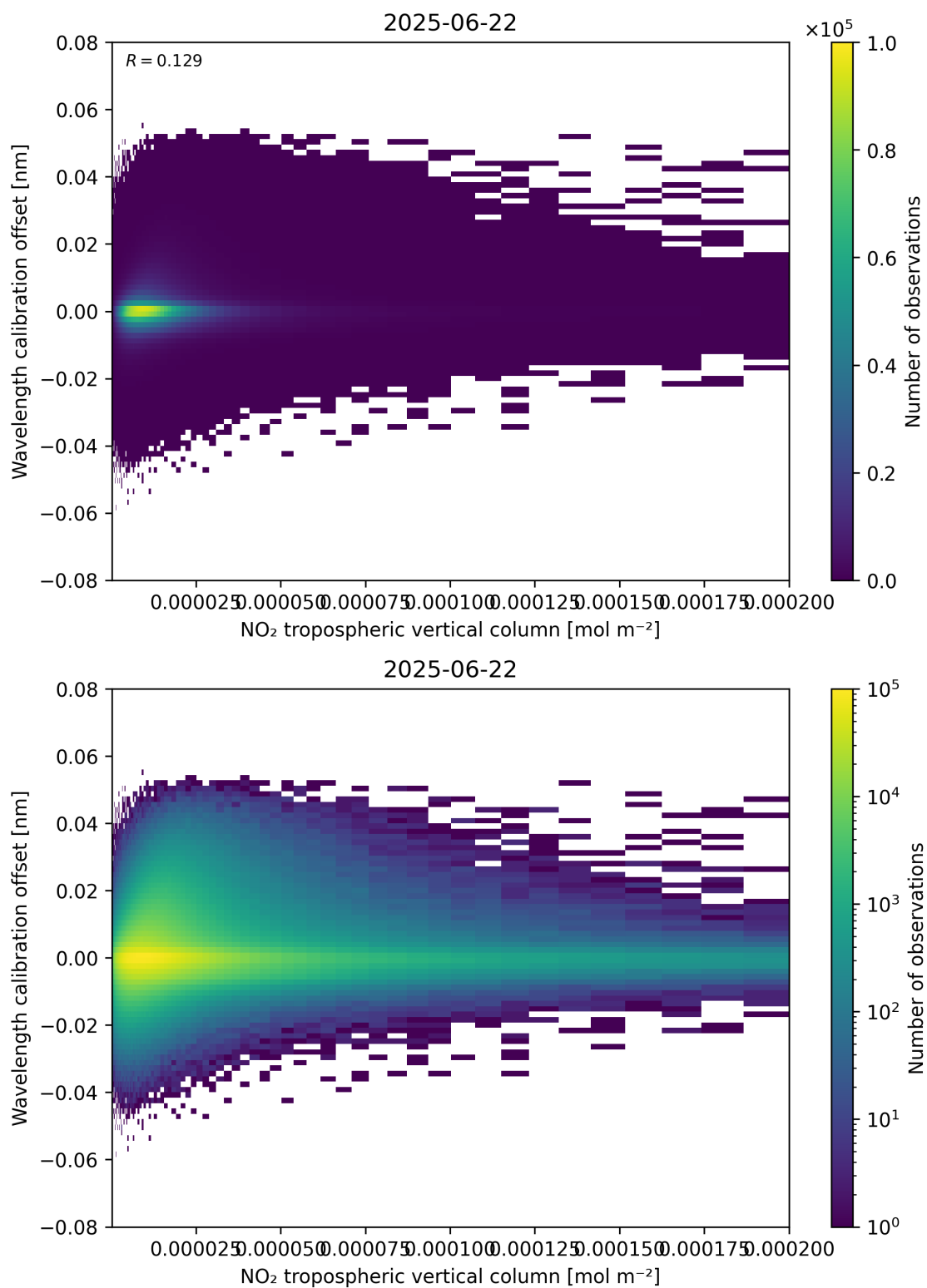
Figure 143: Scatter density plot of “NO 2 tropospheric vertical column” against “Wavelength calibration offset” for 2025-06-22 to 2025-06-23.
