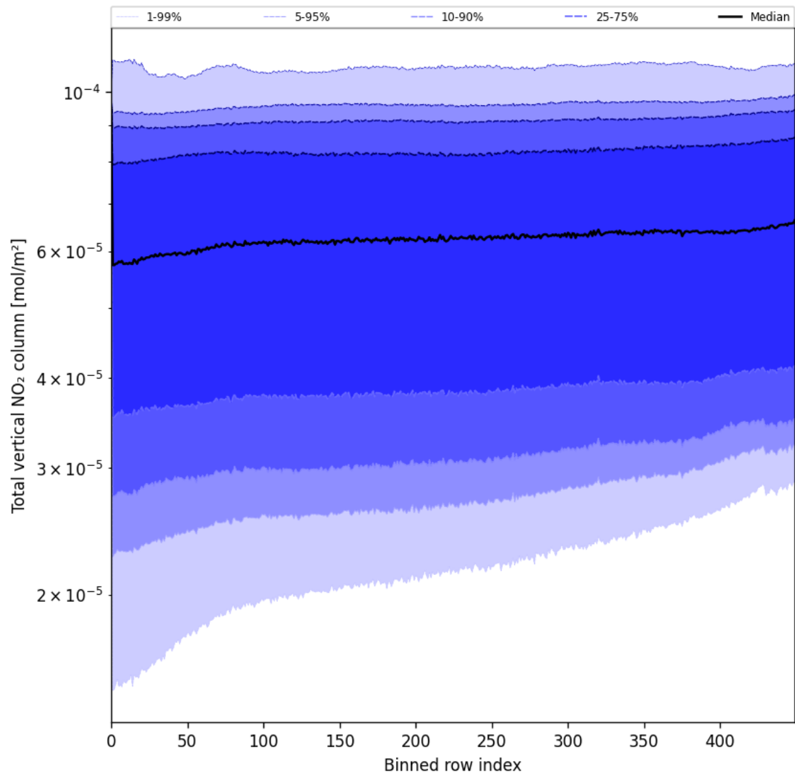
Figure 55: Along track statistics of “Total vertical NO 2 column” for 2025-06-22 to 2025-06-23
