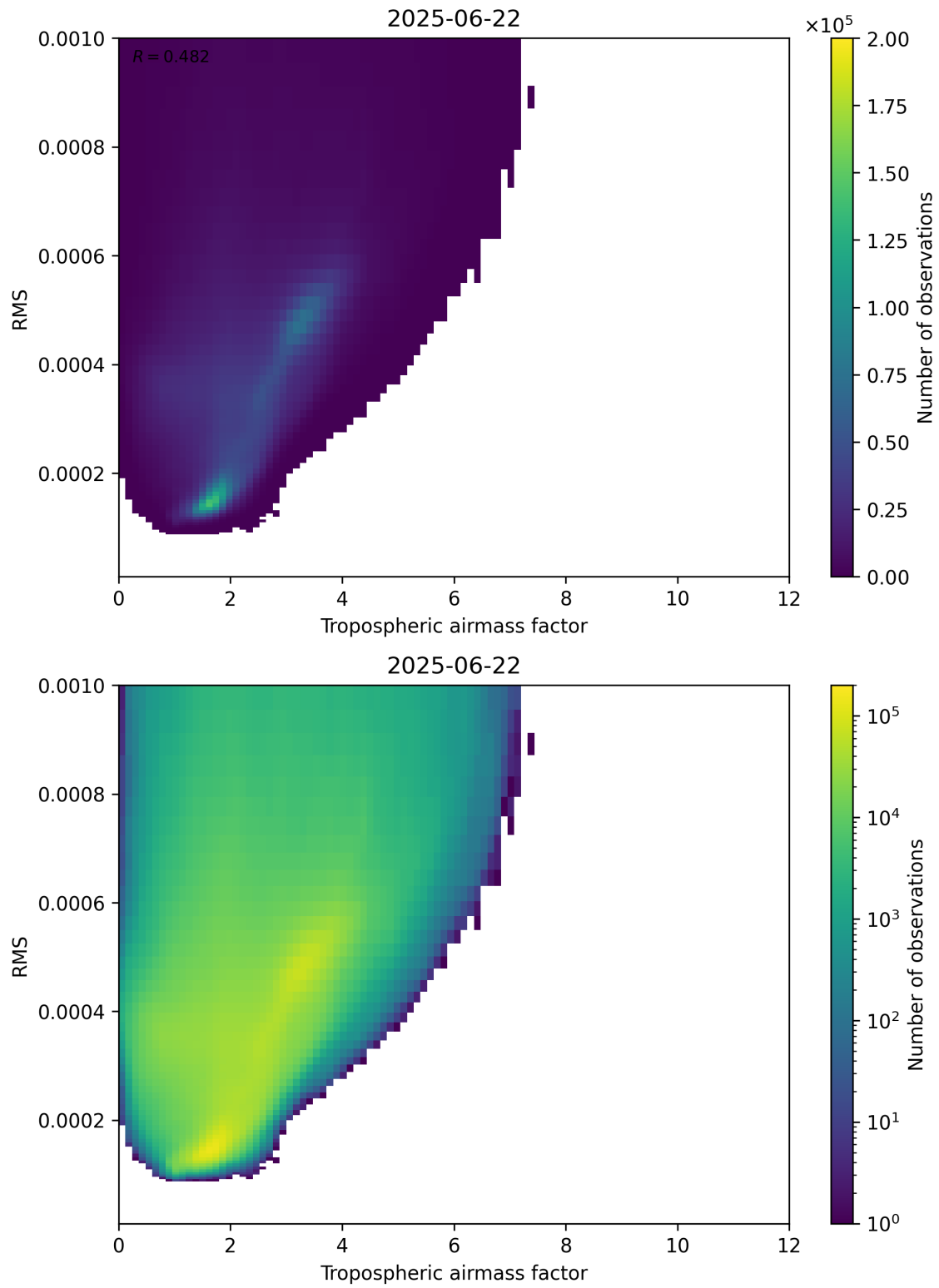
Figure 79: Scatter density plot of “Tropospheric airmass factor” against “RMS” for 2025-06-22 to 2025-06-23.
