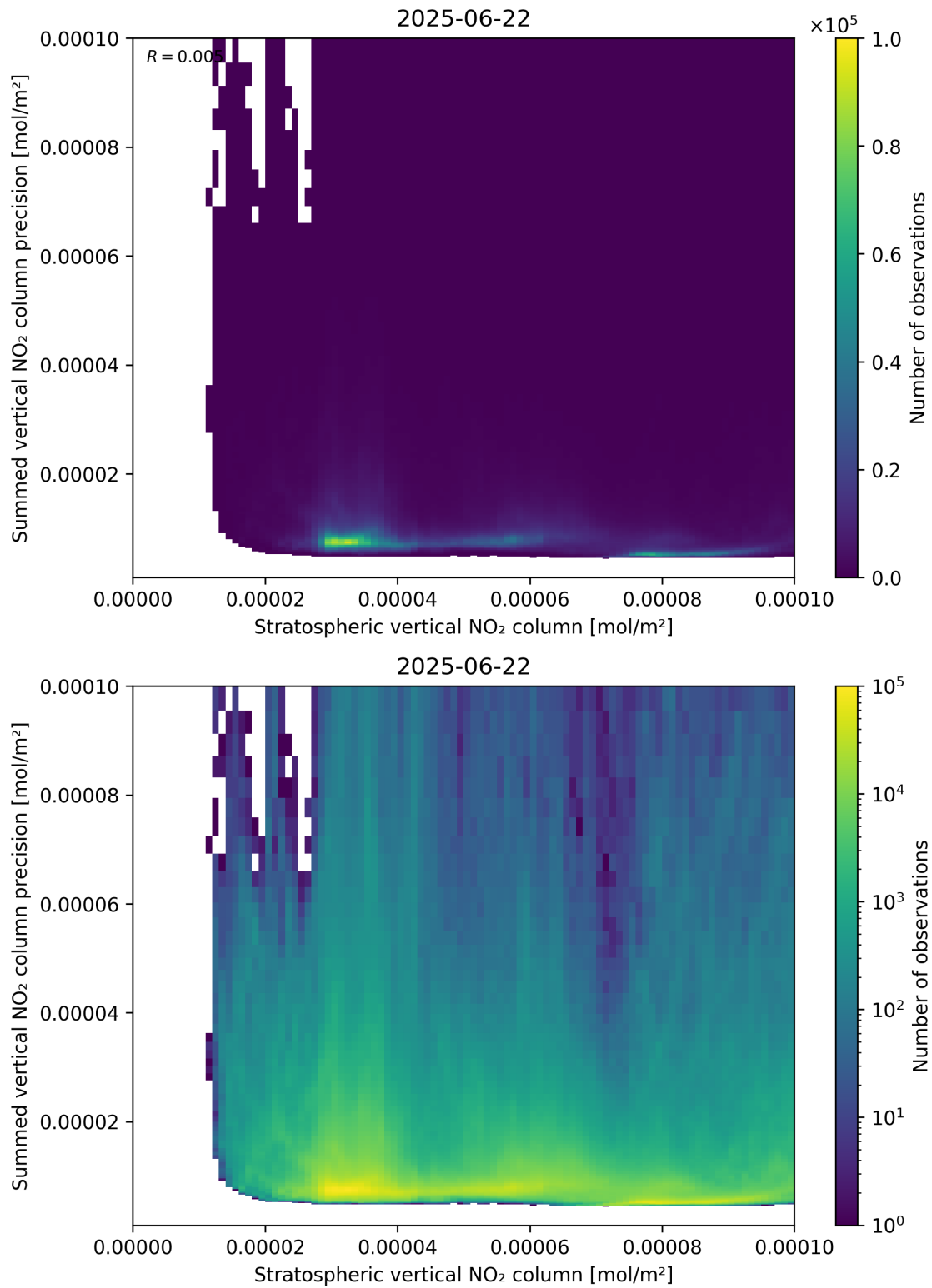
Figure 99: Scatter density plot of “Stratospheric vertical NO 2 column” against “Summed vertical NO 2 column precision” for 2025-06-22 to 2025-06-23.
