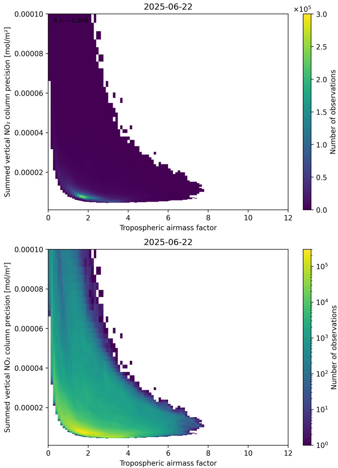
Figure 76: Scatter density plot of “Tropospheric air mass factor” against “Summed vertical NO 2 column precision” for 2025-06-22 to 2025-06-23.
