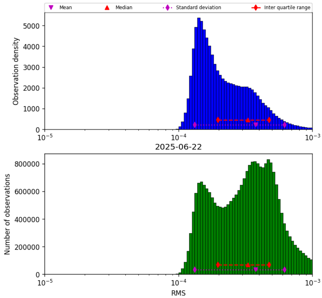
Figure 43: Histogram of “RMS” for 2025-06-22 to 2025-06-23
