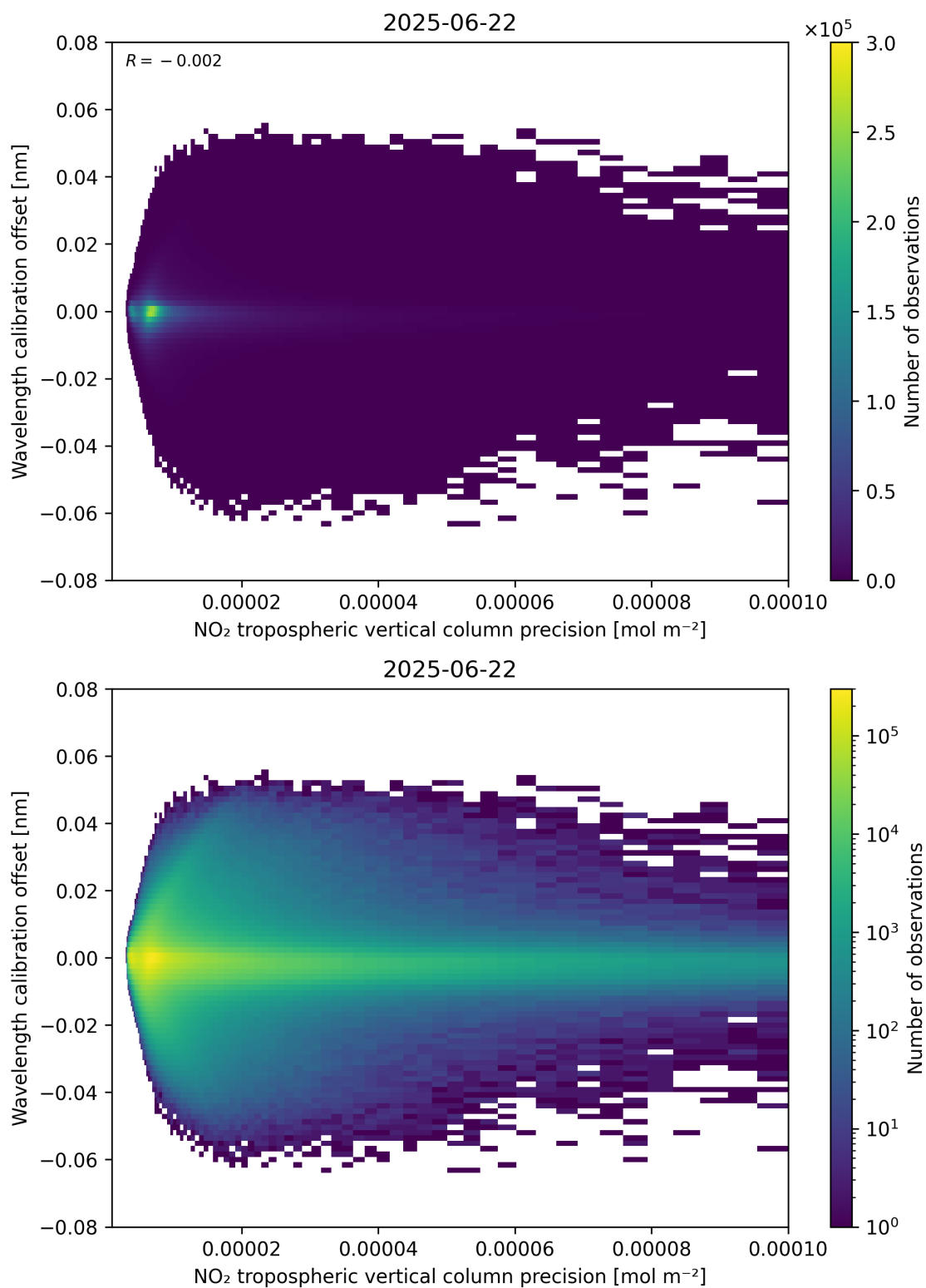
Figure 141: Scatter density plot of “NO 2 tropospheric vertical column precision” against “Wavelength calibration offset” for 2025-06-22 to 2025-06-23.
