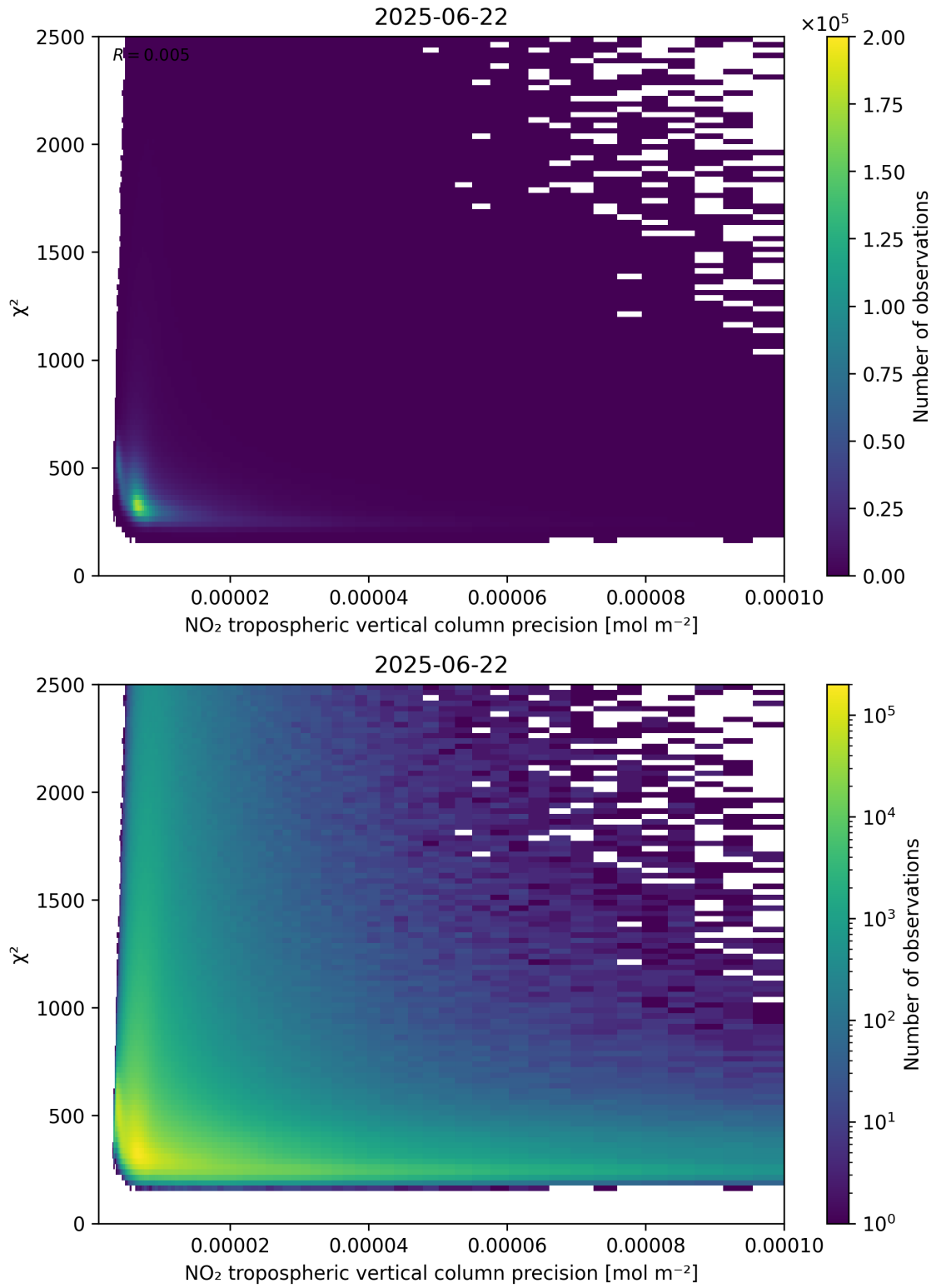
Figure 134: Scatter density plot of “NO 2 tropospheric vertical column precision” against “ \chi^2 ” for 2025-06-22 to 2025-06-23.
