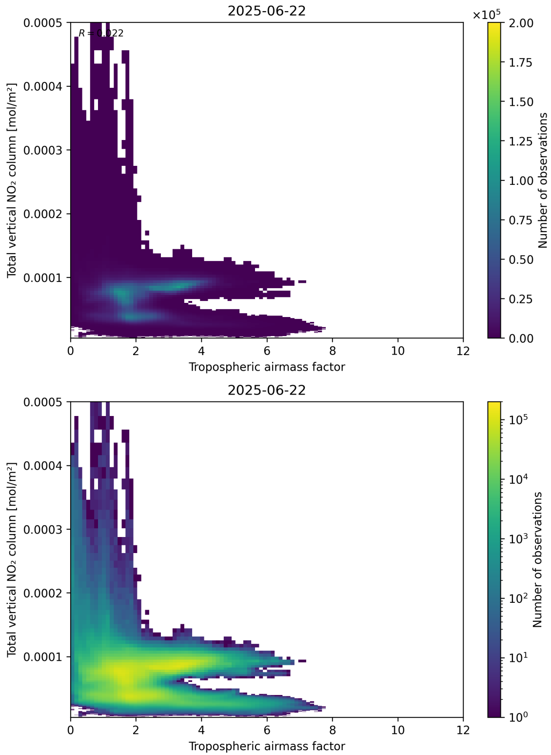
Figure 77: Scatter density plot of “Tropospheric airmass factor” against “Total vertical NO 2 column” for 2025-06-22 to 2025-06-23.
