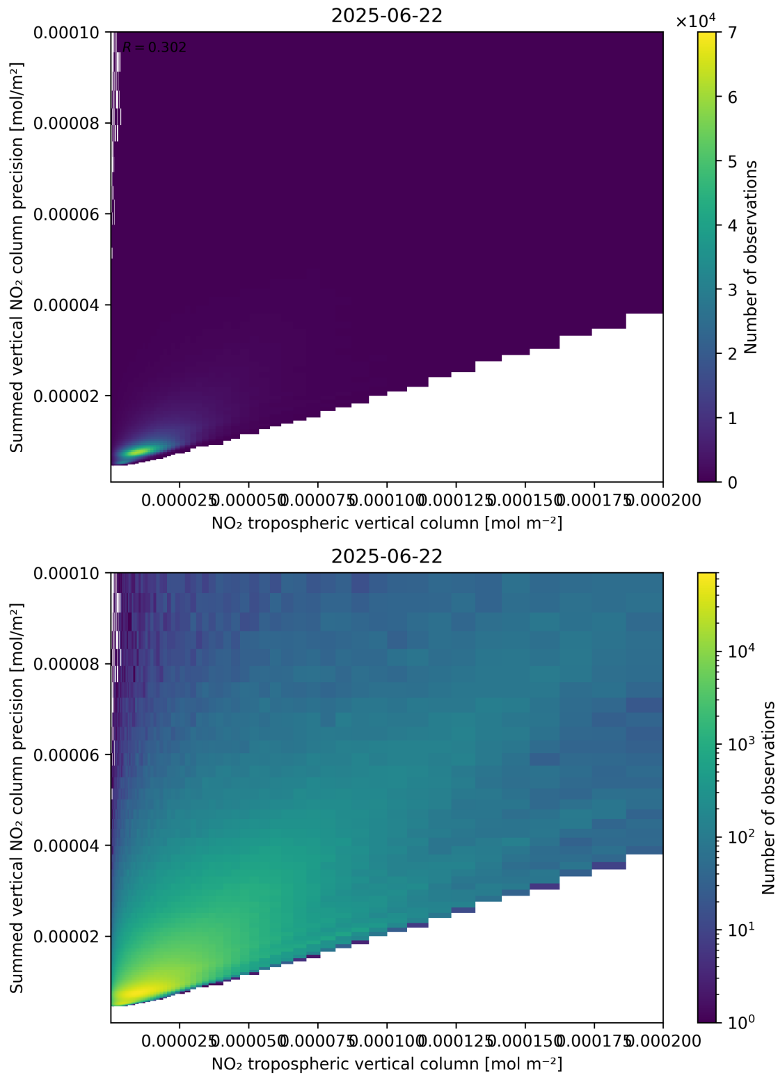
Figure 127: Scatter density plot of “NO 2 tropospheric vertical column” against “Summed vertical NO 2 column precision” for 2025-06-22 to 2025-06-23.
