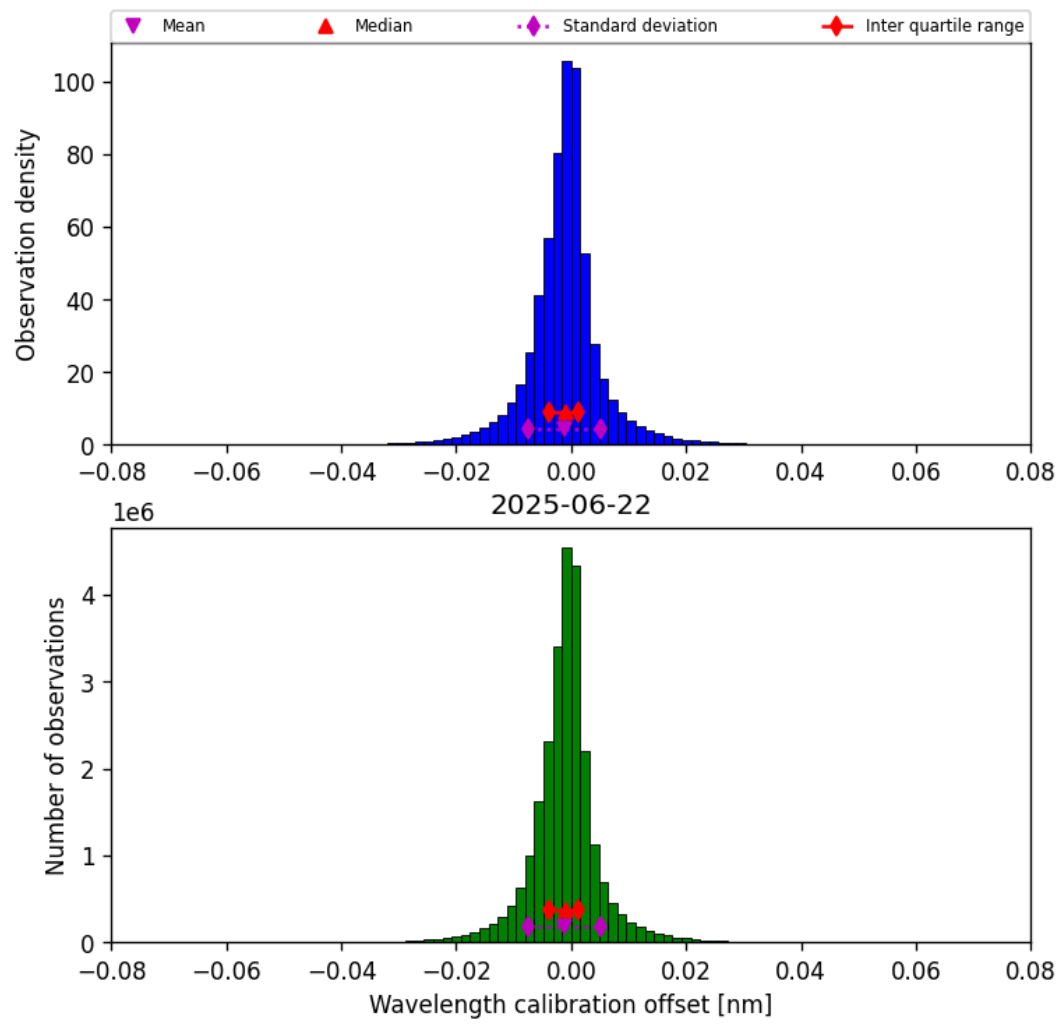
Figure 35: Histogram of “Wavelength calibration offset” for 2025-06-22 to 2025-06-23
