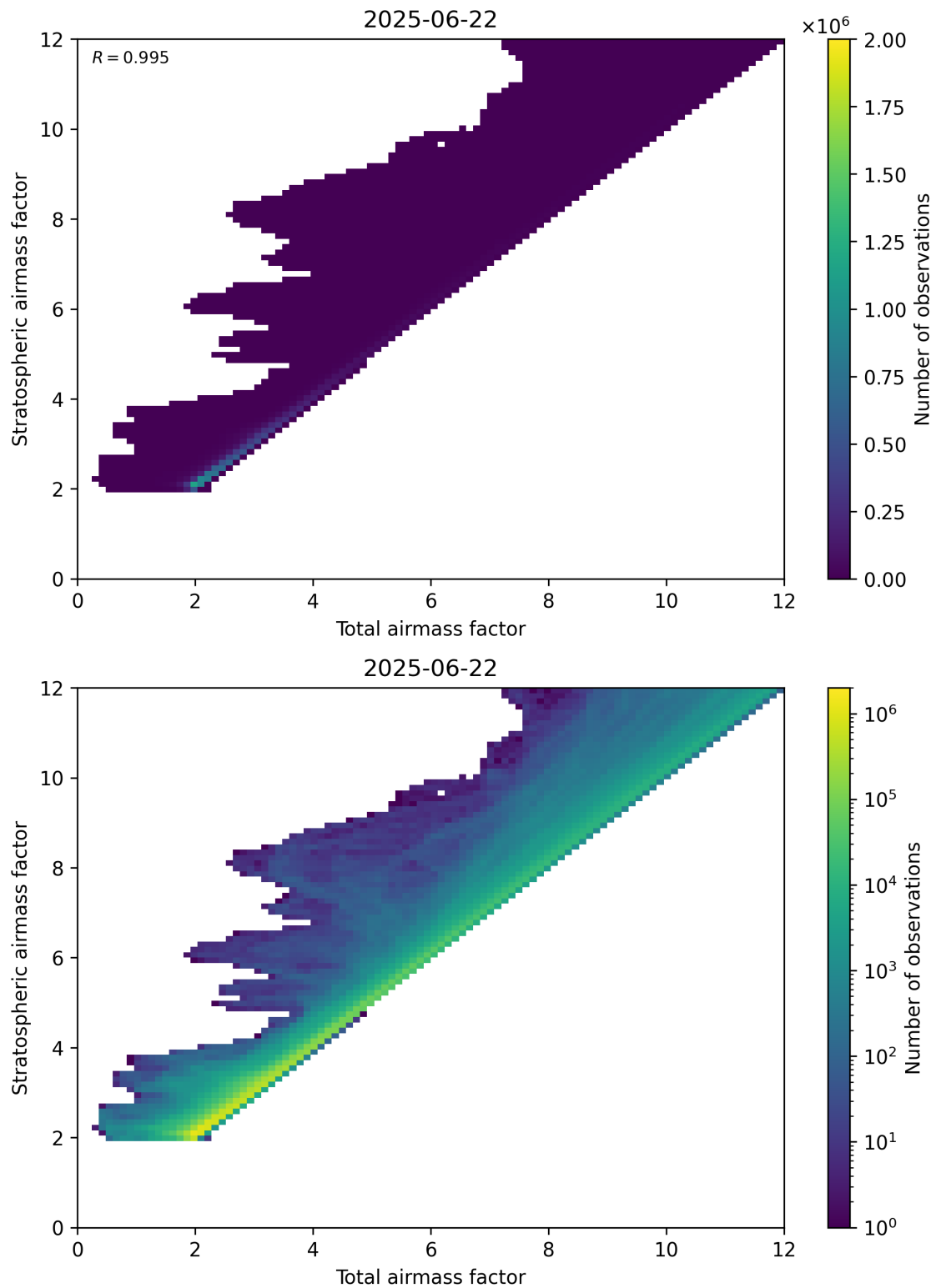
Figure 62: Scatter density plot of “Total air mass factor” against “Stratospheric air mass factor” for 2025-06-22 to 2025-06-23.
