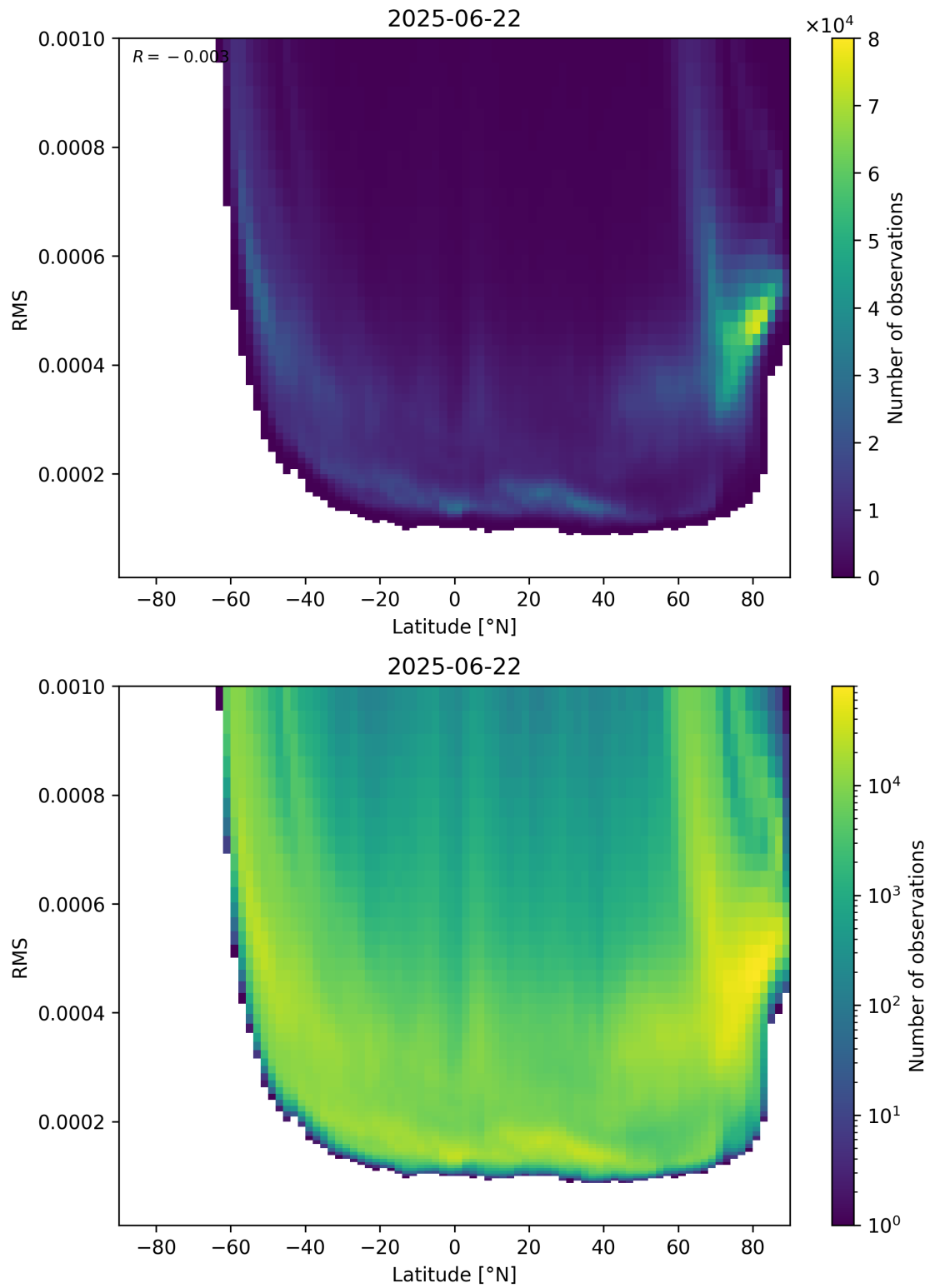
Figure 94: Scatter density plot of “Latitude” against “RMS” for 2025-06-22 to 2025-06-23.
