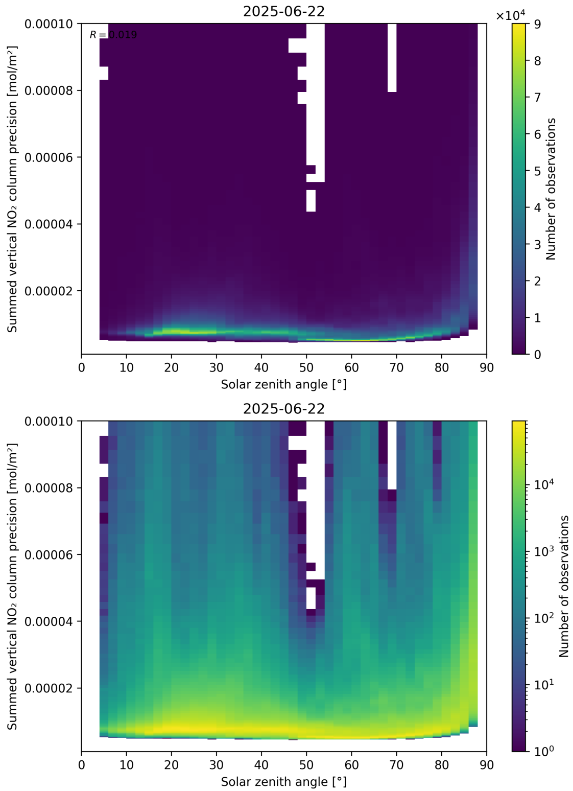
Figure 152: Scatter density plot of “Solar zenith angle” against “Summed vertical NO 2 column precision” for 2025-06-22 to 2025-06-23.
