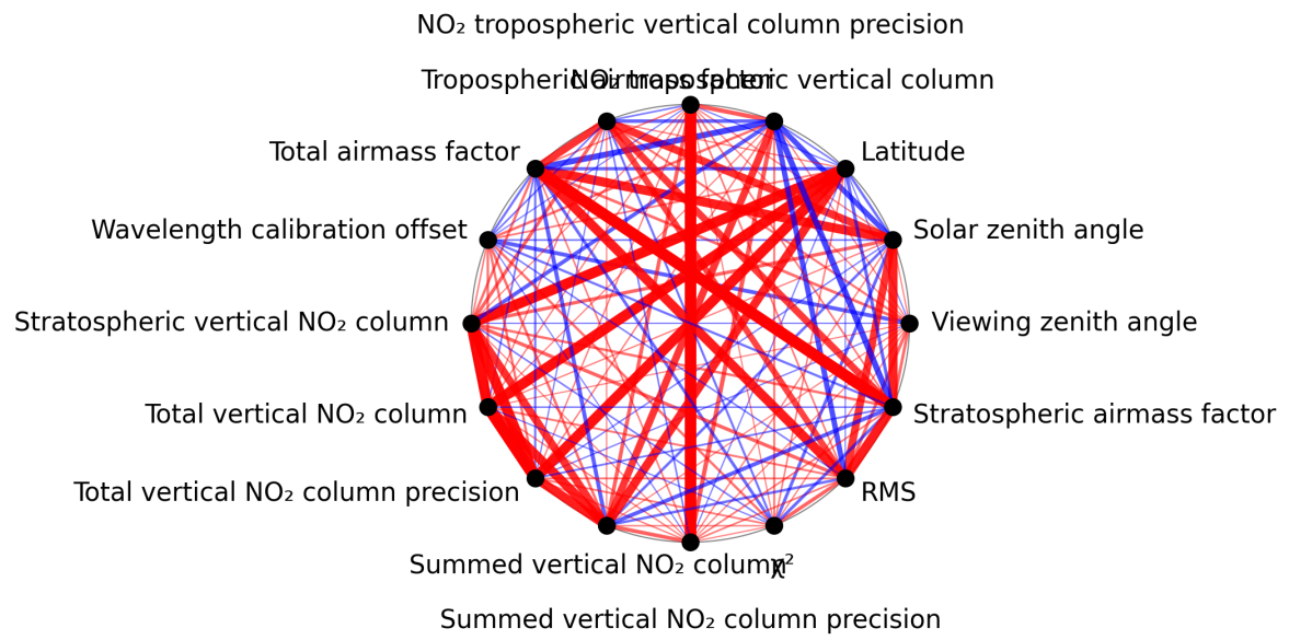
Figure 1: Map of correlation graph for 2025-06-22 to 2025-06-23.
