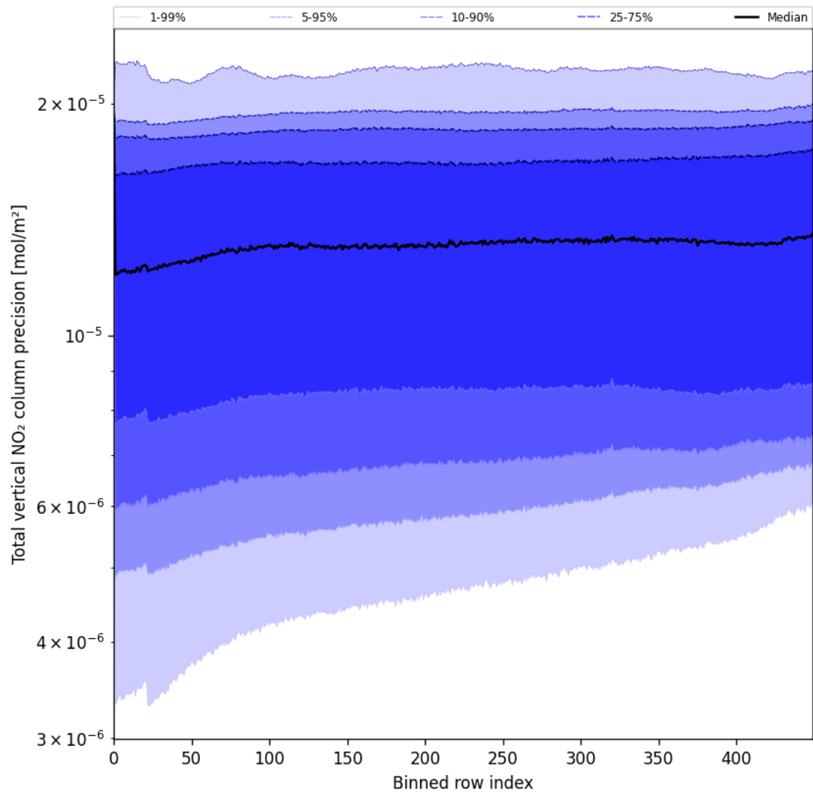
Figure 56: Along track statistics of “Total vertical NO 2 column precision” for 2025-06-22 to 2025-06-23
