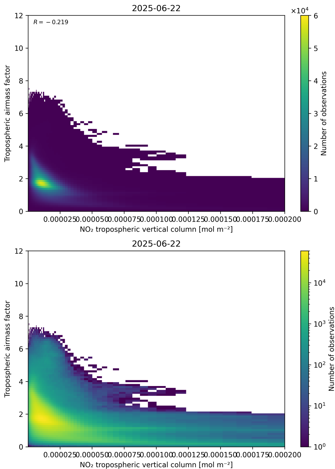
Figure 123: Scatter density plot of “NO 2 tropospheric vertical column” against “Tropospheric airmass factor” for 2025-06-22 to 2025-06-23.
