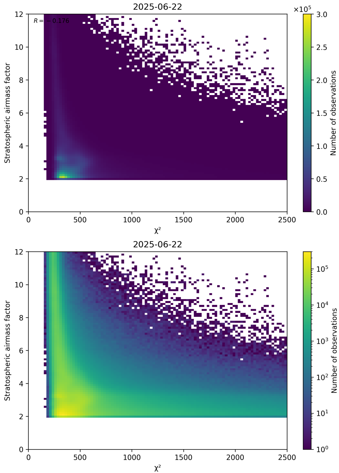
Figure 81: Scatter density plot of “ \chi^2 ” against “Stratospheric airmass factor” for 2025-06-22 to 2025-06-23.
