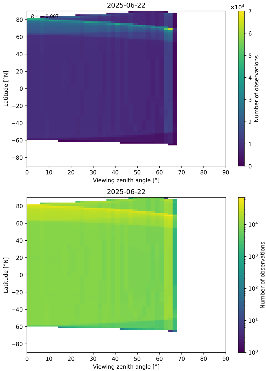
Figure 163: Scatter density plot of “Viewing zenith angle” against “Latitude” for 2025-06-22 to 2025-06-23.
