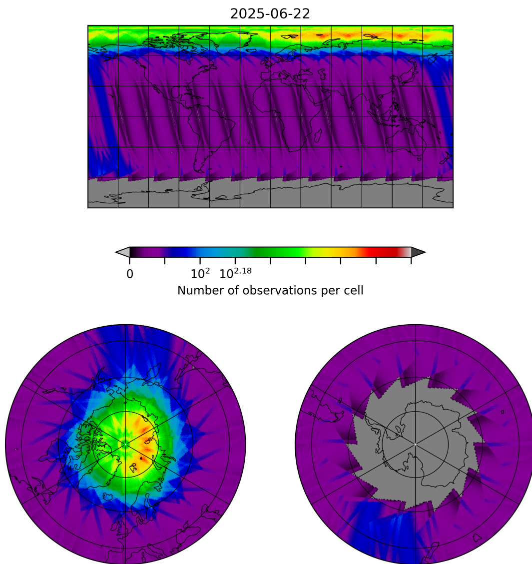
Figure 10: Map of the number of observations for 2025-06-22 to 2025-06-23
