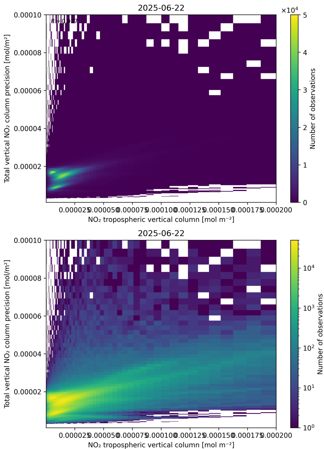
Figure 129: Scatter density plot of “NO 2 tropospheric vertical column” against “Total vertical NO 2 column precision” for 2025-06-22 to 2025-06-23.
