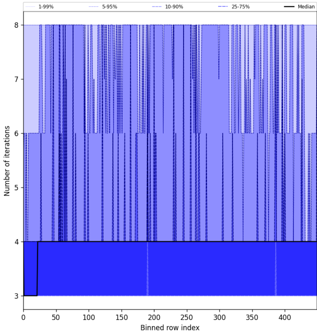
Figure 51: Along track statistics of “Number of iterations” for 2025-06-22 to 2025-06-23
