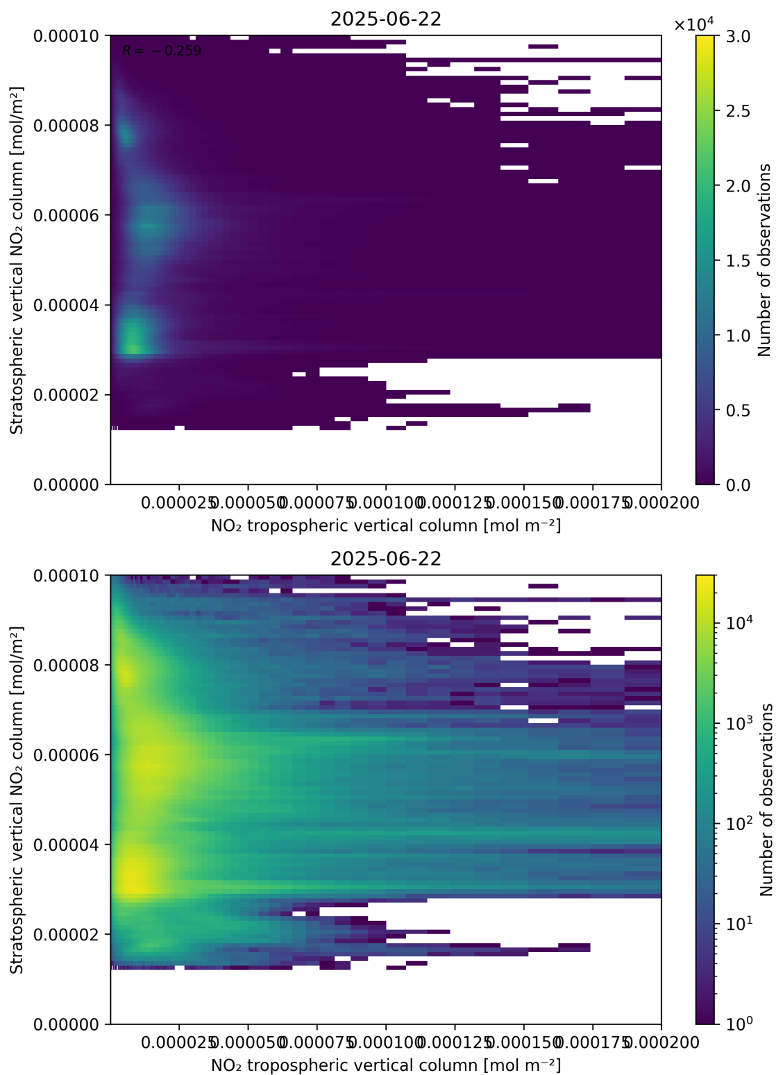
Figure 125: Scatter density plot of “NO 2 tropospheric vertical column” against “Stratospheric vertical NO 2 column” for 2025-06-22 to 2025-06-23.
