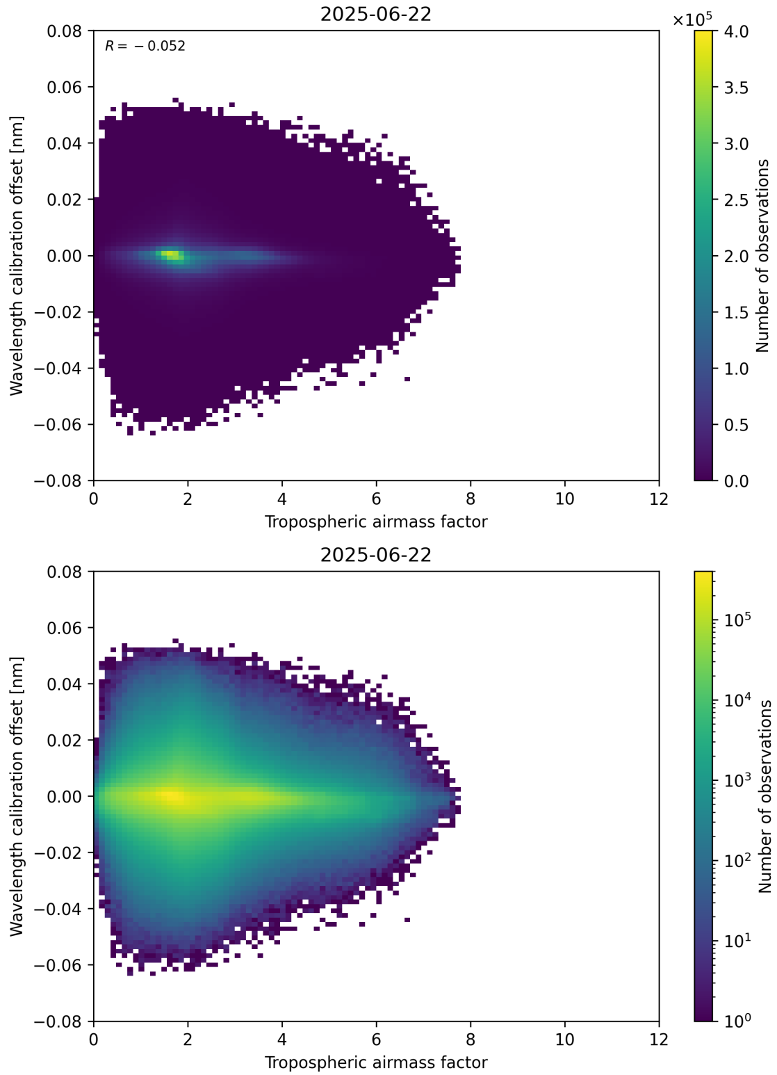
Figure 80: Scatter density plot of “Tropospheric airmass factor” against “Wavelength calibration offset” for 2025-06-22 to 2025-06-23.
