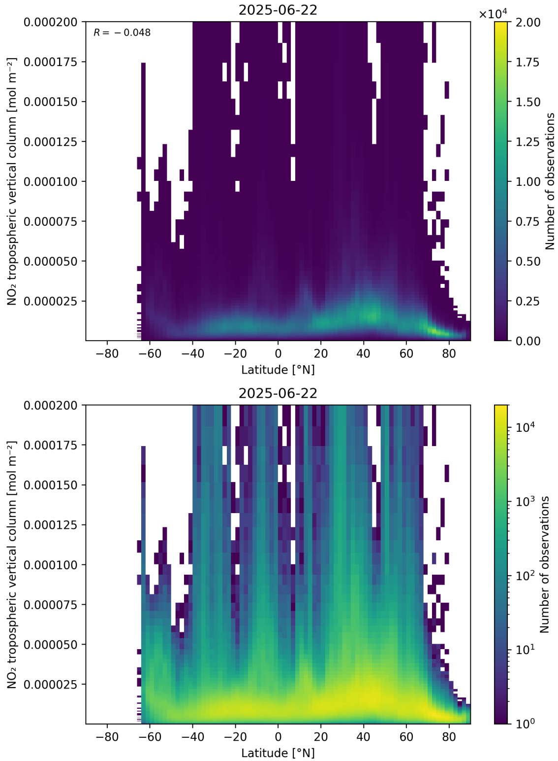
Figure 92: Scatter density plot of “Latitude” against “NO 2 tropospheric vertical column” for 2025-06-22 to 2025-06-23.
