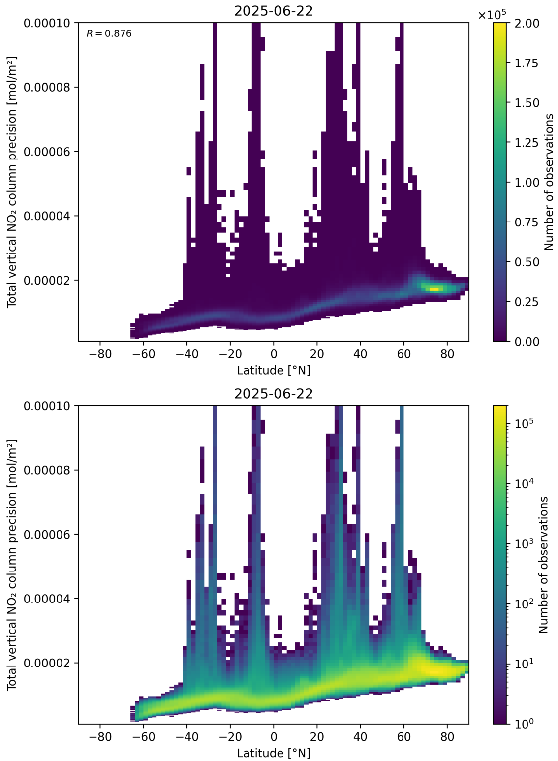
Figure 91: Scatter density plot of “Latitude” against “Total vertical NO 2 column precision” for 2025-06-22 to 2025-06-23.
