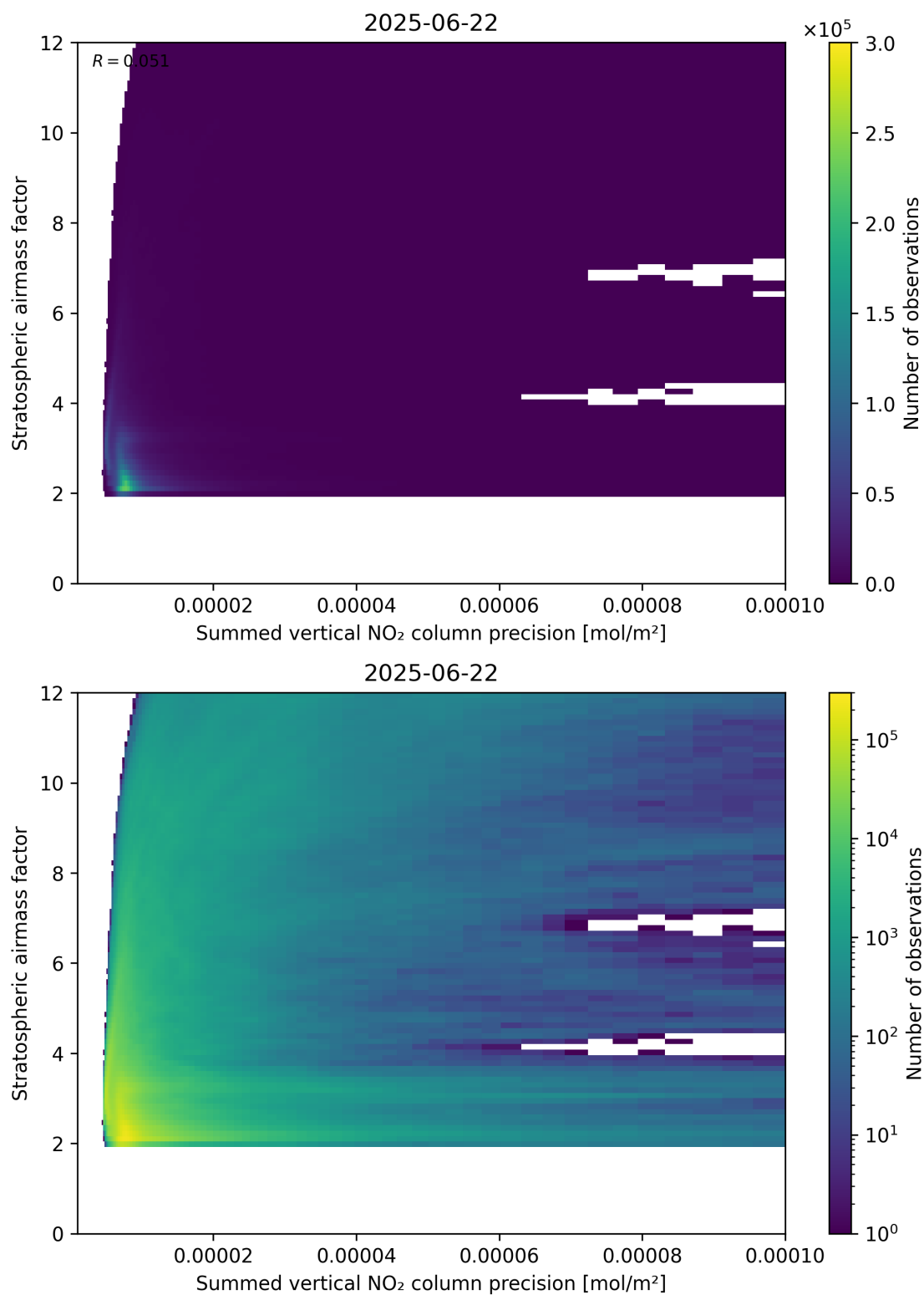
Figure 106: Scatter density plot of “Summed vertical NO 2 column precision” against “Stratospheric airmass factor” for 2025-06-22 to 2025-06-23.
