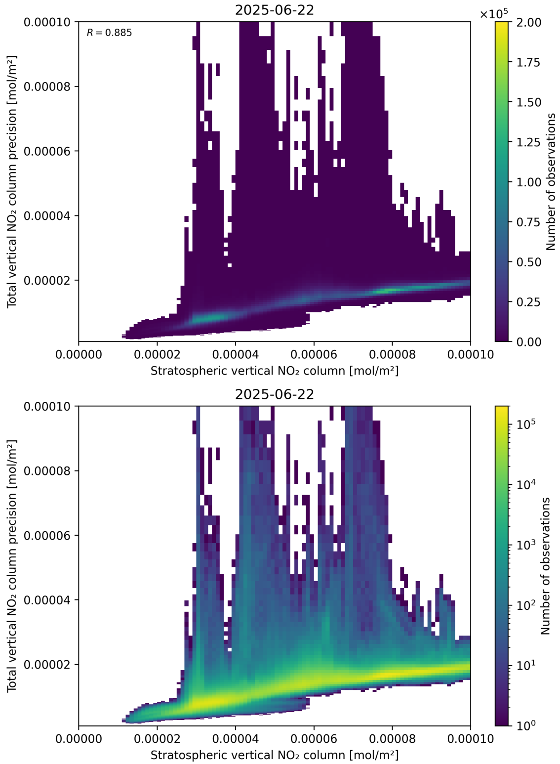
Figure 101: Scatter density plot of “Stratospheric vertical NO 2 column” against “Total vertical NO 2 column precision” for 2025-06-22 to 2025-06-23.
