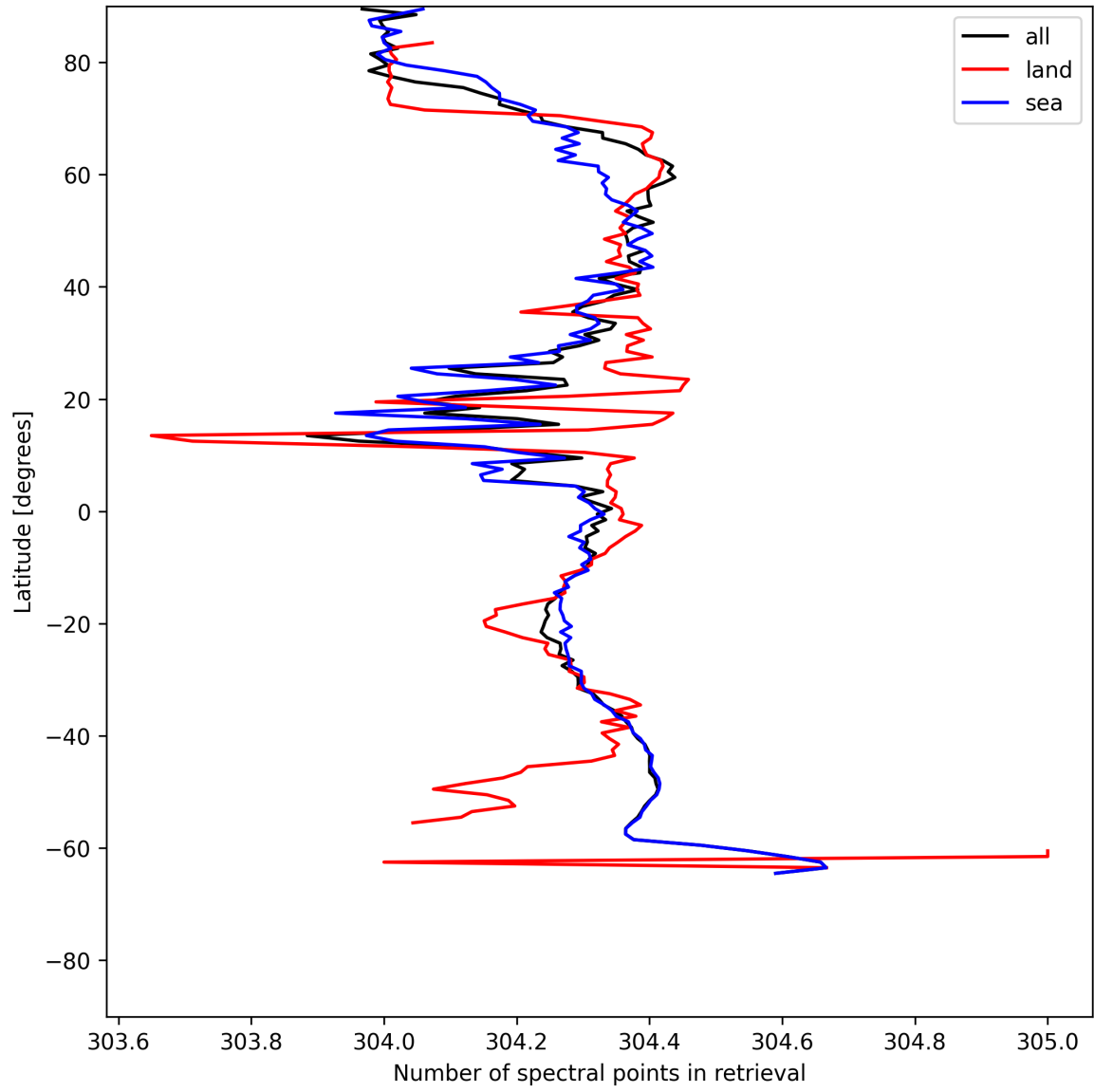
Figure 16: Zonal average of “Number of spectral points in retrieval” for 2025-06-22 to 2025-06-23.
