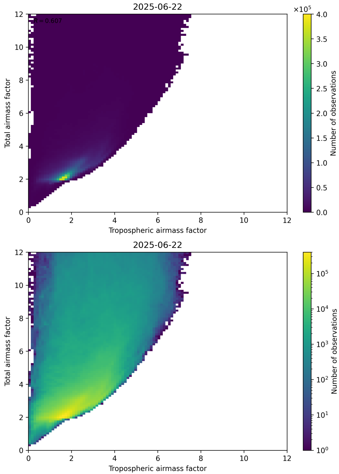
Figure 72: Scatter density plot of “Tropospheric airmass factor” against “Total airmass factor” for 2025-06-22 to 2025-06-23.
