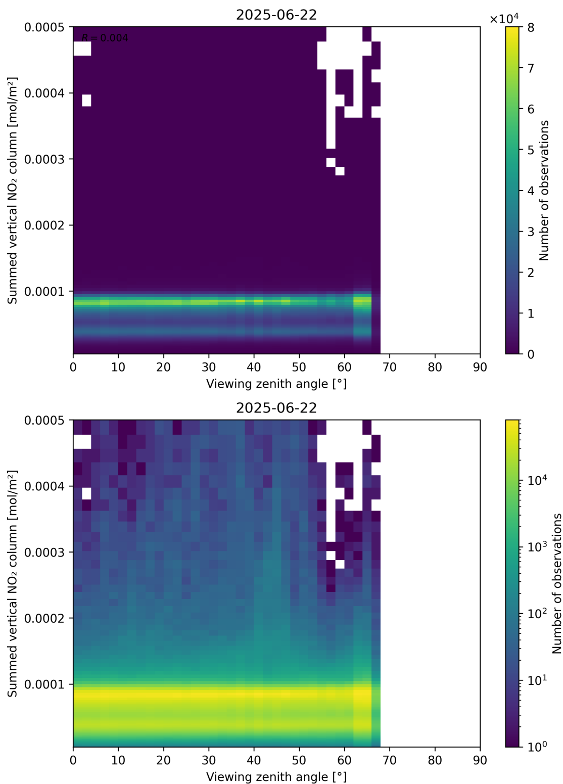
Figure 165: Scatter density plot of “Viewing zenith angle” against “Summed vertical NO 2 column” for 2025-06-22 to 2025-06-23.
