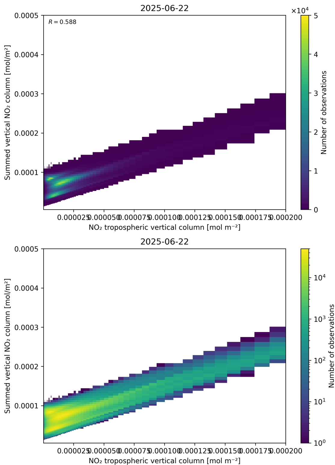
Figure 126: Scatter density plot of “NO 2 tropospheric vertical column” against “Summed vertical NO 2 column” for 2025-06-22 to 2025-06-23.
