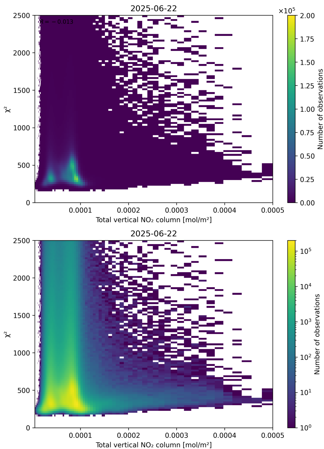
Figure 111: Scatter density plot of “Total vertical NO 2 column” against “ \chi^2 ” for 2025-06-22 to 2025-06-23.
