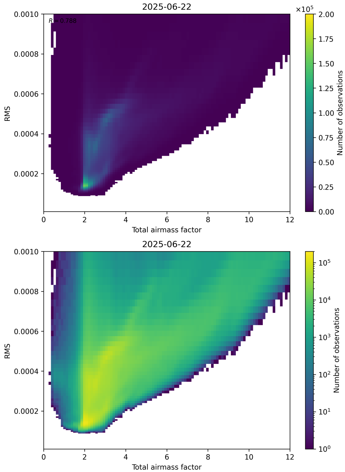
Figure 69: Scatter density plot of “Total airmass factor” against “RMS” for 2025-06-22 to 2025-06-23.
