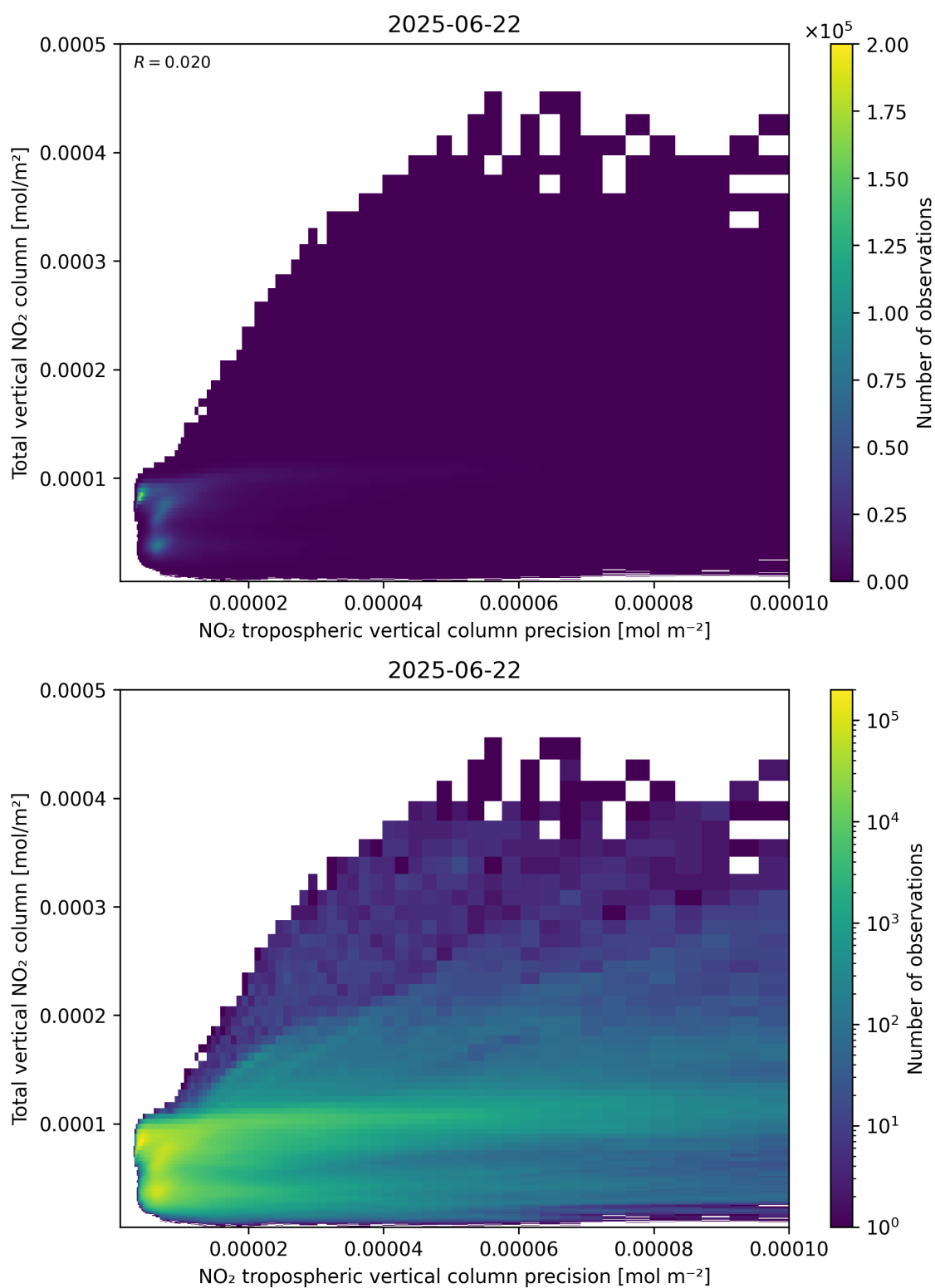
Figure 138: Scatter density plot of “NO 2 tropospheric vertical column precision” against “Total vertical NO 2 column” for 2025-06-22 to 2025-06-23.
