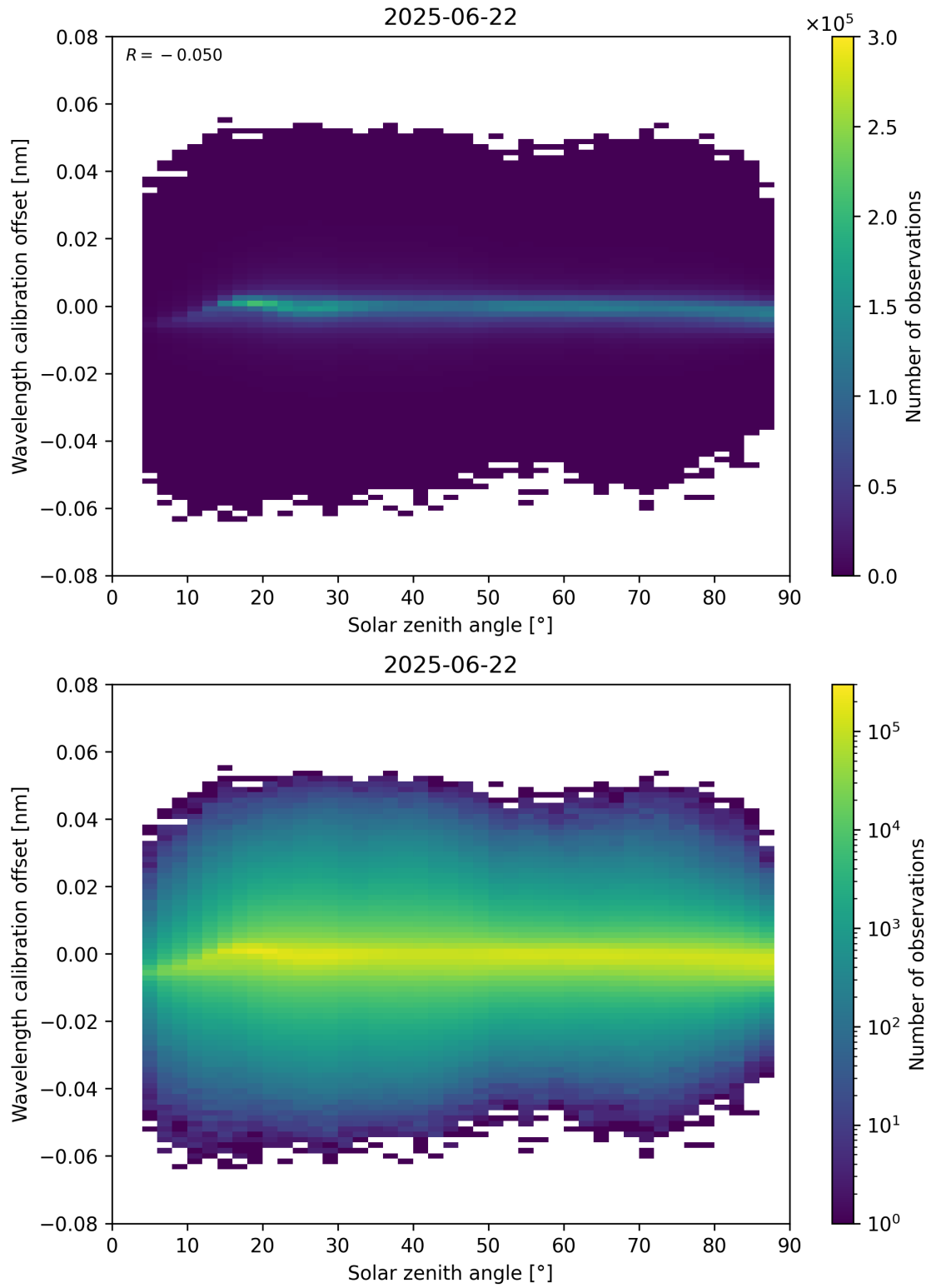
Figure 158: Scatter density plot of “Solar zenith angle” against “Wavelength calibration offset” for 2025-06-22 to 2025-06-23.
