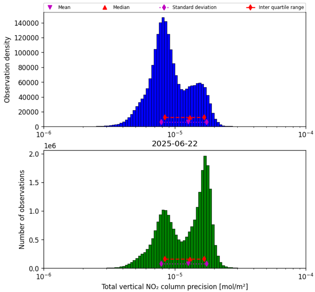
Figure 39: Histogram of “Total vertical NO 2 column precision” for 2025-06-22 to 2025-06-23
