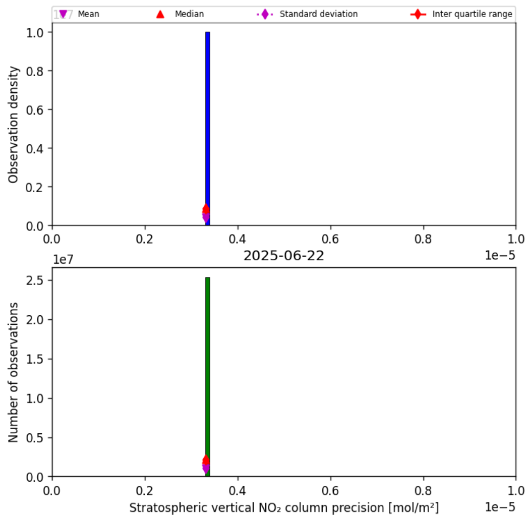
Figure 37: Histogram of “Stratospheric vertical NO 2 column precision” for 2025-06-22 to 2025-06-23
