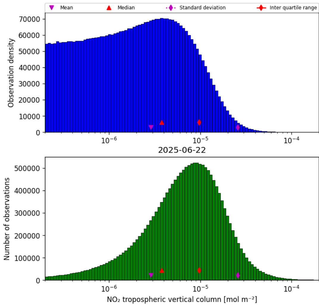
Figure 29: Histogram of “NO 2 tropospheric vertical column” for 2025-06-22 to 2025-06-23
