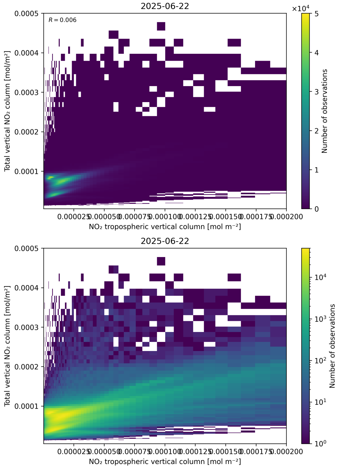
Figure 128: Scatter density plot of “NO 2 tropospheric vertical column” against “Total vertical NO 2 column” for 2025-06-22 to 2025-06-23.
