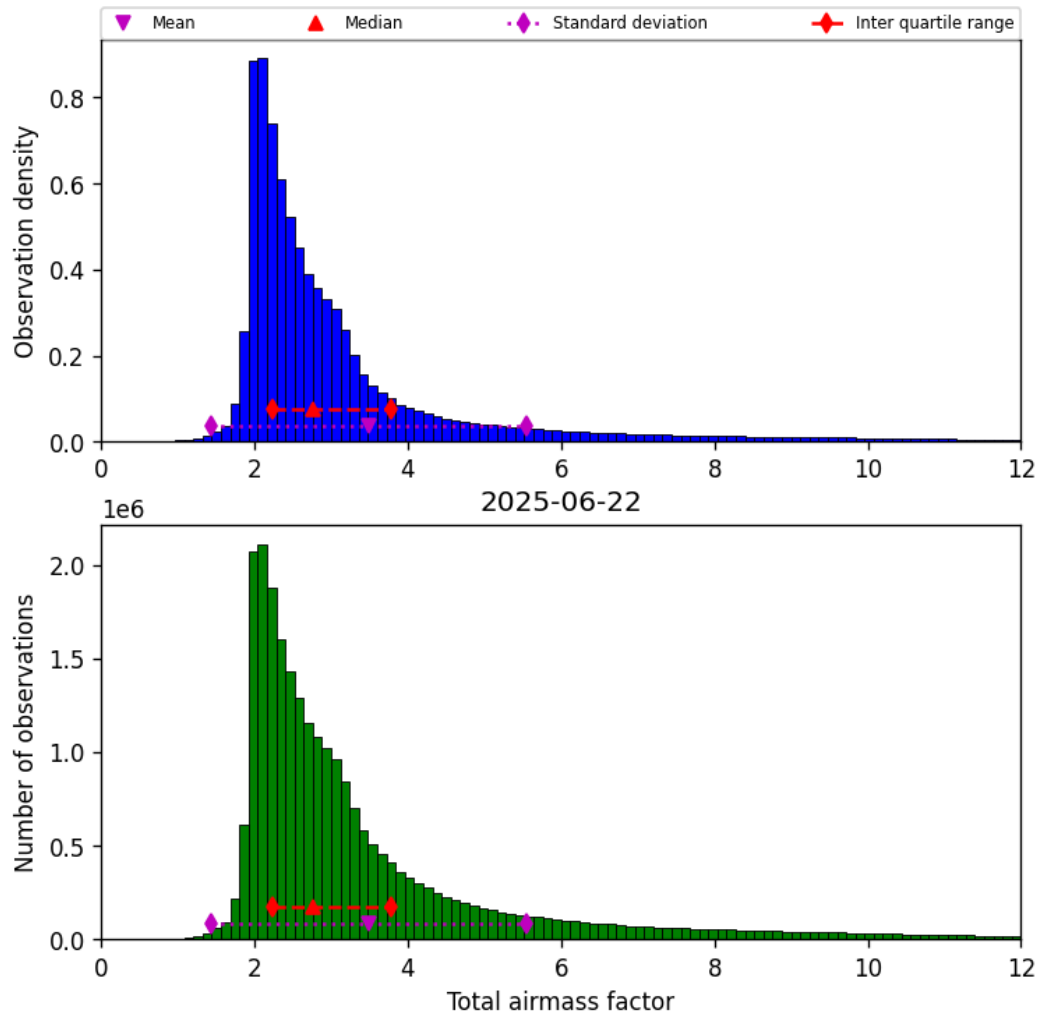
Figure 32: Histogram of “Total airmass factor” for 2025-06-22 to 2025-06-23
