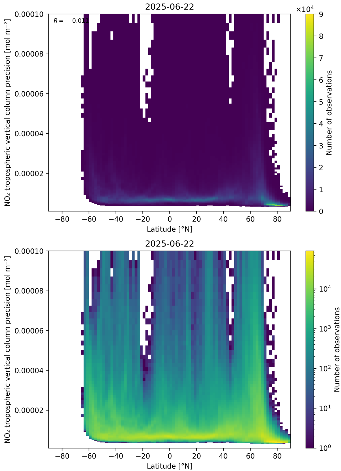
Figure 93: Scatter density plot of “Latitude” against “NO 2 tropospheric vertical column precision” for 2025-06-22 to 2025-06-23.
