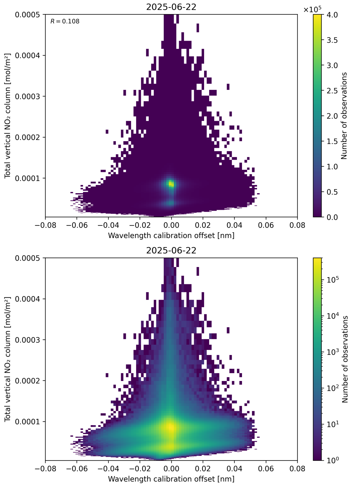
Figure 179: Scatter density plot of “Wavelength calibration offset” against “Total vertical NO 2 column” for 2025-06-22 to 2025-06-23.
