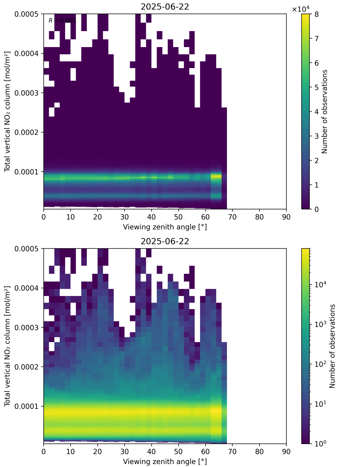
Figure 167: Scatter density plot of “Viewing zenith angle” against “Total vertical NO 2 column” for 2025-06-22 to 2025-06-23.
