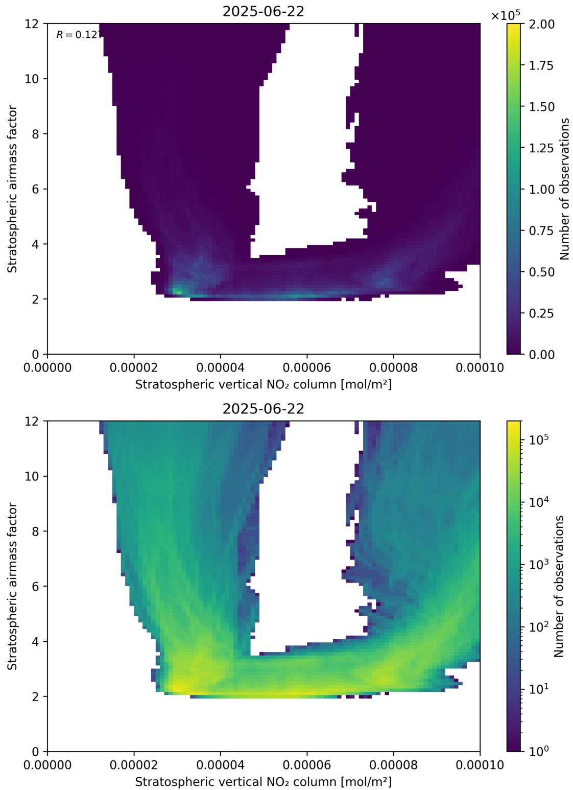
Figure 96: Scatter density plot of “Stratospheric vertical NO 2 column” against “Stratospheric airmass factor” for 2025-06-22 to 2025-06-23.
