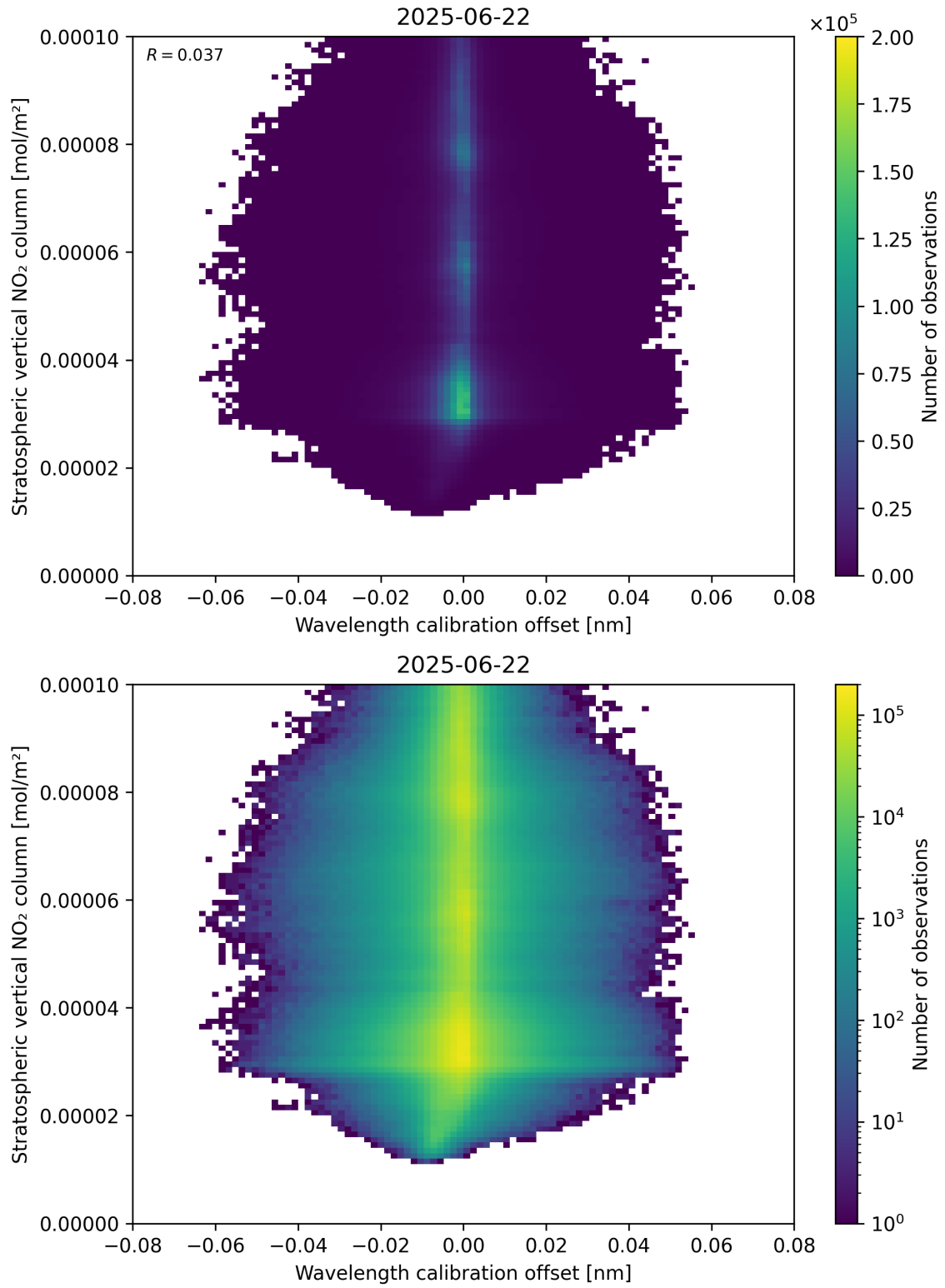
Figure 176: Scatter density plot of “Wavelength calibration offset” against “Stratospheric vertical NO 2 column” for 2025-06-22 to 2025-06-23.
