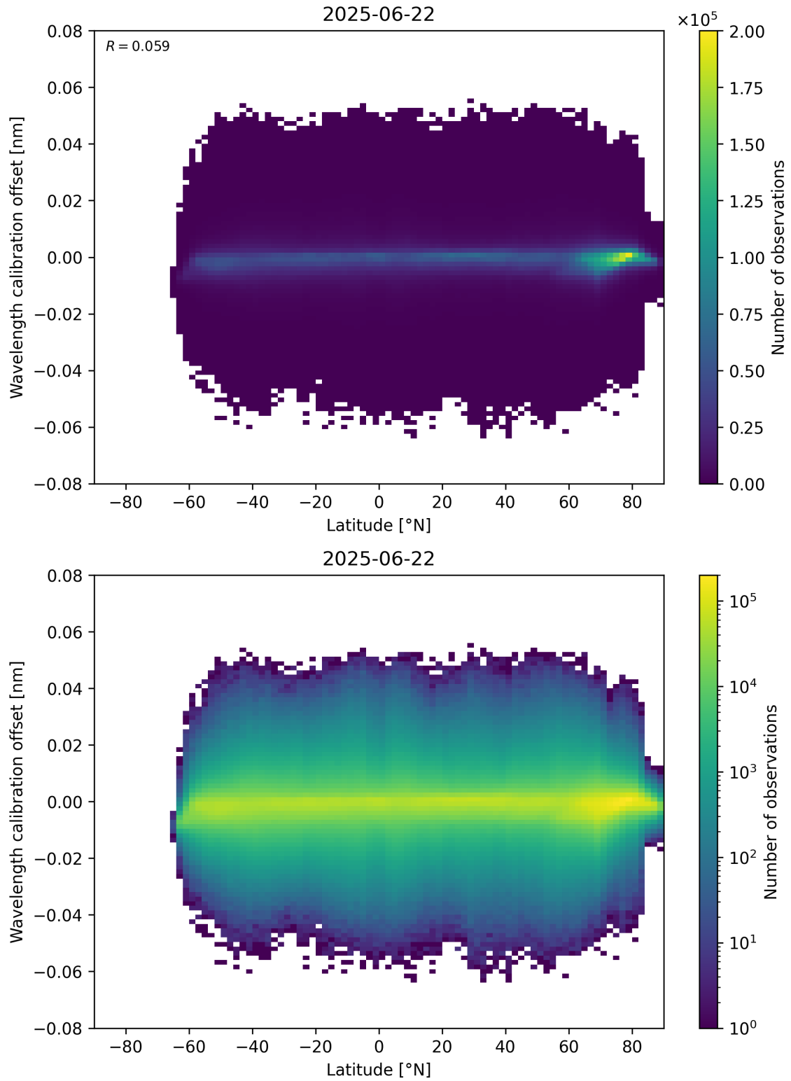
Figure 95: Scatter density plot of “Latitude” against “Wavelength calibration offset” for 2025-06-22 to 2025-06-23.
