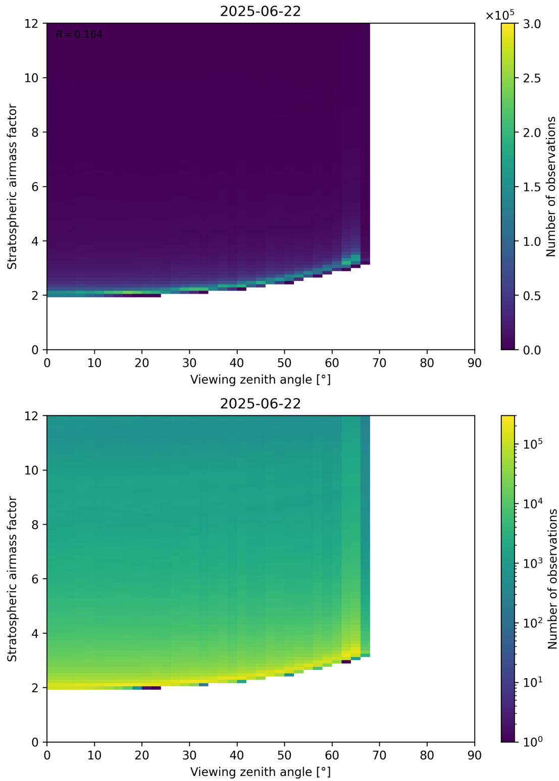
Figure 159: Scatter density plot of “Viewing zenith angle” against “Stratospheric airmass factor” for 2025-06-22 to 2025-06-23.
