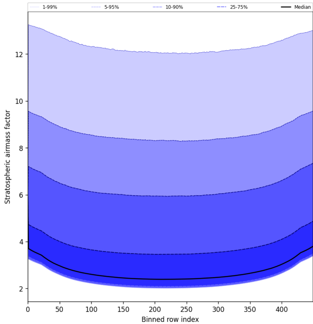
Figure 61: Along track statistics of “Stratospheric airmass factor” for 2025-06-22 to 2025-06-23
