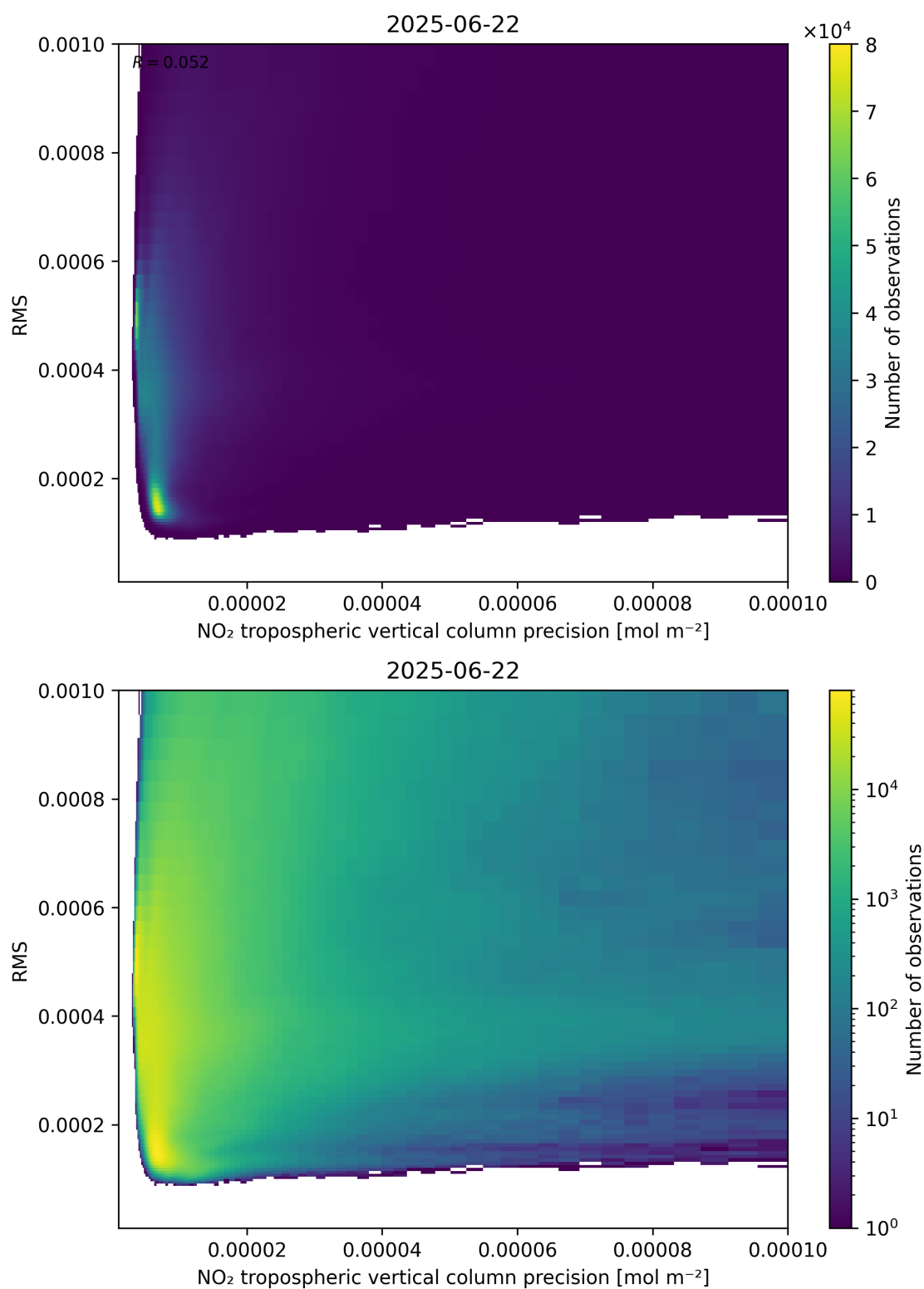
Figure 140: Scatter density plot of “NO 2 tropospheric vertical column precision” against “RMS” for 2025-06-22 to 2025-06-23.
