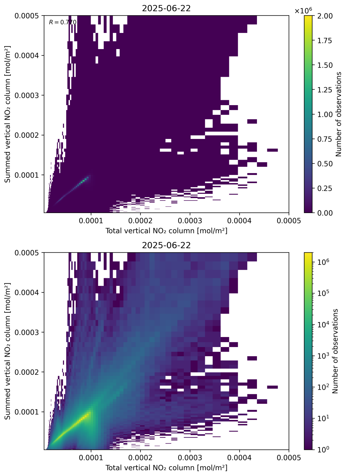
Figure 112: Scatter density plot of “Total vertical NO 2 column” against “Summed vertical NO 2 column” for 2025-06-22 to 2025-06-23.
