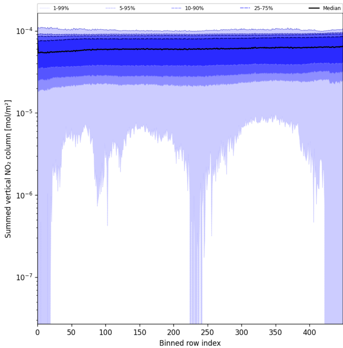
Figure 57: Along track statistics of “Summed vertical NO 2 column” for 2025-06-22 to 2025-06-23
