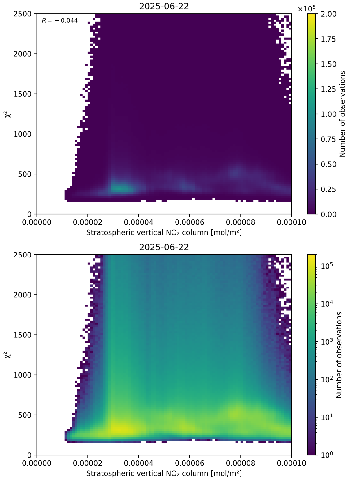
Figure 97: Scatter density plot of “Stratospheric vertical NO 2 column” against “ \chi^2 ” for 2025-06-22 to 2025-06-23.
