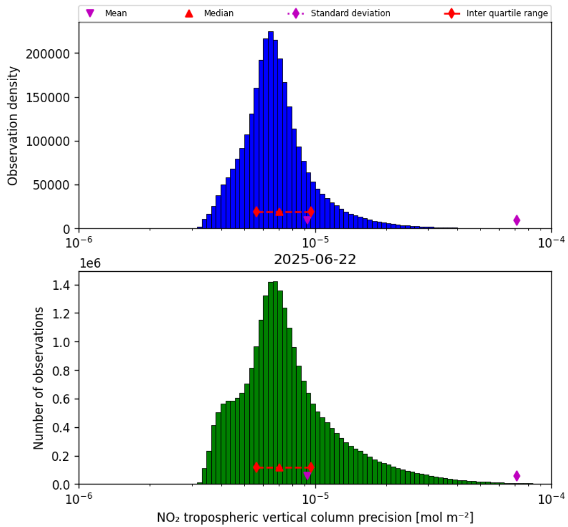
Figure 30: Histogram of “NO 2 tropospheric vertical column precision” for 2025-06-22 to 2025-06-23
