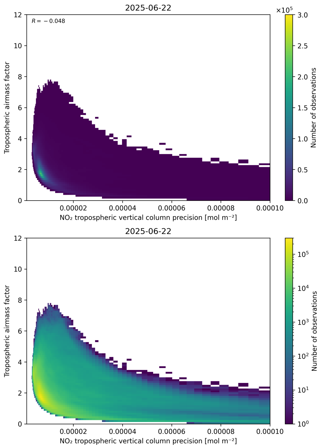
Figure 133: Scatter density plot of “NO 2 tropospheric vertical column precision” against “Tropospheric airmass factor” for 2025-06-22 to 2025-06-23.
