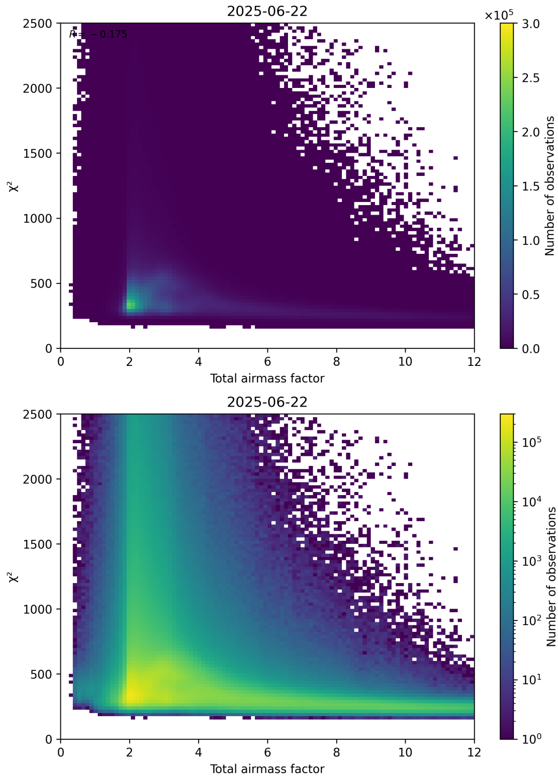
Figure 63: Scatter density plot of “Total airmass factor” against “ \chi^2 ” for 2025-06-22 to 2025-06-23.
