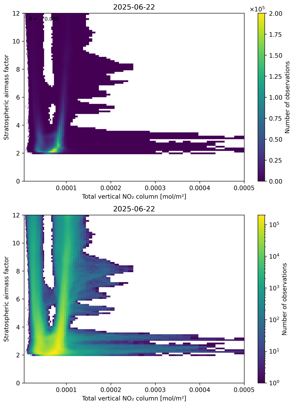
Figure 110: Scatter density plot of “Total vertical NO 2 column” against “Stratospheric airmass factor” for 2025-06-22 to 2025-06-23.
