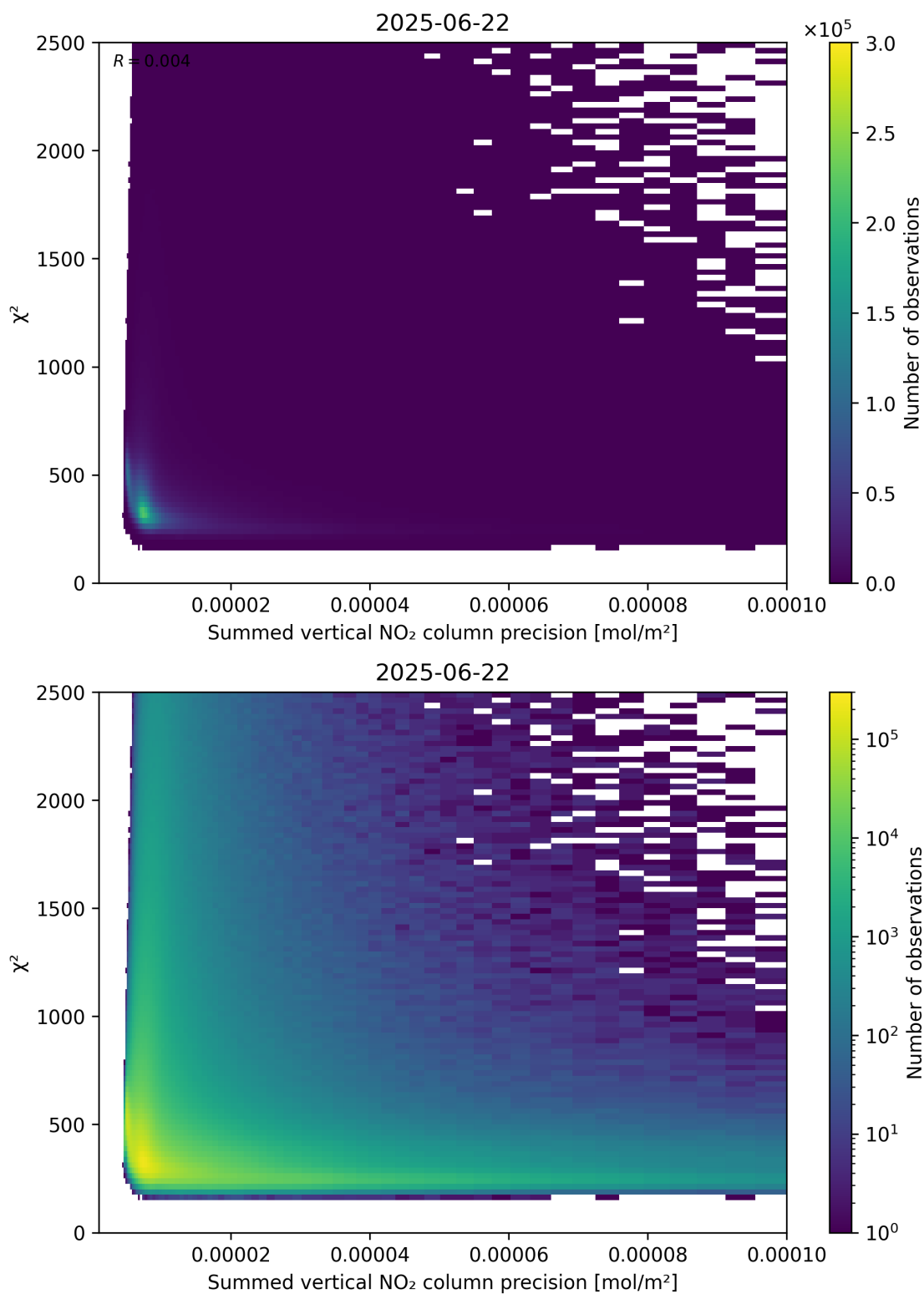
Figure 107: Scatter density plot of “Summed vertical NO 2 column precision” against “ \chi^2 ” for 2025-06-22 to 2025-06-23.
