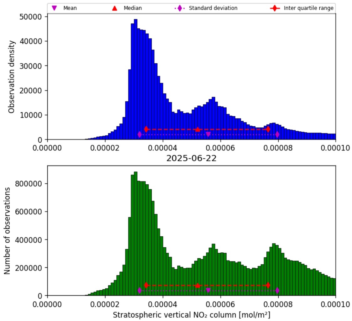
Figure 36: Histogram of “Stratospheric vertical NO 2 column” for 2025-06-22 to 2025-06-23
