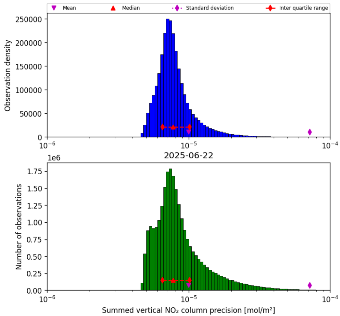
Figure 41: Histogram of "Summed vertical NO 2 column precision" for 2025-06-22 to 2025-06-23
