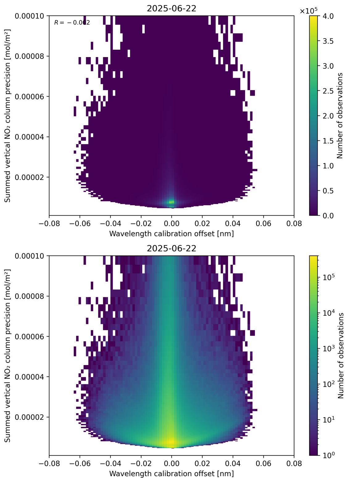
Figure 178: Scatter density plot of “Wavelength calibration offset” against “Summed vertical NO 2 column precision” for 2025-06-22 to 2025-06-23.
