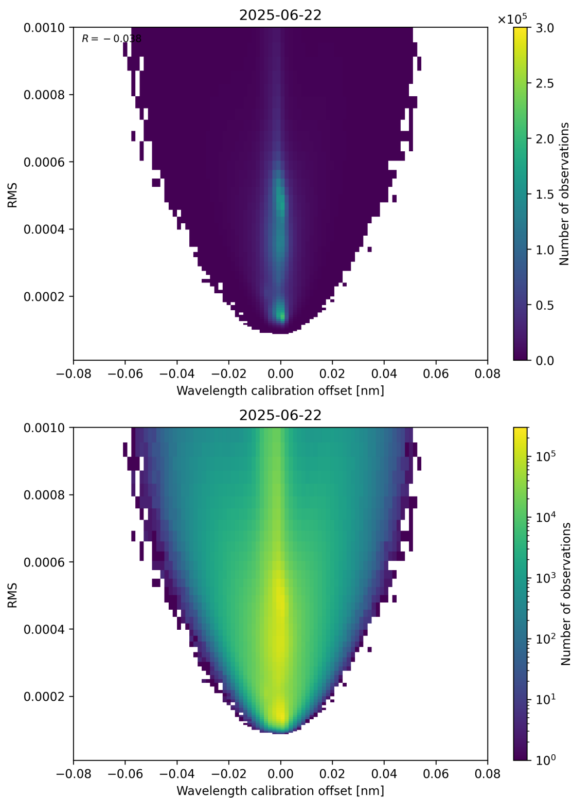
Figure 181: Scatter density plot of “Wavelength calibration offset” against “RMS” for 2025-06-22 to 2025-06-23.
