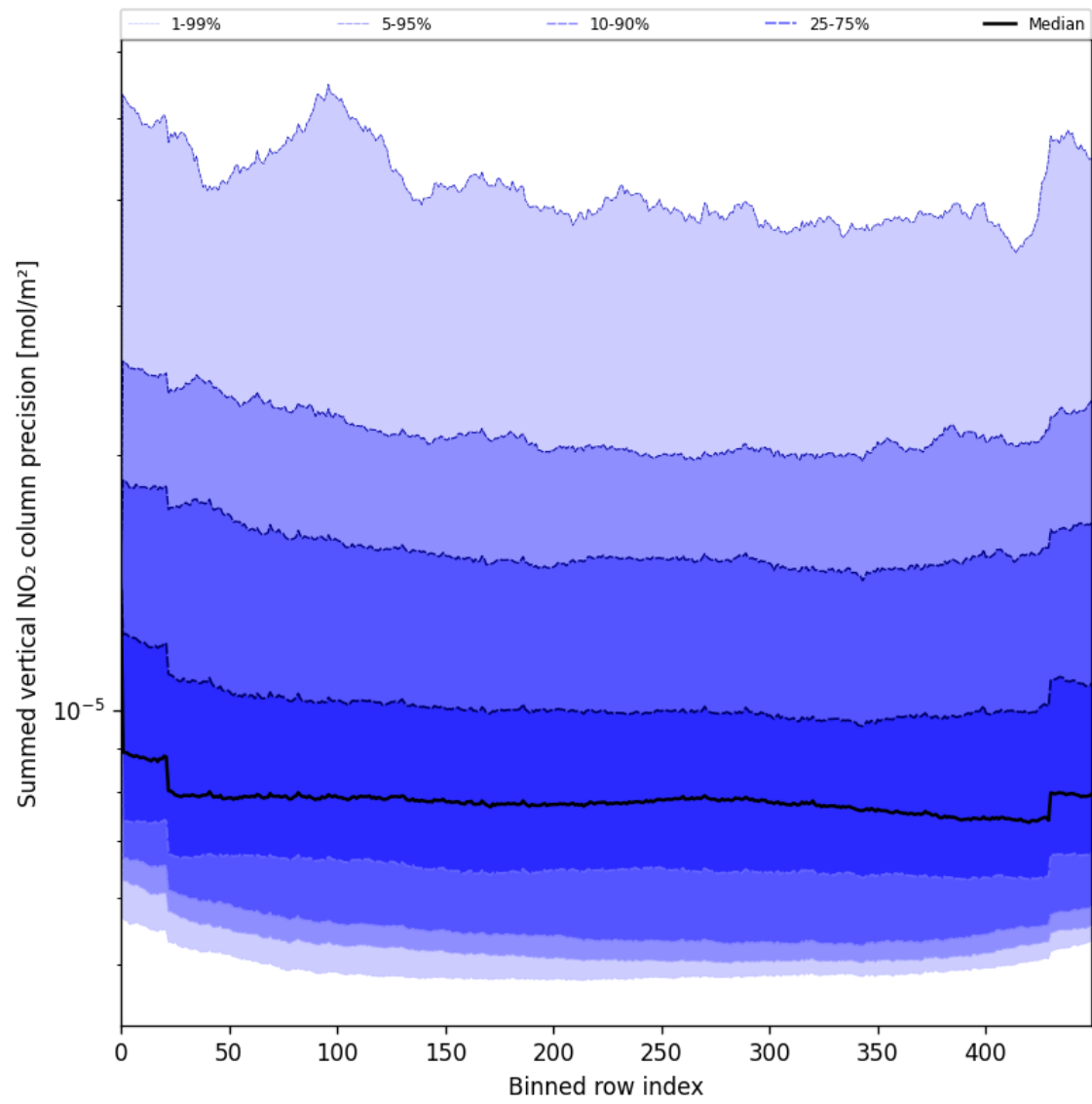
Figure 58: Along track statistics of “Summed vertical NO 2 column precision” for 2025-06-22 to 2025-06-23
