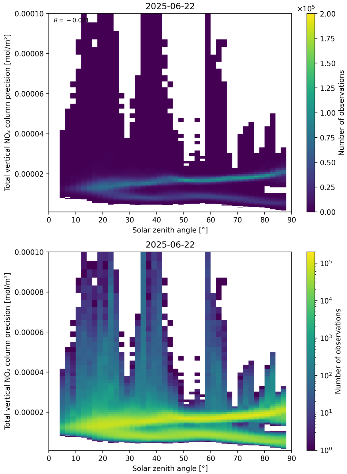
Figure 154: Scatter density plot of “Solar zenith angle” against “Total vertical NO 2 column precision” for 2025-06-22 to 2025-06-23.
