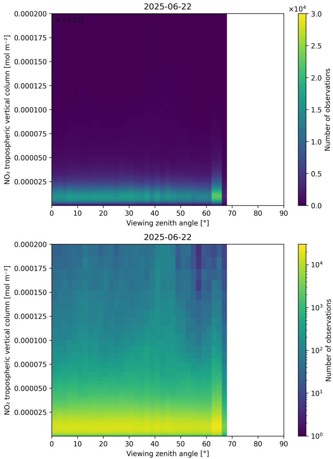
Figure 169: Scatter density plot of “Viewing zenith angle” against “NO 2 tropospheric vertical column” for 2025-06-22 to 2025-06-23.
