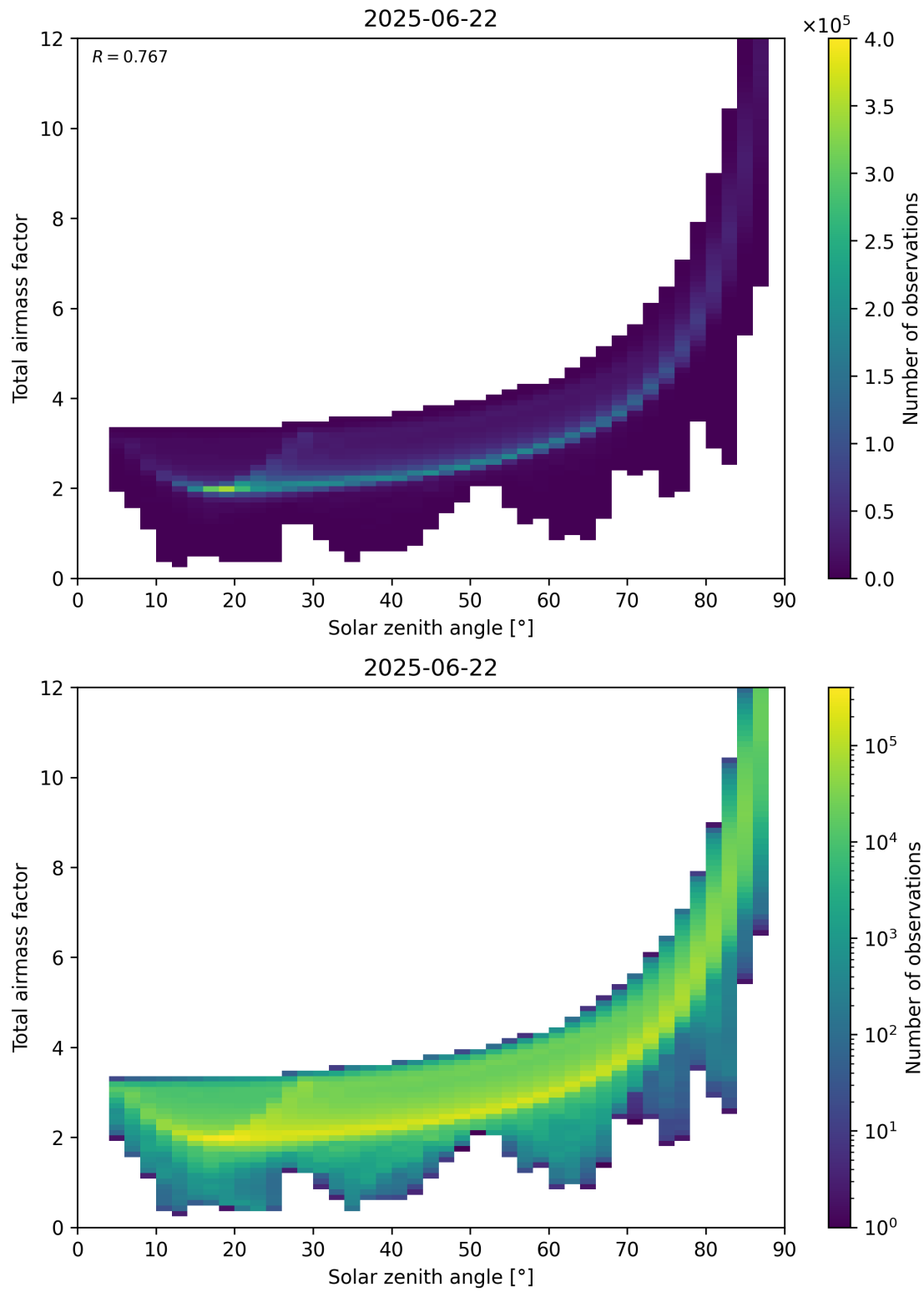
Figure 146: Scatter density plot of “Solar zenith angle” against “Total air mass factor” for 2025-06-22 to 2025-06-23.
