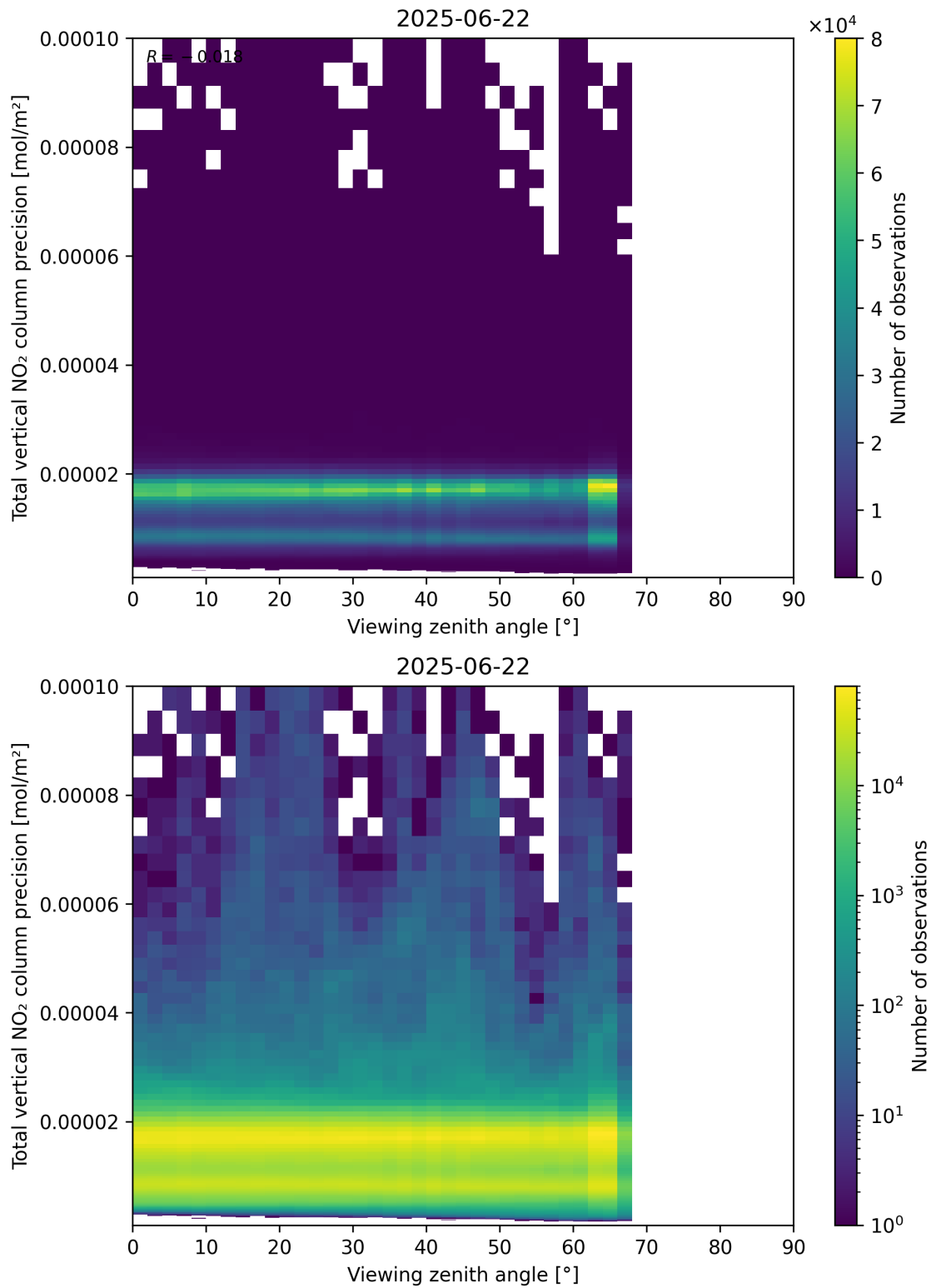
Figure 168: Scatter density plot of “Viewing zenith angle” against “Total vertical NO 2 column precision” for 2025-06-22 to 2025-06-23.
