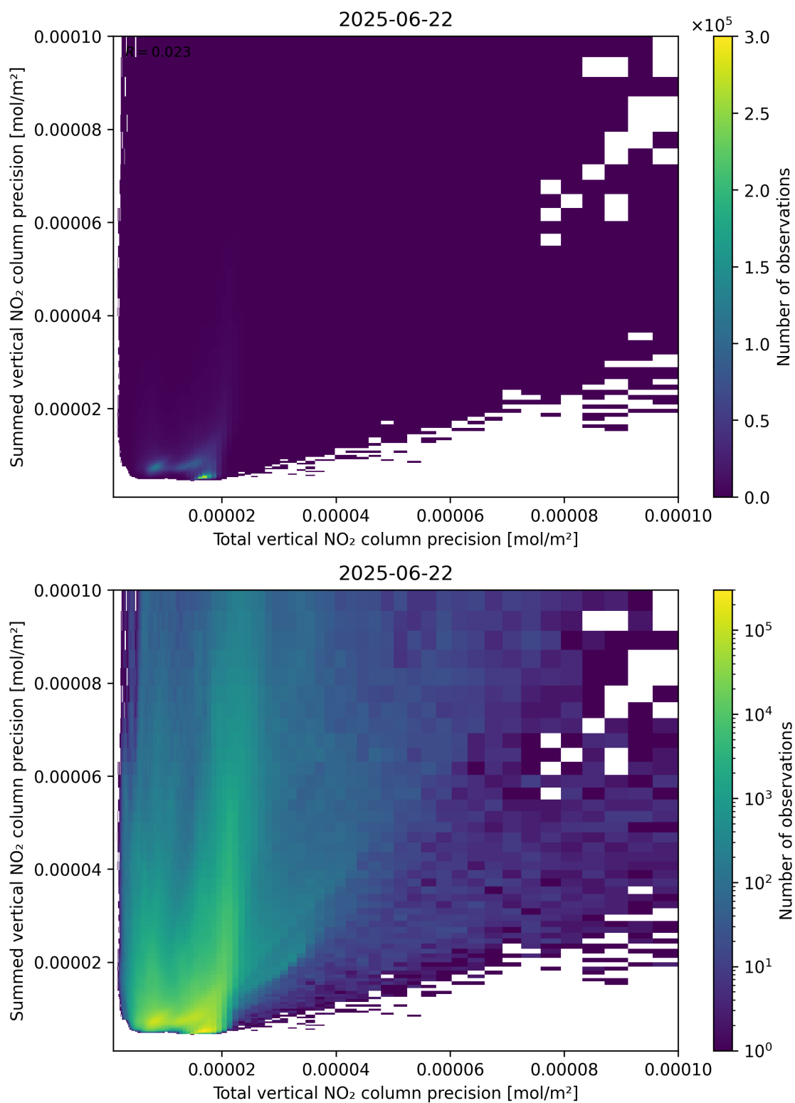
Figure 118: Scatter density plot of “Total vertical NO 2 column precision” against “Summed vertical NO 2 column precision” for 2025-06-22 to 2025-06-23.
