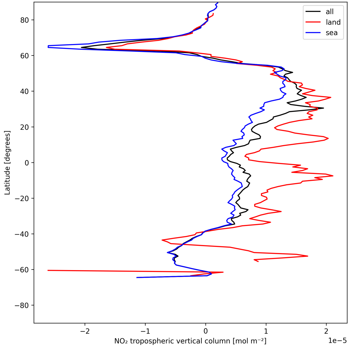
Figure 12: Zonal average of “NO 2 tropospheric vertical column” for 2025-06-22 to 2025-06-23.
