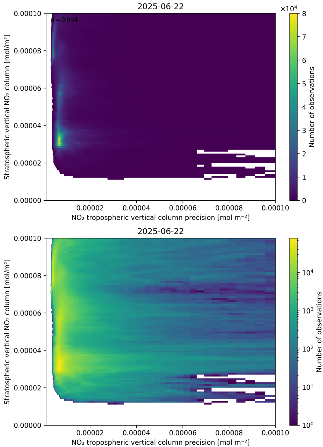
Figure 135: Scatter density plot of “NO 2 tropospheric vertical column precision” against “Stratospheric vertical NO 2 column” for 2025-06-22 to 2025-06-23.
