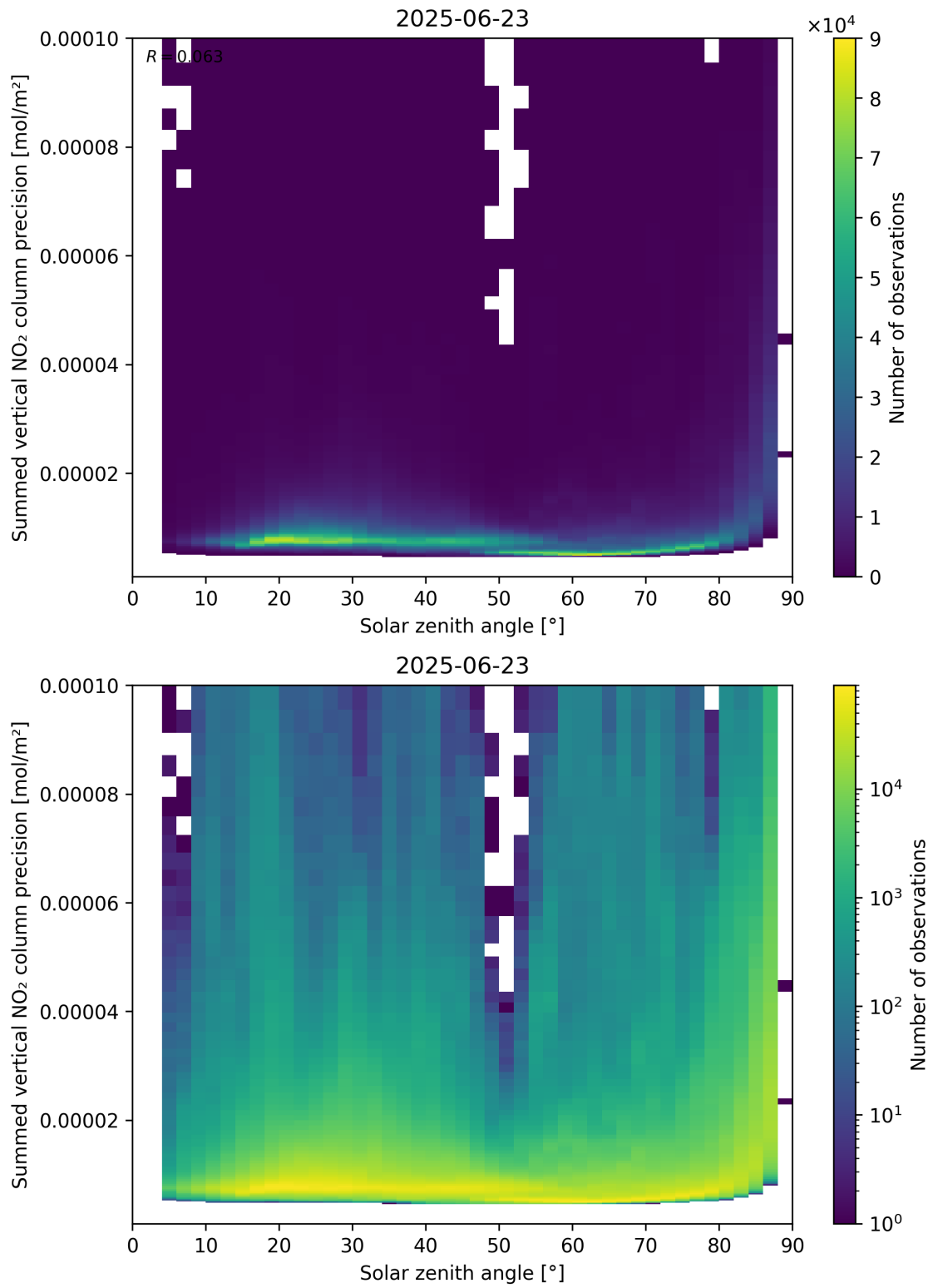
Figure 152: Scatter density plot of “Solar zenith angle” against “Summed vertical NO 2 column precision” for 2025-06-22 to 2025-06-24.
