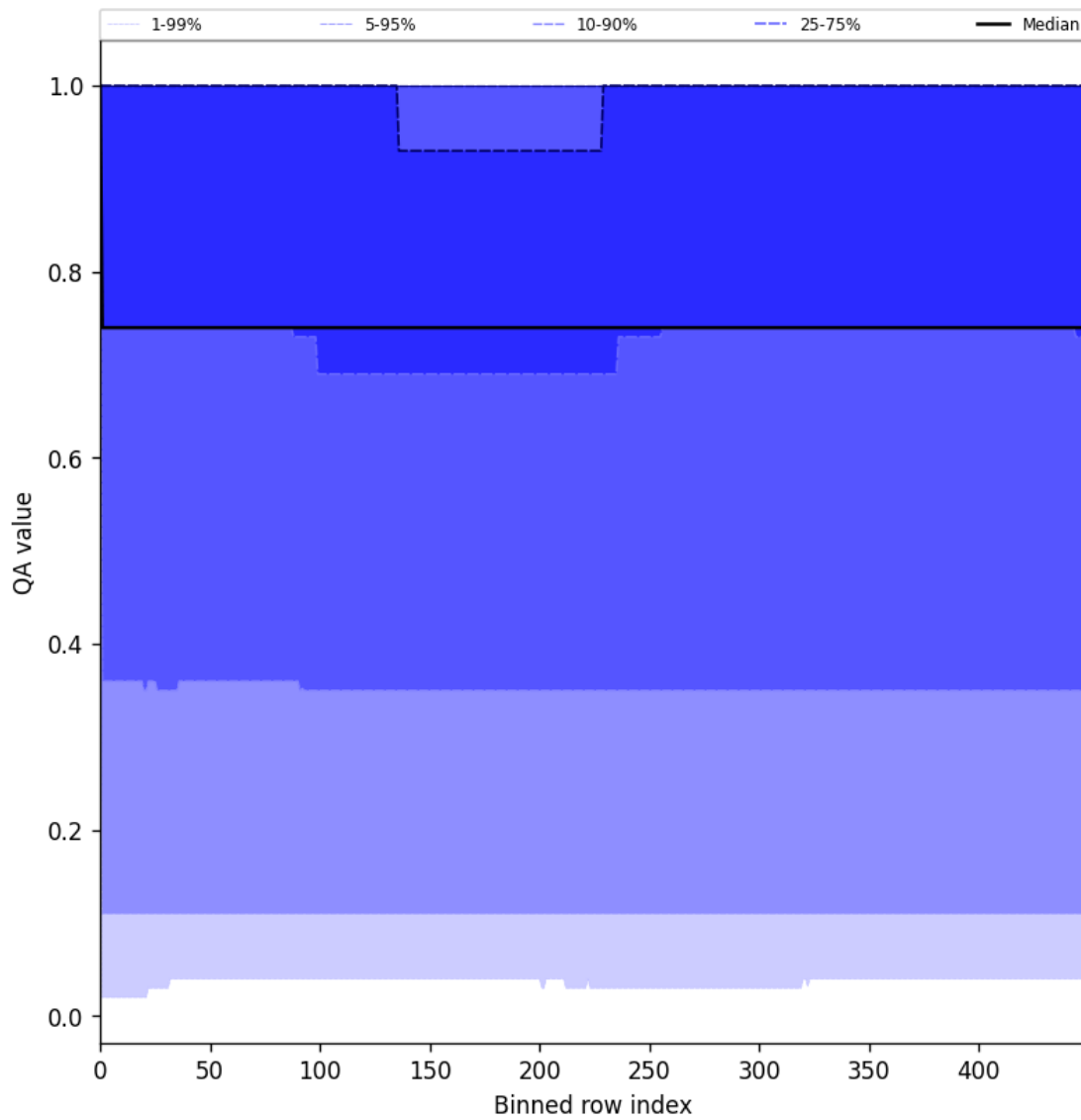
Figure 45: Along track statistics of “QA value” for 2025-06-22 to 2025-06-24
