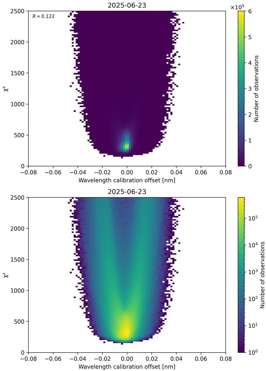
Figure 175: Scatter density plot of “Wavelength calibration offset” against “ \chi^2 ” for 2025-06-22 to 2025-06-24.
