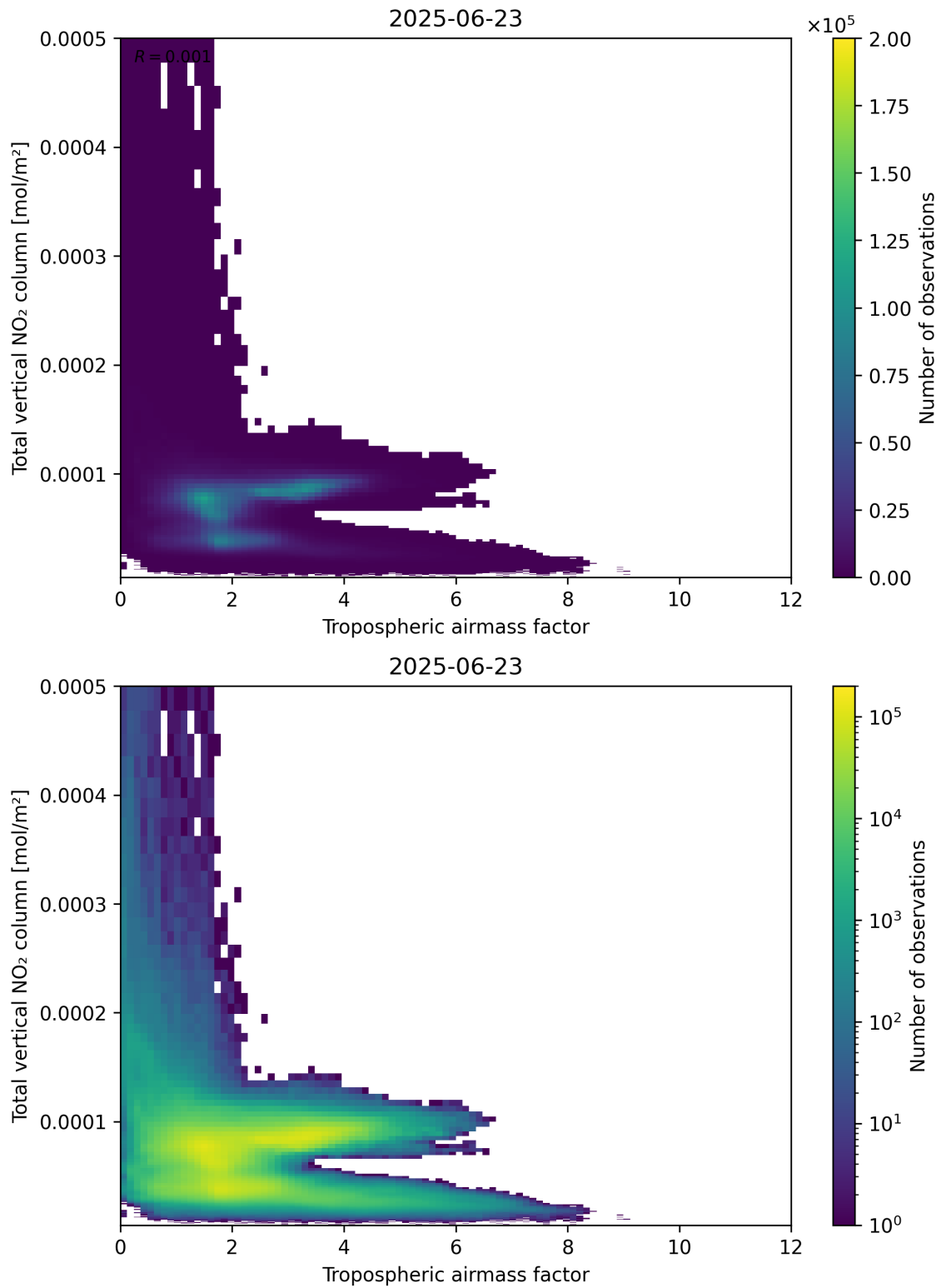
Figure 77: Scatter density plot of “Tropospheric airmass factor” against “Total vertical NO 2 column” for 2025-06-22 to 2025-06-24.
