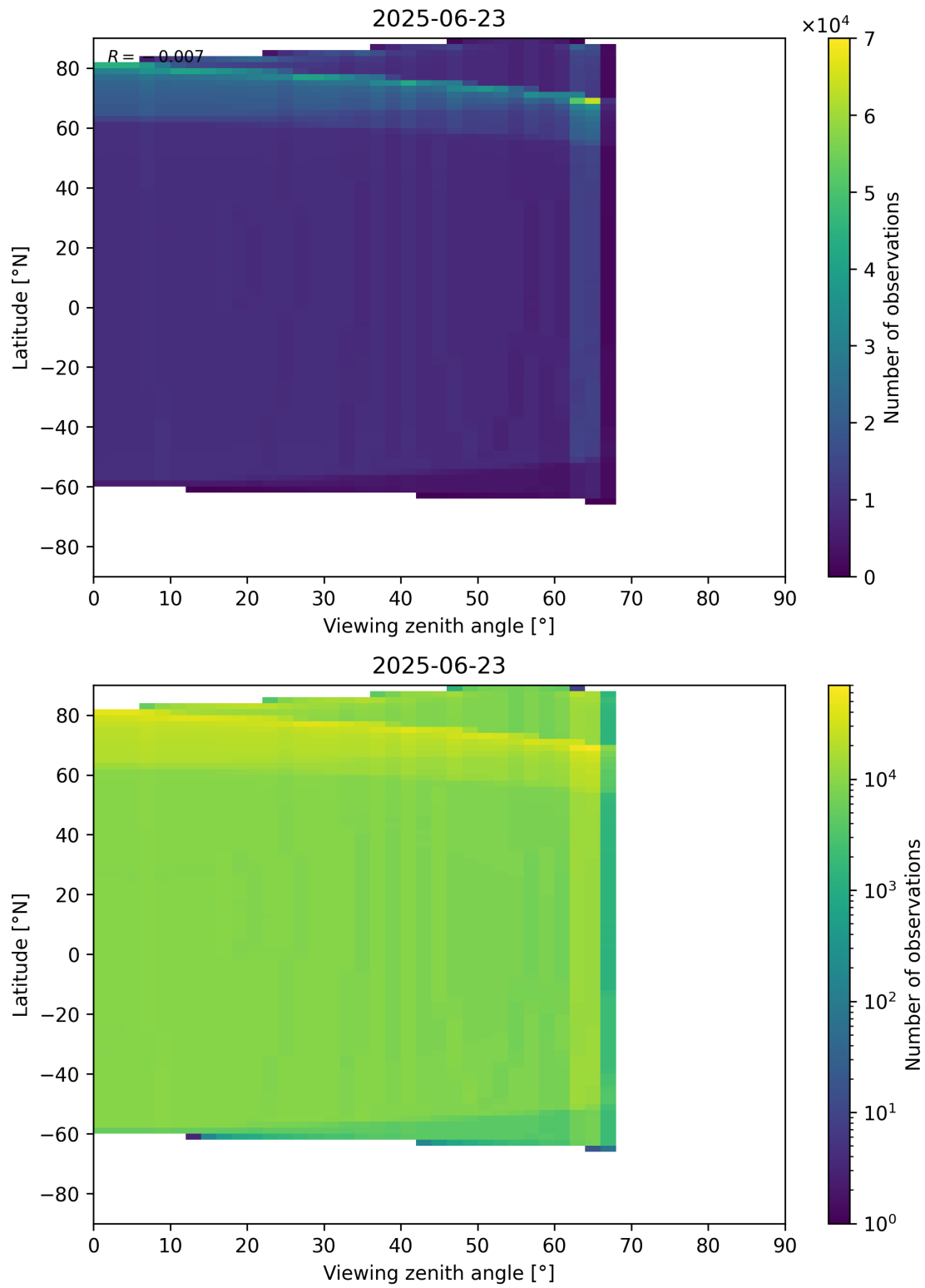
Figure 163: Scatter density plot of “Viewing zenith angle” against “Latitude” for 2025-06-22 to 2025-06-24.
