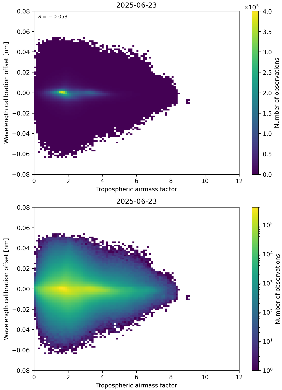
Figure 80: Scatter density plot of “Tropospheric airmass factor” against “Wavelength calibration offset” for 2025-06-22 to 2025-06-24.
