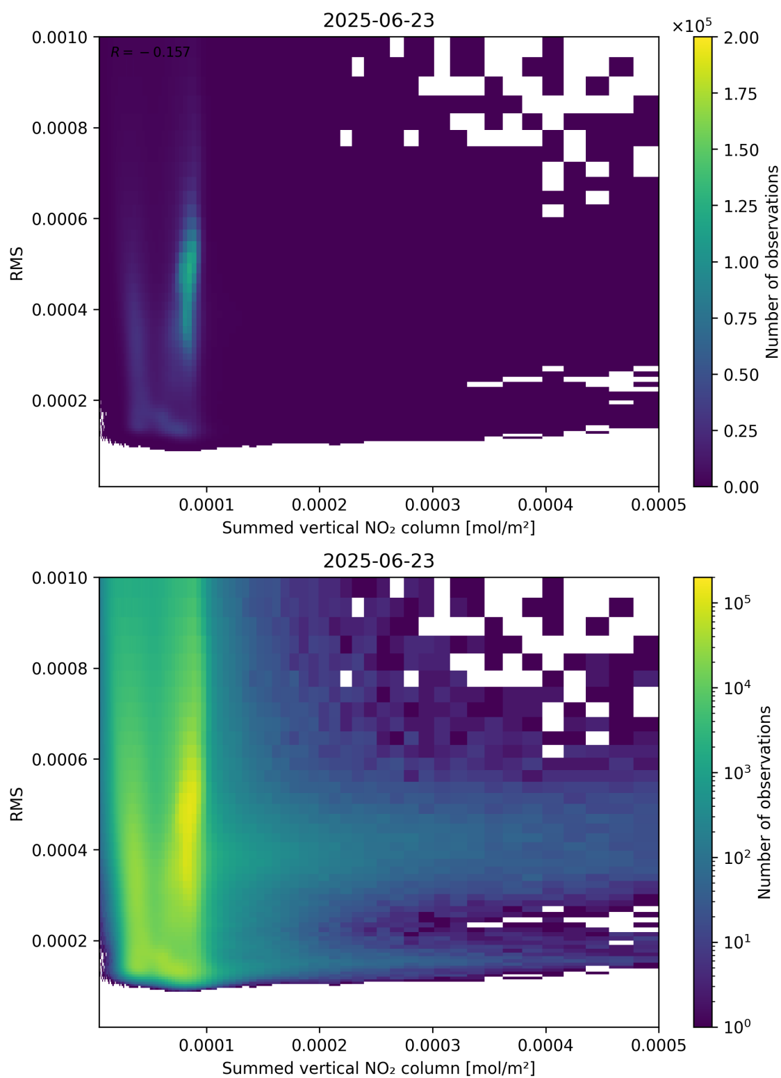
Figure 109: Scatter density plot of “Summed vertical NO 2 column” against “RMS” for 2025-06-22 to 2025-06-24.
