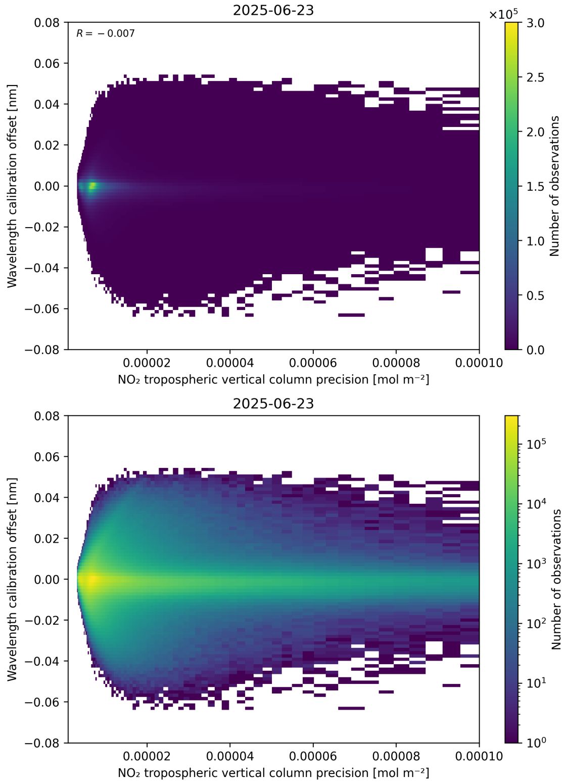
Figure 141: Scatter density plot of “NO 2 tropospheric vertical column precision” against “Wavelength calibration offset” for 2025-06-22 to 2025-06-24.
