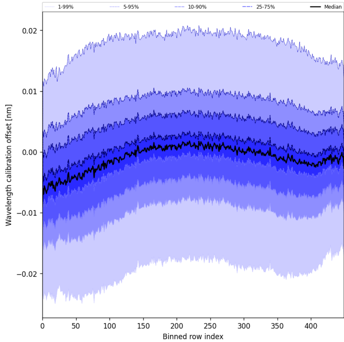
Figure 52: Along track statistics of “Wavelength calibration offset” for 2025-06-22 to 2025-06-24
