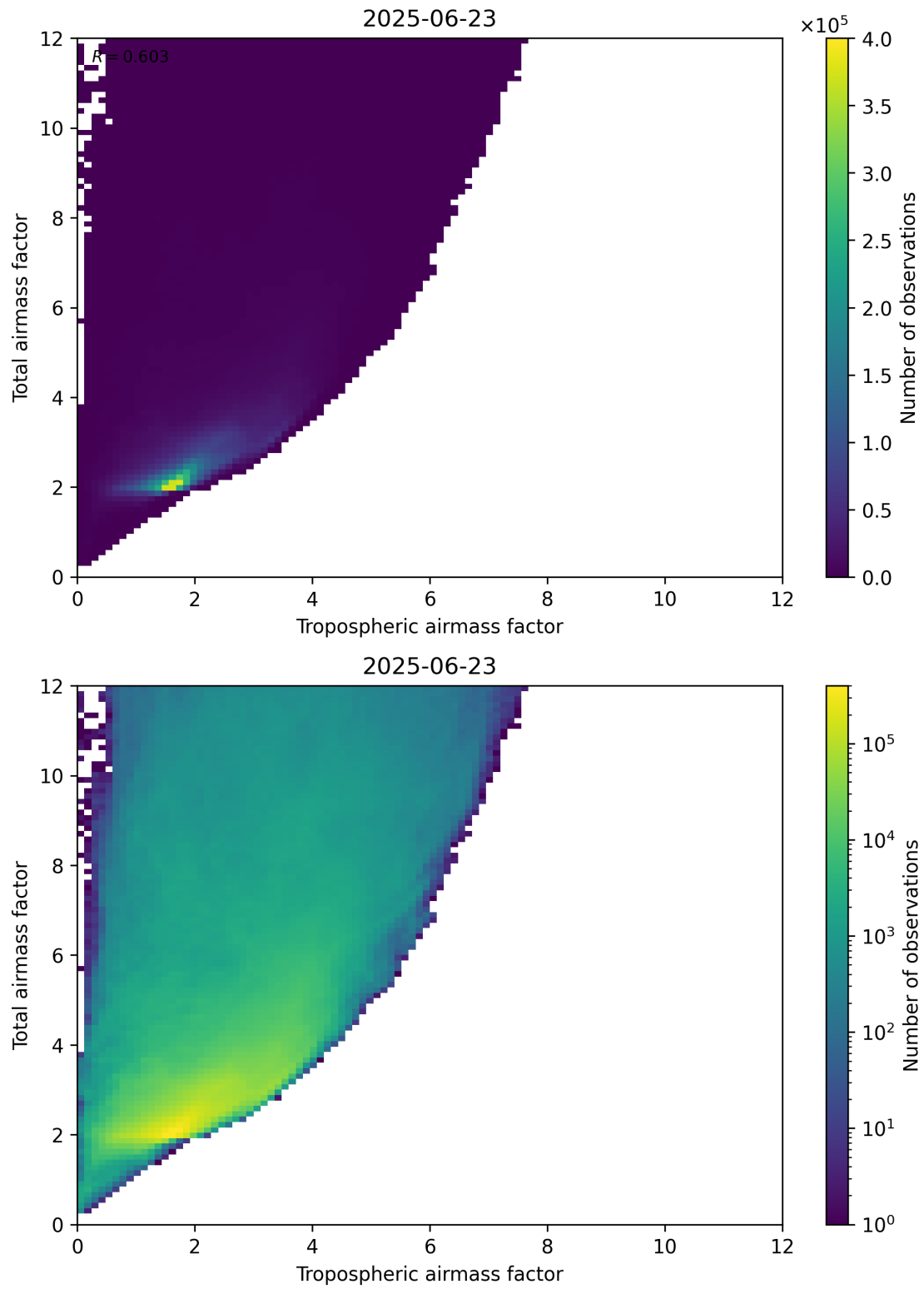
Figure 72: Scatter density plot of “Tropospheric airmass factor” against “Total airmass factor” for 2025-06-22 to 2025-06-24.
