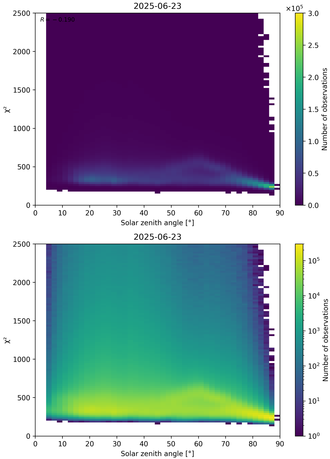
Figure 148: Scatter density plot of “Solar zenith angle” against “ \chi^2 ” for 2025-06-22 to 2025-06-24.
