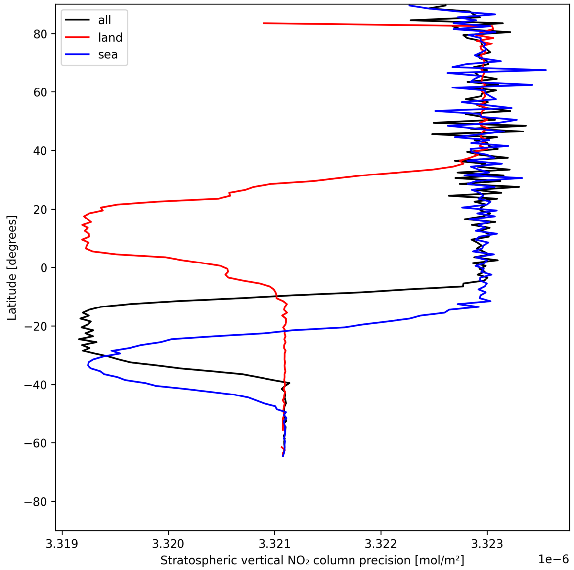
Figure 20: Zonal average of “Stratospheric vertical NO 2 column precision” for 2025-06-22 to 2025-06-24.
