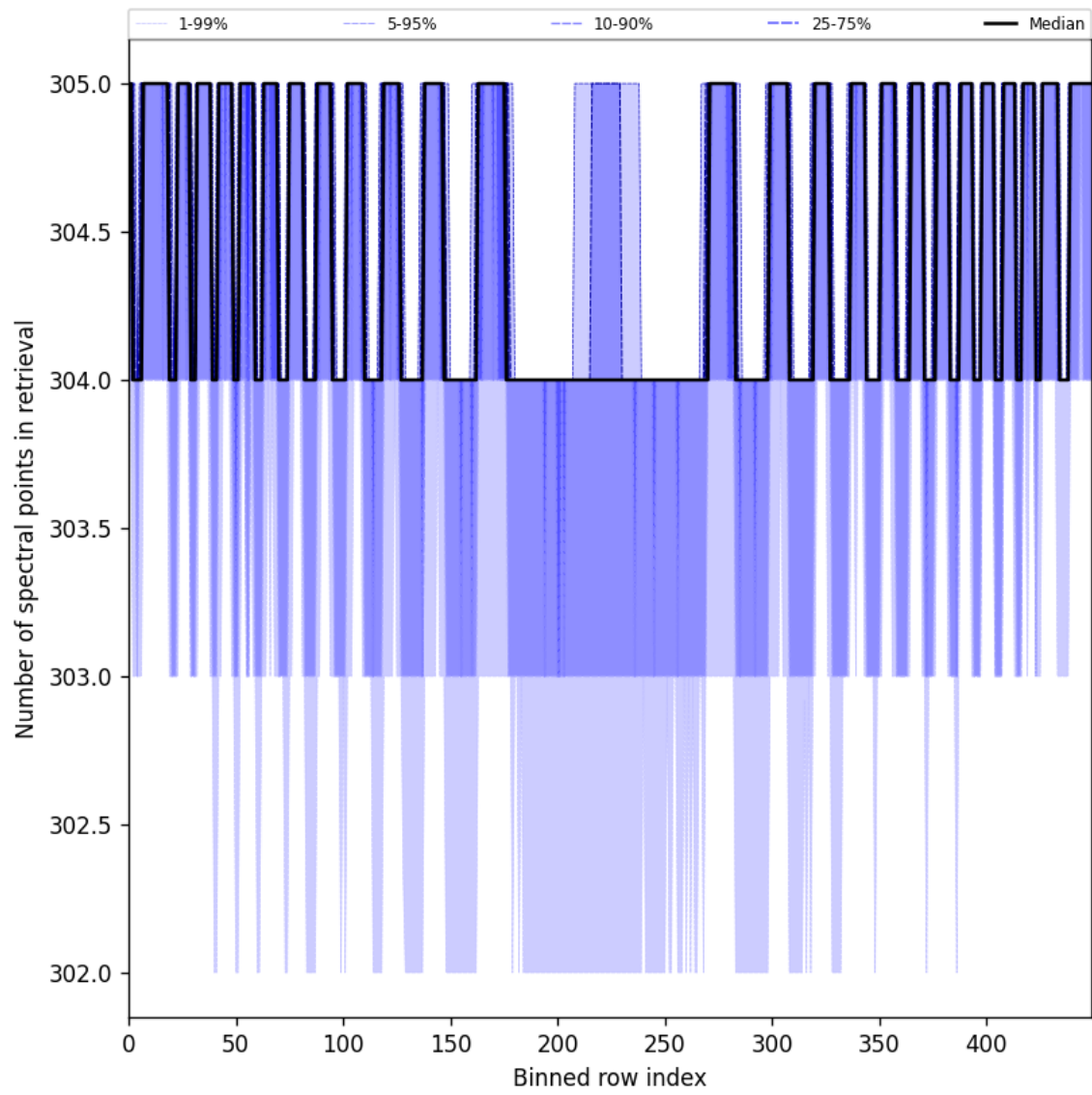
Figure 50: Along track statistics of “Number of spectral points in retrieval” for 2025-06-22 to 2025-06-24
