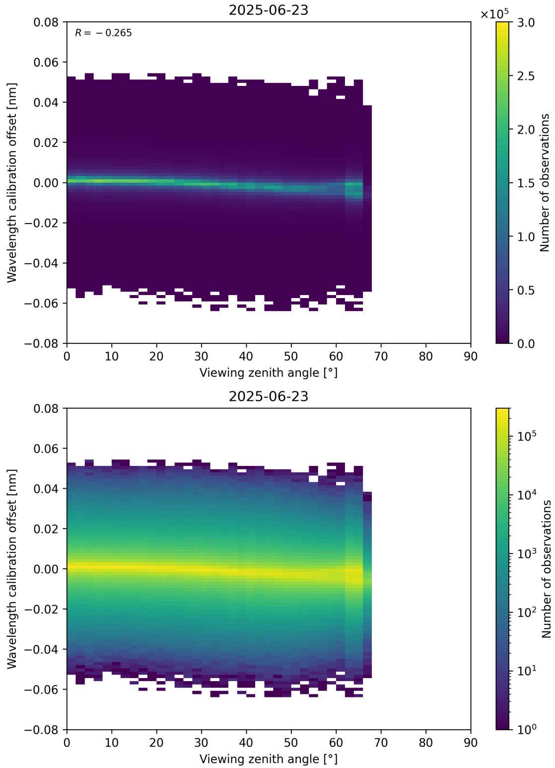
Figure 173: Scatter density plot of “Viewing zenith angle” against “Wavelength calibration offset” for 2025-06-22 to 2025-06-24.
