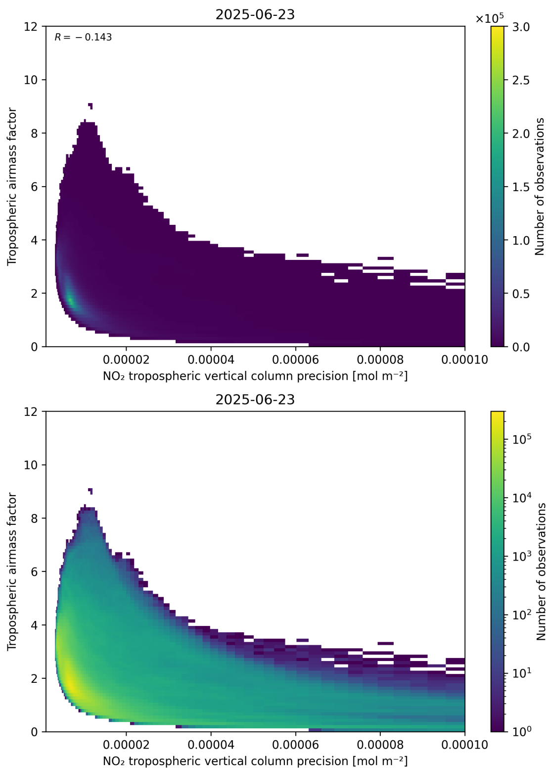
Figure 133: Scatter density plot of “NO 2 tropospheric vertical column precision” against “Tropospheric air mass factor” for 2025-06-22 to 2025-06-24.
