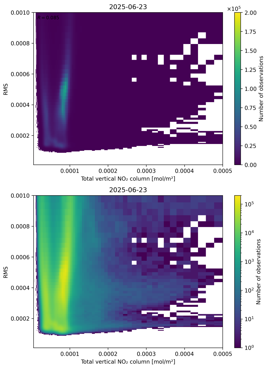
Figure 120: Scatter density plot of “Total vertical NO 2 column” against “RMS” for 2025-06-22 to 2025-06-24.
