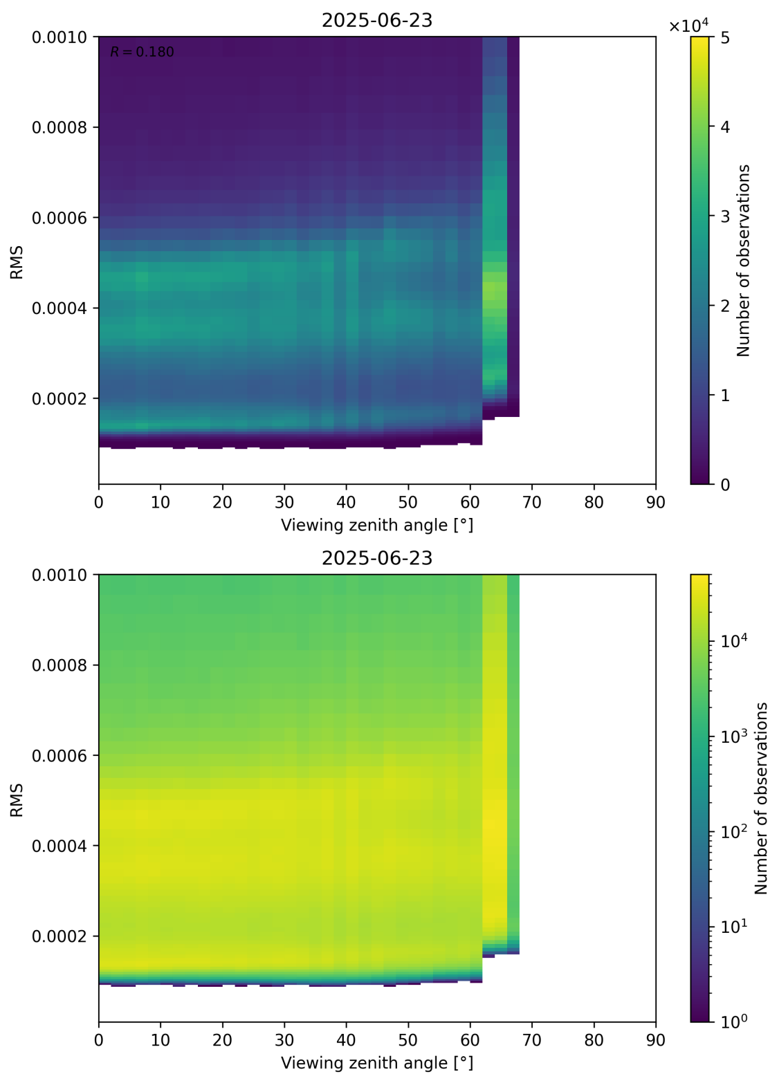
Figure 171: Scatter density plot of “Viewing zenith angle” against “RMS” for 2025-06-22 to 2025-06-24.
