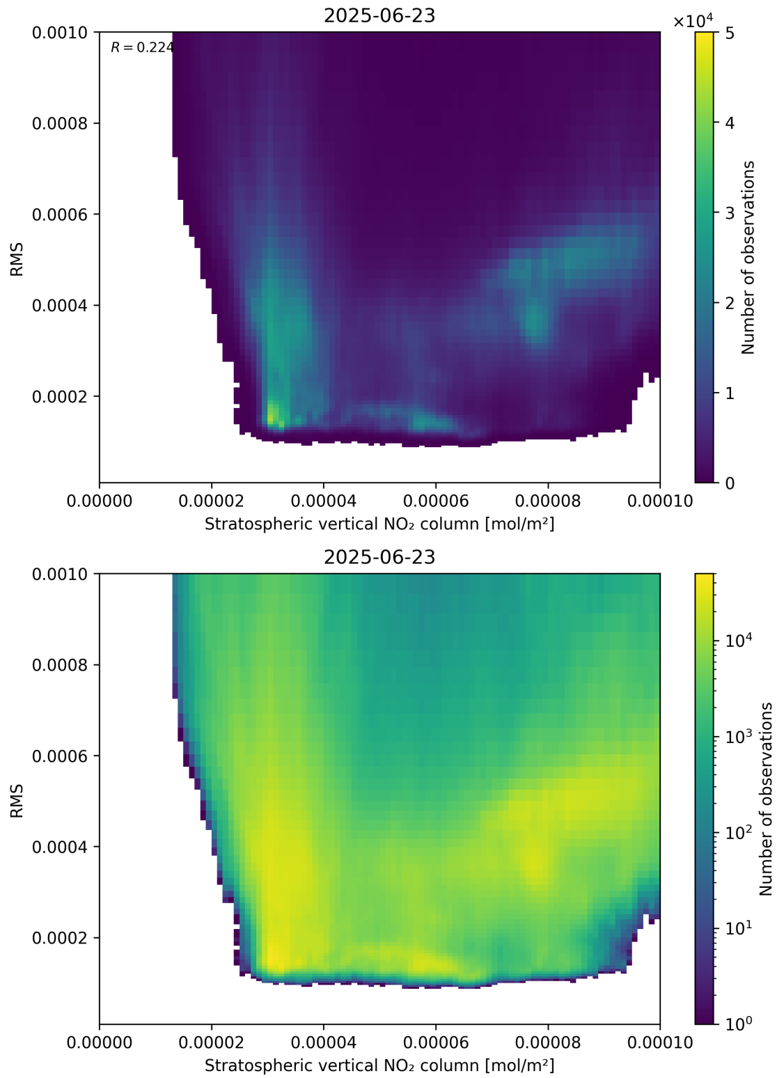
Figure 102: Scatter density plot of “Stratospheric vertical NO 2 column” against “RMS” for 2025-06-22 to 2025-06-24.
