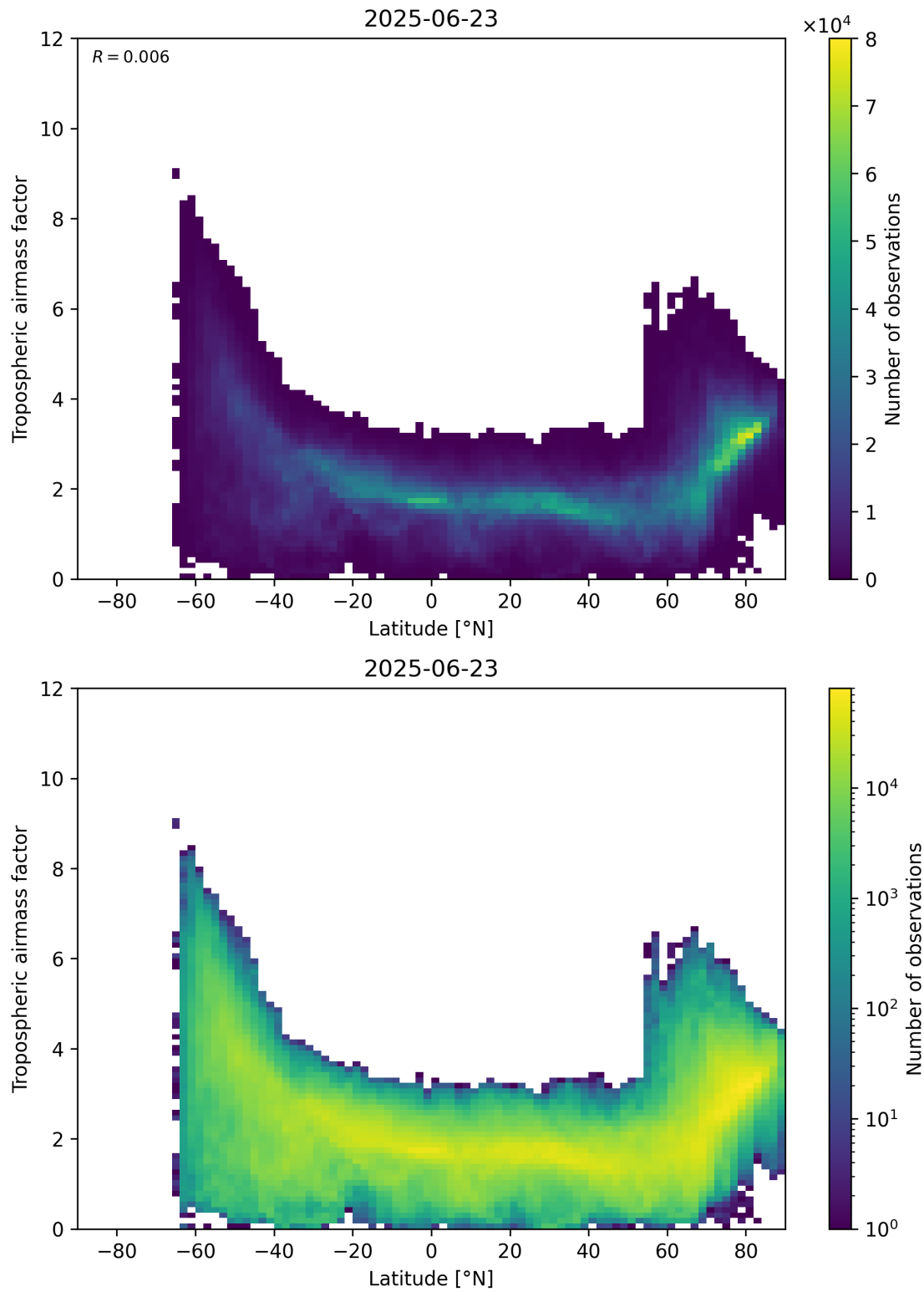
Figure 85: Scatter density plot of “Latitude” against “Tropospheric airmass factor” for 2025-06-22 to 2025-06-24.
