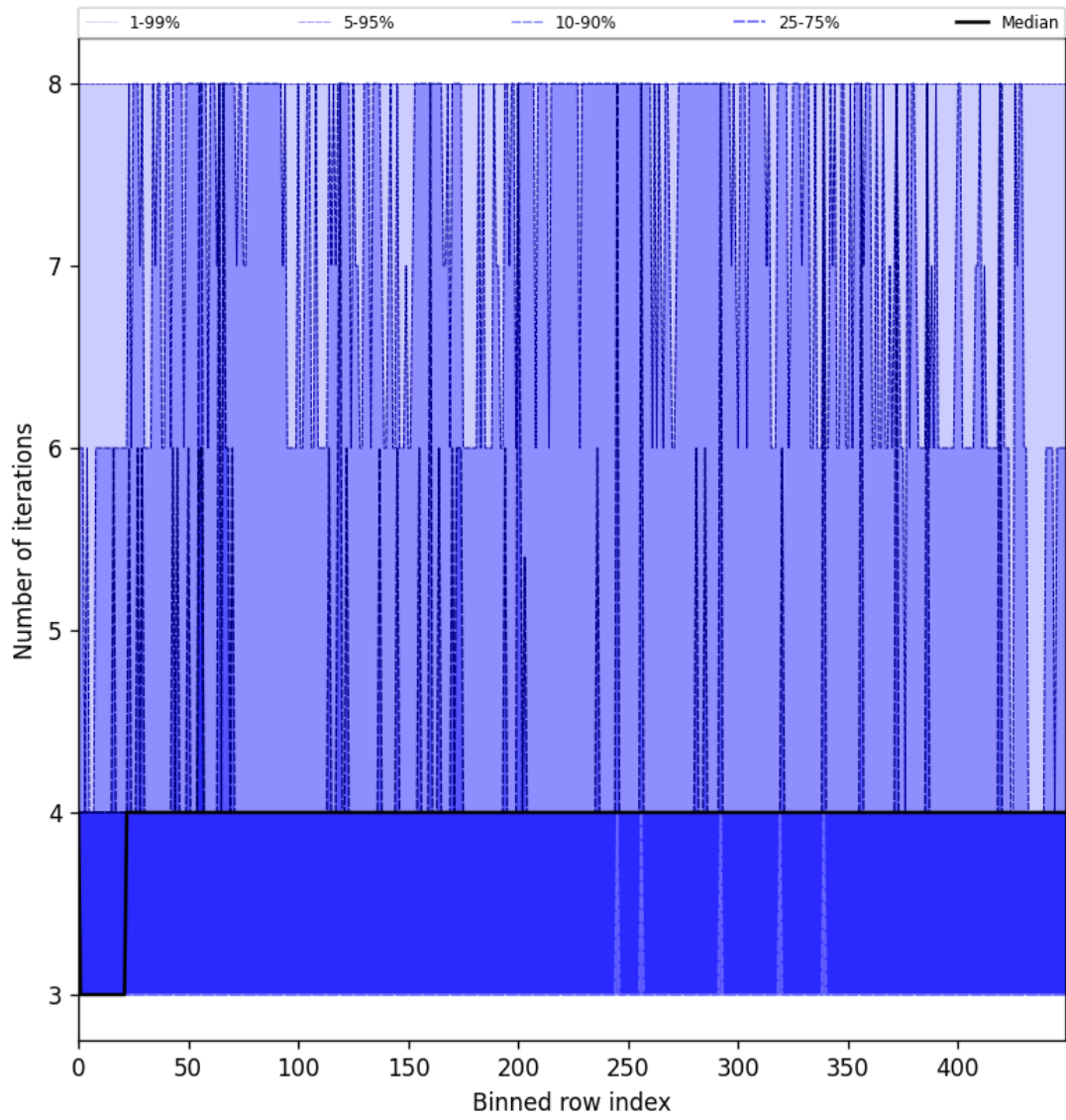
Figure 51: Along track statistics of “Number of iterations” for 2025-06-22 to 2025-06-24
