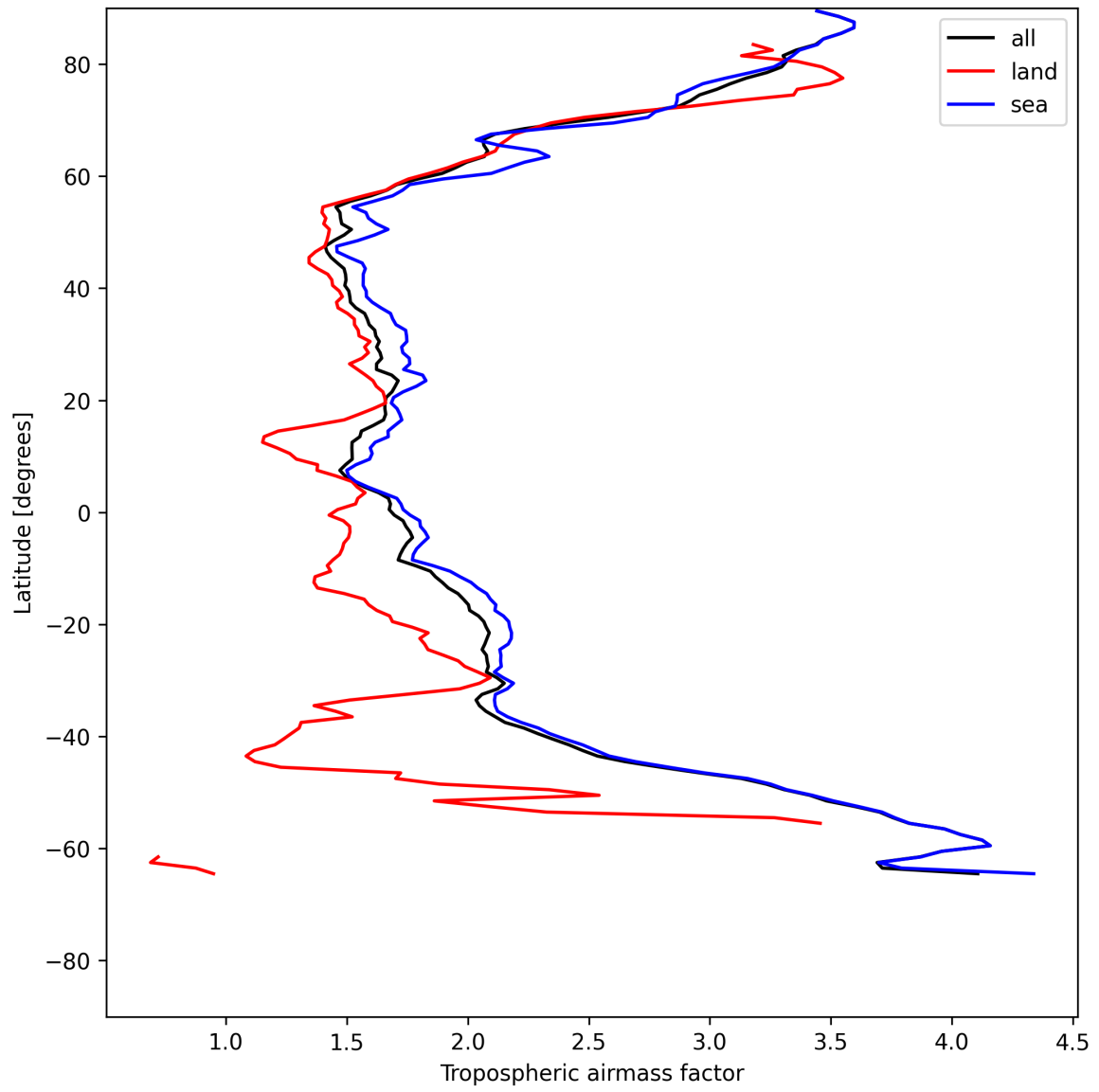
Figure 14: Zonal average of “Tropospheric airmass factor” for 2025-06-22 to 2025-06-24.
