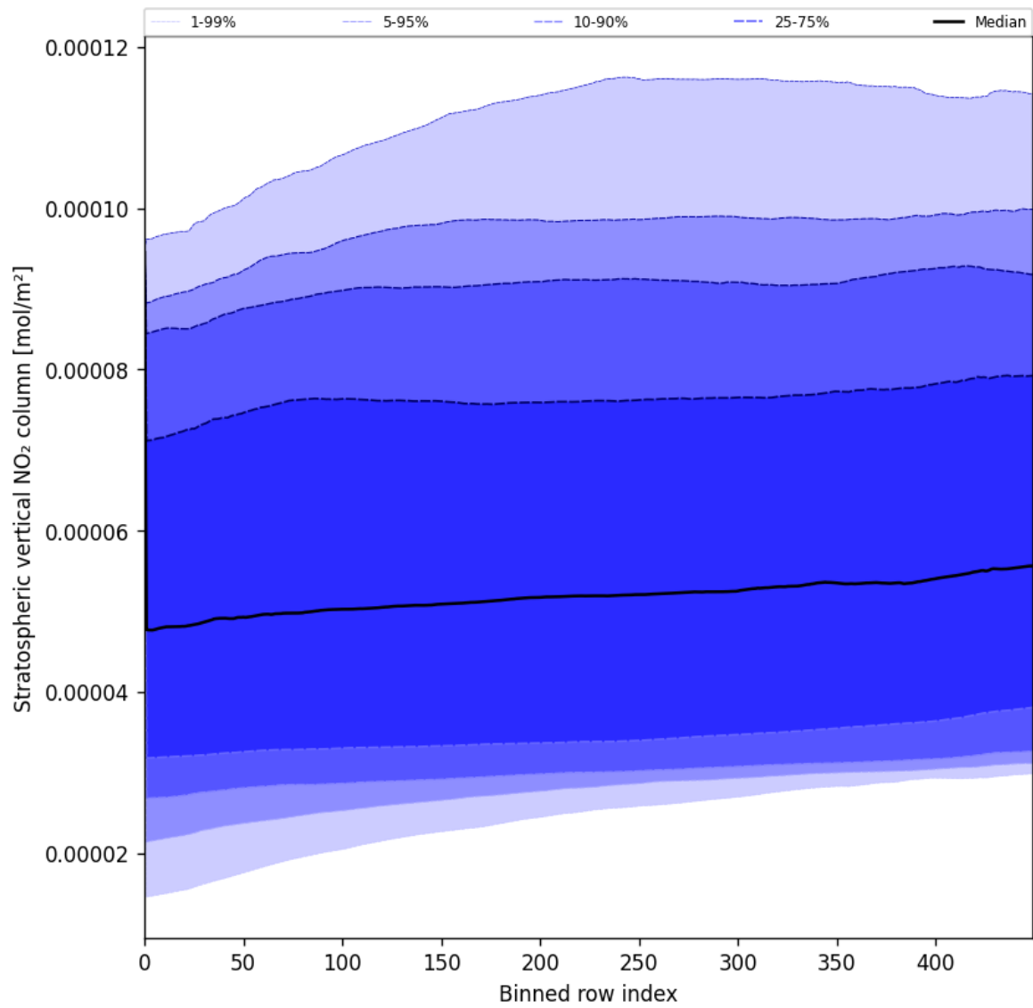
Figure 53: Along track statistics of “Stratospheric vertical NO 2 column” for 2025-06-22 to 2025-06-24
