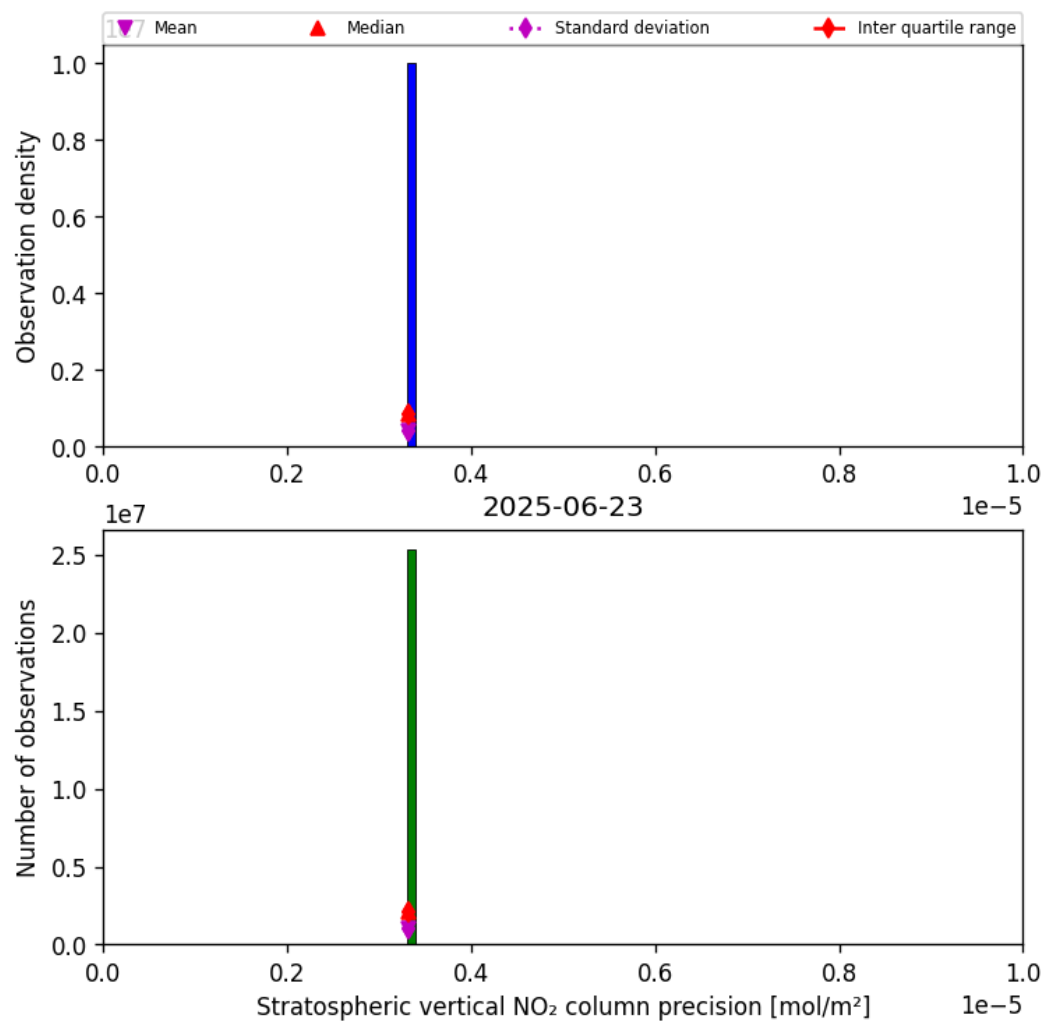
Figure 37: Histogram of “Stratospheric vertical NO 2 column precision” for 2025-06-22 to 2025-06-24
