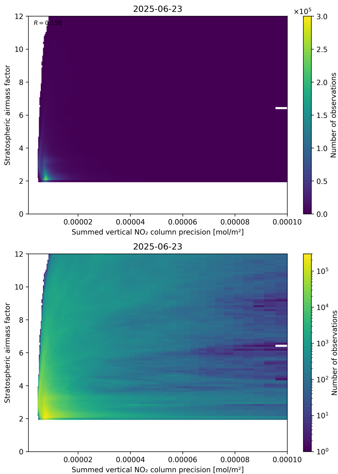
Figure 106: Scatter density plot of “Summed vertical NO 2 column precision” against “Stratospheric airmass factor” for 2025-06-22 to 2025-06-24.
