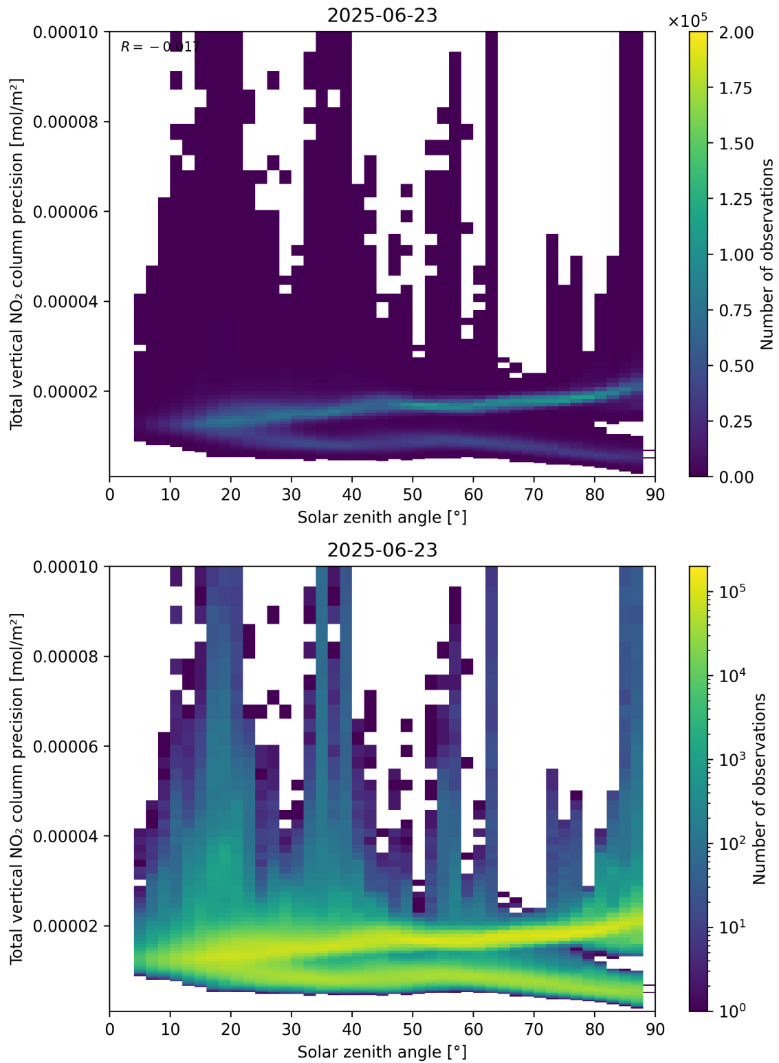
Figure 154: Scatter density plot of “Solar zenith angle” against “Total vertical NO 2 column precision” for 2025-06-22 to 2025-06-24.
