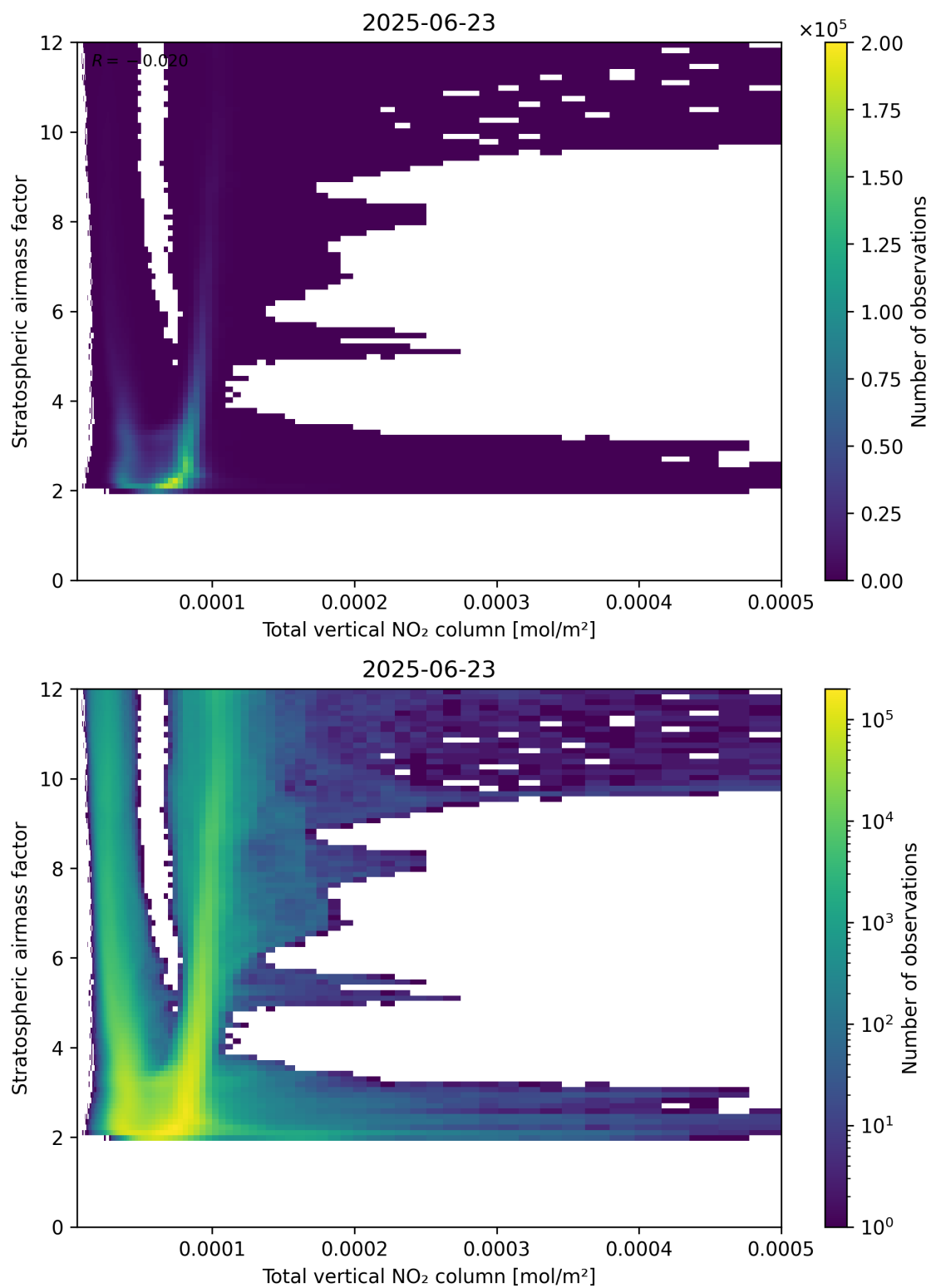
Figure 110: Scatter density plot of “Total vertical NO 2 column” against “Stratospheric airmass factor” for 2025-06-22 to 2025-06-24.
