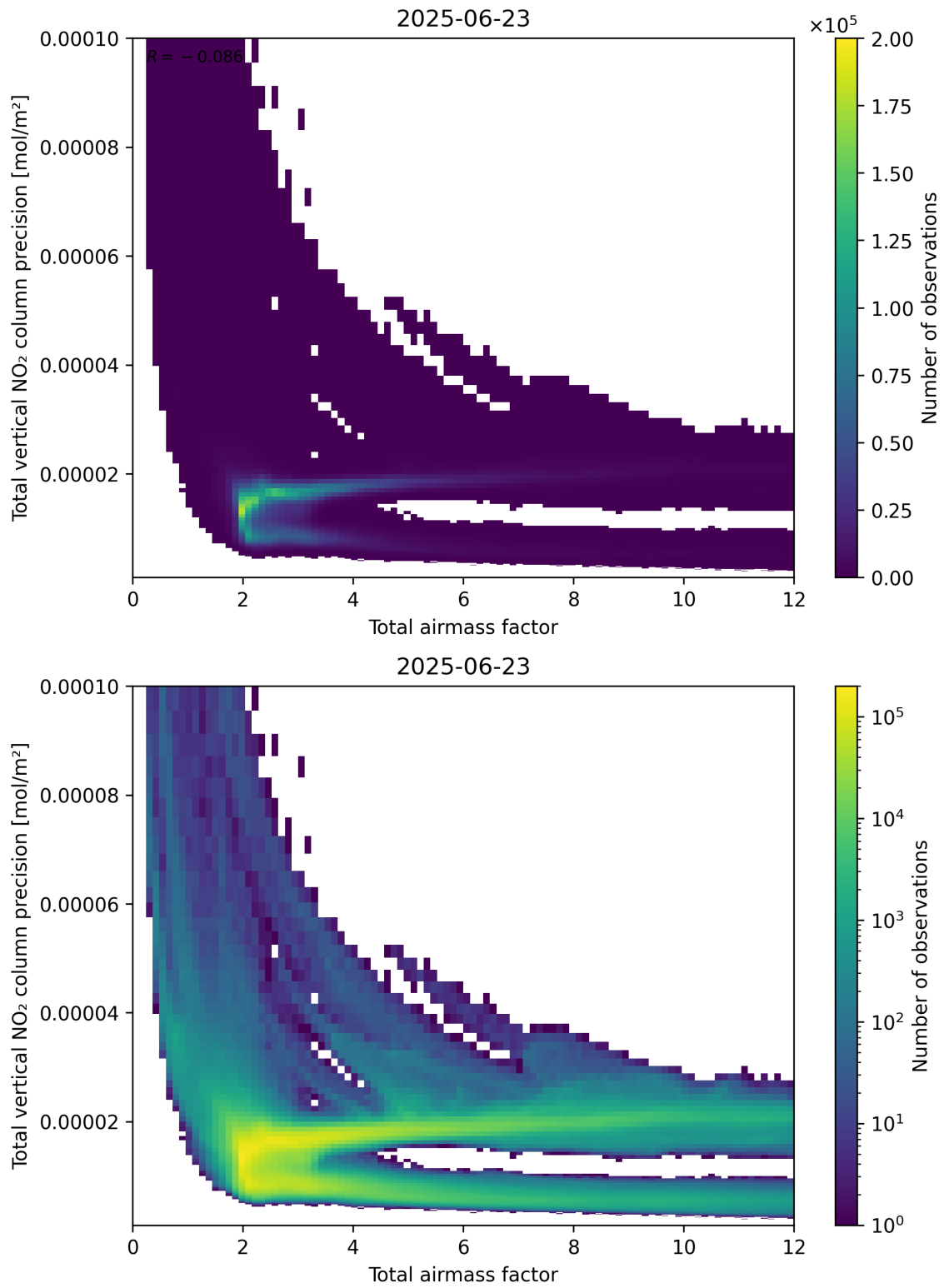
Figure 68: Scatter density plot of “Total airmass factor” against “Total vertical NO 2 column precision” for 2025-06-22 to 2025-06-24.
