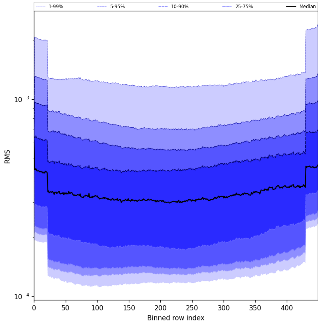
Figure 60: Along track statistics of “RMS” for 2025-06-22 to 2025-06-24
