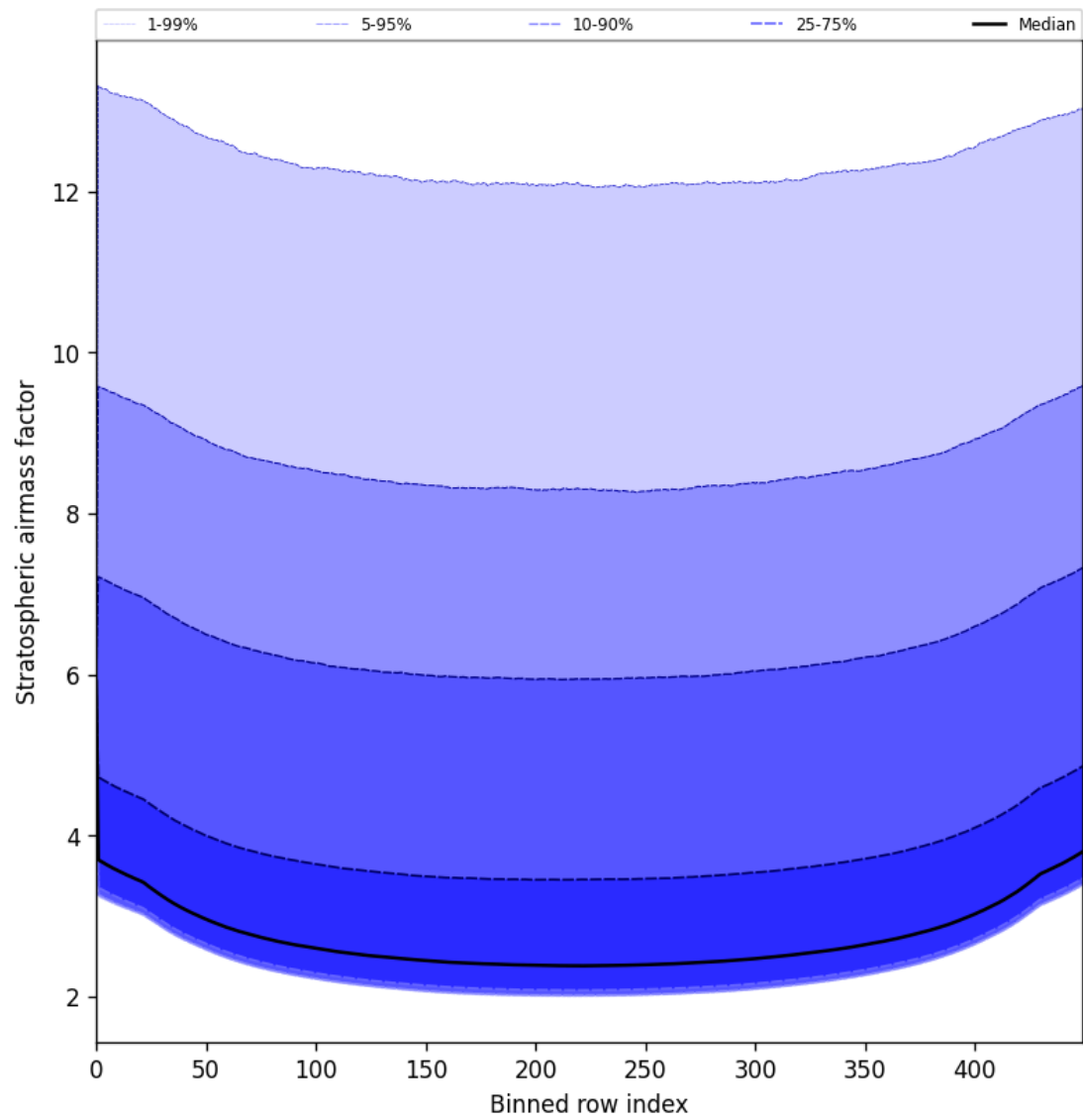
Figure 61: Along track statistics of “Stratospheric airmass factor” for 2025-06-22 to 2025-06-24
