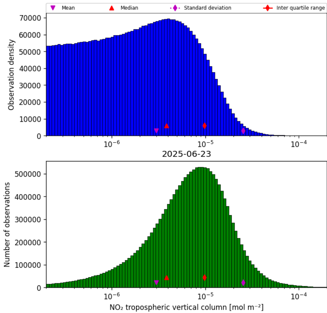
Figure 29: Histogram of “NO 2 tropospheric vertical column” for 2025-06-22 to 2025-06-24
