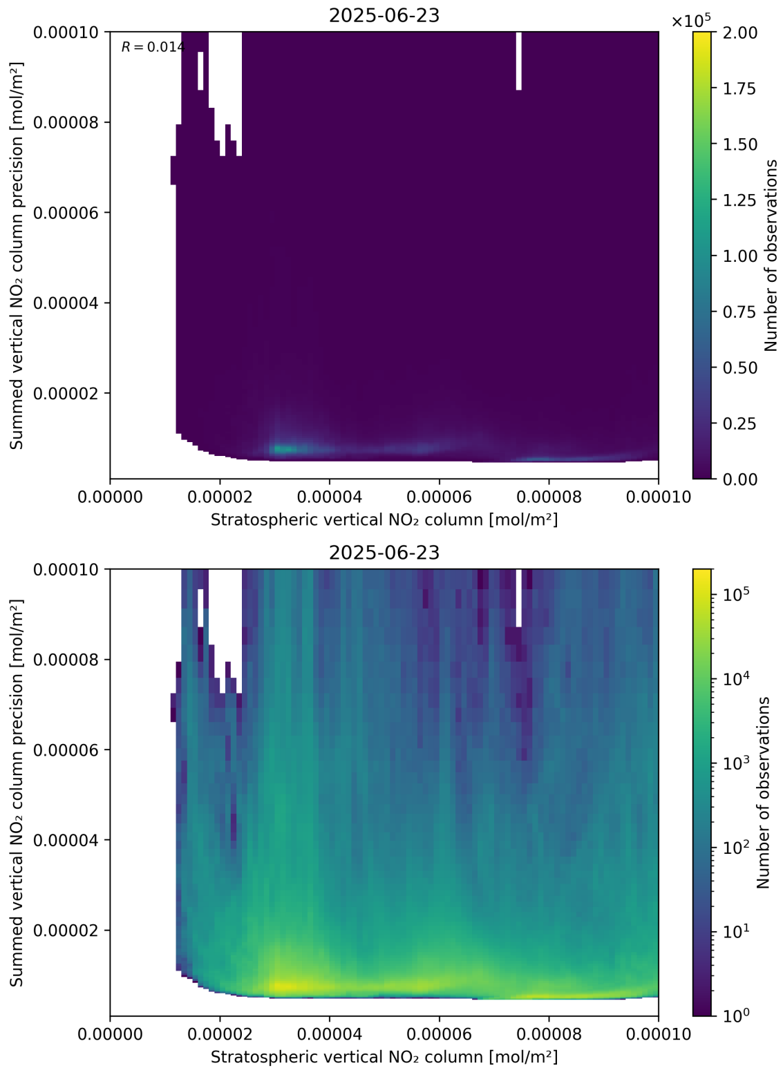
Figure 99: Scatter density plot of “Stratospheric vertical NO 2 column” against “Summed vertical NO 2 column precision” for 2025-06-22 to 2025-06-24.
