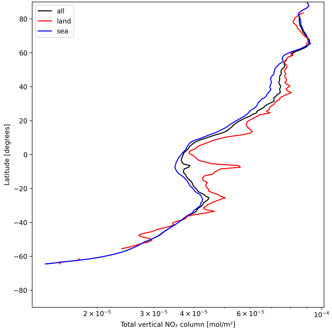
Figure 21: Zonal average of “Total vertical NO 2 column” for 2025-06-22 to 2025-06-24.
