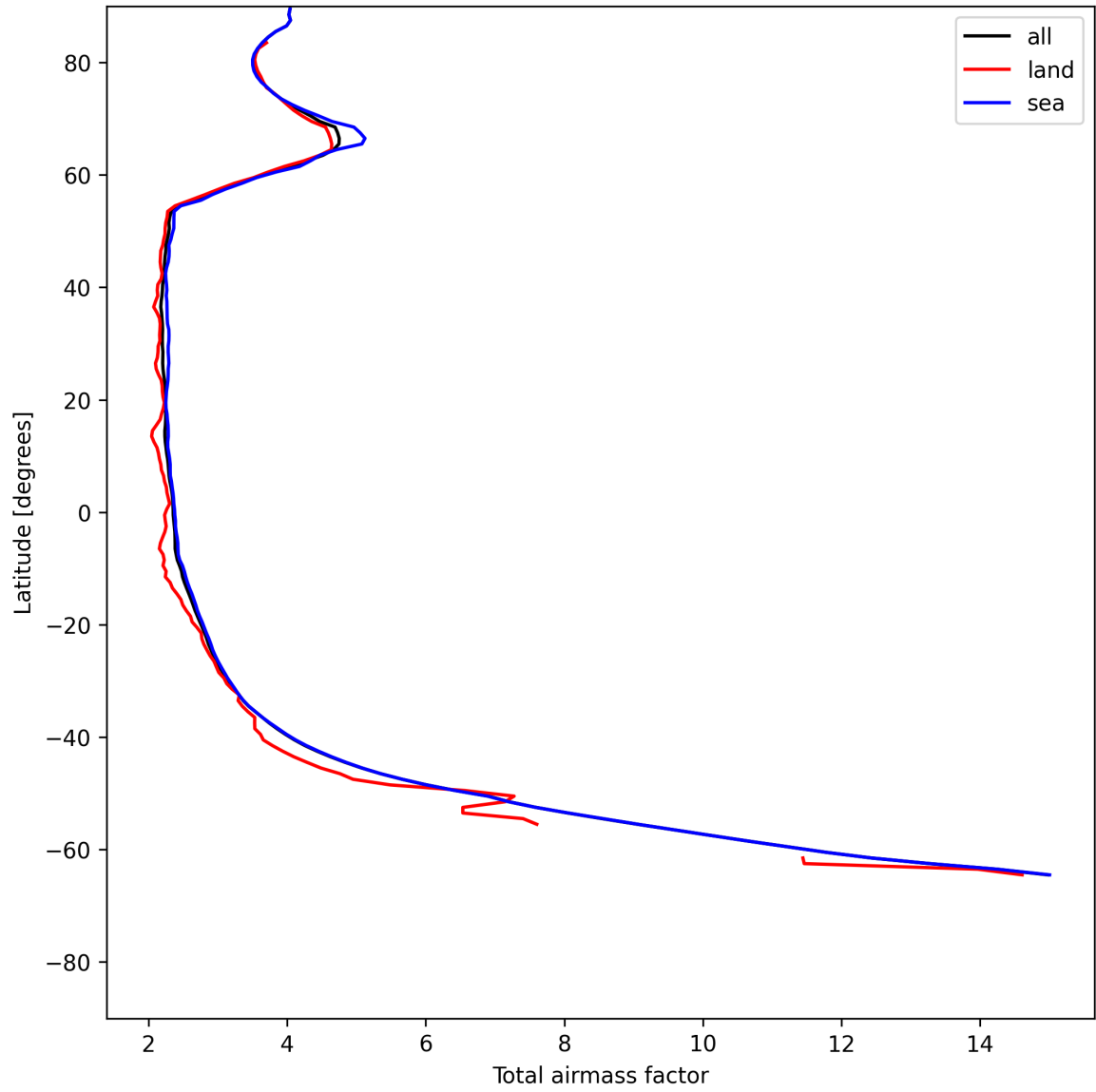
Figure 15: Zonal average of “Total airmass factor” for 2025-06-22 to 2025-06-24.
