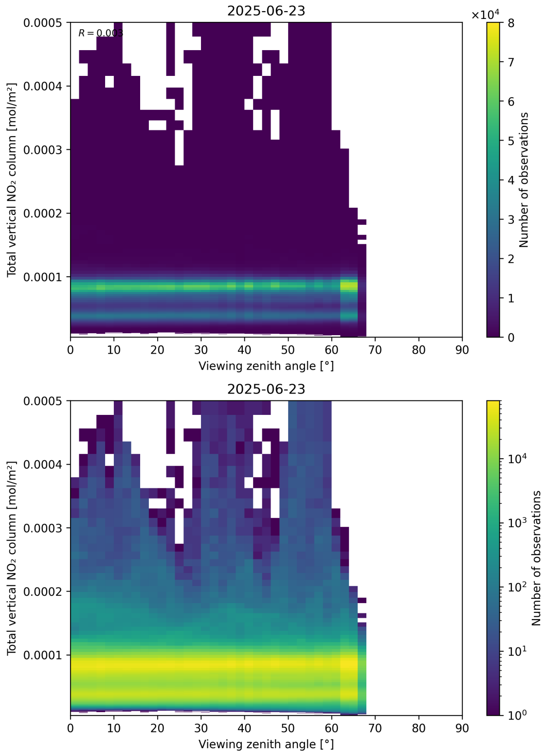
Figure 167: Scatter density plot of “Viewing zenith angle” against “Total vertical NO 2 column” for 2025-06-22 to 2025-06-24.
