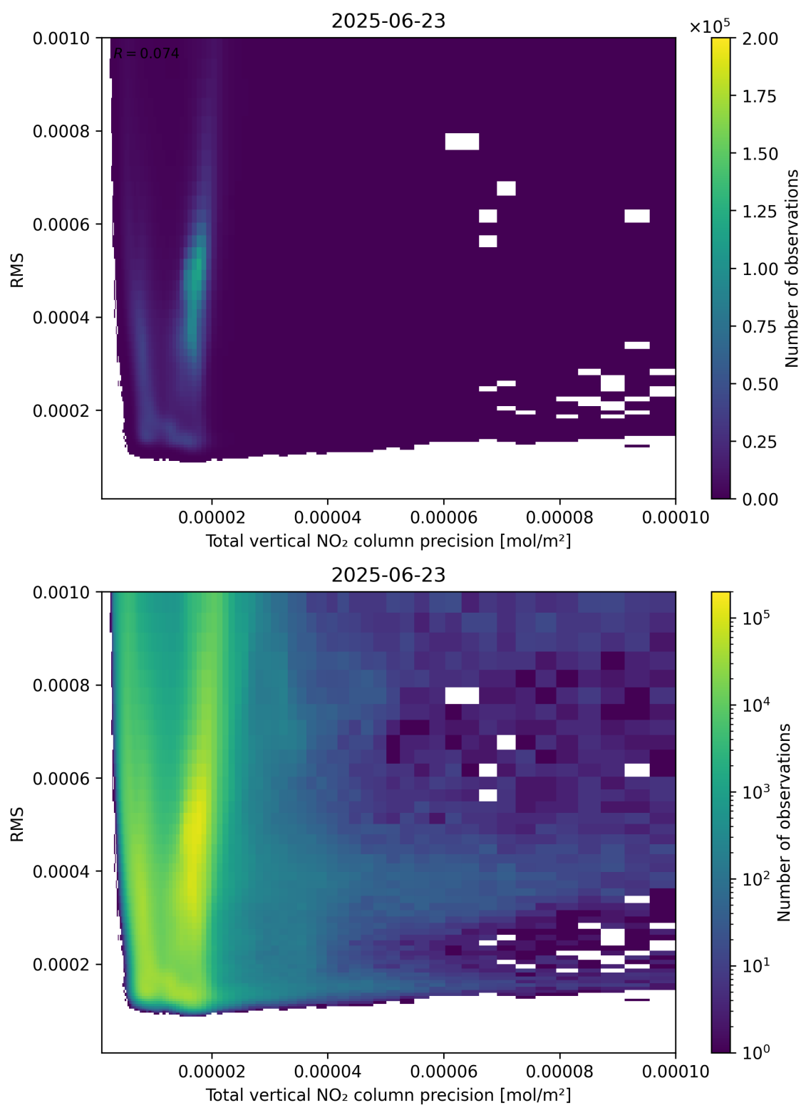
Figure 119: Scatter density plot of “Total vertical NO 2 column precision” against “RMS” for 2025-06-22 to 2025-06-24.
