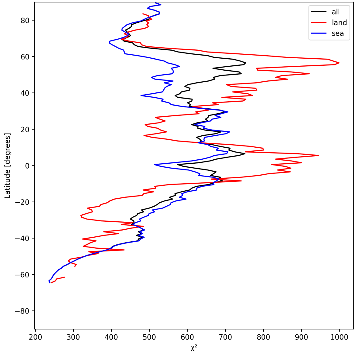
Figure 25: Zonal average of “ \chi^2 ” for 2025-06-22 to 2025-06-24.
