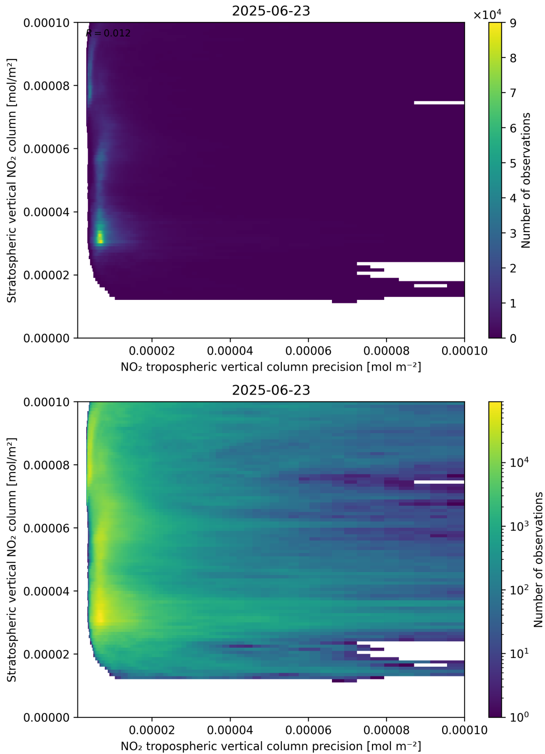
Figure 135: Scatter density plot of “NO 2 tropospheric vertical column precision” against “Stratospheric vertical NO 2 column” for 2025-06-22 to 2025-06-24.
