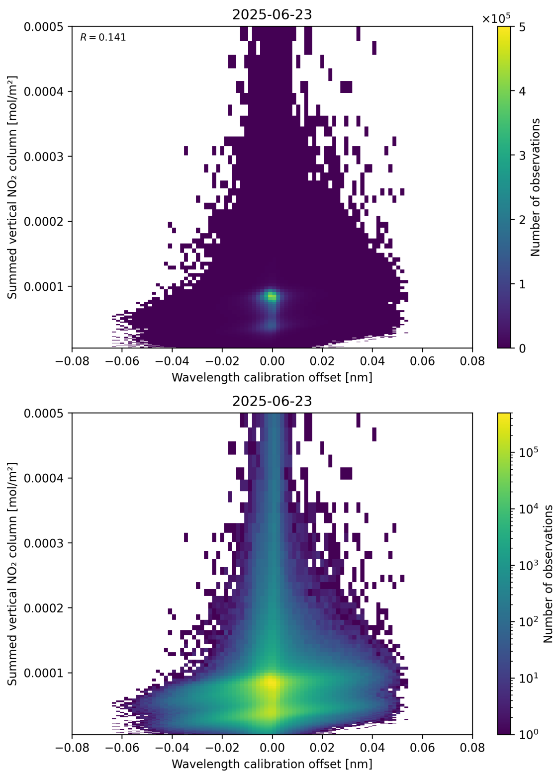
Figure 177: Scatter density plot of “Wavelength calibration offset” against “Summed vertical NO 2 column” for 2025-06-22 to 2025-06-24.
