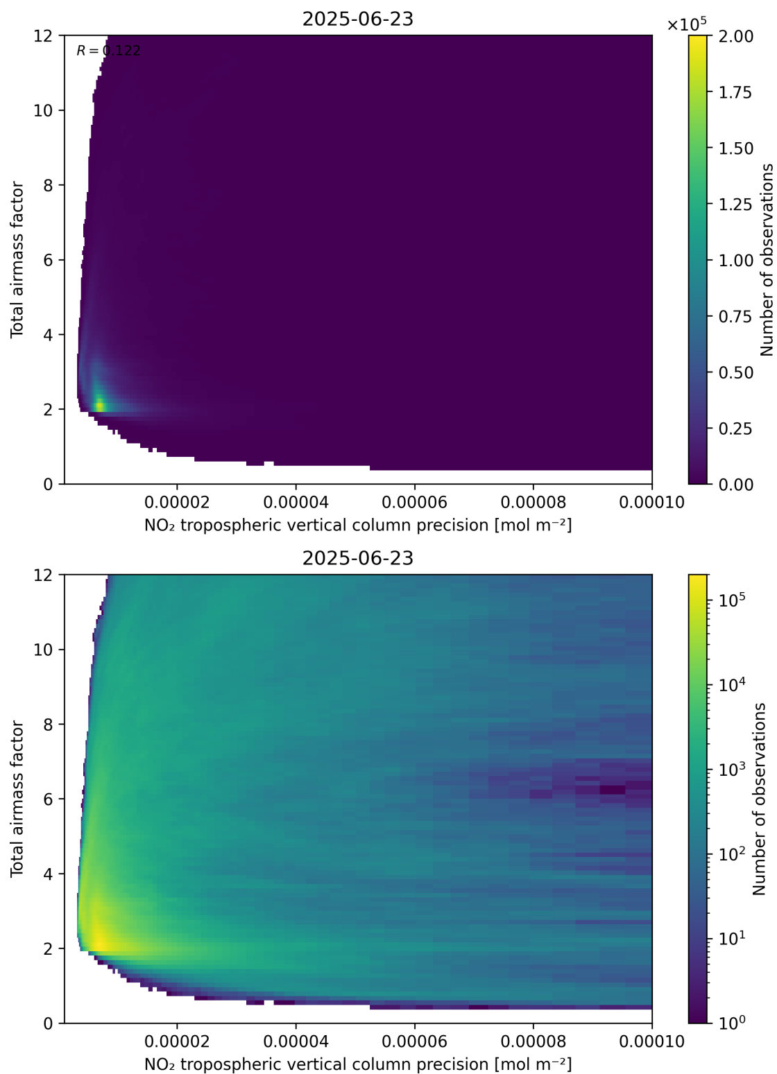
Figure 132: Scatter density plot of “NO 2 tropospheric vertical column precision” against “Total air mass factor” for 2025-06-22 to 2025-06-24.
