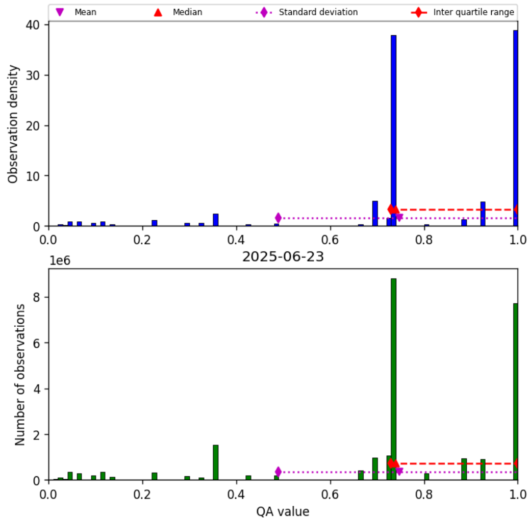
Figure 28: Histogram of “QA value” for 2025-06-22 to 2025-06-24
