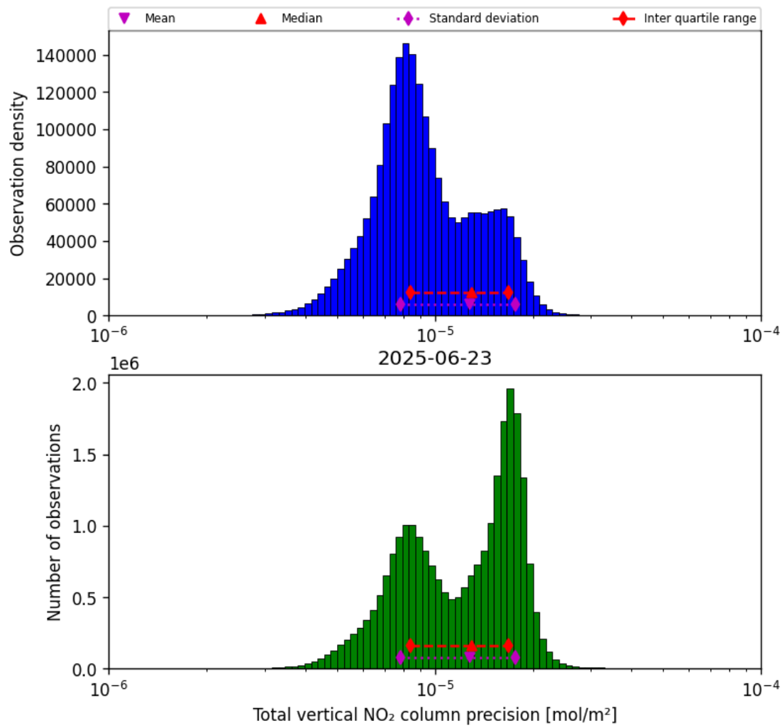
Figure 39: Histogram of “Total vertical NO 2 column precision” for 2025-06-22 to 2025-06-24
