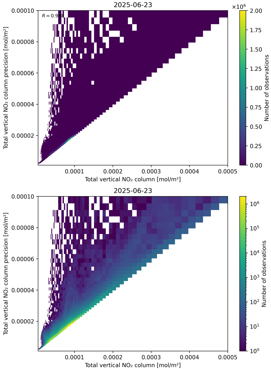
Figure 114: Scatter density plot of “Total vertical NO 2 column” against “Total vertical NO 2 column precision” for 2025-06-22 to 2025-06-24.
