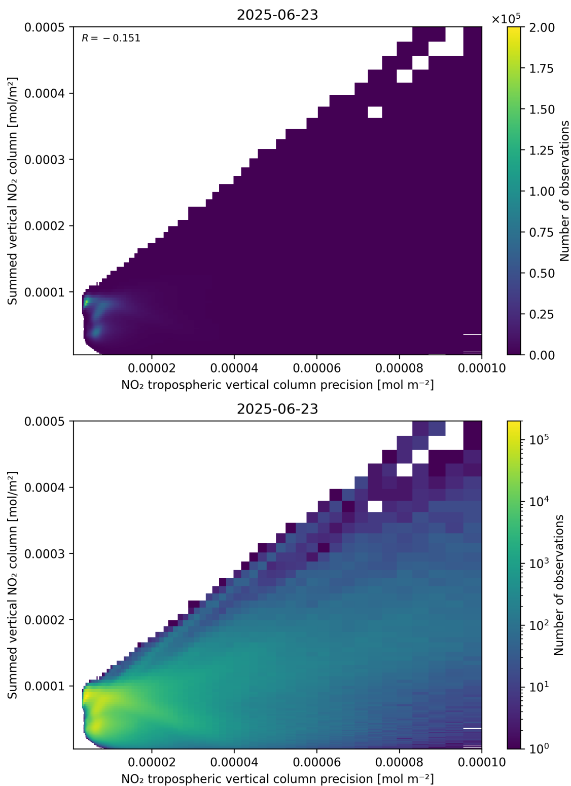
Figure 136: Scatter density plot of “NO 2 tropospheric vertical column precision” against “Summed vertical NO 2 column” for 2025-06-22 to 2025-06-24.
