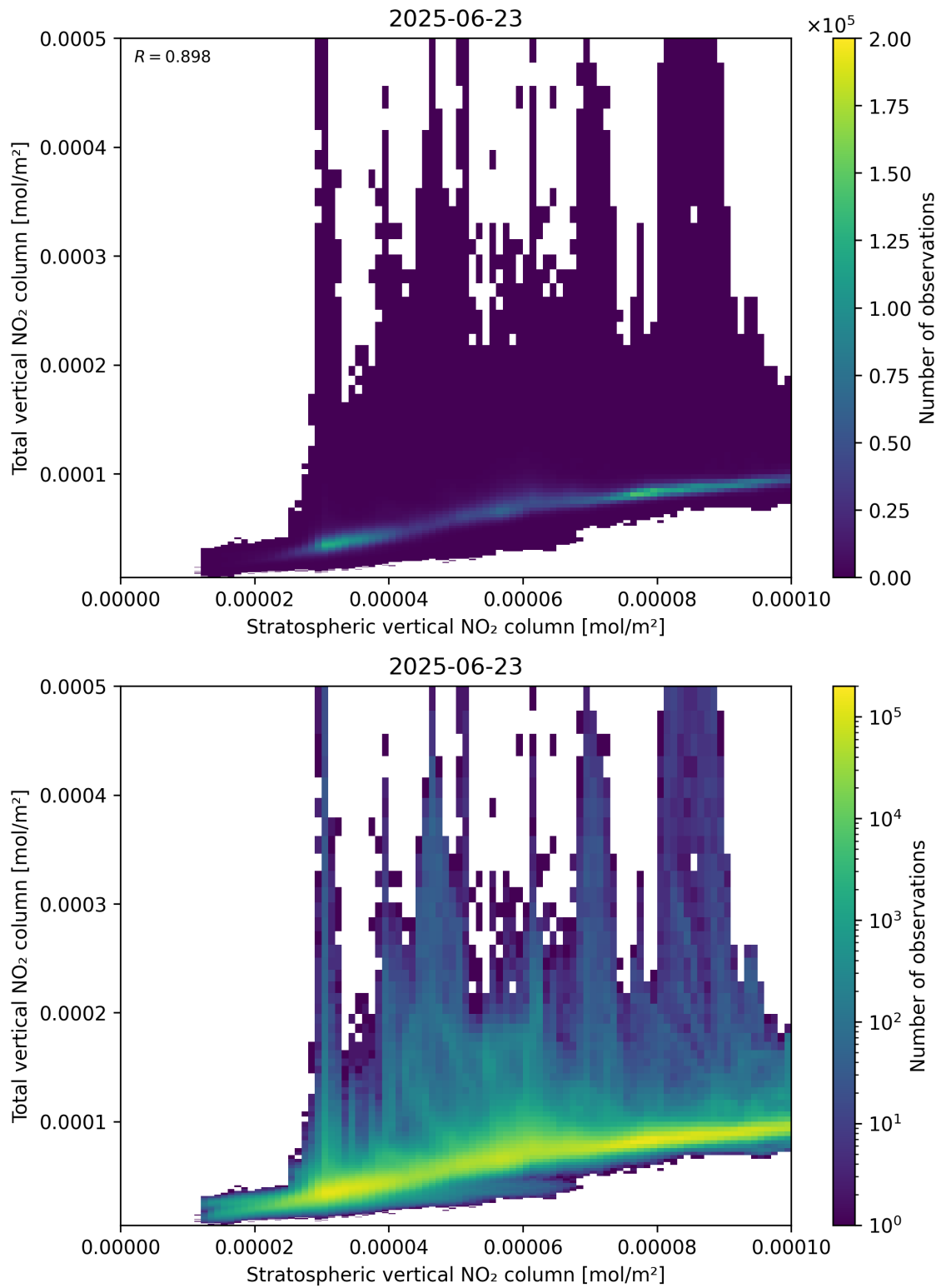
Figure 100: Scatter density plot of “Stratospheric vertical NO 2 column” against “Total vertical NO 2 column” for 2025-06-22 to 2025-06-24.
