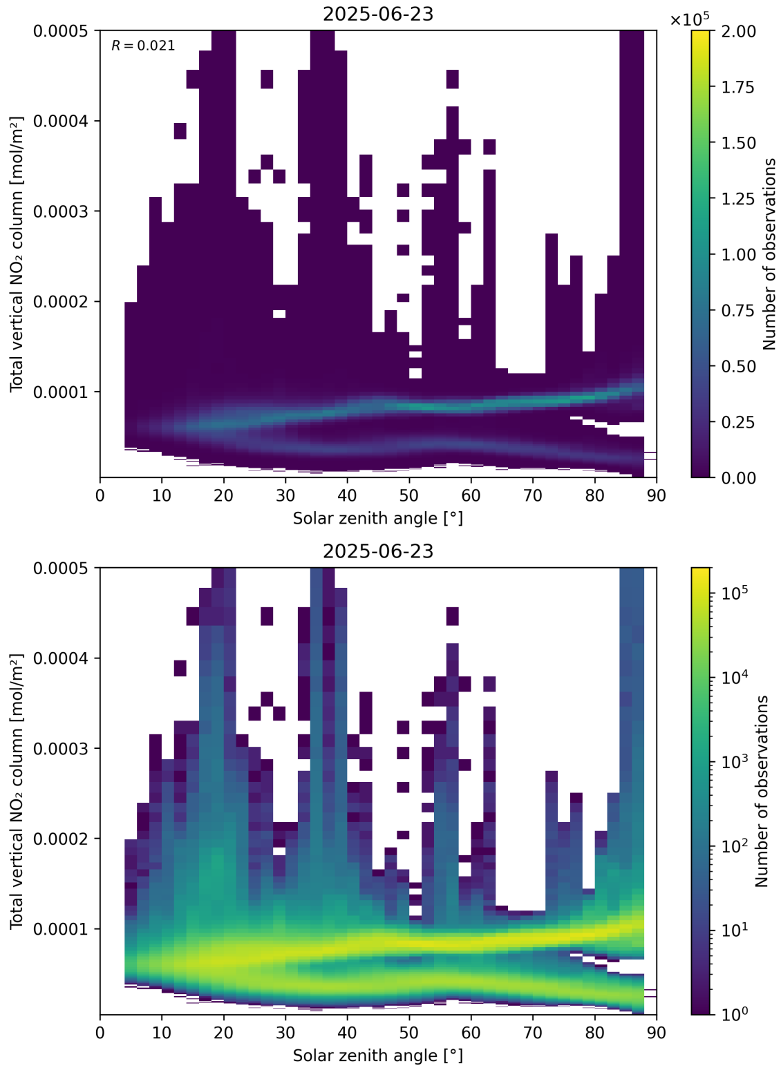
Figure 153: Scatter density plot of “Solar zenith angle” against “Total vertical NO 2 column” for 2025-06-22 to 2025-06-24.
