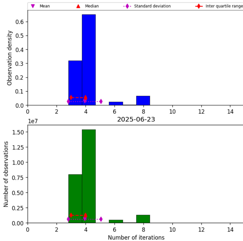
Figure 34: Histogram of “Number of iterations” for 2025-06-22 to 2025-06-24
