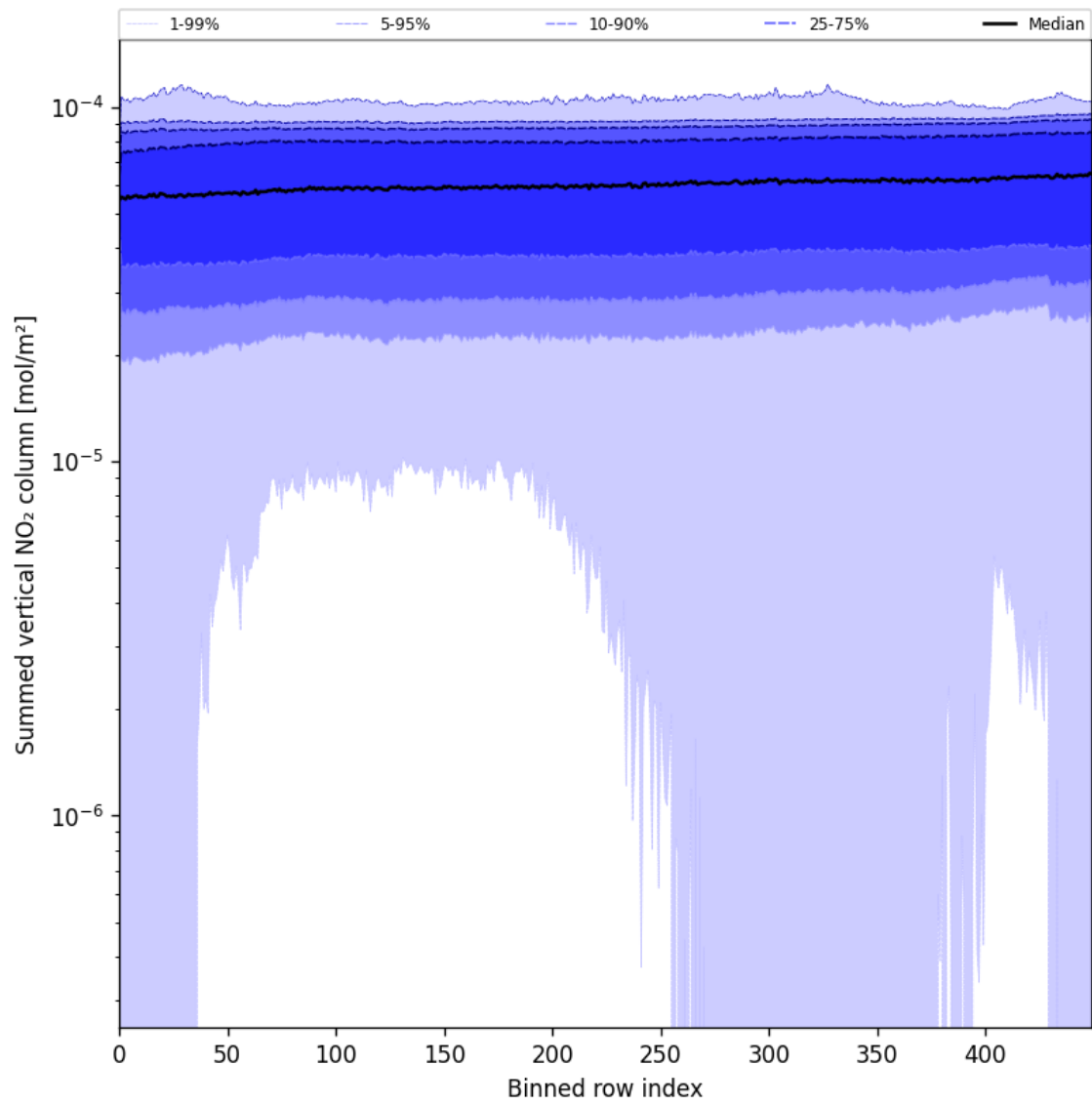
Figure 57: Along track statistics of “Summed vertical NO 2 column” for 2025-06-22 to 2025-06-24
