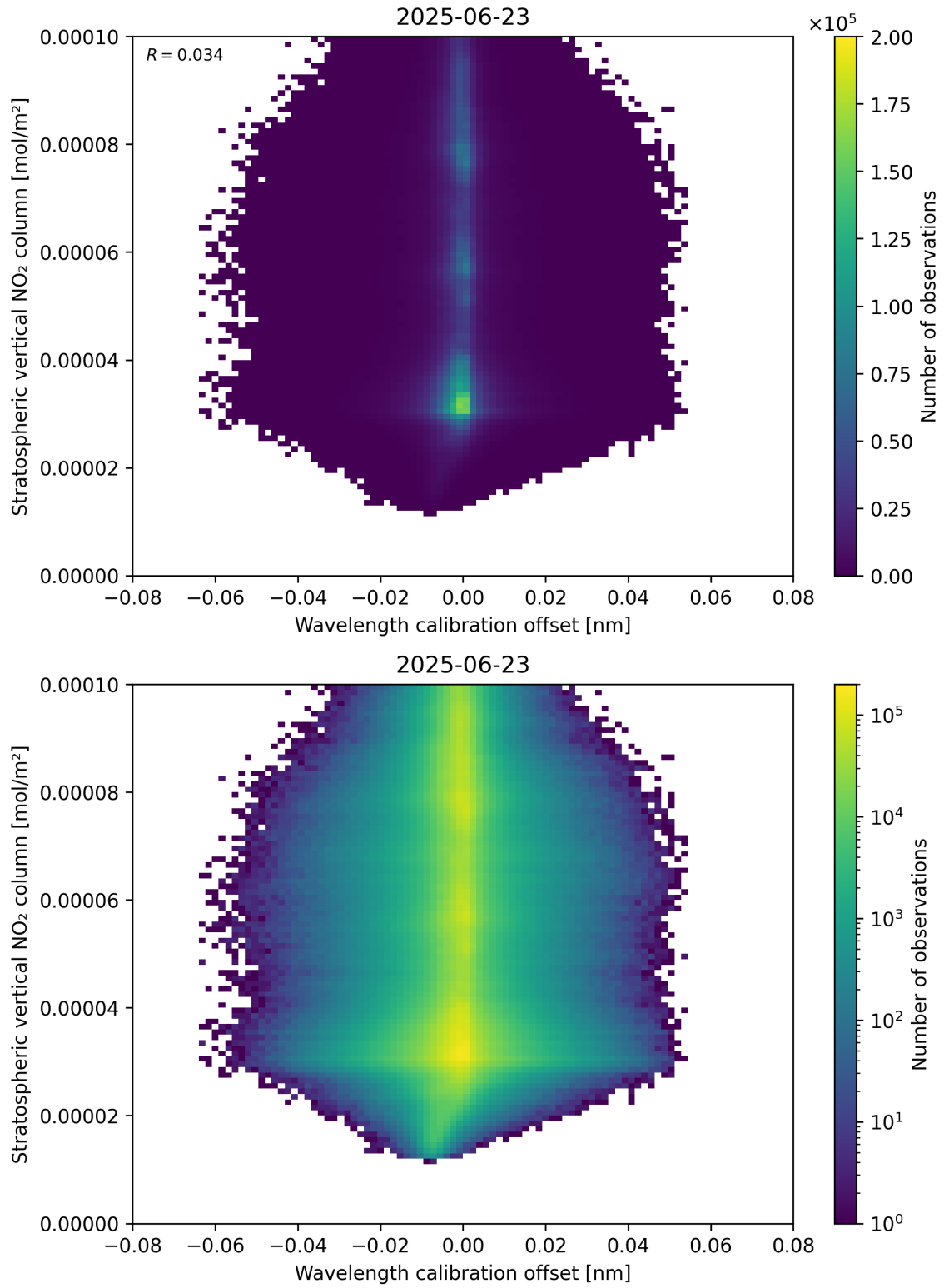
Figure 176: Scatter density plot of “Wavelength calibration offset” against “Stratospheric vertical NO 2 column” for 2025-06-22 to 2025-06-24.
