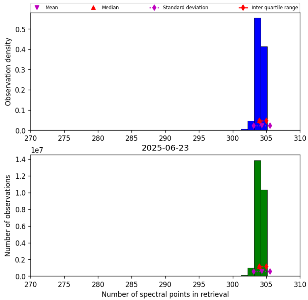
Figure 33: Histogram of “Number of spectral points in retrieval” for 2025-06-22 to 2025-06-24
