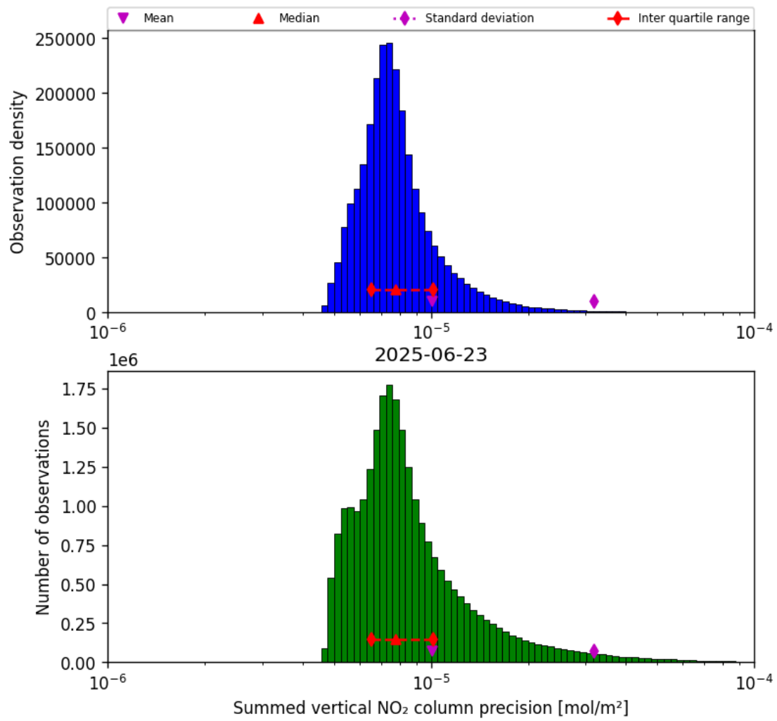
Figure 41: Histogram of “Summed vertical NO 2 column precision” for 2025-06-22 to 2025-06-24
