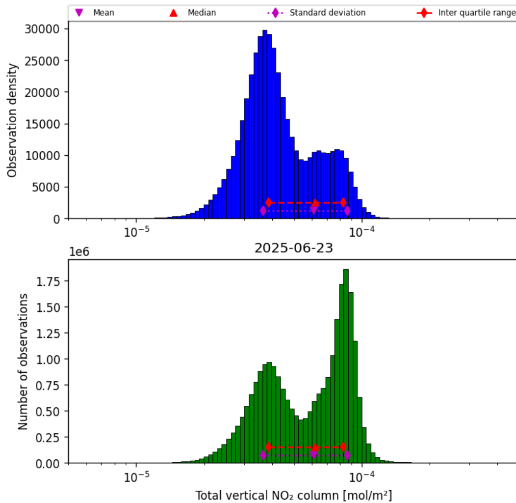
Figure 38: Histogram of “Total vertical NO 2 column” for 2025-06-22 to 2025-06-24
