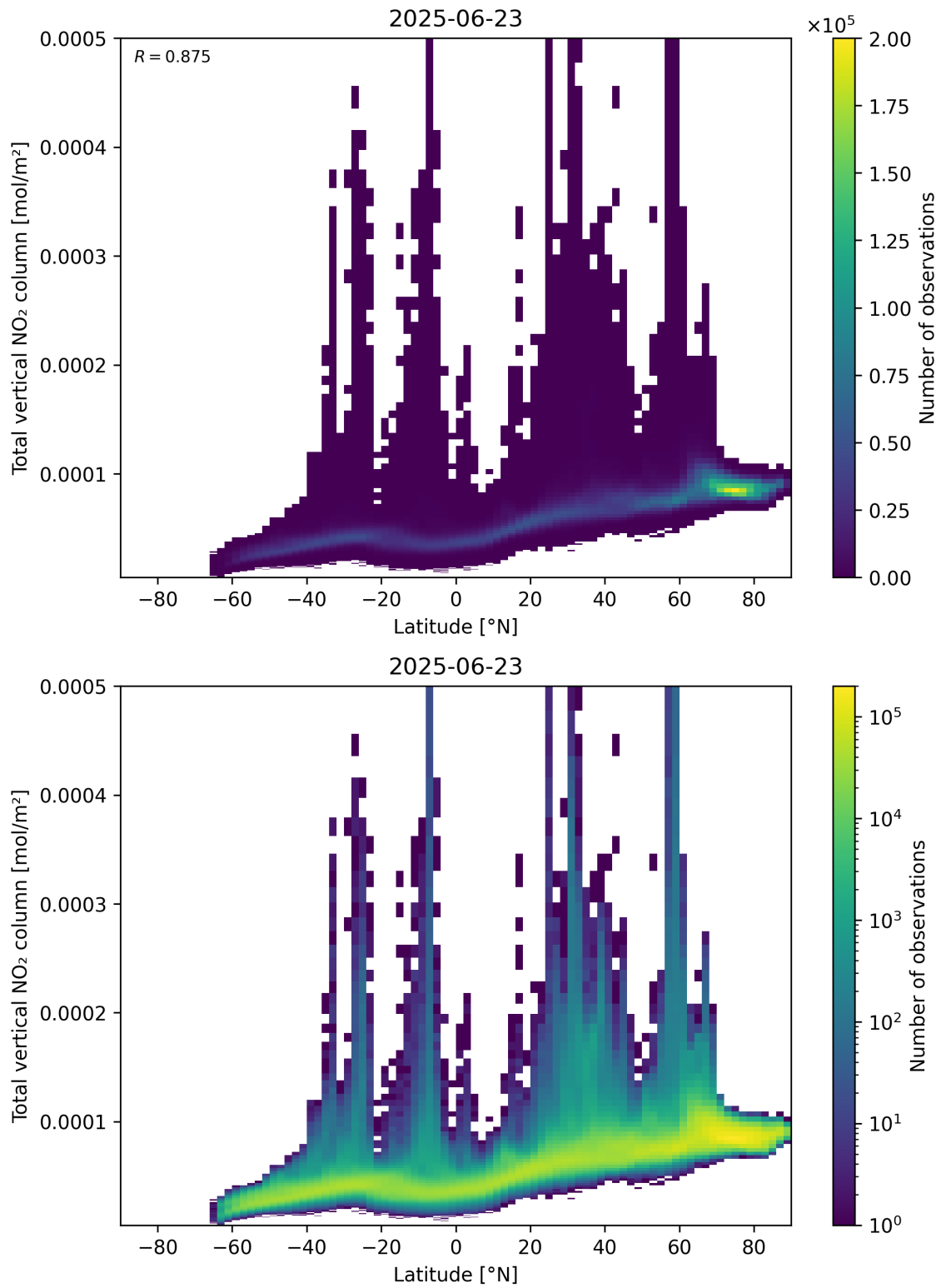
Figure 90: Scatter density plot of “Latitude” against “Total vertical NO 2 column” for 2025-06-22 to 2025-06-24.
