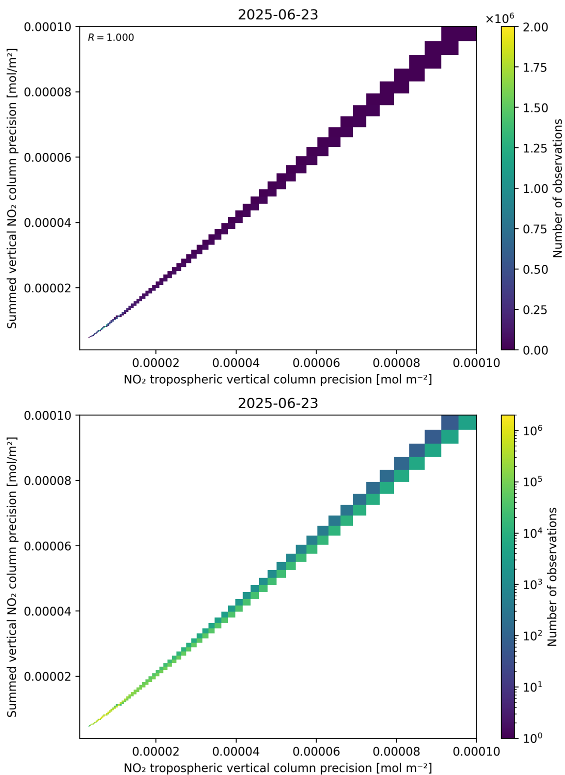
Figure 137: Scatter density plot of “NO 2 tropospheric vertical column precision” against “Summed vertical NO 2 column precision” for 2025-06-22 to 2025-06-24.
