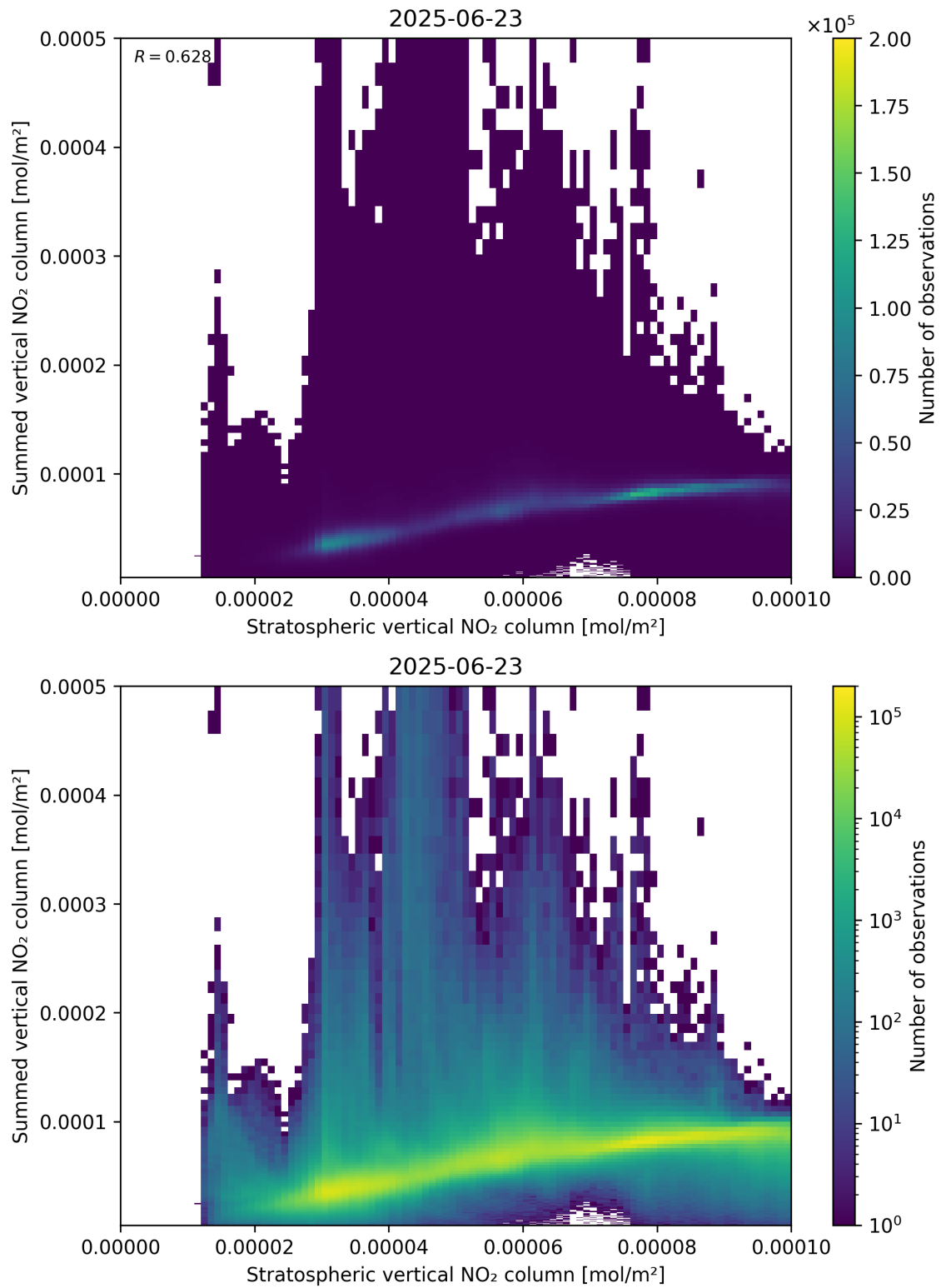
Figure 98: Scatter density plot of “Stratospheric vertical NO 2 column” against “Summed vertical NO 2 column” for 2025-06-22 to 2025-06-24.
