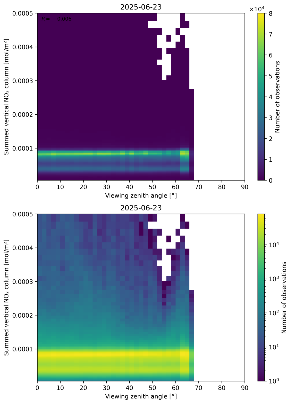
Figure 165: Scatter density plot of “Viewing zenith angle” against “Summed vertical NO 2 column” for 2025-06-22 to 2025-06-24.
