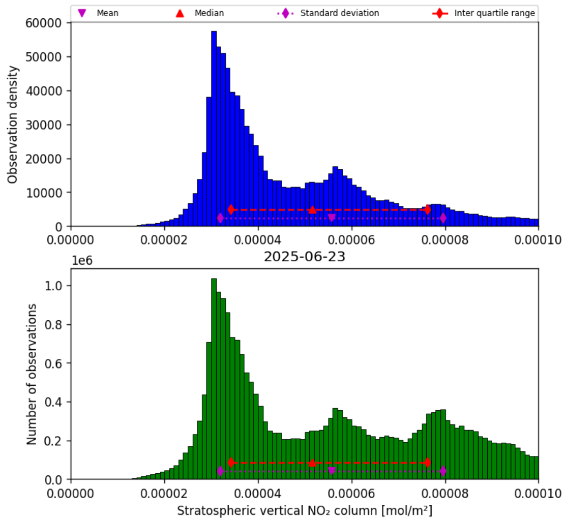
Figure 36: Histogram of “Stratospheric vertical NO 2 column” for 2025-06-22 to 2025-06-24
