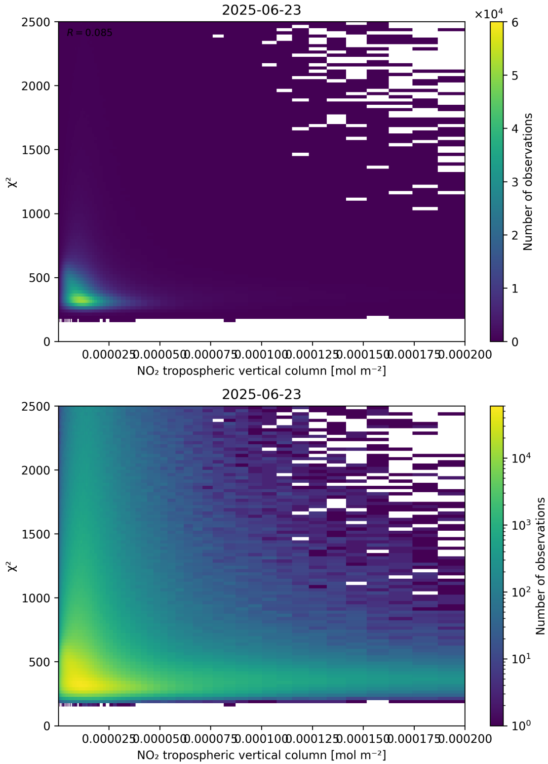
Figure 124: Scatter density plot of “NO 2 tropospheric vertical column” against “ \chi^2 ” for 2025-06-22 to 2025-06-24.
