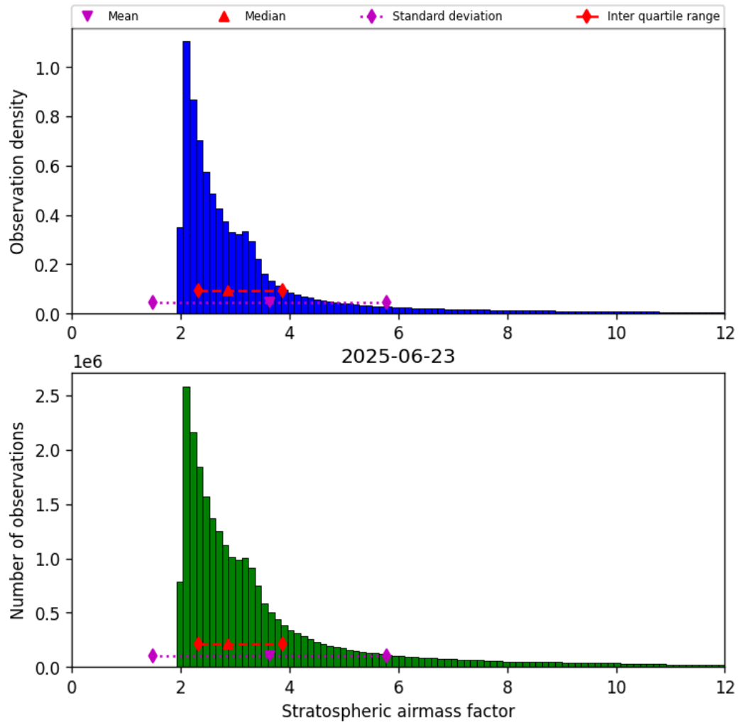
Figure 44: Histogram of “Stratospheric airmass factor” for 2025-06-22 to 2025-06-24
