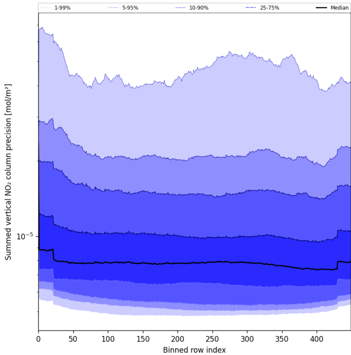
Figure 58: Along track statistics of “Summed vertical NO 2 column precision” for 2025-06-22 to 2025-06-24
