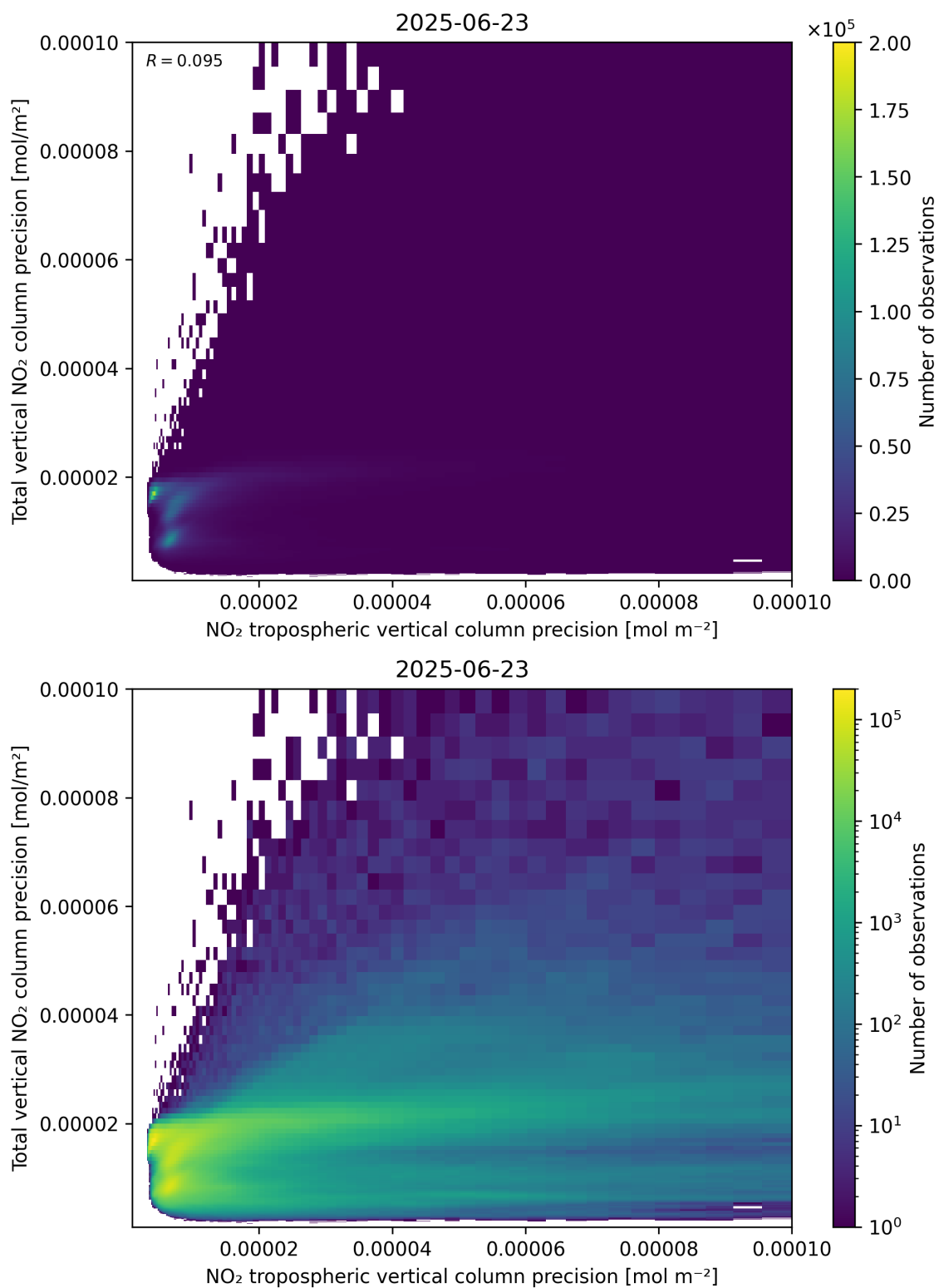
Figure 139: Scatter density plot of “NO 2 tropospheric vertical column precision” against “Total vertical NO 2 column precision” for 2025-06-22 to 2025-06-24.
