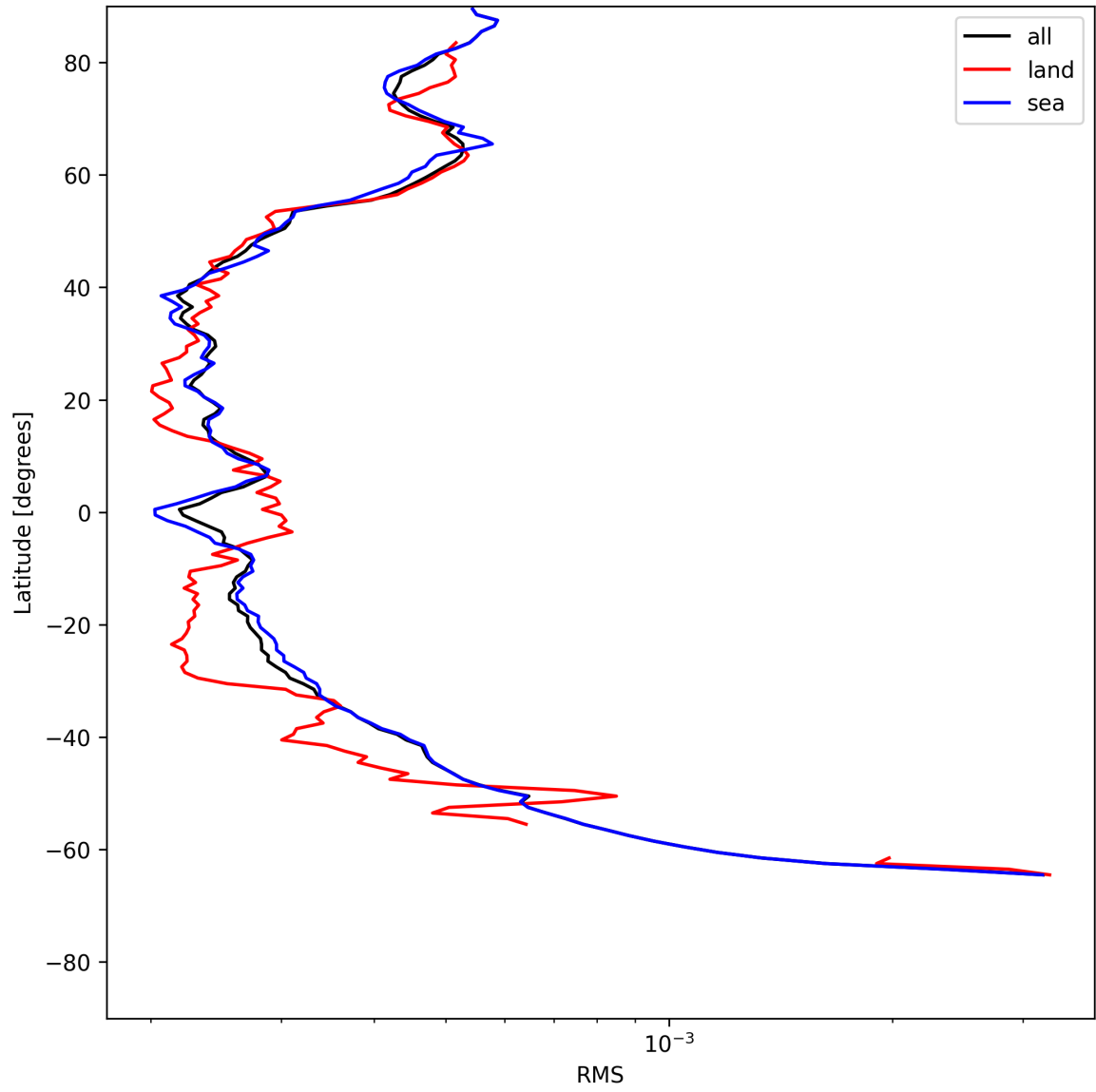
Figure 26: Zonal average of “RMS” for 2025-06-22 to 2025-06-24.
