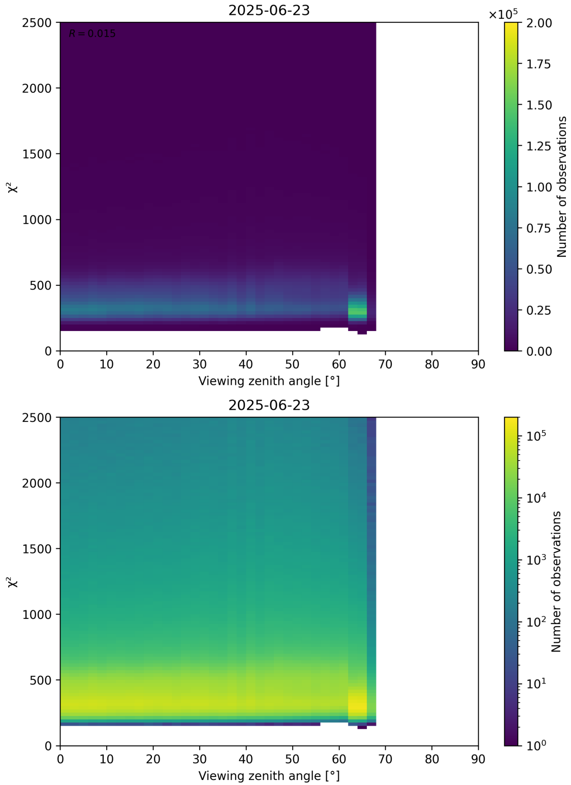
Figure 162: Scatter density plot of “Viewing zenith angle” against “ \chi^2 ” for 2025-06-22 to 2025-06-24.
