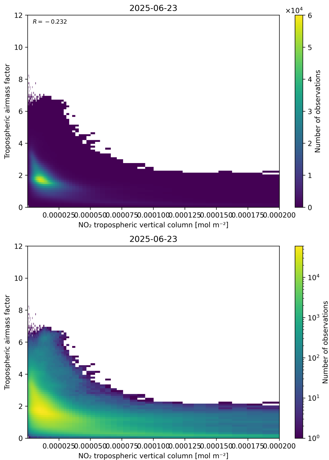
Figure 123: Scatter density plot of “NO 2 tropospheric vertical column” against “Tropospheric air mass factor” for 2025-06-22 to 2025-06-24.
