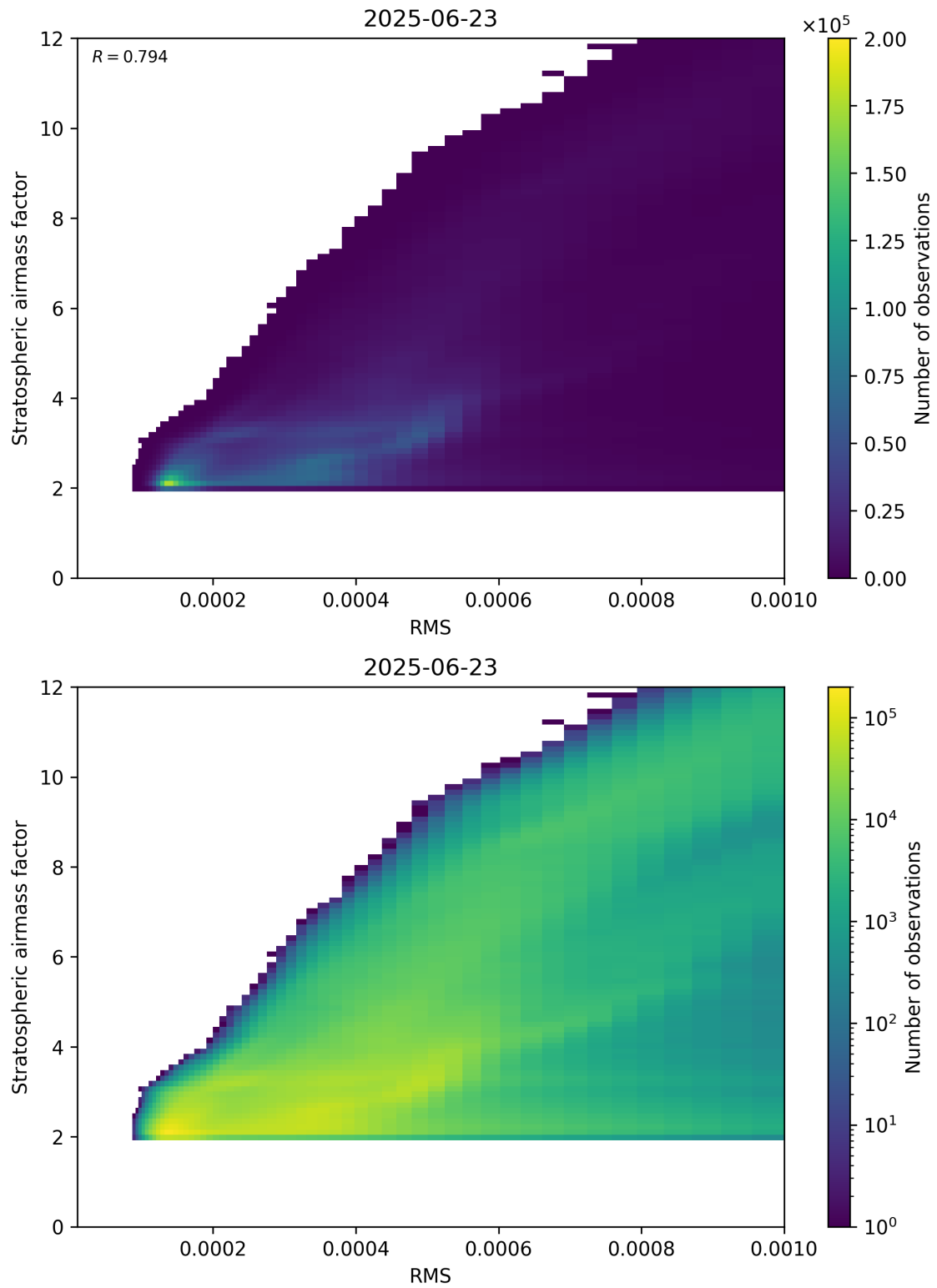
Figure 144: Scatter density plot of “RMS” against “Stratospheric airmass factor” for 2025-06-22 to 2025-06-24.
