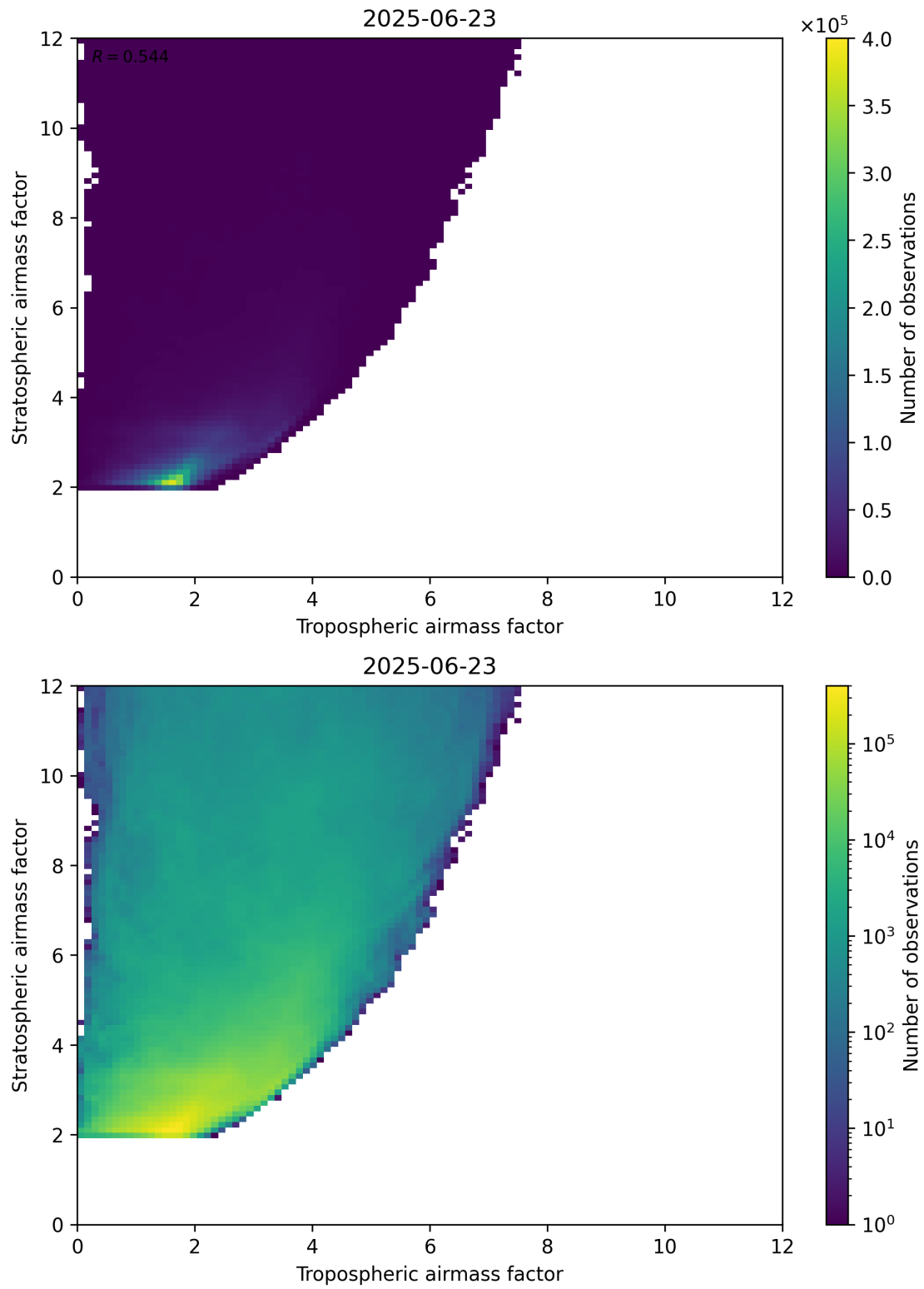
Figure 71: Scatter density plot of “Tropospheric airmass factor” against “Stratospheric airmass factor” for 2025-06-22 to 2025-06-24.
