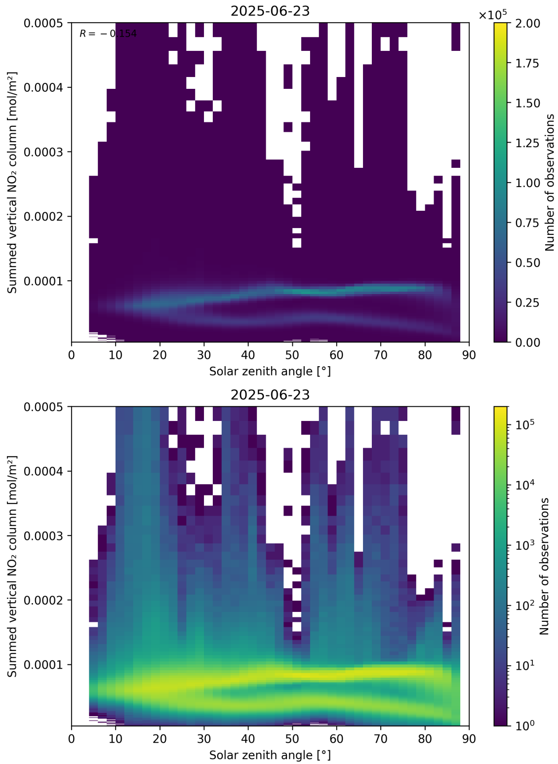
Figure 151: Scatter density plot of “Solar zenith angle” against “Summed vertical NO 2 column” for 2025-06-22 to 2025-06-24.
