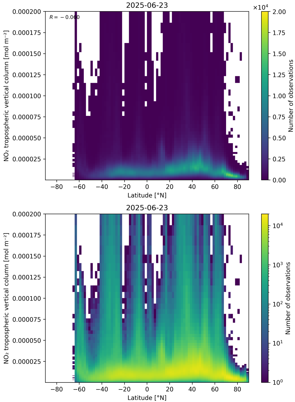
Figure 92: Scatter density plot of “Latitude” against “NO 2 tropospheric vertical column” for 2025-06-22 to 2025-06-24.
