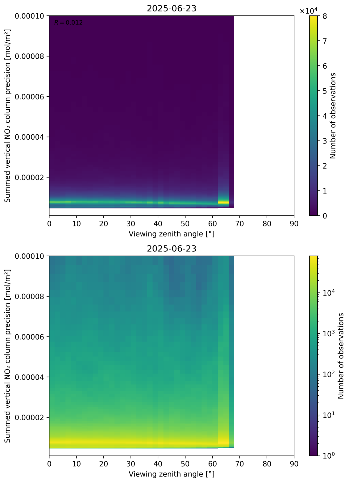
Figure 166: Scatter density plot of “Viewing zenith angle” against “Summed vertical NO 2 column precision” for 2025-06-22 to 2025-06-24.
