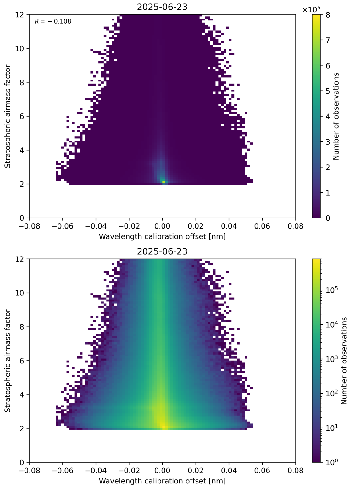
Figure 174: Scatter density plot of “Wavelength calibration offset” against “Stratospheric airmass factor” for 2025-06-22 to 2025-06-24.
