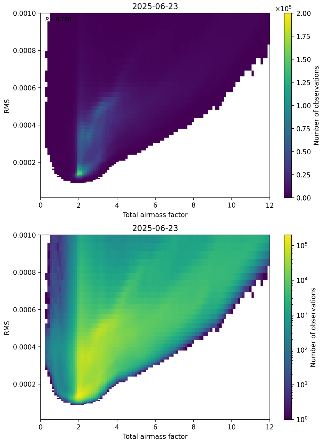
Figure 69: Scatter density plot of “Total airmass factor” against “RMS” for 2025-06-22 to 2025-06-24.
