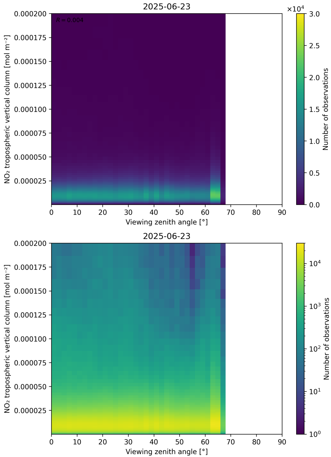
Figure 169: Scatter density plot of “Viewing zenith angle” against “NO 2 tropospheric vertical column” for 2025-06-22 to 2025-06-24.
