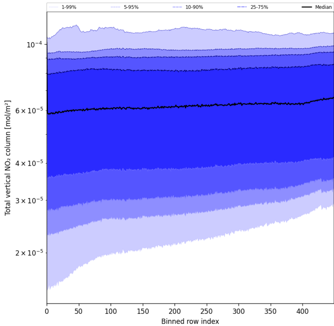
Figure 55: Along track statistics of “Total vertical NO 2 column” for 2025-06-22 to 2025-06-24
