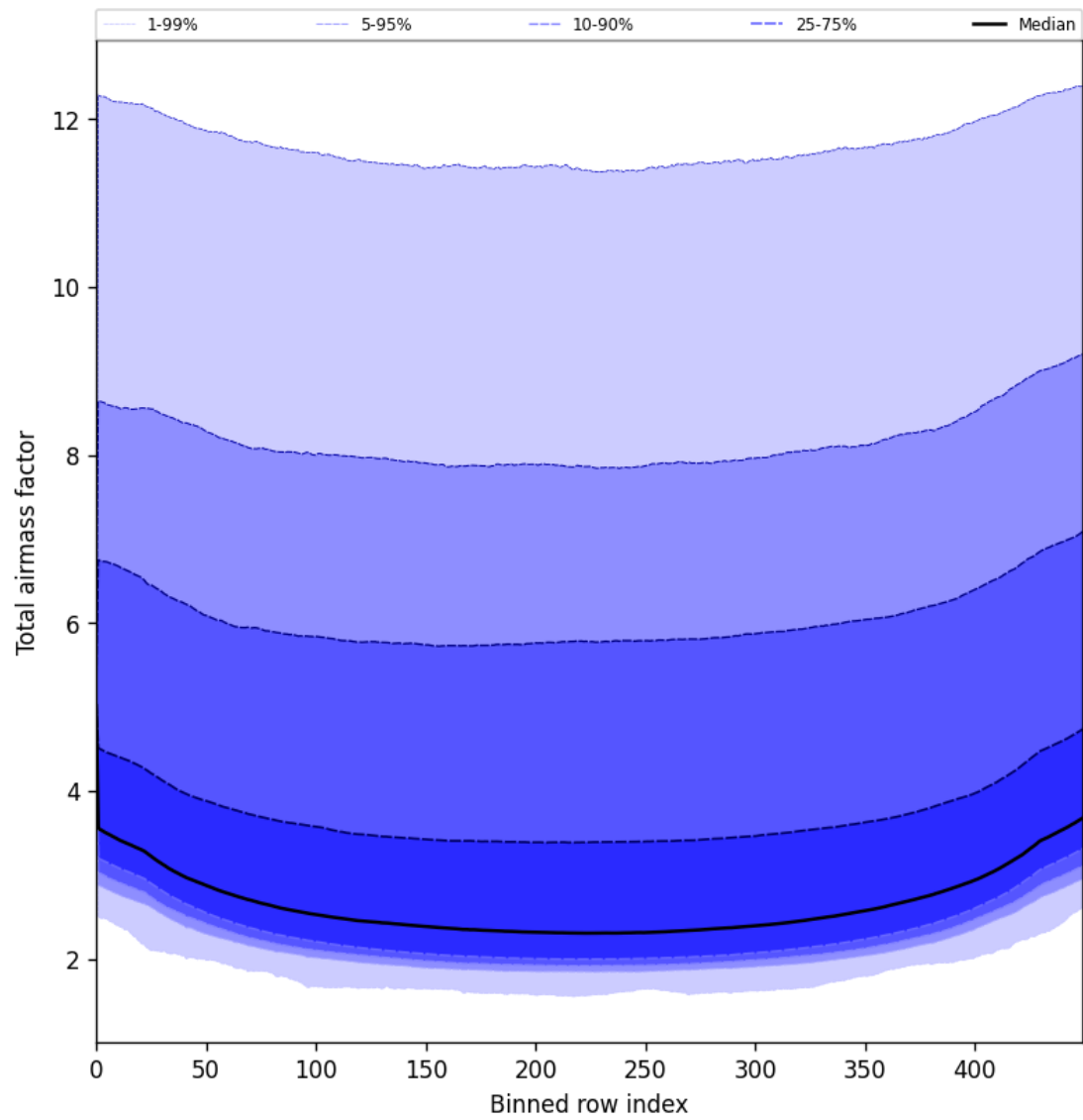
Figure 49: Along track statistics of “Total airmass factor” for 2025-06-22 to 2025-06-24
