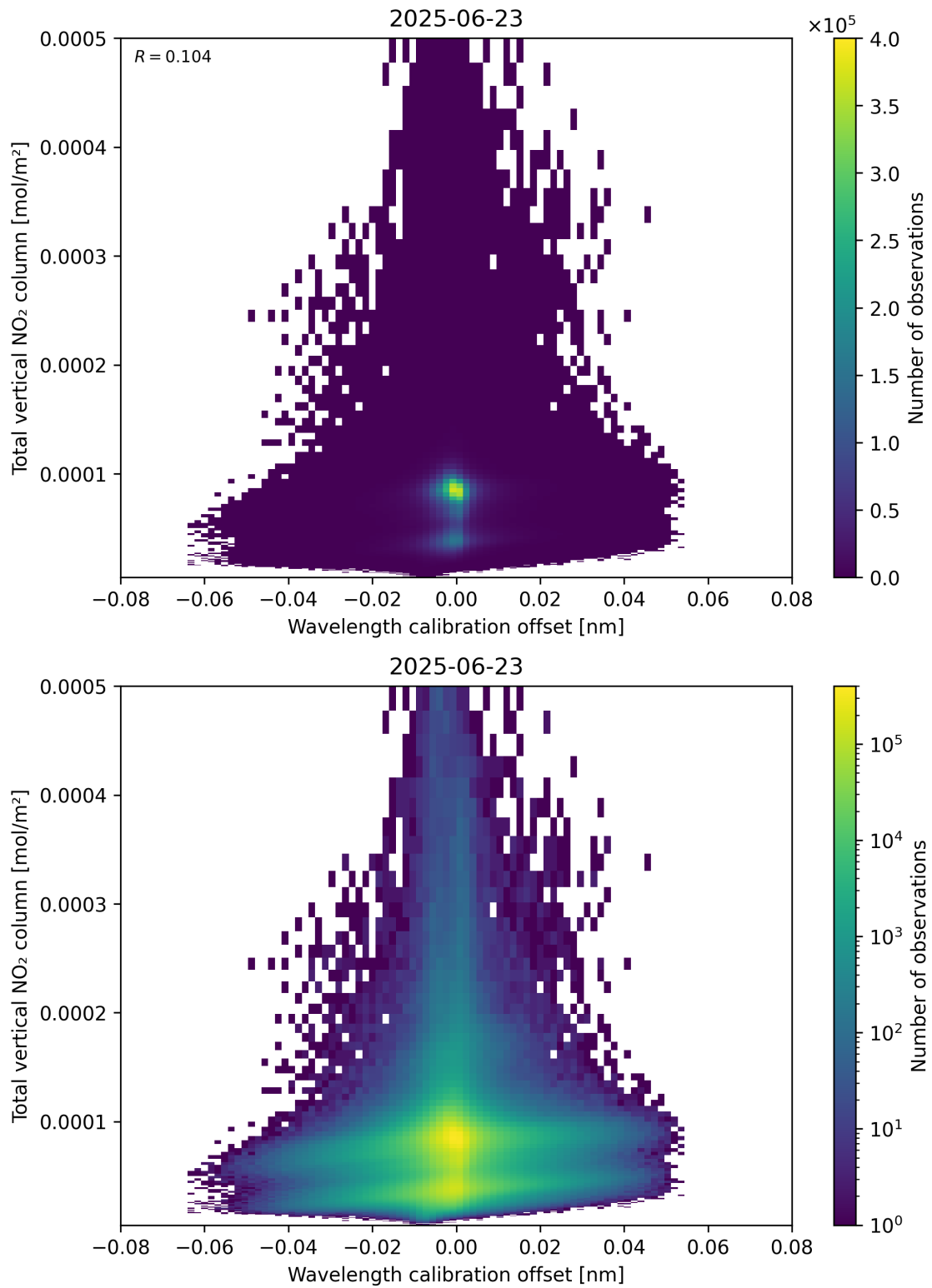
Figure 179: Scatter density plot of “Wavelength calibration offset” against “Total vertical NO 2 column” for 2025-06-22 to 2025-06-24.
