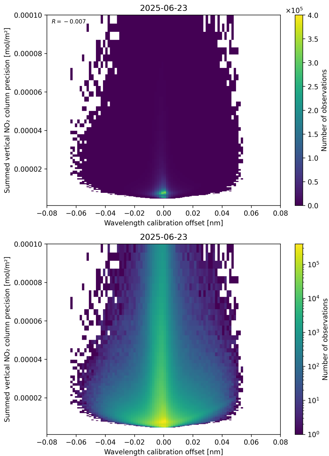
Figure 178: Scatter density plot of “Wavelength calibration offset” against “Summed vertical NO 2 column precision” for 2025-06-22 to 2025-06-24.
