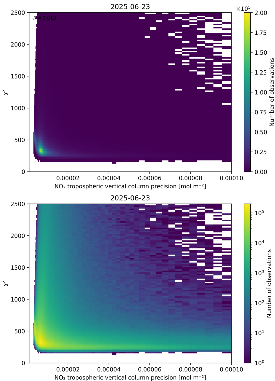
Figure 134: Scatter density plot of “NO 2 tropospheric vertical column precision” against “ \chi^2 ” for 2025-06-22 to 2025-06-24.
