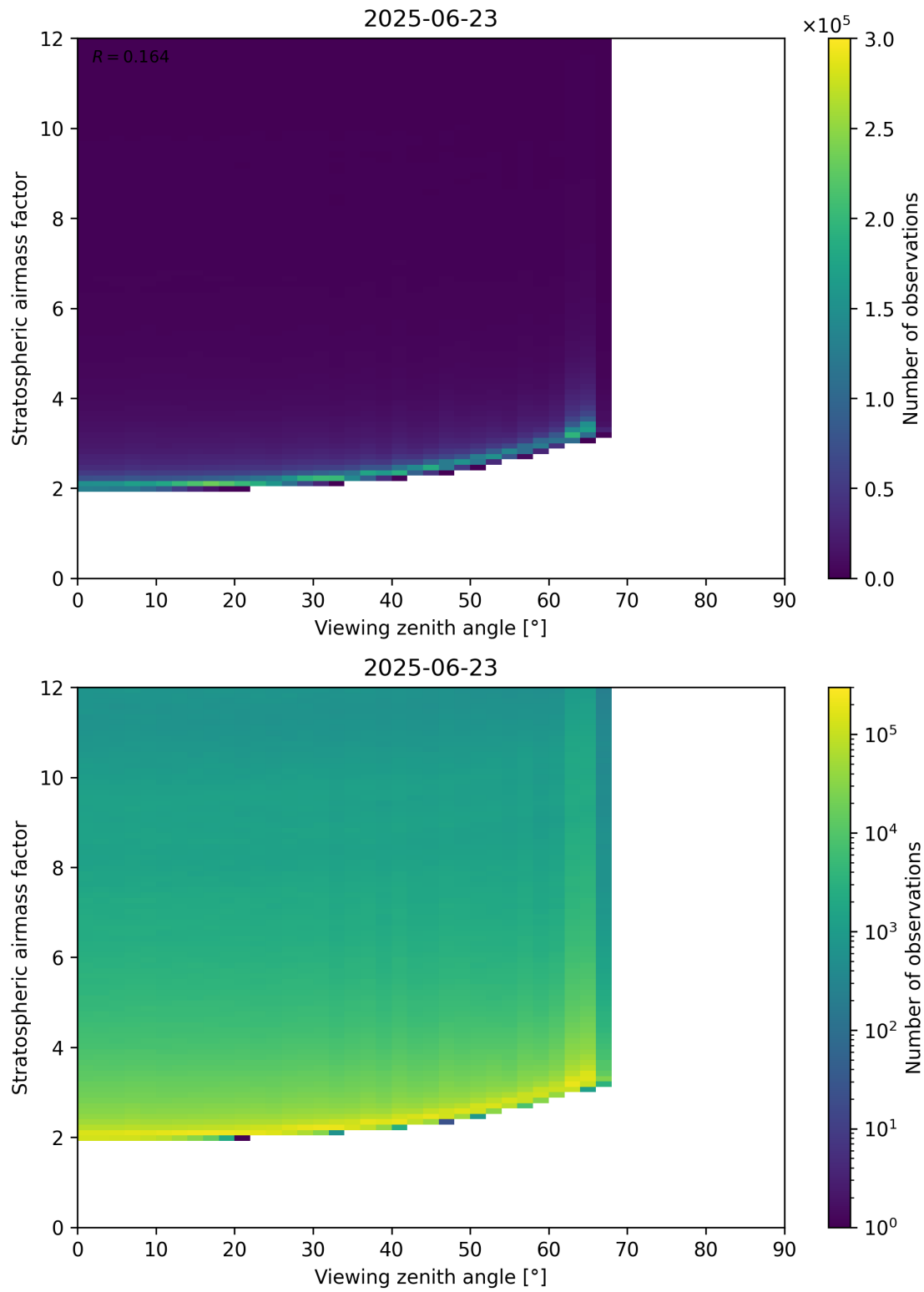
Figure 159: Scatter density plot of “Viewing zenith angle” against “Stratospheric airmass factor” for 2025-06-22 to 2025-06-24.
