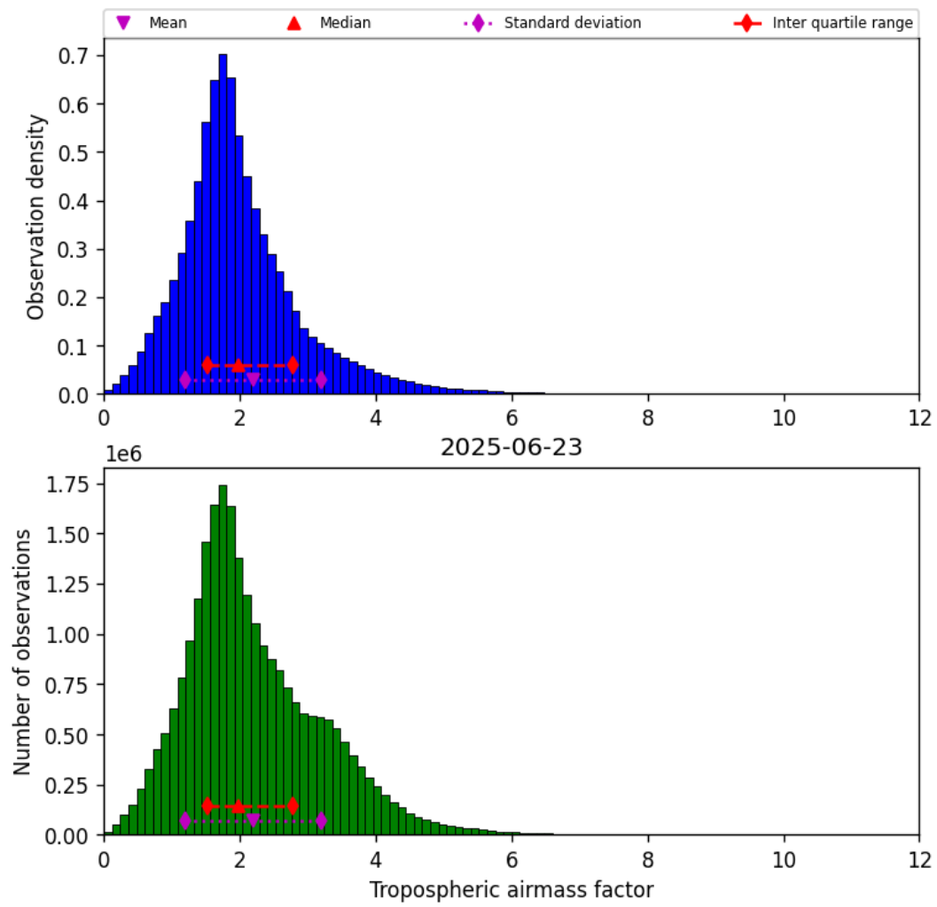
Figure 31: Histogram of “Tropospheric airmass factor” for 2025-06-22 to 2025-06-24
