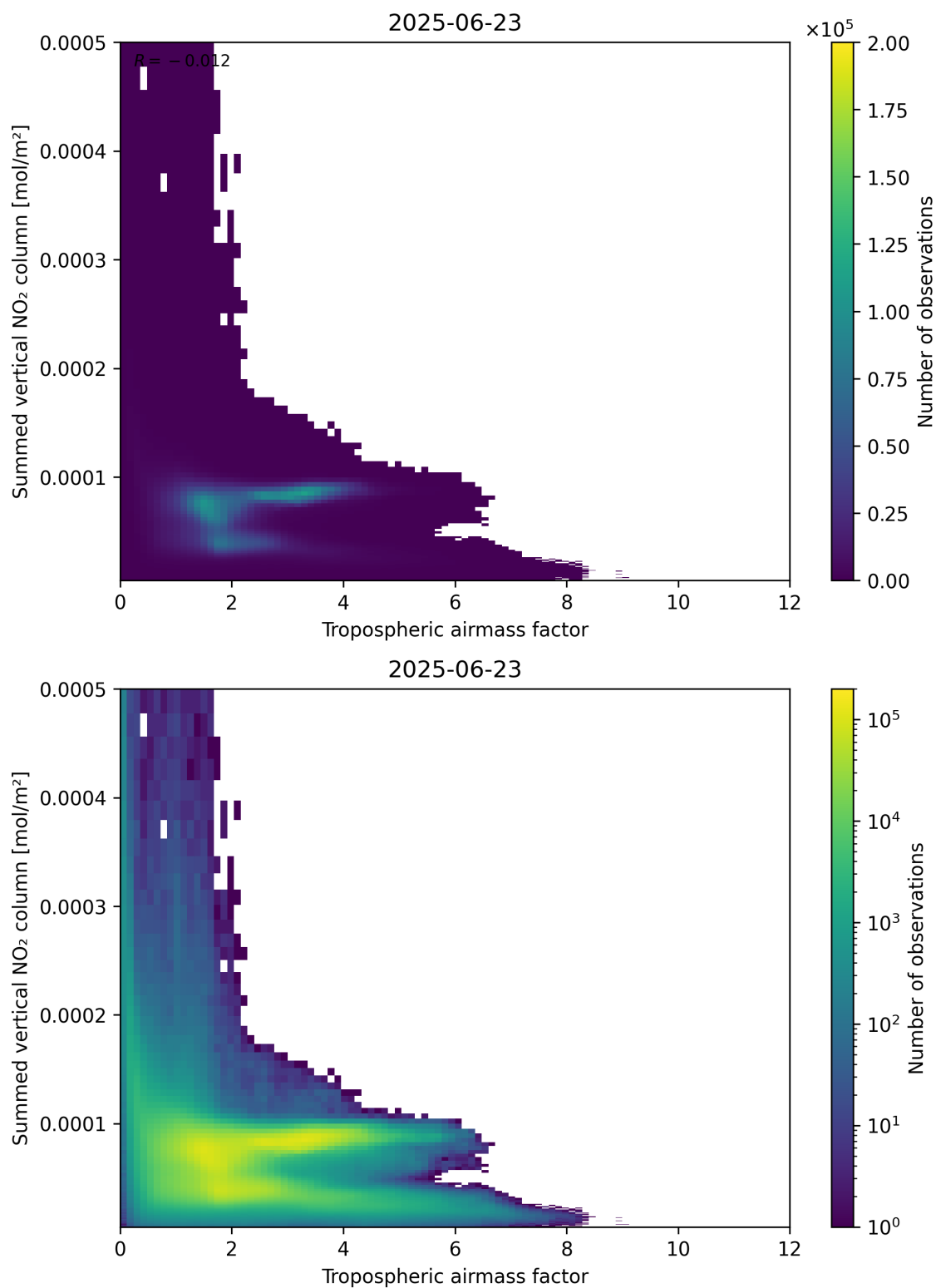
Figure 75: Scatter density plot of “Tropospheric air mass factor” against “Summed vertical NO 2 column” for 2025-06-22 to 2025-06-24.
