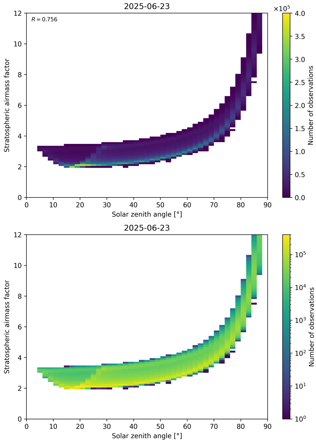
Figure 145: Scatter density plot of “Solar zenith angle” against “Stratospheric airmass factor” for 2025-06-22 to 2025-06-24.
