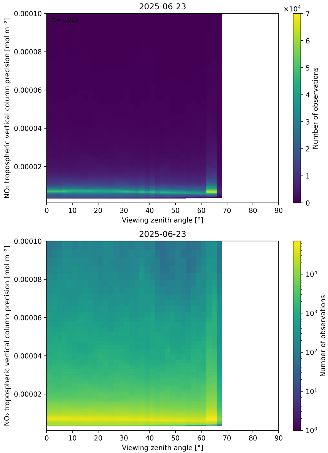
Figure 170: Scatter density plot of “Viewing zenith angle” against “NO 2 tropospheric vertical column precision” for 2025-06-22 to 2025-06-24.
