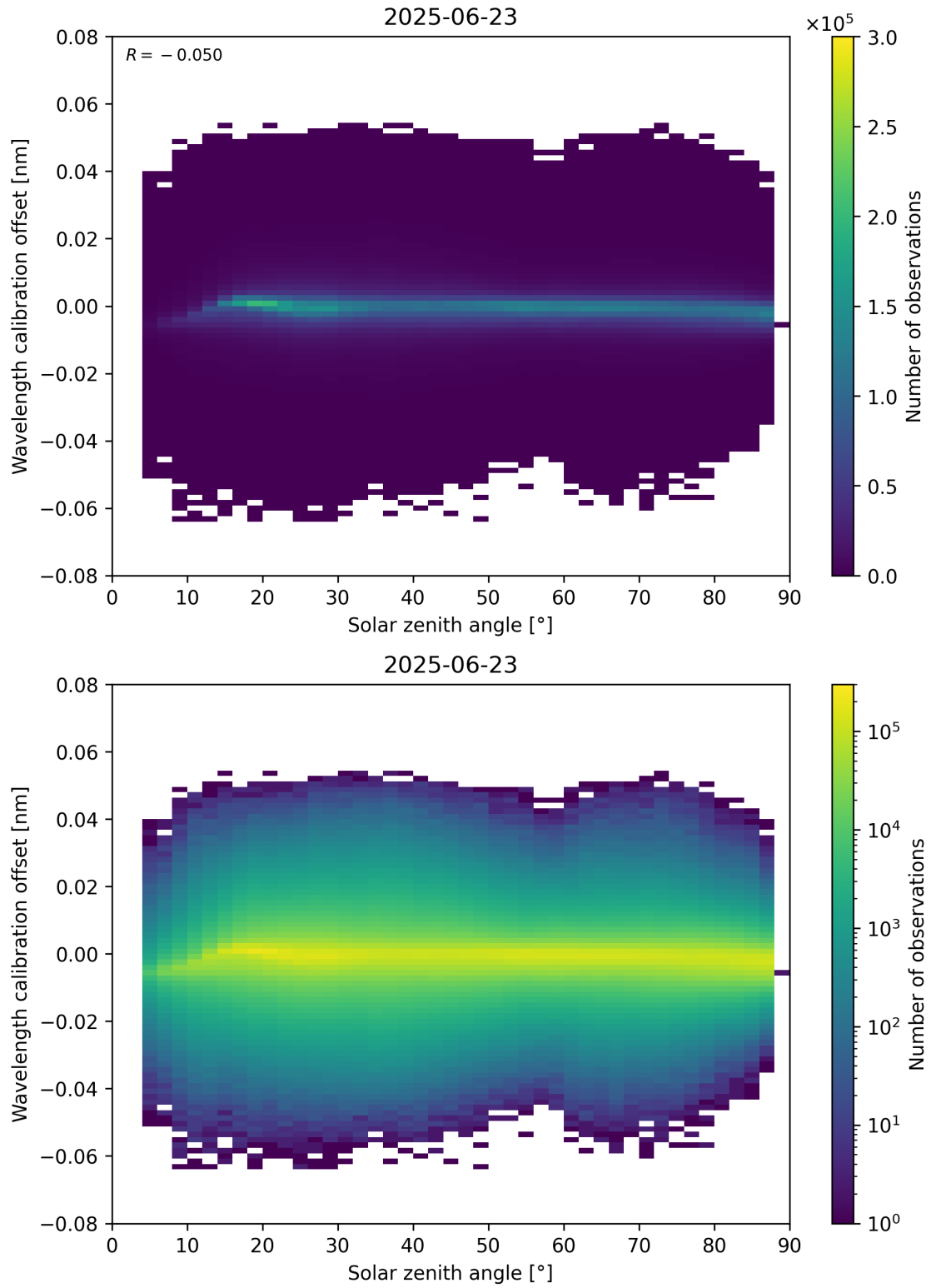
Figure 158: Scatter density plot of “Solar zenith angle” against “Wavelength calibration offset” for 2025-06-22 to 2025-06-24.
