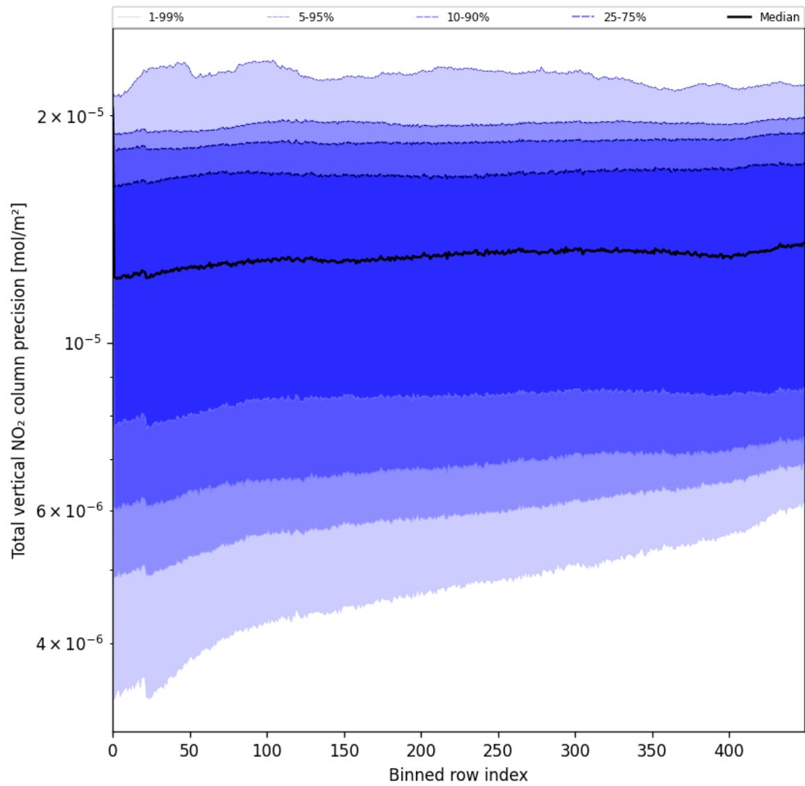
Figure 56: Along track statistics of "Total vertical NO 2 column precision" for 2025-06-22 to 2025-06-24
