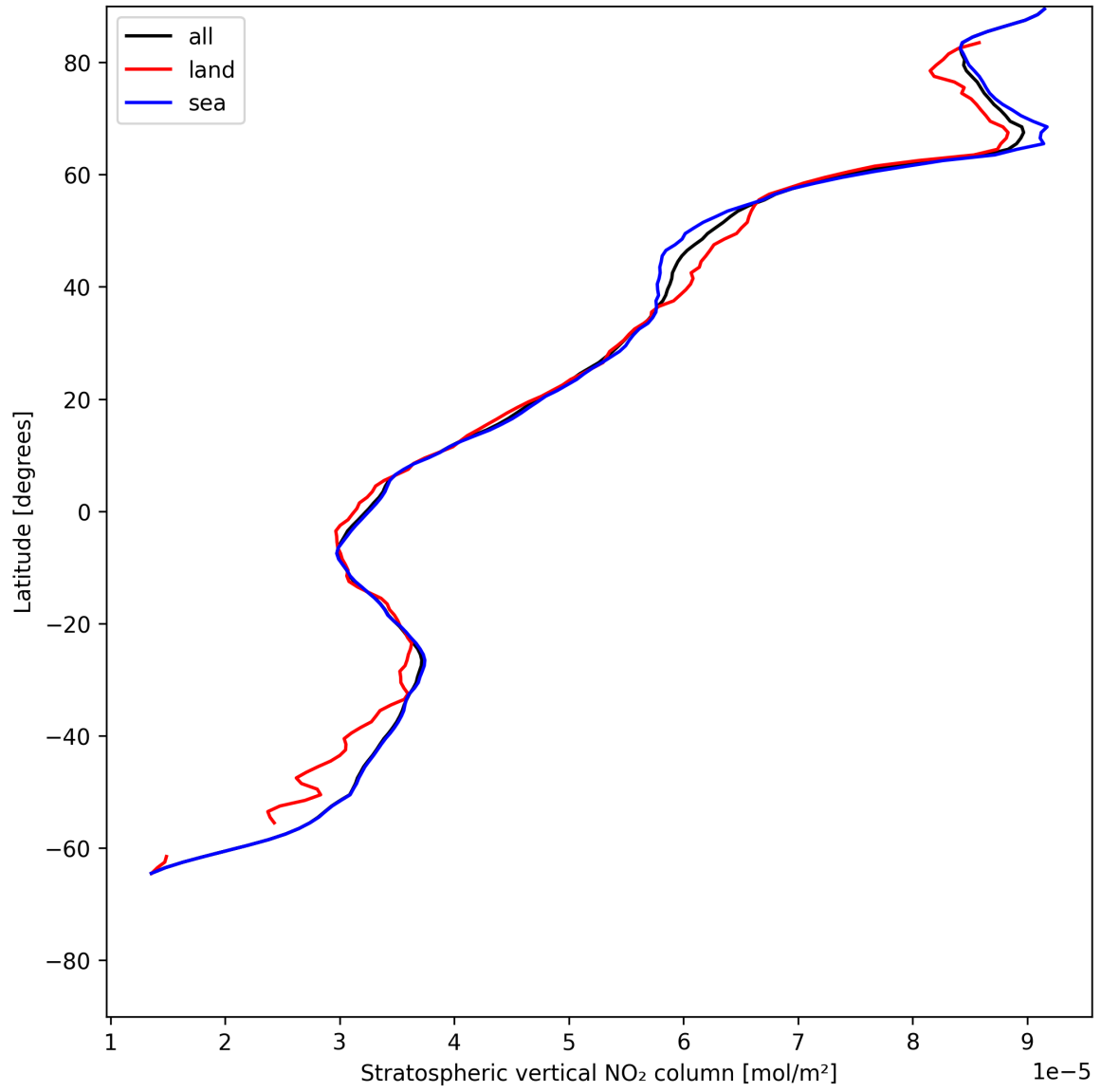
Figure 19: Zonal average of “Stratospheric vertical NO 2 column” for 2025-06-22 to 2025-06-24.
