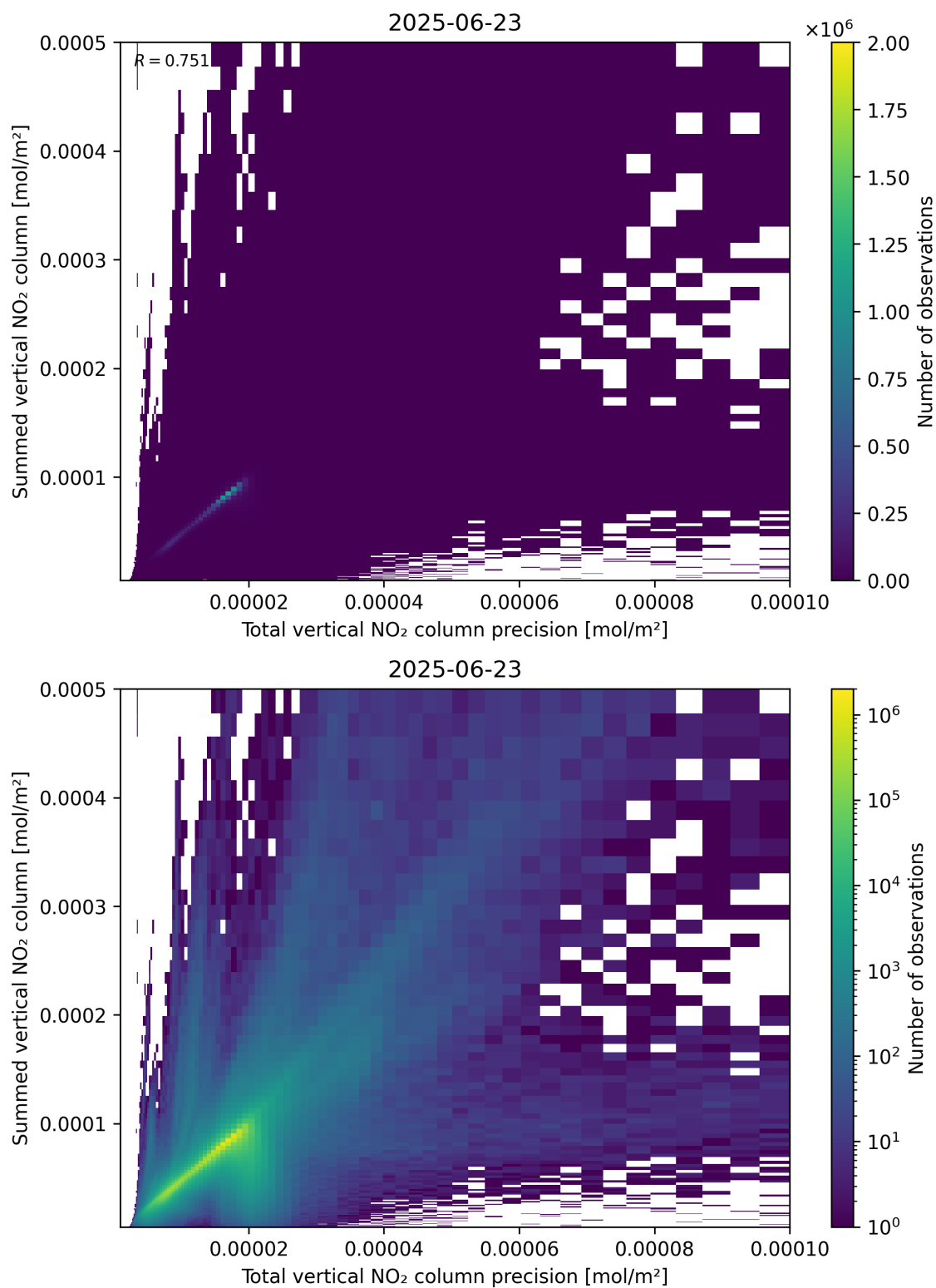
Figure 117: Scatter density plot of “Total vertical NO 2 column precision” against “Summed vertical NO 2 column” for 2025-06-22 to 2025-06-24.
