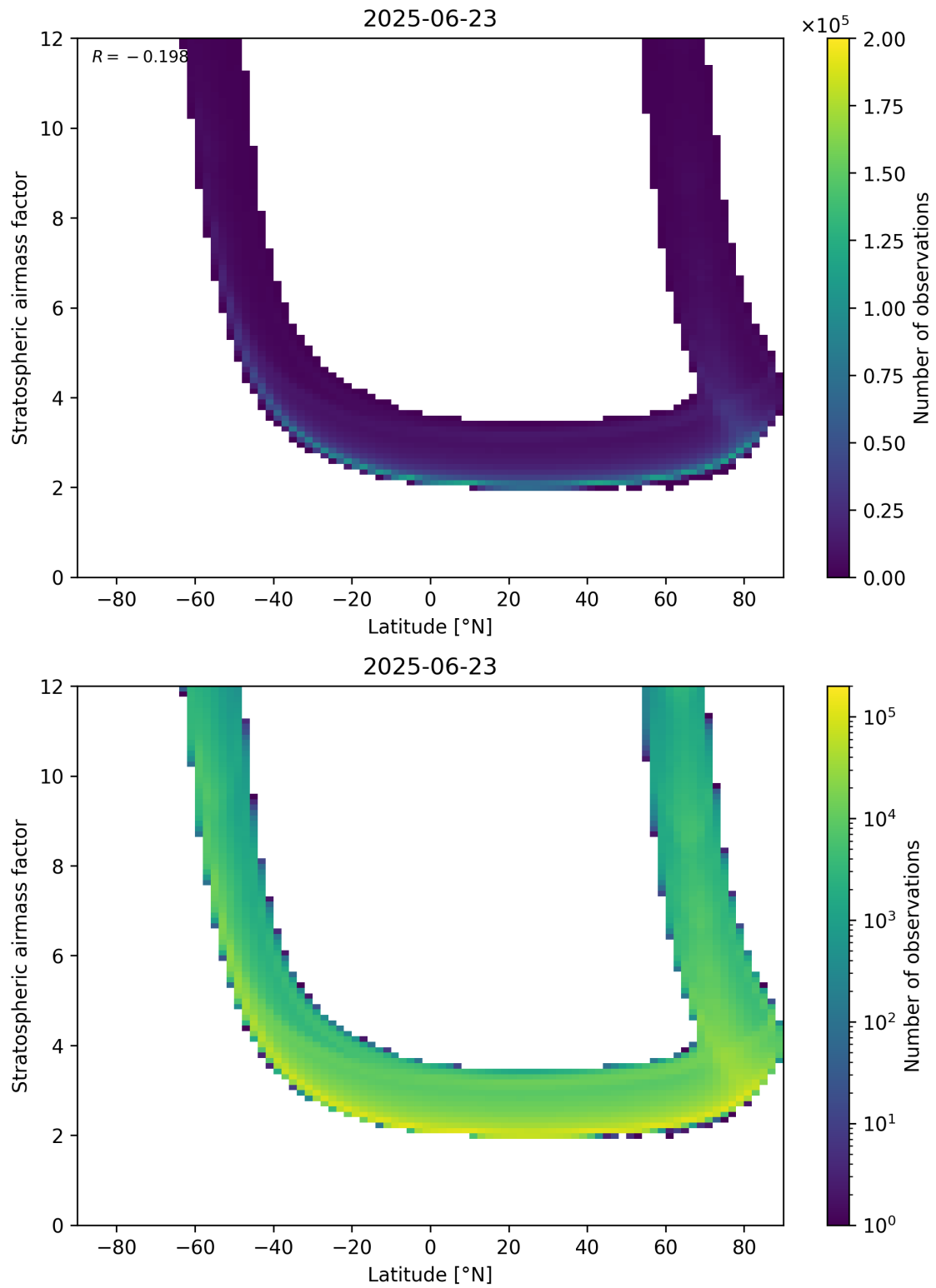
Figure 83: Scatter density plot of “Latitude” against “Stratospheric air mass factor” for 2025-06-22 to 2025-06-24.
