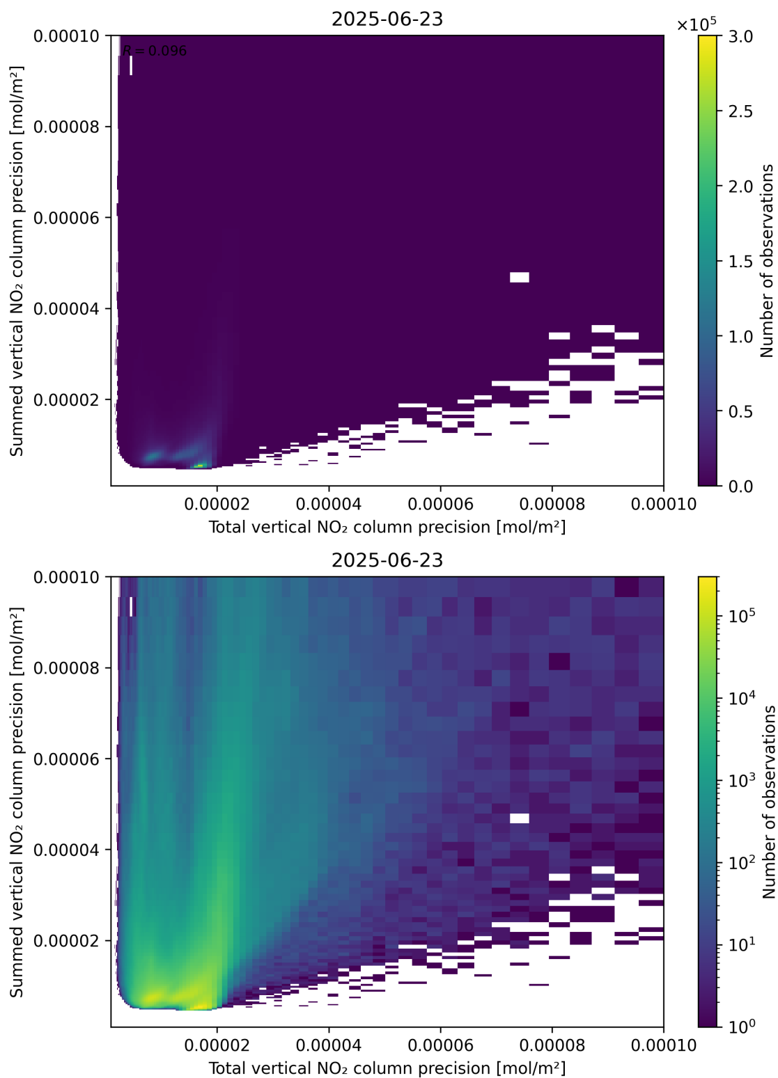
Figure 118: Scatter density plot of “Total vertical NO 2 column precision” against “Summed vertical NO 2 column precision” for 2025-06-22 to 2025-06-24.
