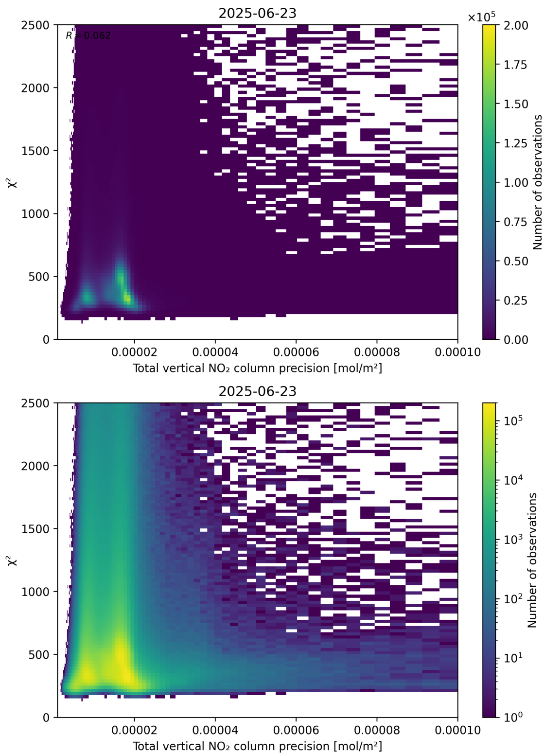
Figure 116: Scatter density plot of “Total vertical NO 2 column precision” against “ \chi^2 ” for 2025-06-22 to 2025-06-24.
