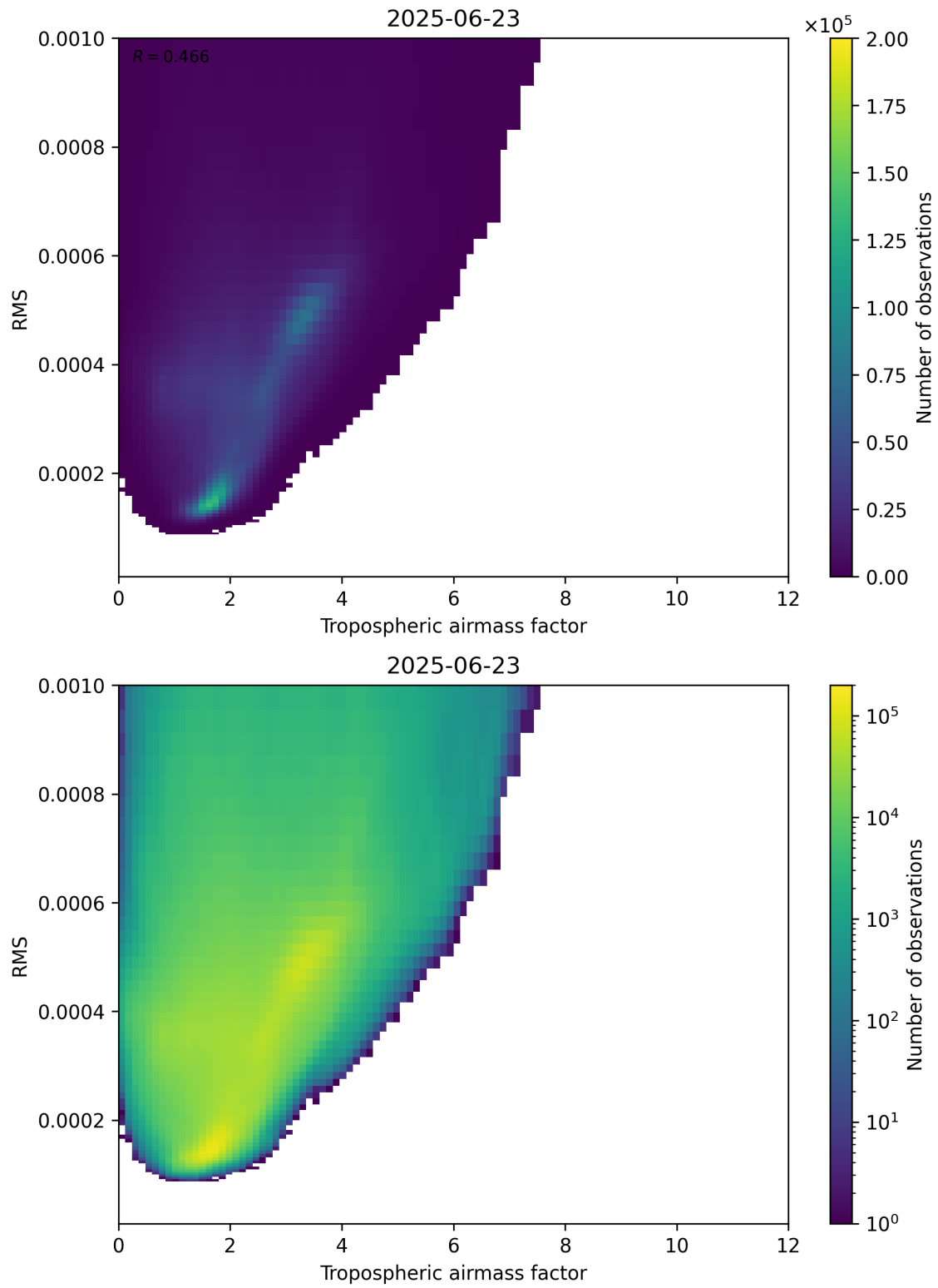
Figure 79: Scatter density plot of “Tropospheric airmass factor” against “RMS” for 2025-06-22 to 2025-06-24.
