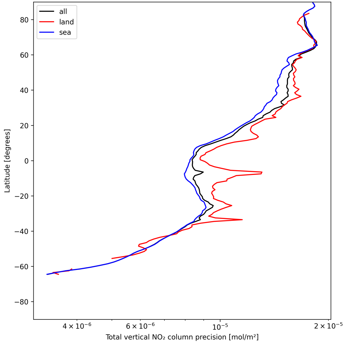
Figure 22: Zonal average of “Total vertical NO 2 column precision” for 2025-06-22 to 2025-06-24.
