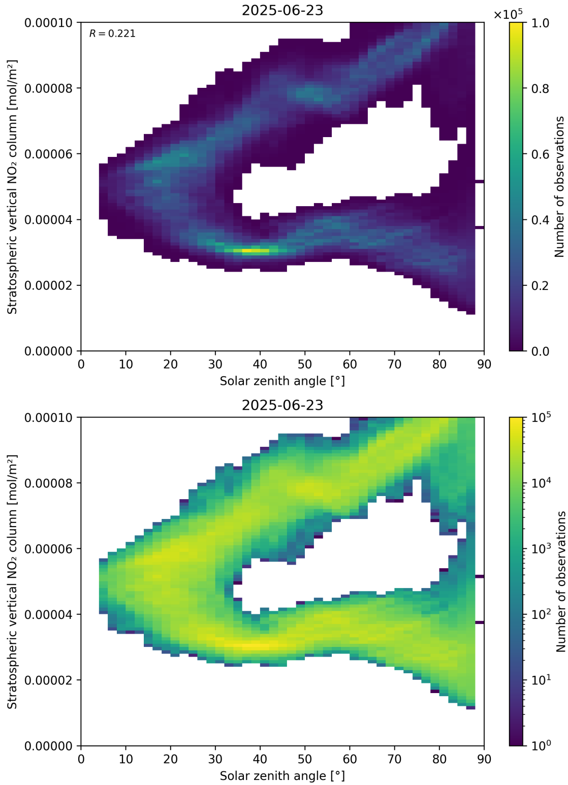
Figure 150: Scatter density plot of “Solar zenith angle” against “Stratospheric vertical NO 2 column” for 2025-06-22 to 2025-06-24.
