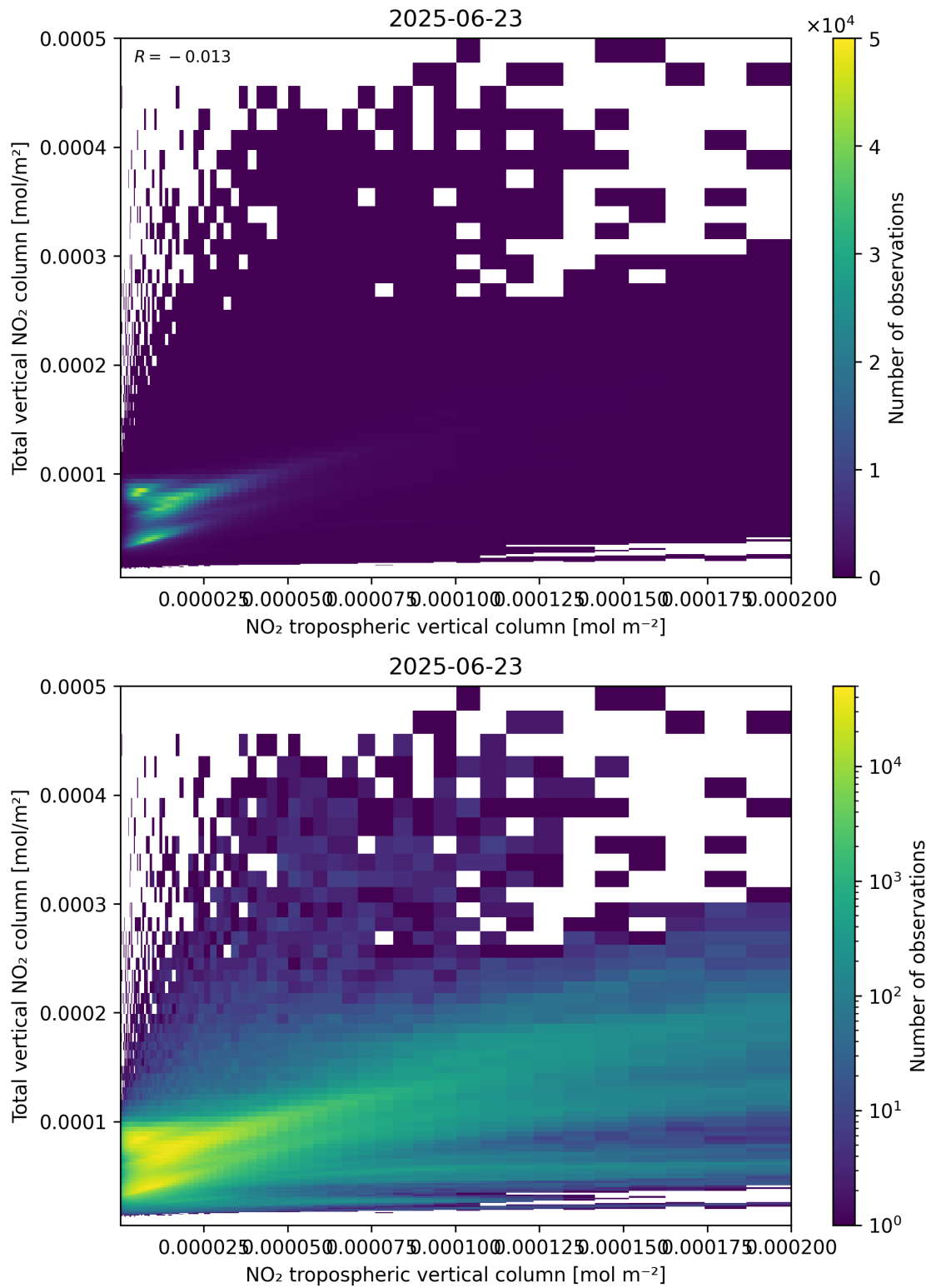
Figure 128: Scatter density plot of “NO 2 tropospheric vertical column” against “Total vertical NO 2 column” for 2025-06-22 to 2025-06-24.
