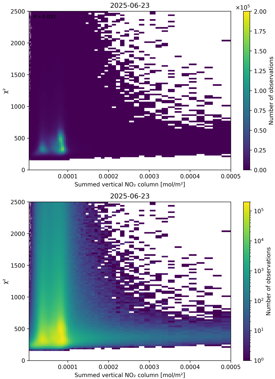
Figure 104: Scatter density plot of “Summed vertical NO 2 column” against “ \chi^2 ” for 2025-06-22 to 2025-06-24.
