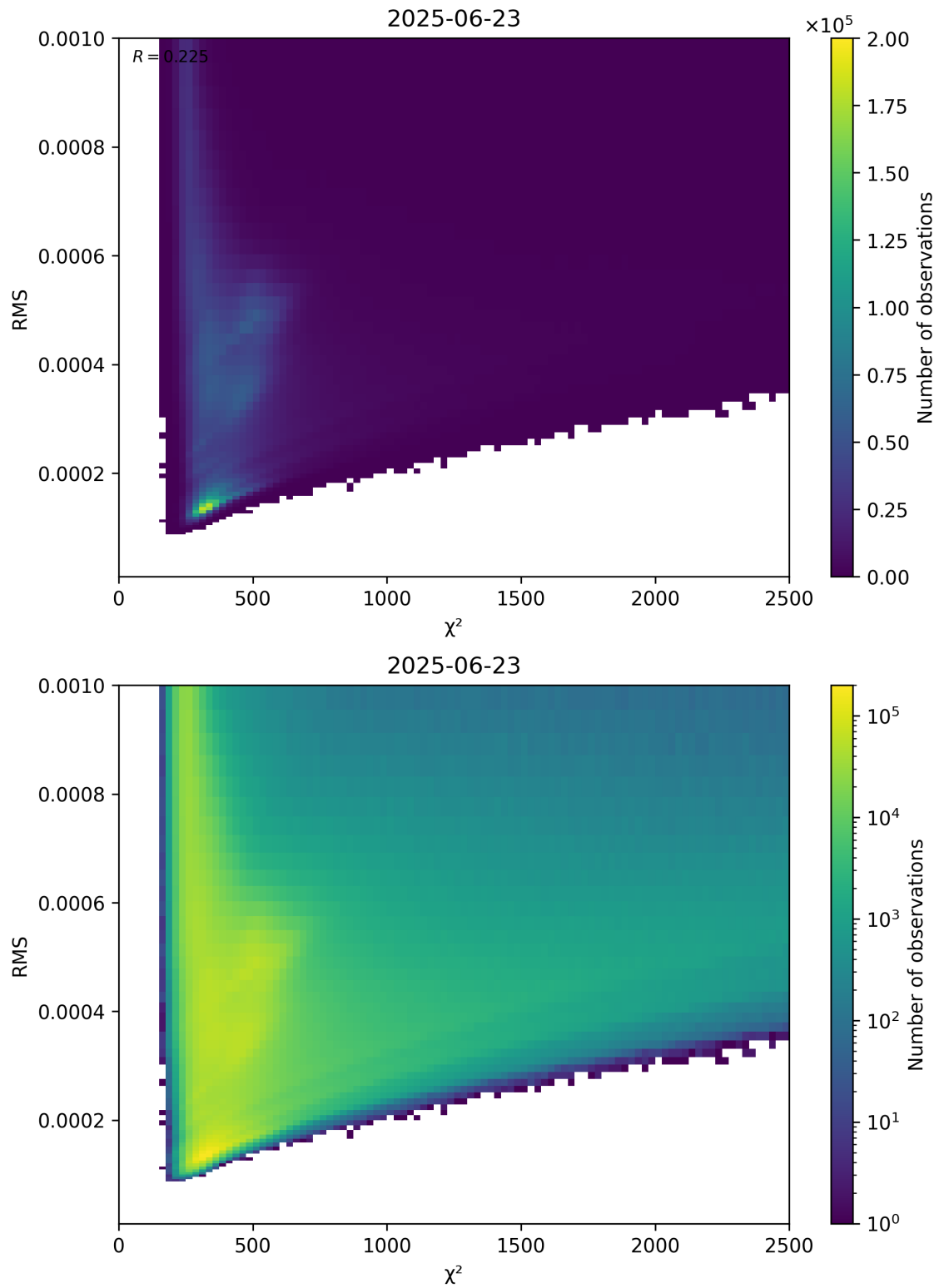
Figure 82: Scatter density plot of “ \chi^2 ” against “RMS” for 2025-06-22 to 2025-06-24.
