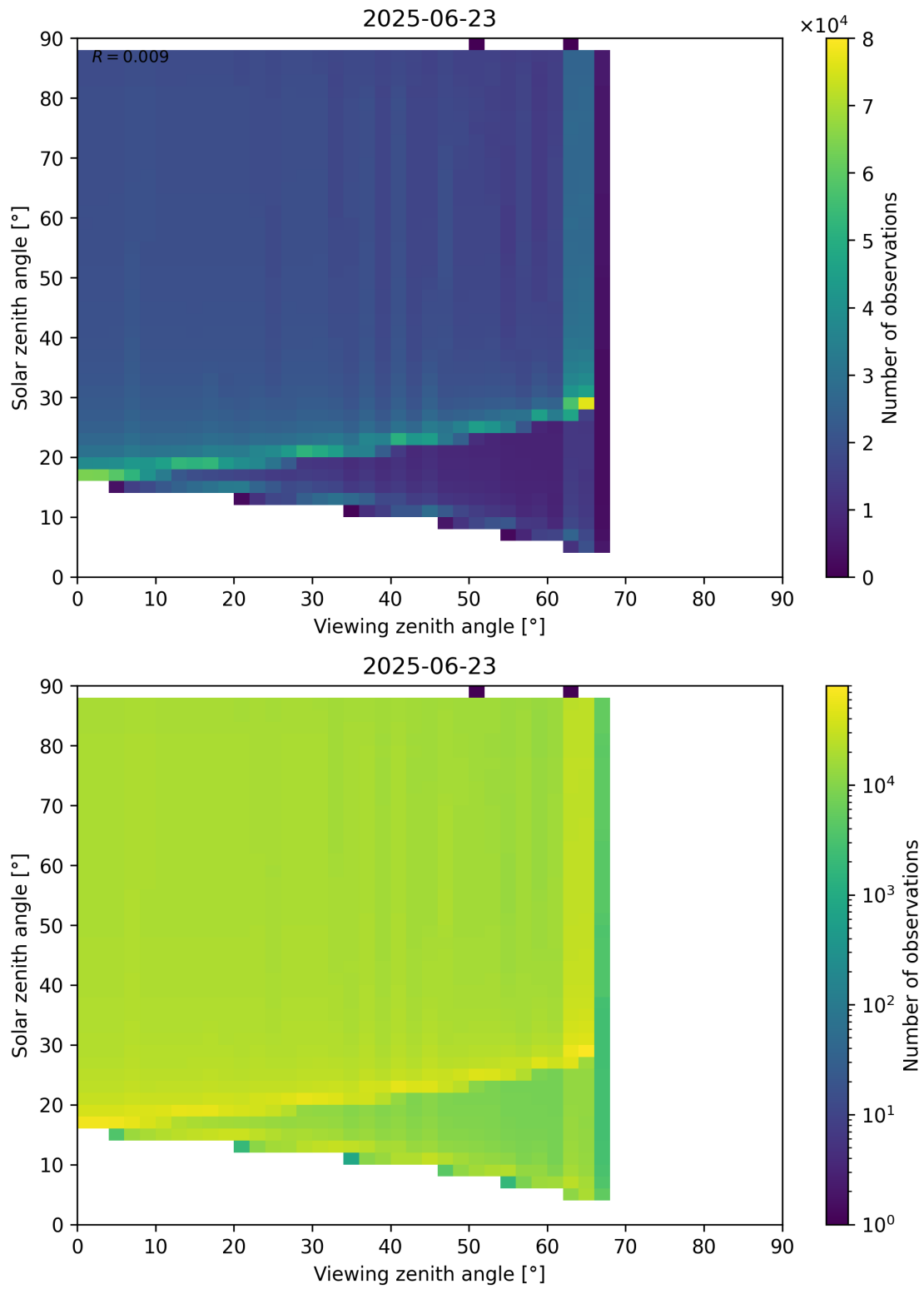
Figure 172: Scatter density plot of “Viewing zenith angle” against “Solar zenith angle” for 2025-06-22 to 2025-06-24.
