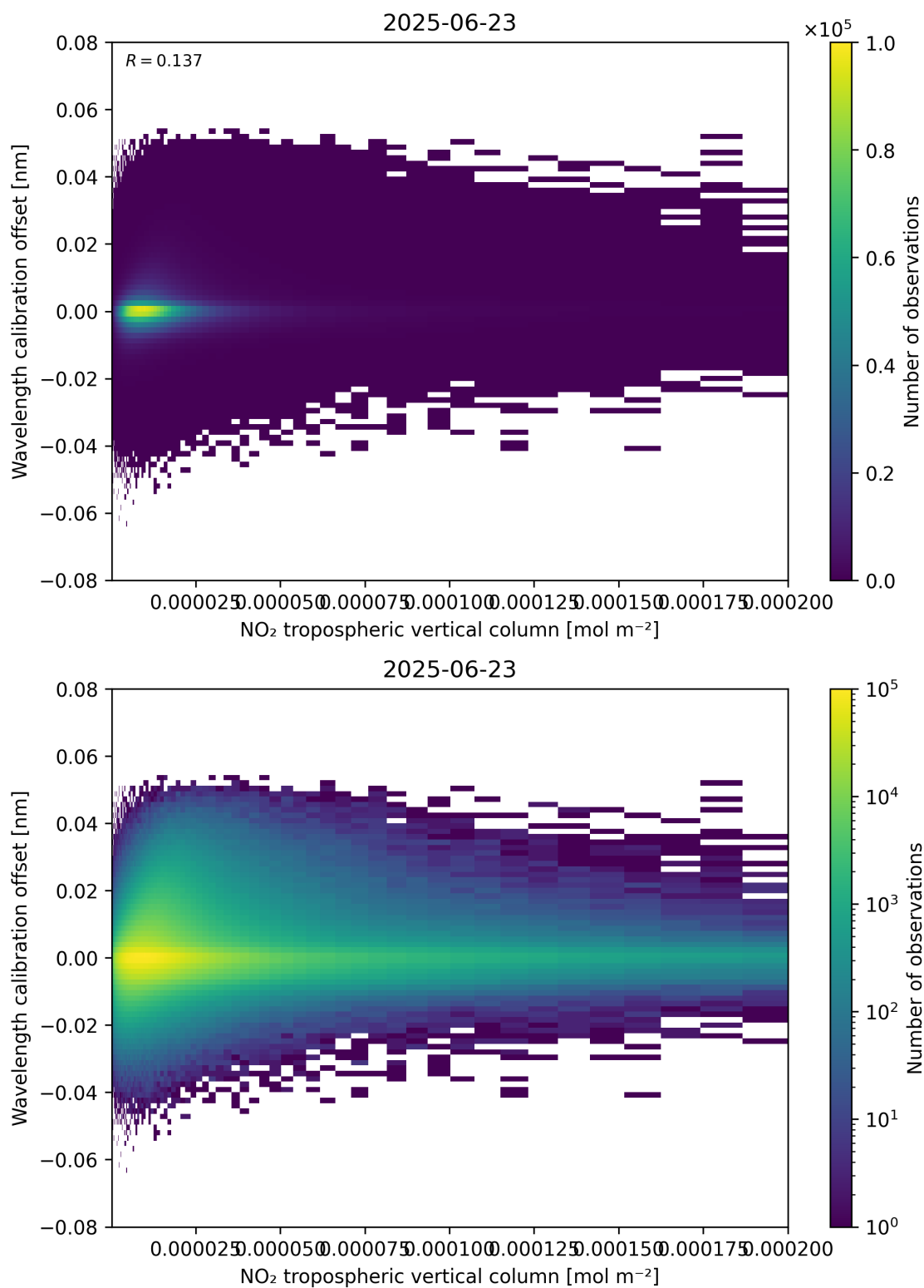
Figure 143: Scatter density plot of “NO 2 tropospheric vertical column” against “Wavelength calibration offset” for 2025-06-22 to 2025-06-24.
