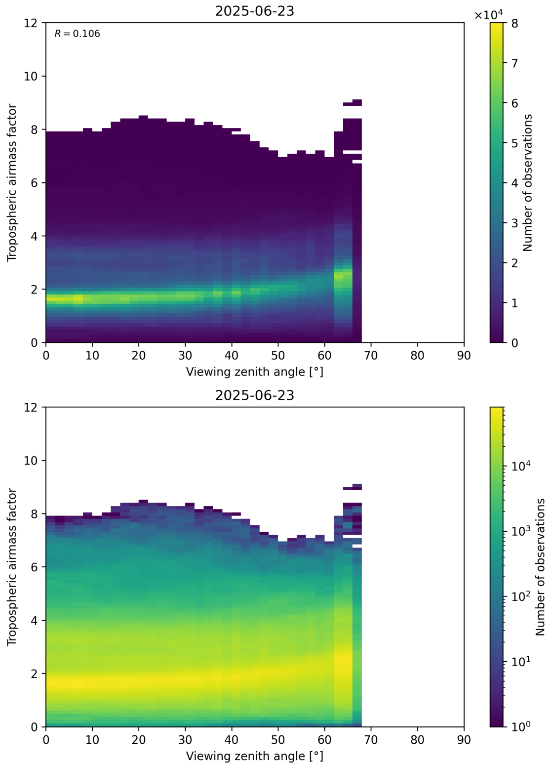
Figure 161: Scatter density plot of “Viewing zenith angle” against “Tropospheric airmass factor” for 2025-06-22 to 2025-06-24.
