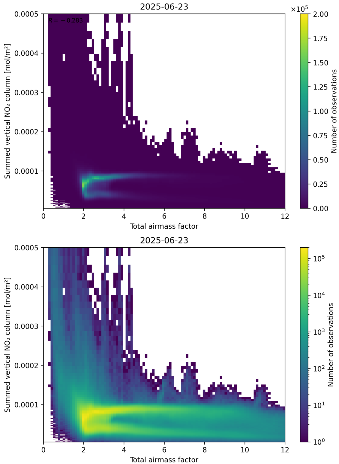
Figure 65: Scatter density plot of “Total airmass factor” against “Summed vertical NO 2 column” for 2025-06-22 to 2025-06-24.
