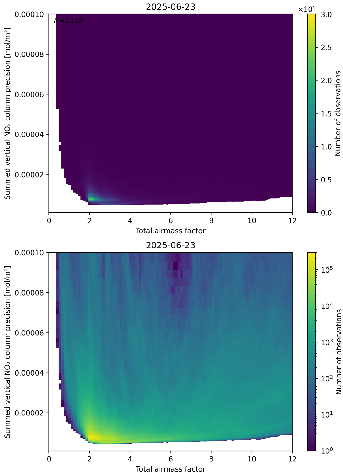
Figure 66: Scatter density plot of “Total airmass factor” against “Summed vertical NO 2 column precision” for 2025-06-22 to 2025-06-24.
