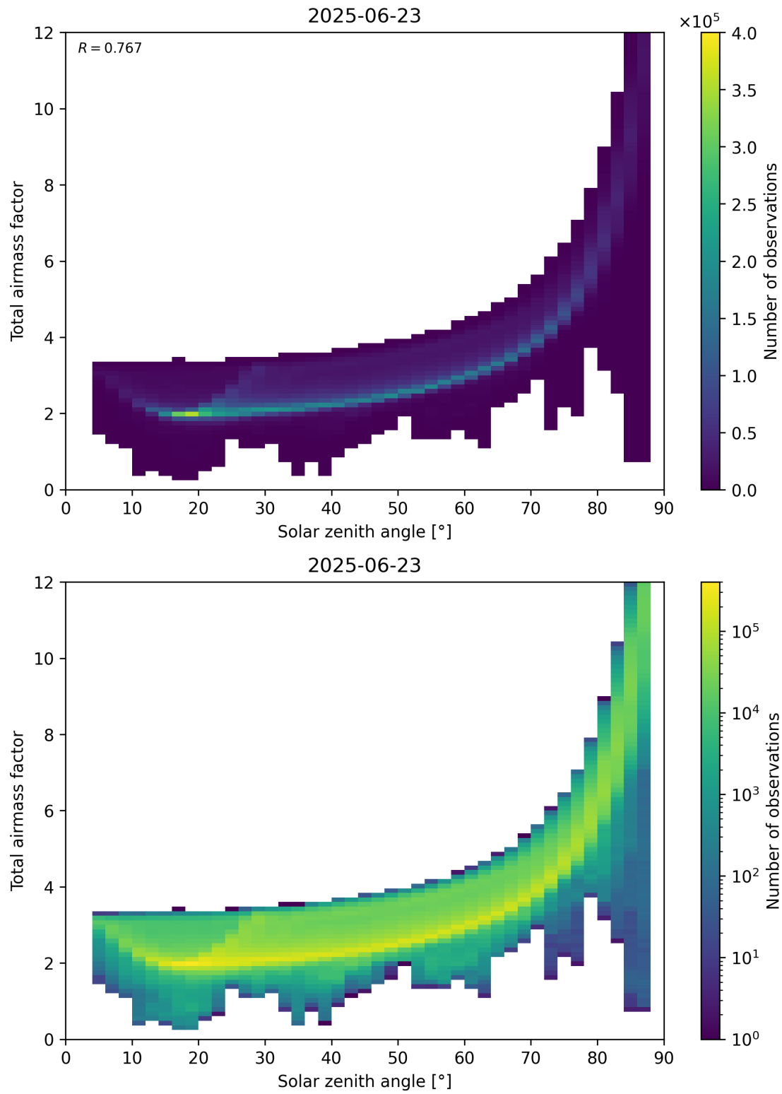
Figure 146: Scatter density plot of “Solar zenith angle” against “Total air mass factor” for 2025-06-22 to 2025-06-24.
