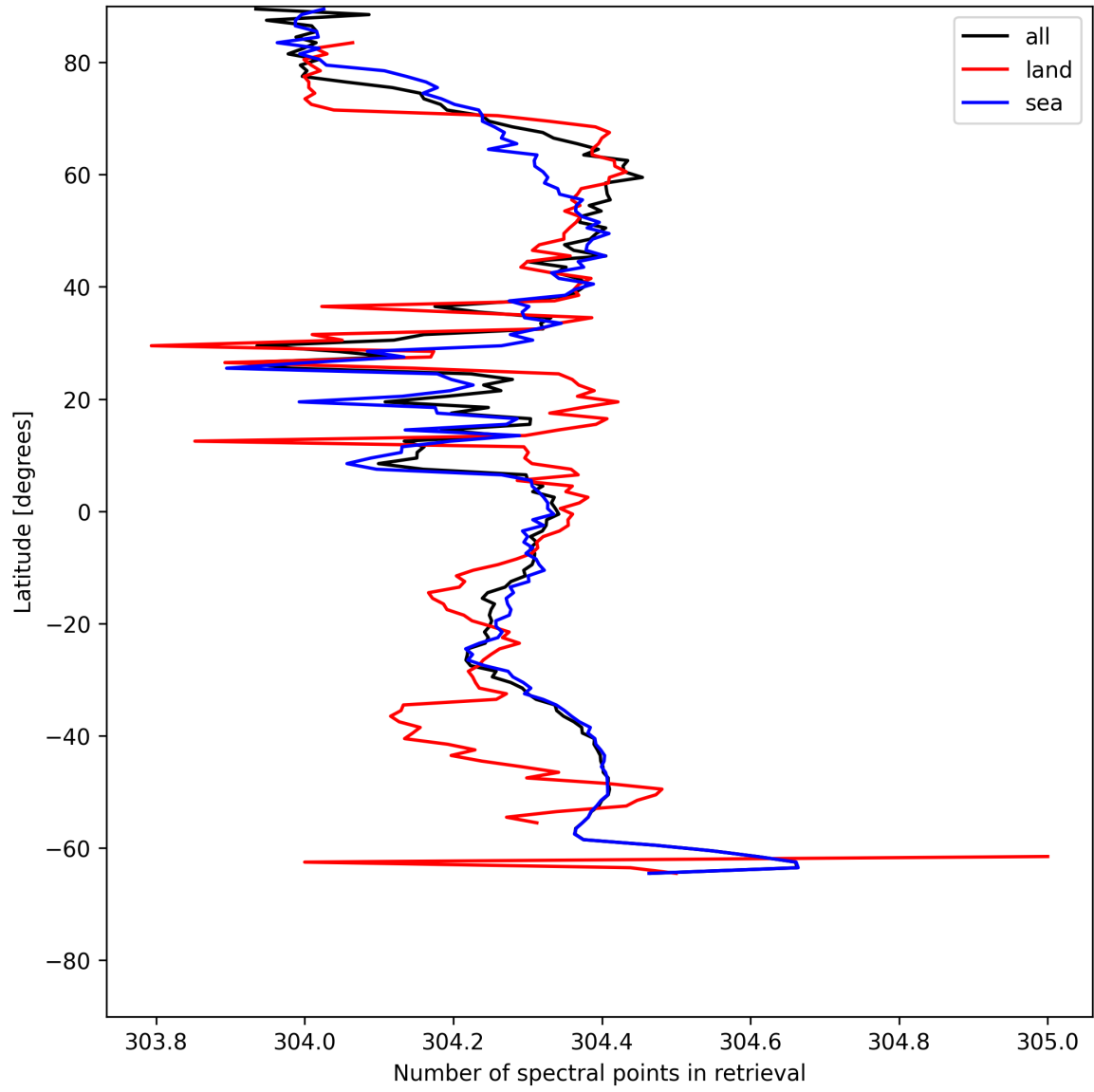
Figure 16: Zonal average of “Number of spectral points in retrieval” for 2025-06-22 to 2025-06-24.
