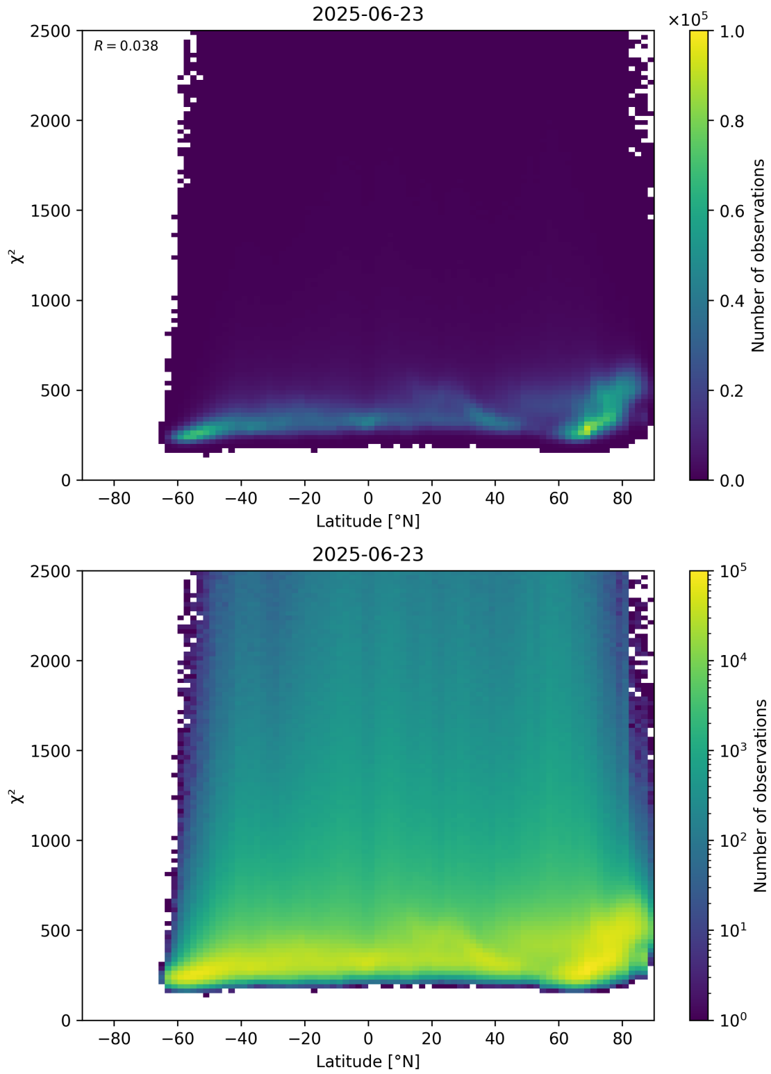
Figure 86: Scatter density plot of “Latitude” against “ \chi^2 ” for 2025-06-22 to 2025-06-24.
