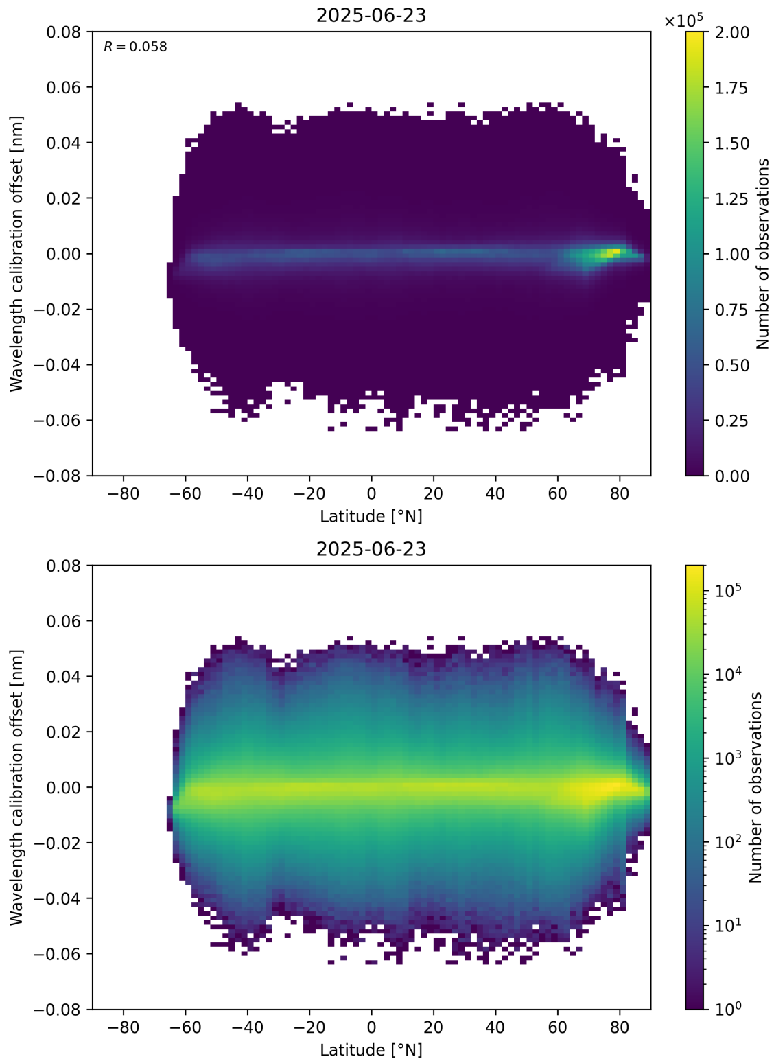
Figure 95: Scatter density plot of “Latitude” against “Wavelength calibration offset” for 2025-06-22 to 2025-06-24.
