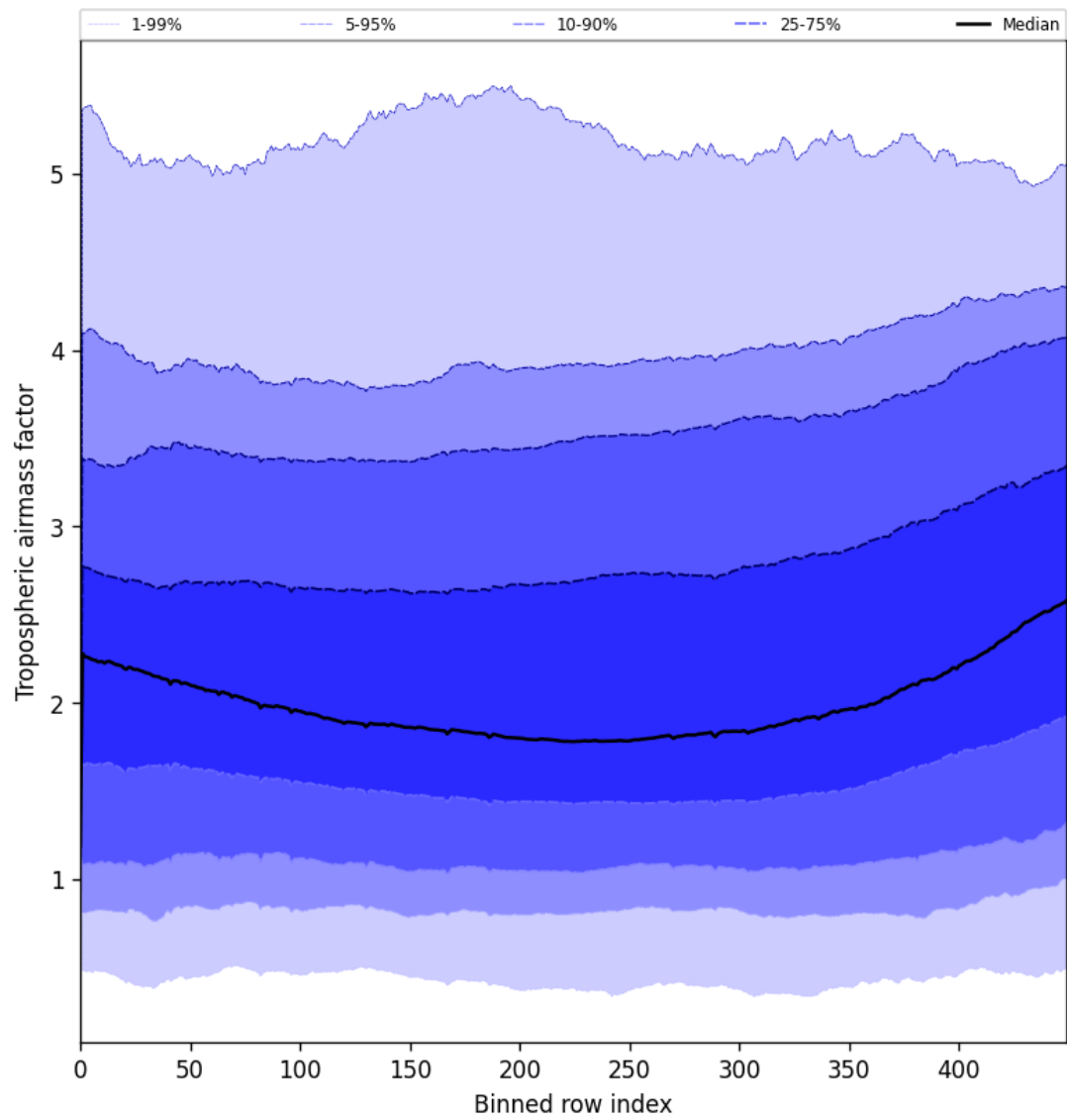
Figure 48: Along track statistics of “Tropospheric airmass factor” for 2025-06-22 to 2025-06-24
