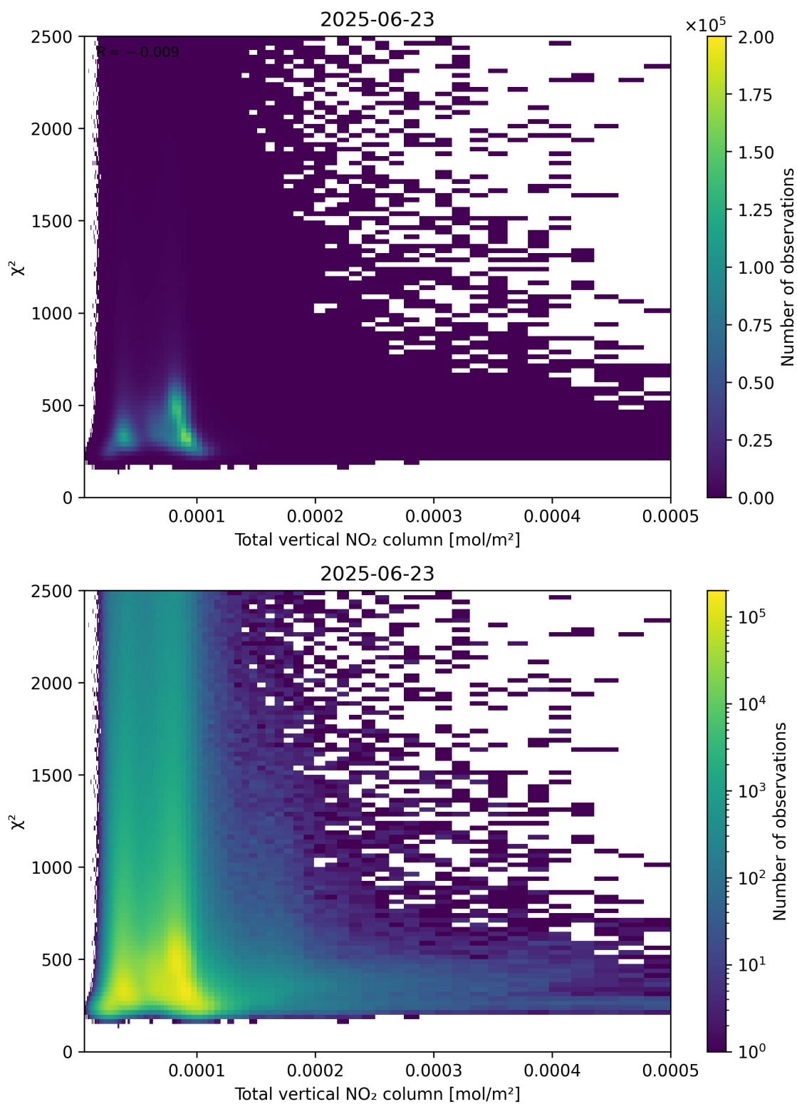
Figure 111: Scatter density plot of “Total vertical NO 2 column” against “ \chi^2 ” for 2025-06-22 to 2025-06-24.
