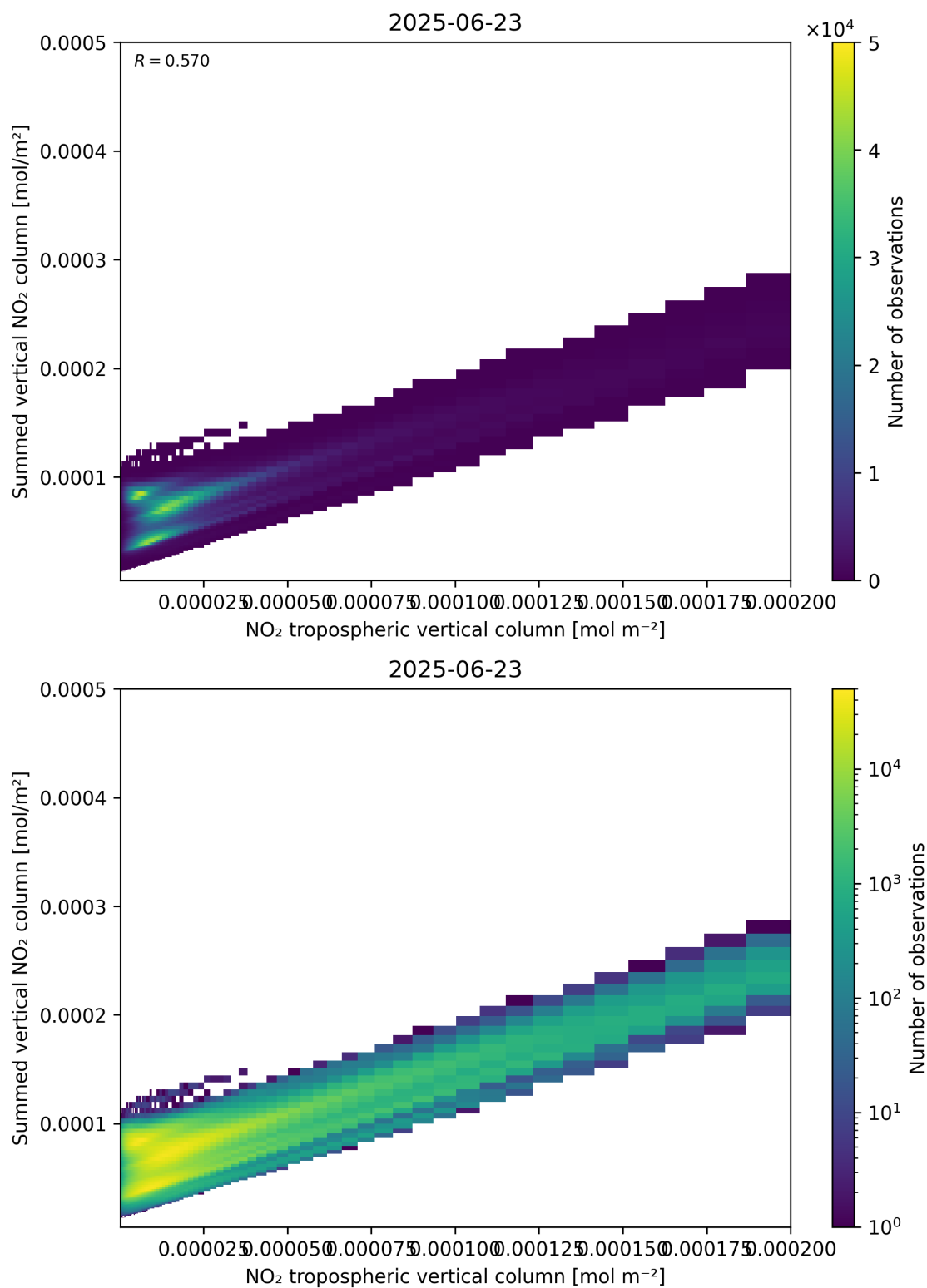
Figure 126: Scatter density plot of “NO 2 tropospheric vertical column” against “Summed vertical NO 2 column” for 2025-06-22 to 2025-06-24.
