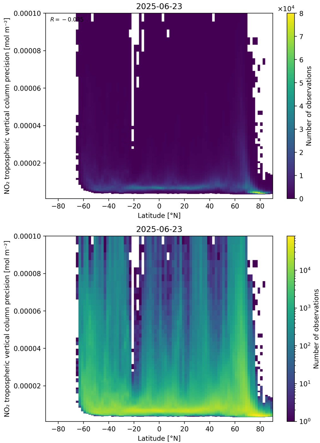
Figure 93: Scatter density plot of “Latitude” against “NO 2 tropospheric vertical column precision” for 2025-06-22 to 2025-06-24.
