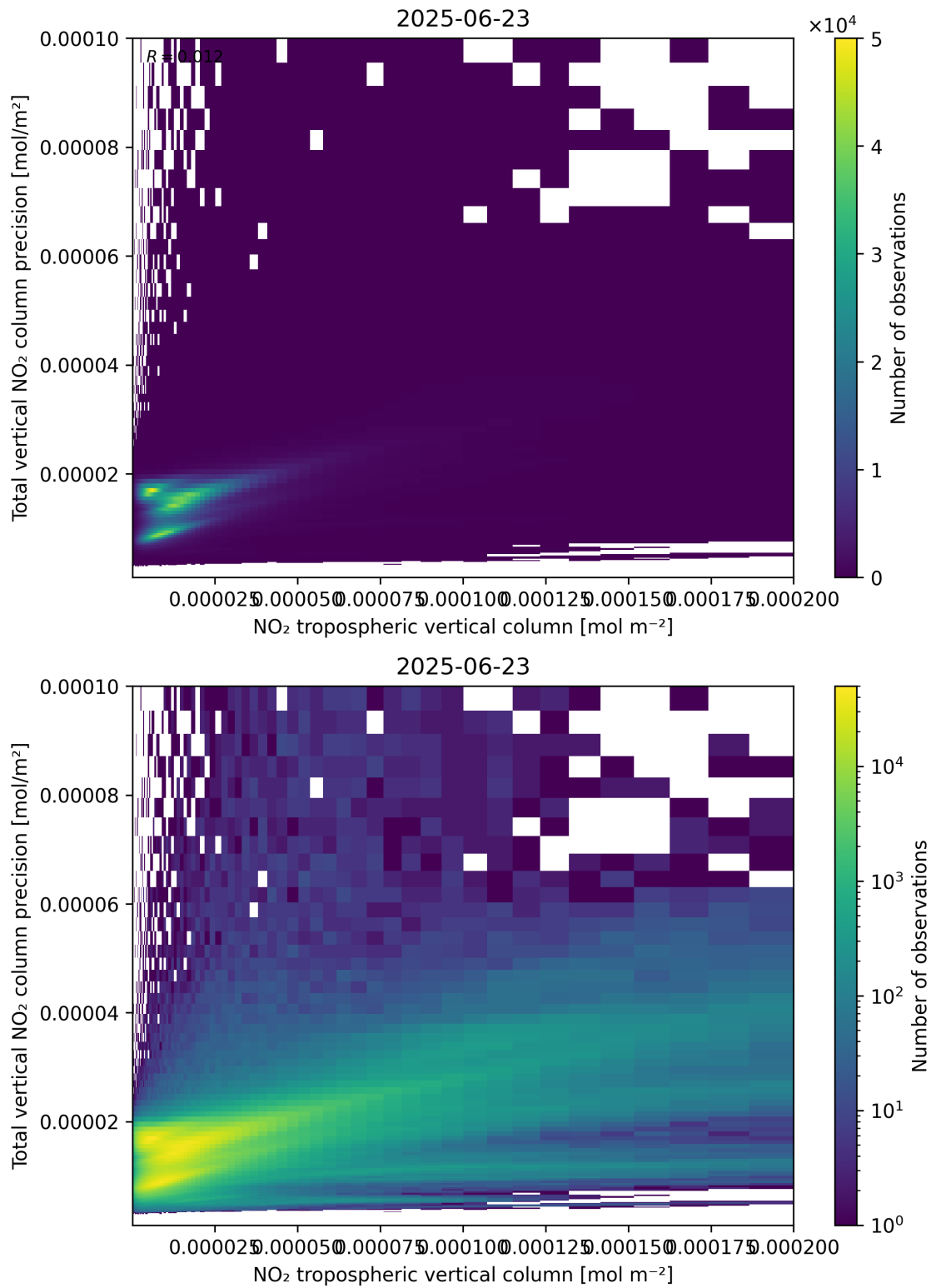
Figure 129: Scatter density plot of “NO 2 tropospheric vertical column” against “Total vertical NO 2 column precision” for 2025-06-22 to 2025-06-24.
