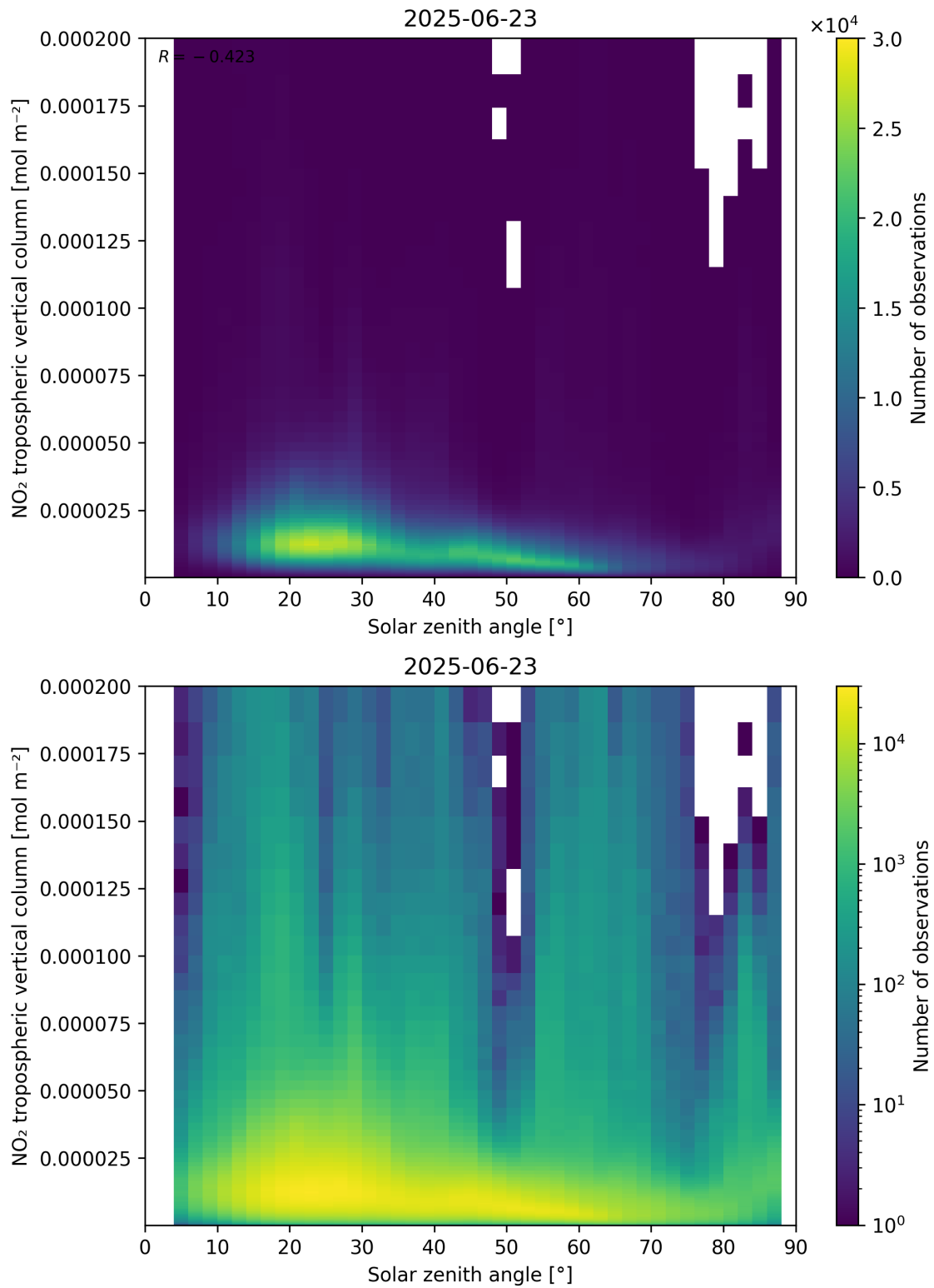
Figure 155: Scatter density plot of “Solar zenith angle” against “NO 2 tropospheric vertical column” for 2025-06-22 to 2025-06-24.
