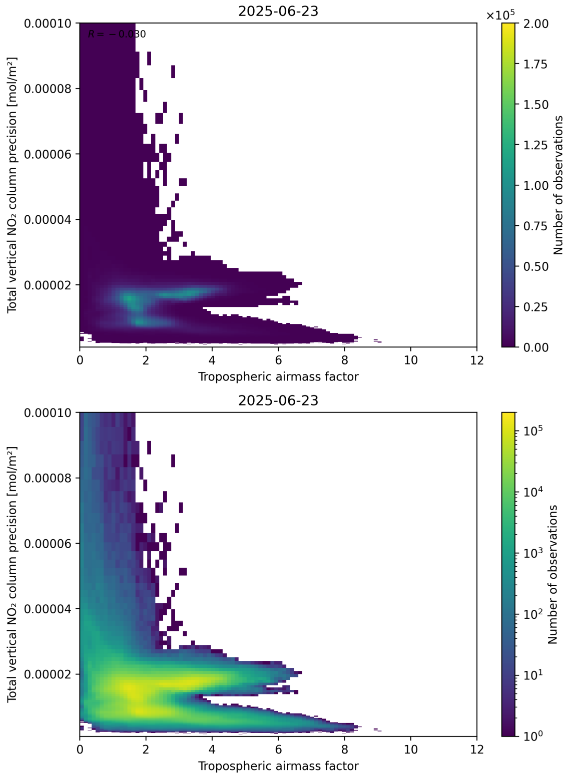
Figure 78: Scatter density plot of “Tropospheric air mass factor” against “Total vertical NO 2 column precision” for 2025-06-22 to 2025-06-24.
