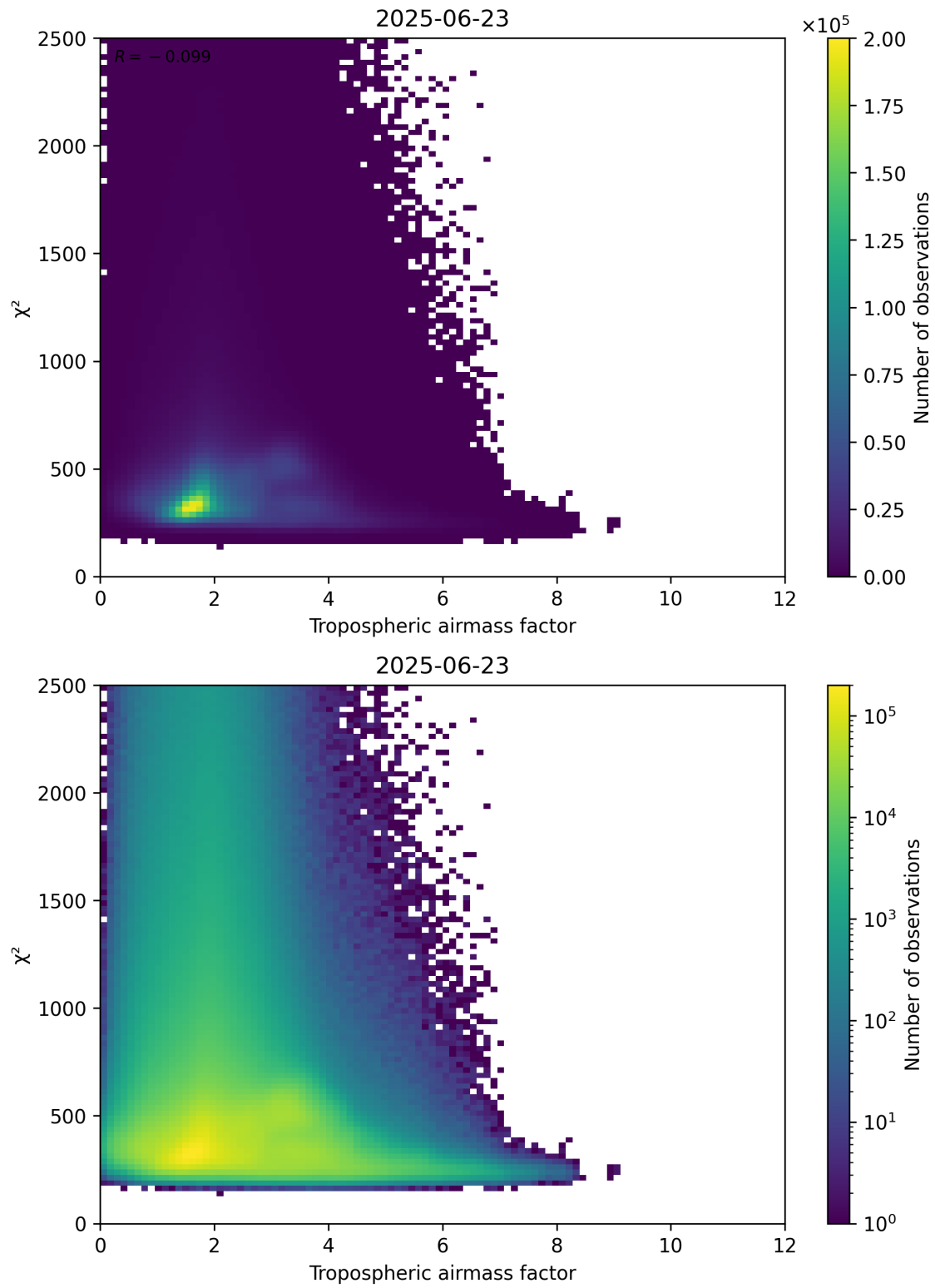
Figure 73: Scatter density plot of “Tropospheric airmass factor” against “ \chi^2 ” for 2025-06-22 to 2025-06-24.
