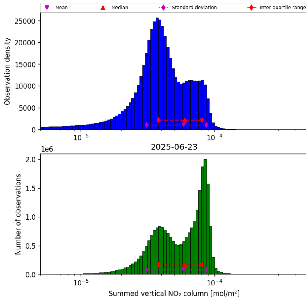
Figure 40: Histogram of “Summed vertical NO 2 column” for 2025-06-22 to 2025-06-24
