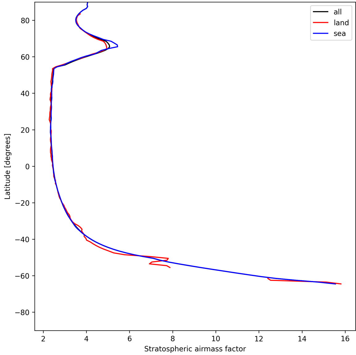
Figure 27: Zonal average of “Stratospheric air mass factor” for 2025-06-22 to 2025-06-24.
