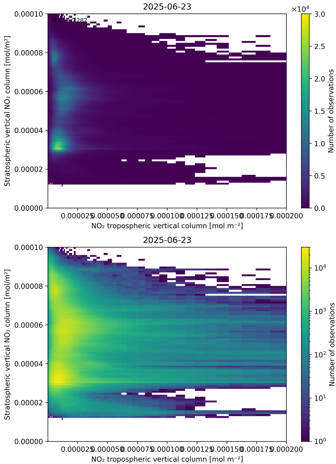
Figure 125: Scatter density plot of “NO 2 tropospheric vertical column” against “Stratospheric vertical NO 2 column” for 2025-06-22 to 2025-06-24.
