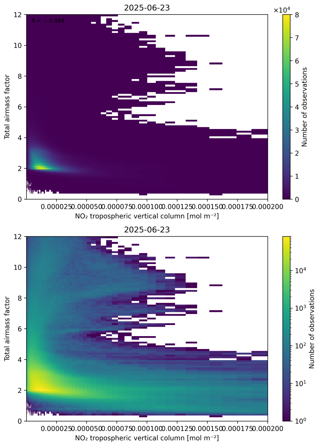
Figure 122: Scatter density plot of “NO 2 tropospheric vertical column” against “Total air mass factor” for 2025-06-22 to 2025-06-24.
