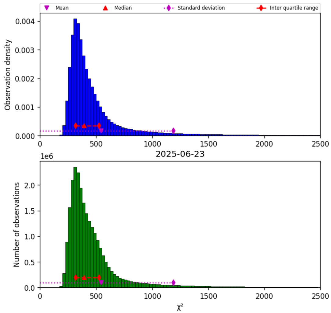
Figure 42: Histogram of “ \chi^2 ” for 2025-06-22 to 2025-06-24
