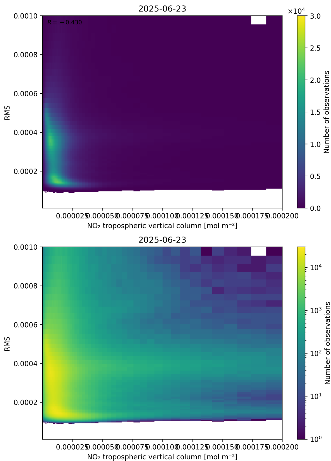
Figure 142: Scatter density plot of “NO 2 tropospheric vertical column” against “RMS” for 2025-06-22 to 2025-06-24.
