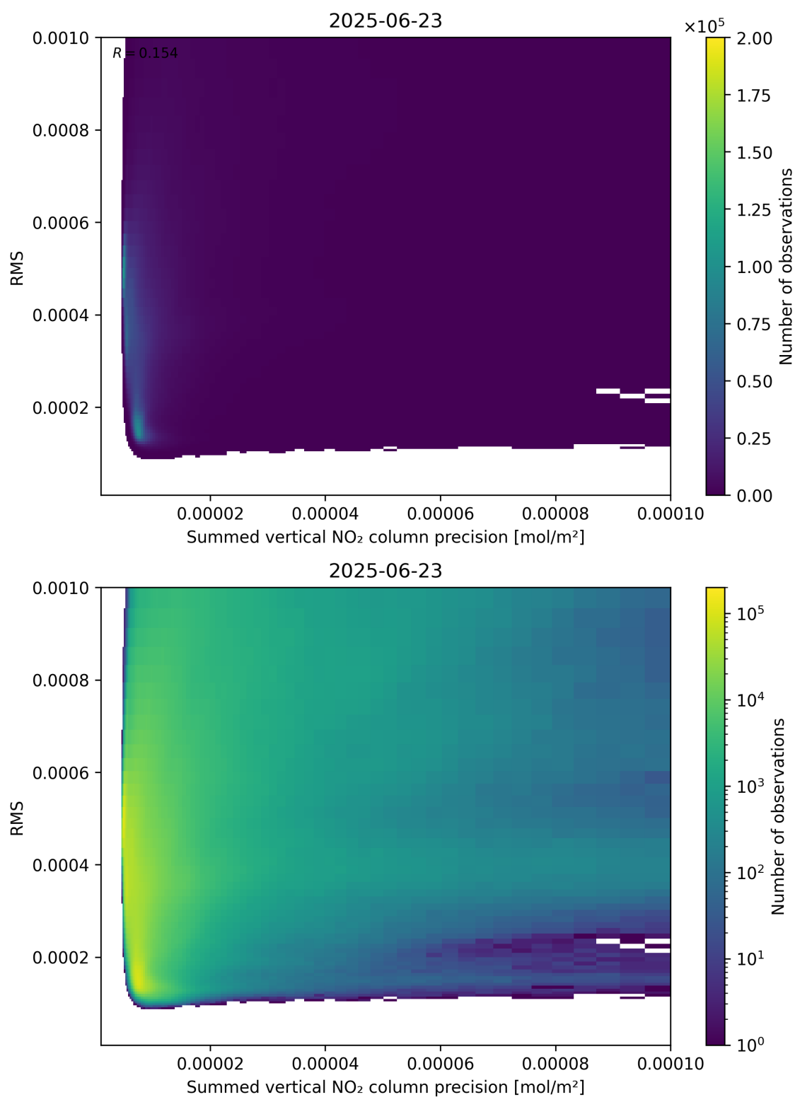
Figure 108: Scatter density plot of “Summed vertical NO 2 column precision” against “RMS” for 2025-06-22 to 2025-06-24.
