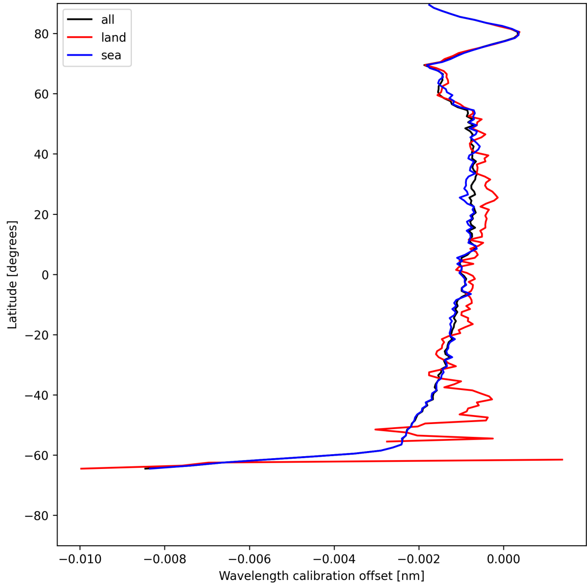
Figure 18: Zonal average of “Wavelength calibration offset” for 2025-06-22 to 2025-06-24.
