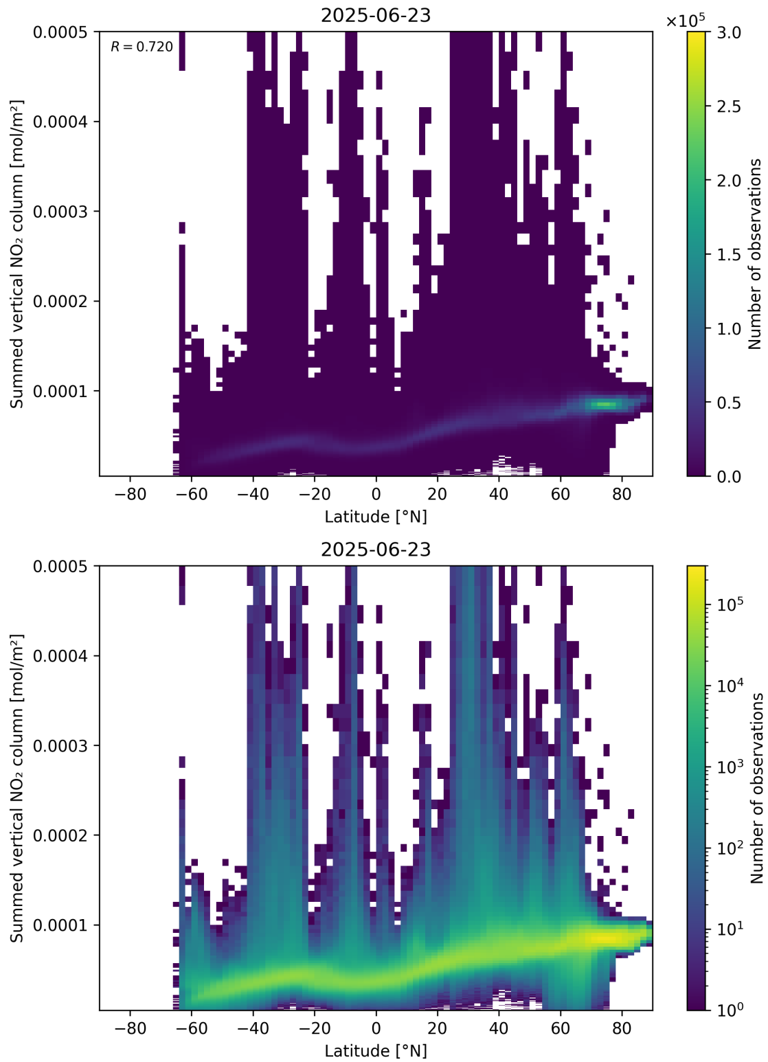
Figure 88: Scatter density plot of “Latitude” against “Summed vertical NO 2 column” for 2025-06-22 to 2025-06-24.
