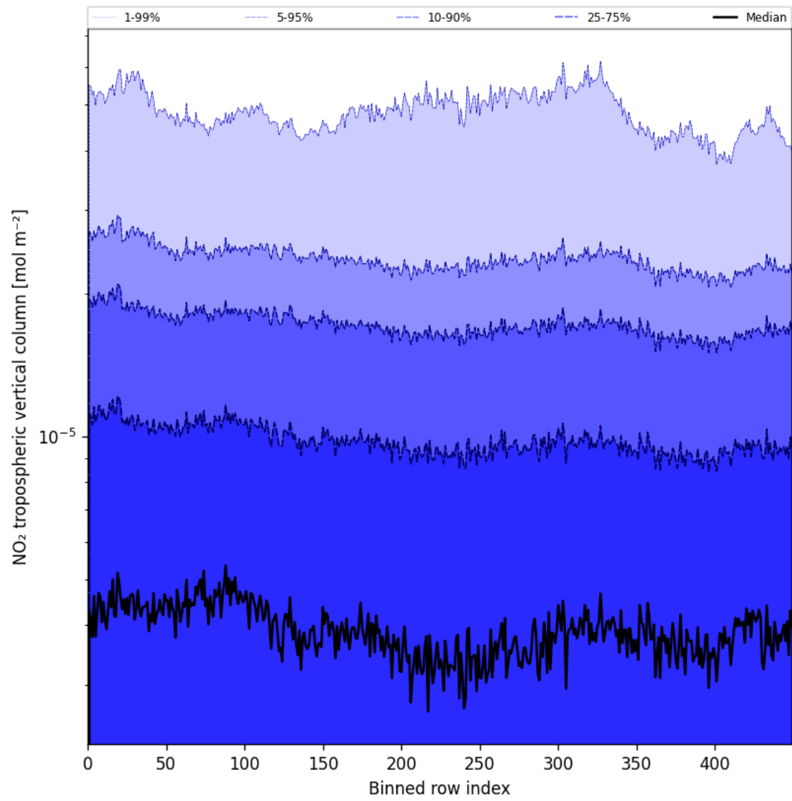
Figure 46: Along track statistics of “NO 2 tropospheric vertical column” for 2025-06-22 to 2025-06-24
