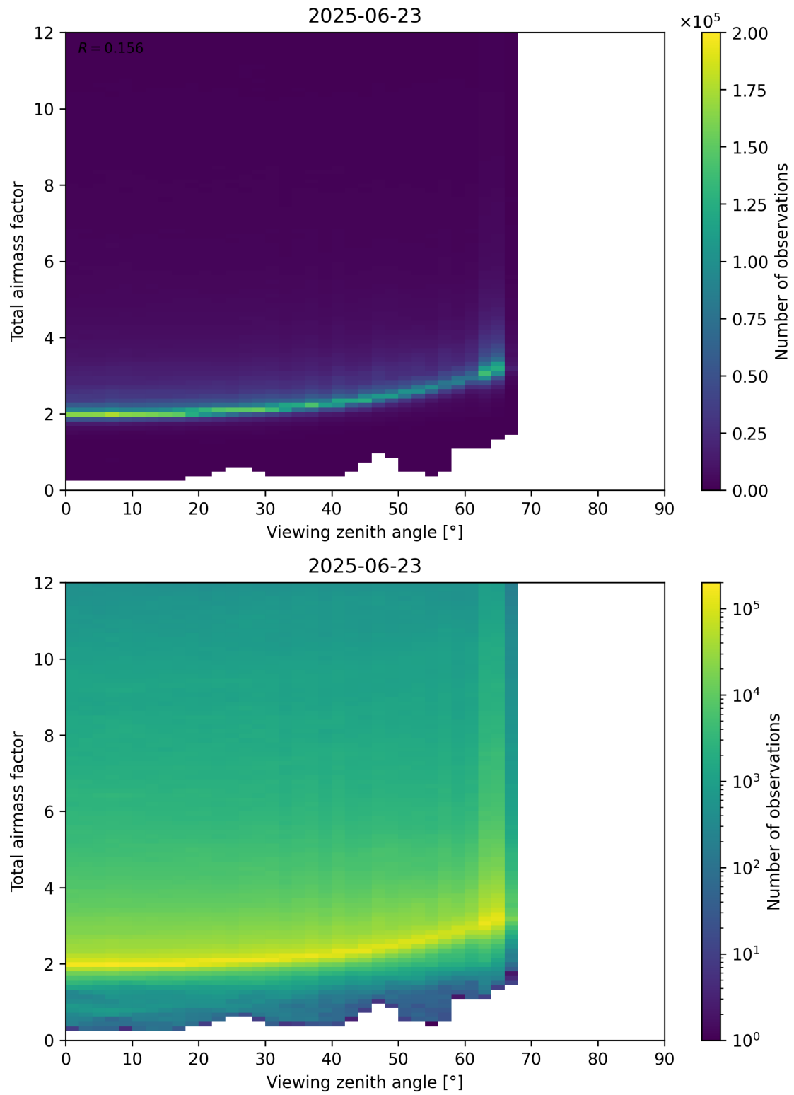
Figure 160: Scatter density plot of “Viewing zenith angle” against “Total airmass factor” for 2025-06-22 to 2025-06-24.
