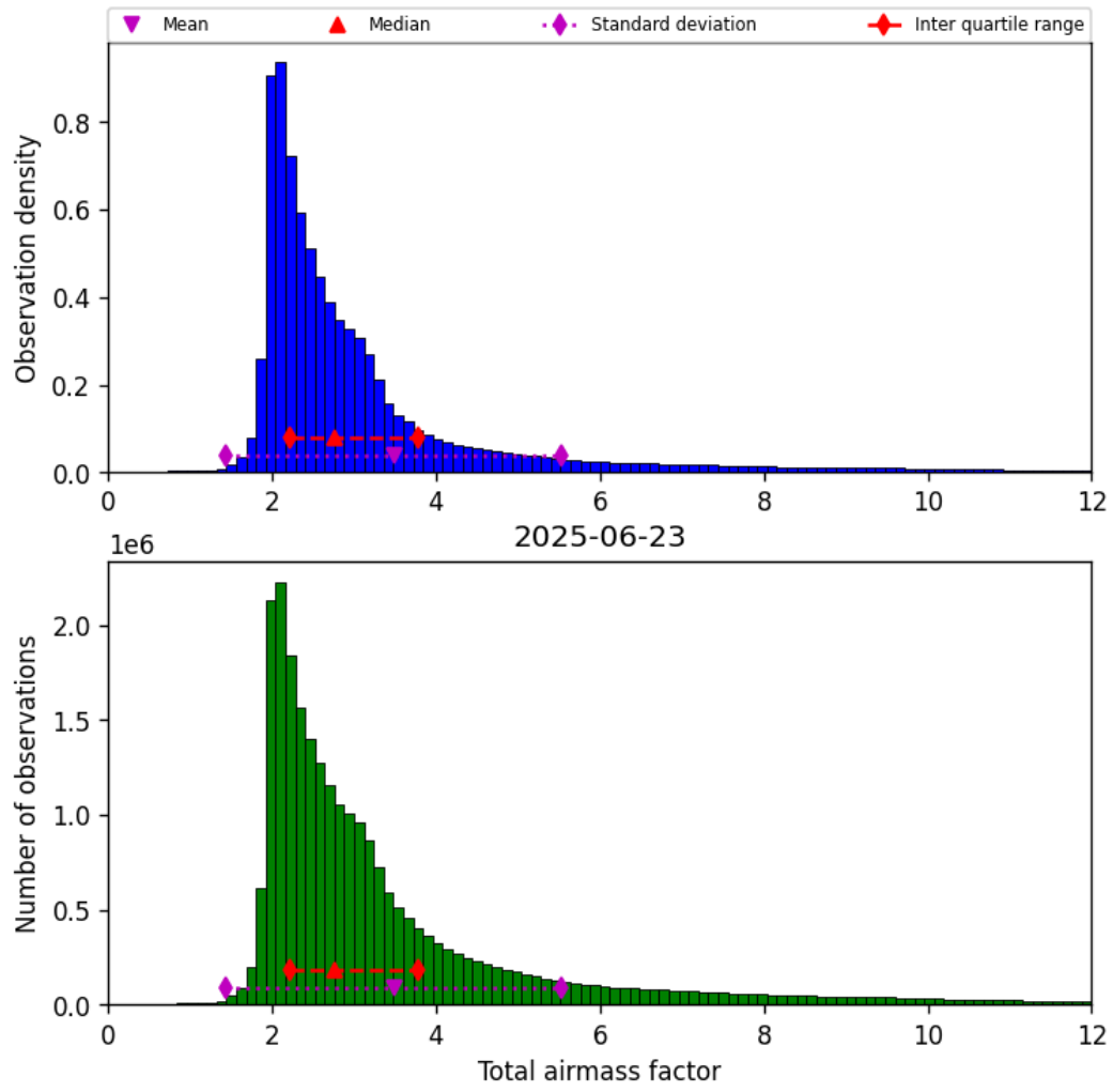
Figure 32: Histogram of “Total airmass factor” for 2025-06-22 to 2025-06-24
