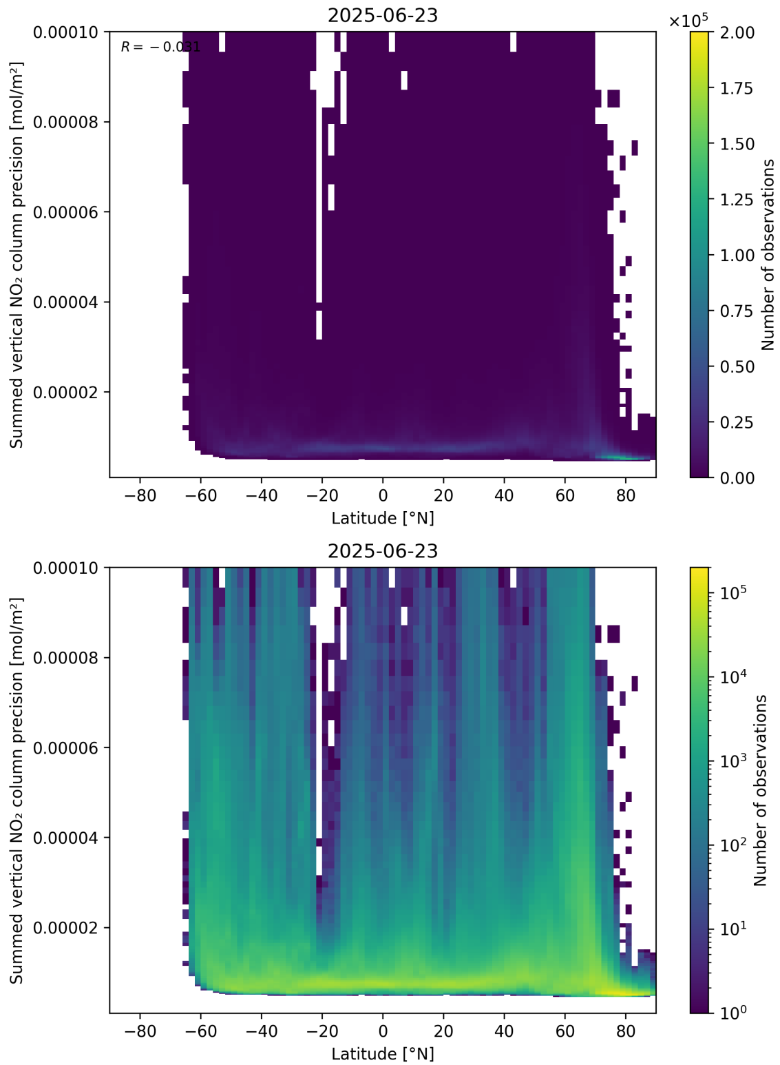
Figure 89: Scatter density plot of “Latitude” against “Summed vertical NO 2 column precision” for 2025-06-22 to 2025-06-24.
