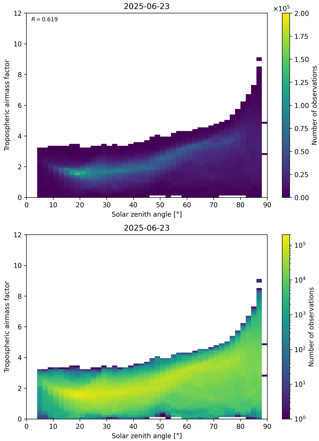
Figure 147: Scatter density plot of “Solar zenith angle” against “Tropospheric airmass factor” for 2025-06-22 to 2025-06-24.
