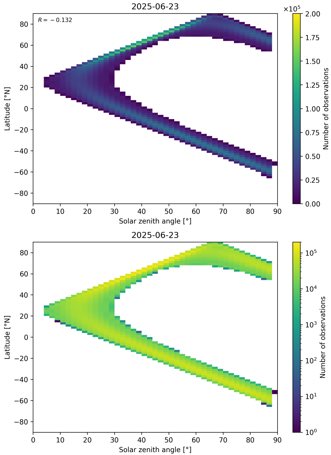
Figure 149: Scatter density plot of “Solar zenith angle” against “Latitude” for 2025-06-22 to 2025-06-24.
