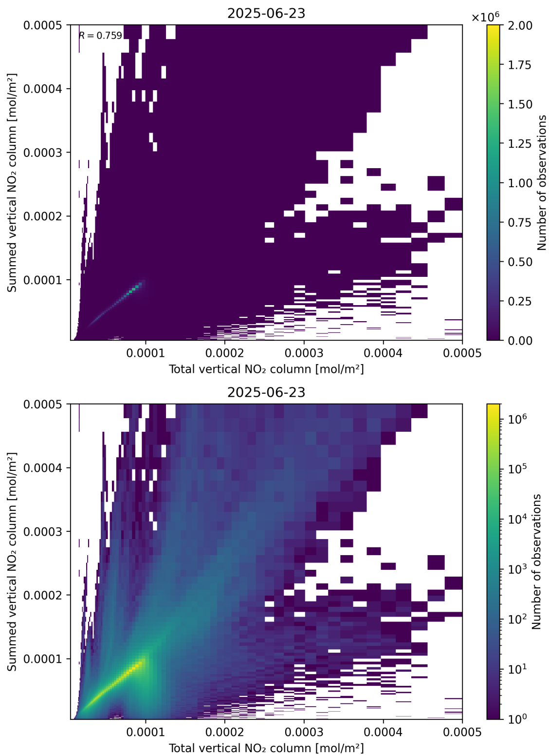
Figure 112: Scatter density plot of “Total vertical NO 2 column” against “Summed vertical NO 2 column” for 2025-06-22 to 2025-06-24.
