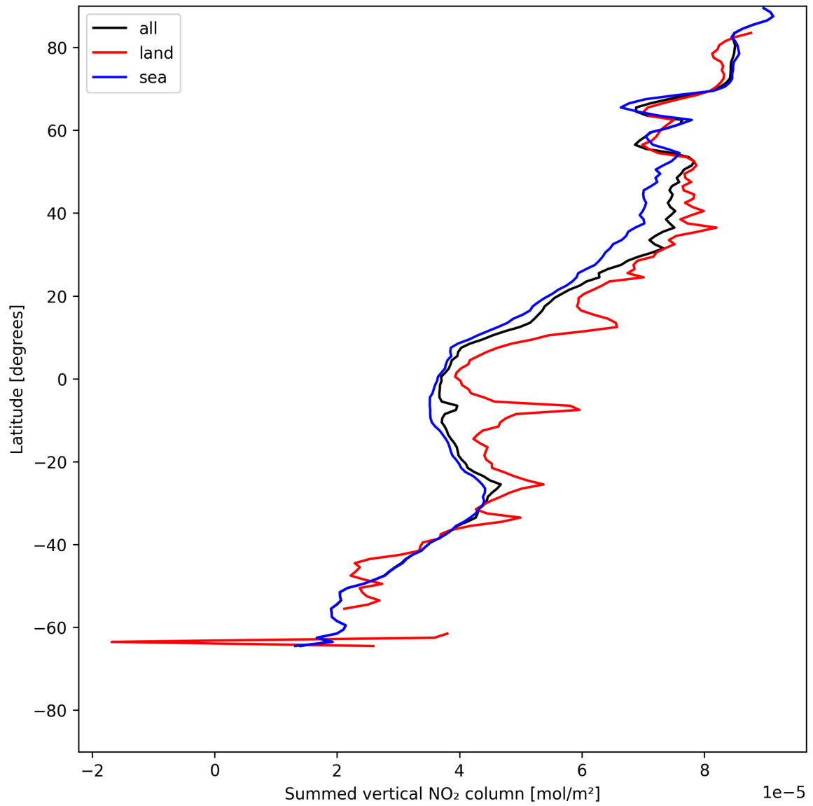
Figure 23: Zonal average of “Summed vertical NO 2 column” for 2025-06-22 to 2025-06-24.
