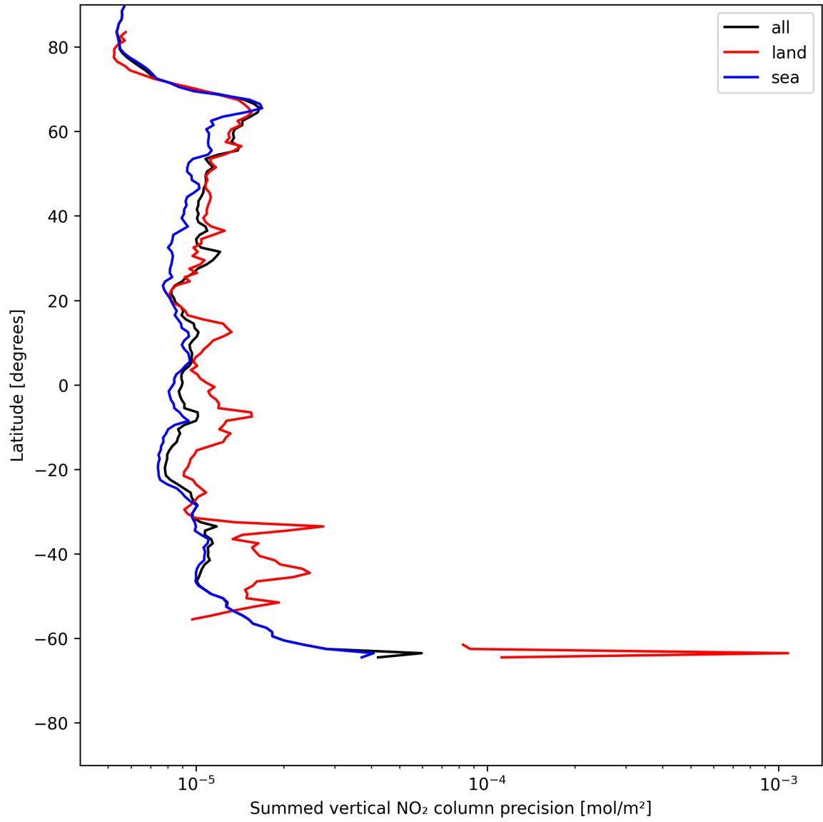
Figure 24: Zonal average of “Summed vertical NO 2 column precision” for 2025-06-22 to 2025-06-24.
