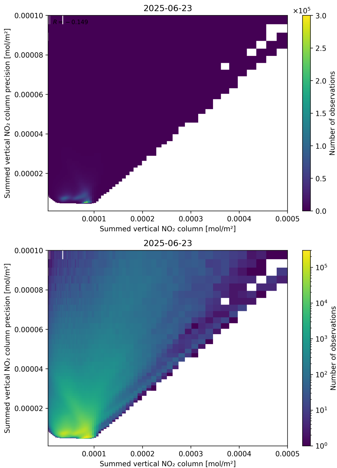
Figure 105: Scatter density plot of “Summed vertical NO 2 column” against “Summed vertical NO 2 column precision” for 2025-06-22 to 2025-06-24.
