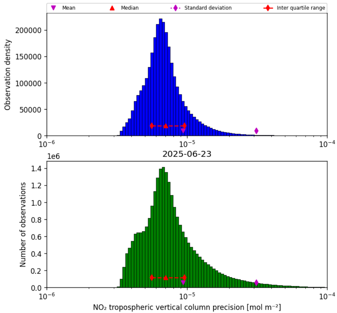
Figure 30: Histogram of “NO 2 tropospheric vertical column precision” for 2025-06-22 to 2025-06-24
