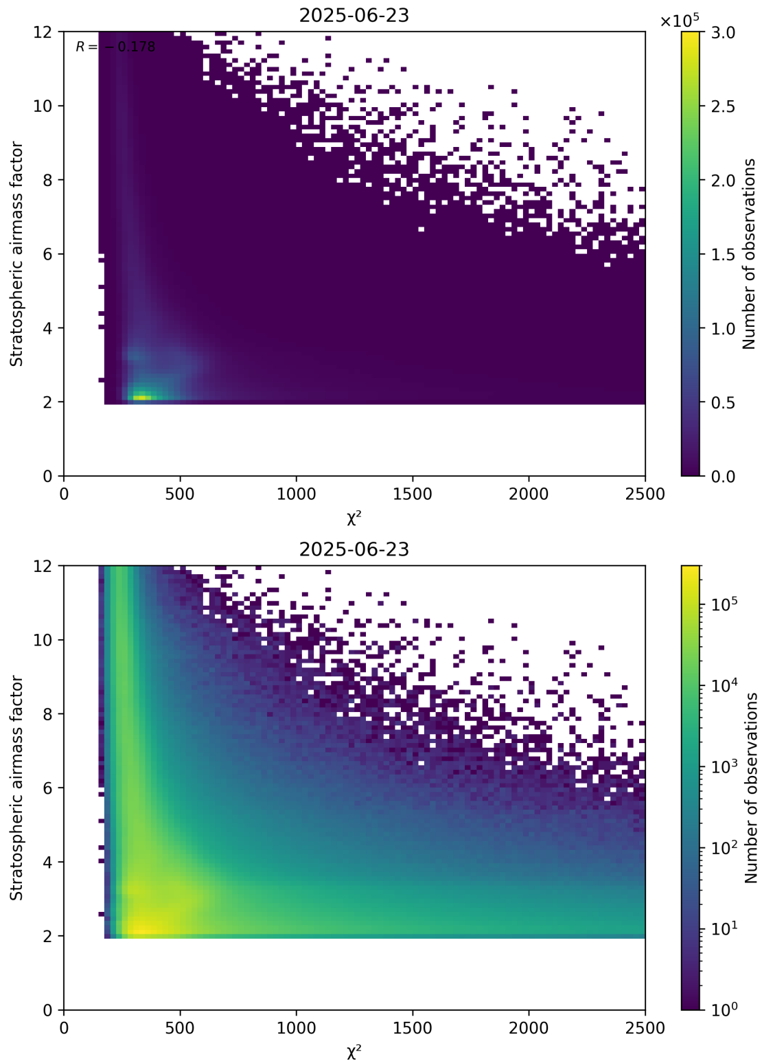
Figure 81: Scatter density plot of “ \chi^2 ” against “Stratospheric airmass factor” for 2025-06-22 to 2025-06-24.
