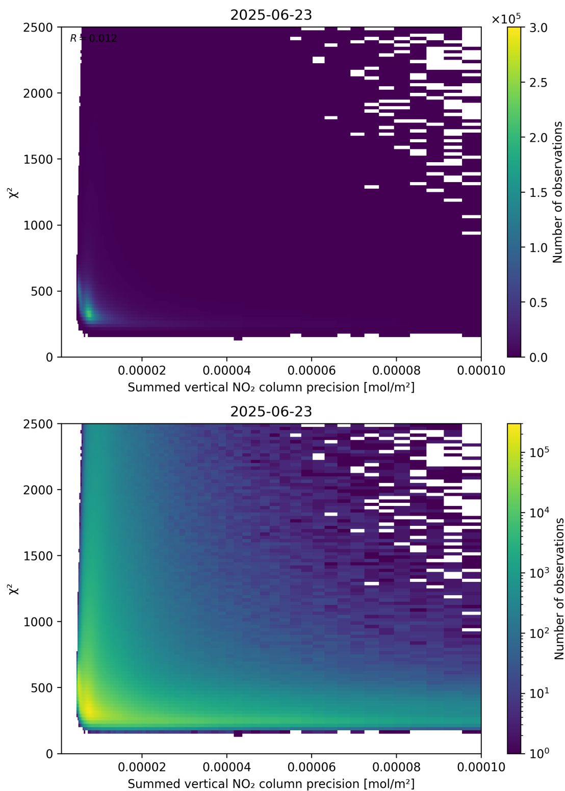
Figure 107: Scatter density plot of “Summed vertical NO 2 column precision” against “ \chi^2 ” for 2025-06-22 to 2025-06-24.
