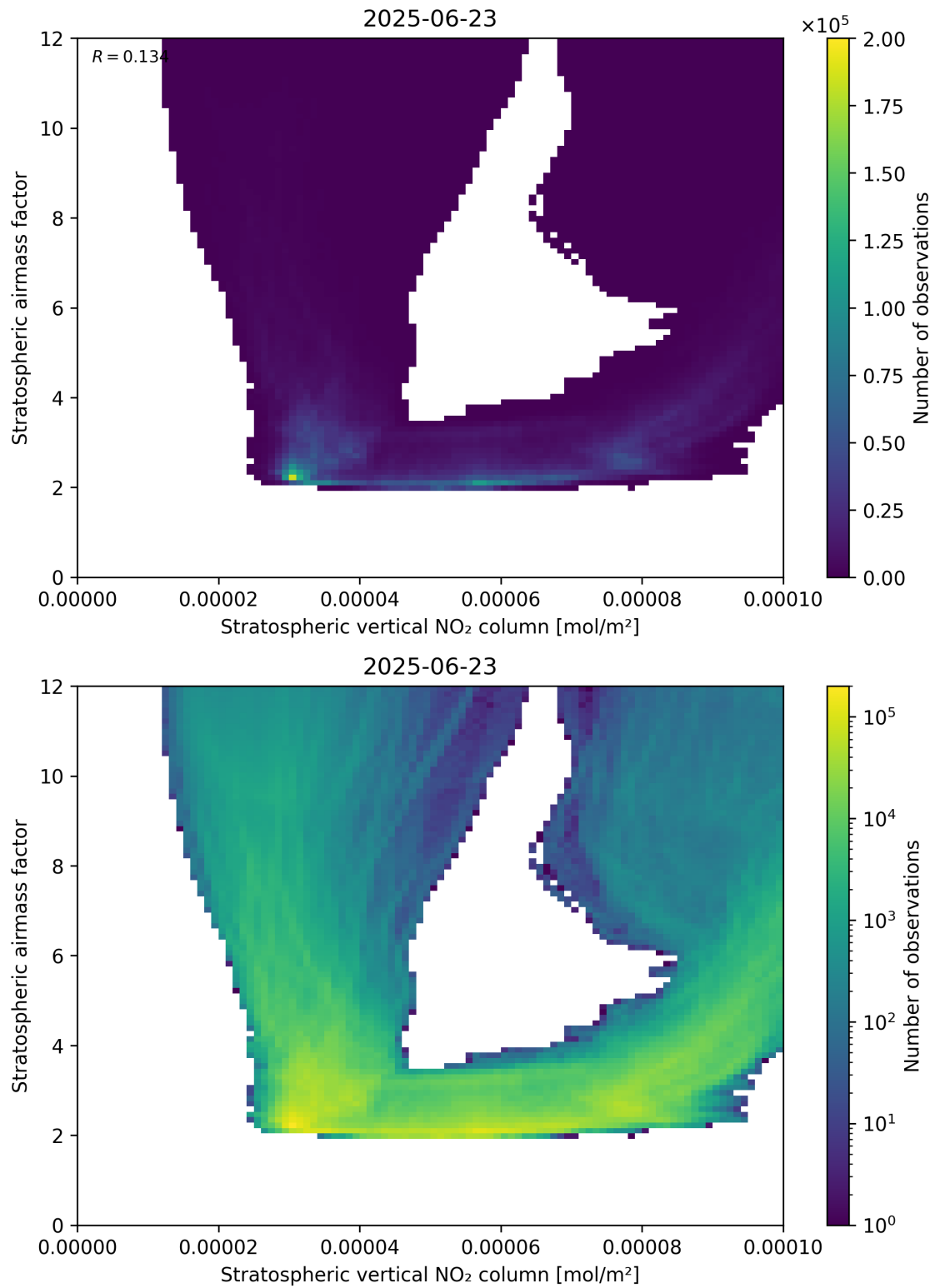
Figure 96: Scatter density plot of “Stratospheric vertical NO 2 column” against “Stratospheric airmass factor” for 2025-06-22 to 2025-06-24.
