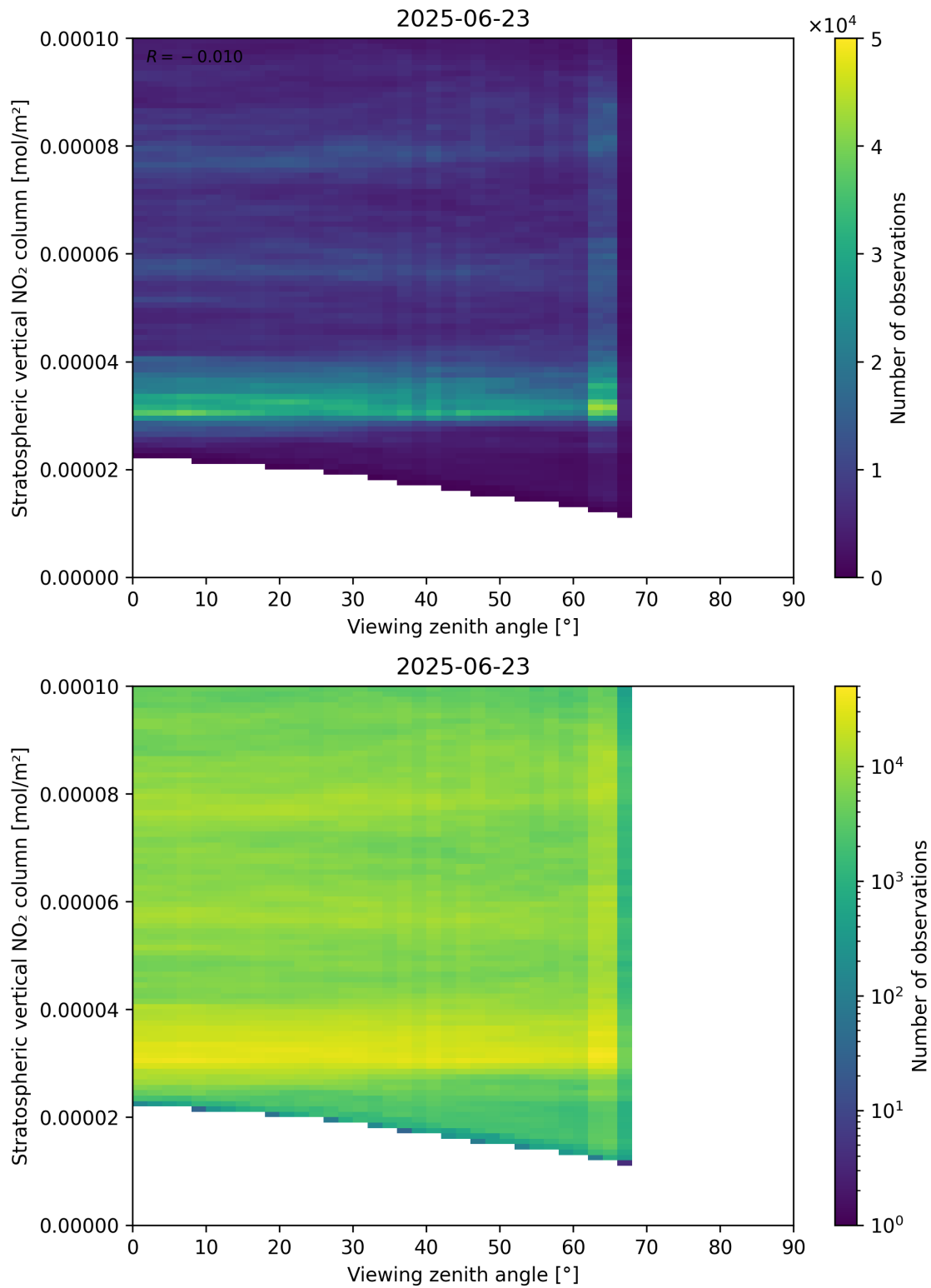
Figure 164: Scatter density plot of “Viewing zenith angle” against “Stratospheric vertical NO 2 column” for 2025-06-22 to 2025-06-24.
