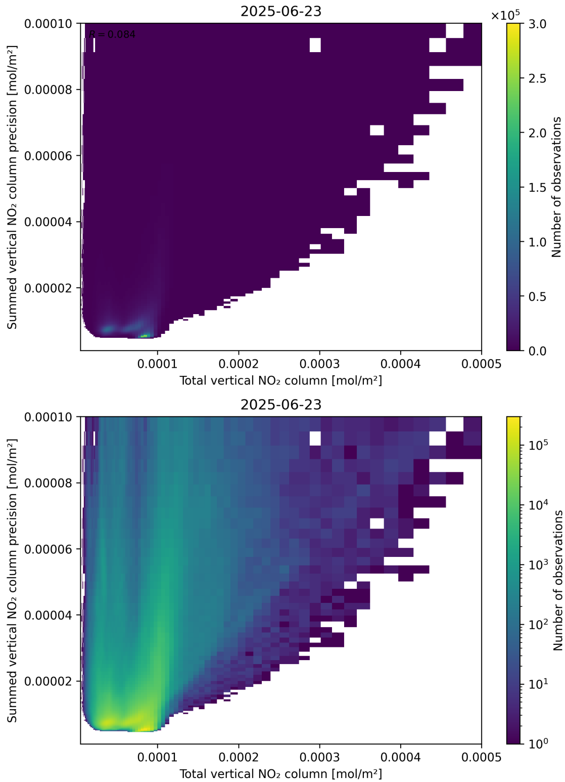
Figure 113: Scatter density plot of “Total vertical NO 2 column” against “Summed vertical NO 2 column precision” for 2025-06-22 to 2025-06-24.
