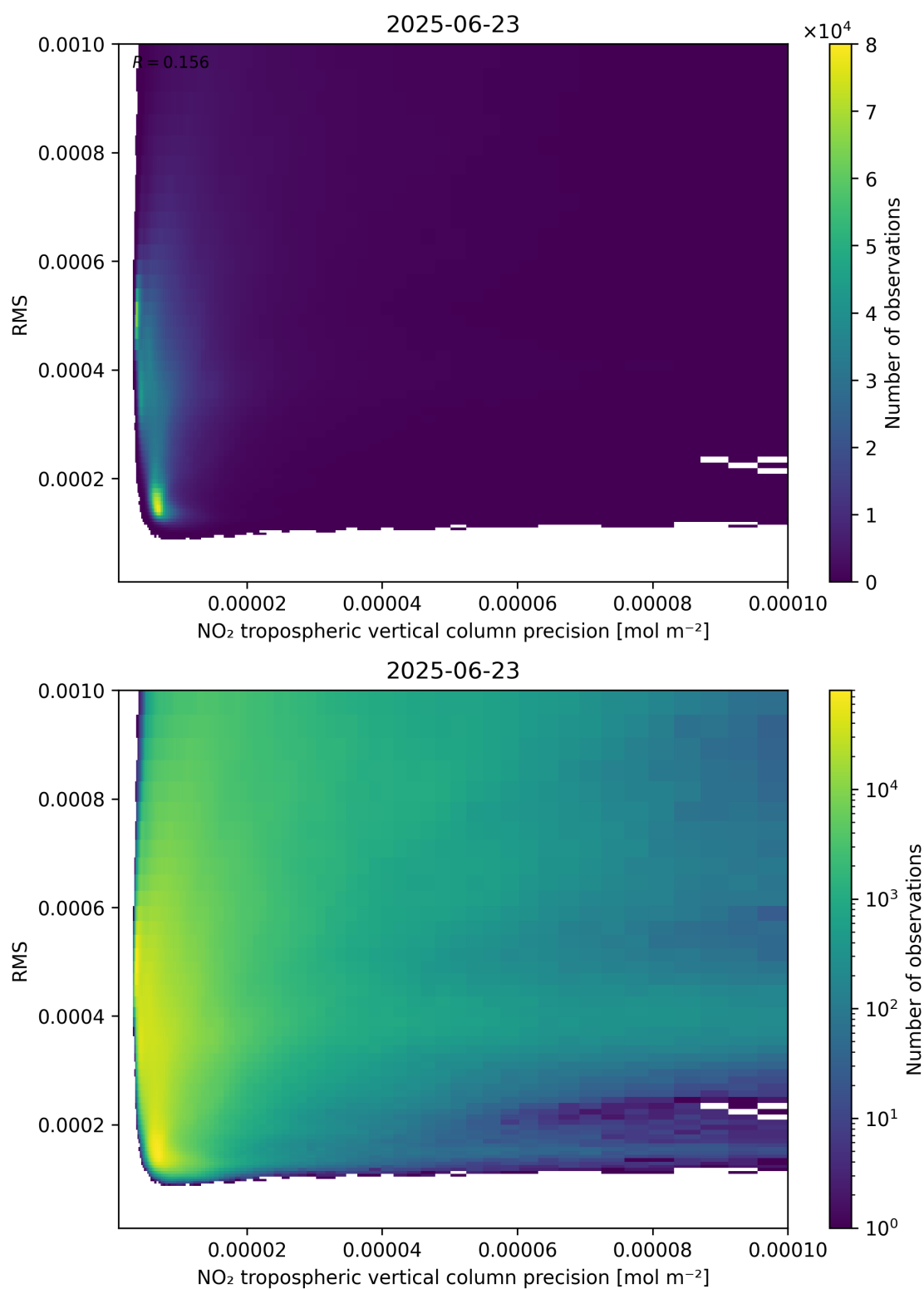
Figure 140: Scatter density plot of “NO 2 tropospheric vertical column precision” against “RMS” for 2025-06-22 to 2025-06-24.
