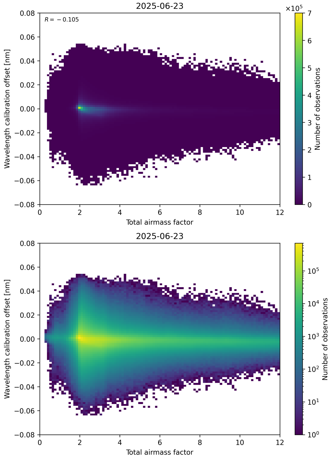
Figure 70: Scatter density plot of “Total airmass factor” against “Wavelength calibration offset” for 2025-06-22 to 2025-06-24.
