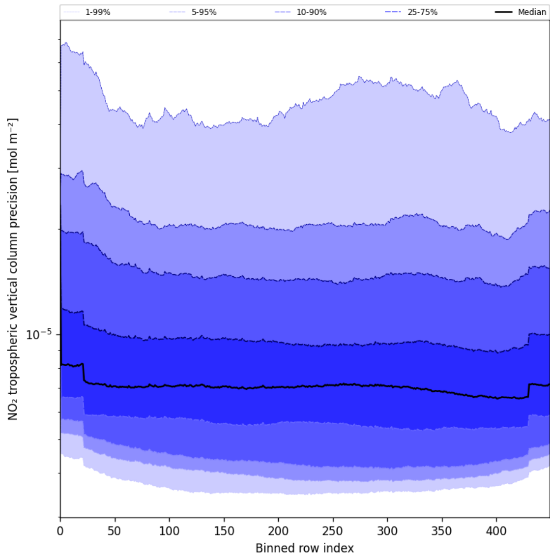
Figure 47: Along track statistics of “NO 2 tropospheric vertical column precision” for 2025-06-22 to 2025-06-24
