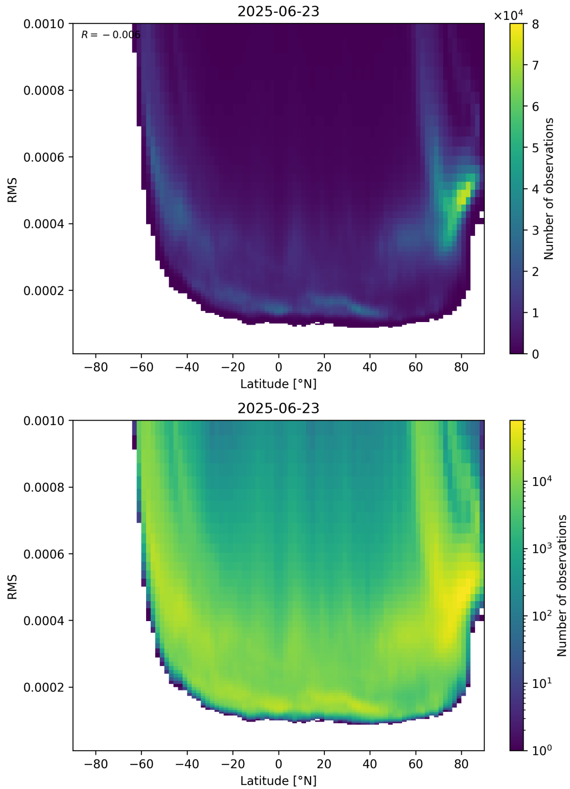
Figure 94: Scatter density plot of “Latitude” against “RMS” for 2025-06-22 to 2025-06-24.
