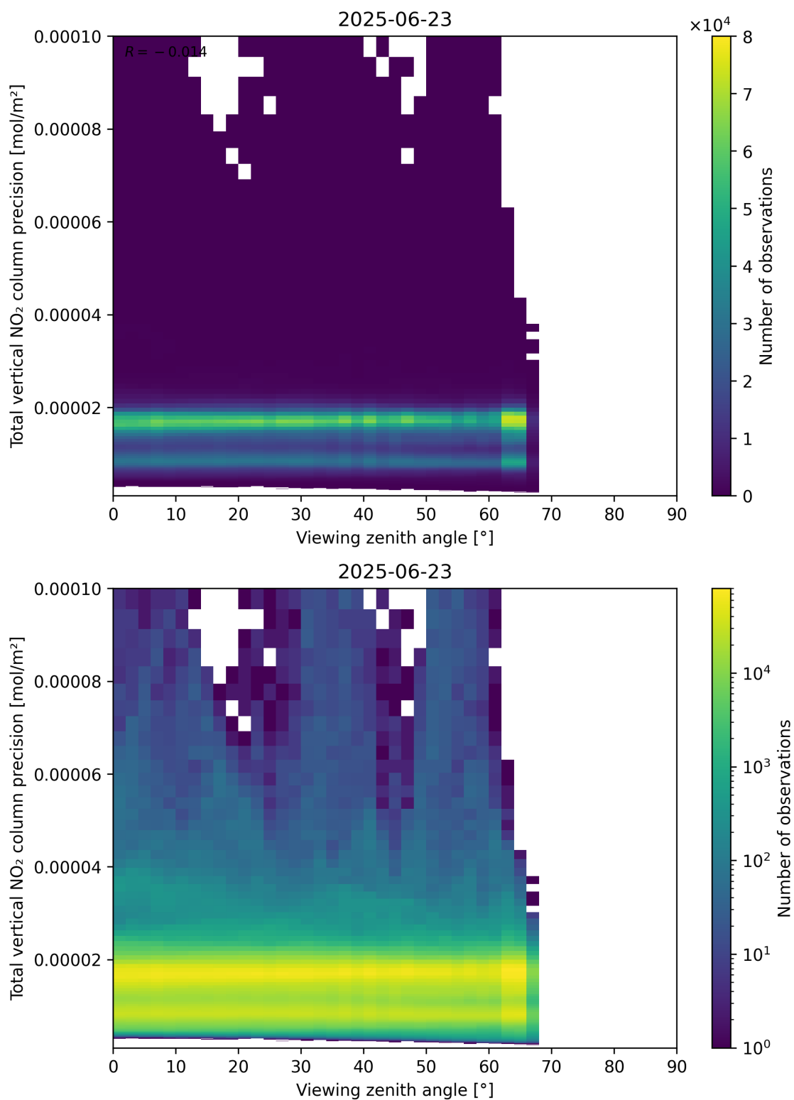
Figure 168: Scatter density plot of “Viewing zenith angle” against “Total vertical NO 2 column precision” for 2025-06-22 to 2025-06-24.
