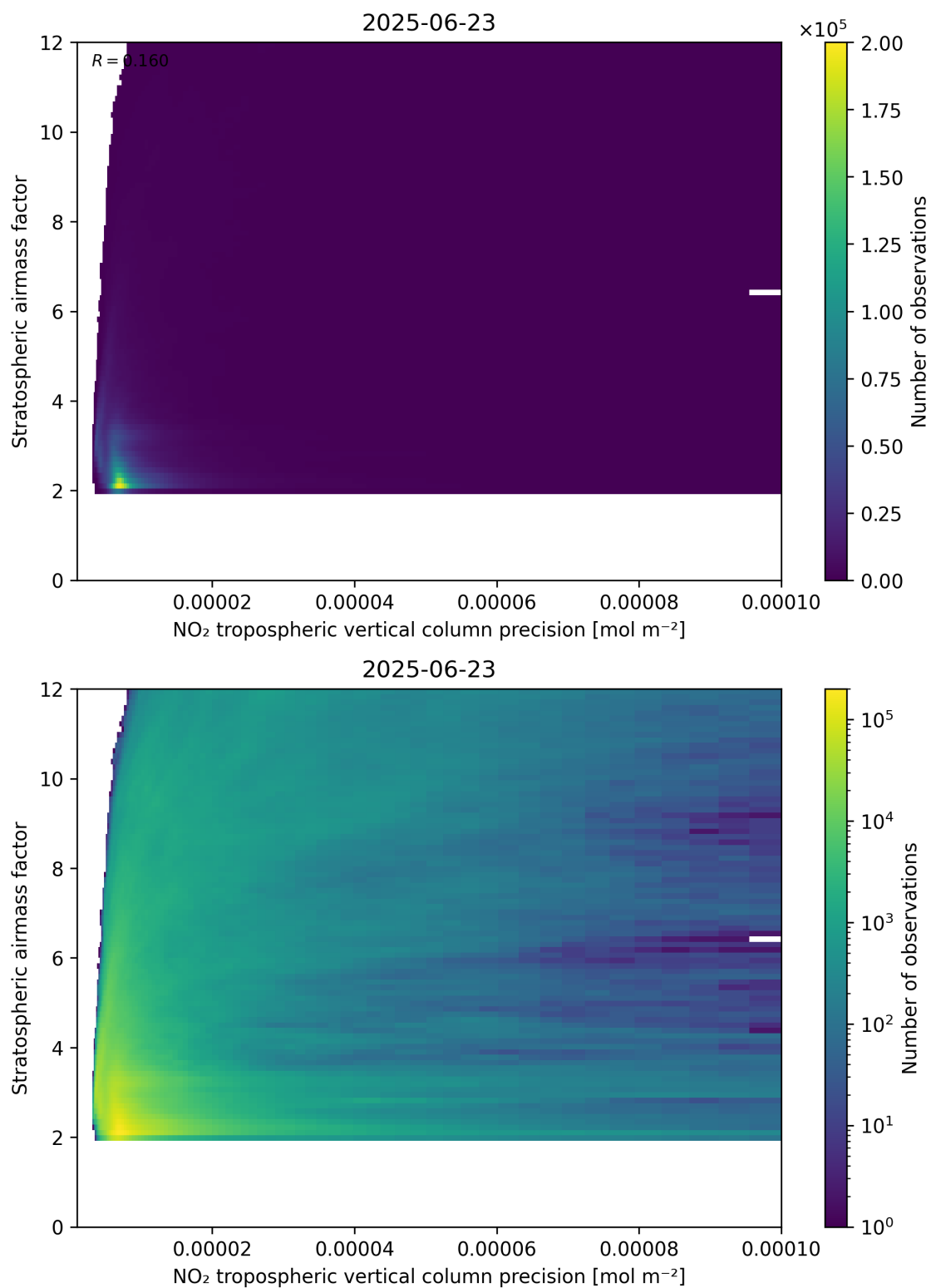
Figure 131: Scatter density plot of “NO 2 tropospheric vertical column precision” against “Stratospheric airmass factor” for 2025-06-22 to 2025-06-24.
