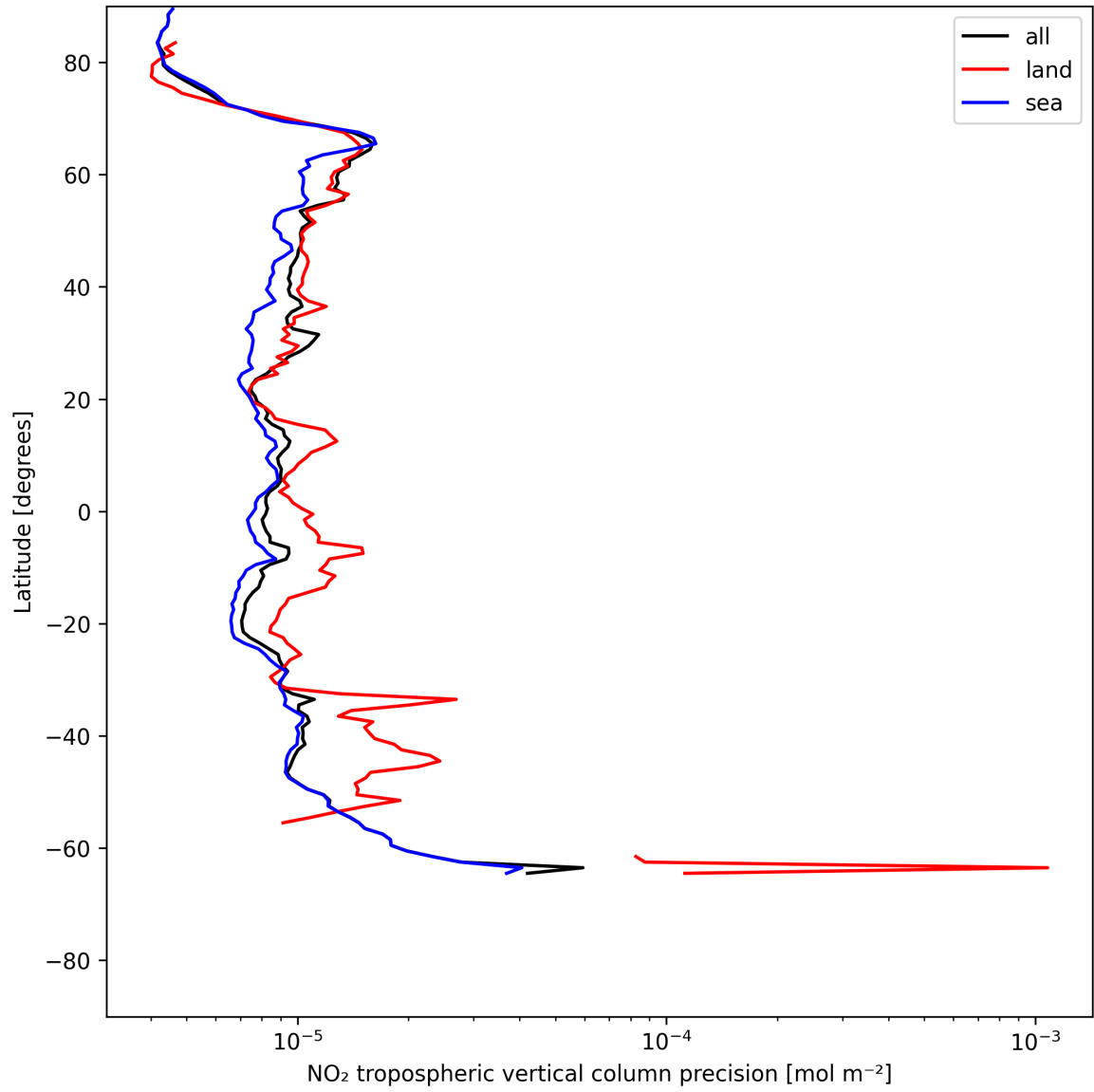
Figure 13: Zonal average of “NO 2 tropospheric vertical column precision” for 2025-06-22 to 2025-06-24.
