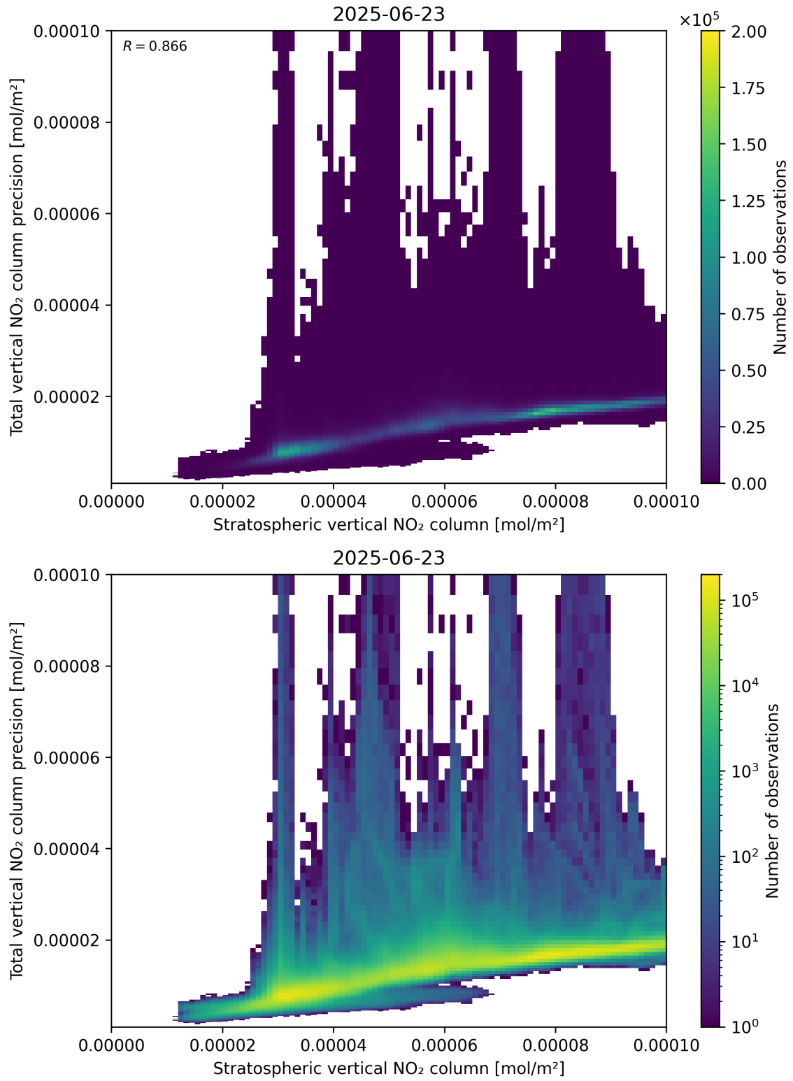
Figure 101: Scatter density plot of “Stratospheric vertical NO 2 column” against “Total vertical NO 2 column precision” for 2025-06-22 to 2025-06-24.
