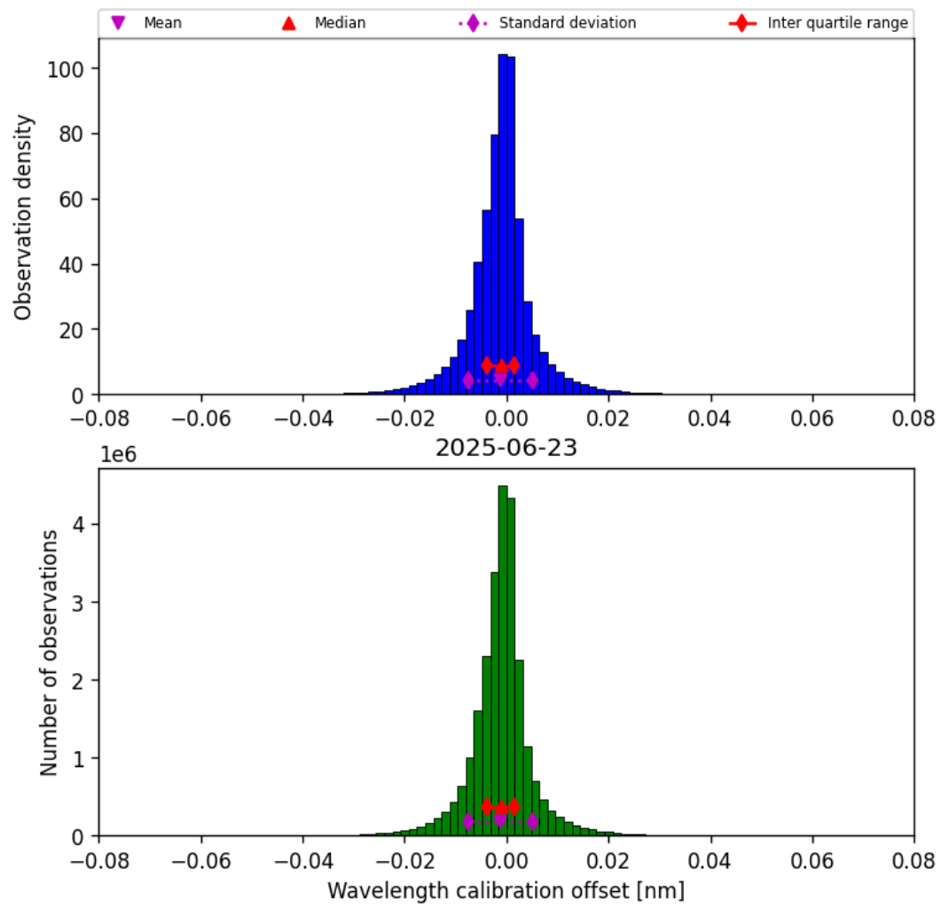
Figure 35: Histogram of “Wavelength calibration offset” for 2025-06-22 to 2025-06-24
