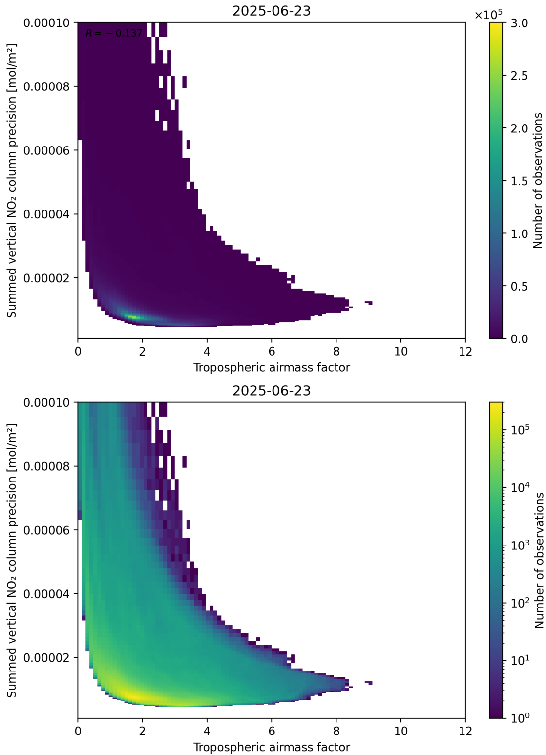
Figure 76: Scatter density plot of “Tropospheric air mass factor” against “Summed vertical NO 2 column precision” for 2025-06-22 to 2025-06-24.
