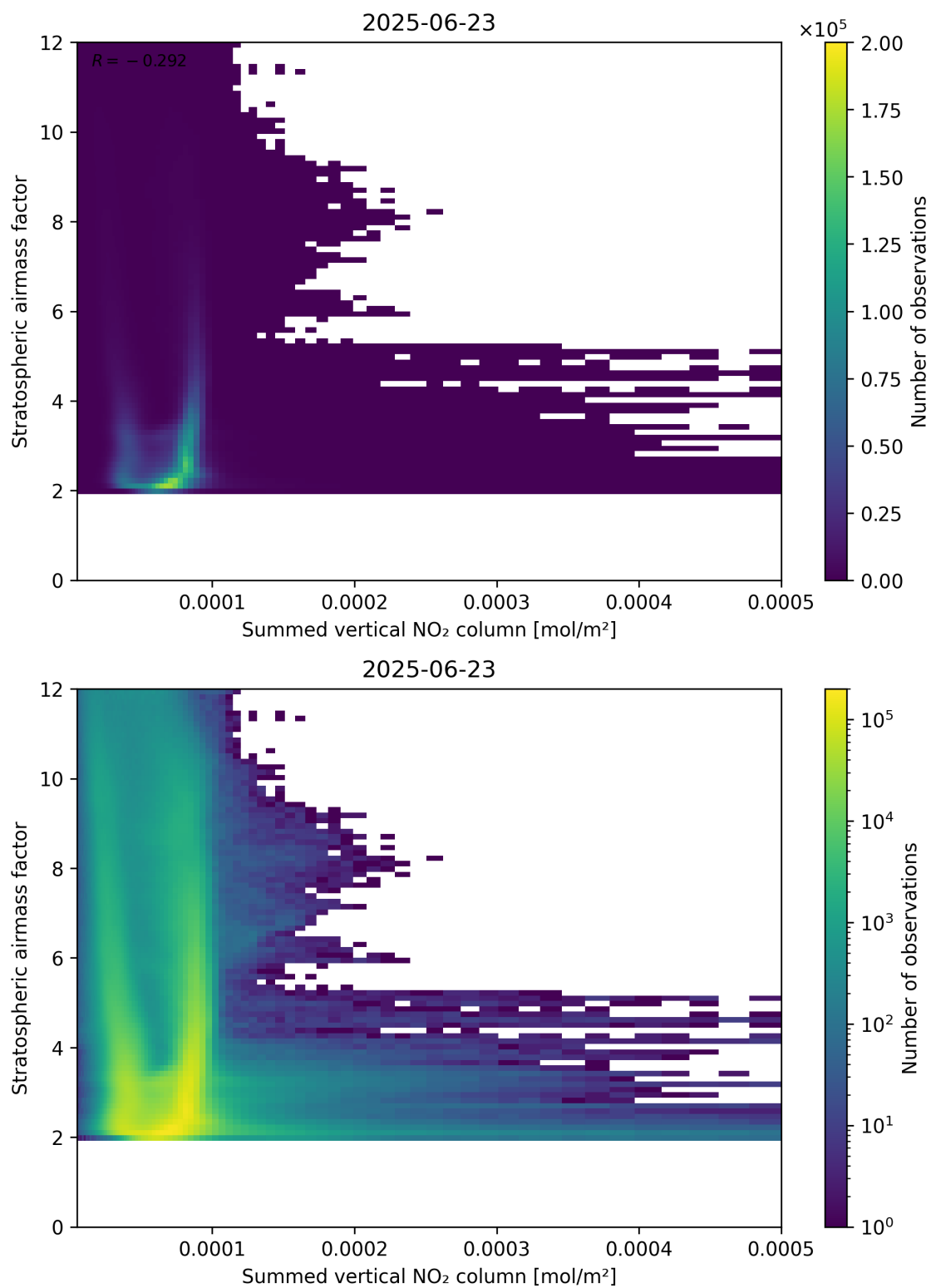
Figure 103: Scatter density plot of “Summed vertical NO 2 column” against “Stratospheric air mass factor” for 2025-06-22 to 2025-06-24.
