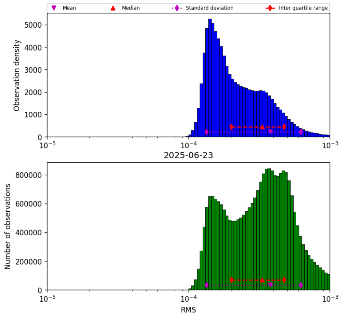
Figure 43: Histogram of “RMS” for 2025-06-22 to 2025-06-24
