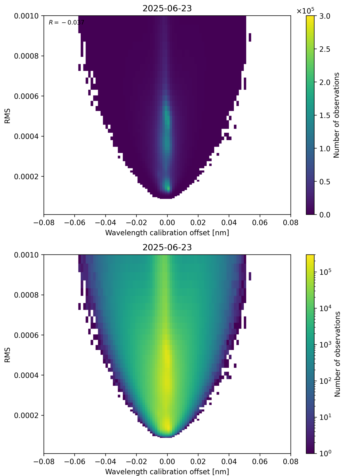
Figure 181: Scatter density plot of “Wavelength calibration offset” against “RMS” for 2025-06-22 to 2025-06-24.
