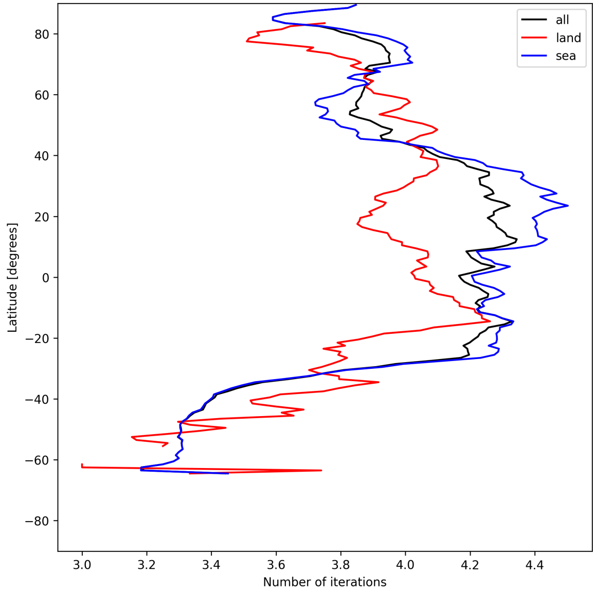
Figure 17: Zonal average of “Number of iterations” for 2025-06-22 to 2025-06-24.
