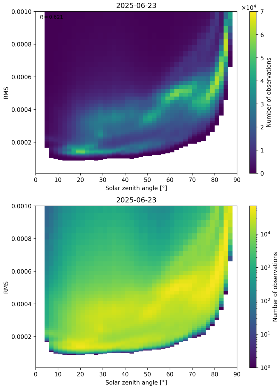
Figure 157: Scatter density plot of “Solar zenith angle” against “RMS” for 2025-06-22 to 2025-06-24.
