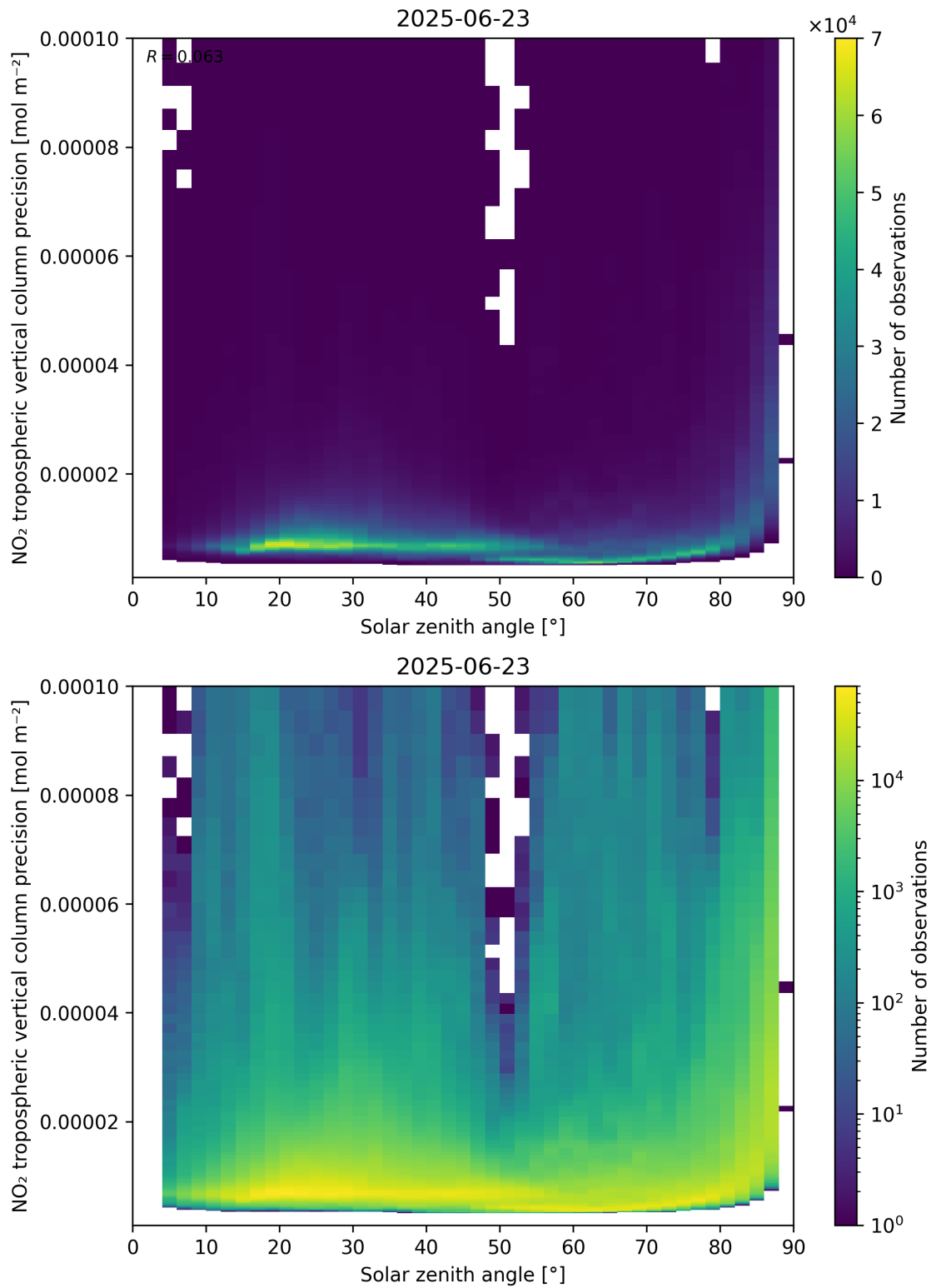
Figure 156: Scatter density plot of “Solar zenith angle” against “NO 2 tropospheric vertical column precision” for 2025-06-22 to 2025-06-24.
