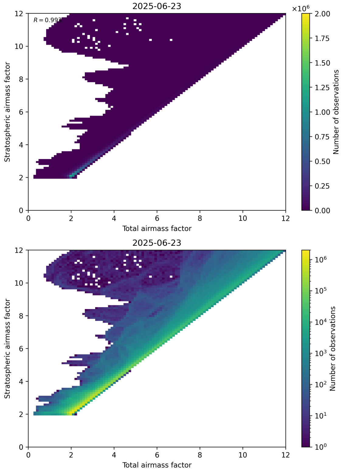
Figure 62: Scatter density plot of “Total airmass factor” against “Stratospheric airmass factor” for 2025-06-22 to 2025-06-24.
