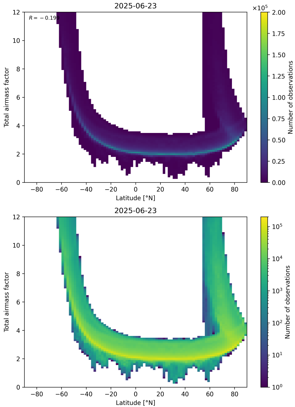
Figure 84: Scatter density plot of “Latitude” against “Total airmass factor” for 2025-06-22 to 2025-06-24.
