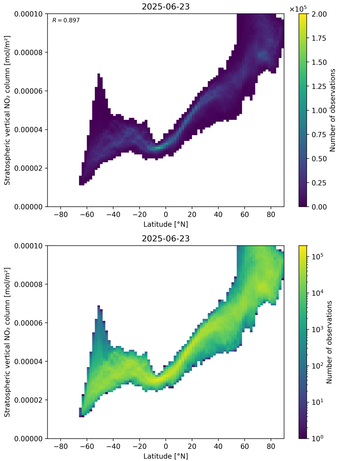
Figure 87: Scatter density plot of “Latitude” against “Stratospheric vertical \text{NO}_2 column” for 2025-06-22 to 2025-06-24.
