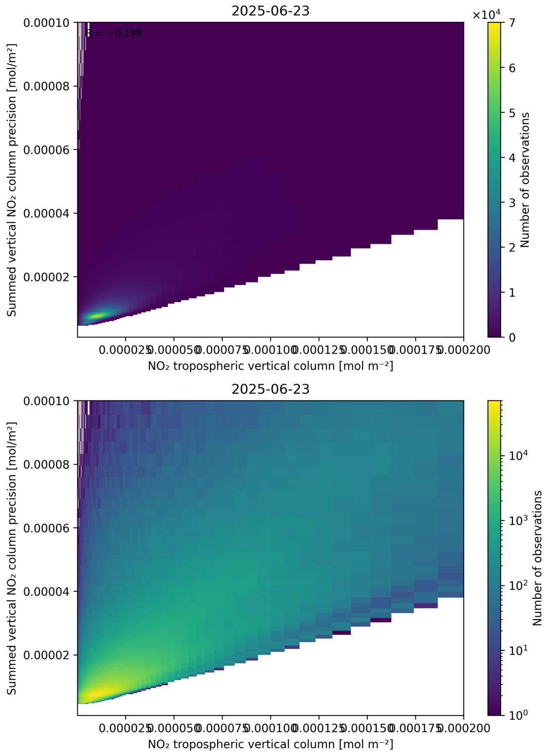
Figure 127: Scatter density plot of “NO 2 tropospheric vertical column” against “Summed vertical NO 2 column precision” for 2025-06-22 to 2025-06-24.
