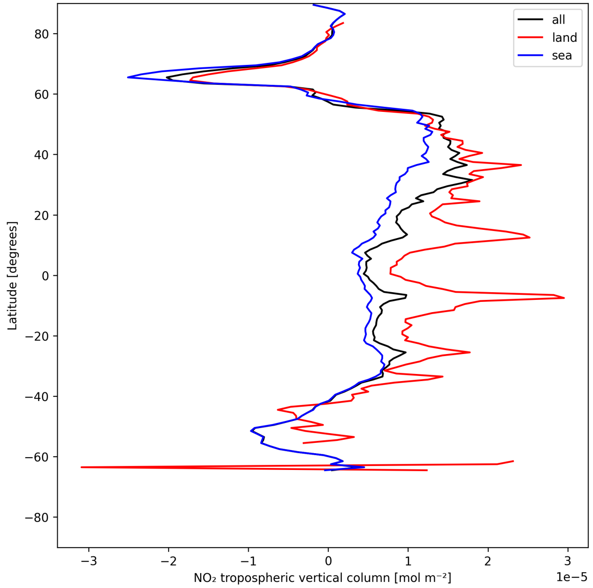
Figure 12: Zonal average of “NO 2 tropospheric vertical column” for 2025-06-22 to 2025-06-24.
