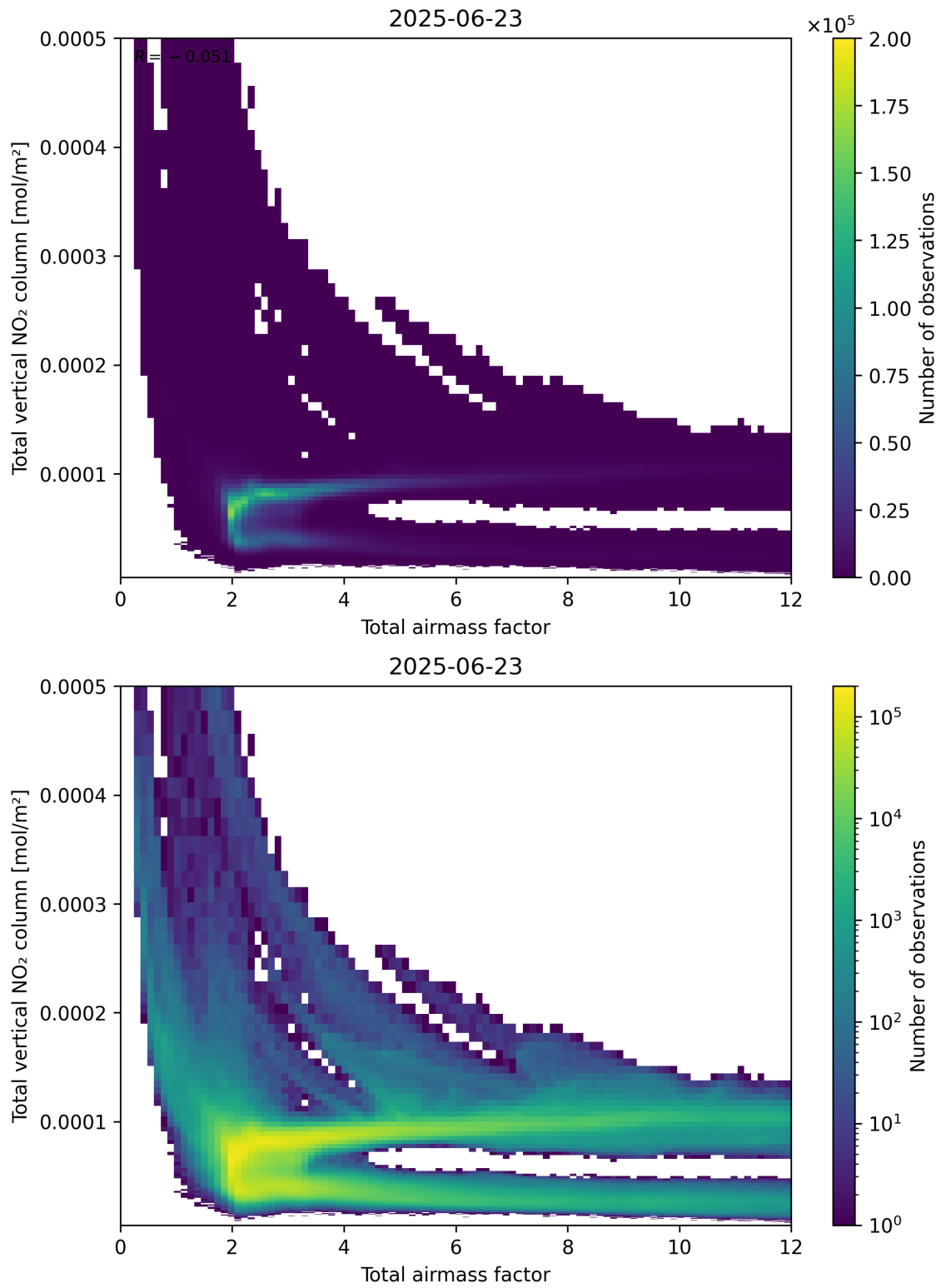
Figure 67: Scatter density plot of “Total airmass factor” against “Total vertical NO 2 column” for 2025-06-22 to 2025-06-24.
