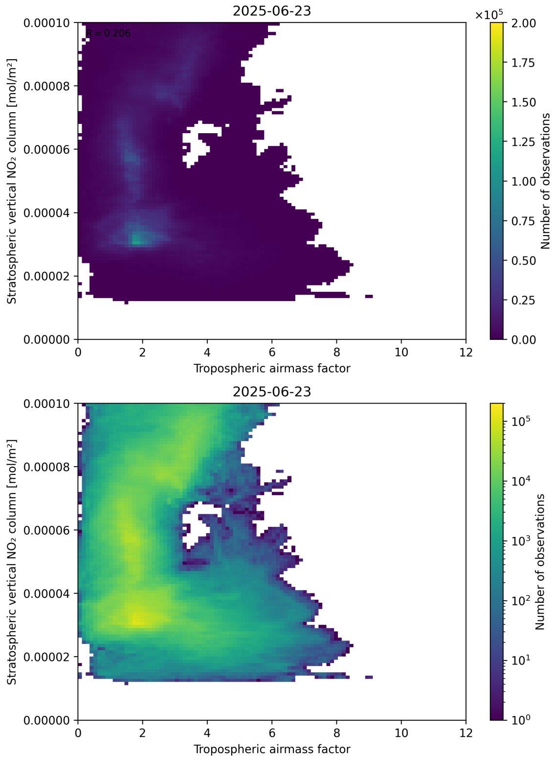
Figure 74: Scatter density plot of “Tropospheric air mass factor” against “Stratospheric vertical NO 2 column” for 2025-06-22 to 2025-06-24.
