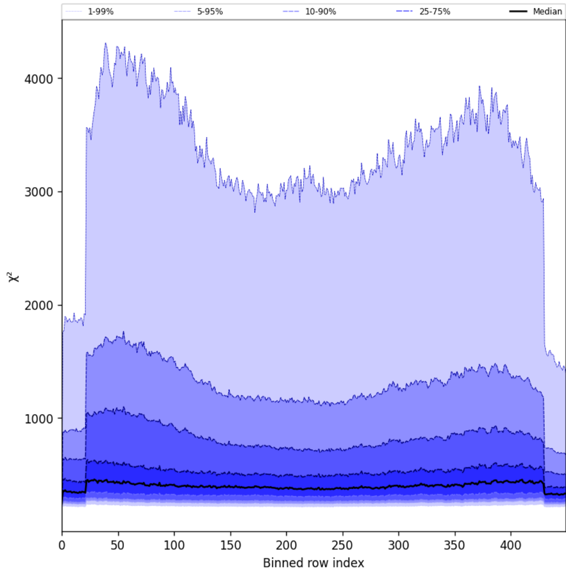
Figure 59: Along track statistics of “ \chi^2 ” for 2025-06-22 to 2025-06-24
