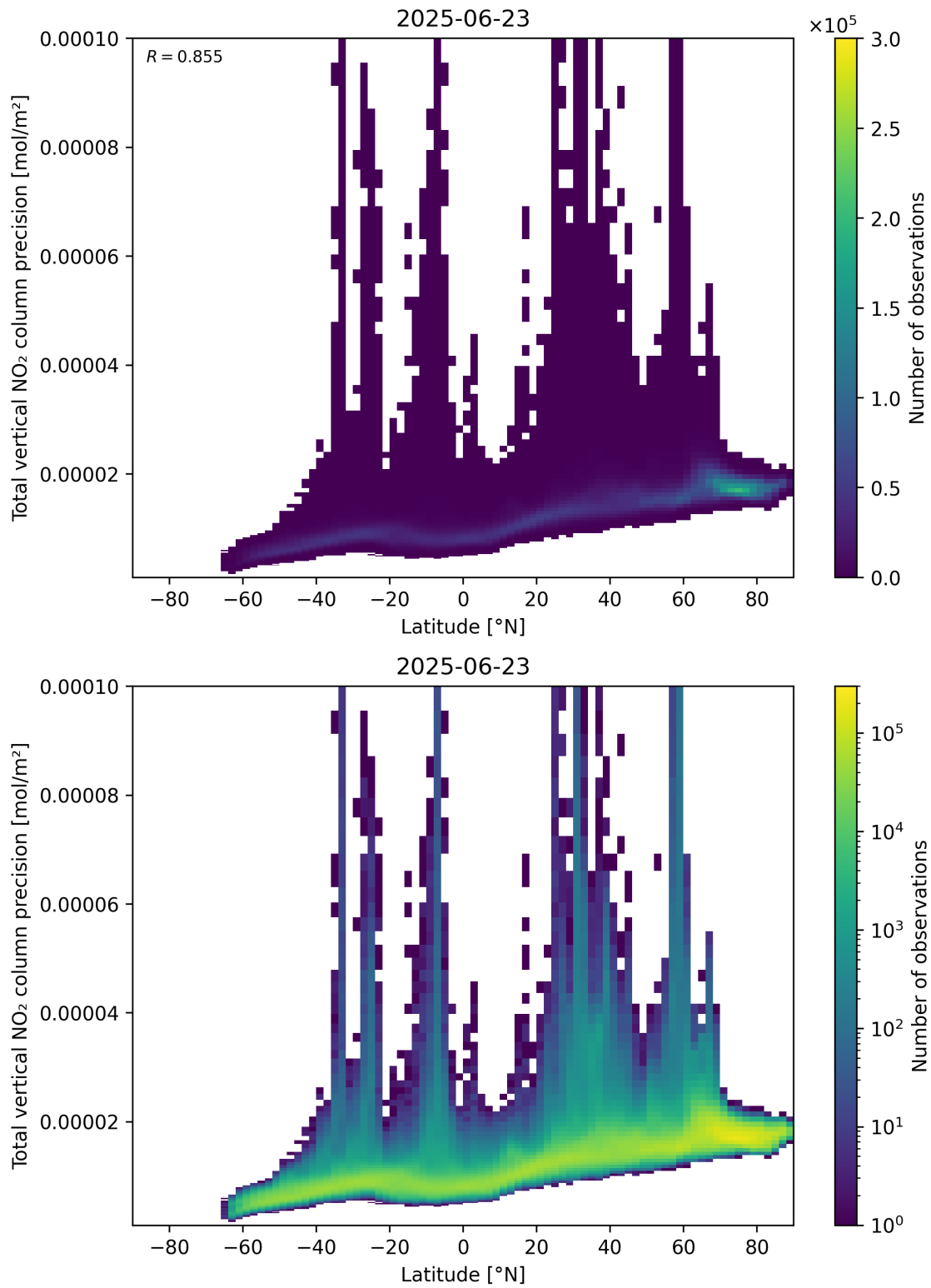
Figure 91: Scatter density plot of “Latitude” against “Total vertical NO 2 column precision” for 2025-06-22 to 2025-06-24.
