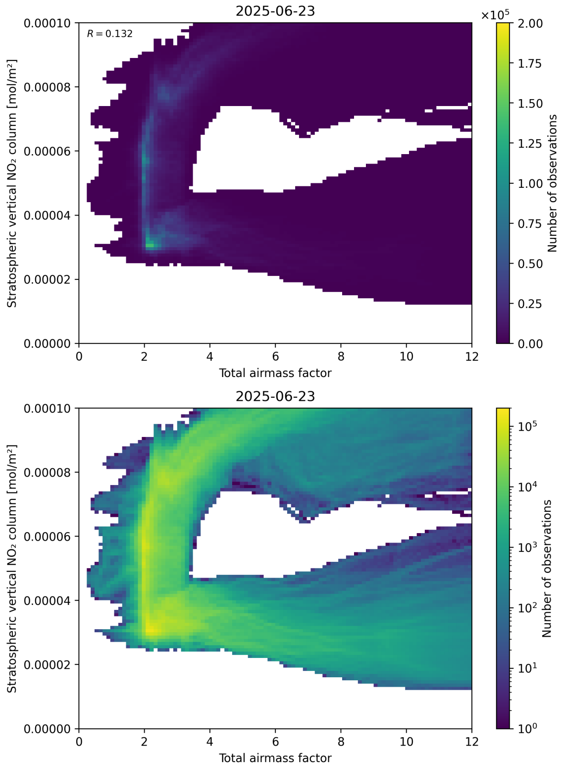
Figure 64: Scatter density plot of “Total airmass factor” against “Stratospheric vertical \text{NO}_2 column” for 2025-06-22 to 2025-06-24.
