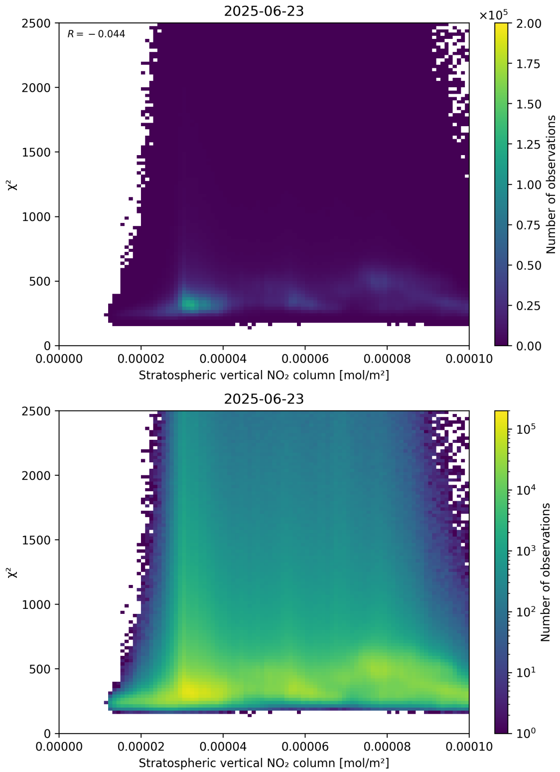
Figure 97: Scatter density plot of “Stratospheric vertical NO 2 column” against “ \chi^2 ” for 2025-06-22 to 2025-06-24.
