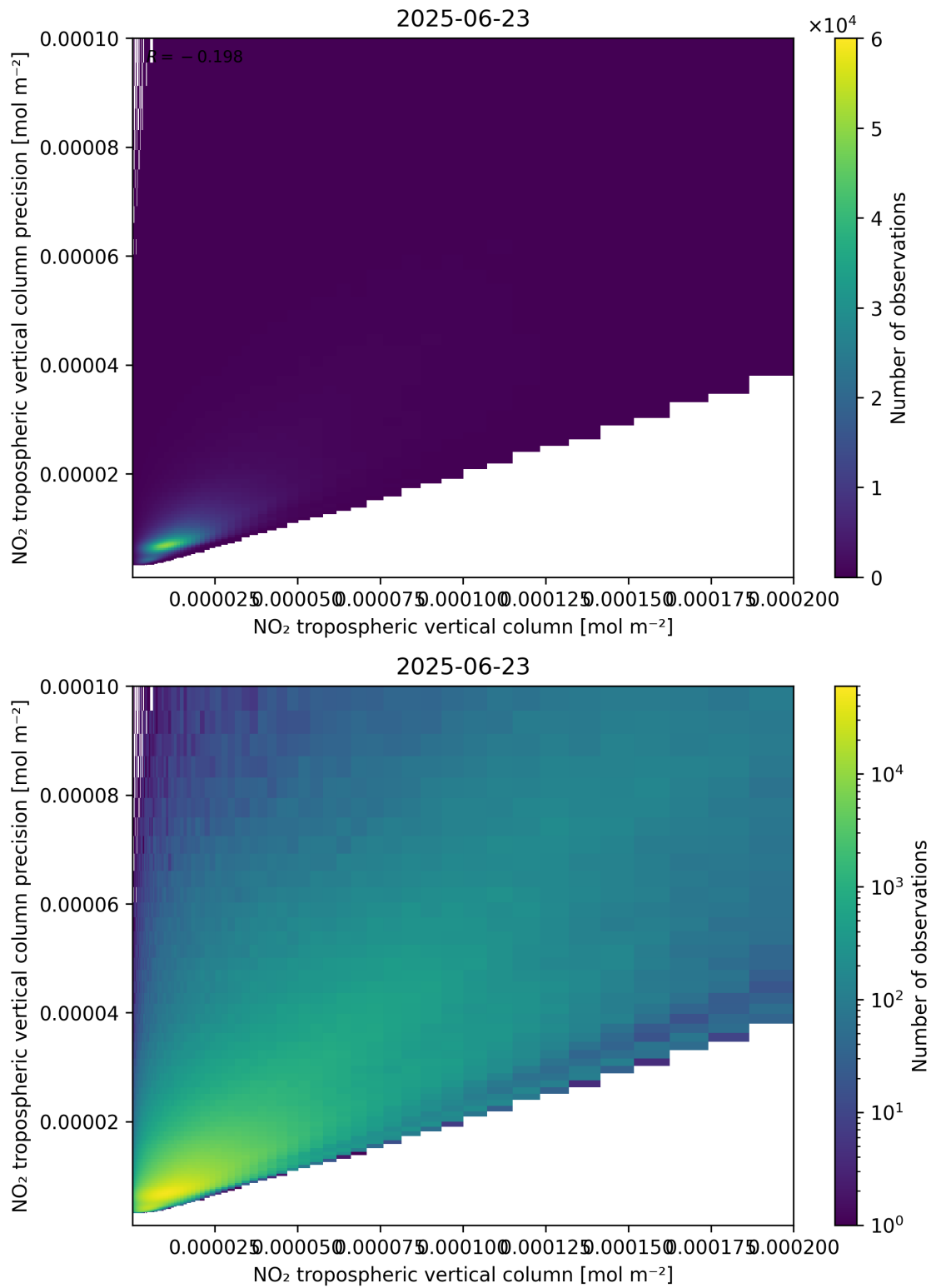
Figure 130: Scatter density plot of “NO 2 tropospheric vertical column” against “NO 2 tropospheric vertical column precision” for 2025-06-22 to 2025-06-24.
