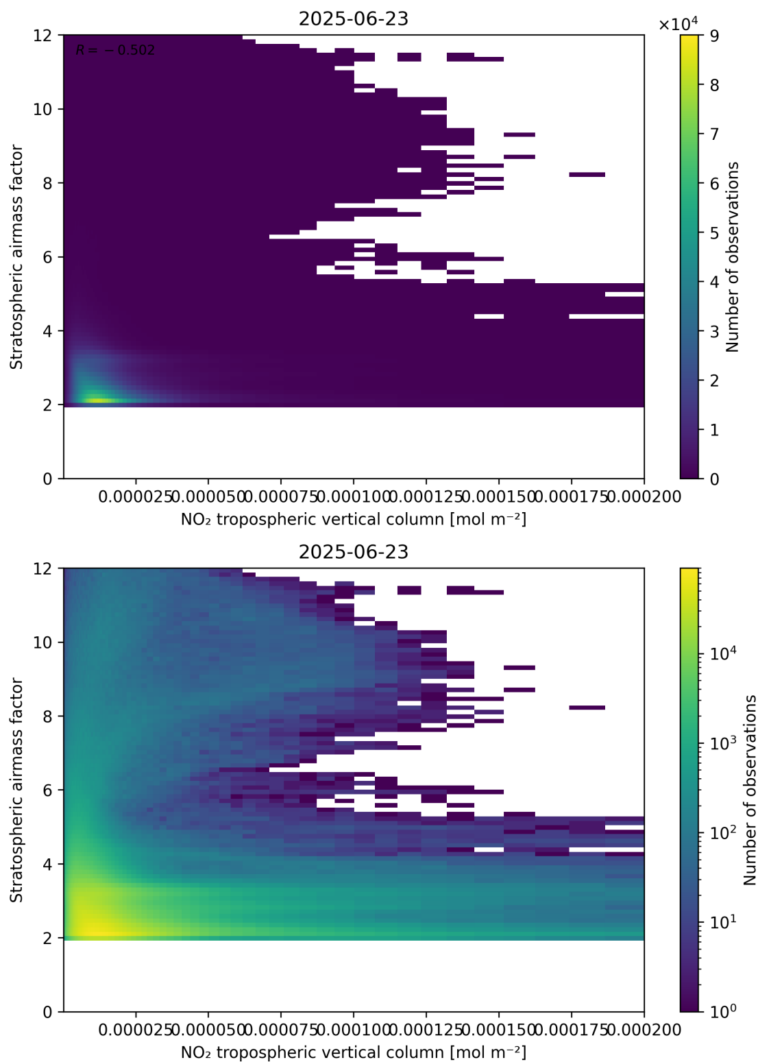
Figure 121: Scatter density plot of “NO 2 tropospheric vertical column” against “Stratospheric air mass factor” for 2025-06-22 to 2025-06-24.
