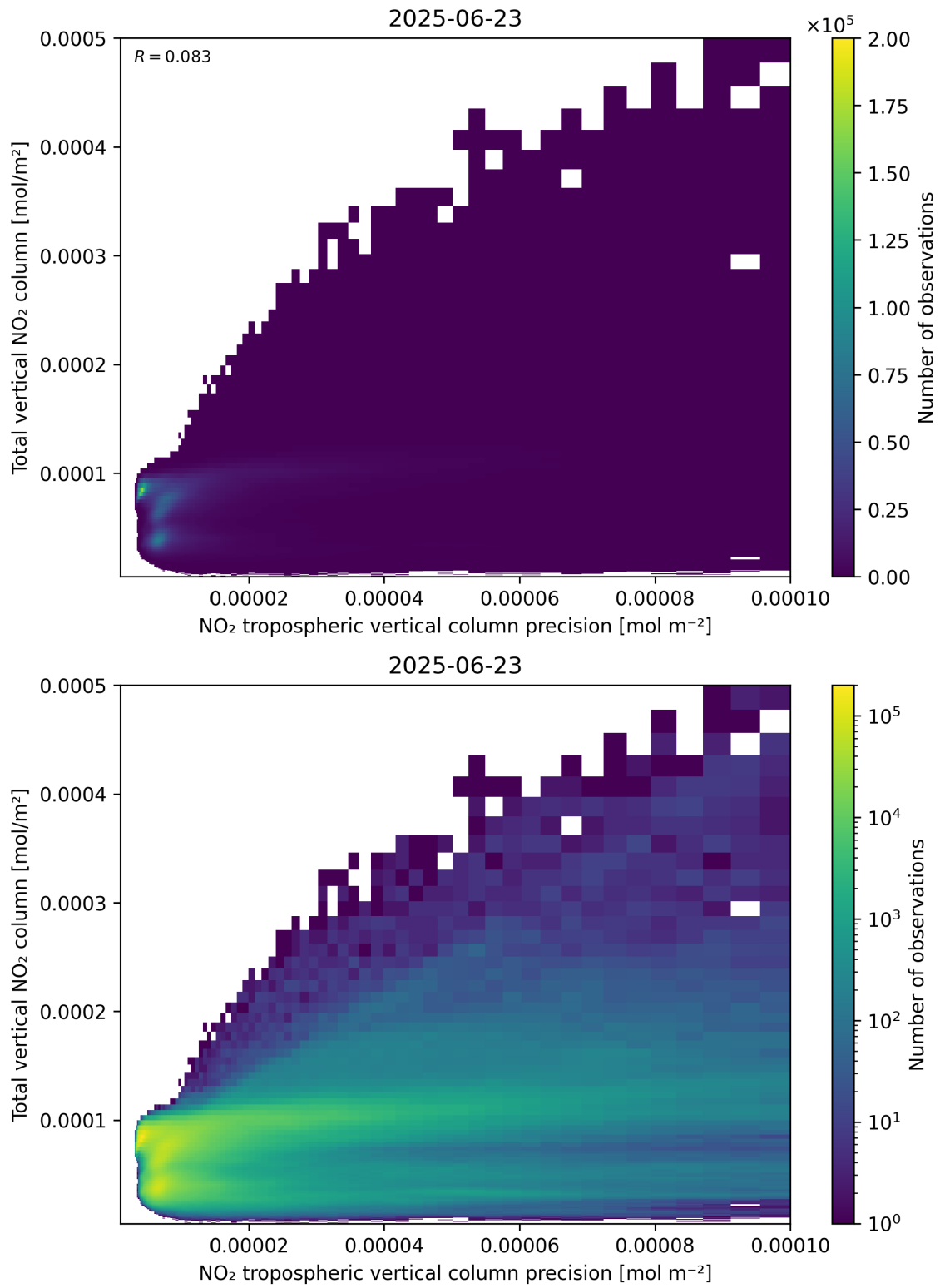
Figure 138: Scatter density plot of “NO 2 tropospheric vertical column precision” against “Total vertical NO 2 column” for 2025-06-22 to 2025-06-24.
