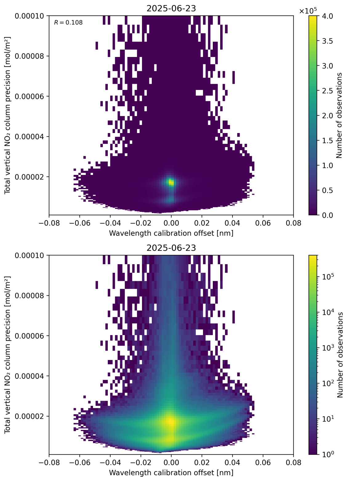
Figure 180: Scatter density plot of “Wavelength calibration offset” against “Total vertical NO 2 column precision” for 2025-06-22 to 2025-06-24.
