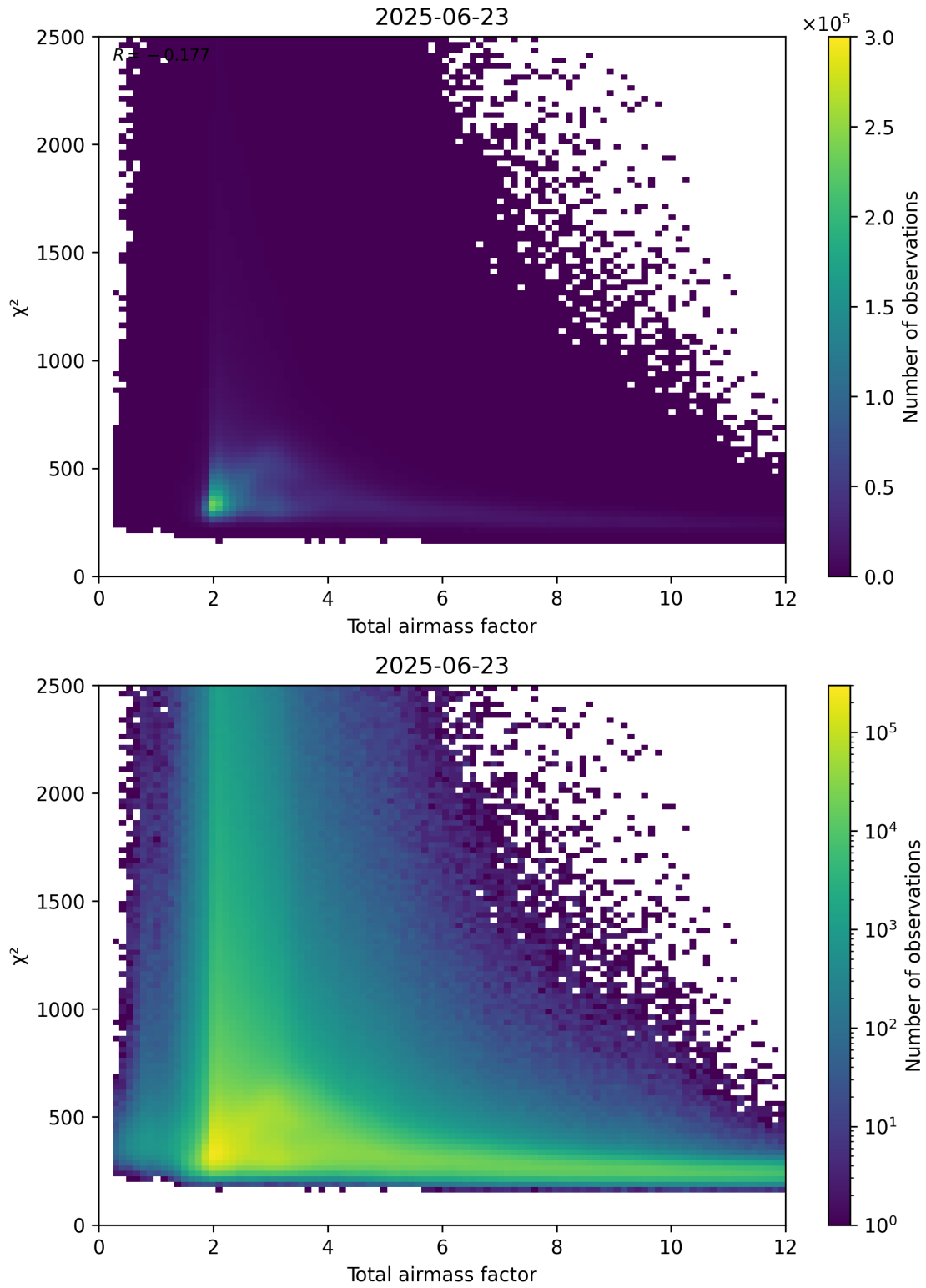
Figure 63: Scatter density plot of “Total airmass factor” against “ \chi^2 ” for 2025-06-22 to 2025-06-24.
