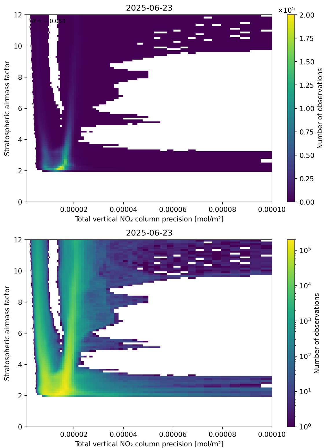
Figure 115: Scatter density plot of “Total vertical NO 2 column precision” against “Stratospheric air mass factor” for 2025-06-22 to 2025-06-24.
