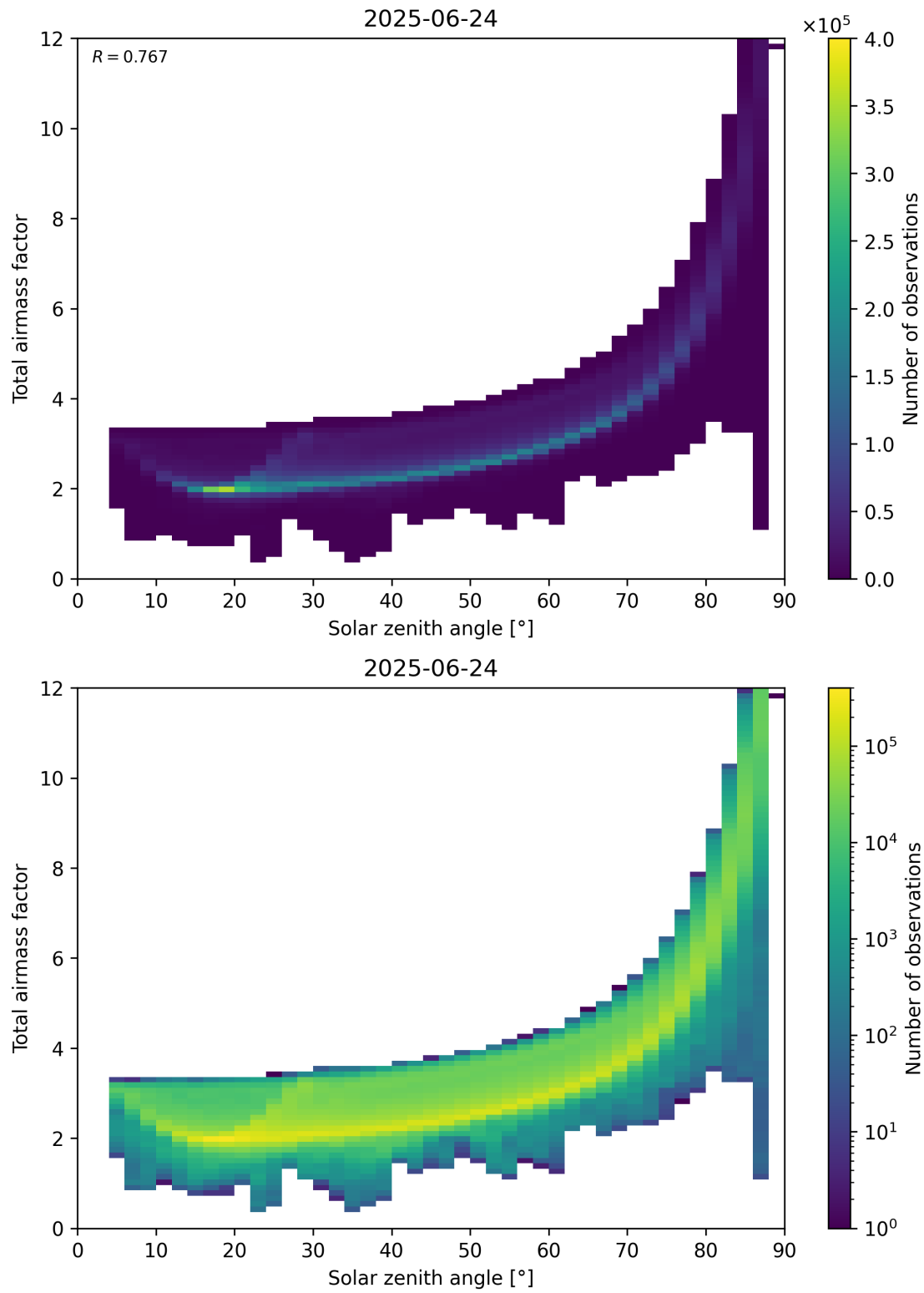
Figure 146: Scatter density plot of “Solar zenith angle” against “Total air mass factor” for 2025-06-23 to 2025-06-25.
