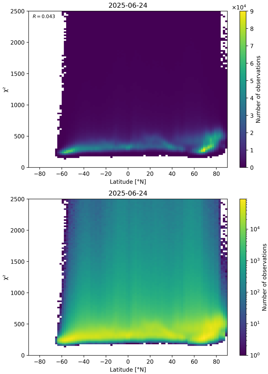
Figure 86: Scatter density plot of “Latitude” against “ \chi^2 ” for 2025-06-23 to 2025-06-25.
