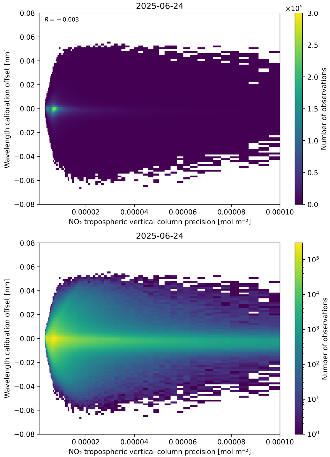
Figure 141: Scatter density plot of “NO 2 tropospheric vertical column precision” against “Wavelength calibration offset” for 2025-06-23 to 2025-06-25.
