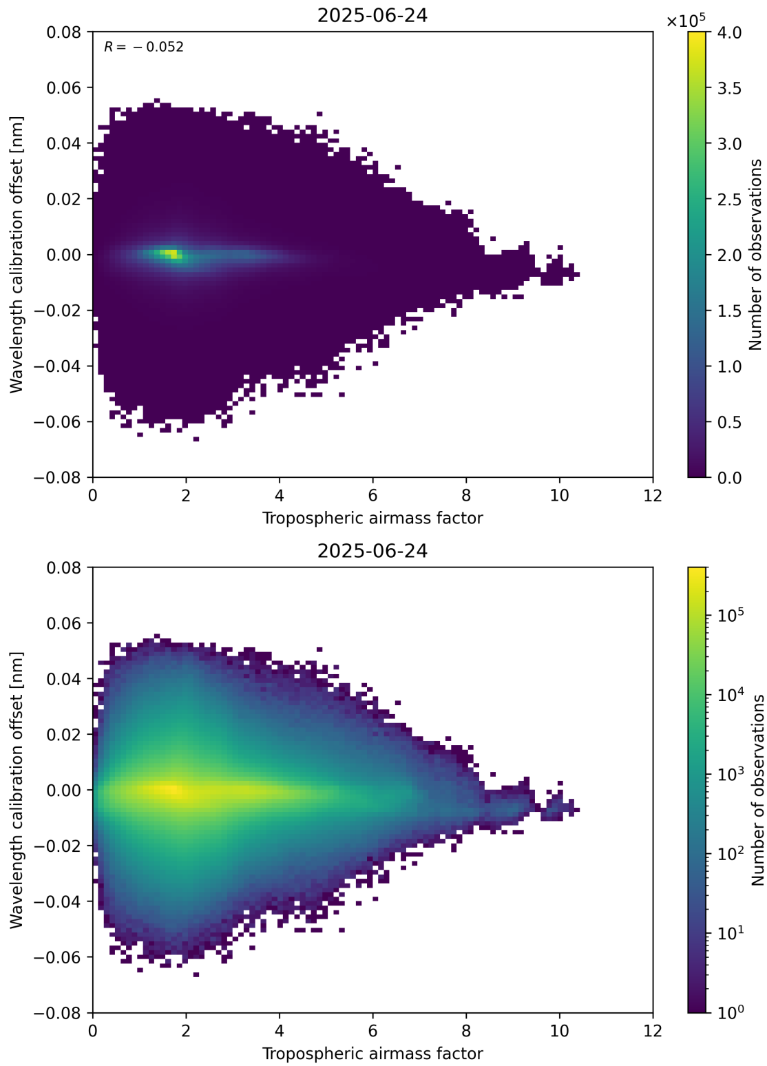
Figure 80: Scatter density plot of “Tropospheric airmass factor” against “Wavelength calibration offset” for 2025-06-23 to 2025-06-25.
