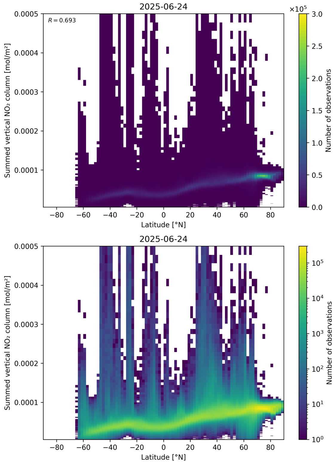
Figure 88: Scatter density plot of “Latitude” against “Summed vertical NO 2 column” for 2025-06-23 to 2025-06-25.
