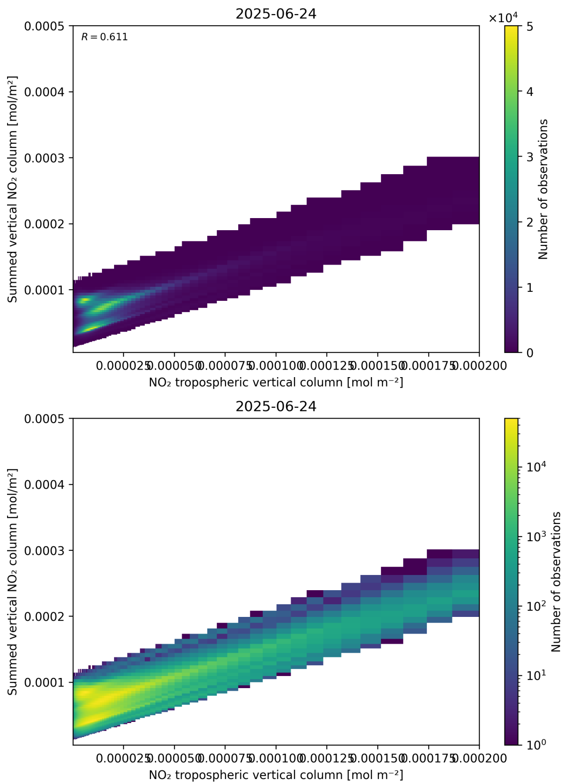
Figure 126: Scatter density plot of “NO 2 tropospheric vertical column” against “Summed vertical NO 2 column” for 2025-06-23 to 2025-06-25.
