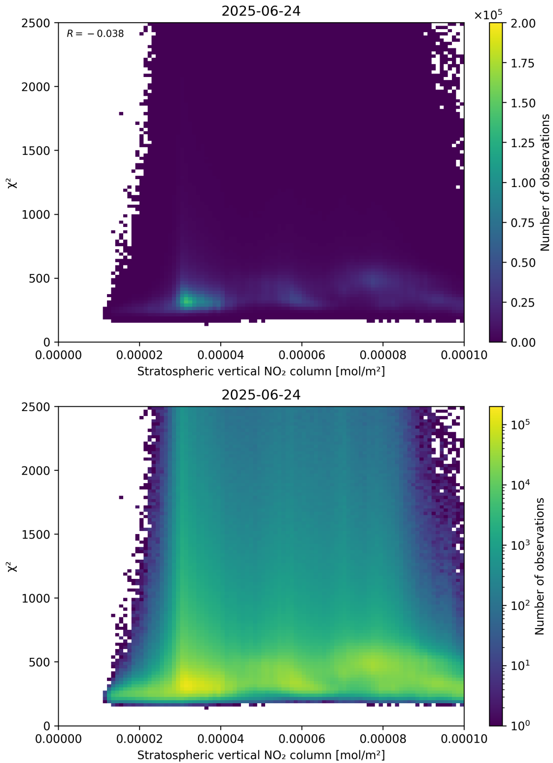
Figure 97: Scatter density plot of “Stratospheric vertical NO 2 column” against “ \chi^2 ” for 2025-06-23 to 2025-06-25.
