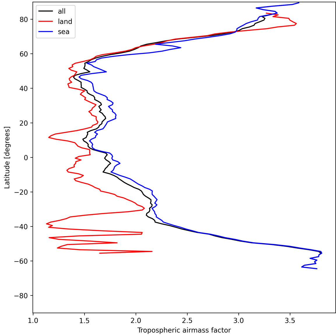
Figure 14: Zonal average of “Tropospheric air mass factor” for 2025-06-23 to 2025-06-25.
