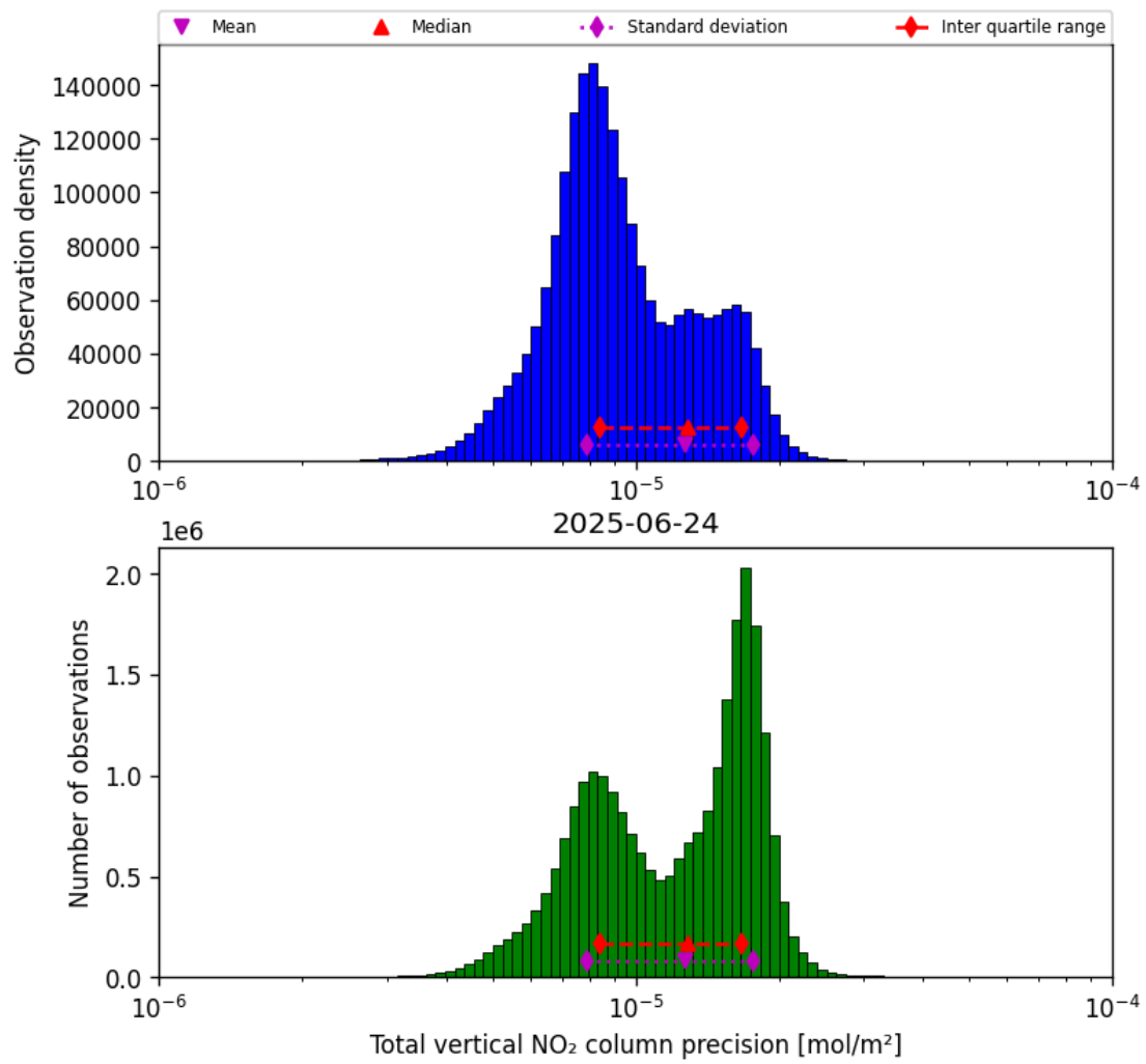
Figure 39: Histogram of “Total vertical NO 2 column precision” for 2025-06-23 to 2025-06-25
