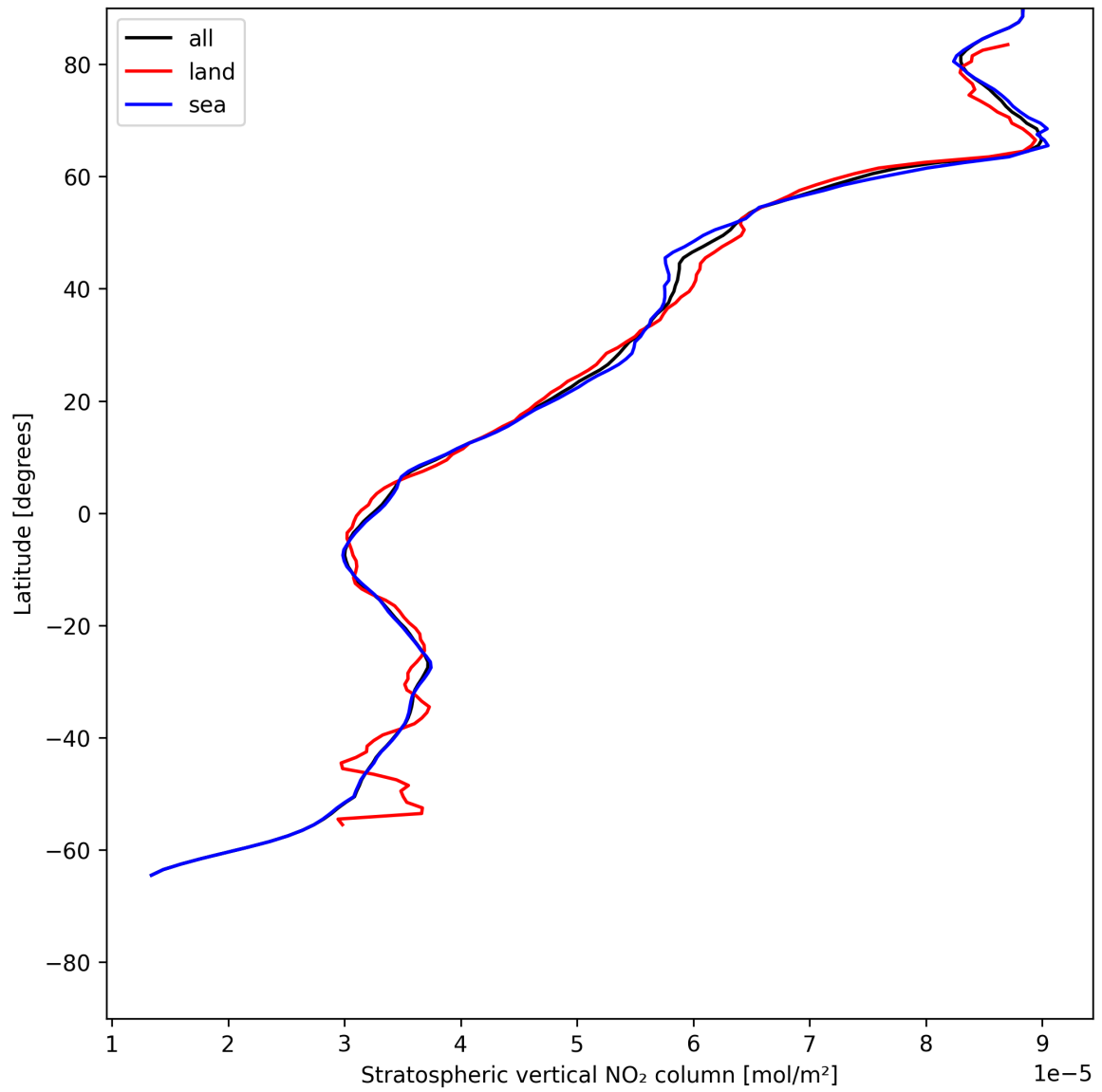
Figure 19: Zonal average of “Stratospheric vertical NO 2 column” for 2025-06-23 to 2025-06-25.
