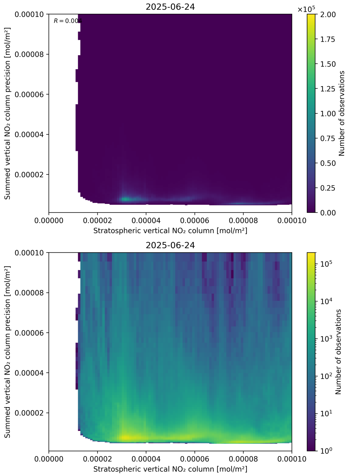
Figure 99: Scatter density plot of “Stratospheric vertical NO 2 column” against “Summed vertical NO 2 column precision” for 2025-06-23 to 2025-06-25.
