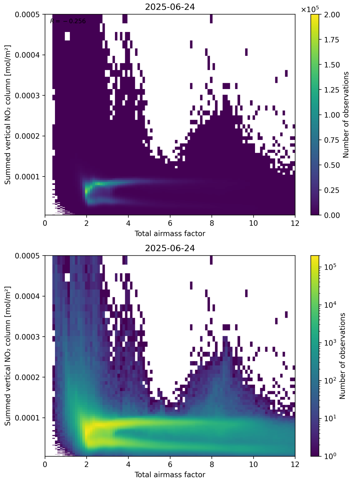
Figure 65: Scatter density plot of “Total airmass factor” against “Summed vertical NO 2 column” for 2025-06-23 to 2025-06-25.
