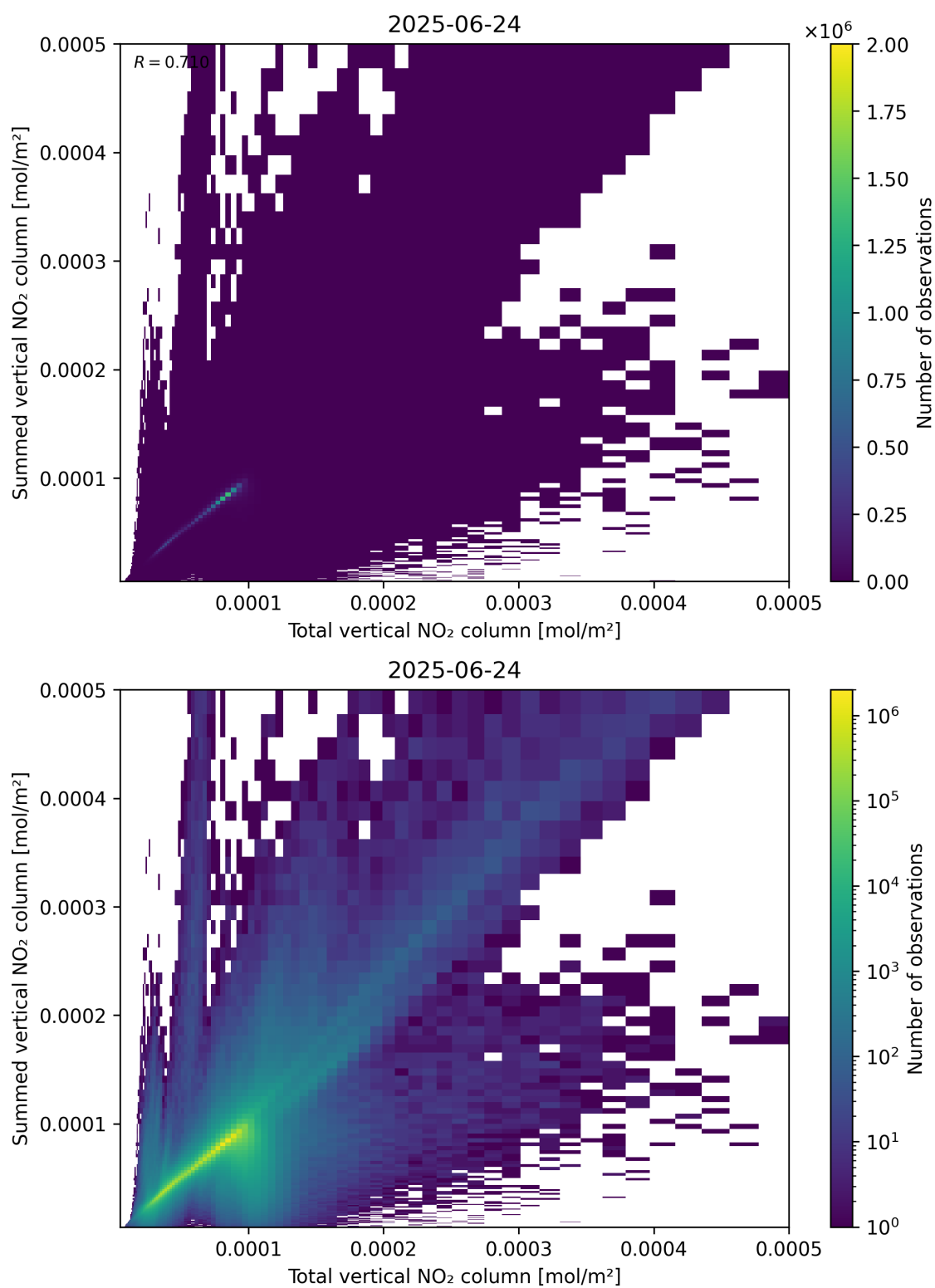
Figure 112: Scatter density plot of “Total vertical NO 2 column” against “Summed vertical NO 2 column” for 2025-06-23 to 2025-06-25.
