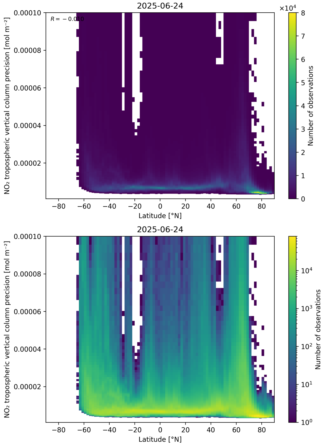
Figure 93: Scatter density plot of “Latitude” against “NO 2 tropospheric vertical column precision” for 2025-06-23 to 2025-06-25.
