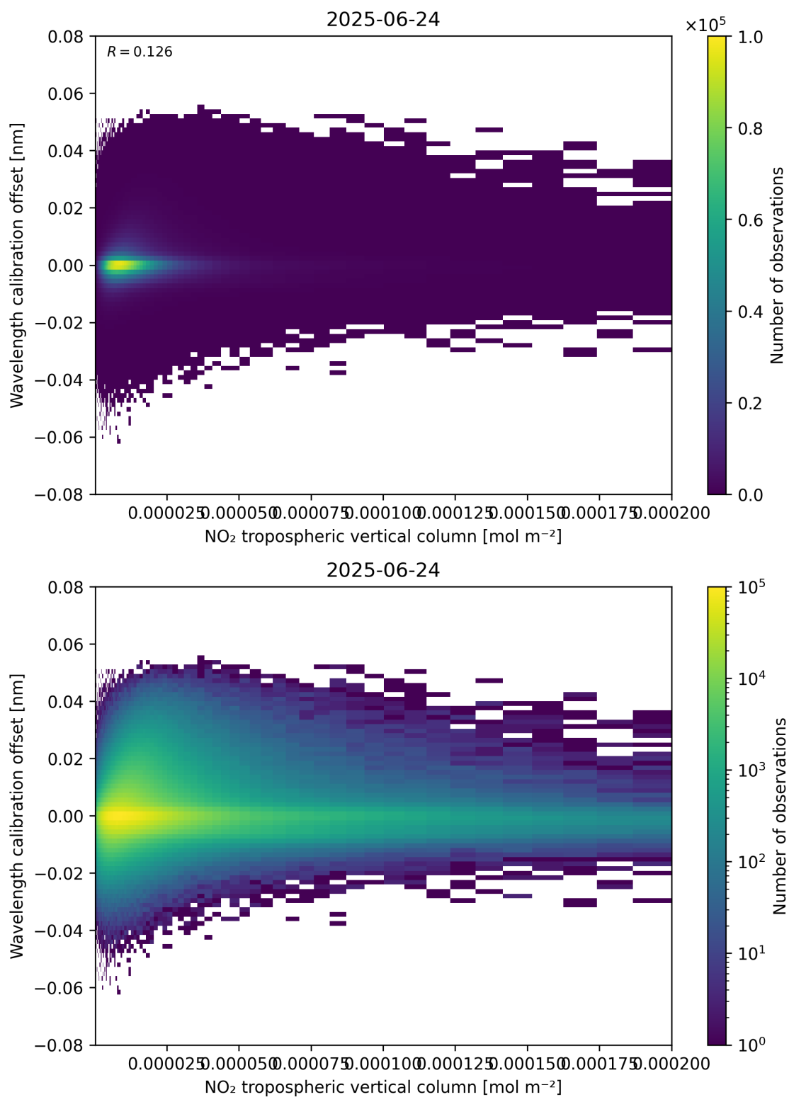
Figure 143: Scatter density plot of “NO 2 tropospheric vertical column” against “Wavelength calibration offset” for 2025-06-23 to 2025-06-25.
