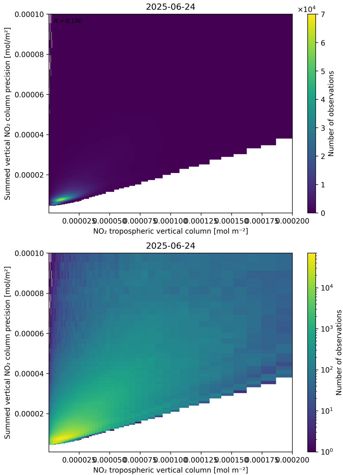
Figure 127: Scatter density plot of “NO 2 tropospheric vertical column” against “Summed vertical NO 2 column precision” for 2025-06-23 to 2025-06-25.
