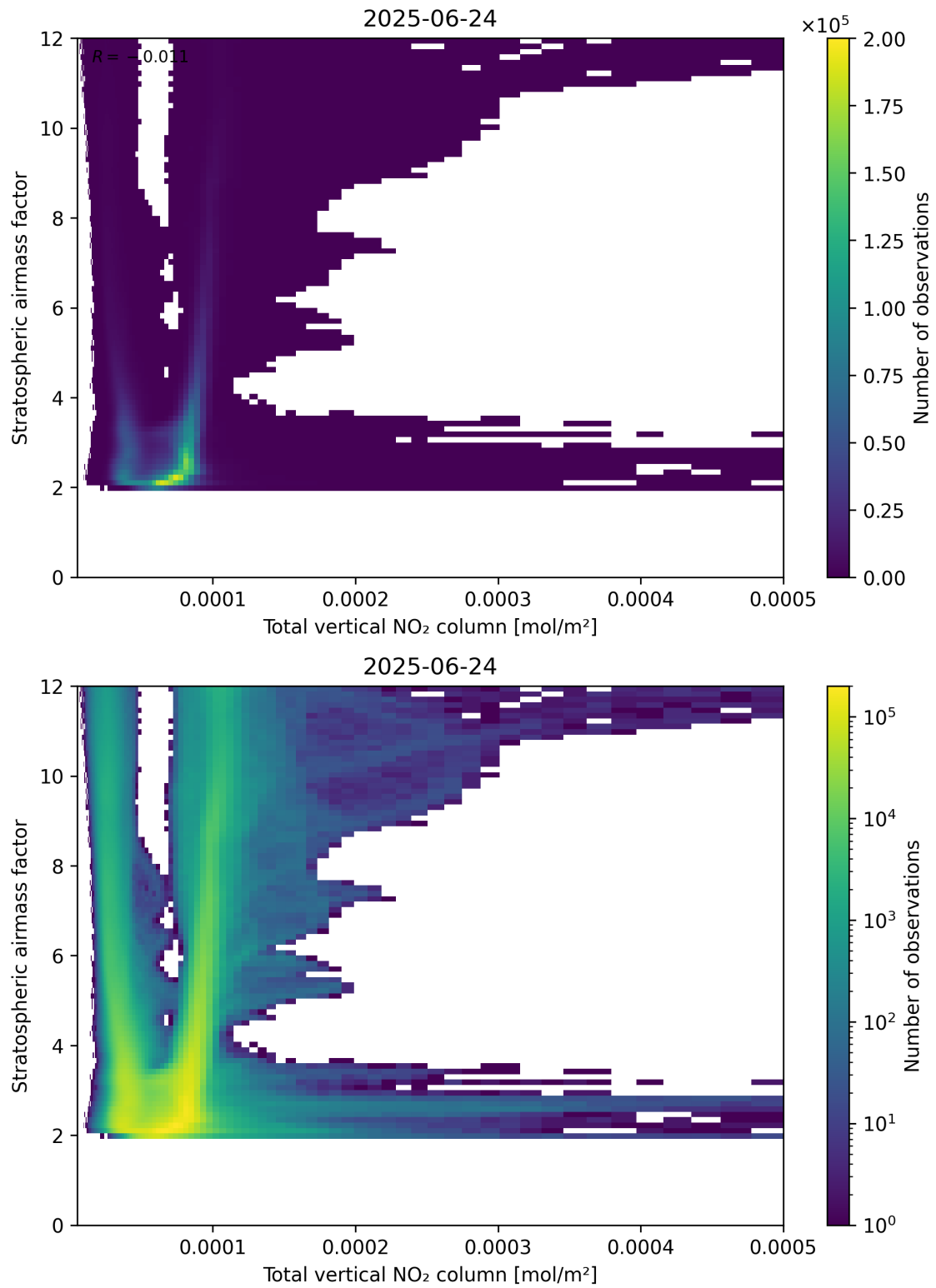
Figure 110: Scatter density plot of “Total vertical NO 2 column” against “Stratospheric airmass factor” for 2025-06-23 to 2025-06-25.
