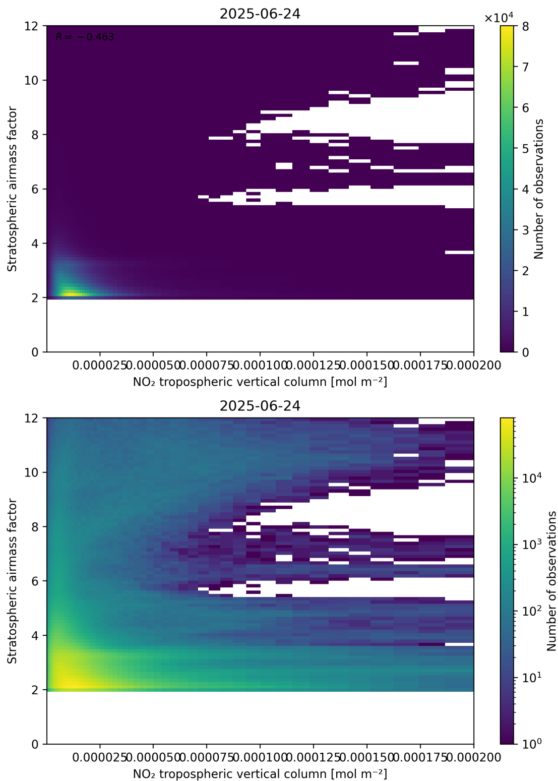
Figure 121: Scatter density plot of “NO 2 tropospheric vertical column” against “Stratospheric air mass factor” for 2025-06-23 to 2025-06-25.
