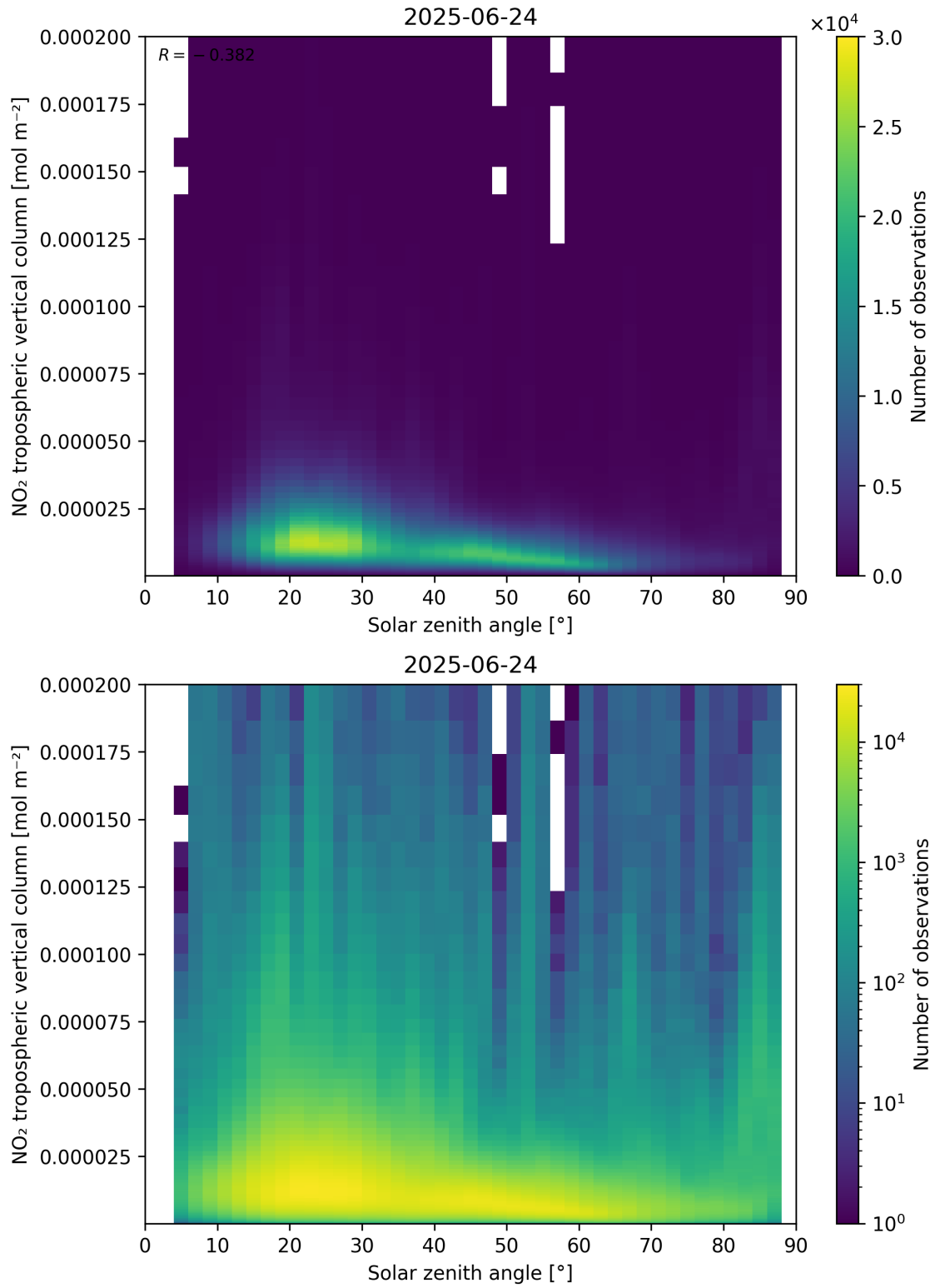
Figure 155: Scatter density plot of “Solar zenith angle” against “NO 2 tropospheric vertical column” for 2025-06-23 to 2025-06-25.
