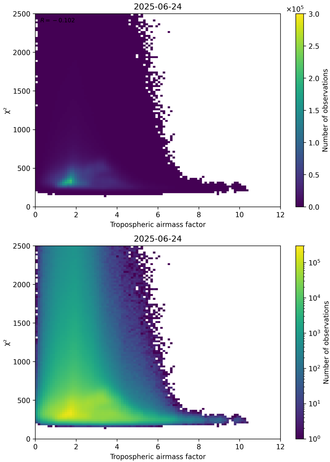
Figure 73: Scatter density plot of “Tropospheric airmass factor” against “ \chi^2 ” for 2025-06-23 to 2025-06-25.
