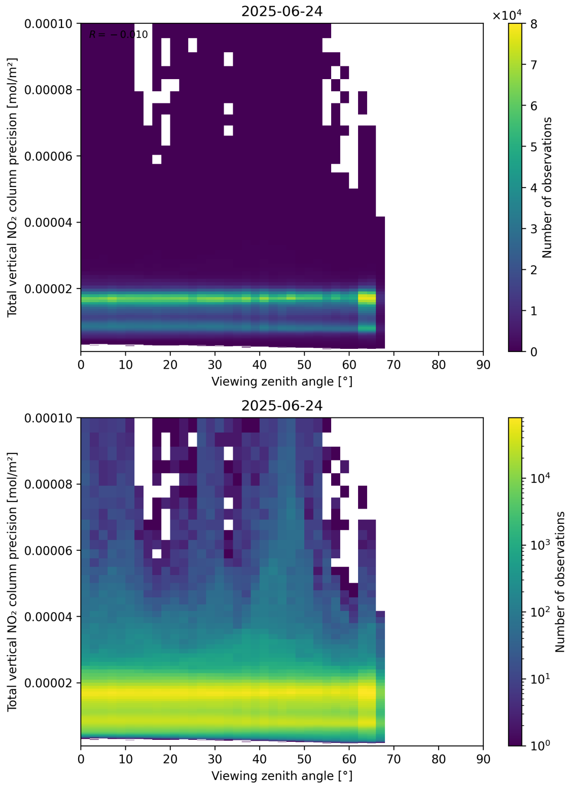
Figure 168: Scatter density plot of “Viewing zenith angle” against “Total vertical NO 2 column precision” for 2025-06-23 to 2025-06-25.
