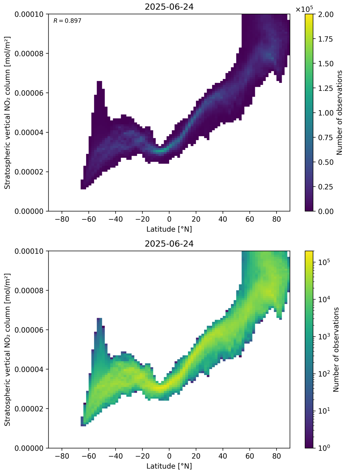
Figure 87: Scatter density plot of “Latitude” against “Stratospheric vertical \text{NO}_2 column” for 2025-06-23 to 2025-06-25.
