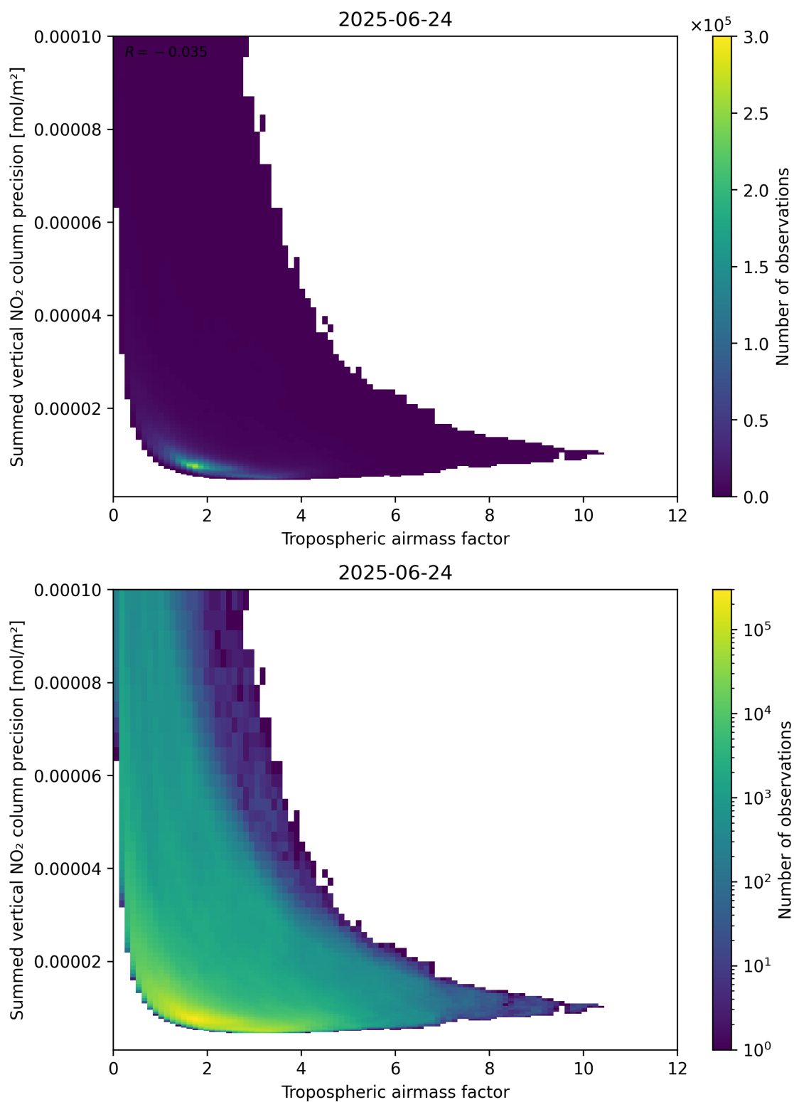
Figure 76: Scatter density plot of “Tropospheric air mass factor” against “Summed vertical NO 2 column precision” for 2025-06-23 to 2025-06-25.
