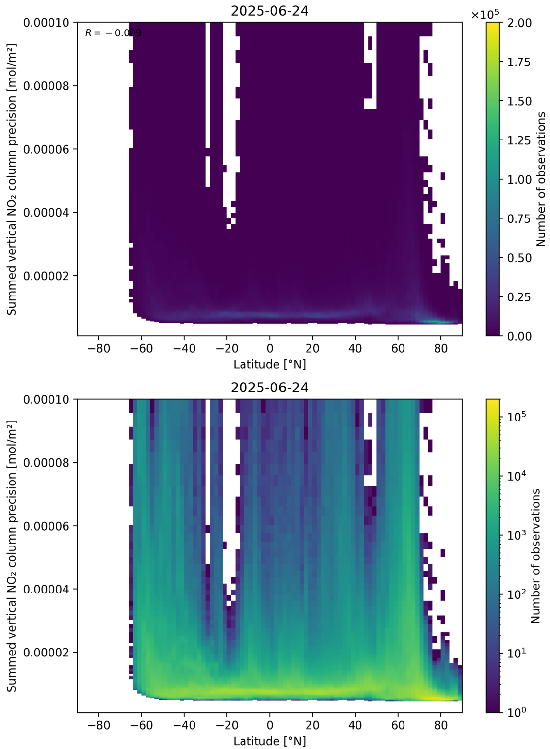
Figure 89: Scatter density plot of “Latitude” against “Summed vertical NO 2 column precision” for 2025-06-23 to 2025-06-25.
