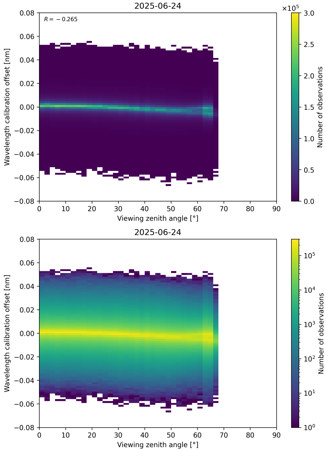
Figure 173: Scatter density plot of “Viewing zenith angle” against “Wavelength calibration offset” for 2025-06-23 to 2025-06-25.
