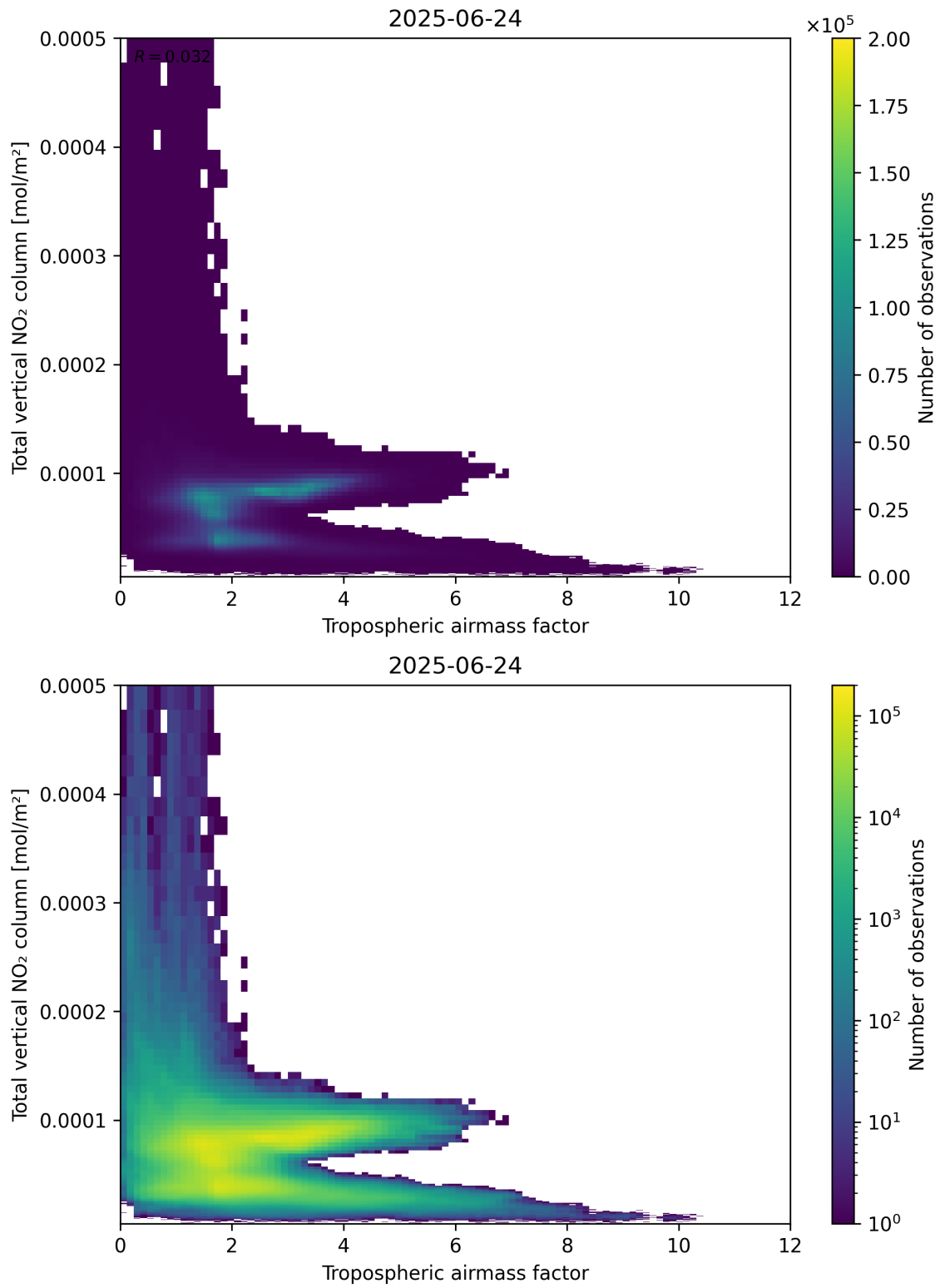
Figure 77: Scatter density plot of “Tropospheric airmass factor” against “Total vertical NO 2 column” for 2025-06-23 to 2025-06-25.
