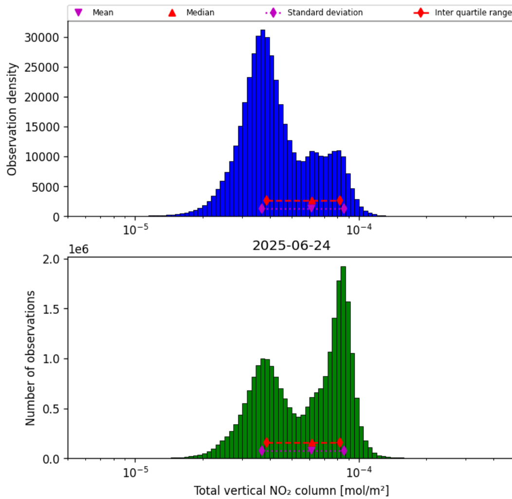
Figure 38: Histogram of “Total vertical NO 2 column” for 2025-06-23 to 2025-06-25
