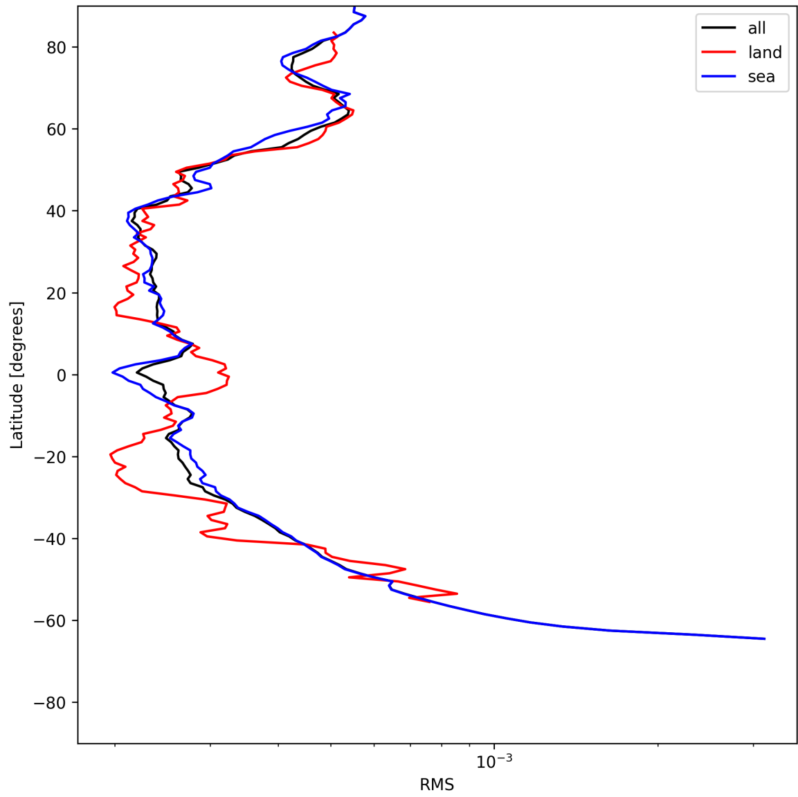
Figure 26: Zonal average of “RMS” for 2025-06-23 to 2025-06-25.
