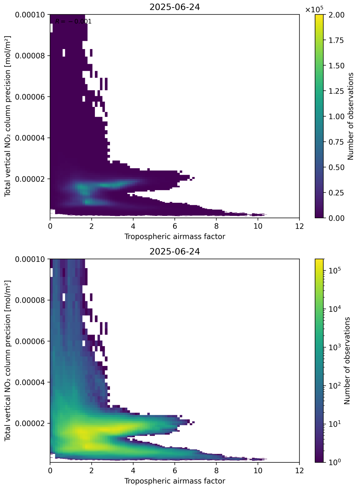
Figure 78: Scatter density plot of “Tropospheric airmass factor” against “Total vertical NO 2 column precision” for 2025-06-23 to 2025-06-25.
