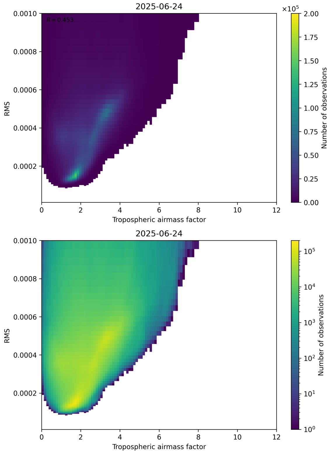
Figure 79: Scatter density plot of “Tropospheric airmass factor” against “RMS” for 2025-06-23 to 2025-06-25.
