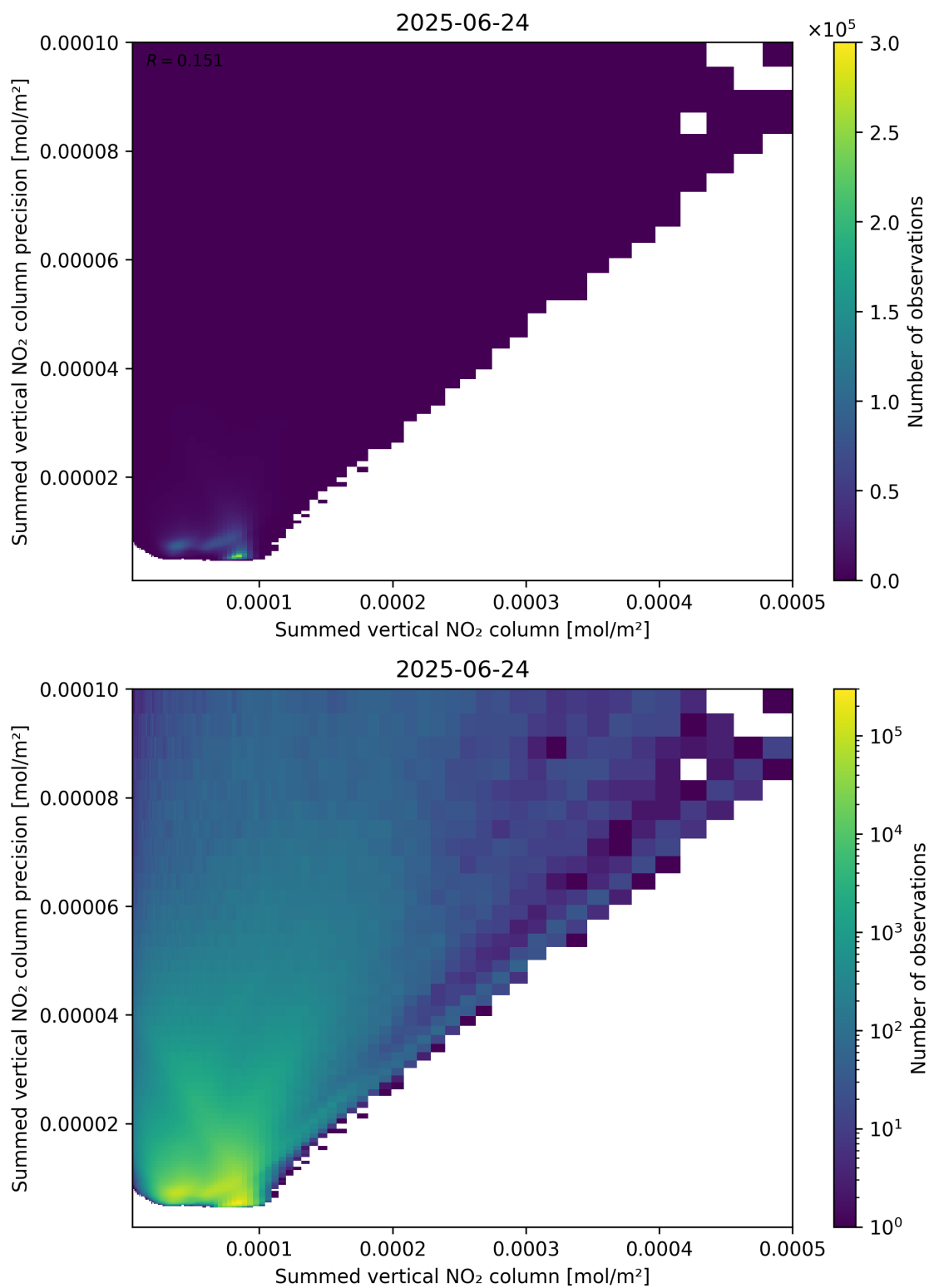
Figure 105: Scatter density plot of “Summed vertical NO 2 column” against “Summed vertical NO 2 column precision” for 2025-06-23 to 2025-06-25.
