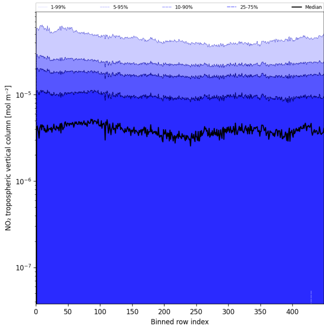
Figure 46: Along track statistics of "NO 2 tropospheric vertical column" for 2025-06-23 to 2025-06-25
