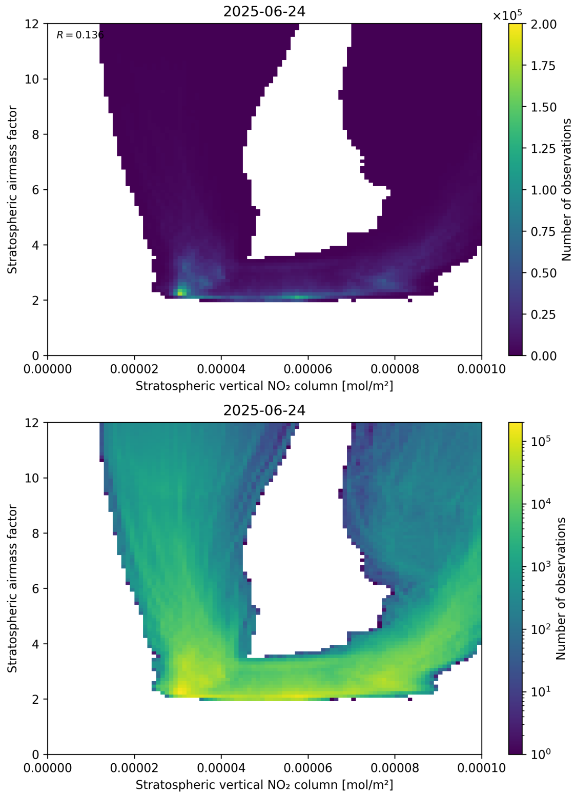
Figure 96: Scatter density plot of “Stratospheric vertical NO 2 column” against “Stratospheric airmass factor” for 2025-06-23 to 2025-06-25.
