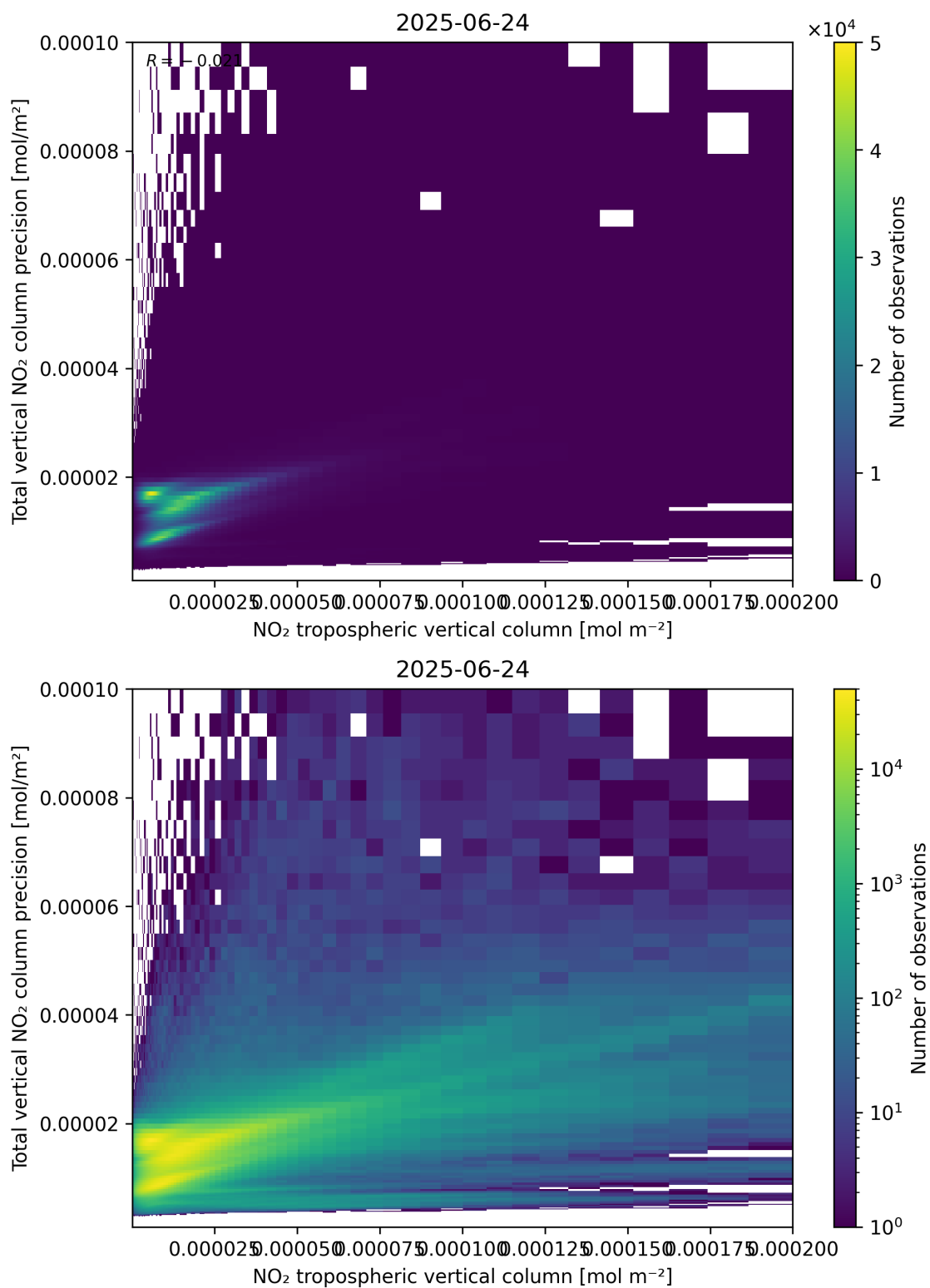
Figure 129: Scatter density plot of “NO 2 tropospheric vertical column” against “Total vertical NO 2 column precision” for 2025-06-23 to 2025-06-25.
