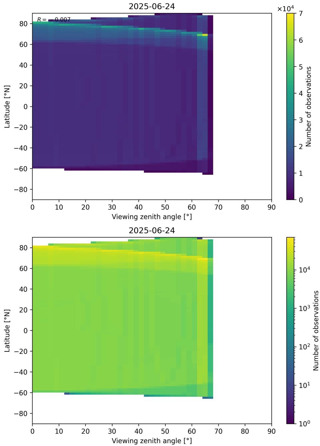
Figure 163: Scatter density plot of “Viewing zenith angle” against “Latitude” for 2025-06-23 to 2025-06-25.
