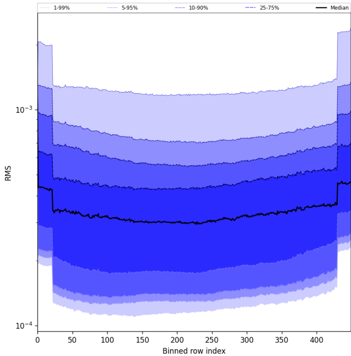
Figure 60: Along track statistics of “RMS” for 2025-06-23 to 2025-06-25
