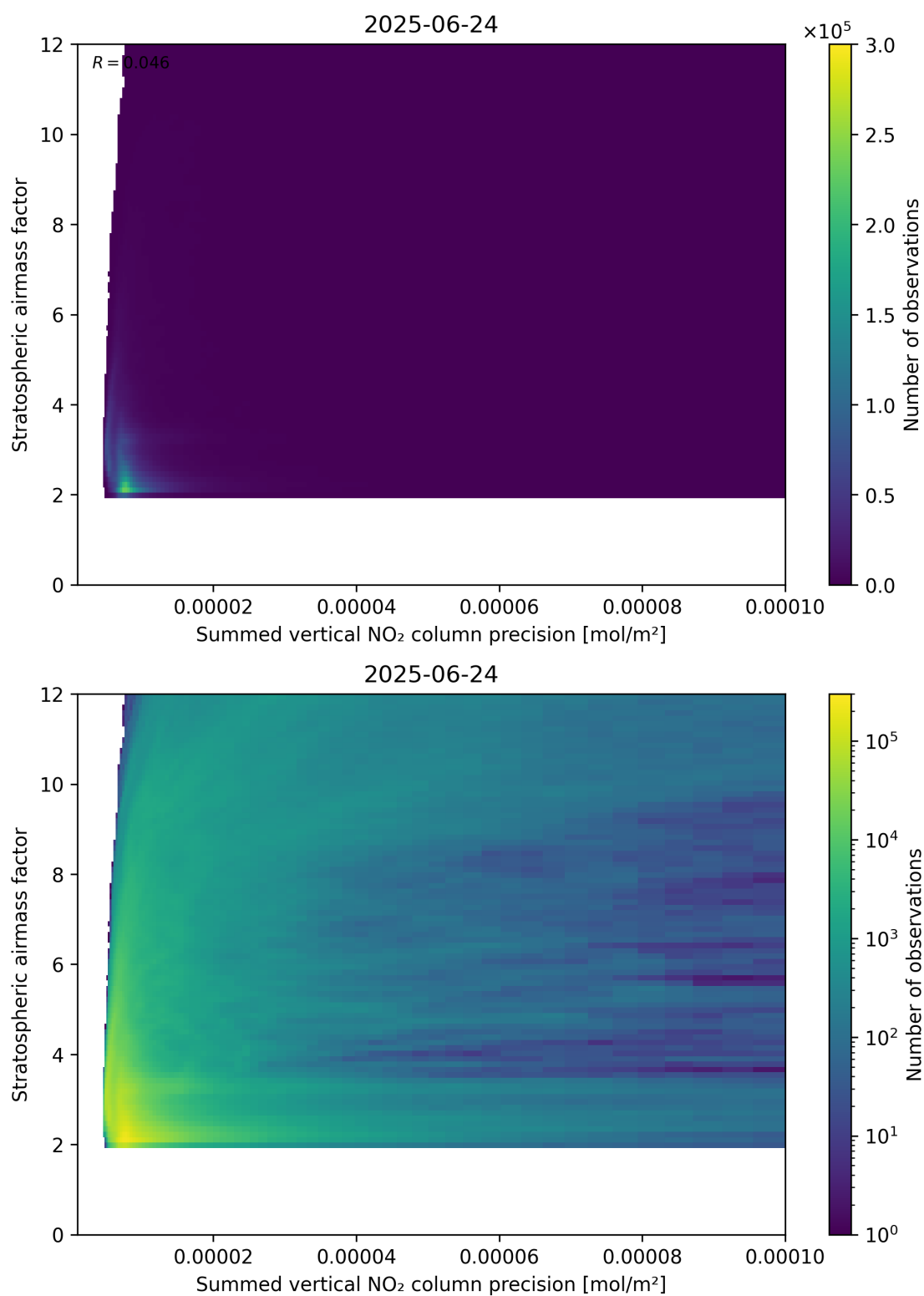
Figure 106: Scatter density plot of “Summed vertical NO 2 column precision” against “Stratospheric airmass factor” for 2025-06-23 to 2025-06-25.
