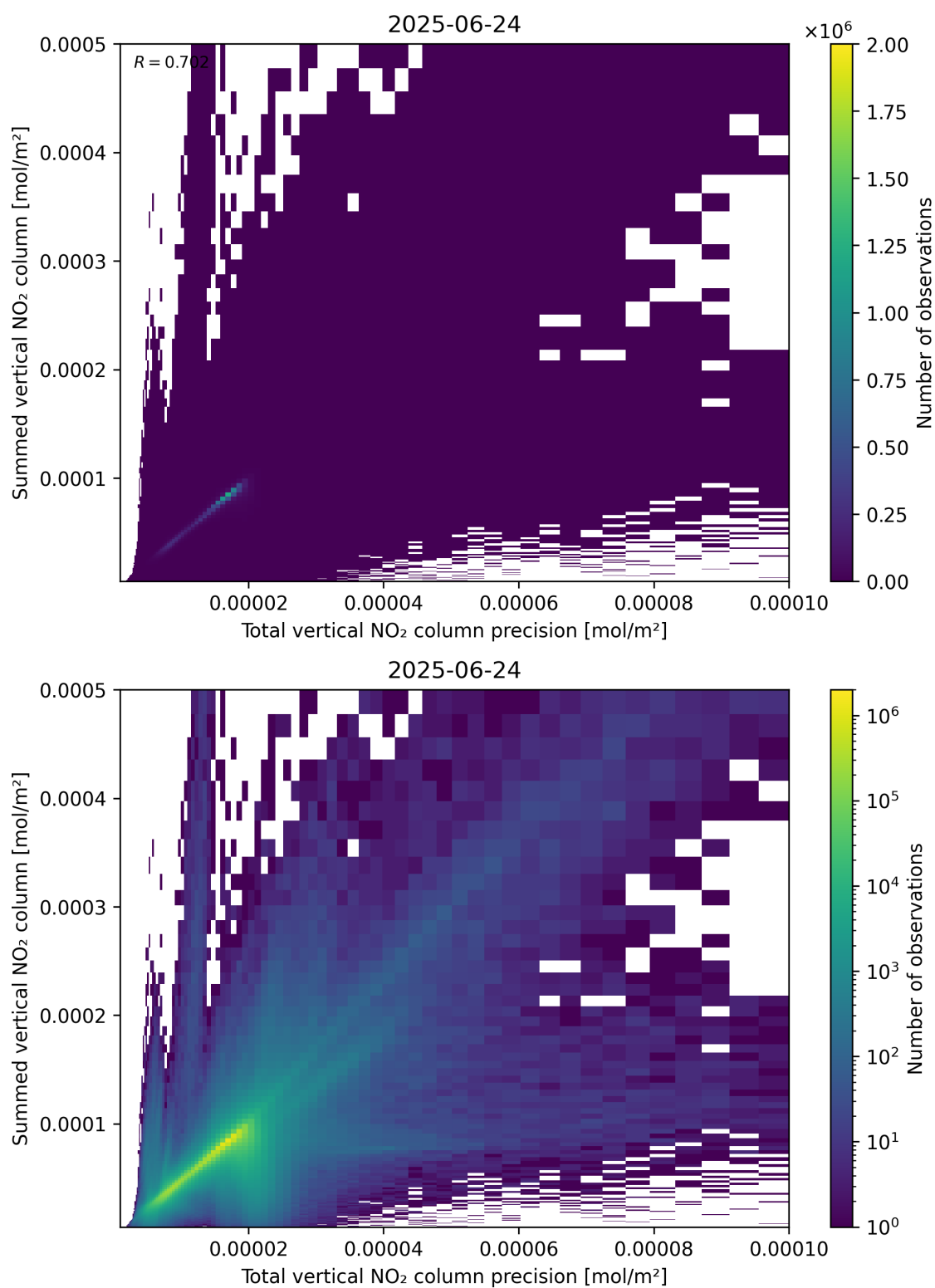
Figure 117: Scatter density plot of “Total vertical NO 2 column precision” against “Summed vertical NO 2 column” for 2025-06-23 to 2025-06-25.
