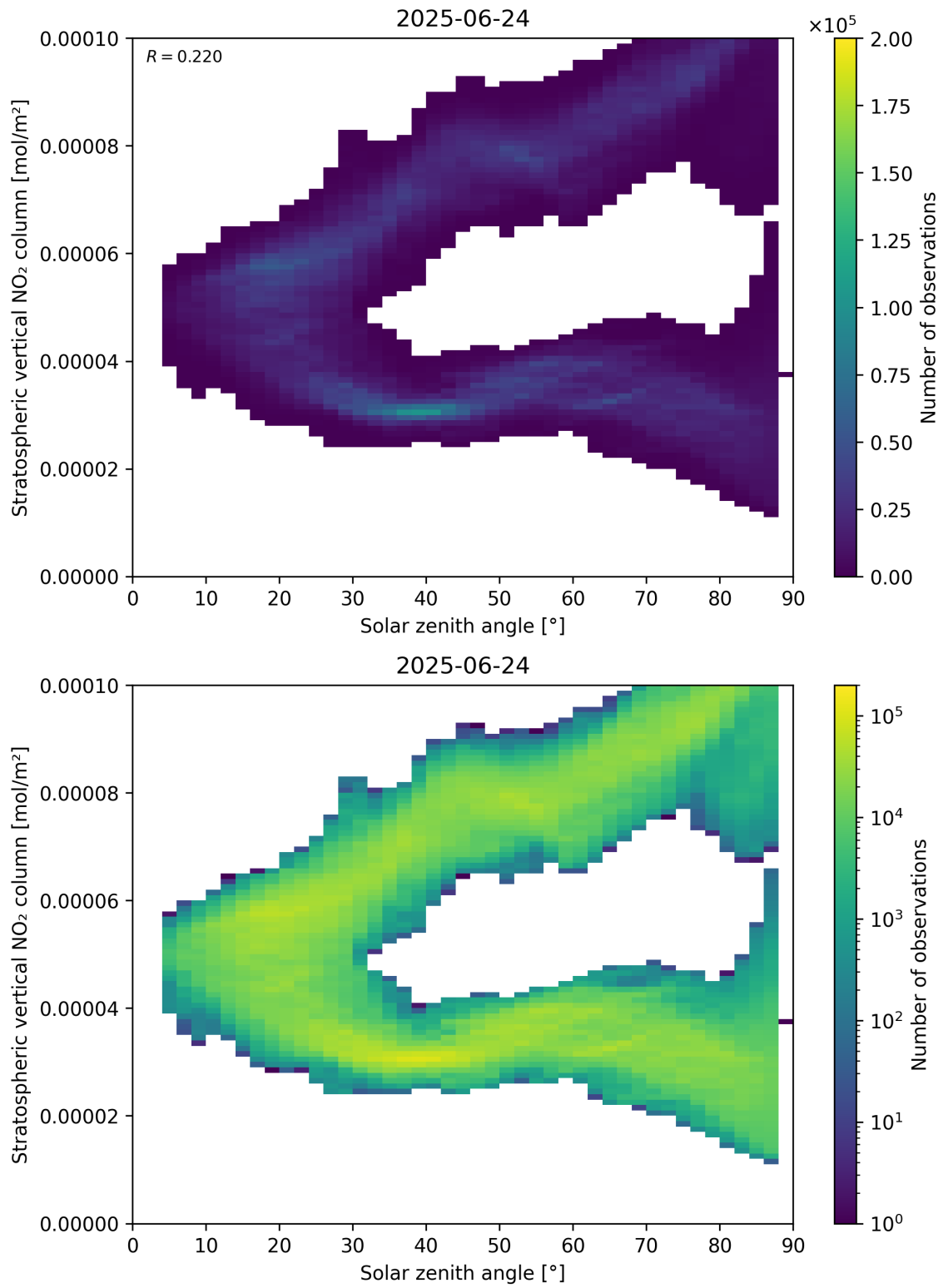
Figure 150: Scatter density plot of “Solar zenith angle” against “Stratospheric vertical NO 2 column” for 2025-06-23 to 2025-06-25.
