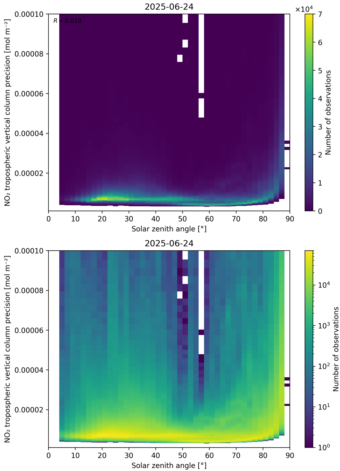
Figure 156: Scatter density plot of “Solar zenith angle” against “NO 2 tropospheric vertical column precision” for 2025-06-23 to 2025-06-25.
