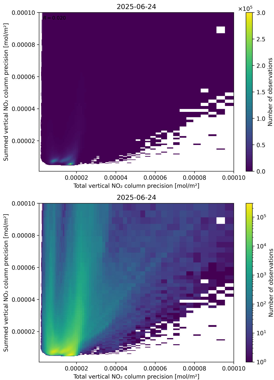
Figure 118: Scatter density plot of “Total vertical NO 2 column precision” against “Summed vertical NO 2 column precision” for 2025-06-23 to 2025-06-25.
