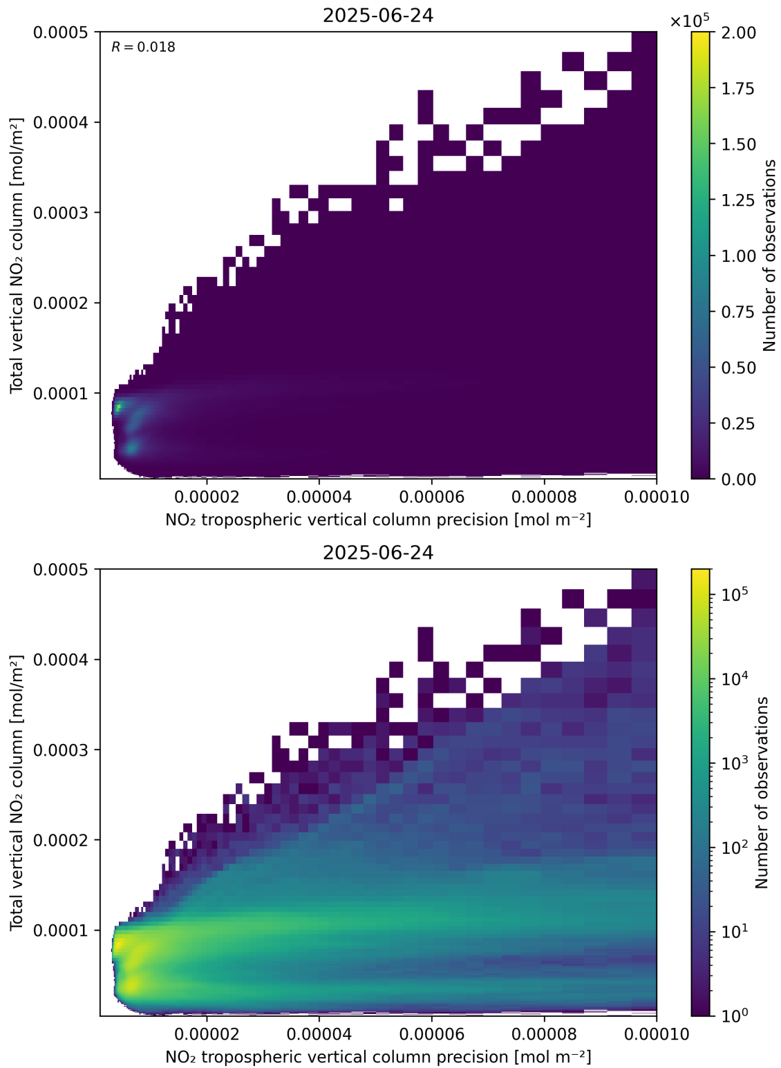
Figure 138: Scatter density plot of “NO 2 tropospheric vertical column precision” against “Total vertical NO 2 column” for 2025-06-23 to 2025-06-25.
