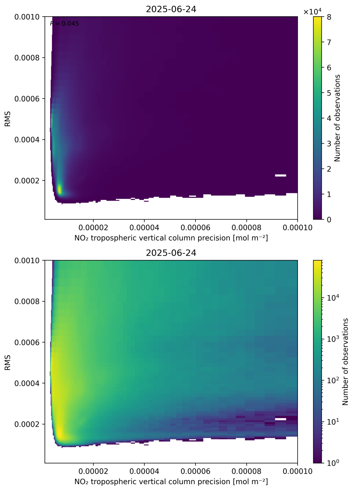
Figure 140: Scatter density plot of “NO 2 tropospheric vertical column precision” against “RMS” for 2025-06-23 to 2025-06-25.
