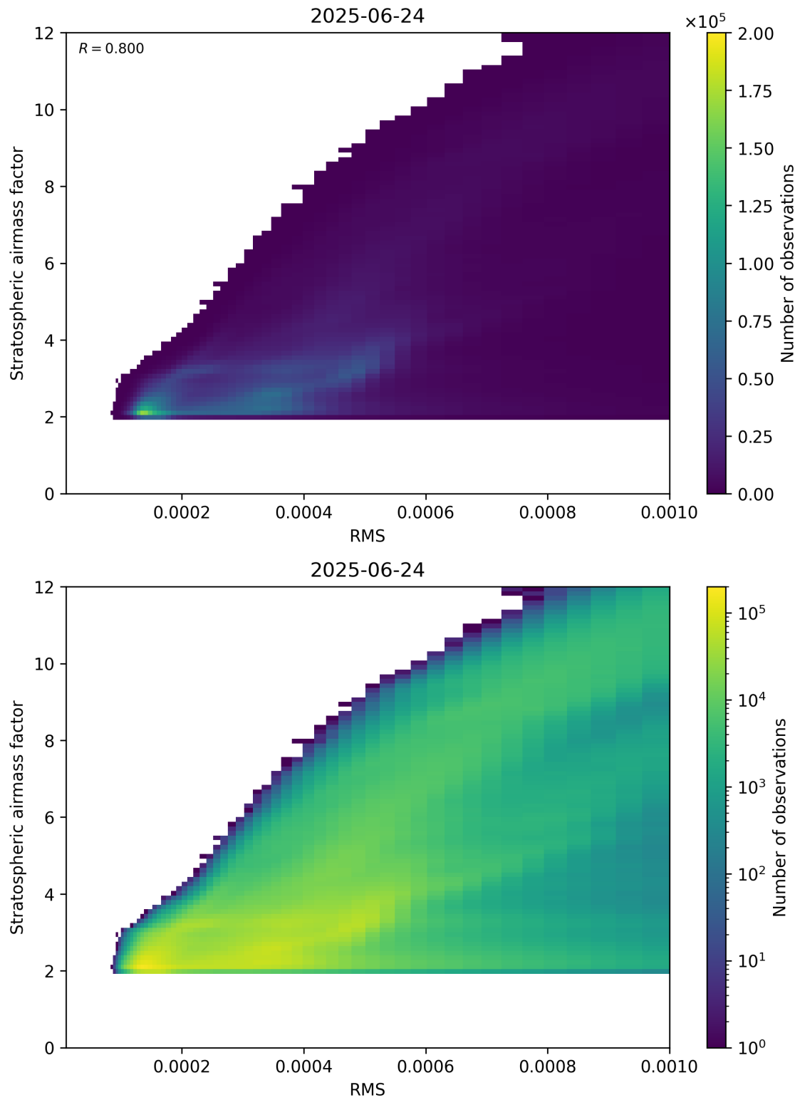
Figure 144: Scatter density plot of “RMS” against “Stratospheric airmass factor” for 2025-06-23 to 2025-06-25.
