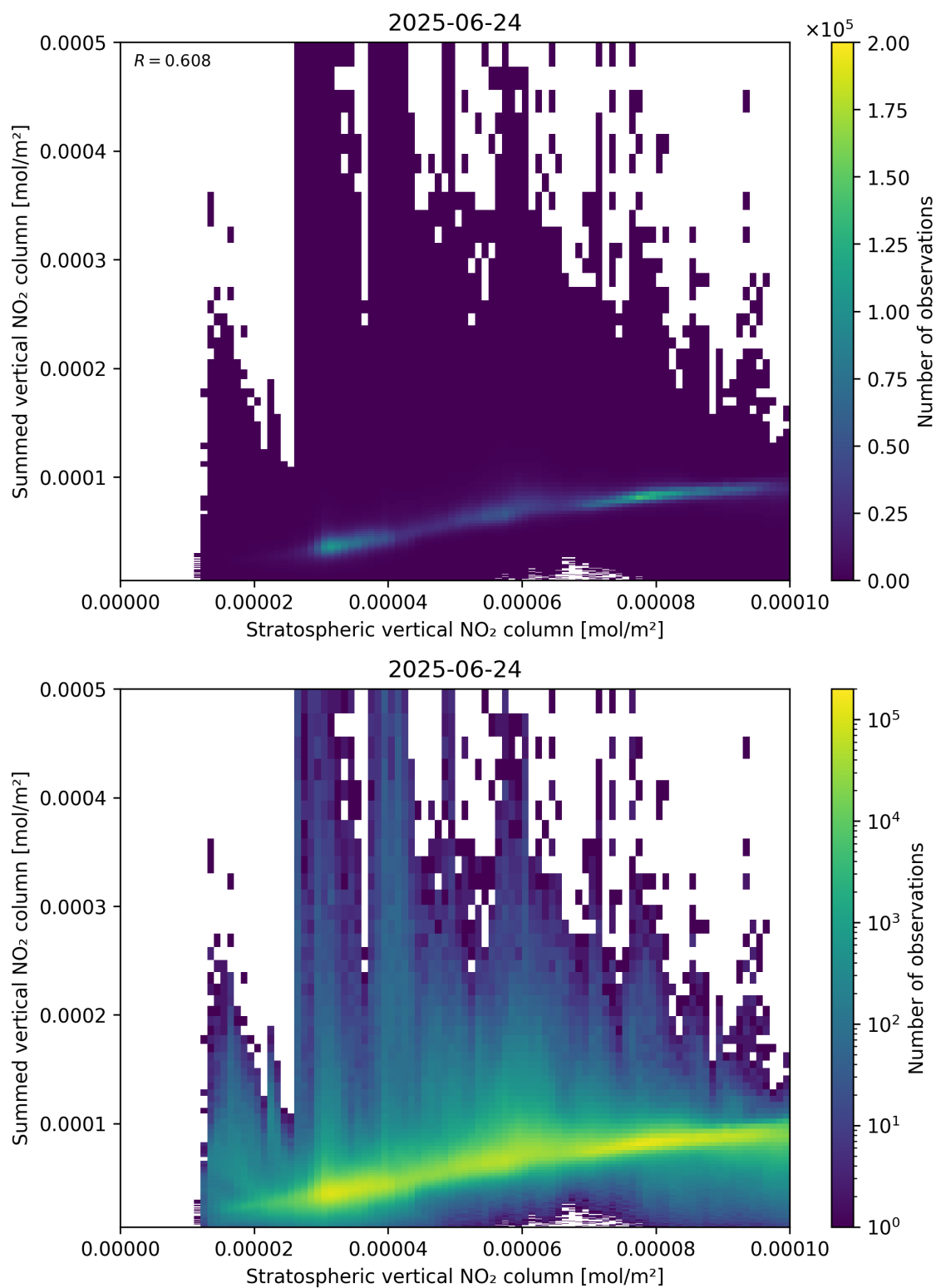
Figure 98: Scatter density plot of “Stratospheric vertical NO 2 column” against “Summed vertical NO 2 column” for 2025-06-23 to 2025-06-25.
