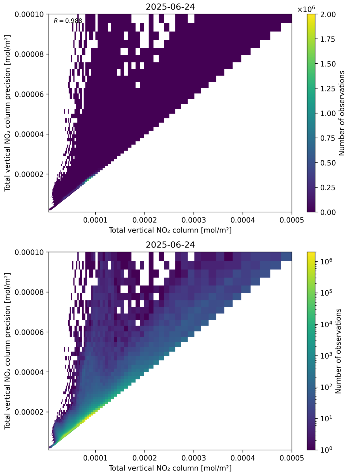
Figure 114: Scatter density plot of “Total vertical NO 2 column” against “Total vertical NO 2 column precision” for 2025-06-23 to 2025-06-25.
