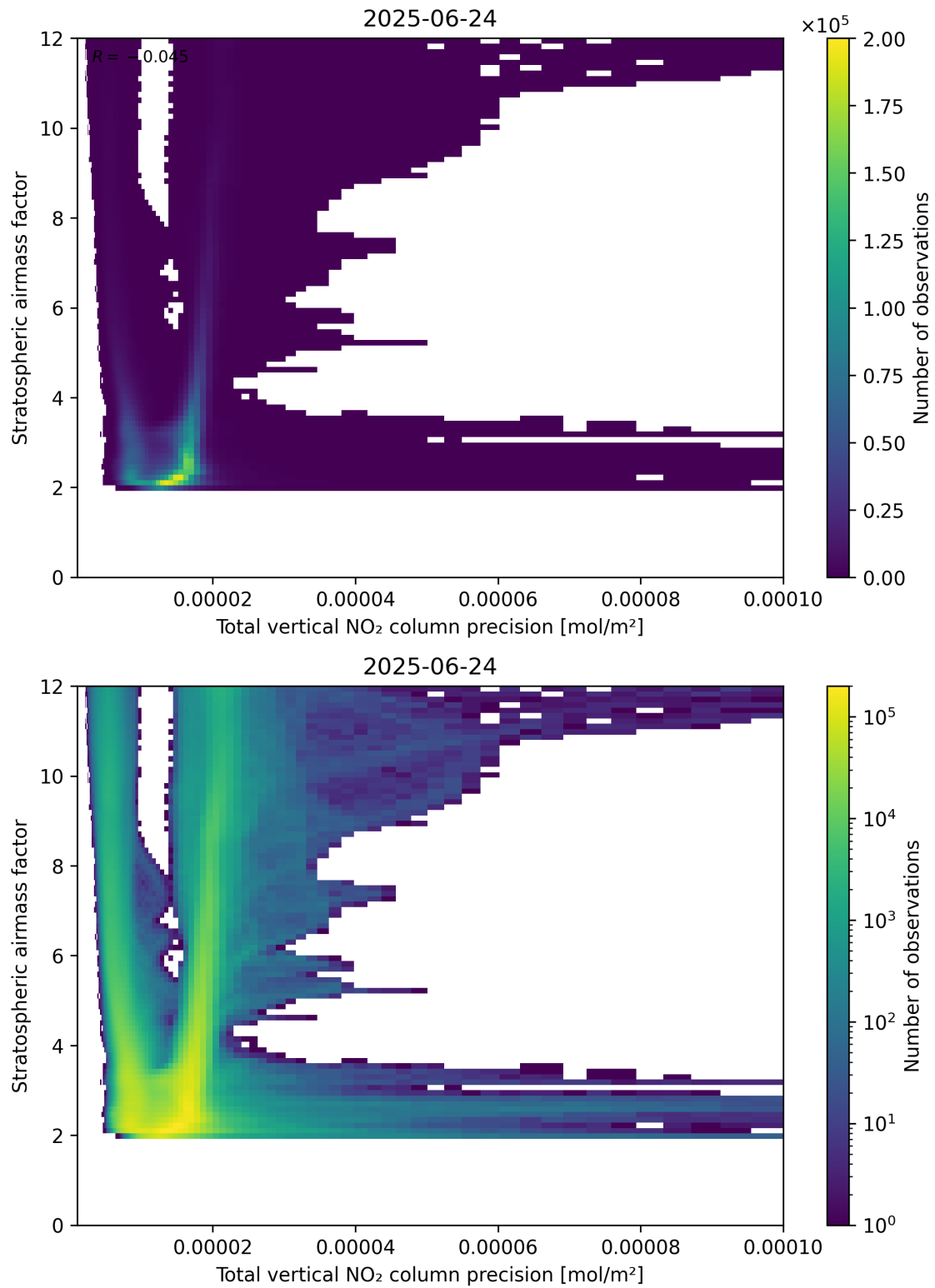
Figure 115: Scatter density plot of “Total vertical NO 2 column precision” against “Stratospheric air mass factor” for 2025-06-23 to 2025-06-25.
