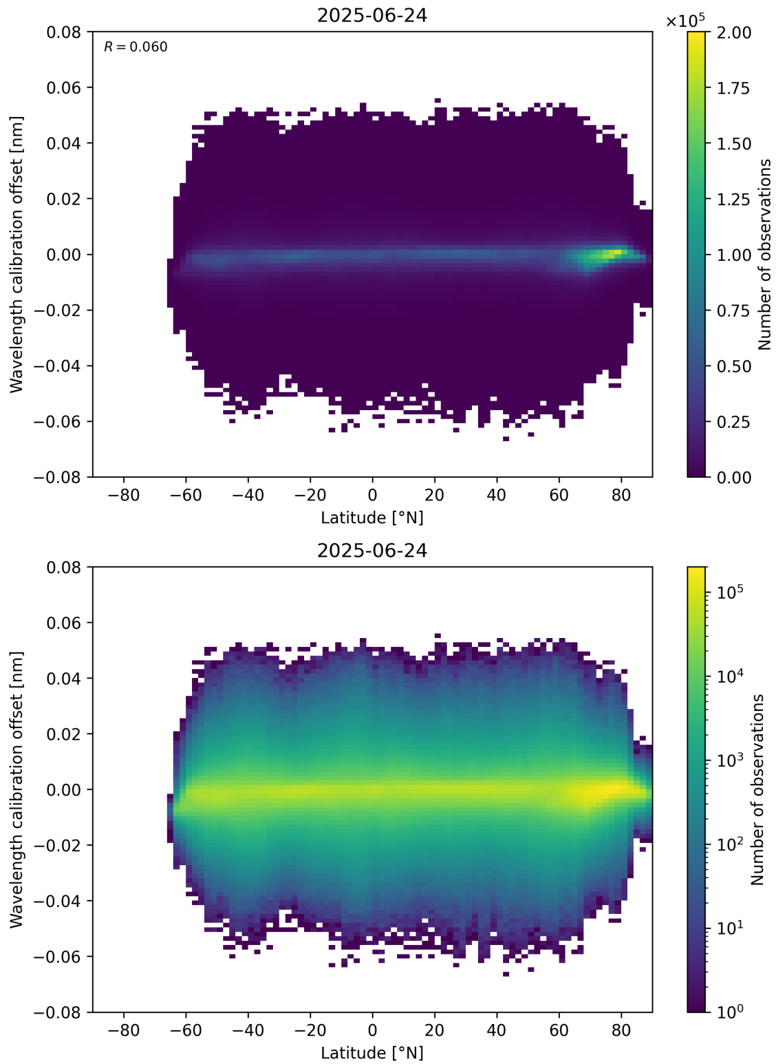
Figure 95: Scatter density plot of “Latitude” against “Wavelength calibration offset” for 2025-06-23 to 2025-06-25.
