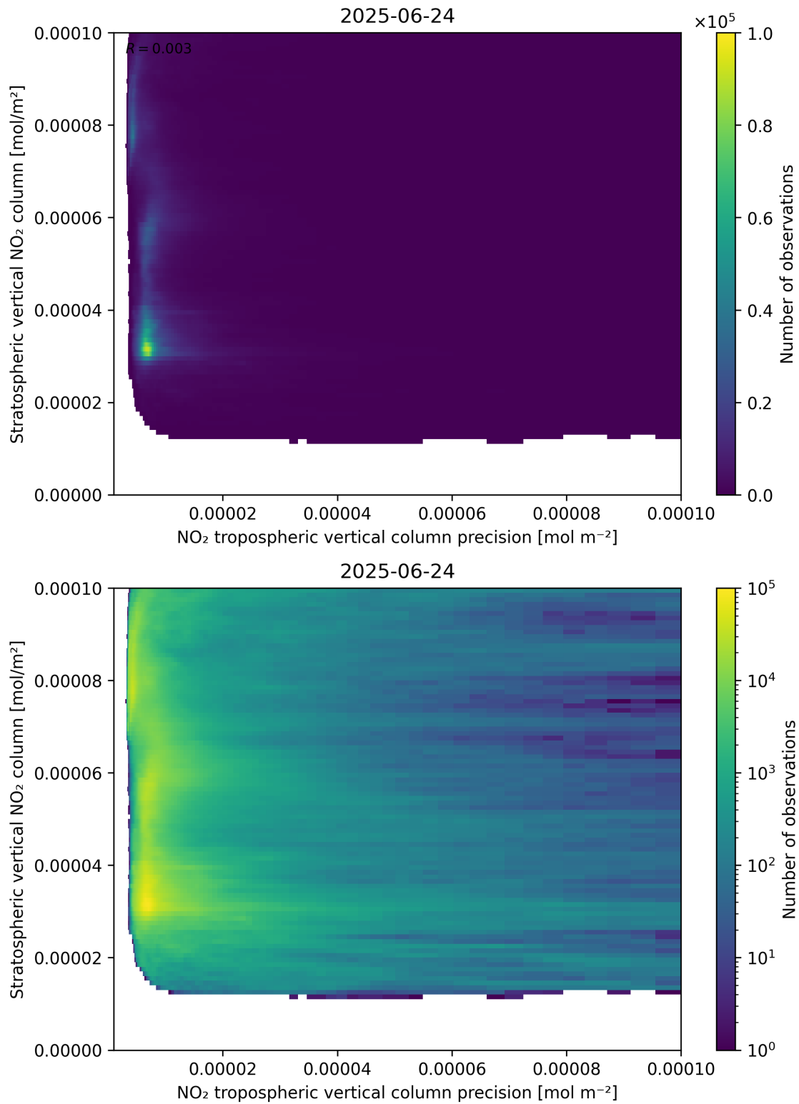
Figure 135: Scatter density plot of “NO 2 tropospheric vertical column precision” against “Stratospheric vertical NO 2 column” for 2025-06-23 to 2025-06-25.
