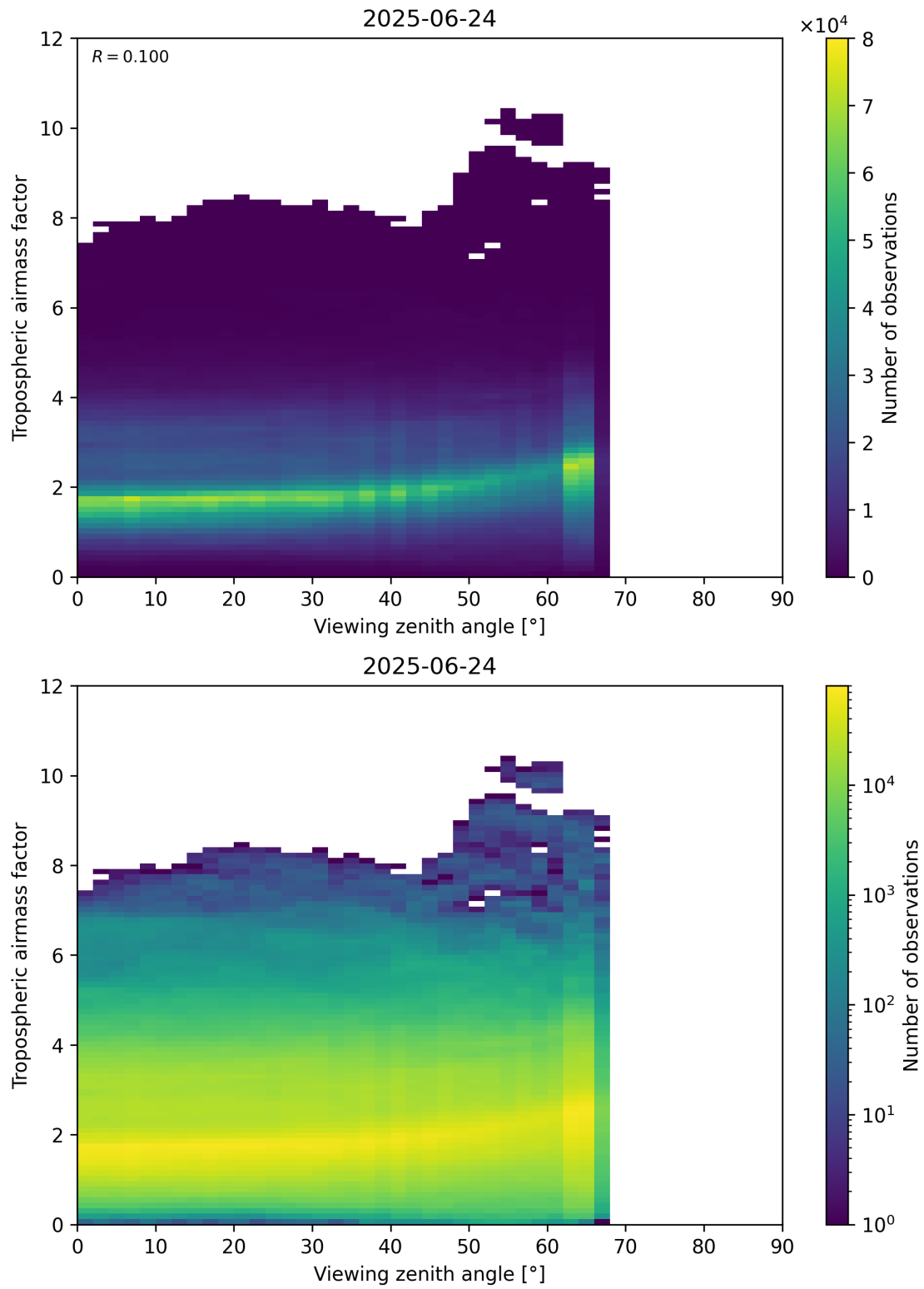
Figure 161: Scatter density plot of “Viewing zenith angle” against “Tropospheric airmass factor” for 2025-06-23 to 2025-06-25.
