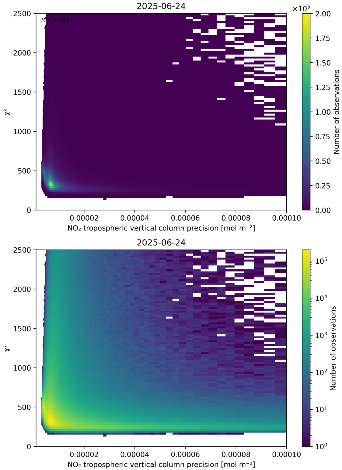
Figure 134: Scatter density plot of “NO 2 tropospheric vertical column precision” against “ \chi^2 ” for 2025-06-23 to 2025-06-25.
