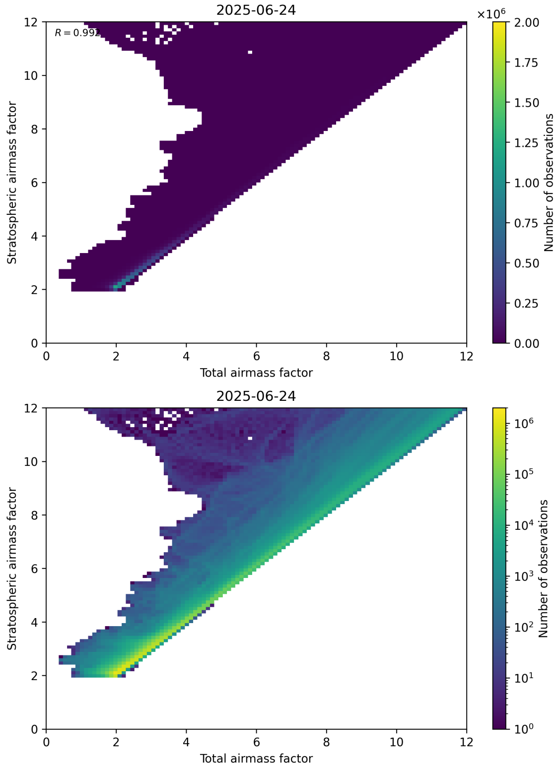
Figure 62: Scatter density plot of “Total air mass factor” against “Stratospheric air mass factor” for 2025-06-23 to 2025-06-25.
