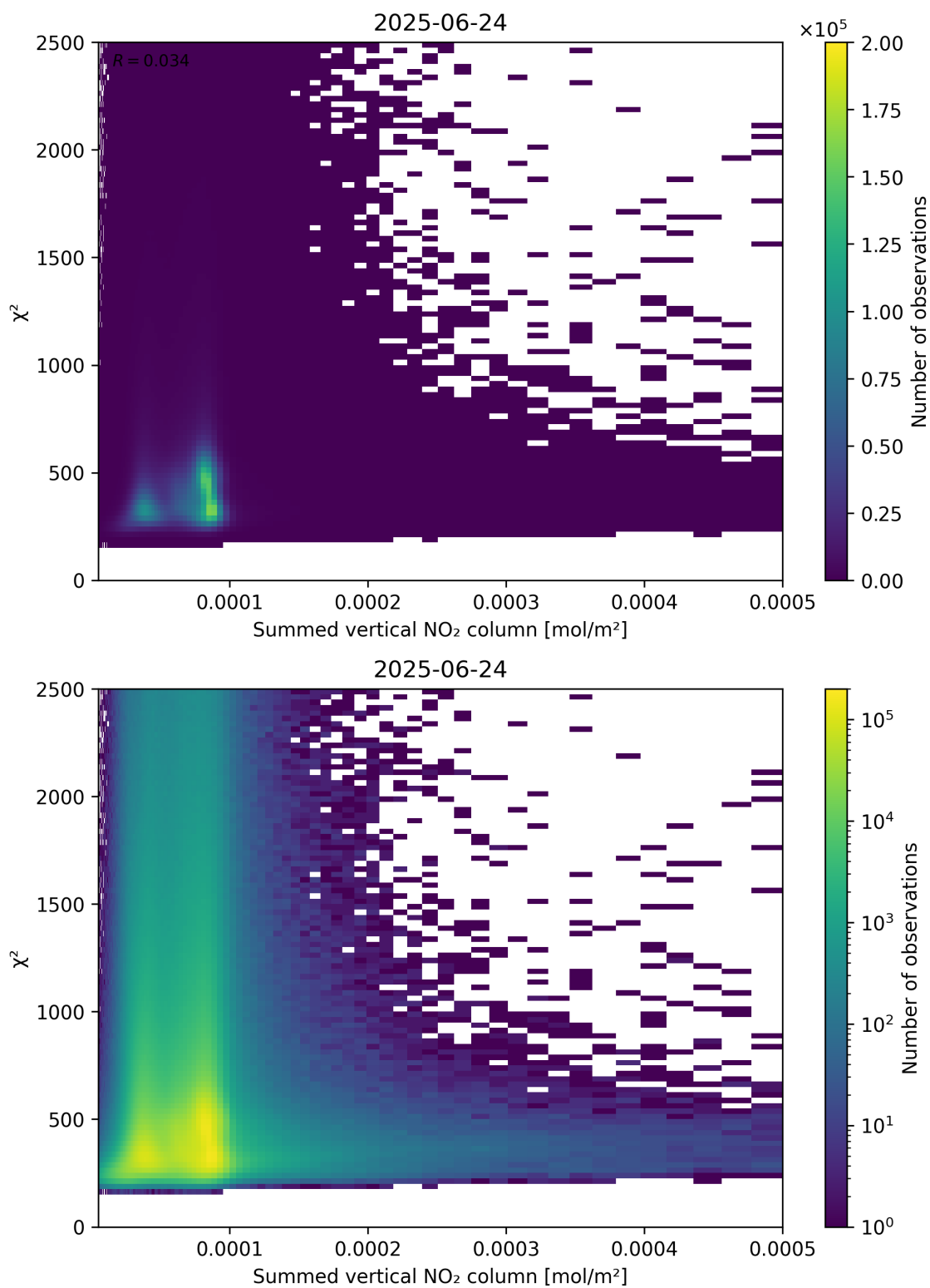
Figure 104: Scatter density plot of “Summed vertical NO 2 column” against “ \chi^2 ” for 2025-06-23 to 2025-06-25.
