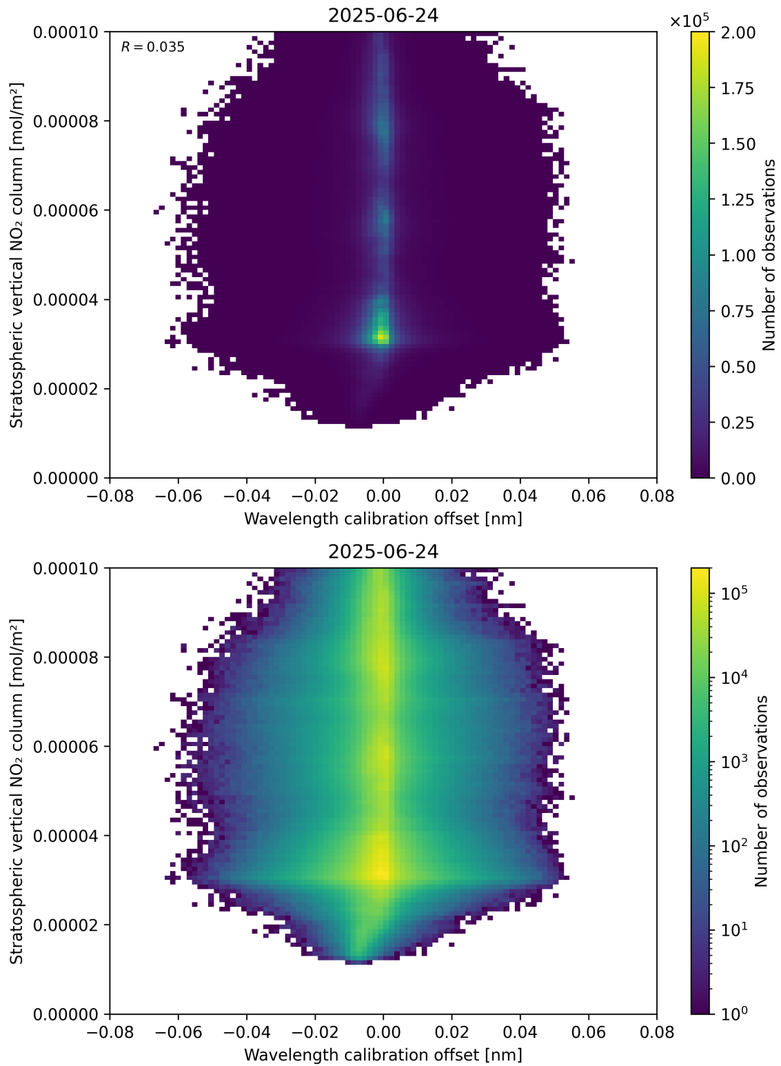
Figure 176: Scatter density plot of “Wavelength calibration offset” against “Stratospheric vertical NO 2 column” for 2025-06-23 to 2025-06-25.
