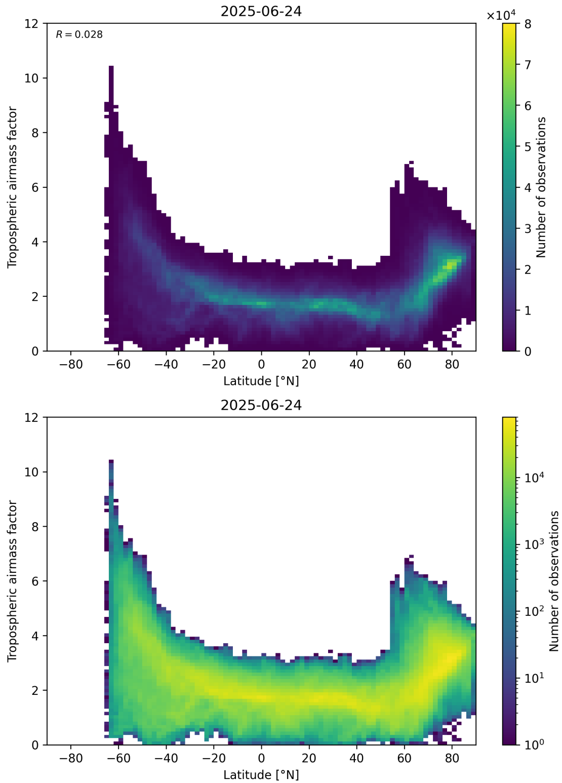
Figure 85: Scatter density plot of “Latitude” against “Tropospheric air mass factor” for 2025-06-23 to 2025-06-25.
