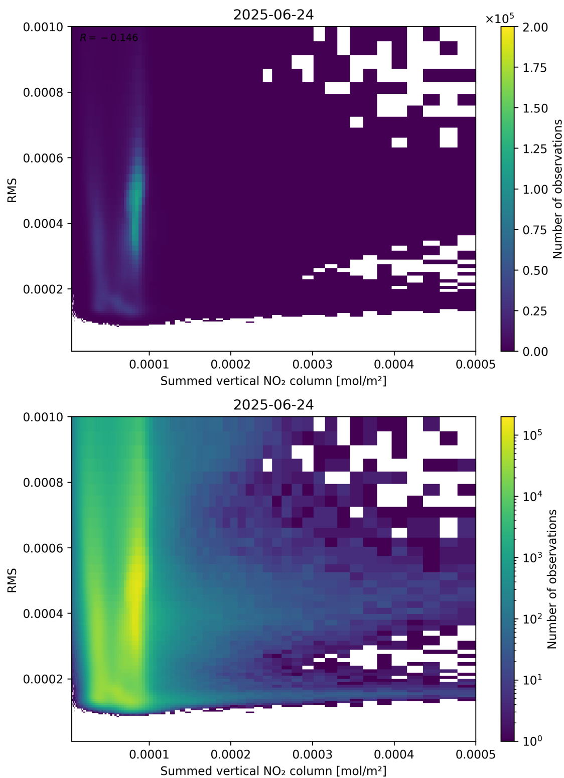
Figure 109: Scatter density plot of “Summed vertical NO 2 column” against “RMS” for 2025-06-23 to 2025-06-25.
