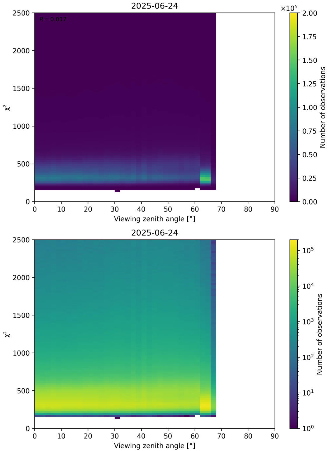
Figure 162: Scatter density plot of “Viewing zenith angle” against “ \chi^2 ” for 2025-06-23 to 2025-06-25.
