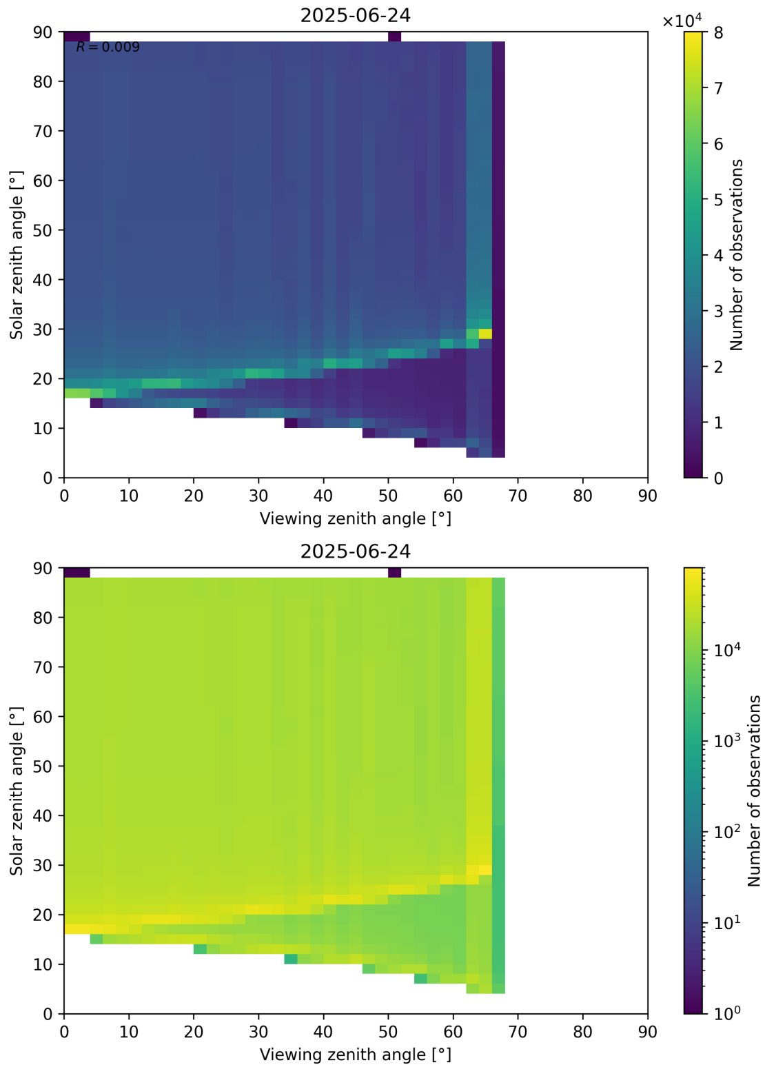
Figure 172: Scatter density plot of “Viewing zenith angle” against “Solar zenith angle” for 2025-06-23 to 2025-06-25.
