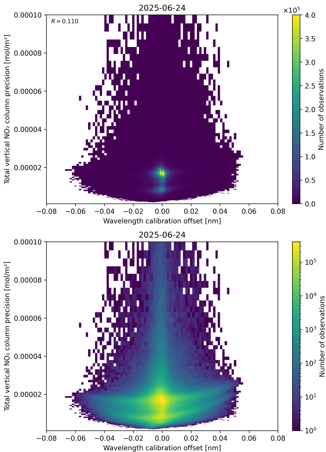
Figure 180: Scatter density plot of “Wavelength calibration offset” against “Total vertical NO 2 column precision” for 2025-06-23 to 2025-06-25.
