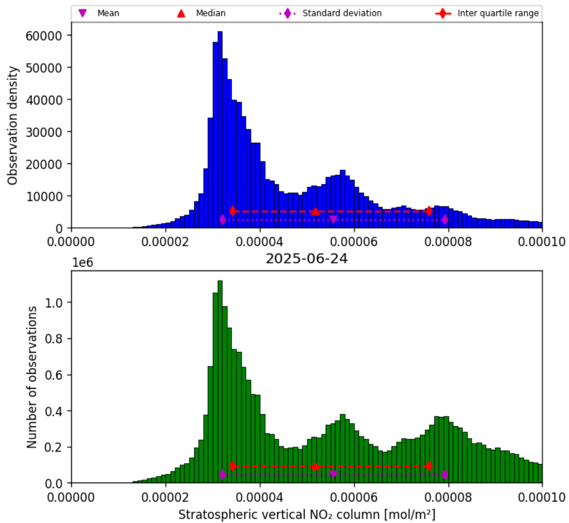
Figure 36: Histogram of “Stratospheric vertical NO 2 column” for 2025-06-23 to 2025-06-25
