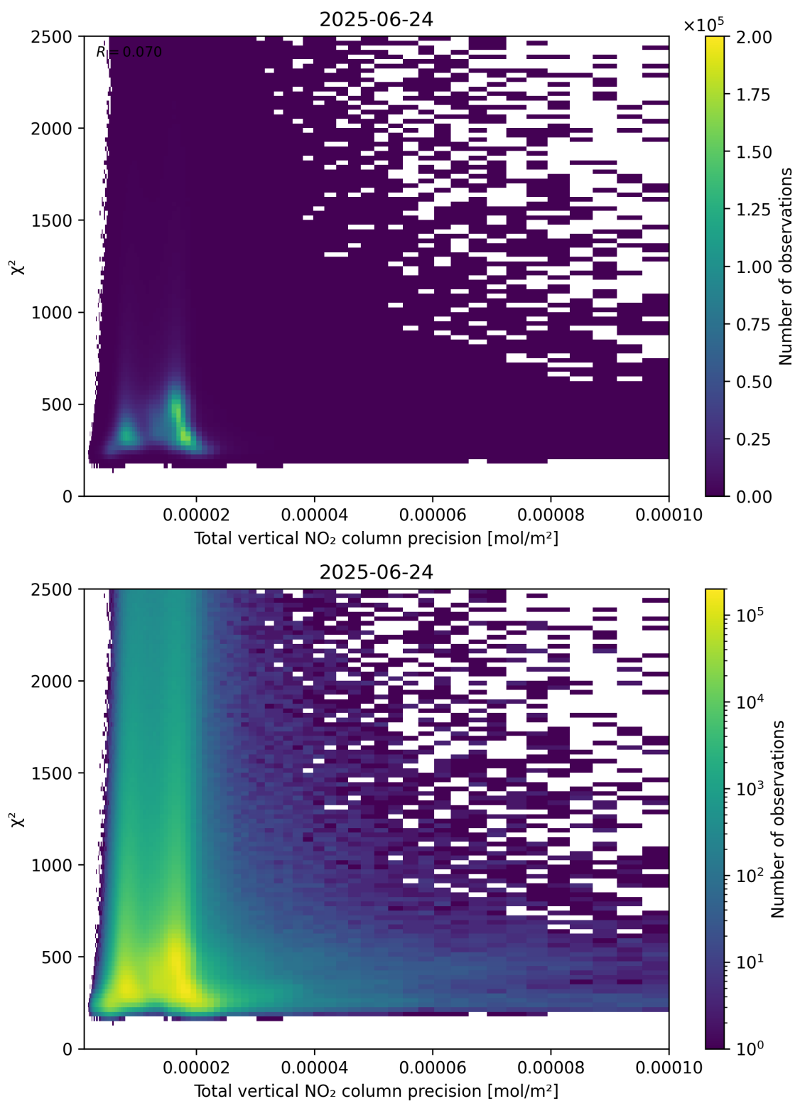
Figure 116: Scatter density plot of “Total vertical NO 2 column precision” against “ \chi^2 ” for 2025-06-23 to 2025-06-25.
