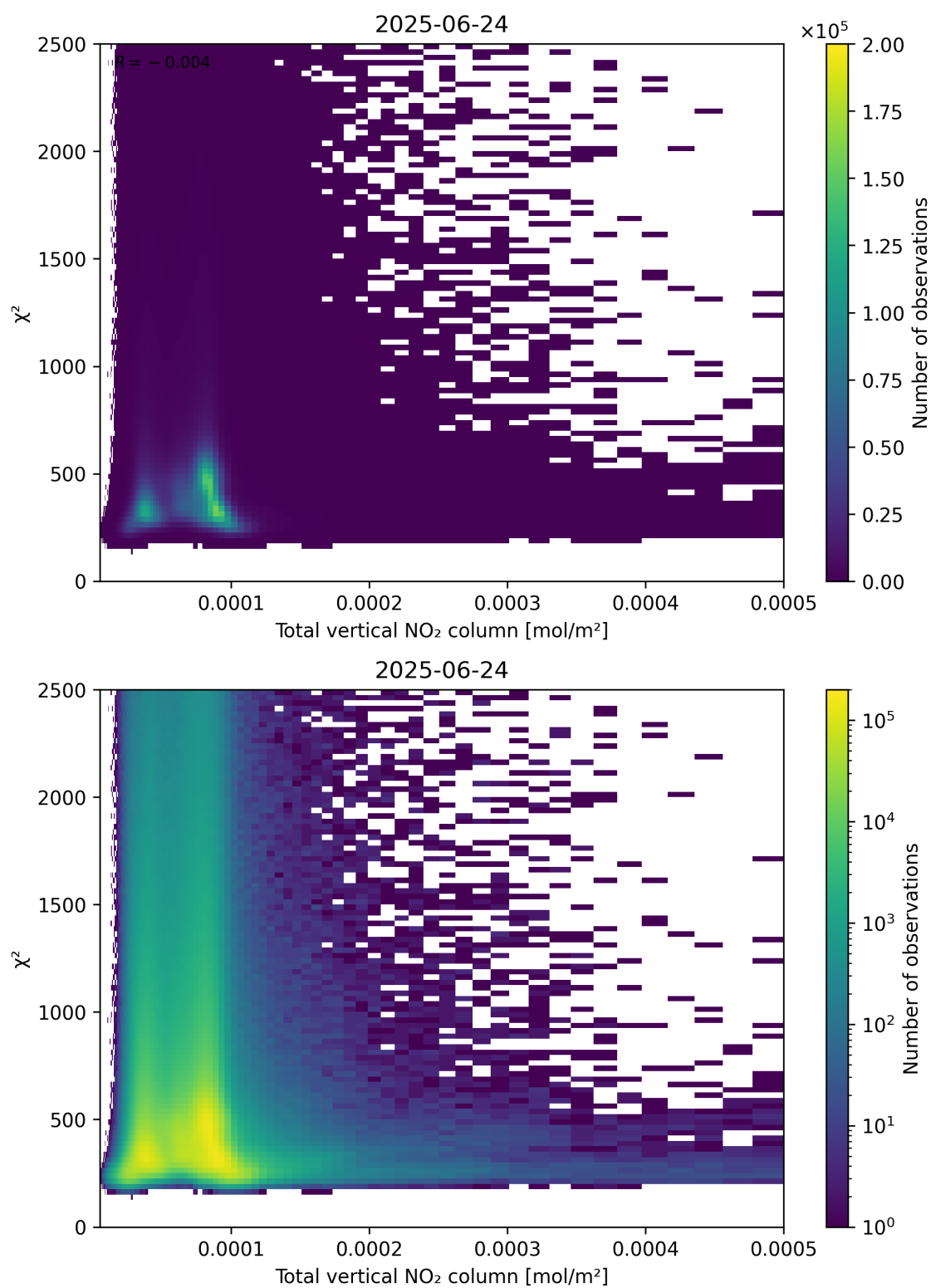
Figure 111: Scatter density plot of “Total vertical NO 2 column” against “ \chi^2 ” for 2025-06-23 to 2025-06-25.
