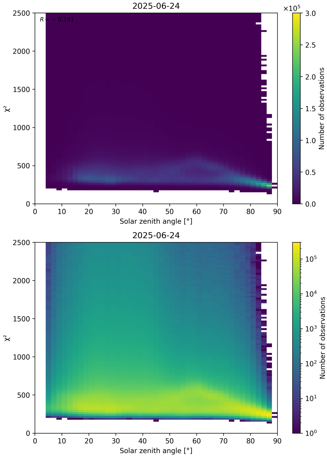
Figure 148: Scatter density plot of “Solar zenith angle” against “ \chi^2 ” for 2025-06-23 to 2025-06-25.
