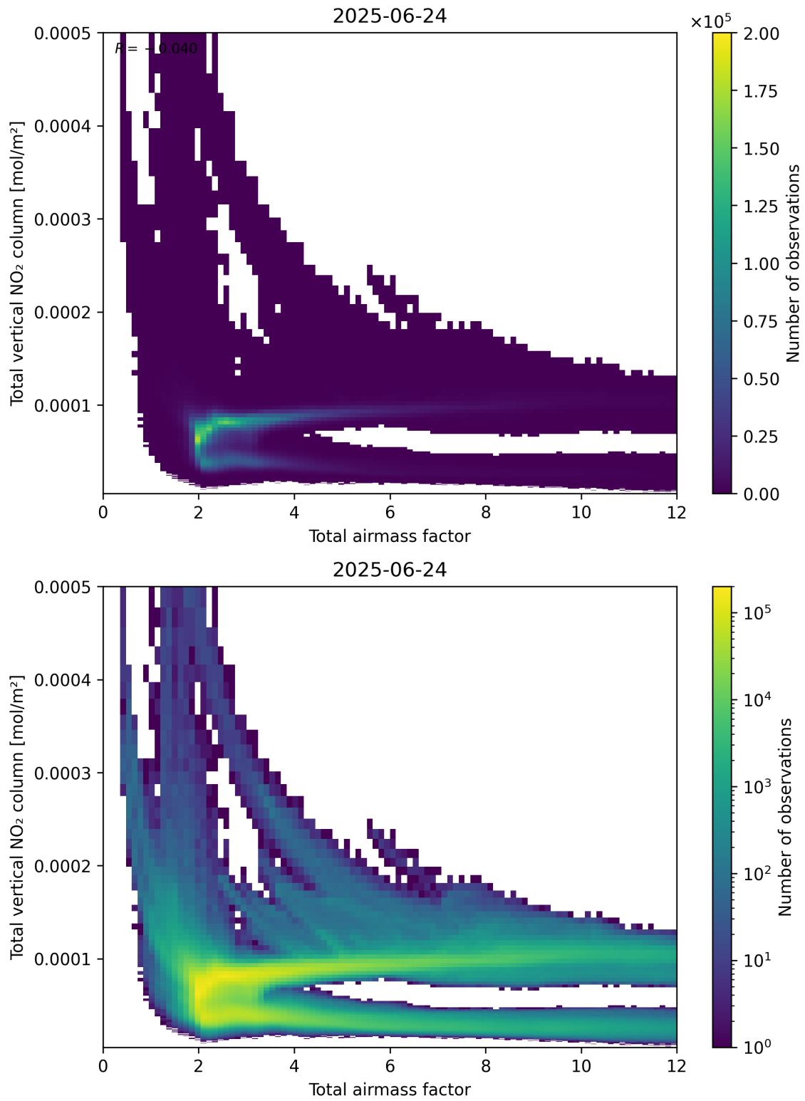
Figure 67: Scatter density plot of “Total airmass factor” against “Total vertical NO 2 column” for 2025-06-23 to 2025-06-25.
