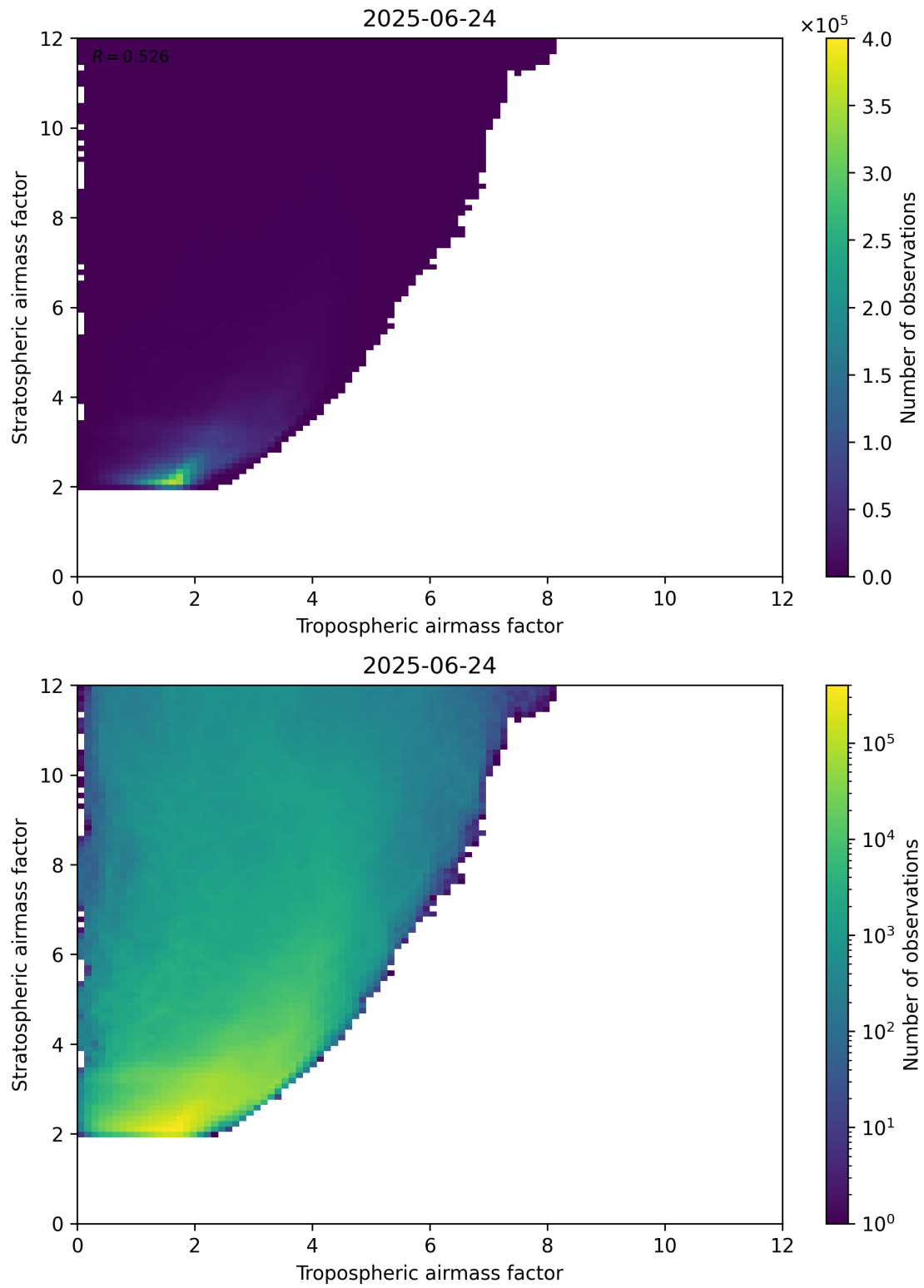
Figure 71: Scatter density plot of “Tropospheric airmass factor” against “Stratospheric airmass factor” for 2025-06-23 to 2025-06-25.
