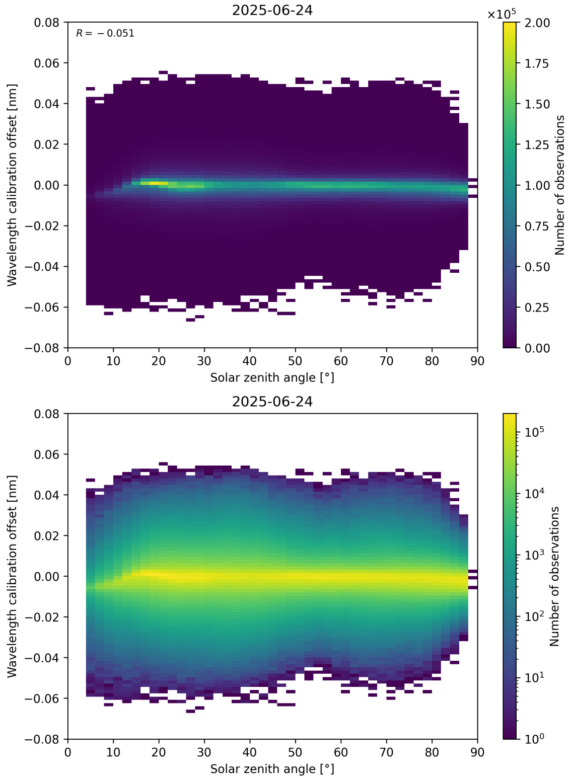
Figure 158: Scatter density plot of “Solar zenith angle” against “Wavelength calibration offset” for 2025-06-23 to 2025-06-25.
