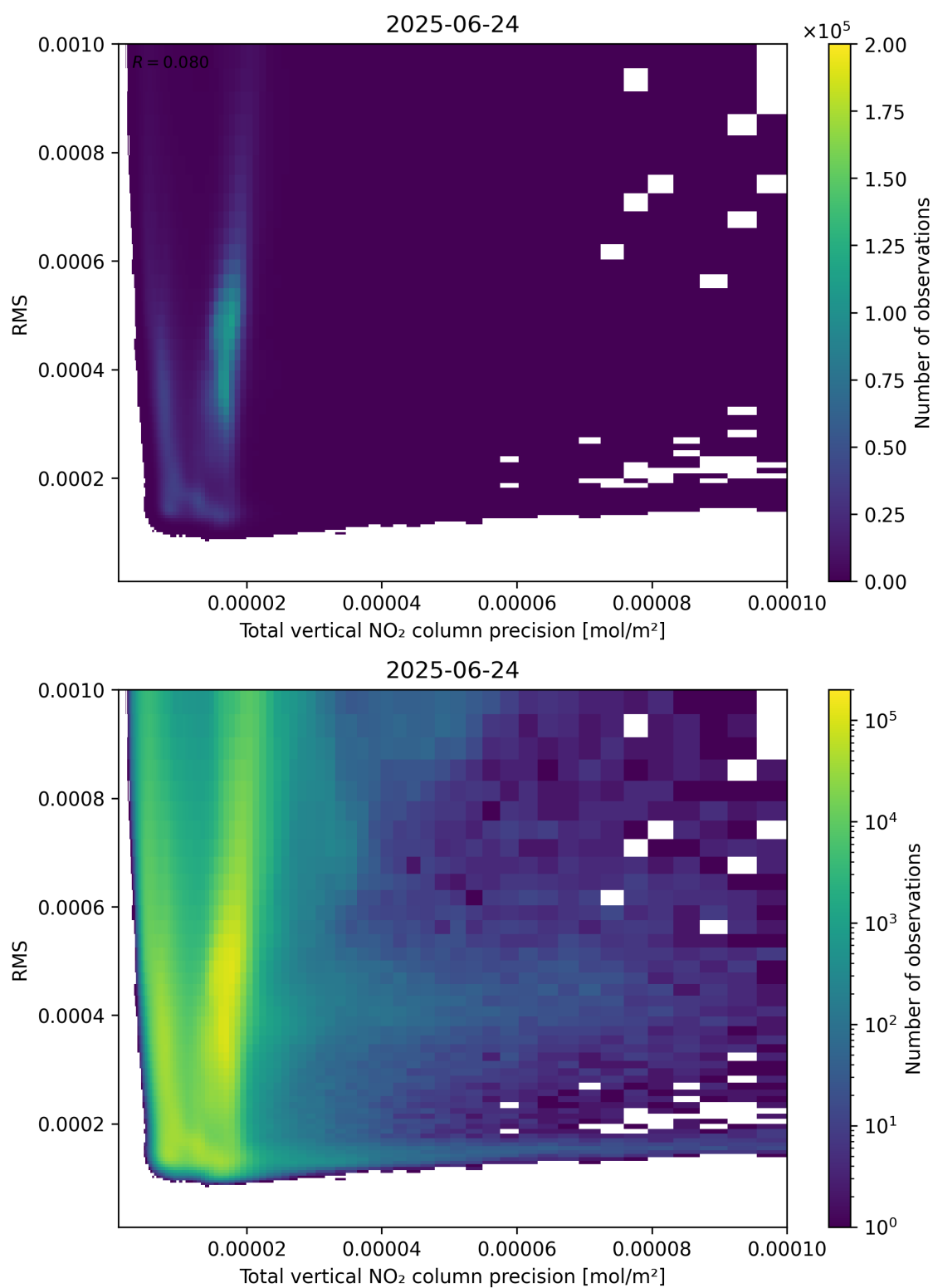
Figure 119: Scatter density plot of “Total vertical NO 2 column precision” against “RMS” for 2025-06-23 to 2025-06-25.
