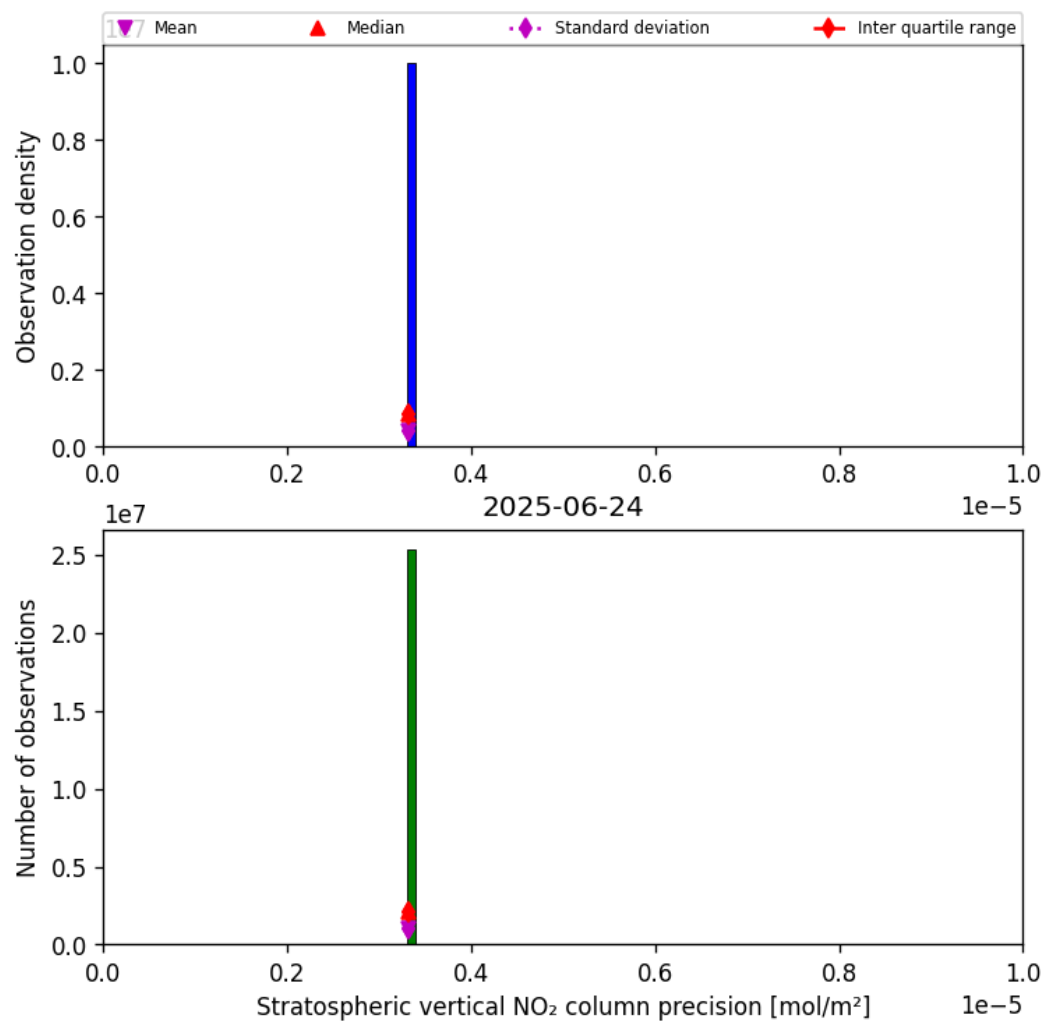
Figure 37: Histogram of “Stratospheric vertical NO 2 column precision” for 2025-06-23 to 2025-06-25
