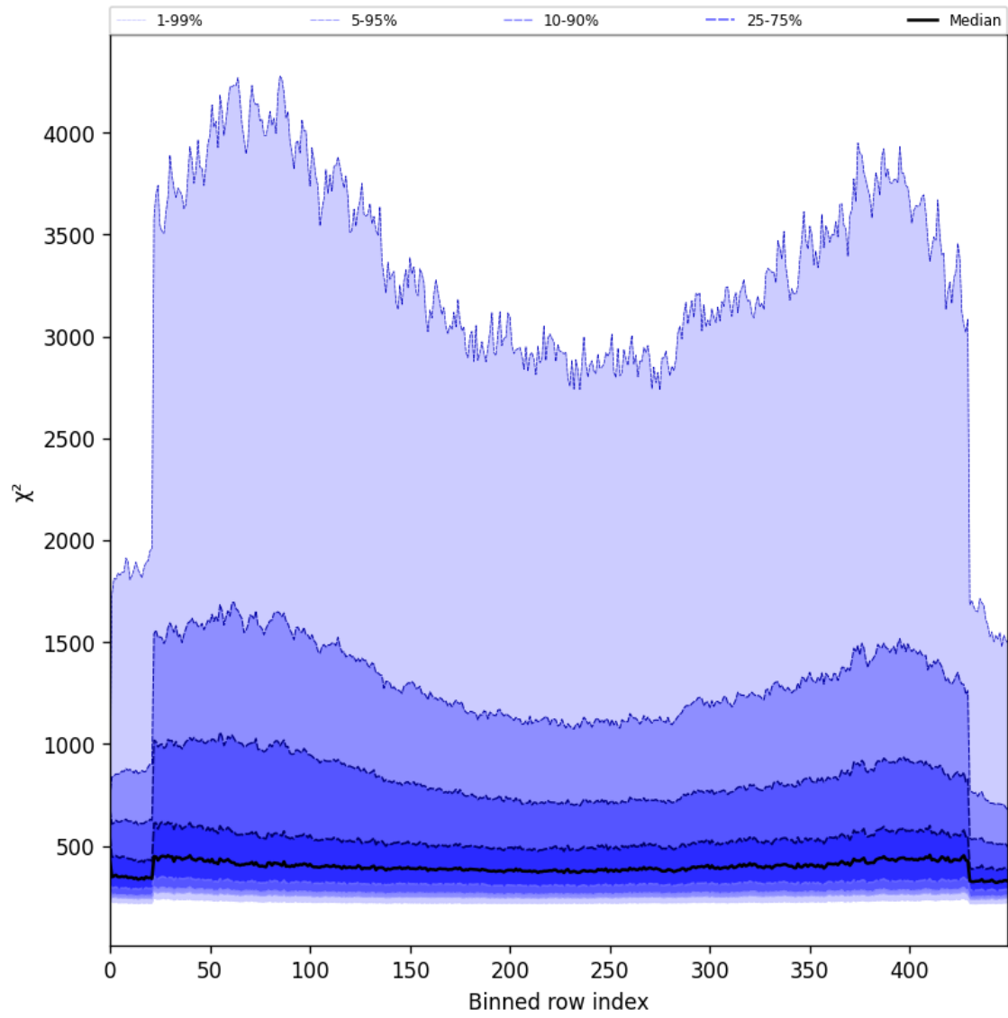
Figure 59: Along track statistics of “ \chi^2 ” for 2025-06-23 to 2025-06-25
