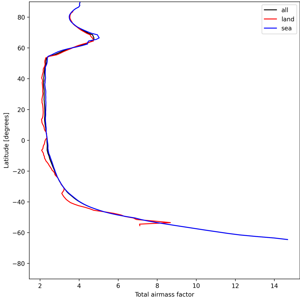
Figure 15: Zonal average of “Total airmass factor” for 2025-06-23 to 2025-06-25.
