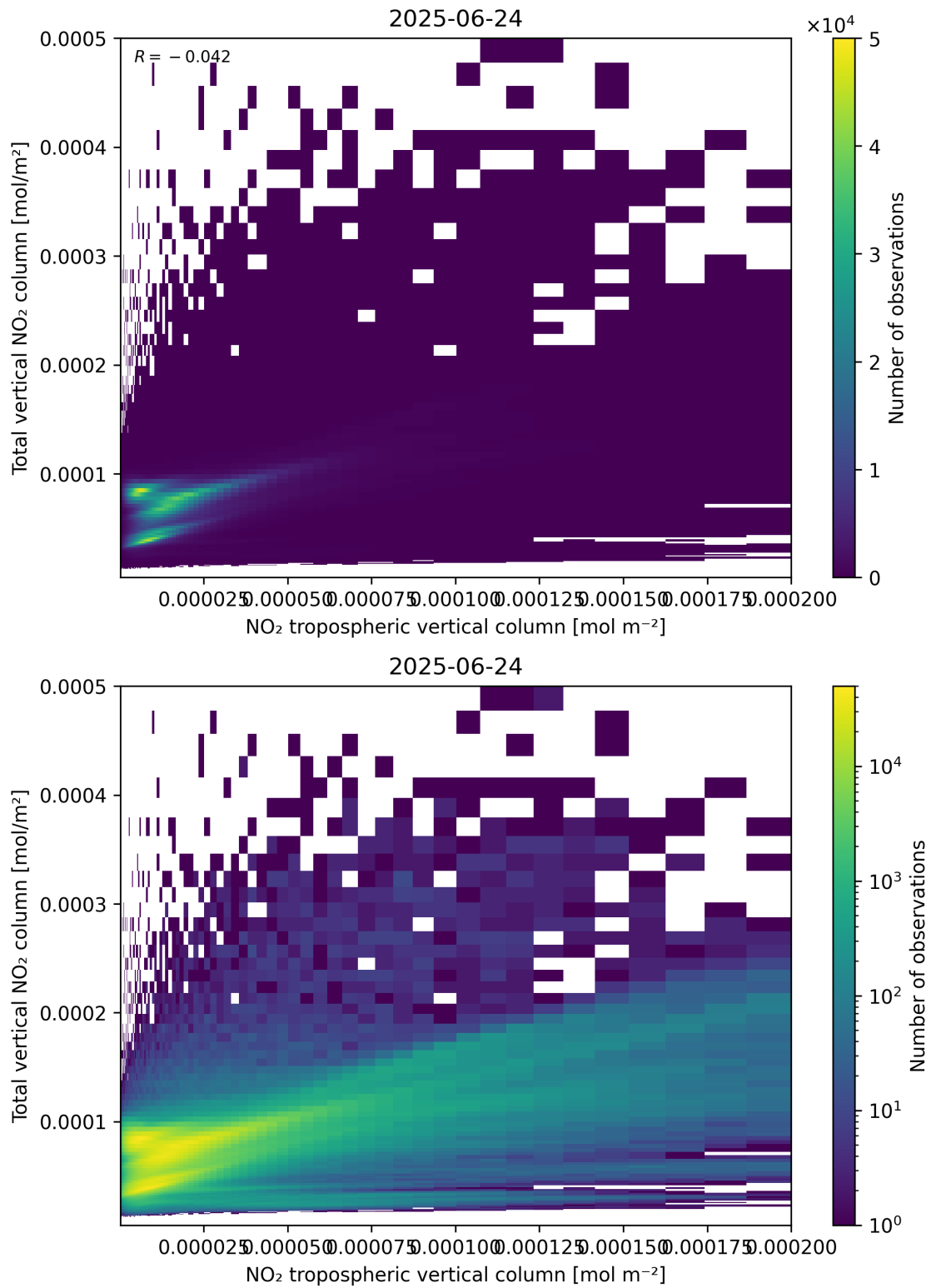
Figure 128: Scatter density plot of “NO 2 tropospheric vertical column” against “Total vertical NO 2 column” for 2025-06-23 to 2025-06-25.
