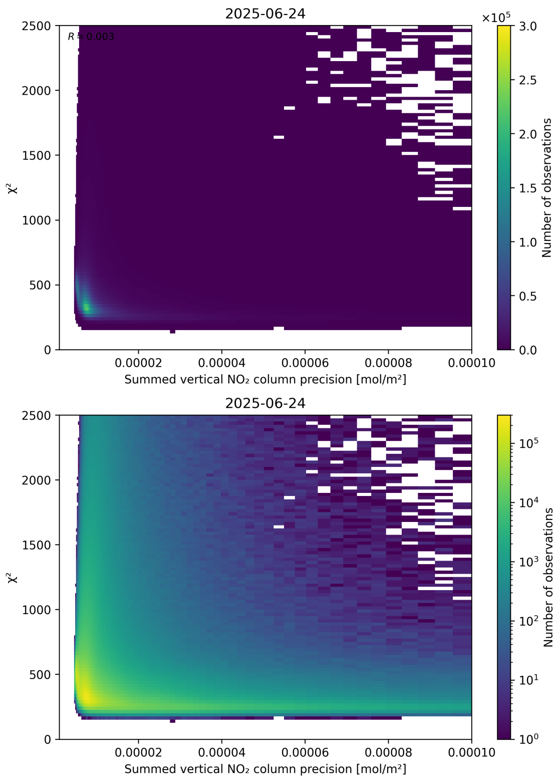
Figure 107: Scatter density plot of “Summed vertical NO 2 column precision” against “ \chi^2 ” for 2025-06-23 to 2025-06-25.
