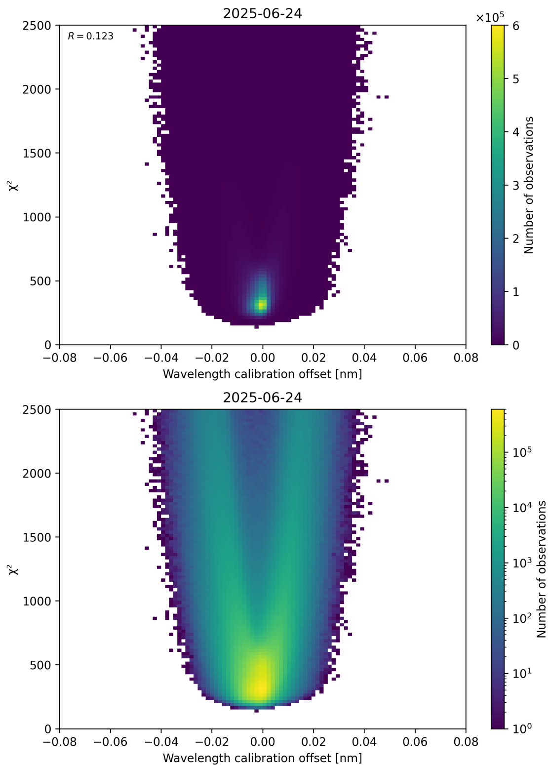
Figure 175: Scatter density plot of “Wavelength calibration offset” against “ \chi^2 ” for 2025-06-23 to 2025-06-25.
