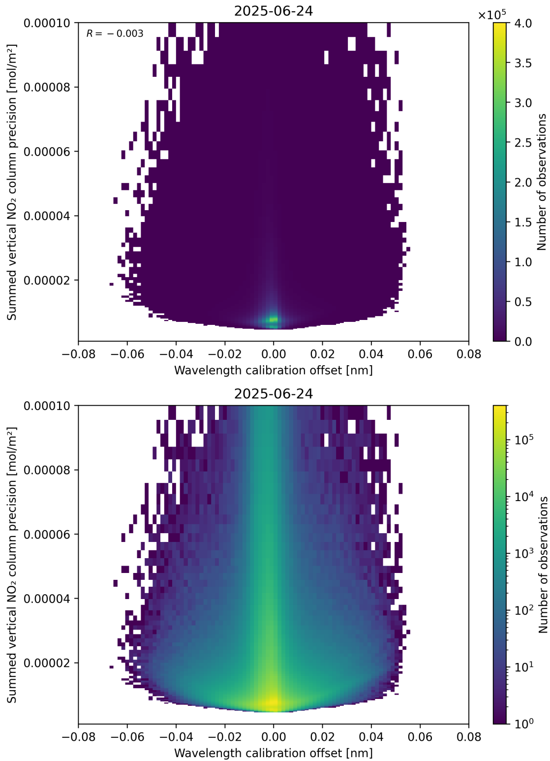
Figure 178: Scatter density plot of “Wavelength calibration offset” against “Summed vertical NO 2 column precision” for 2025-06-23 to 2025-06-25.
