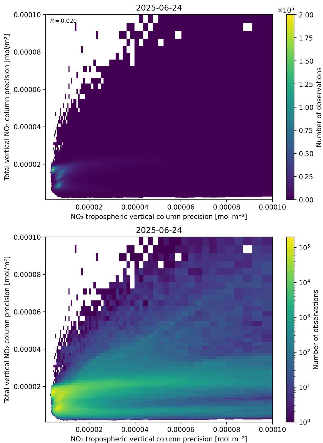
Figure 139: Scatter density plot of “NO 2 tropospheric vertical column precision” against “Total vertical NO 2 column precision” for 2025-06-23 to 2025-06-25.
