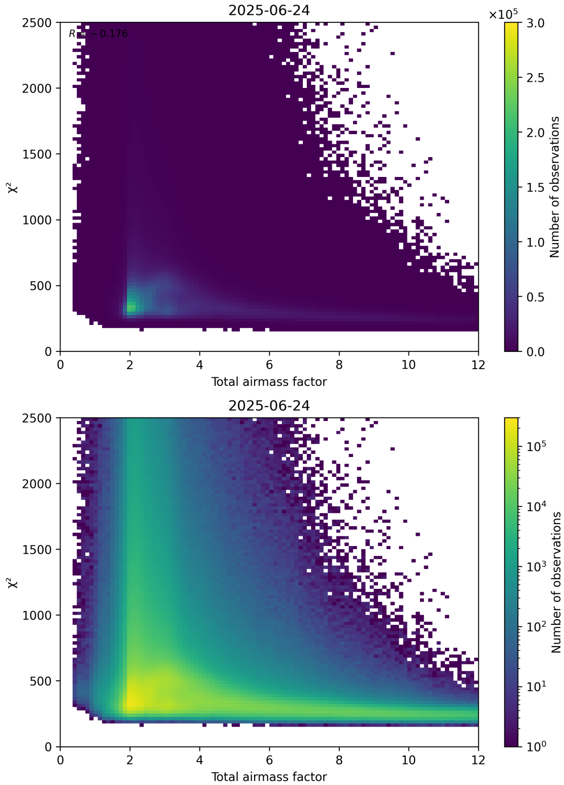
Figure 63: Scatter density plot of “Total airmass factor” against “ \chi^2 ” for 2025-06-23 to 2025-06-25.
