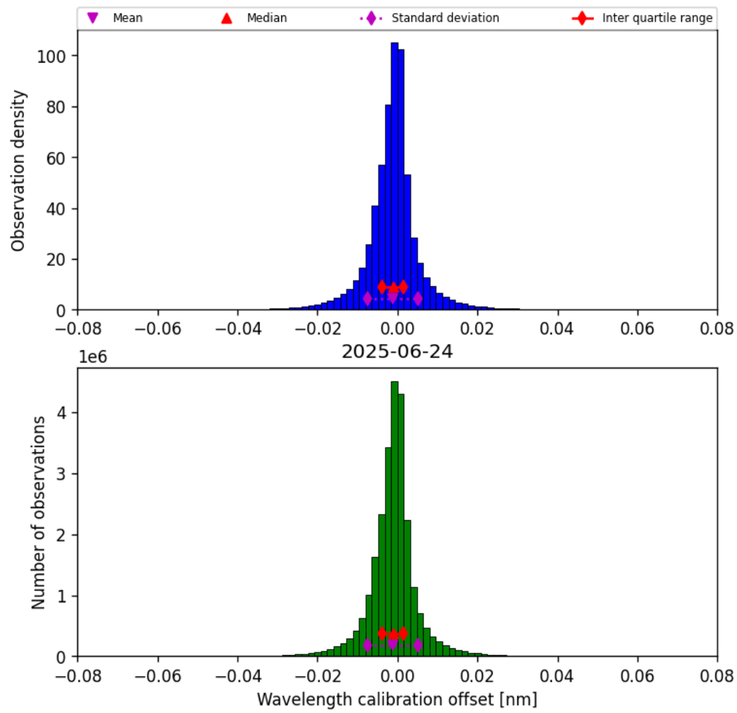
Figure 35: Histogram of “Wavelength calibration offset” for 2025-06-23 to 2025-06-25
