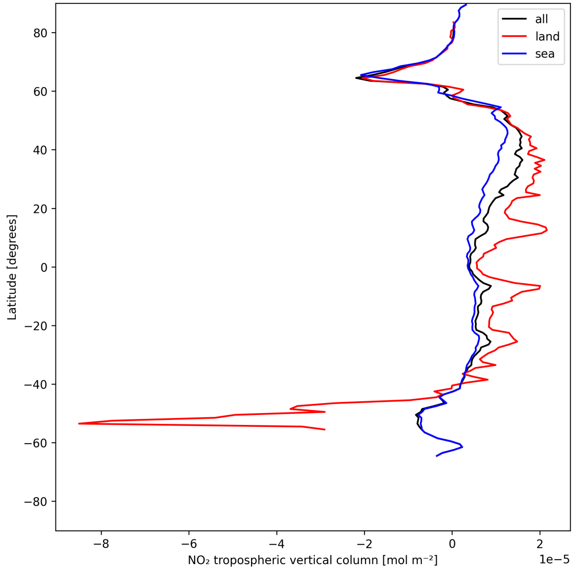
Figure 12: Zonal average of “NO 2 tropospheric vertical column” for 2025-06-23 to 2025-06-25.
