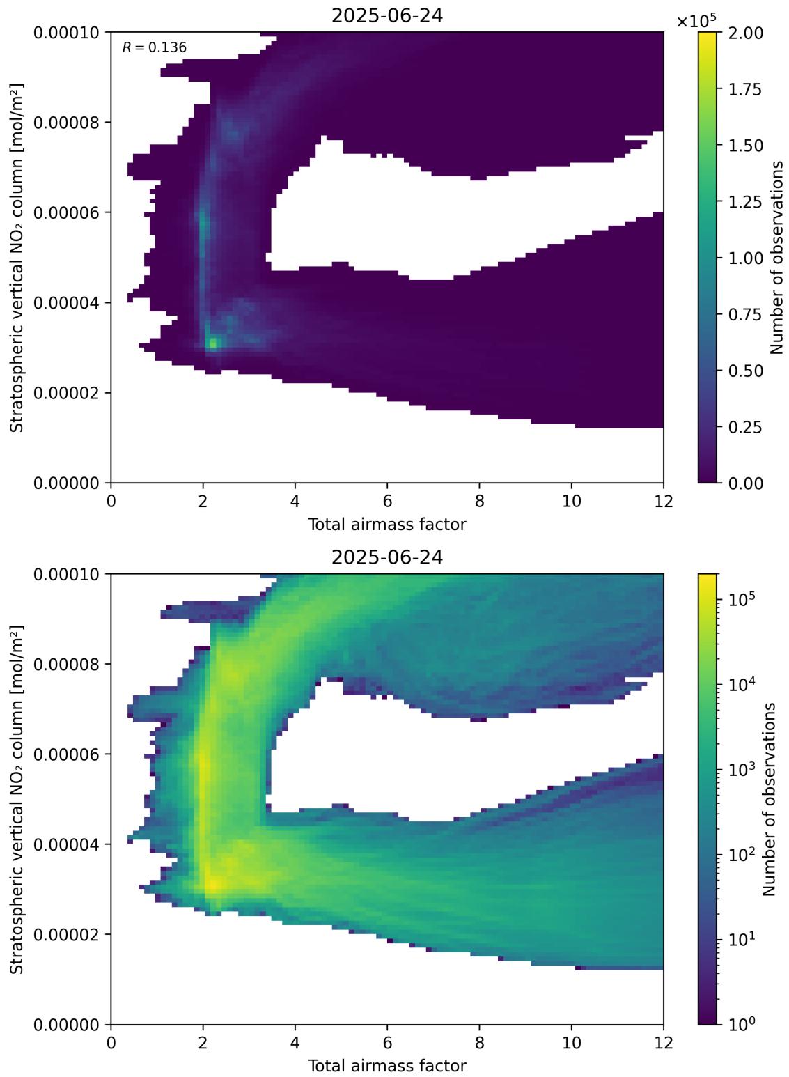
Figure 64: Scatter density plot of “Total airmass factor” against “Stratospheric vertical \text{NO}_2 column” for 2025-06-23 to 2025-06-25.
