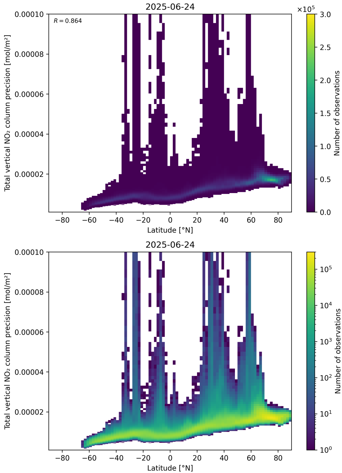
Figure 91: Scatter density plot of “Latitude” against “Total vertical NO 2 column precision” for 2025-06-23 to 2025-06-25.
