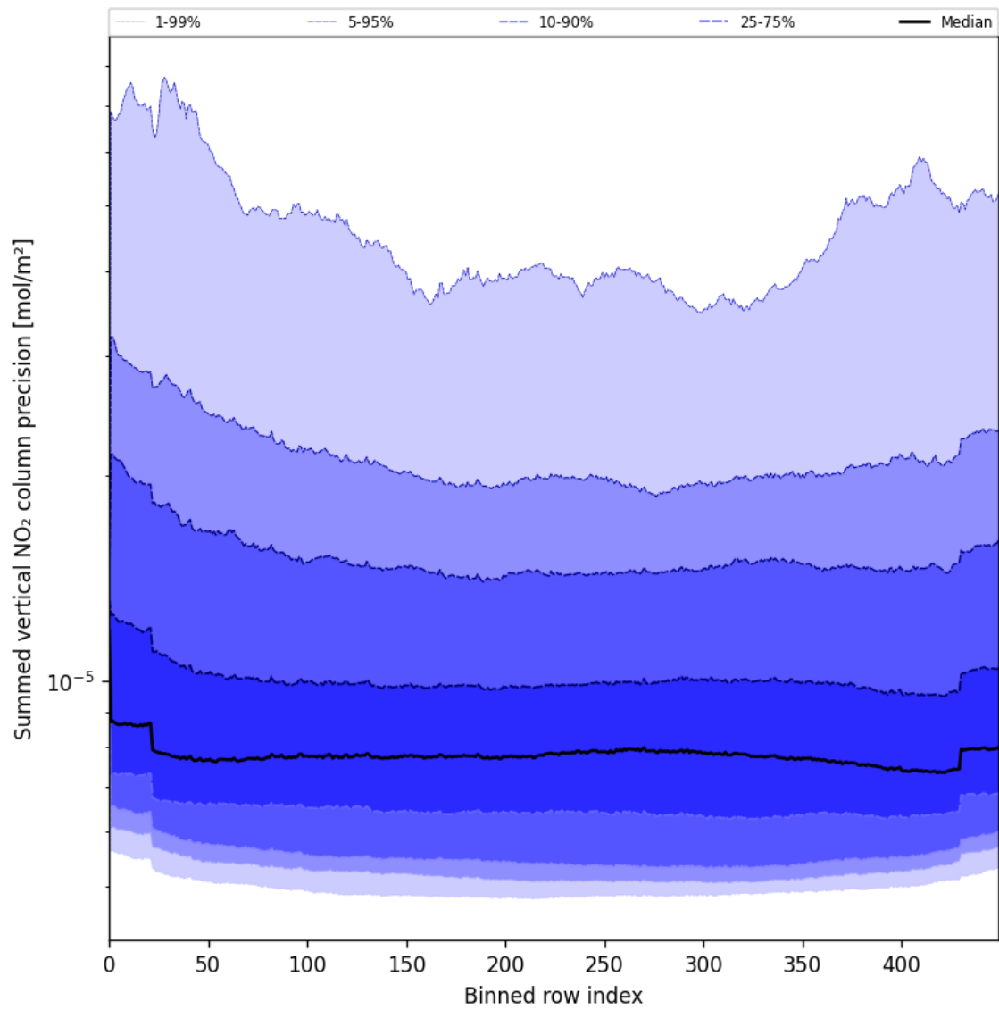
Figure 58: Along track statistics of “Summed vertical NO 2 column precision” for 2025-06-23 to 2025-06-25
