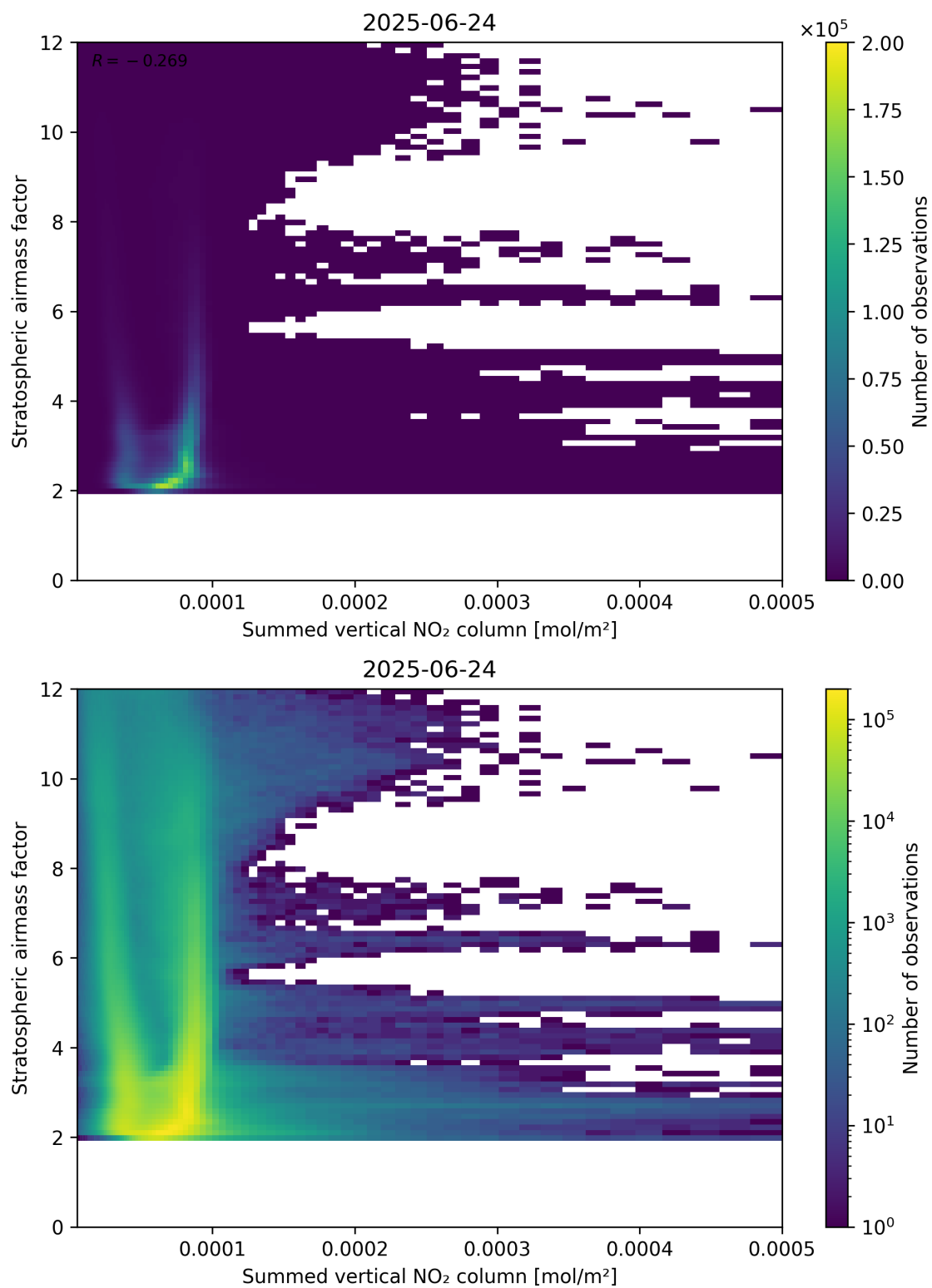
Figure 103: Scatter density plot of “Summed vertical NO 2 column” against “Stratospheric air mass factor” for 2025-06-23 to 2025-06-25.
