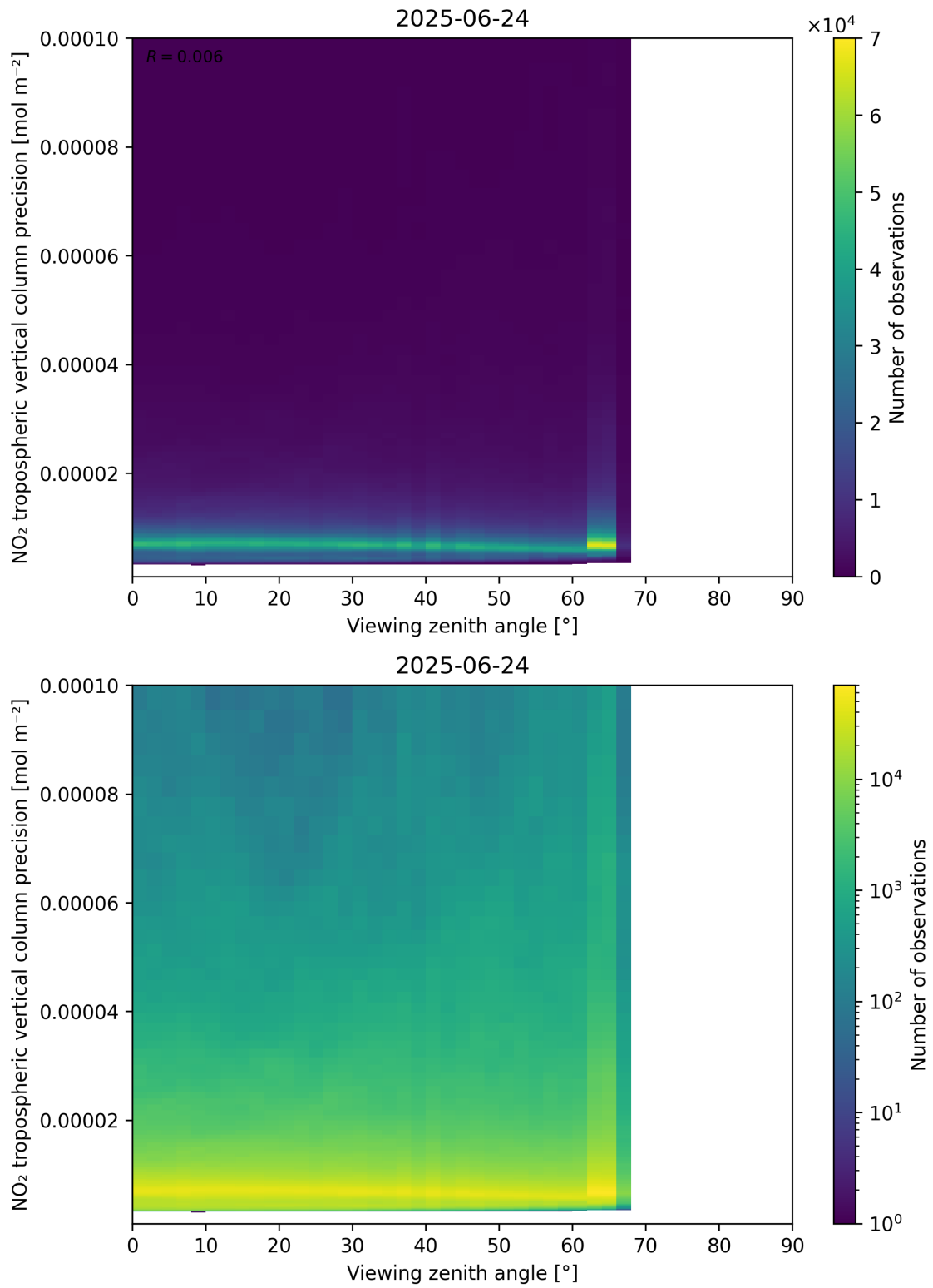
Figure 170: Scatter density plot of “Viewing zenith angle” against “NO 2 tropospheric vertical column precision” for 2025-06-23 to 2025-06-25.
