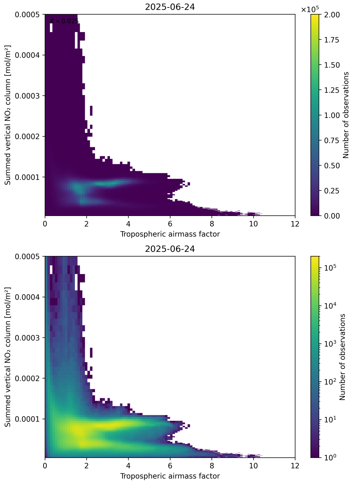
Figure 75: Scatter density plot of “Tropospheric air mass factor” against “Summed vertical NO 2 column” for 2025-06-23 to 2025-06-25.
