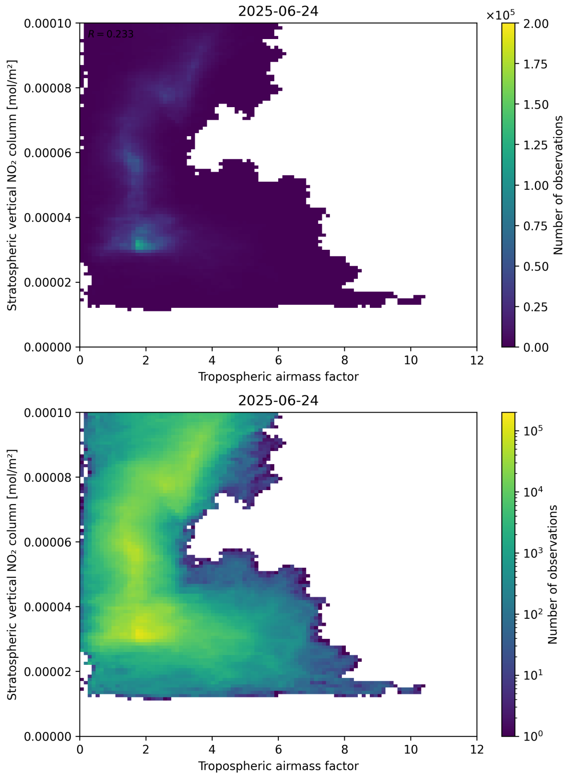
Figure 74: Scatter density plot of “Tropospheric air mass factor” against “Stratospheric vertical NO 2 column” for 2025-06-23 to 2025-06-25.
