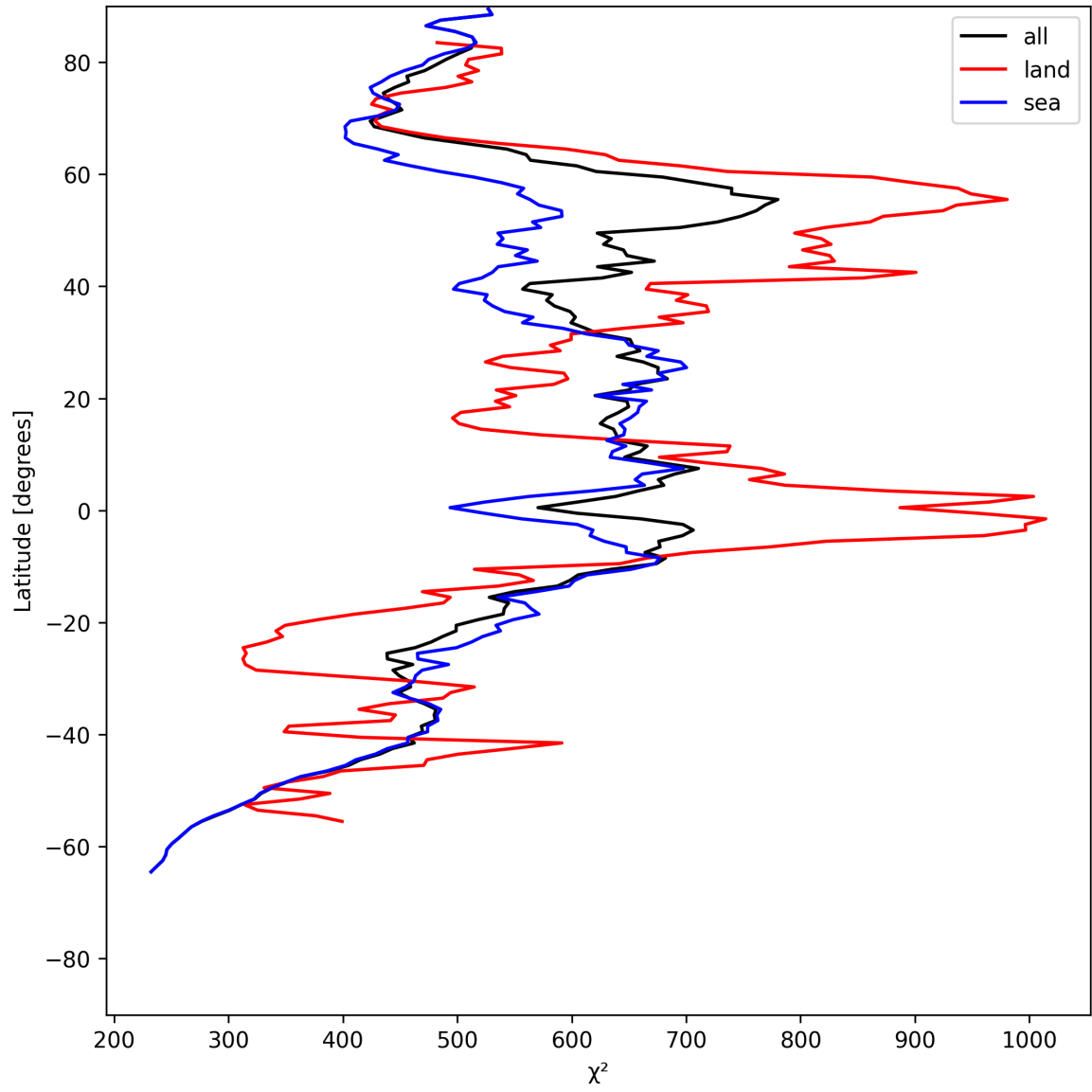
Figure 25: Zonal average of “ \chi^2 ” for 2025-06-23 to 2025-06-25.
