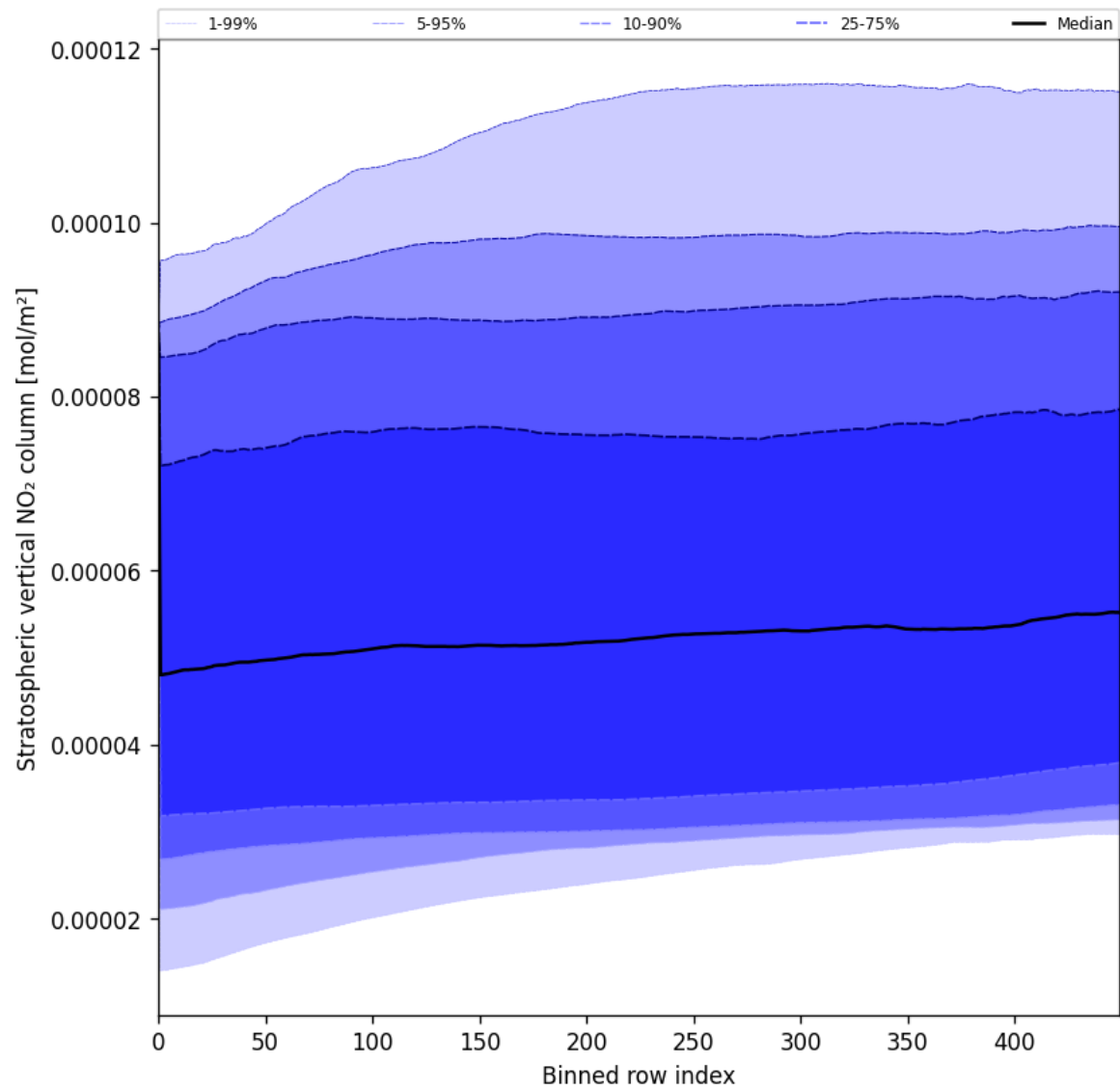
Figure 53: Along track statistics of “Stratospheric vertical NO 2 column” for 2025-06-23 to 2025-06-25
