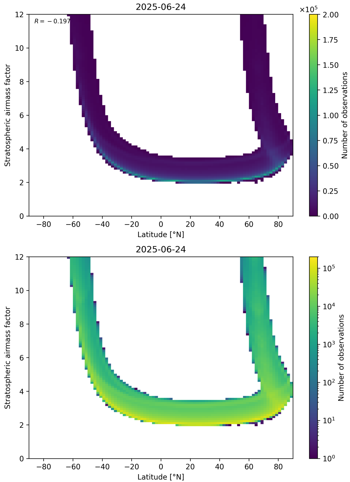
Figure 83: Scatter density plot of “Latitude” against “Stratospheric air mass factor” for 2025-06-23 to 2025-06-25.
