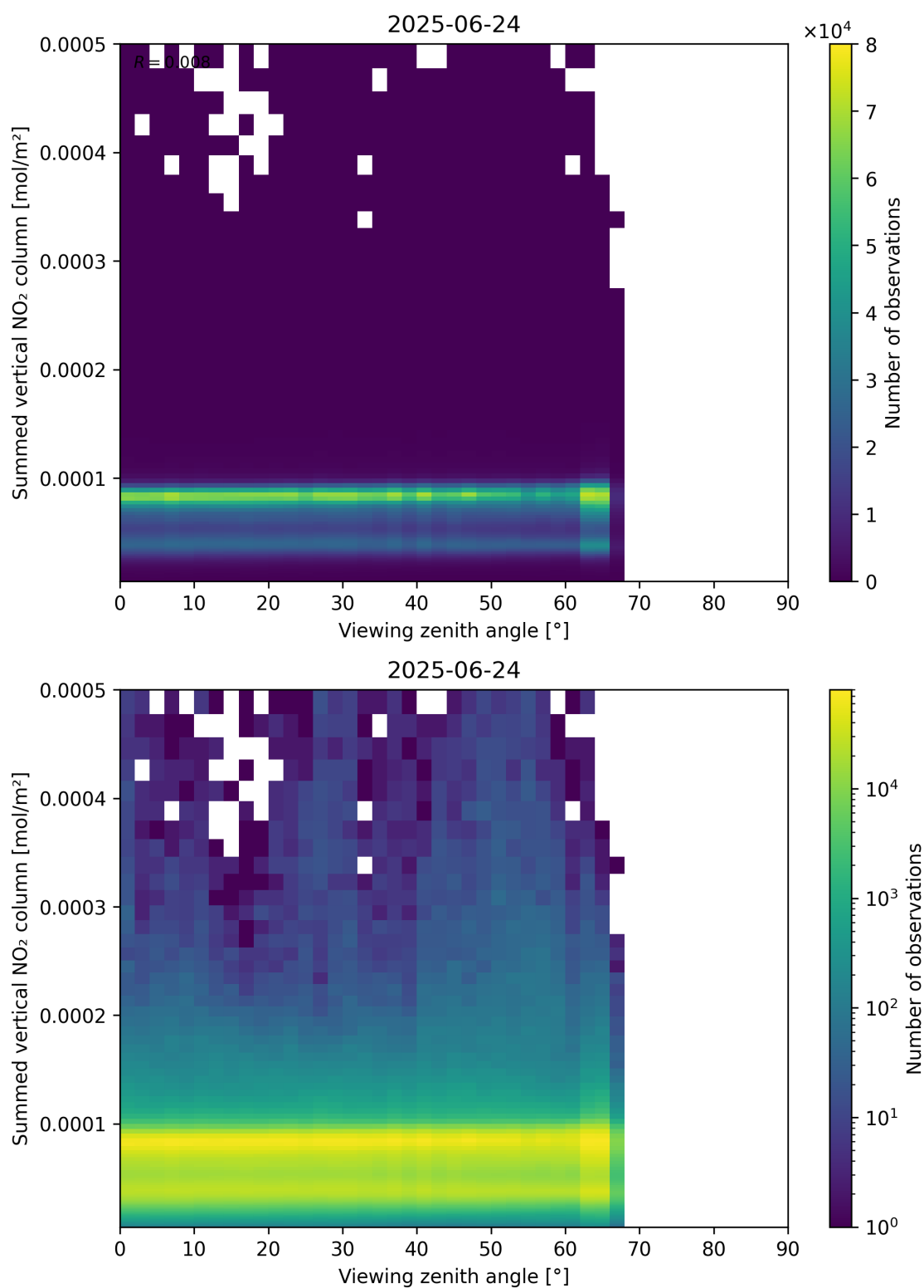
Figure 165: Scatter density plot of “Viewing zenith angle” against “Summed vertical NO 2 column” for 2025-06-23 to 2025-06-25.
