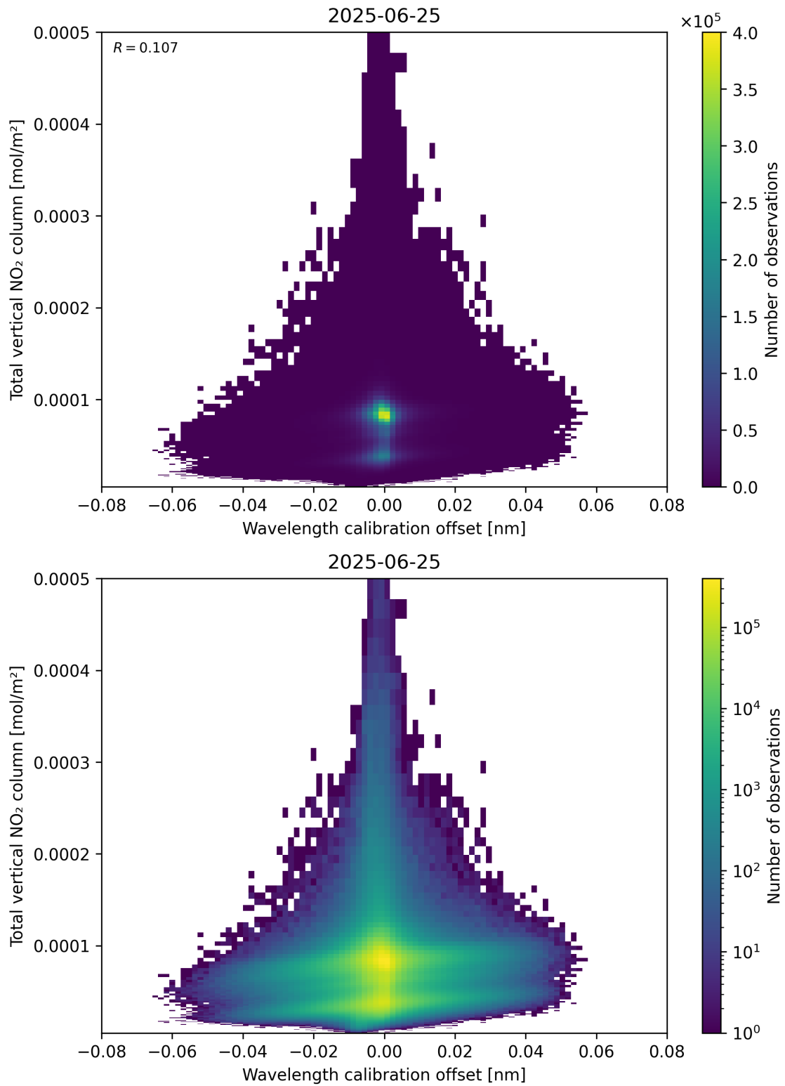
Figure 179: Scatter density plot of “Wavelength calibration offset” against “Total vertical NO 2 column” for 2025-06-24 to 2025-06-26.
