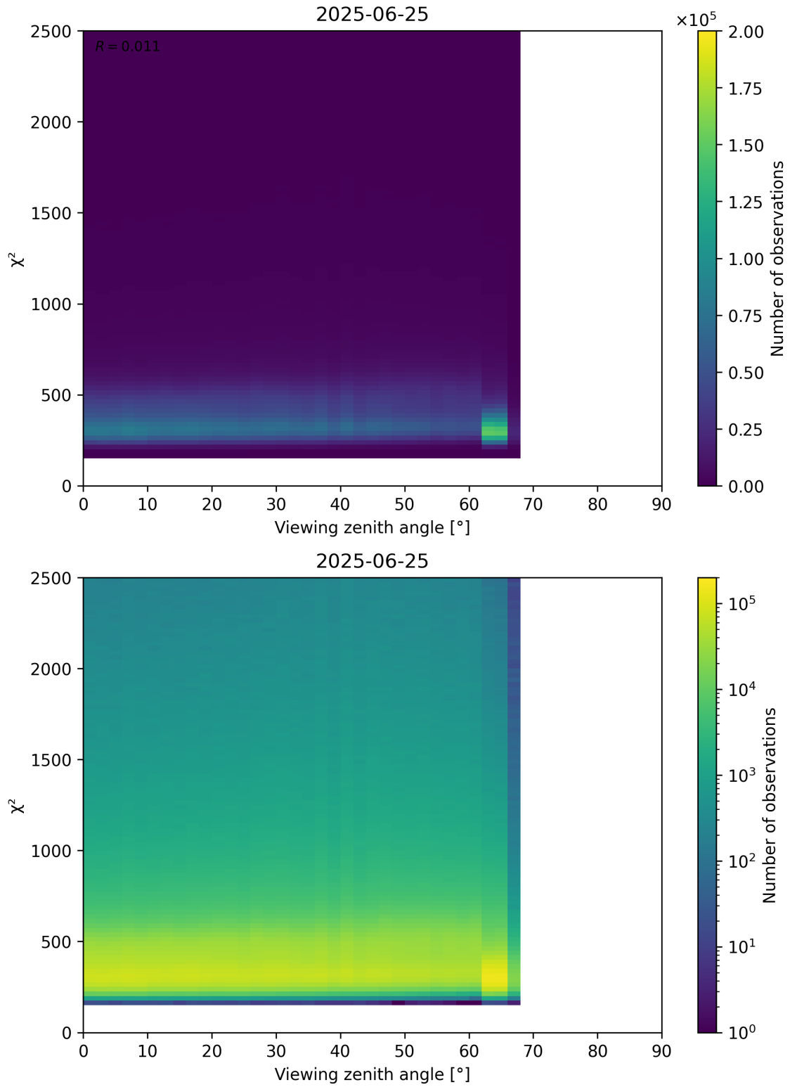
Figure 162: Scatter density plot of “Viewing zenith angle” against “ \chi^2 ” for 2025-06-24 to 2025-06-26.
