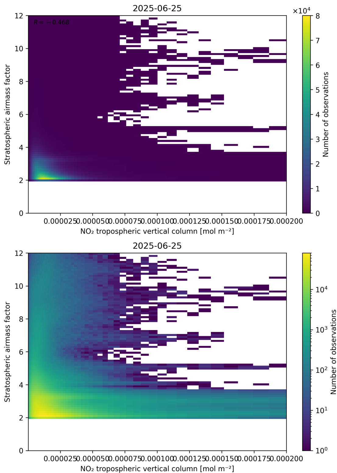
Figure 121: Scatter density plot of “NO 2 tropospheric vertical column” against “Stratospheric air mass factor” for 2025-06-24 to 2025-06-26.
