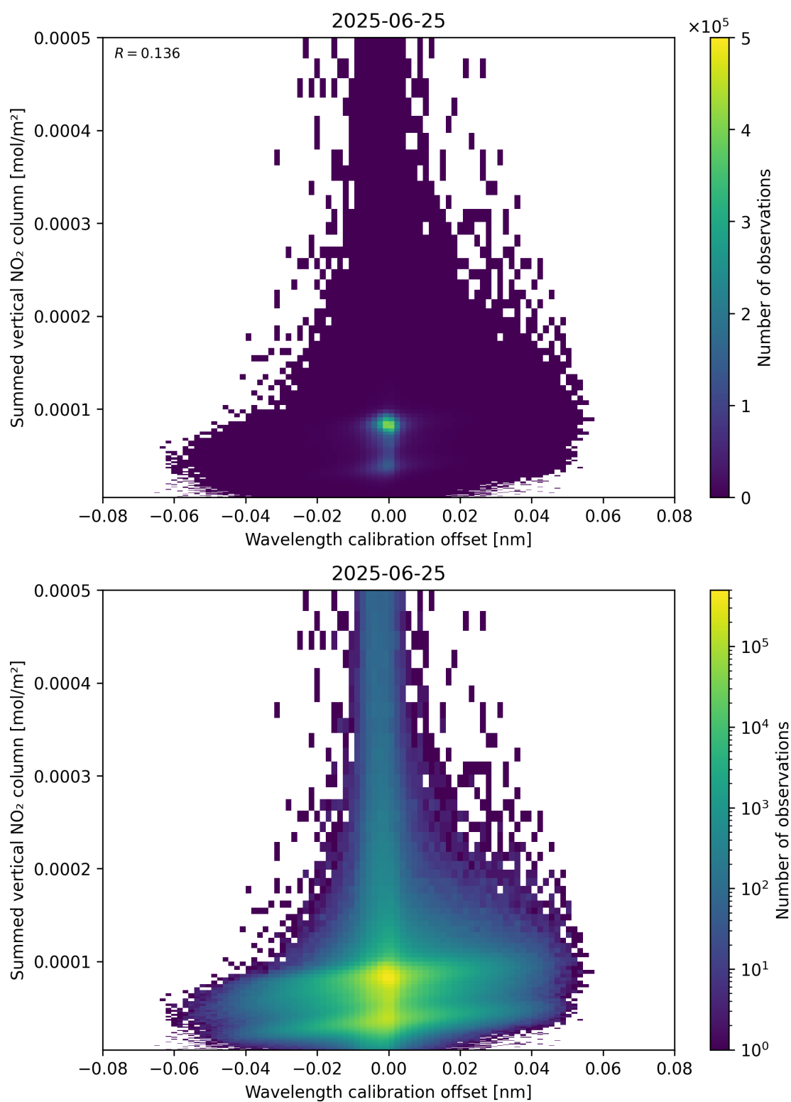
Figure 177: Scatter density plot of “Wavelength calibration offset” against “Summed vertical NO 2 column” for 2025-06-24 to 2025-06-26.
