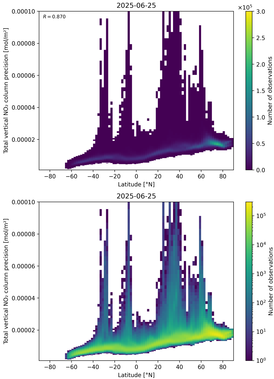
Figure 91: Scatter density plot of “Latitude” against “Total vertical NO 2 column precision” for 2025-06-24 to 2025-06-26.
