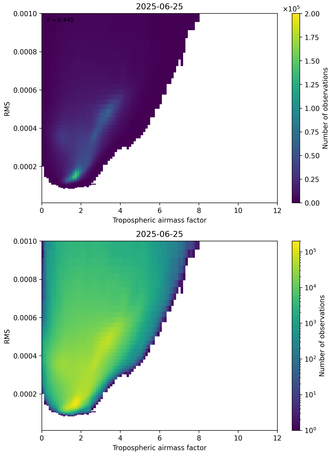
Figure 79: Scatter density plot of “Tropospheric airmass factor” against “RMS” for 2025-06-24 to 2025-06-26.
