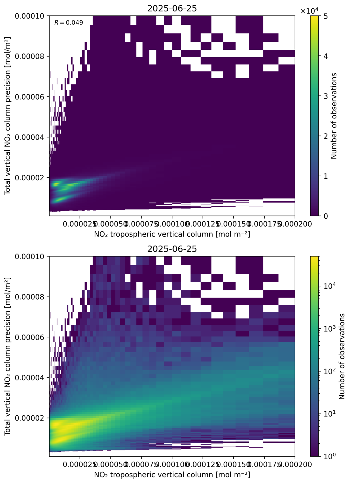
Figure 129: Scatter density plot of “NO 2 tropospheric vertical column” against “Total vertical NO 2 column precision” for 2025-06-24 to 2025-06-26.
