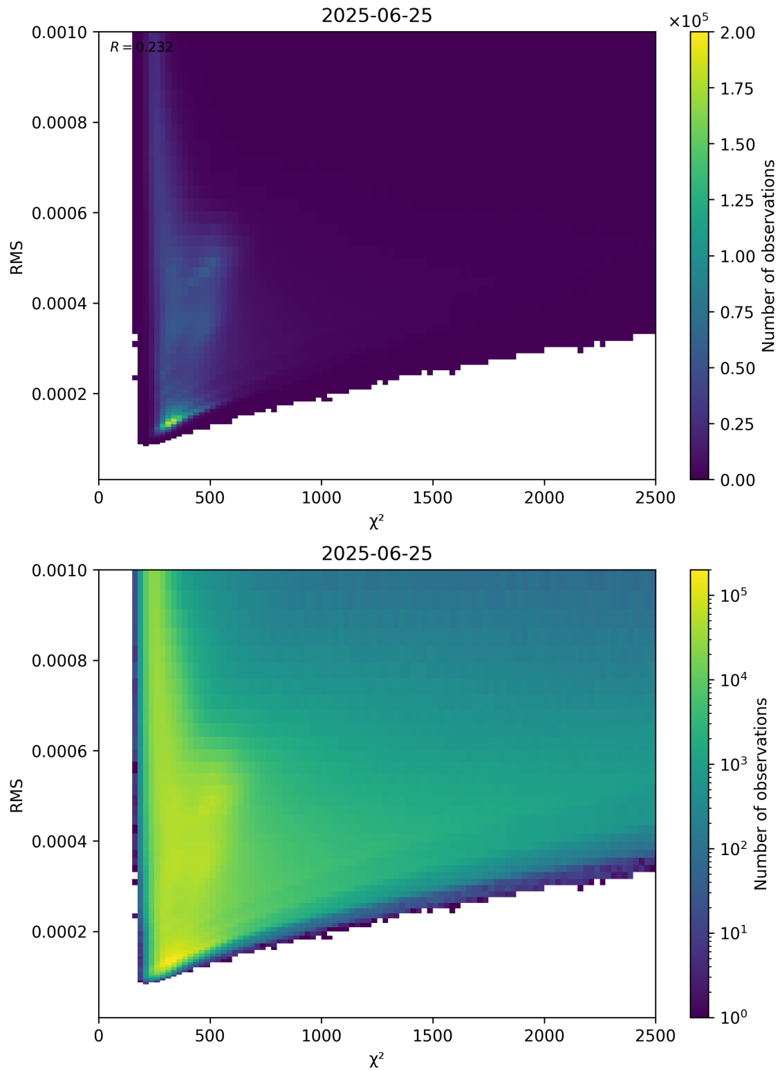
Figure 82: Scatter density plot of “ \chi^2 ” against “RMS” for 2025-06-24 to 2025-06-26.
