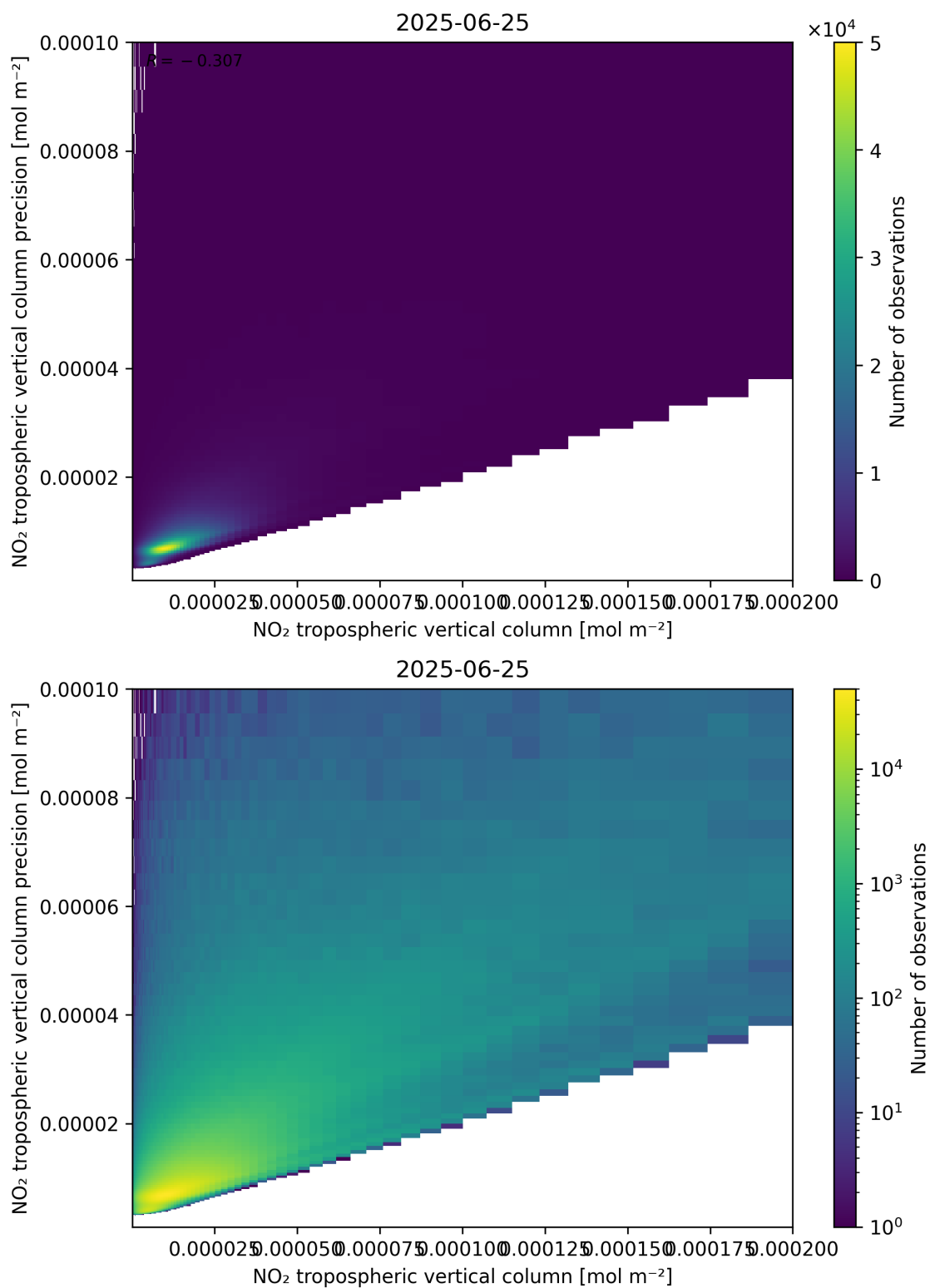
Figure 130: Scatter density plot of “NO 2 tropospheric vertical column” against “NO 2 tropospheric vertical column precision” for 2025-06-24 to 2025-06-26.
