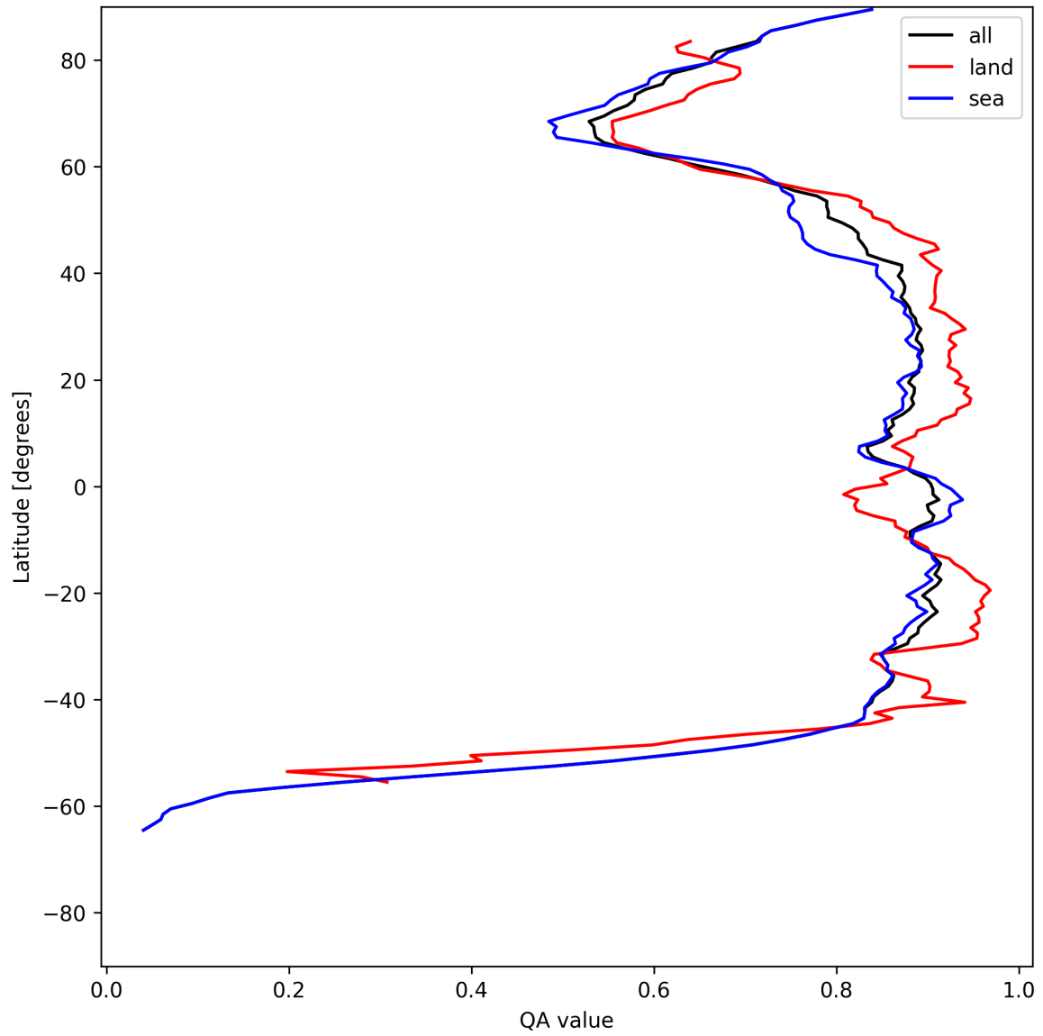
Figure 11: Zonal average of “QA value” for 2025-06-24 to 2025-06-26.
