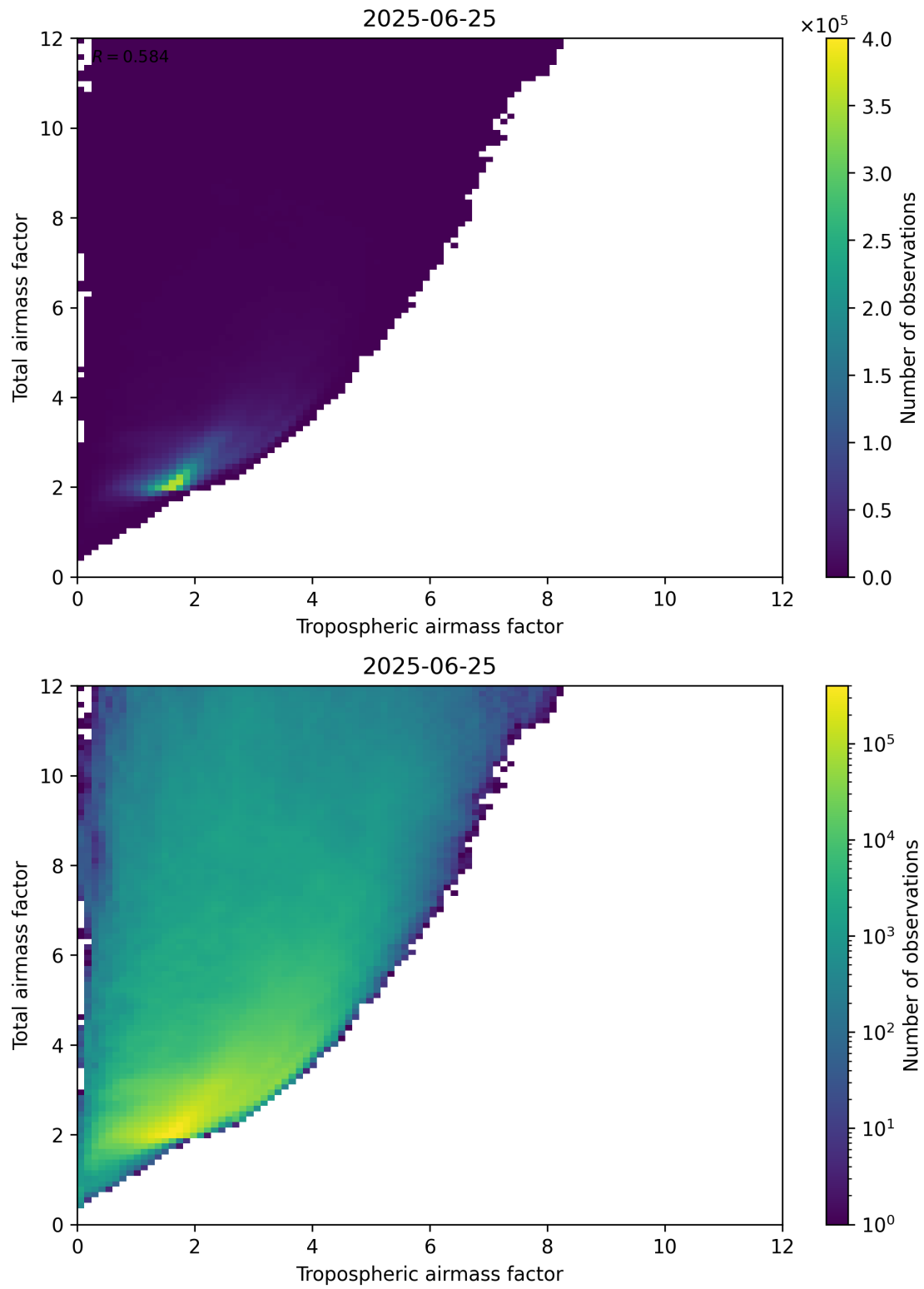
Figure 72: Scatter density plot of “Tropospheric airmass factor” against “Total airmass factor” for 2025-06-24 to 2025-06-26.
