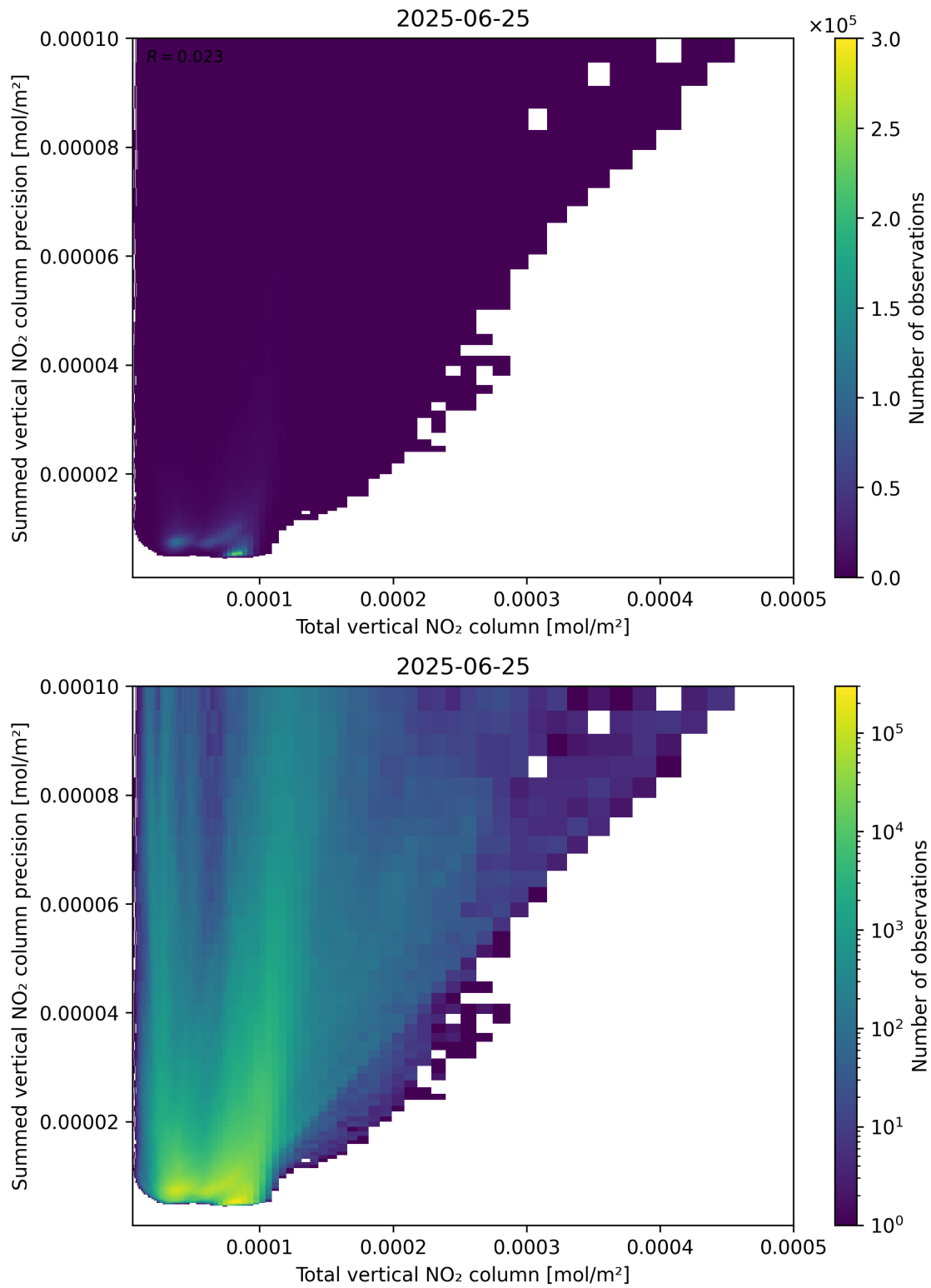
Figure 113: Scatter density plot of “Total vertical NO 2 column” against “Summed vertical NO 2 column precision” for 2025-06-24 to 2025-06-26.
