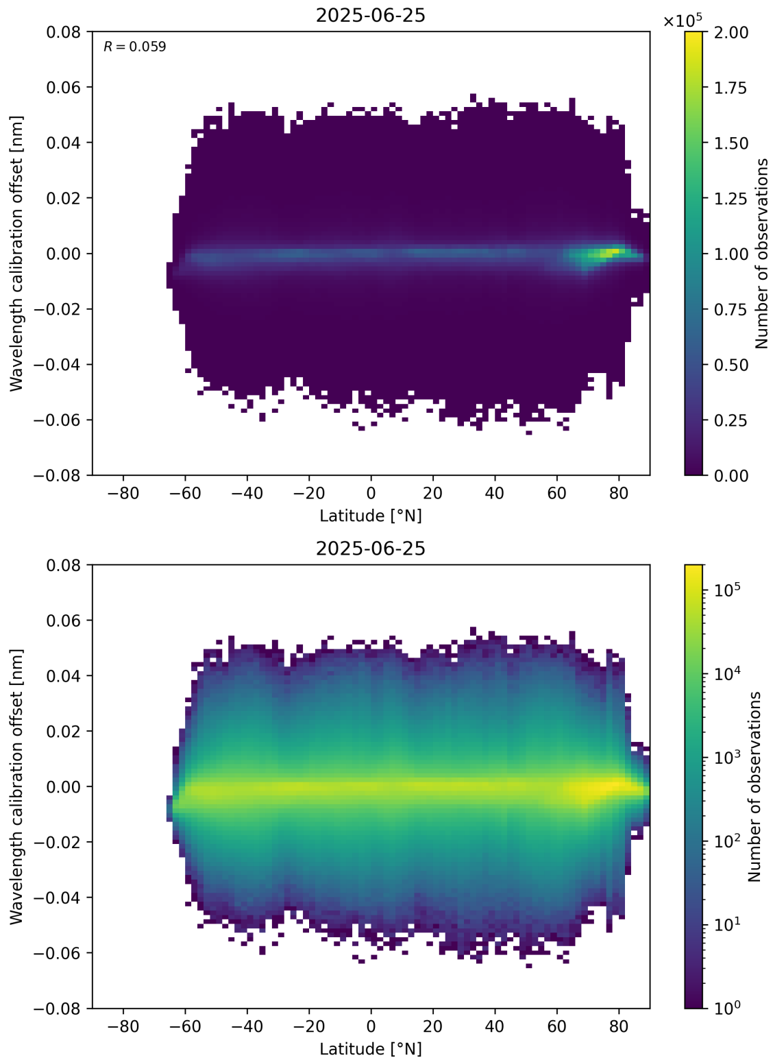
Figure 95: Scatter density plot of “Latitude” against “Wavelength calibration offset” for 2025-06-24 to 2025-06-26.
