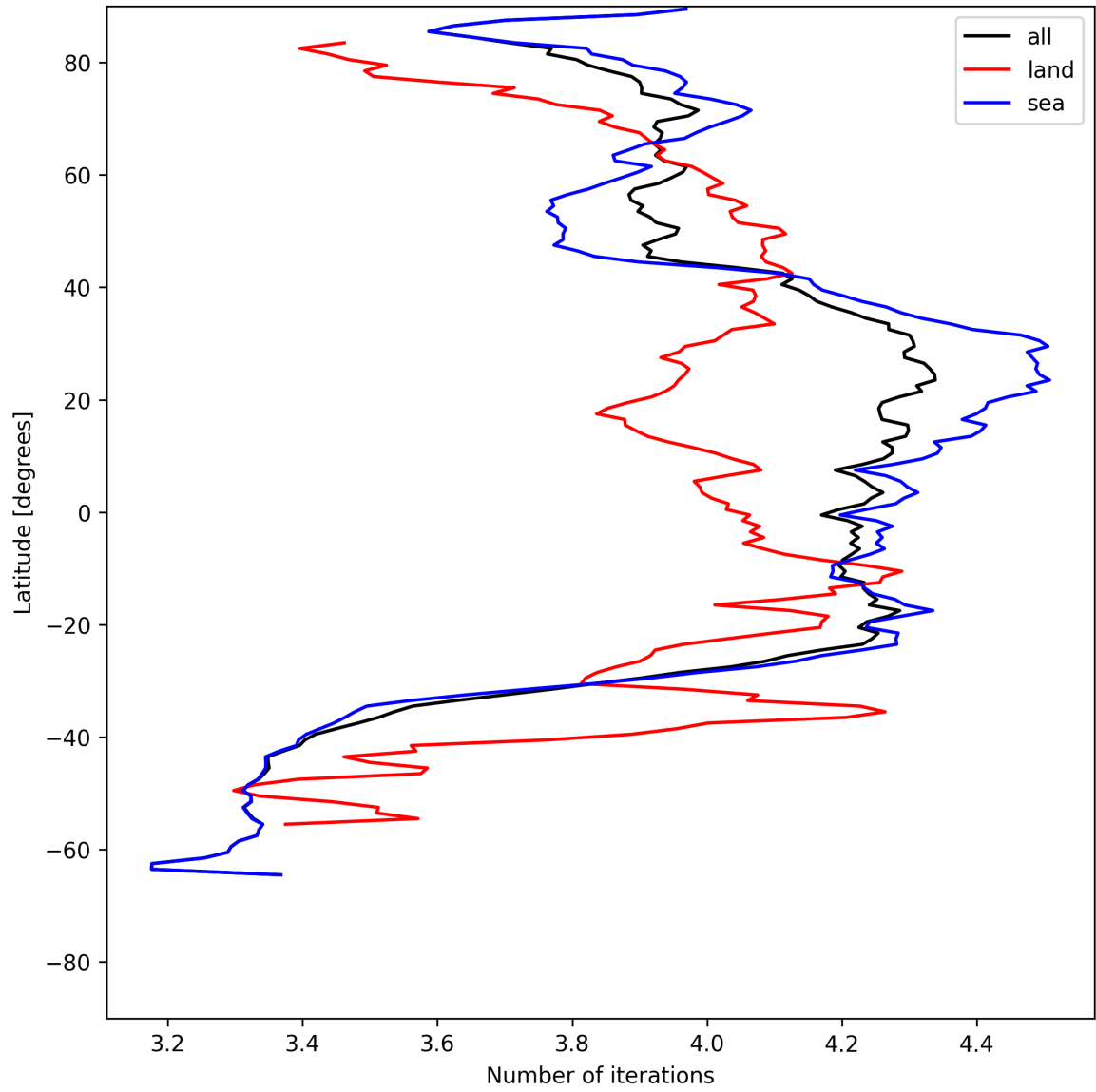
Figure 17: Zonal average of “Number of iterations” for 2025-06-24 to 2025-06-26.
