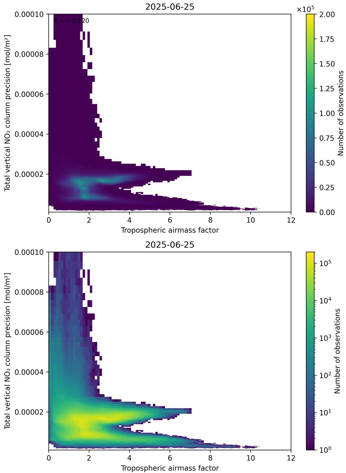
Figure 78: Scatter density plot of “Tropospheric air mass factor” against “Total vertical NO 2 column precision” for 2025-06-24 to 2025-06-26.
