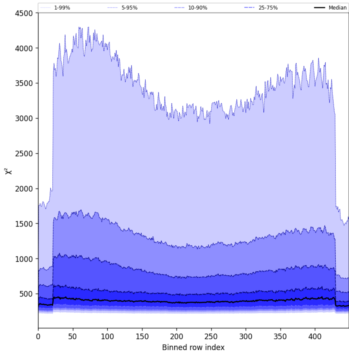
Figure 59: Along track statistics of “ \chi^2 ” for 2025-06-24 to 2025-06-26
