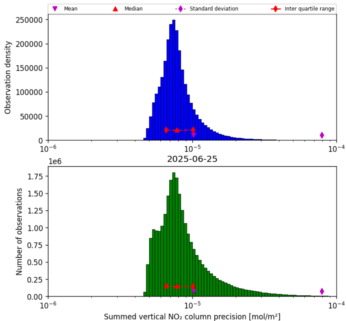
Figure 41: Histogram of “Summed vertical NO 2 column precision” for 2025-06-24 to 2025-06-26
