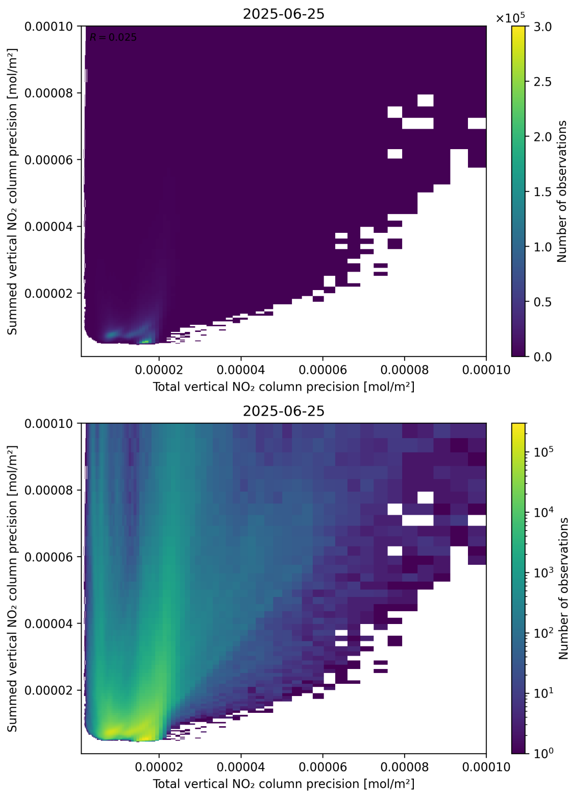
Figure 118: Scatter density plot of “Total vertical NO 2 column precision” against “Summed vertical NO 2 column precision” for 2025-06-24 to 2025-06-26.
