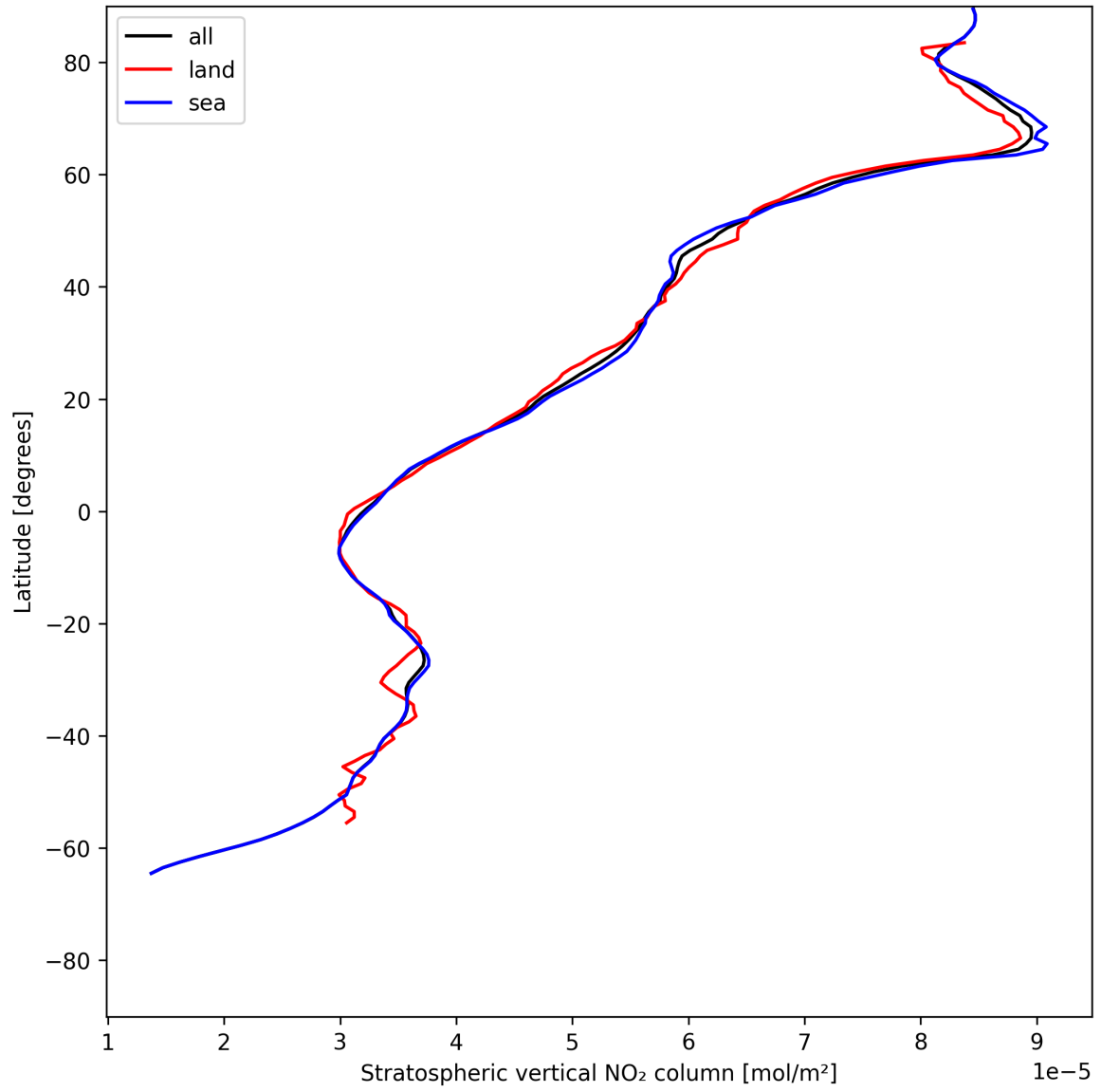
Figure 19: Zonal average of “Stratospheric vertical NO 2 column” for 2025-06-24 to 2025-06-26.
