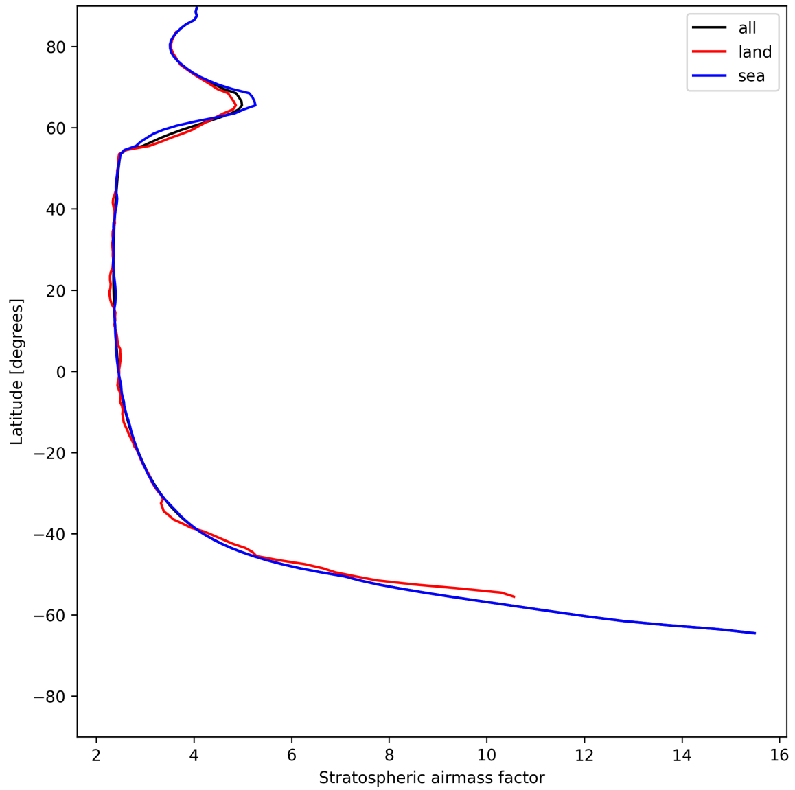
Figure 27: Zonal average of “Stratospheric airmass factor” for 2025-06-24 to 2025-06-26.
