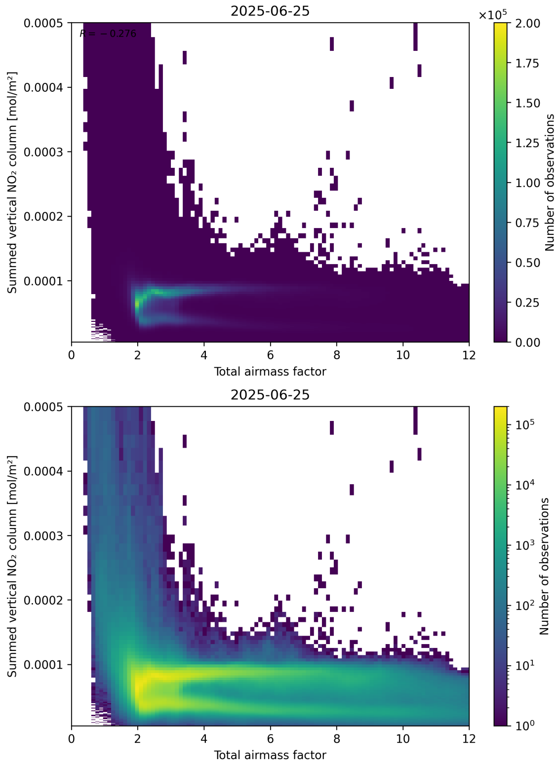
Figure 65: Scatter density plot of “Total airmass factor” against “Summed vertical NO 2 column” for 2025-06-24 to 2025-06-26.
