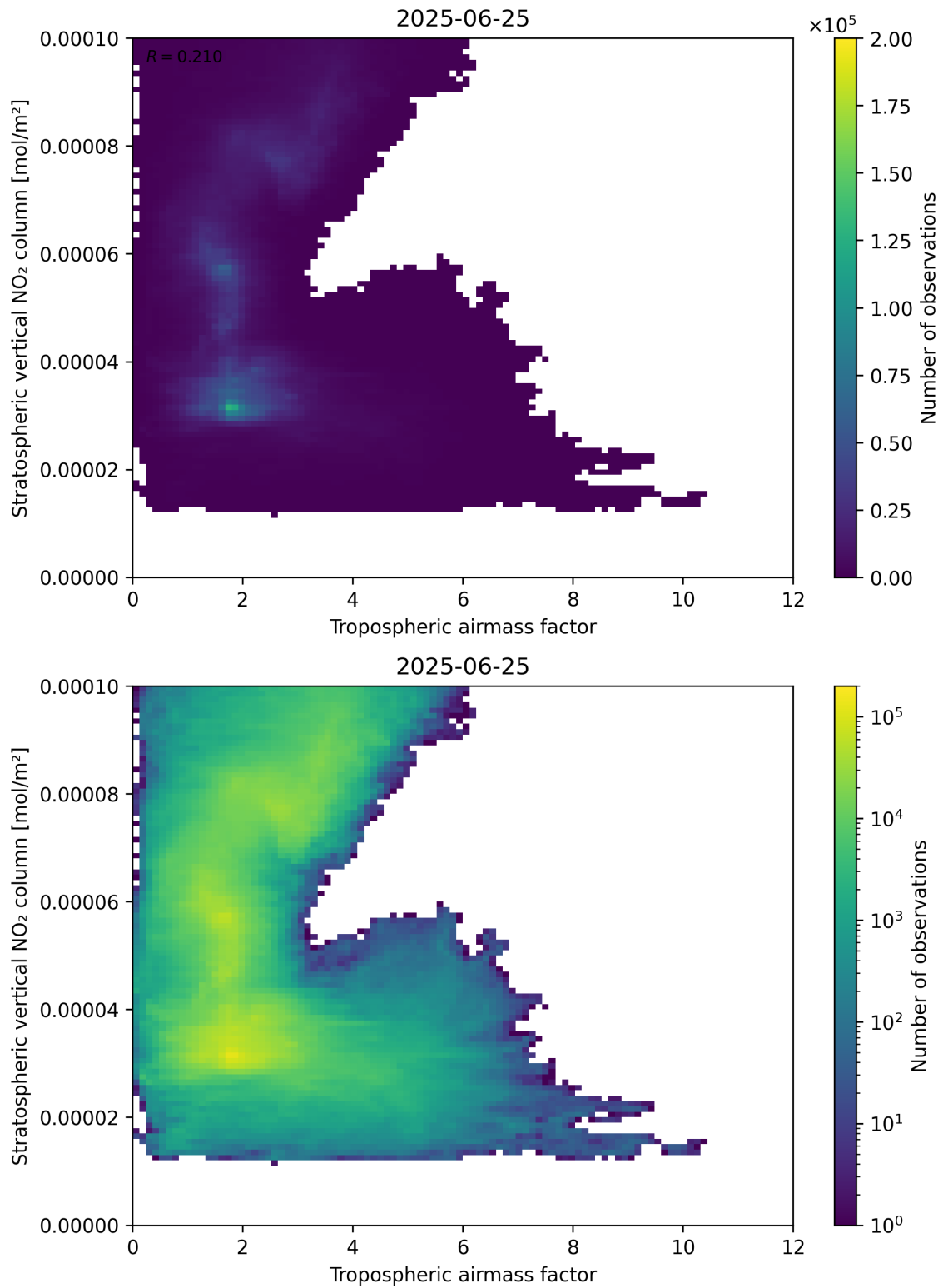
Figure 74: Scatter density plot of “Tropospheric air mass factor” against “Stratospheric vertical NO 2 column” for 2025-06-24 to 2025-06-26.
