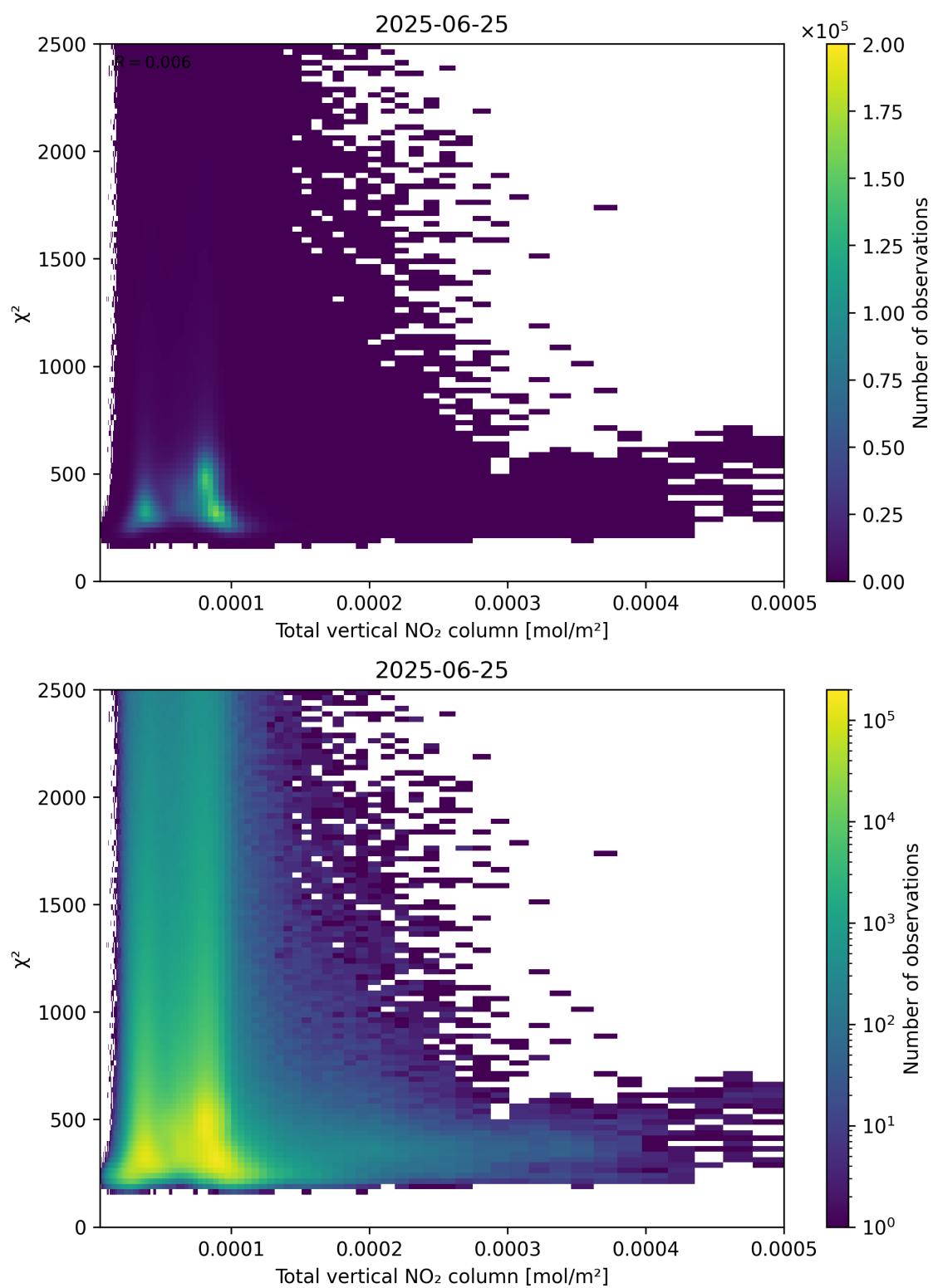
Figure 111: Scatter density plot of “Total vertical NO 2 column” against “ \chi^2 ” for 2025-06-24 to 2025-06-26.
