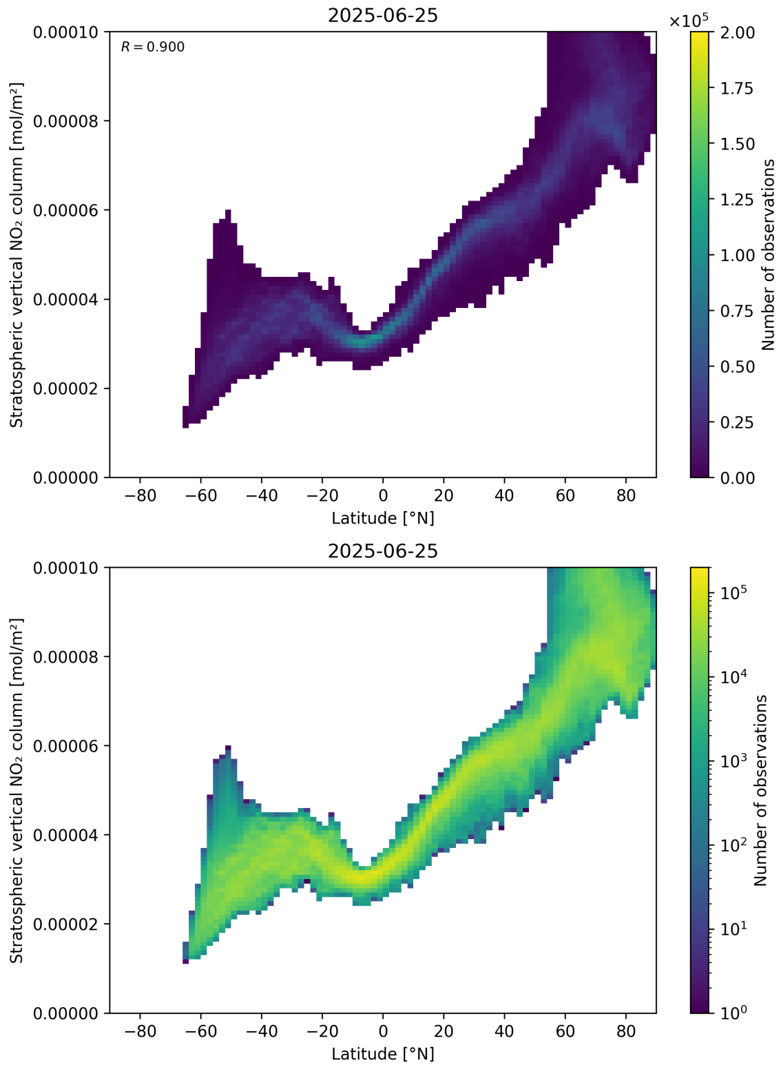
Figure 87: Scatter density plot of “Latitude” against “Stratospheric vertical NO 2 column” for 2025-06-24 to 2025-06-26.
