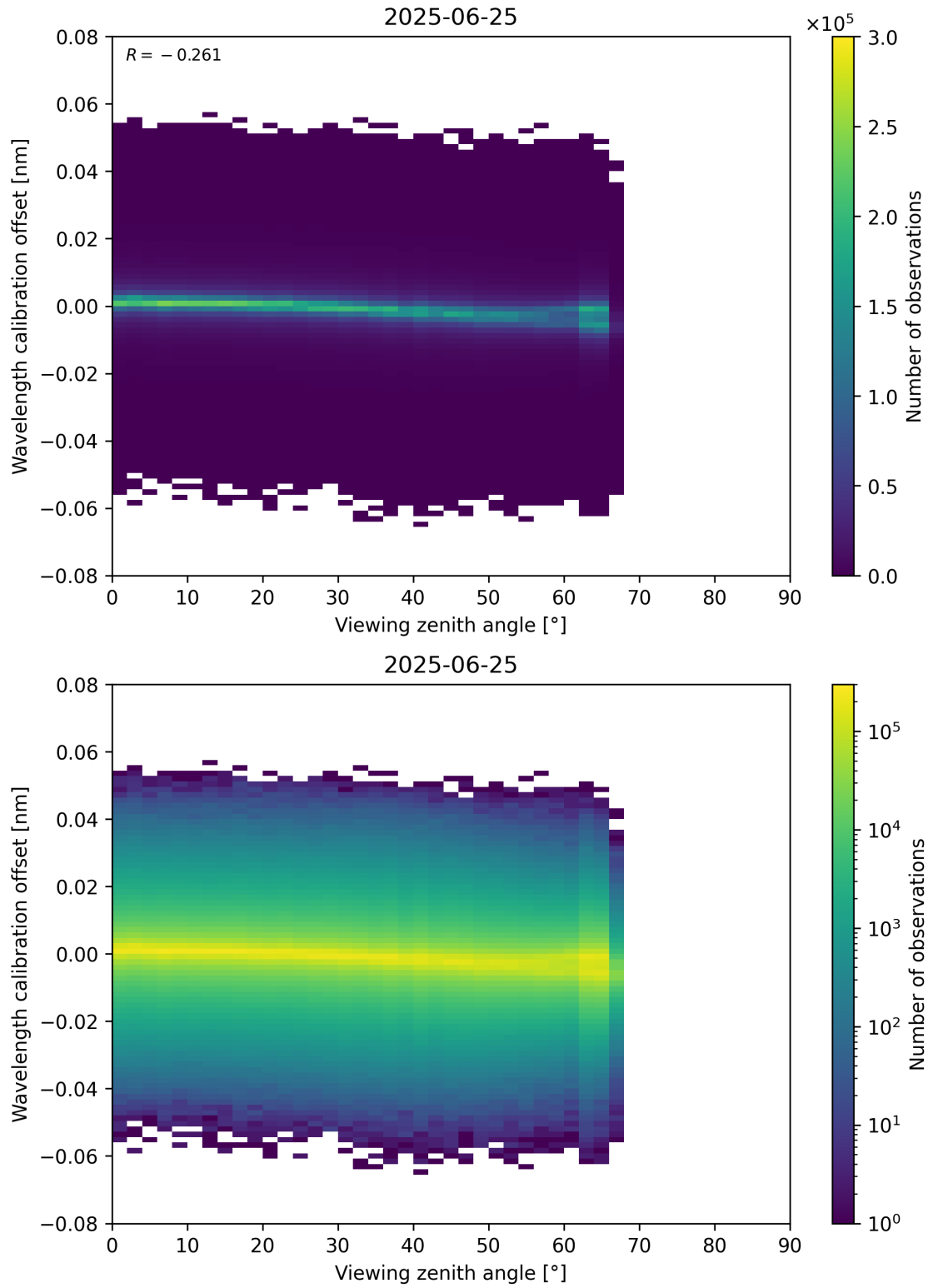
Figure 173: Scatter density plot of “Viewing zenith angle” against “Wavelength calibration offset” for 2025-06-24 to 2025-06-26.
