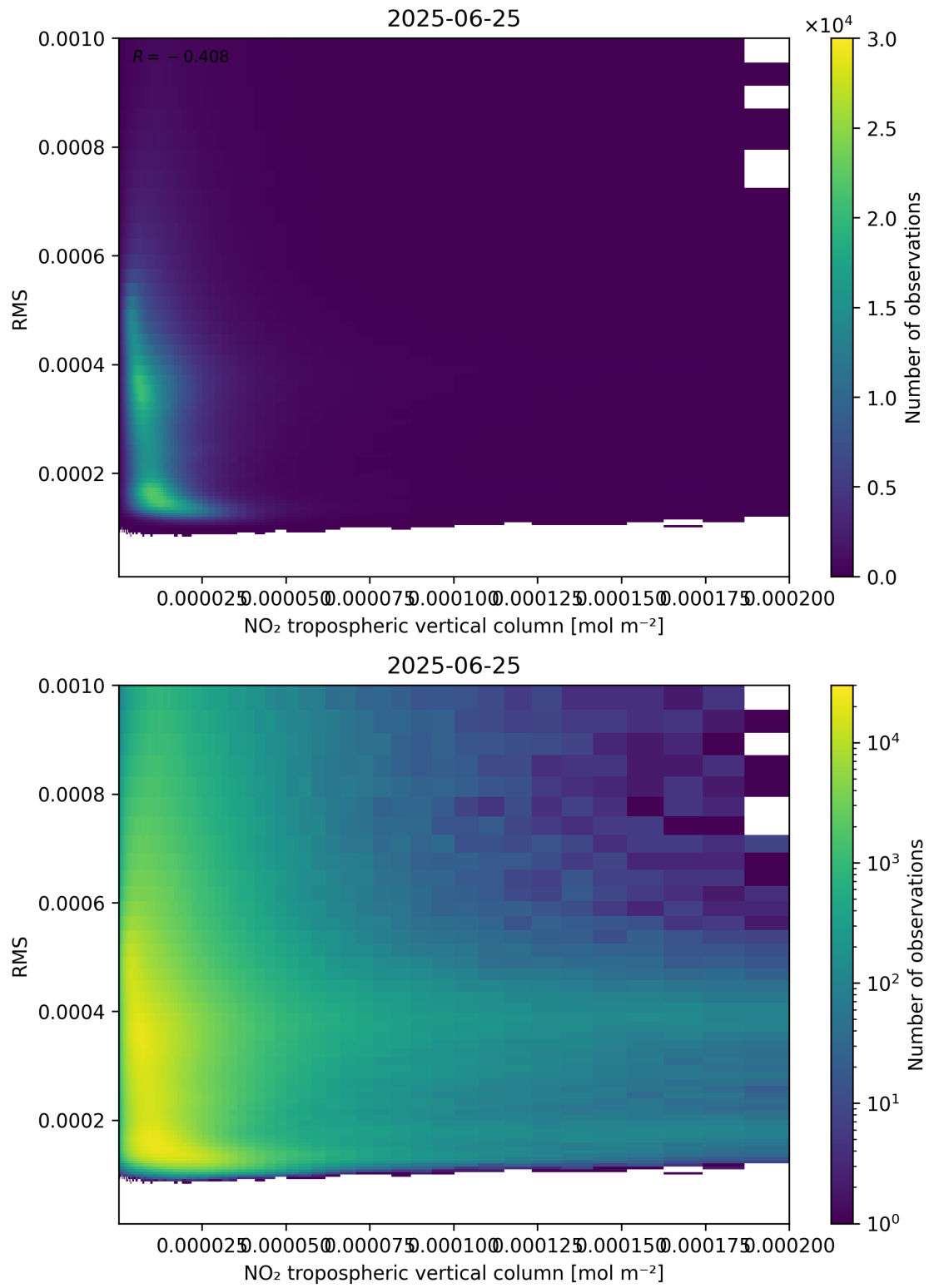
Figure 142: Scatter density plot of “NO 2 tropospheric vertical column” against “RMS” for 2025-06-24 to 2025-06-26.
