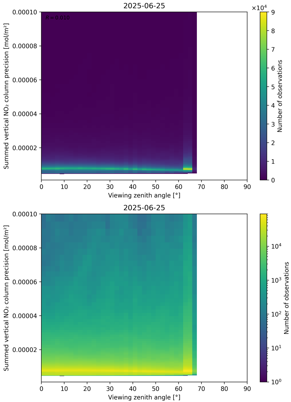
Figure 166: Scatter density plot of “Viewing zenith angle” against “Summed vertical NO 2 column precision” for 2025-06-24 to 2025-06-26.
