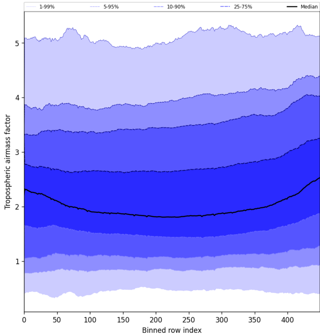
Figure 48: Along track statistics of “Tropospheric airmass factor” for 2025-06-24 to 2025-06-26
