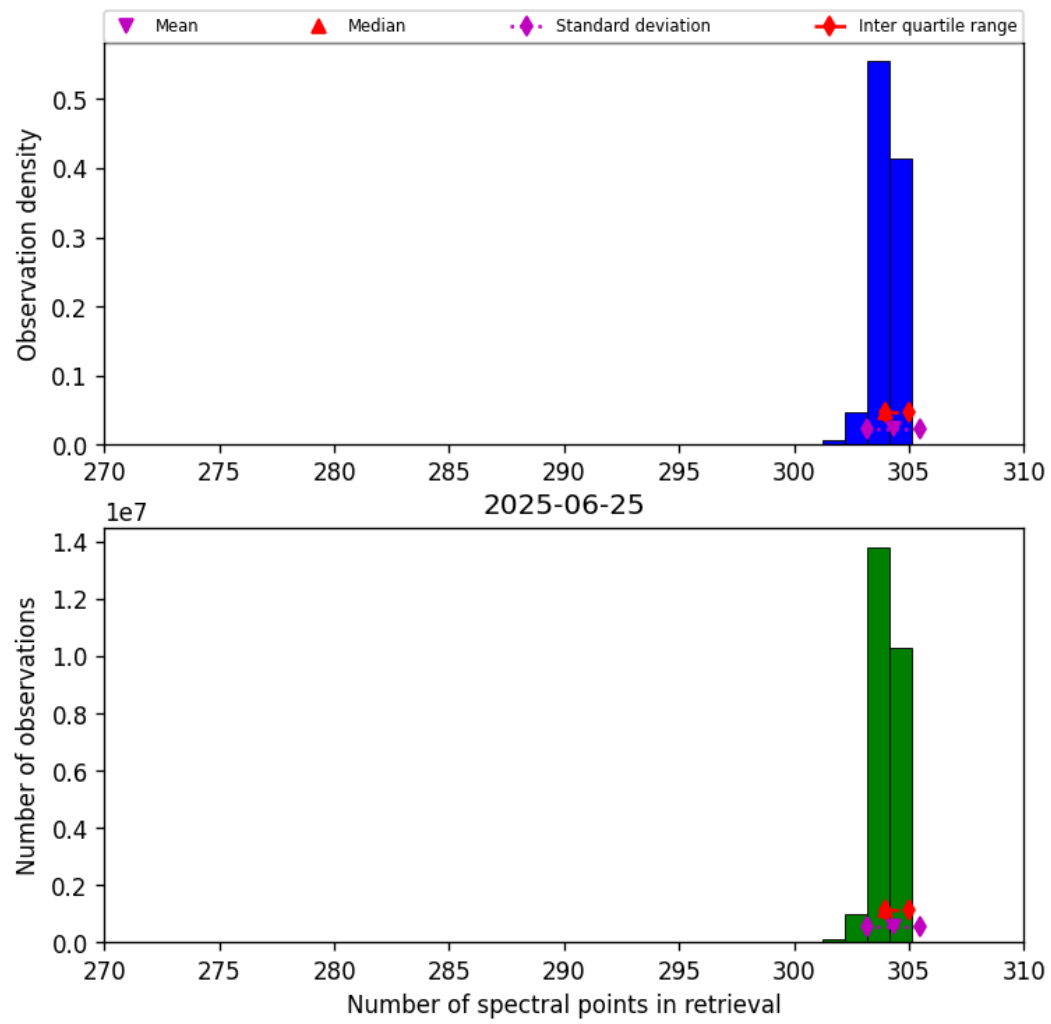
Figure 33: Histogram of “Number of spectral points in retrieval” for 2025-06-24 to 2025-06-26
