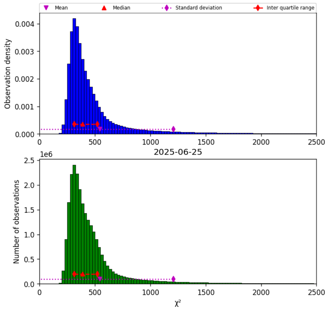
Figure 42: Histogram of “ \chi^2 ” for 2025-06-24 to 2025-06-26
