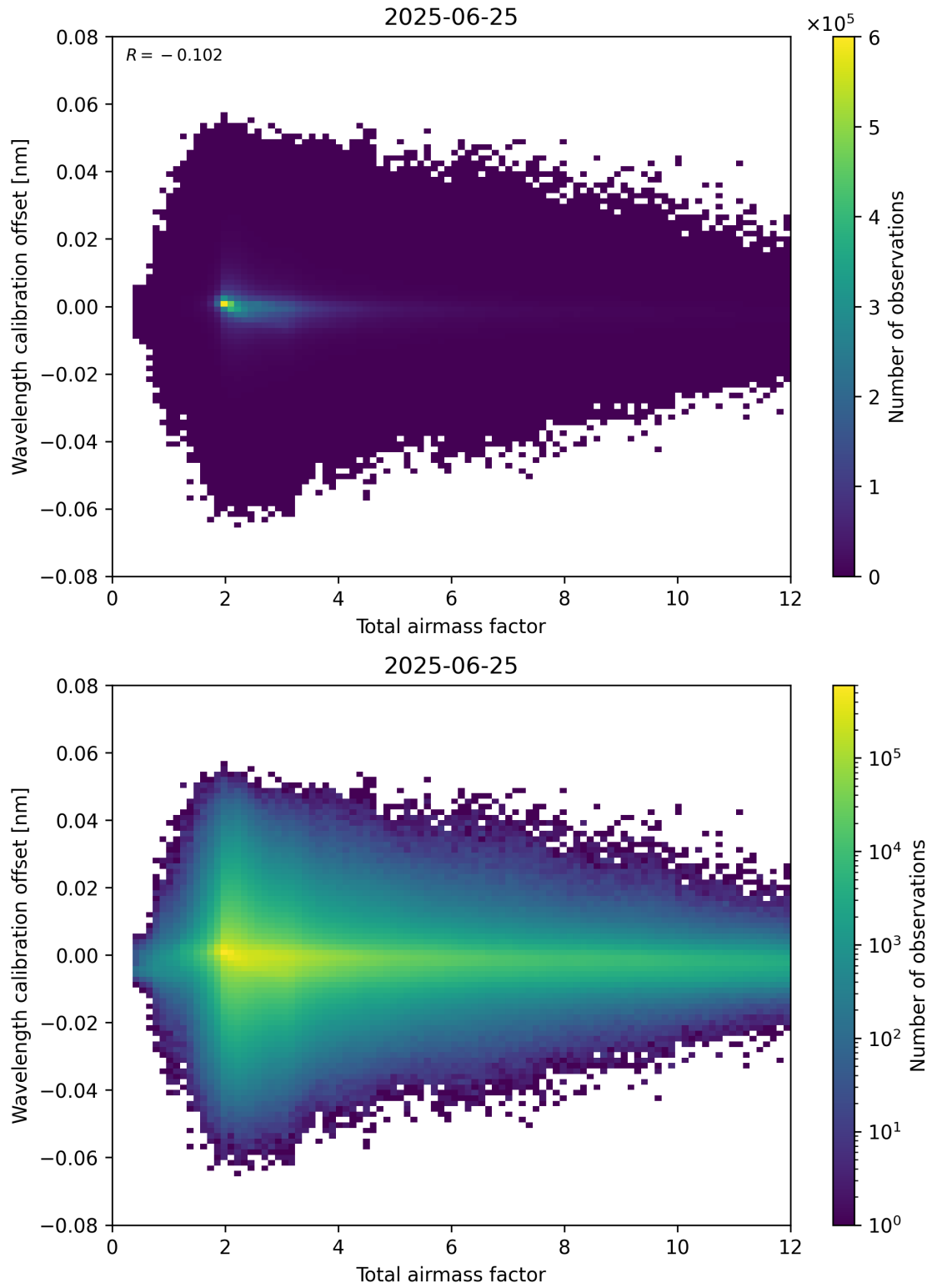
Figure 70: Scatter density plot of “Total airmass factor” against “Wavelength calibration offset” for 2025-06-24 to 2025-06-26.
