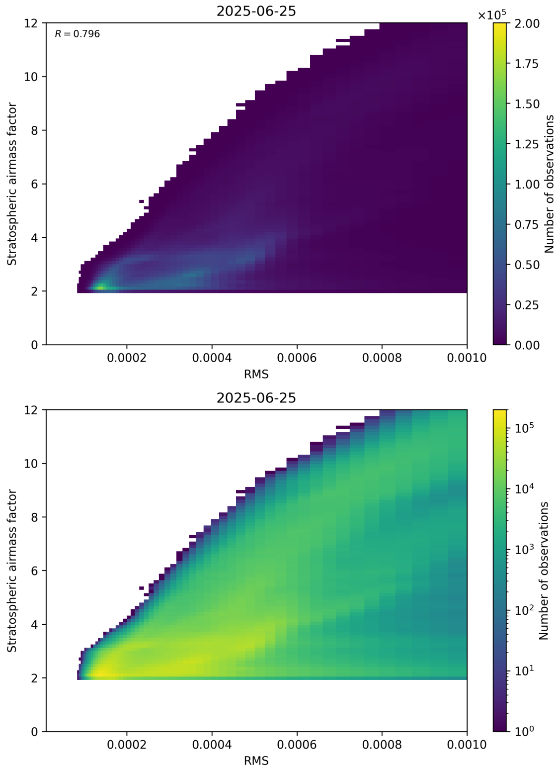
Figure 144: Scatter density plot of “RMS” against “Stratospheric airmass factor” for 2025-06-24 to 2025-06-26.
