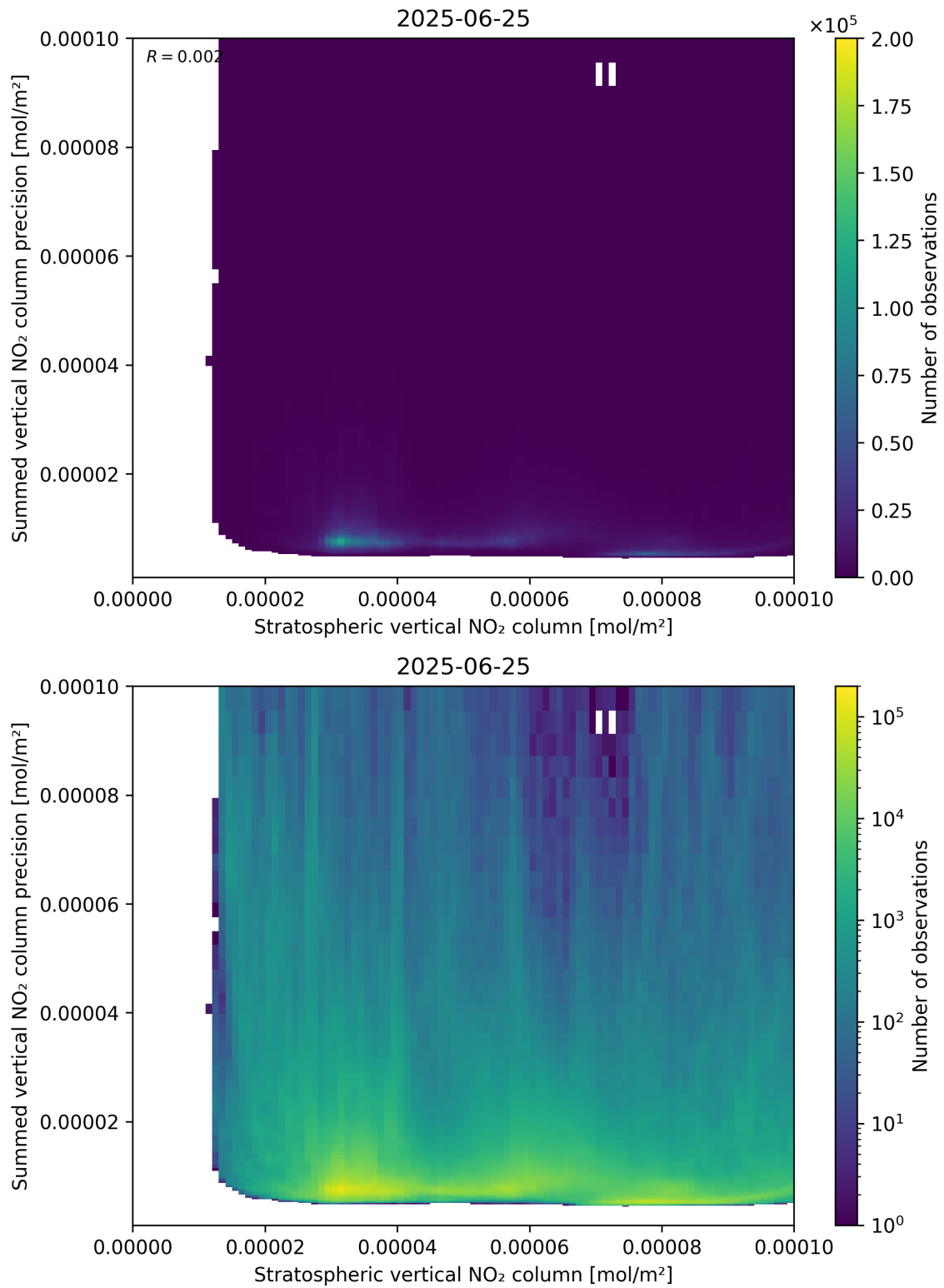
Figure 99: Scatter density plot of “Stratospheric vertical NO 2 column” against “Summed vertical NO 2 column precision” for 2025-06-24 to 2025-06-26.
