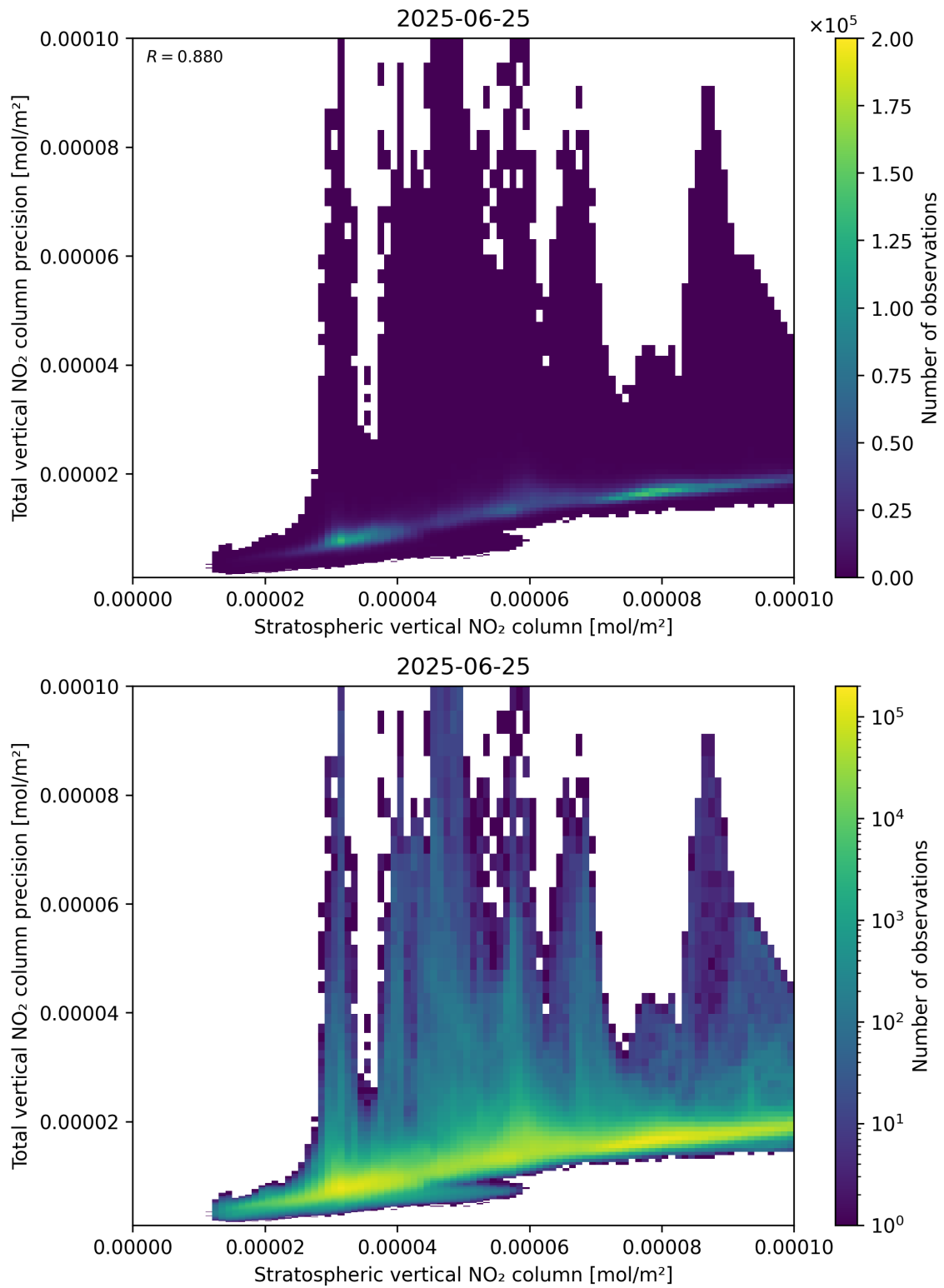
Figure 101: Scatter density plot of “Stratospheric vertical NO 2 column” against “Total vertical NO 2 column precision” for 2025-06-24 to 2025-06-26.
