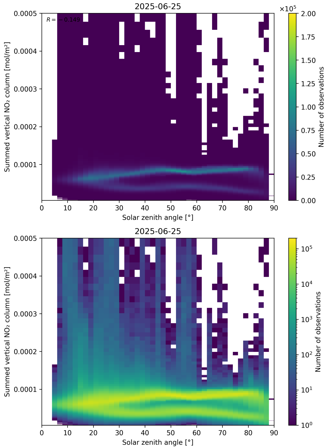
Figure 151: Scatter density plot of “Solar zenith angle” against “Summed vertical NO 2 column” for 2025-06-24 to 2025-06-26.
