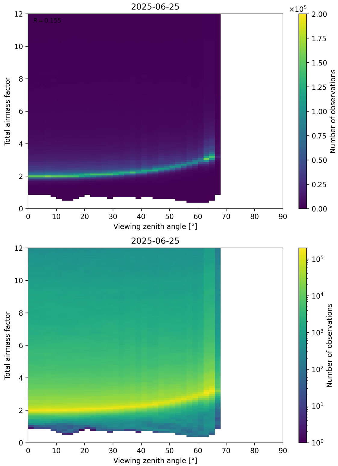
Figure 160: Scatter density plot of “Viewing zenith angle” against “Total airmass factor” for 2025-06-24 to 2025-06-26.
