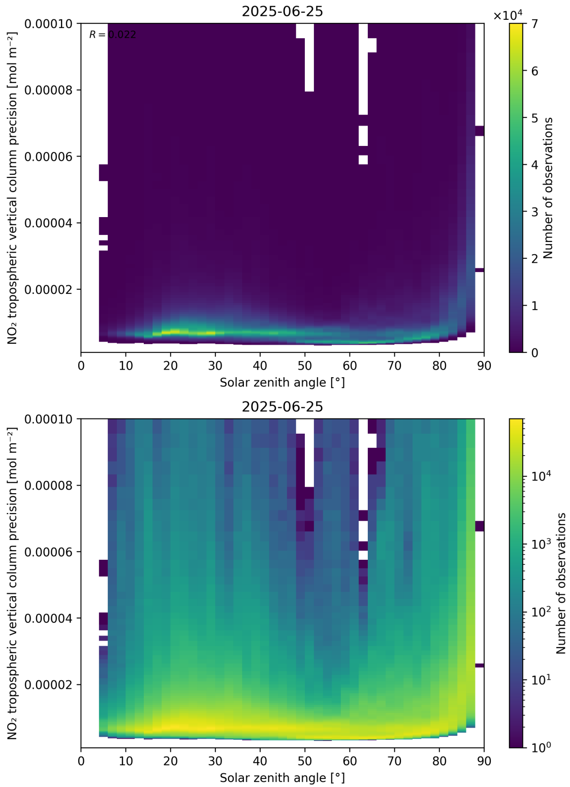
Figure 156: Scatter density plot of “Solar zenith angle” against “NO 2 tropospheric vertical column precision” for 2025-06-24 to 2025-06-26.
