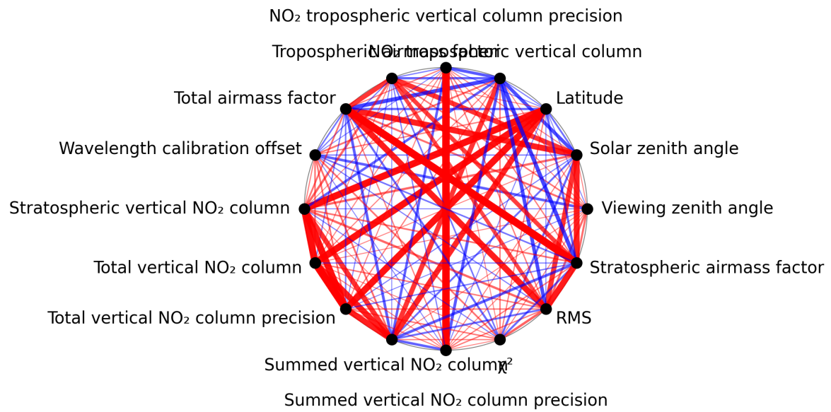
Figure 1: Map of correlation graph for 2025-06-24 to 2025-06-26.
