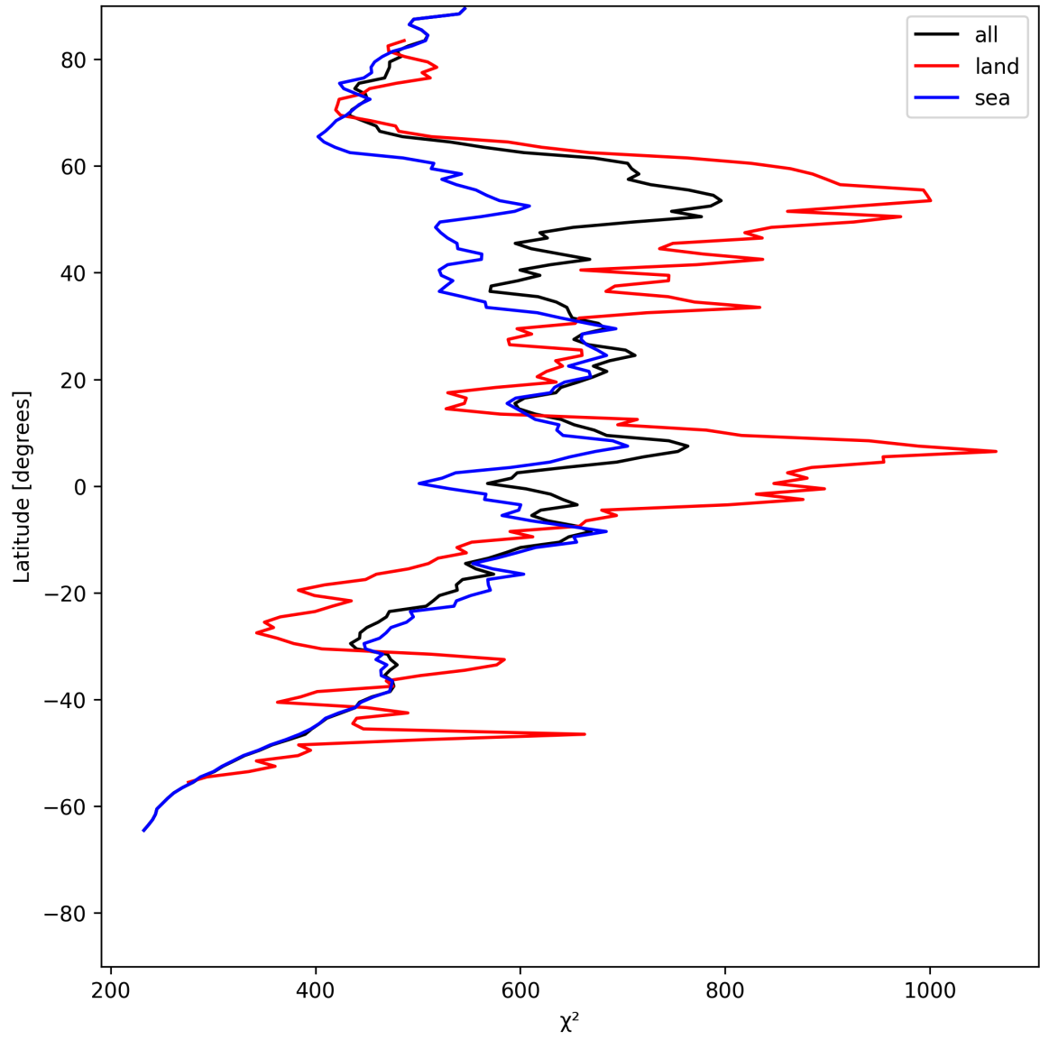
Figure 25: Zonal average of “ \chi^2 ” for 2025-06-24 to 2025-06-26.
