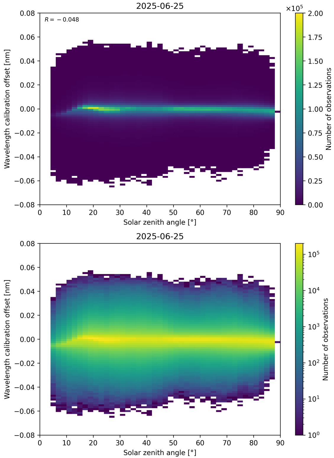
Figure 158: Scatter density plot of “Solar zenith angle” against “Wavelength calibration offset” for 2025-06-24 to 2025-06-26.
