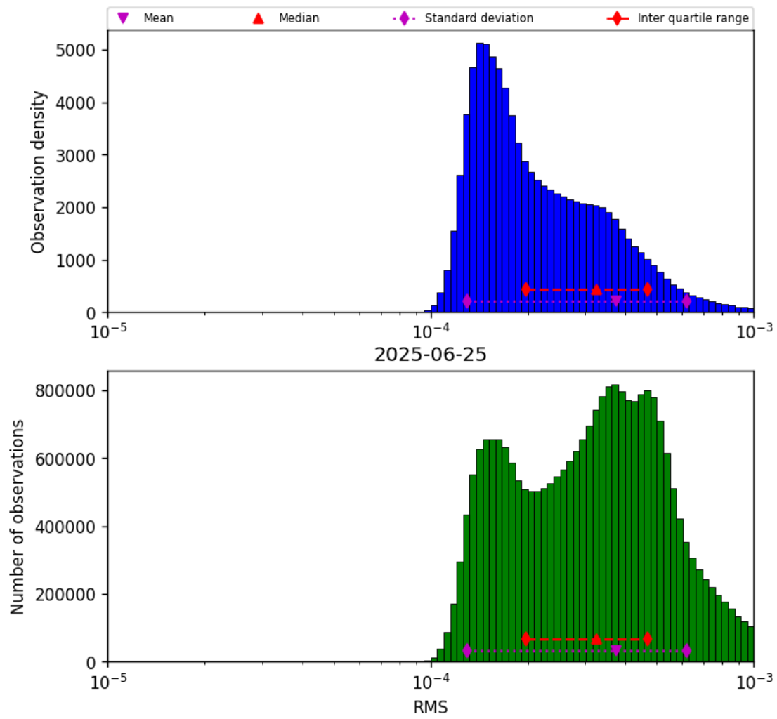
Figure 43: Histogram of “RMS” for 2025-06-24 to 2025-06-26
