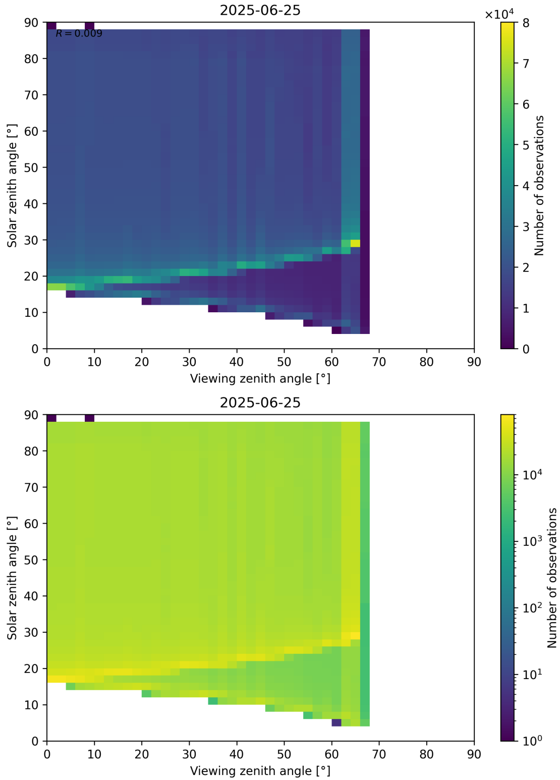
Figure 172: Scatter density plot of “Viewing zenith angle” against “Solar zenith angle” for 2025-06-24 to 2025-06-26.
