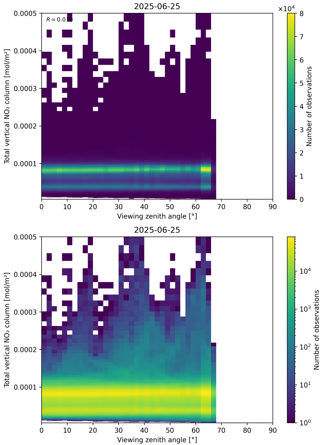
Figure 167: Scatter density plot of “Viewing zenith angle” against “Total vertical NO 2 column” for 2025-06-24 to 2025-06-26.
