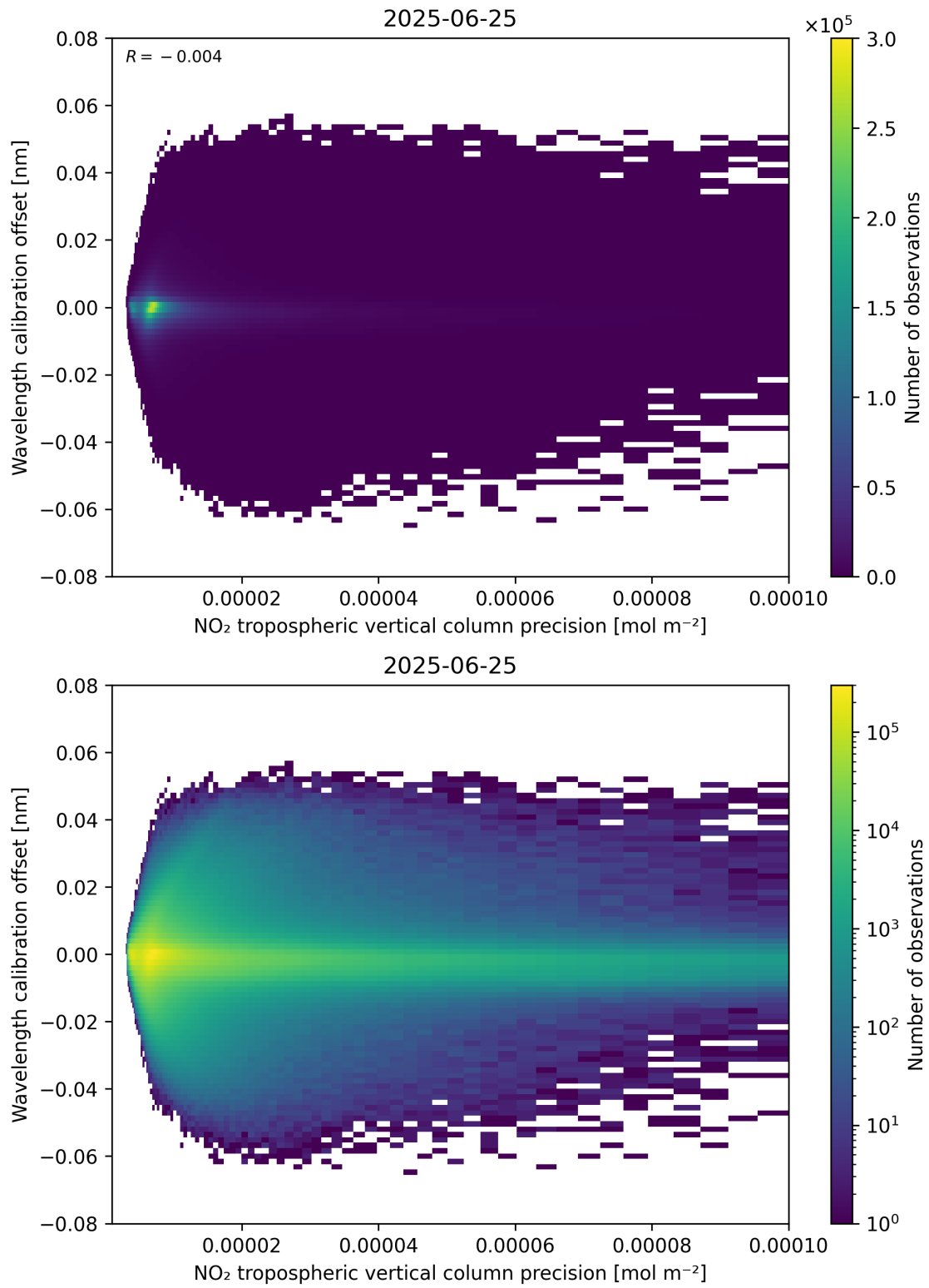
Figure 141: Scatter density plot of “NO 2 tropospheric vertical column precision” against “Wavelength calibration offset” for 2025-06-24 to 2025-06-26.
