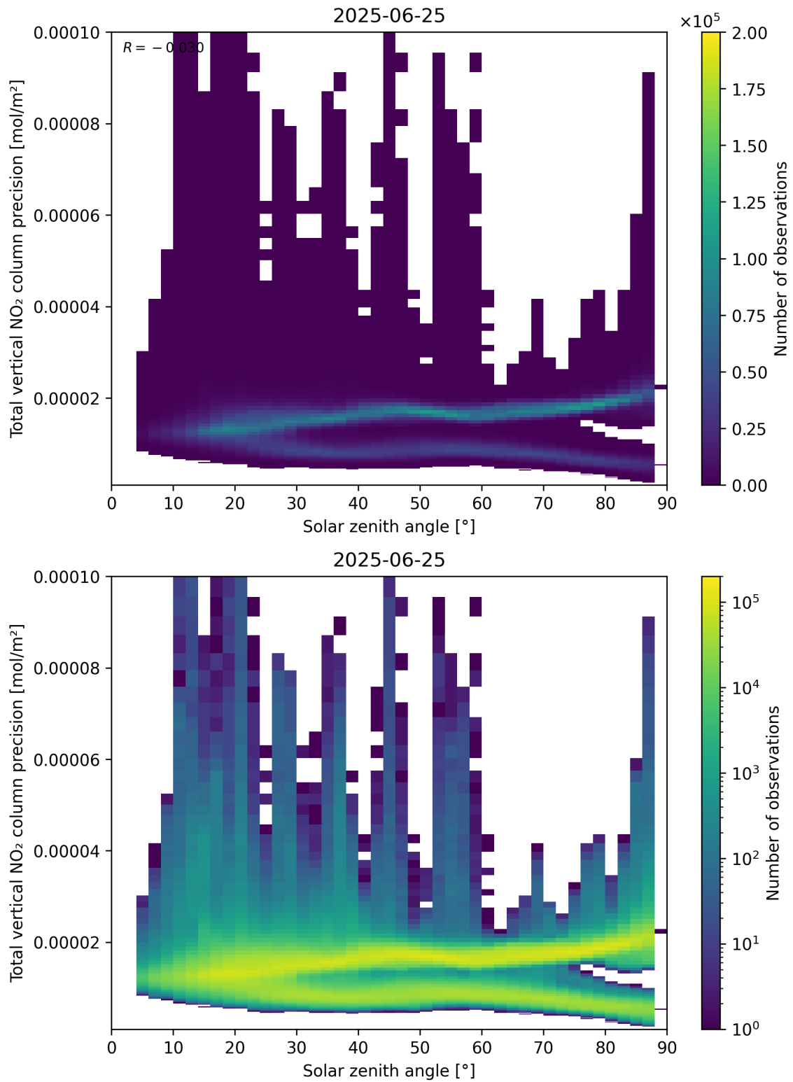
Figure 154: Scatter density plot of “Solar zenith angle” against “Total vertical NO 2 column precision” for 2025-06-24 to 2025-06-26.
