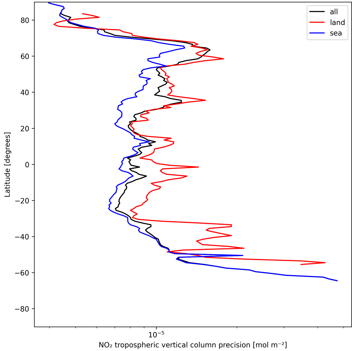
Figure 13: Zonal average of “NO 2 tropospheric vertical column precision” for 2025-06-24 to 2025-06-26.
