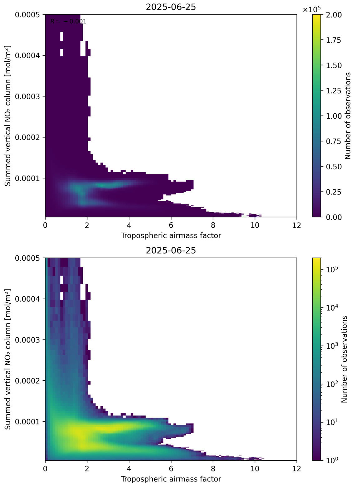
Figure 75: Scatter density plot of “Tropospheric air mass factor” against “Summed vertical NO 2 column” for 2025-06-24 to 2025-06-26.
