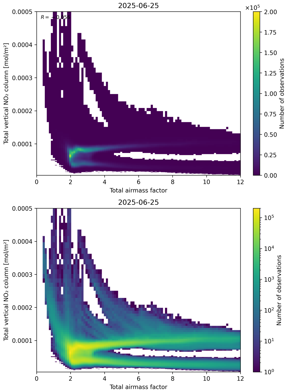
Figure 67: Scatter density plot of “Total airmass factor” against “Total vertical NO 2 column” for 2025-06-24 to 2025-06-26.
