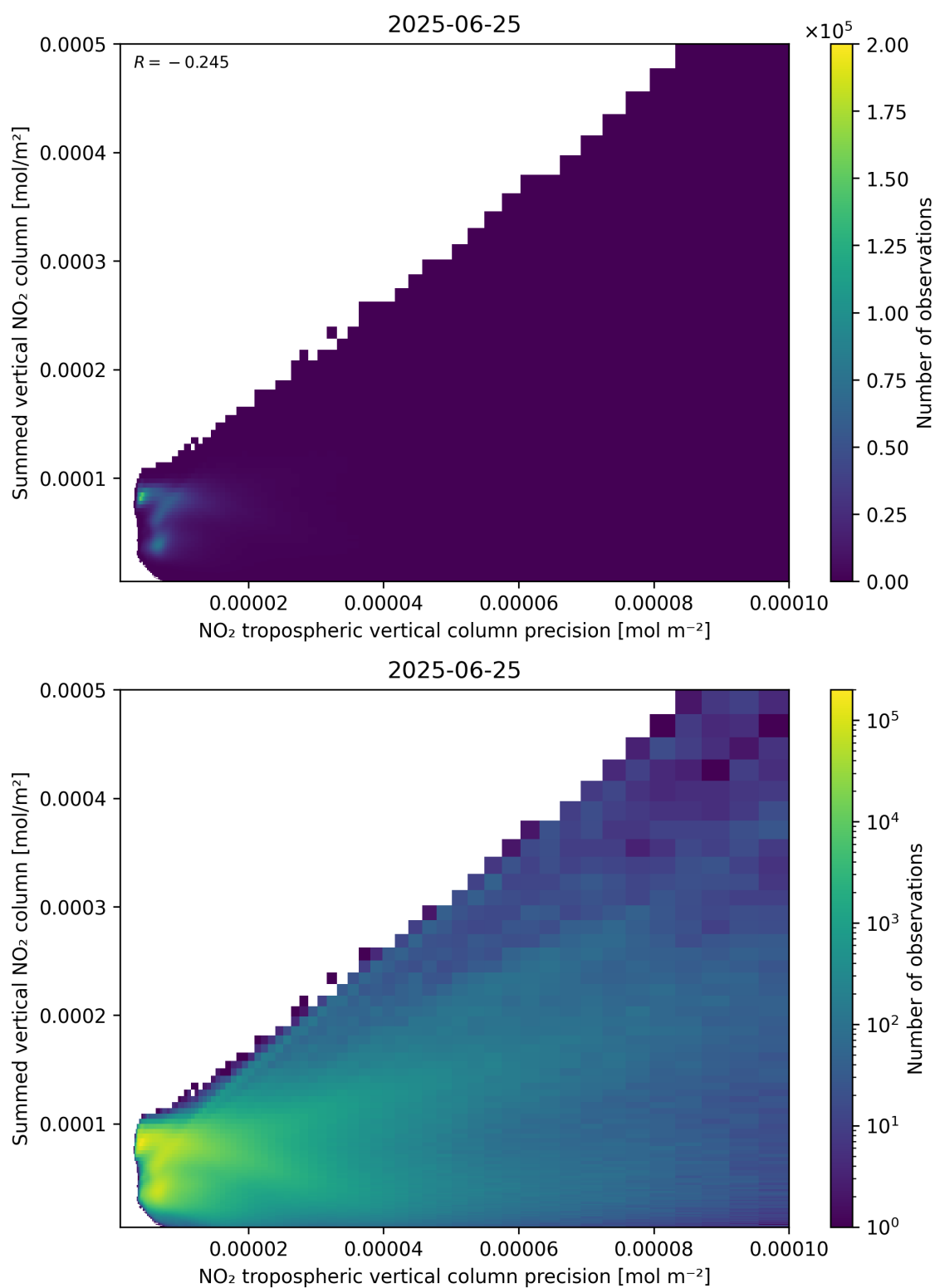
Figure 136: Scatter density plot of “NO 2 tropospheric vertical column precision” against “Summed vertical NO 2 column” for 2025-06-24 to 2025-06-26.
