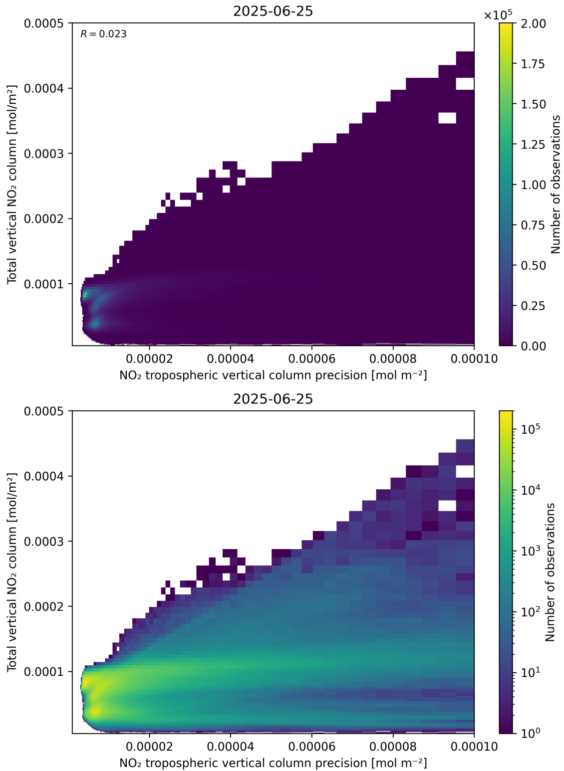
Figure 138: Scatter density plot of “NO 2 tropospheric vertical column precision” against “Total vertical NO 2 column” for 2025-06-24 to 2025-06-26.
