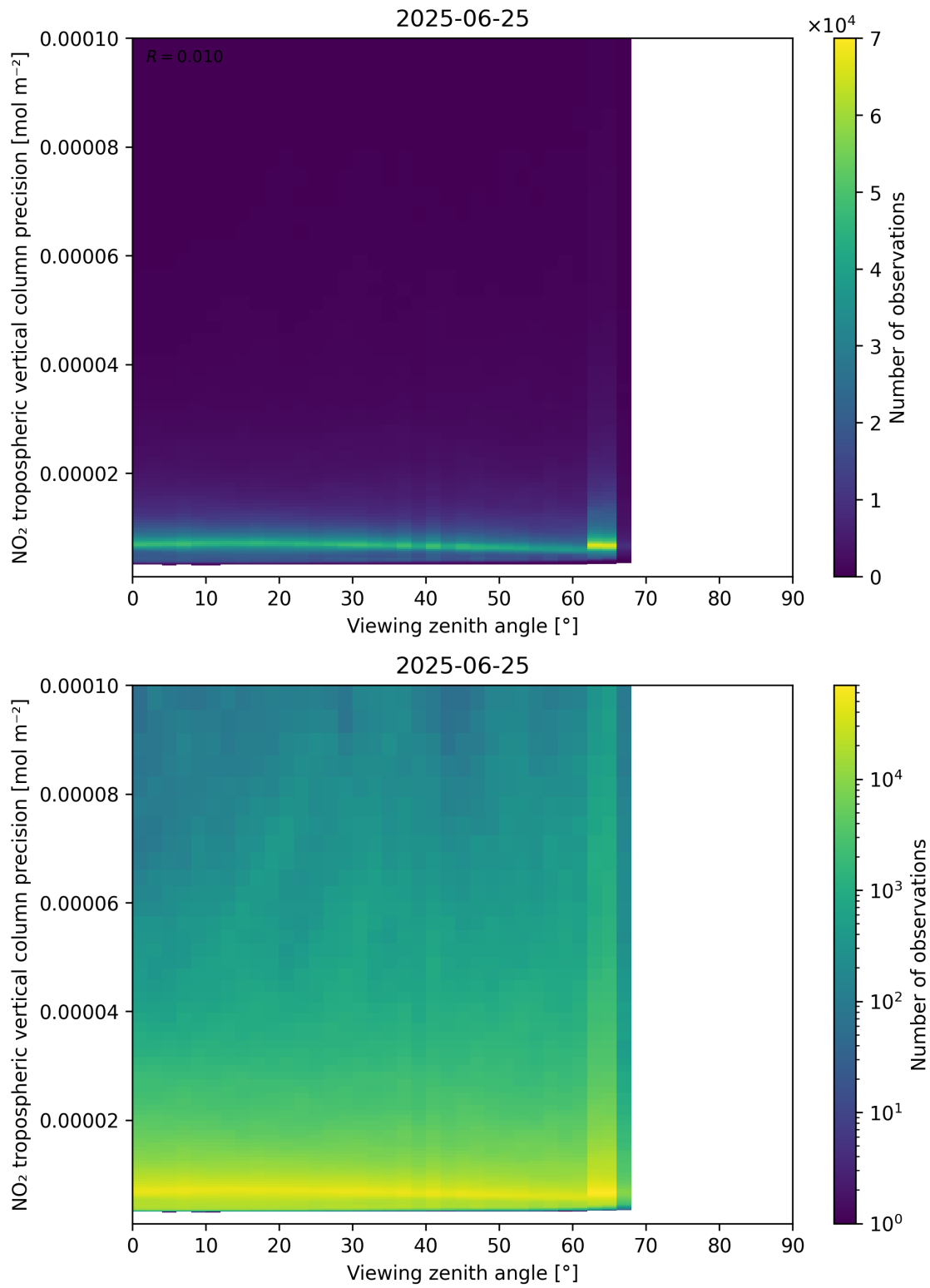
Figure 170: Scatter density plot of “Viewing zenith angle” against “NO 2 tropospheric vertical column precision” for 2025-06-24 to 2025-06-26.
