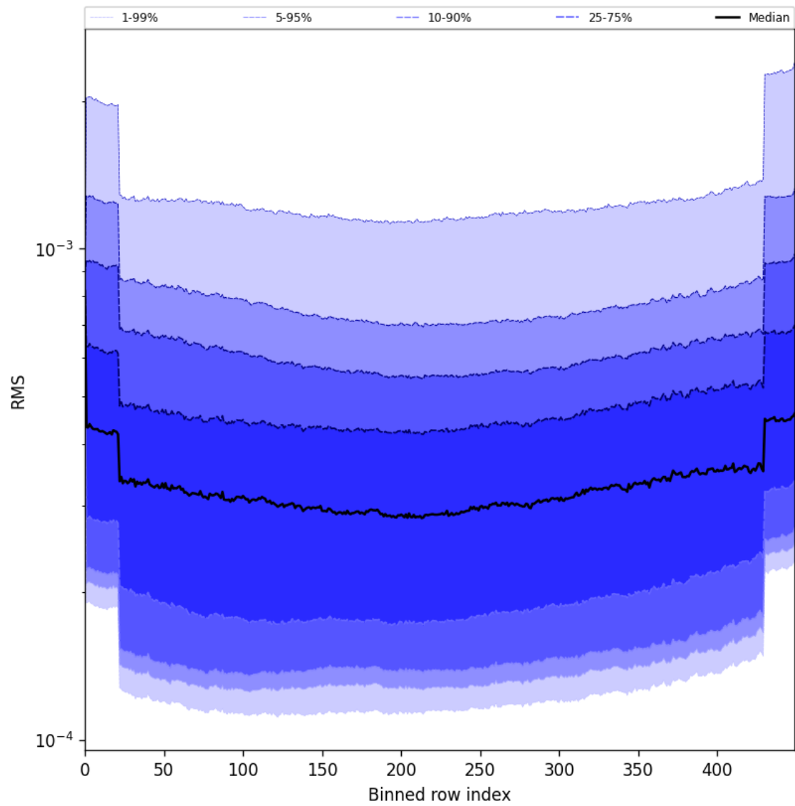
Figure 60: Along track statistics of “RMS” for 2025-06-24 to 2025-06-26
