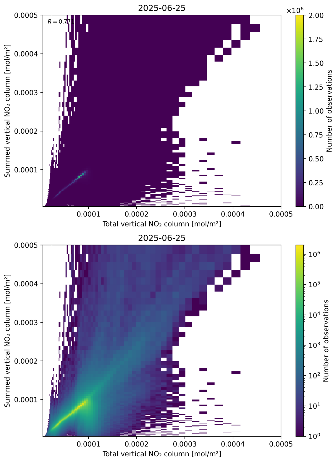
Figure 112: Scatter density plot of “Total vertical NO 2 column” against “Summed vertical NO 2 column” for 2025-06-24 to 2025-06-26.
