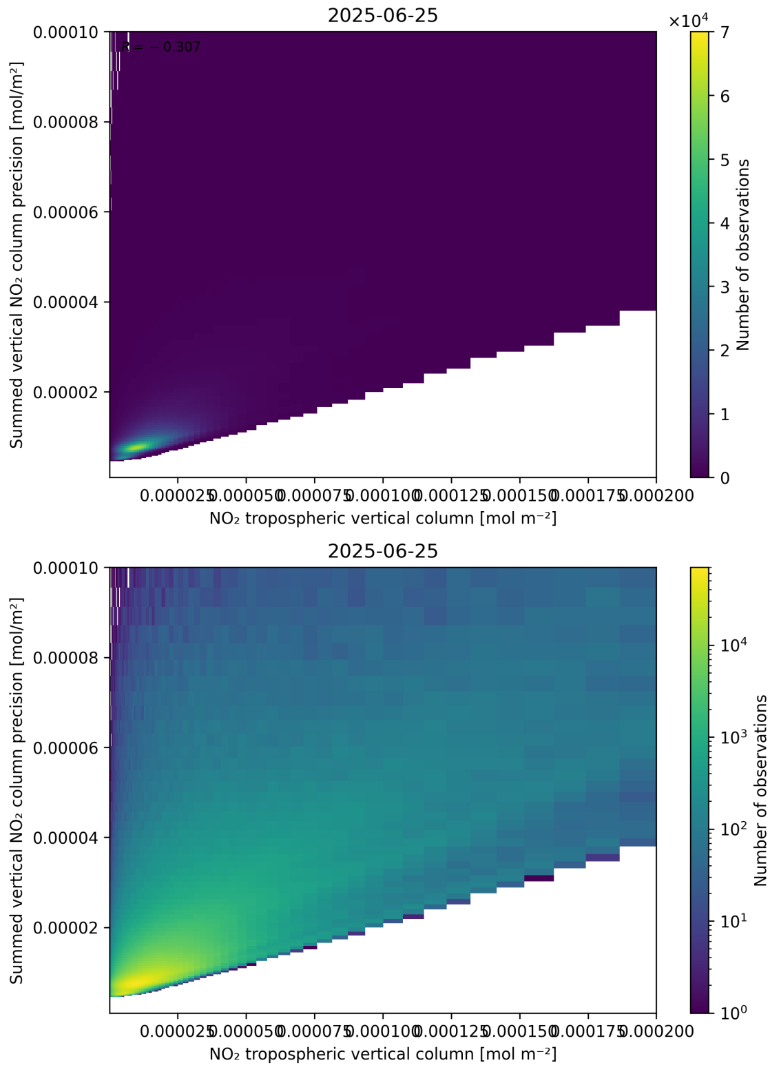
Figure 127: Scatter density plot of “NO 2 tropospheric vertical column” against “Summed vertical NO 2 column precision” for 2025-06-24 to 2025-06-26.
