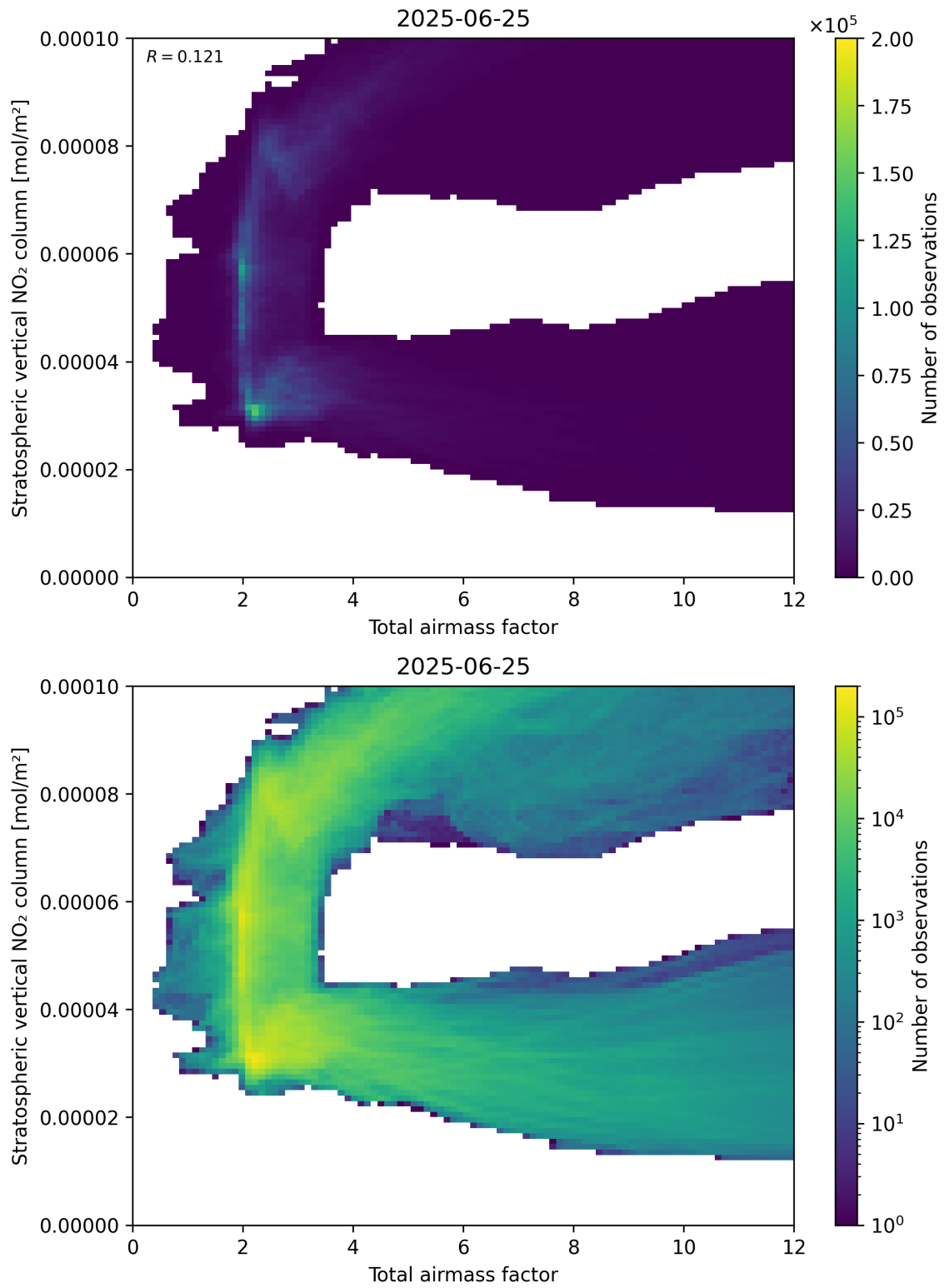
Figure 64: Scatter density plot of “Total airmass factor” against “Stratospheric vertical \text{NO}_2 column” for 2025-06-24 to 2025-06-26.
