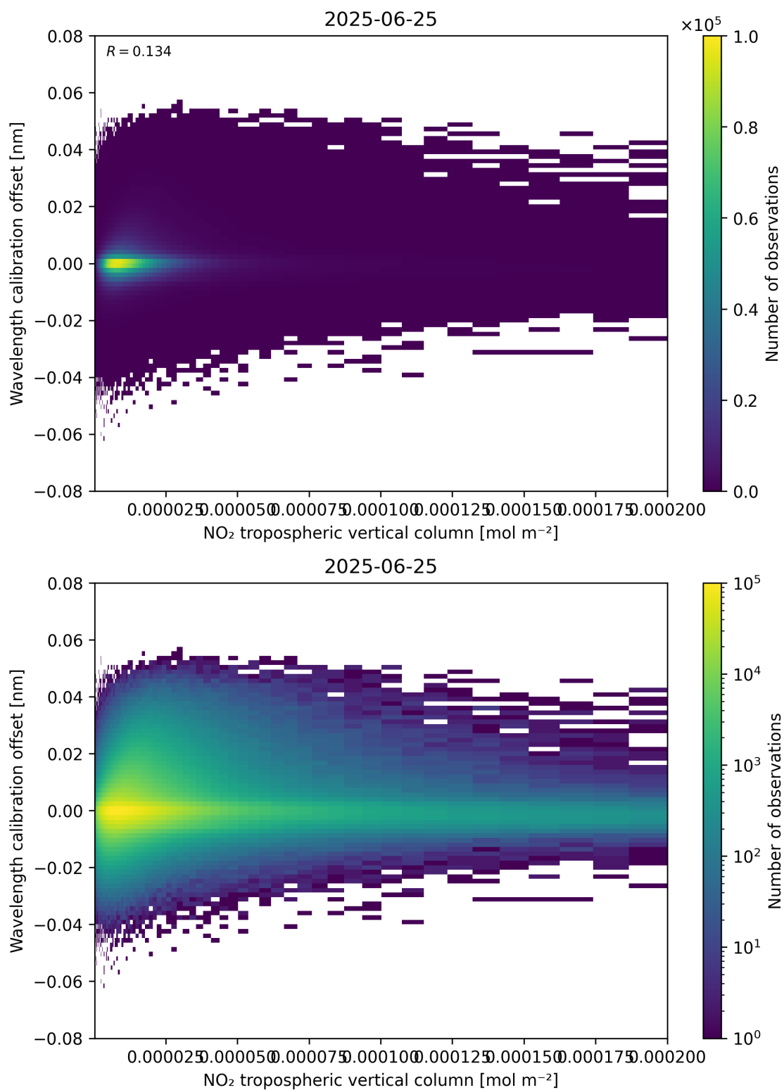
Figure 143: Scatter density plot of “NO 2 tropospheric vertical column” against “Wavelength calibration offset” for 2025-06-24 to 2025-06-26.
