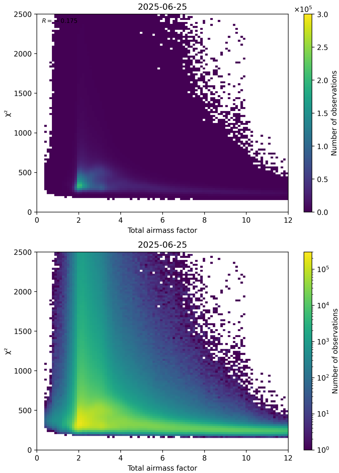
Figure 63: Scatter density plot of “Total airmass factor” against “ \chi^2 ” for 2025-06-24 to 2025-06-26.
