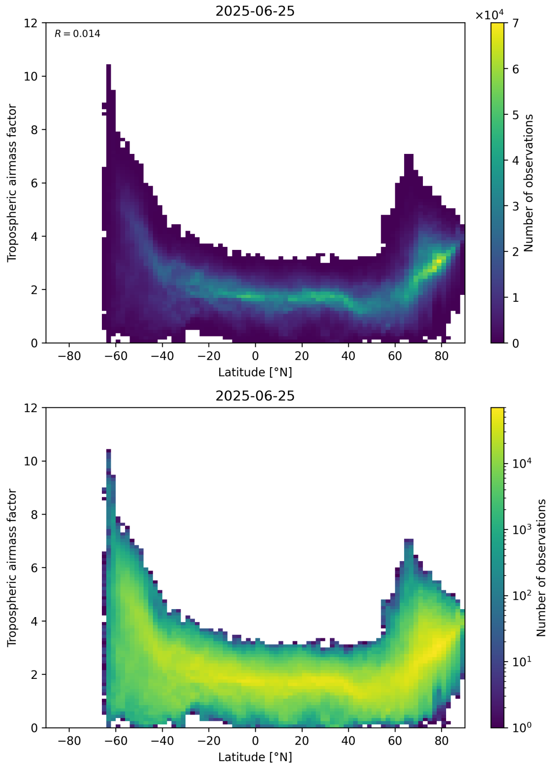
Figure 85: Scatter density plot of “Latitude” against “Tropospheric air mass factor” for 2025-06-24 to 2025-06-26.
