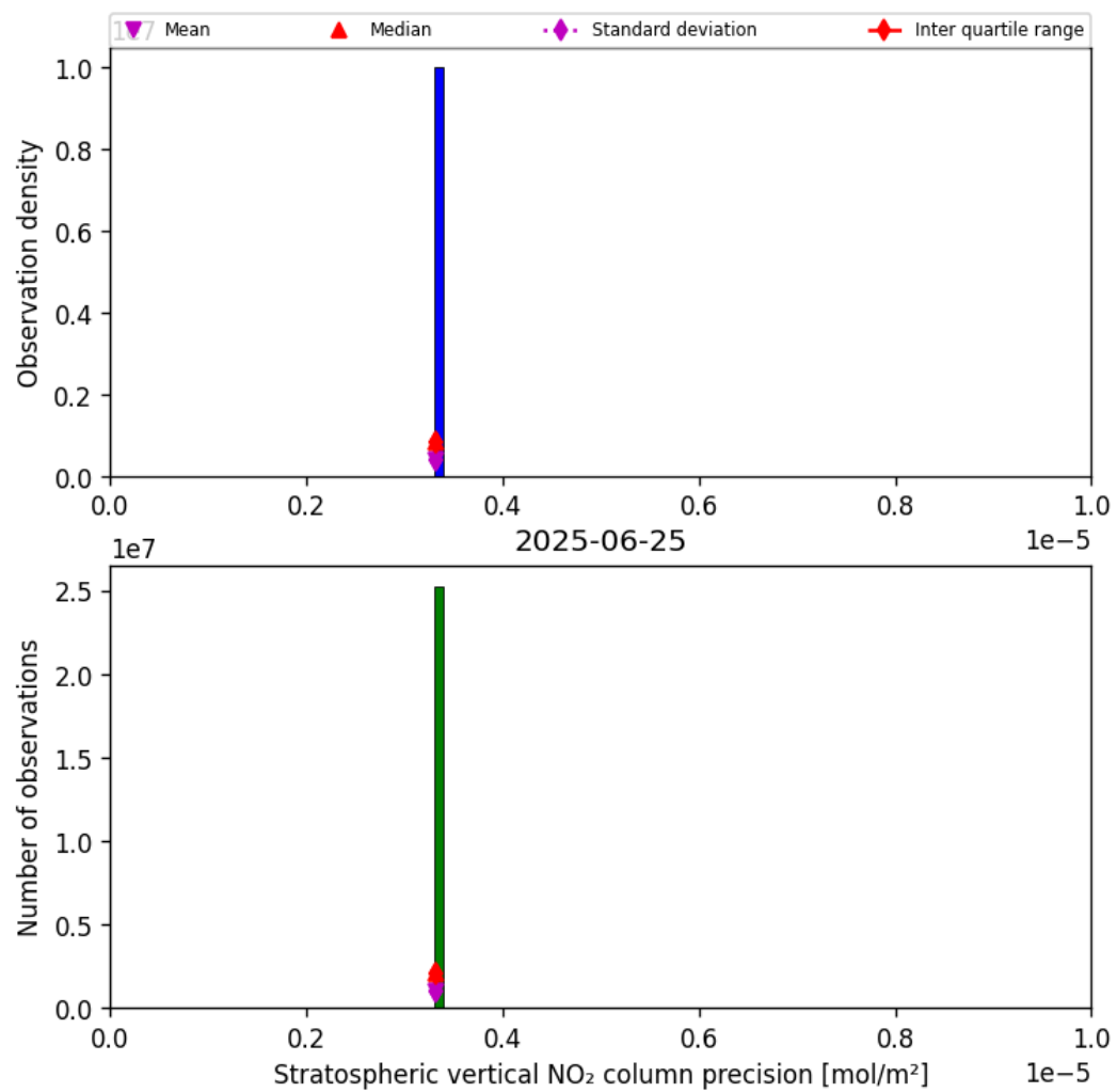
Figure 37: Histogram of “Stratospheric vertical NO 2 column precision” for 2025-06-24 to 2025-06-26
