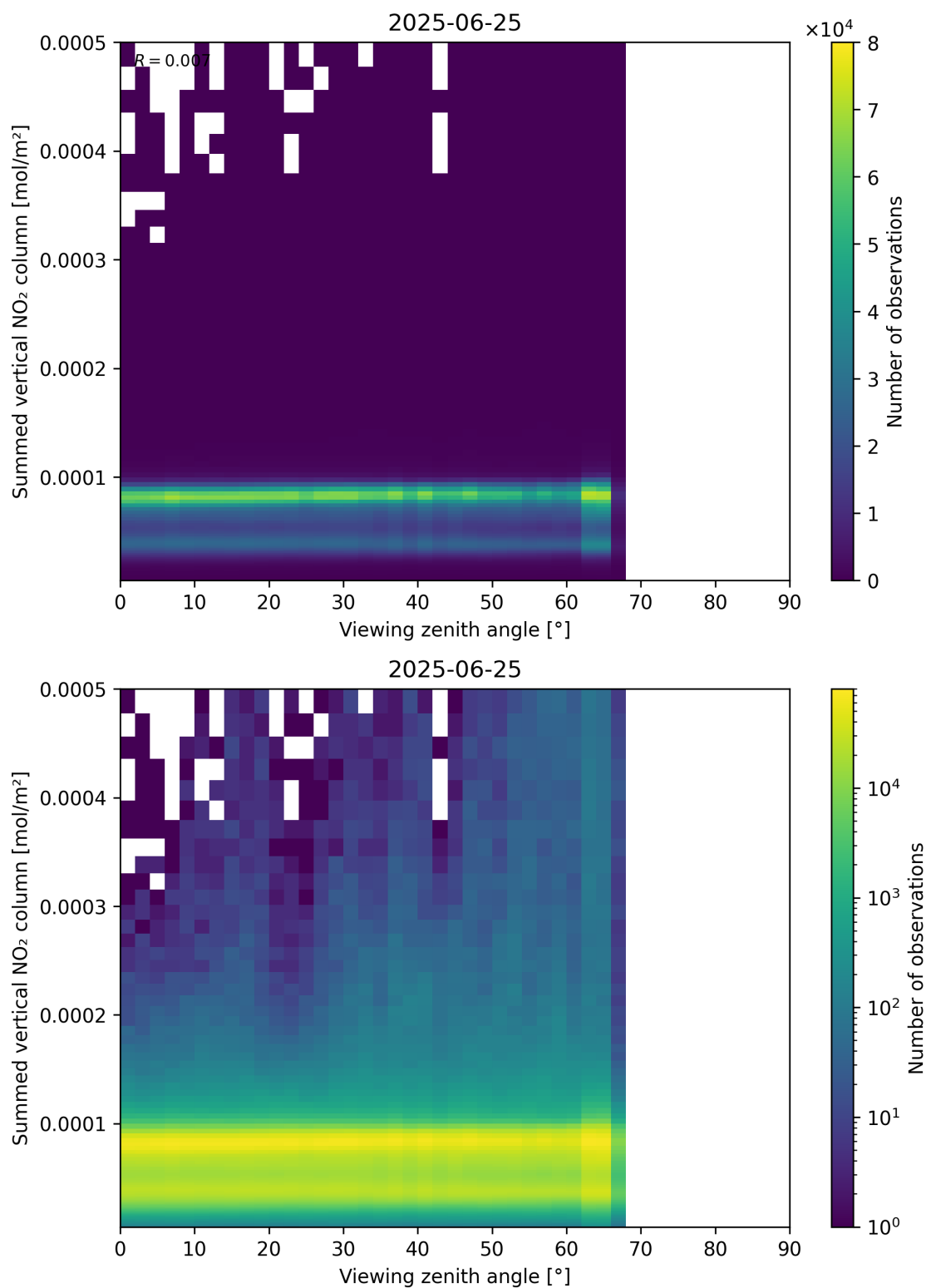
Figure 165: Scatter density plot of “Viewing zenith angle” against “Summed vertical NO 2 column” for 2025-06-24 to 2025-06-26.
