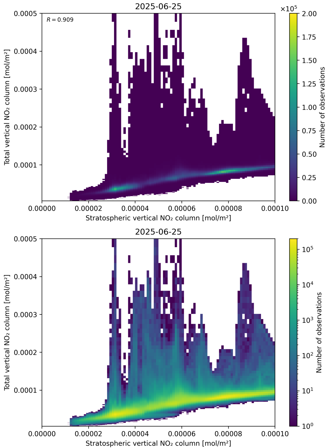
Figure 100: Scatter density plot of “Stratospheric vertical NO 2 column” against “Total vertical NO 2 column” for 2025-06-24 to 2025-06-26.
