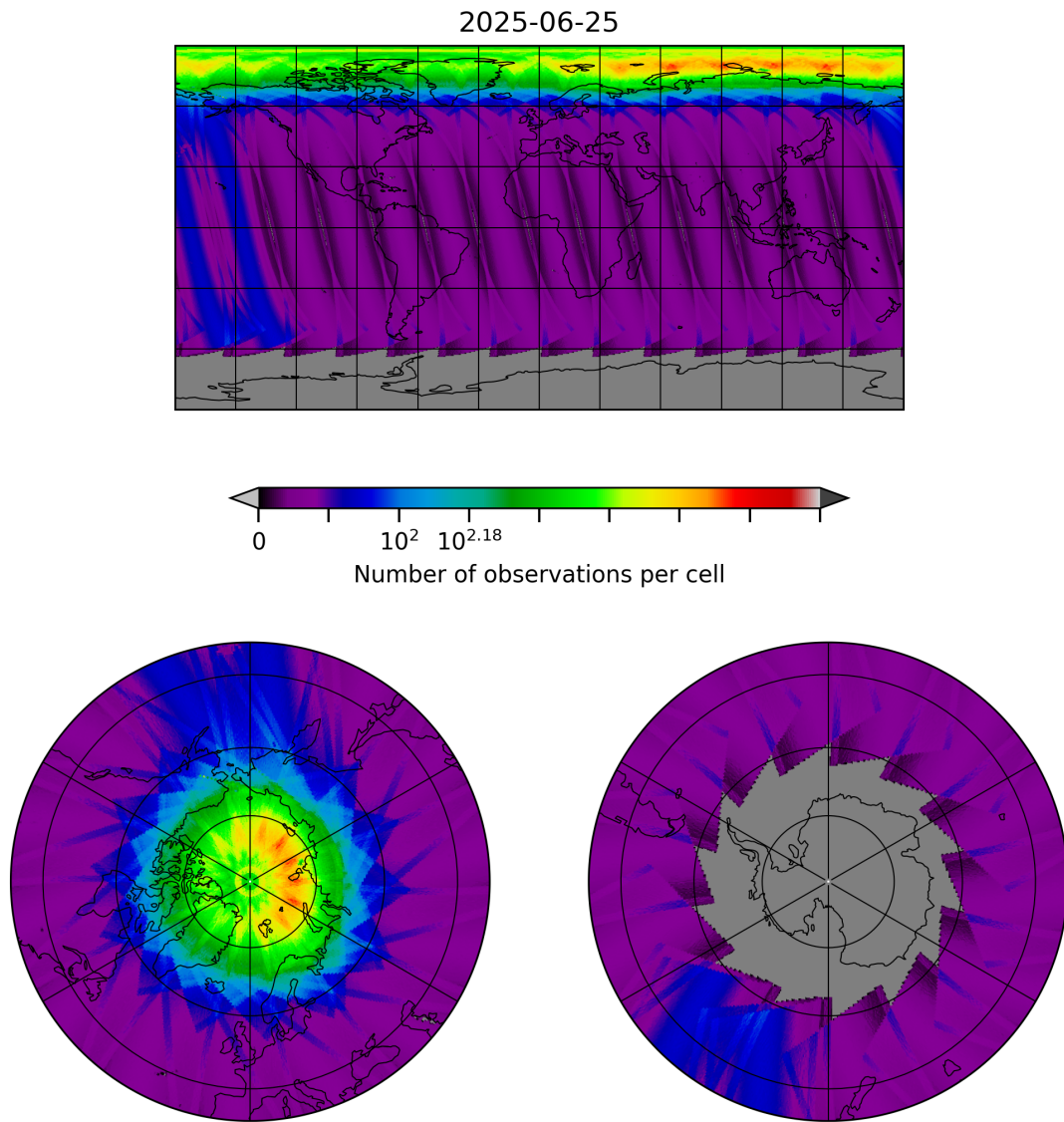
Figure 10: Map of the number of observations for 2025-06-24 to 2025-06-26
