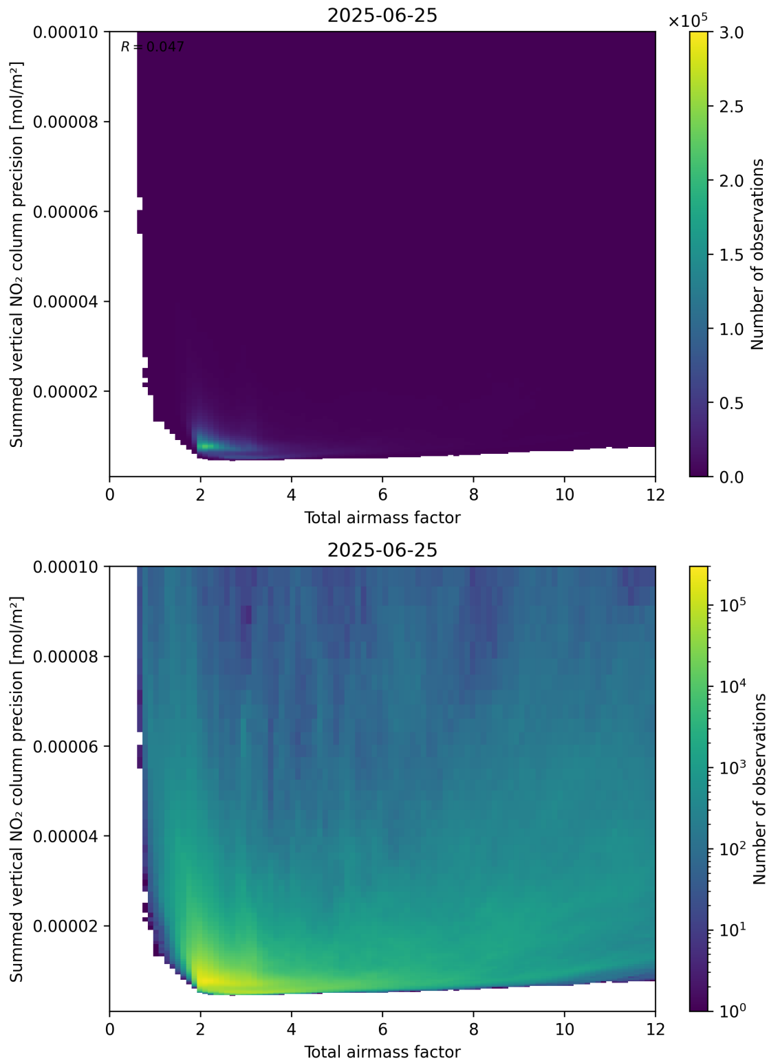
Figure 66: Scatter density plot of “Total airmass factor” against “Summed vertical NO 2 column precision” for 2025-06-24 to 2025-06-26.
