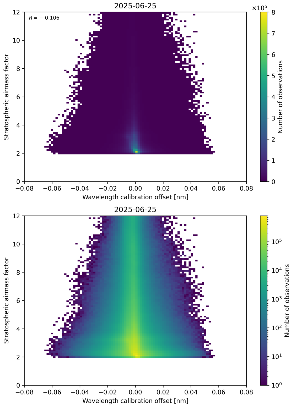
Figure 174: Scatter density plot of “Wavelength calibration offset” against “Stratospheric air mass factor” for 2025-06-24 to 2025-06-26.
