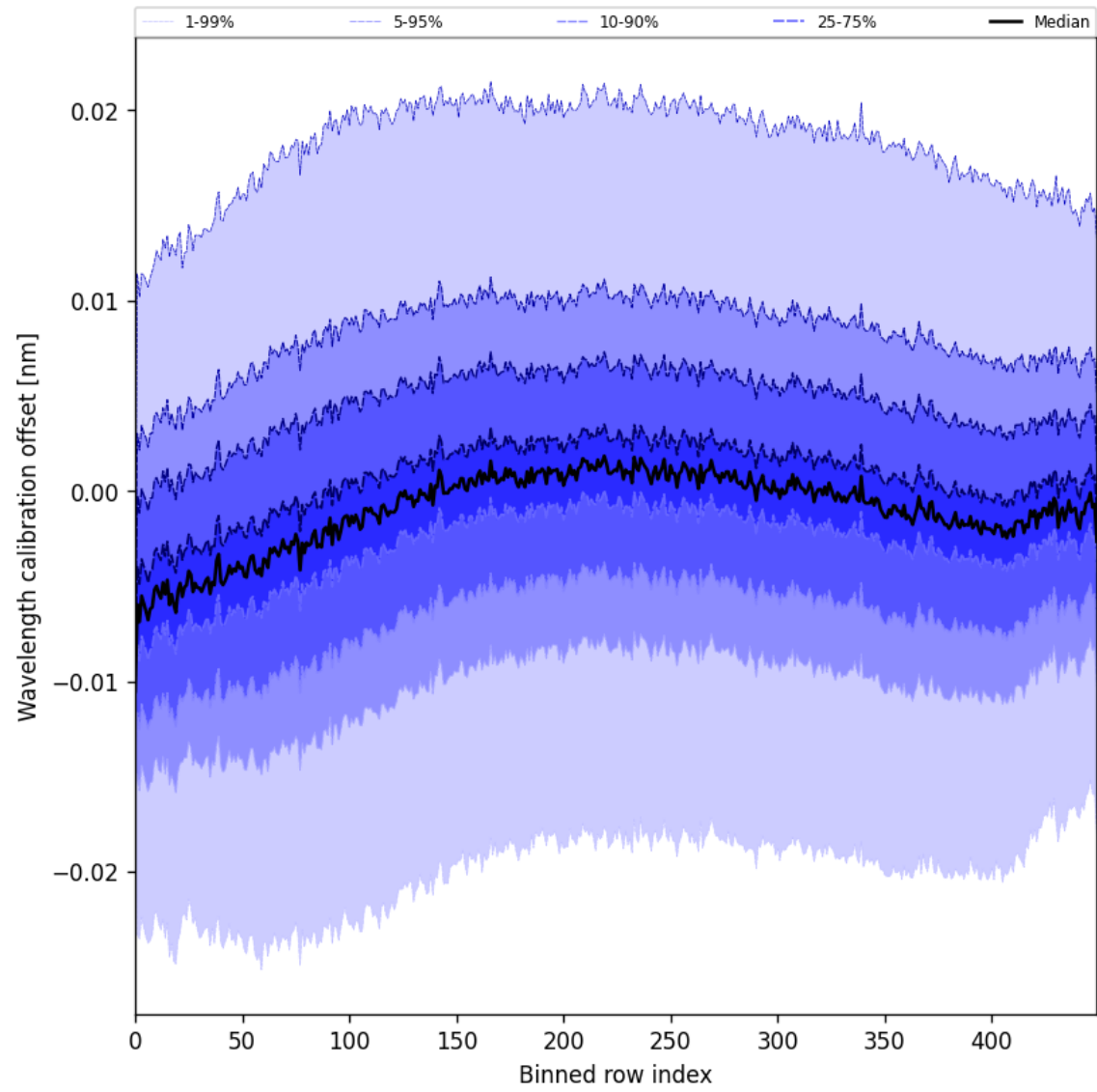
Figure 52: Along track statistics of “Wavelength calibration offset” for 2025-06-24 to 2025-06-26
