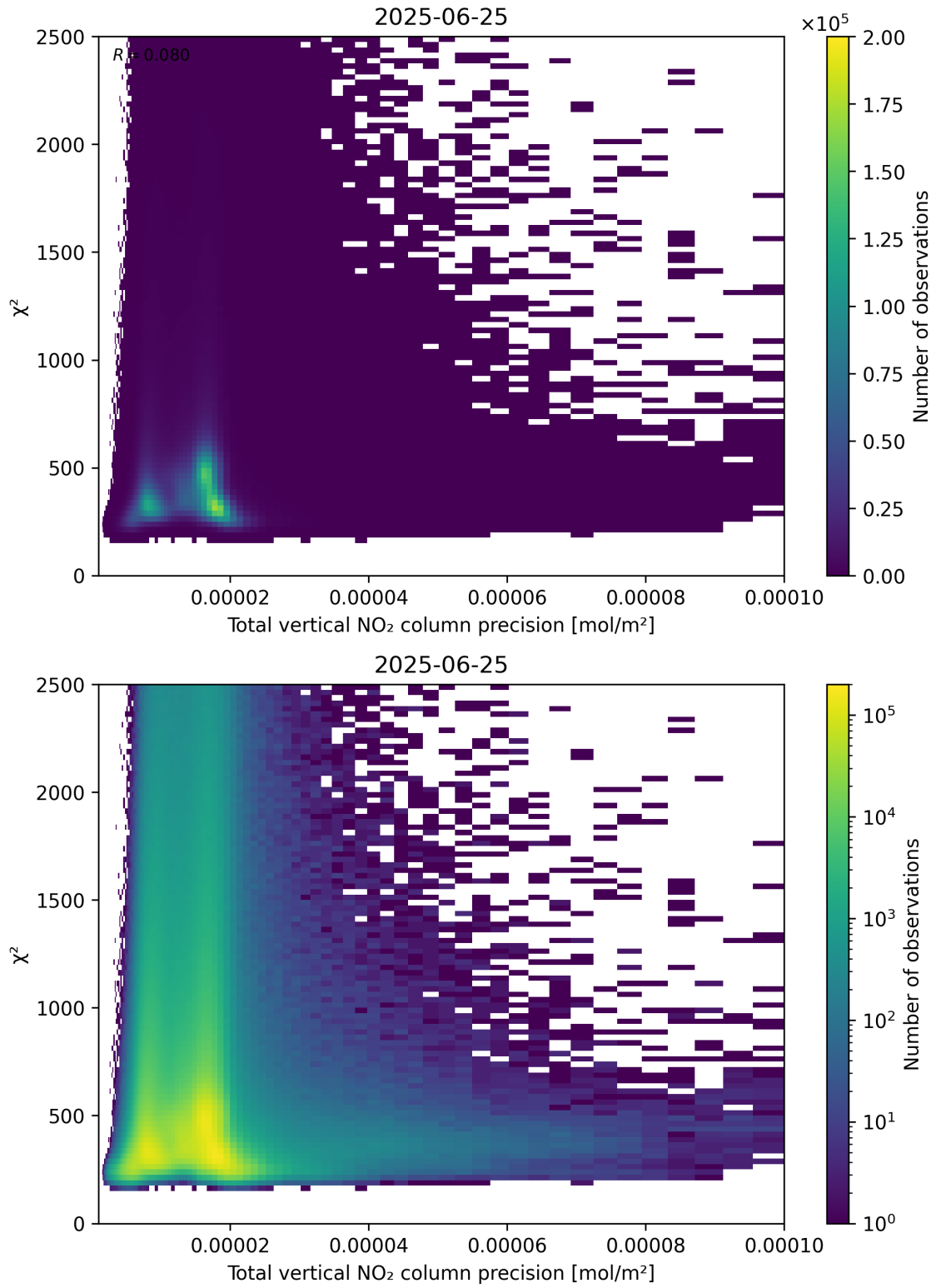
Figure 116: Scatter density plot of “Total vertical NO 2 column precision” against “ \chi^2 ” for 2025-06-24 to 2025-06-26.
