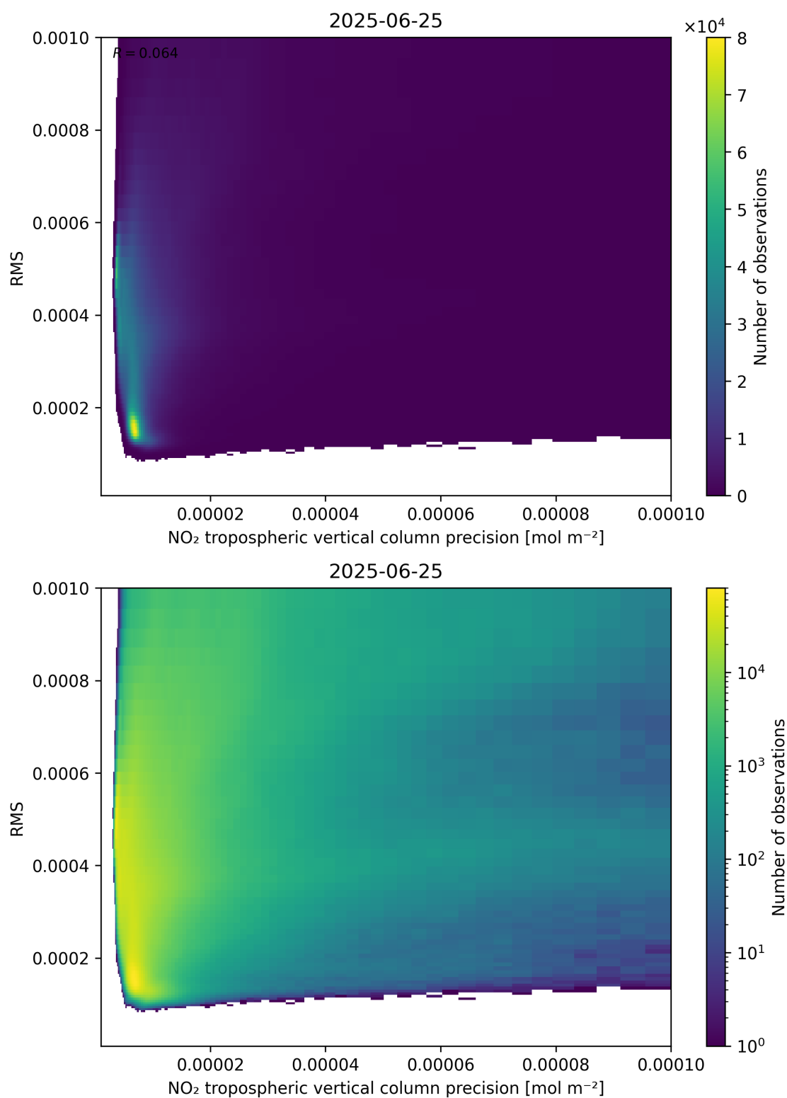
Figure 140: Scatter density plot of “NO 2 tropospheric vertical column precision” against “RMS” for 2025-06-24 to 2025-06-26.
