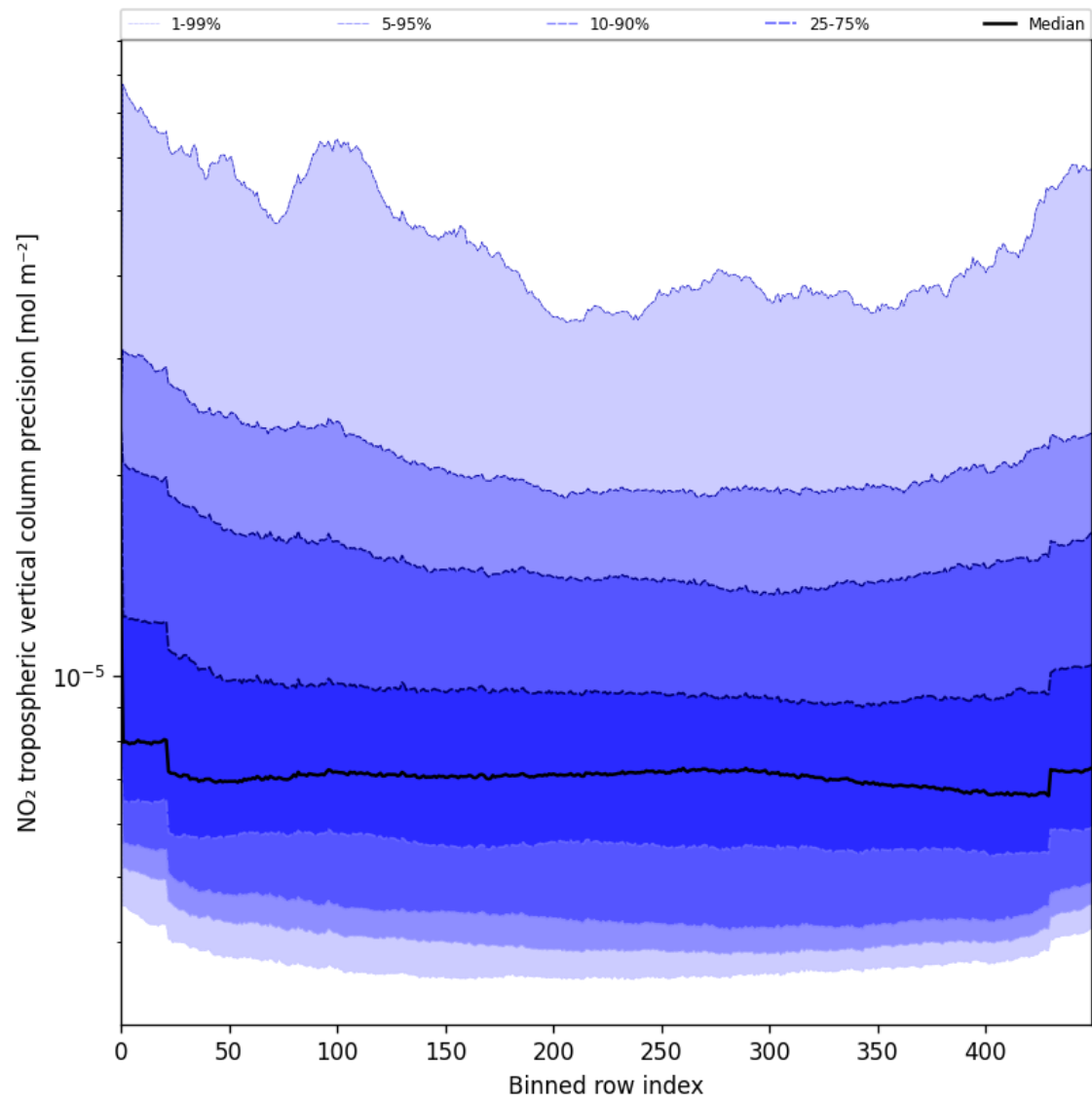
Figure 47: Along track statistics of “NO 2 tropospheric vertical column precision” for 2025-06-24 to 2025-06-26
