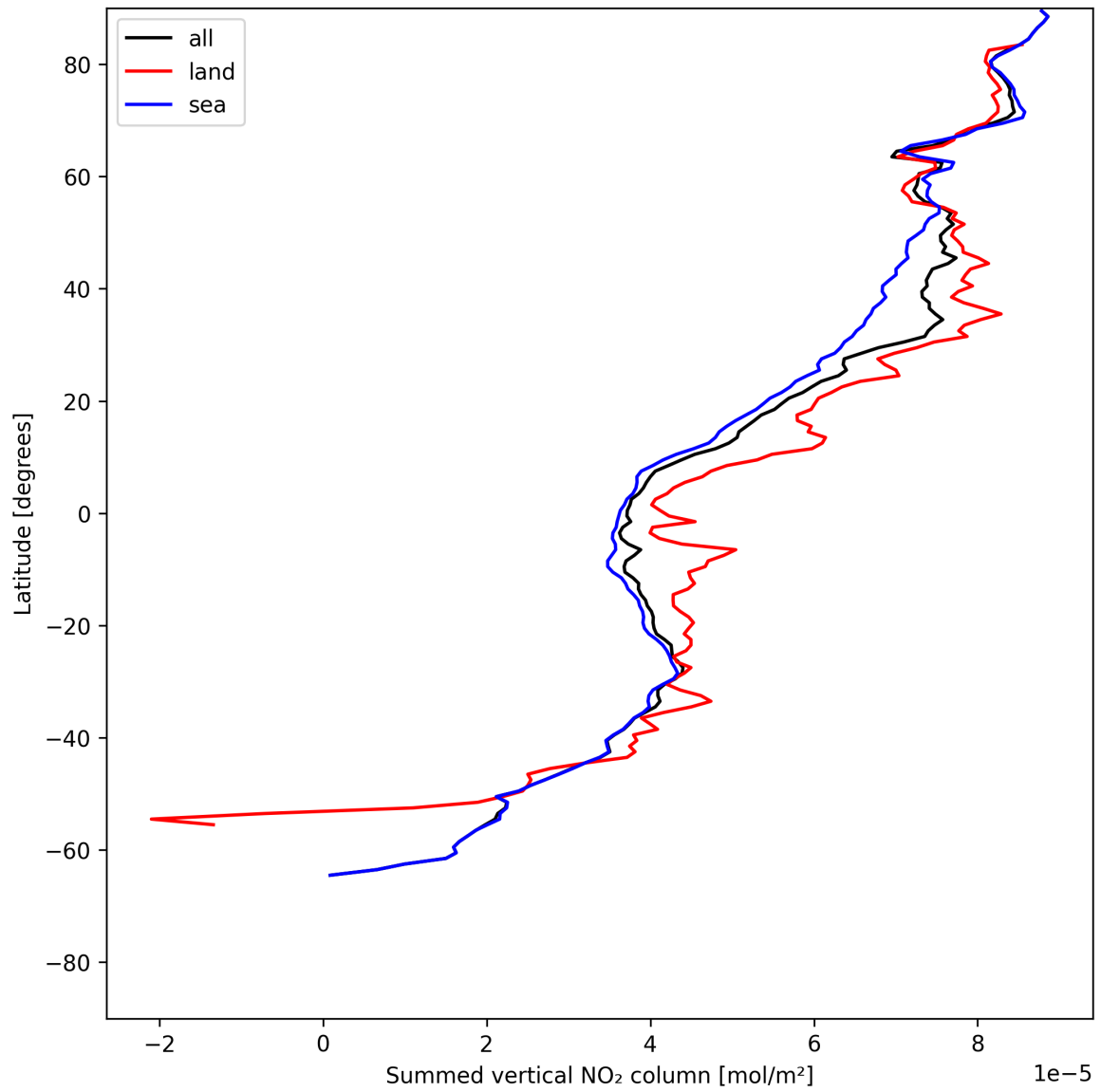
Figure 23: Zonal average of “Summed vertical NO 2 column” for 2025-06-24 to 2025-06-26.
