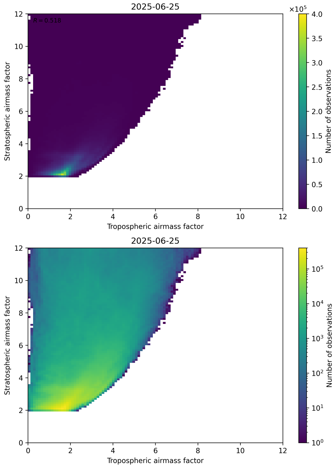
Figure 71: Scatter density plot of “Tropospheric airmass factor” against “Stratospheric airmass factor” for 2025-06-24 to 2025-06-26.
