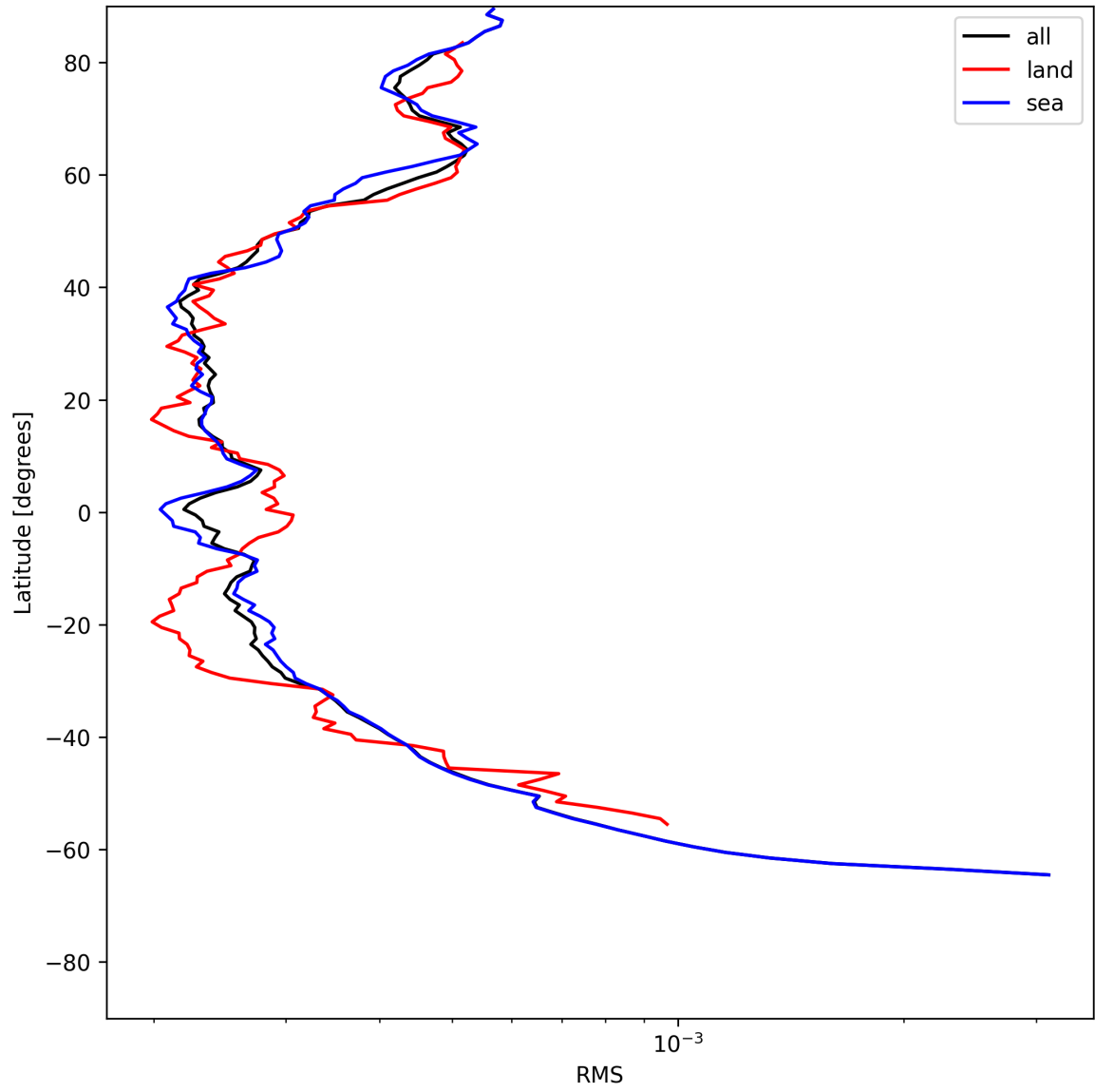
Figure 26: Zonal average of “RMS” for 2025-06-24 to 2025-06-26.
