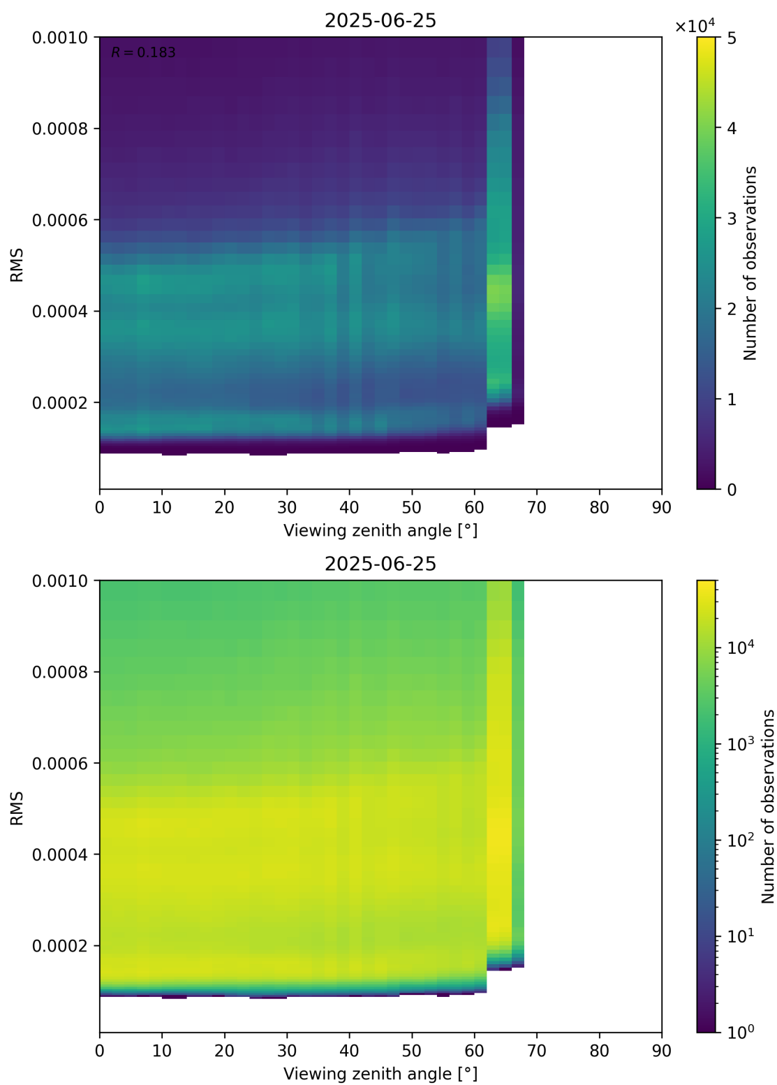
Figure 171: Scatter density plot of “Viewing zenith angle” against “RMS” for 2025-06-24 to 2025-06-26.
