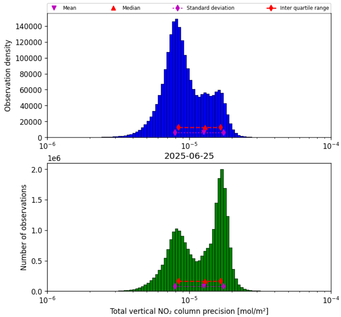
Figure 39: Histogram of “Total vertical NO 2 column precision” for 2025-06-24 to 2025-06-26
