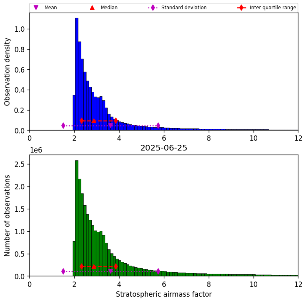
Figure 44: Histogram of “Stratospheric airmass factor” for 2025-06-24 to 2025-06-26
