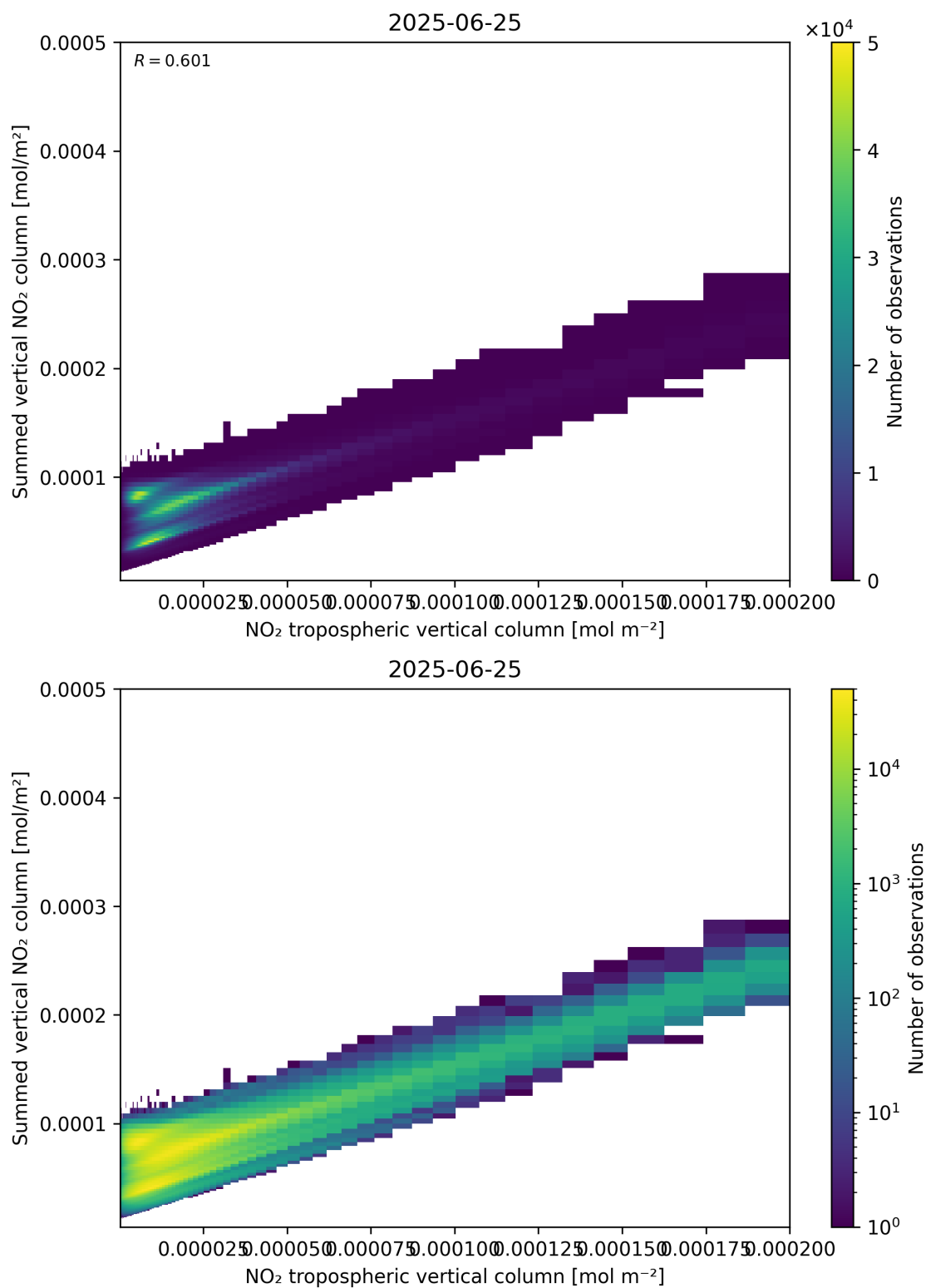
Figure 126: Scatter density plot of “NO 2 tropospheric vertical column” against “Summed vertical NO 2 column” for 2025-06-24 to 2025-06-26.
