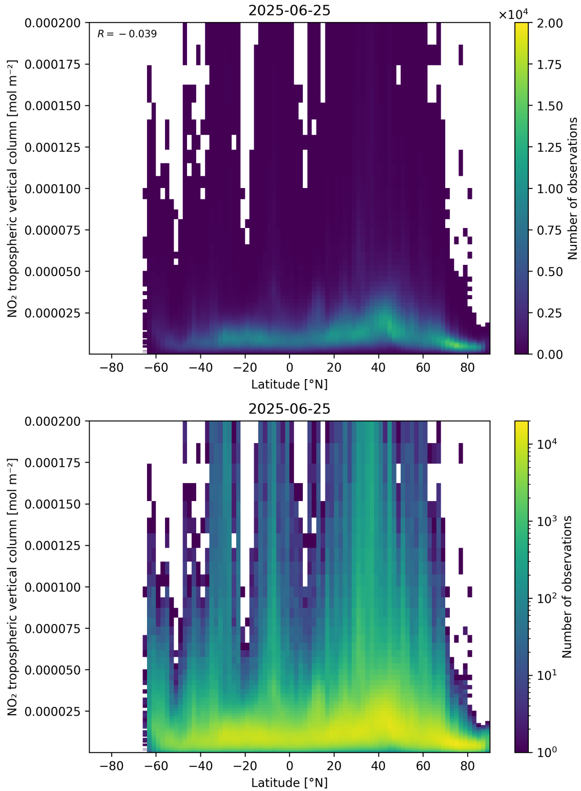
Figure 92: Scatter density plot of “Latitude” against “NO 2 tropospheric vertical column” for 2025-06-24 to 2025-06-26.
