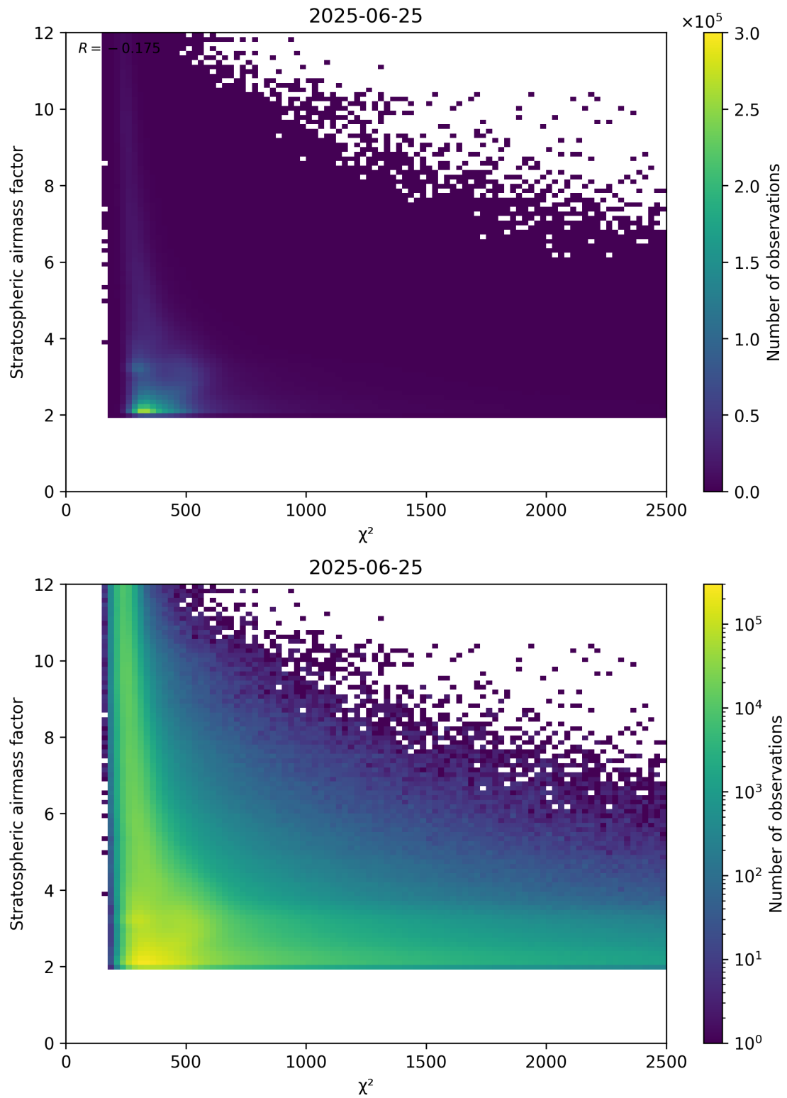
Figure 81: Scatter density plot of “ \chi^2 ” against “Stratospheric airmass factor” for 2025-06-24 to 2025-06-26.
