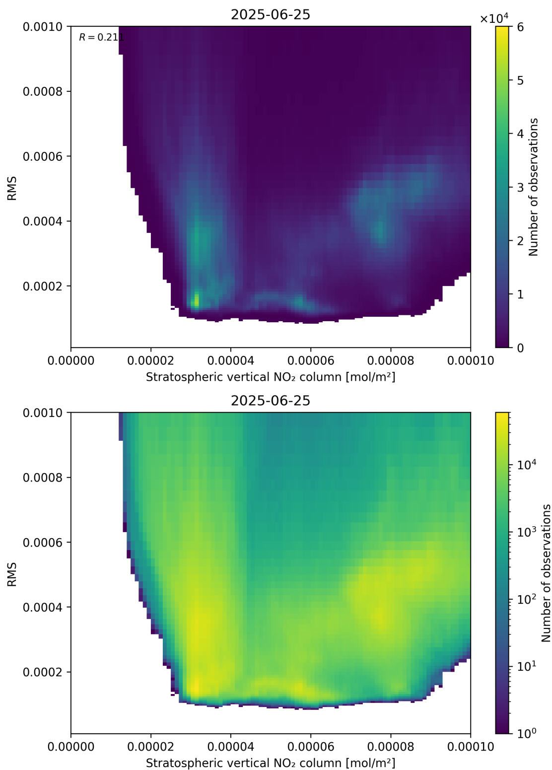
Figure 102: Scatter density plot of “Stratospheric vertical NO 2 column” against “RMS” for 2025-06-24 to 2025-06-26.
