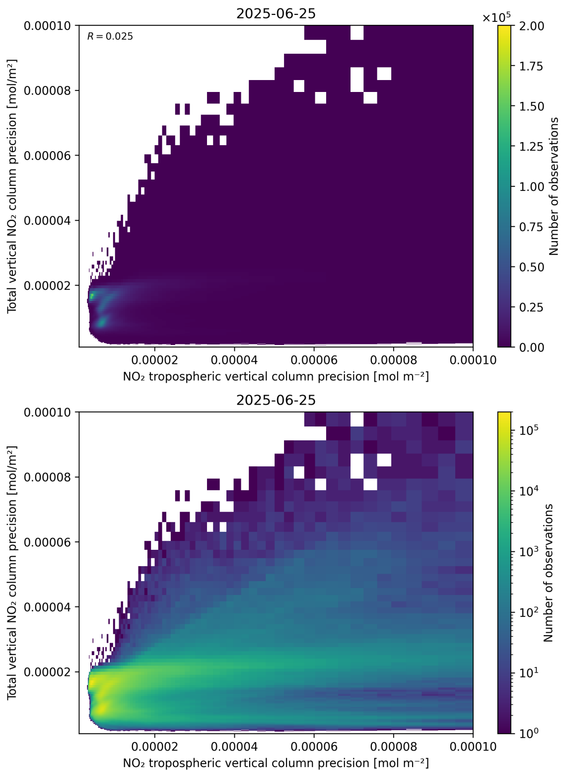
Figure 139: Scatter density plot of “NO 2 tropospheric vertical column precision” against “Total vertical NO 2 column precision” for 2025-06-24 to 2025-06-26.
