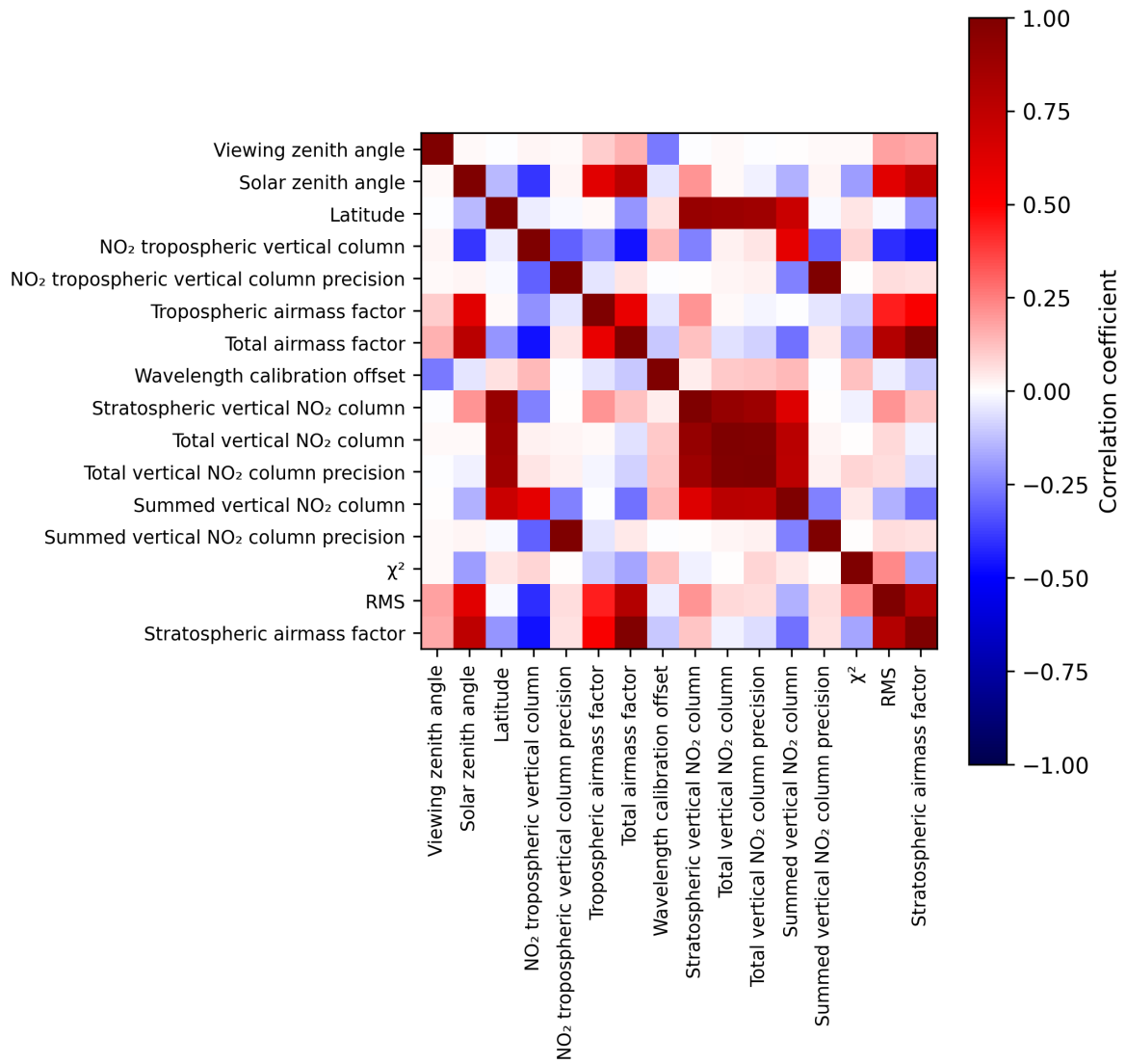
Figure 2: Map of correlation matrix for 2025-06-24 to 2025-06-26.
