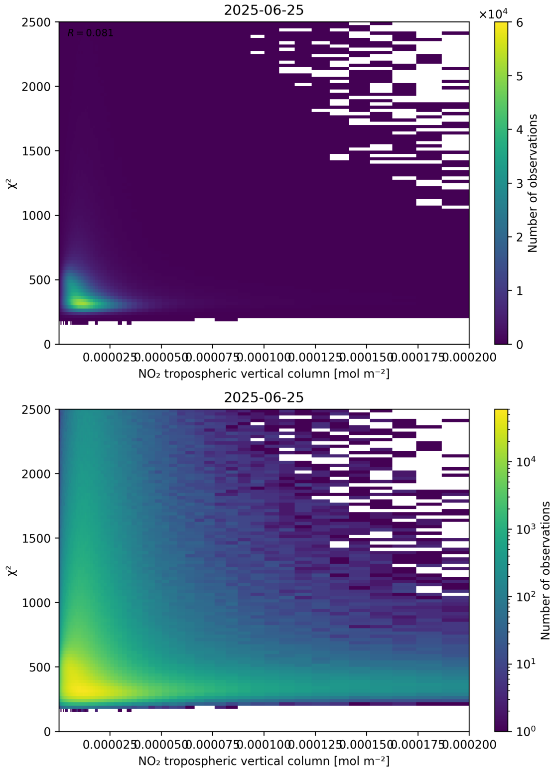
Figure 124: Scatter density plot of “NO 2 tropospheric vertical column” against “ \chi^2 ” for 2025-06-24 to 2025-06-26.
