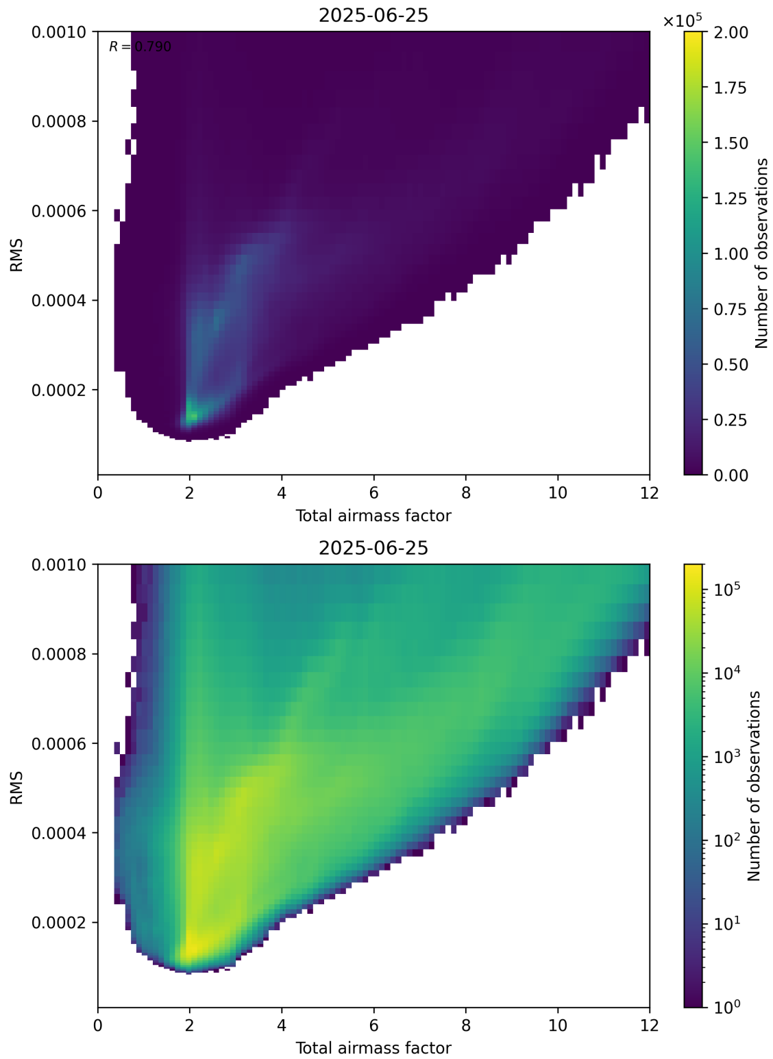
Figure 69: Scatter density plot of “Total airmass factor” against “RMS” for 2025-06-24 to 2025-06-26.
