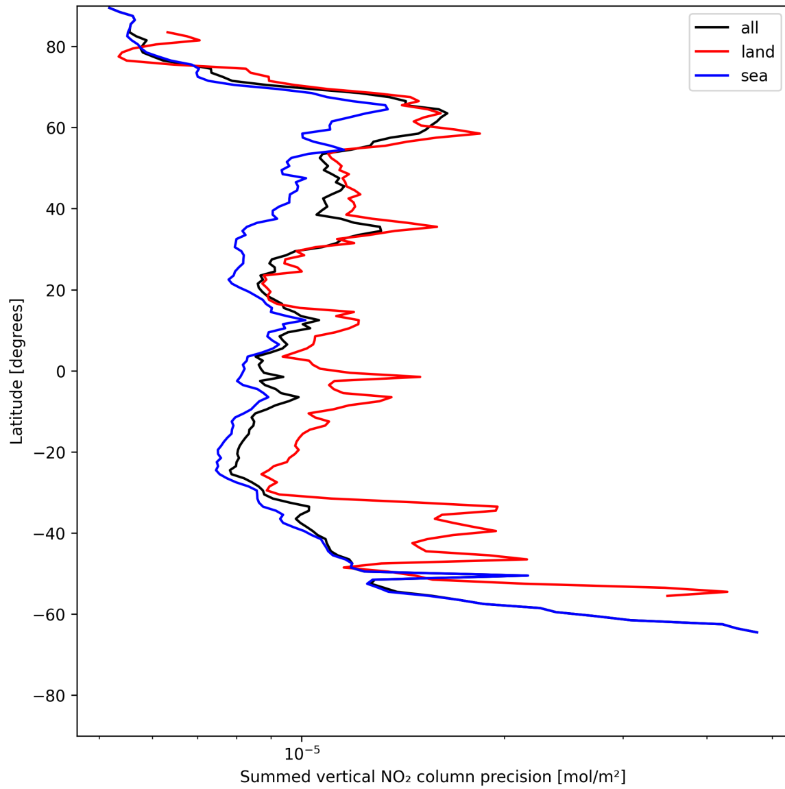
Figure 24: Zonal average of “Summed vertical NO 2 column precision” for 2025-06-24 to 2025-06-26.
