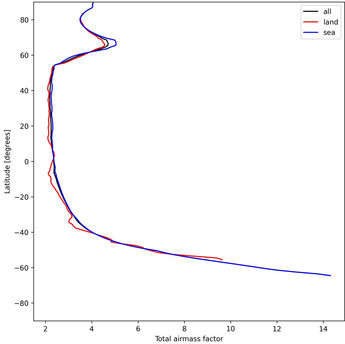
Figure 15: Zonal average of “Total airmass factor” for 2025-06-24 to 2025-06-26.
