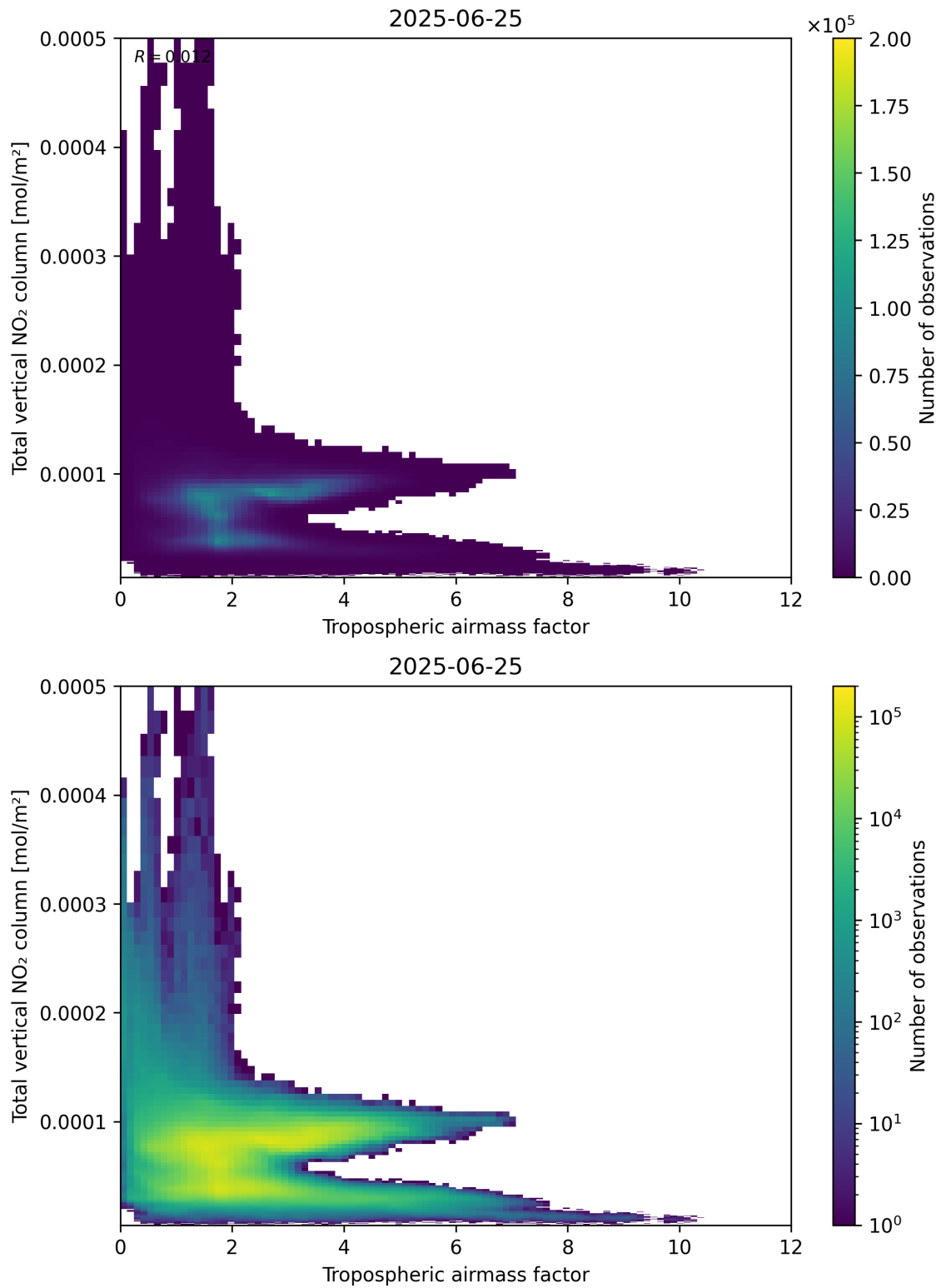
Figure 77: Scatter density plot of “Tropospheric airmass factor” against “Total vertical NO 2 column” for 2025-06-24 to 2025-06-26.
