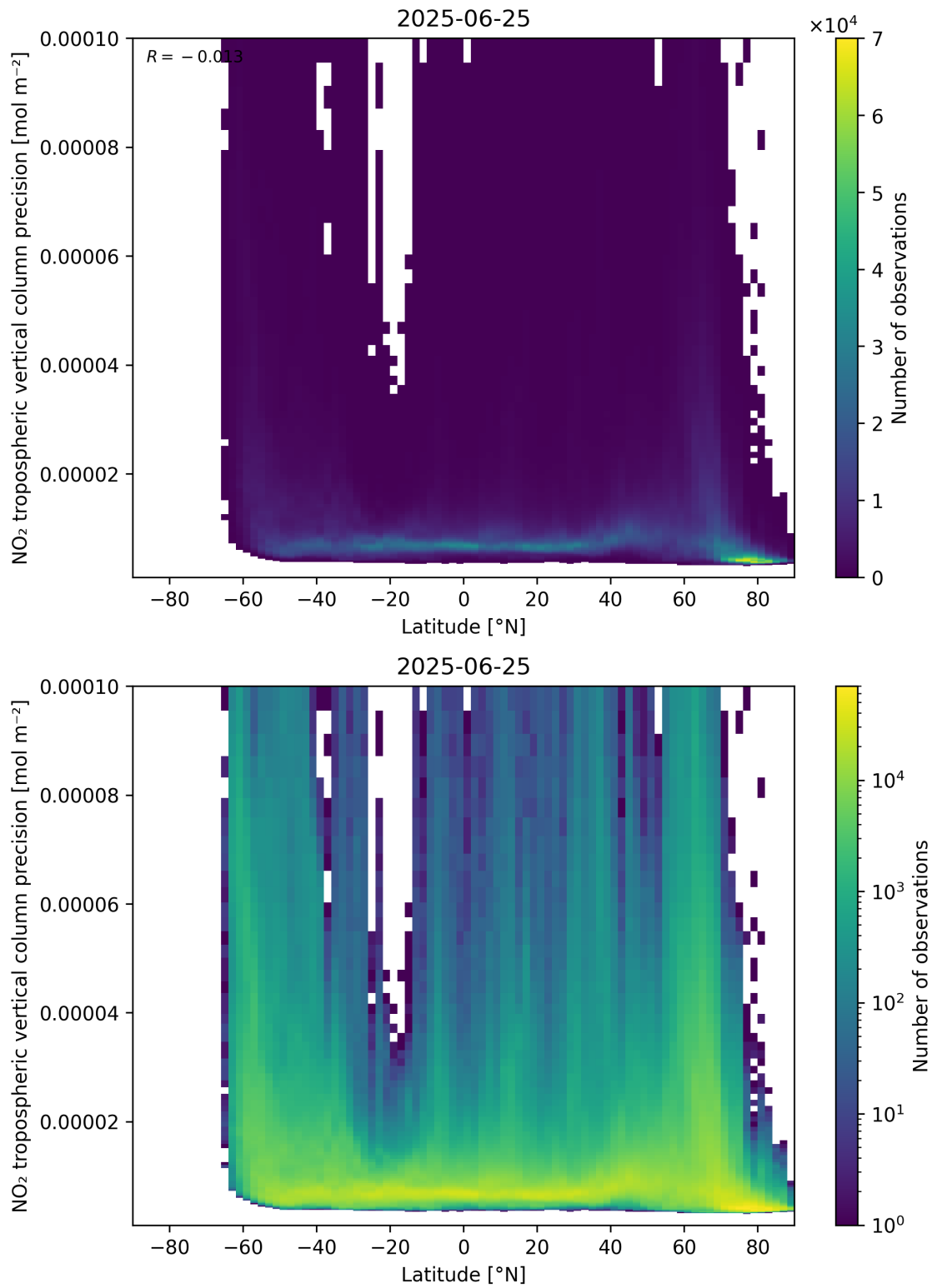
Figure 93: Scatter density plot of “Latitude” against “NO 2 tropospheric vertical column precision” for 2025-06-24 to 2025-06-26.
