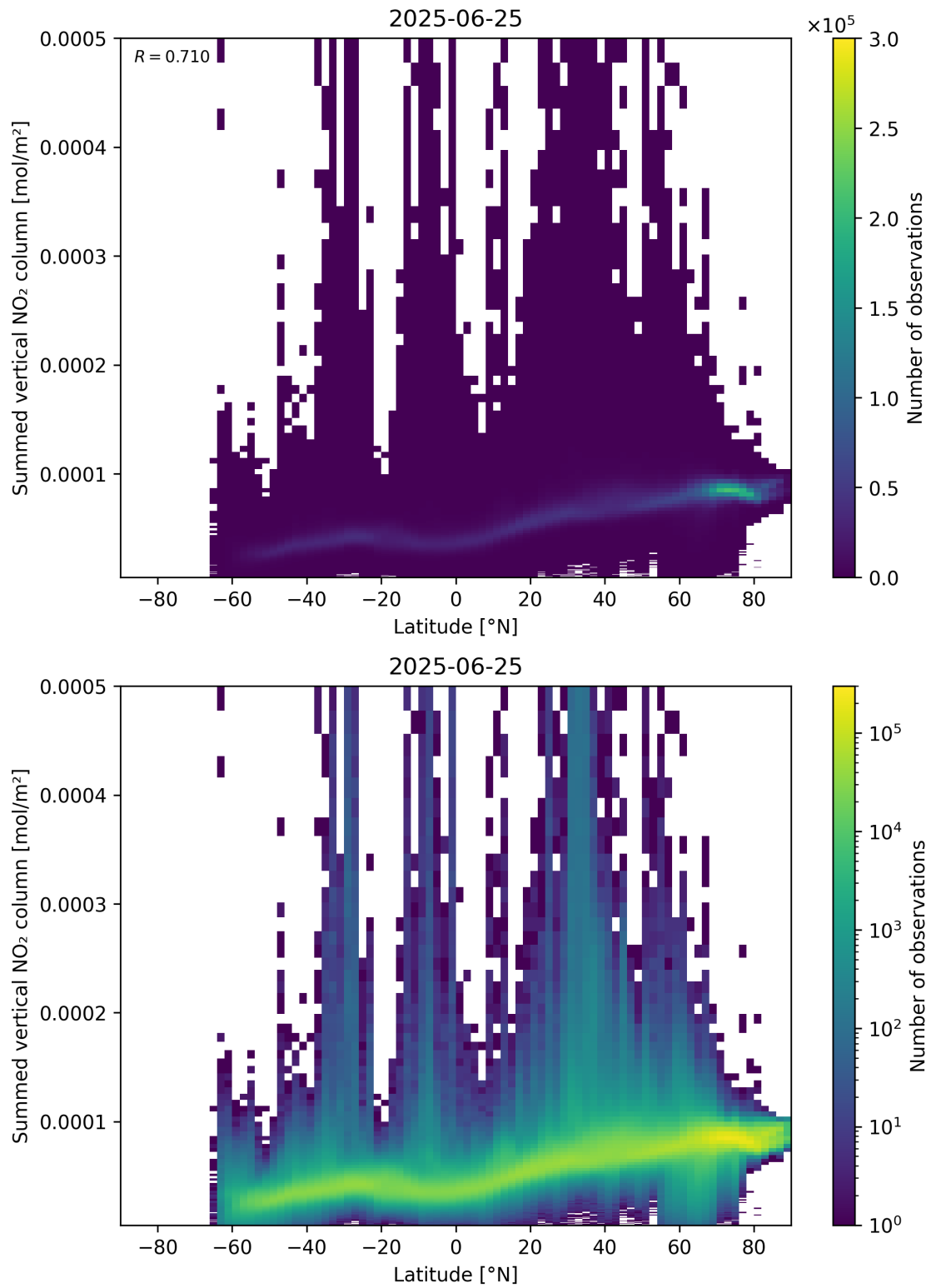
Figure 88: Scatter density plot of “Latitude” against “Summed vertical NO 2 column” for 2025-06-24 to 2025-06-26.
