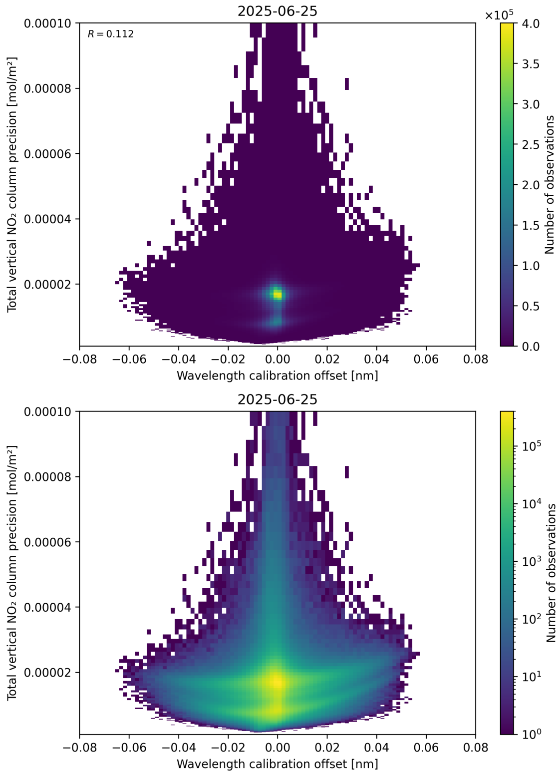
Figure 180: Scatter density plot of “Wavelength calibration offset” against “Total vertical NO 2 column precision” for 2025-06-24 to 2025-06-26.
