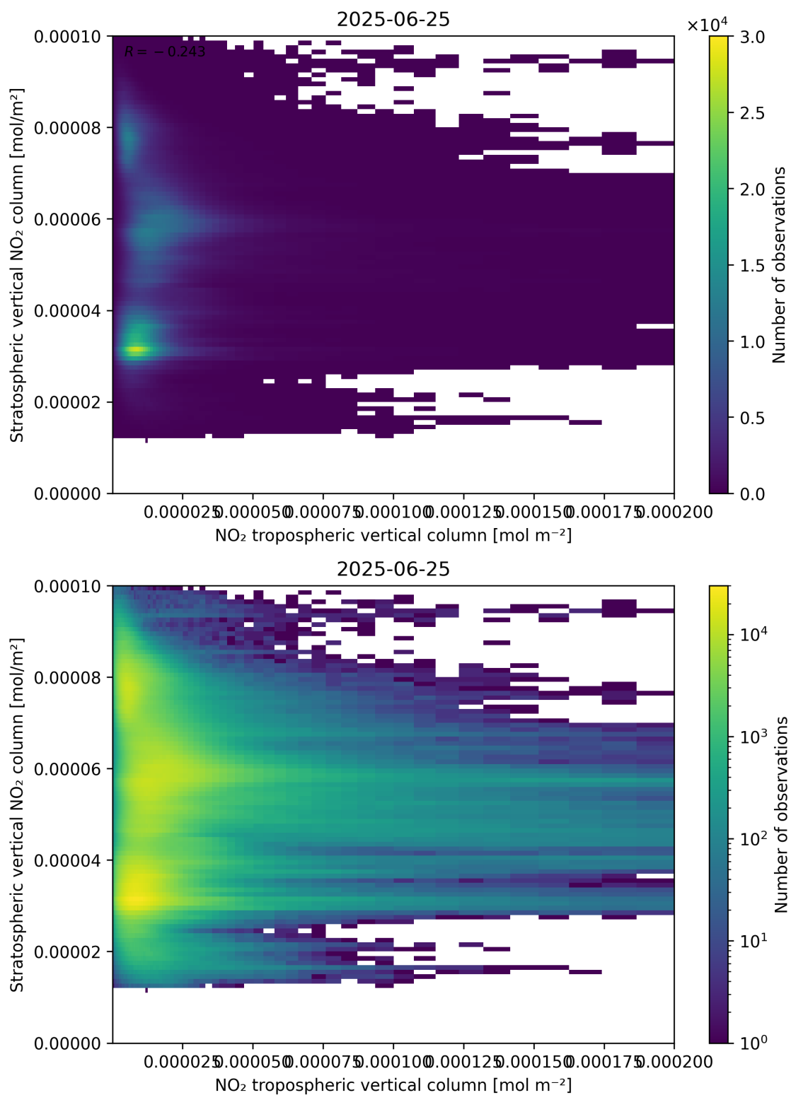
Figure 125: Scatter density plot of “NO 2 tropospheric vertical column” against “Stratospheric vertical NO 2 column” for 2025-06-24 to 2025-06-26.
