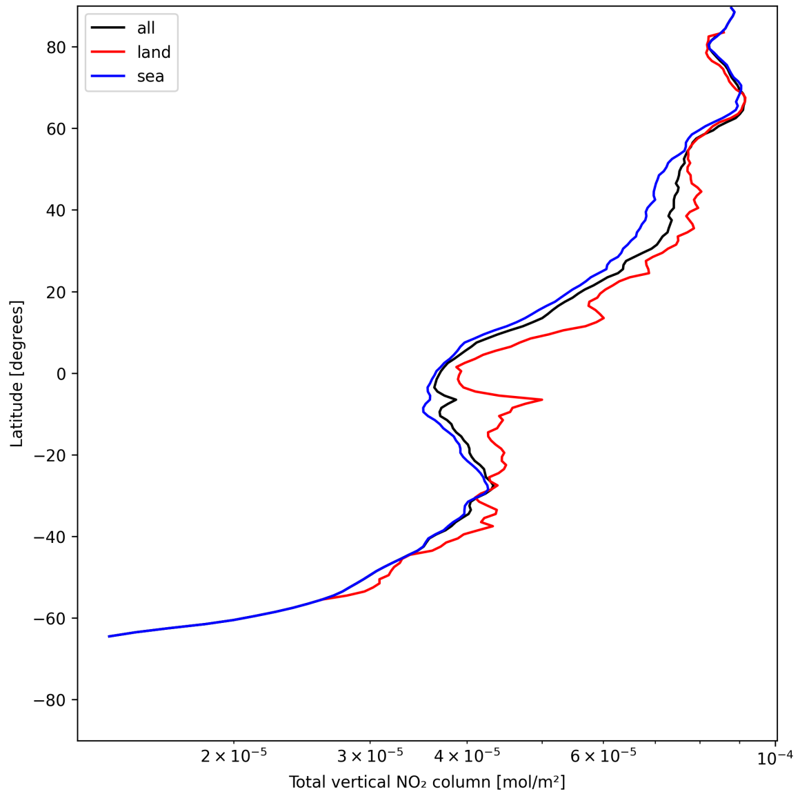
Figure 21: Zonal average of “Total vertical NO 2 column” for 2025-06-24 to 2025-06-26.
