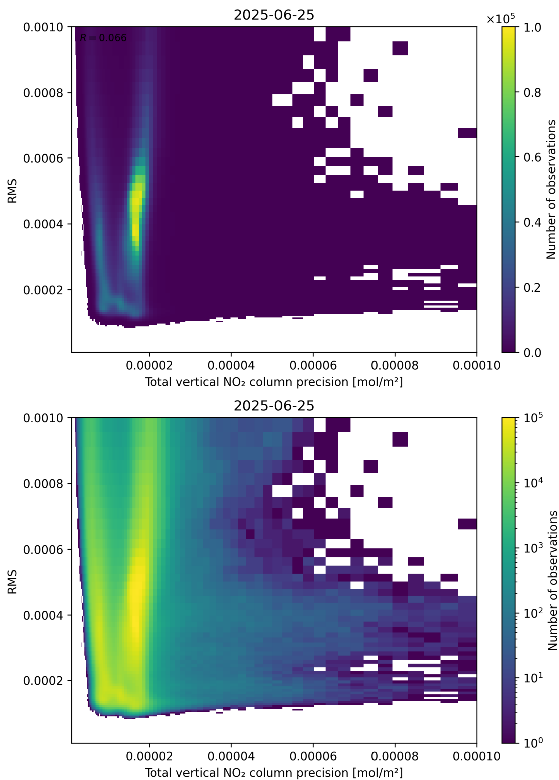
Figure 119: Scatter density plot of “Total vertical NO 2 column precision” against “RMS” for 2025-06-24 to 2025-06-26.
