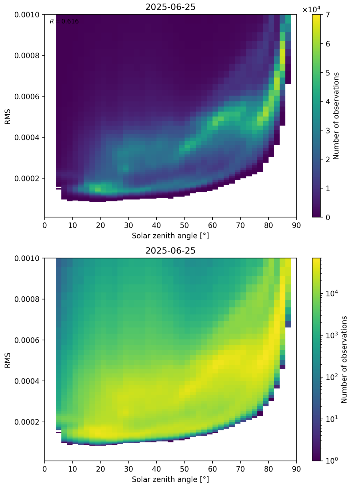
Figure 157: Scatter density plot of “Solar zenith angle” against “RMS” for 2025-06-24 to 2025-06-26.
