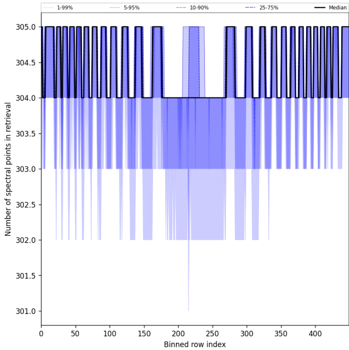
Figure 50: Along track statistics of “Number of spectral points in retrieval” for 2025-06-24 to 2025-06-26
