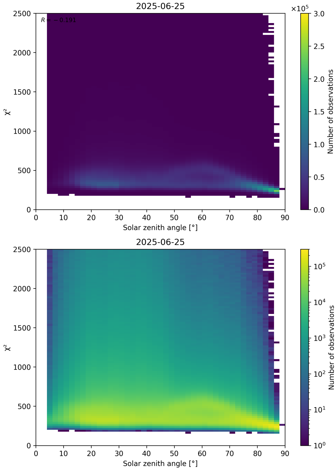
Figure 148: Scatter density plot of “Solar zenith angle” against “ \chi^2 ” for 2025-06-24 to 2025-06-26.
