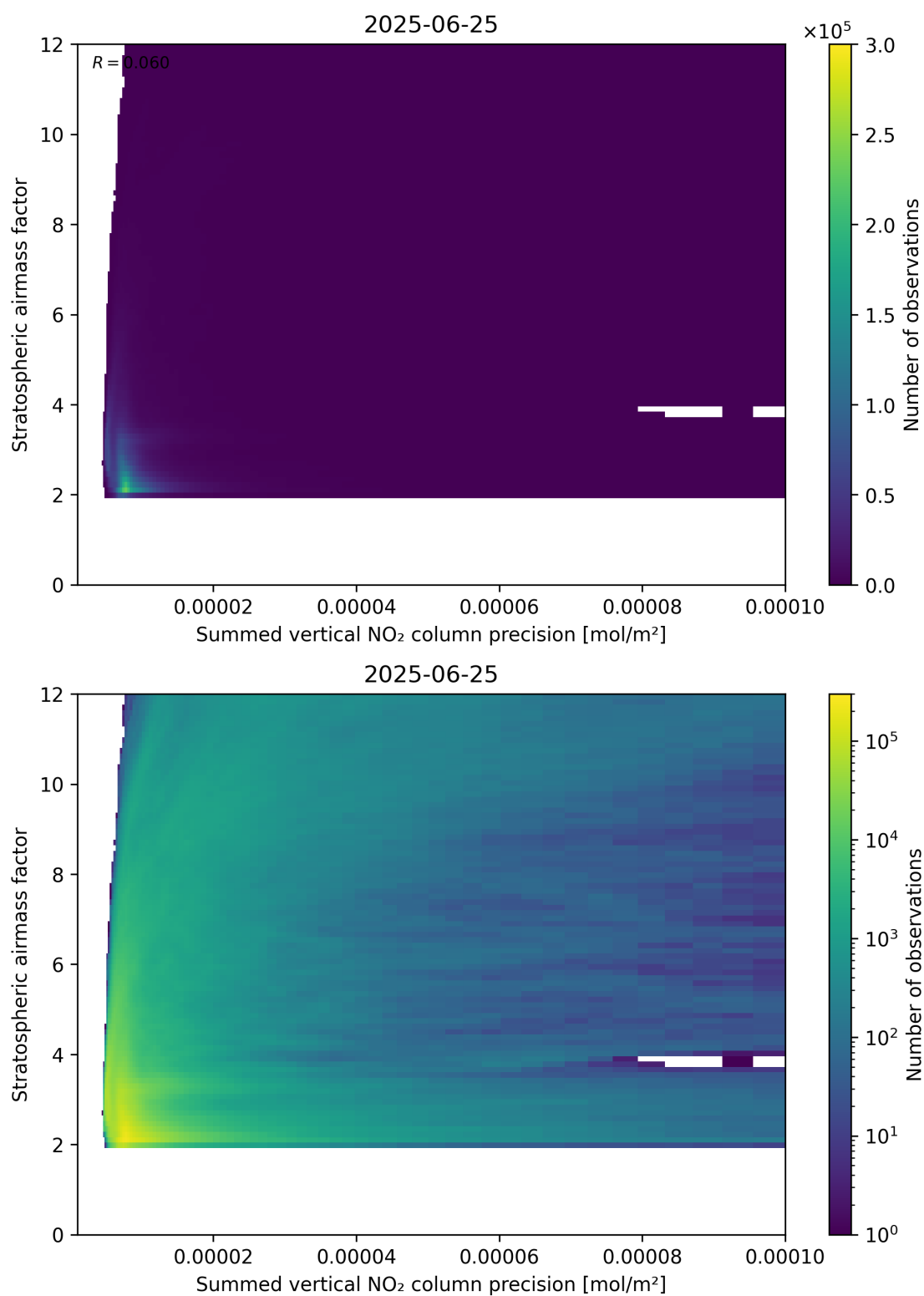
Figure 106: Scatter density plot of “Summed vertical NO 2 column precision” against “Stratospheric airmass factor” for 2025-06-24 to 2025-06-26.
