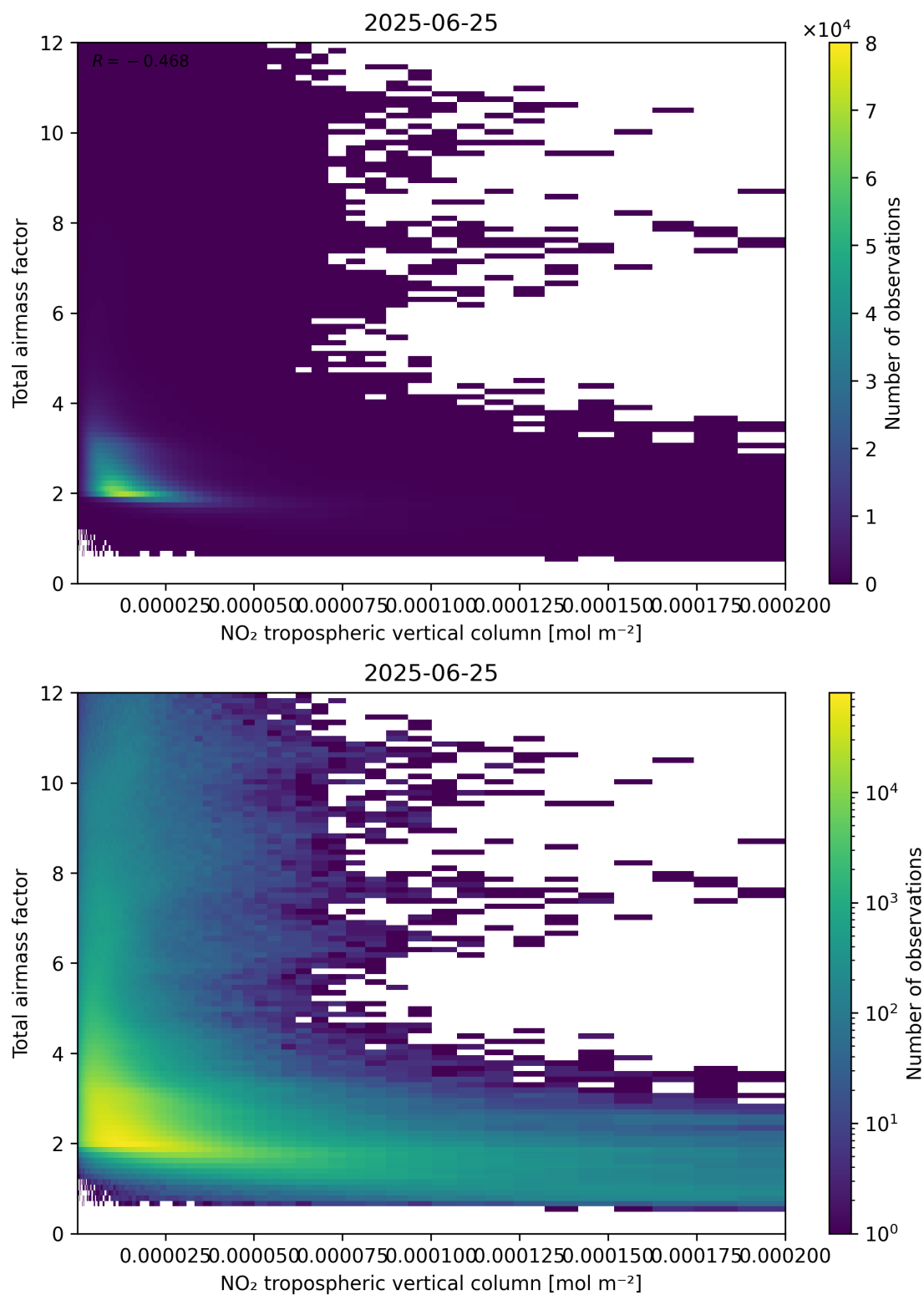
Figure 122: Scatter density plot of “NO 2 tropospheric vertical column” against “Total air mass factor” for 2025-06-24 to 2025-06-26.
