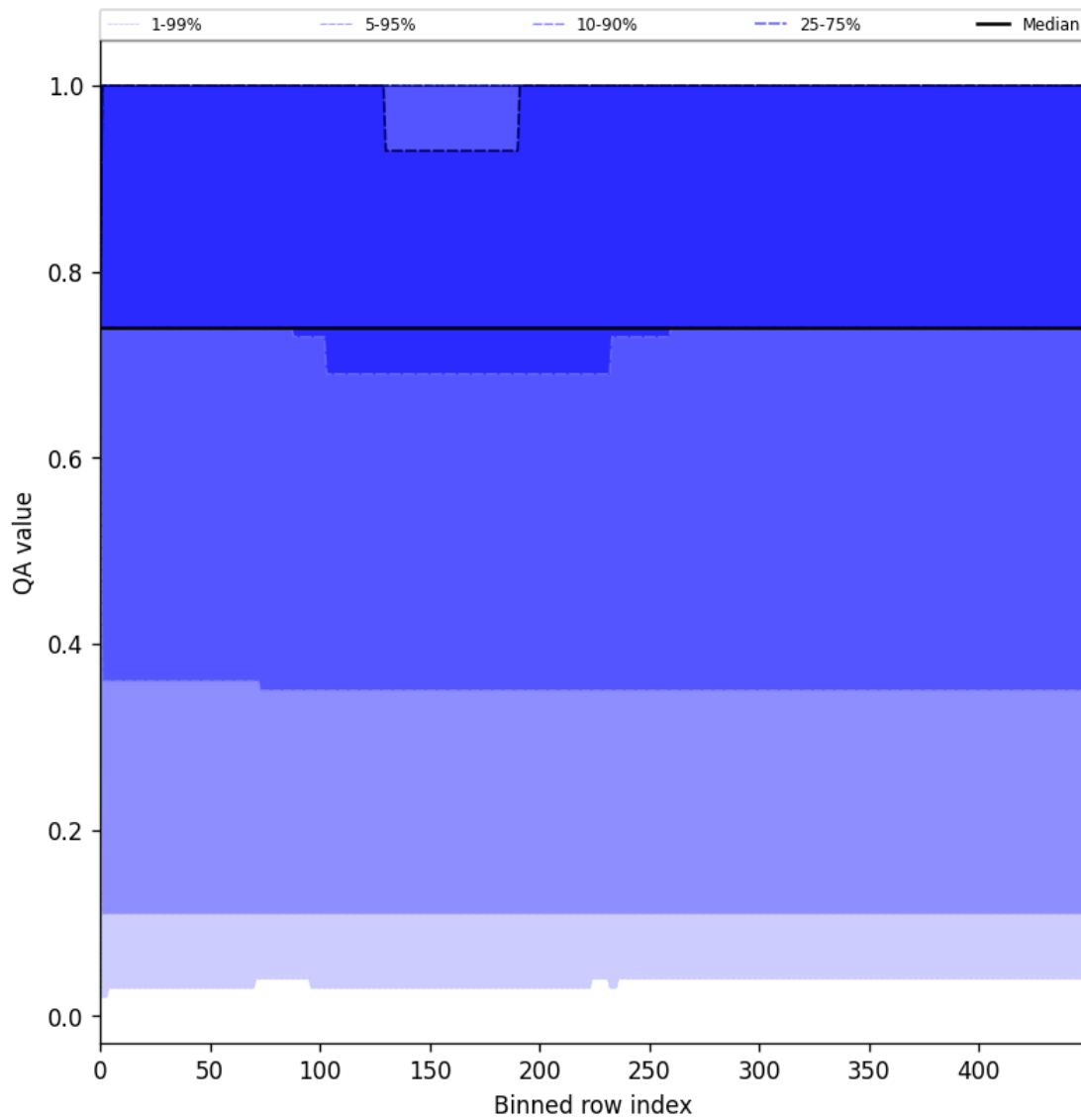
Figure 45: Along track statistics of "QA value" for 2025-06-24 to 2025-06-26
