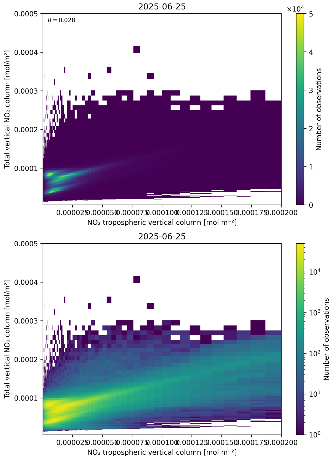
Figure 128: Scatter density plot of “NO 2 tropospheric vertical column” against “Total vertical NO 2 column” for 2025-06-24 to 2025-06-26.
