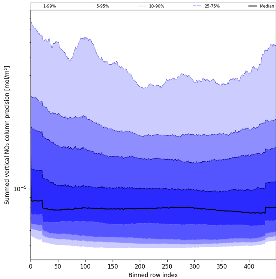
Figure 58: Along track statistics of “Summed vertical NO 2 column precision” for 2025-06-24 to 2025-06-26
