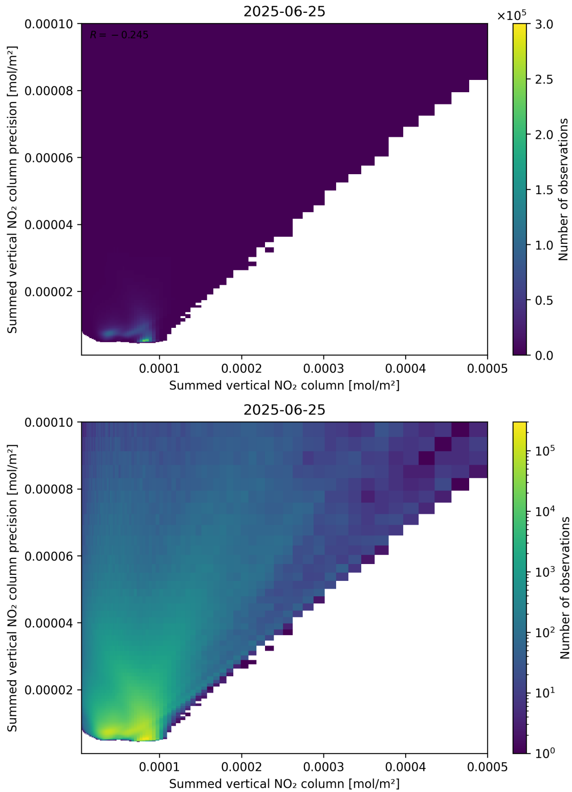
Figure 105: Scatter density plot of “Summed vertical NO 2 column” against “Summed vertical NO 2 column precision” for 2025-06-24 to 2025-06-26.
