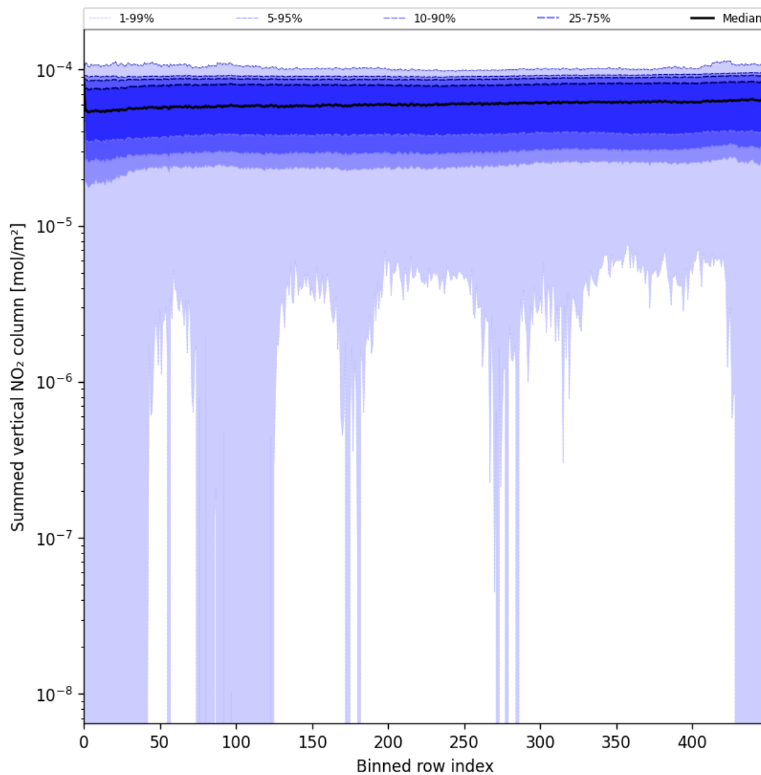
Figure 57: Along track statistics of “Summed vertical NO 2 column” for 2025-06-24 to 2025-06-26
