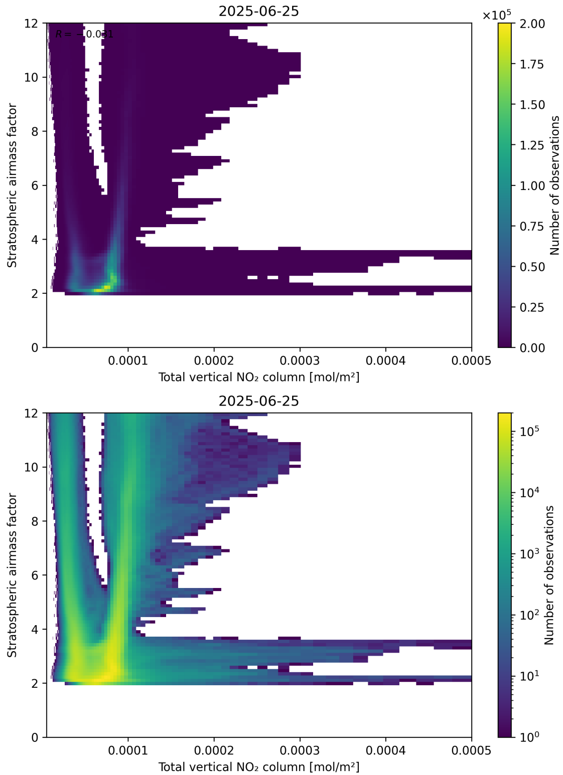
Figure 110: Scatter density plot of “Total vertical NO 2 column” against “Stratospheric airmass factor” for 2025-06-24 to 2025-06-26.
