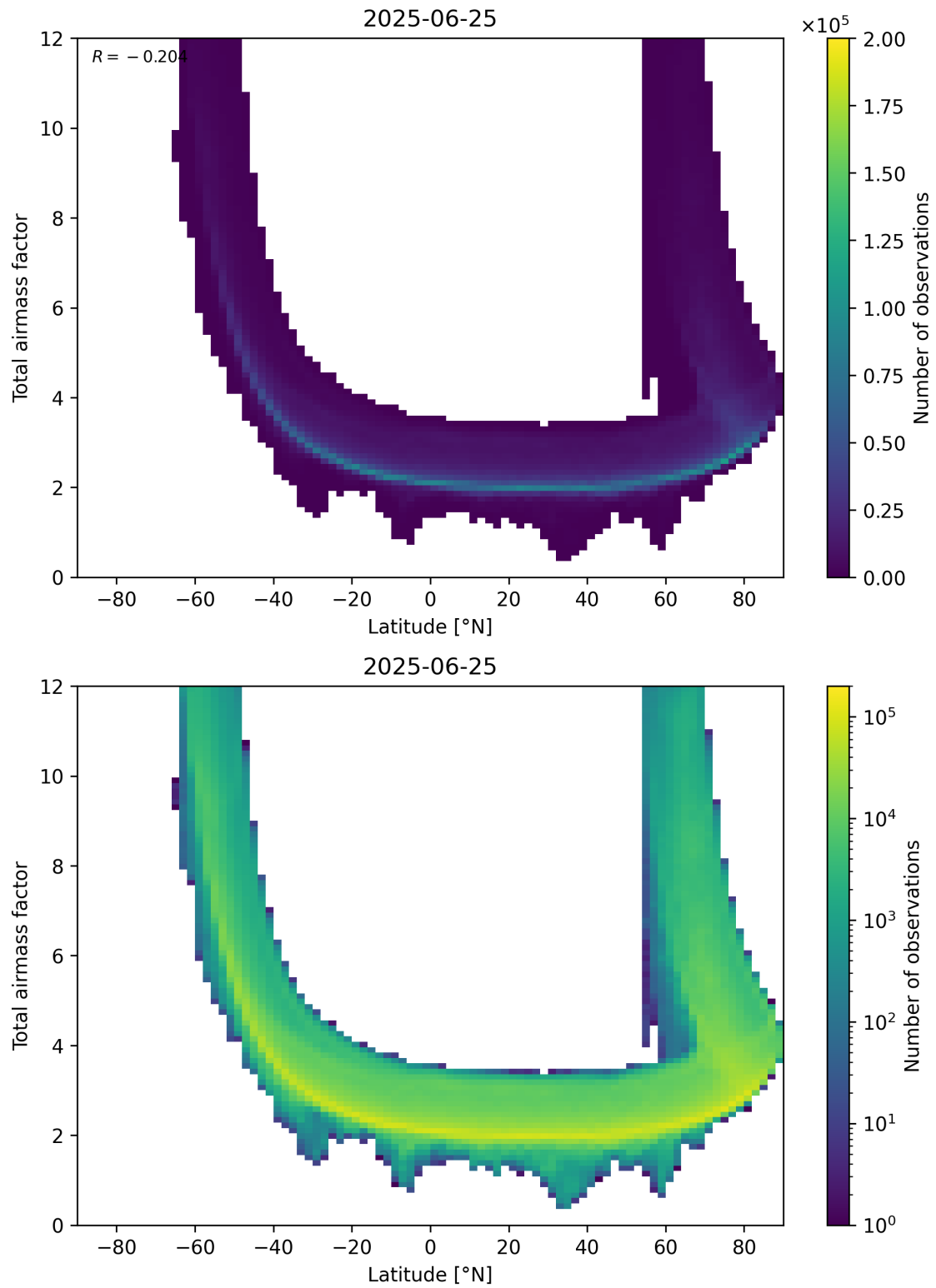
Figure 84: Scatter density plot of “Latitude” against “Total airmass factor” for 2025-06-24 to 2025-06-26.
