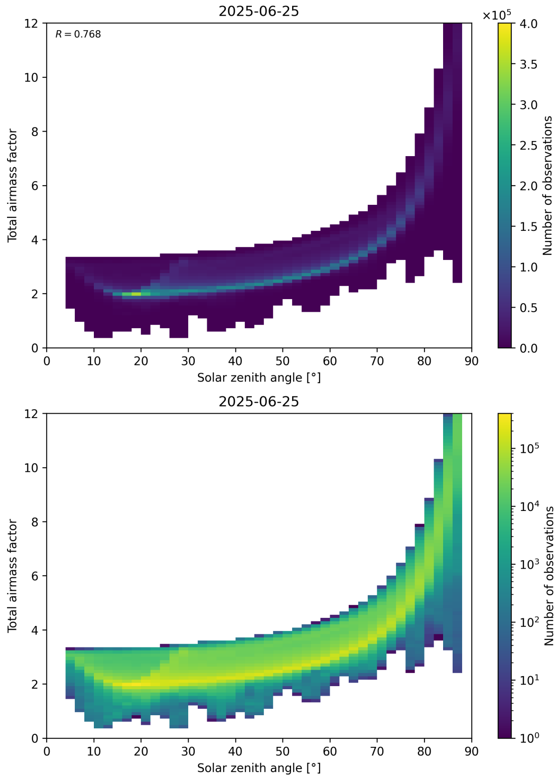
Figure 146: Scatter density plot of “Solar zenith angle” against “Total air mass factor” for 2025-06-24 to 2025-06-26.
