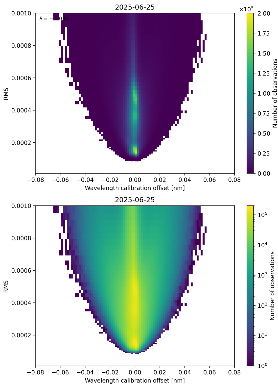
Figure 181: Scatter density plot of “Wavelength calibration offset” against “RMS” for 2025-06-24 to 2025-06-26.
