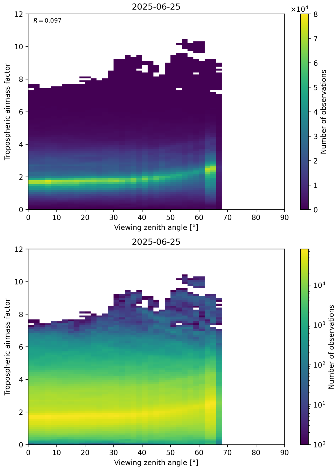
Figure 161: Scatter density plot of “Viewing zenith angle” against “Tropospheric airmass factor” for 2025-06-24 to 2025-06-26.
