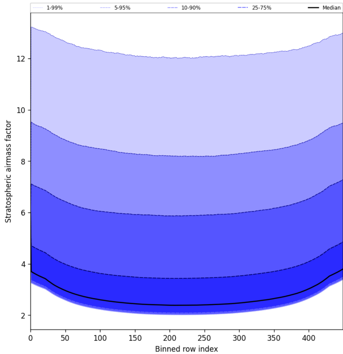
Figure 61: Along track statistics of “Stratospheric airmass factor” for 2025-06-24 to 2025-06-26
