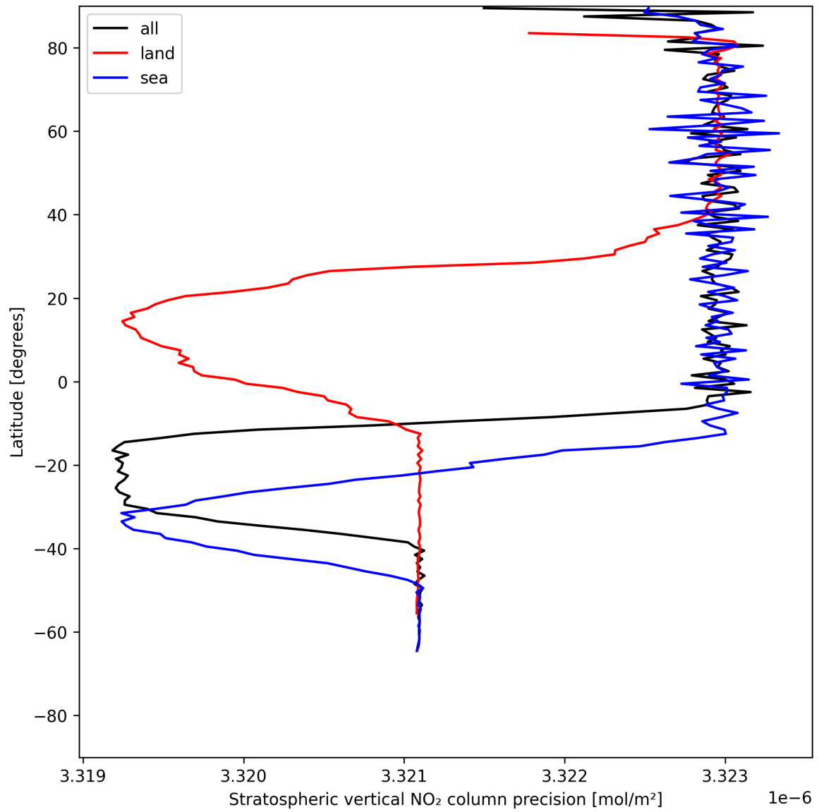
Figure 20: Zonal average of “Stratospheric vertical NO 2 column precision” for 2025-06-24 to 2025-06-26.
