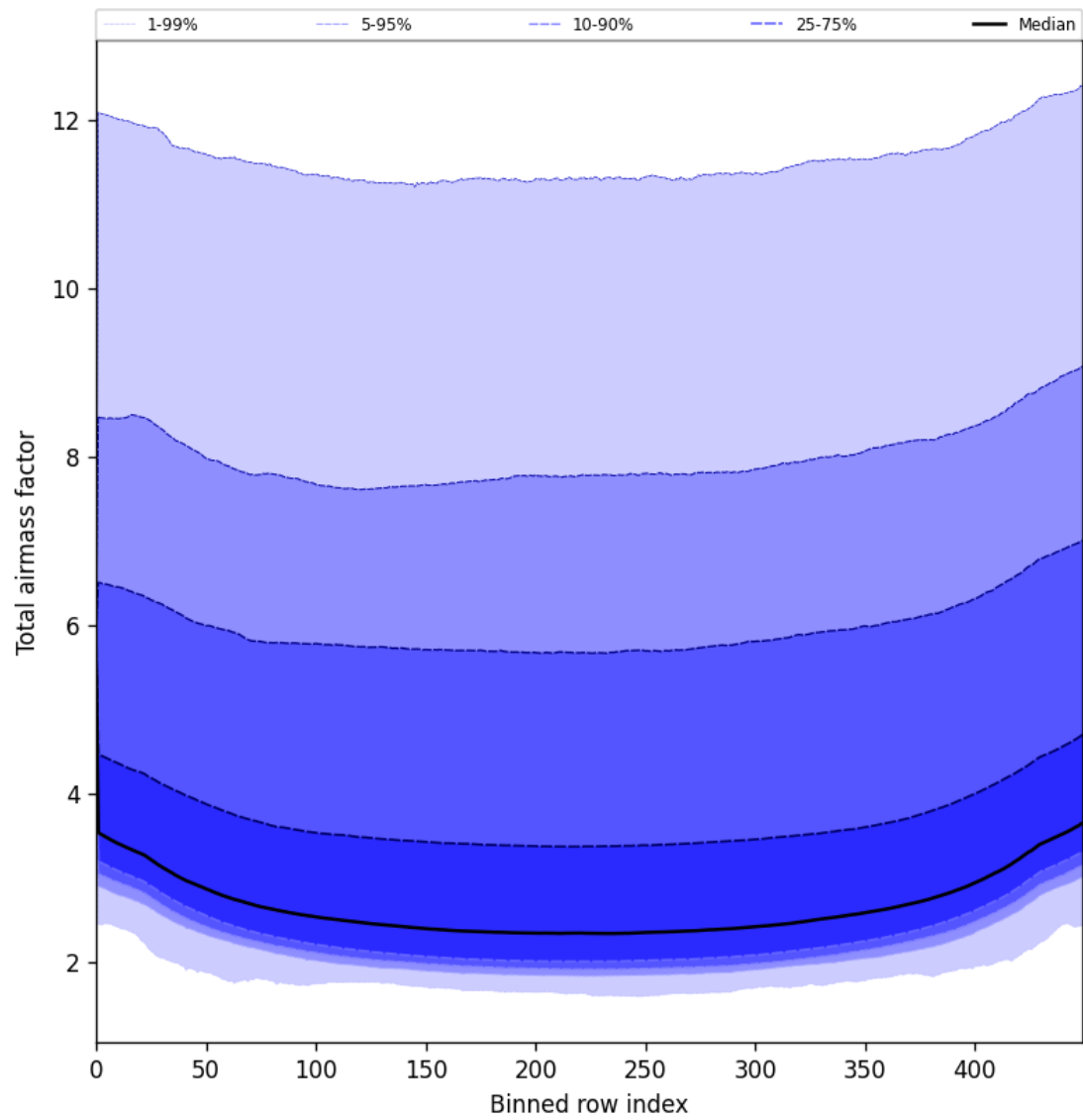
Figure 49: Along track statistics of “Total airmass factor” for 2025-06-24 to 2025-06-26
