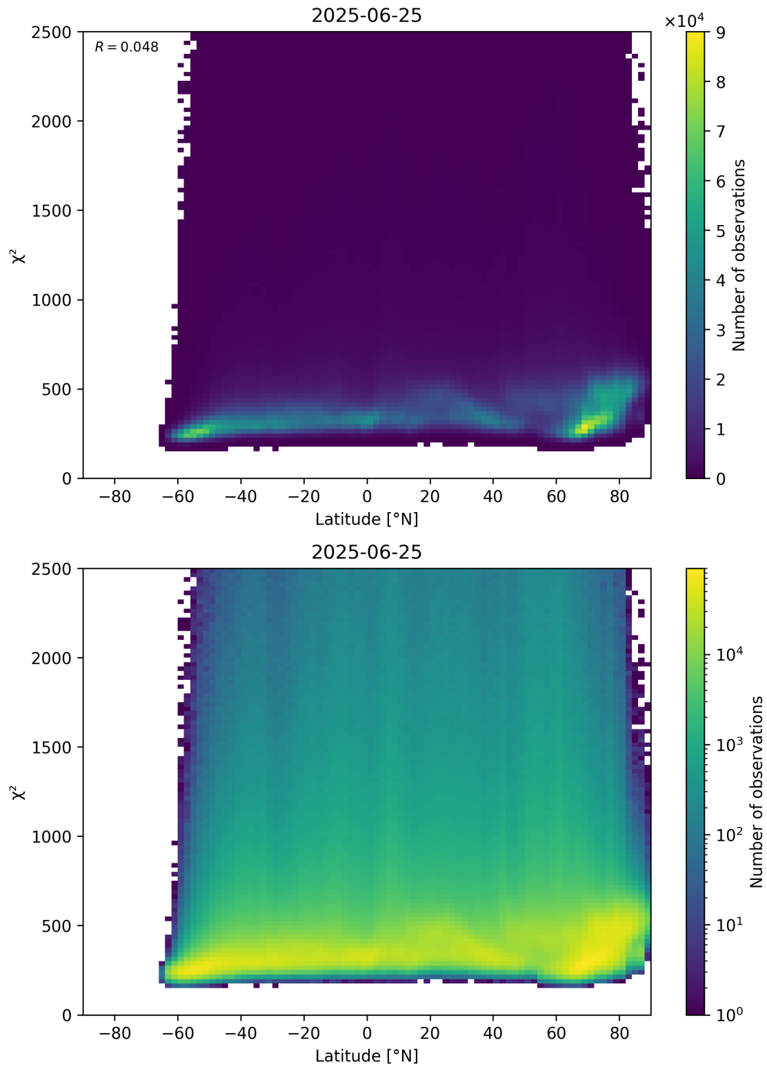
Figure 86: Scatter density plot of “Latitude” against “ \chi^2 ” for 2025-06-24 to 2025-06-26.
