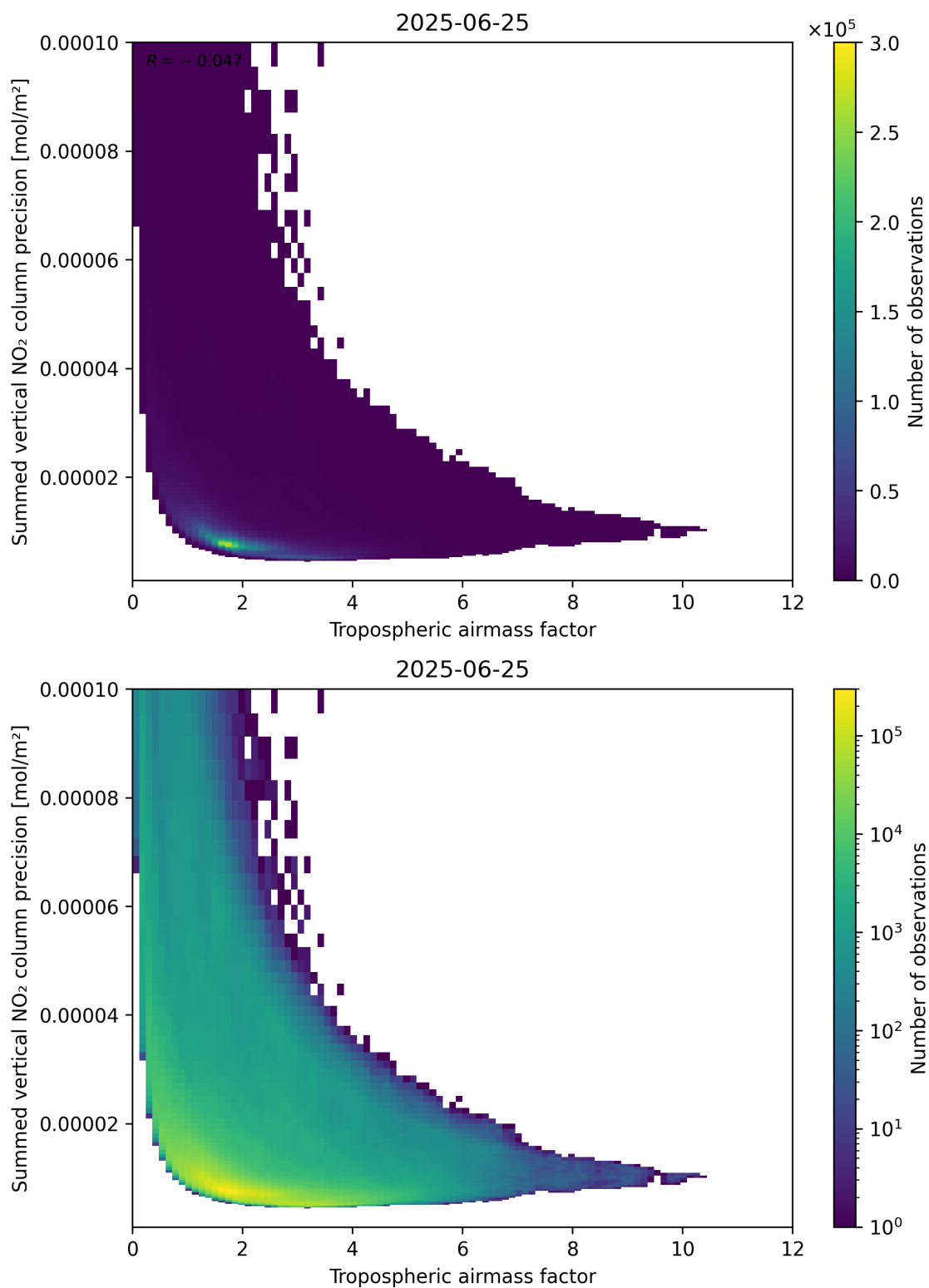
Figure 76: Scatter density plot of “Tropospheric air mass factor” against “Summed vertical NO 2 column precision” for 2025-06-24 to 2025-06-26.
