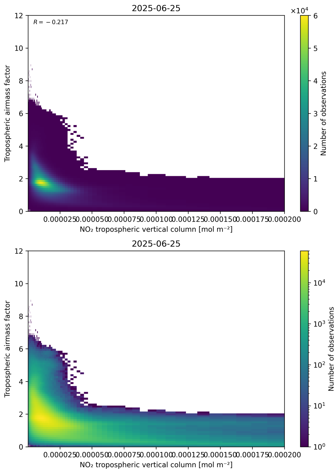
Figure 123: Scatter density plot of “NO 2 tropospheric vertical column” against “Tropospheric air mass factor” for 2025-06-24 to 2025-06-26.
