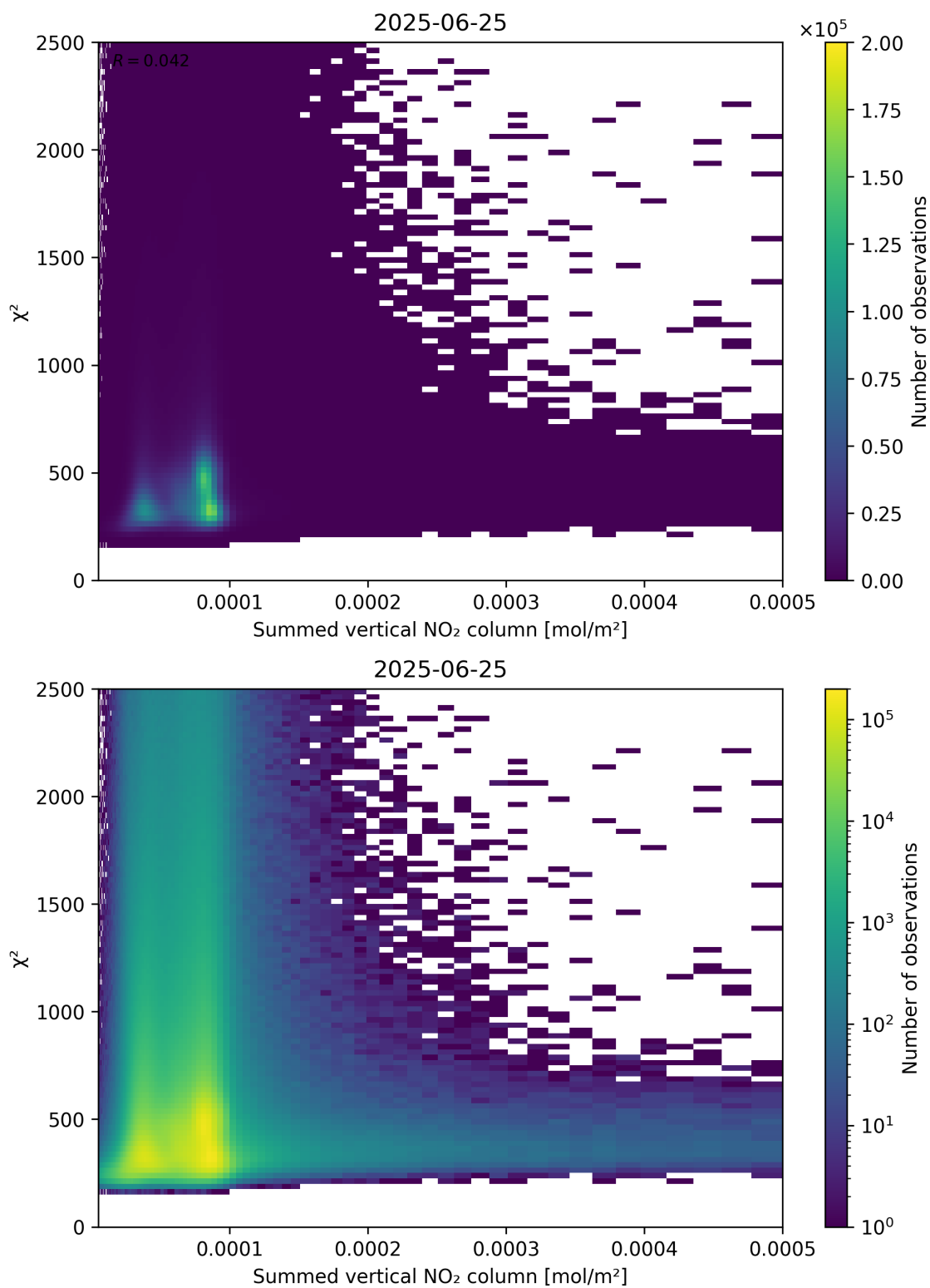
Figure 104: Scatter density plot of “Summed vertical NO 2 column” against “ \chi^2 ” for 2025-06-24 to 2025-06-26.
