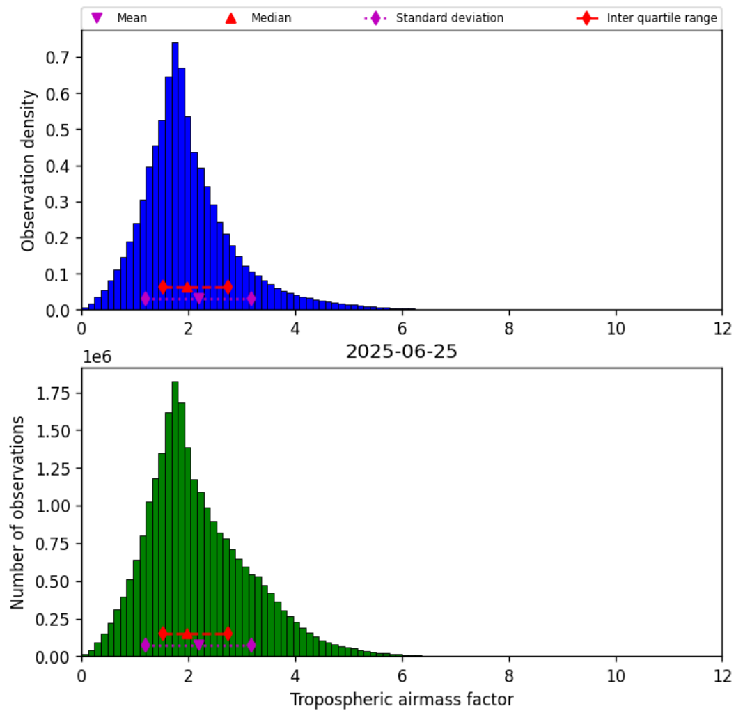
Figure 31: Histogram of “Tropospheric airmass factor” for 2025-06-24 to 2025-06-26
