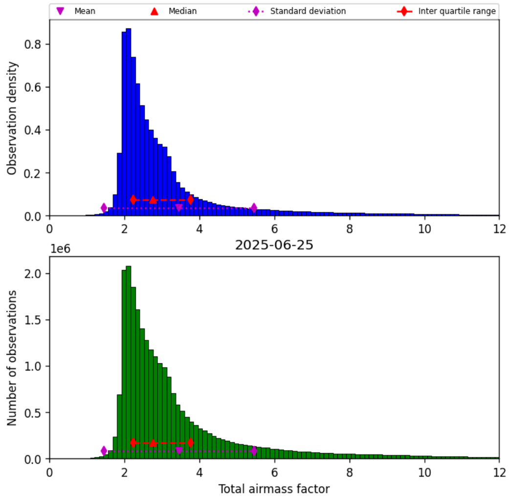
Figure 32: Histogram of “Total airmass factor” for 2025-06-24 to 2025-06-26
