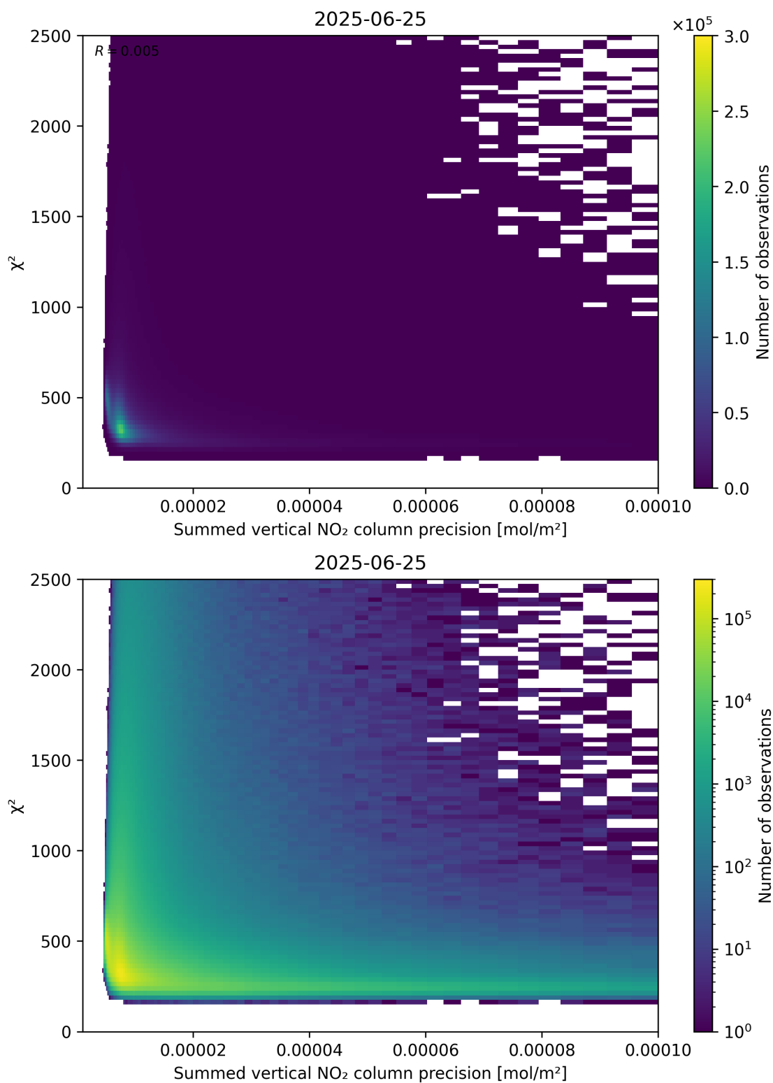
Figure 107: Scatter density plot of “Summed vertical NO 2 column precision” against “ \chi^2 ” for 2025-06-24 to 2025-06-26.
