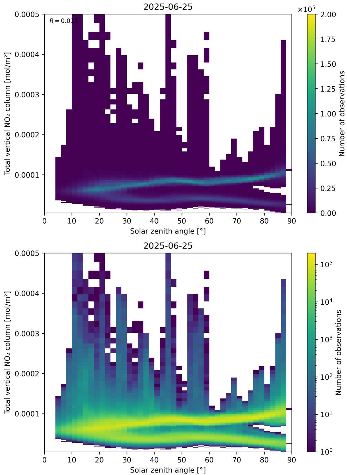
Figure 153: Scatter density plot of “Solar zenith angle” against “Total vertical NO 2 column” for 2025-06-24 to 2025-06-26.
