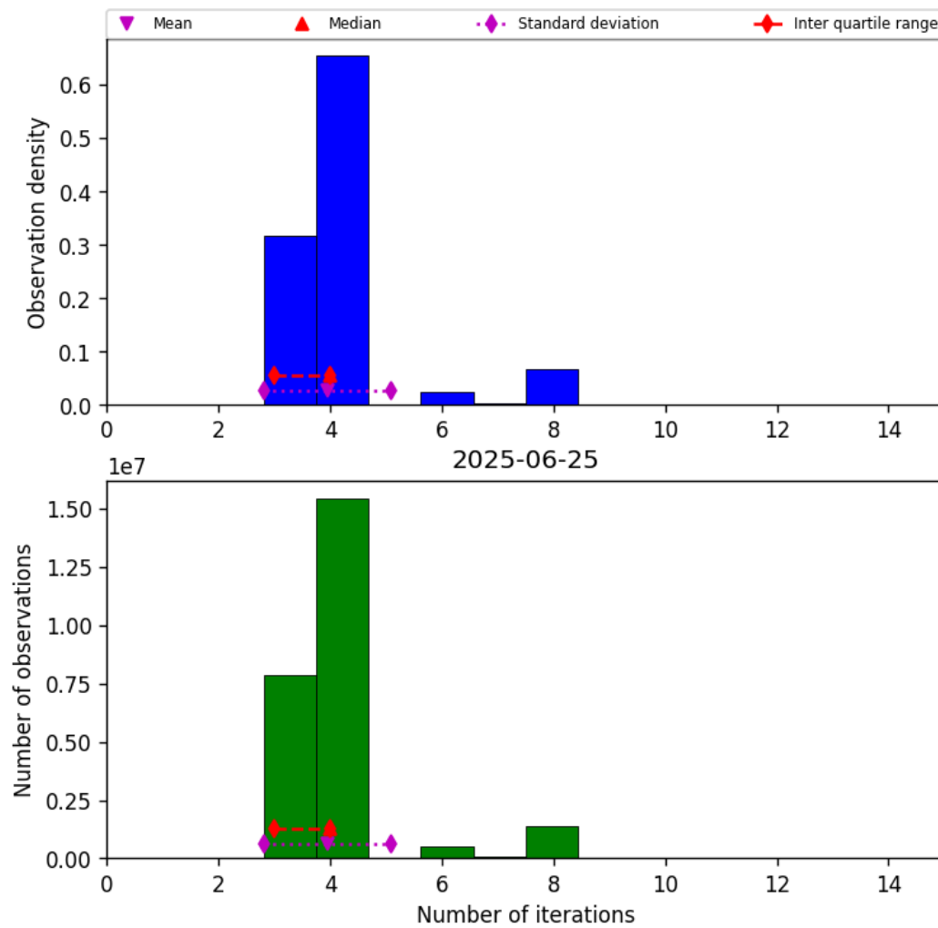
Figure 34: Histogram of “Number of iterations” for 2025-06-24 to 2025-06-26
