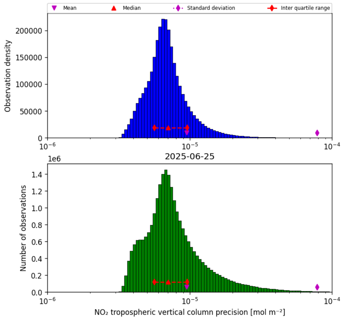
Figure 30: Histogram of “NO 2 tropospheric vertical column precision” for 2025-06-24 to 2025-06-26
