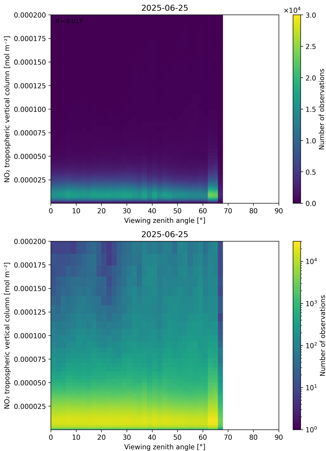
Figure 169: Scatter density plot of “Viewing zenith angle” against “NO 2 tropospheric vertical column” for 2025-06-24 to 2025-06-26.
