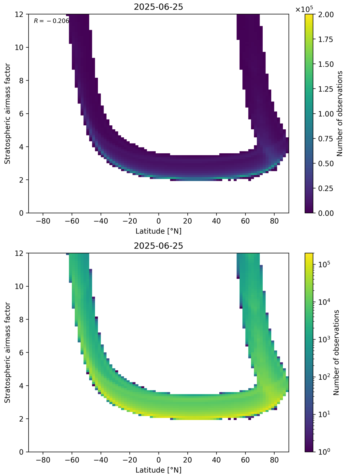
Figure 83: Scatter density plot of “Latitude” against “Stratospheric air mass factor” for 2025-06-24 to 2025-06-26.
