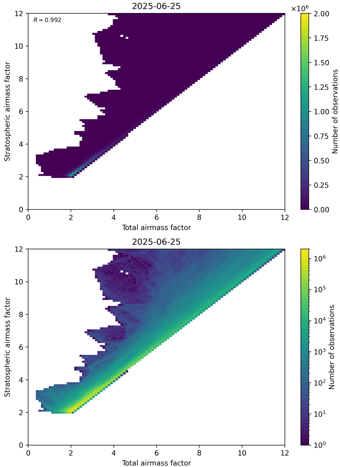
Figure 62: Scatter density plot of “Total airmass factor” against “Stratospheric airmass factor” for 2025-06-24 to 2025-06-26.
