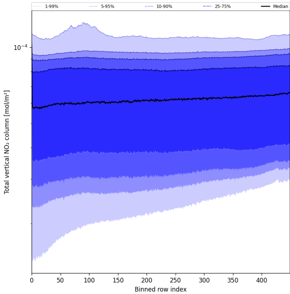
Figure 55: Along track statistics of “Total vertical NO 2 column” for 2025-06-24 to 2025-06-26
