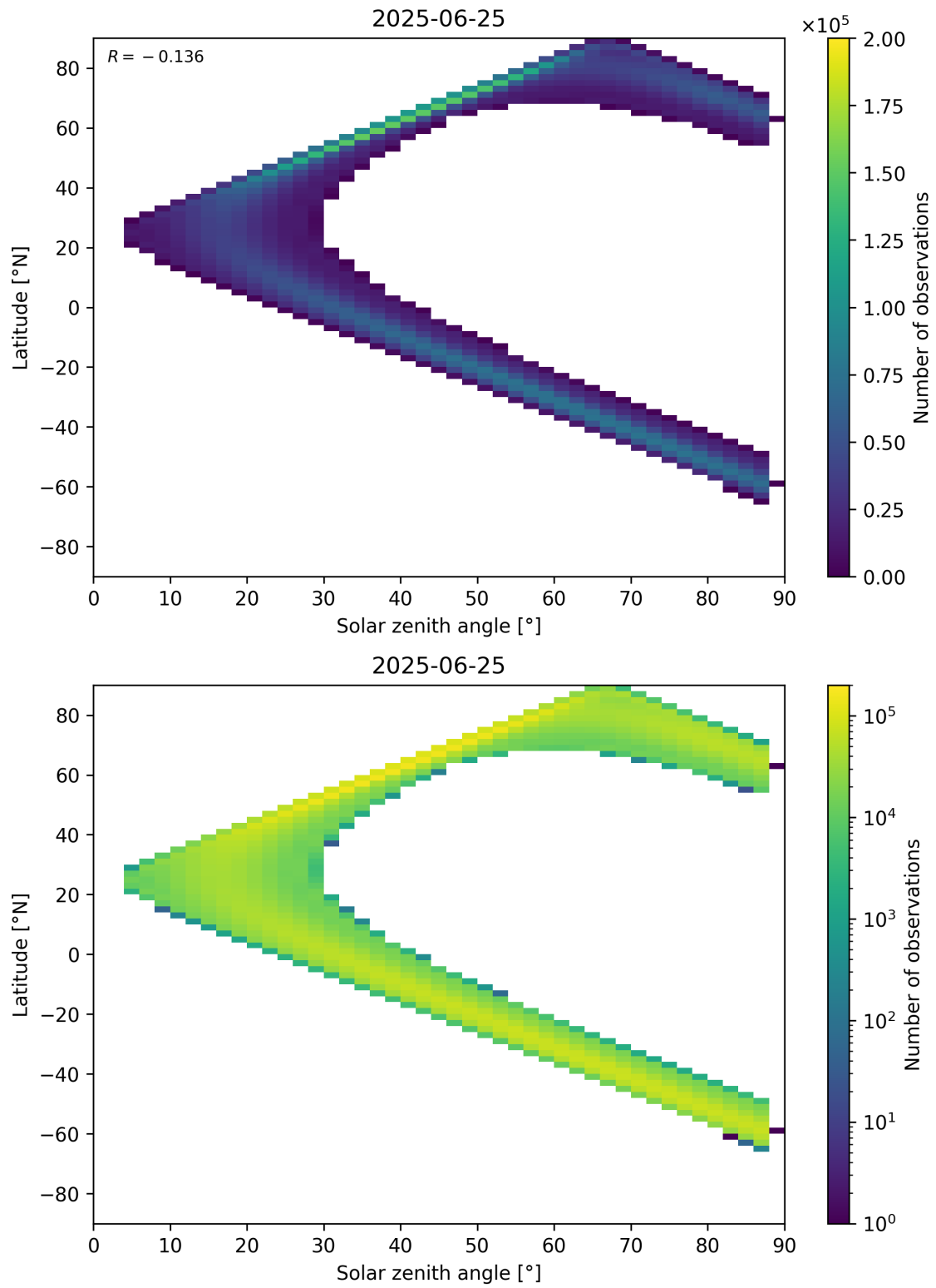
Figure 149: Scatter density plot of “Solar zenith angle” against “Latitude” for 2025-06-24 to 2025-06-26.
