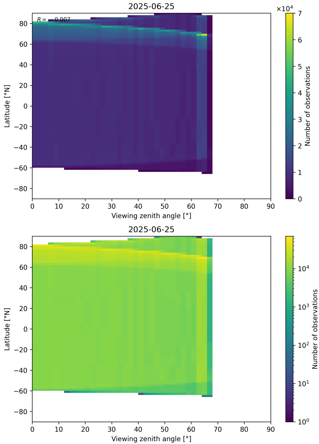
Figure 163: Scatter density plot of “Viewing zenith angle” against “Latitude” for 2025-06-24 to 2025-06-26.
