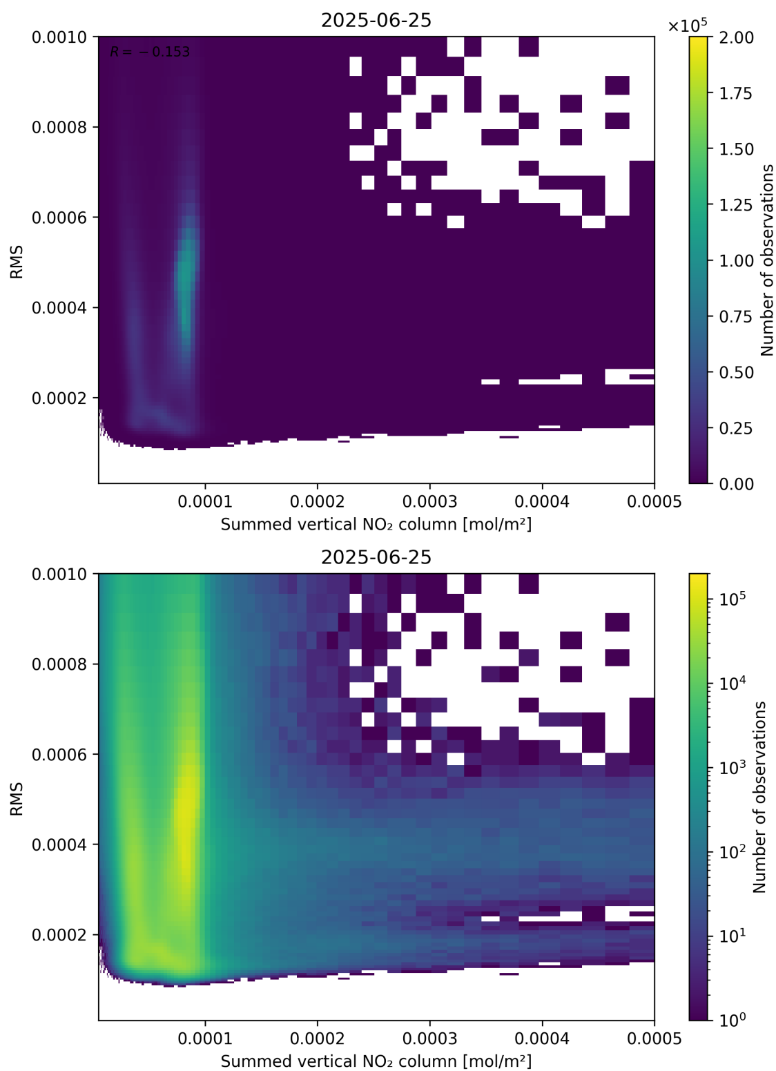
Figure 109: Scatter density plot of “Summed vertical NO 2 column” against “RMS” for 2025-06-24 to 2025-06-26.
