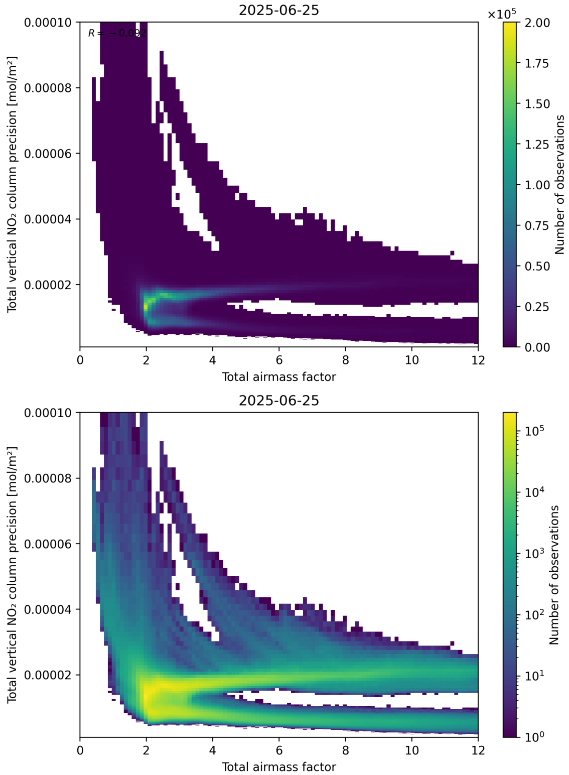
Figure 68: Scatter density plot of “Total airmass factor” against “Total vertical NO 2 column precision” for 2025-06-24 to 2025-06-26.
