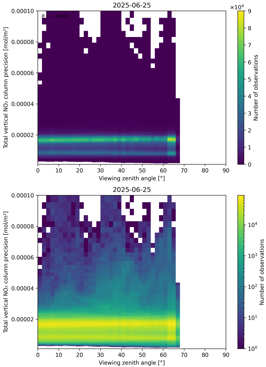
Figure 168: Scatter density plot of “Viewing zenith angle” against “Total vertical NO 2 column precision” for 2025-06-24 to 2025-06-26.
