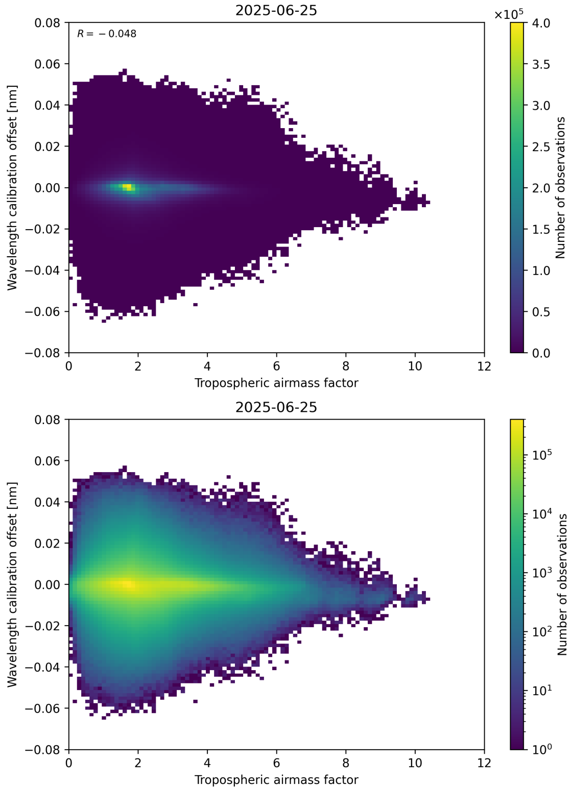
Figure 80: Scatter density plot of “Tropospheric airmass factor” against “Wavelength calibration offset” for 2025-06-24 to 2025-06-26.
