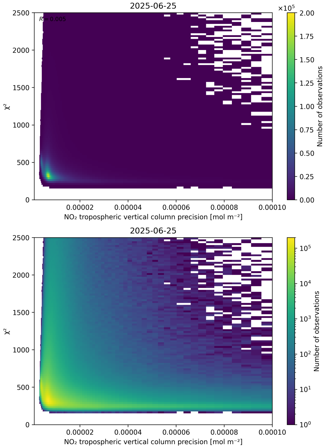
Figure 134: Scatter density plot of “NO 2 tropospheric vertical column precision” against “ \chi^2 ” for 2025-06-24 to 2025-06-26.
