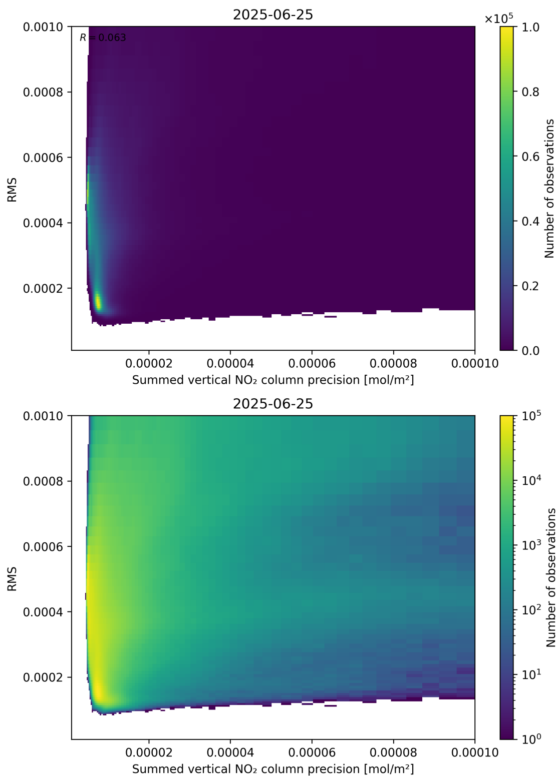
Figure 108: Scatter density plot of “Summed vertical NO 2 column precision” against “RMS” for 2025-06-24 to 2025-06-26.
