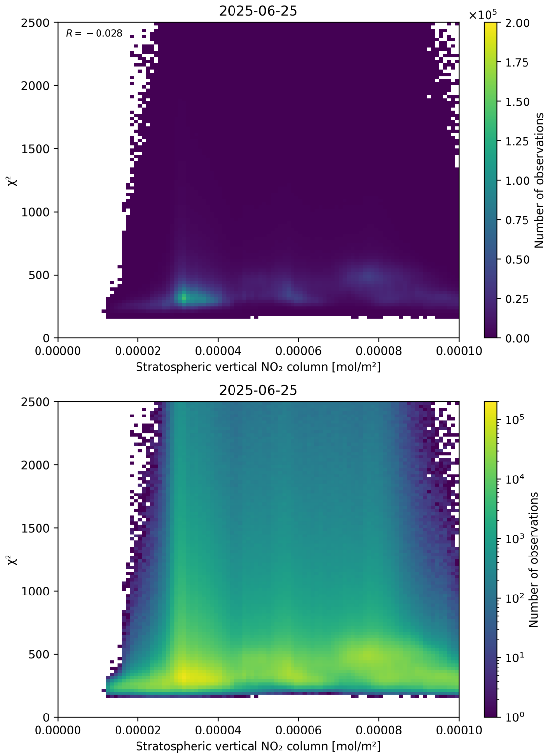
Figure 97: Scatter density plot of “Stratospheric vertical NO 2 column” against “ \chi^2 ” for 2025-06-24 to 2025-06-26.
