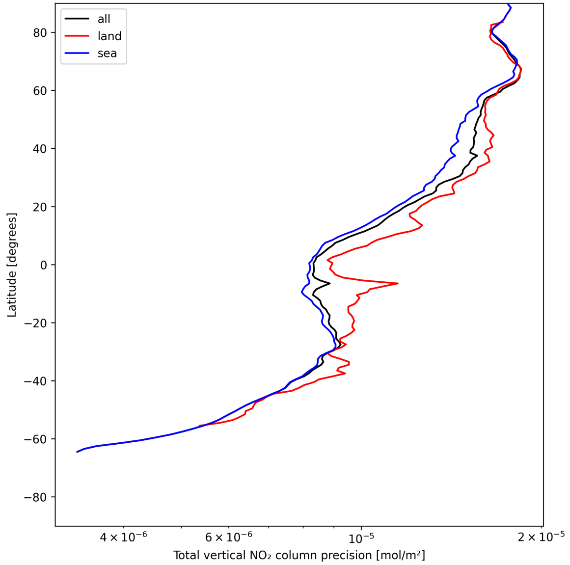
Figure 22: Zonal average of “Total vertical NO 2 column precision” for 2025-06-24 to 2025-06-26.
