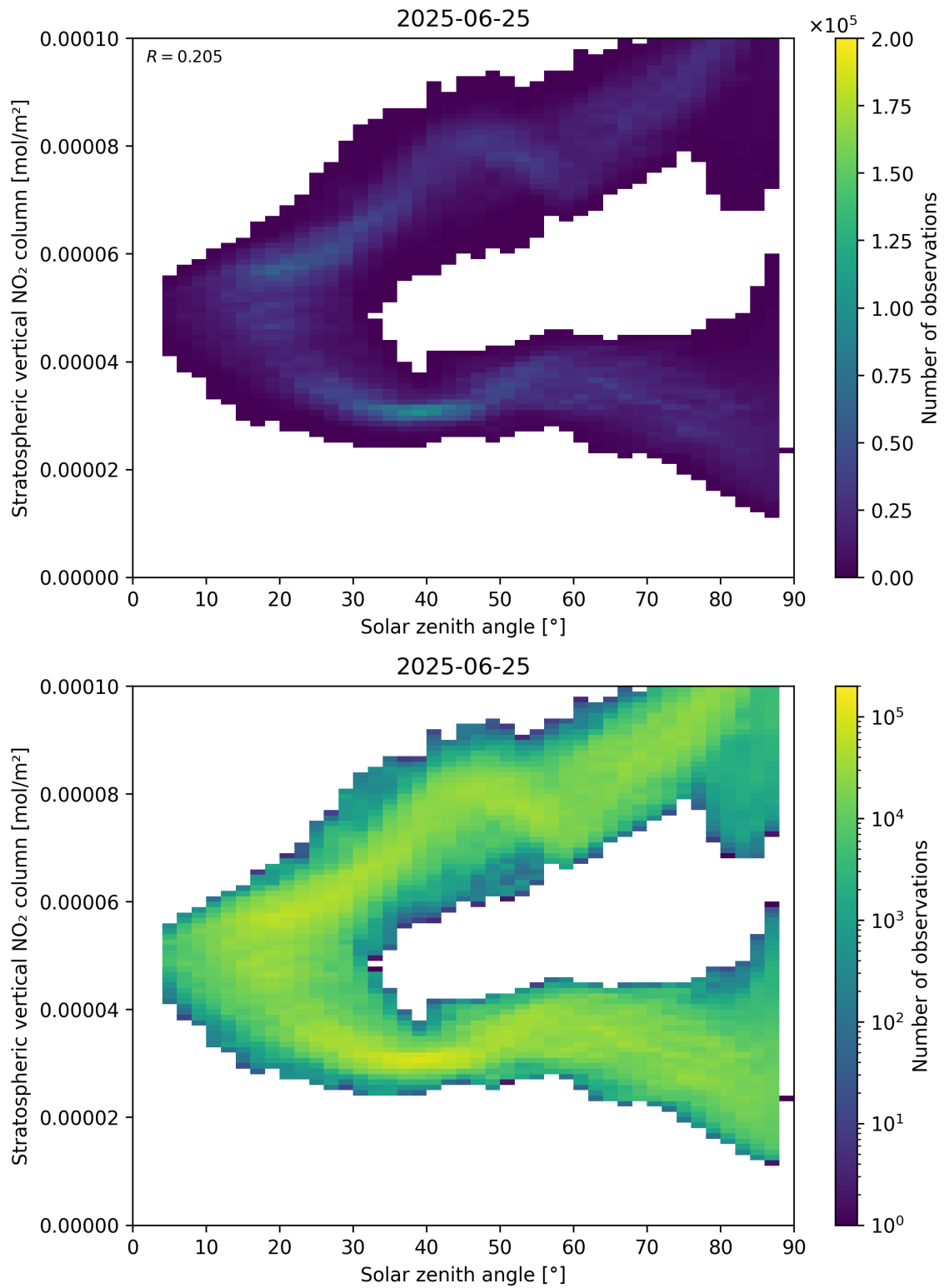
Figure 150: Scatter density plot of “Solar zenith angle” against “Stratospheric vertical NO 2 column” for 2025-06-24 to 2025-06-26.
