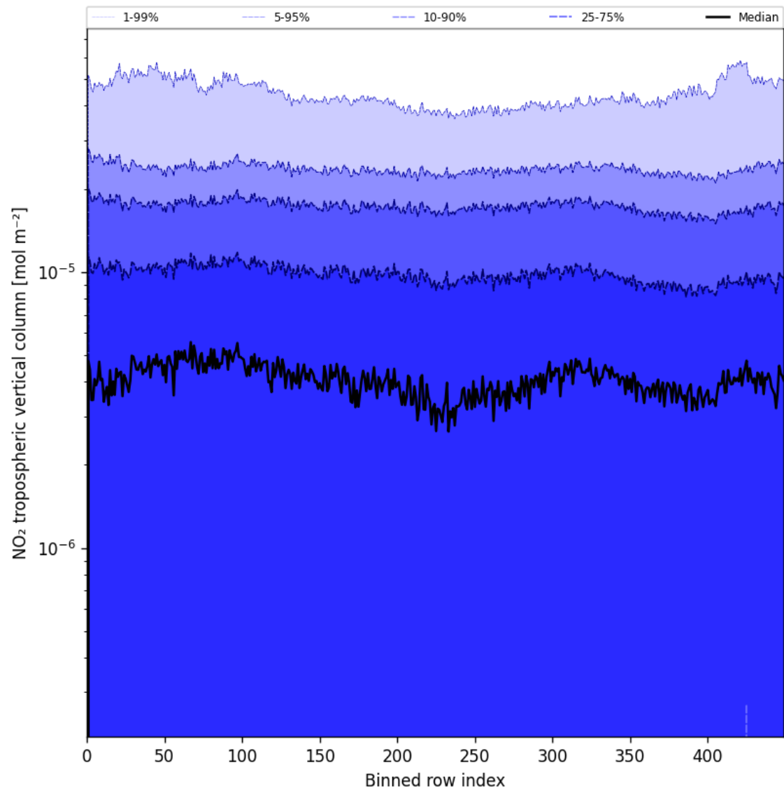
Figure 46: Along track statistics of “NO 2 tropospheric vertical column” for 2025-06-24 to 2025-06-26
