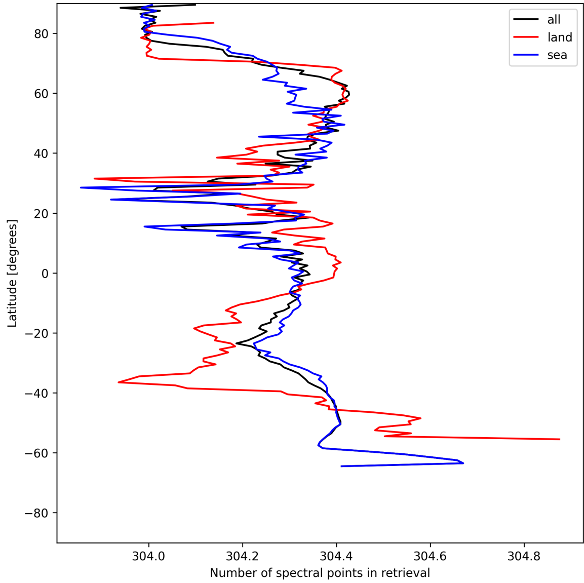
Figure 16: Zonal average of “Number of spectral points in retrieval” for 2025-06-24 to 2025-06-26.
