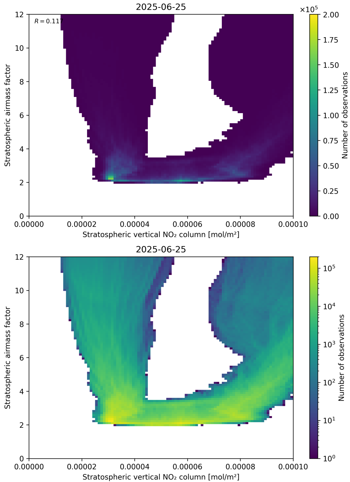
Figure 96: Scatter density plot of “Stratospheric vertical NO 2 column” against “Stratospheric airmass factor” for 2025-06-24 to 2025-06-26.
