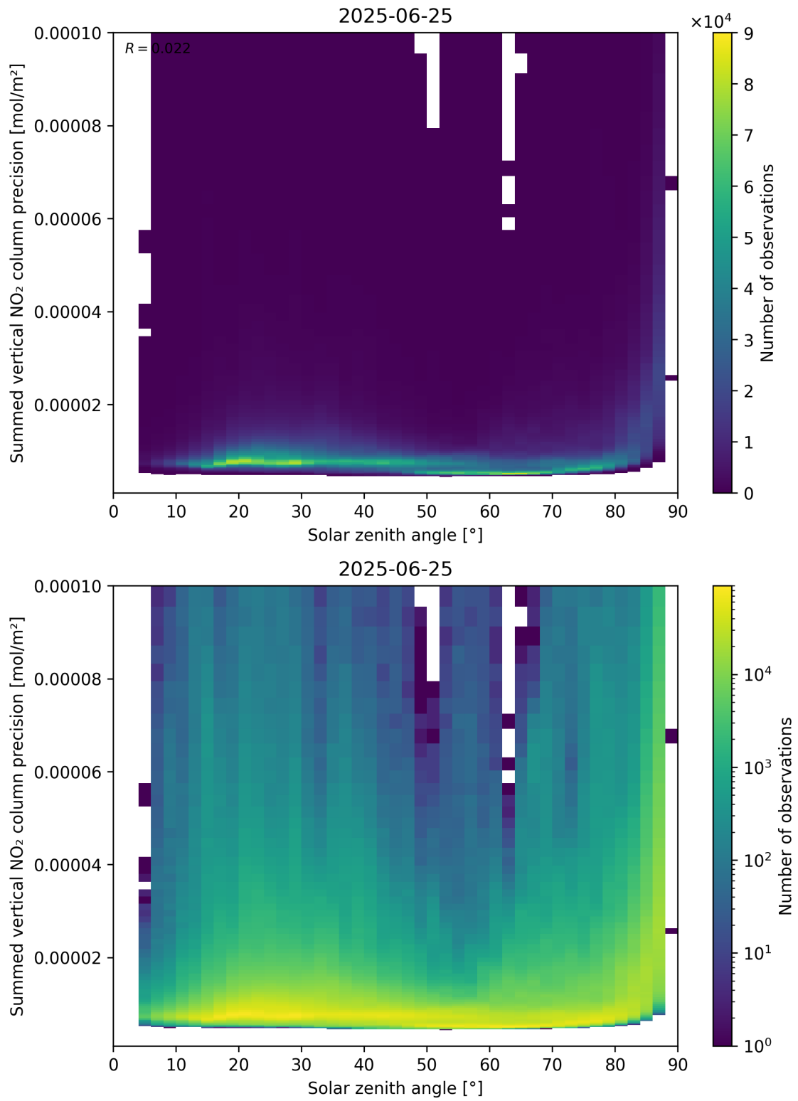
Figure 152: Scatter density plot of “Solar zenith angle” against “Summed vertical NO 2 column precision” for 2025-06-24 to 2025-06-26.
