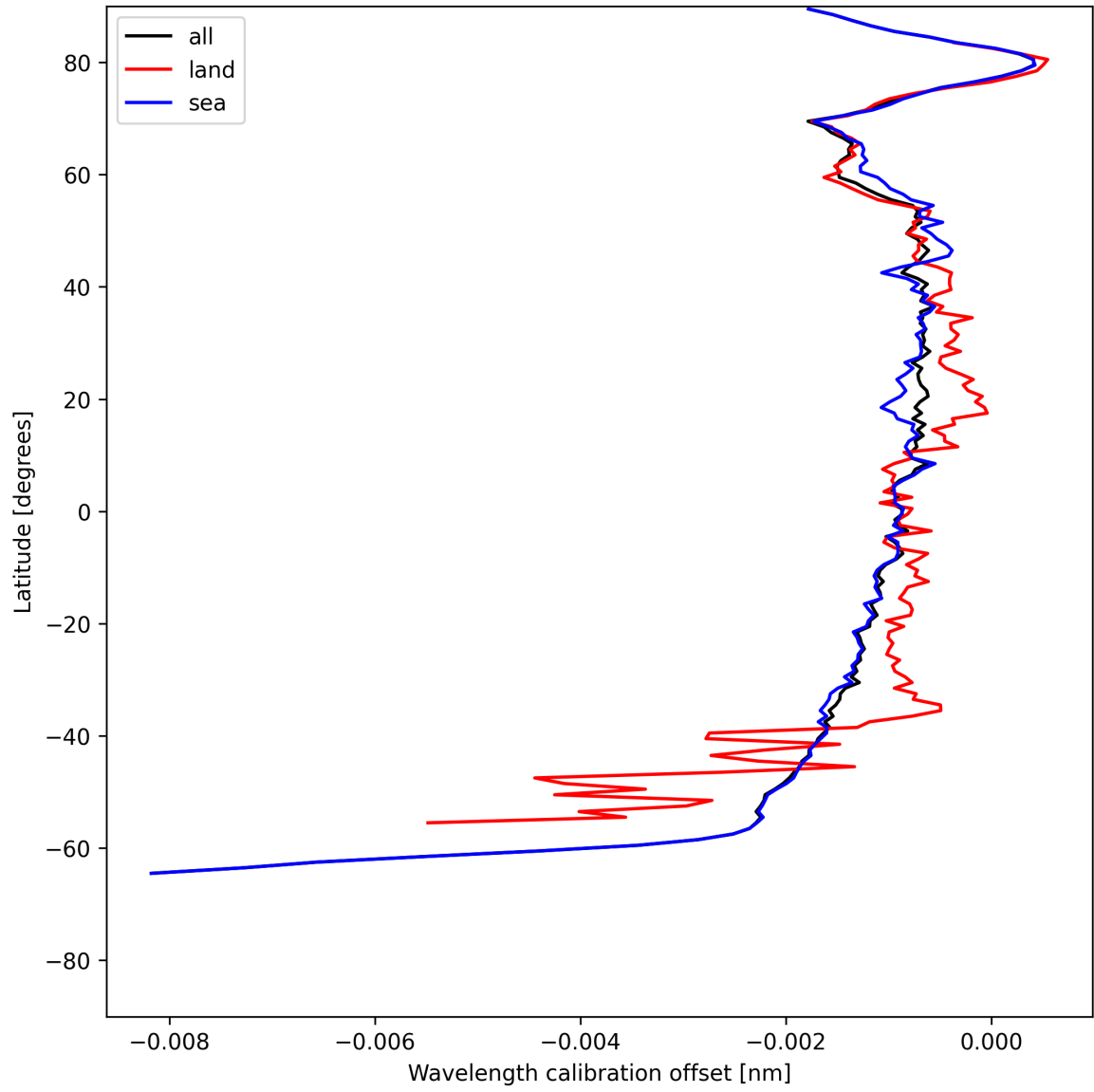
Figure 18: Zonal average of “Wavelength calibration offset” for 2025-06-24 to 2025-06-26.
