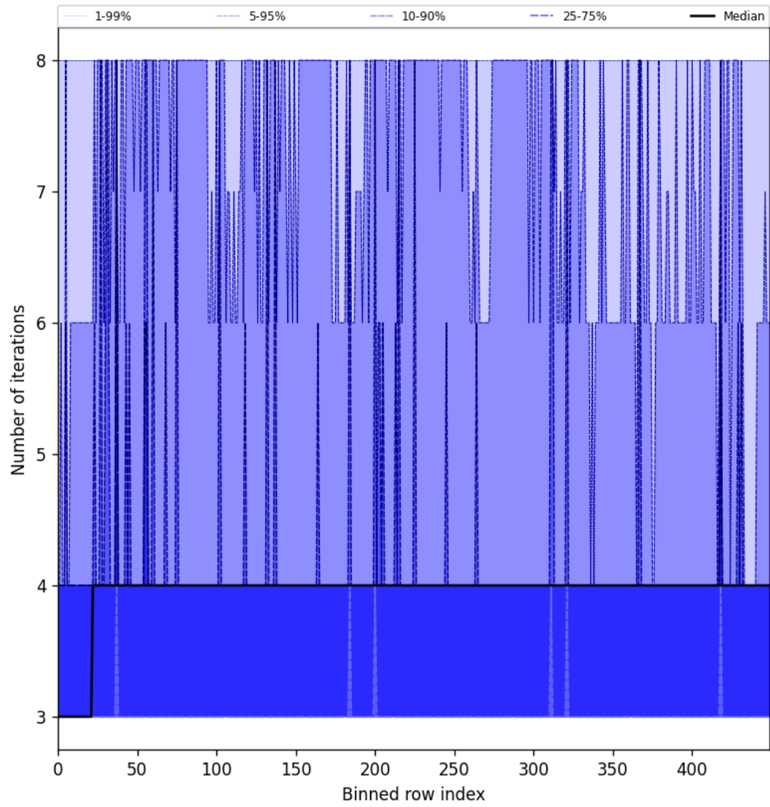
Figure 51: Along track statistics of “Number of iterations” for 2025-06-24 to 2025-06-26
