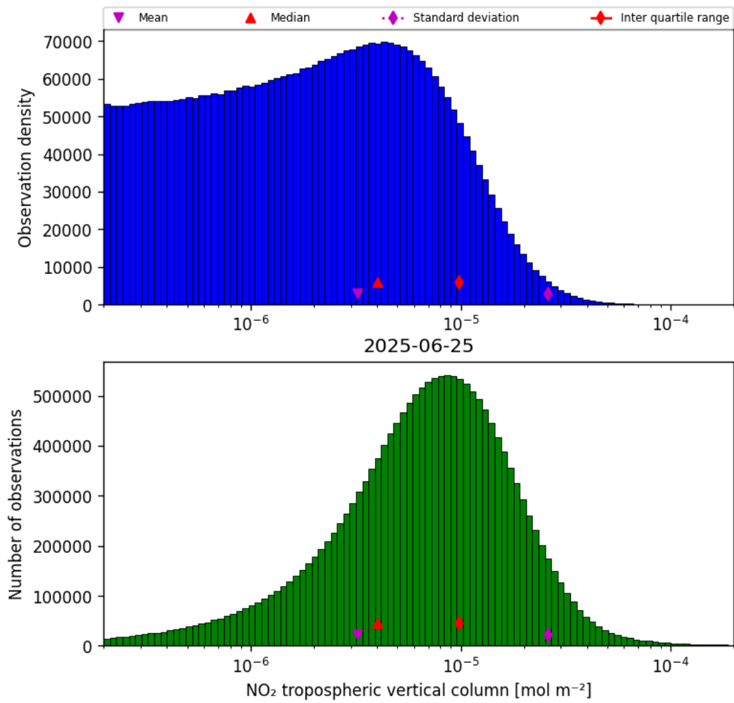
Figure 29: Histogram of “NO 2 tropospheric vertical column” for 2025-06-24 to 2025-06-26
