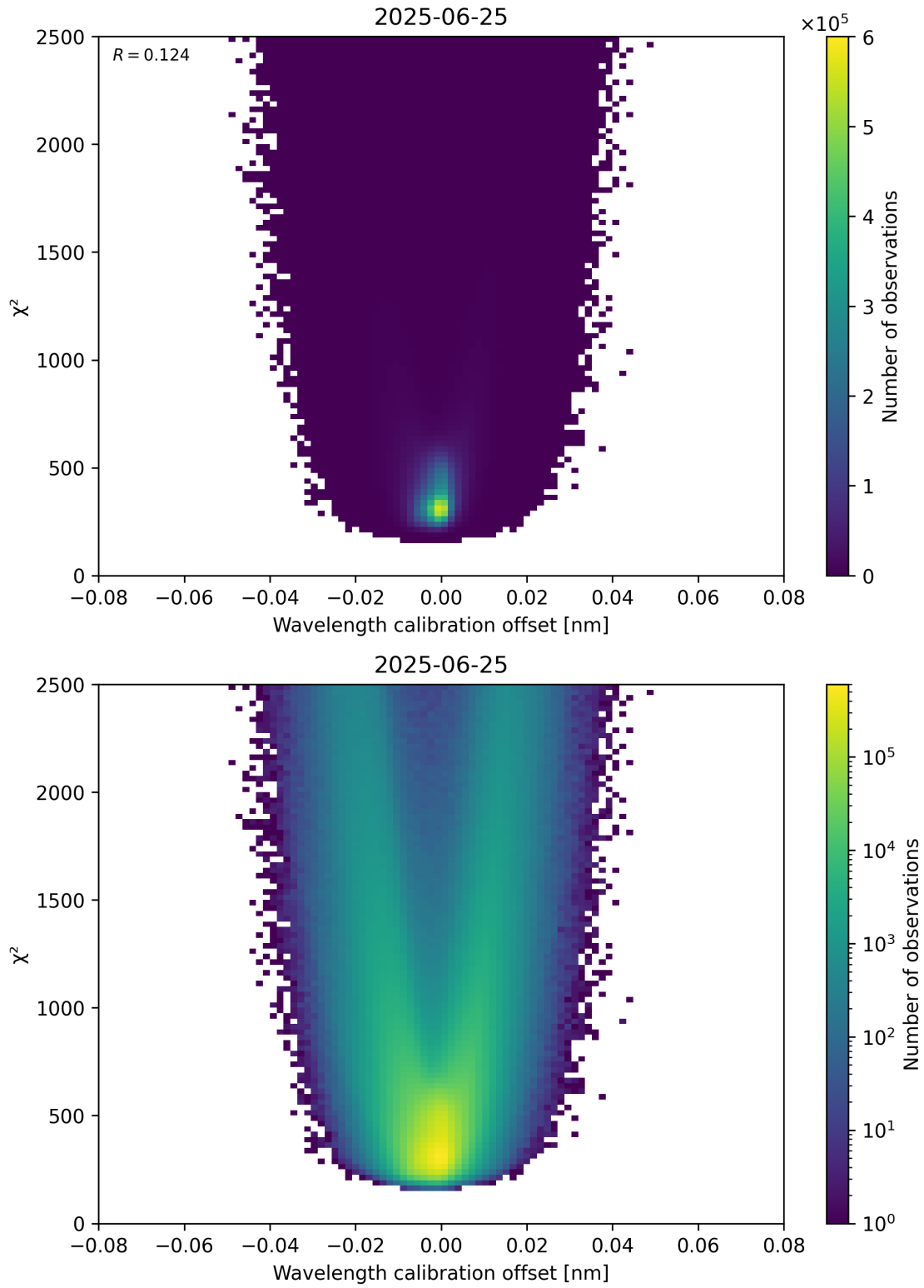
Figure 175: Scatter density plot of “Wavelength calibration offset” against “ \chi^2 ” for 2025-06-24 to 2025-06-26.
