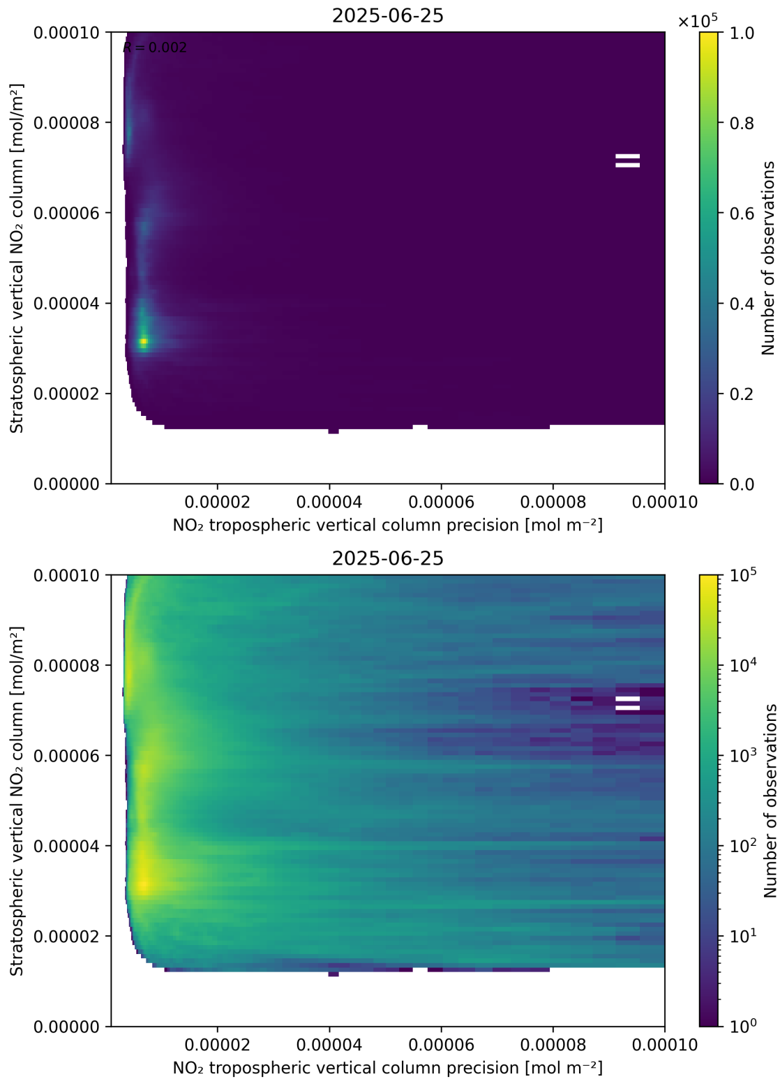
Figure 135: Scatter density plot of “NO 2 tropospheric vertical column precision” against “Stratospheric vertical NO 2 column” for 2025-06-24 to 2025-06-26.
