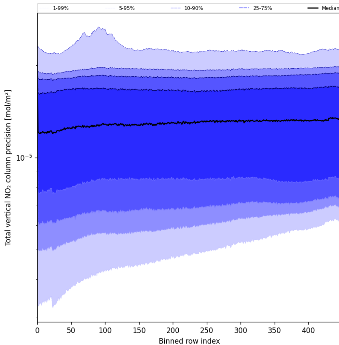
Figure 56: Along track statistics of “Total vertical NO 2 column precision” for 2025-06-24 to 2025-06-26
