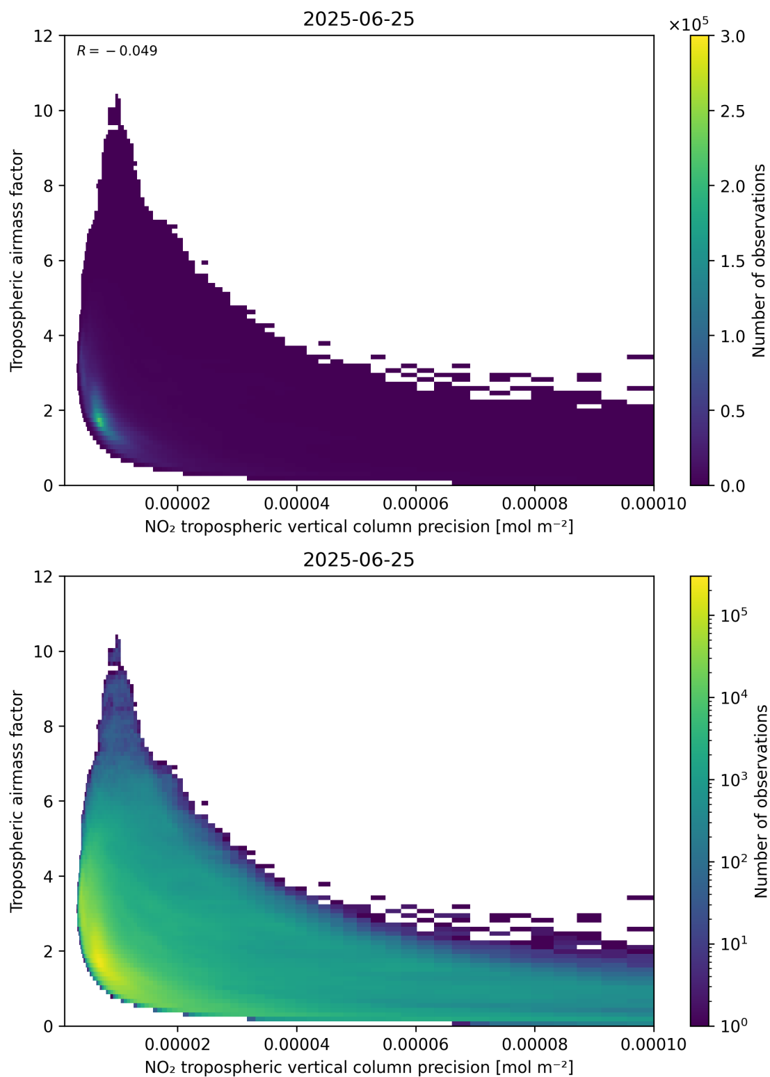
Figure 133: Scatter density plot of “NO 2 tropospheric vertical column precision” against “Tropospheric air mass factor” for 2025-06-24 to 2025-06-26.
