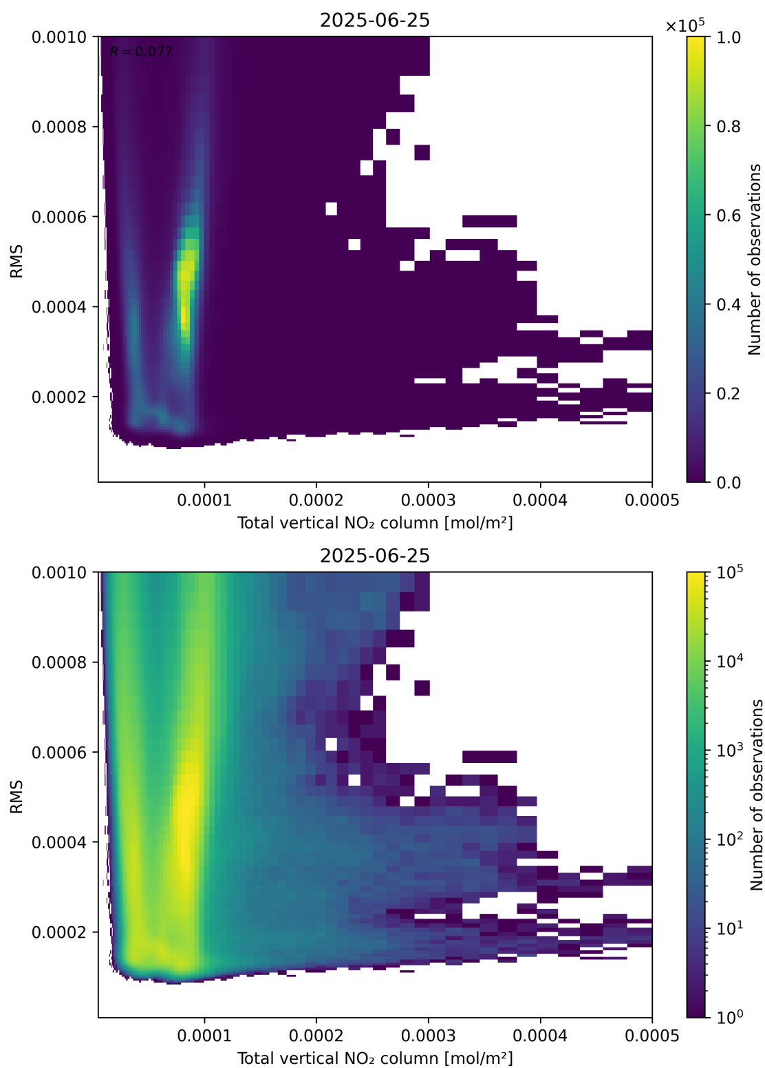
Figure 120: Scatter density plot of “Total vertical NO 2 column” against “RMS” for 2025-06-24 to 2025-06-26.
