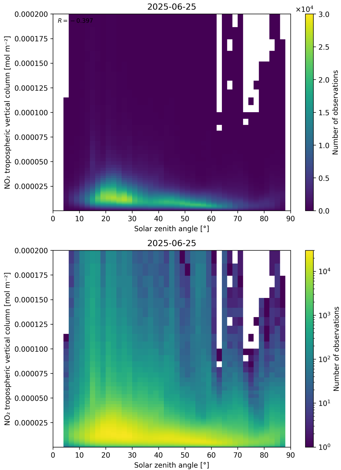
Figure 155: Scatter density plot of “Solar zenith angle” against “NO 2 tropospheric vertical column” for 2025-06-24 to 2025-06-26.
