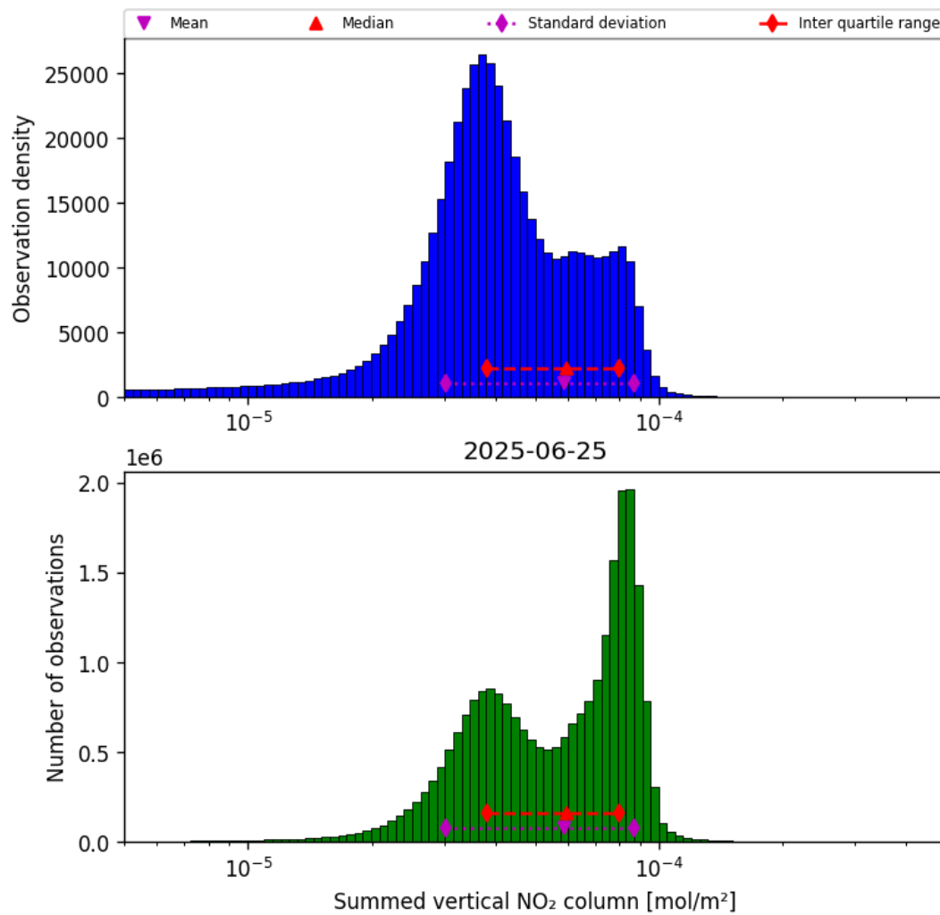
Figure 40: Histogram of “Summed vertical NO 2 column” for 2025-06-24 to 2025-06-26
