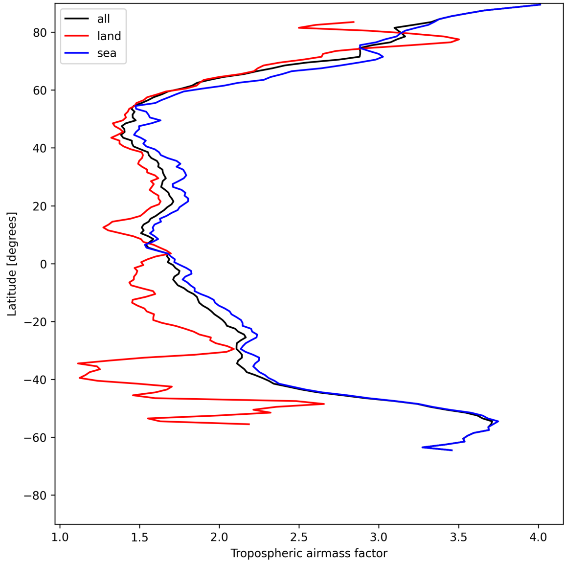
Figure 14: Zonal average of “Tropospheric airmass factor” for 2025-06-24 to 2025-06-26.
