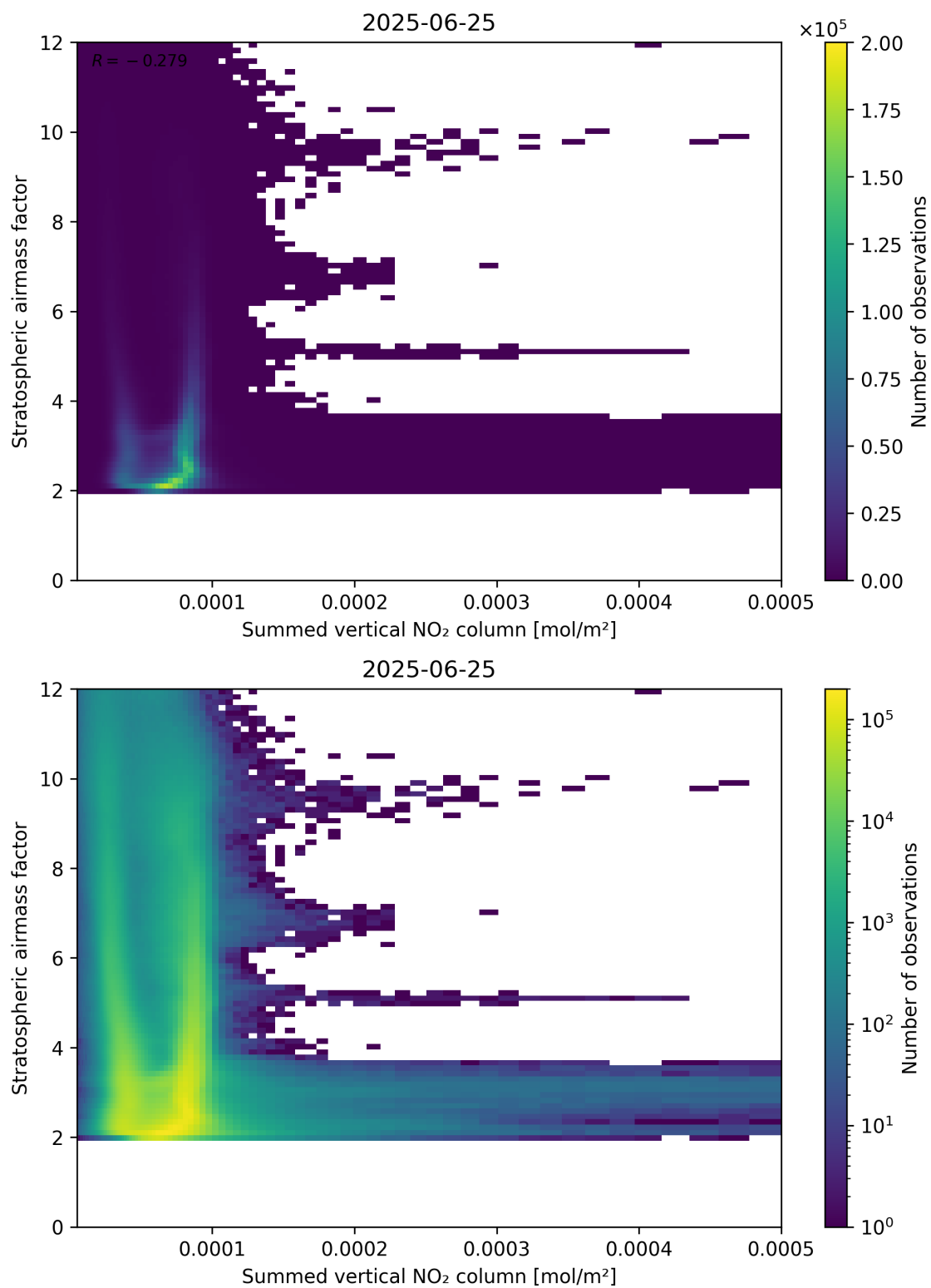
Figure 103: Scatter density plot of “Summed vertical NO 2 column” against “Stratospheric airmass factor” for 2025-06-24 to 2025-06-26.
