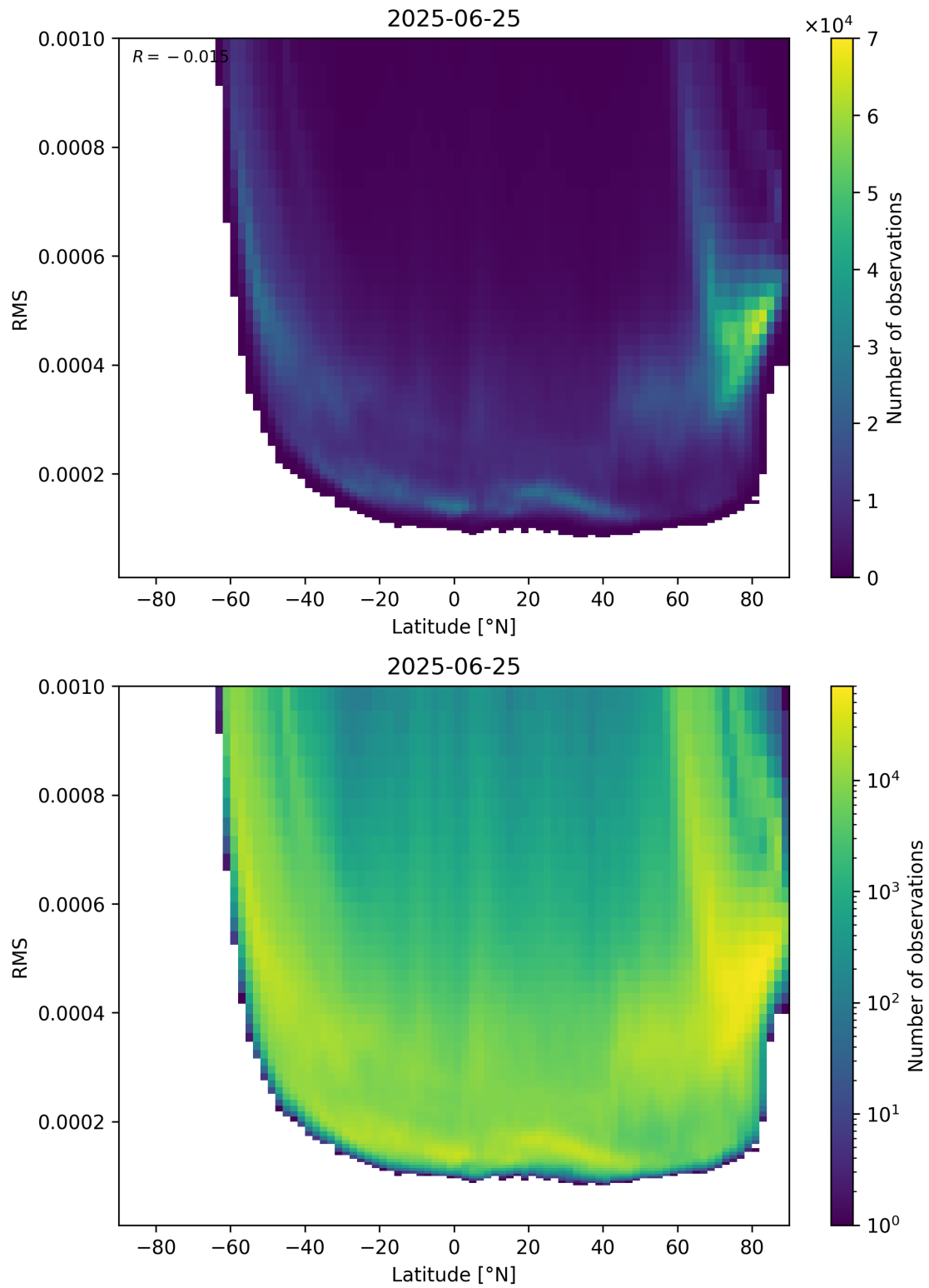
Figure 94: Scatter density plot of “Latitude” against “RMS” for 2025-06-24 to 2025-06-26.
