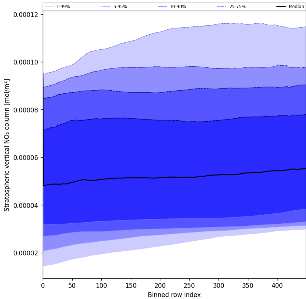
Figure 53: Along track statistics of “Stratospheric vertical NO 2 column” for 2025-06-24 to 2025-06-26
