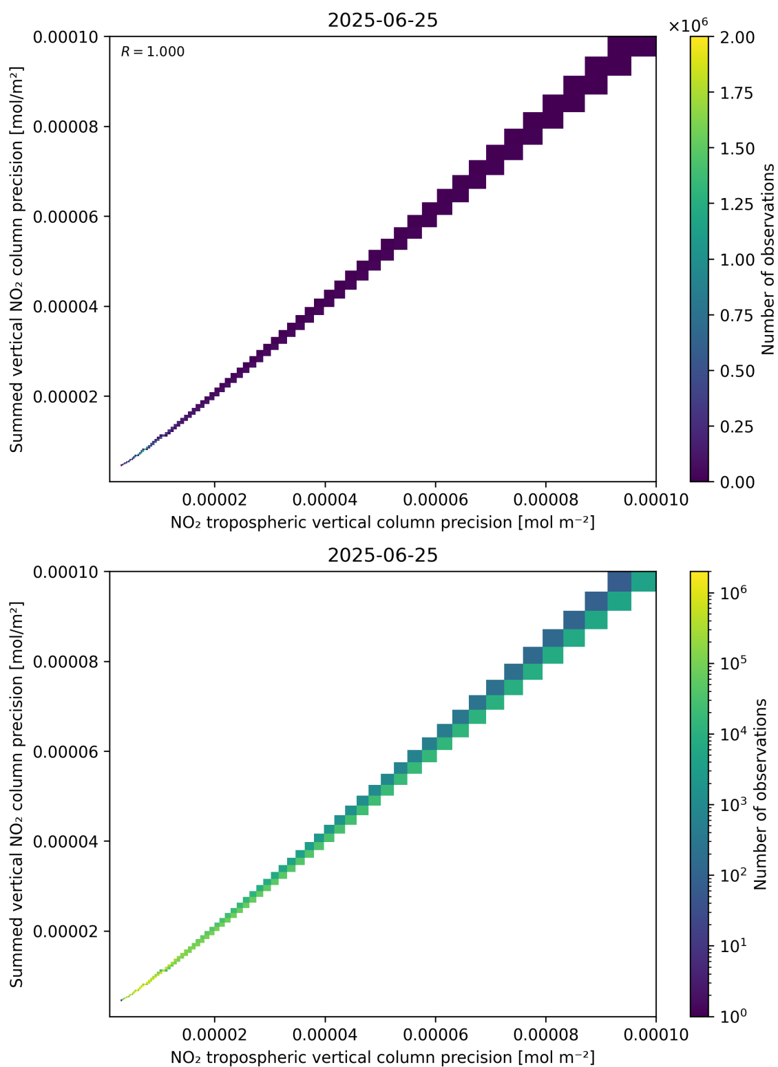
Figure 137: Scatter density plot of “NO 2 tropospheric vertical column precision” against “Summed vertical NO 2 column precision” for 2025-06-24 to 2025-06-26.
