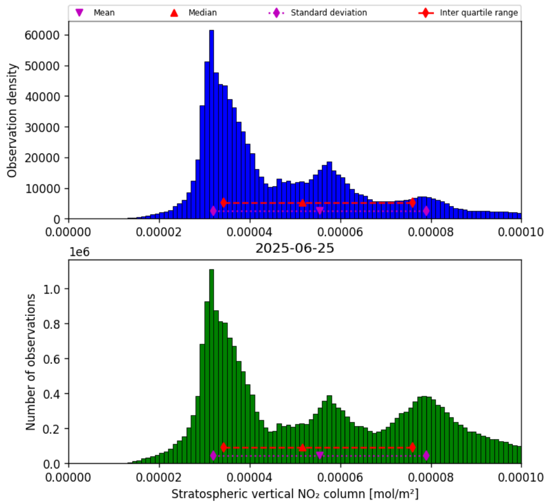
Figure 36: Histogram of “Stratospheric vertical NO 2 column” for 2025-06-24 to 2025-06-26
