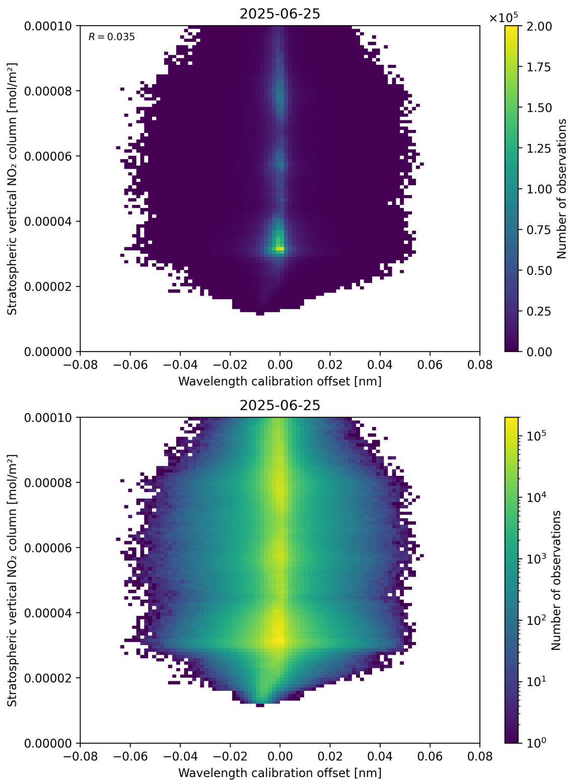
Figure 176: Scatter density plot of “Wavelength calibration offset” against “Stratospheric vertical NO 2 column” for 2025-06-24 to 2025-06-26.
