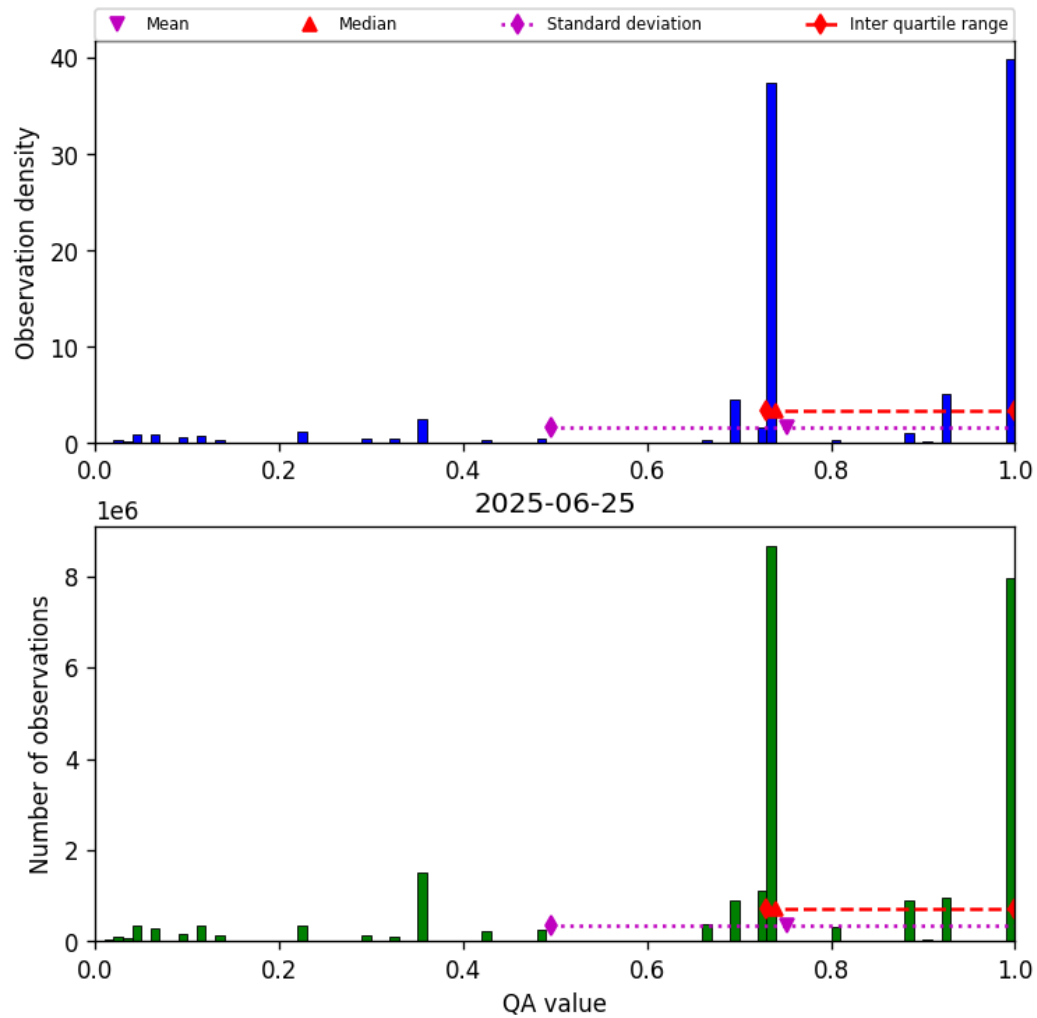
Figure 28: Histogram of “QA value” for 2025-06-24 to 2025-06-26
