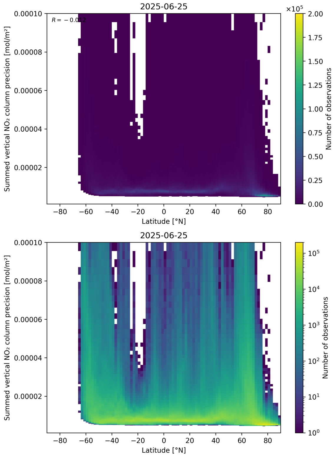
Figure 89: Scatter density plot of “Latitude” against “Summed vertical NO 2 column precision” for 2025-06-24 to 2025-06-26.
