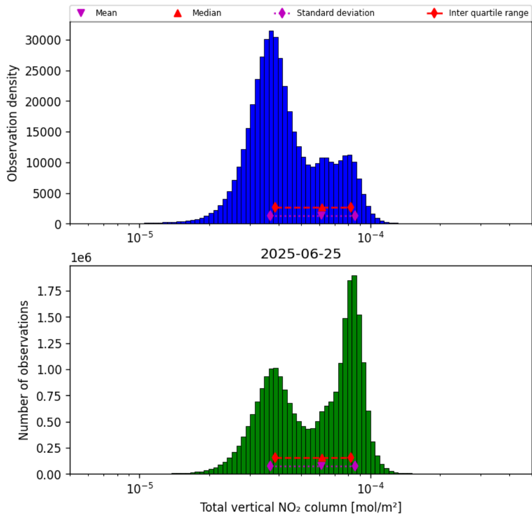
Figure 38: Histogram of “Total vertical NO 2 column” for 2025-06-24 to 2025-06-26
