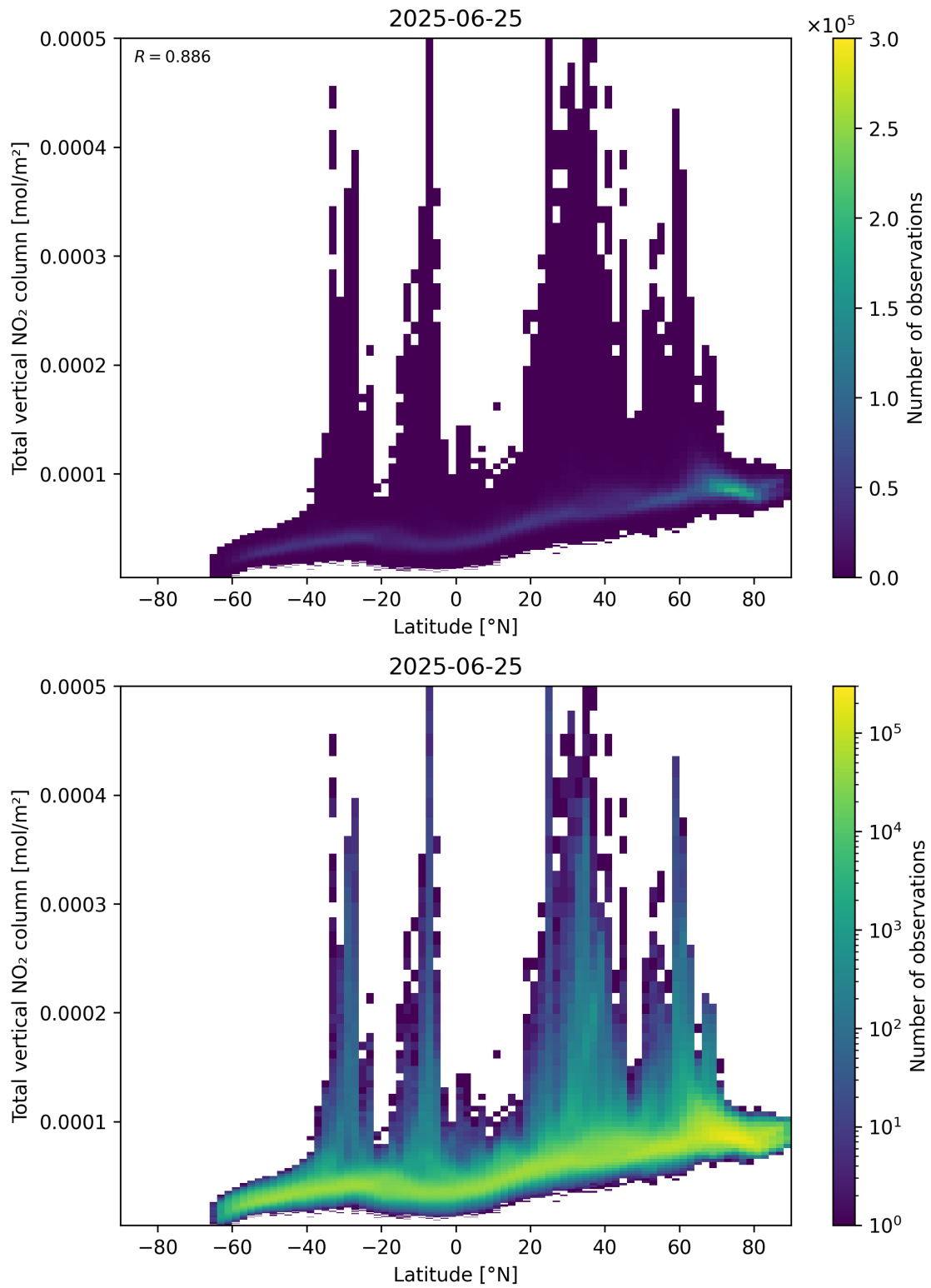
Figure 90: Scatter density plot of “Latitude” against “Total vertical NO 2 column” for 2025-06-24 to 2025-06-26.
