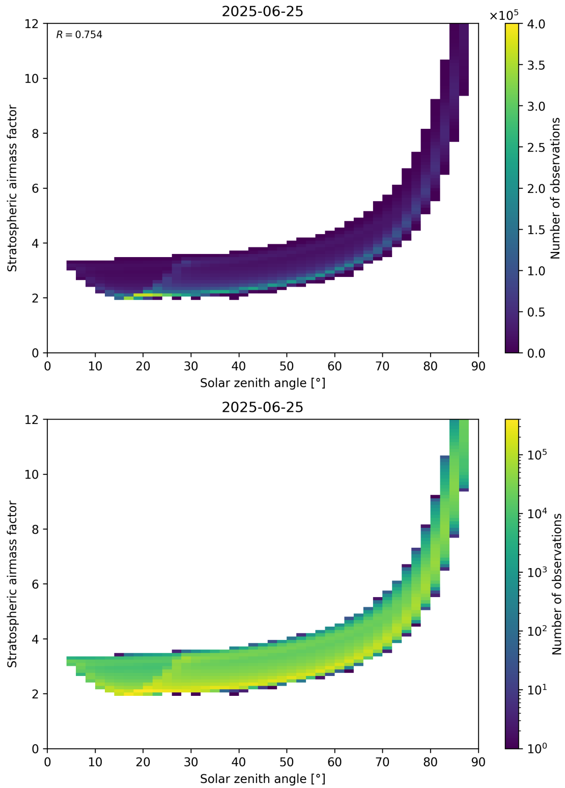
Figure 145: Scatter density plot of “Solar zenith angle” against “Stratospheric airmass factor” for 2025-06-24 to 2025-06-26.
