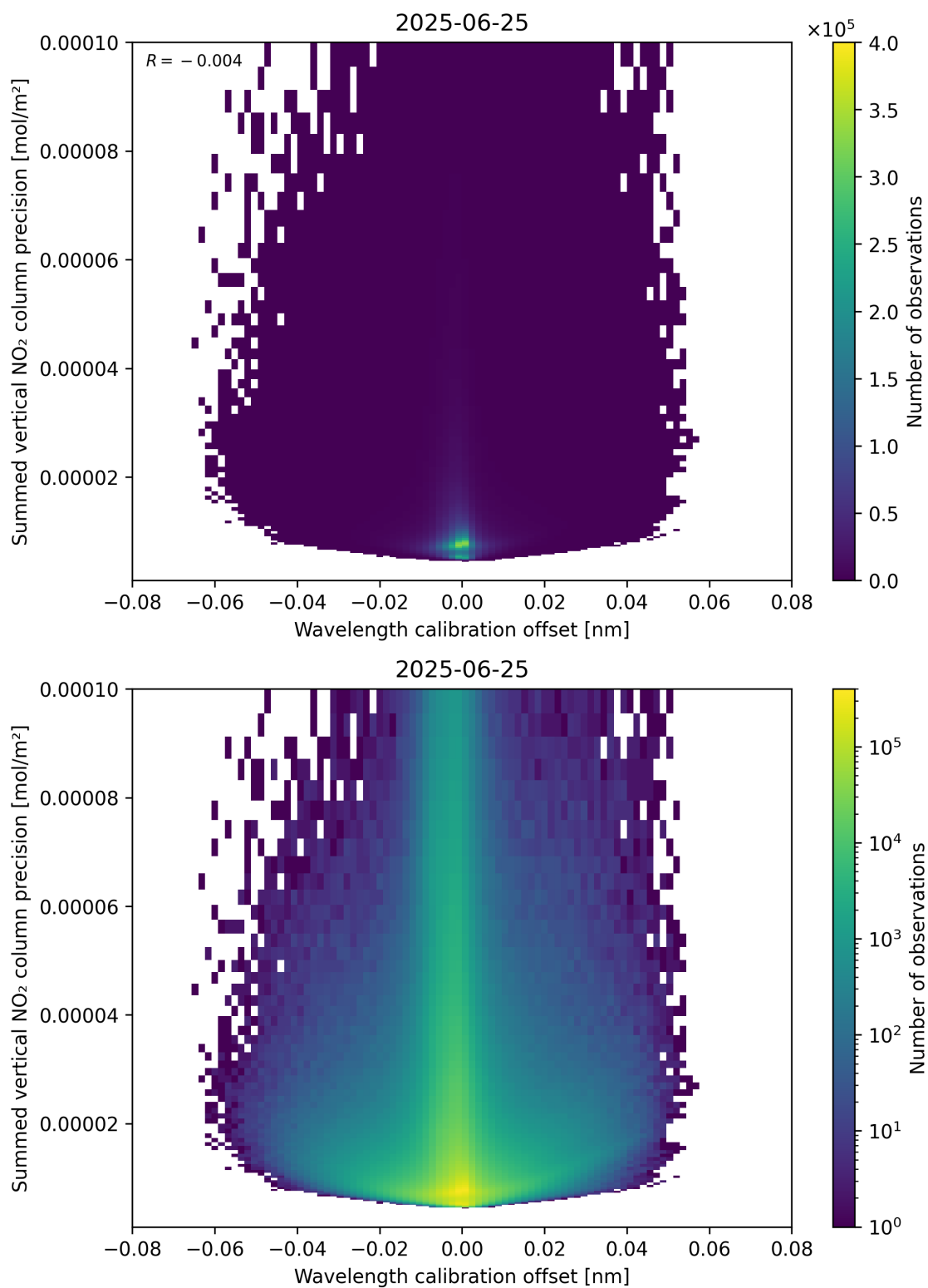
Figure 178: Scatter density plot of “Wavelength calibration offset” against “Summed vertical NO 2 column precision” for 2025-06-24 to 2025-06-26.
