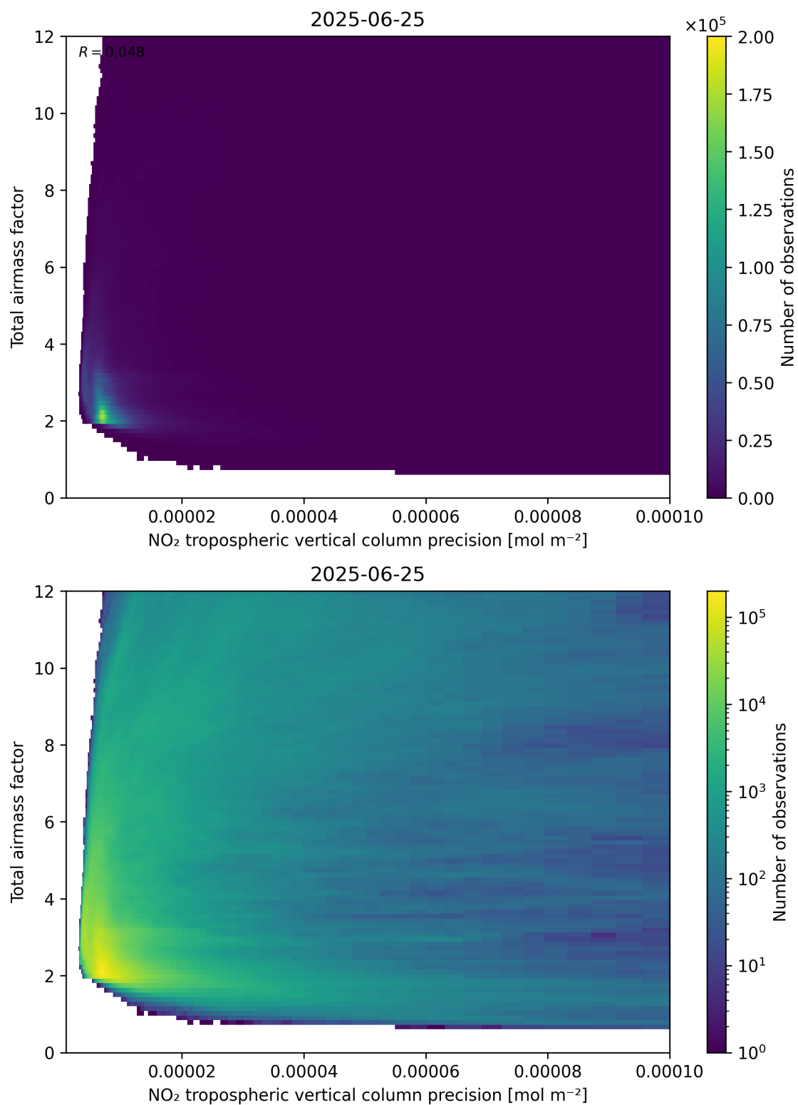
Figure 132: Scatter density plot of “NO 2 tropospheric vertical column precision” against “Total air mass factor” for 2025-06-24 to 2025-06-26.
