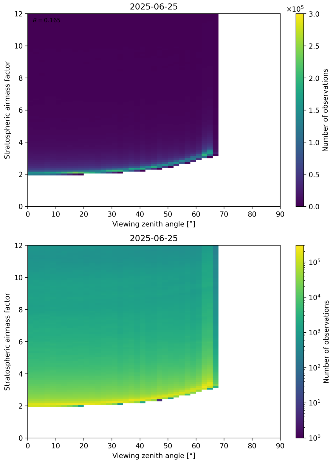
Figure 159: Scatter density plot of “Viewing zenith angle” against “Stratospheric airmass factor” for 2025-06-24 to 2025-06-26.
