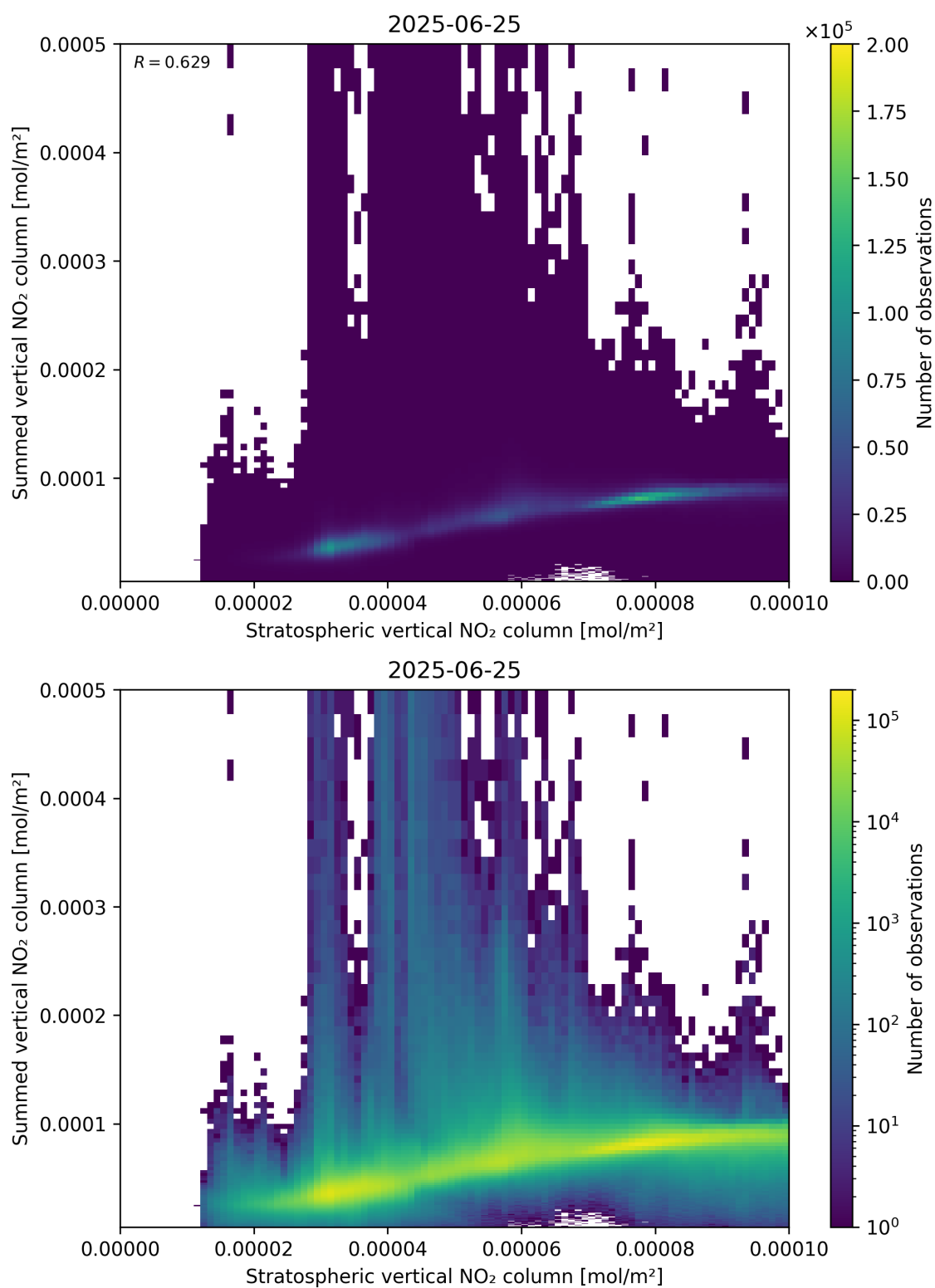
Figure 98: Scatter density plot of “Stratospheric vertical NO 2 column” against “Summed vertical NO 2 column” for 2025-06-24 to 2025-06-26.
