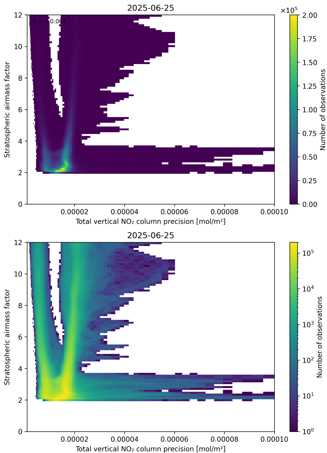
Figure 115: Scatter density plot of “Total vertical NO 2 column precision” against “Stratospheric airmass factor” for 2025-06-24 to 2025-06-26.
