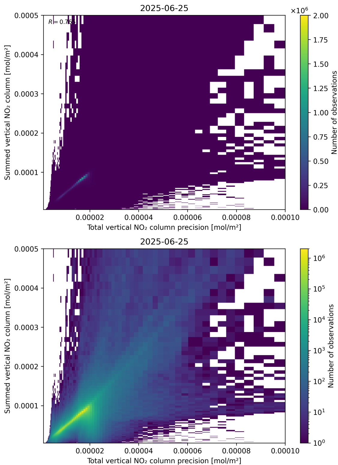
Figure 117: Scatter density plot of “Total vertical NO 2 column precision” against “Summed vertical NO 2 column” for 2025-06-24 to 2025-06-26.
