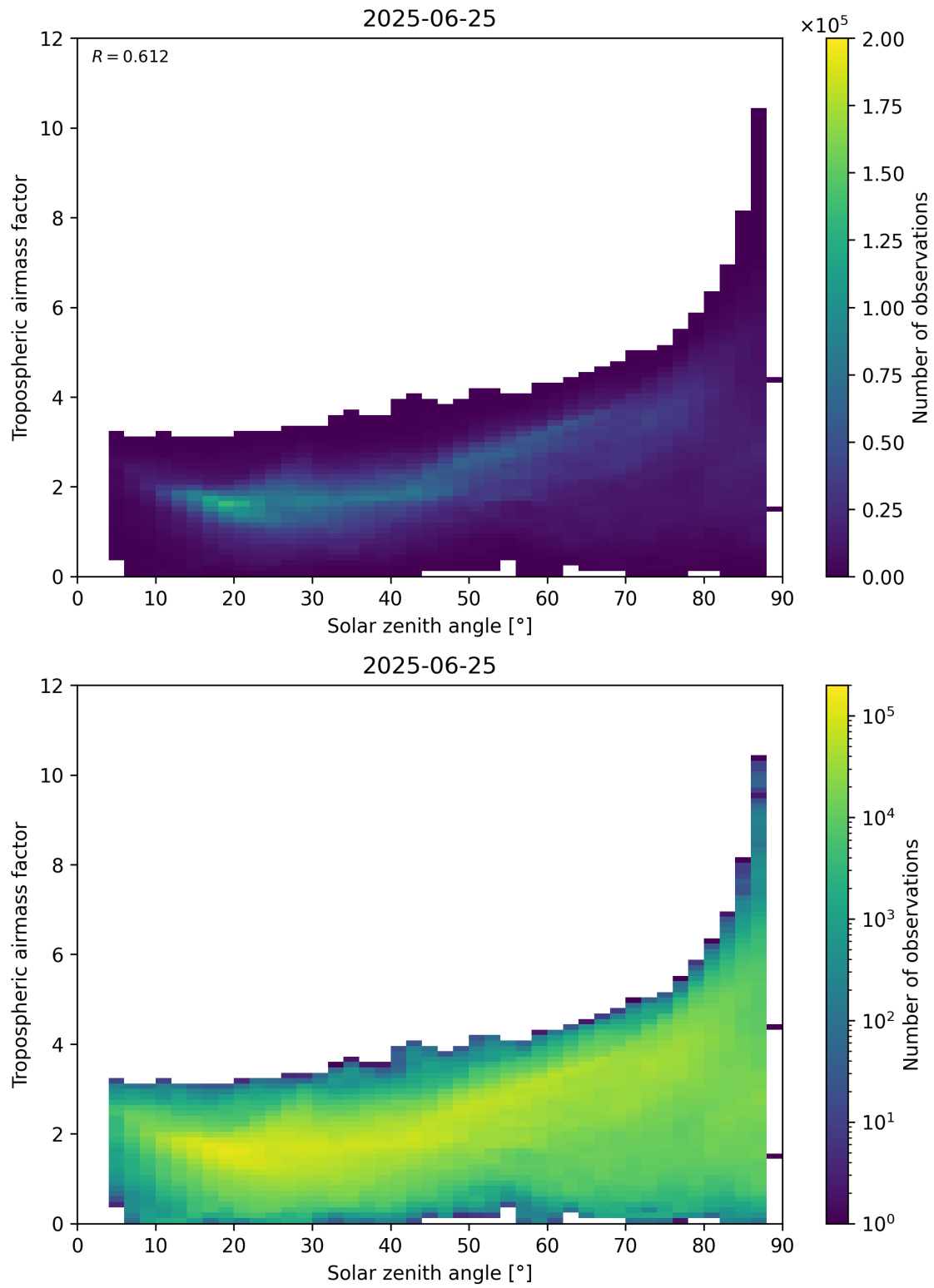
Figure 147: Scatter density plot of “Solar zenith angle” against “Tropospheric airmass factor” for 2025-06-24 to 2025-06-26.
