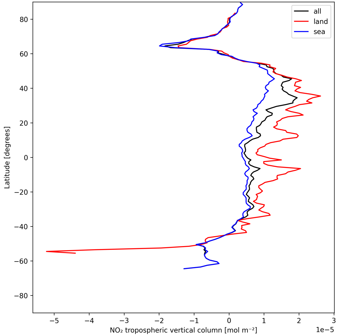
Figure 12: Zonal average of “NO 2 tropospheric vertical column” for 2025-06-24 to 2025-06-26.
