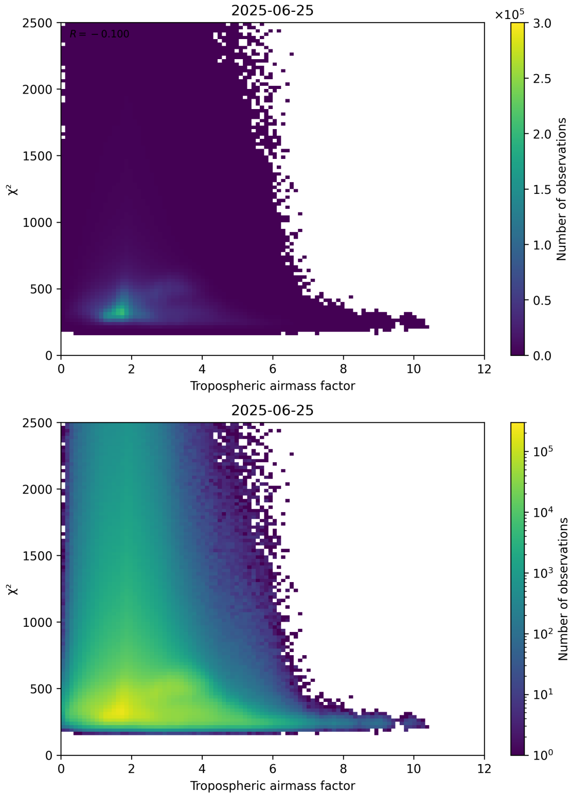
Figure 73: Scatter density plot of “Tropospheric airmass factor” against “ \chi^2 ” for 2025-06-24 to 2025-06-26.
