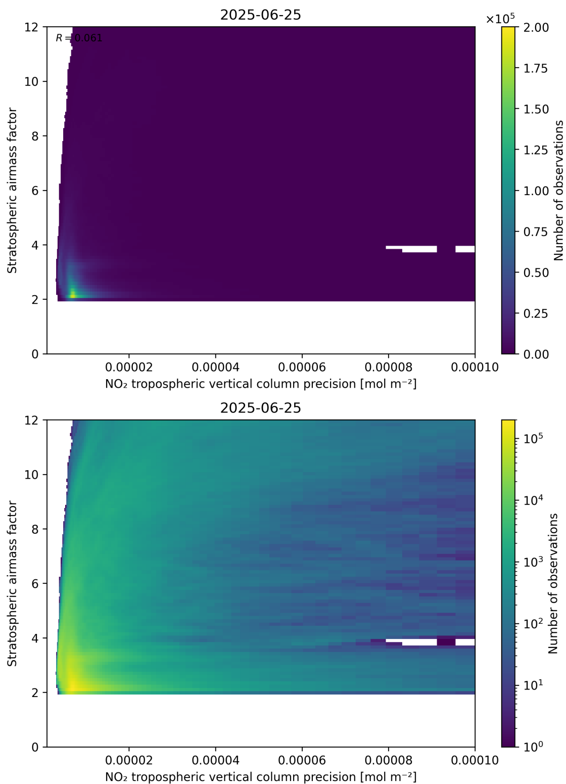
Figure 131: Scatter density plot of “NO 2 tropospheric vertical column precision” against “Stratospheric airmass factor” for 2025-06-24 to 2025-06-26.
