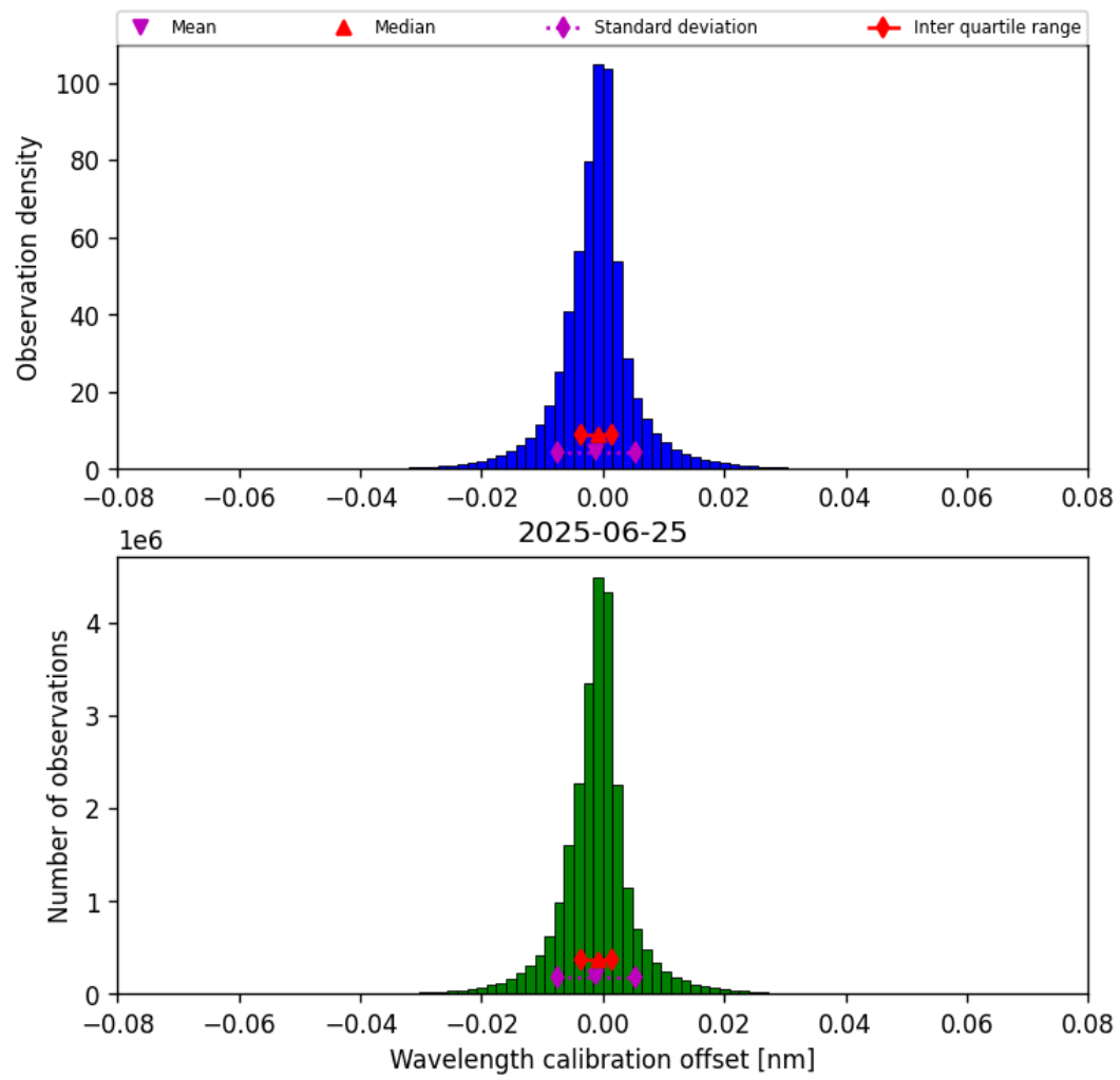
Figure 35: Histogram of “Wavelength calibration offset” for 2025-06-24 to 2025-06-26
