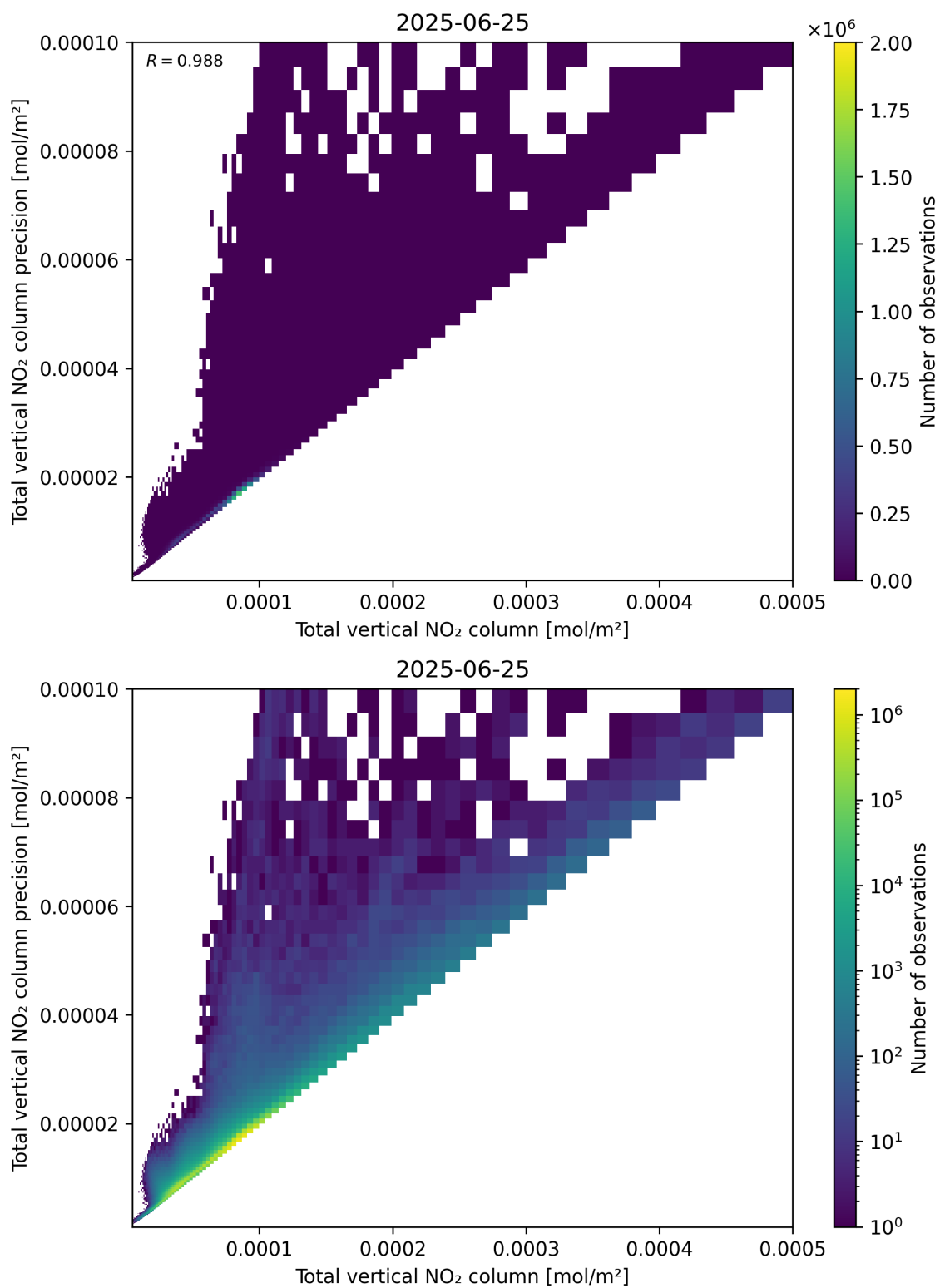
Figure 114: Scatter density plot of “Total vertical NO 2 column” against “Total vertical NO 2 column precision” for 2025-06-24 to 2025-06-26.
