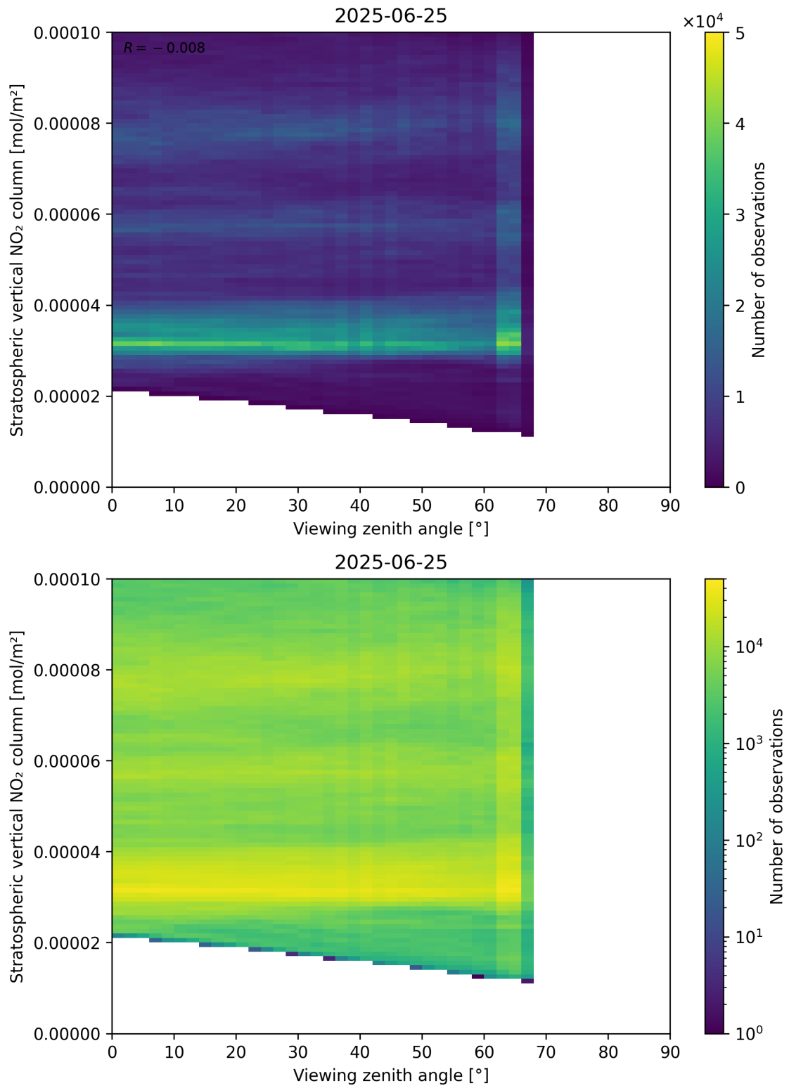
Figure 164: Scatter density plot of “Viewing zenith angle” against “Stratospheric vertical NO 2 column” for 2025-06-24 to 2025-06-26.
