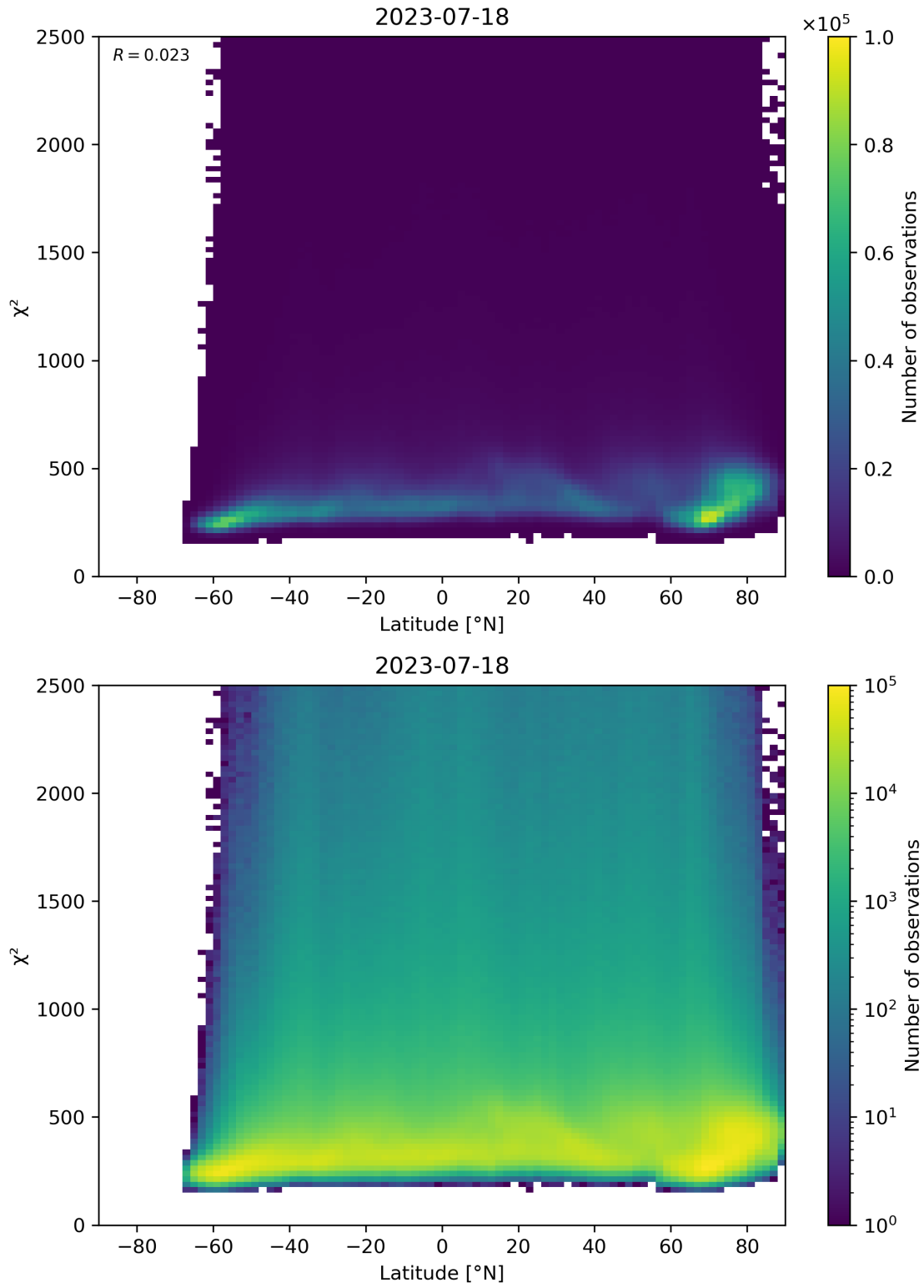
Figure 86: Scatter density plot of “Latitude” against “ \chi^2 ” for 2023-07-17 to 2023-07-19.
