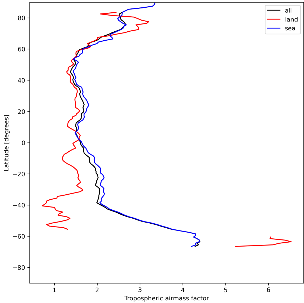
Figure 14: Zonal average of “Tropospheric airmass factor” for 2023-07-17 to 2023-07-19.
