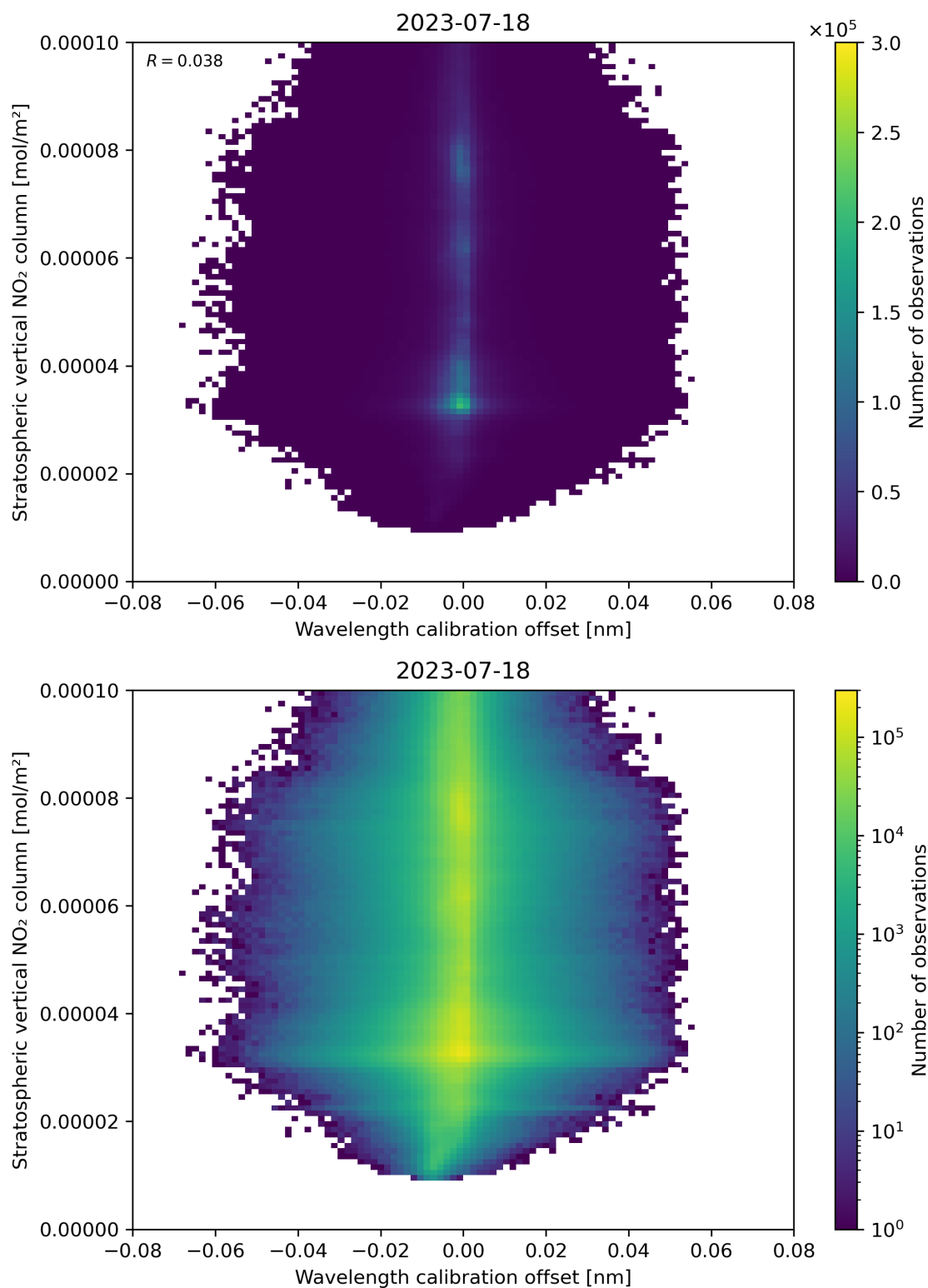
Figure 176: Scatter density plot of “Wavelength calibration offset” against “Stratospheric vertical NO 2 column” for 2023-07-17 to 2023-07-19.
