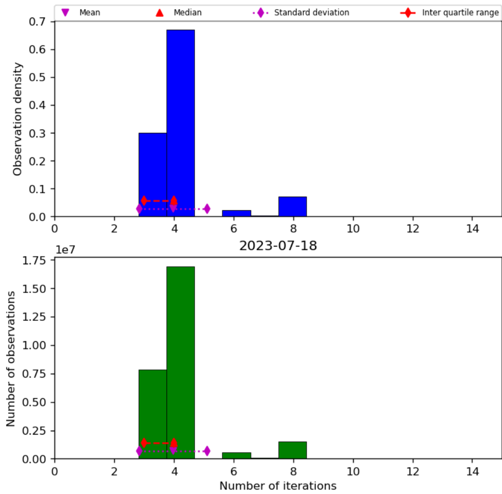
Figure 34: Histogram of “Number of iterations” for 2023-07-17 to 2023-07-19
