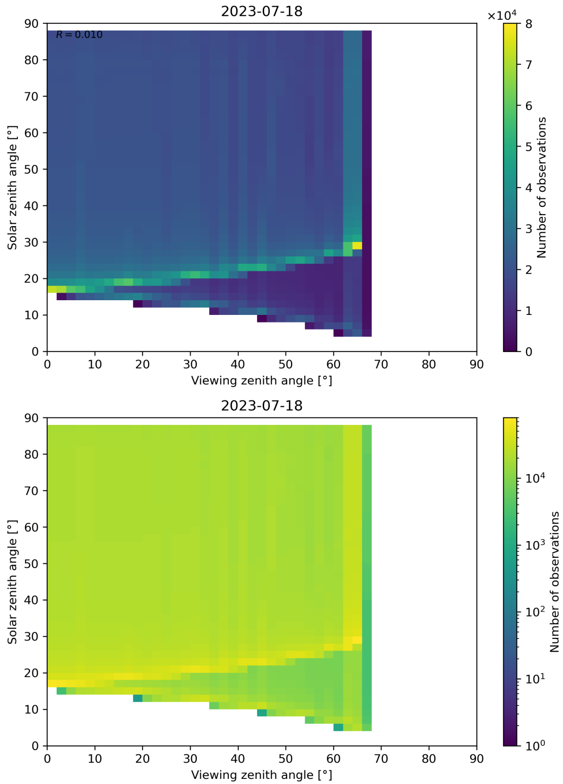
Figure 172: Scatter density plot of “Viewing zenith angle” against “Solar zenith angle” for 2023-07-17 to 2023-07-19.
