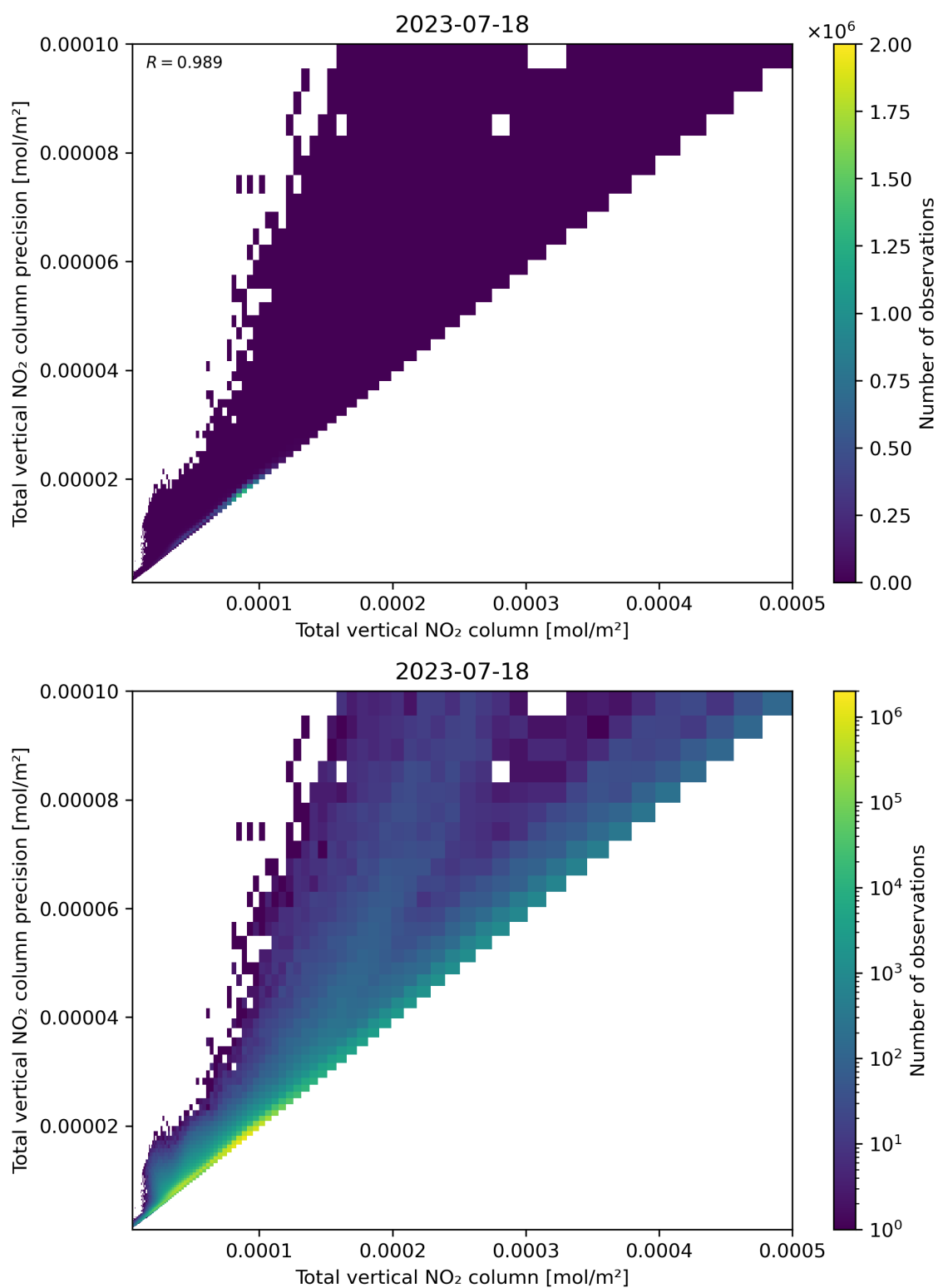
Figure 114: Scatter density plot of “Total vertical NO 2 column” against “Total vertical NO 2 column precision” for 2023-07-17 to 2023-07-19.
