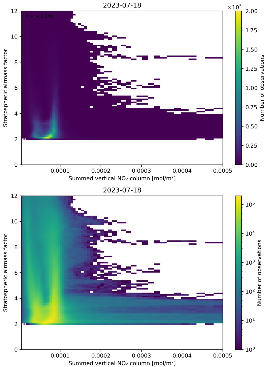
Figure 103: Scatter density plot of “Summed vertical NO 2 column” against “Stratospheric airmass factor” for 2023-07-17 to 2023-07-19.
