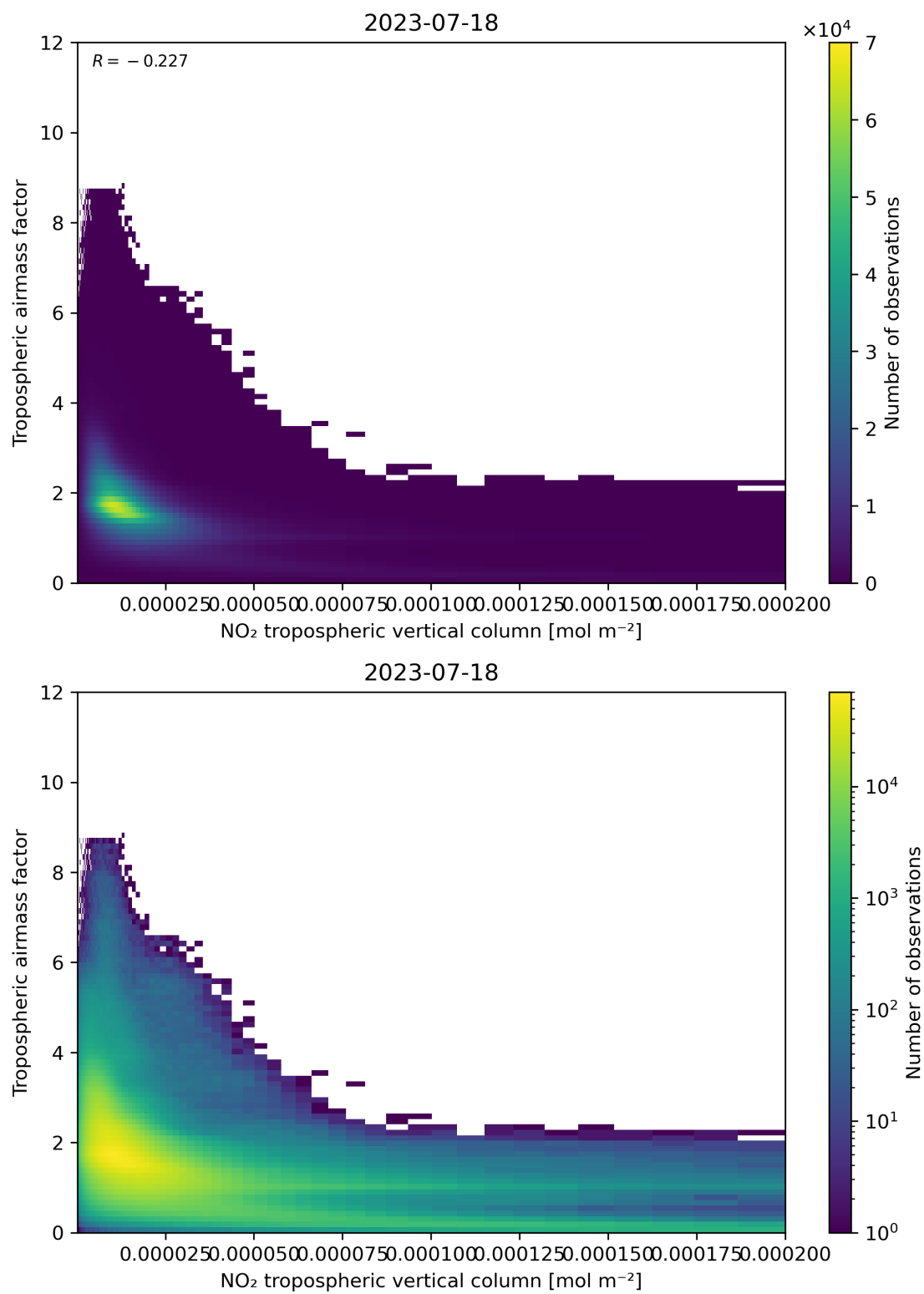
Figure 123: Scatter density plot of “NO 2 tropospheric vertical column” against “Tropospheric air mass factor” for 2023-07-17 to 2023-07-19.
