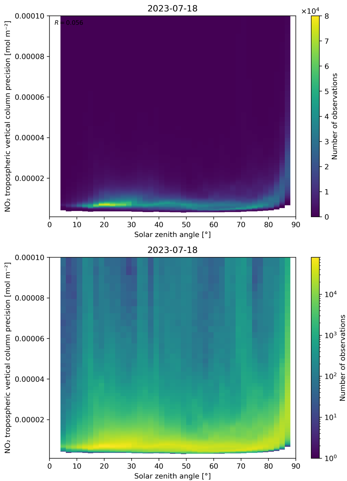
Figure 156: Scatter density plot of “Solar zenith angle” against “NO 2 tropospheric vertical column precision” for 2023-07-17 to 2023-07-19.
