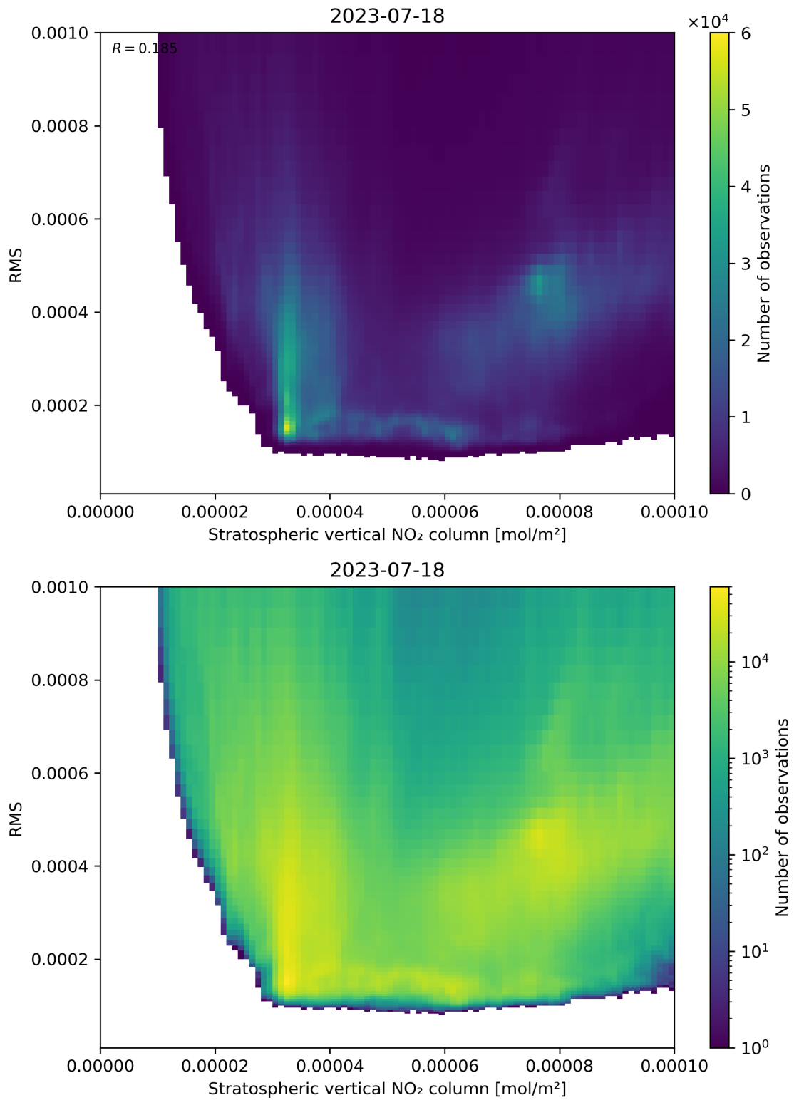
Figure 102: Scatter density plot of “Stratospheric vertical NO 2 column” against “RMS” for 2023-07-17 to 2023-07-19.
