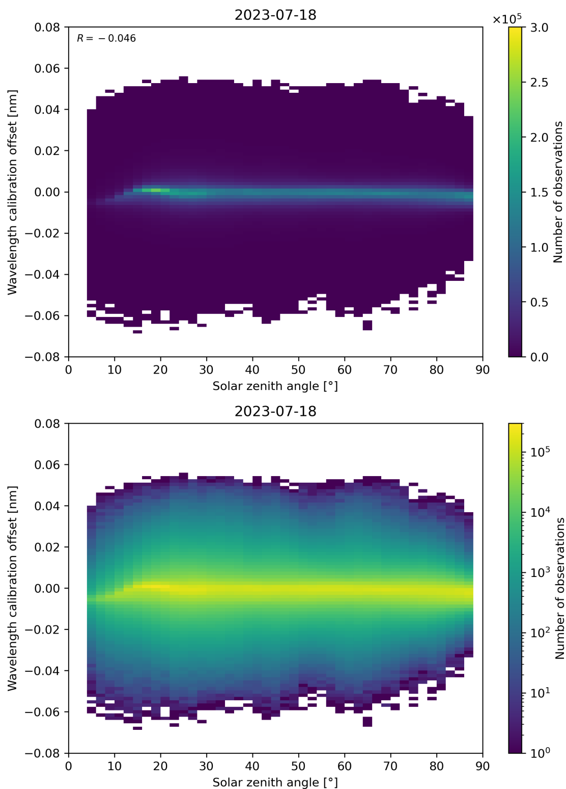
Figure 158: Scatter density plot of “Solar zenith angle” against “Wavelength calibration offset” for 2023-07-17 to 2023-07-19.
