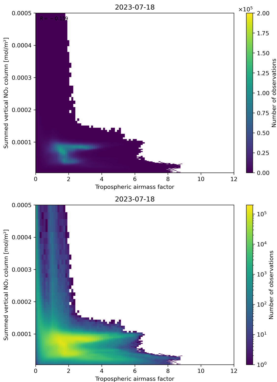
Figure 75: Scatter density plot of “Tropospheric airmass factor” against “Summed vertical NO 2 column” for 2023-07-17 to 2023-07-19.
