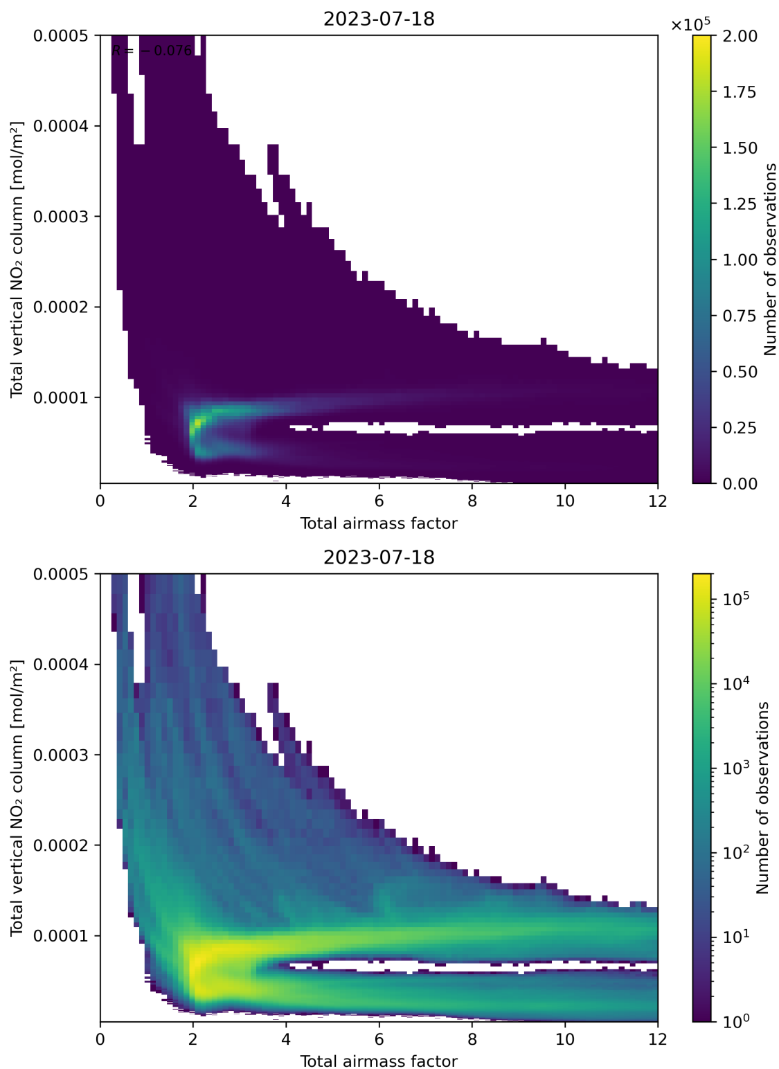
Figure 67: Scatter density plot of “Total air mass factor” against “Total vertical NO 2 column” for 2023-07-17 to 2023-07-19.
