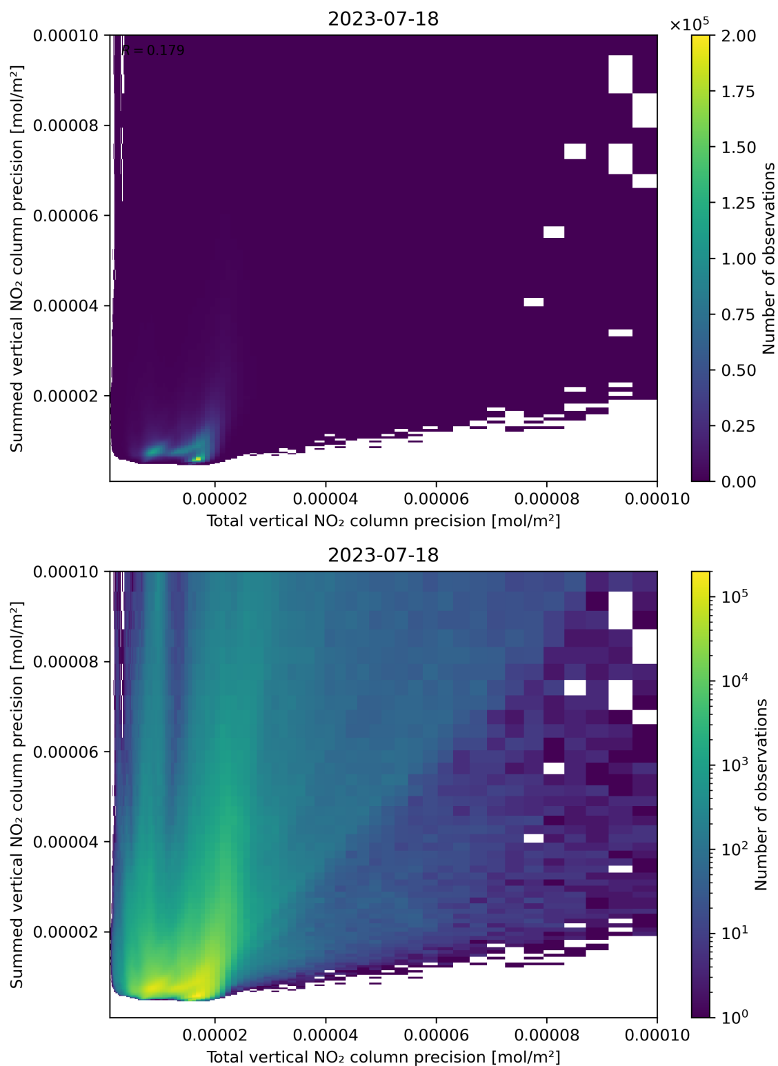
Figure 118: Scatter density plot of “Total vertical NO 2 column precision” against “Summed vertical NO 2 column precision” for 2023-07-17 to 2023-07-19.
