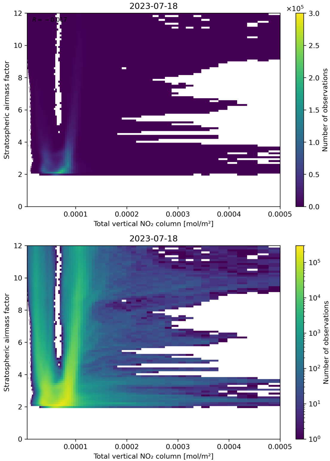
Figure 110: Scatter density plot of “Total vertical NO 2 column” against “Stratospheric airmass factor” for 2023-07-17 to 2023-07-19.
