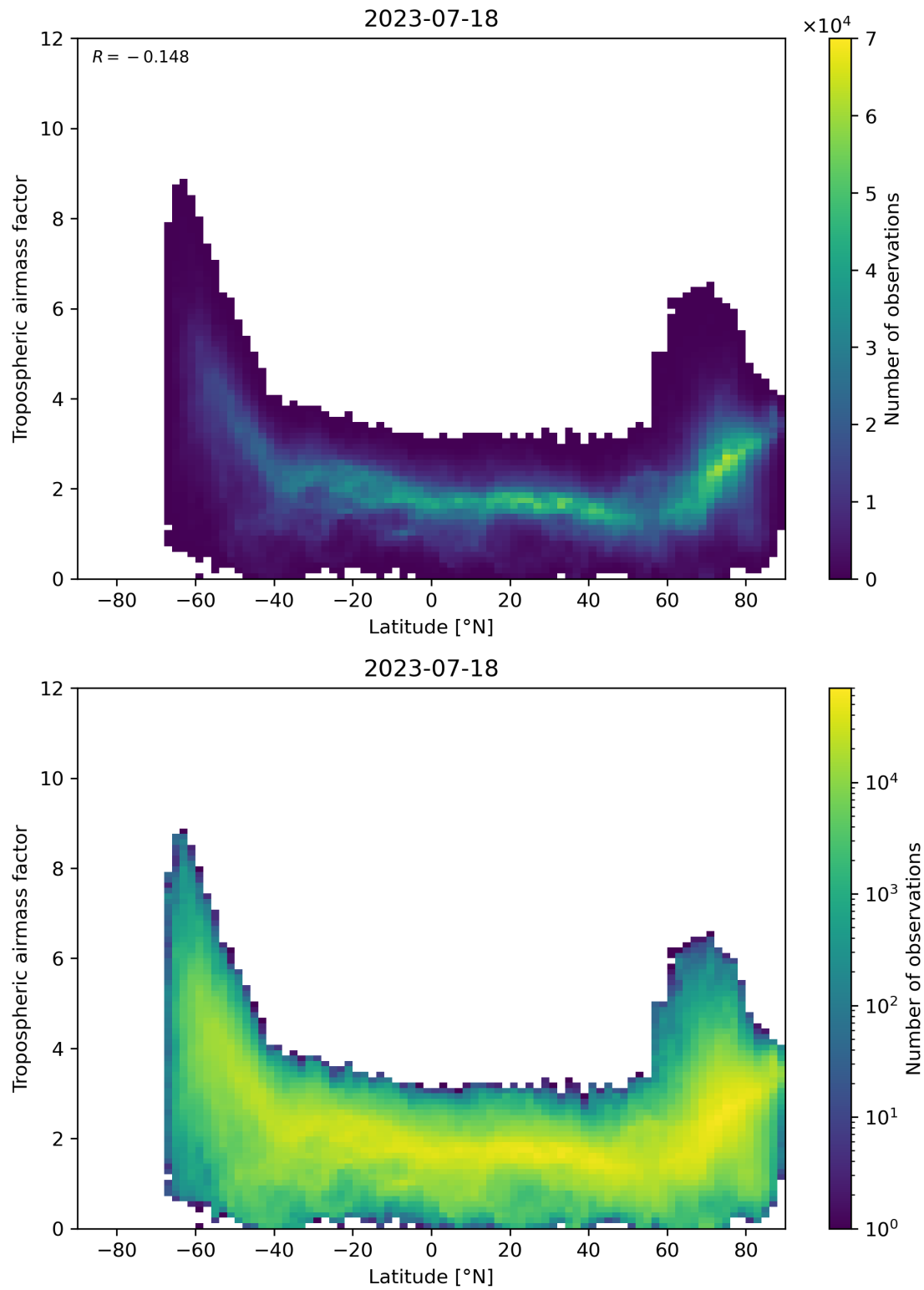
Figure 85: Scatter density plot of “Latitude” against “Tropospheric air mass factor” for 2023-07-17 to 2023-07-19.
