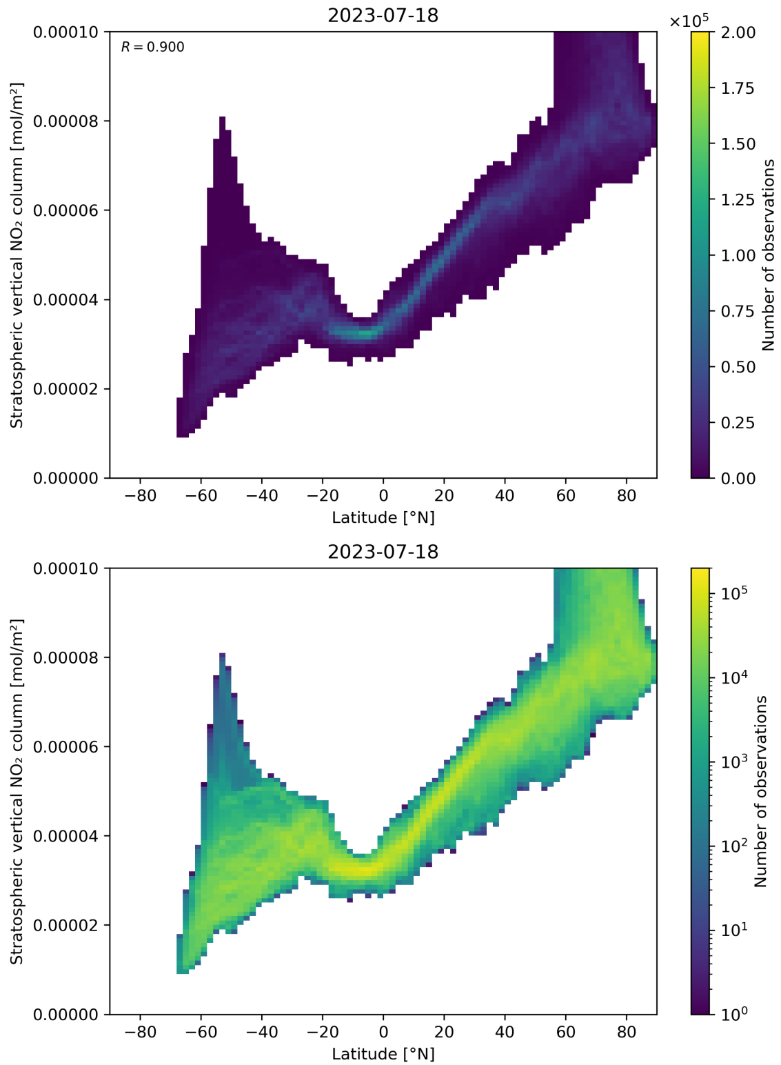
Figure 87: Scatter density plot of “Latitude” against “Stratospheric vertical NO 2 column” for 2023-07-17 to 2023-07-19.
