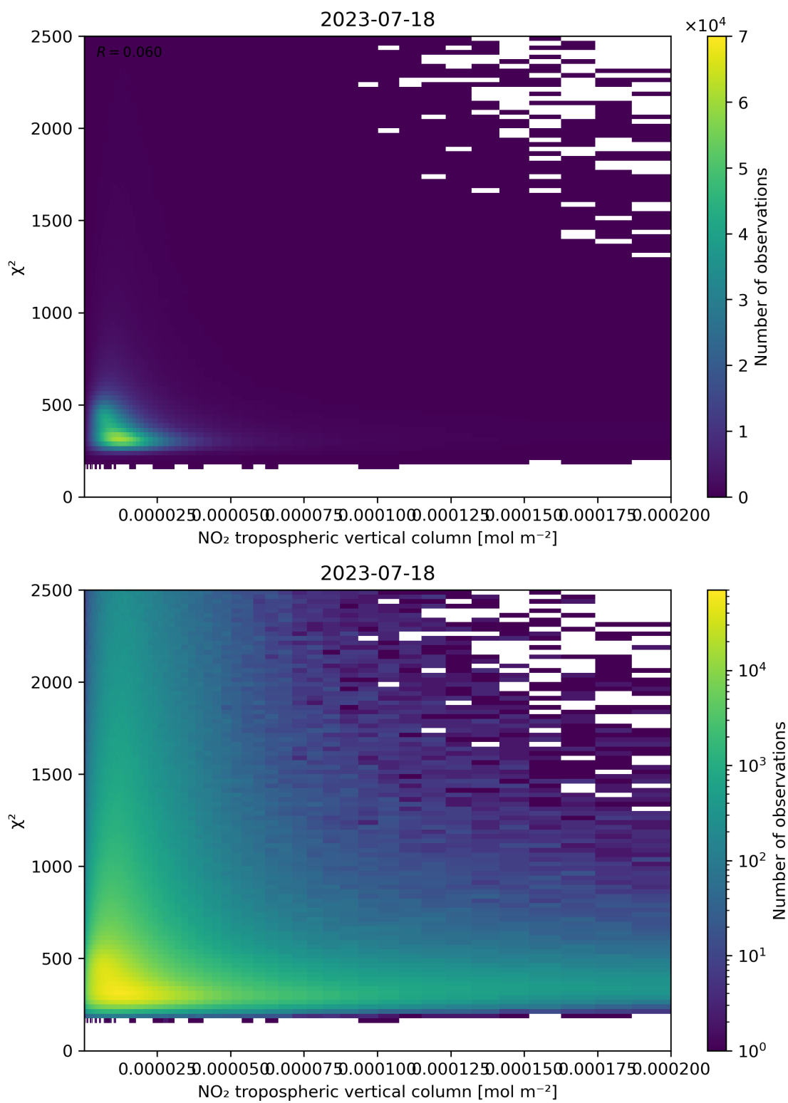
Figure 124: Scatter density plot of “NO 2 tropospheric vertical column” against “ \chi^2 ” for 2023-07-17 to 2023-07-19.
