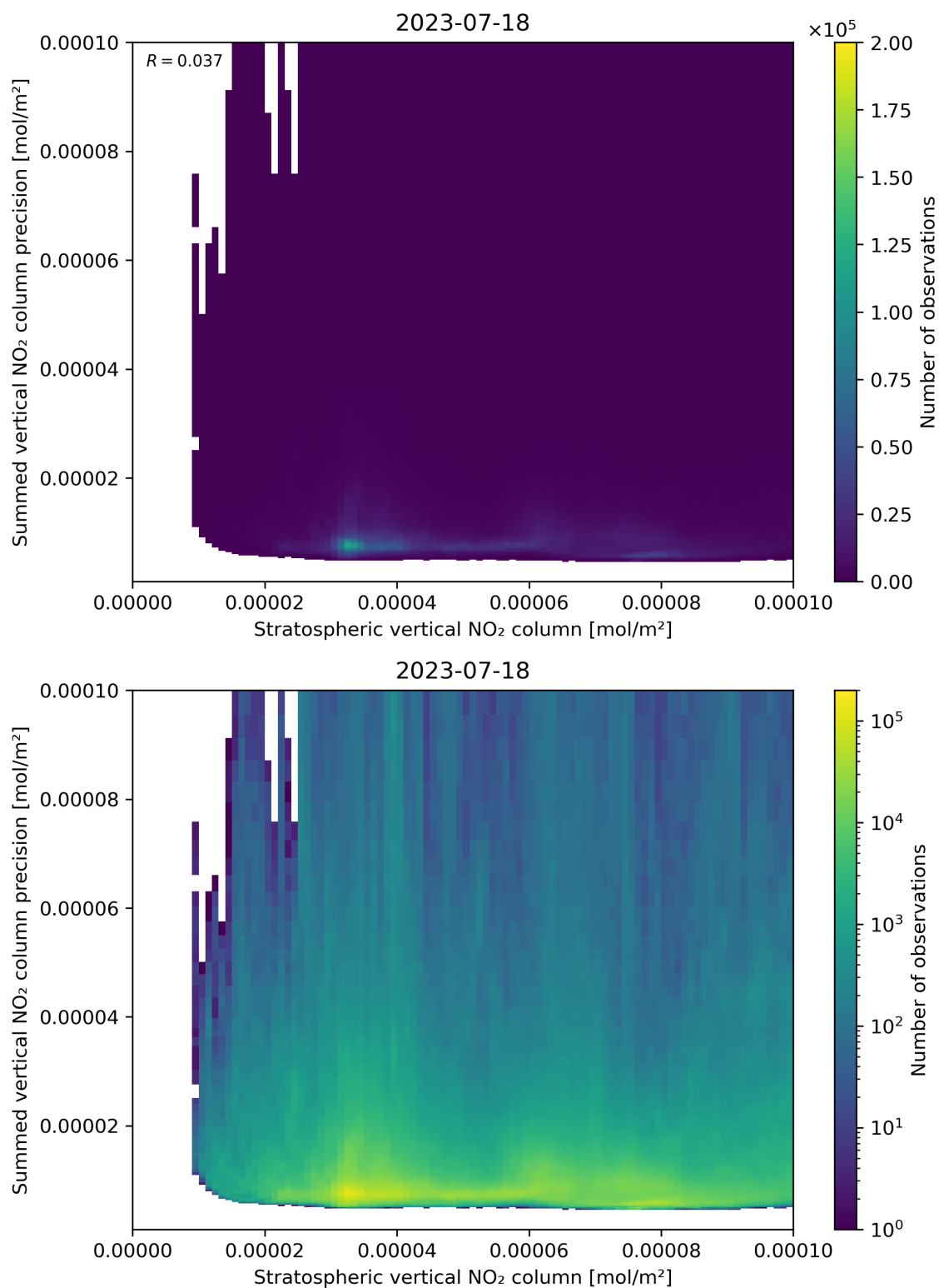
Figure 99: Scatter density plot of “Stratospheric vertical NO 2 column” against “Summed vertical NO 2 column precision” for 2023-07-17 to 2023-07-19.
