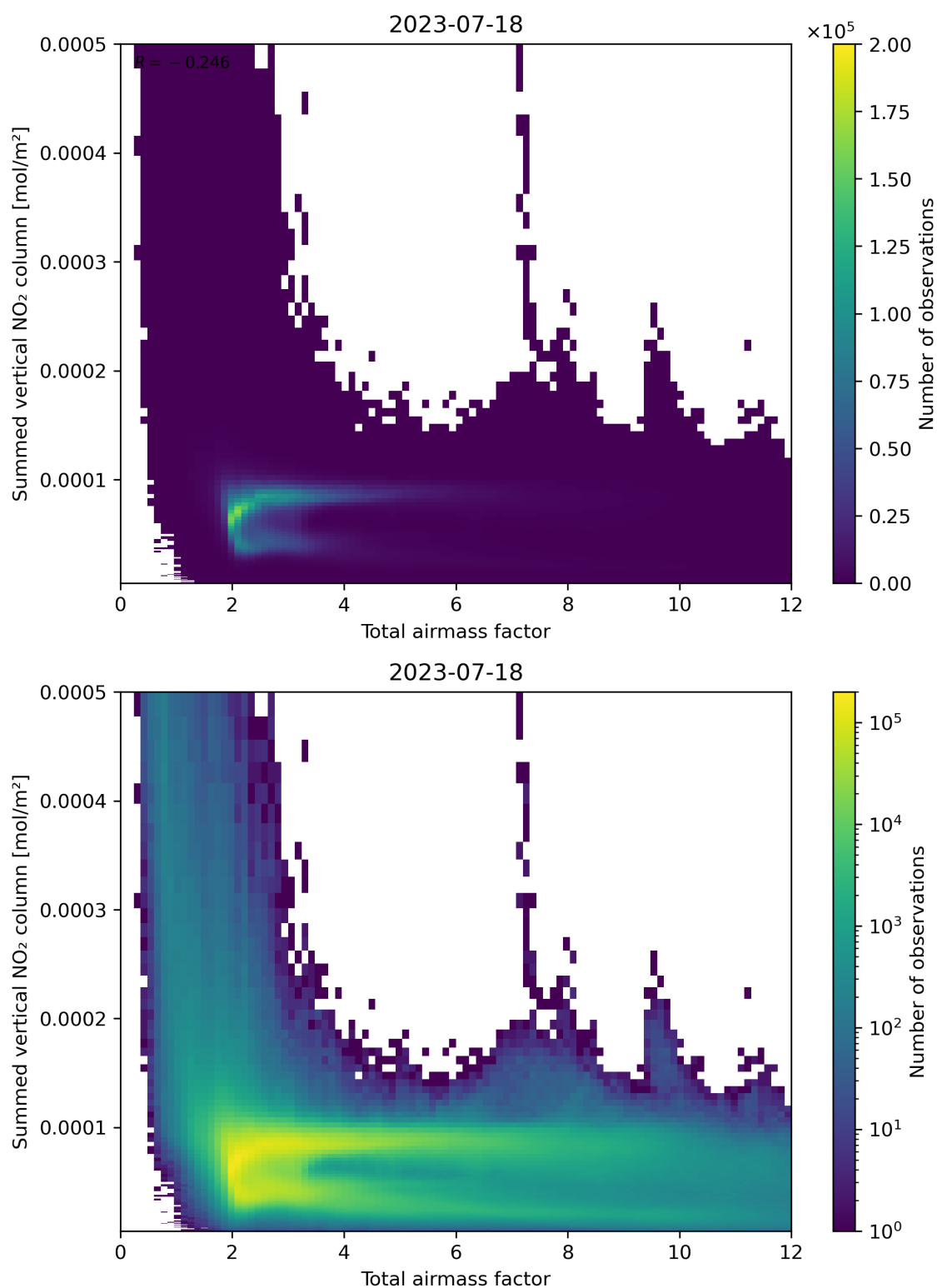
Figure 65: Scatter density plot of “Total airmass factor” against “Summed vertical NO 2 column” for 2023-07-17 to 2023-07-19.
