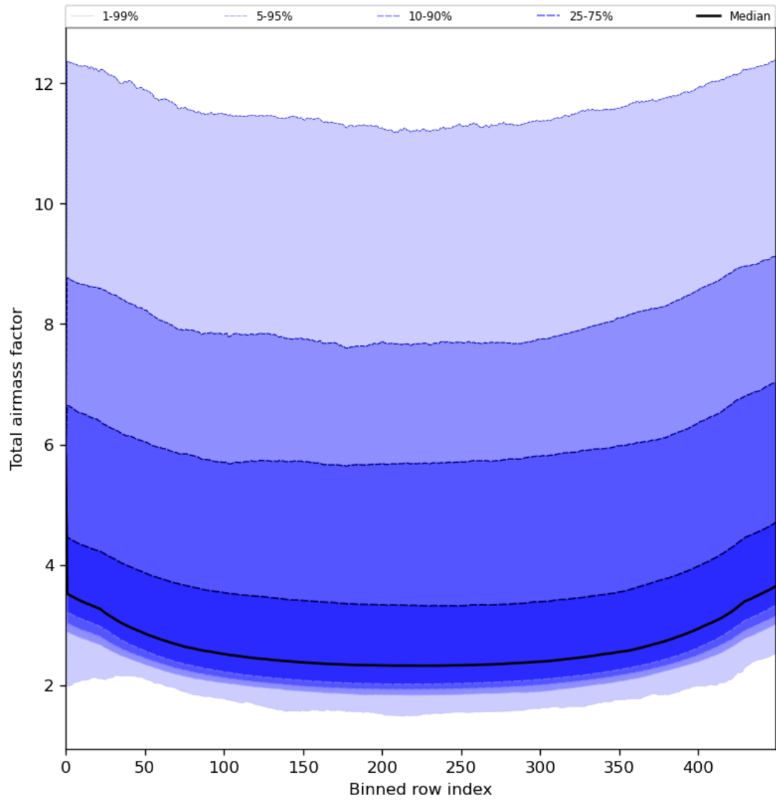
Figure 49: Along track statistics of “Total airmass factor” for 2023-07-17 to 2023-07-19
