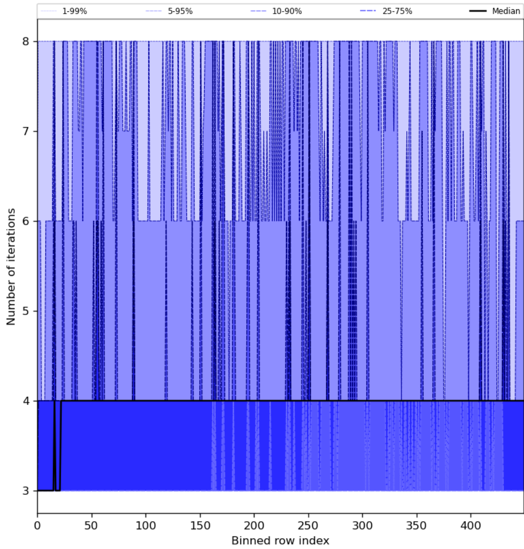
Figure 51: Along track statistics of “Number of iterations” for 2023-07-17 to 2023-07-19
