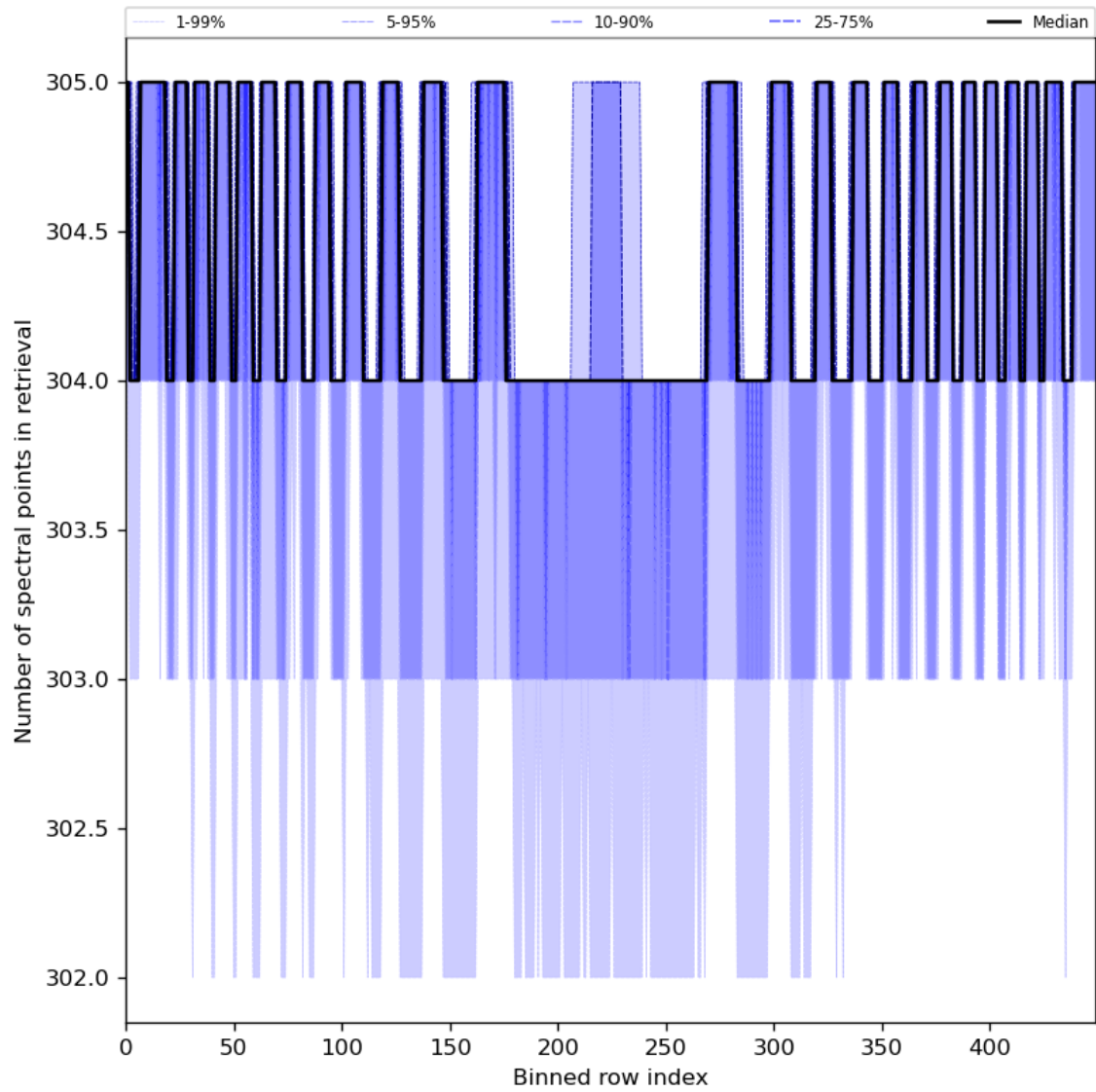
Figure 50: Along track statistics of “Number of spectral points in retrieval” for 2023-07-17 to 2023-07-19
