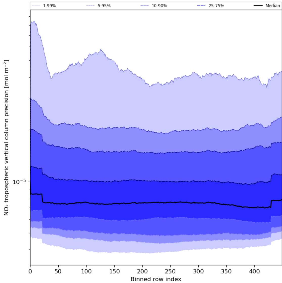
Figure 47: Along track statistics of “NO 2 tropospheric vertical column precision” for 2023-07-17 to 2023-07-19
