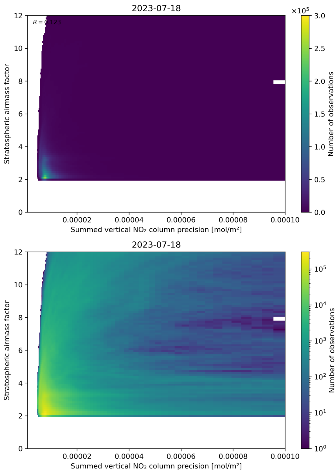
Figure 106: Scatter density plot of “Summed vertical NO 2 column precision” against “Stratospheric airmass factor” for 2023-07-17 to 2023-07-19.
