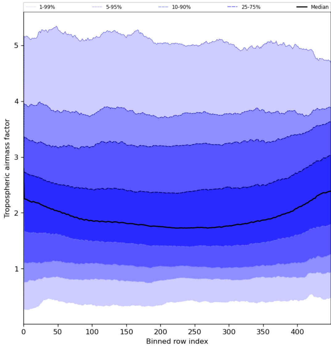
Figure 48: Along track statistics of “Tropospheric air mass factor” for 2023-07-17 to 2023-07-19
