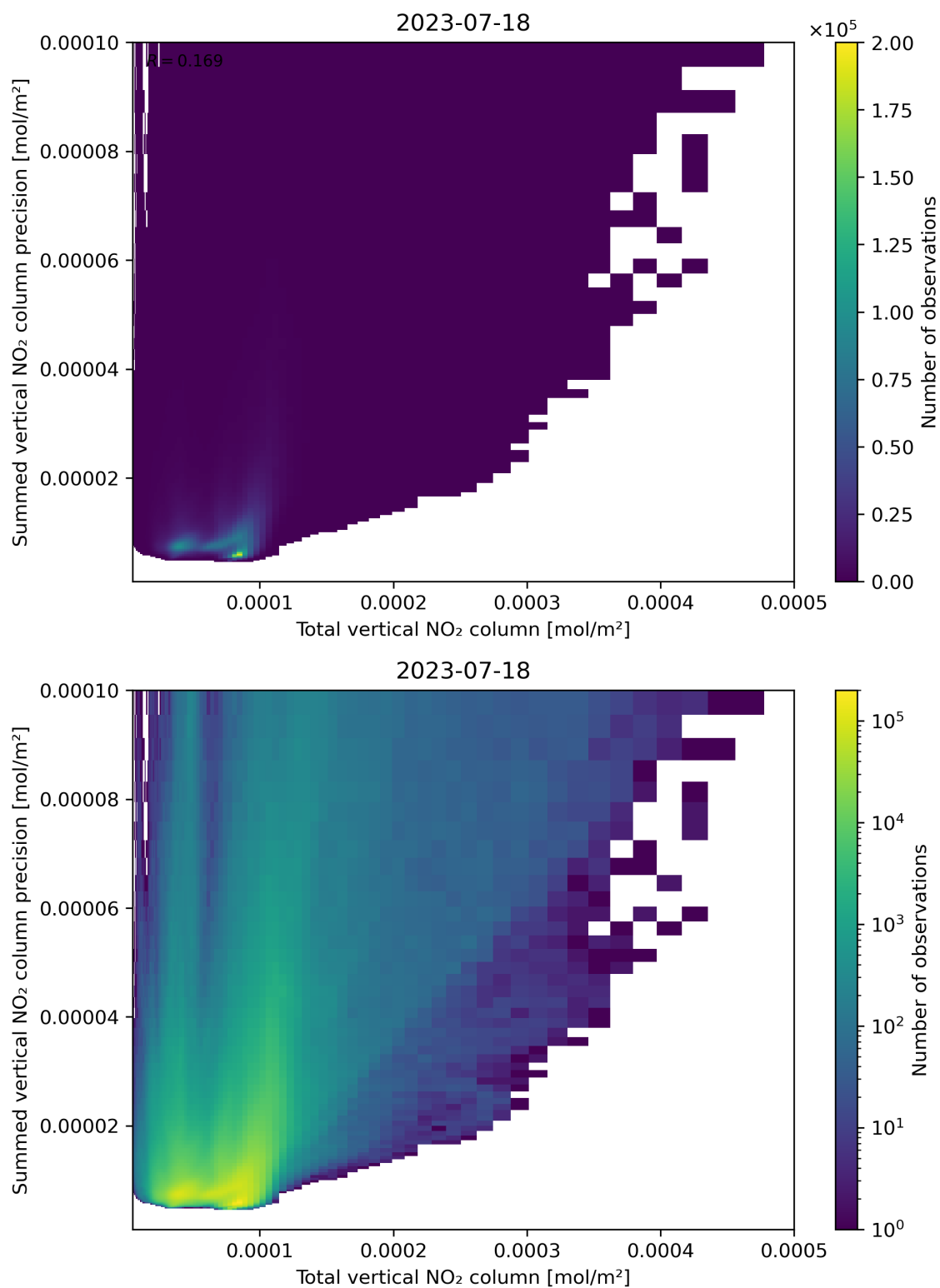
Figure 113: Scatter density plot of “Total vertical NO 2 column” against “Summed vertical NO 2 column precision” for 2023-07-17 to 2023-07-19.
