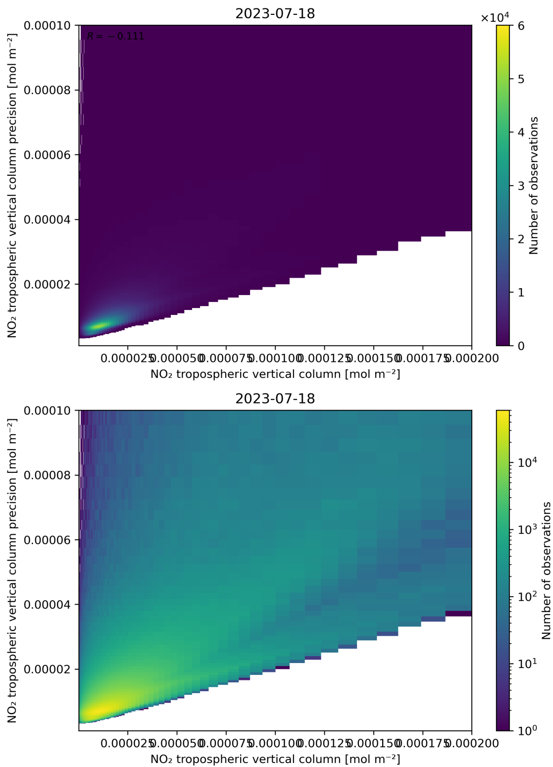
Figure 130: Scatter density plot of “NO 2 tropospheric vertical column” against “NO 2 tropospheric vertical column precision” for 2023-07-17 to 2023-07-19.
