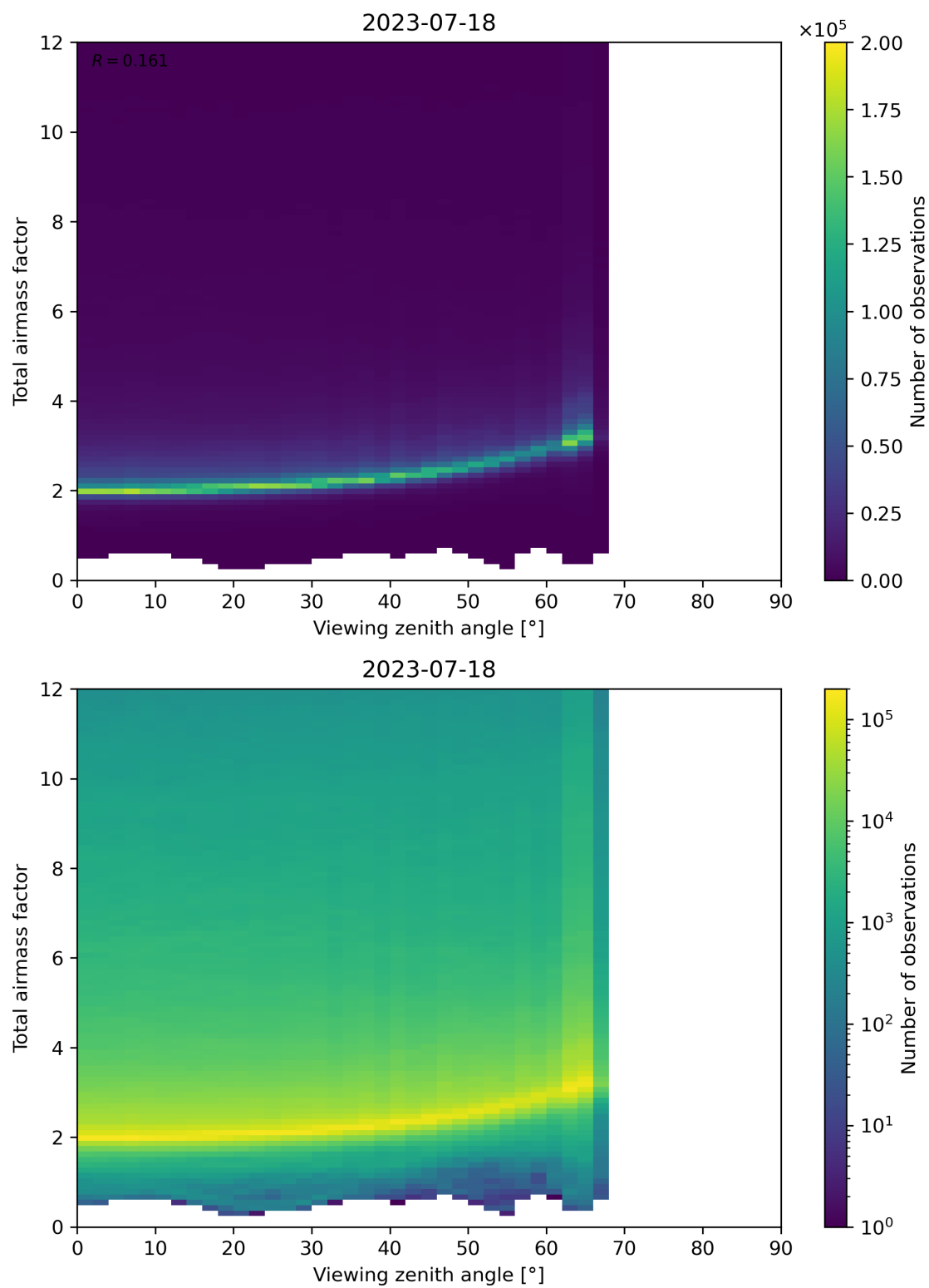
Figure 160: Scatter density plot of “Viewing zenith angle” against “Total airmass factor” for 2023-07-17 to 2023-07-19.
