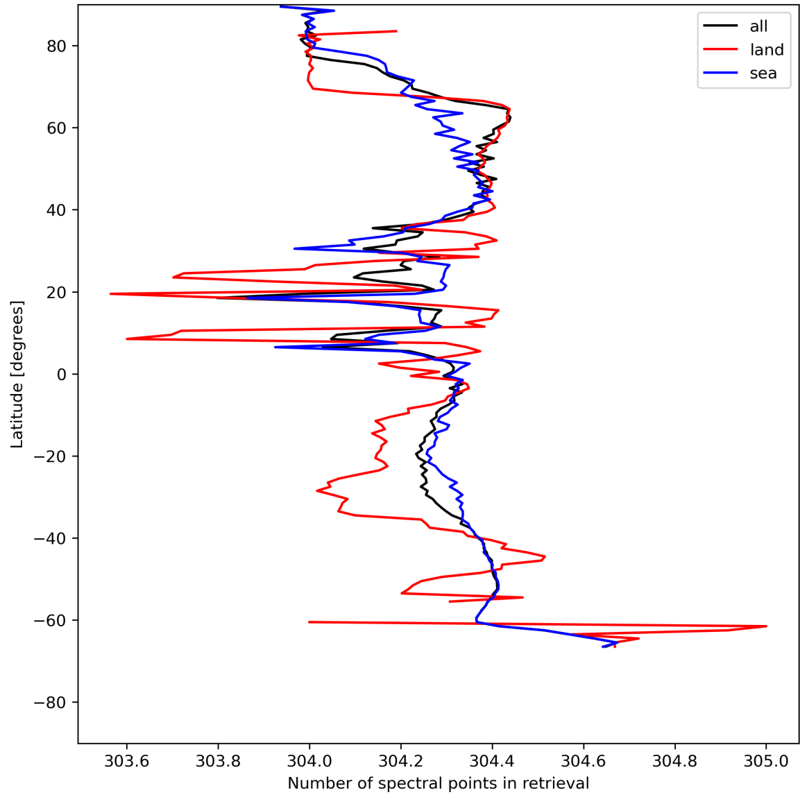
Figure 16: Zonal average of “Number of spectral points in retrieval” for 2023-07-17 to 2023-07-19.
