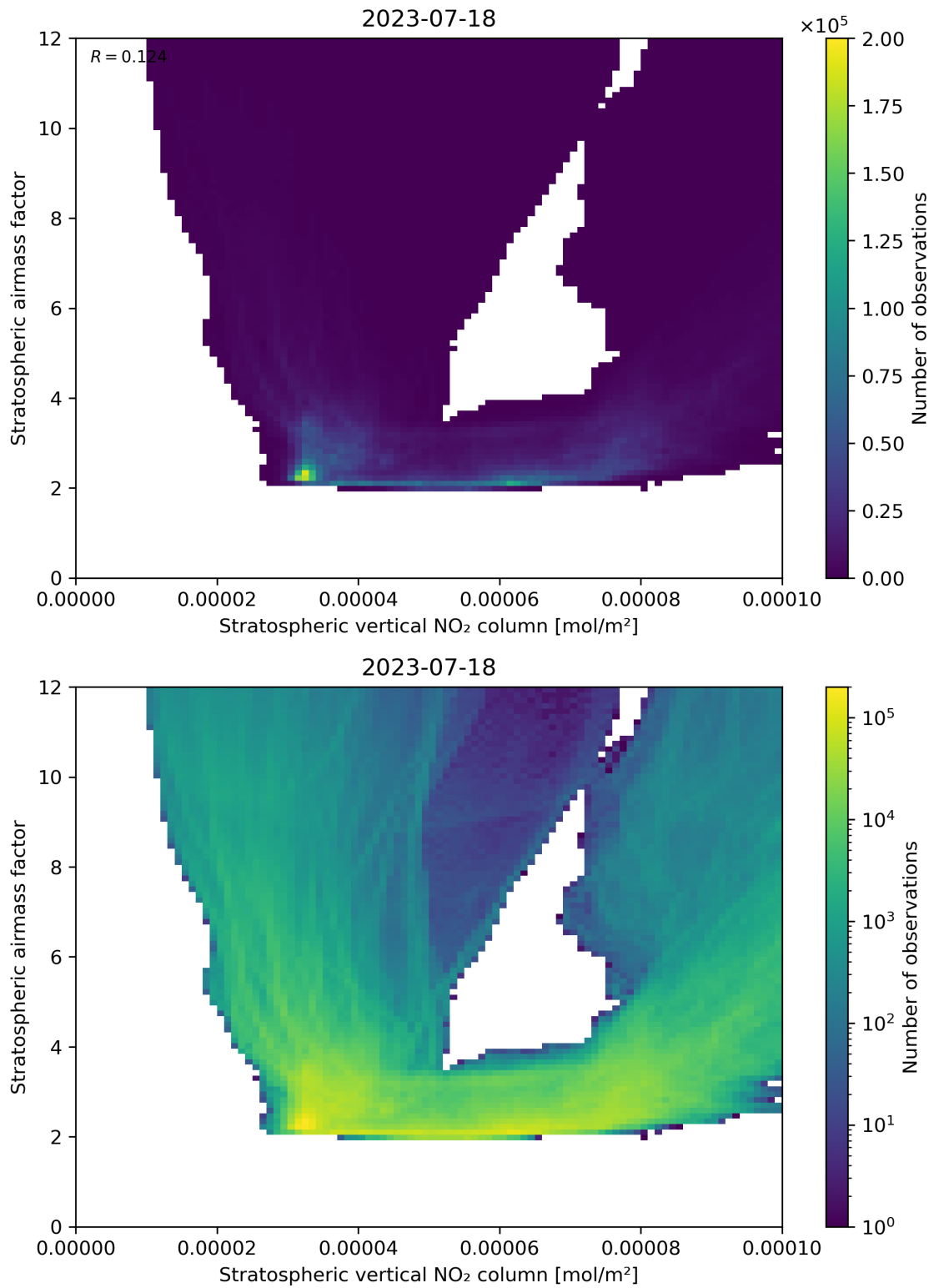
Figure 96: Scatter density plot of “Stratospheric vertical NO 2 column” against “Stratospheric airmass factor” for 2023-07-17 to 2023-07-19.
