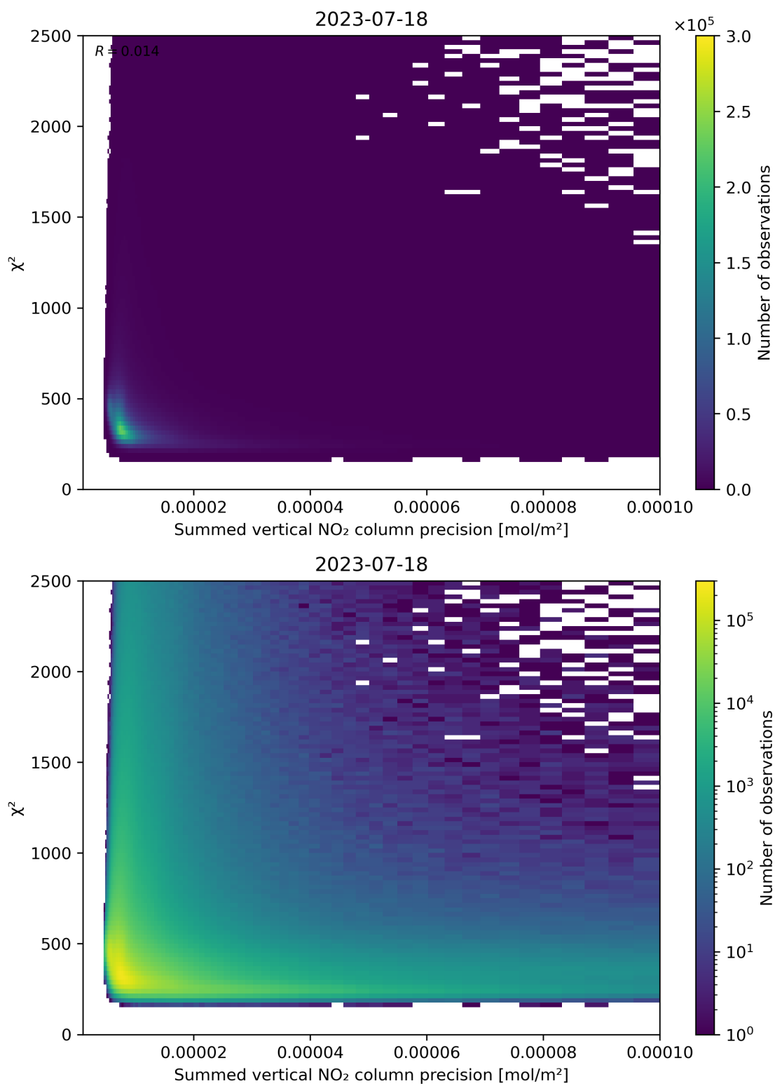
Figure 107: Scatter density plot of “Summed vertical NO 2 column precision” against “ \chi^2 ” for 2023-07-17 to 2023-07-19.
