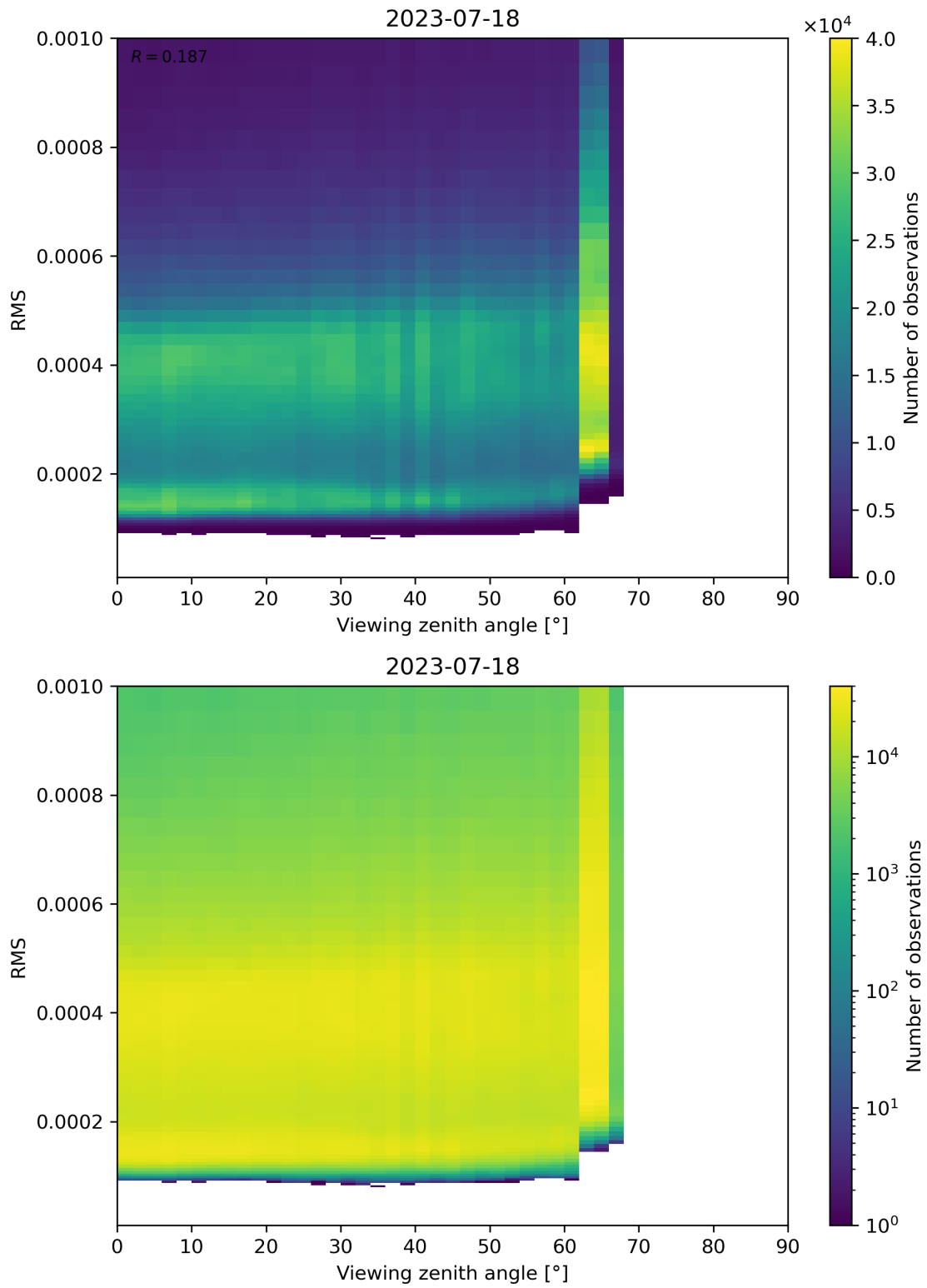
Figure 171: Scatter density plot of “Viewing zenith angle” against “RMS” for 2023-07-17 to 2023-07-19.
