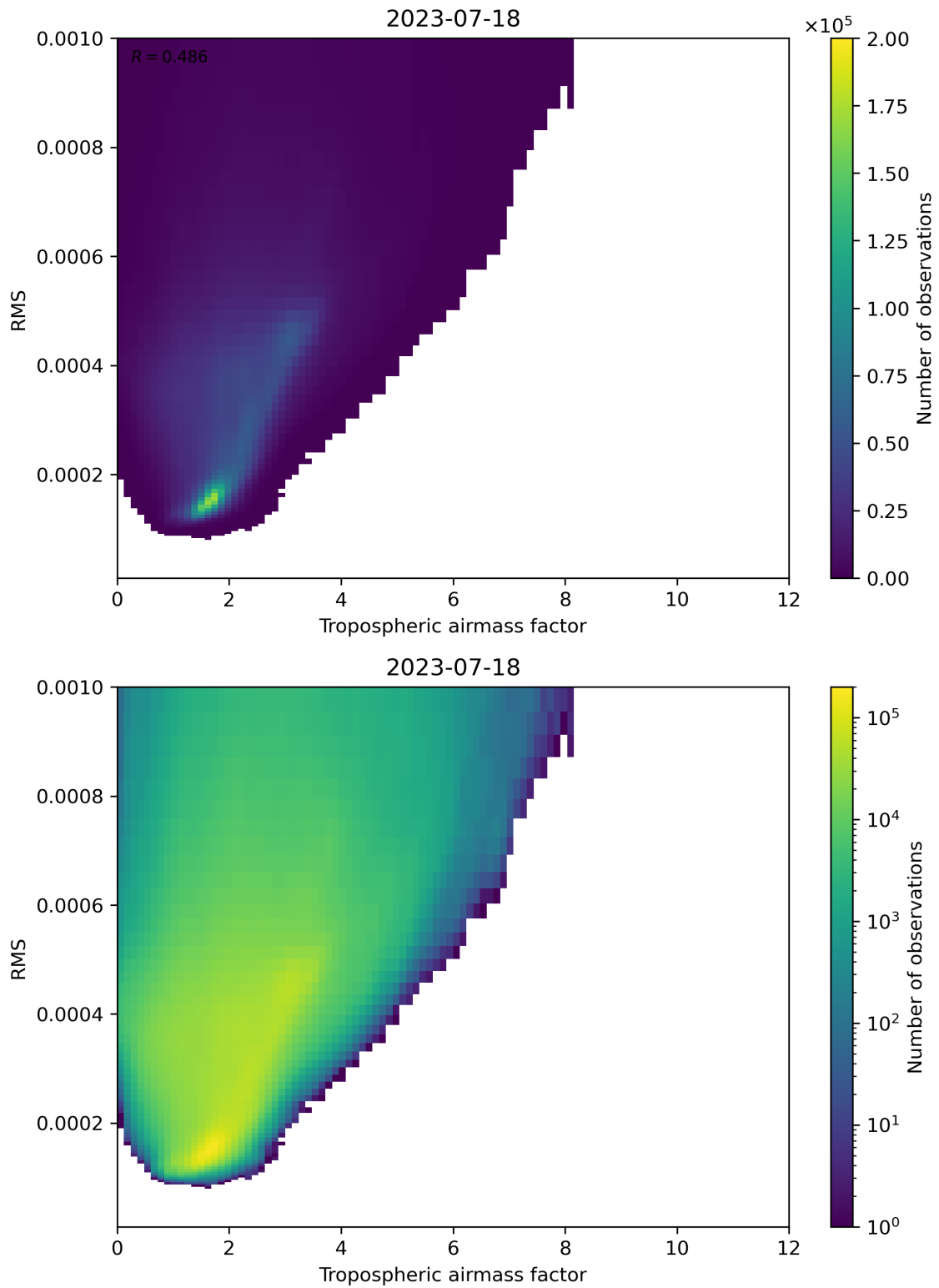
Figure 79: Scatter density plot of “Tropospheric airmass factor” against “RMS” for 2023-07-17 to 2023-07-19.
