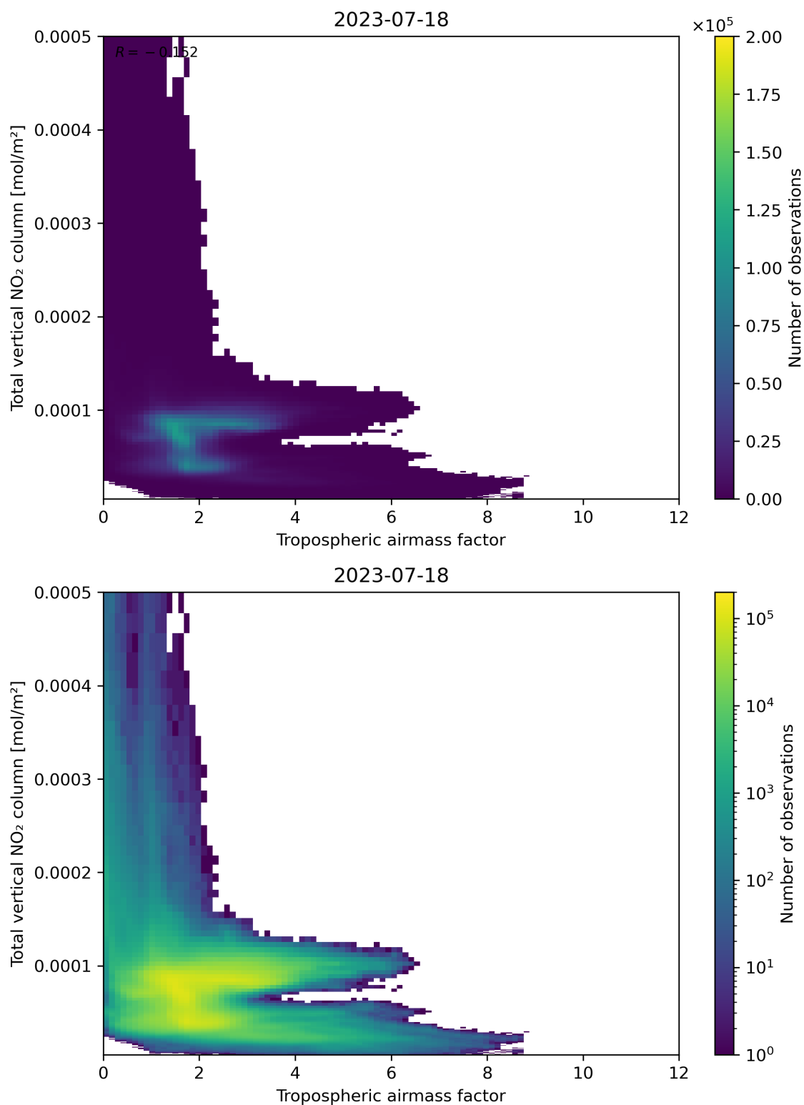
Figure 77: Scatter density plot of “Tropospheric airmass factor” against “Total vertical NO 2 column” for 2023-07-17 to 2023-07-19.
