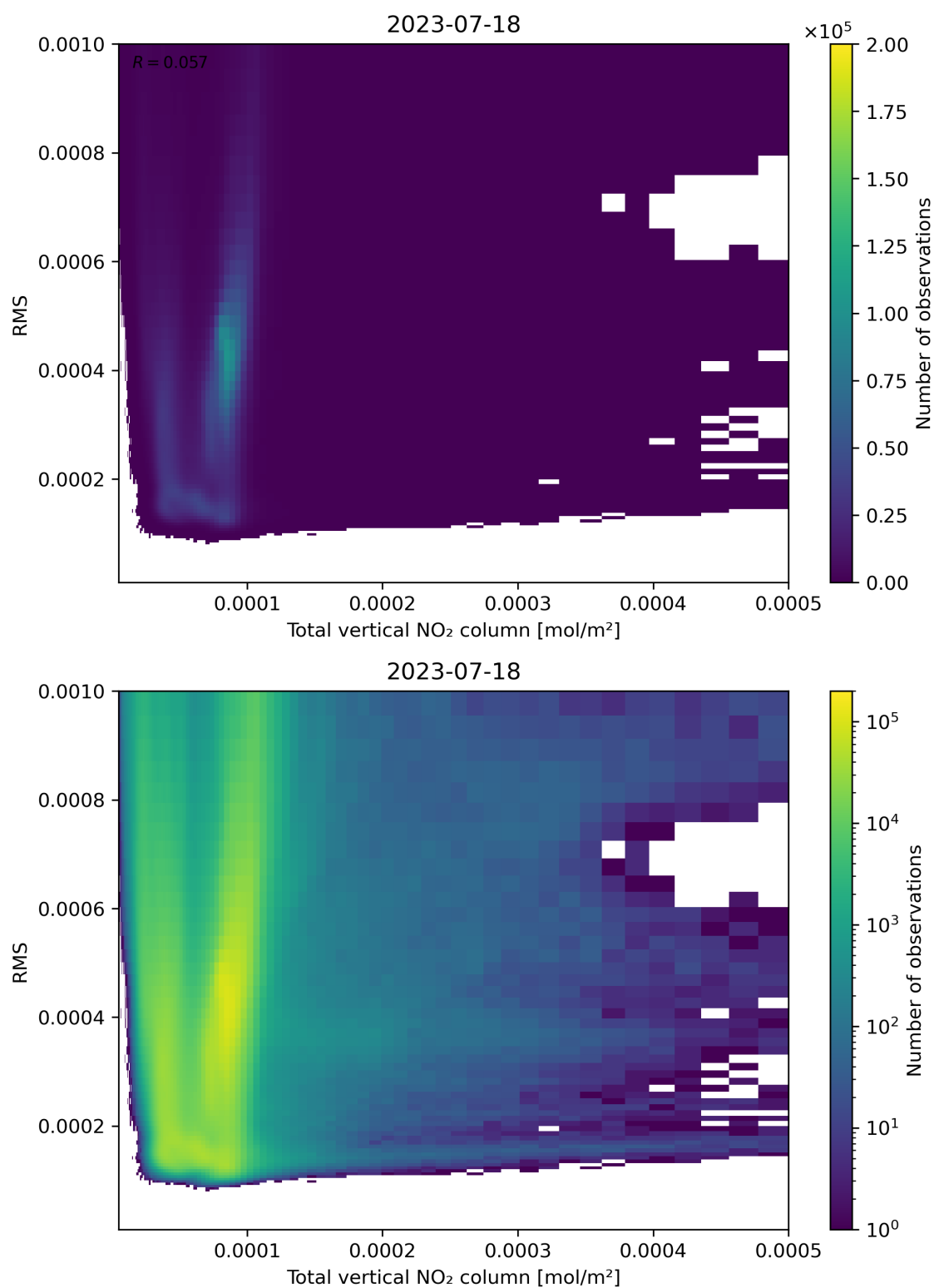
Figure 120: Scatter density plot of “Total vertical NO 2 column” against “RMS” for 2023-07-17 to 2023-07-19.
