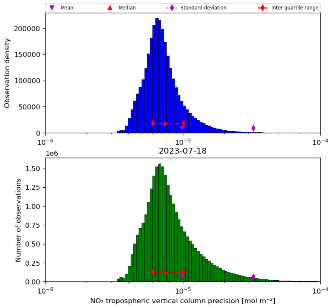
Figure 30: Histogram of “NO 2 tropospheric vertical column precision” for 2023-07-17 to 2023-07-19
