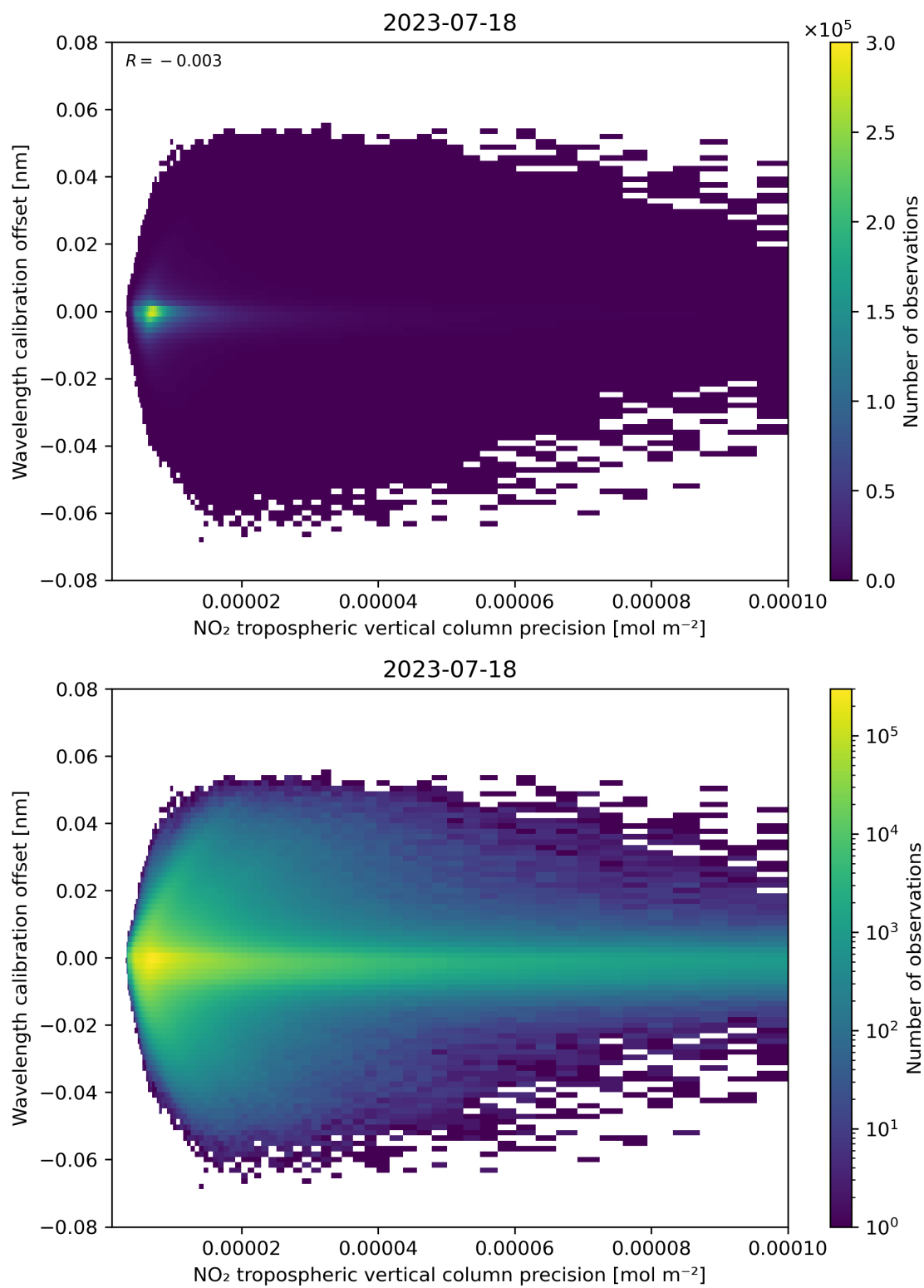
Figure 141: Scatter density plot of “NO 2 tropospheric vertical column precision” against “Wavelength calibration offset” for 2023-07-17 to 2023-07-19.
