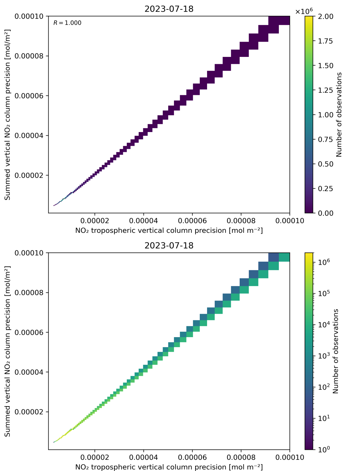
Figure 137: Scatter density plot of “NO 2 tropospheric vertical column precision” against “Summed vertical NO 2 column precision” for 2023-07-17 to 2023-07-19.
