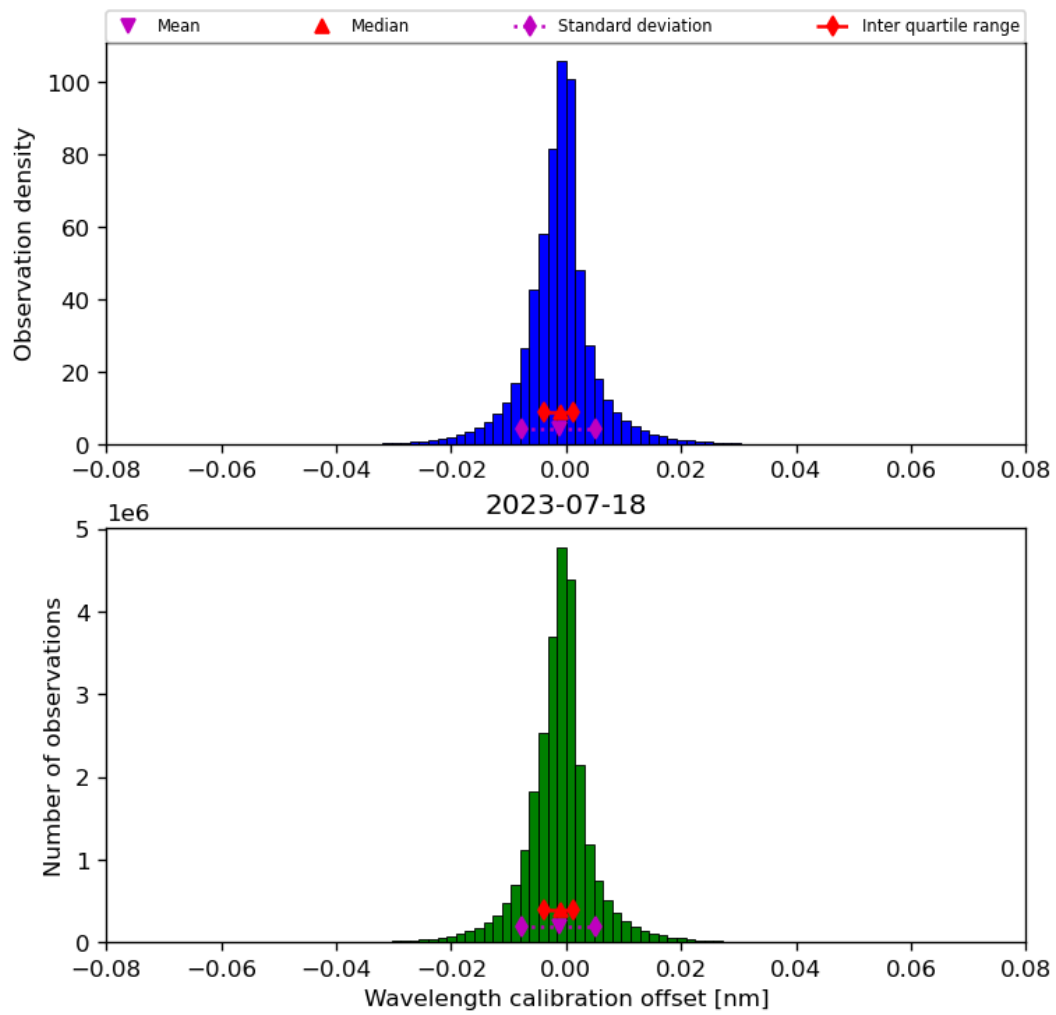
Figure 35: Histogram of “Wavelength calibration offset” for 2023-07-17 to 2023-07-19
