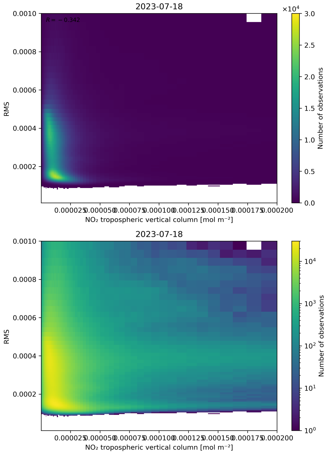
Figure 142: Scatter density plot of “NO 2 tropospheric vertical column” against “RMS” for 2023-07-17 to 2023-07-19.
