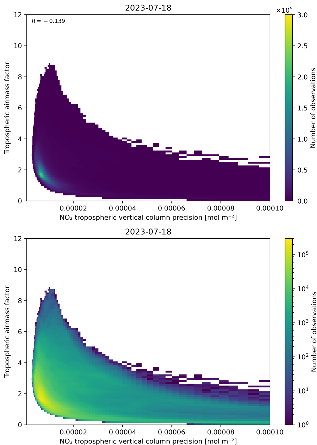
Figure 133: Scatter density plot of “NO 2 tropospheric vertical column precision” against “Tropospheric airmass factor” for 2023-07-17 to 2023-07-19.
