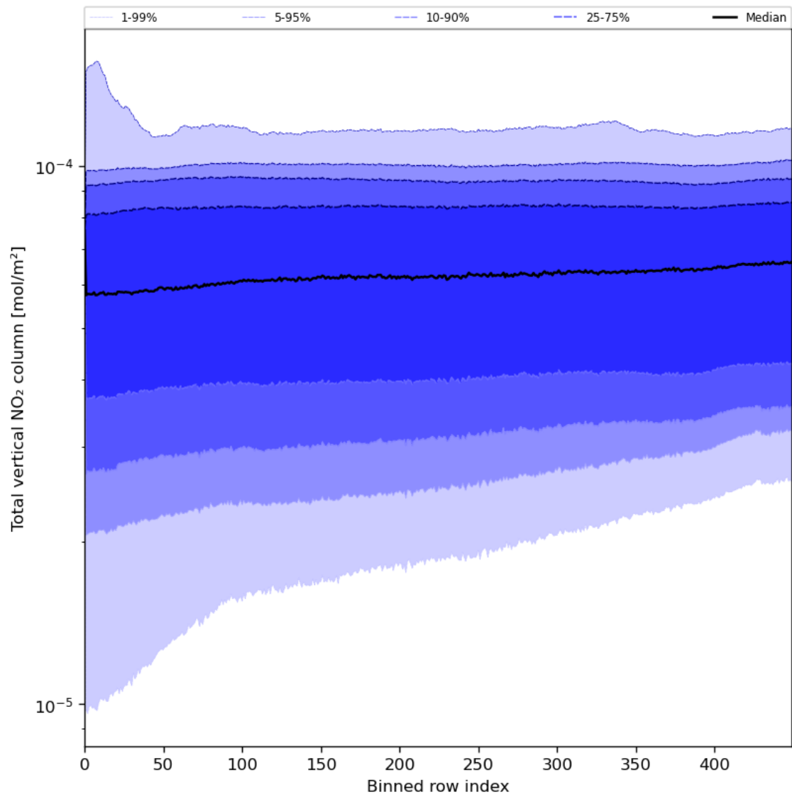
Figure 55: Along track statistics of “Total vertical NO 2 column” for 2023-07-17 to 2023-07-19
