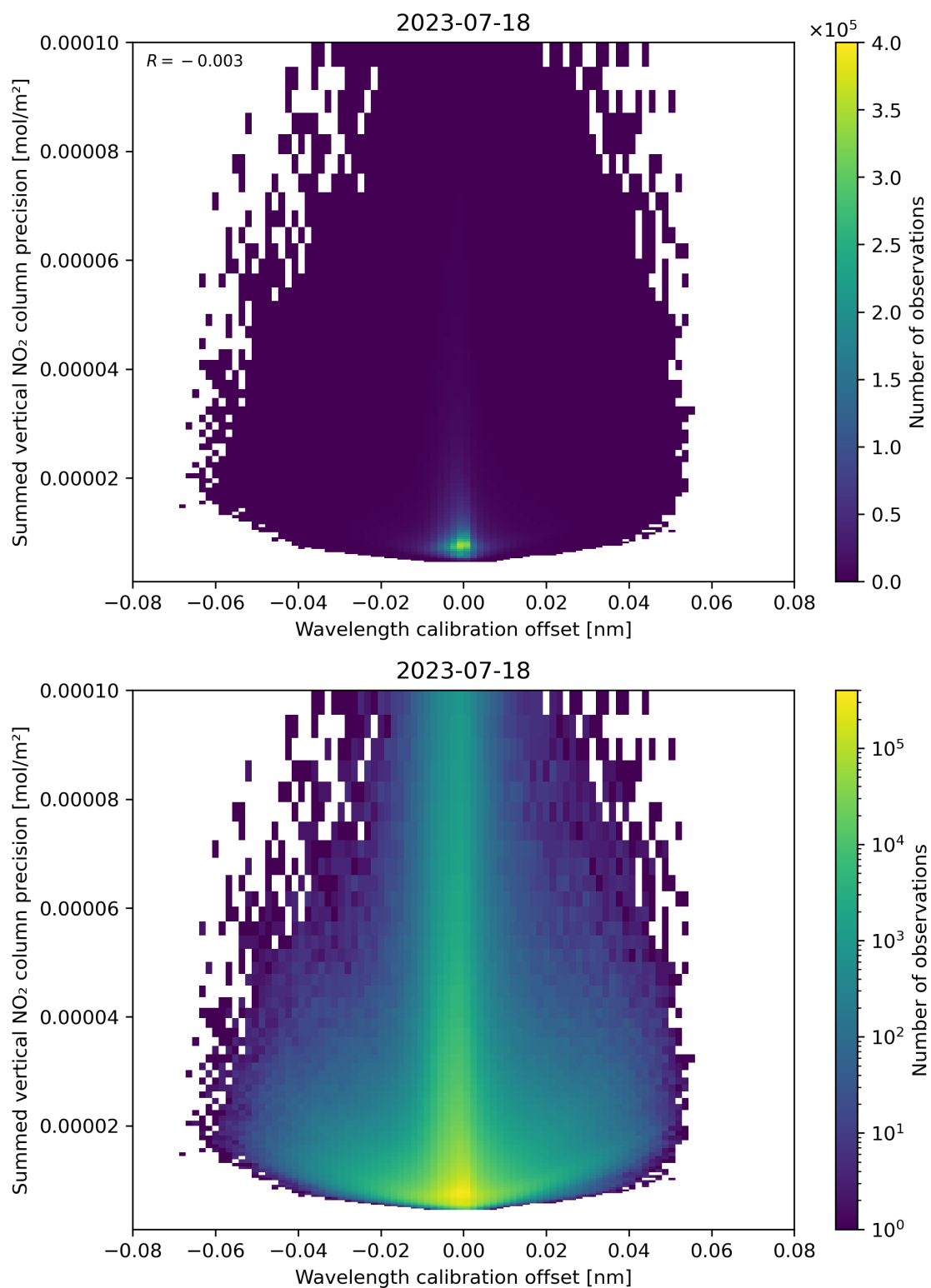
Figure 178: Scatter density plot of “Wavelength calibration offset” against “Summed vertical NO 2 column precision” for 2023-07-17 to 2023-07-19.
