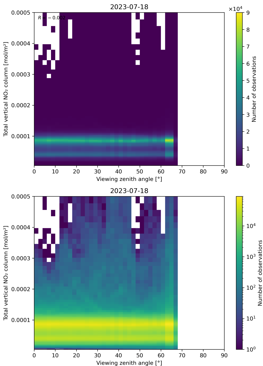
Figure 167: Scatter density plot of “Viewing zenith angle” against “Total vertical NO 2 column” for 2023-07-17 to 2023-07-19.
