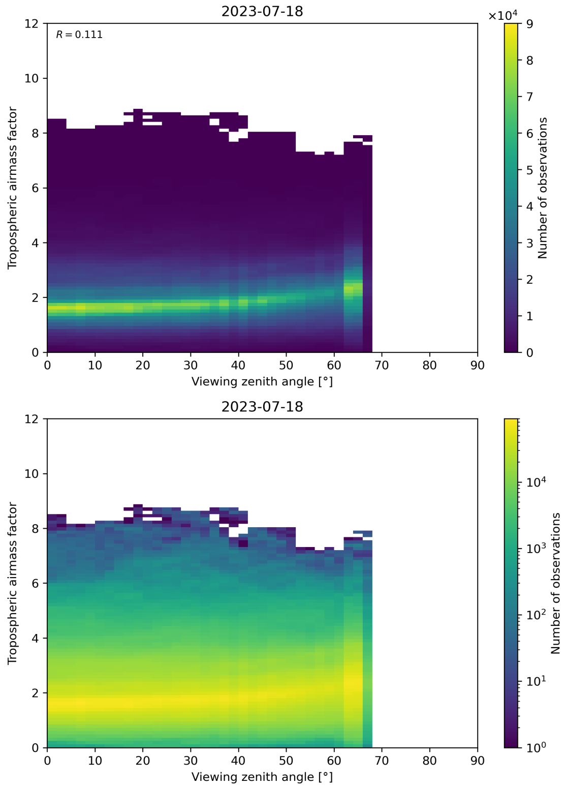
Figure 161: Scatter density plot of “Viewing zenith angle” against “Tropospheric airmass factor” for 2023-07-17 to 2023-07-19.
