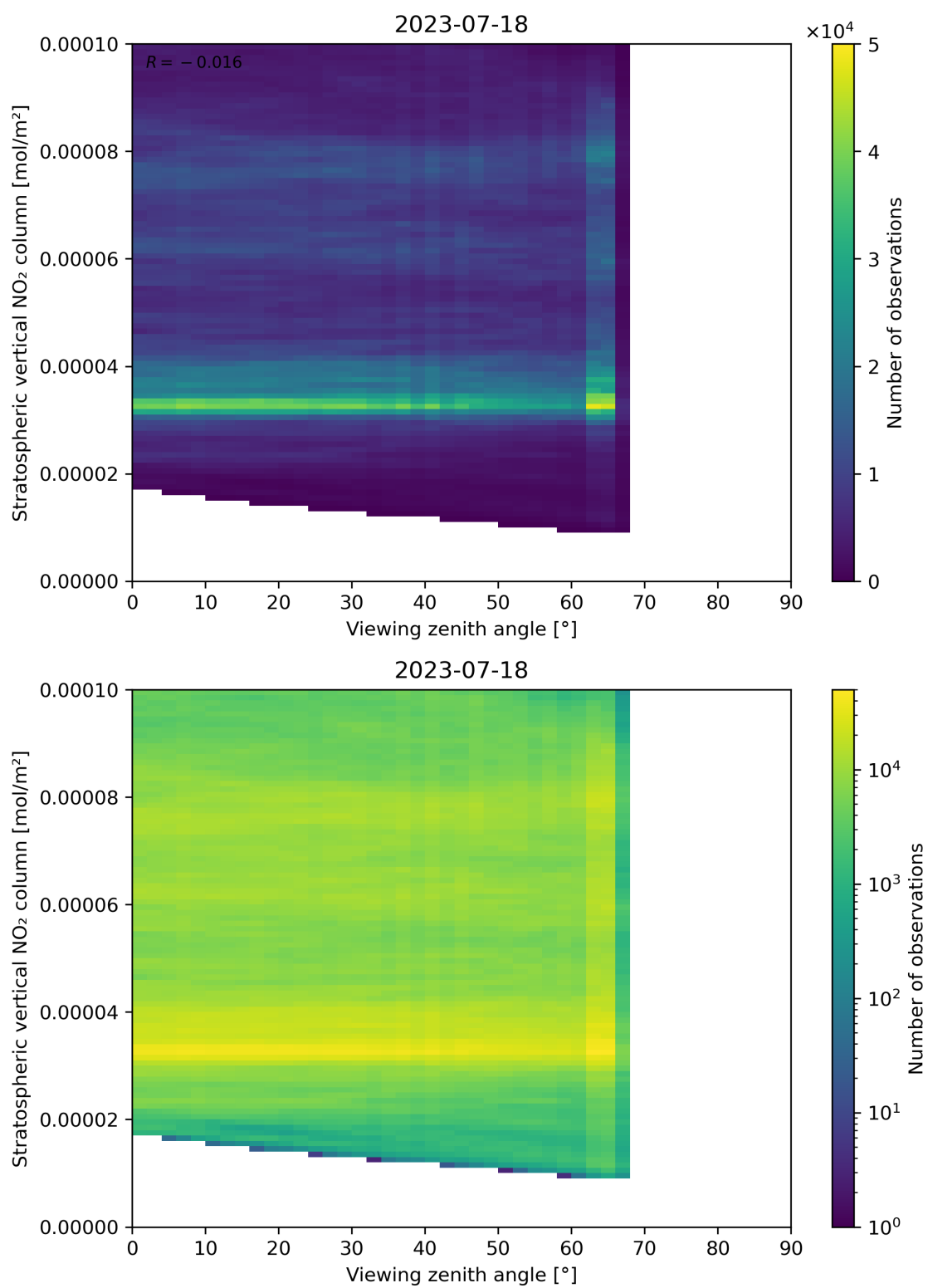
Figure 164: Scatter density plot of “Viewing zenith angle” against “Stratospheric vertical NO 2 column” for 2023-07-17 to 2023-07-19.
