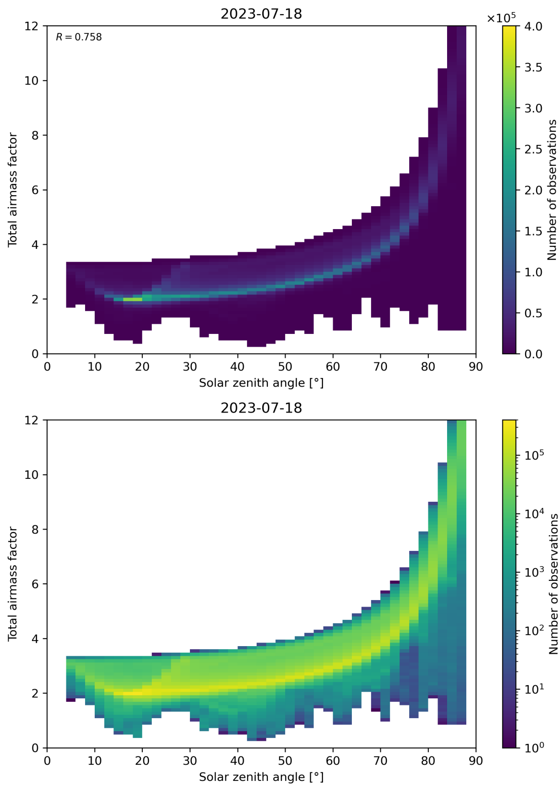
Figure 146: Scatter density plot of “Solar zenith angle” against “Total air mass factor” for 2023-07-17 to 2023-07-19.
