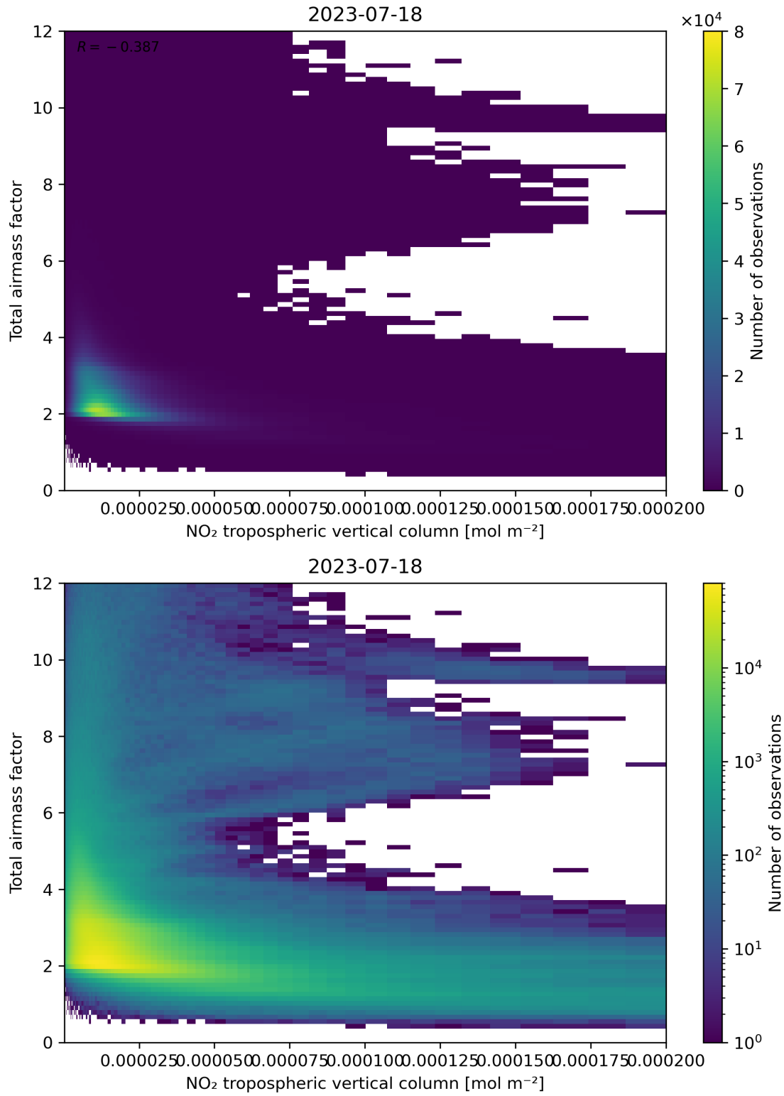
Figure 122: Scatter density plot of “NO 2 tropospheric vertical column” against “Total air mass factor” for 2023-07-17 to 2023-07-19.
