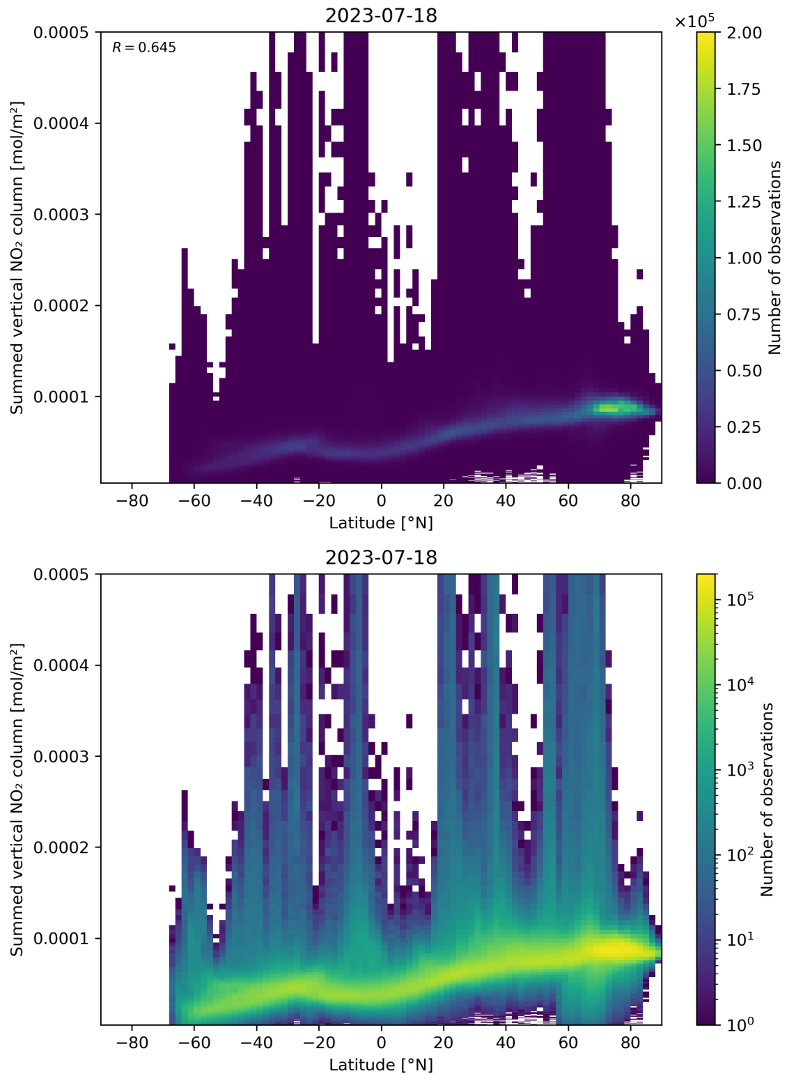
Figure 88: Scatter density plot of “Latitude” against “Summed vertical NO 2 column” for 2023-07-17 to 2023-07-19.
