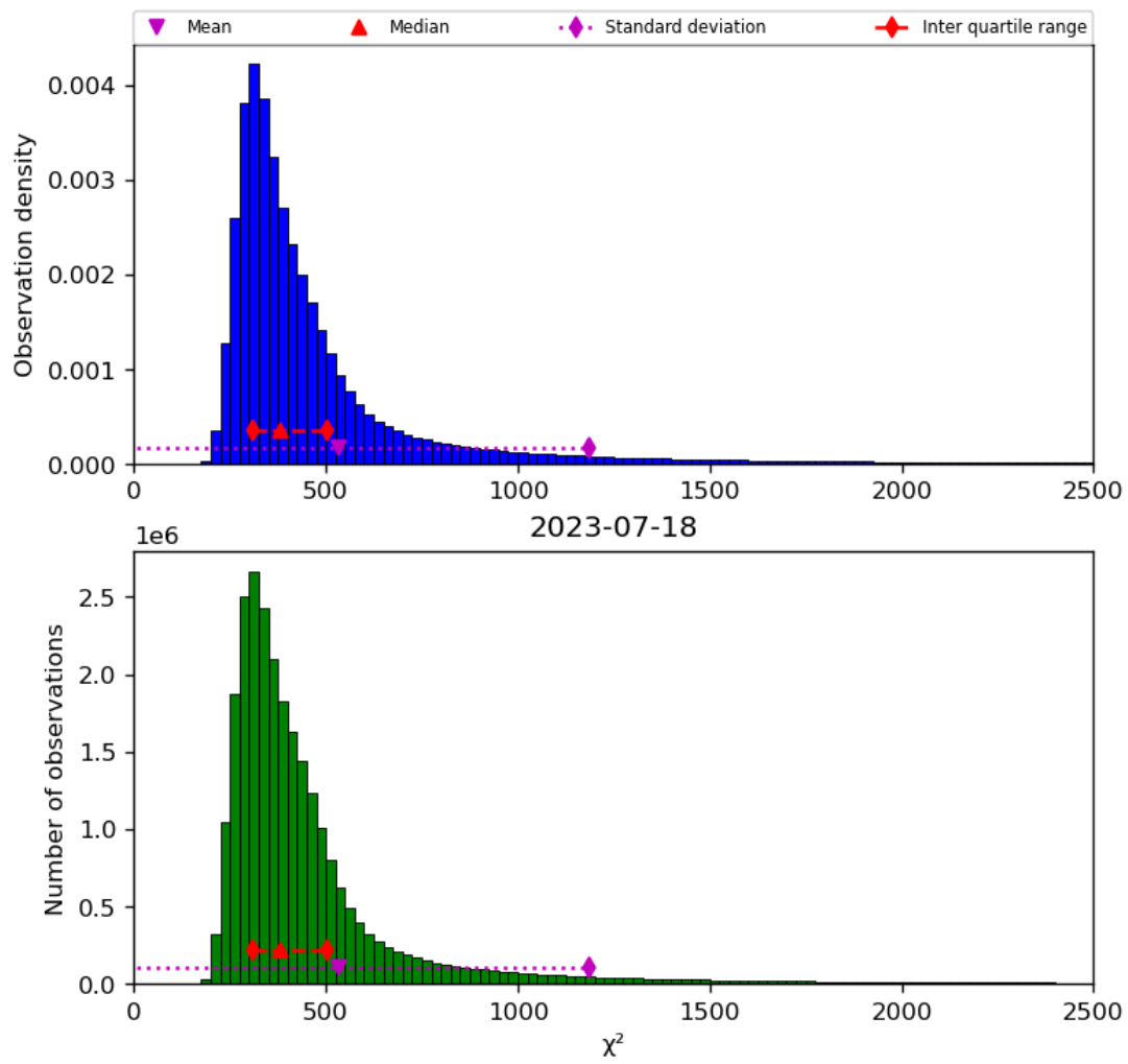
Figure 42: Histogram of " \chi^2 " for 2023-07-17 to 2023-07-19
