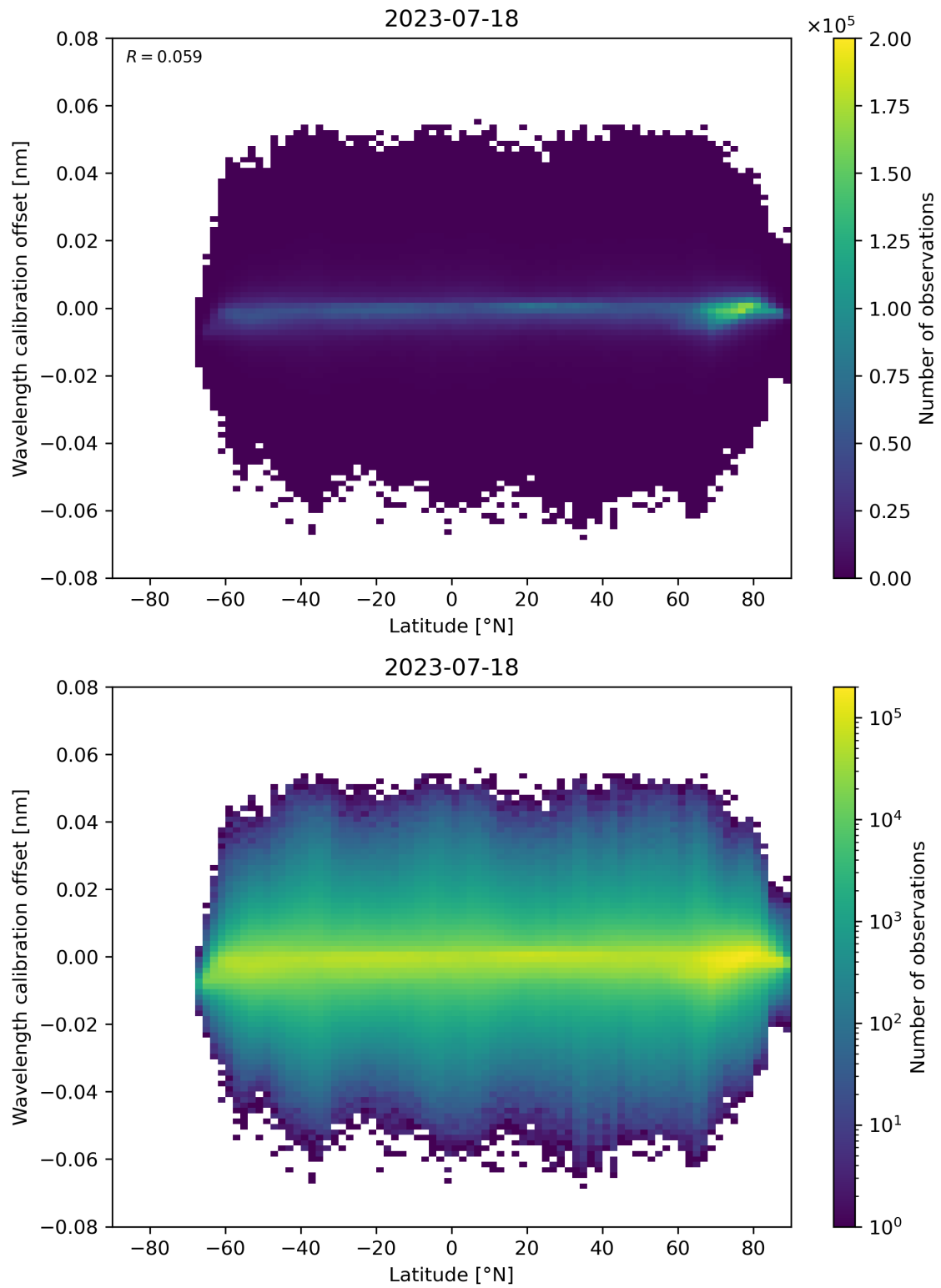
Figure 95: Scatter density plot of “Latitude” against “Wavelength calibration offset” for 2023-07-17 to 2023-07-19.
