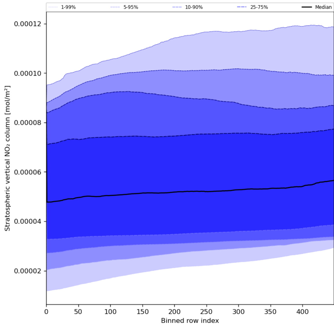
Figure 53: Along track statistics of “Stratospheric vertical NO 2 column” for 2023-07-17 to 2023-07-19
