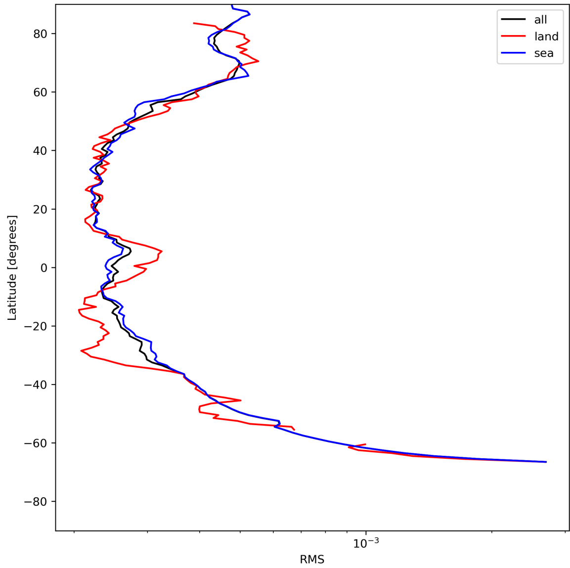
Figure 26: Zonal average of “RMS” for 2023-07-17 to 2023-07-19.
