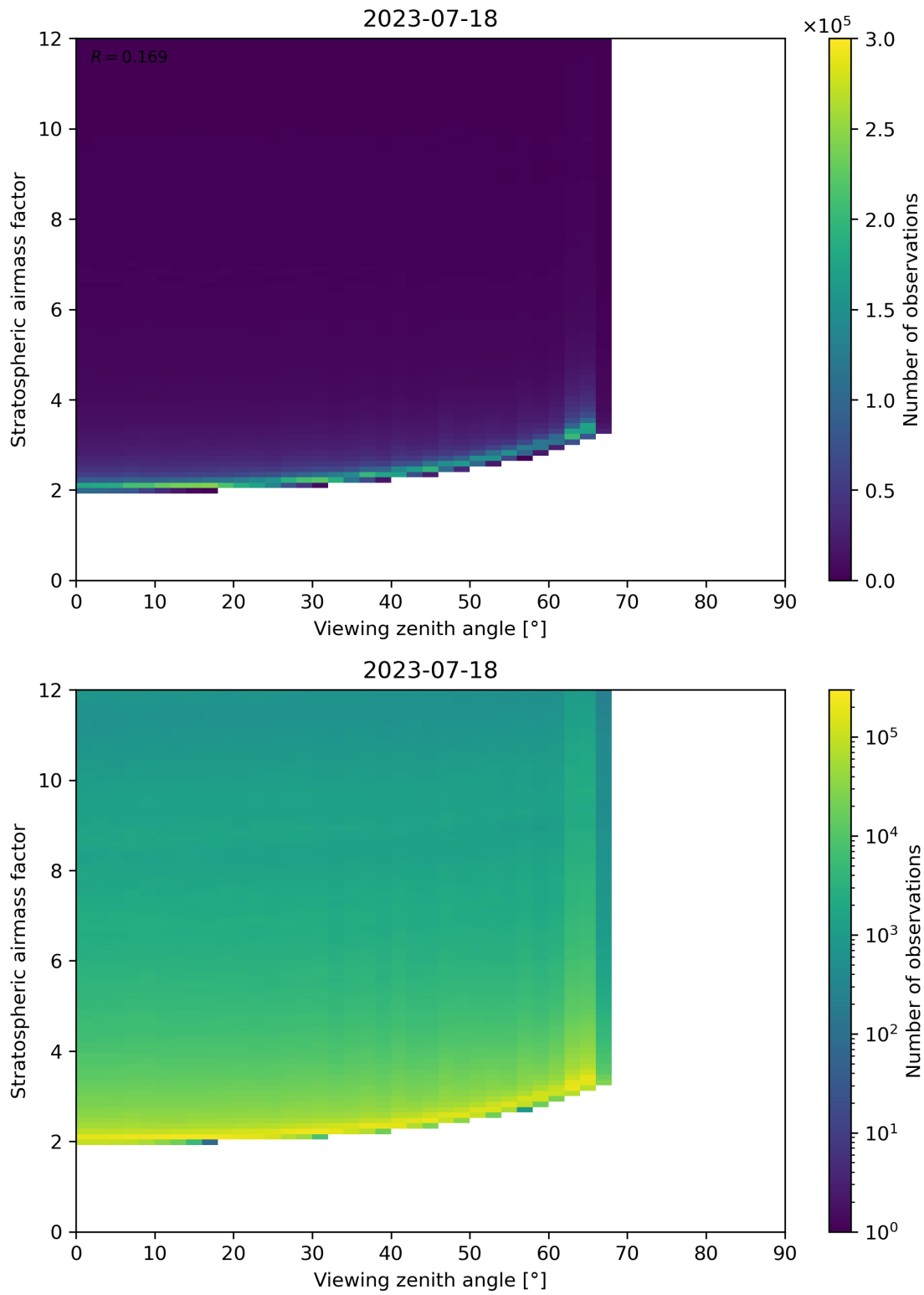
Figure 159: Scatter density plot of “Viewing zenith angle” against “Stratospheric airmass factor” for 2023-07-17 to 2023-07-19.
