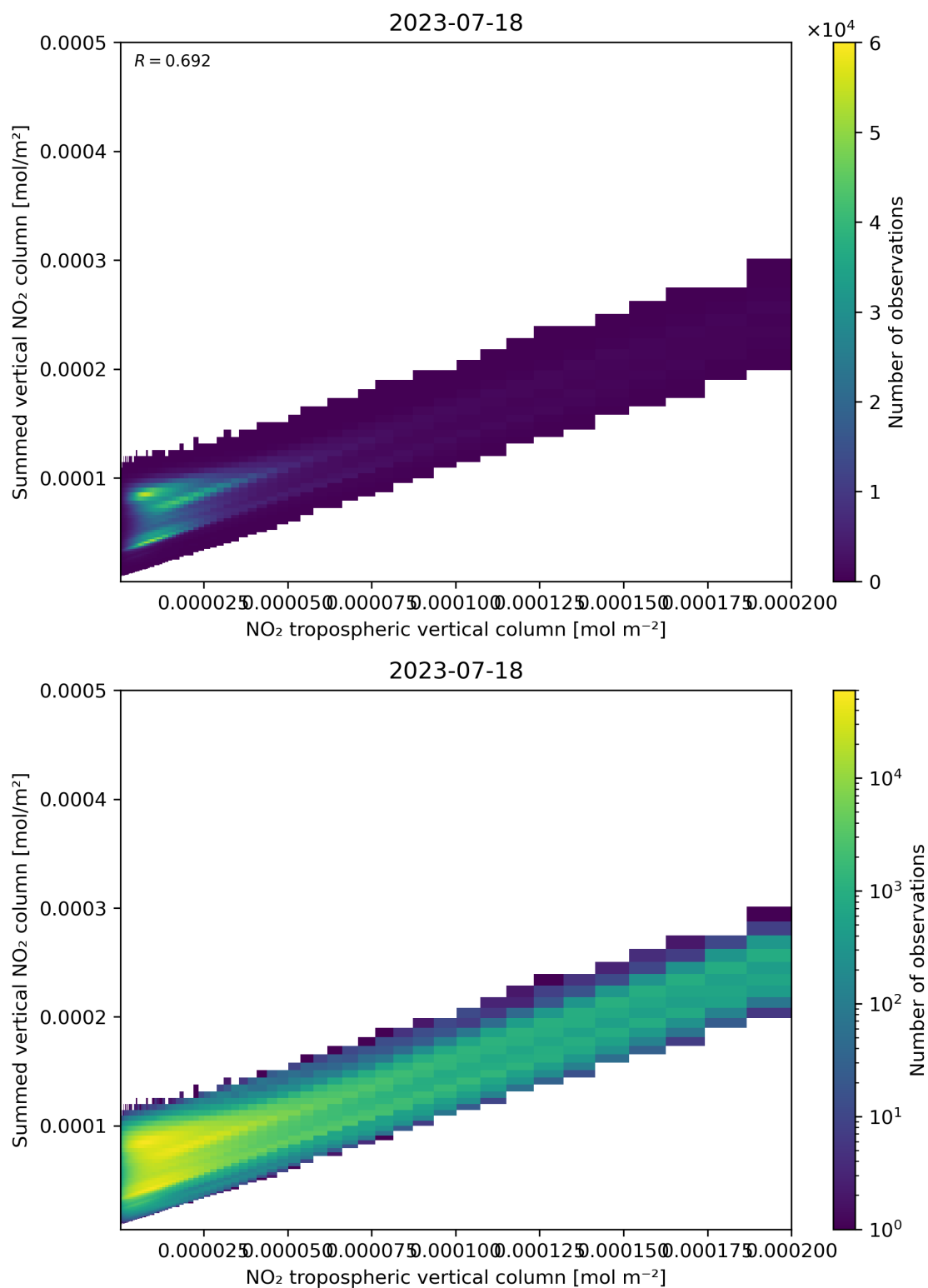
Figure 126: Scatter density plot of “NO 2 tropospheric vertical column” against “Summed vertical NO 2 column” for 2023-07-17 to 2023-07-19.
