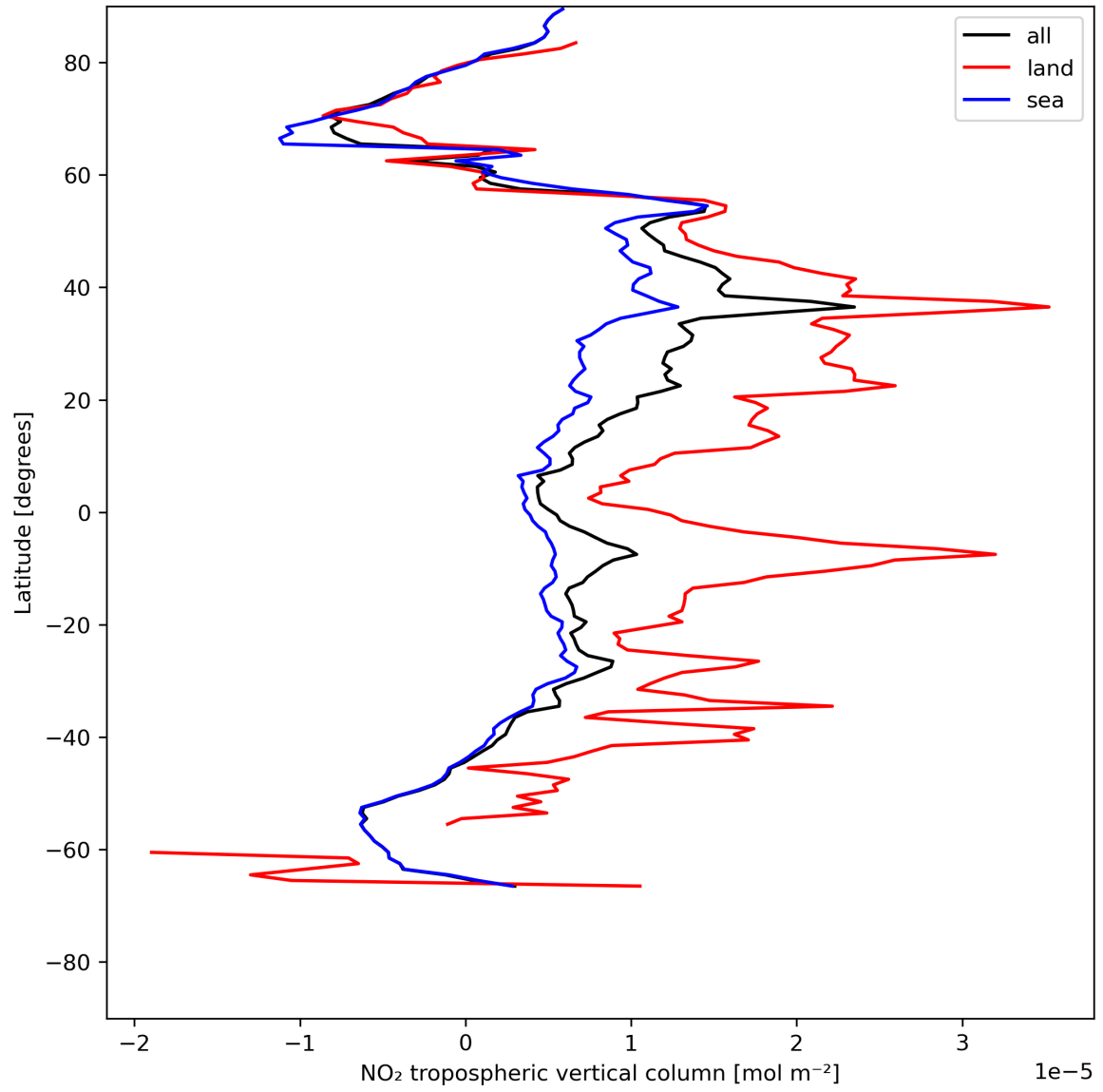
Figure 12: Zonal average of “NO 2 tropospheric vertical column” for 2023-07-17 to 2023-07-19.
