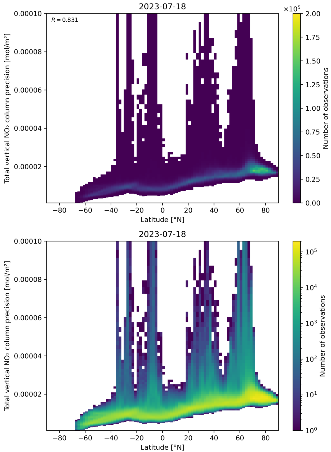
Figure 91: Scatter density plot of “Latitude” against “Total vertical NO 2 column precision” for 2023-07-17 to 2023-07-19.
