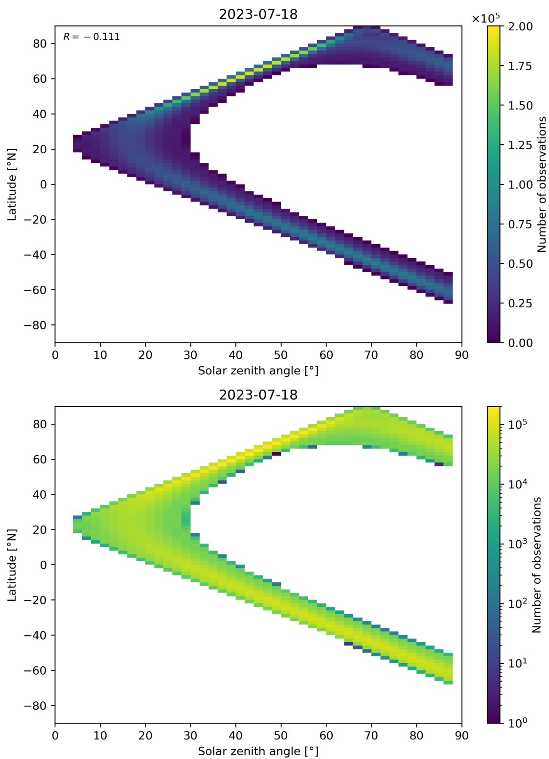
Figure 149: Scatter density plot of “Solar zenith angle” against “Latitude” for 2023-07-17 to 2023-07-19.
