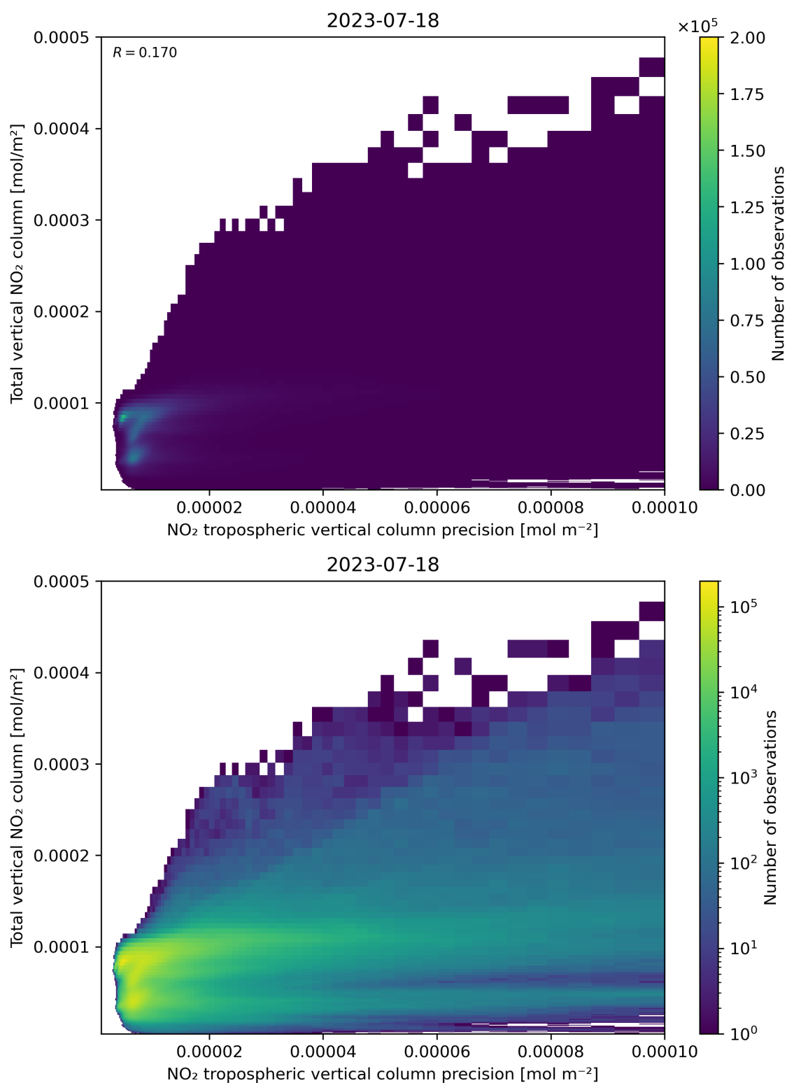
Figure 138: Scatter density plot of “NO 2 tropospheric vertical column precision” against “Total vertical NO 2 column” for 2023-07-17 to 2023-07-19.
