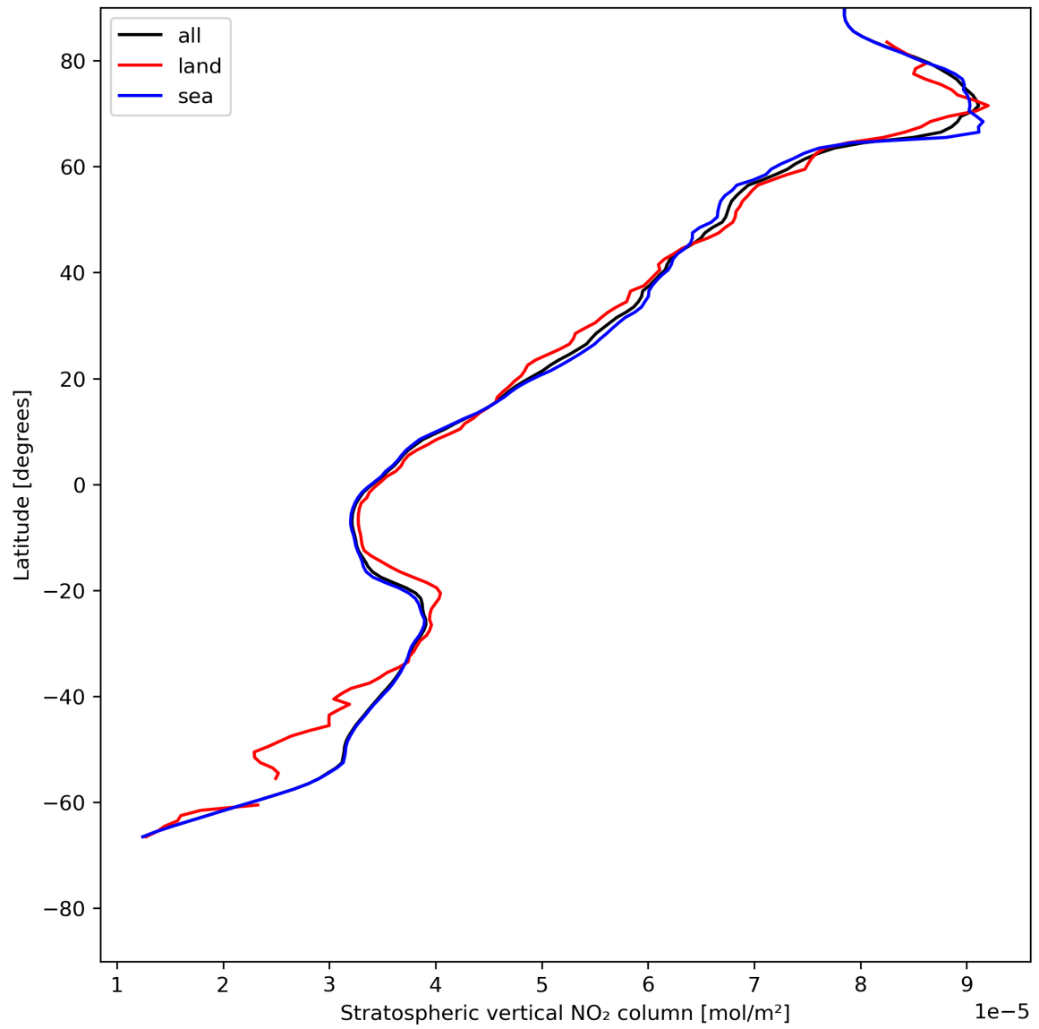
Figure 19: Zonal average of “Stratospheric vertical NO 2 column” for 2023-07-17 to 2023-07-19.
