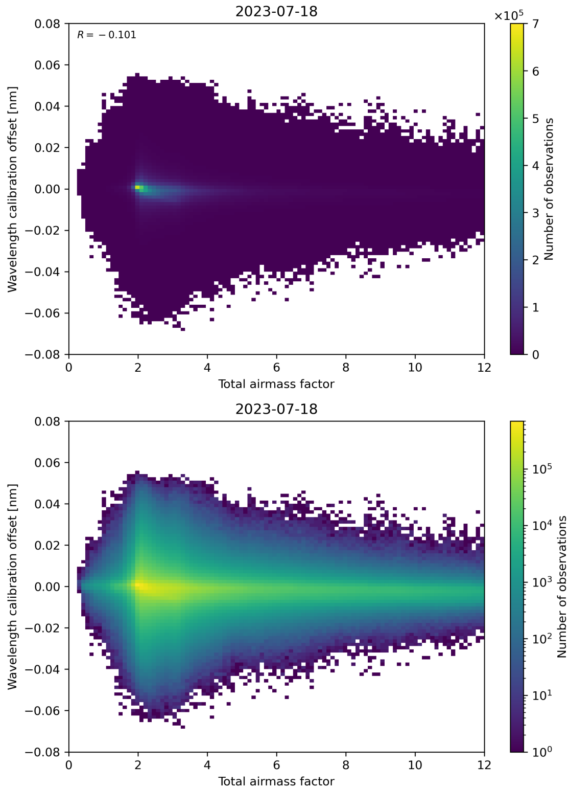
Figure 70: Scatter density plot of “Total airmass factor” against “Wavelength calibration offset” for 2023-07-17 to 2023-07-19.
