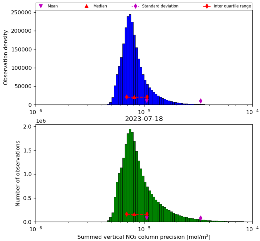
Figure 41: Histogram of "Summed vertical NO 2 column precision" for 2023-07-17 to 2023-07-19
