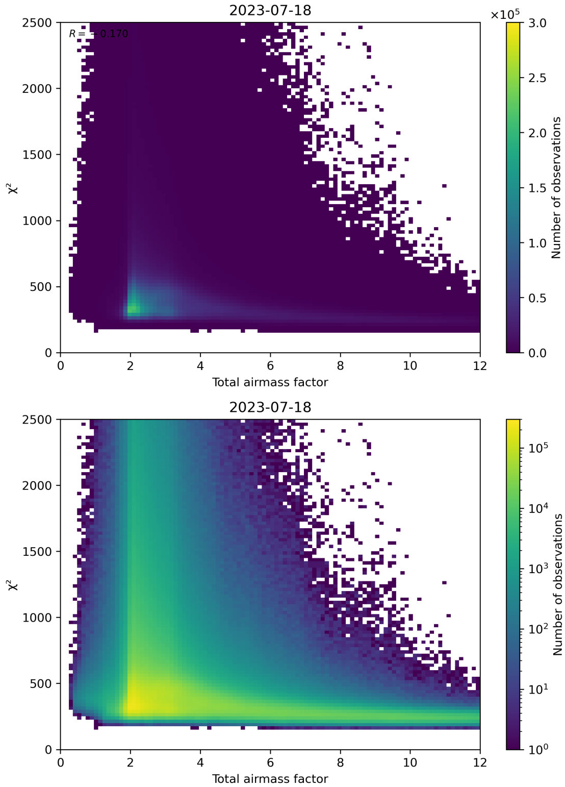
Figure 63: Scatter density plot of “Total airmass factor” against “ \chi^2 ” for 2023-07-17 to 2023-07-19.
