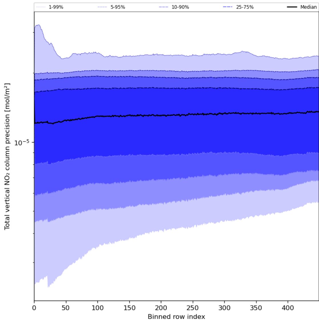
Figure 56: Along track statistics of “Total vertical NO 2 column precision” for 2023-07-17 to 2023-07-19
