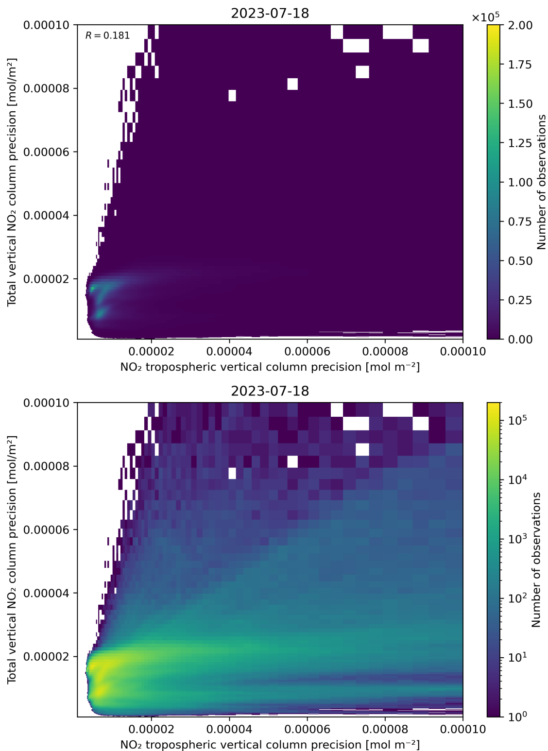
Figure 139: Scatter density plot of “NO 2 tropospheric vertical column precision” against “Total vertical NO 2 column precision” for 2023-07-17 to 2023-07-19.
