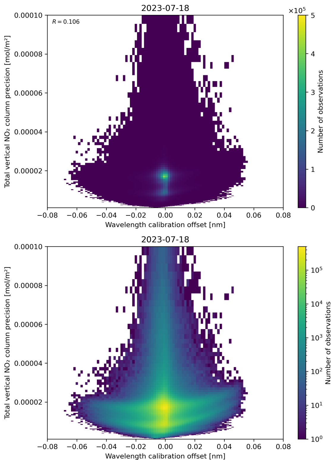
Figure 180: Scatter density plot of “Wavelength calibration offset” against “Total vertical NO 2 column precision” for 2023-07-17 to 2023-07-19.
