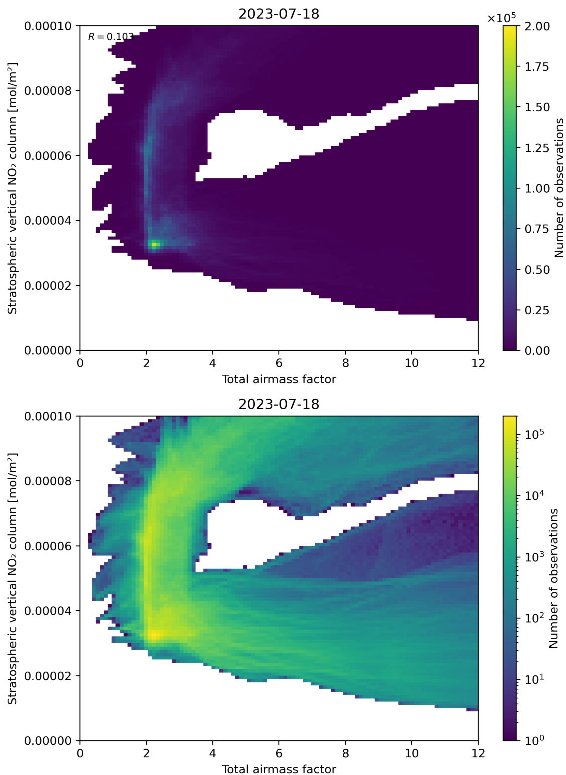
Figure 64: Scatter density plot of “Total airmass factor” against “Stratospheric vertical NO 2 column” for 2023-07-17 to 2023-07-19.
