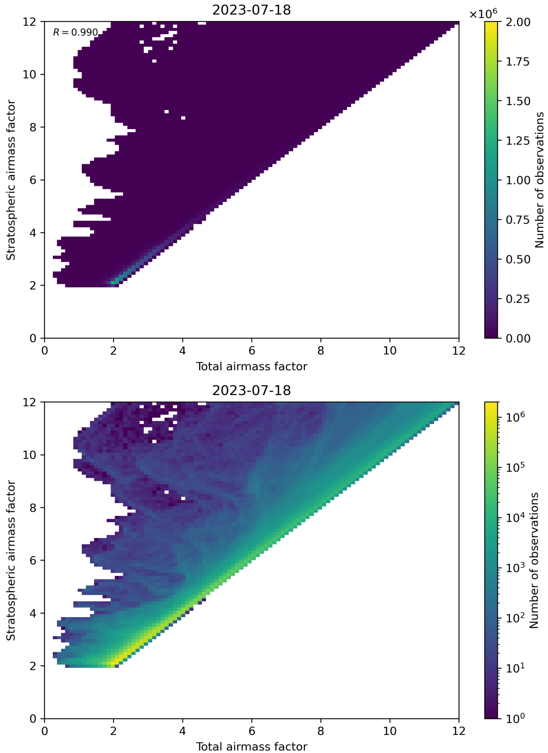
Figure 62: Scatter density plot of “Total airmass factor” against “Stratospheric airmass factor” for 2023-07-17 to 2023-07-19.
