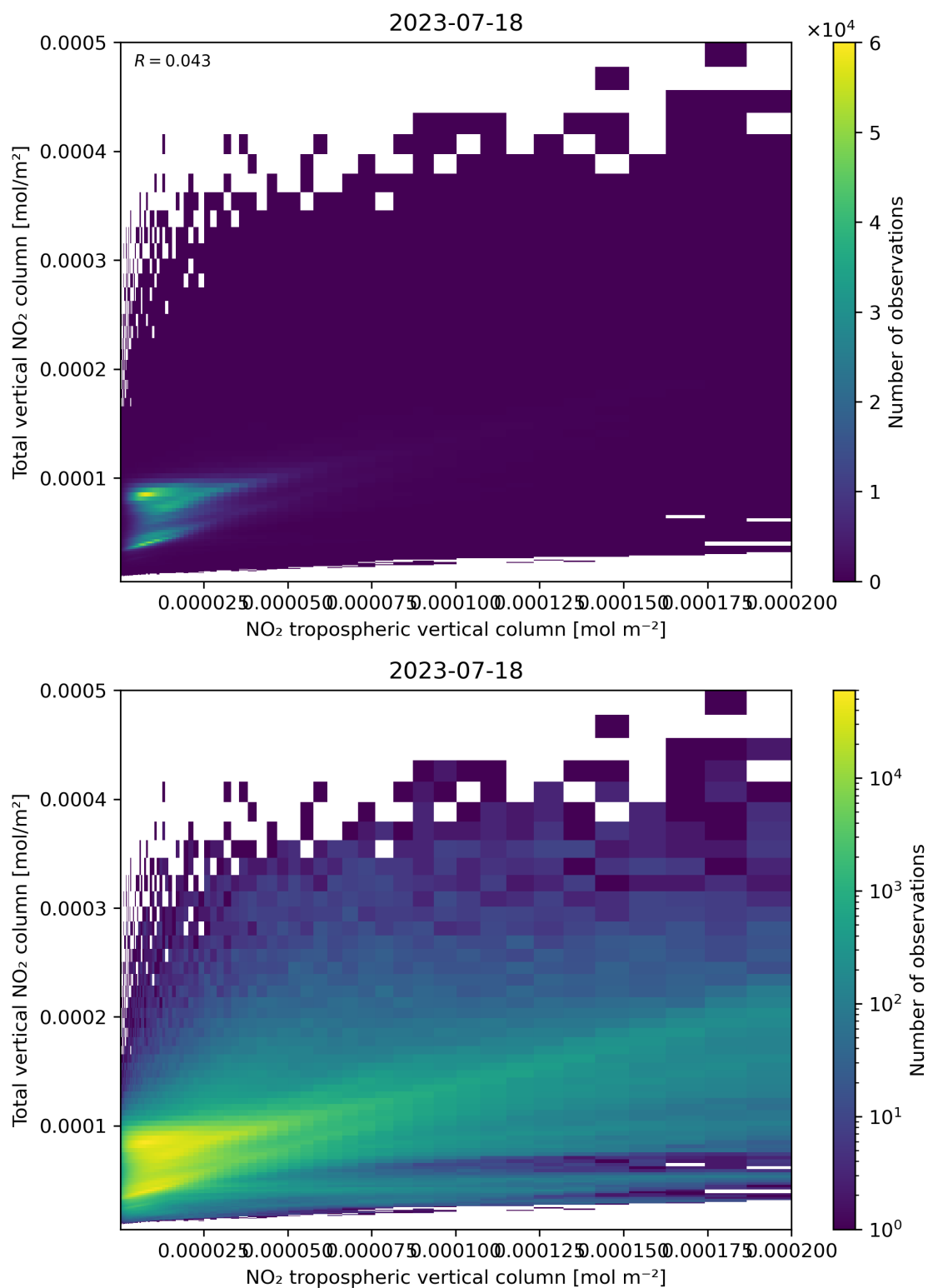
Figure 128: Scatter density plot of “NO 2 tropospheric vertical column” against “Total vertical NO 2 column” for 2023-07-17 to 2023-07-19.
