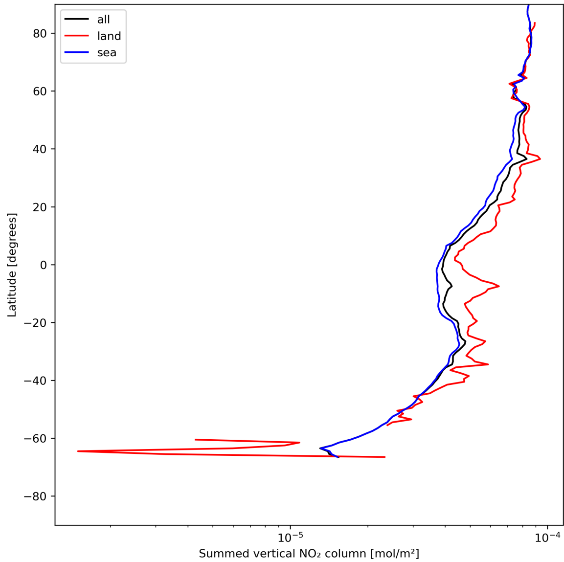
Figure 23: Zonal average of “Summed vertical NO 2 column” for 2023-07-17 to 2023-07-19.
