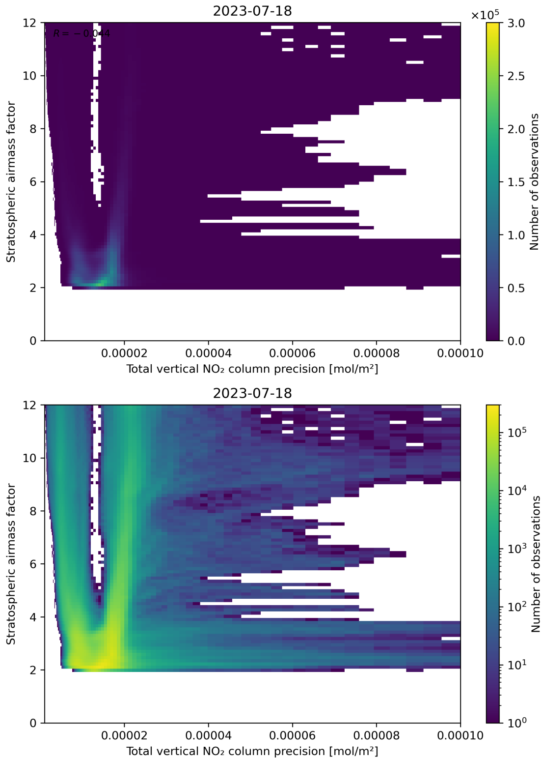
Figure 115: Scatter density plot of “Total vertical NO 2 column precision” against “Stratospheric airmass factor” for 2023-07-17 to 2023-07-19.
