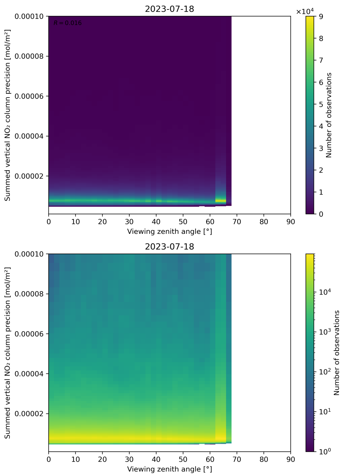
Figure 166: Scatter density plot of “Viewing zenith angle” against “Summed vertical NO 2 column precision” for 2023-07-17 to 2023-07-19.
