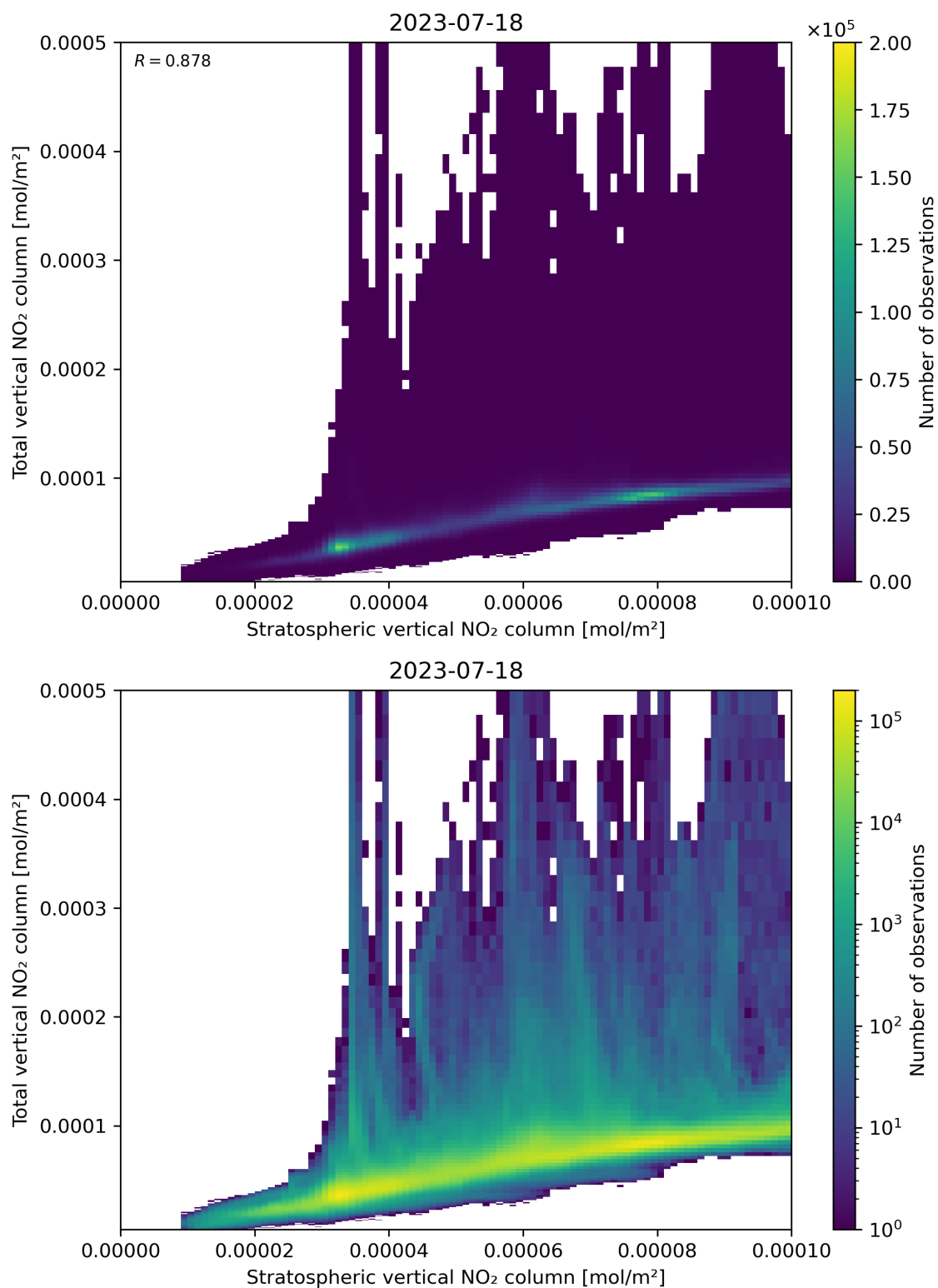
Figure 100: Scatter density plot of “Stratospheric vertical NO 2 column” against “Total vertical NO 2 column” for 2023-07-17 to 2023-07-19.
