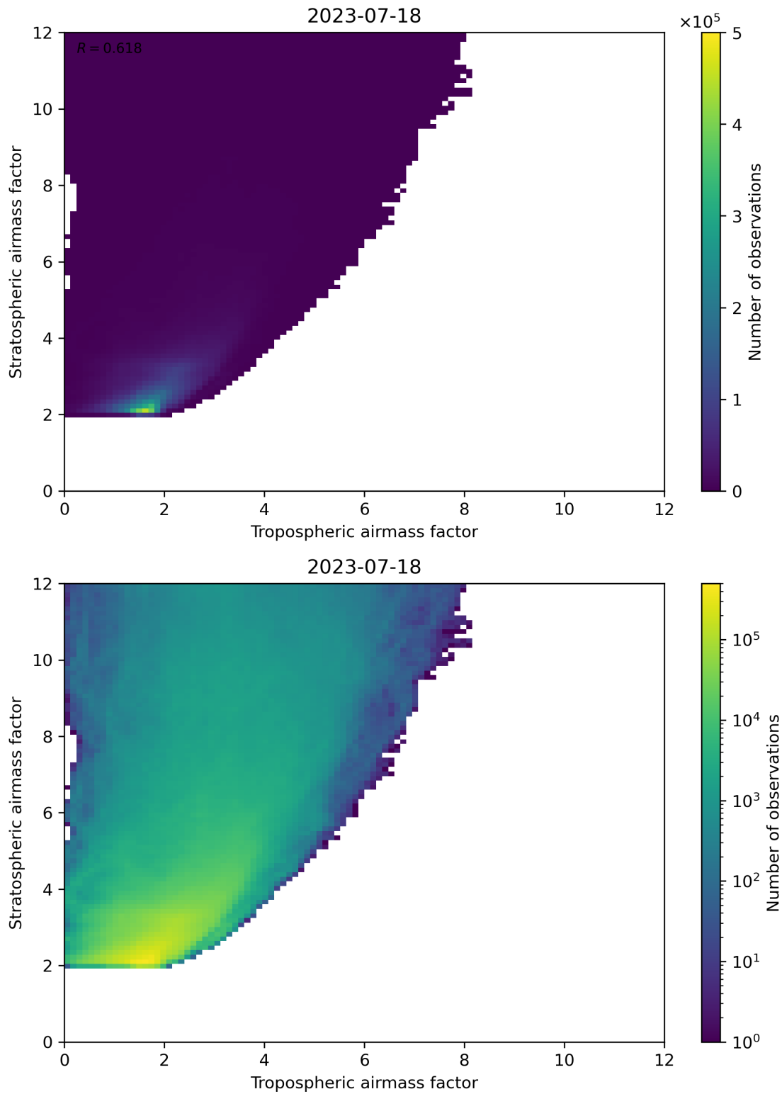
Figure 71: Scatter density plot of “Tropospheric airmass factor” against “Stratospheric airmass factor” for 2023-07-17 to 2023-07-19.
