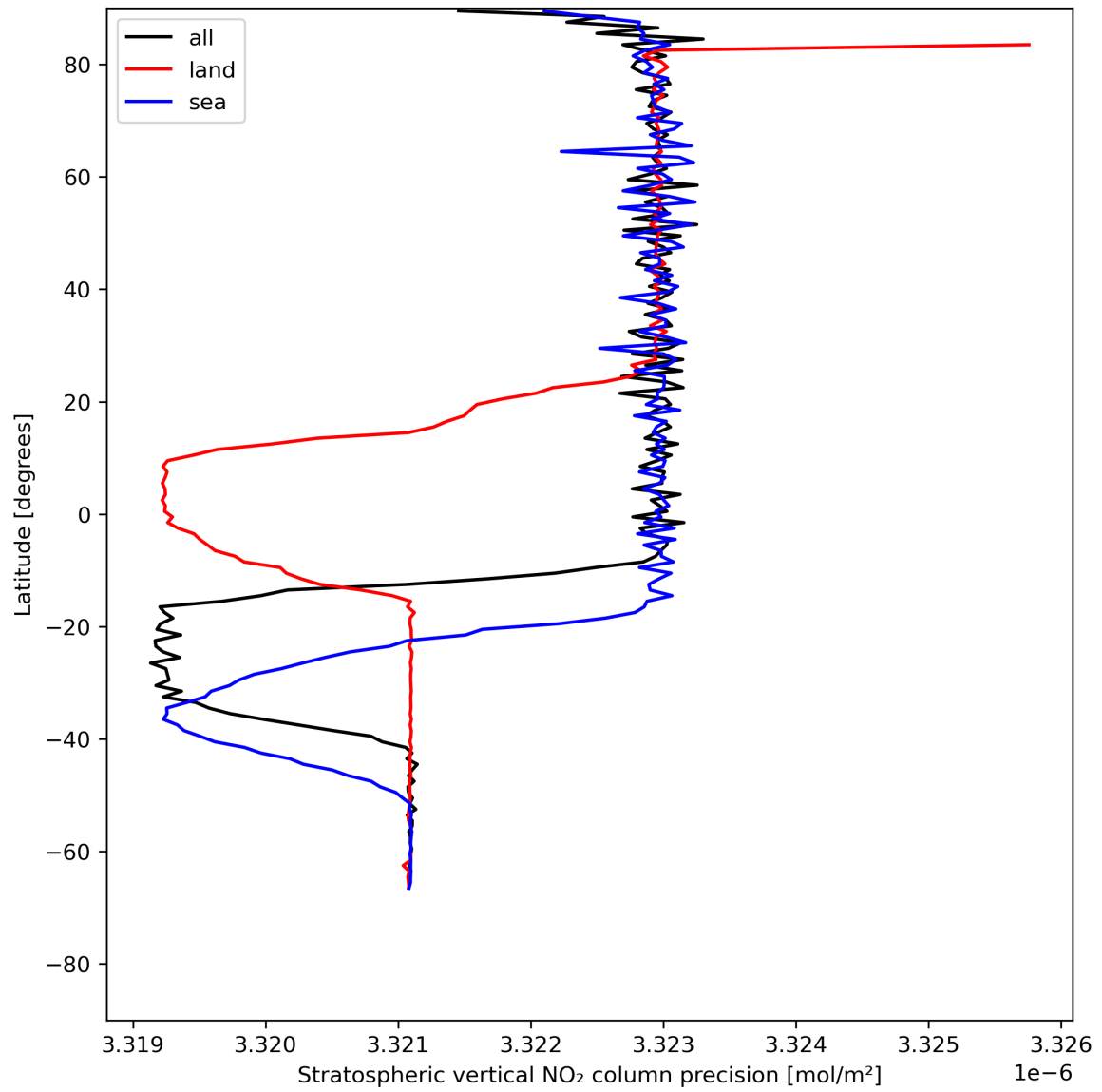
Figure 20: Zonal average of “Stratospheric vertical NO 2 column precision” for 2023-07-17 to 2023-07-19.
