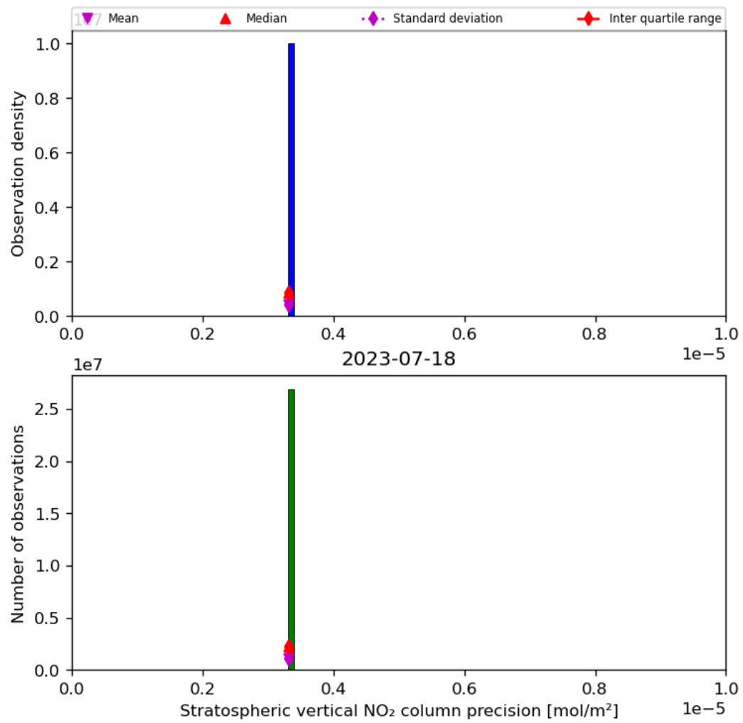
Figure 37: Histogram of “Stratospheric vertical NO 2 column precision” for 2023-07-17 to 2023-07-19
