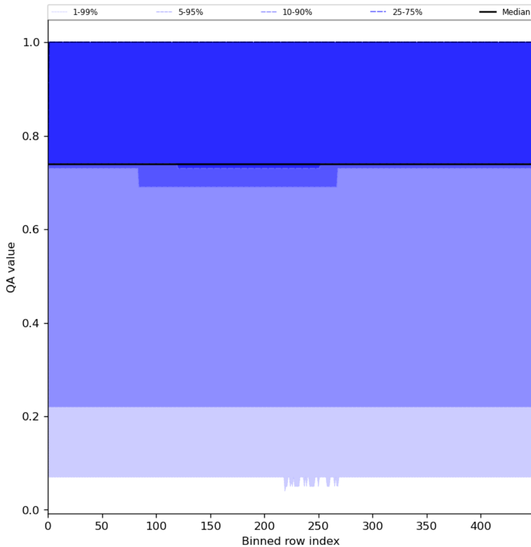
Figure 45: Along track statistics of “QA value” for 2023-07-17 to 2023-07-19
