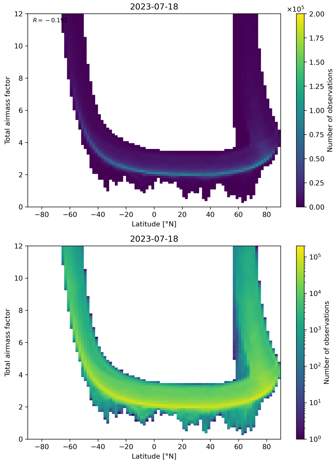
Figure 84: Scatter density plot of “Latitude” against “Total airmass factor” for 2023-07-17 to 2023-07-19.
