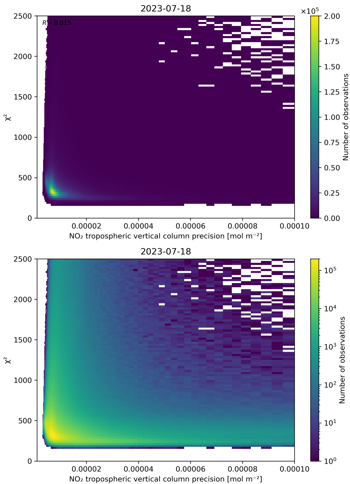
Figure 134: Scatter density plot of “NO 2 tropospheric vertical column precision” against “ \chi^2 ” for 2023-07-17 to 2023-07-19.
