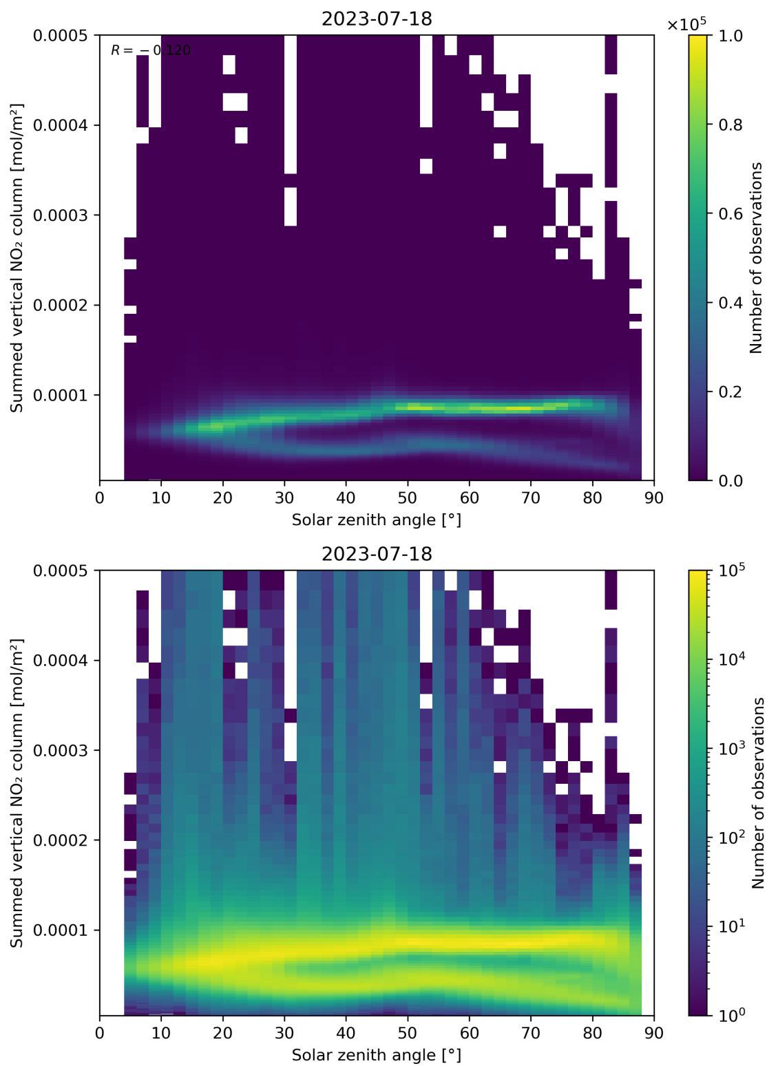
Figure 151: Scatter density plot of “Solar zenith angle” against “Summed vertical NO 2 column” for 2023-07-17 to 2023-07-19.
