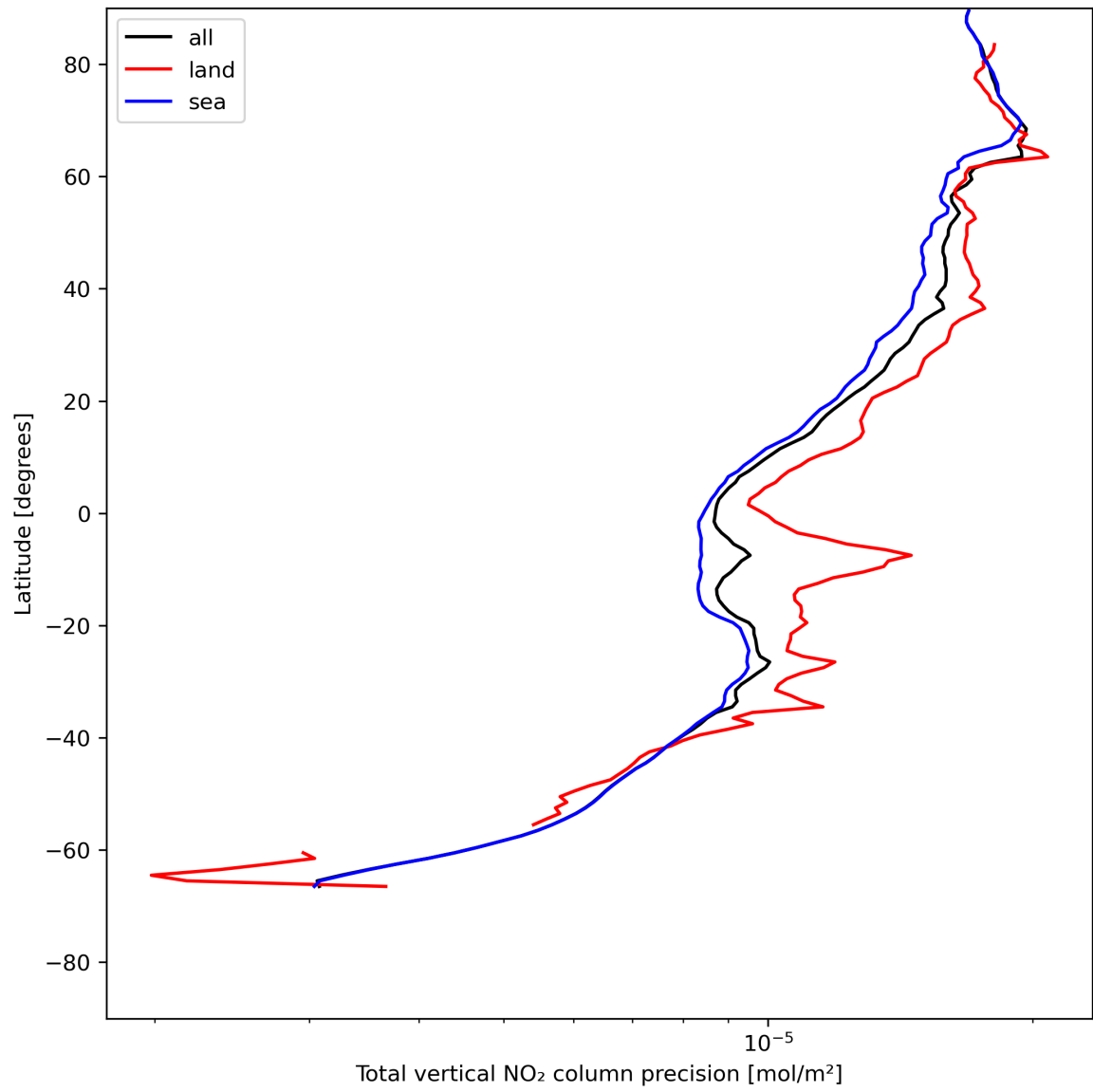
Figure 22: Zonal average of “Total vertical NO 2 column precision” for 2023-07-17 to 2023-07-19.
