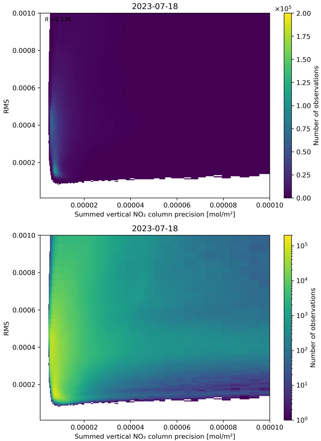
Figure 108: Scatter density plot of “Summed vertical NO 2 column precision” against “RMS” for 2023-07-17 to 2023-07-19.
