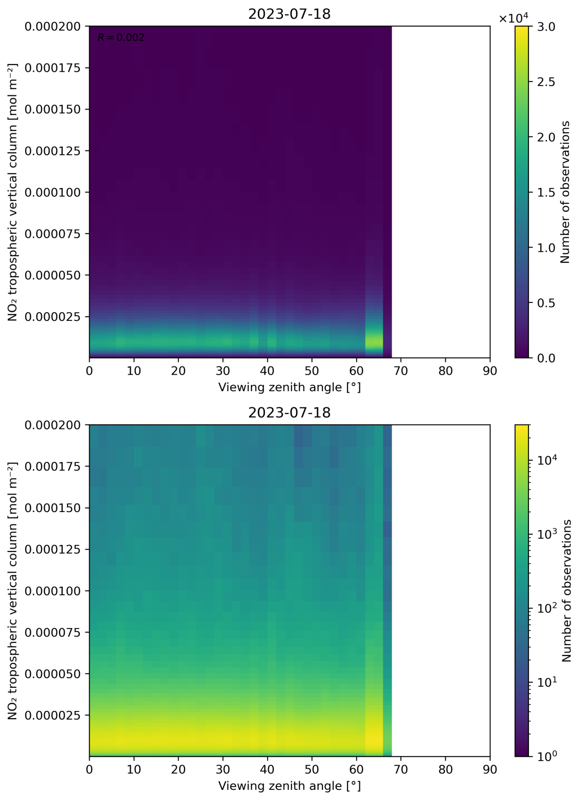
Figure 169: Scatter density plot of “Viewing zenith angle” against “NO 2 tropospheric vertical column” for 2023-07-17 to 2023-07-19.
