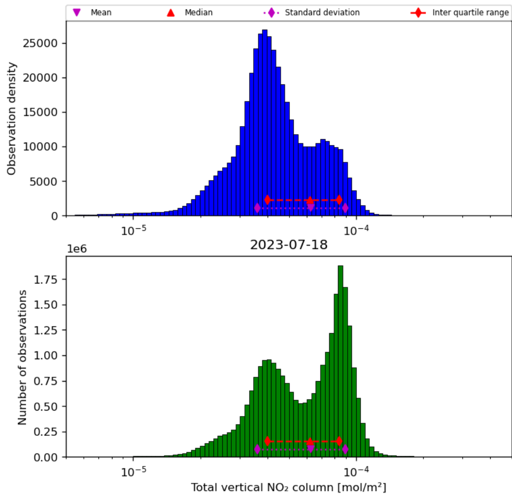
Figure 38: Histogram of “Total vertical NO 2 column” for 2023-07-17 to 2023-07-19
