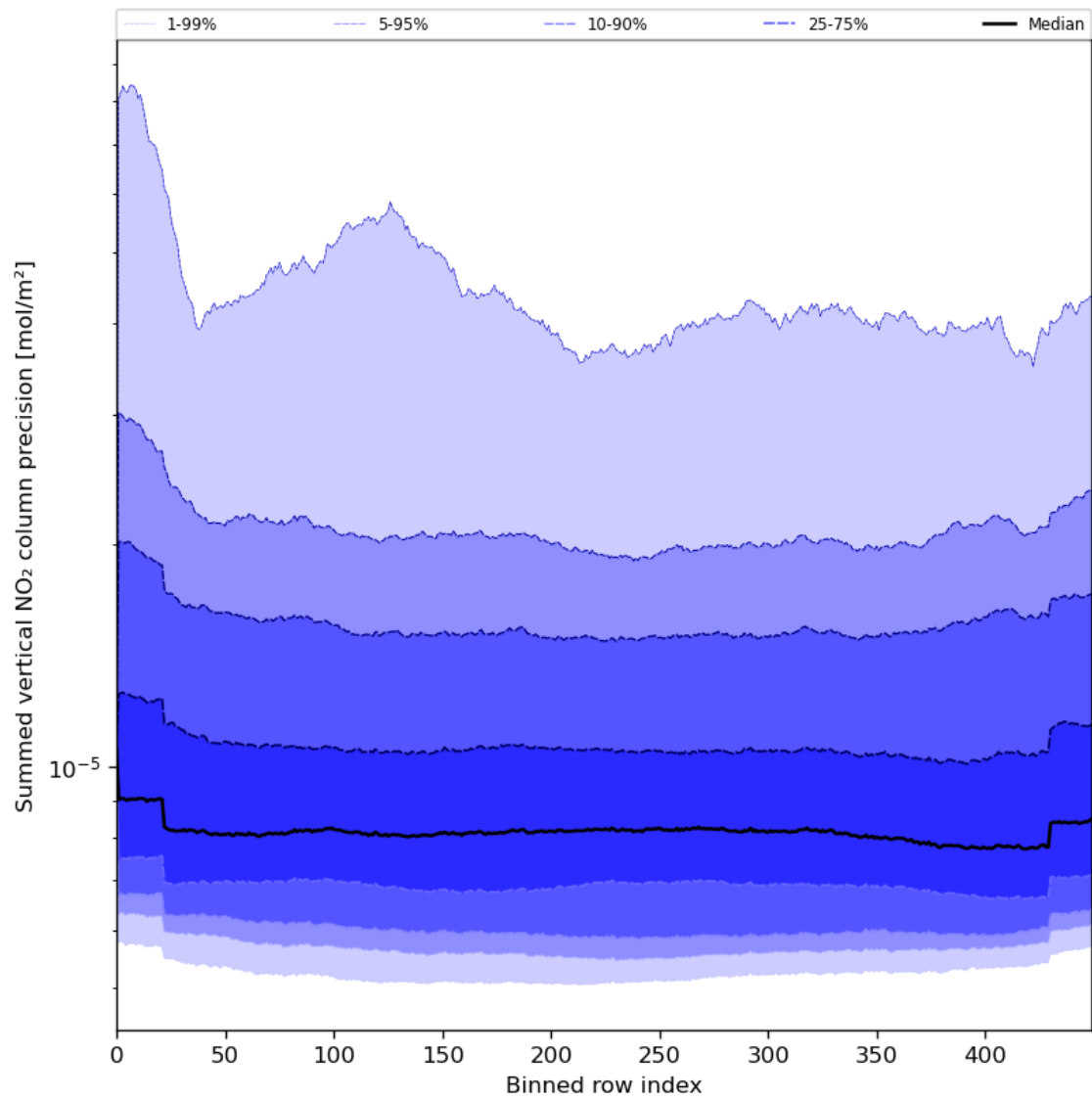
Figure 58: Along track statistics of “Summed vertical NO 2 column precision” for 2023-07-17 to 2023-07-19
