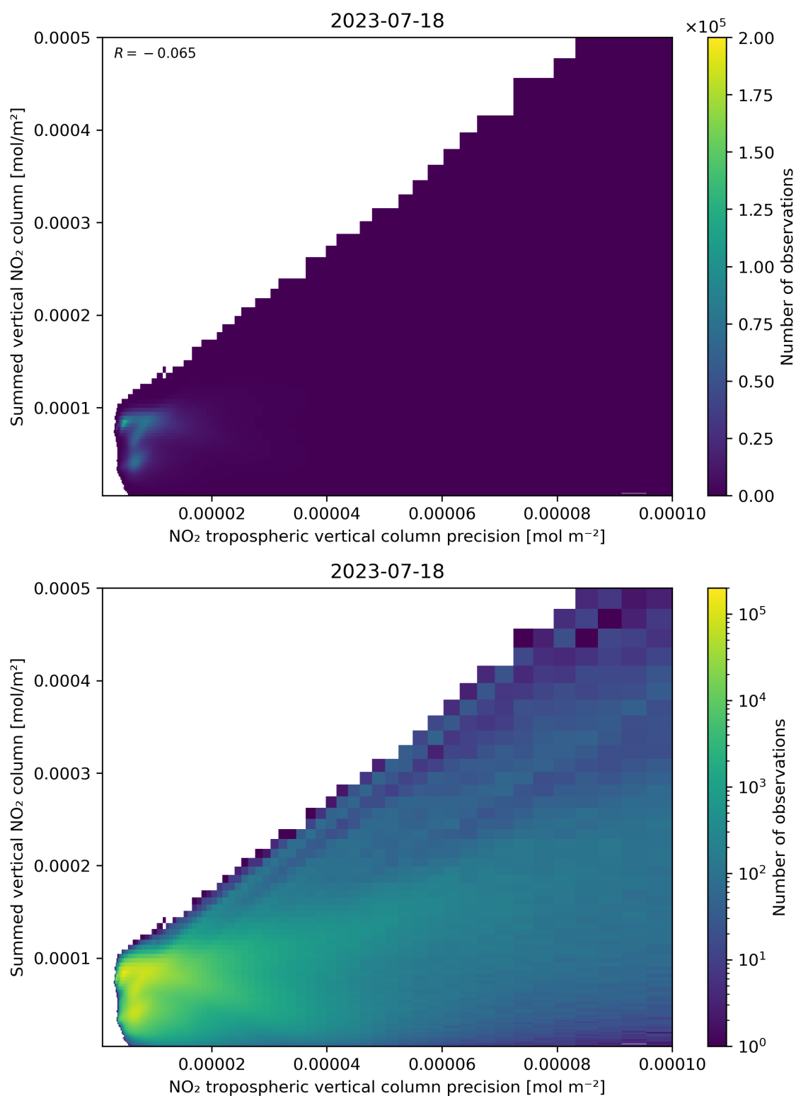
Figure 136: Scatter density plot of “NO 2 tropospheric vertical column precision” against “Summed vertical NO 2 column” for 2023-07-17 to 2023-07-19.
