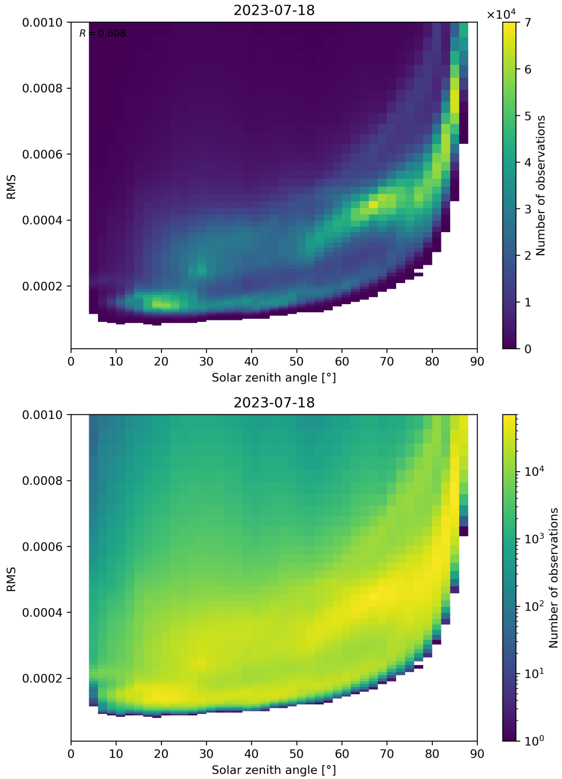
Figure 157: Scatter density plot of “Solar zenith angle” against “RMS” for 2023-07-17 to 2023-07-19.
