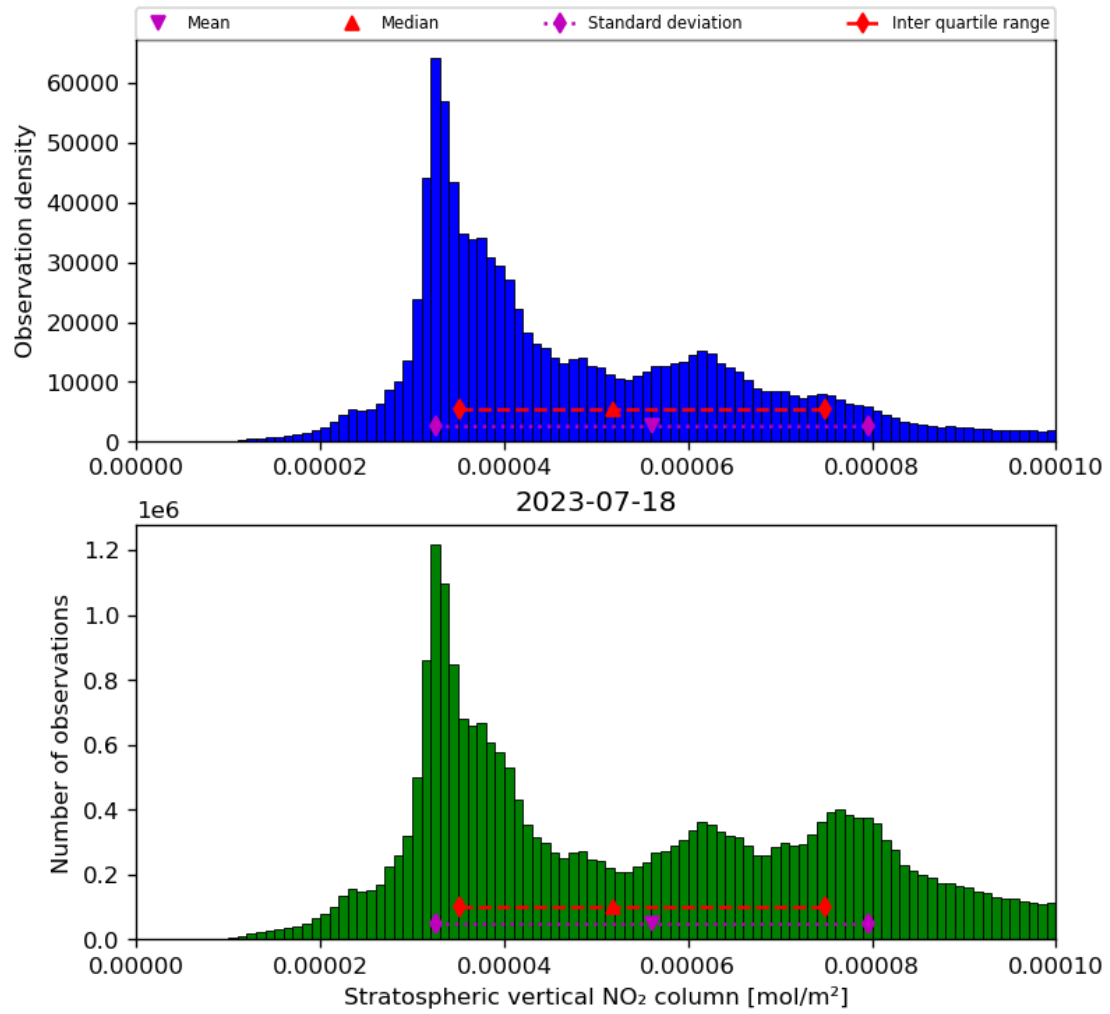
Figure 36: Histogram of “Stratospheric vertical NO 2 column” for 2023-07-17 to 2023-07-19
