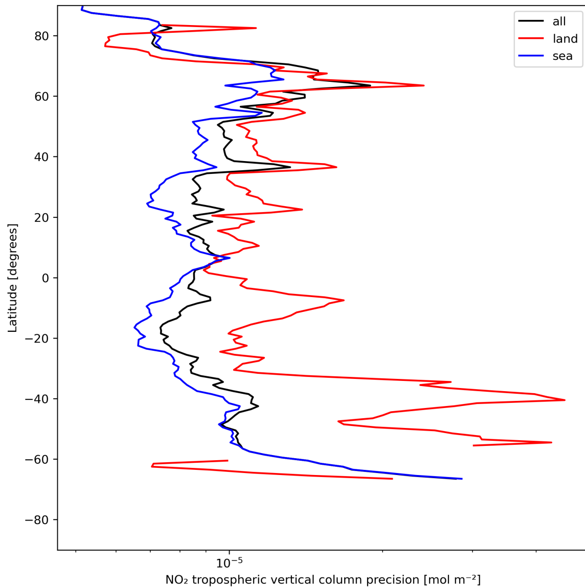
Figure 13: Zonal average of “NO 2 tropospheric vertical column precision” for 2023-07-17 to 2023-07-19.
