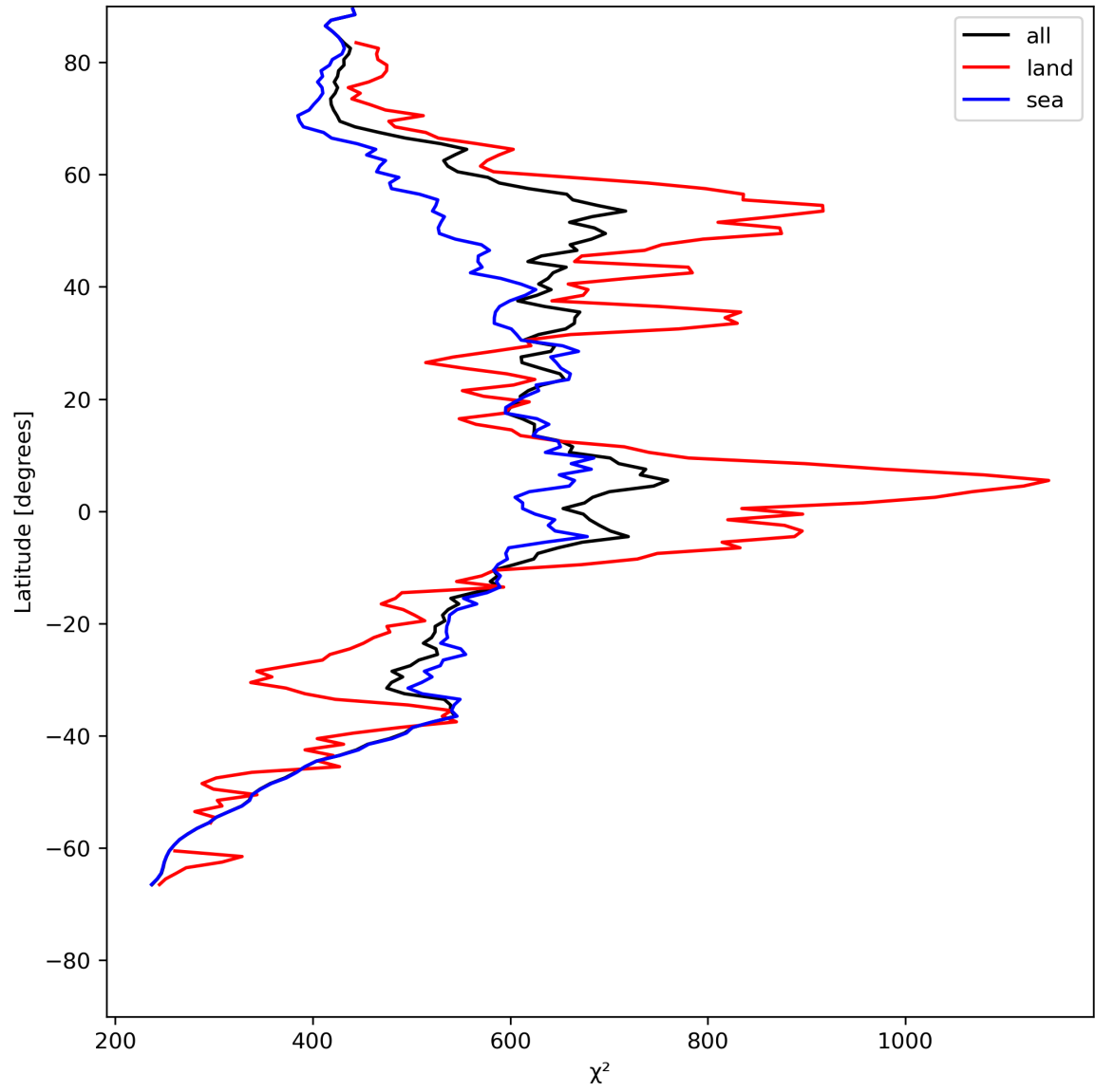
Figure 25: Zonal average of “ \chi^2 ” for 2023-07-17 to 2023-07-19.
