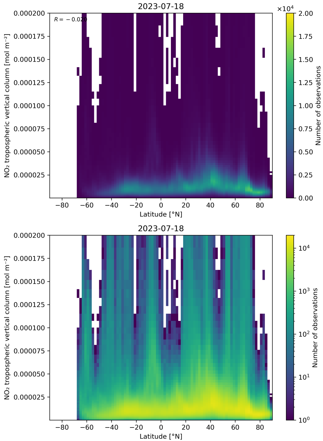
Figure 92: Scatter density plot of “Latitude” against “NO 2 tropospheric vertical column” for 2023-07-17 to 2023-07-19.
