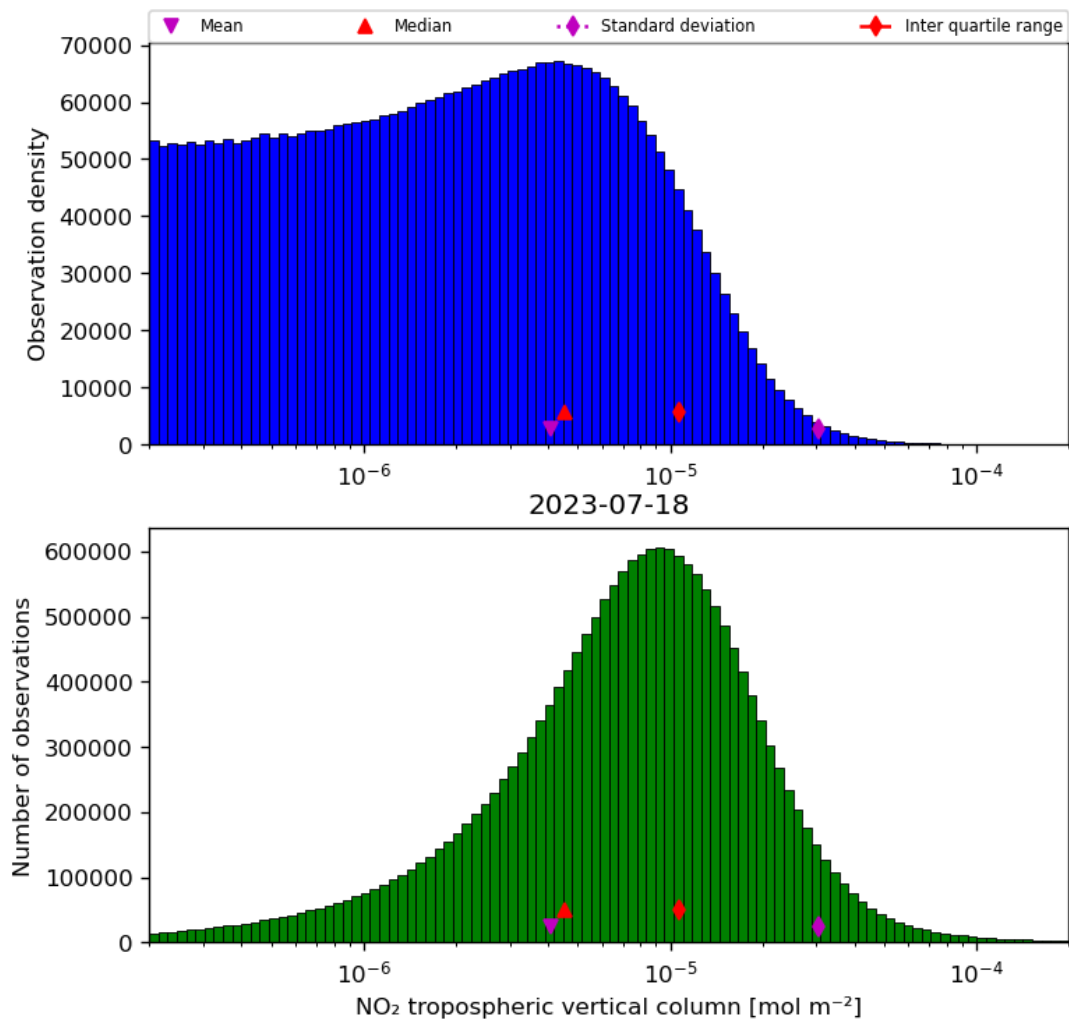
Figure 29: Histogram of “NO 2 tropospheric vertical column” for 2023-07-17 to 2023-07-19
