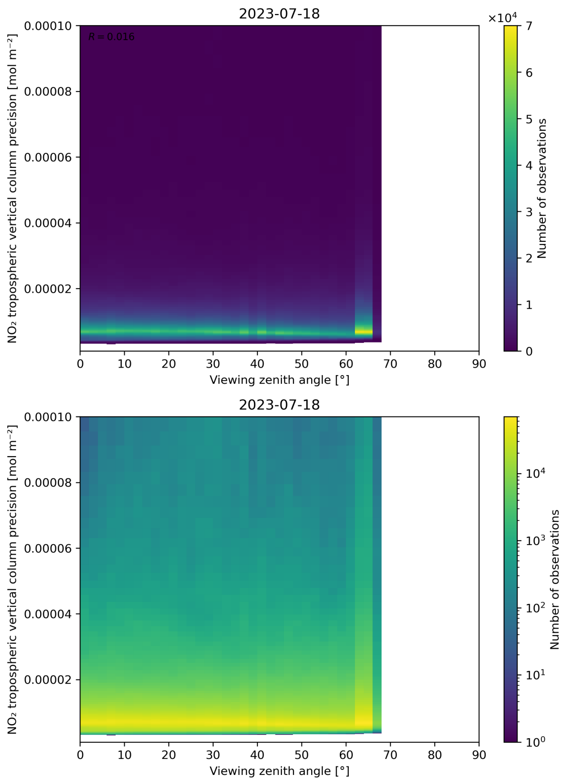
Figure 170: Scatter density plot of “Viewing zenith angle” against “NO 2 tropospheric vertical column precision” for 2023-07-17 to 2023-07-19.
