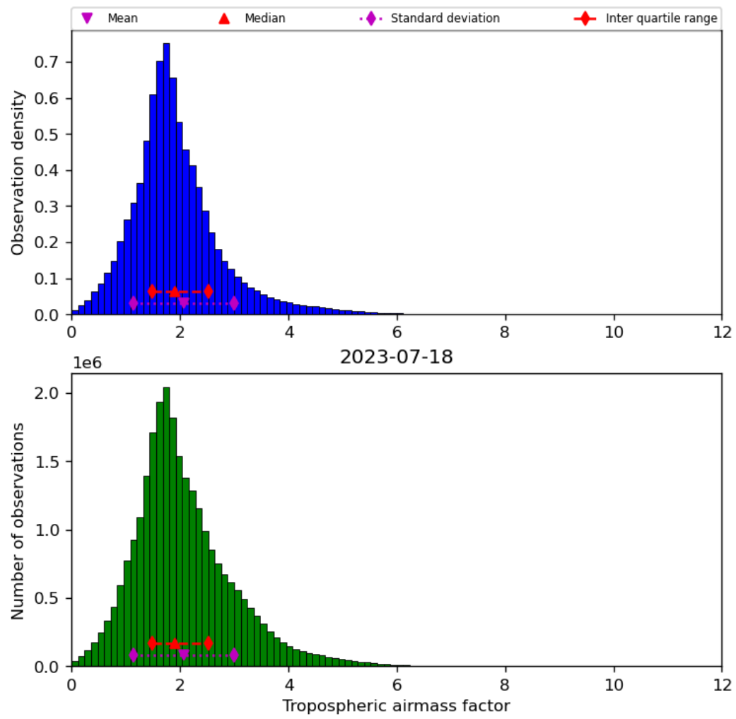
Figure 31: Histogram of “Tropospheric airmass factor” for 2023-07-17 to 2023-07-19
