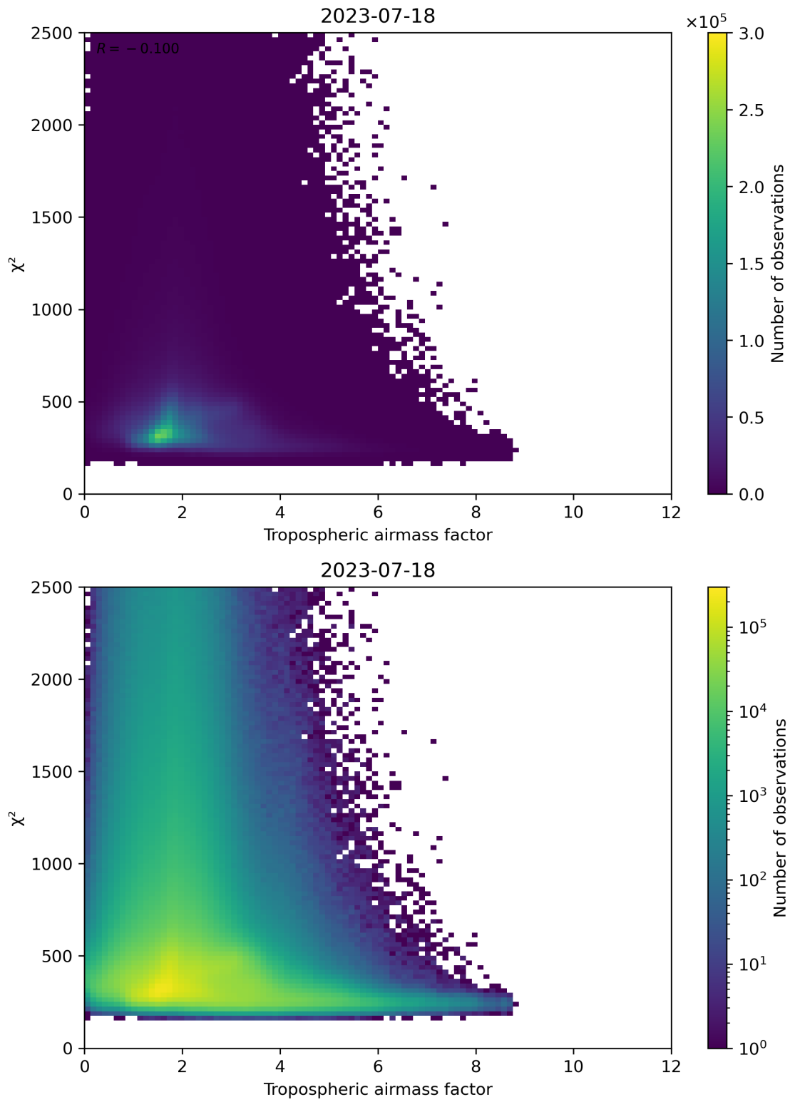
Figure 73: Scatter density plot of “Tropospheric airmass factor” against “ \chi^2 ” for 2023-07-17 to 2023-07-19.
