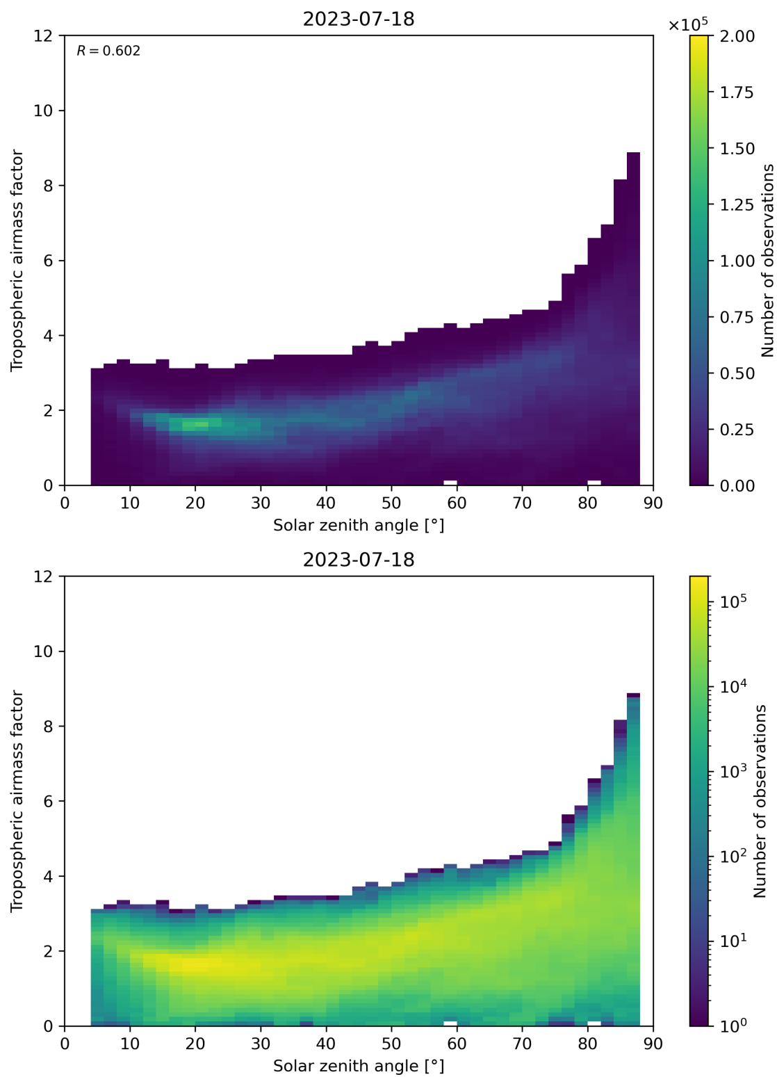
Figure 147: Scatter density plot of “Solar zenith angle” against “Tropospheric airmass factor” for 2023-07-17 to 2023-07-19.
