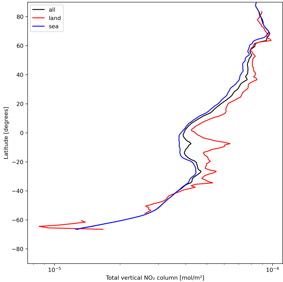
Figure 21: Zonal average of “Total vertical NO 2 column” for 2023-07-17 to 2023-07-19.
