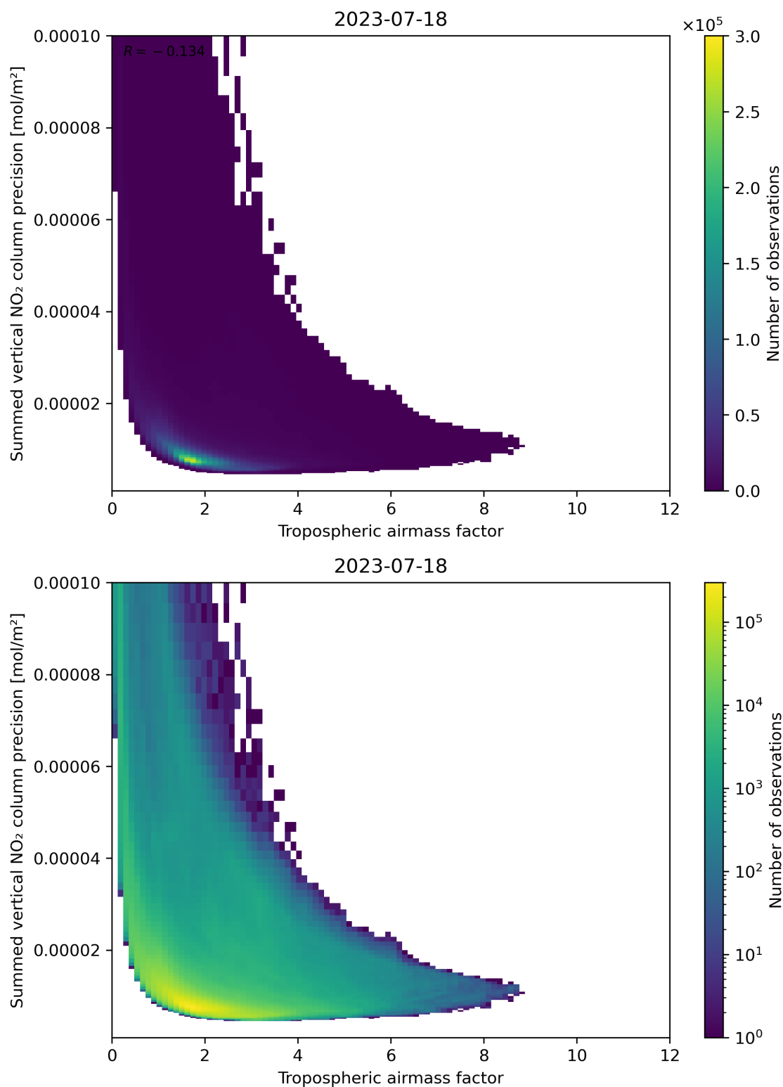
Figure 76: Scatter density plot of “Tropospheric air mass factor” against “Summed vertical NO 2 column precision” for 2023-07-17 to 2023-07-19.
