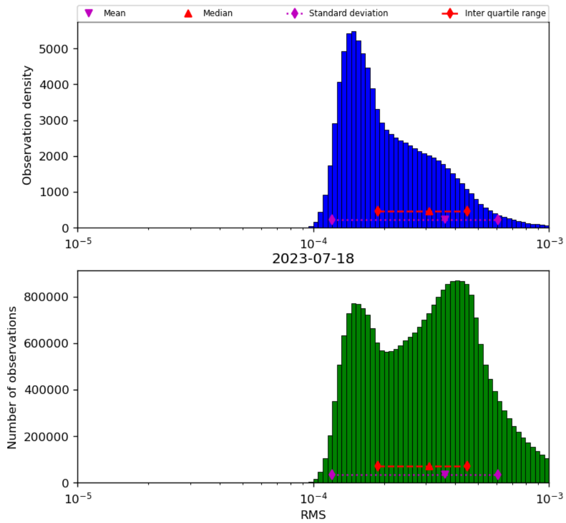
Figure 43: Histogram of “RMS” for 2023-07-17 to 2023-07-19
