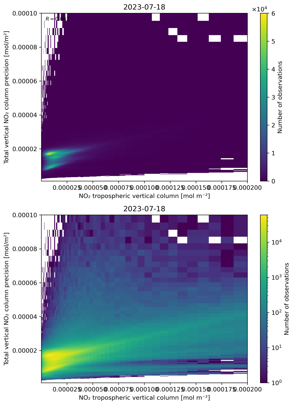
Figure 129: Scatter density plot of “NO 2 tropospheric vertical column” against “Total vertical NO 2 column precision” for 2023-07-17 to 2023-07-19.
