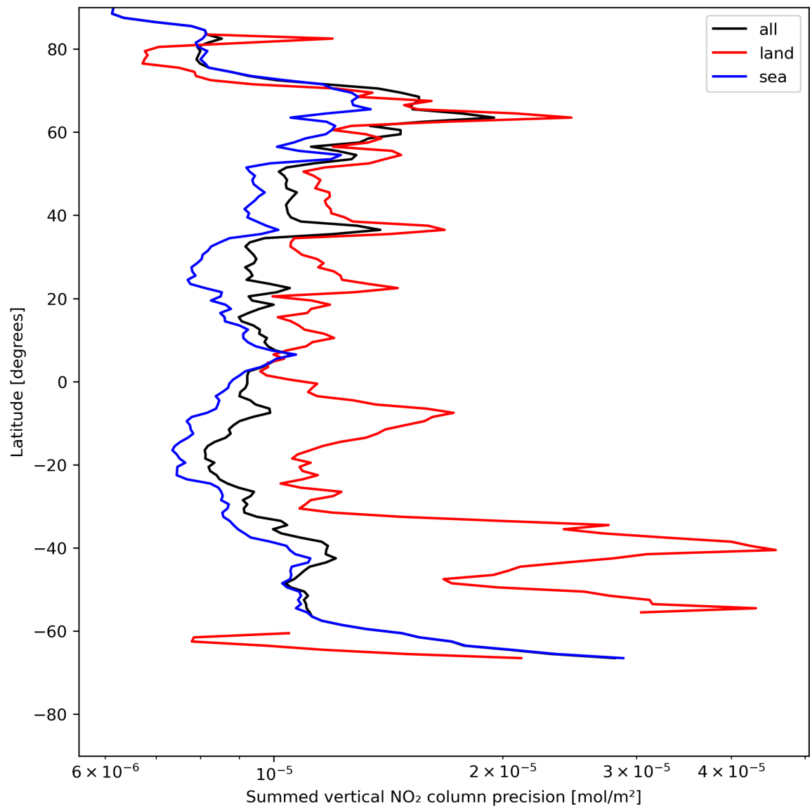
Figure 24: Zonal average of “Summed vertical NO 2 column precision” for 2023-07-17 to 2023-07-19.
