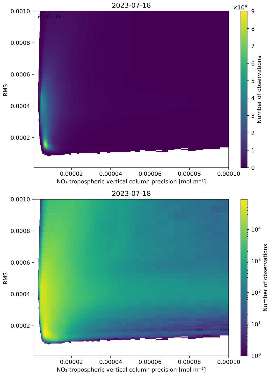
Figure 140: Scatter density plot of “NO 2 tropospheric vertical column precision” against “RMS” for 2023-07-17 to 2023-07-19.
