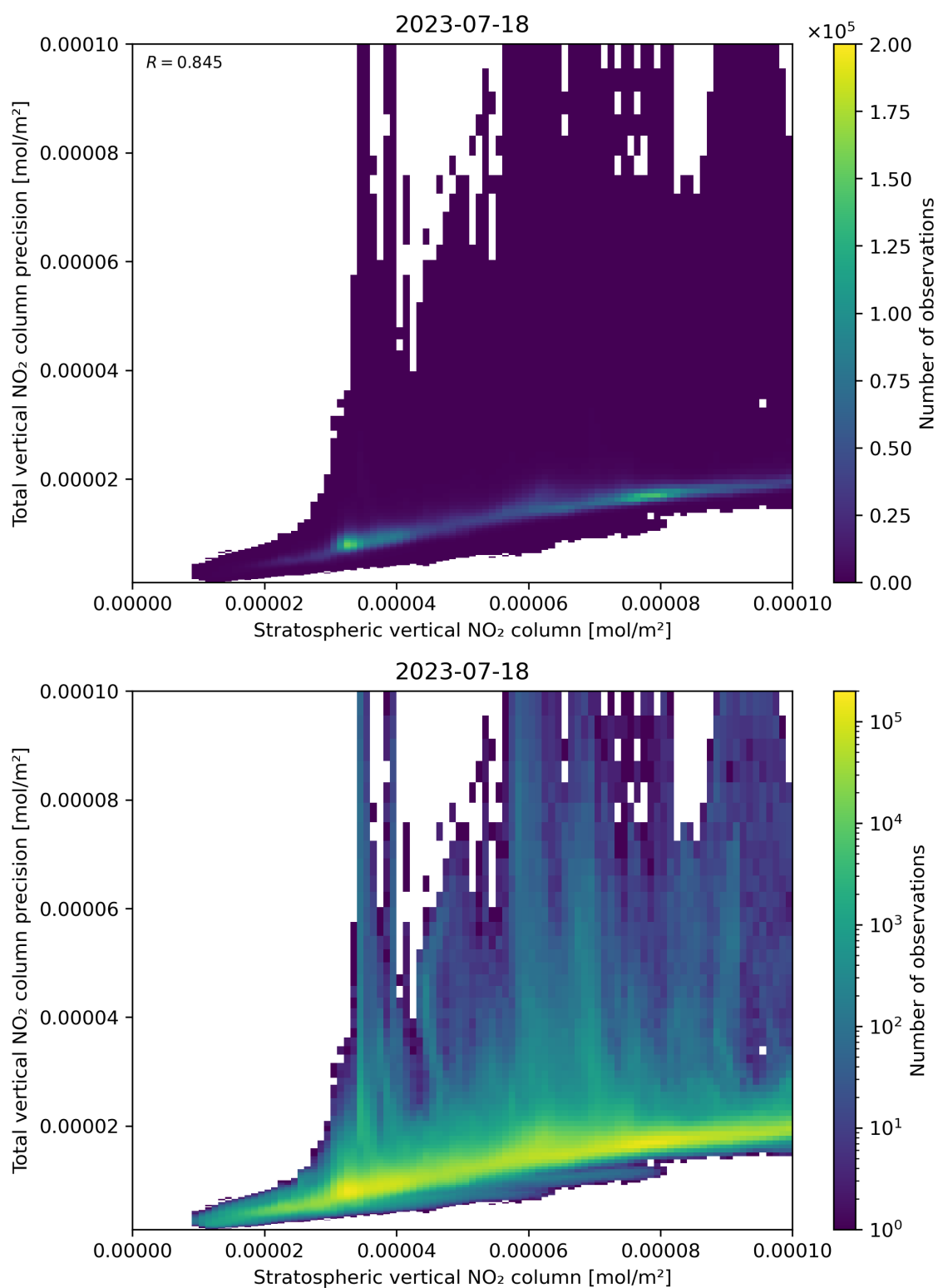
Figure 101: Scatter density plot of “Stratospheric vertical NO 2 column” against “Total vertical NO 2 column precision” for 2023-07-17 to 2023-07-19.
