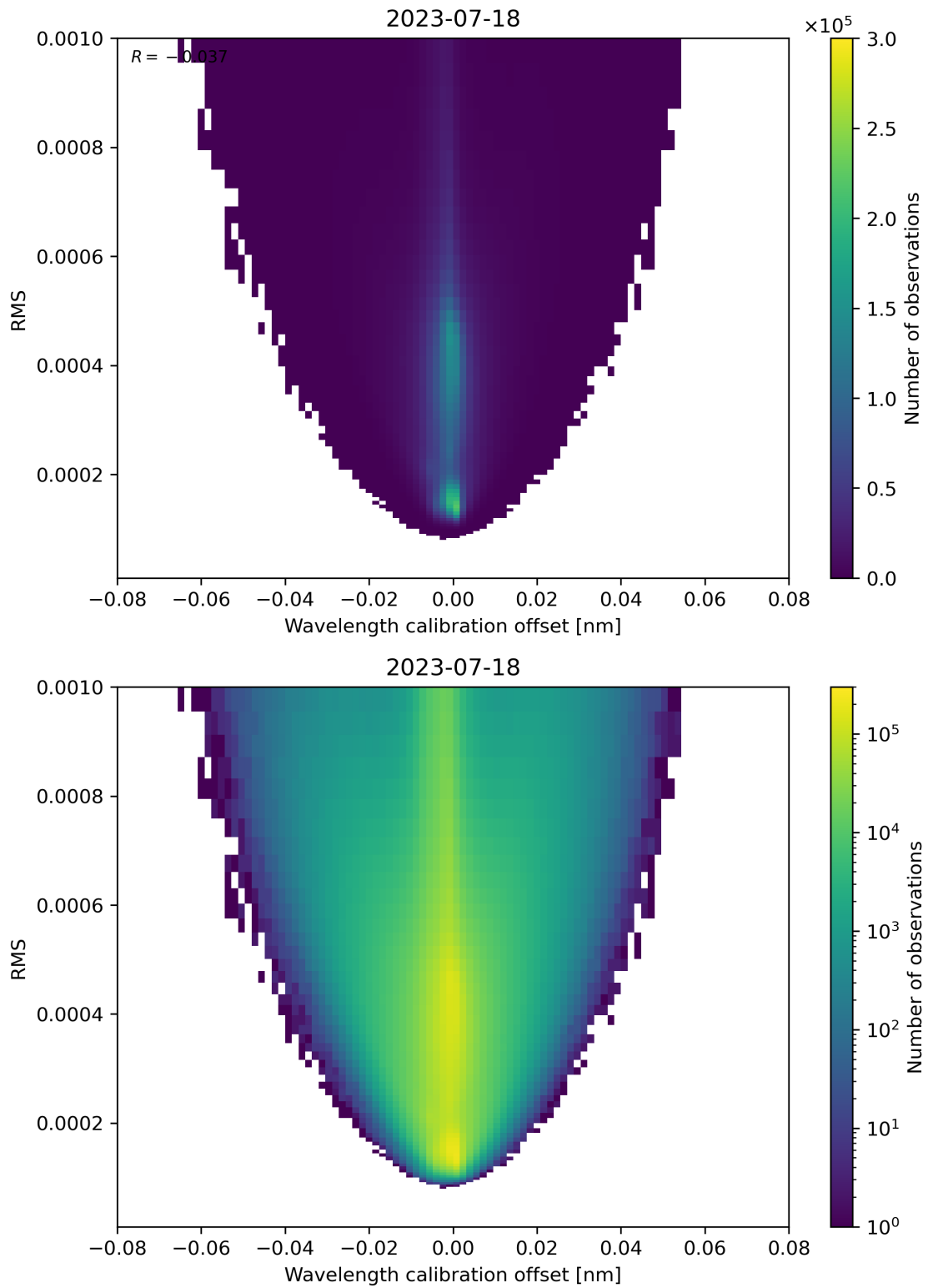
Figure 181: Scatter density plot of “Wavelength calibration offset” against “RMS” for 2023-07-17 to 2023-07-19.
