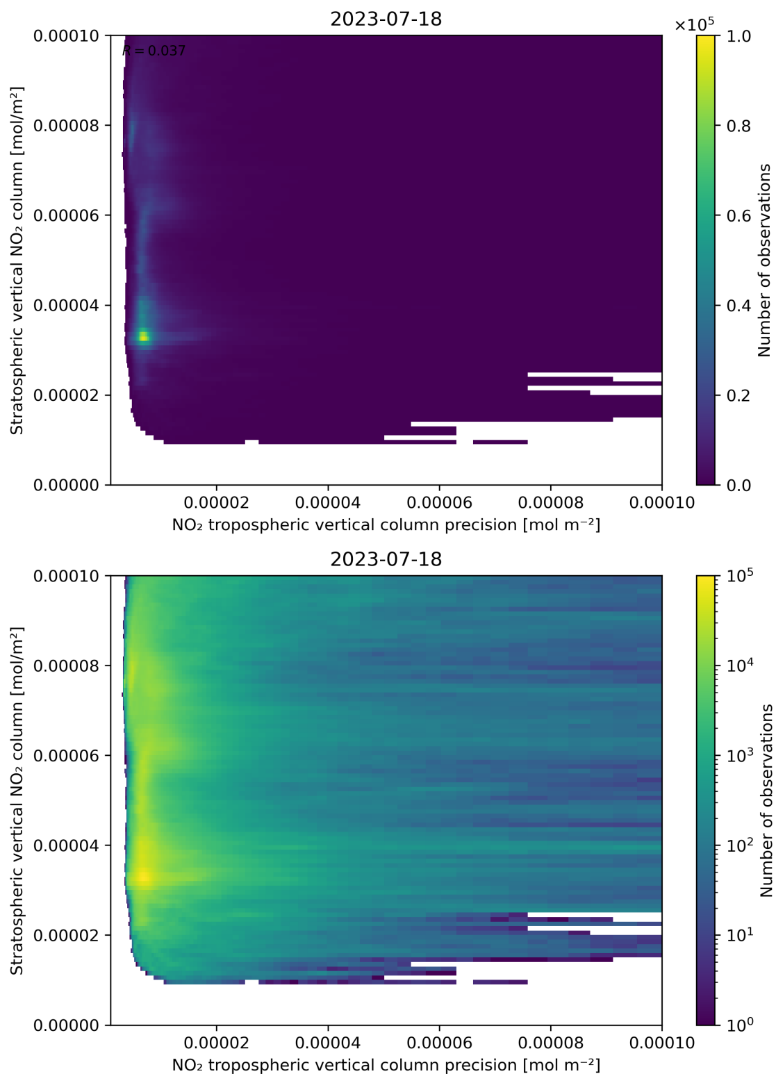
Figure 135: Scatter density plot of “NO 2 tropospheric vertical column precision” against “Stratospheric vertical NO 2 column” for 2023-07-17 to 2023-07-19.
