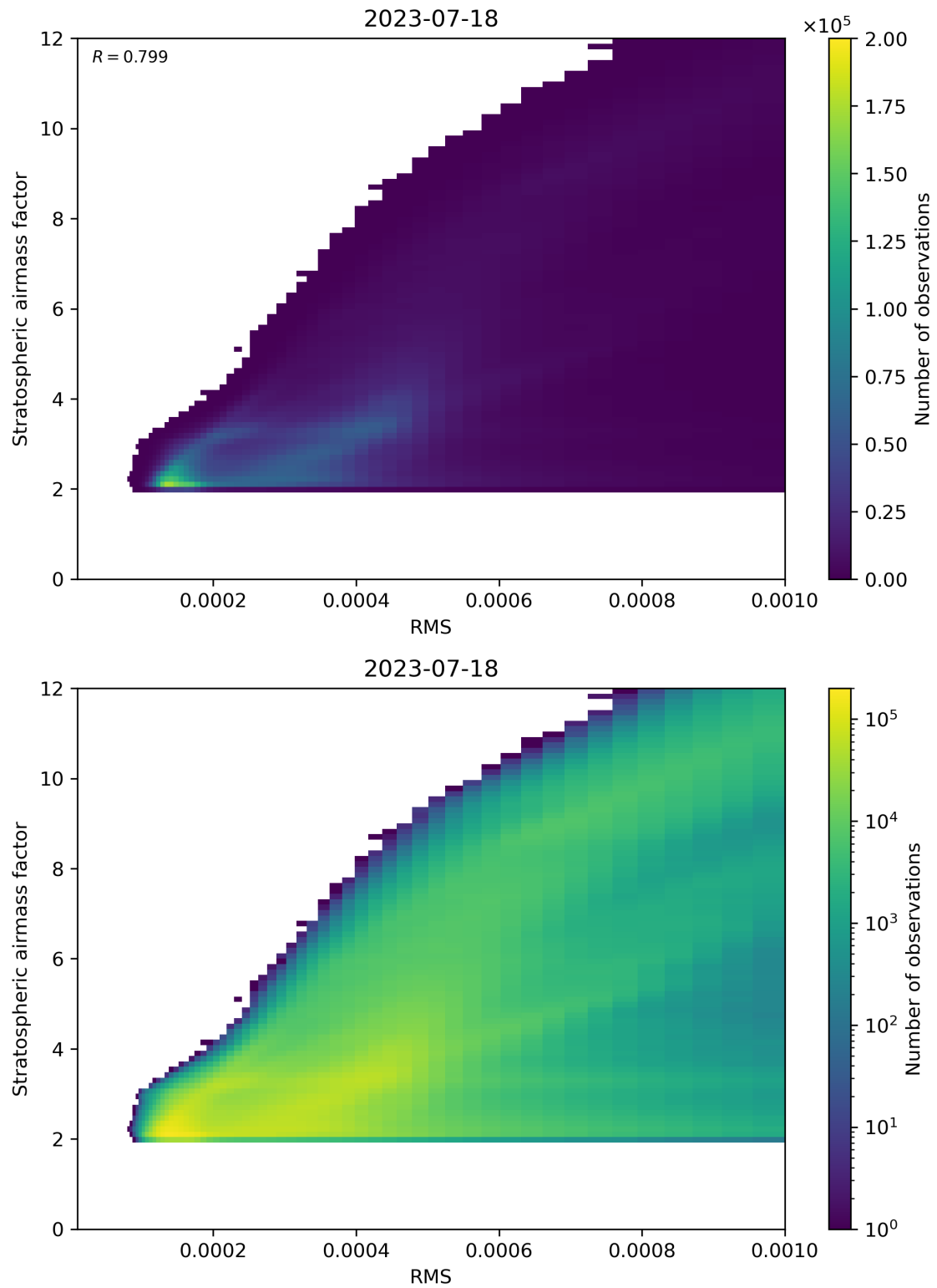
Figure 144: Scatter density plot of “RMS” against “Stratospheric airmass factor” for 2023-07-17 to 2023-07-19.
