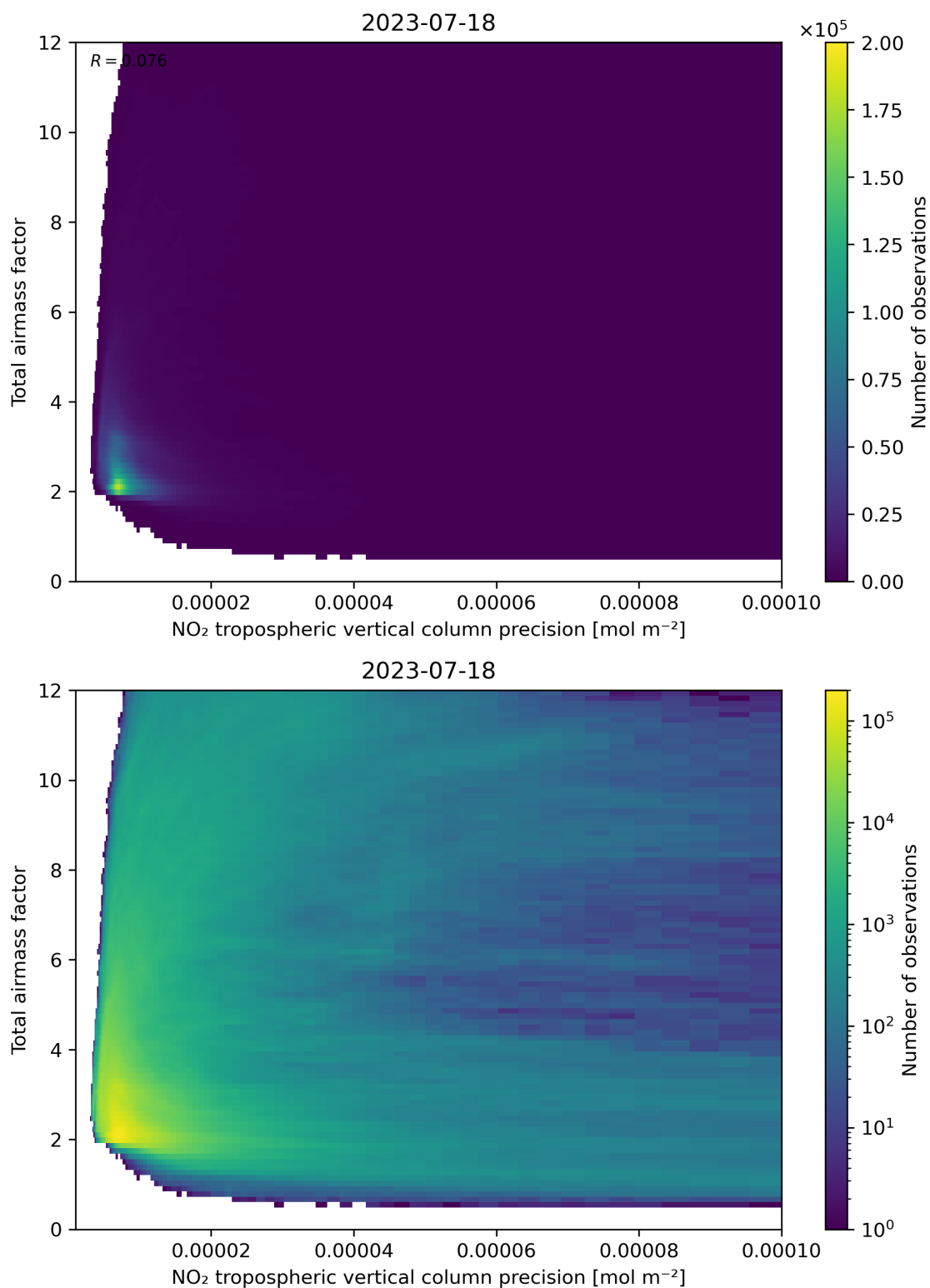
Figure 132: Scatter density plot of “NO 2 tropospheric vertical column precision” against “Total air mass factor” for 2023-07-17 to 2023-07-19.
