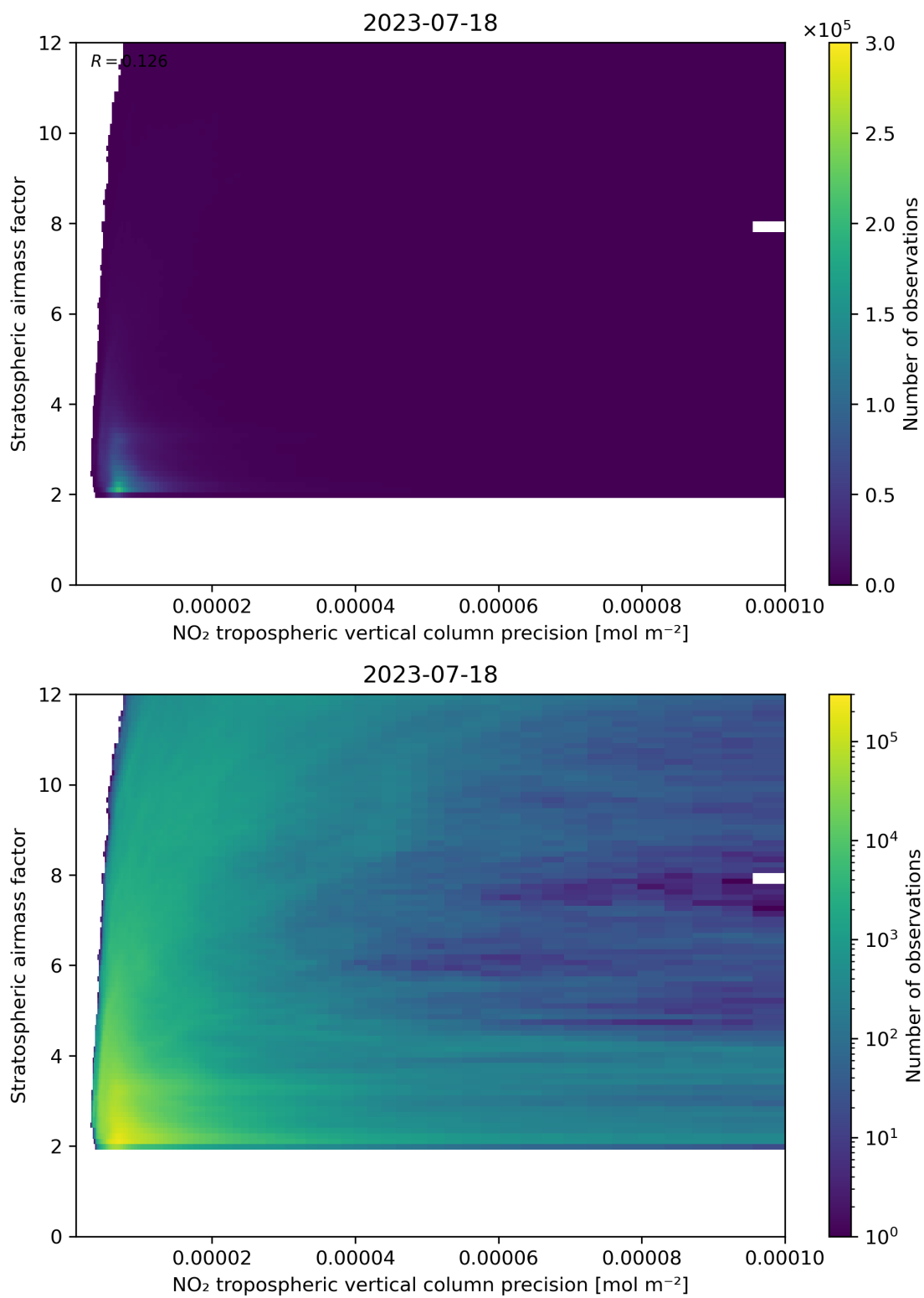
Figure 131: Scatter density plot of “NO 2 tropospheric vertical column precision” against “Stratospheric airmass factor” for 2023-07-17 to 2023-07-19.
