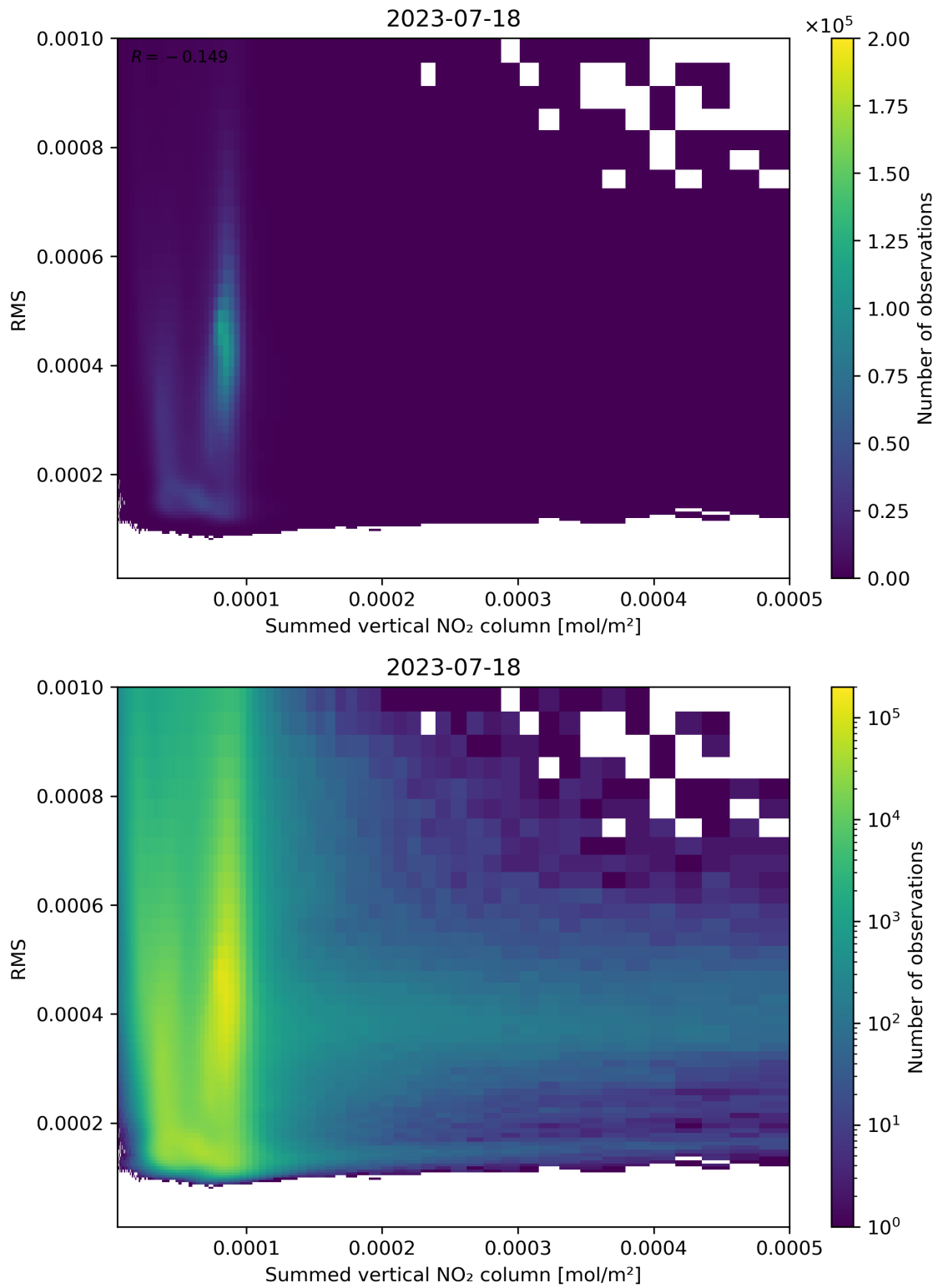
Figure 109: Scatter density plot of “Summed vertical NO 2 column” against “RMS” for 2023-07-17 to 2023-07-19.
