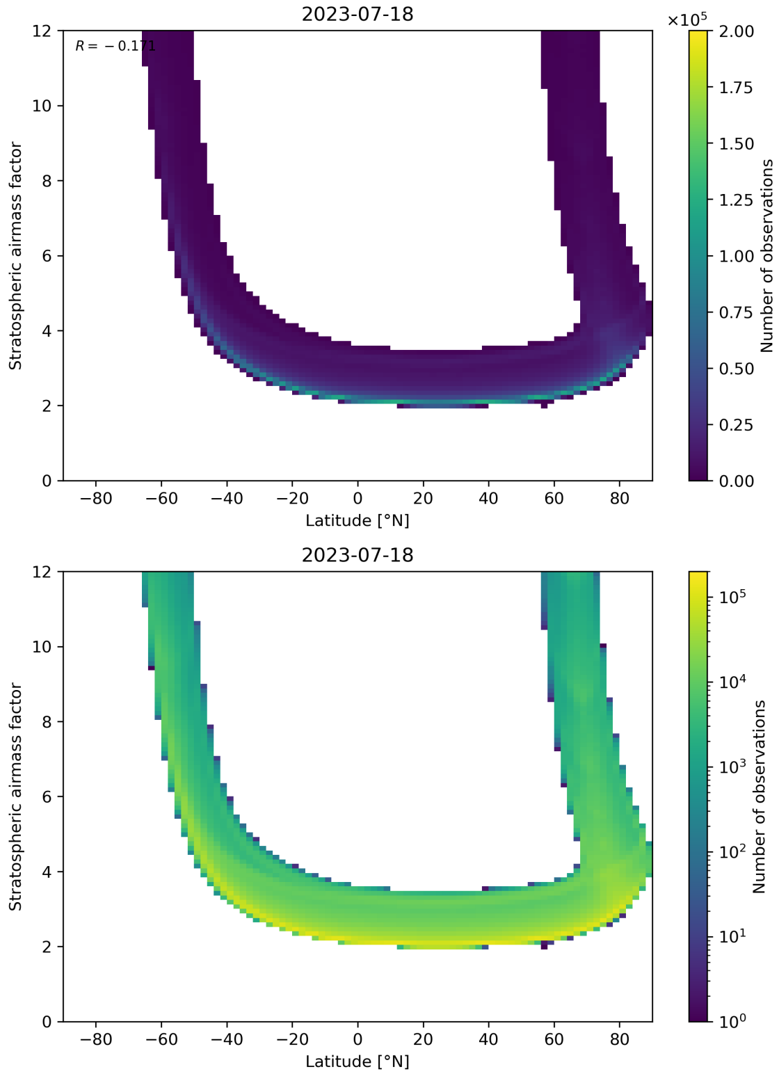
Figure 83: Scatter density plot of “Latitude” against “Stratospheric air mass factor” for 2023-07-17 to 2023-07-19.
