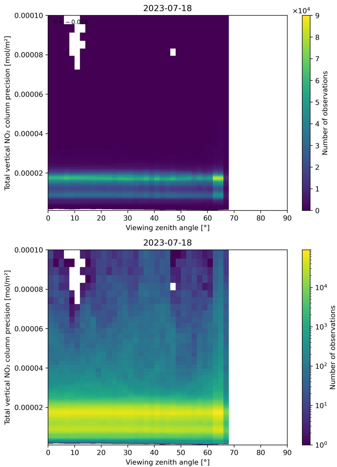
Figure 168: Scatter density plot of “Viewing zenith angle” against “Total vertical NO 2 column precision” for 2023-07-17 to 2023-07-19.
