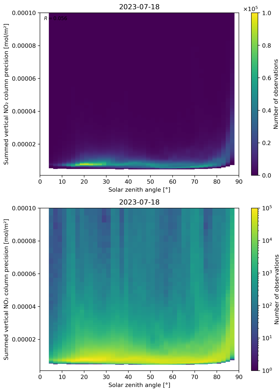
Figure 152: Scatter density plot of “Solar zenith angle” against “Summed vertical NO 2 column precision” for 2023-07-17 to 2023-07-19.
