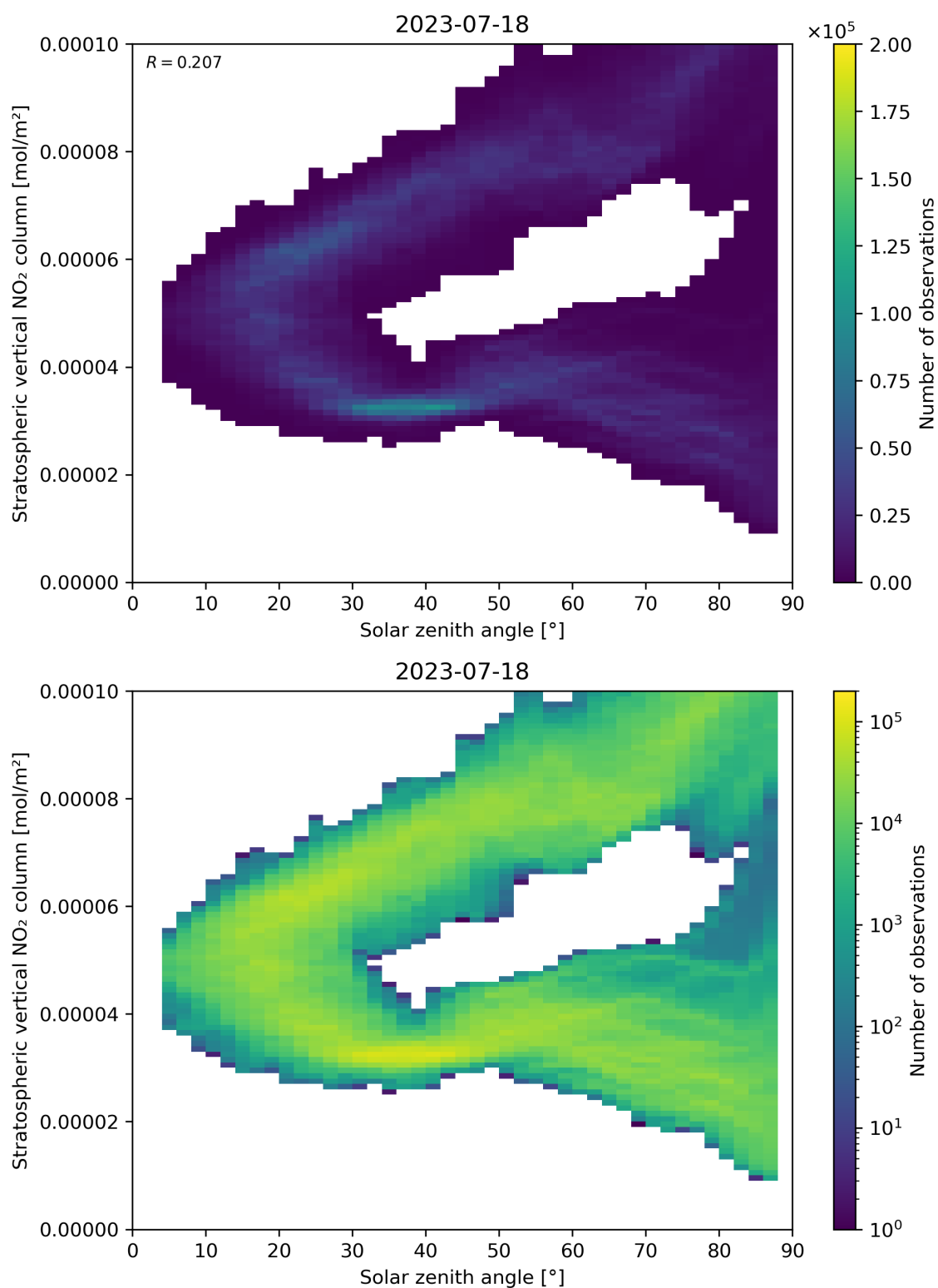
Figure 150: Scatter density plot of “Solar zenith angle” against “Stratospheric vertical NO 2 column” for 2023-07-17 to 2023-07-19.
