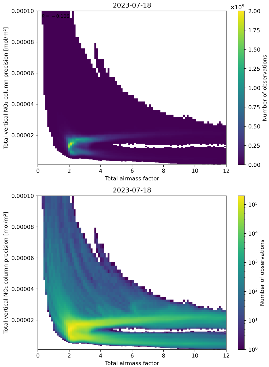
Figure 68: Scatter density plot of “Total airmass factor” against “Total vertical NO 2 column precision” for 2023-07-17 to 2023-07-19.
