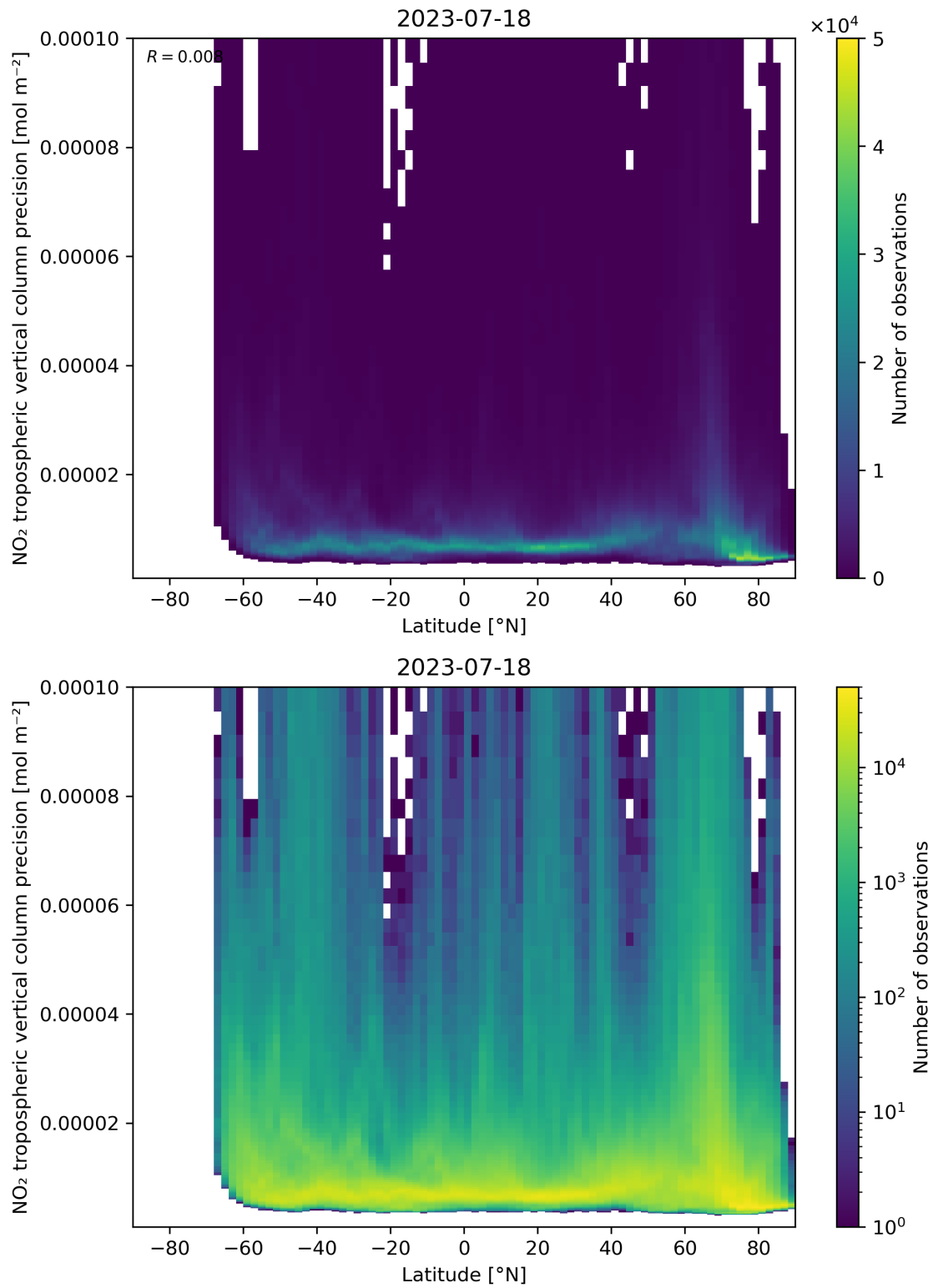
Figure 93: Scatter density plot of “Latitude” against “NO 2 tropospheric vertical column precision” for 2023-07-17 to 2023-07-19.
