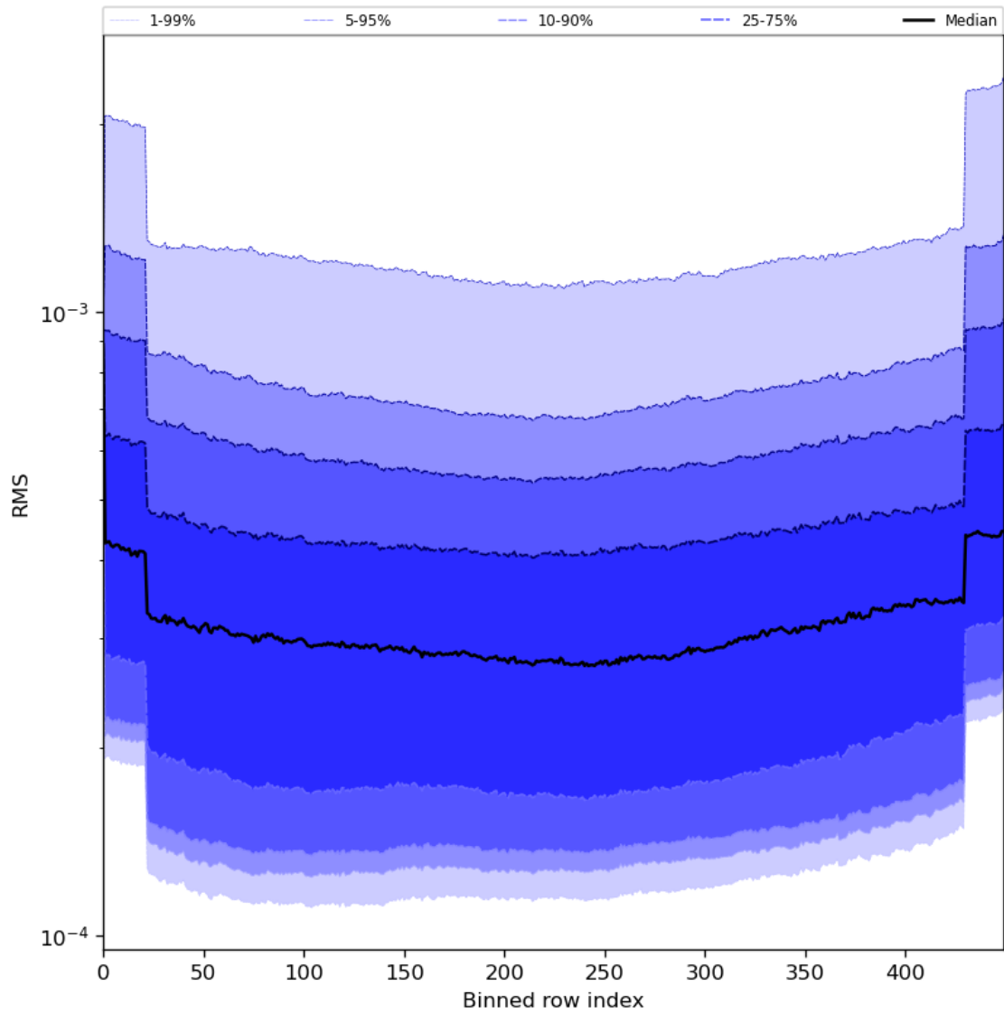
Figure 60: Along track statistics of “RMS” for 2023-07-17 to 2023-07-19
