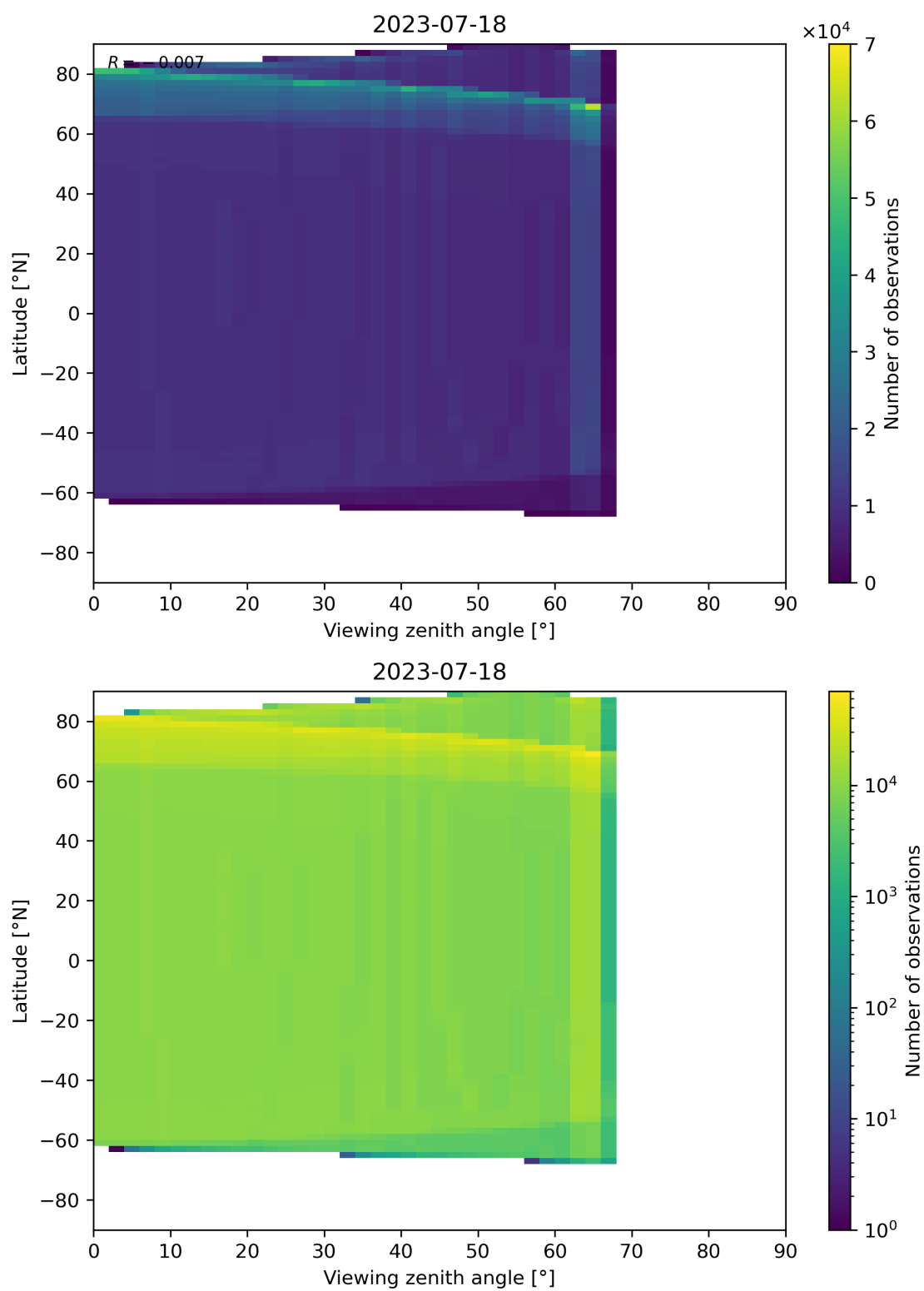
Figure 163: Scatter density plot of “Viewing zenith angle” against “Latitude” for 2023-07-17 to 2023-07-19.
