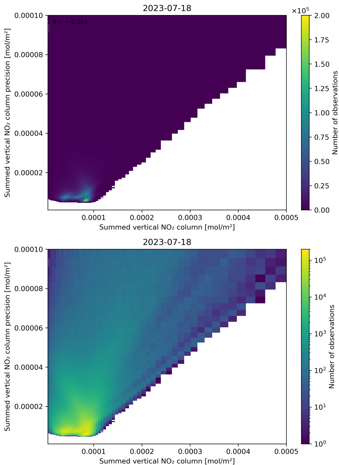
Figure 105: Scatter density plot of “Summed vertical NO 2 column” against “Summed vertical NO 2 column precision” for 2023-07-17 to 2023-07-19.
