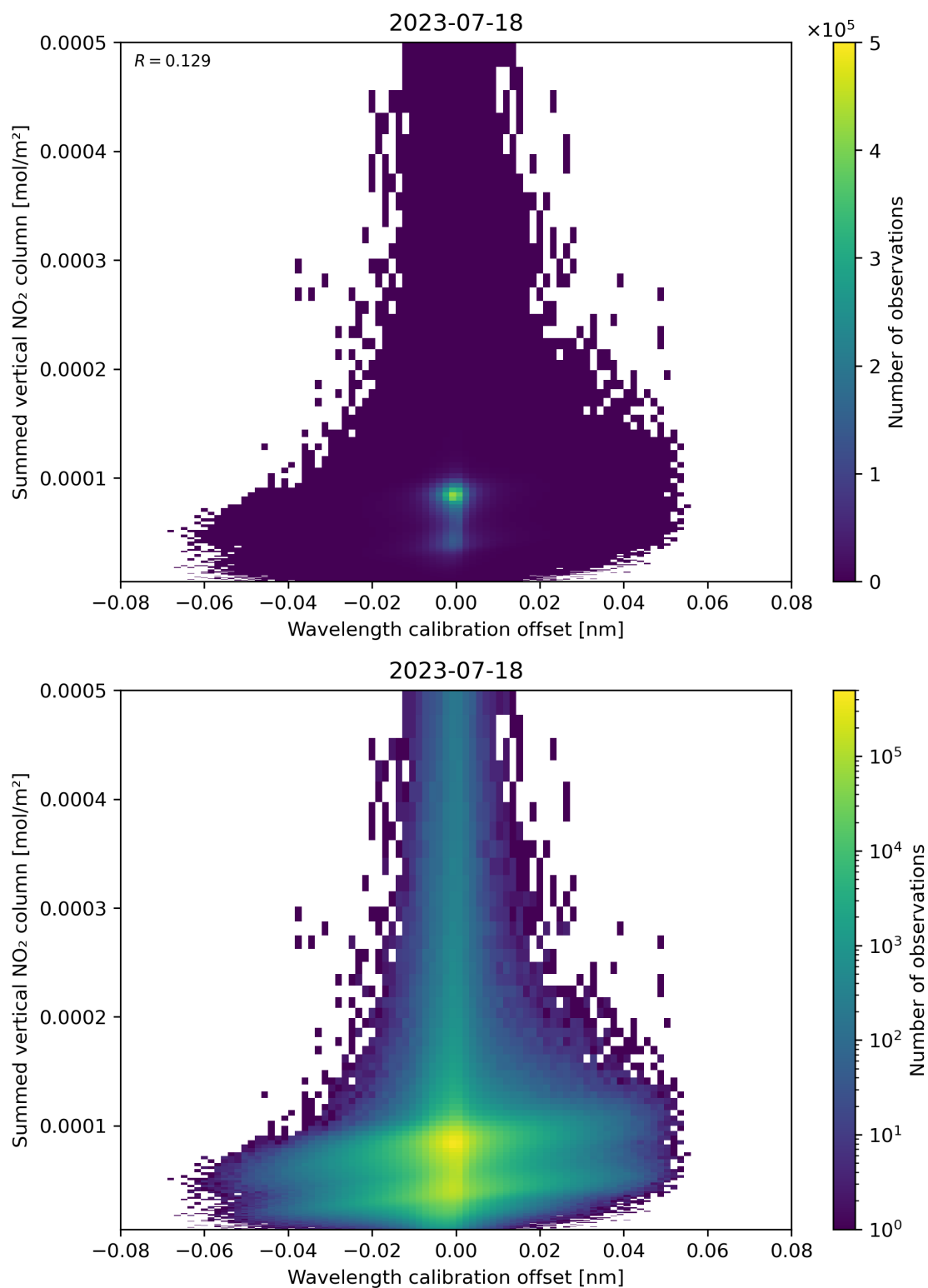
Figure 177: Scatter density plot of “Wavelength calibration offset” against “Summed vertical NO 2 column” for 2023-07-17 to 2023-07-19.
