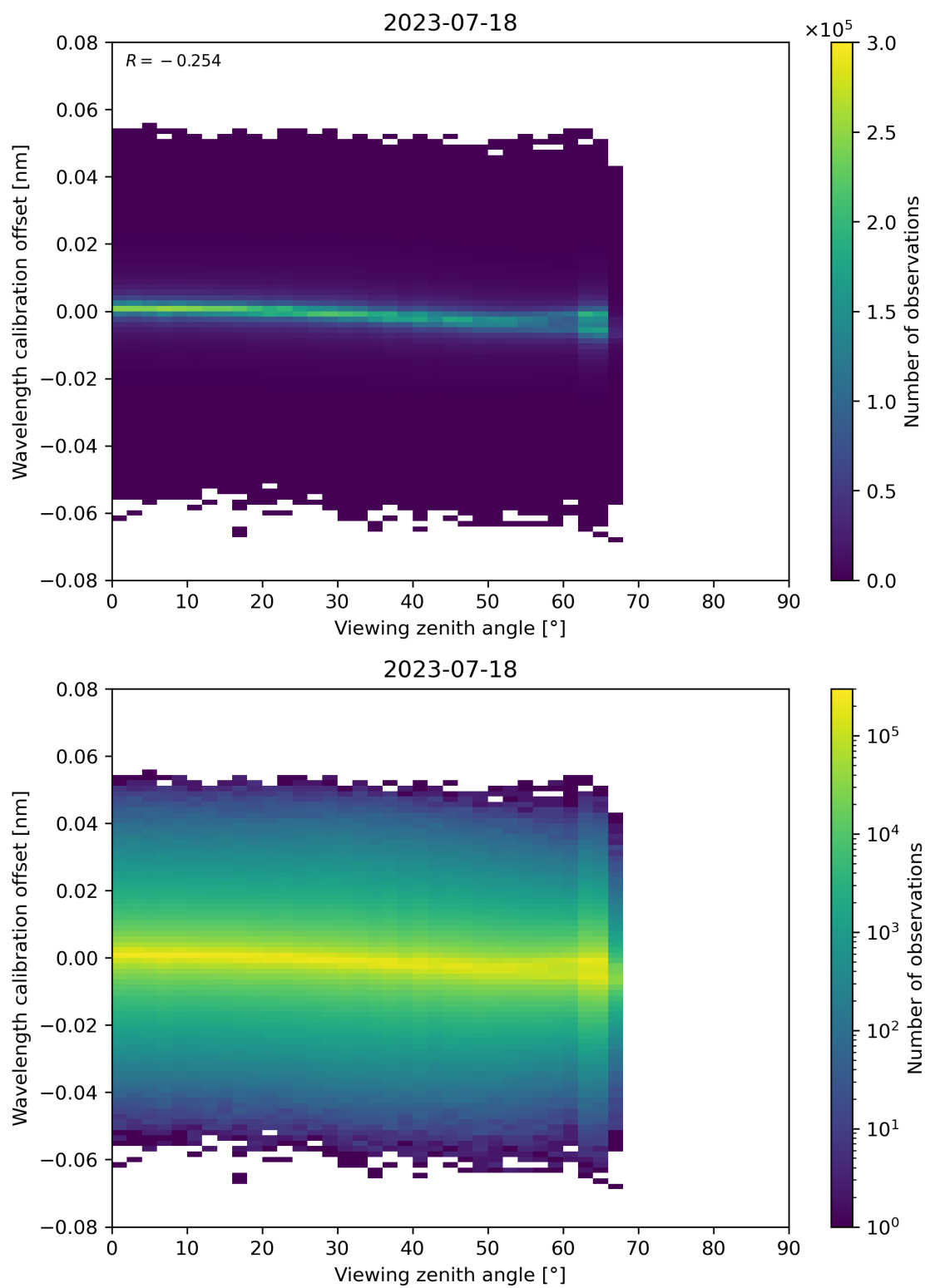
Figure 173: Scatter density plot of “Viewing zenith angle” against “Wavelength calibration offset” for 2023-07-17 to 2023-07-19.
