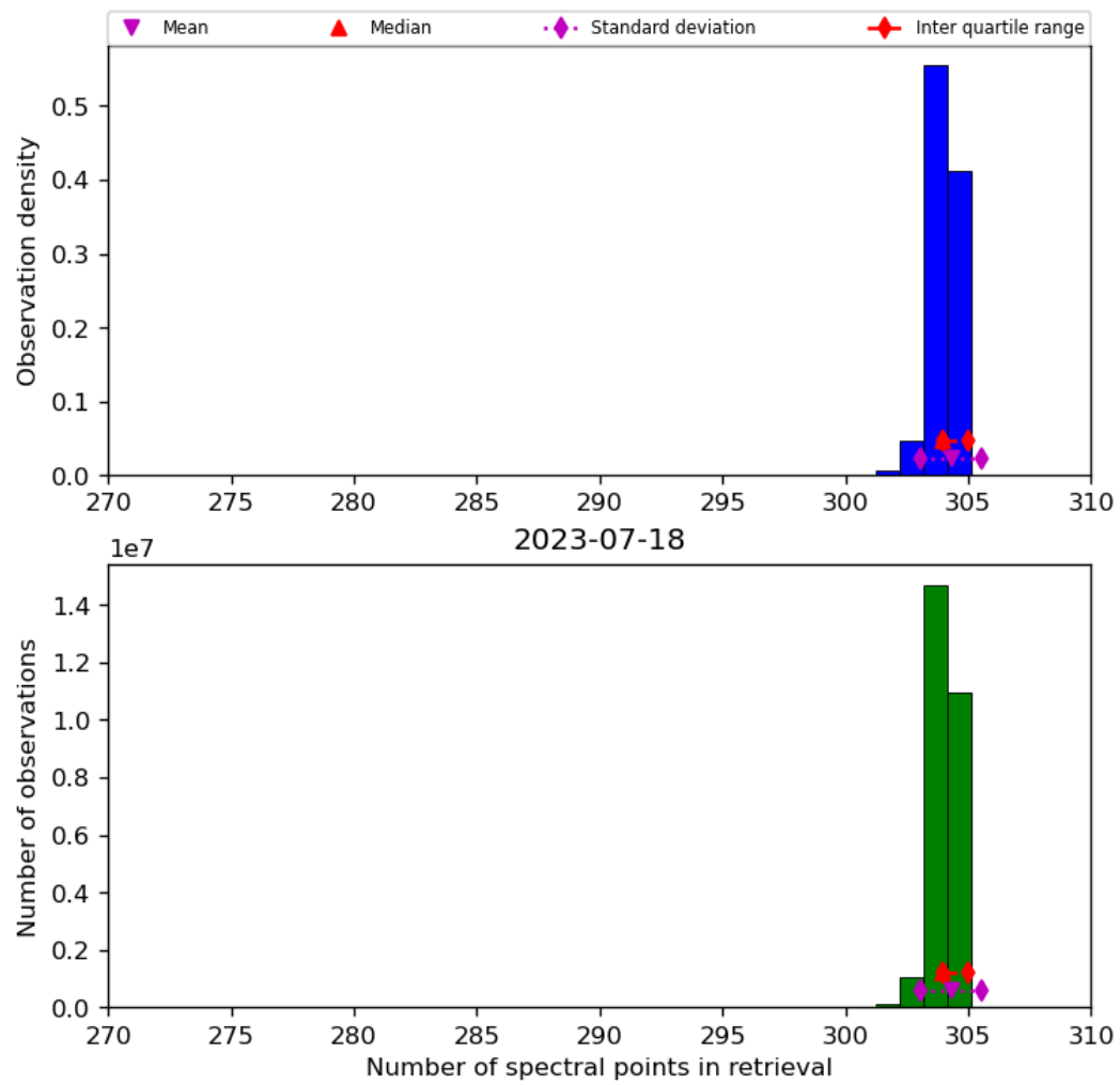
Figure 33: Histogram of “Number of spectral points in retrieval” for 2023-07-17 to 2023-07-19
