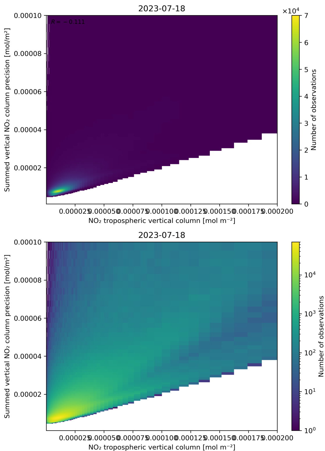
Figure 127: Scatter density plot of “NO 2 tropospheric vertical column” against “Summed vertical NO 2 column precision” for 2023-07-17 to 2023-07-19.
