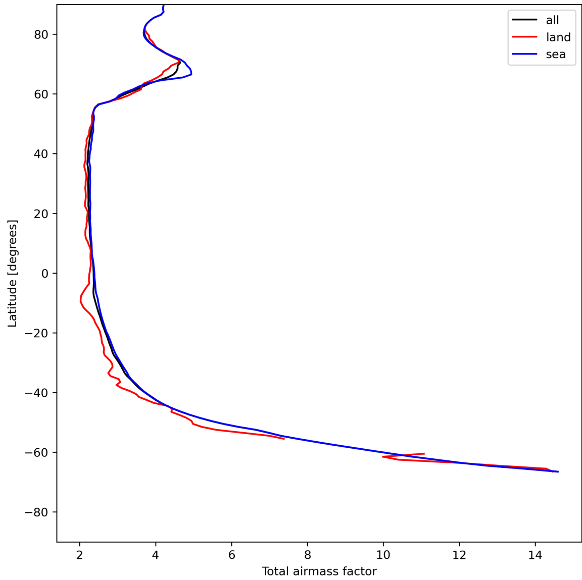
Figure 15: Zonal average of “Total airmass factor” for 2023-07-17 to 2023-07-19.
