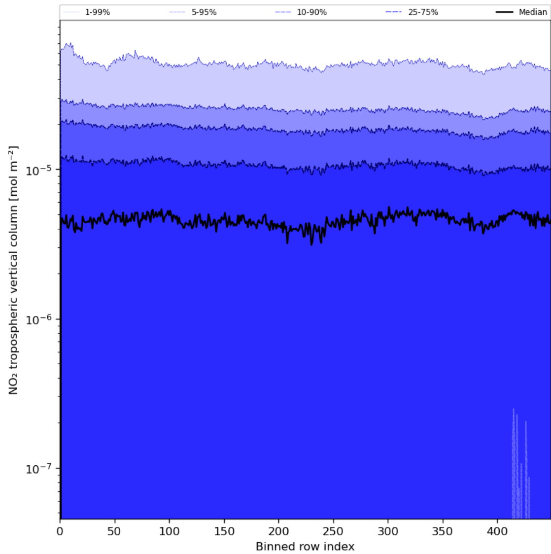
Figure 46: Along track statistics of “NO 2 tropospheric vertical column” for 2023-07-17 to 2023-07-19
