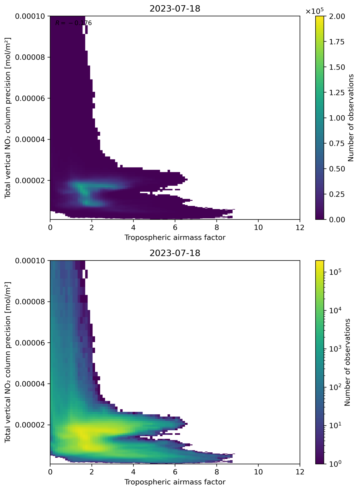
Figure 78: Scatter density plot of “Tropospheric airmass factor” against “Total vertical NO 2 column precision” for 2023-07-17 to 2023-07-19.
