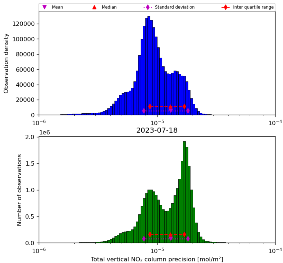
Figure 39: Histogram of “Total vertical NO 2 column precision” for 2023-07-17 to 2023-07-19
