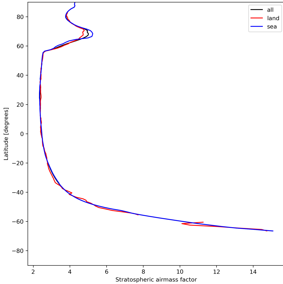
Figure 27: Zonal average of “Stratospheric air mass factor” for 2023-07-17 to 2023-07-19.
