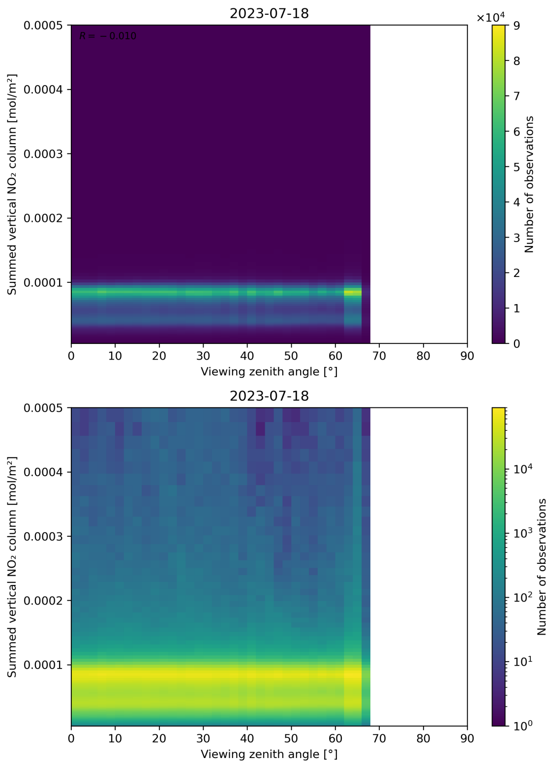
Figure 165: Scatter density plot of “Viewing zenith angle” against “Summed vertical NO 2 column” for 2023-07-17 to 2023-07-19.
