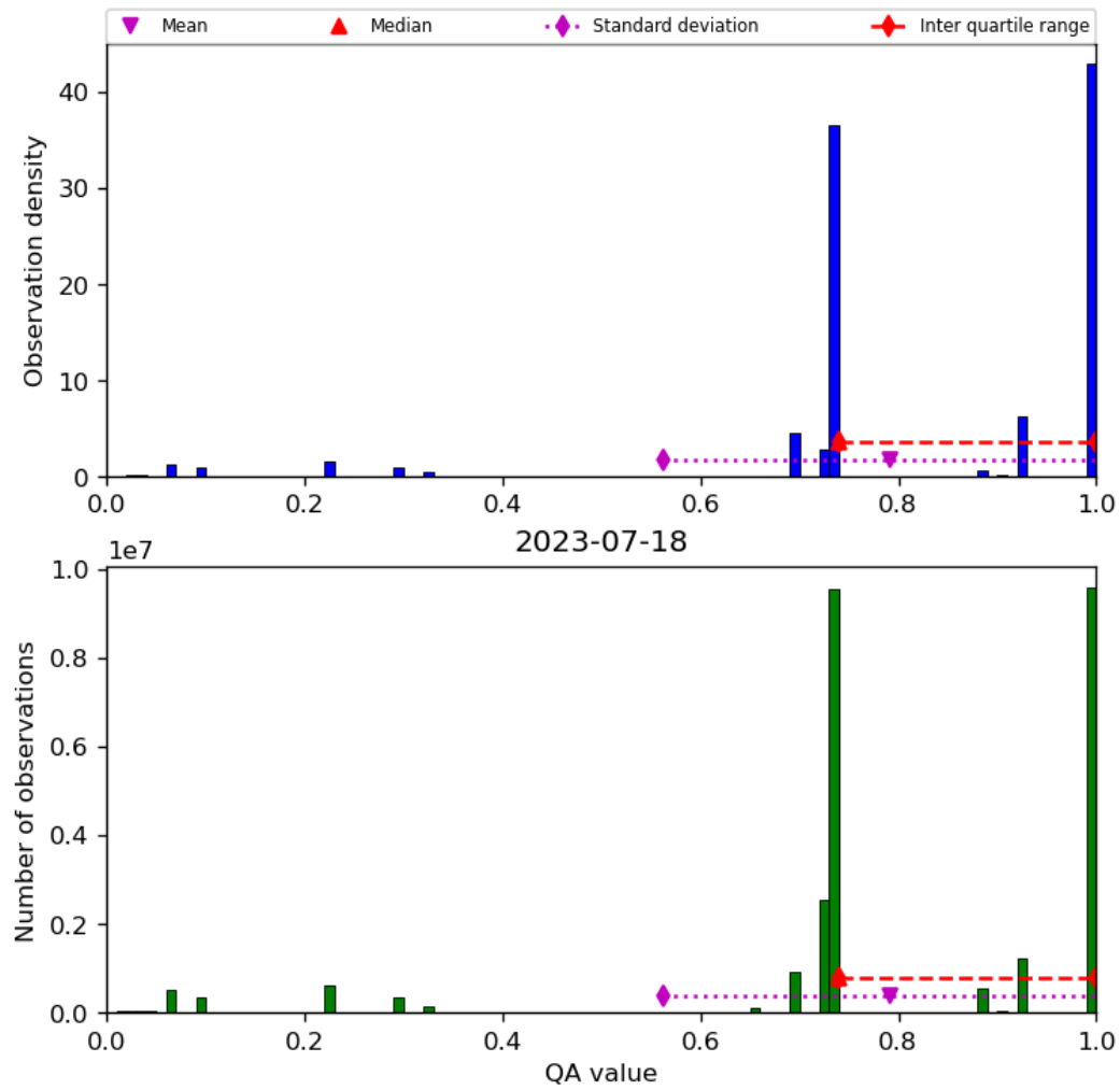
Figure 28: Histogram of “QA value” for 2023-07-17 to 2023-07-19
