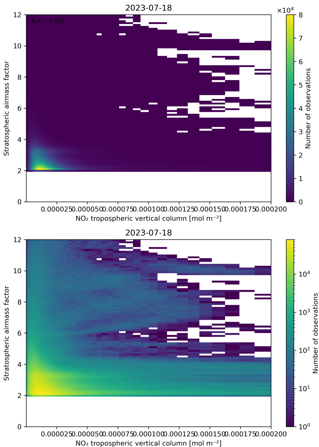
Figure 121: Scatter density plot of “NO 2 tropospheric vertical column” against “Stratospheric air mass factor” for 2023-07-17 to 2023-07-19.
