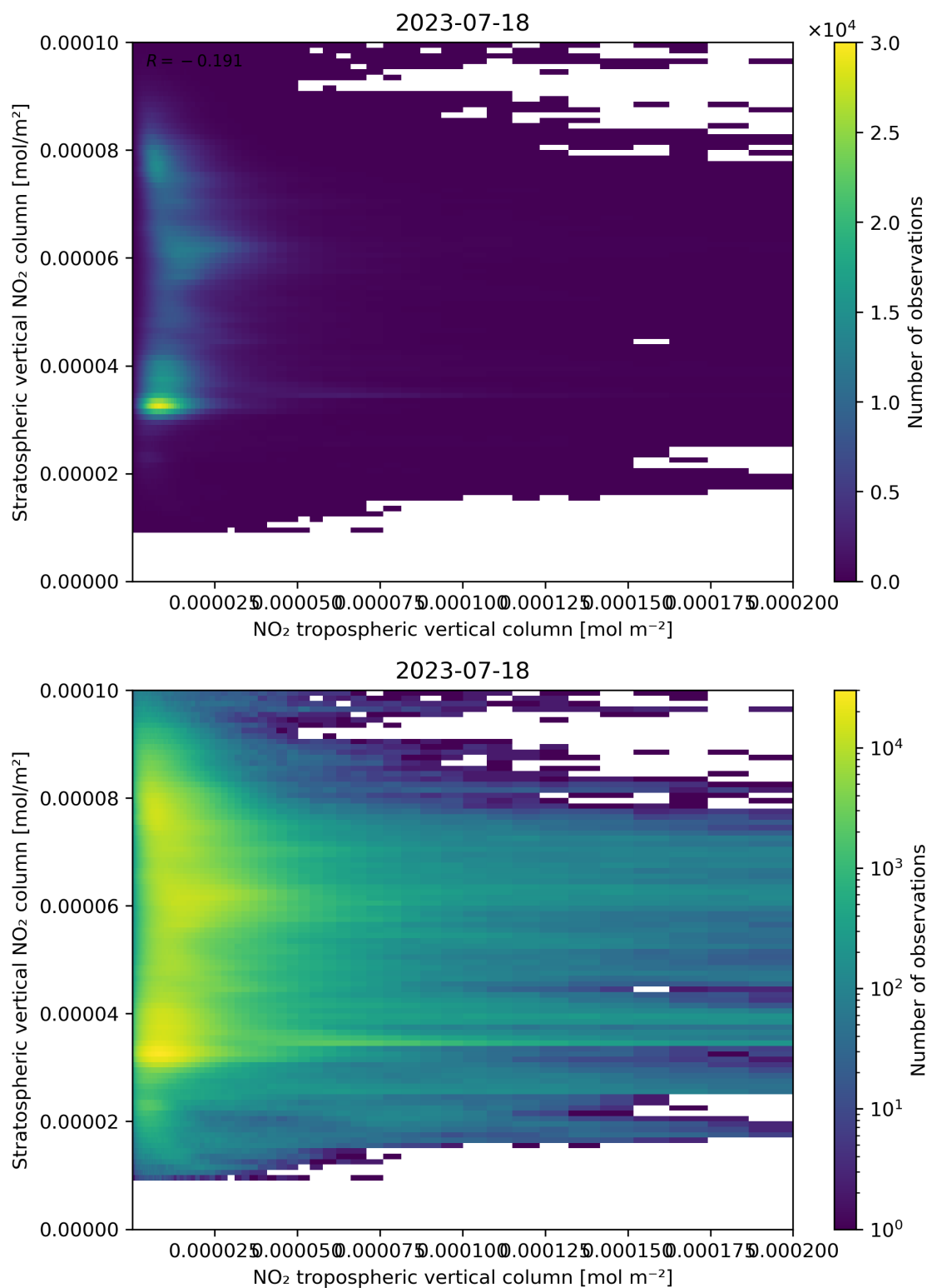
Figure 125: Scatter density plot of “NO 2 tropospheric vertical column” against “Stratospheric vertical NO 2 column” for 2023-07-17 to 2023-07-19.
