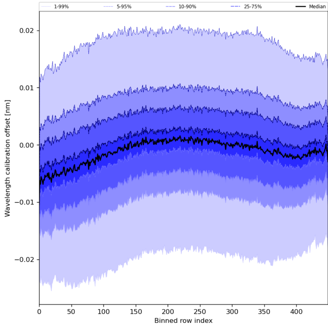
Figure 52: Along track statistics of “Wavelength calibration offset” for 2023-07-17 to 2023-07-19
