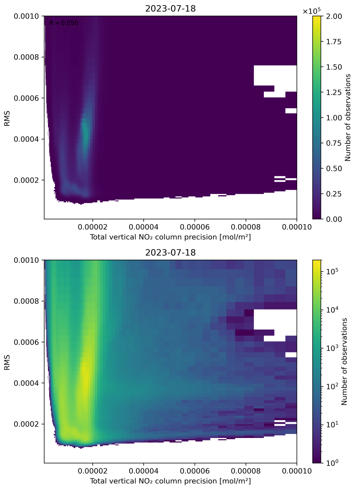
Figure 119: Scatter density plot of “Total vertical NO 2 column precision” against “RMS” for 2023-07-17 to 2023-07-19.
