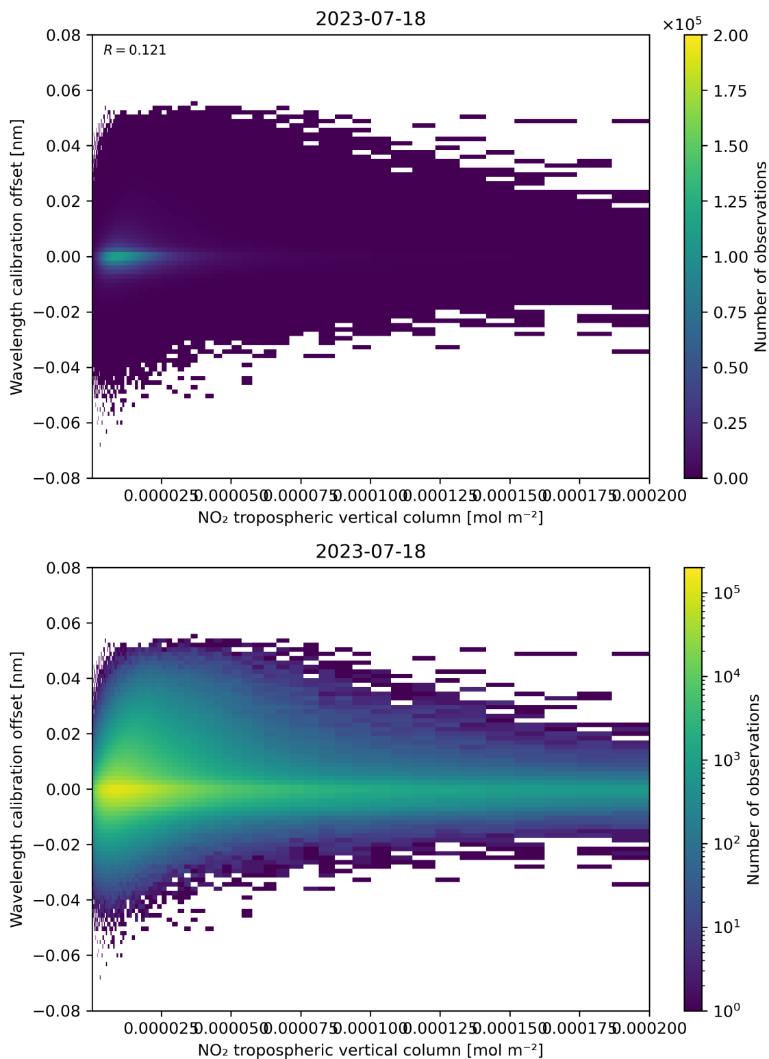
Figure 143: Scatter density plot of “NO 2 tropospheric vertical column” against “Wavelength calibration offset” for 2023-07-17 to 2023-07-19.
