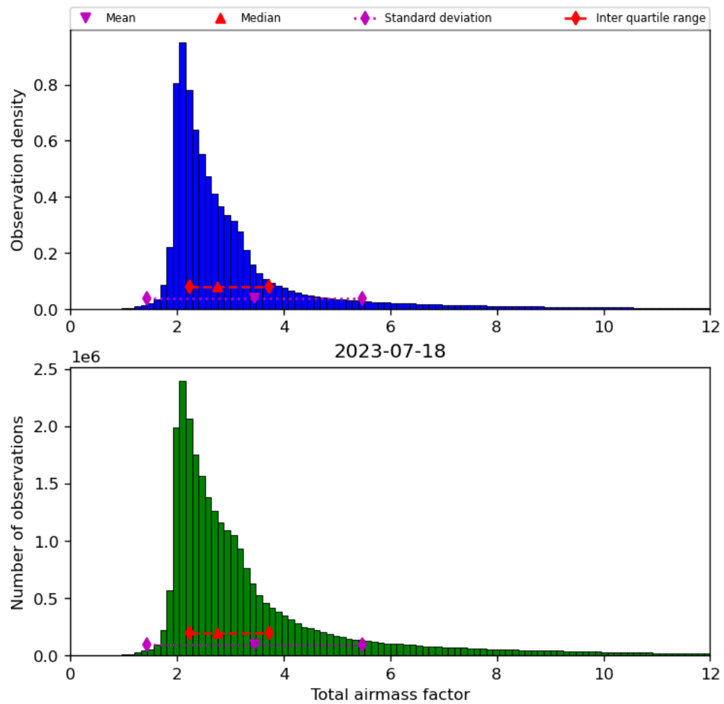
Figure 32: Histogram of “Total airmass factor” for 2023-07-17 to 2023-07-19
