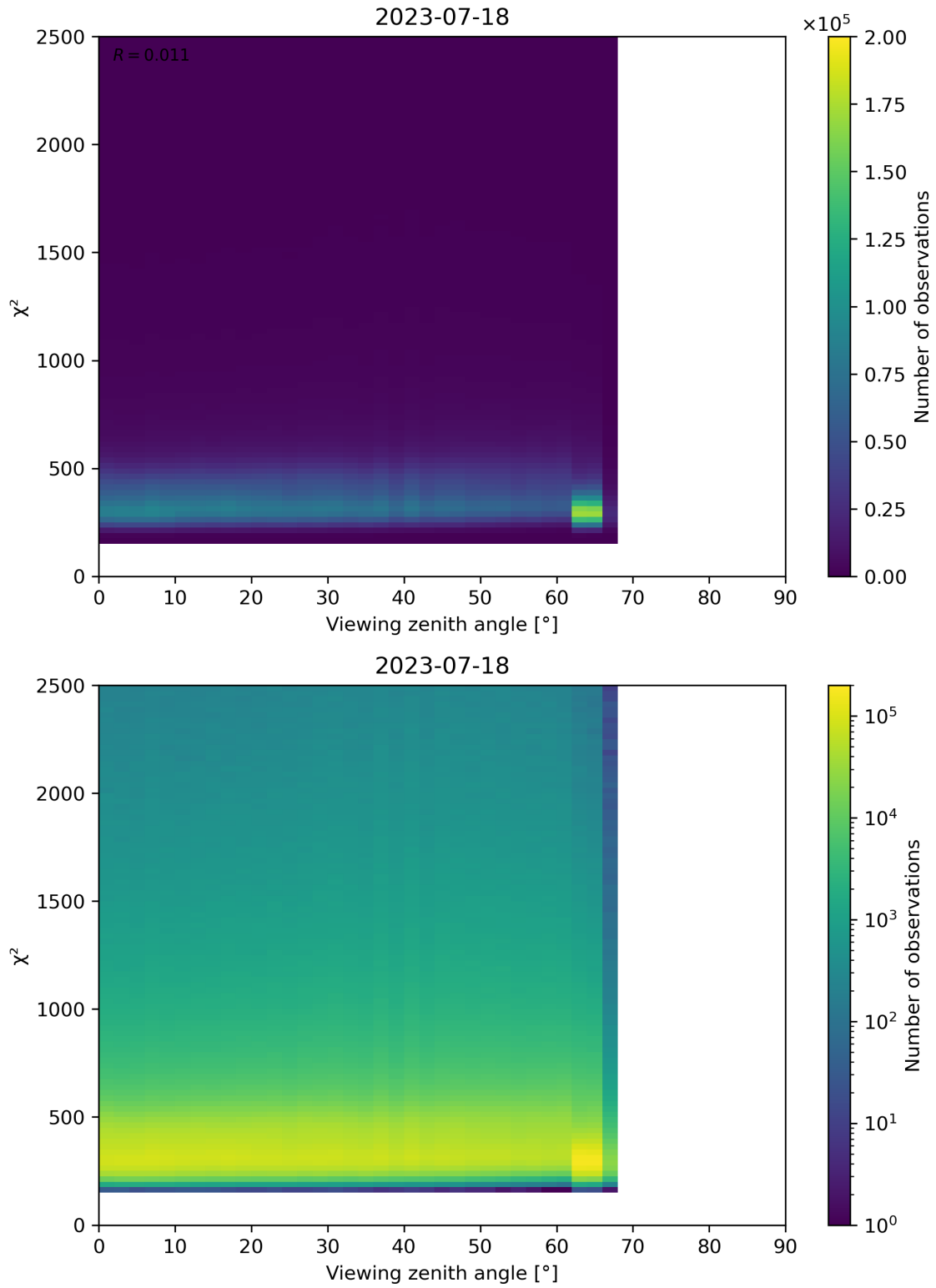
Figure 162: Scatter density plot of “Viewing zenith angle” against “ \chi^2 ” for 2023-07-17 to 2023-07-19.
