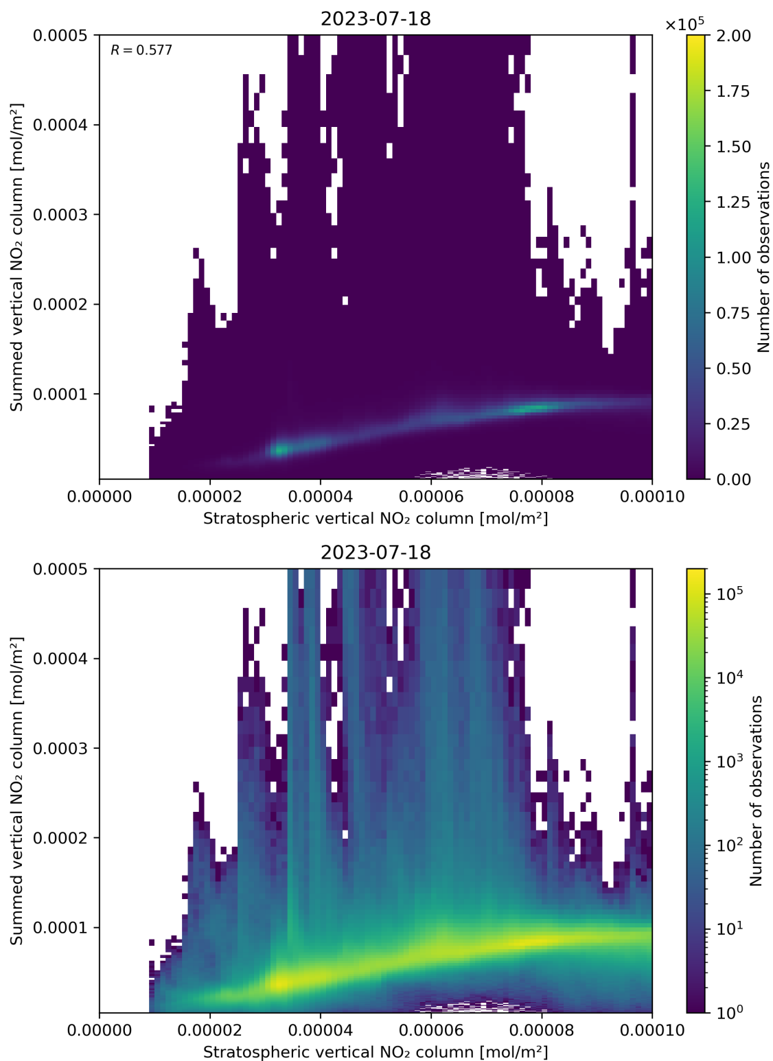
Figure 98: Scatter density plot of “Stratospheric vertical NO 2 column” against “Summed vertical NO 2 column” for 2023-07-17 to 2023-07-19.
