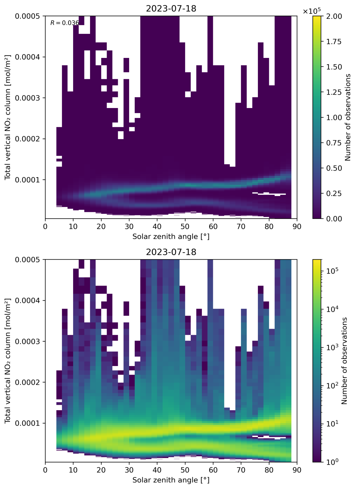
Figure 153: Scatter density plot of “Solar zenith angle” against “Total vertical NO 2 column” for 2023-07-17 to 2023-07-19.
