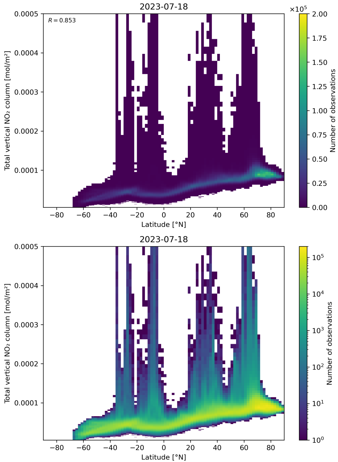
Figure 90: Scatter density plot of “Latitude” against “Total vertical NO 2 column” for 2023-07-17 to 2023-07-19.
