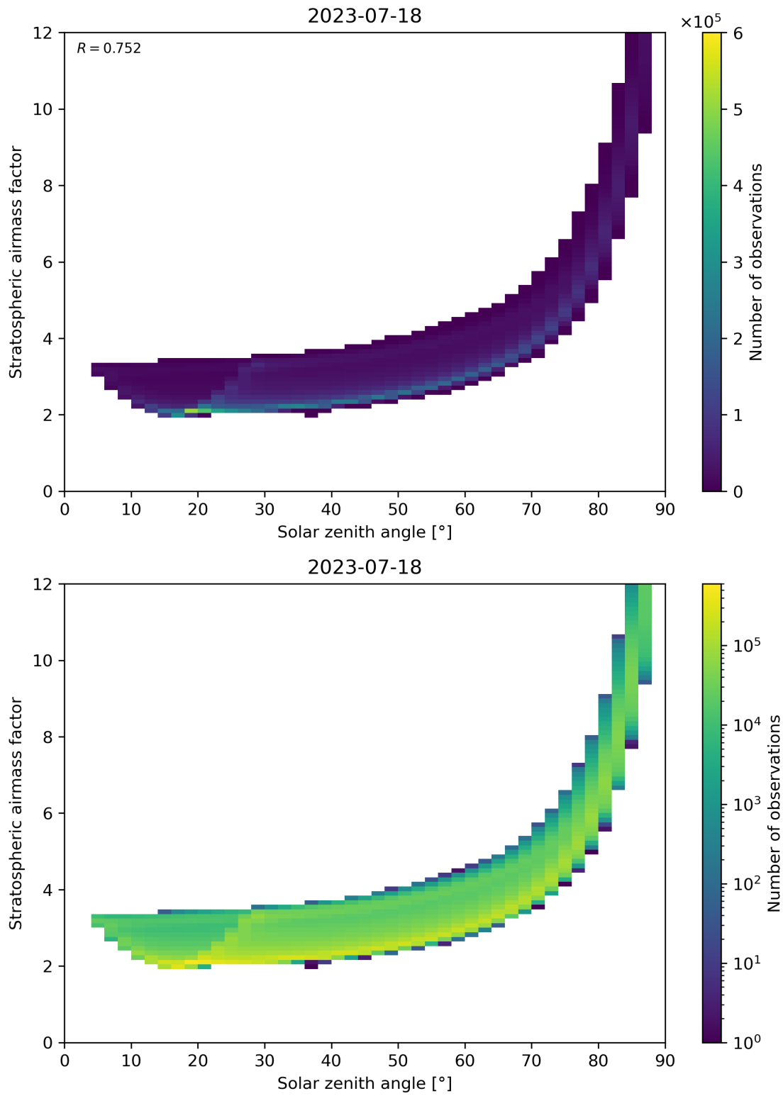
Figure 145: Scatter density plot of “Solar zenith angle” against “Stratospheric airmass factor” for 2023-07-17 to 2023-07-19.
