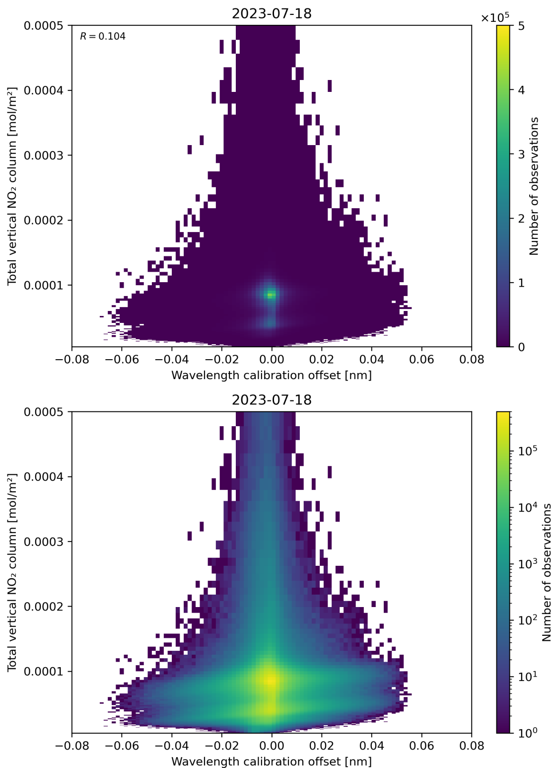
Figure 179: Scatter density plot of “Wavelength calibration offset” against “Total vertical NO 2 column” for 2023-07-17 to 2023-07-19.
