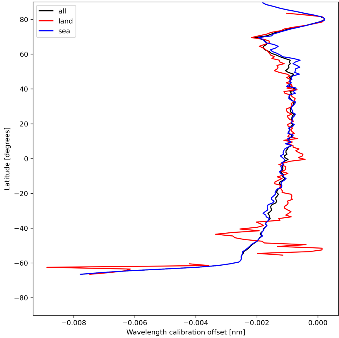
Figure 18: Zonal average of “Wavelength calibration offset” for 2023-07-17 to 2023-07-19.
