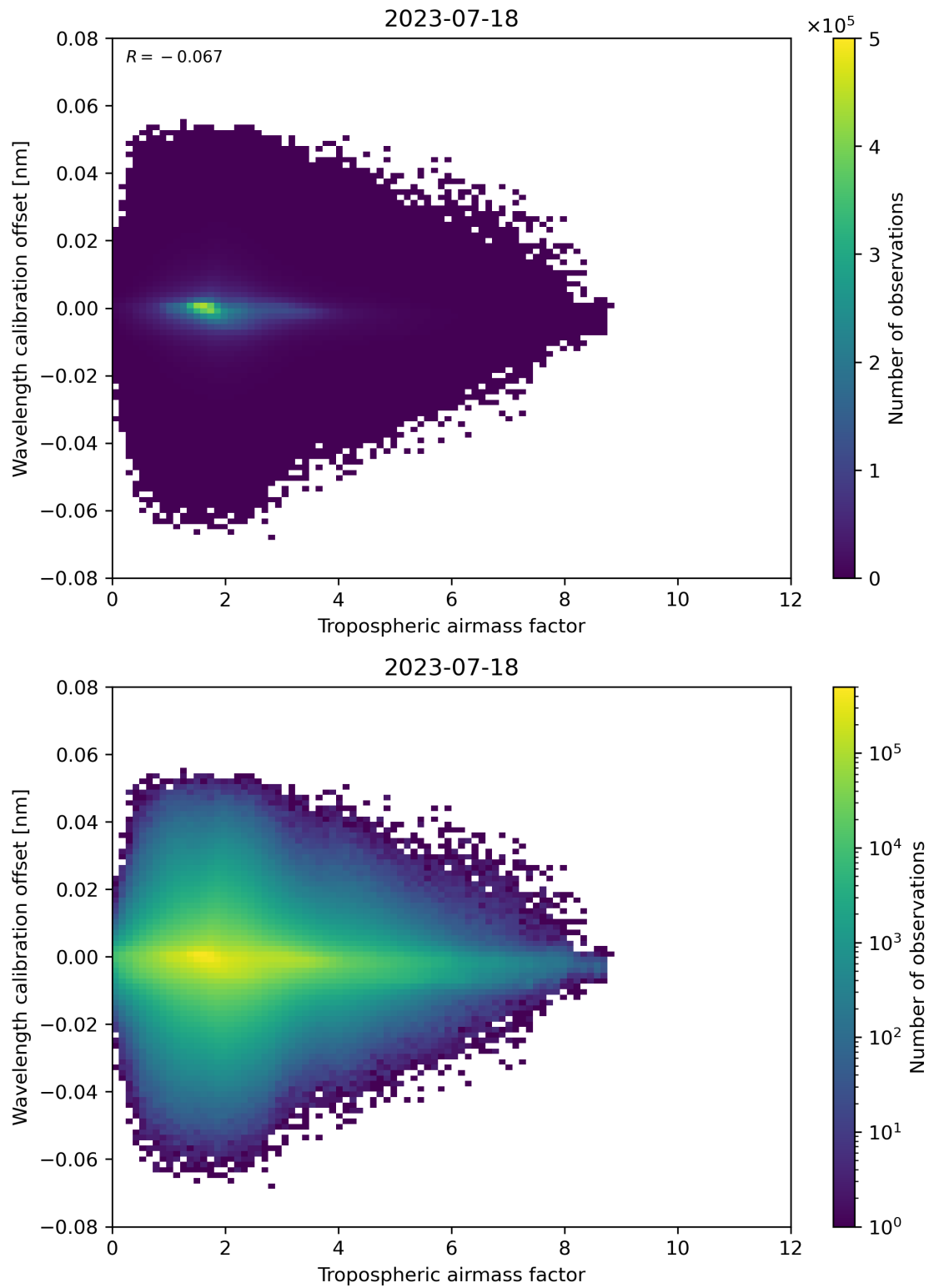
Figure 80: Scatter density plot of “Tropospheric airmass factor” against “Wavelength calibration offset” for 2023-07-17 to 2023-07-19.
