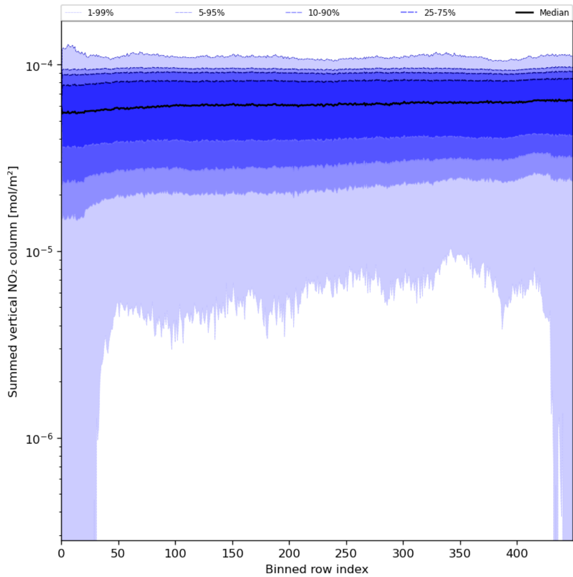
Figure 57: Along track statistics of “Summed vertical NO 2 column” for 2023-07-17 to 2023-07-19
