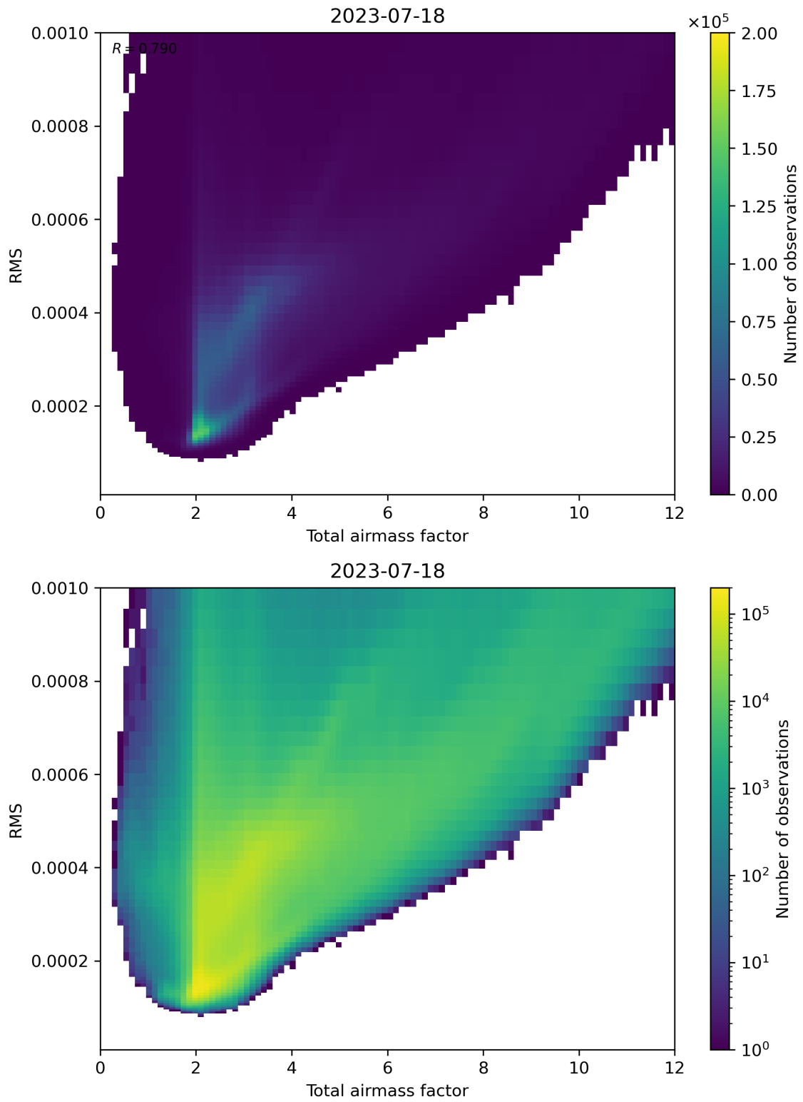
Figure 69: Scatter density plot of “Total airmass factor” against “RMS” for 2023-07-17 to 2023-07-19.
