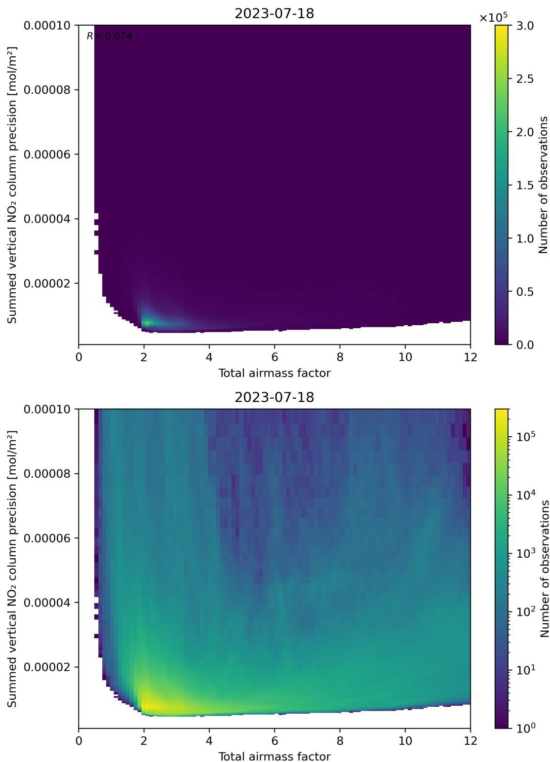
Figure 66: Scatter density plot of “Total airmass factor” against “Summed vertical NO 2 column precision” for 2023-07-17 to 2023-07-19.
