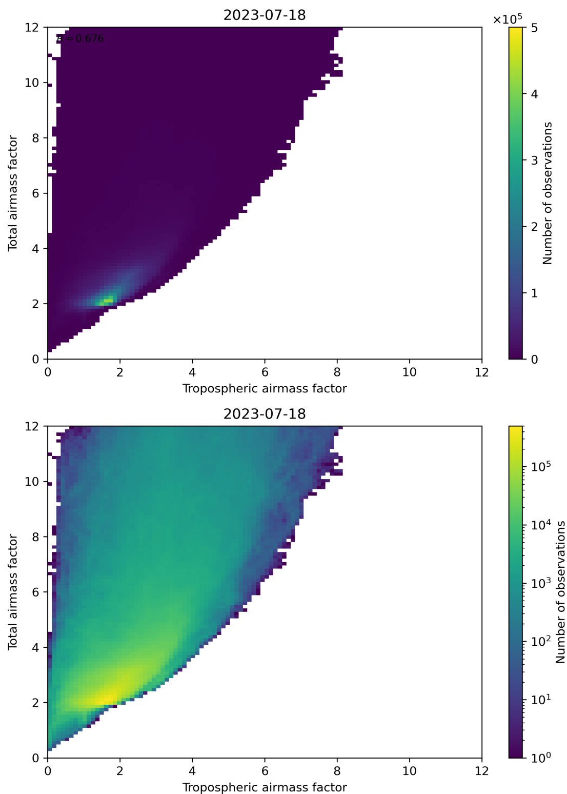
Figure 72: Scatter density plot of “Tropospheric airmass factor” against “Total airmass factor” for 2023-07-17 to 2023-07-19.
