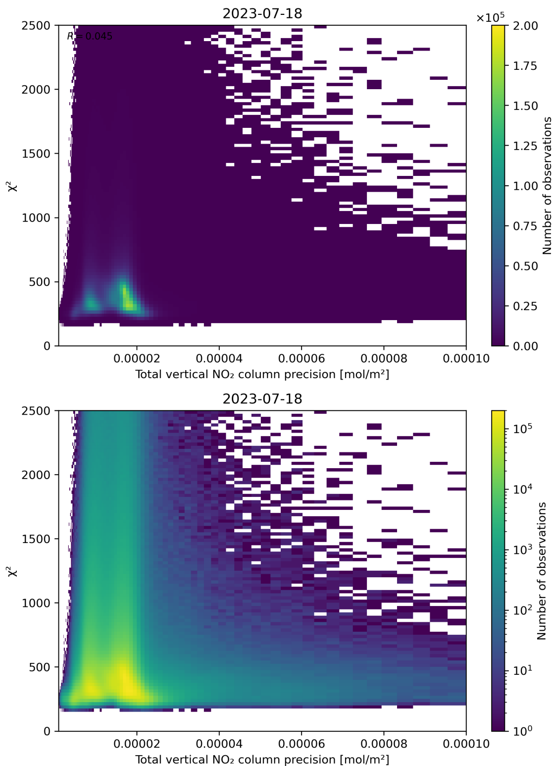
Figure 116: Scatter density plot of “Total vertical NO 2 column precision” against “ \chi^2 ” for 2023-07-17 to 2023-07-19.
