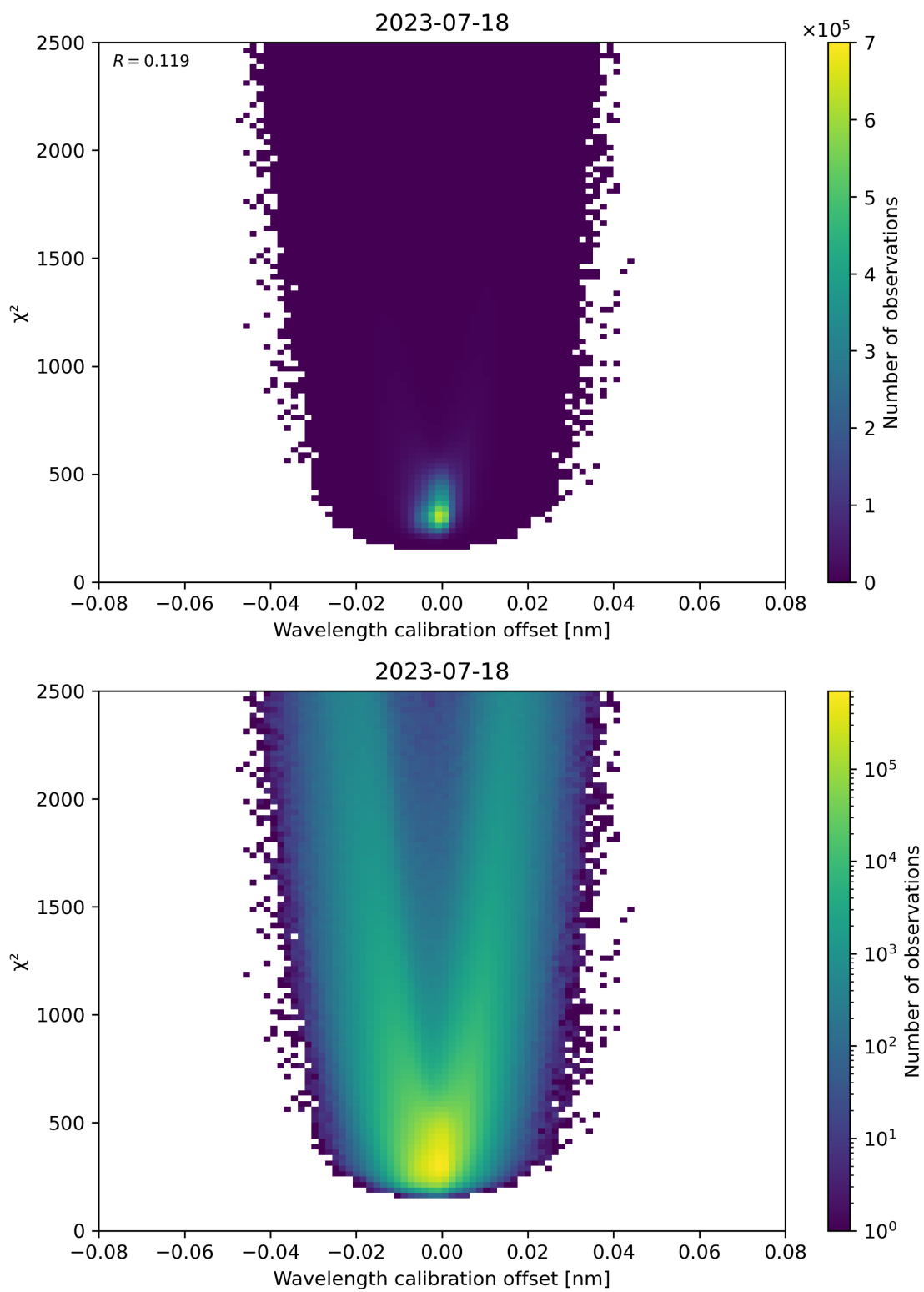
Figure 175: Scatter density plot of “Wavelength calibration offset” against “ \chi^2 ” for 2023-07-17 to 2023-07-19.
