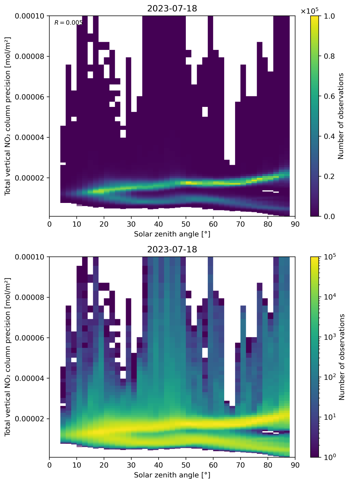
Figure 154: Scatter density plot of “Solar zenith angle” against “Total vertical NO 2 column precision” for 2023-07-17 to 2023-07-19.
