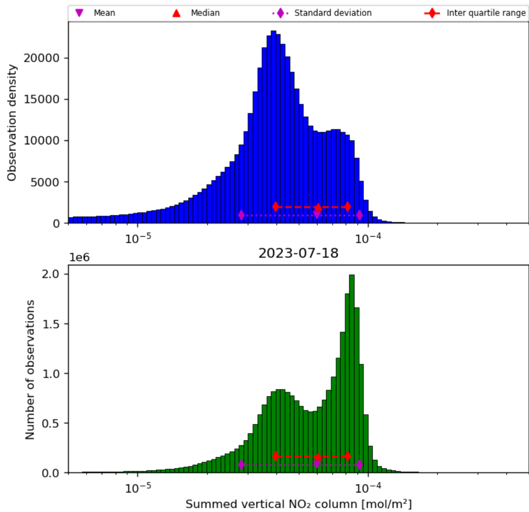
Figure 40: Histogram of “Summed vertical NO 2 column” for 2023-07-17 to 2023-07-19
