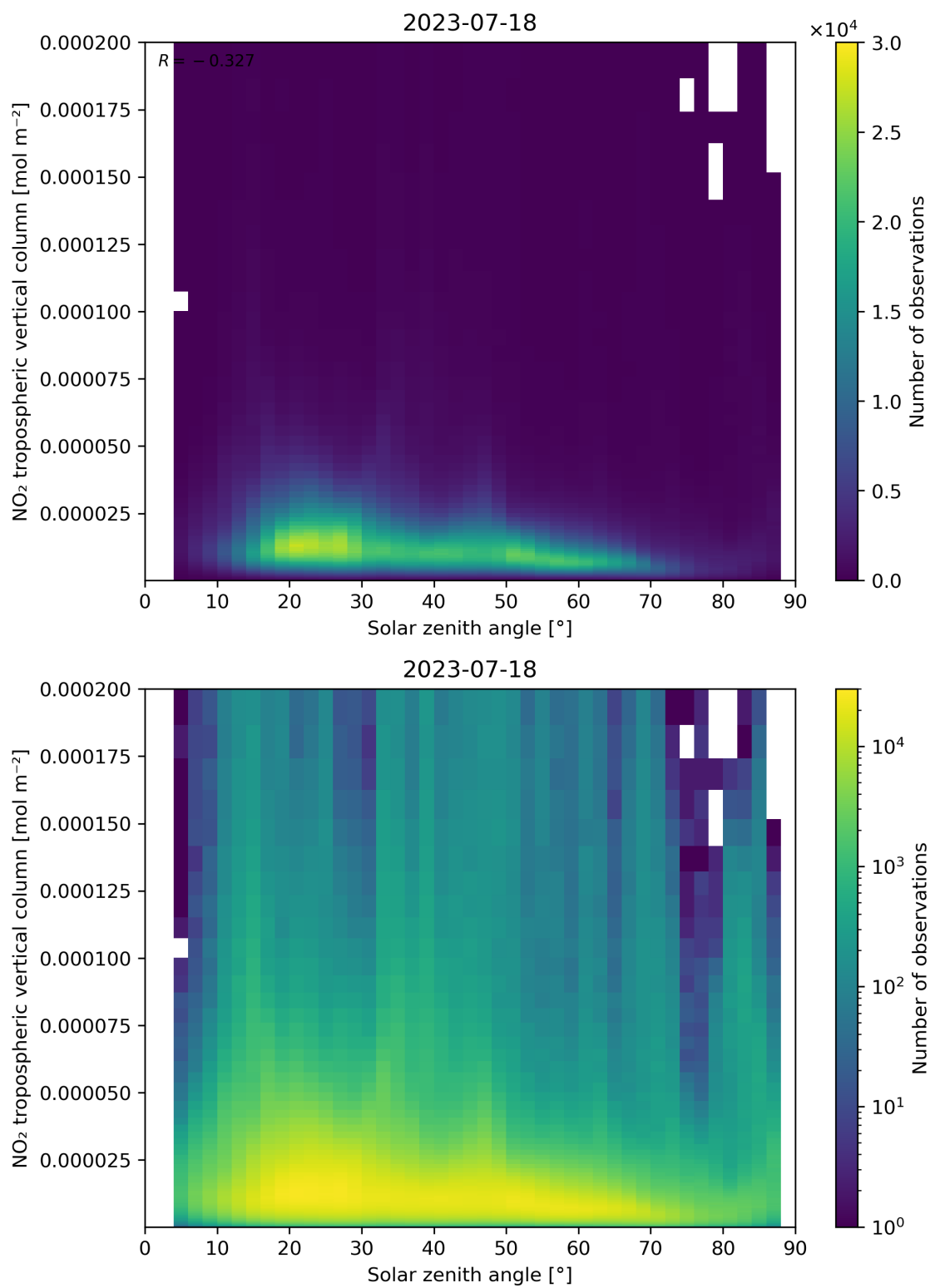
Figure 155: Scatter density plot of “Solar zenith angle” against “NO 2 tropospheric vertical column” for 2023-07-17 to 2023-07-19.
