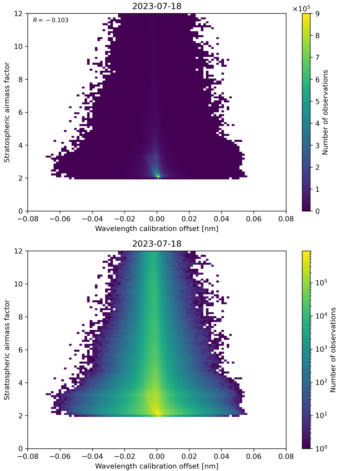
Figure 174: Scatter density plot of “Wavelength calibration offset” against “Stratospheric air mass factor” for 2023-07-17 to 2023-07-19.
