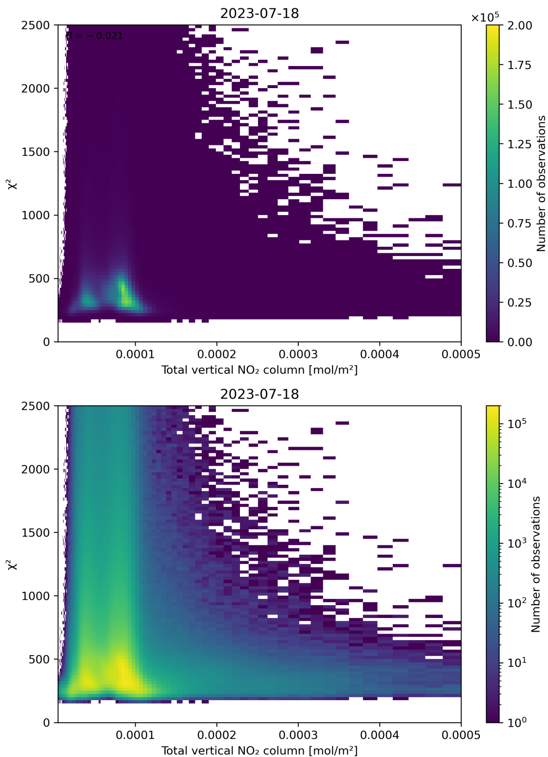
Figure 111: Scatter density plot of “Total vertical NO 2 column” against “ \chi^2 ” for 2023-07-17 to 2023-07-19.
