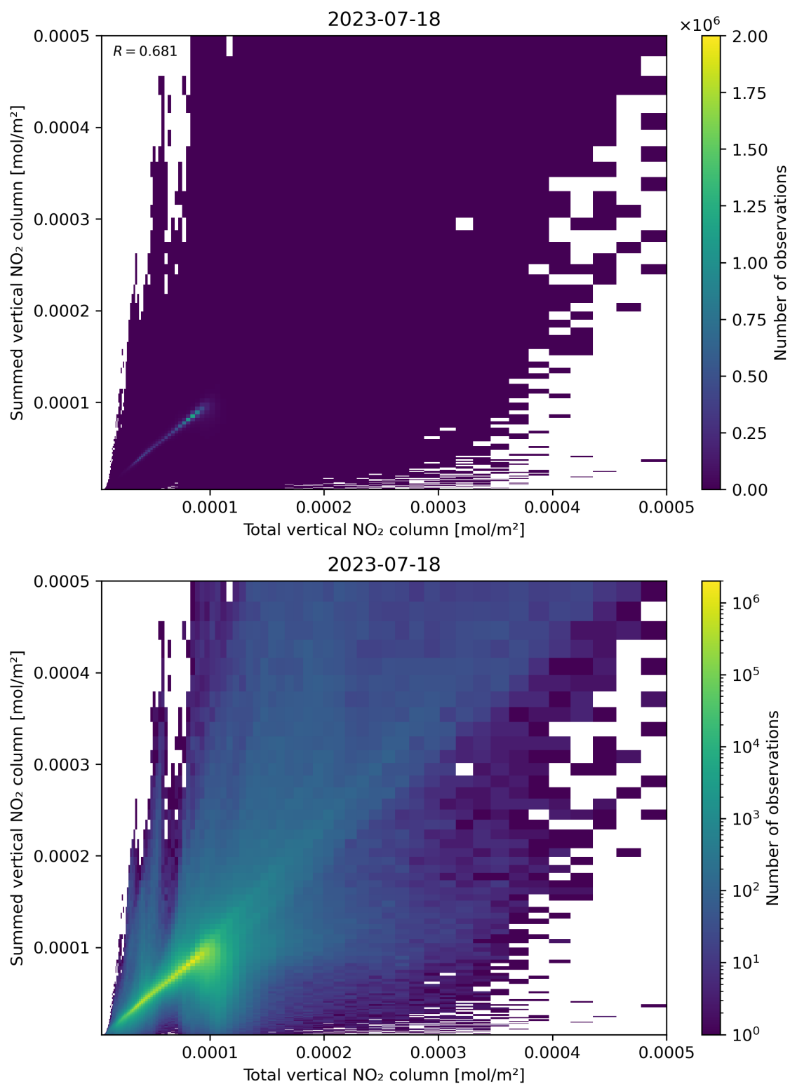
Figure 112: Scatter density plot of “Total vertical NO 2 column” against “Summed vertical NO 2 column” for 2023-07-17 to 2023-07-19.
