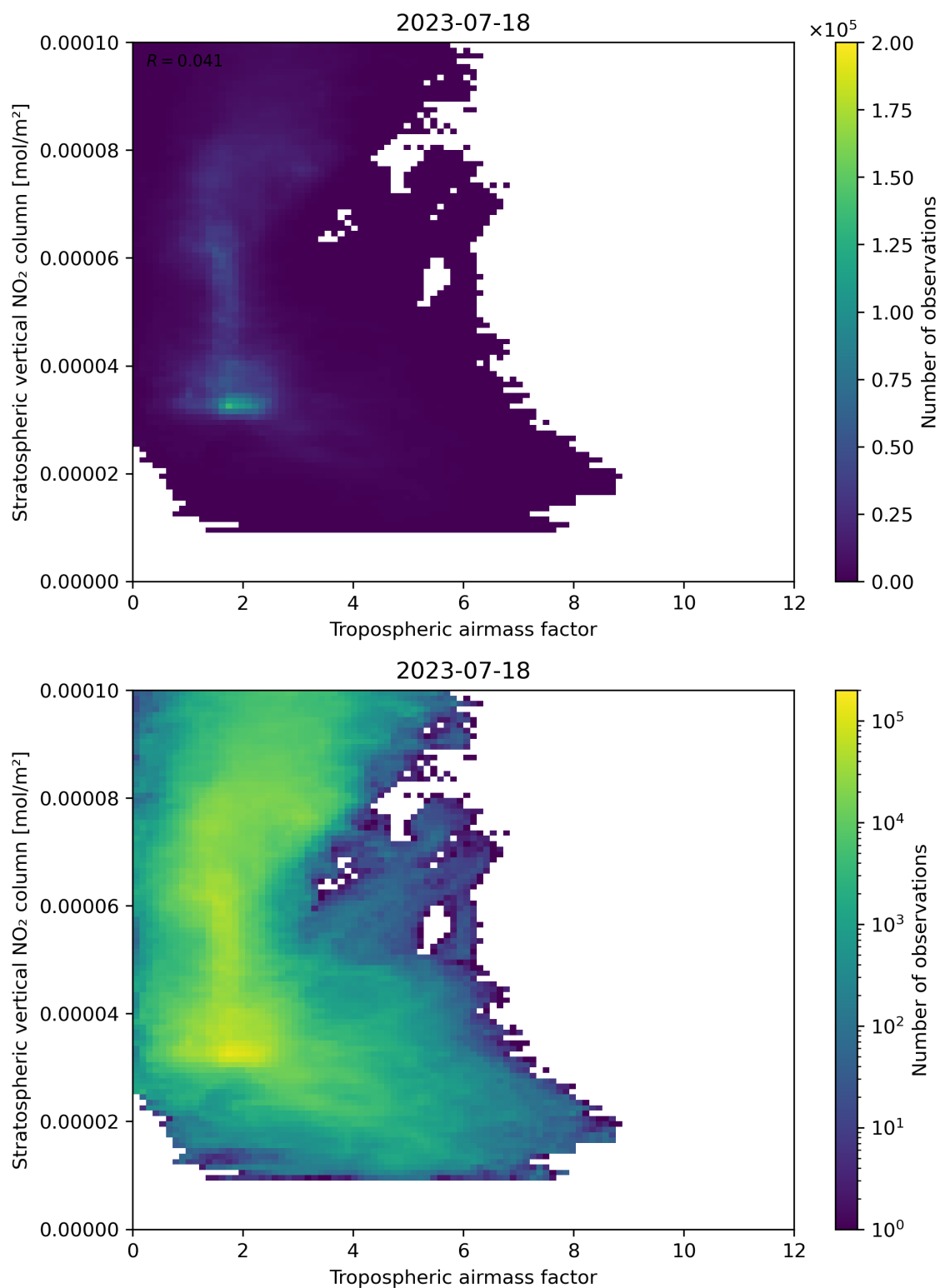
Figure 74: Scatter density plot of “Tropospheric air mass factor” against “Stratospheric vertical NO 2 column” for 2023-07-17 to 2023-07-19.
