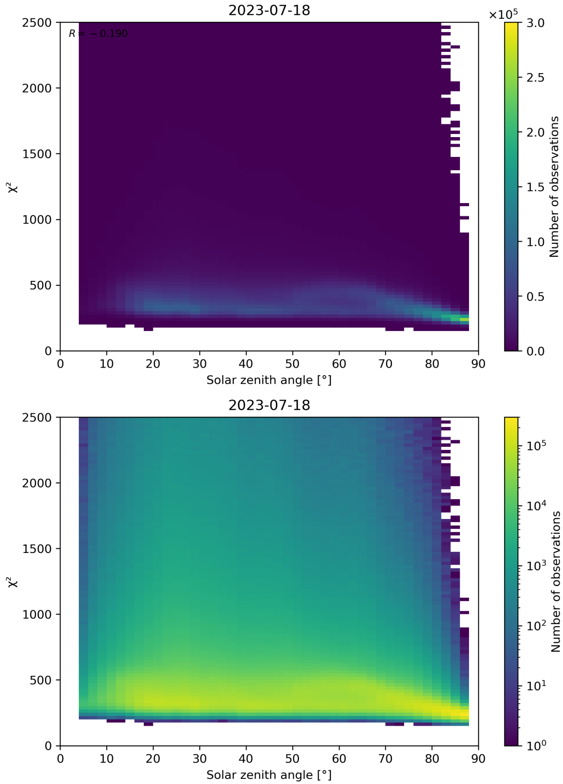
Figure 148: Scatter density plot of “Solar zenith angle” against “ \chi^2 ” for 2023-07-17 to 2023-07-19.
