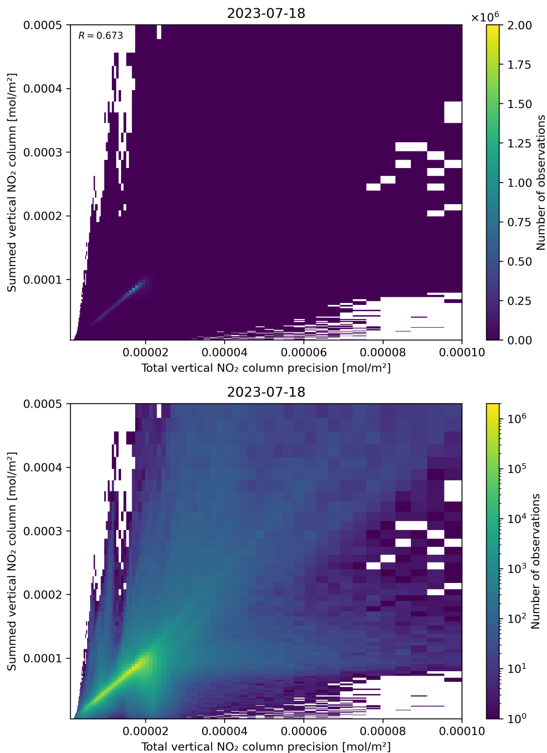
Figure 117: Scatter density plot of “Total vertical NO 2 column precision” against “Summed vertical NO 2 column” for 2023-07-17 to 2023-07-19.
