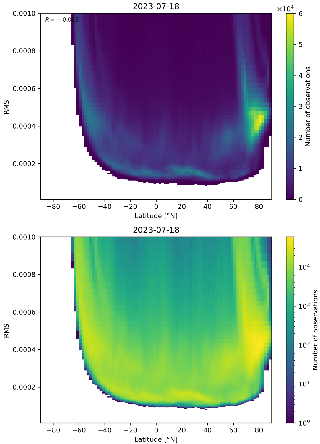
Figure 94: Scatter density plot of “Latitude” against “RMS” for 2023-07-17 to 2023-07-19.
