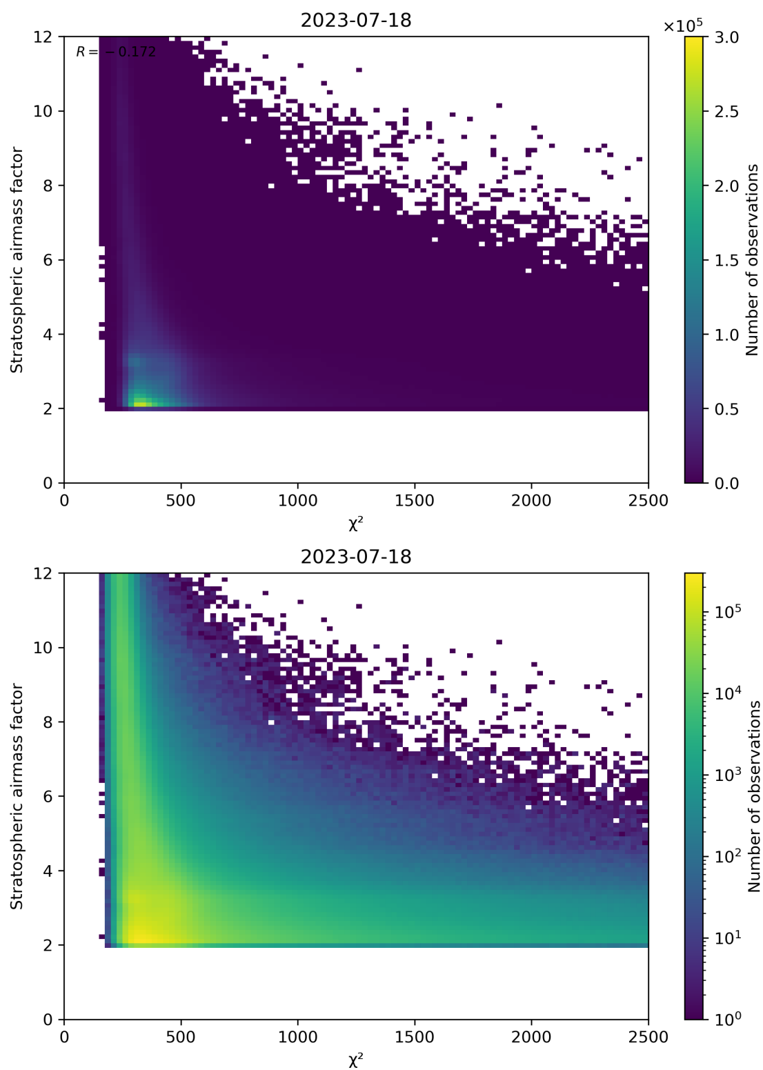
Figure 81: Scatter density plot of “ \chi^2 ” against “Stratospheric airmass factor” for 2023-07-17 to 2023-07-19.
