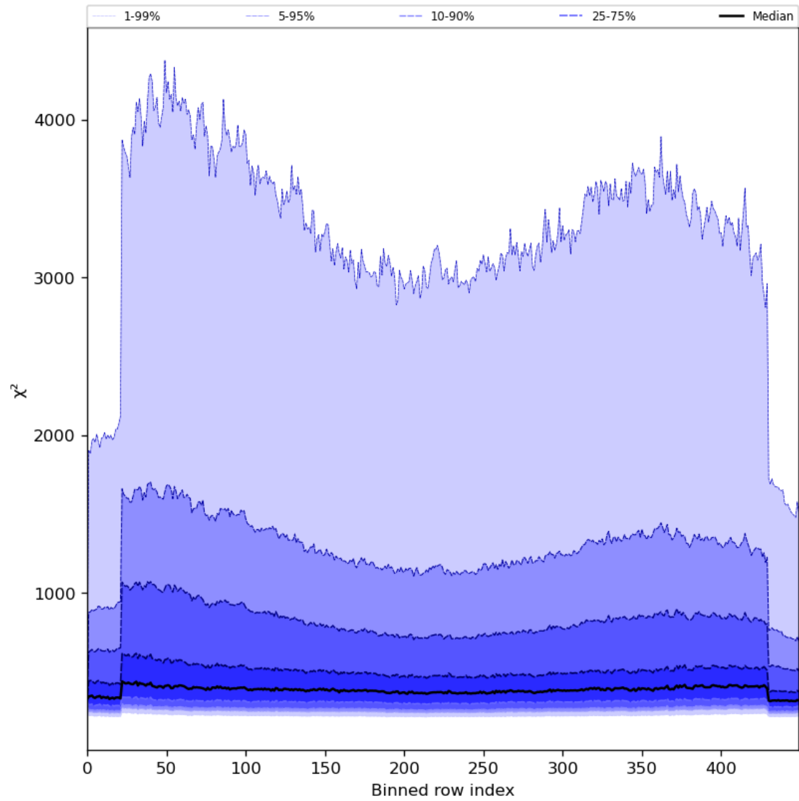
Figure 59: Along track statistics of “ \chi^2 ” for 2023-07-17 to 2023-07-19
