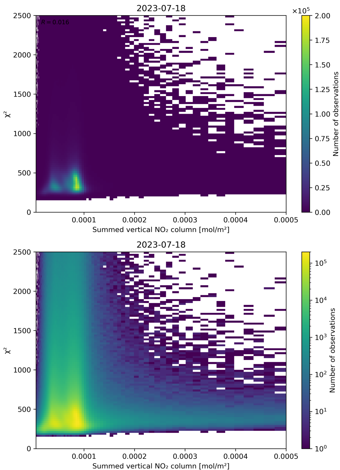
Figure 104: Scatter density plot of “Summed vertical NO 2 column” against “ \chi^2 ” for 2023-07-17 to 2023-07-19.
