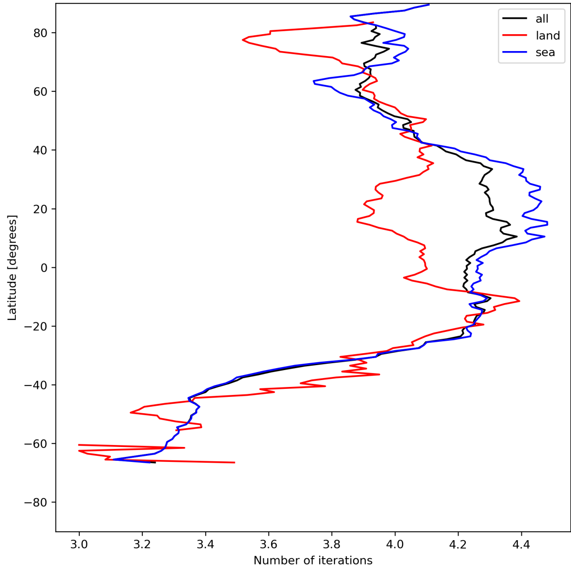
Figure 17: Zonal average of “Number of iterations” for 2023-07-17 to 2023-07-19.
