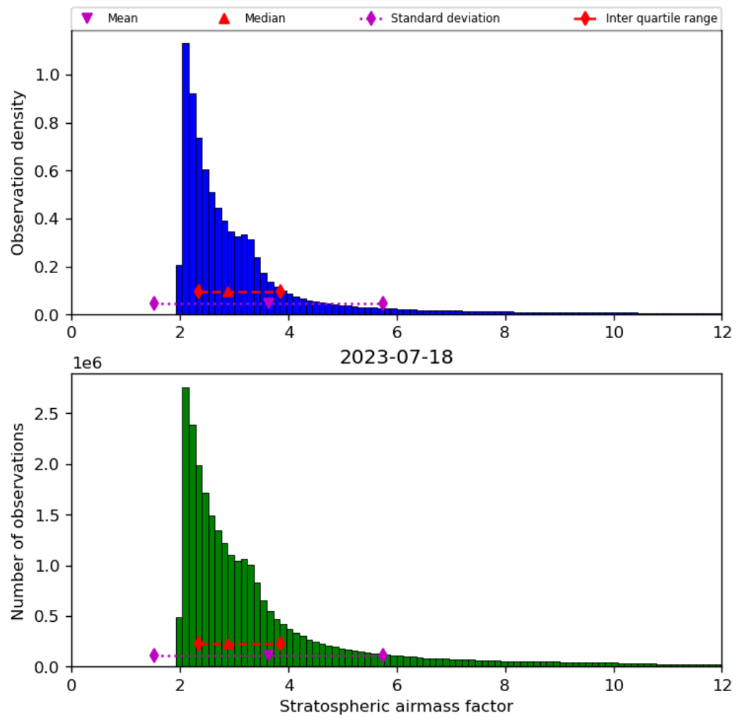
Figure 44: Histogram of “Stratospheric airmass factor” for 2023-07-17 to 2023-07-19
