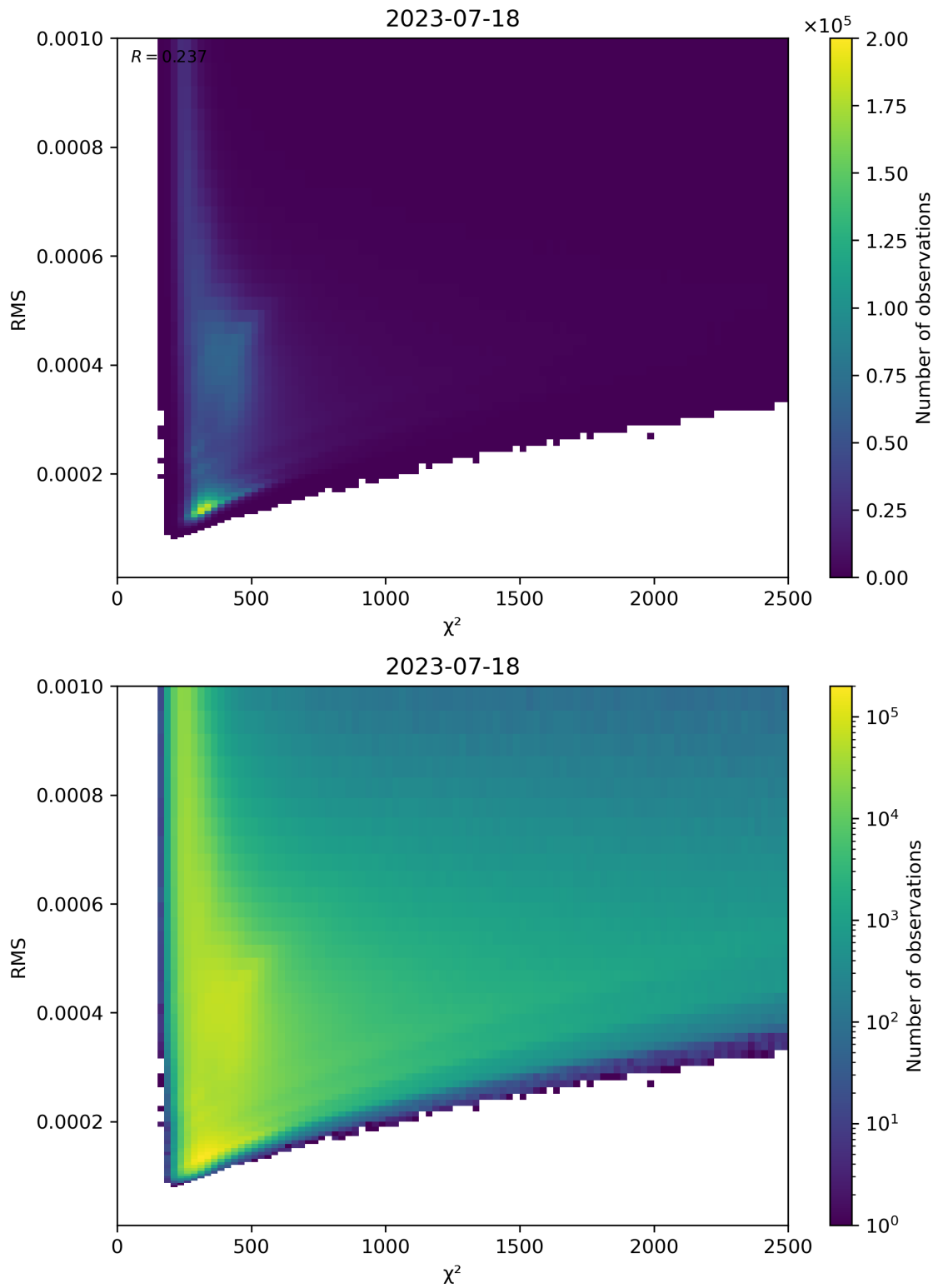
Figure 82: Scatter density plot of “ \chi^2 ” against “RMS” for 2023-07-17 to 2023-07-19.
