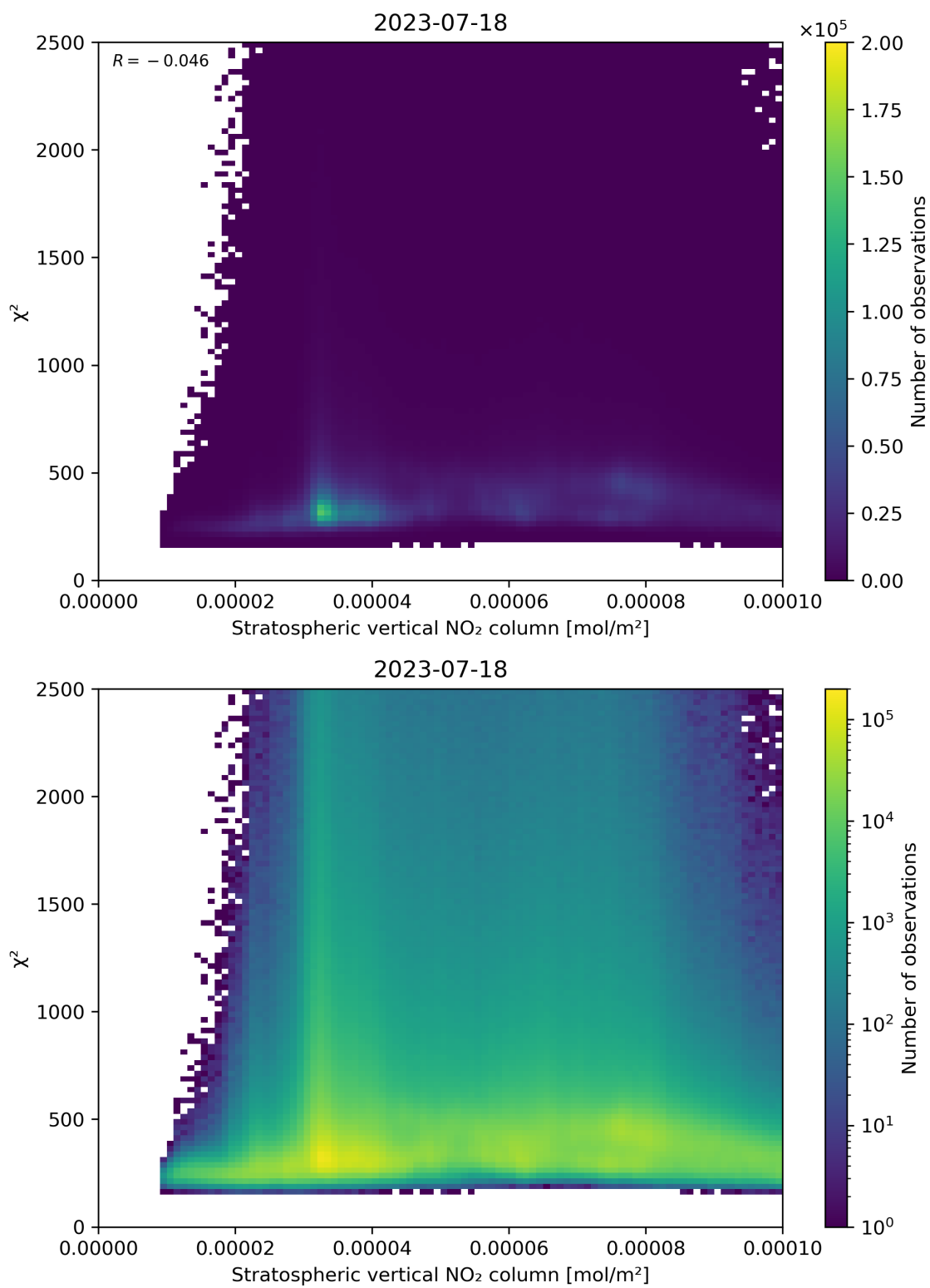
Figure 97: Scatter density plot of “Stratospheric vertical NO 2 column” against “ \chi^2 ” for 2023-07-17 to 2023-07-19.
