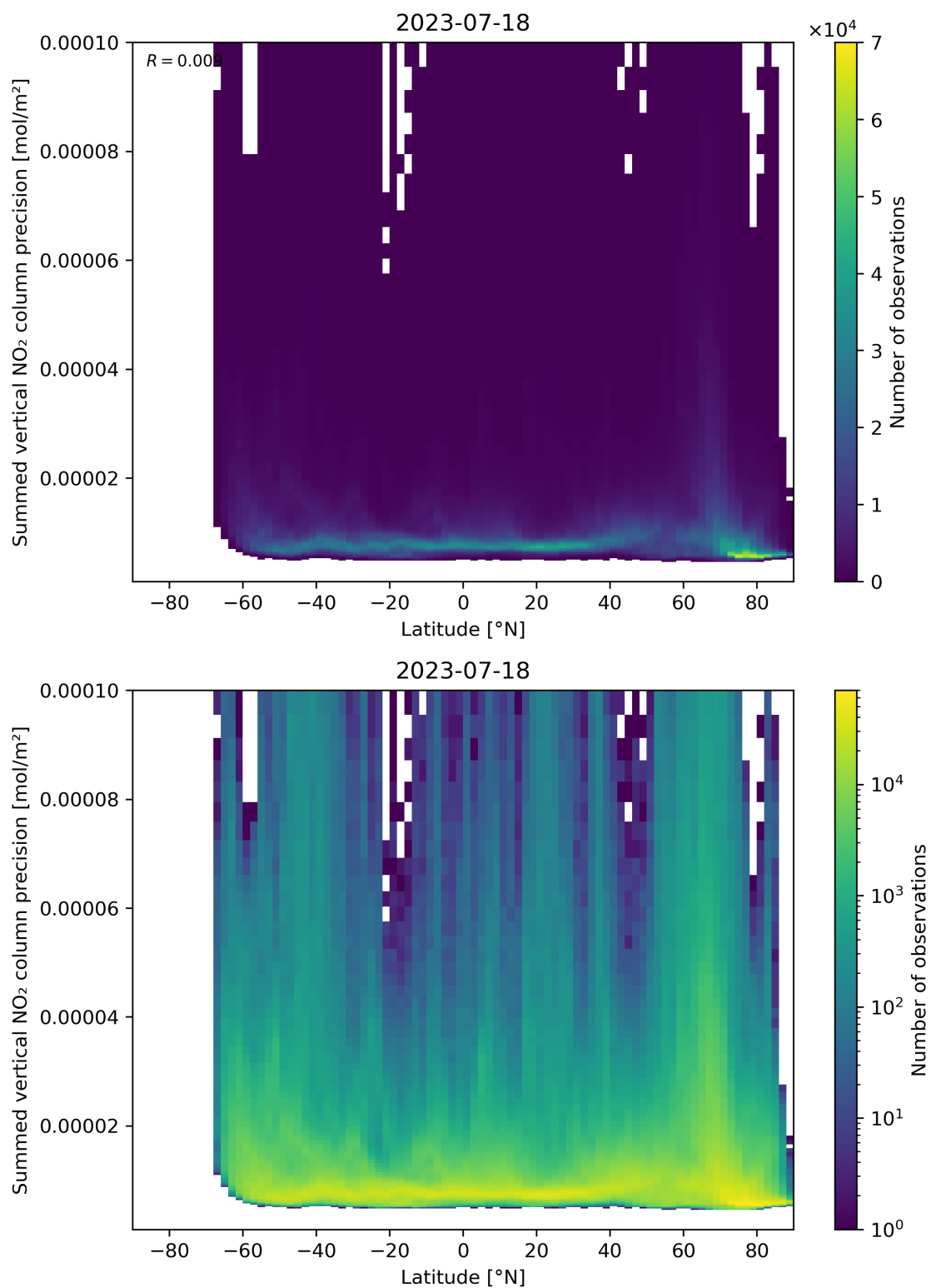
Figure 89: Scatter density plot of “Latitude” against “Summed vertical NO 2 column precision” for 2023-07-17 to 2023-07-19.
