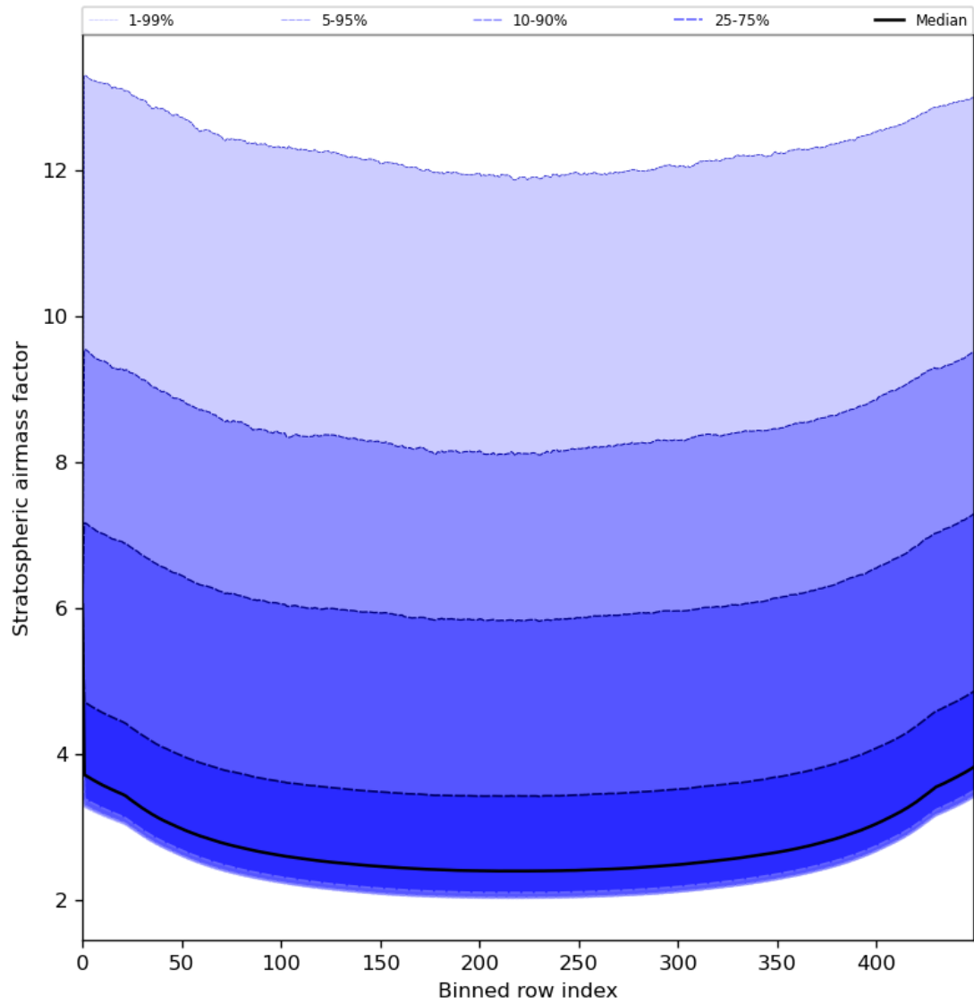
Figure 61: Along track statistics of “Stratospheric airmass factor” for 2023-07-17 to 2023-07-19
