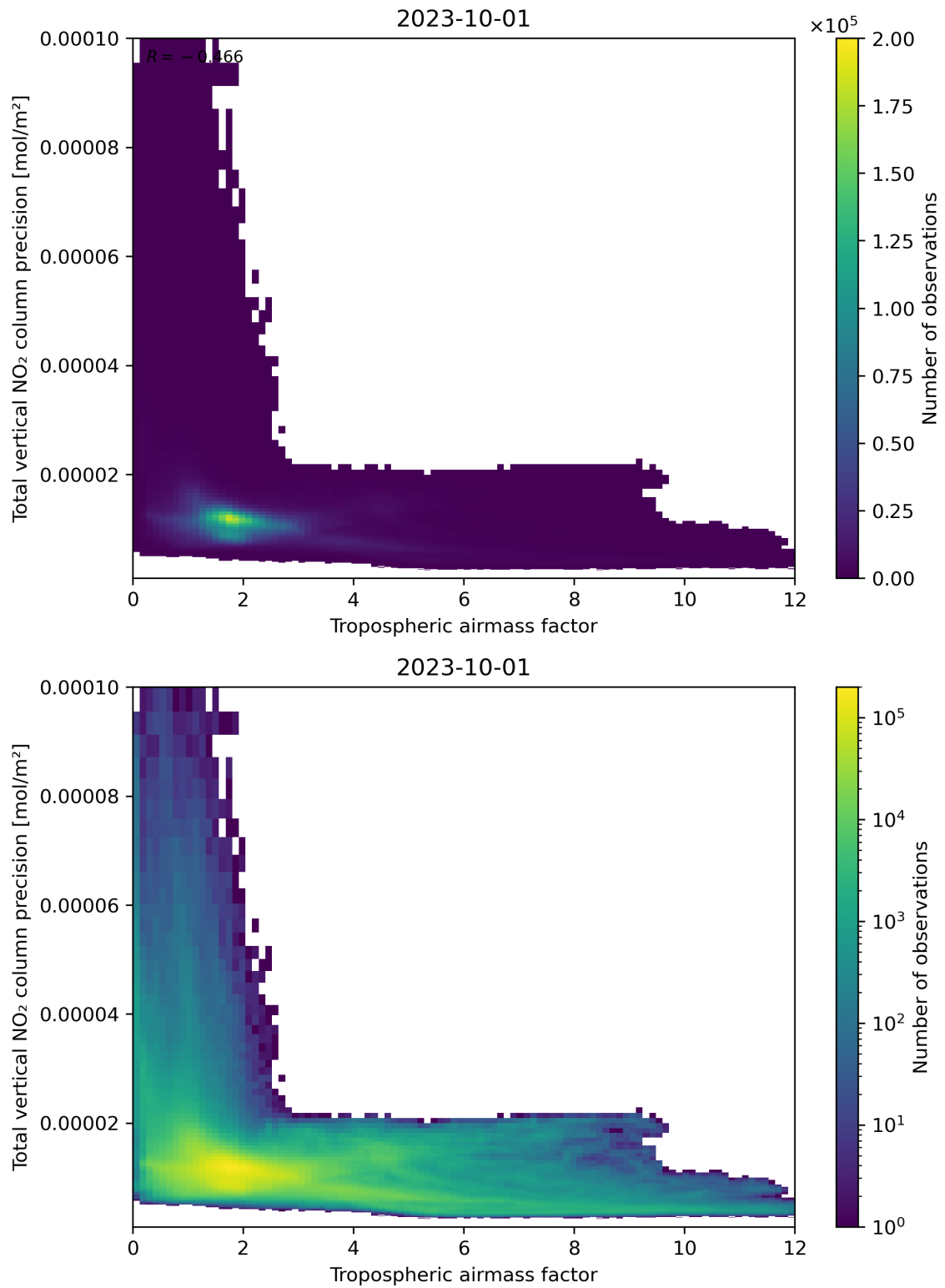
Figure 78: Scatter density plot of “Tropospheric air mass factor” against “Total vertical NO 2 column precision” for 2023-10-01 to 2023-10-02.
