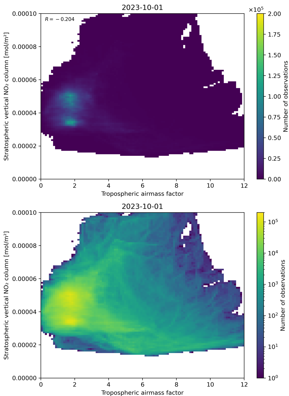
Figure 74: Scatter density plot of “Tropospheric air mass factor” against “Stratospheric vertical NO 2 column” for 2023-10-01 to 2023-10-02.
