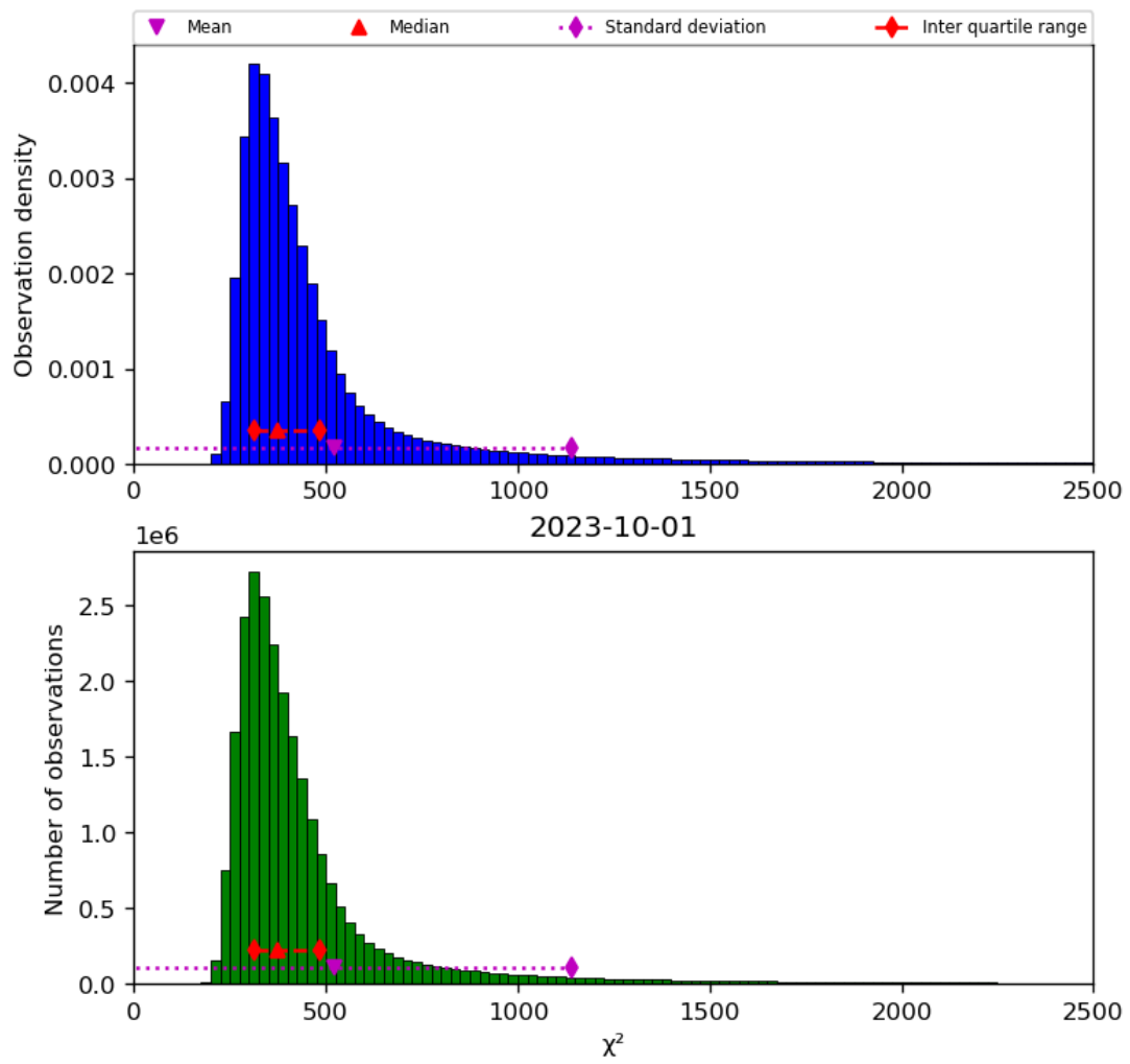
Figure 42: Histogram of “ \chi^2 ” for 2023-10-01 to 2023-10-02
