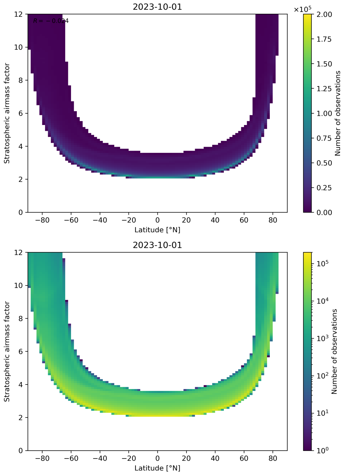
Figure 83: Scatter density plot of “Latitude” against “Stratospheric air mass factor” for 2023-10-01 to 2023-10-02.
