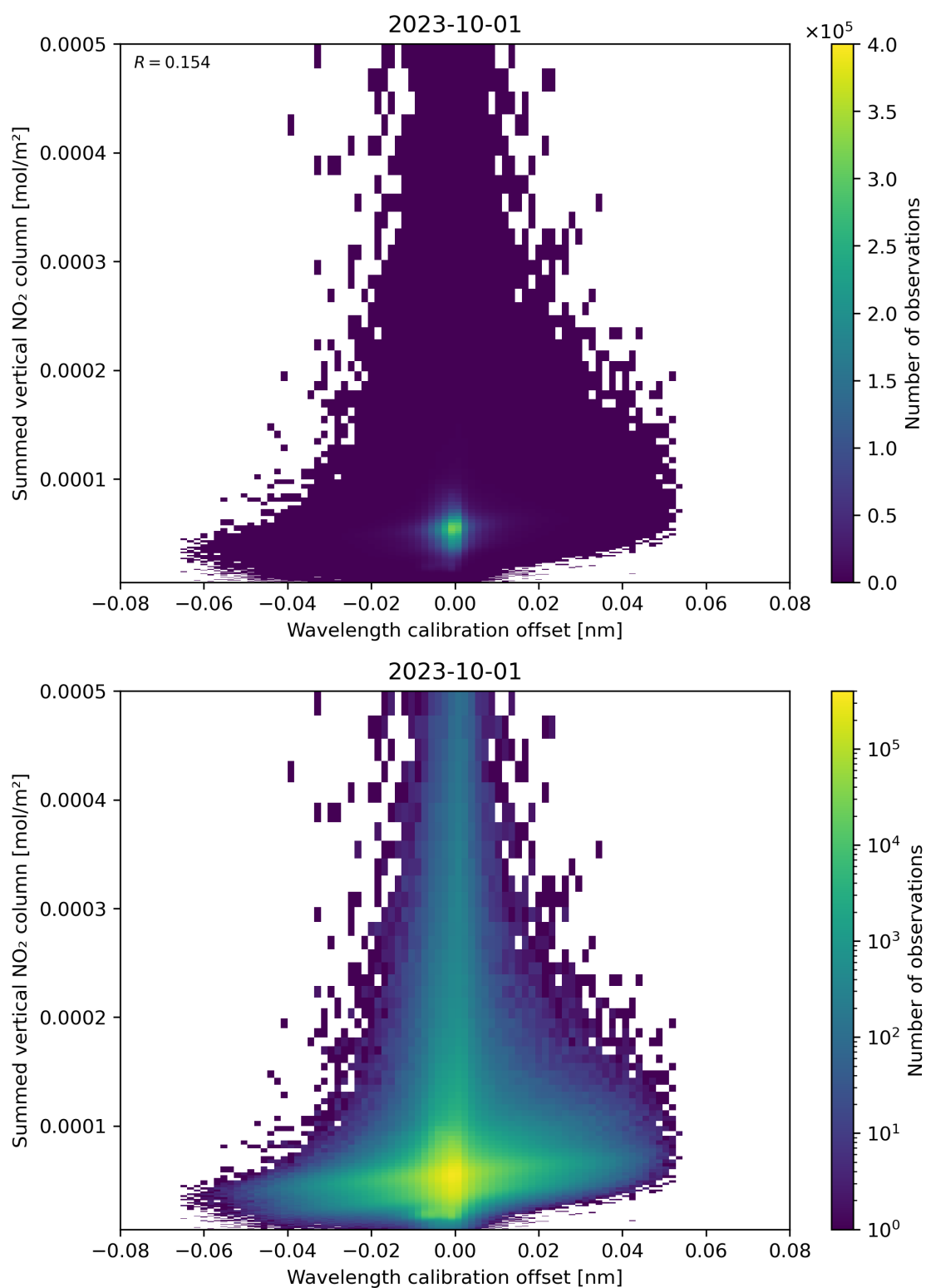
Figure 177: Scatter density plot of “Wavelength calibration offset” against “Summed vertical NO 2 column” for 2023-10-01 to 2023-10-02.
