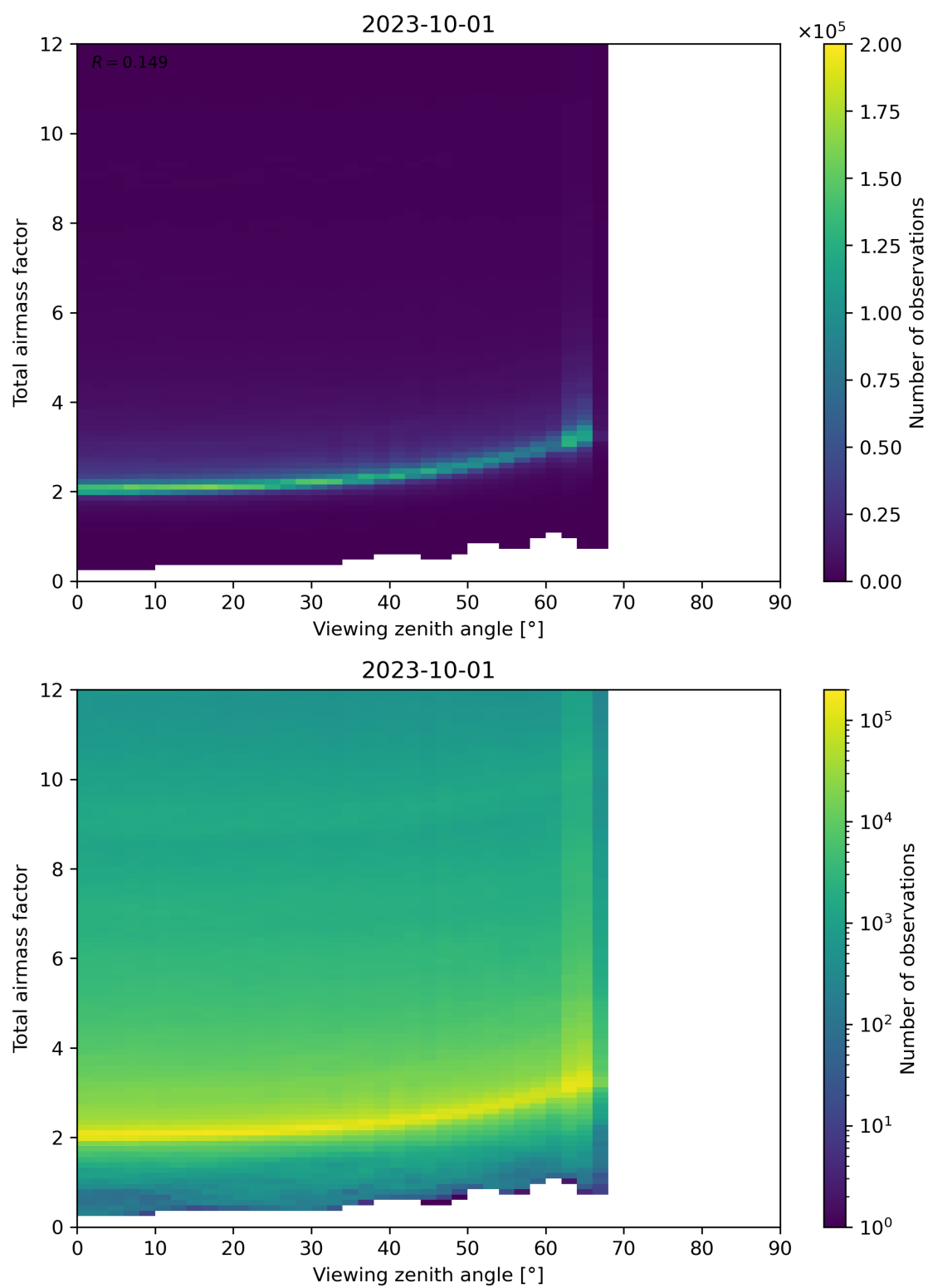
Figure 160: Scatter density plot of “Viewing zenith angle” against “Total airmass factor” for 2023-10-01 to 2023-10-02.
