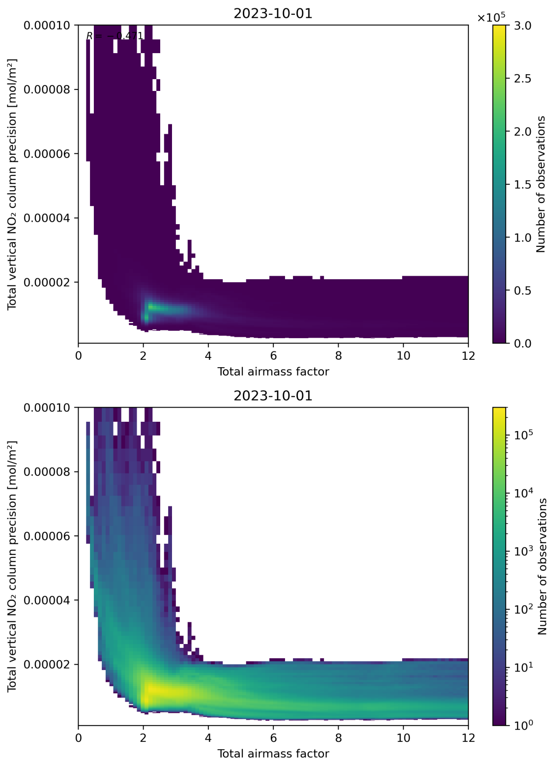
Figure 68: Scatter density plot of “Total airmass factor” against “Total vertical NO 2 column precision” for 2023-10-01 to 2023-10-02.
