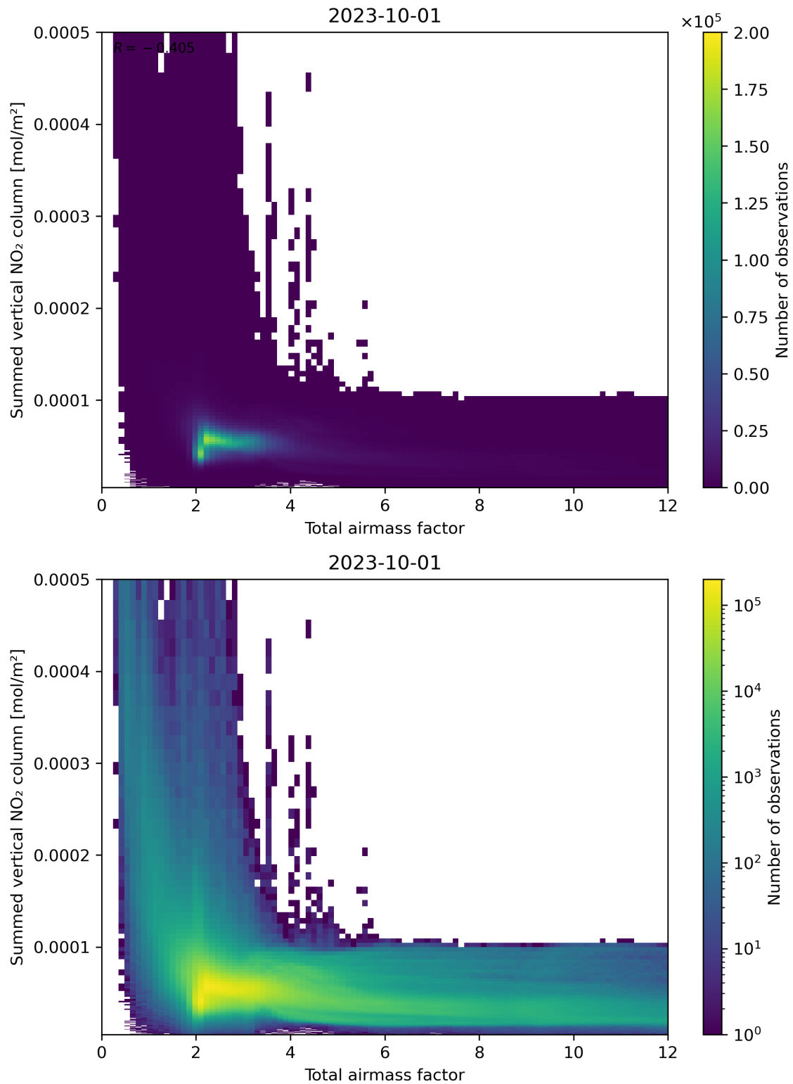
Figure 65: Scatter density plot of “Total airmass factor” against “Summed vertical NO 2 column” for 2023-10-01 to 2023-10-02.
