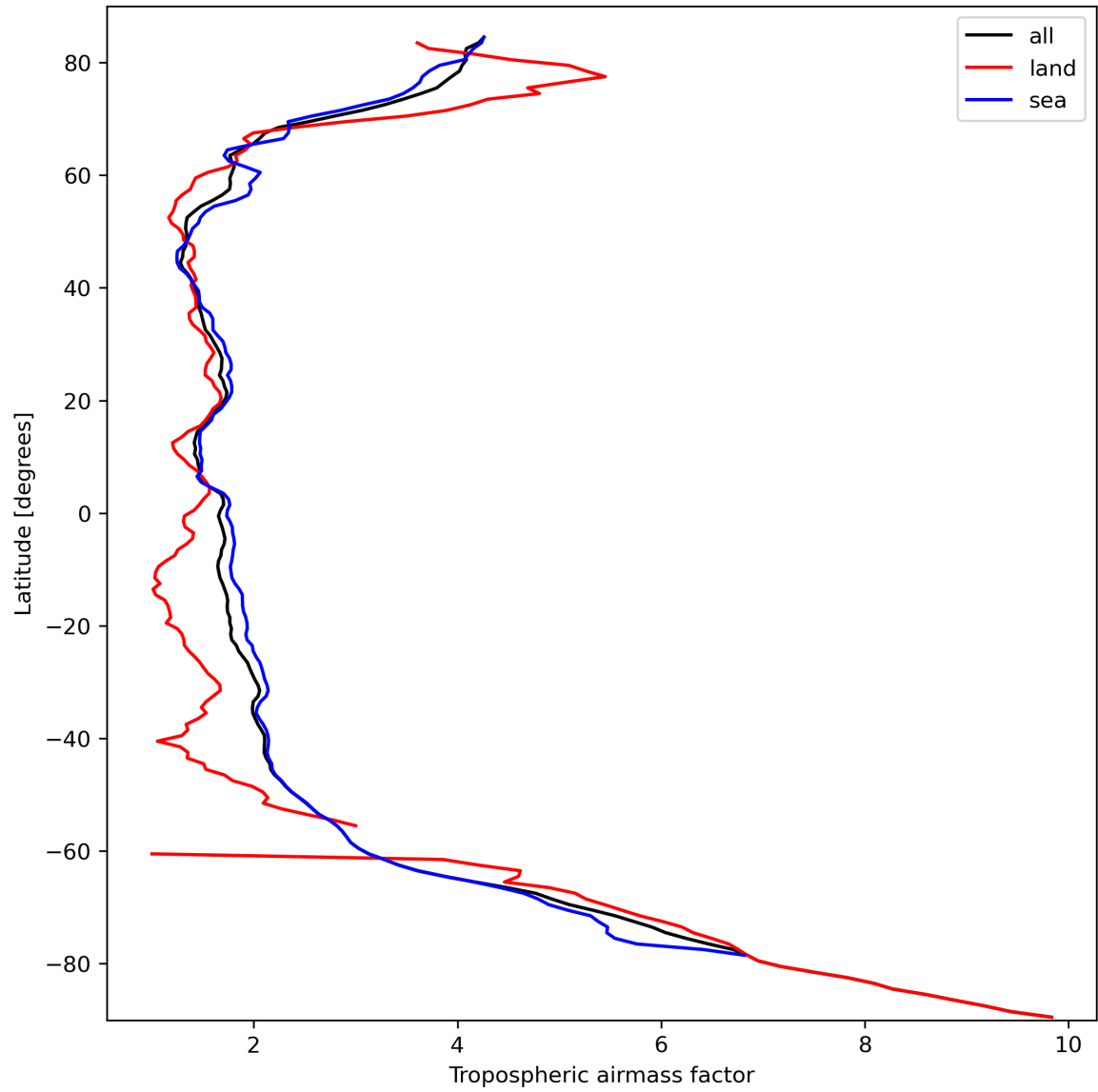
Figure 14: Zonal average of “Tropospheric airmass factor” for 2023-10-01 to 2023-10-02.
