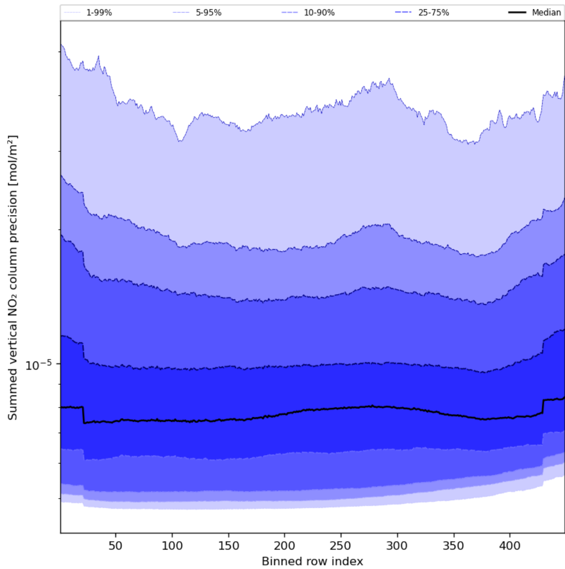
Figure 58: Along track statistics of “Summed vertical NO 2 column precision” for 2023-10-01 to 2023-10-02
