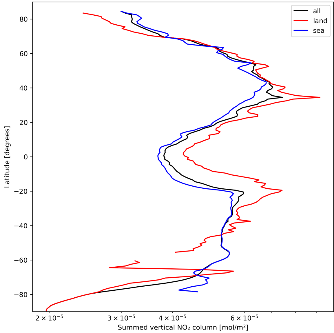
Figure 23: Zonal average of “Summed vertical NO 2 column” for 2023-10-01 to 2023-10-02.
