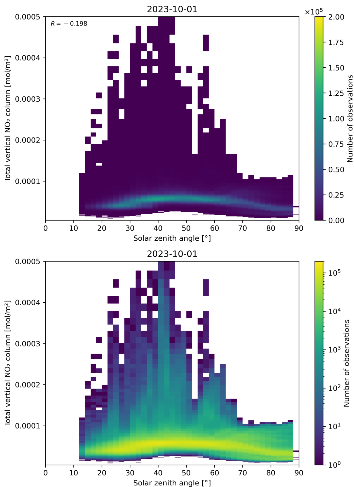
Figure 153: Scatter density plot of “Solar zenith angle” against “Total vertical NO 2 column” for 2023-10-01 to 2023-10-02.
