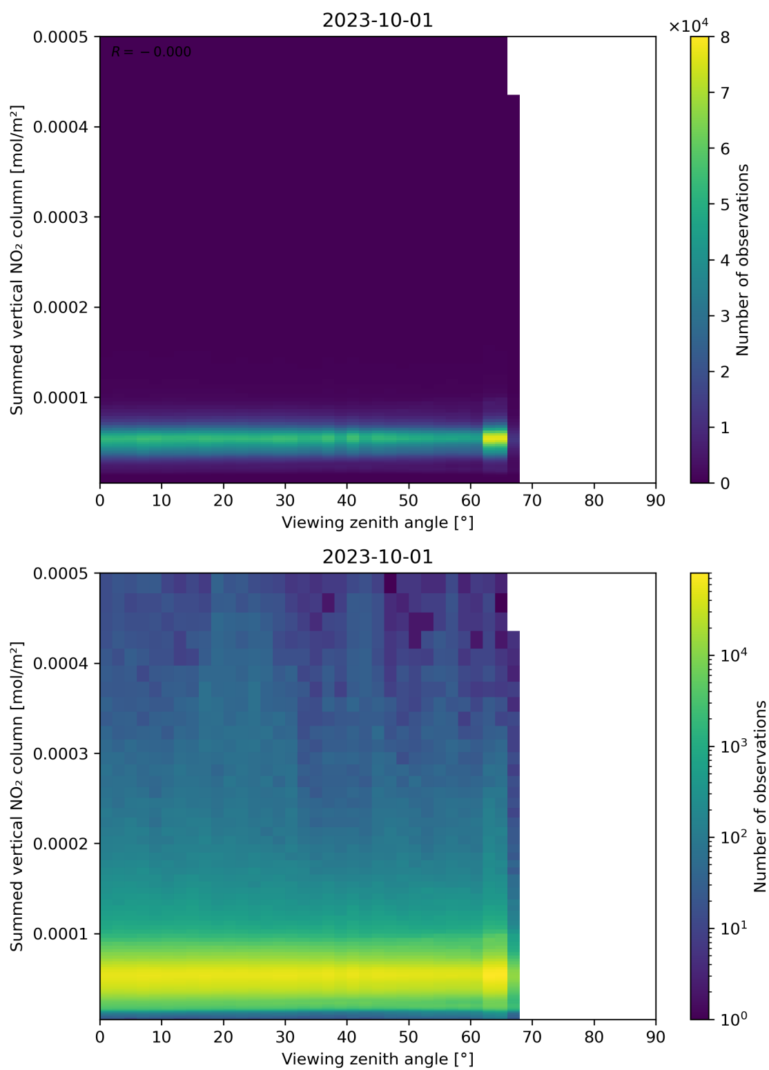
Figure 165: Scatter density plot of “Viewing zenith angle” against “Summed vertical NO 2 column” for 2023-10-01 to 2023-10-02.
