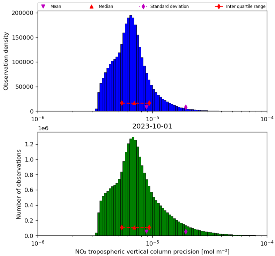
Figure 30: Histogram of “ \text{NO}_2 tropospheric vertical column precision” for 2023-10-01 to 2023-10-02
