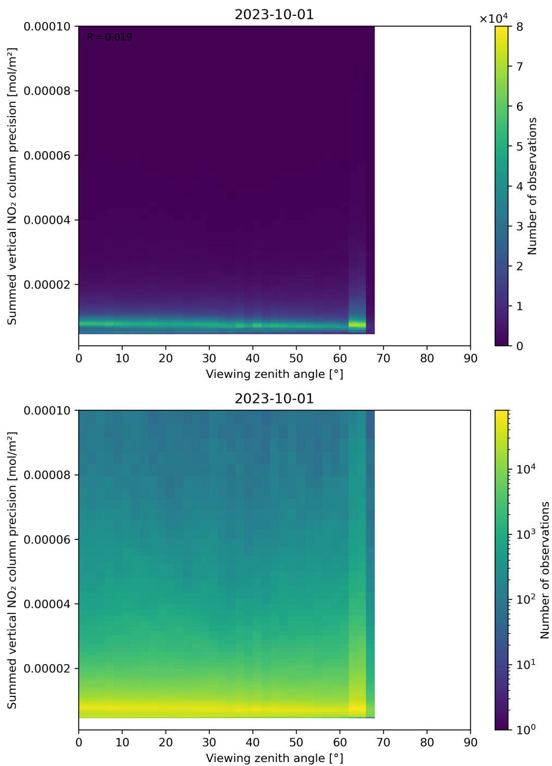
Figure 166: Scatter density plot of “Viewing zenith angle” against “Summed vertical NO 2 column precision” for 2023-10-01 to 2023-10-02.
