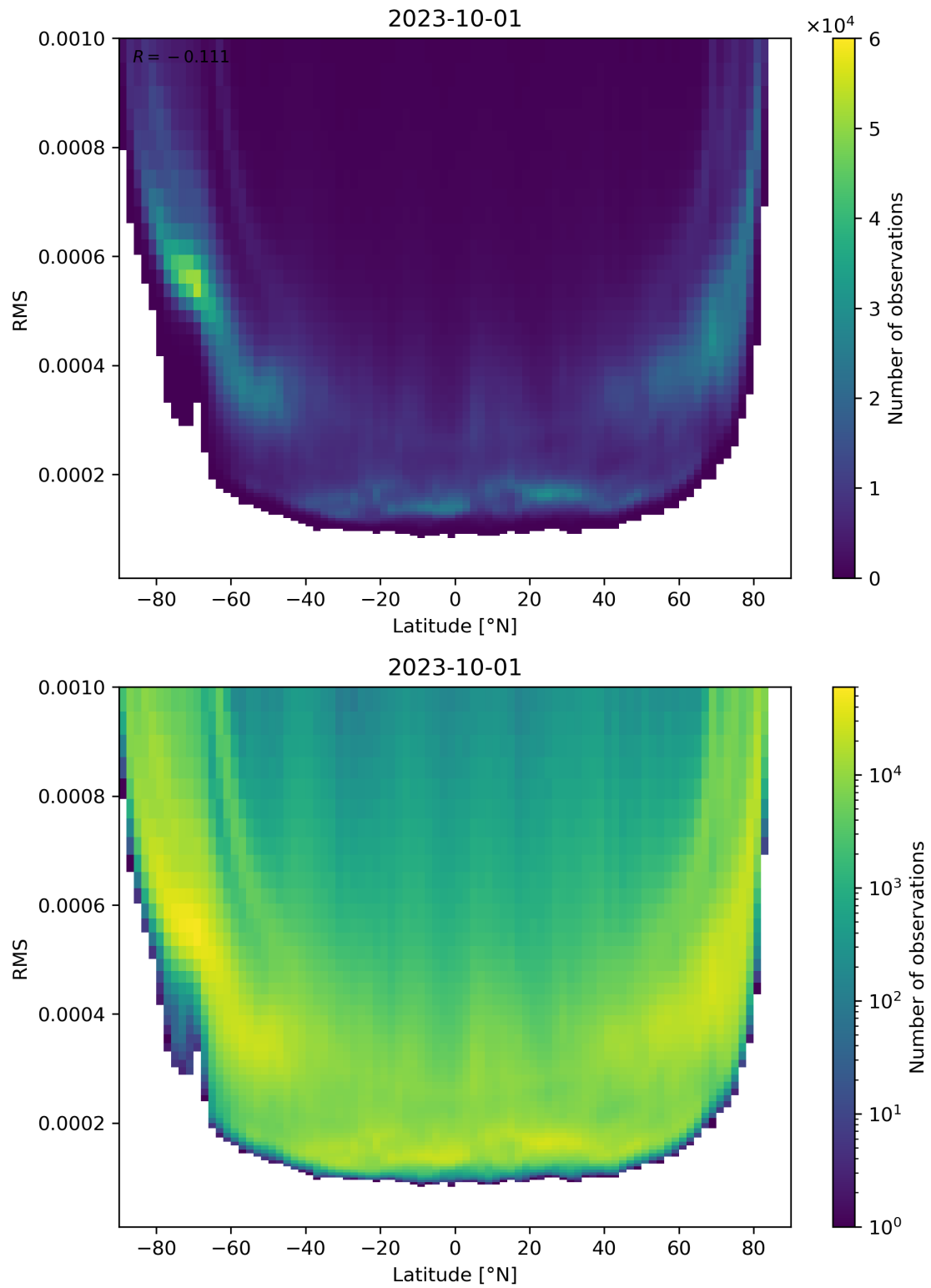
Figure 94: Scatter density plot of “Latitude” against “RMS” for 2023-10-01 to 2023-10-02.
