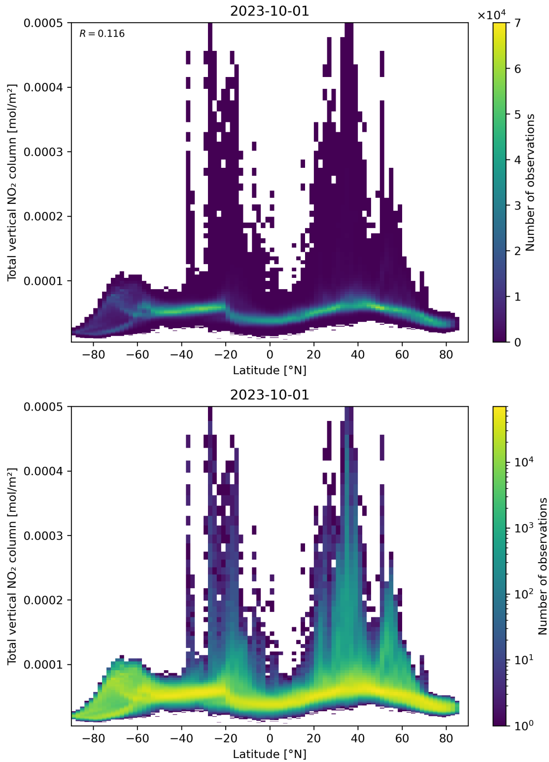
Figure 90: Scatter density plot of “Latitude” against “Total vertical NO 2 column” for 2023-10-01 to 2023-10-02.
