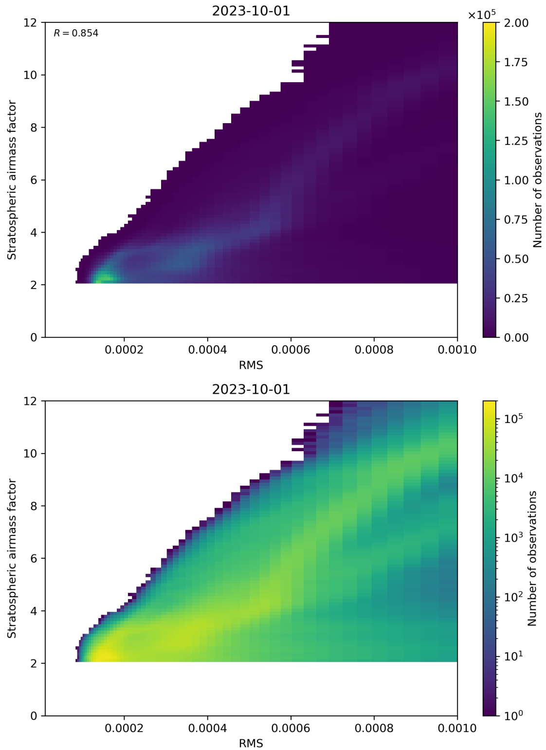
Figure 144: Scatter density plot of “RMS” against “Stratospheric airmass factor” for 2023-10-01 to 2023-10-02.
