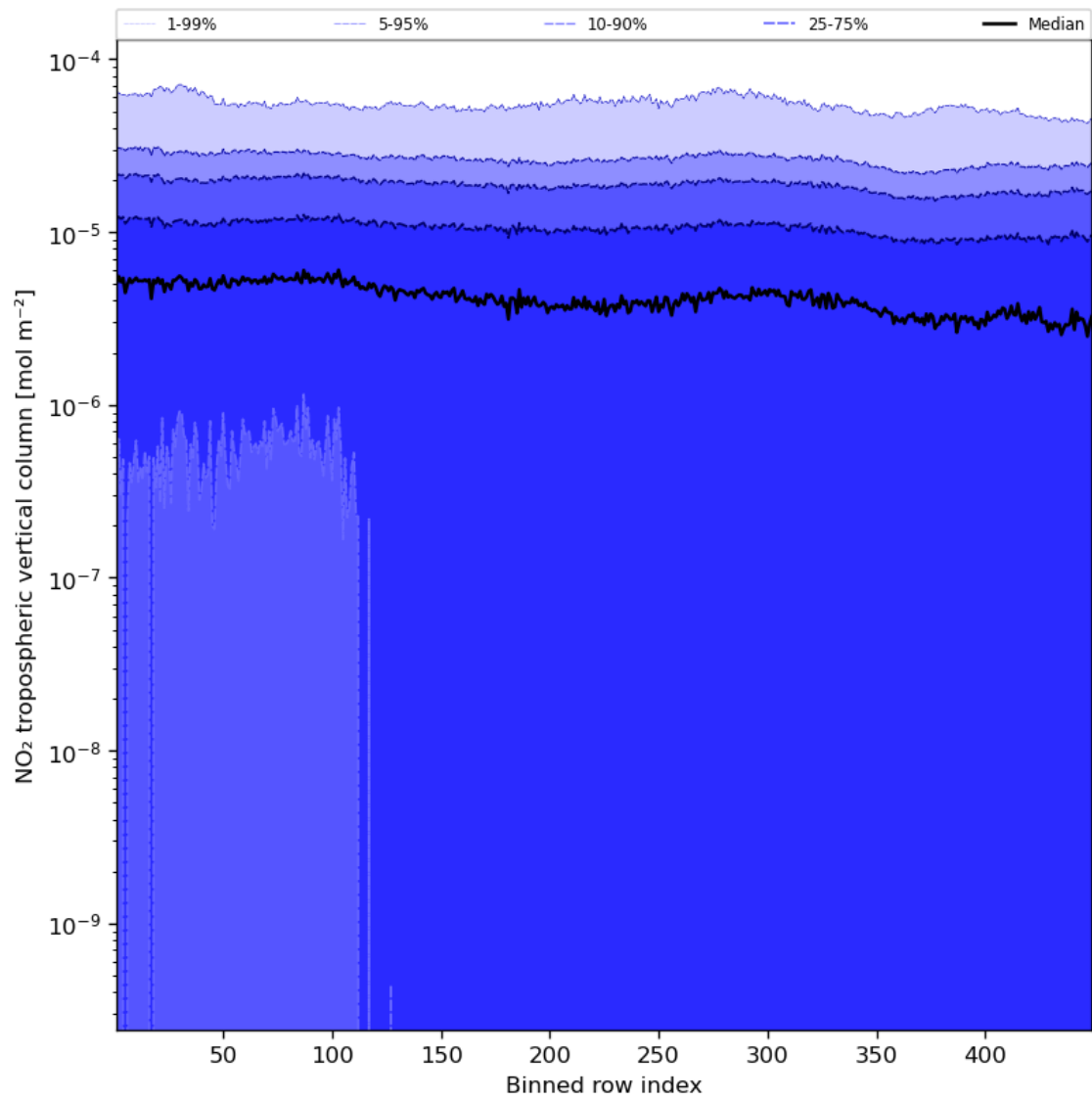
Figure 46: Along track statistics of “NO 2 tropospheric vertical column” for 2023-10-01 to 2023-10-02
