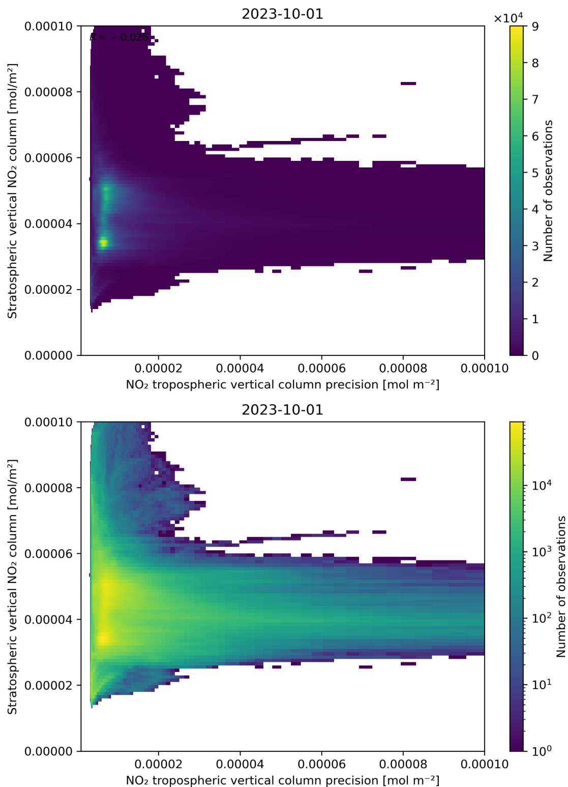
Figure 135: Scatter density plot of “NO 2 tropospheric vertical column precision” against “Stratospheric vertical NO 2 column” for 2023-10-01 to 2023-10-02.
