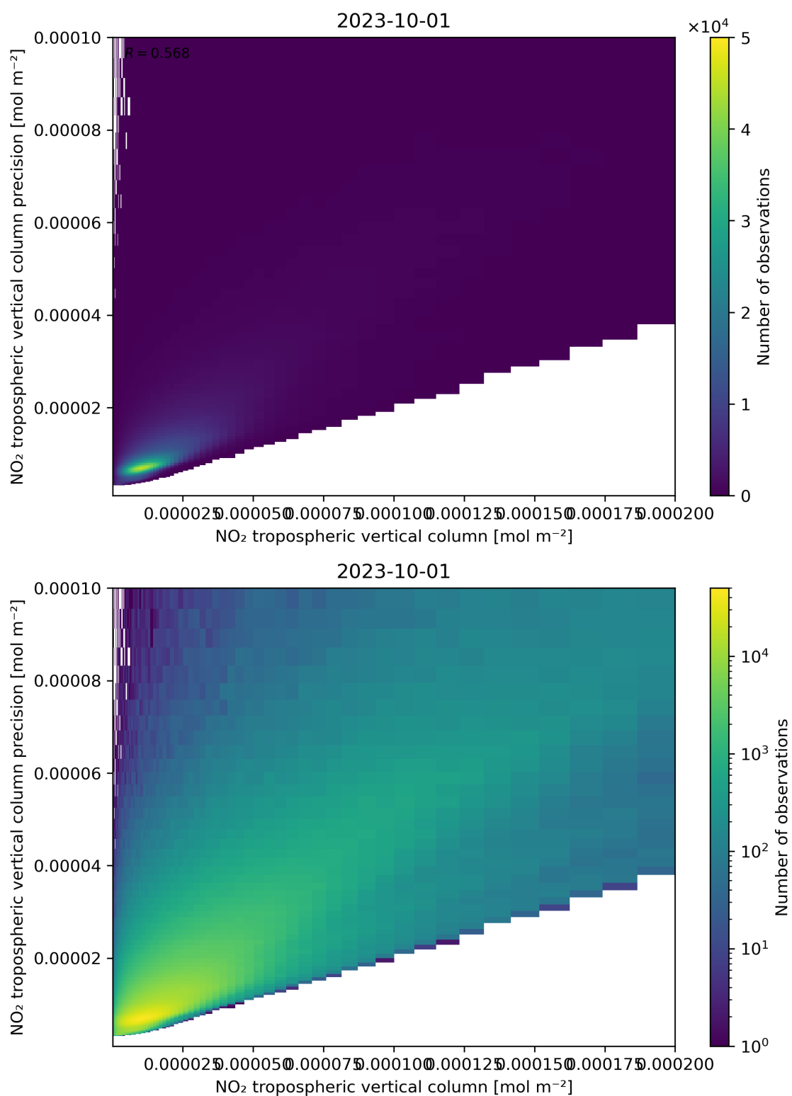
Figure 130: Scatter density plot of “NO 2 tropospheric vertical column” against “NO 2 tropospheric vertical column precision” for 2023-10-01 to 2023-10-02.
