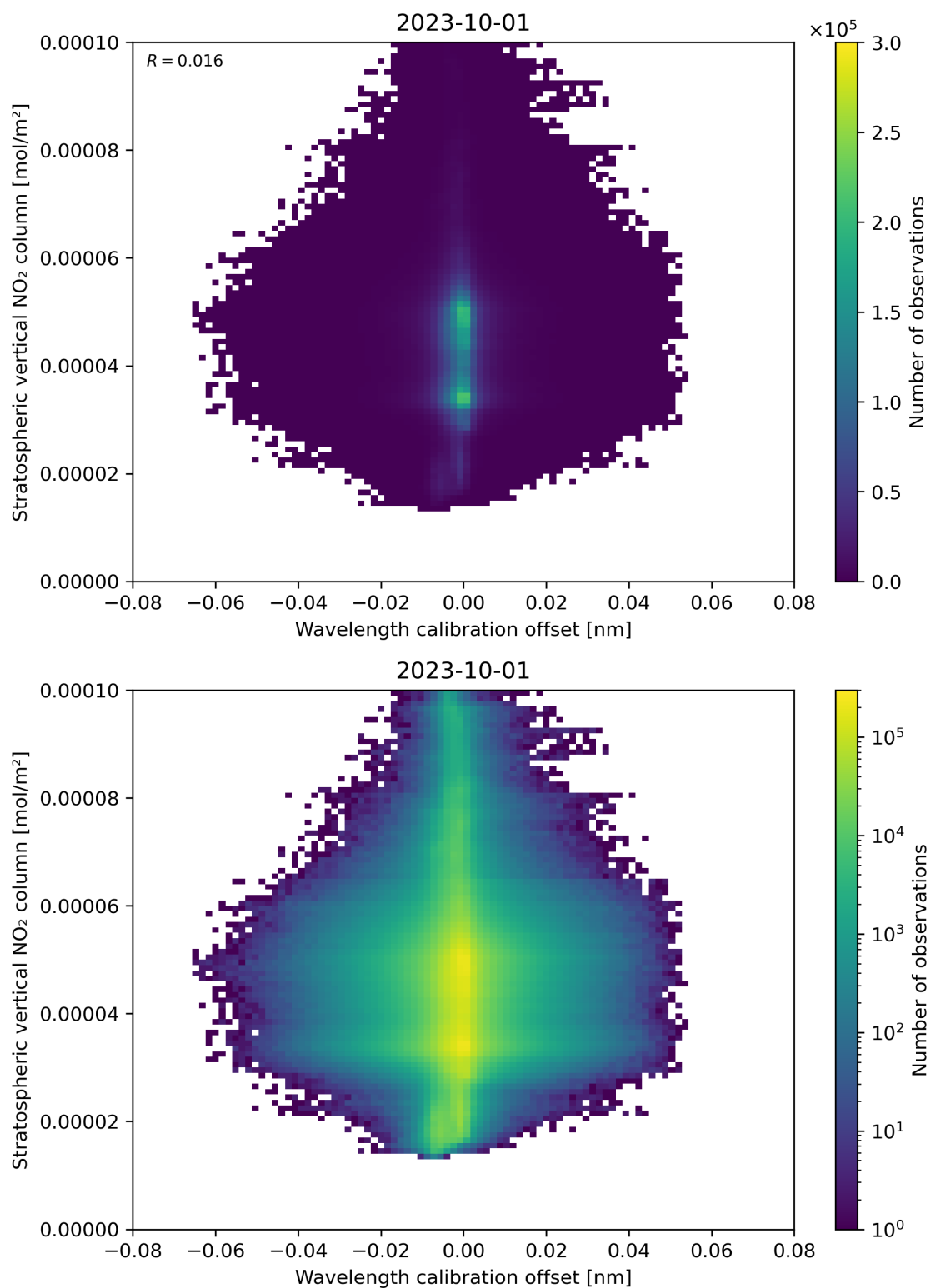
Figure 176: Scatter density plot of “Wavelength calibration offset” against “Stratospheric vertical NO 2 column” for 2023-10-01 to 2023-10-02.
