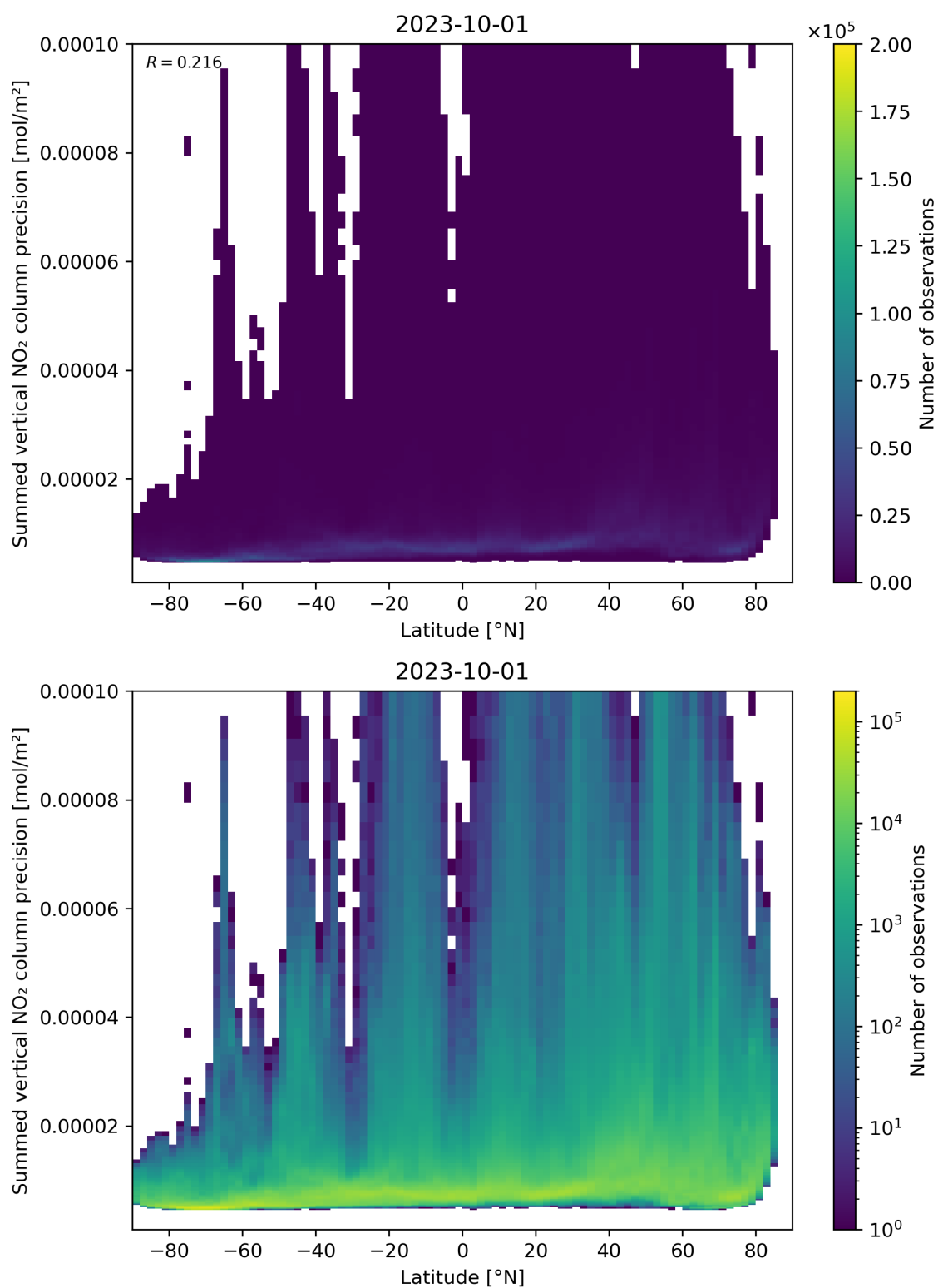
Figure 89: Scatter density plot of “Latitude” against “Summed vertical NO 2 column precision” for 2023-10-01 to 2023-10-02.
