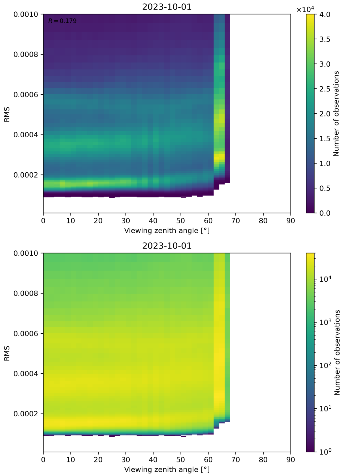
Figure 171: Scatter density plot of “Viewing zenith angle” against “RMS” for 2023-10-01 to 2023-10-02.
