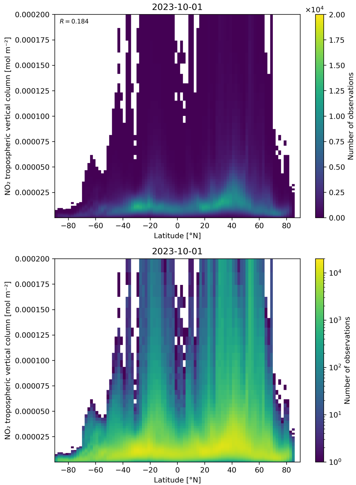
Figure 92: Scatter density plot of “Latitude” against “NO 2 tropospheric vertical column” for 2023-10-01 to 2023-10-02.
