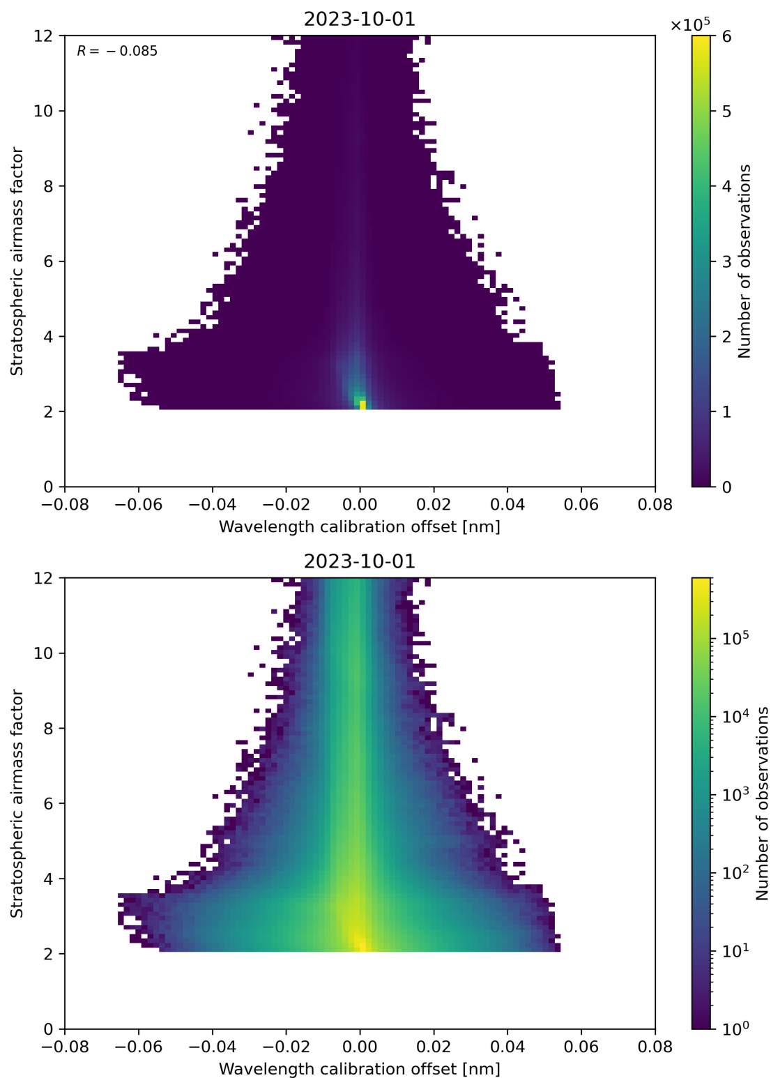
Figure 174: Scatter density plot of “Wavelength calibration offset” against “Stratospheric air mass factor” for 2023-10-01 to 2023-10-02.
