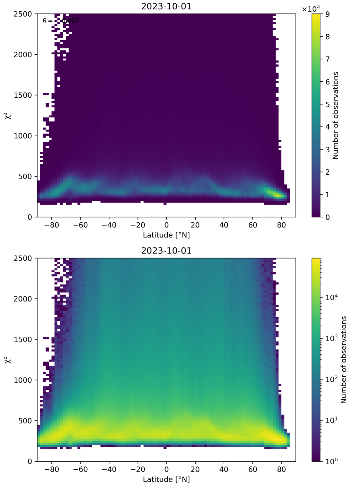
Figure 86: Scatter density plot of “Latitude” against “ \chi^2 ” for 2023-10-01 to 2023-10-02.
