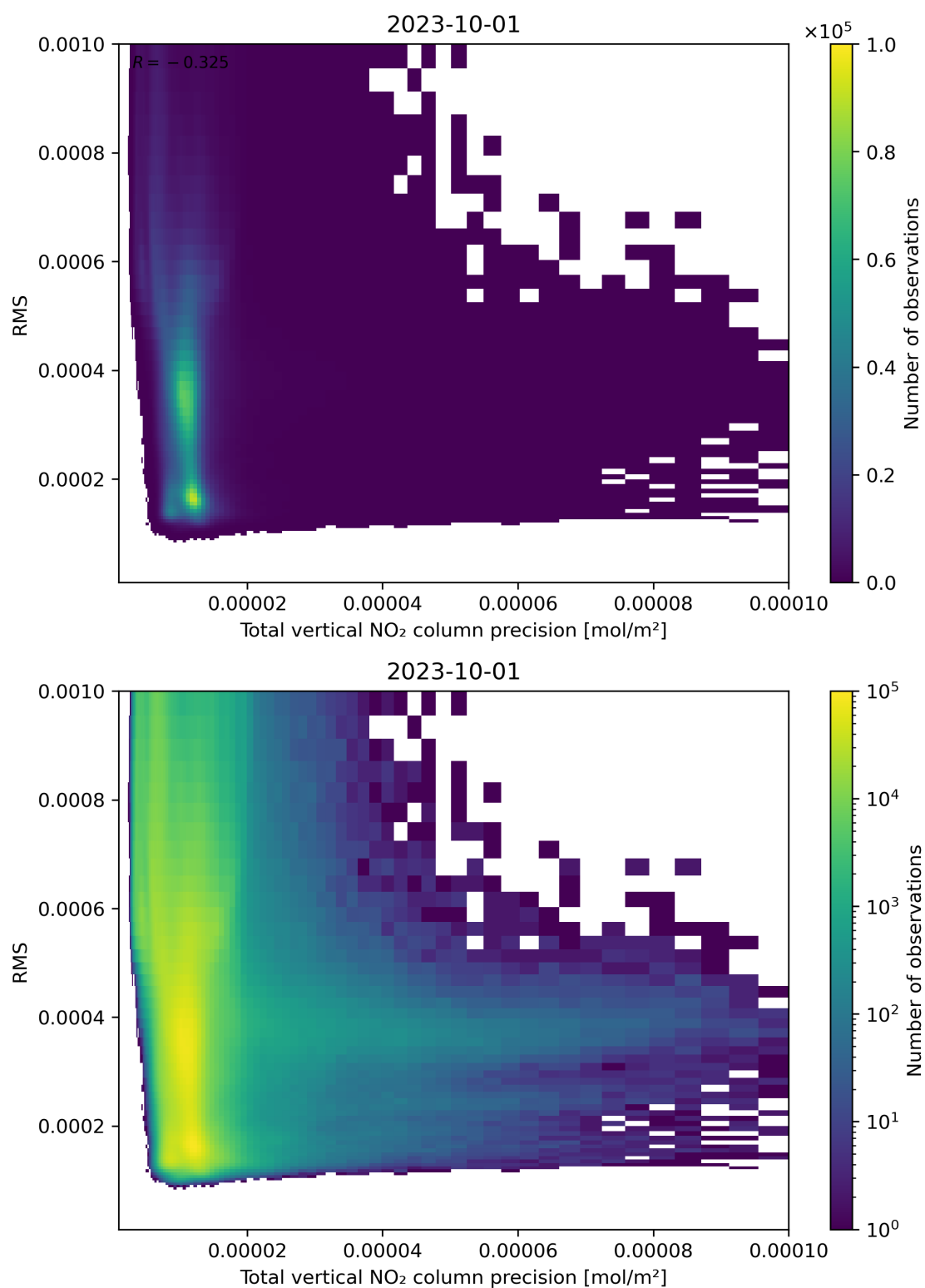
Figure 119: Scatter density plot of “Total vertical NO 2 column precision” against “RMS” for 2023-10-01 to 2023-10-02.
