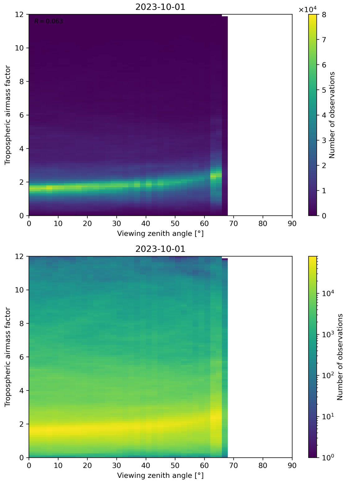
Figure 161: Scatter density plot of “Viewing zenith angle” against “Tropospheric airmass factor” for 2023-10-01 to 2023-10-02.
