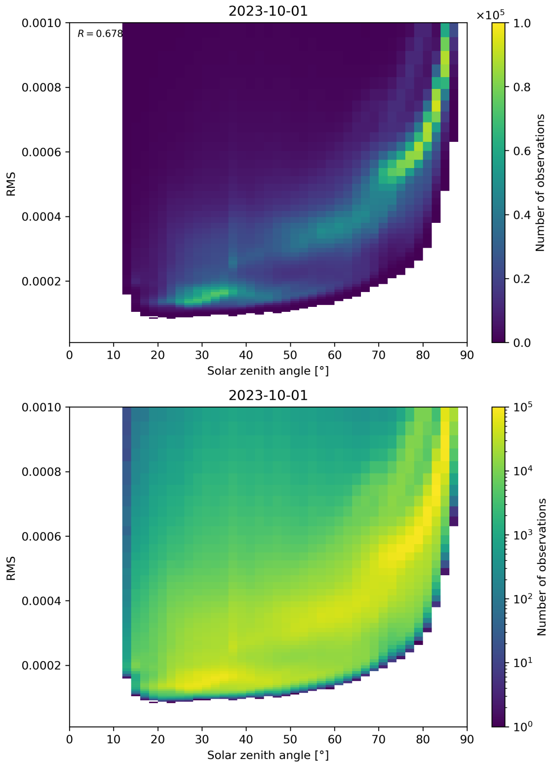
Figure 157: Scatter density plot of “Solar zenith angle” against “RMS” for 2023-10-01 to 2023-10-02.
