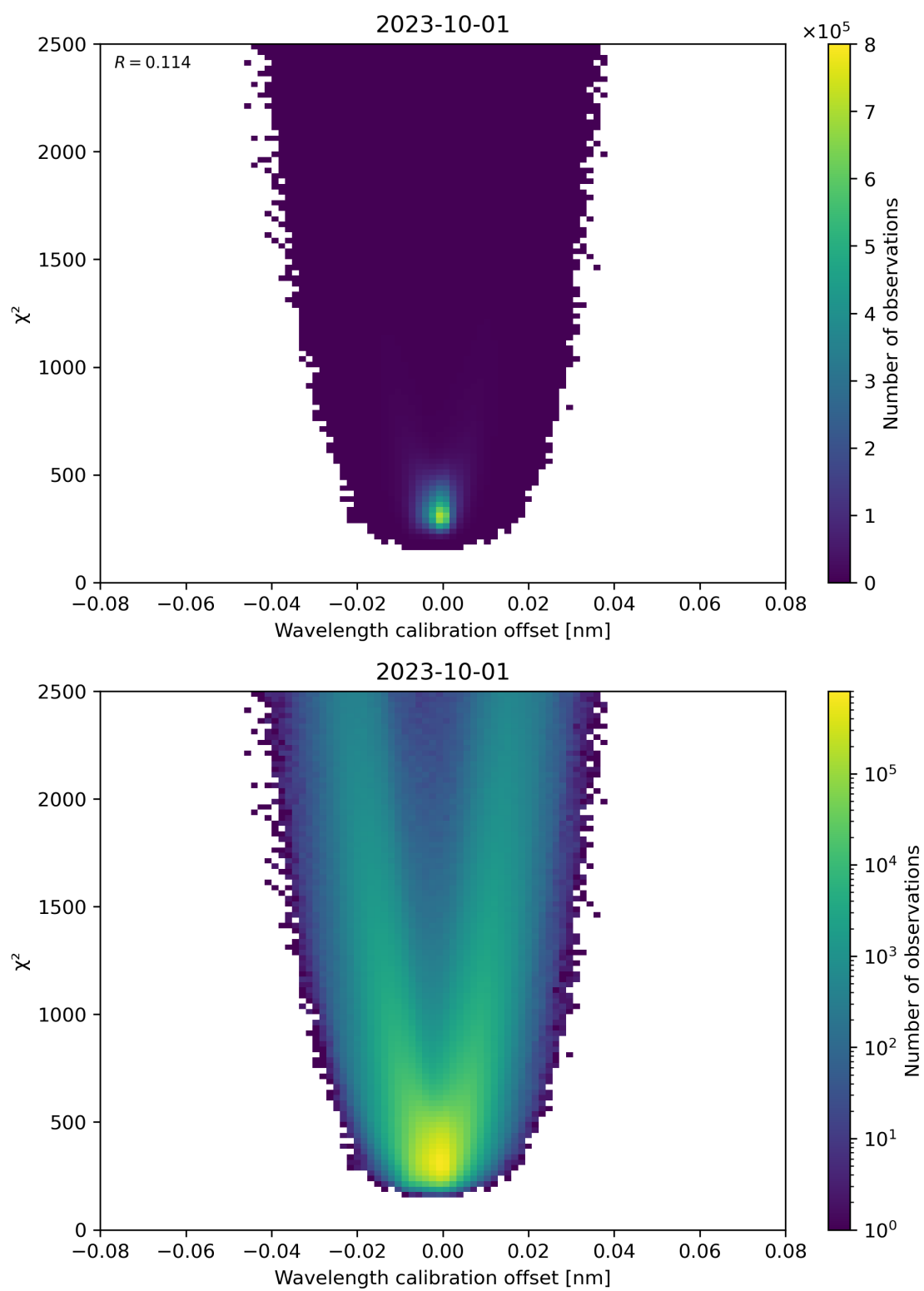
Figure 175: Scatter density plot of “Wavelength calibration offset” against “ \chi^2 ” for 2023-10-01 to 2023-10-02.
