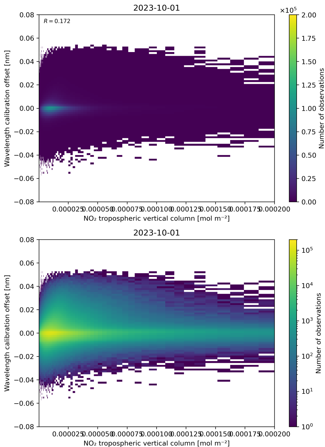
Figure 143: Scatter density plot of “NO 2 tropospheric vertical column” against “Wavelength calibration offset” for 2023-10-01 to 2023-10-02.
