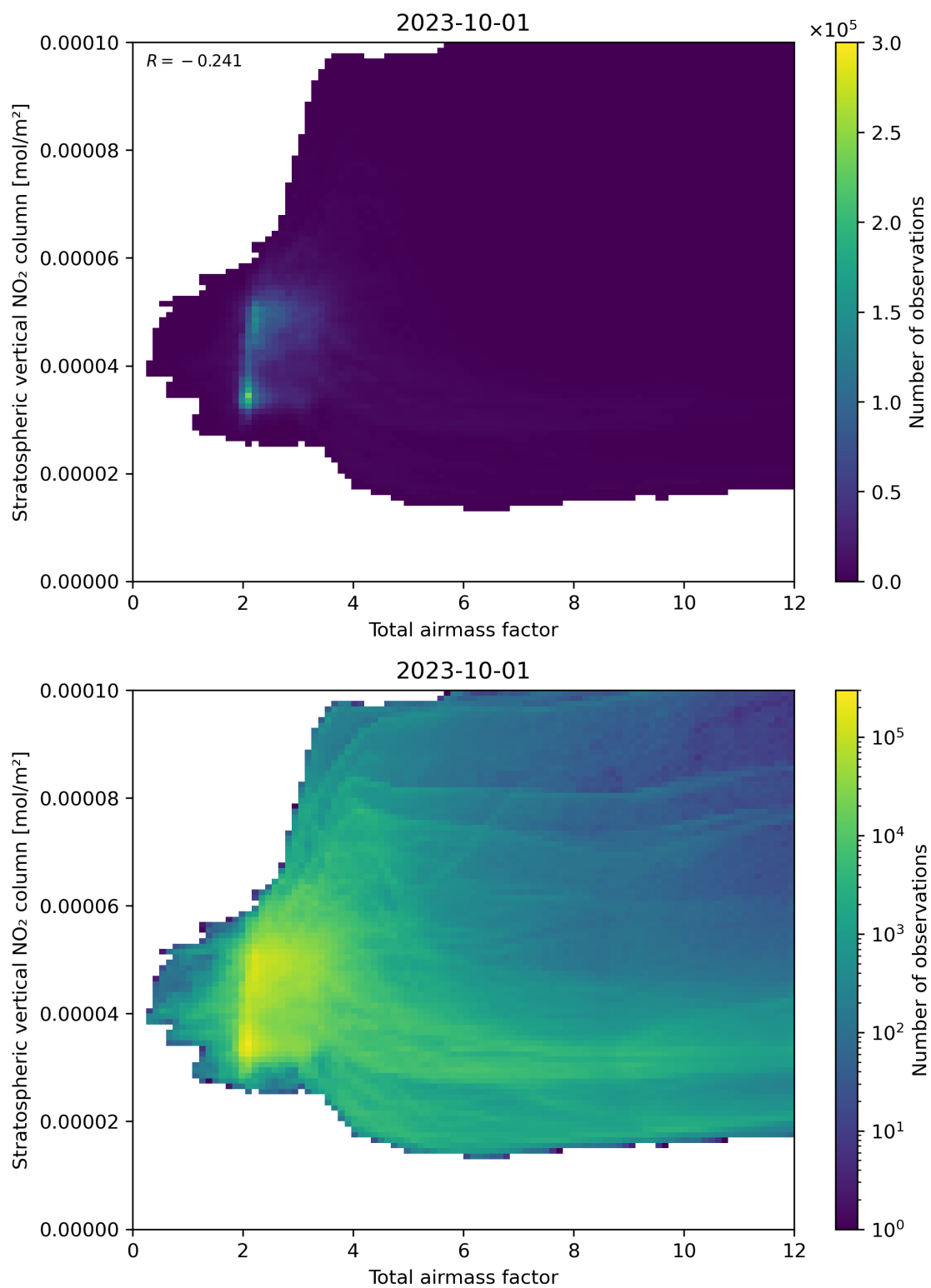
Figure 64: Scatter density plot of “Total airmass factor” against “Stratospheric vertical NO 2 column” for 2023-10-01 to 2023-10-02.
