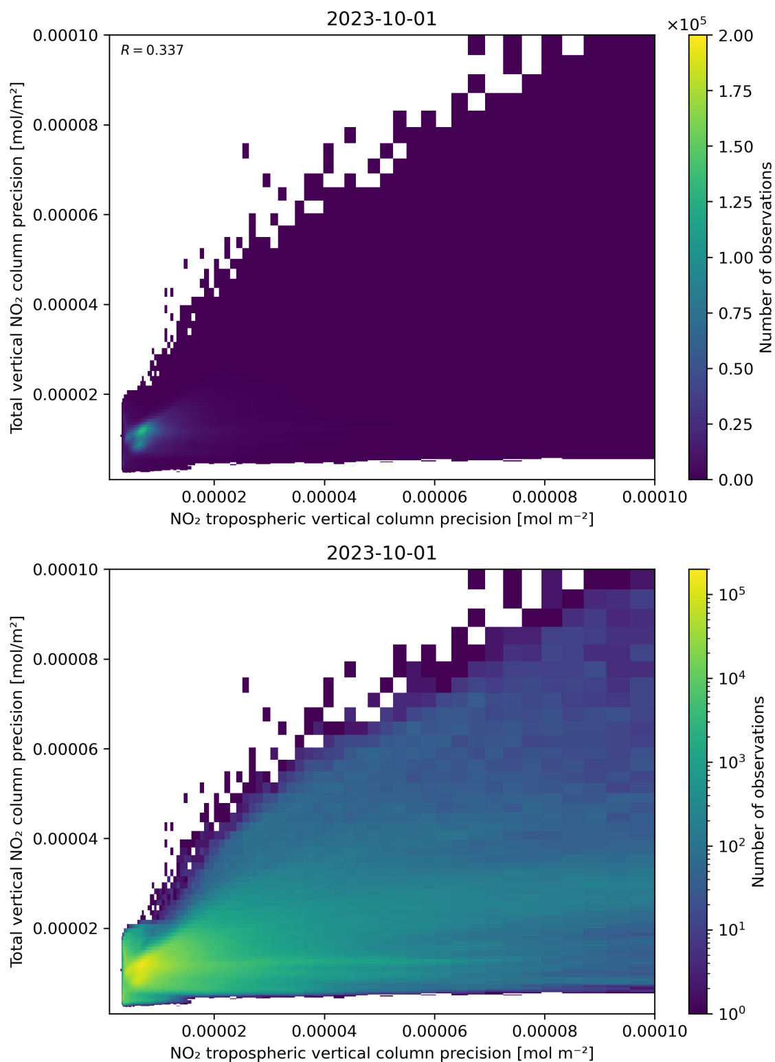
Figure 139: Scatter density plot of “NO 2 tropospheric vertical column precision” against “Total vertical NO 2 column precision” for 2023-10-01 to 2023-10-02.
