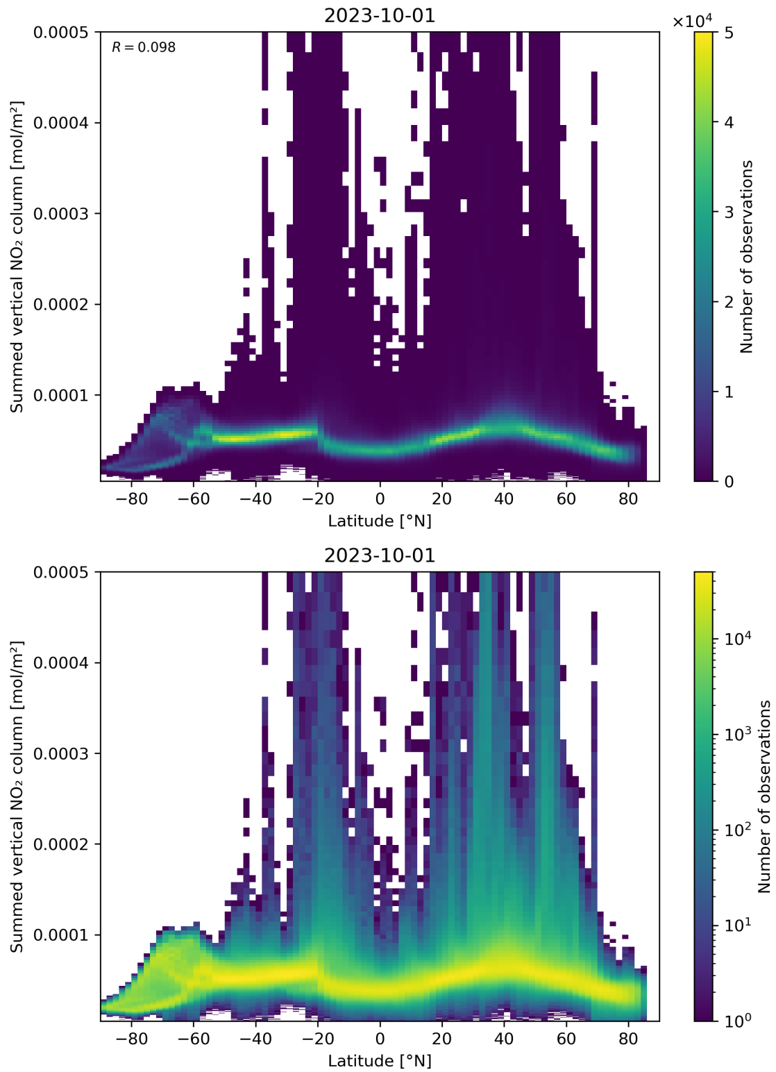
Figure 88: Scatter density plot of “Latitude” against “Summed vertical NO 2 column” for 2023-10-01 to 2023-10-02.
