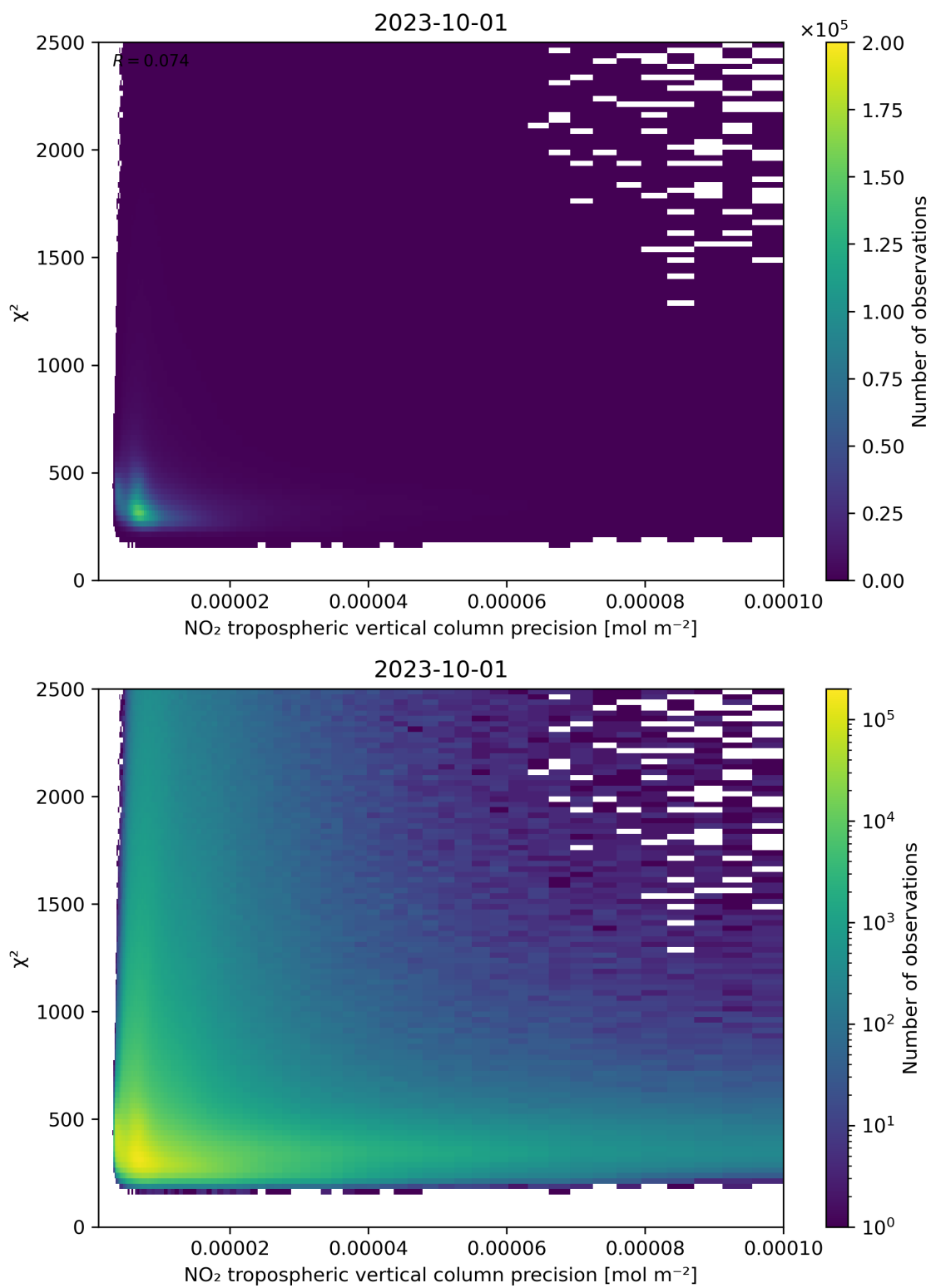
Figure 134: Scatter density plot of “NO 2 tropospheric vertical column precision” against “ \chi^2 ” for 2023-10-01 to 2023-10-02.
