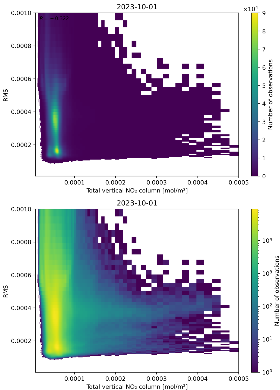
Figure 120: Scatter density plot of “Total vertical NO 2 column” against “RMS” for 2023-10-01 to 2023-10-02.
