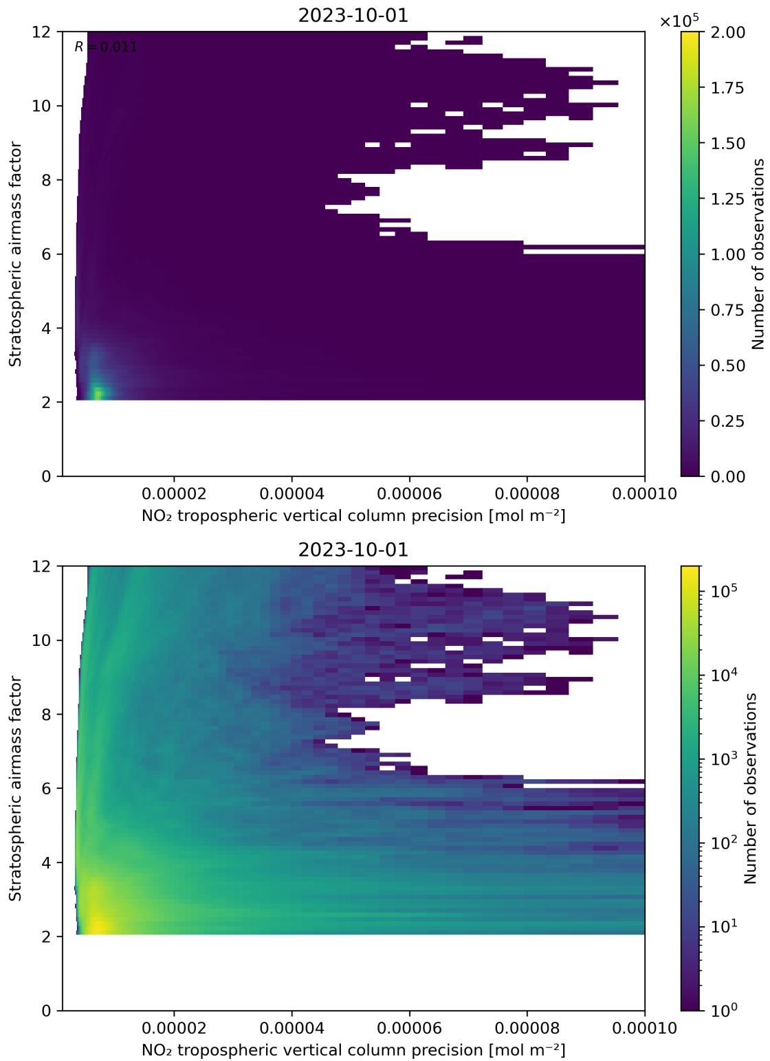
Figure 131: Scatter density plot of “NO 2 tropospheric vertical column precision” against “Stratospheric airmass factor” for 2023-10-01 to 2023-10-02.
