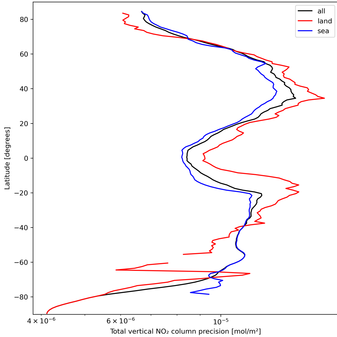
Figure 22: Zonal average of "Total vertical NO 2 column precision" for 2023-10-01 to 2023-10-02.
