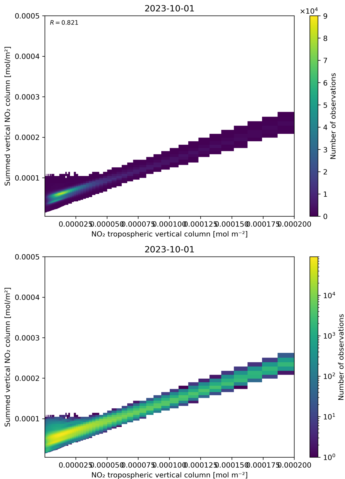
Figure 126: Scatter density plot of “NO 2 tropospheric vertical column” against “Summed vertical NO 2 column” for 2023-10-01 to 2023-10-02.
