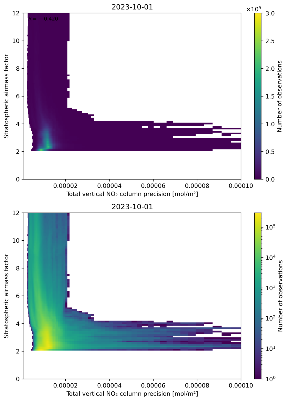
Figure 115: Scatter density plot of “Total vertical NO 2 column precision” against “Stratospheric air mass factor” for 2023-10-01 to 2023-10-02.
