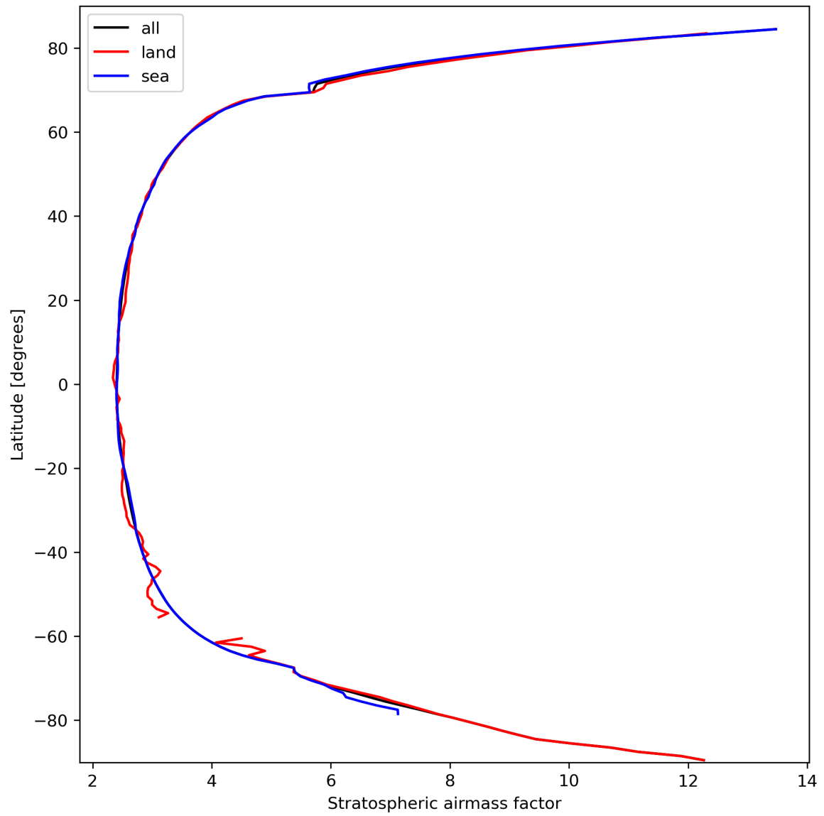
Figure 27: Zonal average of “Stratospheric airmass factor” for 2023-10-01 to 2023-10-02.
