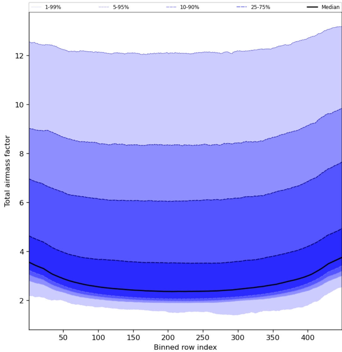
Figure 49: Along track statistics of “Total airmass factor” for 2023-10-01 to 2023-10-02
