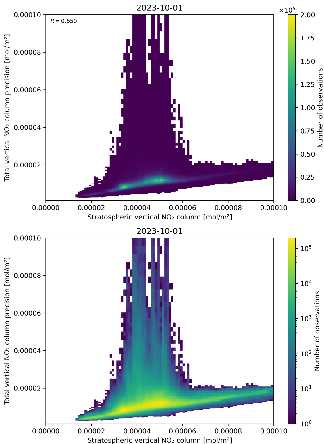
Figure 101: Scatter density plot of “Stratospheric vertical NO 2 column” against “Total vertical NO 2 column precision” for 2023-10-01 to 2023-10-02.
