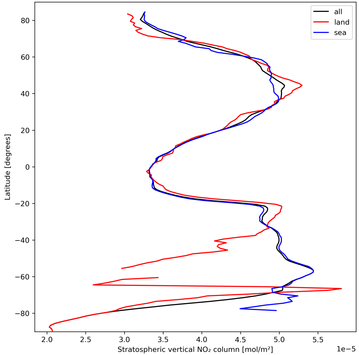
Figure 19: Zonal average of “Stratospheric vertical NO 2 column” for 2023-10-01 to 2023-10-02.
