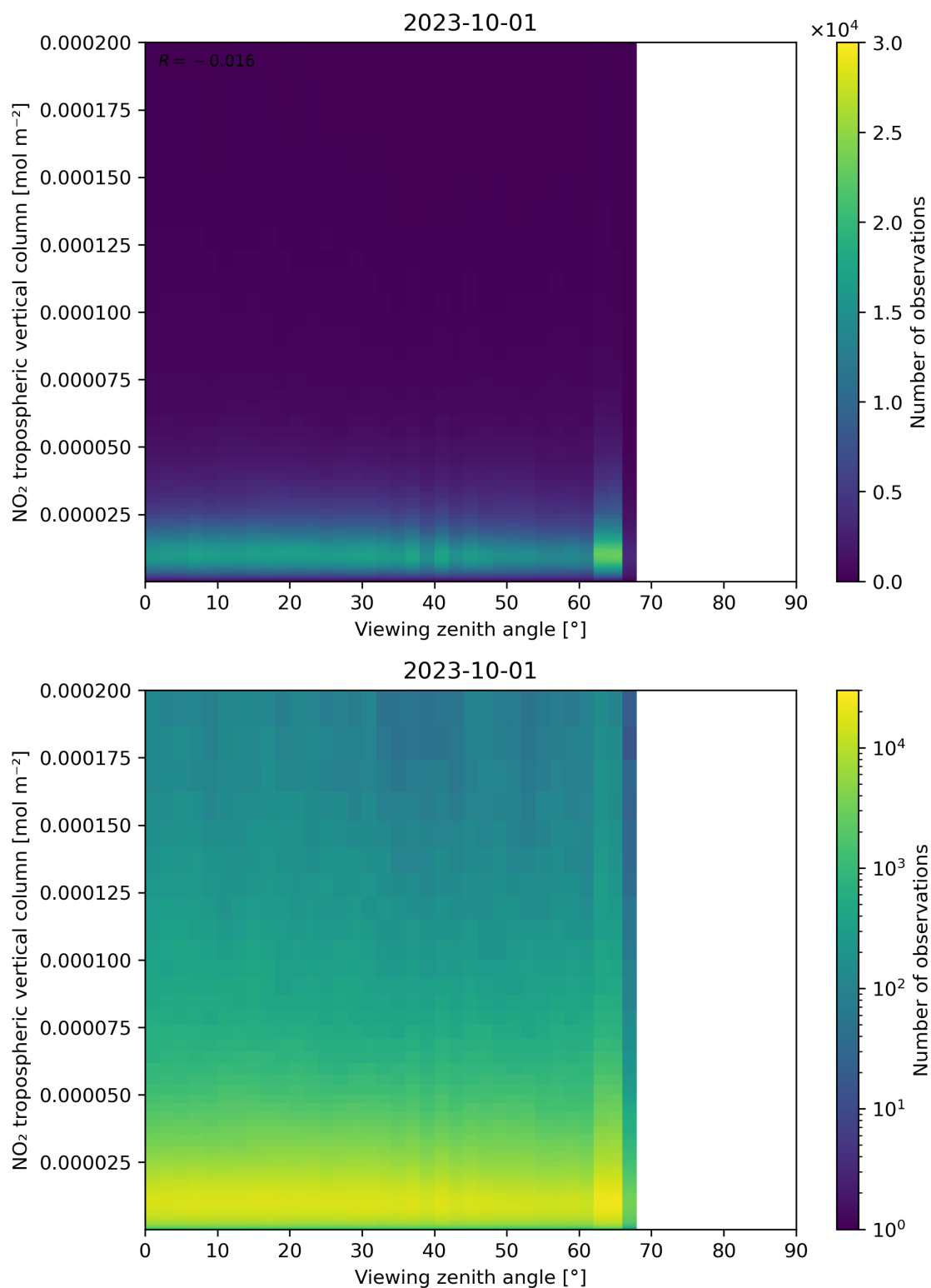
Figure 169: Scatter density plot of “Viewing zenith angle” against “NO 2 tropospheric vertical column” for 2023-10-01 to 2023-10-02.
