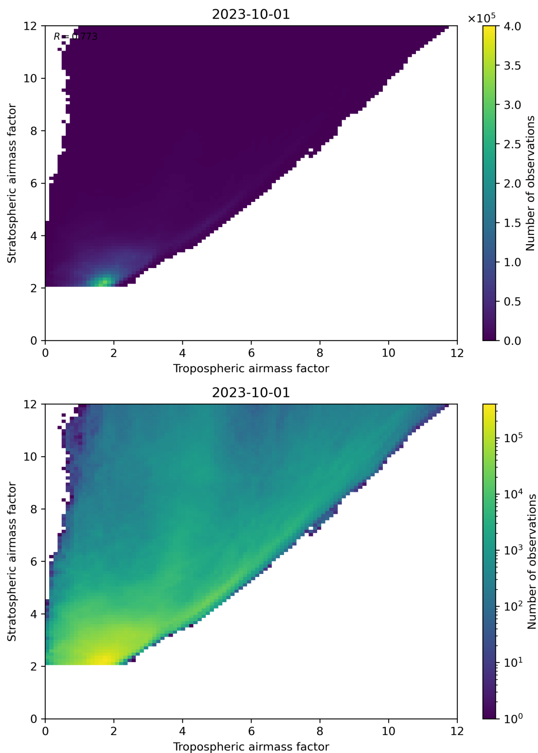
Figure 71: Scatter density plot of “Tropospheric airmass factor” against “Stratospheric airmass factor” for 2023-10-01 to 2023-10-02.
