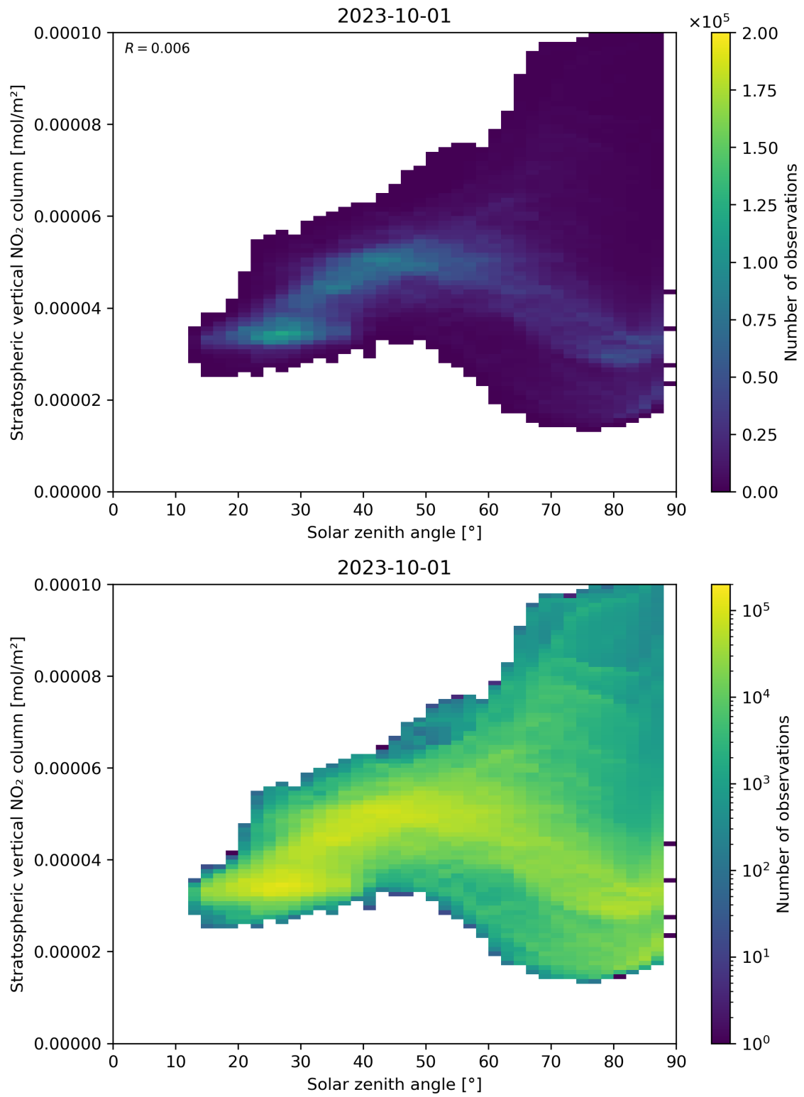
Figure 150: Scatter density plot of “Solar zenith angle” against “Stratospheric vertical NO 2 column” for 2023-10-01 to 2023-10-02.
