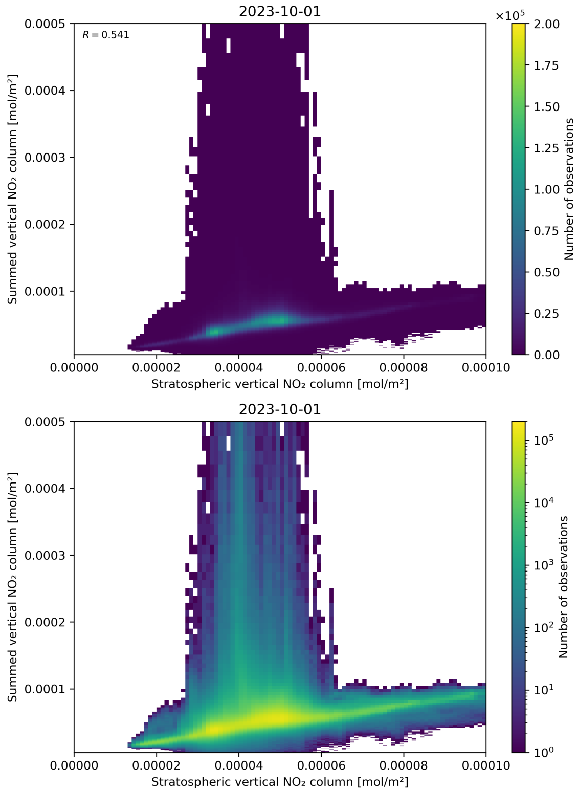
Figure 98: Scatter density plot of “Stratospheric vertical NO 2 column” against “Summed vertical NO 2 column” for 2023-10-01 to 2023-10-02.
