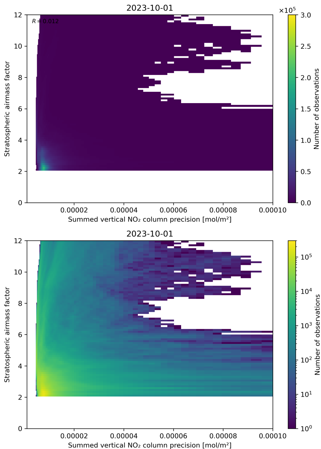
Figure 106: Scatter density plot of “Summed vertical NO 2 column precision” against “Stratospheric airmass factor” for 2023-10-01 to 2023-10-02.
