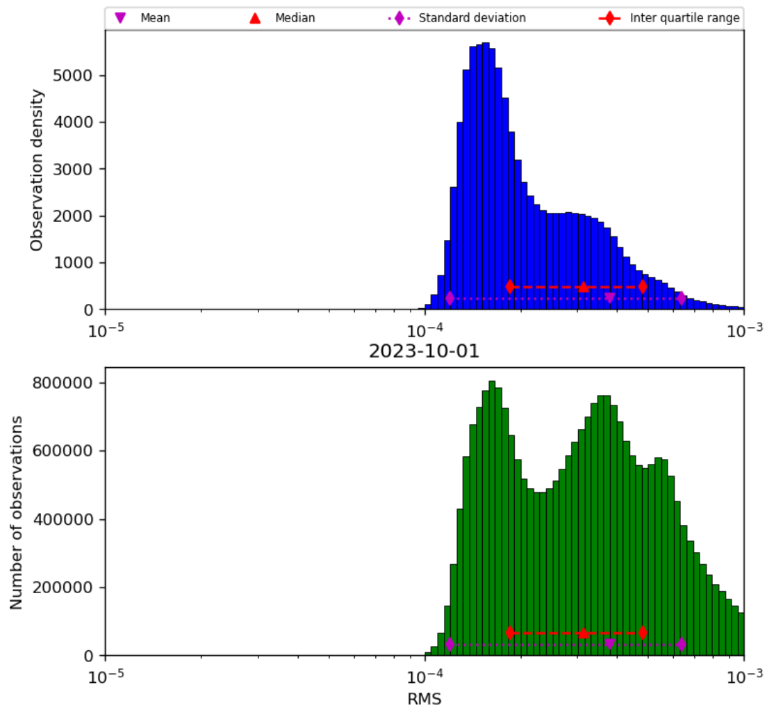
Figure 43: Histogram of “RMS” for 2023-10-01 to 2023-10-02
