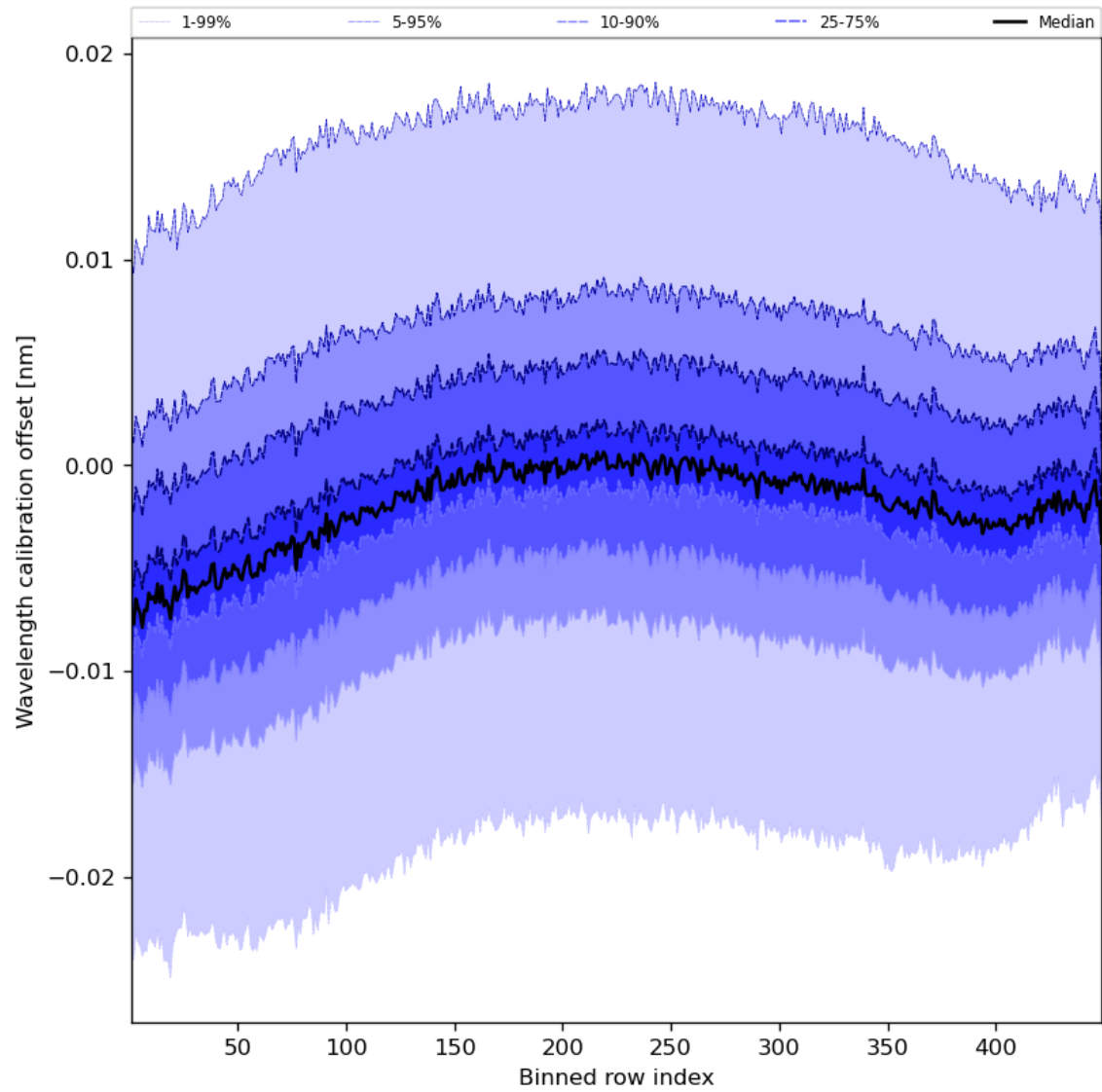
Figure 52: Along track statistics of “Wavelength calibration offset” for 2023-11-20 to 2023-11-22
