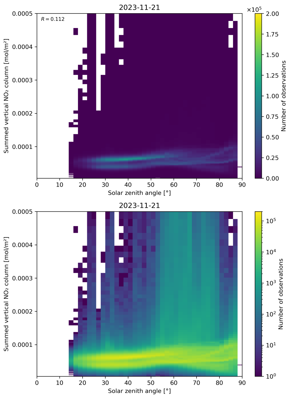
Figure 151: Scatter density plot of “Solar zenith angle” against “Summed vertical NO 2 column” for 2023-11-20 to 2023-11-22.
