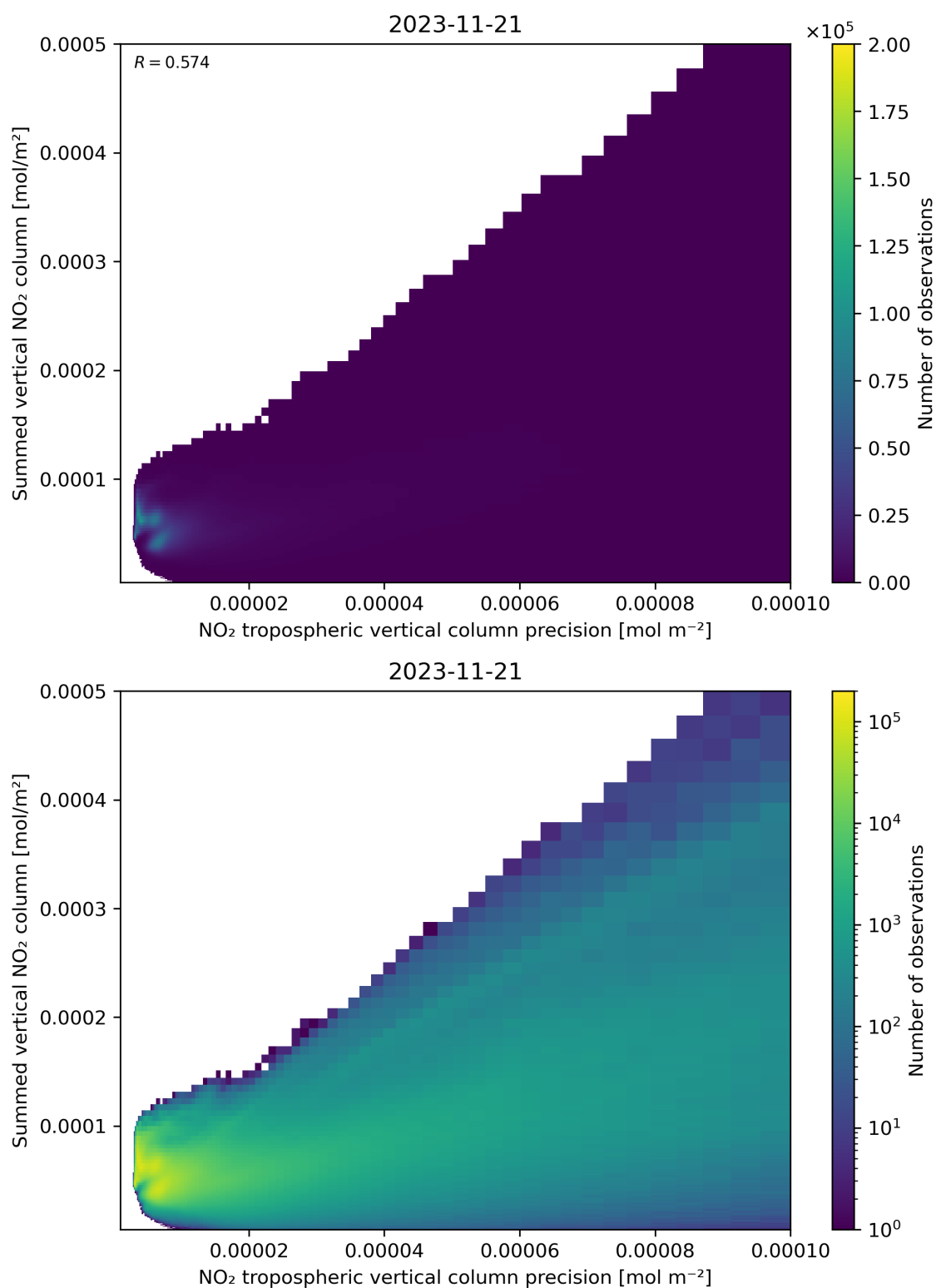
Figure 136: Scatter density plot of “NO 2 tropospheric vertical column precision” against “Summed vertical NO 2 column” for 2023-11-20 to 2023-11-22.
