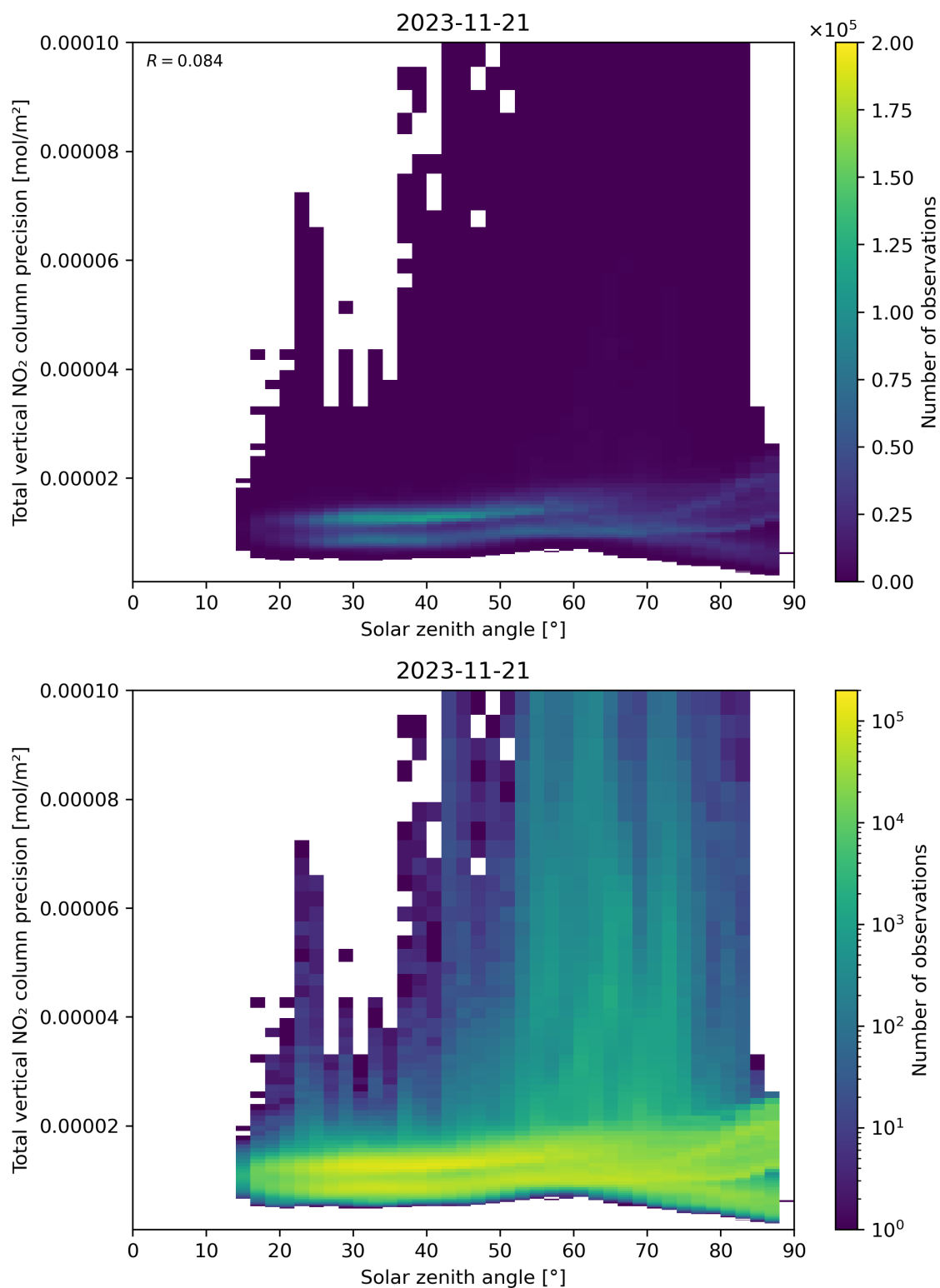
Figure 154: Scatter density plot of “Solar zenith angle” against “Total vertical NO 2 column precision” for 2023-11-20 to 2023-11-22.
