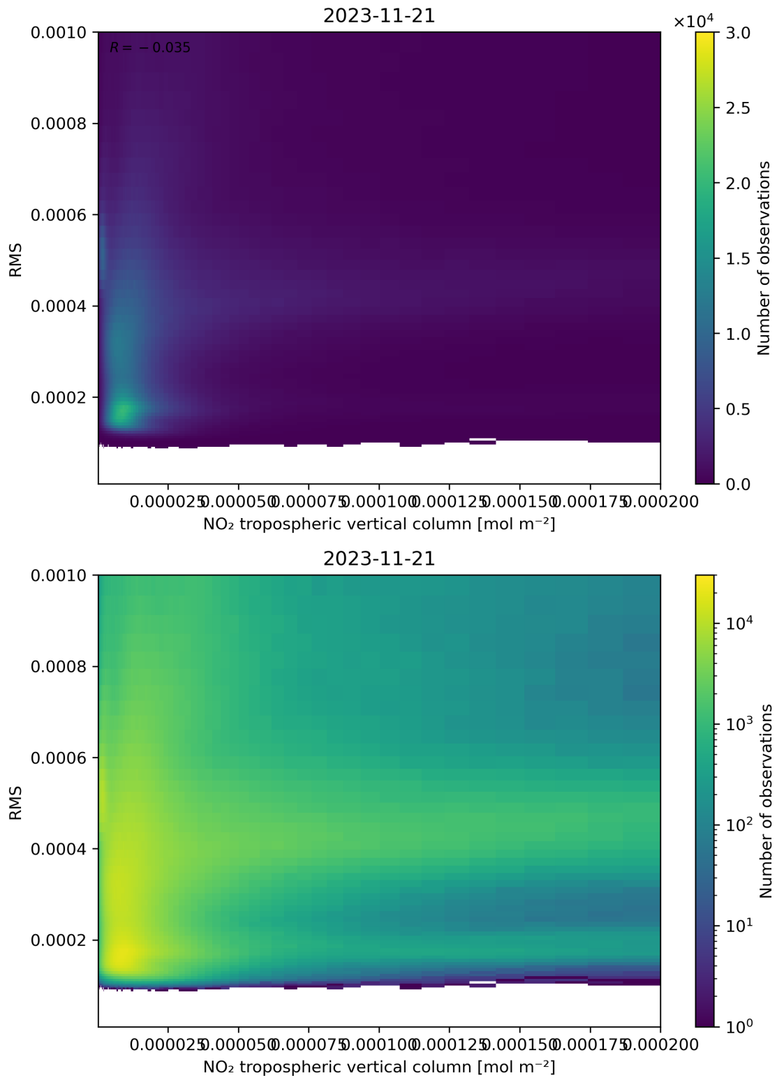
Figure 142: Scatter density plot of “NO 2 tropospheric vertical column” against “RMS” for 2023-11-20 to 2023-11-22.
