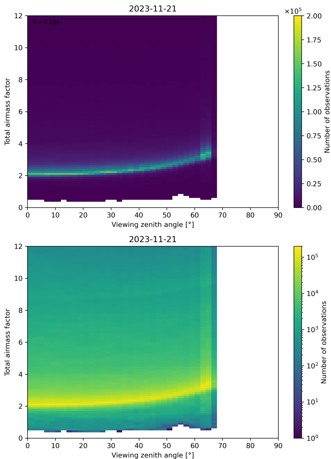
Figure 160: Scatter density plot of “Viewing zenith angle” against “Total airmass factor” for 2023-11-20 to 2023-11-22.
