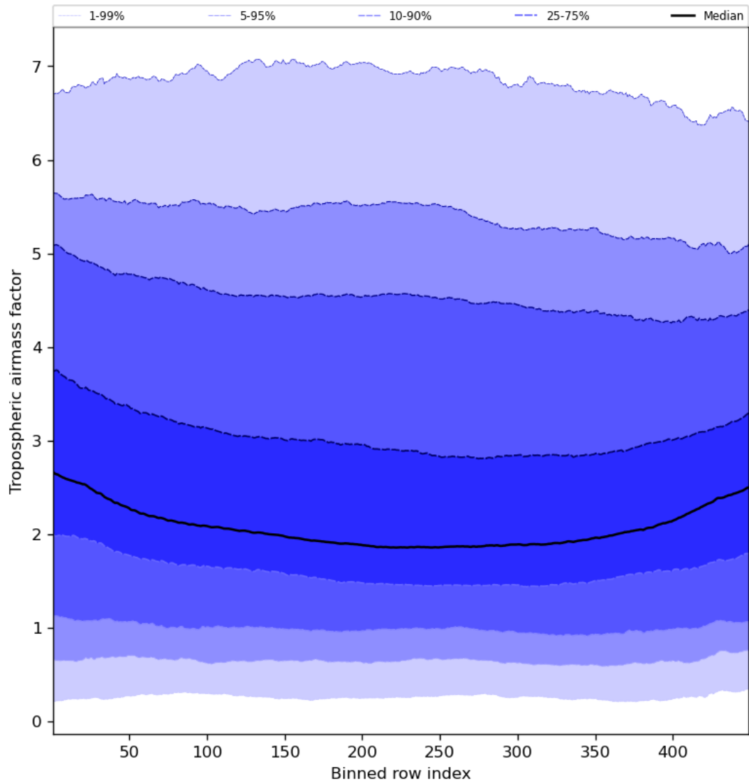
Figure 48: Along track statistics of “Tropospheric air mass factor” for 2023-11-20 to 2023-11-22
