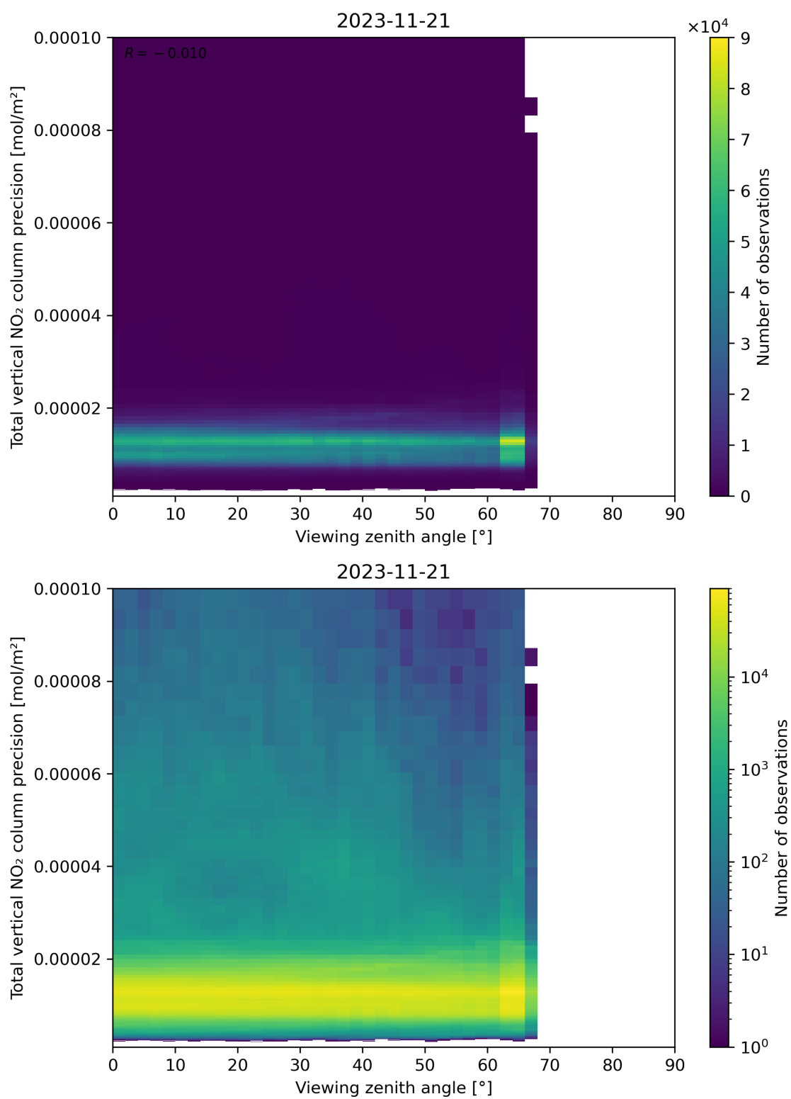
Figure 168: Scatter density plot of “Viewing zenith angle” against “Total vertical NO 2 column precision” for 2023-11-20 to 2023-11-22.
