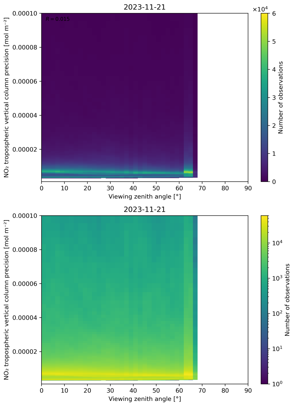
Figure 170: Scatter density plot of “Viewing zenith angle” against “NO 2 tropospheric vertical column precision” for 2023-11-20 to 2023-11-22.
