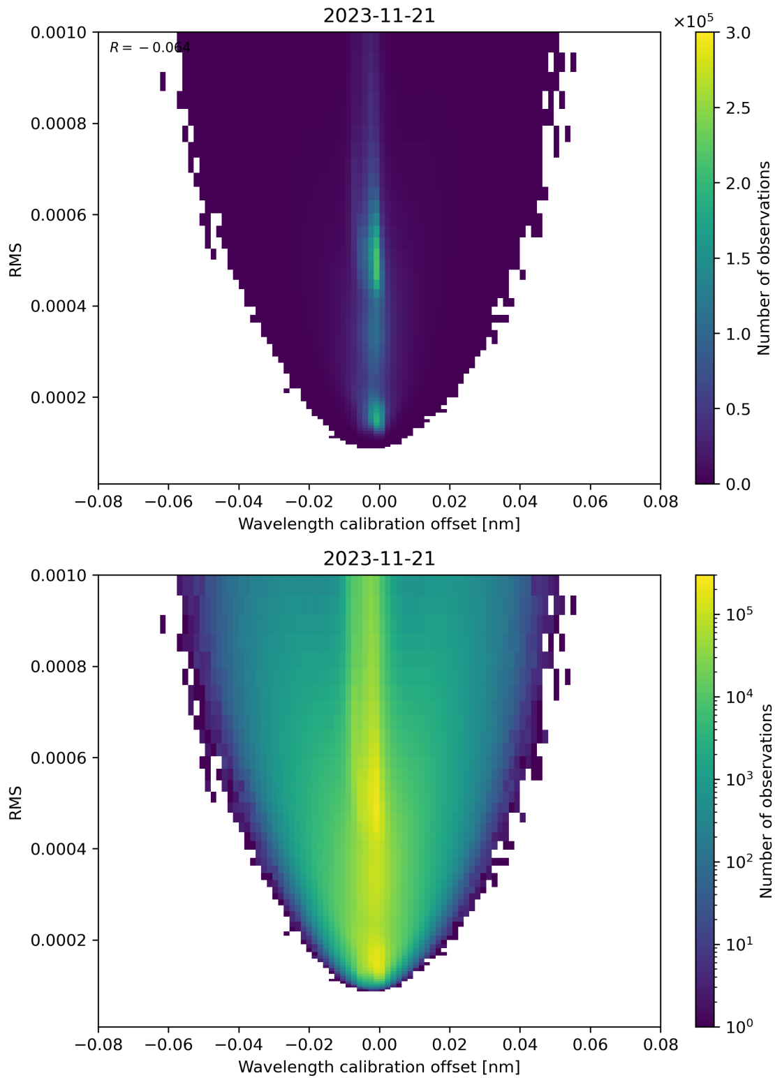
Figure 181: Scatter density plot of “Wavelength calibration offset” against “RMS” for 2023-11-20 to 2023-11-22.
