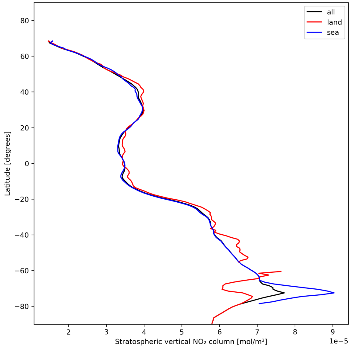
Figure 19: Zonal average of “Stratospheric vertical NO 2 column” for 2023-11-20 to 2023-11-22.
