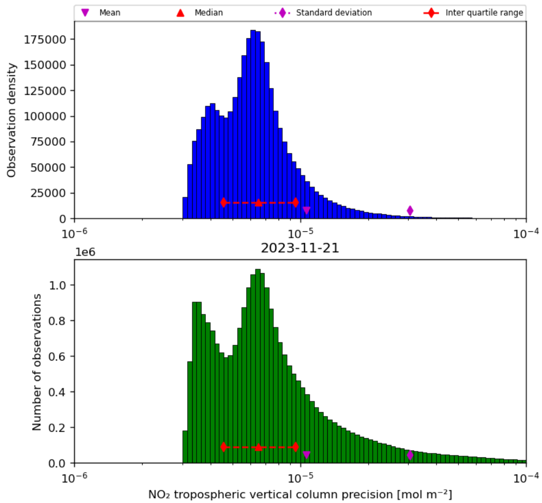
Figure 30: Histogram of “NO 2 tropospheric vertical column precision” for 2023-11-20 to 2023-11-22
