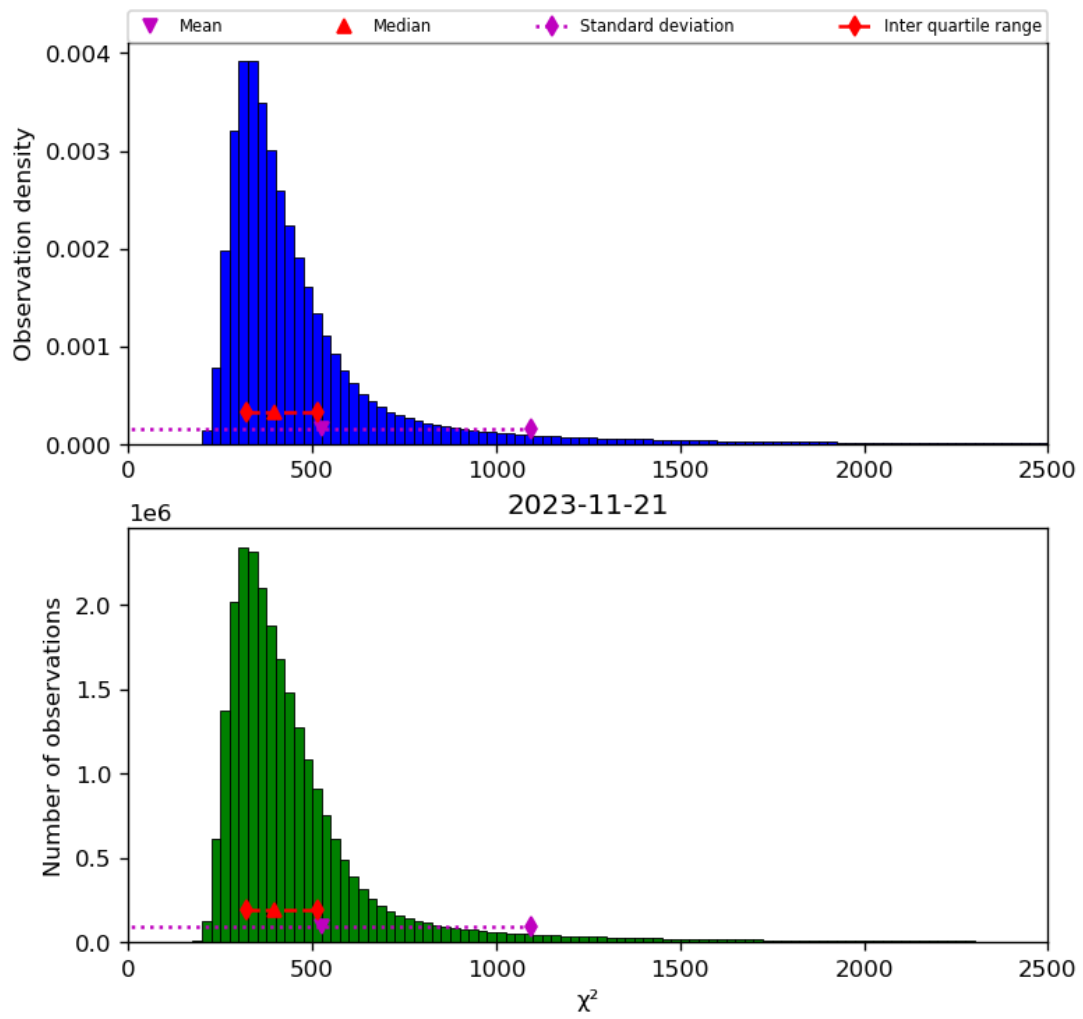
Figure 42: Histogram of “ \chi^2 ” for 2023-11-20 to 2023-11-22
