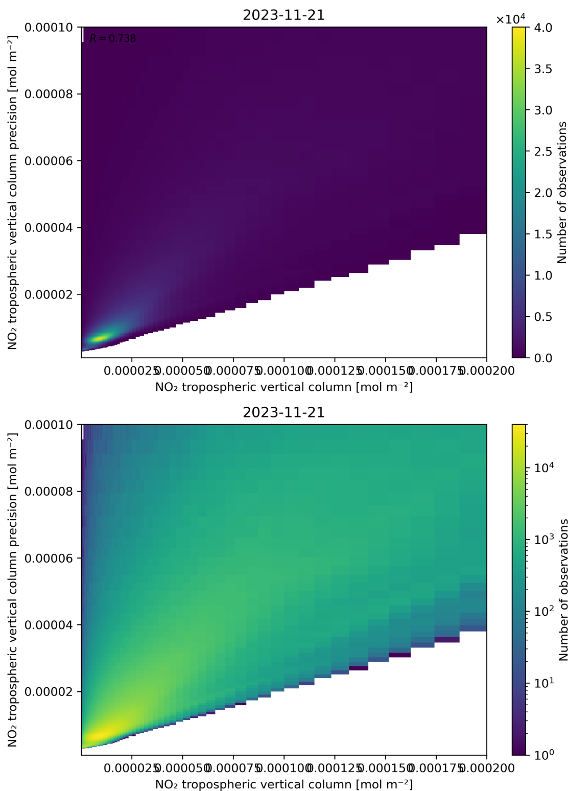
Figure 130: Scatter density plot of “NO 2 tropospheric vertical column” against “NO 2 tropospheric vertical column precision” for 2023-11-20 to 2023-11-22.
