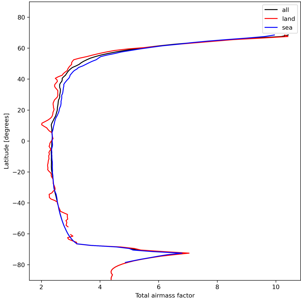
Figure 15: Zonal average of “Total airmass factor” for 2023-11-20 to 2023-11-22.
