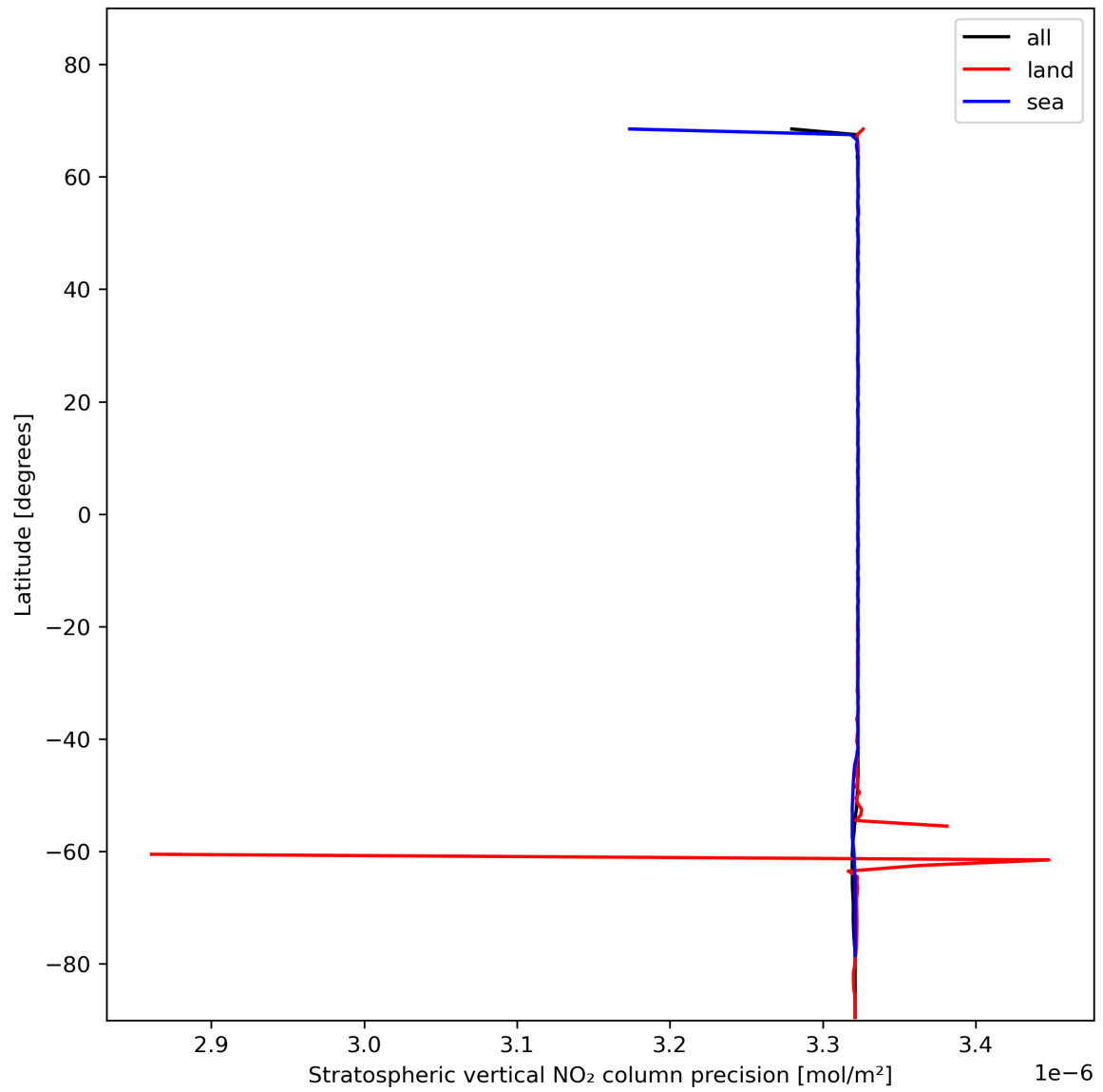
Figure 20: Zonal average of “Stratospheric vertical NO 2 column precision” for 2023-11-20 to 2023-11-22.
