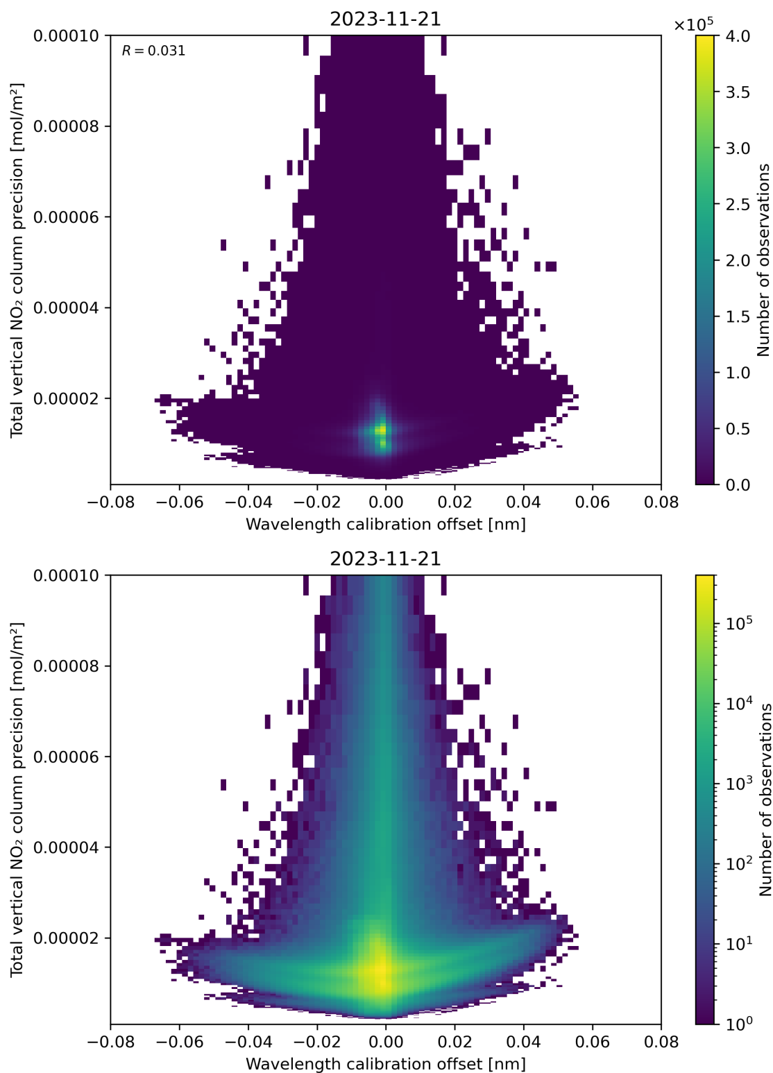
Figure 180: Scatter density plot of “Wavelength calibration offset” against “Total vertical NO 2 column precision” for 2023-11-20 to 2023-11-22.
