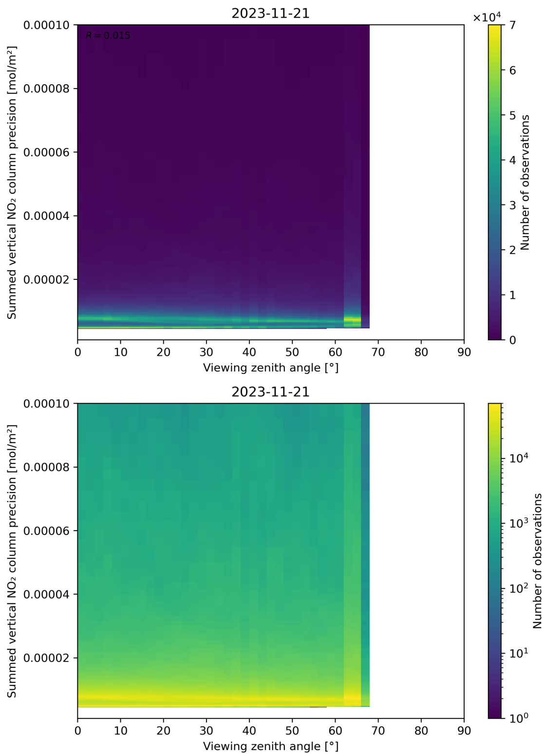
Figure 166: Scatter density plot of “Viewing zenith angle” against “Summed vertical NO 2 column precision” for 2023-11-20 to 2023-11-22.
