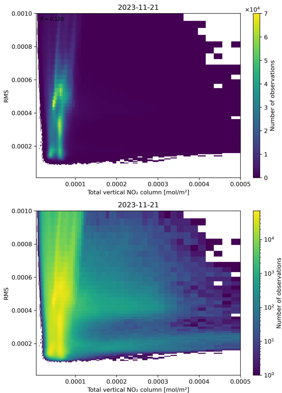
Figure 120: Scatter density plot of “Total vertical NO 2 column” against “RMS” for 2023-11-20 to 2023-11-22.
