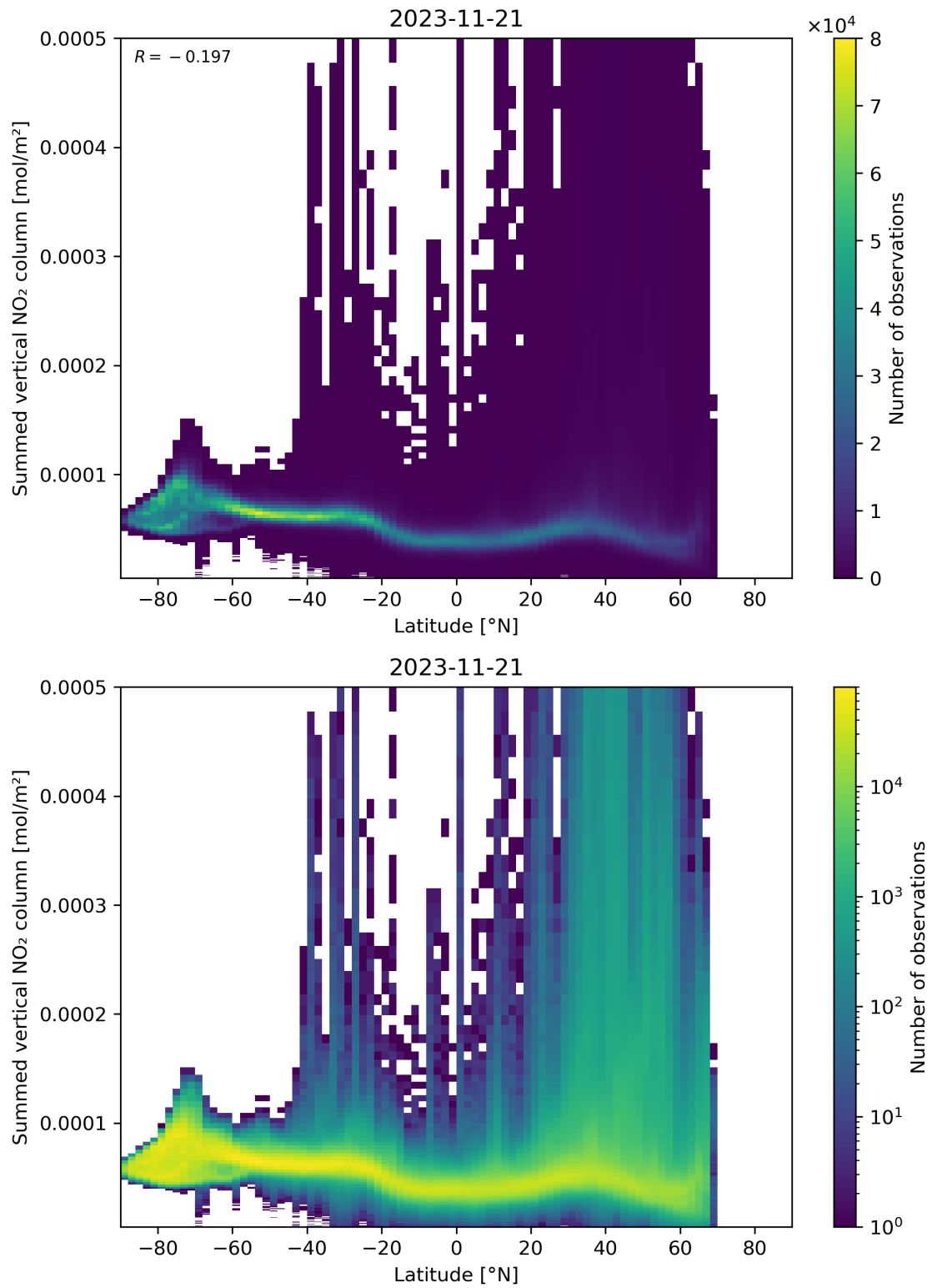
Figure 88: Scatter density plot of “Latitude” against “Summed vertical NO 2 column” for 2023-11-20 to 2023-11-22.
