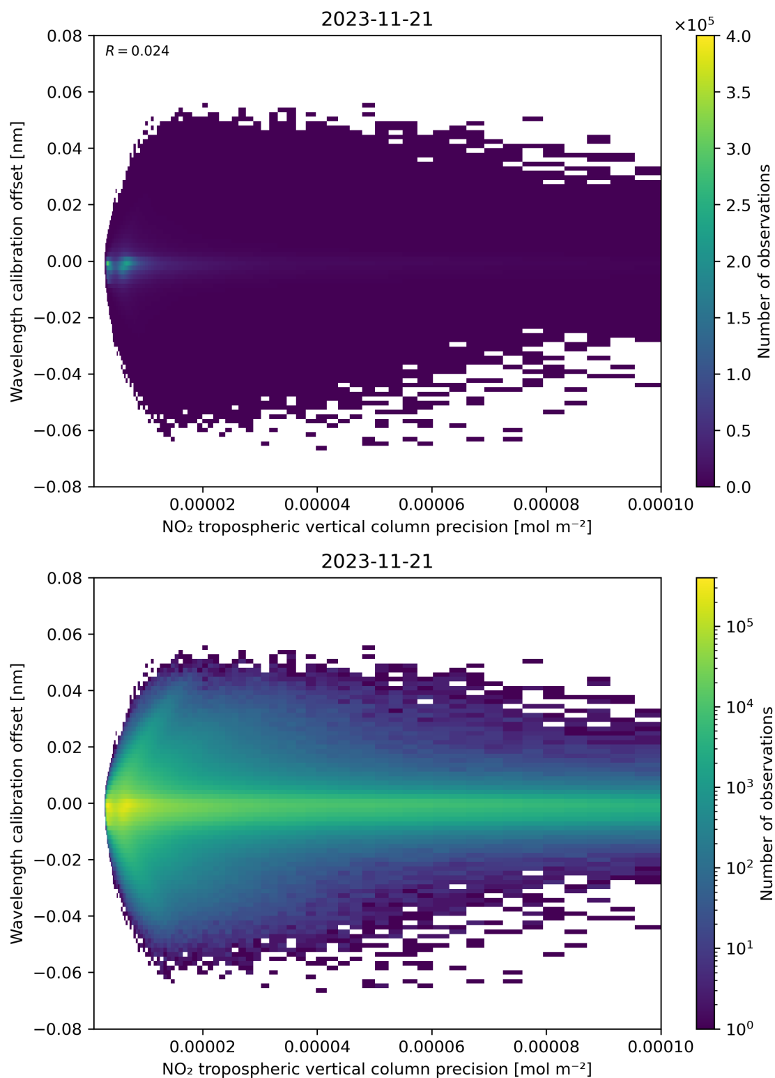
Figure 141: Scatter density plot of “NO 2 tropospheric vertical column precision” against “Wavelength calibration offset” for 2023-11-20 to 2023-11-22.
