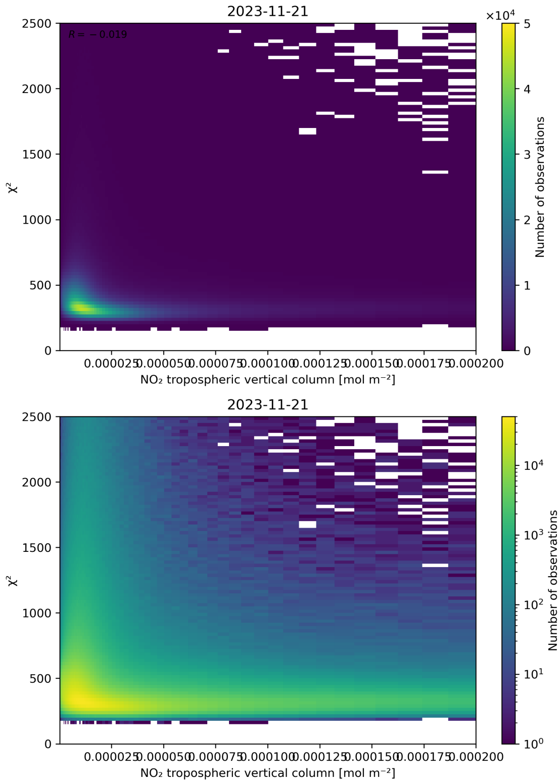
Figure 124: Scatter density plot of “NO 2 tropospheric vertical column” against “ \chi^2 ” for 2023-11-20 to 2023-11-22.
