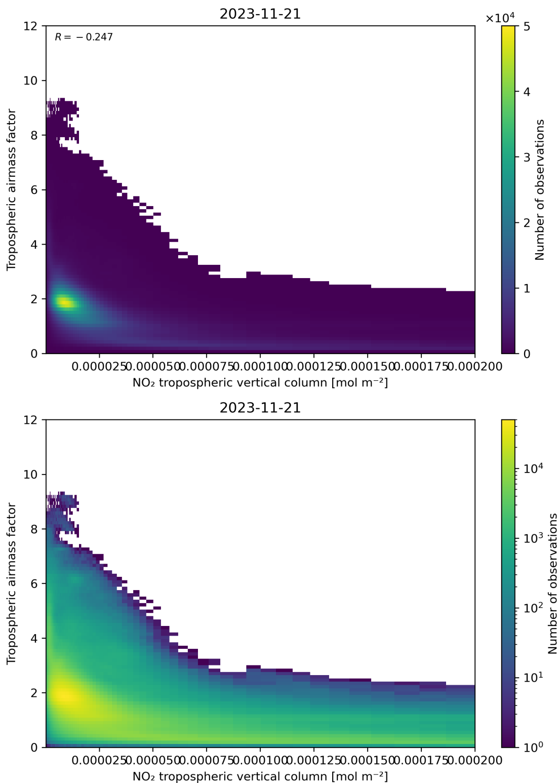
Figure 123: Scatter density plot of “NO 2 tropospheric vertical column” against “Tropospheric air mass factor” for 2023-11-20 to 2023-11-22.
