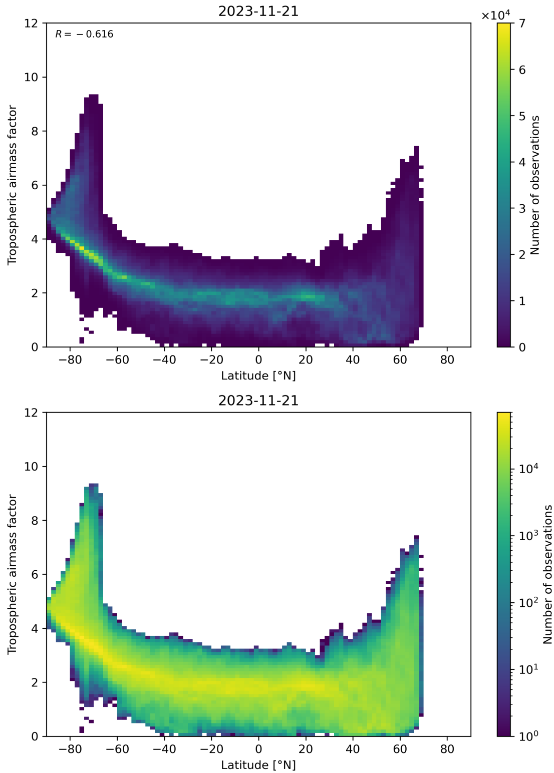
Figure 85: Scatter density plot of “Latitude” against “Tropospheric airmass factor” for 2023-11-20 to 2023-11-22.
