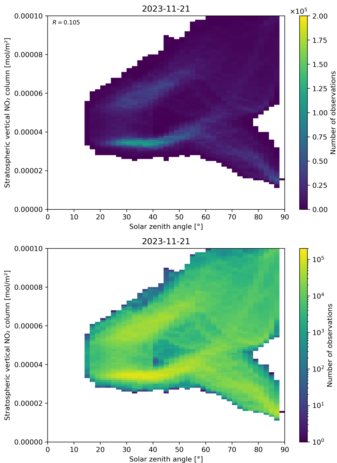
Figure 150: Scatter density plot of “Solar zenith angle” against “Stratospheric vertical NO 2 column” for 2023-11-20 to 2023-11-22.
