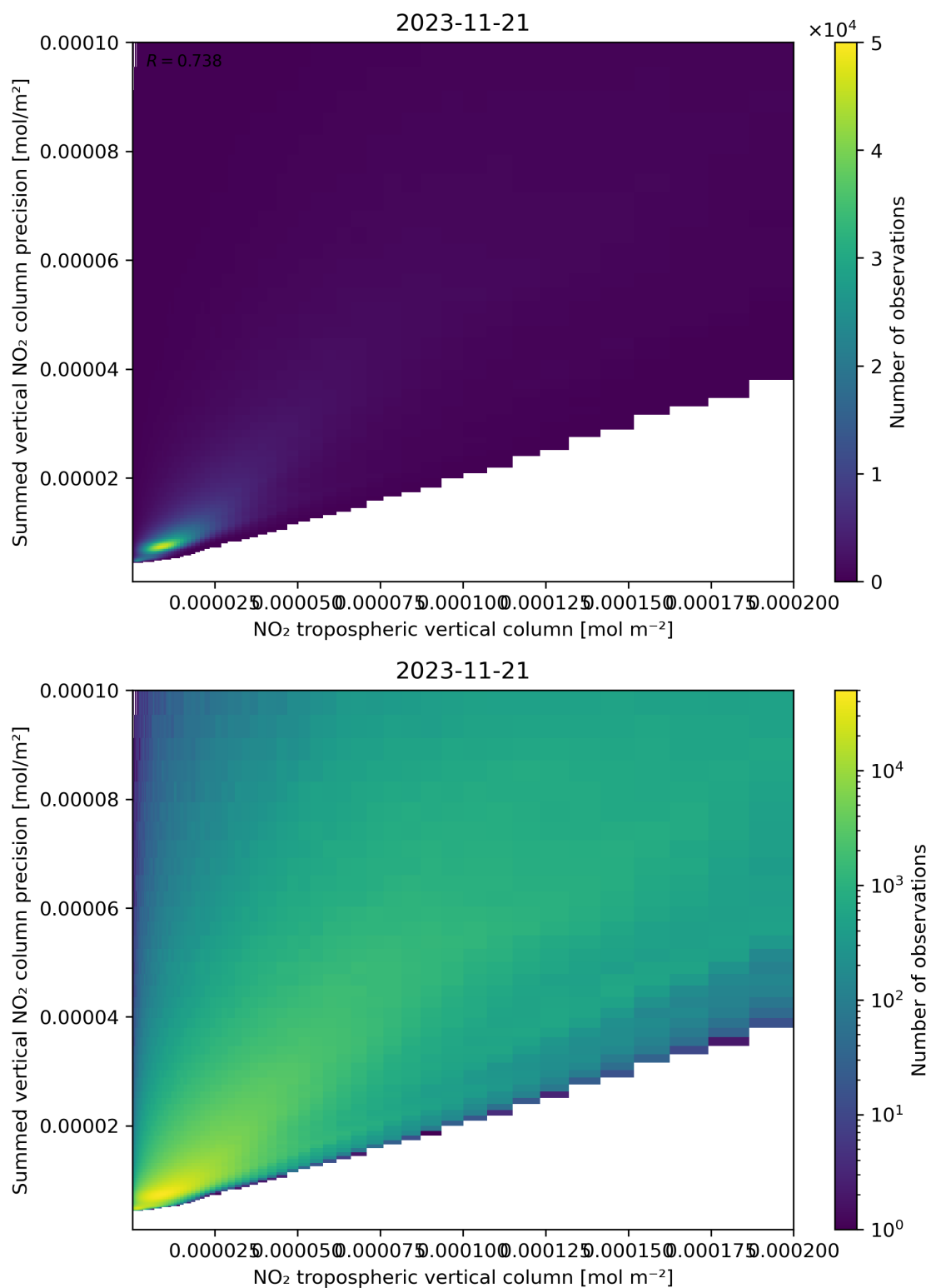
Figure 127: Scatter density plot of “NO 2 tropospheric vertical column” against “Summed vertical NO 2 column precision” for 2023-11-20 to 2023-11-22.
