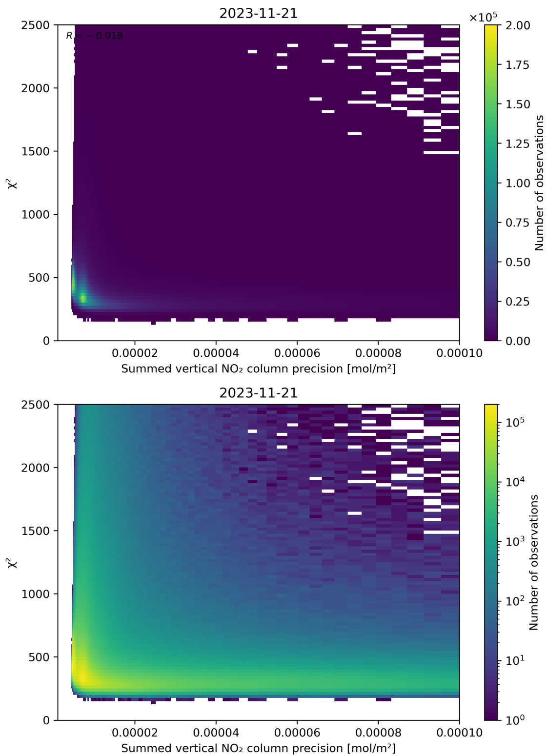
Figure 107: Scatter density plot of “Summed vertical NO 2 column precision” against “ \chi^2 ” for 2023-11-20 to 2023-11-22.
