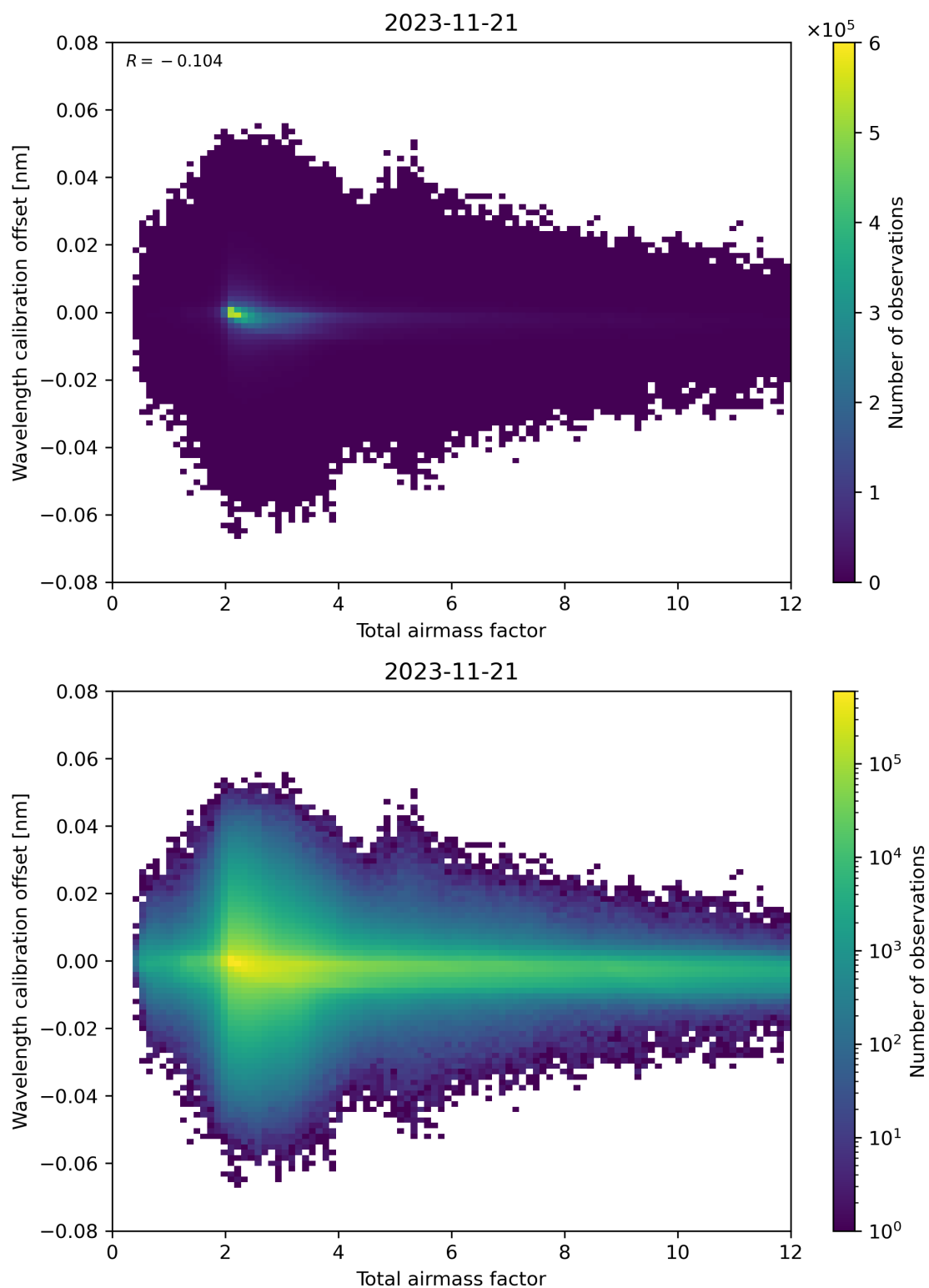
Figure 70: Scatter density plot of “Total airmass factor” against “Wavelength calibration offset” for 2023-11-20 to 2023-11-22.
