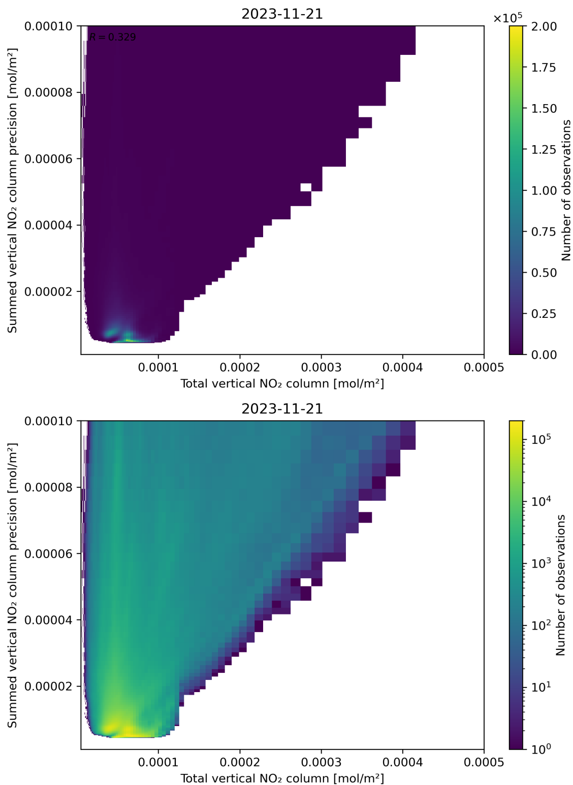
Figure 113: Scatter density plot of “Total vertical NO 2 column” against “Summed vertical NO 2 column precision” for 2023-11-20 to 2023-11-22.
