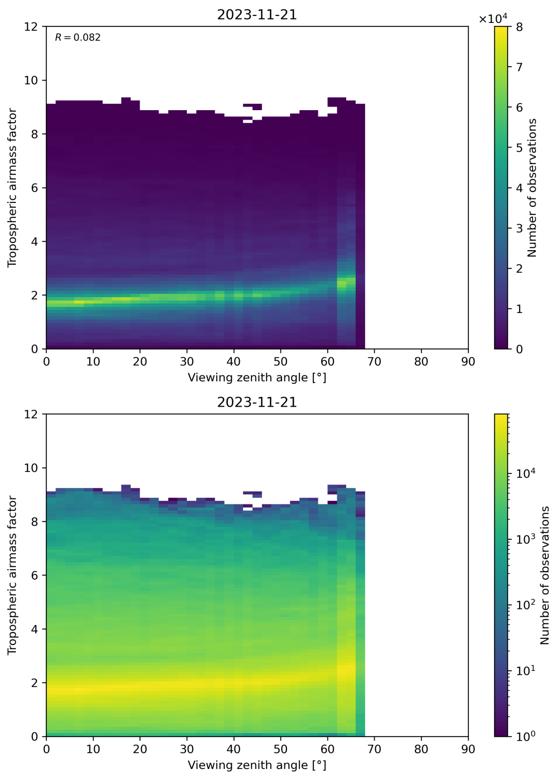
Figure 161: Scatter density plot of “Viewing zenith angle” against “Tropospheric airmass factor” for 2023-11-20 to 2023-11-22.
