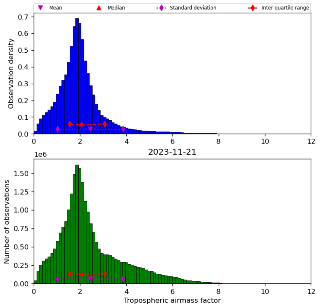
Figure 31: Histogram of “Tropospheric airmass factor” for 2023-11-20 to 2023-11-22
