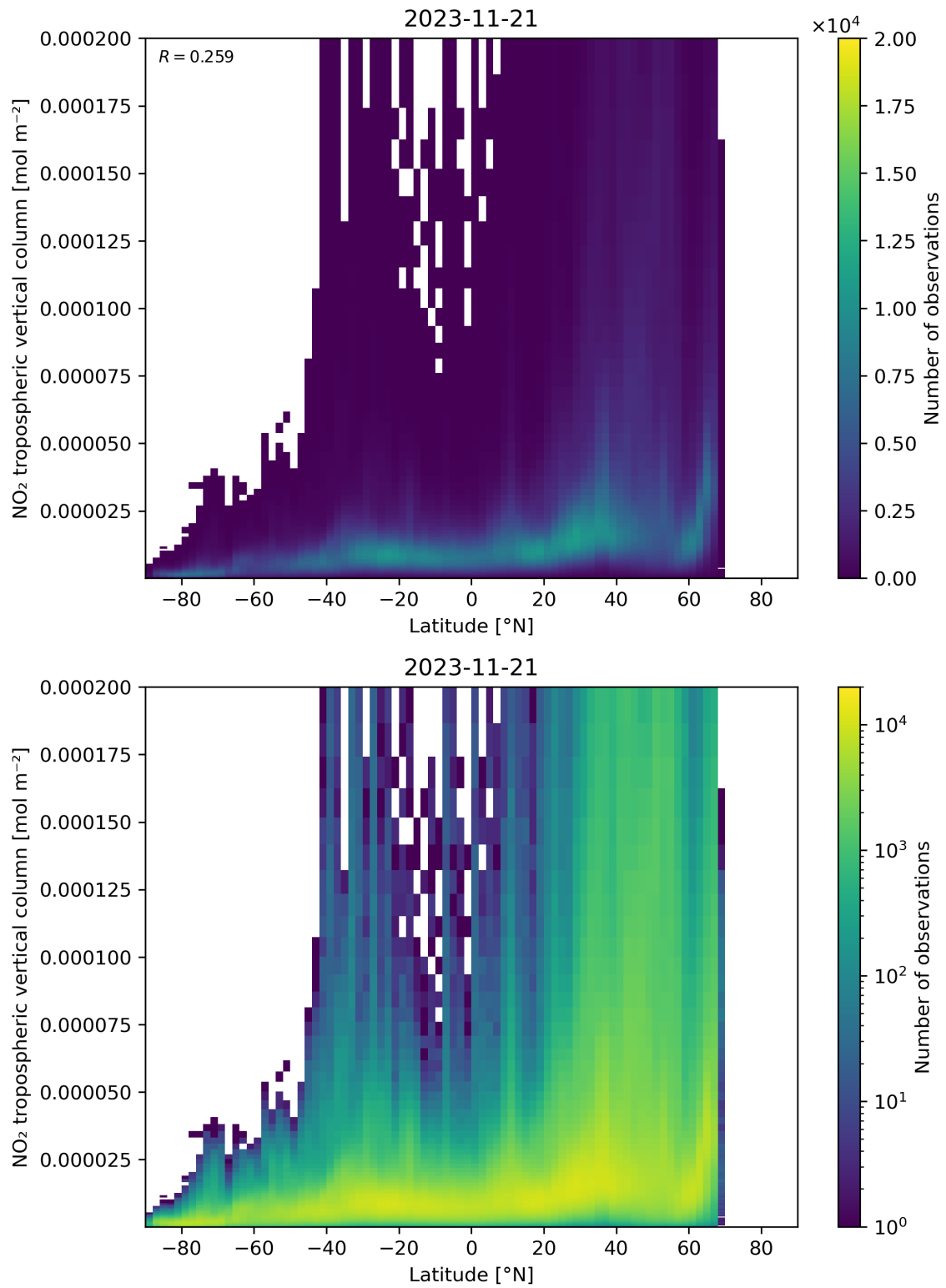
Figure 92: Scatter density plot of “Latitude” against “NO 2 tropospheric vertical column” for 2023-11-20 to 2023-11-22.
