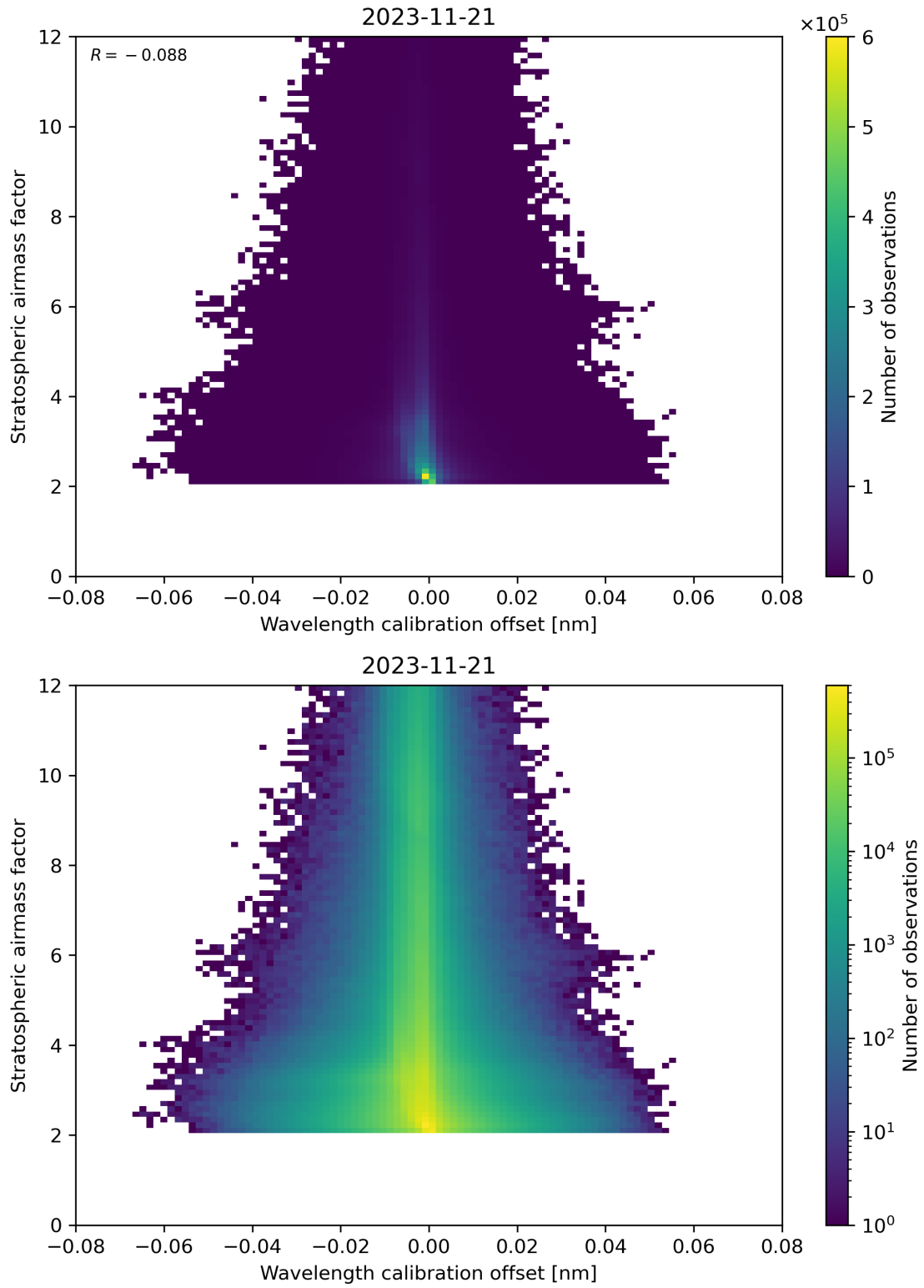
Figure 174: Scatter density plot of “Wavelength calibration offset” against “Stratospheric airmass factor” for 2023-11-20 to 2023-11-22.
