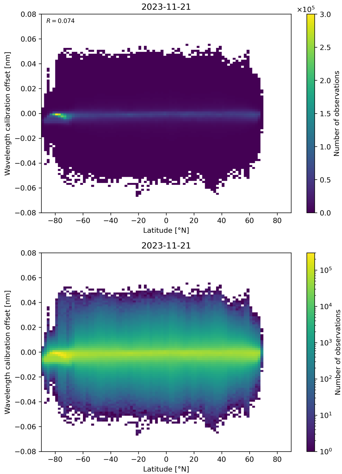
Figure 95: Scatter density plot of “Latitude” against “Wavelength calibration offset” for 2023-11-20 to 2023-11-22.
