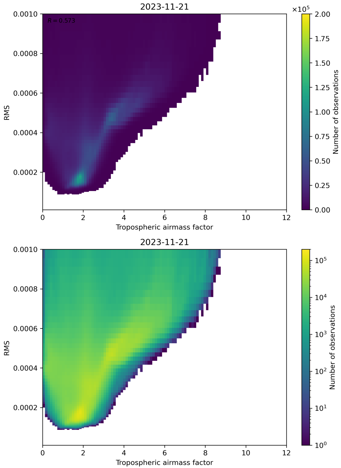
Figure 79: Scatter density plot of “Tropospheric airmass factor” against “RMS” for 2023-11-20 to 2023-11-22.
