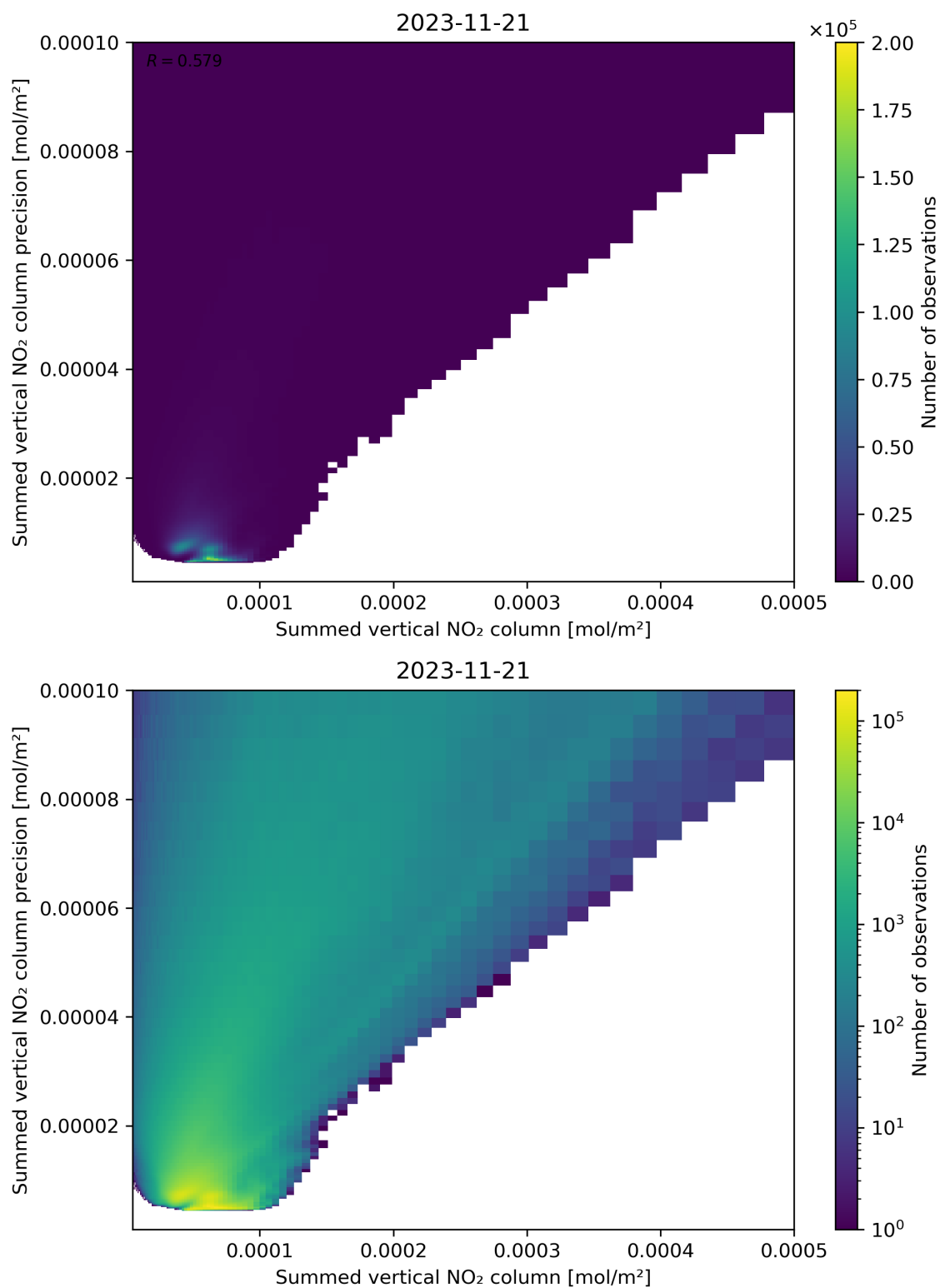
Figure 105: Scatter density plot of “Summed vertical NO 2 column” against “Summed vertical NO 2 column precision” for 2023-11-20 to 2023-11-22.
