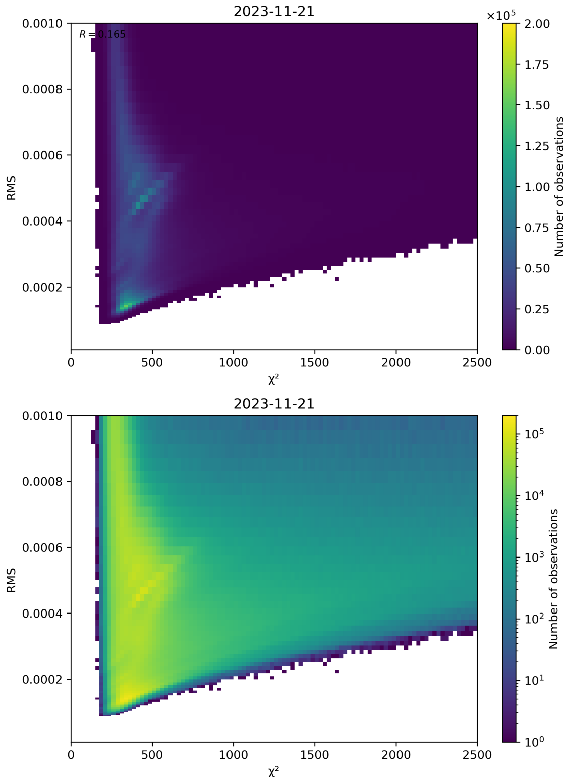
Figure 82: Scatter density plot of “ \chi^2 ” against “RMS” for 2023-11-20 to 2023-11-22.
