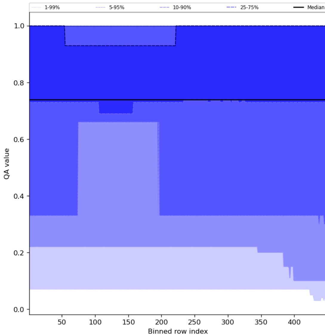
Figure 45: Along track statistics of “QA value” for 2023-11-20 to 2023-11-22
