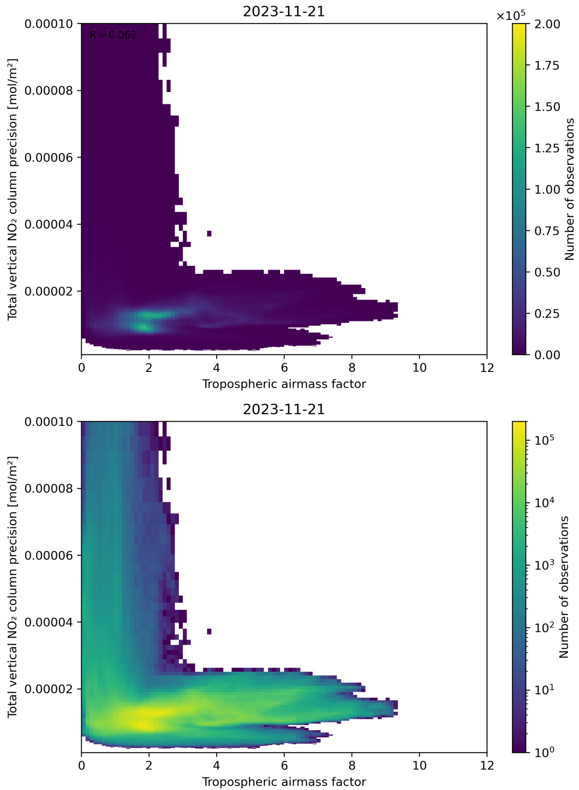
Figure 78: Scatter density plot of “Tropospheric air mass factor” against “Total vertical NO 2 column precision” for 2023-11-20 to 2023-11-22.
