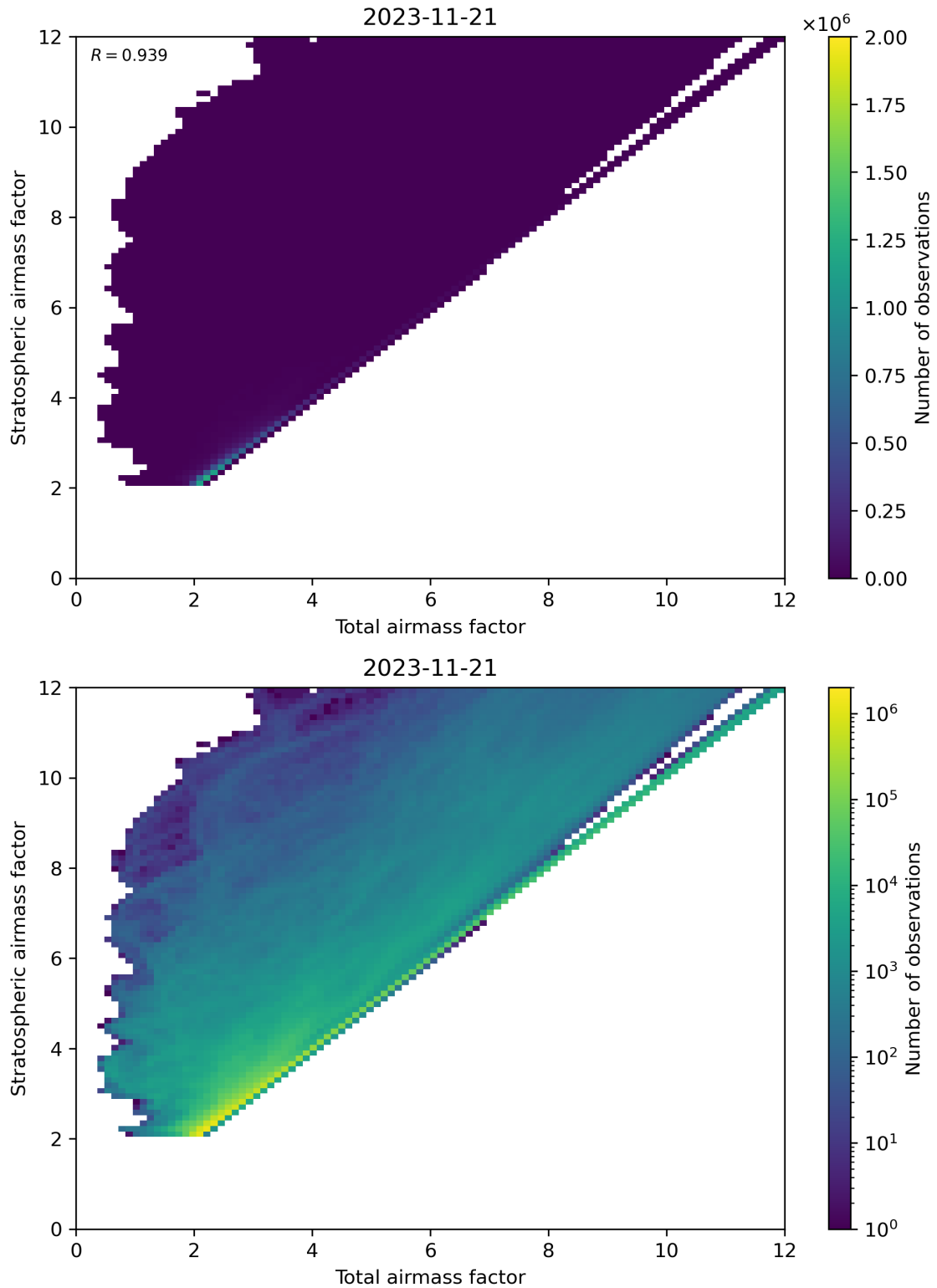
Figure 62: Scatter density plot of “Total airmass factor” against “Stratospheric airmass factor” for 2023-11-20 to 2023-11-22.
