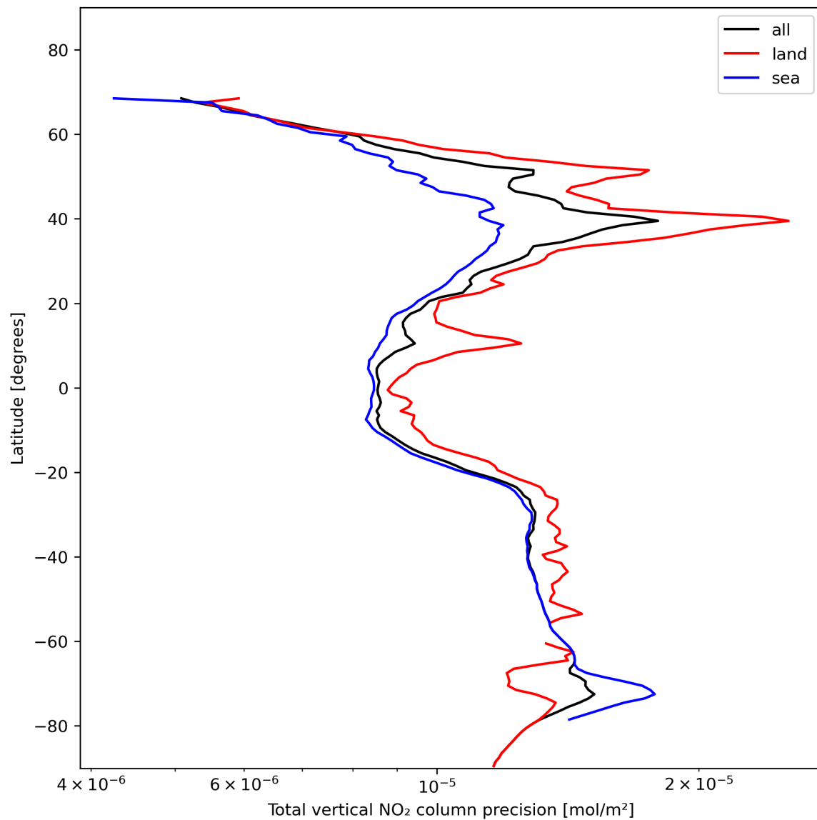
Figure 22: Zonal average of “Total vertical NO 2 column precision” for 2023-11-20 to 2023-11-22.
