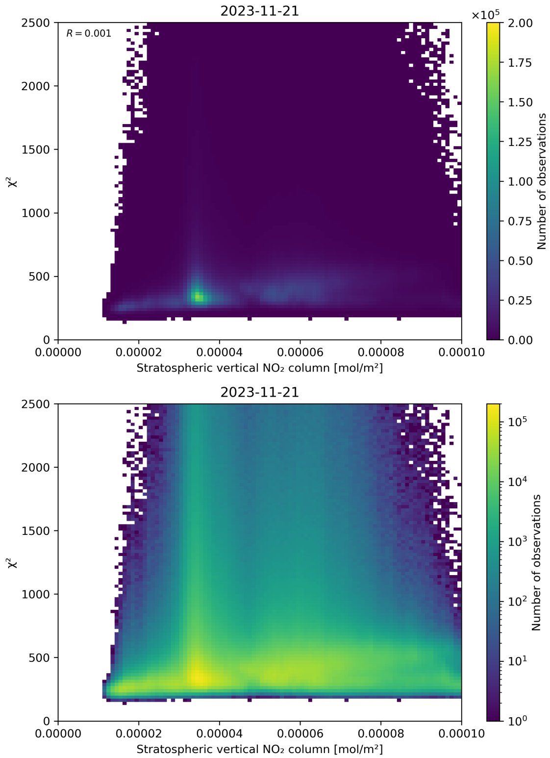
Figure 97: Scatter density plot of “Stratospheric vertical NO 2 column” against “ \chi^2 ” for 2023-11-20 to 2023-11-22.
