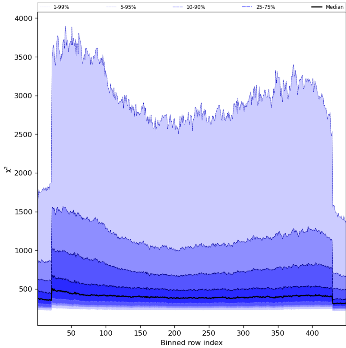
Figure 59: Along track statistics of “ \chi^2 ” for 2023-11-20 to 2023-11-22
