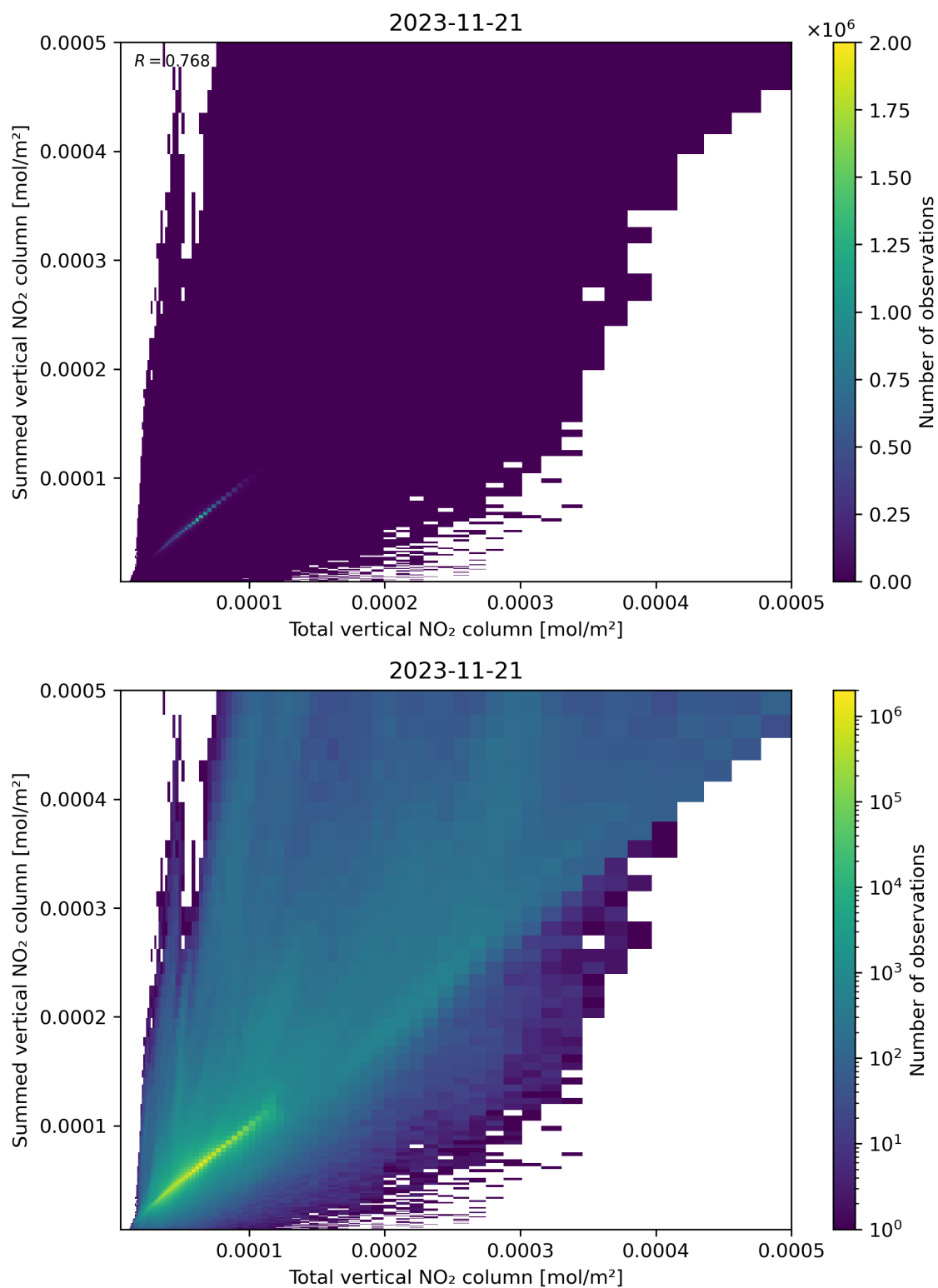
Figure 112: Scatter density plot of “Total vertical NO 2 column” against “Summed vertical NO 2 column” for 2023-11-20 to 2023-11-22.
