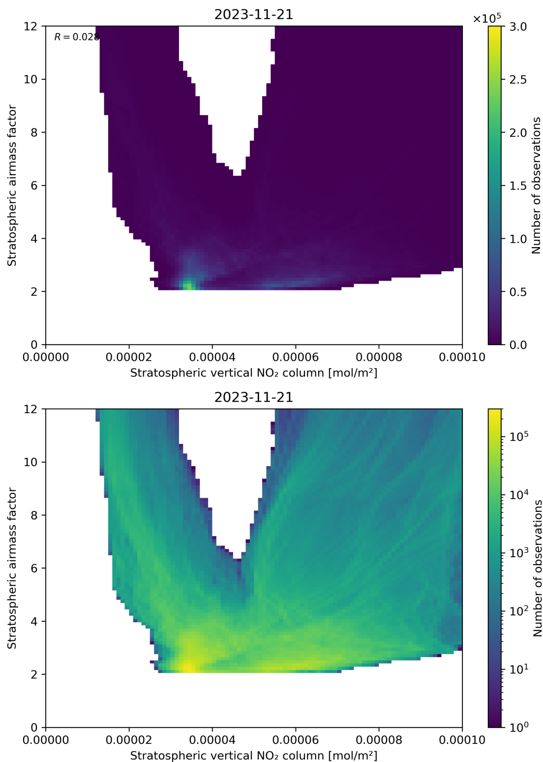
Figure 96: Scatter density plot of “Stratospheric vertical NO 2 column” against “Stratospheric airmass factor” for 2023-11-20 to 2023-11-22.
