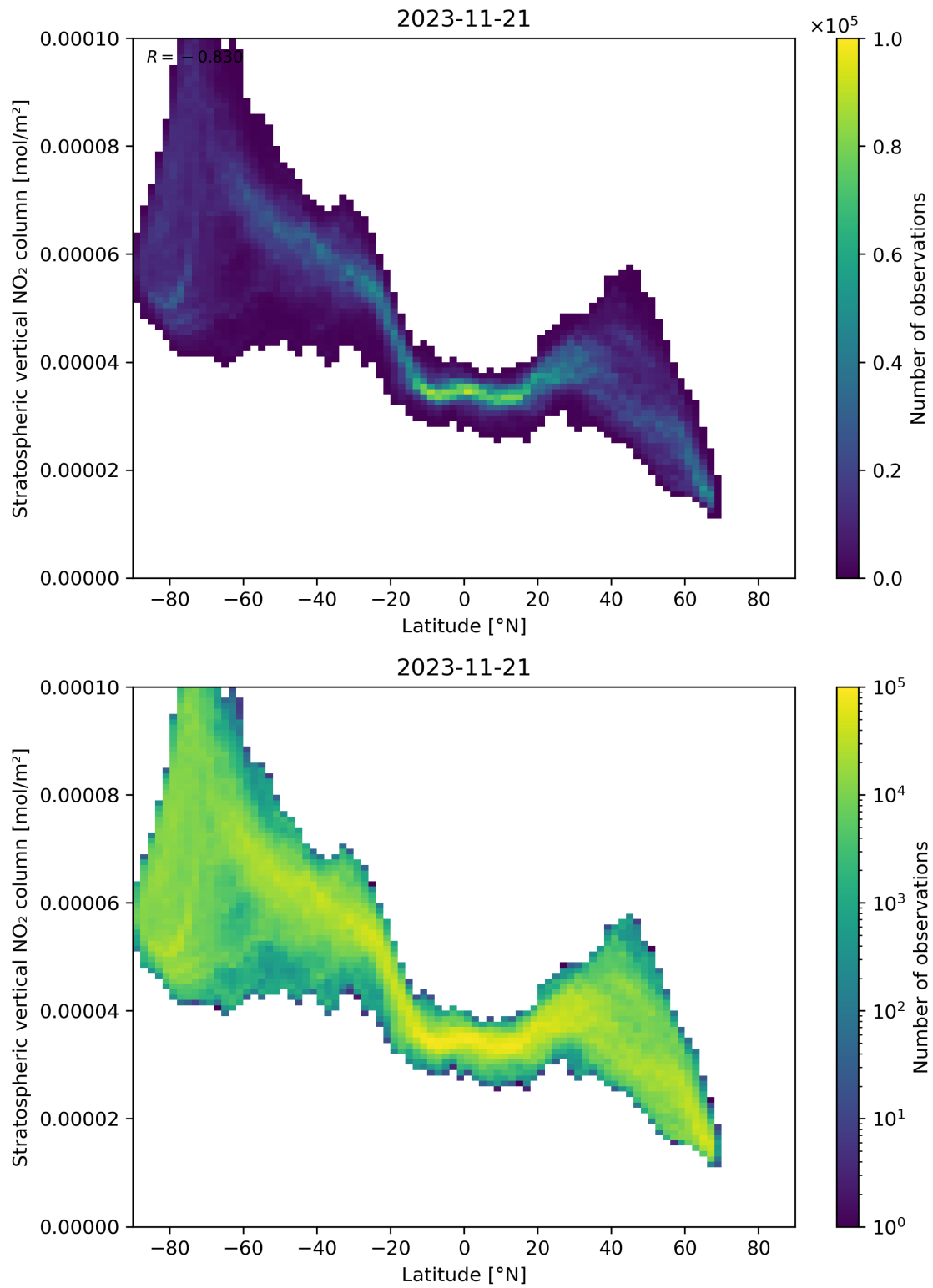
Figure 87: Scatter density plot of “Latitude” against “Stratospheric vertical NO 2 column” for 2023-11-20 to 2023-11-22.
