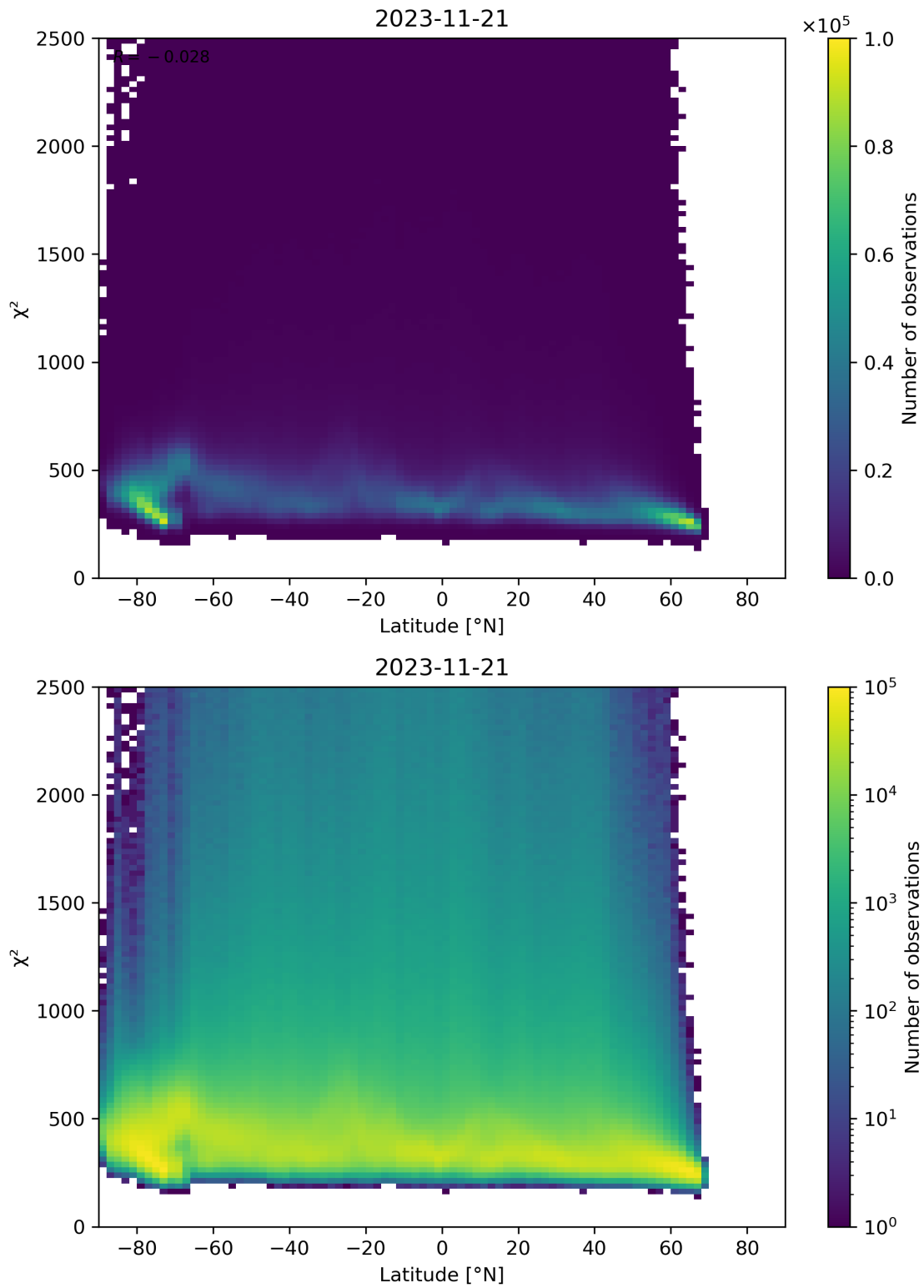
Figure 86: Scatter density plot of “Latitude” against “ \chi^2 ” for 2023-11-20 to 2023-11-22.
