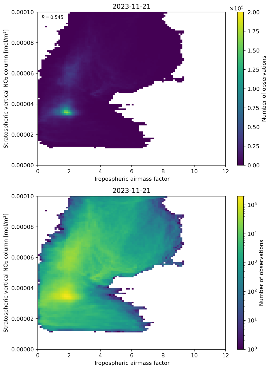
Figure 74: Scatter density plot of “Tropospheric air mass factor” against “Stratospheric vertical NO 2 column” for 2023-11-20 to 2023-11-22.
