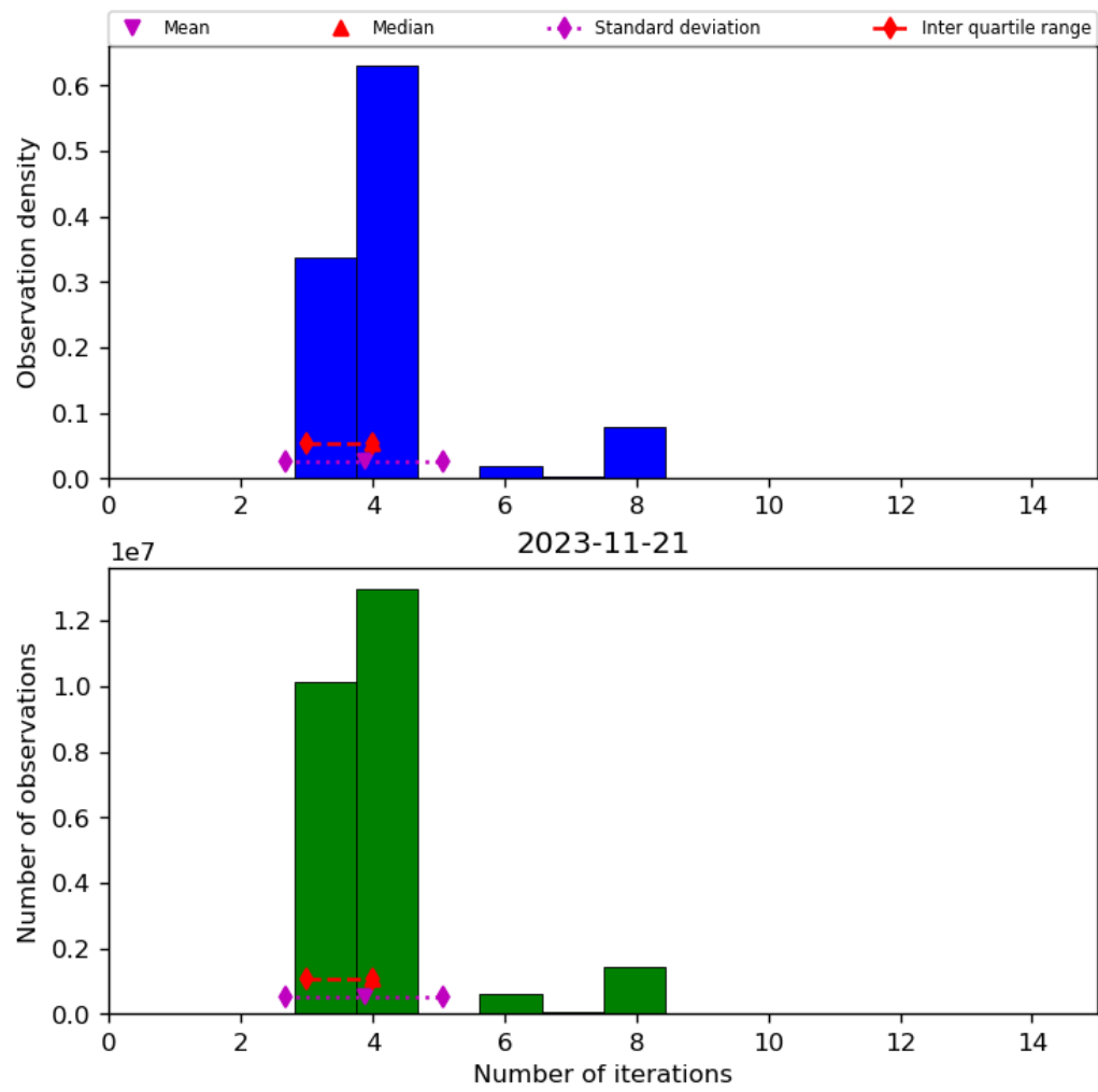
Figure 34: Histogram of “Number of iterations” for 2023-11-20 to 2023-11-22
