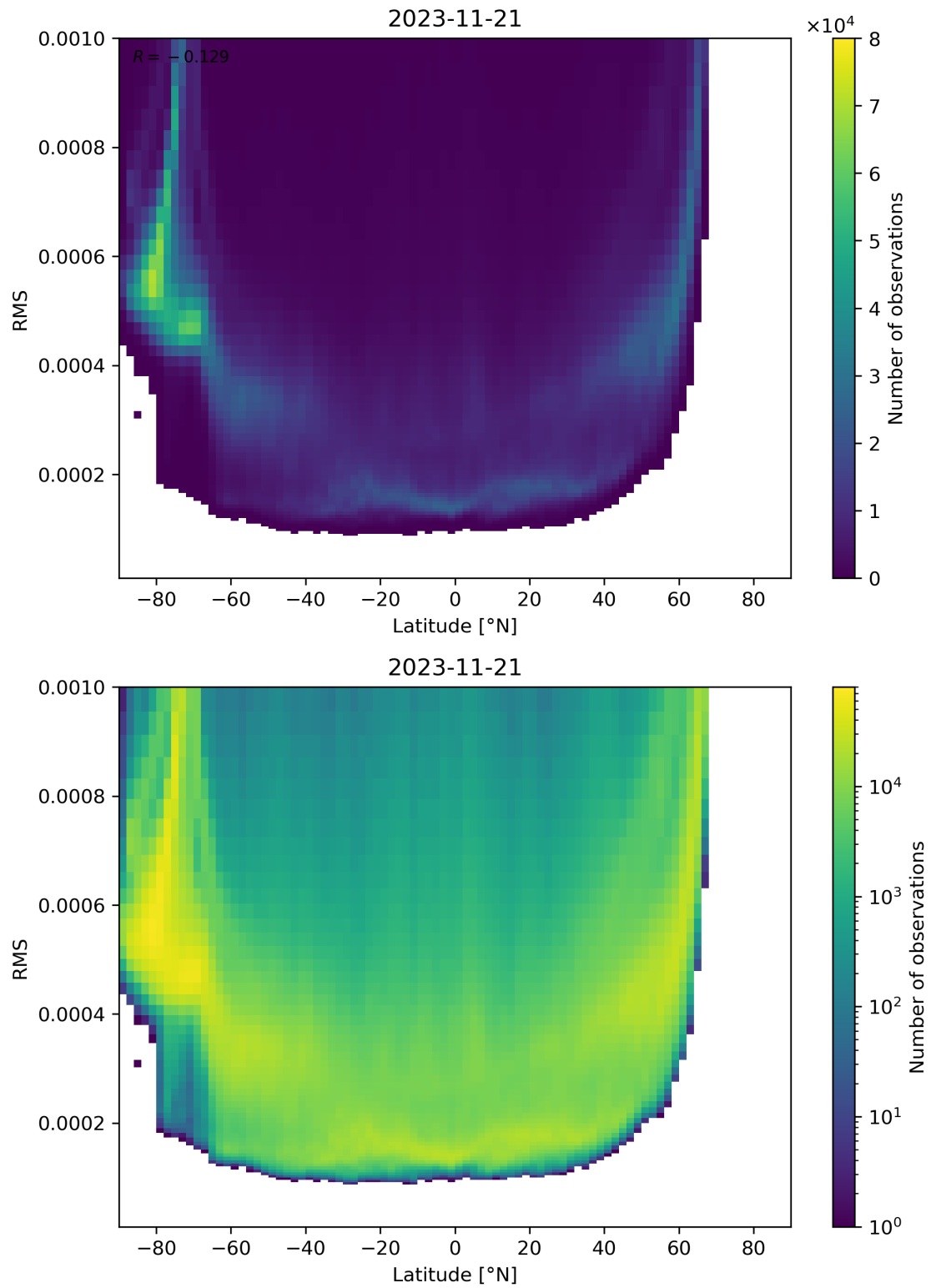
Figure 94: Scatter density plot of “Latitude” against “RMS” for 2023-11-20 to 2023-11-22.
