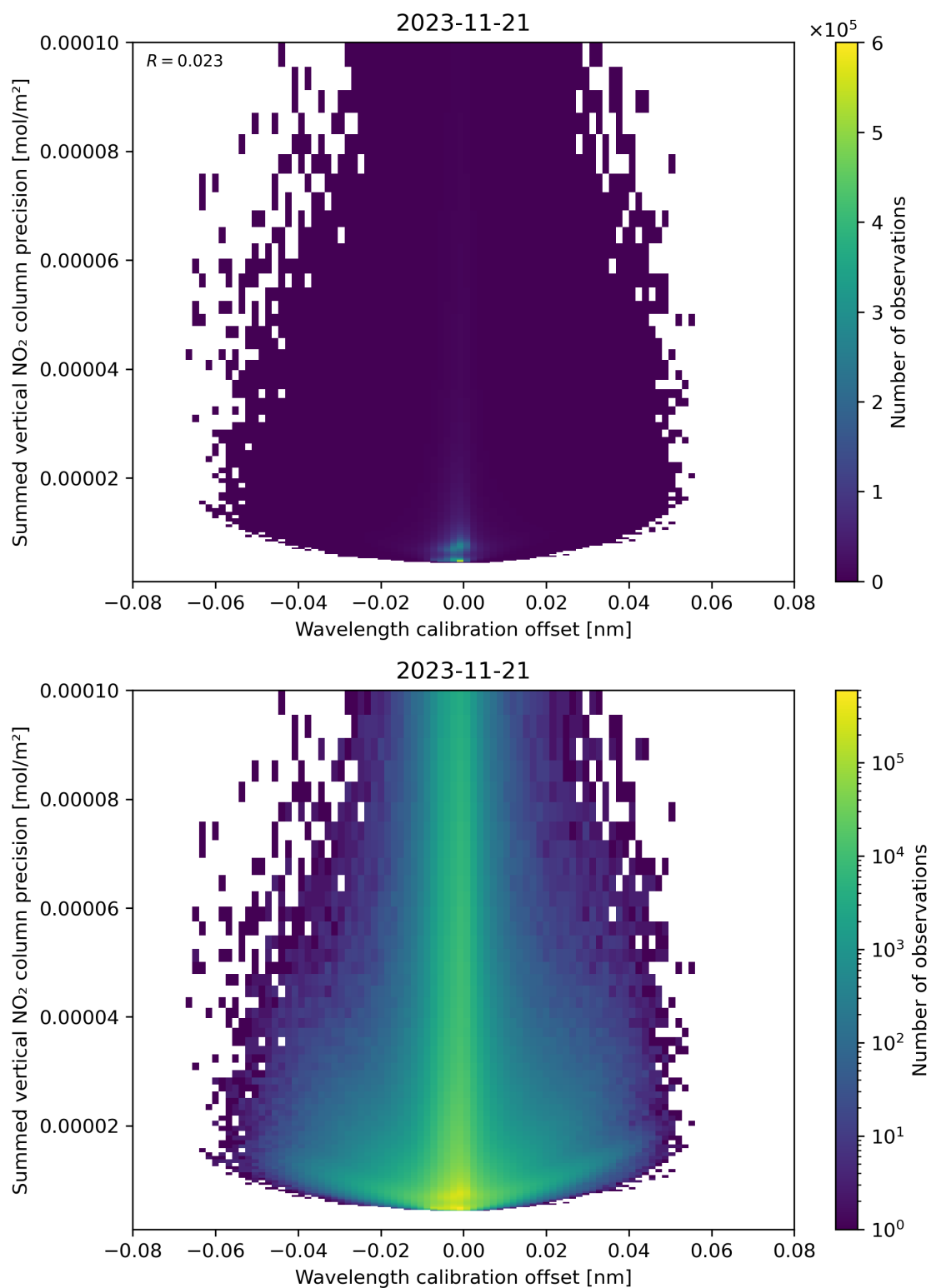
Figure 178: Scatter density plot of “Wavelength calibration offset” against “Summed vertical NO 2 column precision” for 2023-11-20 to 2023-11-22.
