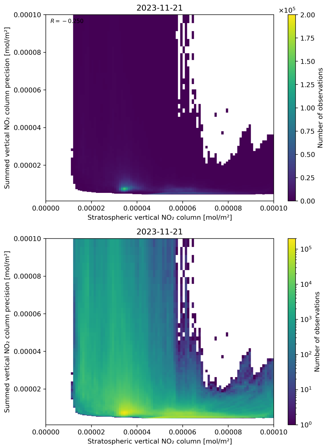
Figure 99: Scatter density plot of “Stratospheric vertical NO 2 column” against “Summed vertical NO 2 column precision” for 2023-11-20 to 2023-11-22.
