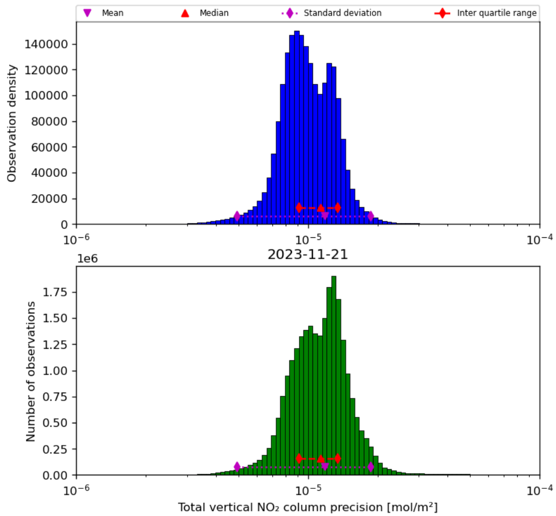
Figure 39: Histogram of “Total vertical NO 2 column precision” for 2023-11-20 to 2023-11-22
