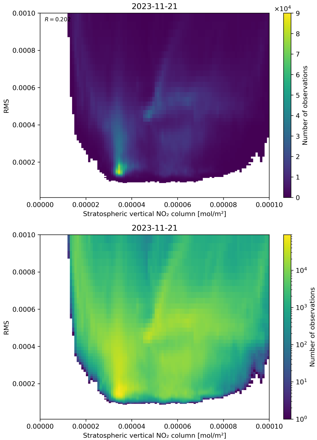
Figure 102: Scatter density plot of “Stratospheric vertical NO 2 column” against “RMS” for 2023-11-20 to 2023-11-22.
