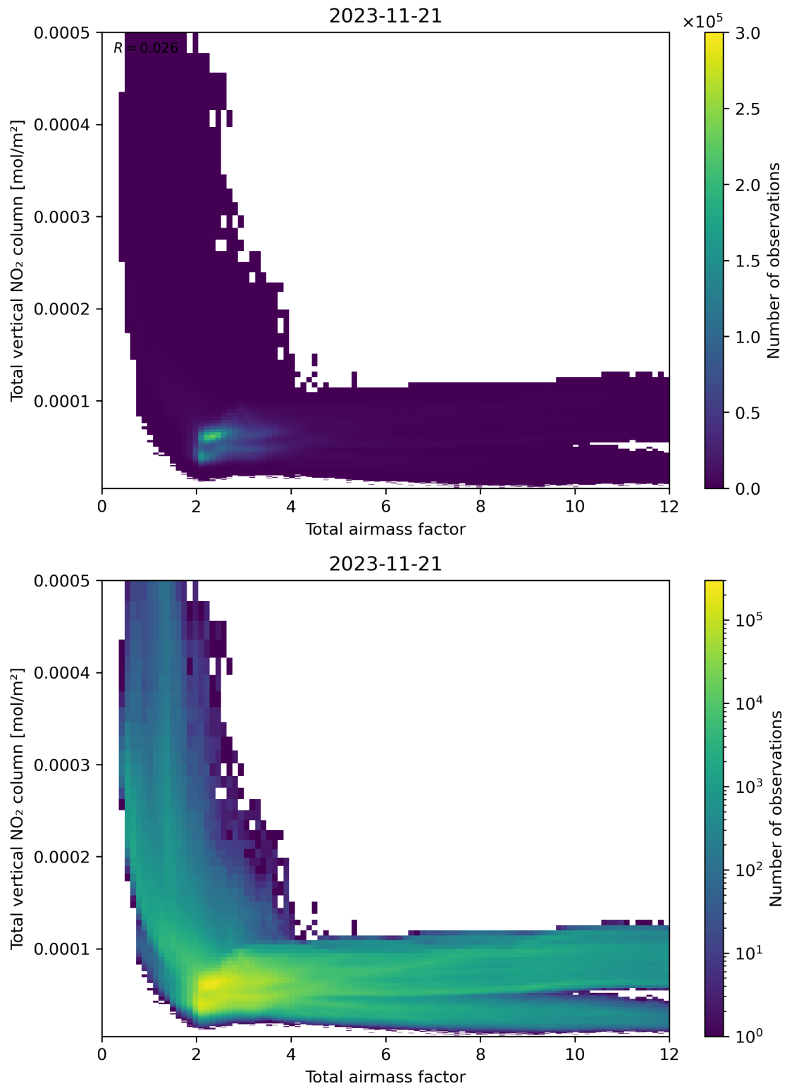
Figure 67: Scatter density plot of “Total airmass factor” against “Total vertical NO 2 column” for 2023-11-20 to 2023-11-22.
