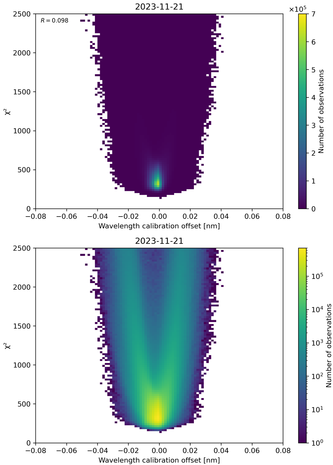
Figure 175: Scatter density plot of “Wavelength calibration offset” against “ \chi^2 ” for 2023-11-20 to 2023-11-22.
