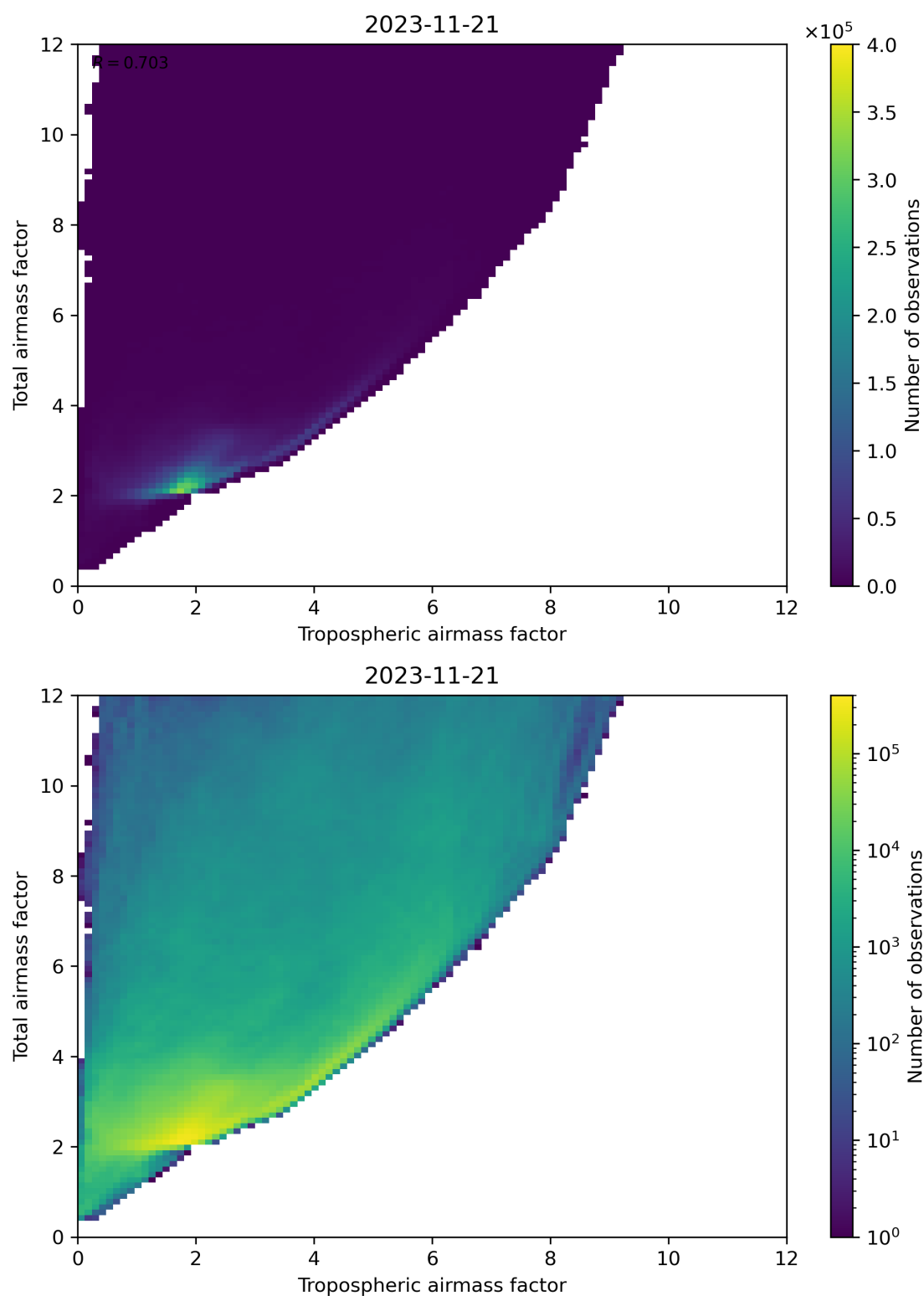
Figure 72: Scatter density plot of “Tropospheric airmass factor” against “Total airmass factor” for 2023-11-20 to 2023-11-22.
