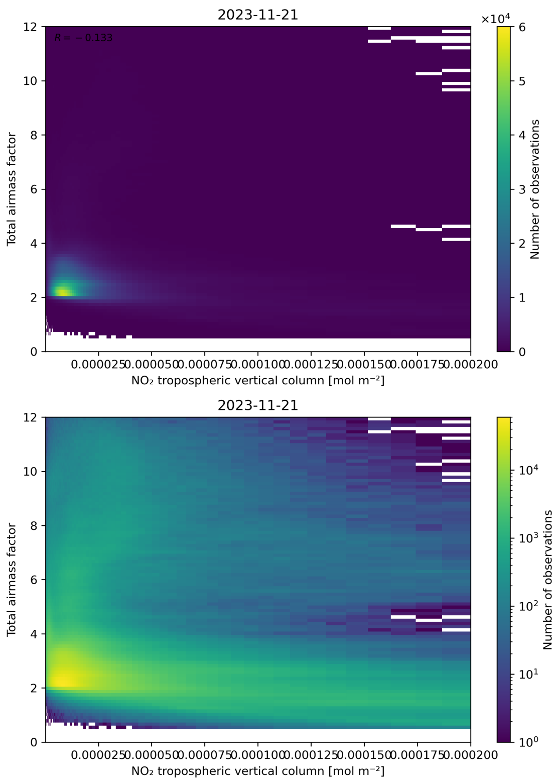
Figure 122: Scatter density plot of “NO 2 tropospheric vertical column” against “Total air mass factor” for 2023-11-20 to 2023-11-22.
