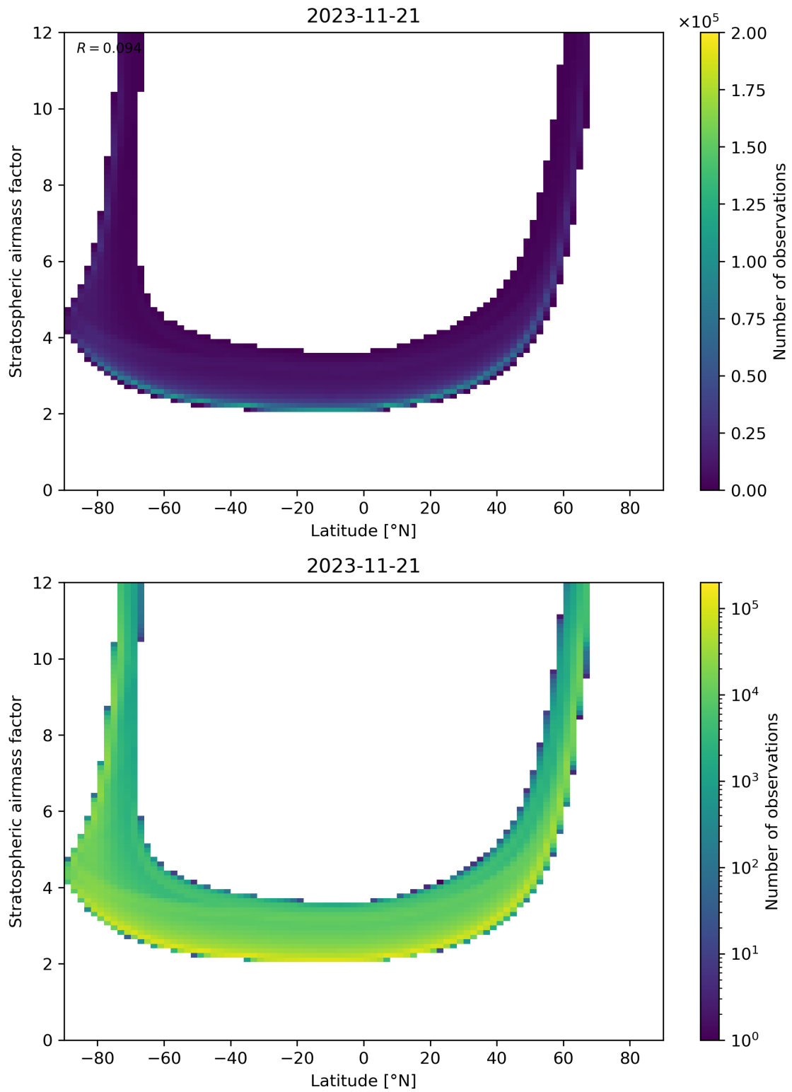
Figure 83: Scatter density plot of “Latitude” against “Stratospheric airmass factor” for 2023-11-20 to 2023-11-22.
