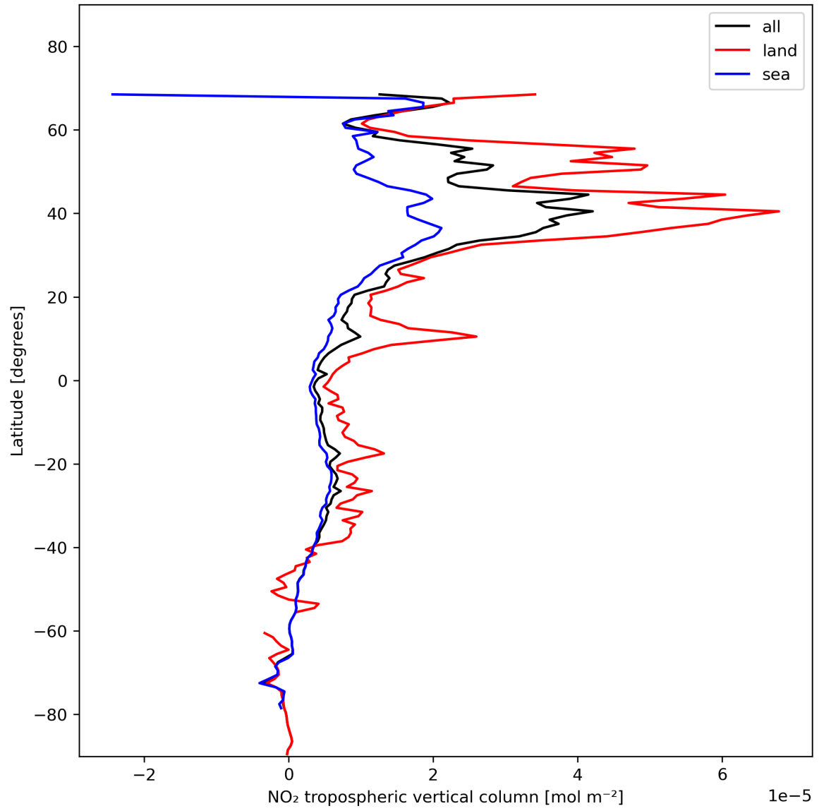
Figure 12: Zonal average of “NO 2 tropospheric vertical column” for 2023-11-20 to 2023-11-22.
