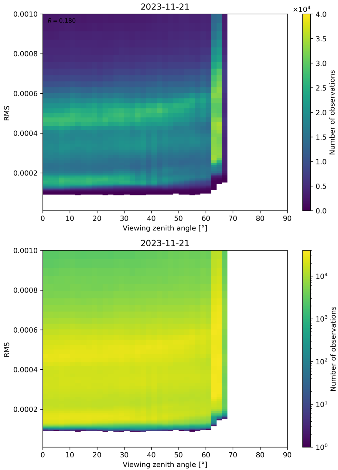
Figure 171: Scatter density plot of “Viewing zenith angle” against “RMS” for 2023-11-20 to 2023-11-22.
