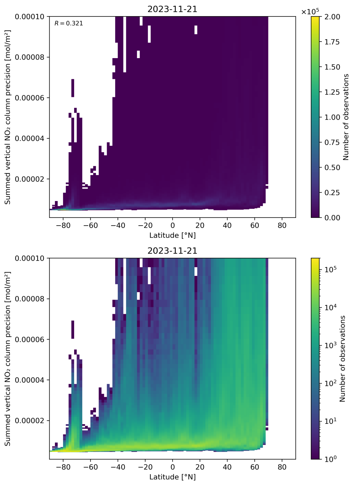
Figure 89: Scatter density plot of “Latitude” against “Summed vertical NO 2 column precision” for 2023-11-20 to 2023-11-22.
