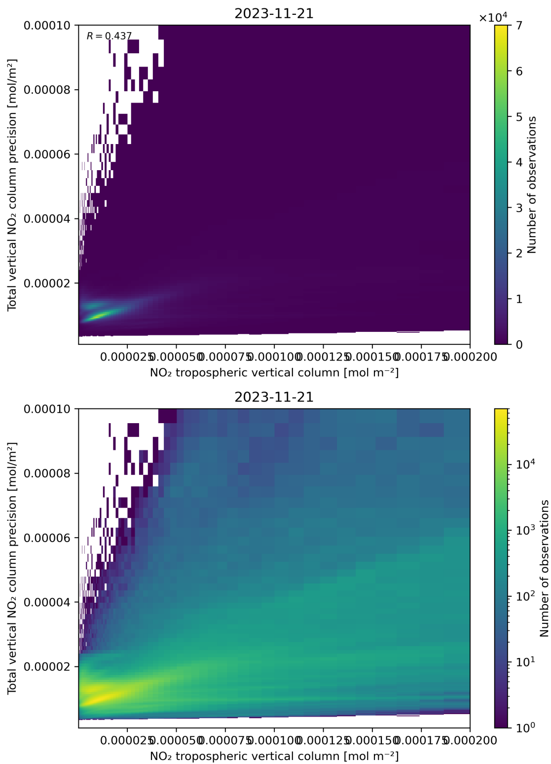
Figure 129: Scatter density plot of “NO 2 tropospheric vertical column” against “Total vertical NO 2 column precision” for 2023-11-20 to 2023-11-22.
