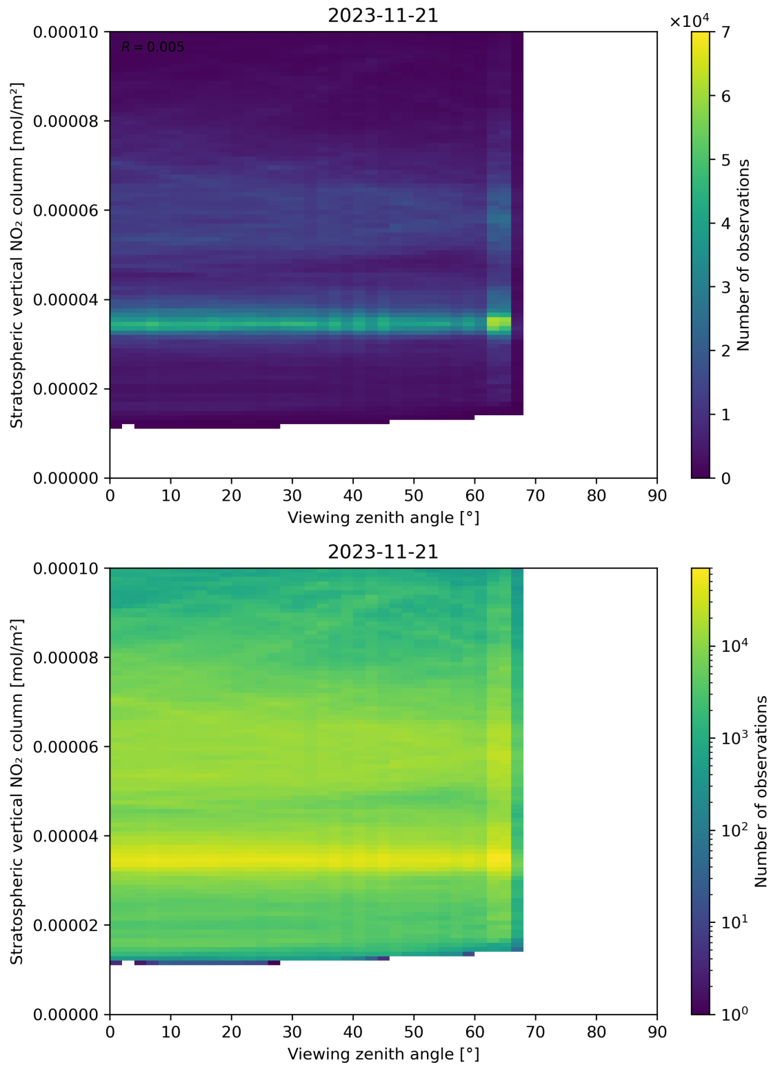
Figure 164: Scatter density plot of “Viewing zenith angle” against “Stratospheric vertical NO 2 column” for 2023-11-20 to 2023-11-22.
