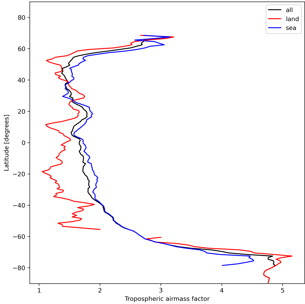
Figure 14: Zonal average of “Tropospheric airmass factor” for 2023-11-20 to 2023-11-22.
