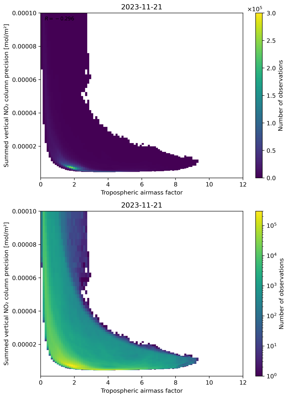
Figure 76: Scatter density plot of “Tropospheric air mass factor” against “Summed vertical NO 2 column precision” for 2023-11-20 to 2023-11-22.
