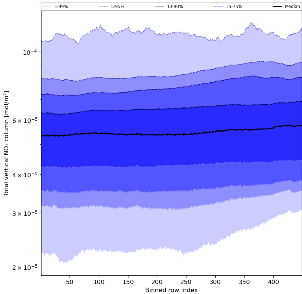
Figure 55: Along track statistics of “Total vertical NO 2 column” for 2023-11-20 to 2023-11-22
