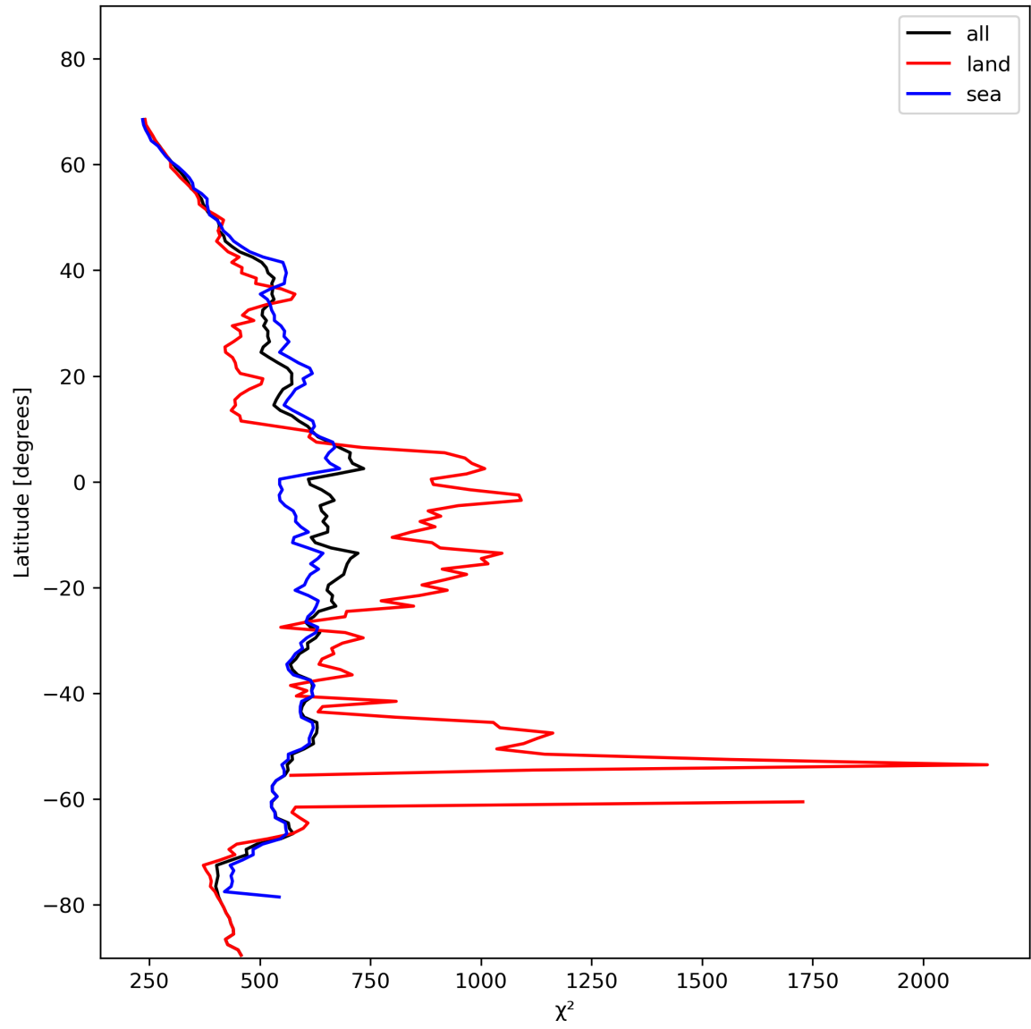
Figure 25: Zonal average of “ \chi^2 ” for 2023-11-20 to 2023-11-22.
