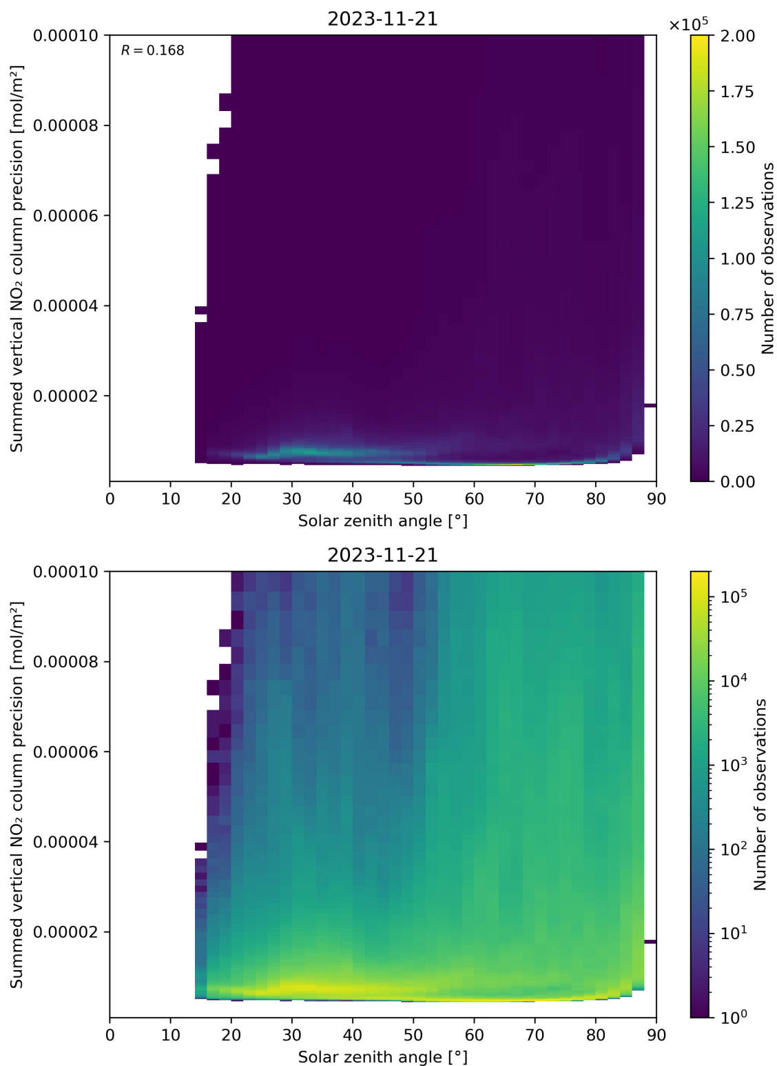
Figure 152: Scatter density plot of “Solar zenith angle” against “Summed vertical NO 2 column precision” for 2023-11-20 to 2023-11-22.
