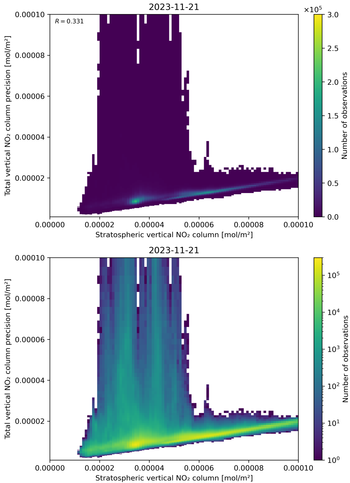
Figure 101: Scatter density plot of “Stratospheric vertical NO 2 column” against “Total vertical NO 2 column precision” for 2023-11-20 to 2023-11-22.
