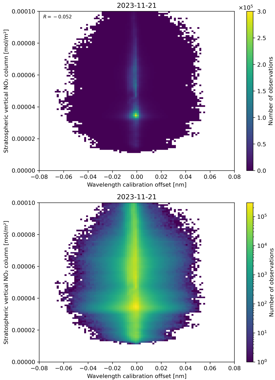
Figure 176: Scatter density plot of “Wavelength calibration offset” against “Stratospheric vertical NO 2 column” for 2023-11-20 to 2023-11-22.
