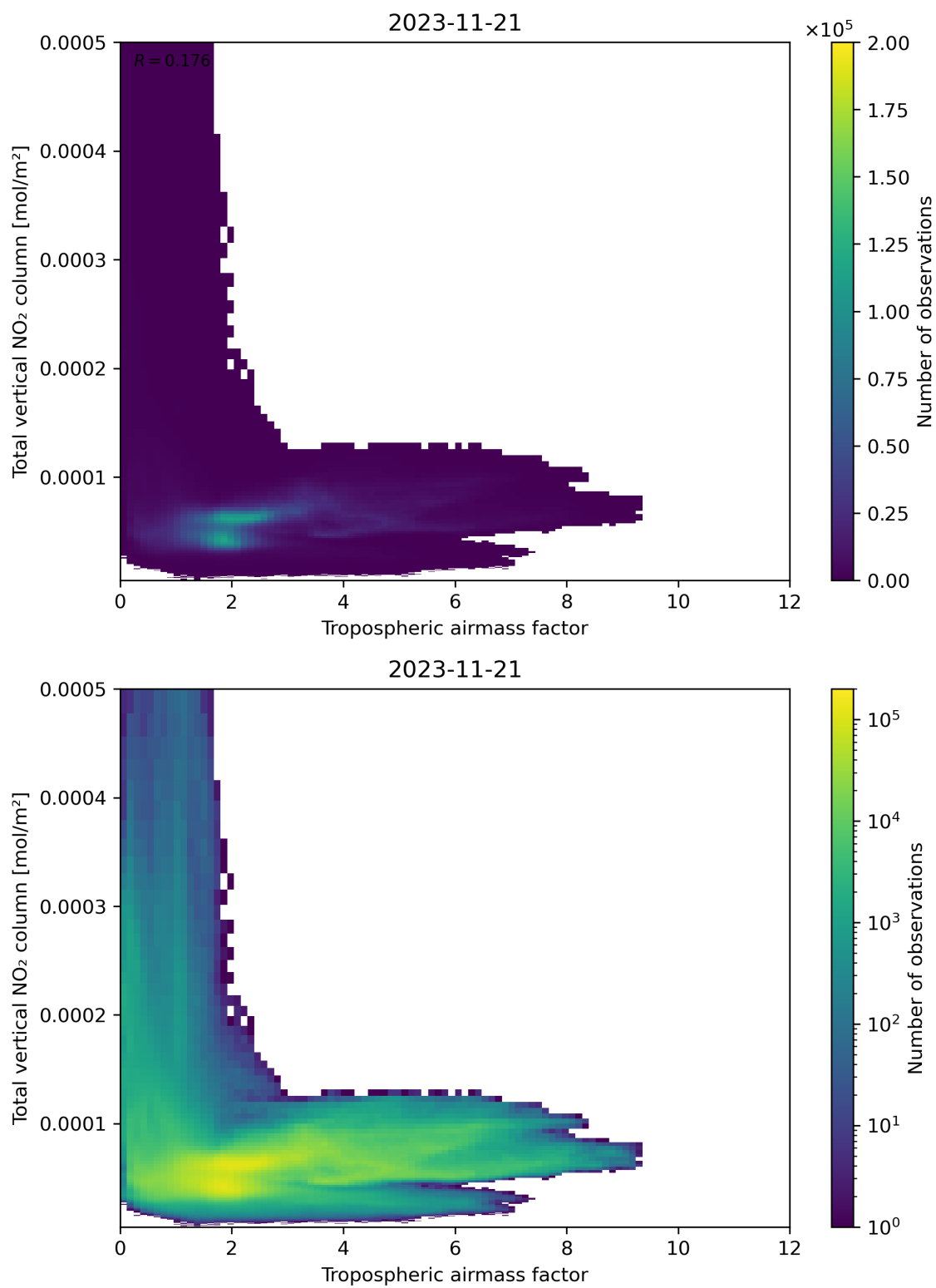
Figure 77: Scatter density plot of “Tropospheric airmass factor” against “Total vertical NO 2 column” for 2023-11-20 to 2023-11-22.
