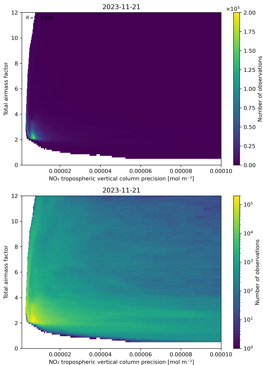
Figure 132: Scatter density plot of “NO 2 tropospheric vertical column precision” against “Total air mass factor” for 2023-11-20 to 2023-11-22.
