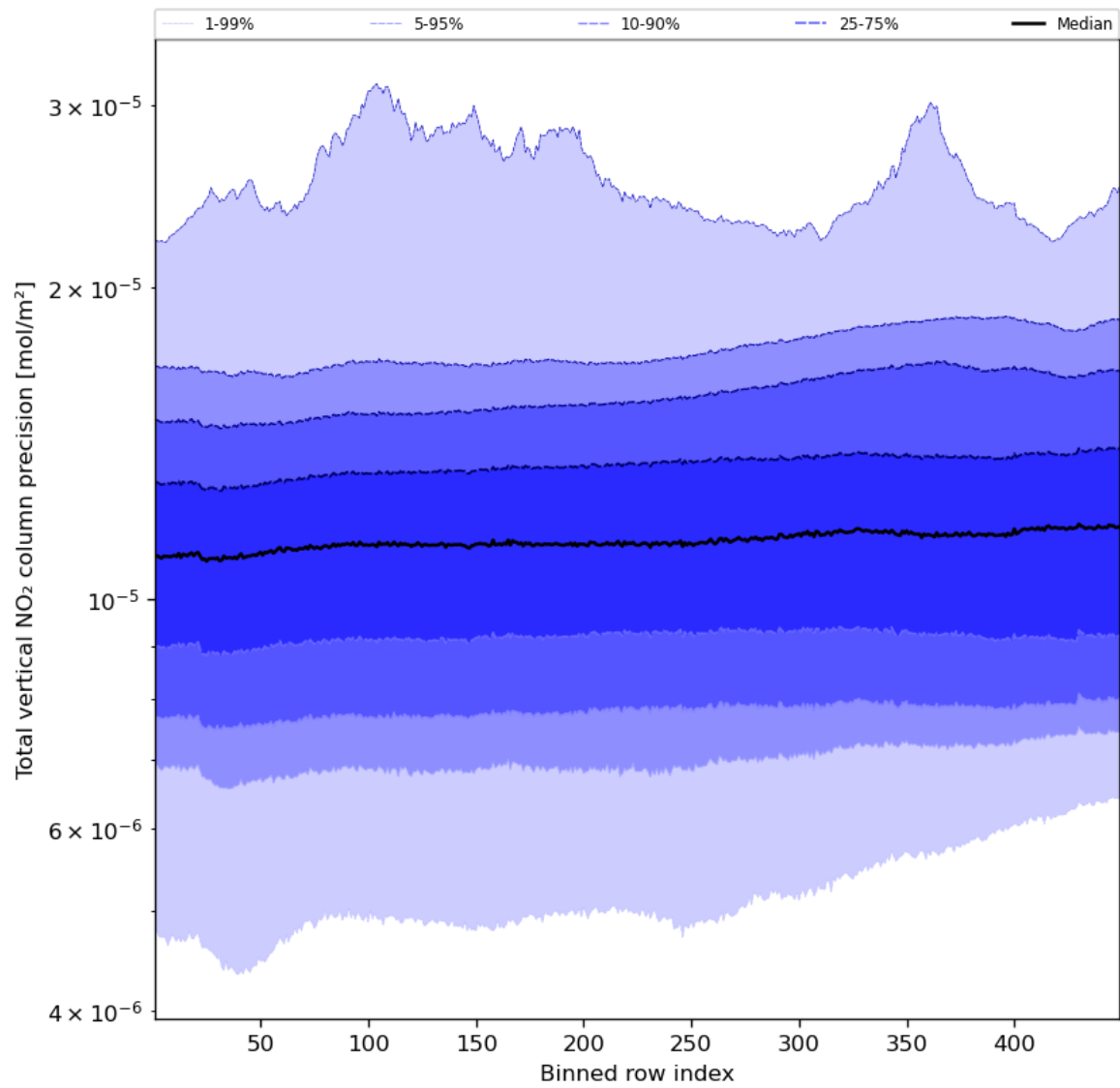
Figure 56: Along track statistics of “Total vertical NO 2 column precision” for 2023-11-20 to 2023-11-22
