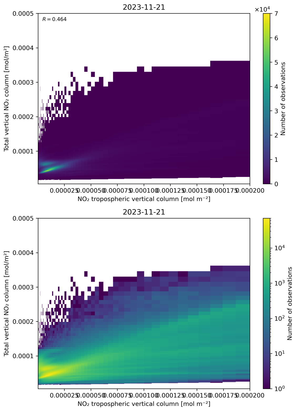
Figure 128: Scatter density plot of “NO 2 tropospheric vertical column” against “Total vertical NO 2 column” for 2023-11-20 to 2023-11-22.
