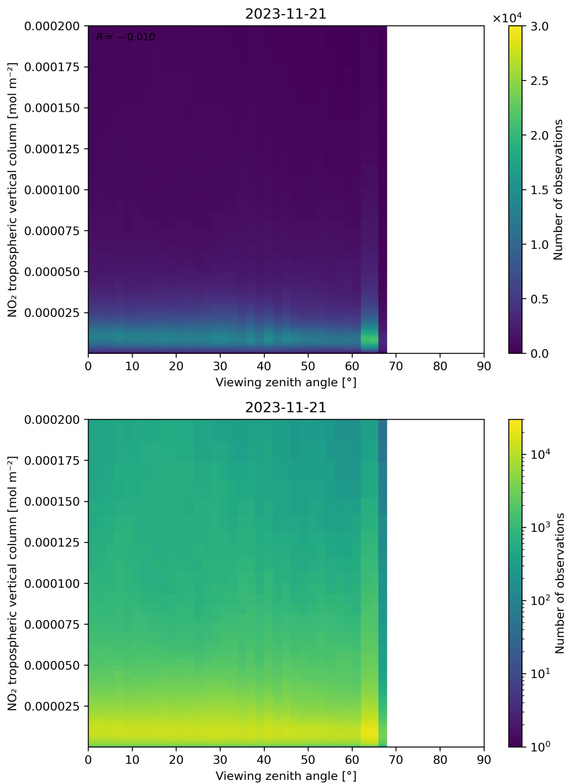
Figure 169: Scatter density plot of “Viewing zenith angle” against “NO 2 tropospheric vertical column” for 2023-11-20 to 2023-11-22.
