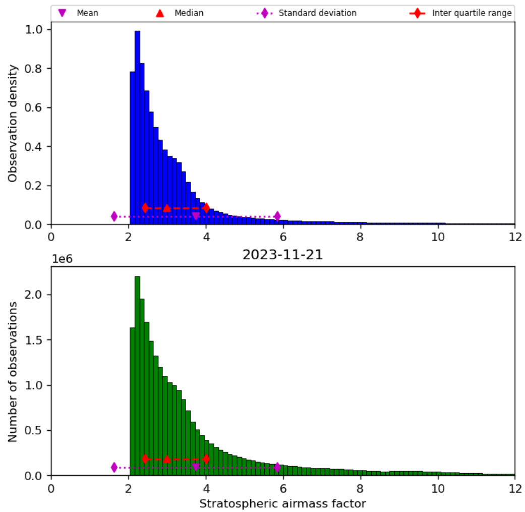
Figure 44: Histogram of “Stratospheric airmass factor” for 2023-11-20 to 2023-11-22
