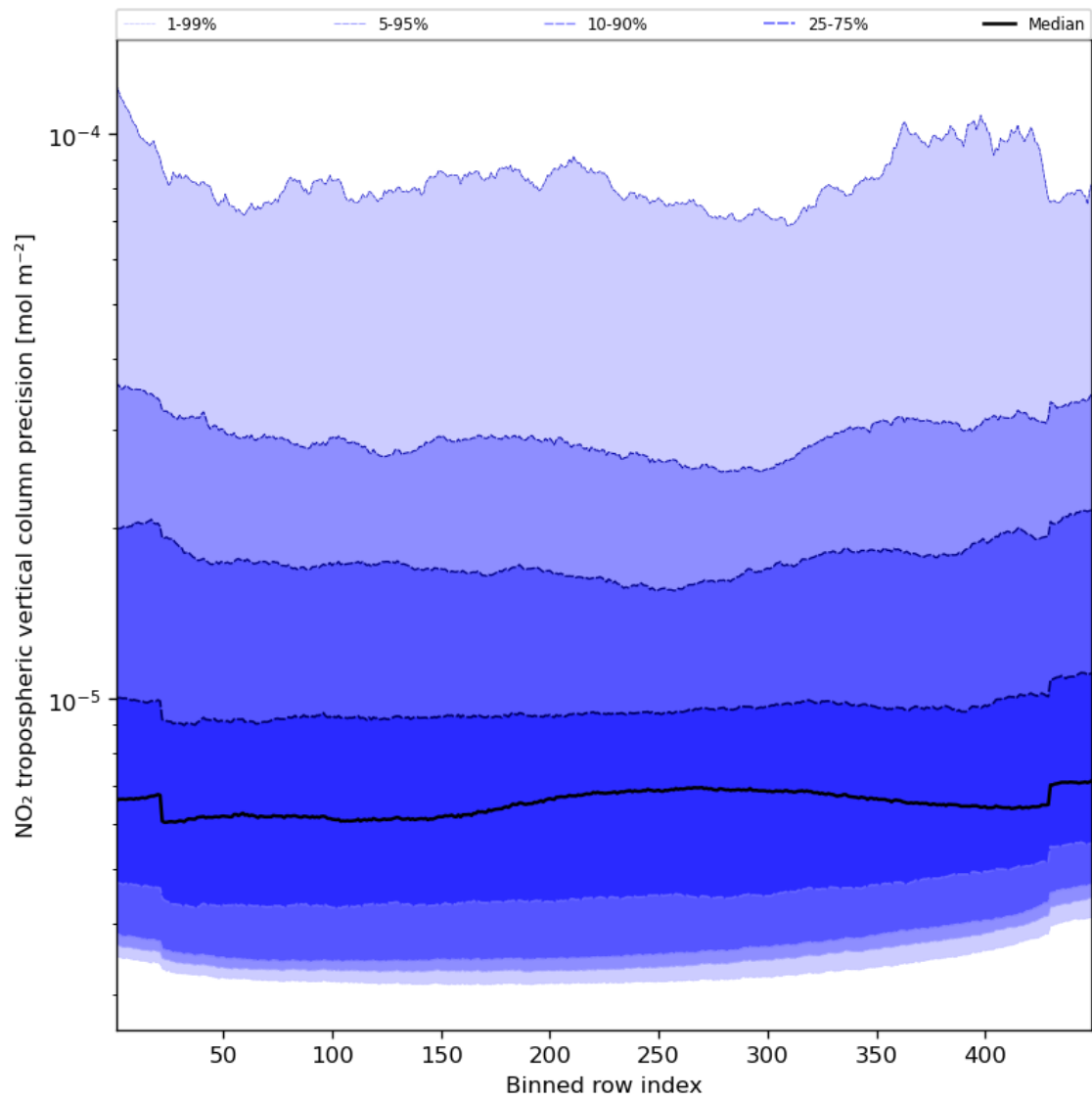
Figure 47: Along track statistics of “NO 2 tropospheric vertical column precision” for 2023-11-20 to 2023-11-22
