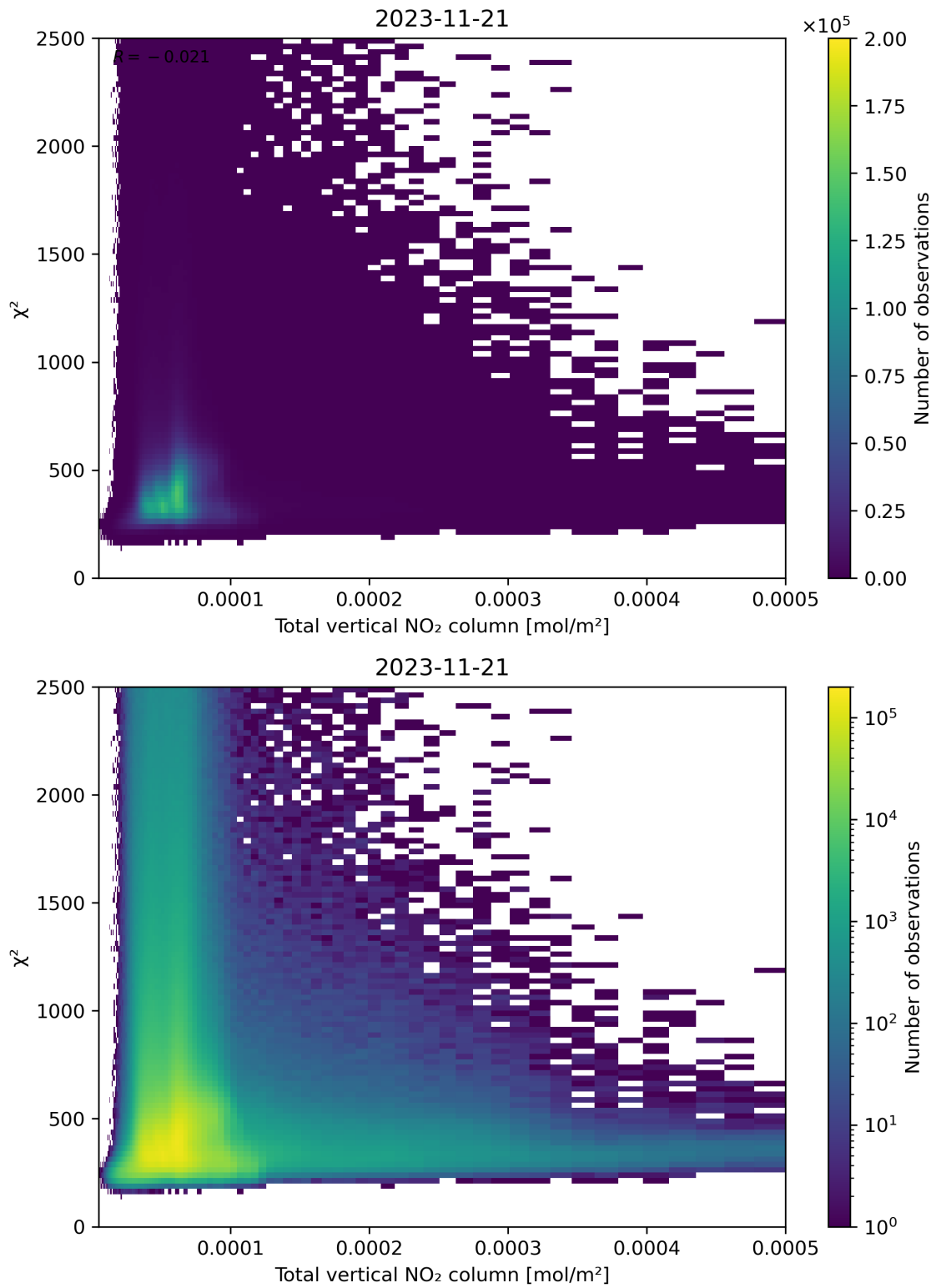
Figure 111: Scatter density plot of “Total vertical NO 2 column” against “ \chi^2 ” for 2023-11-20 to 2023-11-22.
