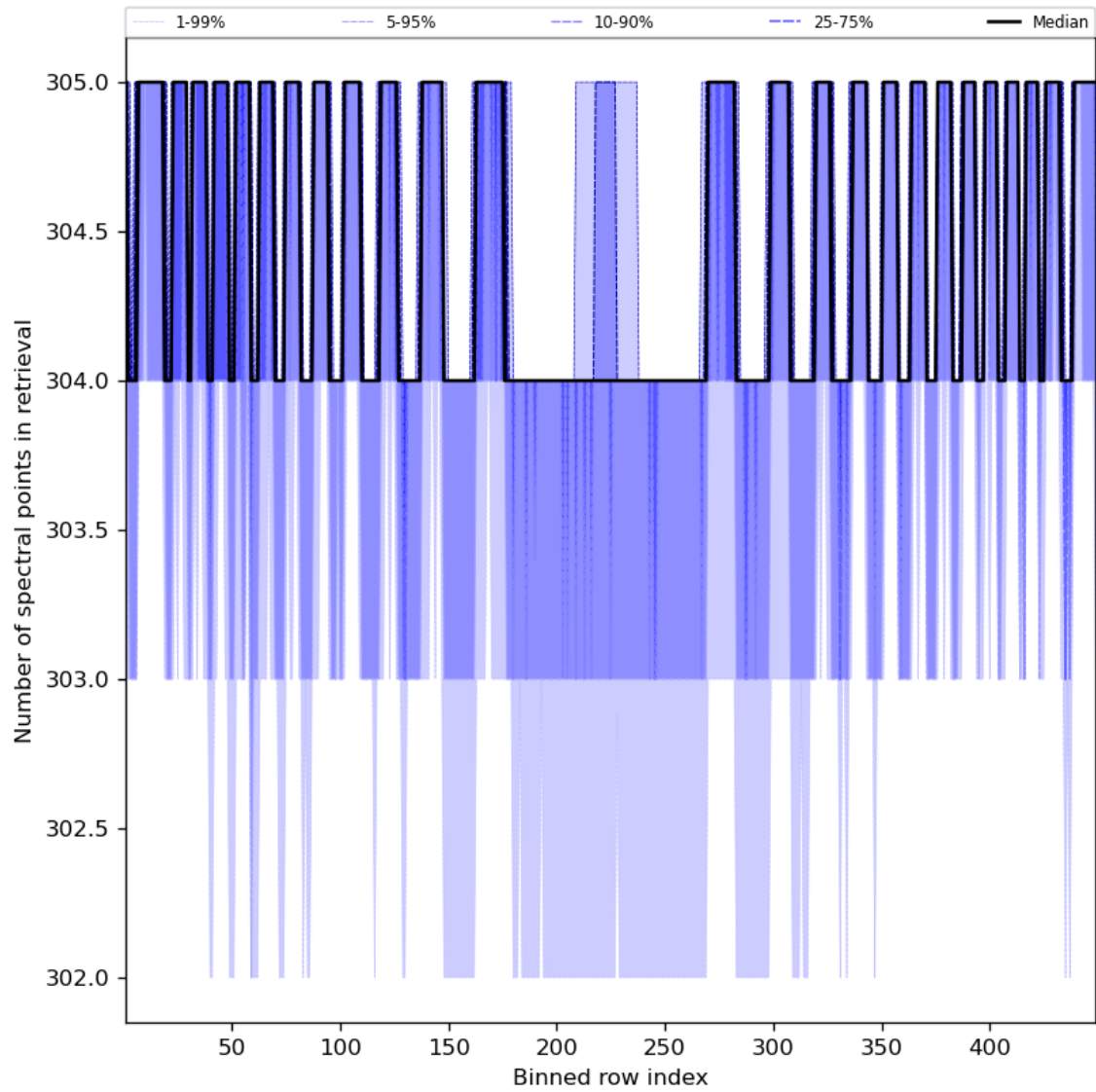
Figure 50: Along track statistics of “Number of spectral points in retrieval” for 2023-11-20 to 2023-11-22
