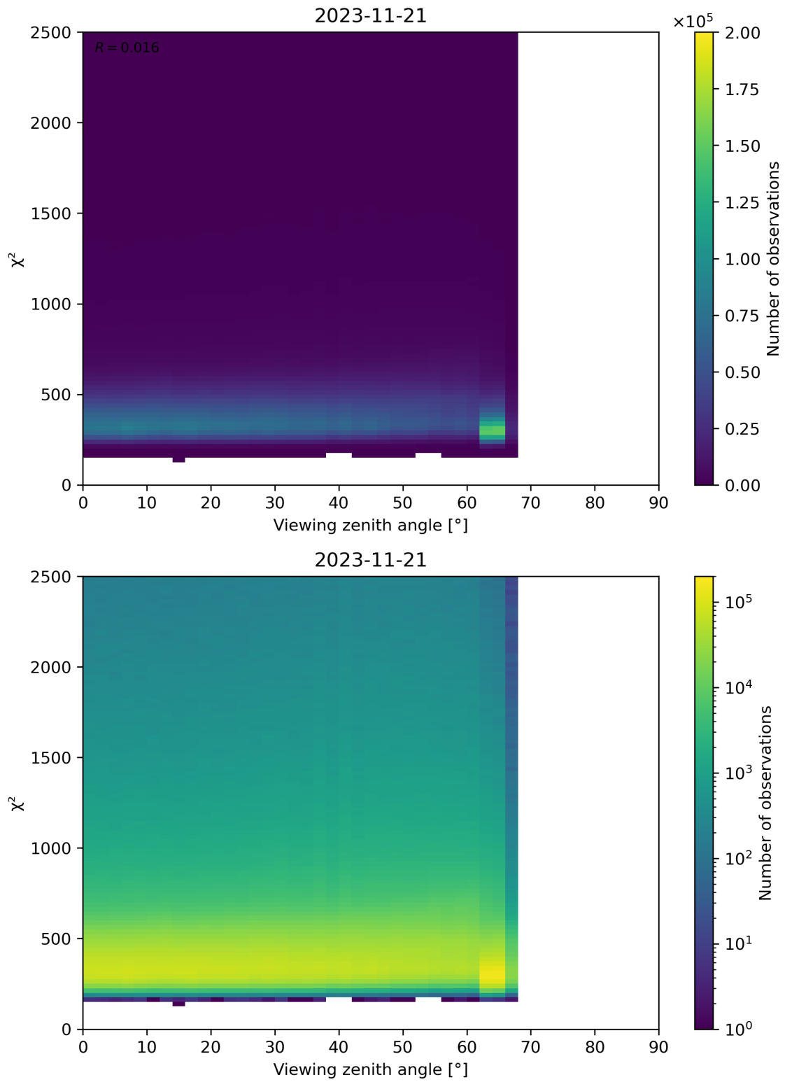
Figure 162: Scatter density plot of “Viewing zenith angle” against “ \chi^2 ” for 2023-11-20 to 2023-11-22.
