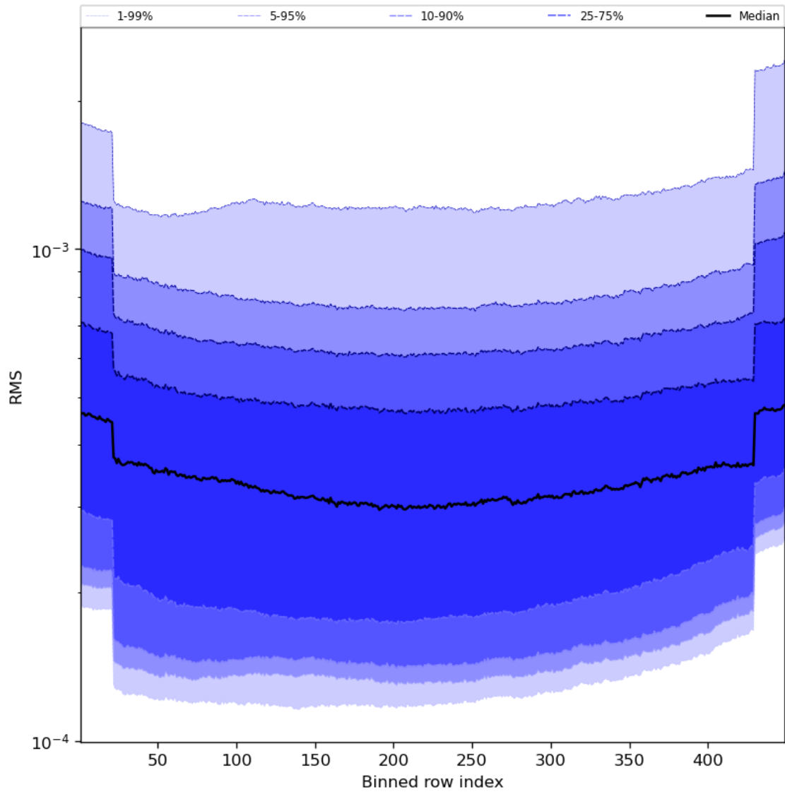
Figure 60: Along track statistics of “RMS” for 2023-11-20 to 2023-11-22
