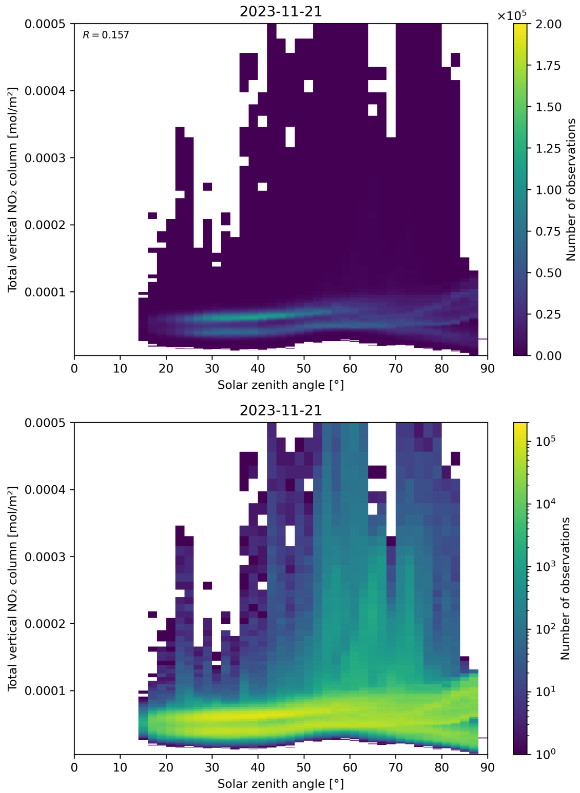
Figure 153: Scatter density plot of “Solar zenith angle” against “Total vertical NO 2 column” for 2023-11-20 to 2023-11-22.
