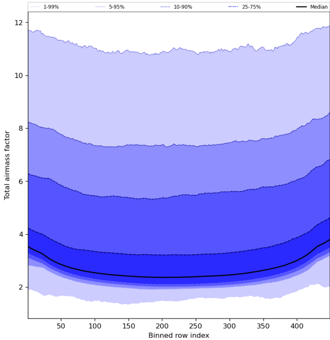
Figure 49: Along track statistics of “Total airmass factor” for 2023-11-20 to 2023-11-22
