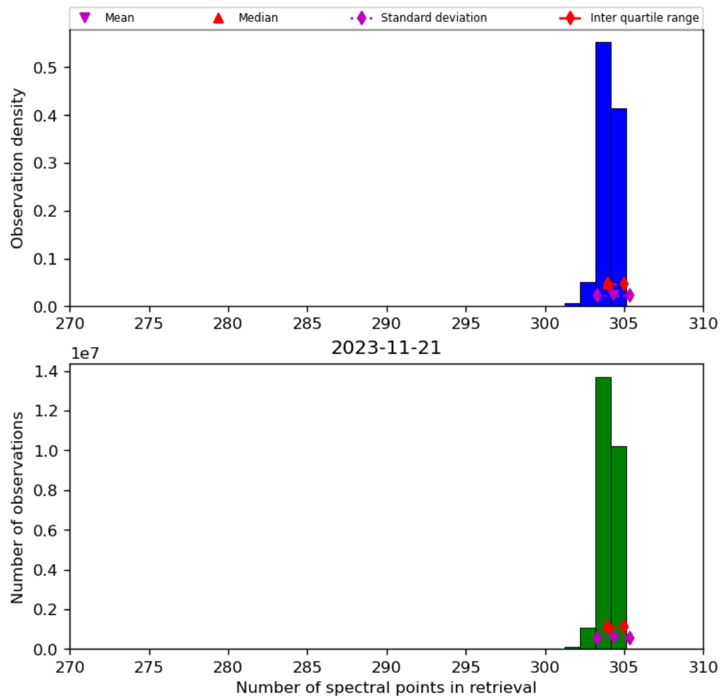
Figure 33: Histogram of “Number of spectral points in retrieval” for 2023-11-20 to 2023-11-22
