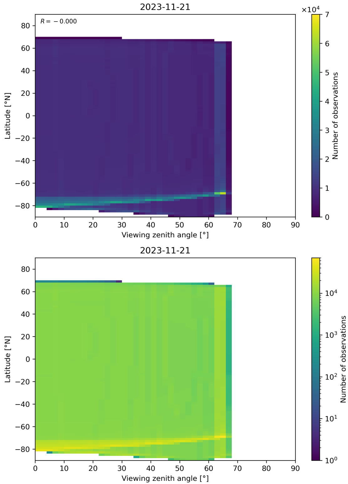
Figure 163: Scatter density plot of “Viewing zenith angle” against “Latitude” for 2023-11-20 to 2023-11-22.
