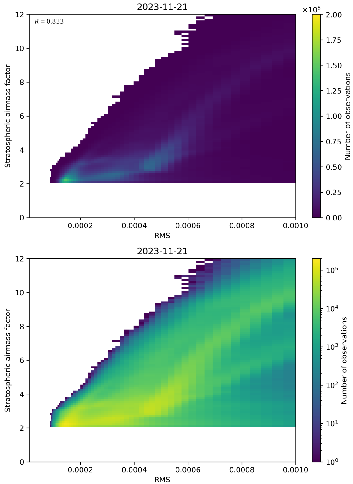
Figure 144: Scatter density plot of “RMS” against “Stratospheric airmass factor” for 2023-11-20 to 2023-11-22.
