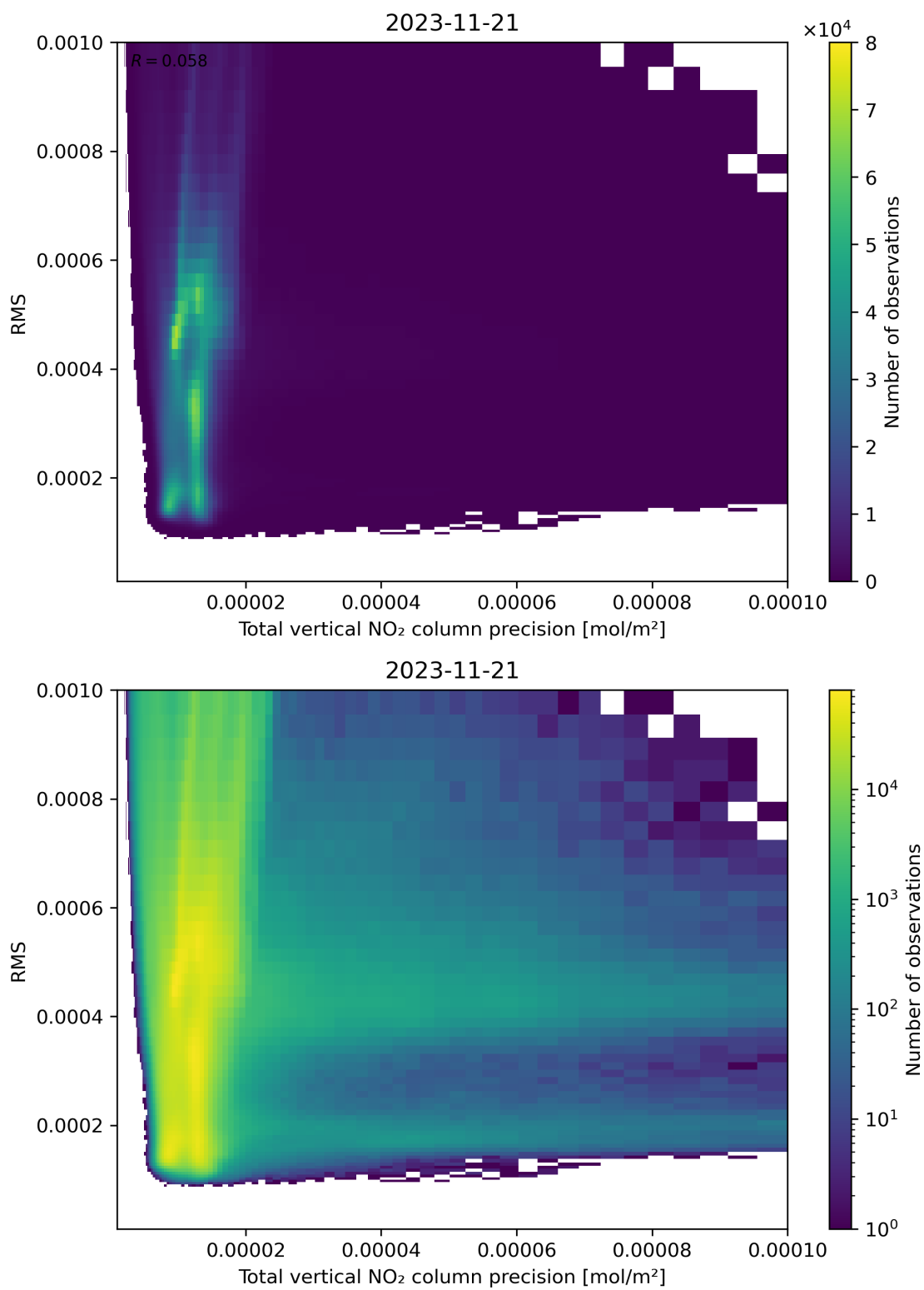
Figure 119: Scatter density plot of “Total vertical NO 2 column precision” against “RMS” for 2023-11-20 to 2023-11-22.
