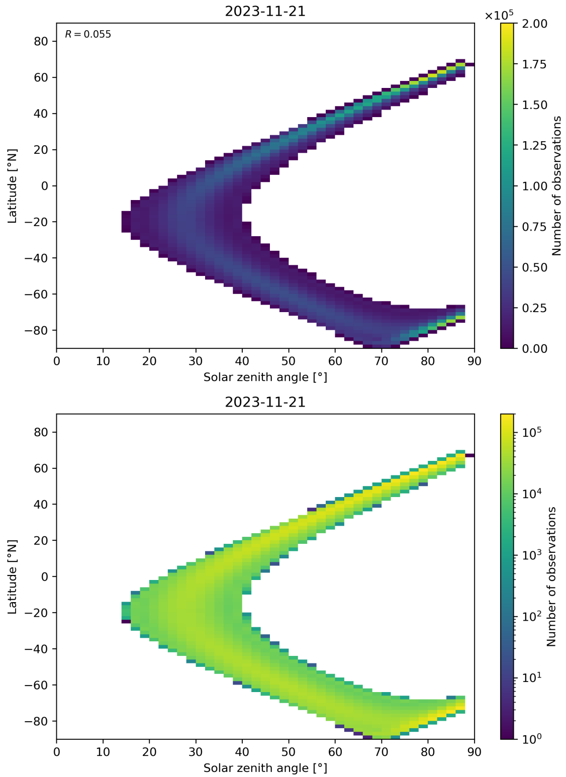
Figure 149: Scatter density plot of “Solar zenith angle” against “Latitude” for 2023-11-20 to 2023-11-22.
