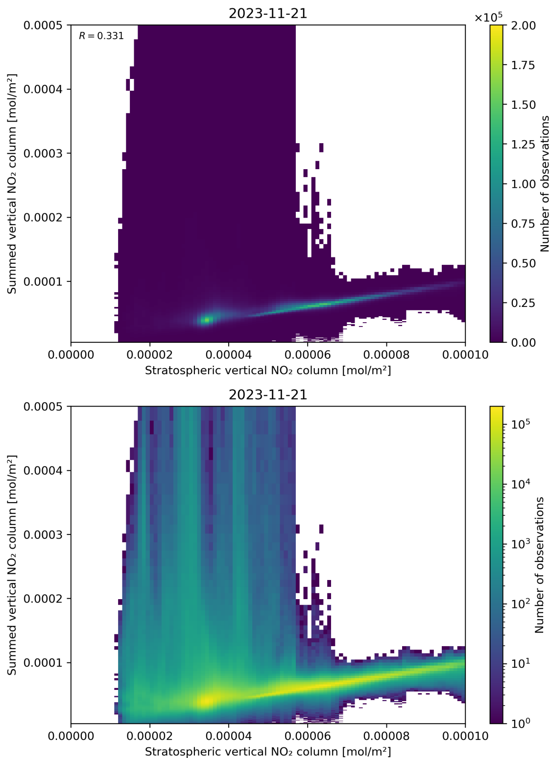
Figure 98: Scatter density plot of “Stratospheric vertical NO 2 column” against “Summed vertical NO 2 column” for 2023-11-20 to 2023-11-22.
