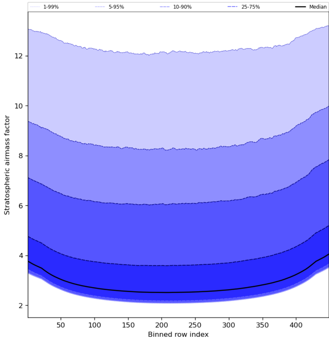
Figure 61: Along track statistics of “Stratospheric airmass factor” for 2023-11-20 to 2023-11-22
