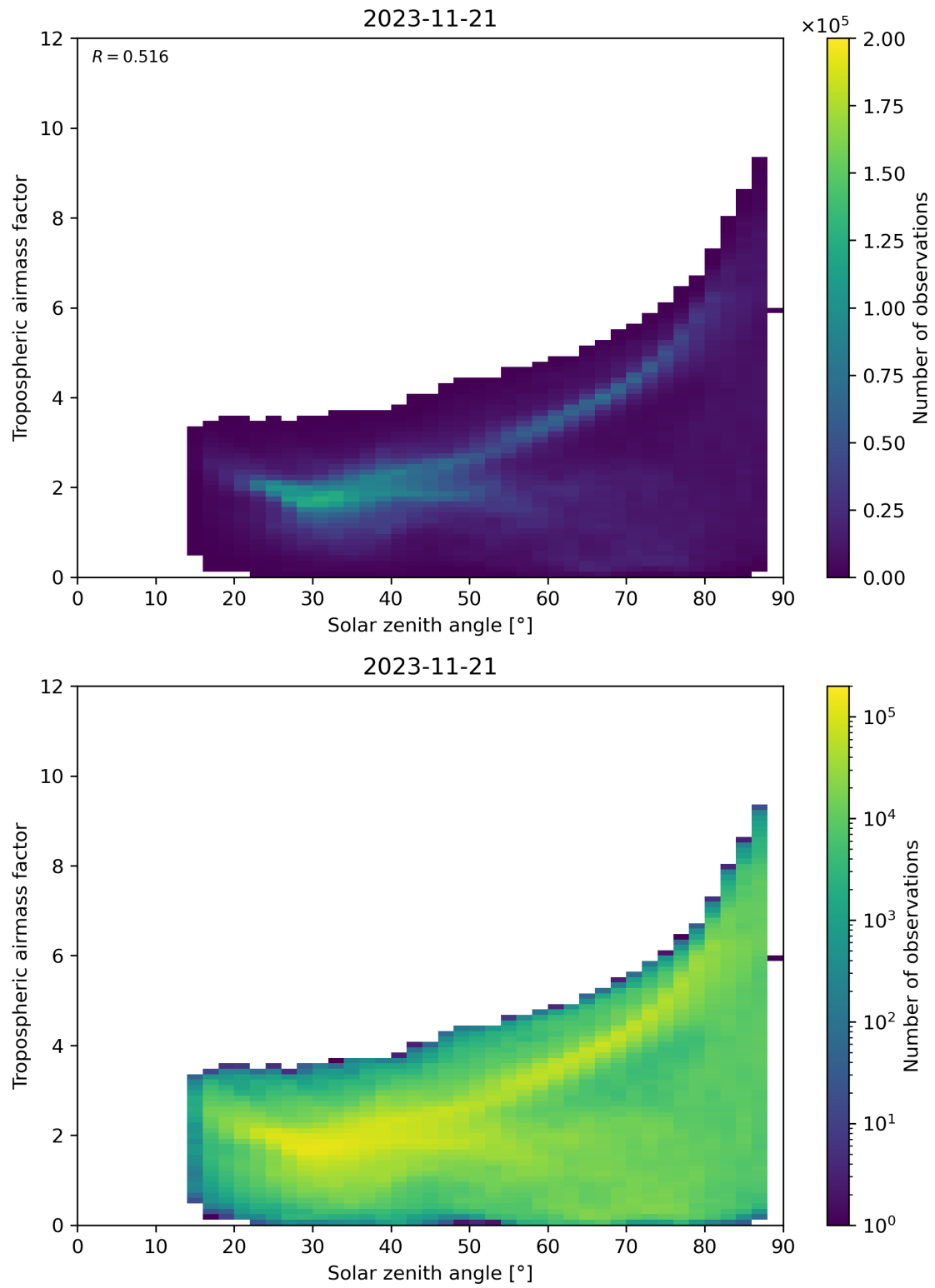
Figure 147: Scatter density plot of “Solar zenith angle” against “Tropospheric airmass factor” for 2023-11-20 to 2023-11-22.
