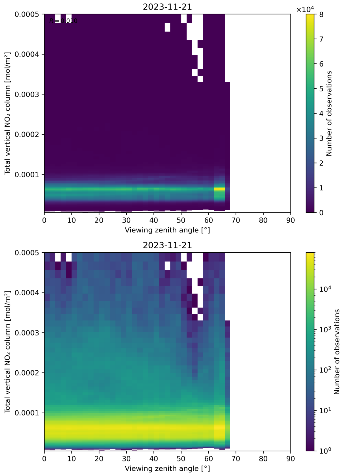
Figure 167: Scatter density plot of “Viewing zenith angle” against “Total vertical NO 2 column” for 2023-11-20 to 2023-11-22.
