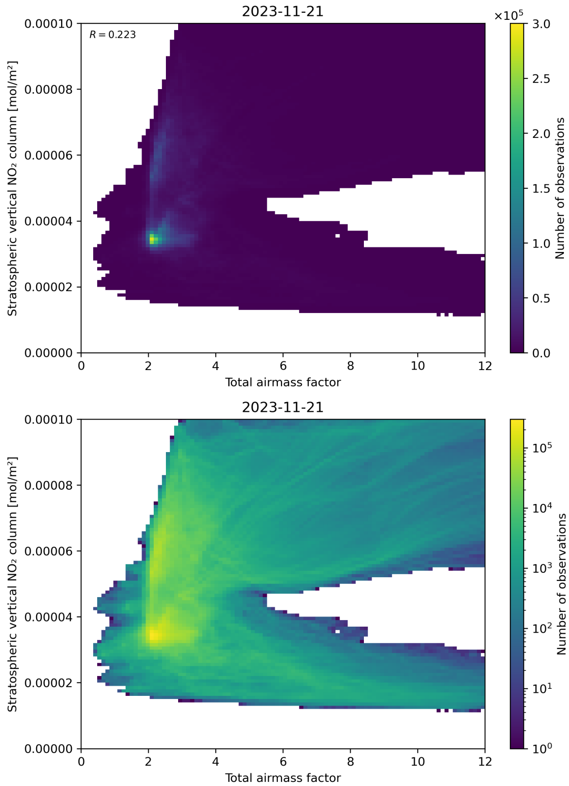
Figure 64: Scatter density plot of “Total airmass factor” against “Stratospheric vertical \text{NO}_2 column” for 2023-11-20 to 2023-11-22.
