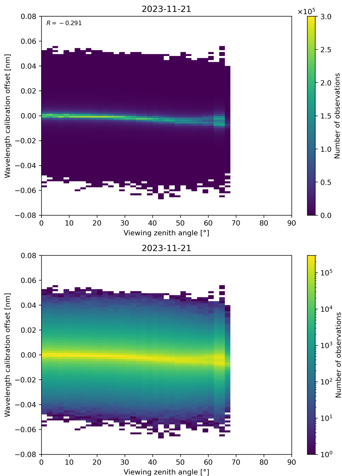
Figure 173: Scatter density plot of “Viewing zenith angle” against “Wavelength calibration offset” for 2023-11-20 to 2023-11-22.
