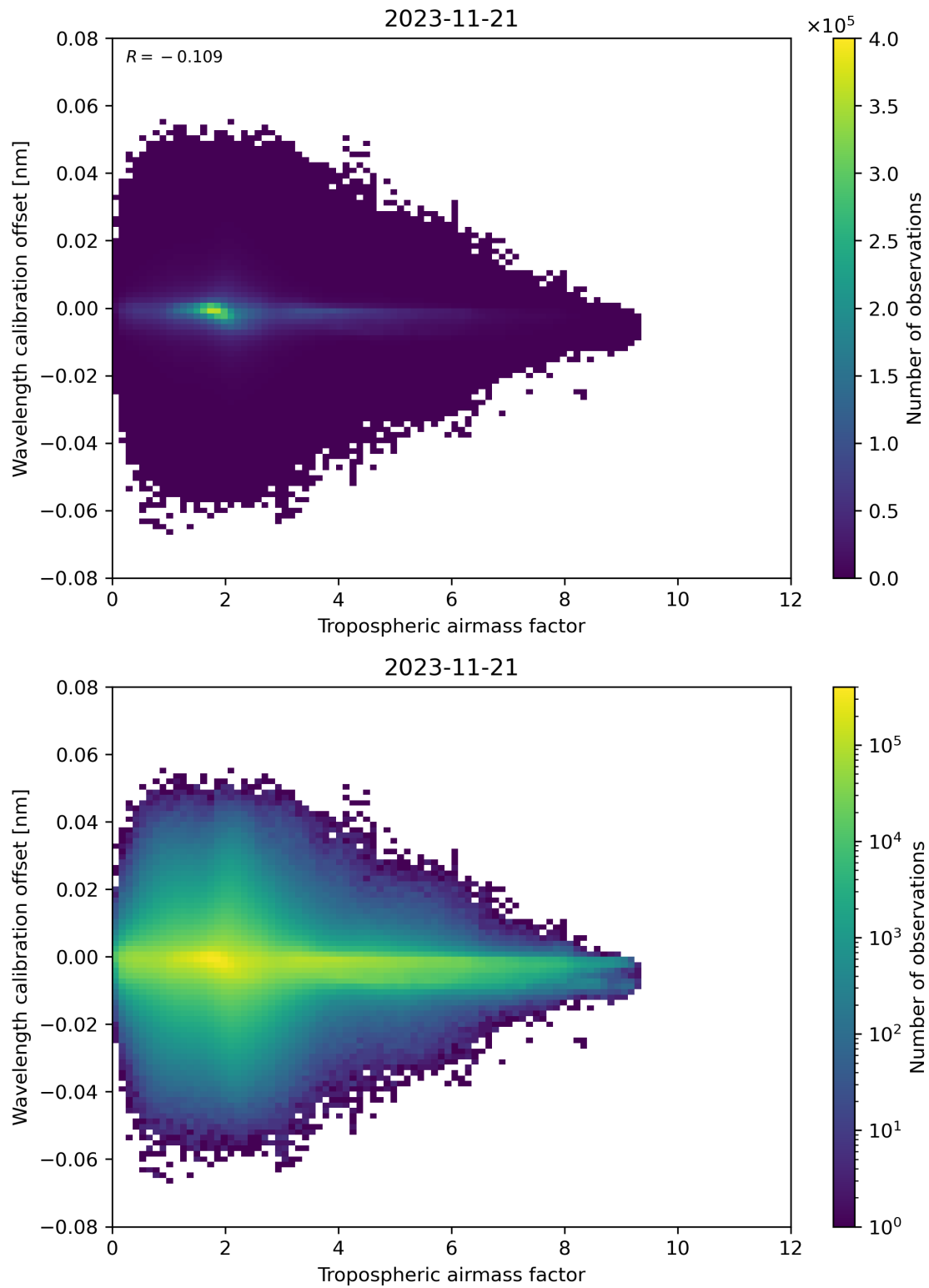
Figure 80: Scatter density plot of “Tropospheric airmass factor” against “Wavelength calibration offset” for 2023-11-20 to 2023-11-22.
