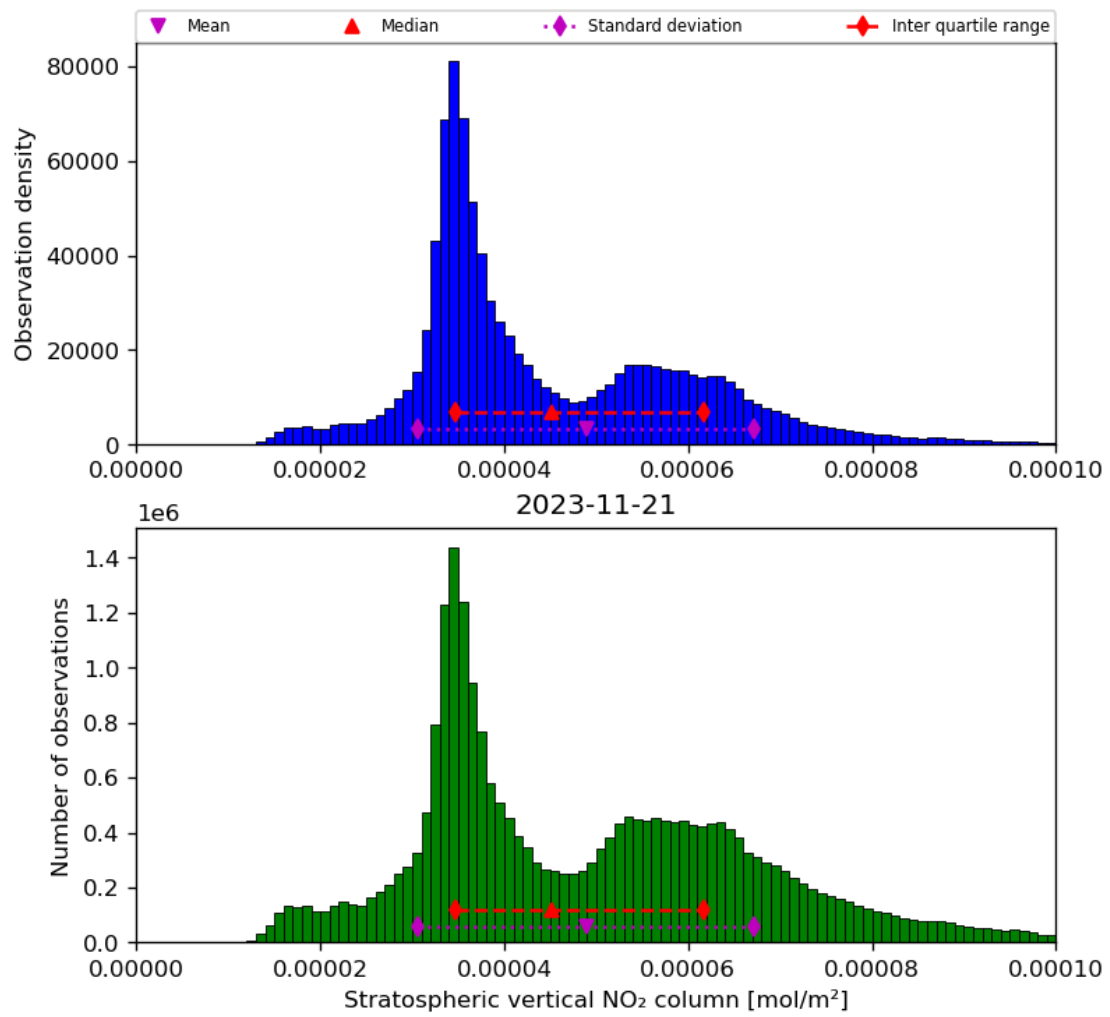
Figure 36: Histogram of “Stratospheric vertical NO 2 column” for 2023-11-20 to 2023-11-22
