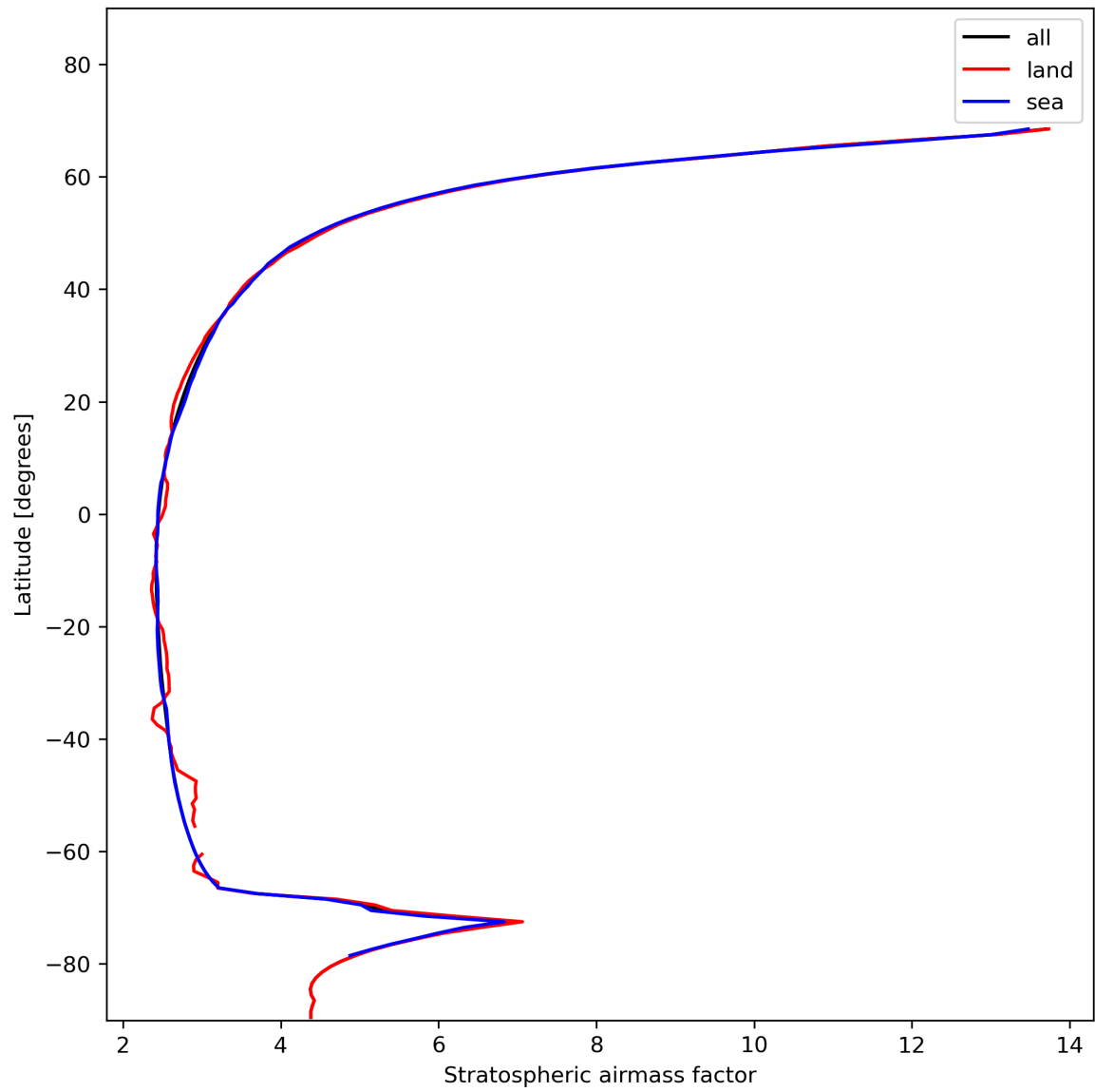
Figure 27: Zonal average of “Stratospheric airmass factor” for 2023-11-20 to 2023-11-22.
