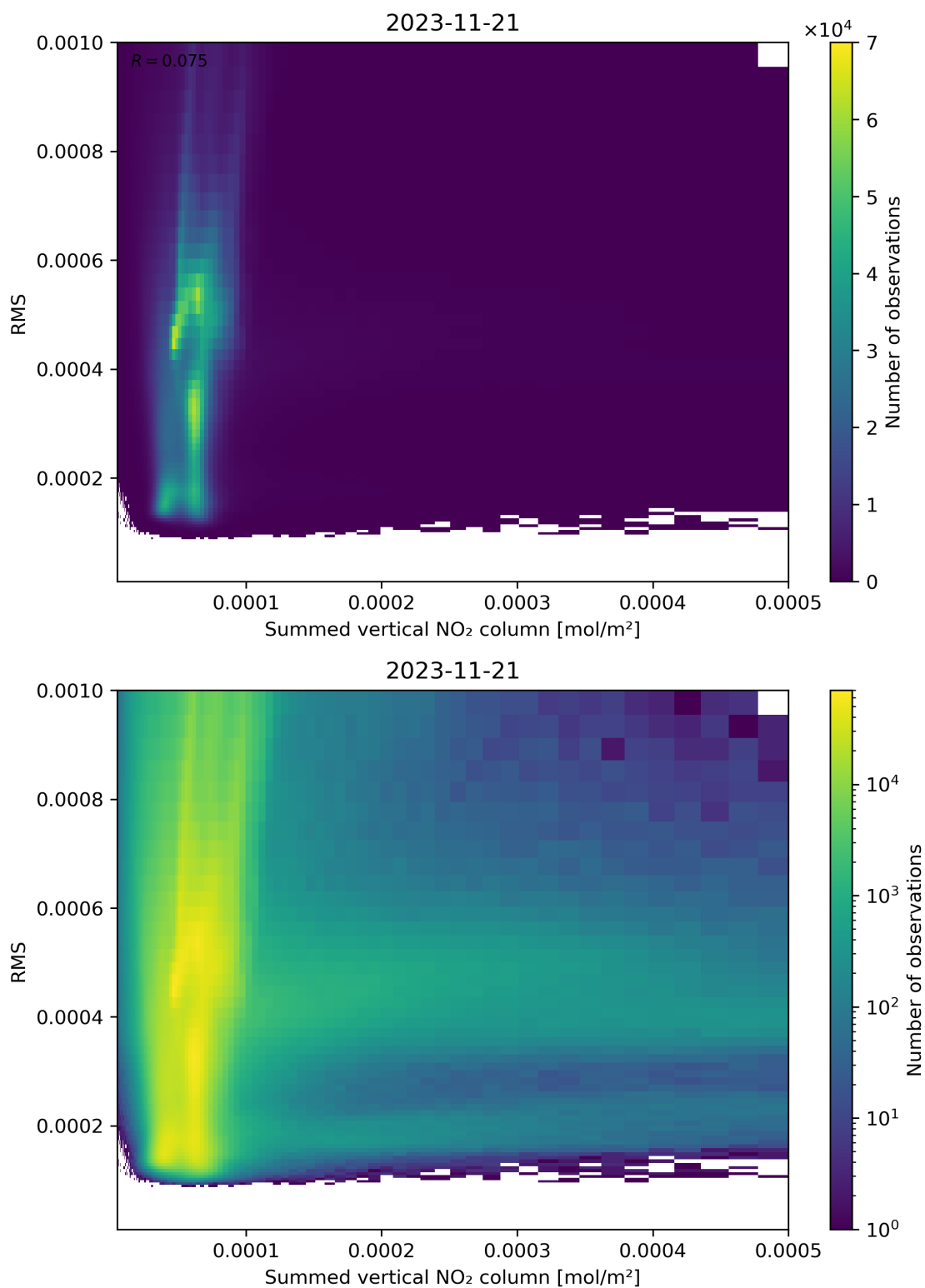
Figure 109: Scatter density plot of “Summed vertical NO 2 column” against “RMS” for 2023-11-20 to 2023-11-22.
