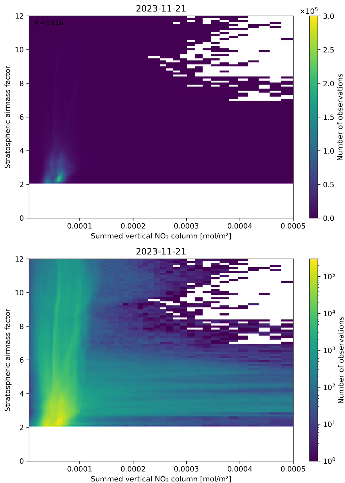
Figure 103: Scatter density plot of “Summed vertical NO 2 column” against “Stratospheric air mass factor” for 2023-11-20 to 2023-11-22.
