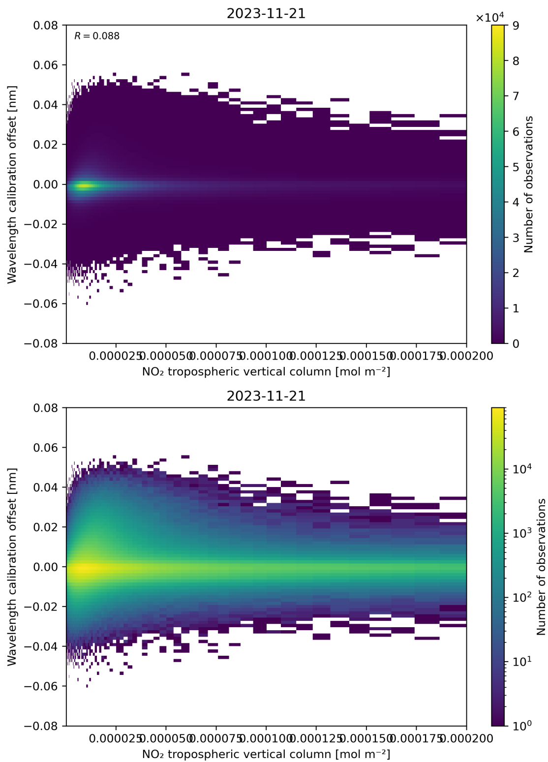
Figure 143: Scatter density plot of “NO 2 tropospheric vertical column” against “Wavelength calibration offset” for 2023-11-20 to 2023-11-22.
