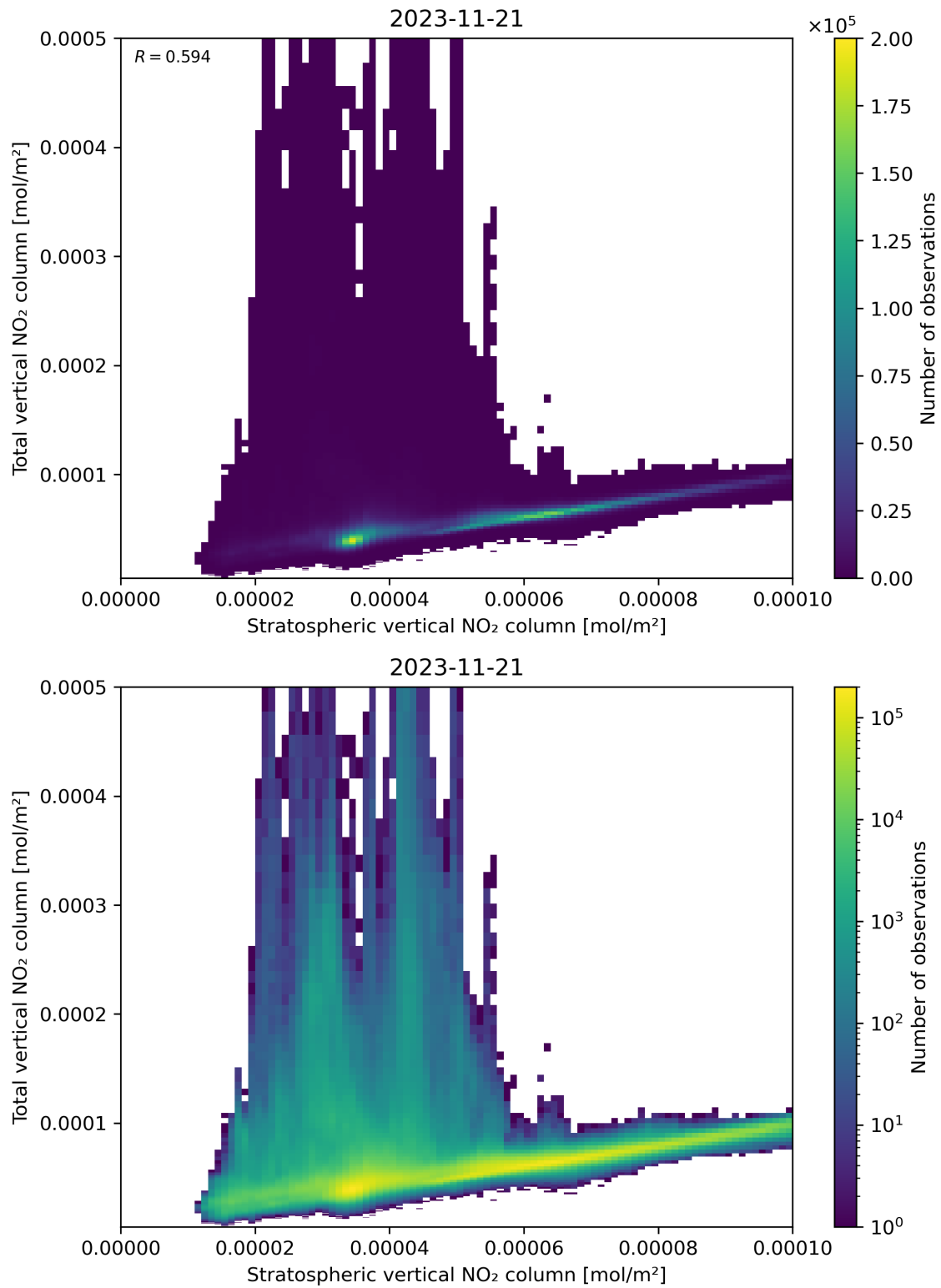
Figure 100: Scatter density plot of “Stratospheric vertical NO 2 column” against “Total vertical NO 2 column” for 2023-11-20 to 2023-11-22.
