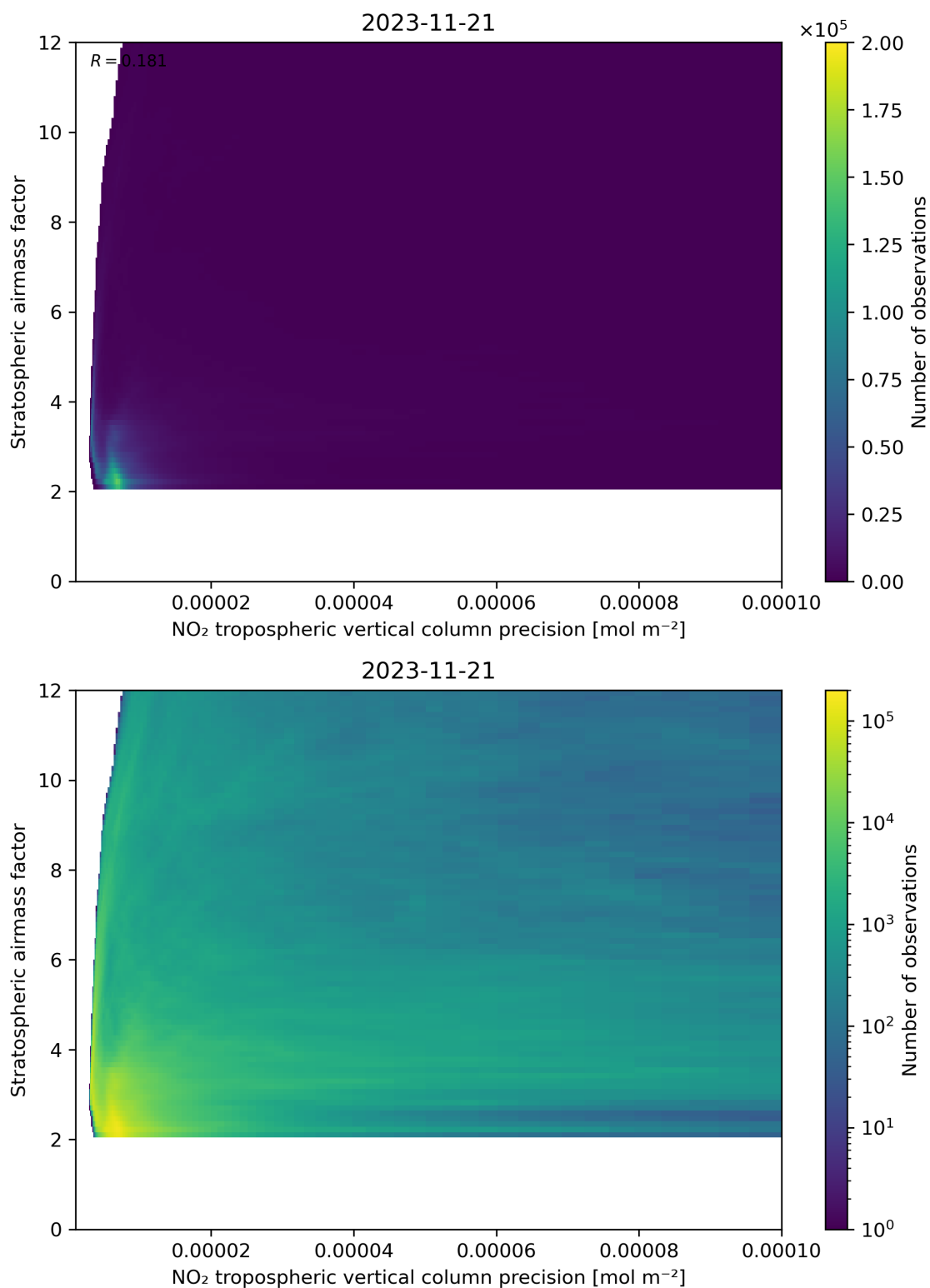
Figure 131: Scatter density plot of “NO 2 tropospheric vertical column precision” against “Stratospheric airmass factor” for 2023-11-20 to 2023-11-22.
