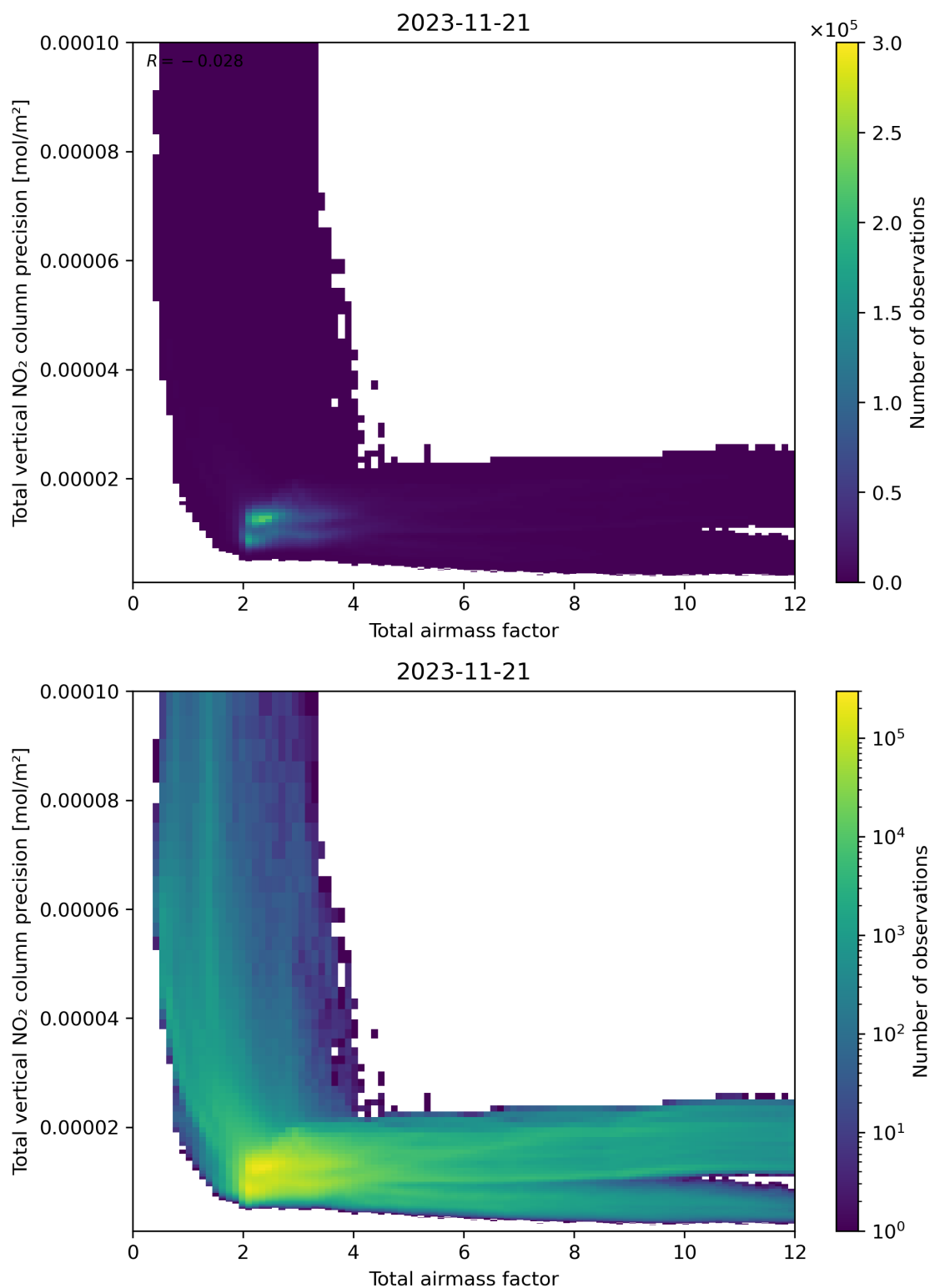
Figure 68: Scatter density plot of “Total airmass factor” against “Total vertical NO 2 column precision” for 2023-11-20 to 2023-11-22.
