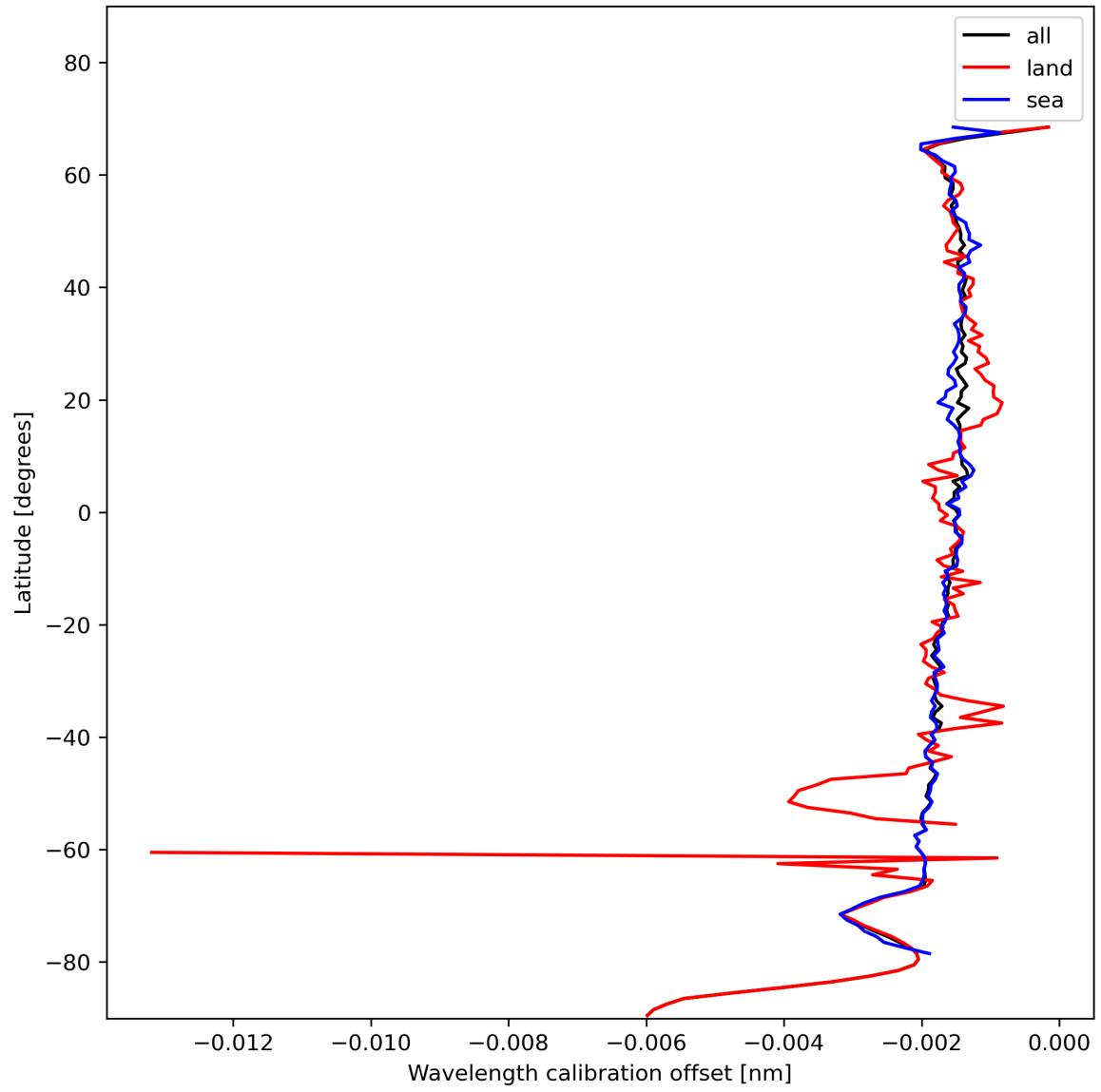
Figure 18: Zonal average of “Wavelength calibration offset” for 2023-11-20 to 2023-11-22.
