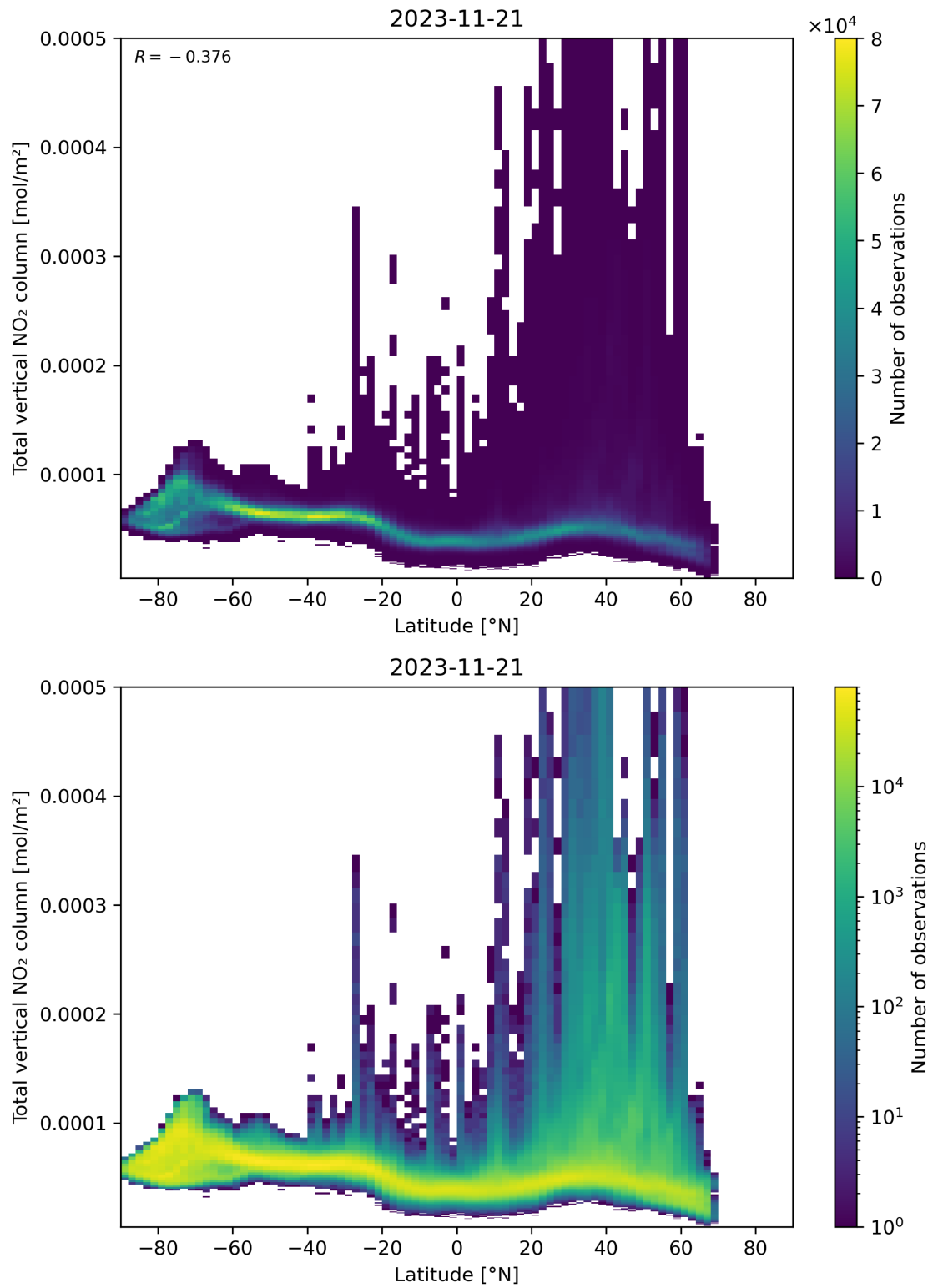
Figure 90: Scatter density plot of “Latitude” against “Total vertical NO 2 column” for 2023-11-20 to 2023-11-22.
