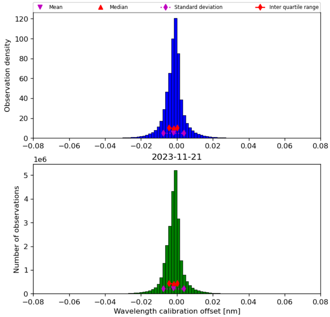
Figure 35: Histogram of “Wavelength calibration offset” for 2023-11-20 to 2023-11-22
