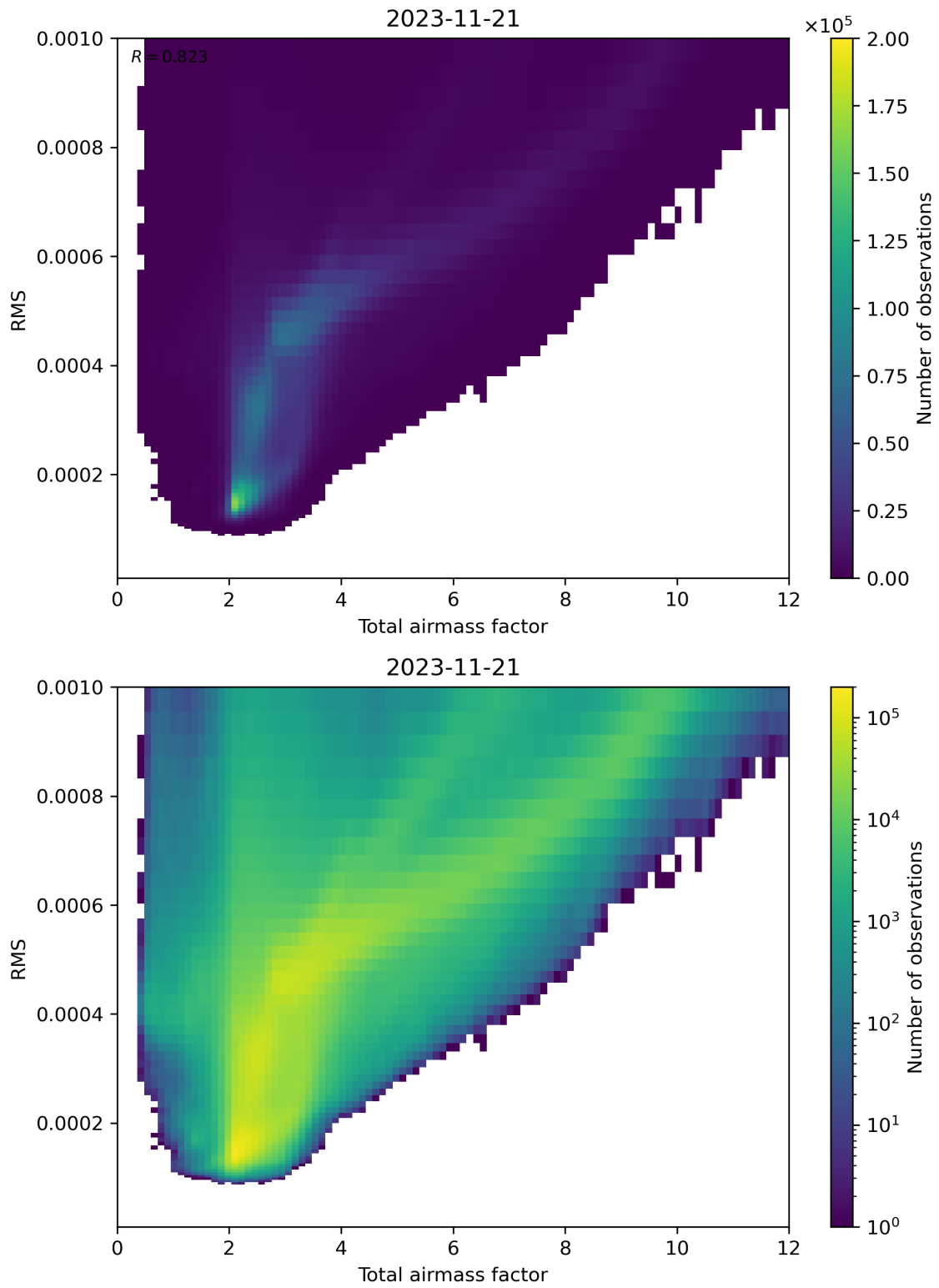
Figure 69: Scatter density plot of “Total airmass factor” against “RMS” for 2023-11-20 to 2023-11-22.
