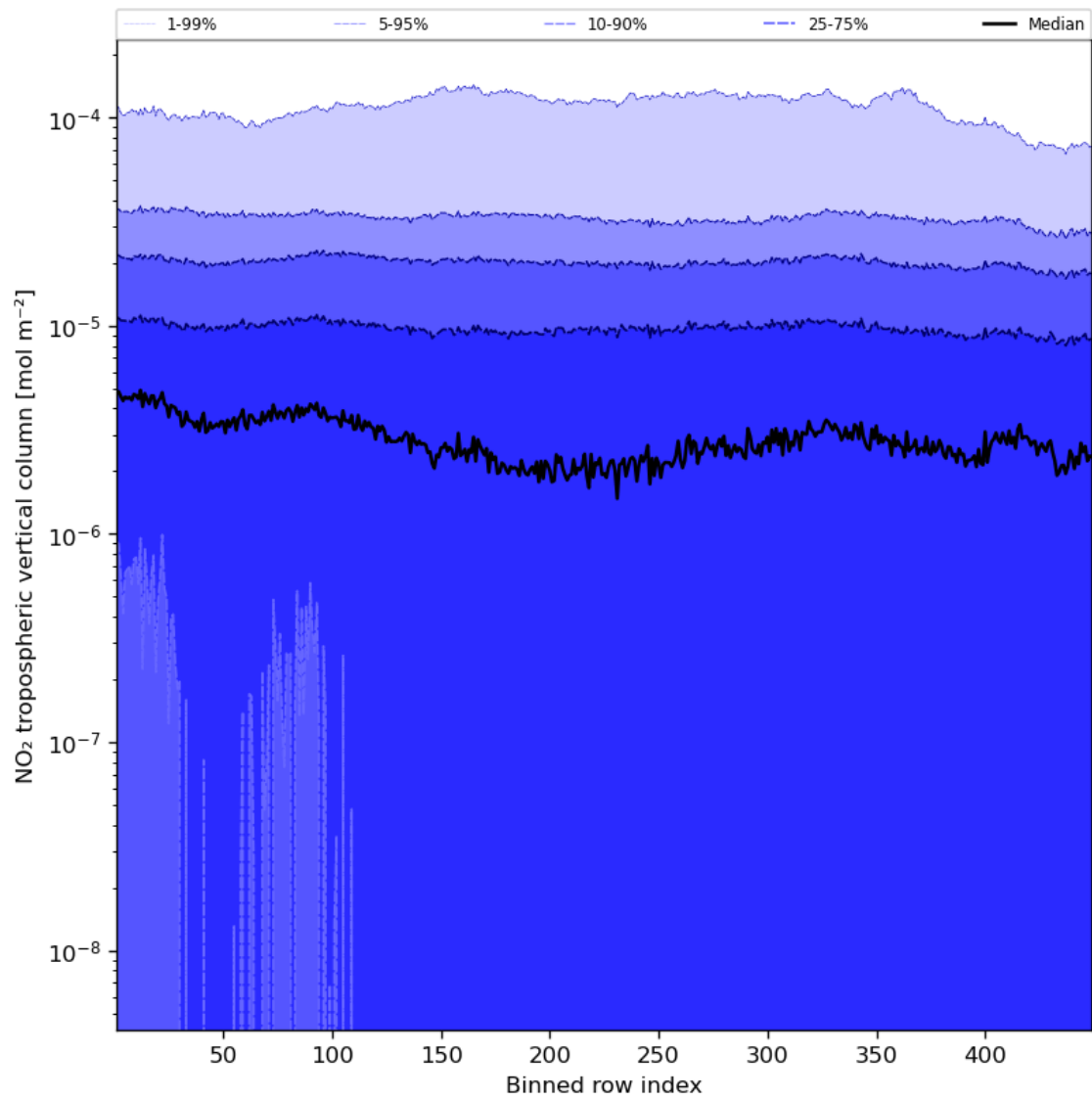
Figure 46: Along track statistics of “NO 2 tropospheric vertical column” for 2023-11-20 to 2023-11-22
