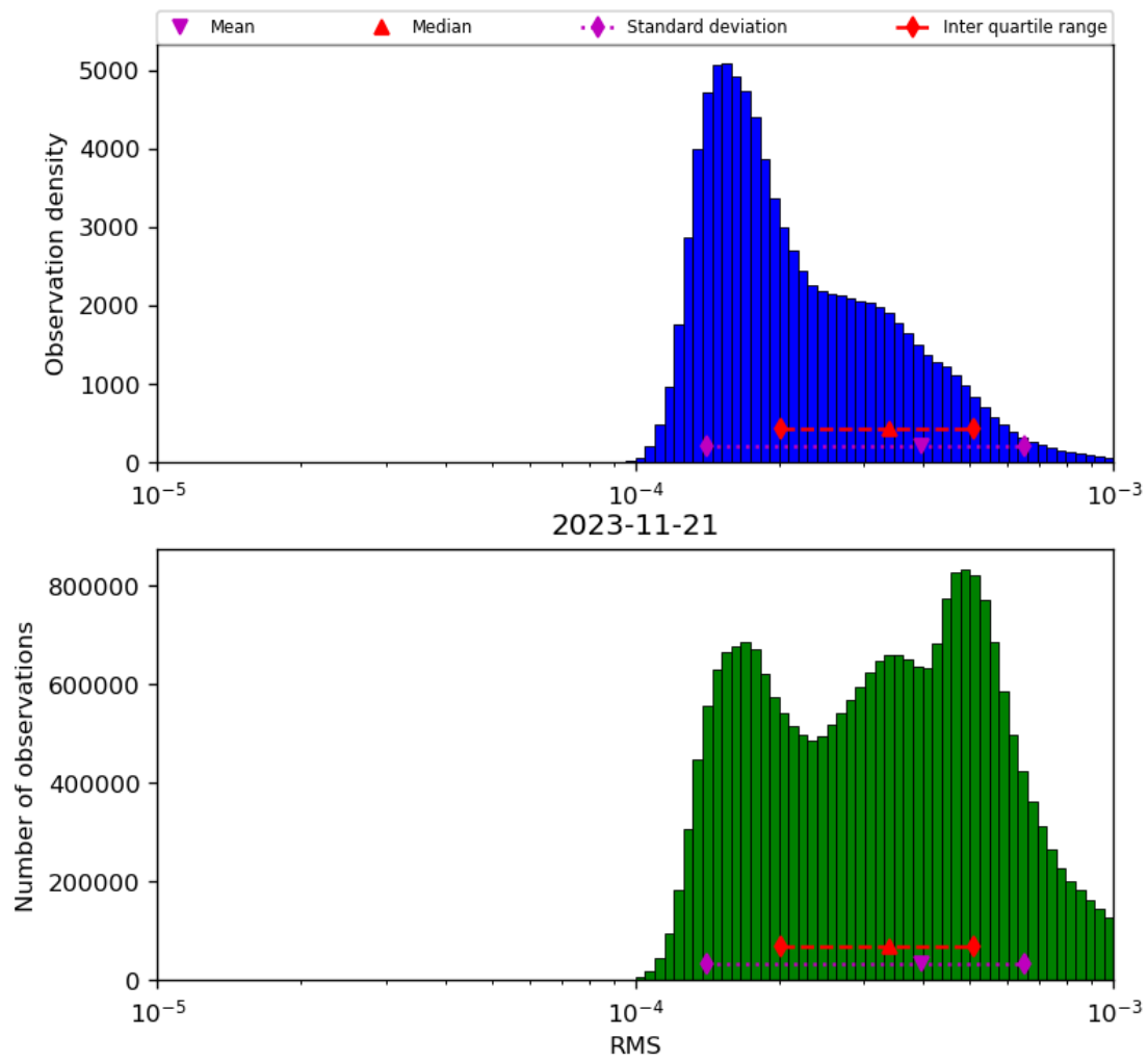
Figure 43: Histogram of “RMS” for 2023-11-20 to 2023-11-22
