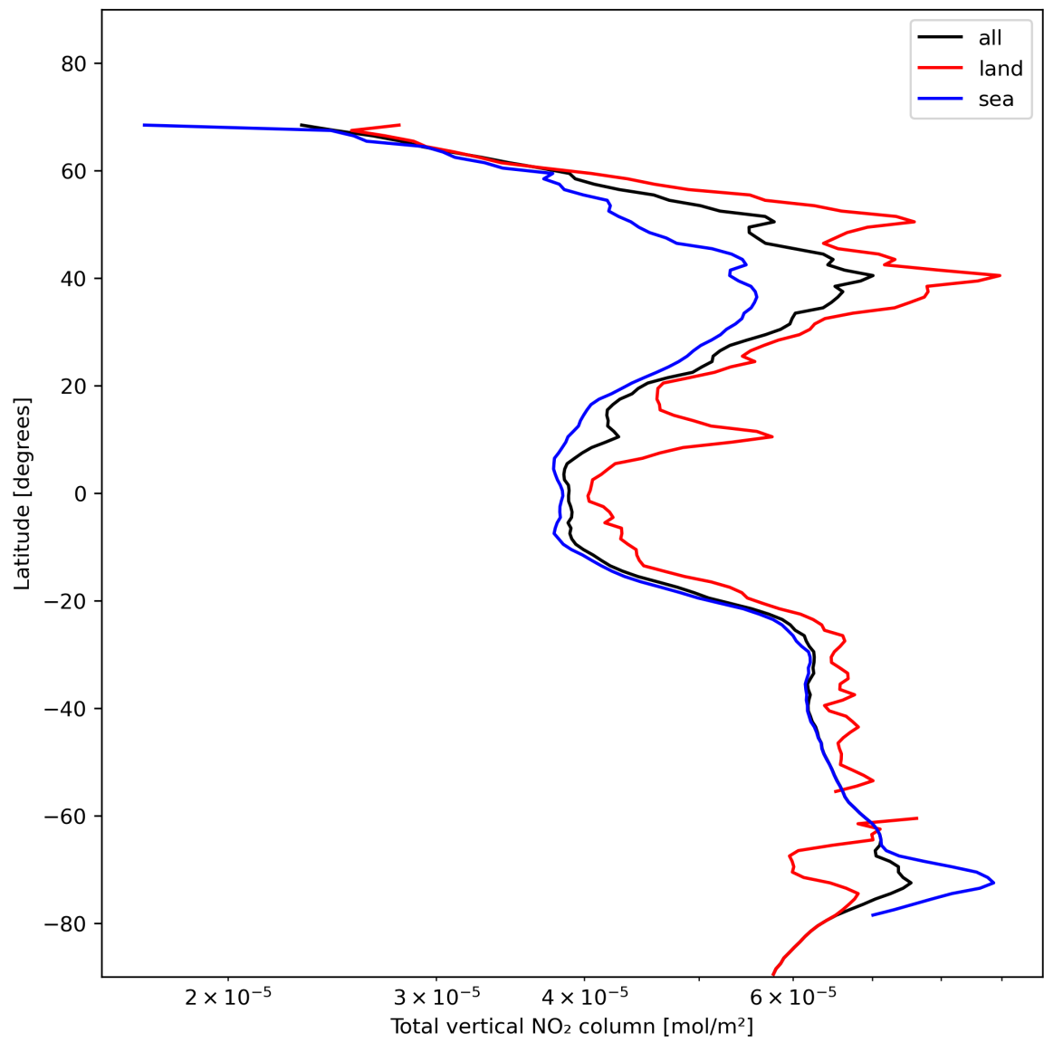
Figure 21: Zonal average of “Total vertical NO 2 column” for 2023-11-20 to 2023-11-22.
