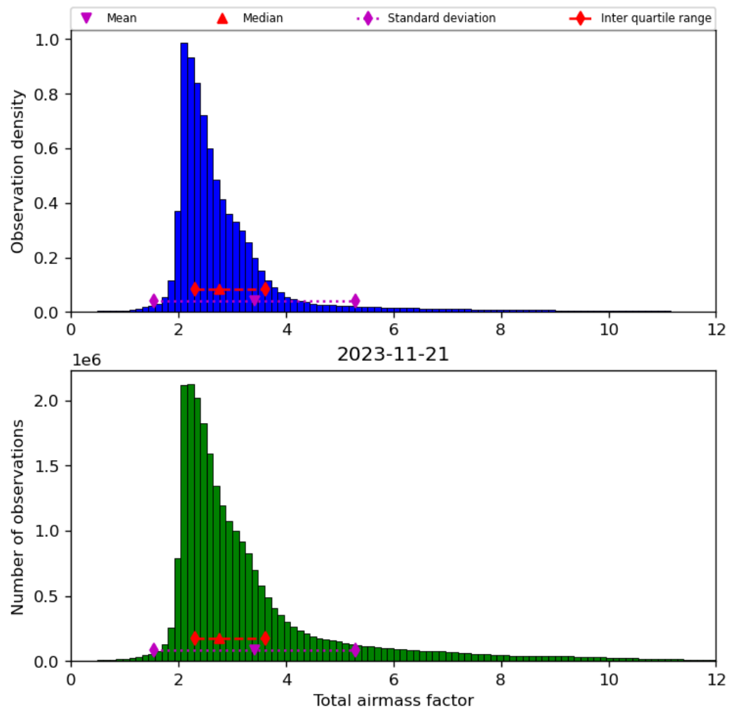
Figure 32: Histogram of “Total airmass factor” for 2023-11-20 to 2023-11-22
