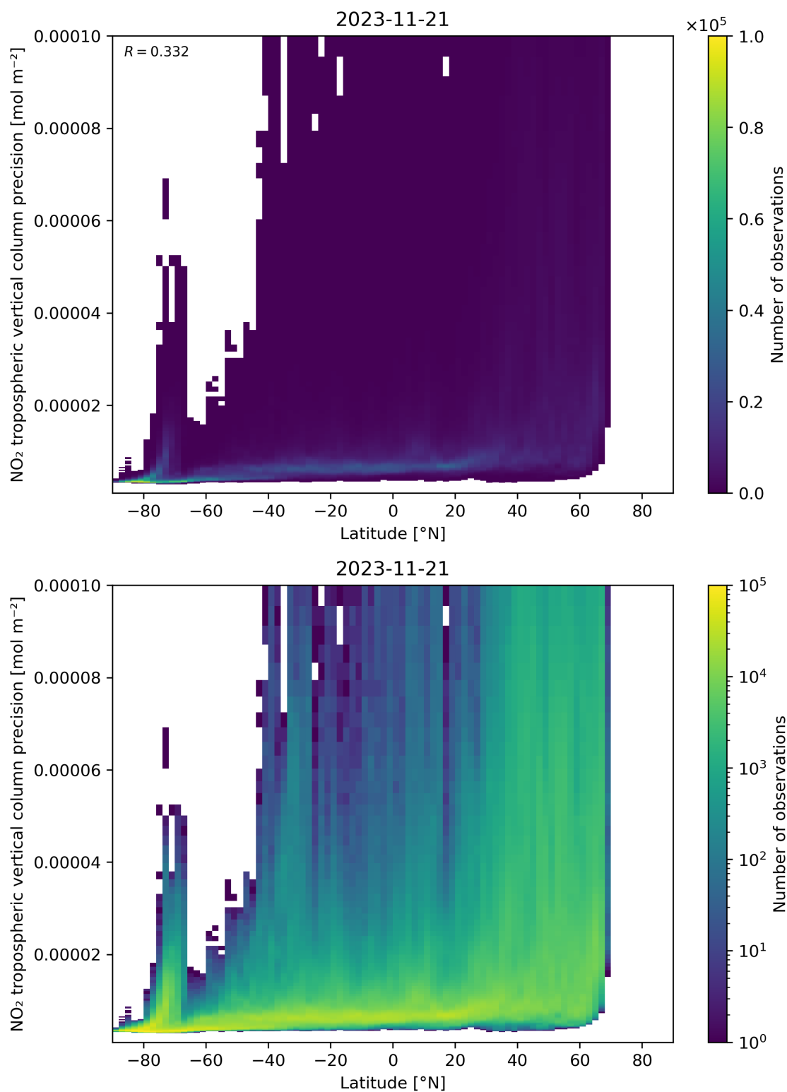
Figure 93: Scatter density plot of “Latitude” against “NO 2 tropospheric vertical column precision” for 2023-11-20 to 2023-11-22.
