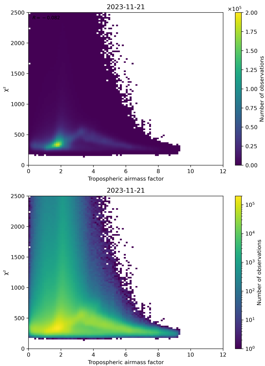
Figure 73: Scatter density plot of “Tropospheric airmass factor” against “ \chi^2 ” for 2023-11-20 to 2023-11-22.
