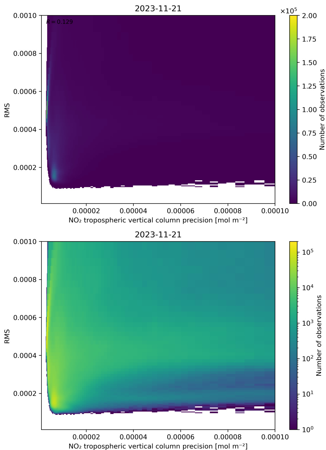
Figure 140: Scatter density plot of “NO 2 tropospheric vertical column precision” against “RMS” for 2023-11-20 to 2023-11-22.
