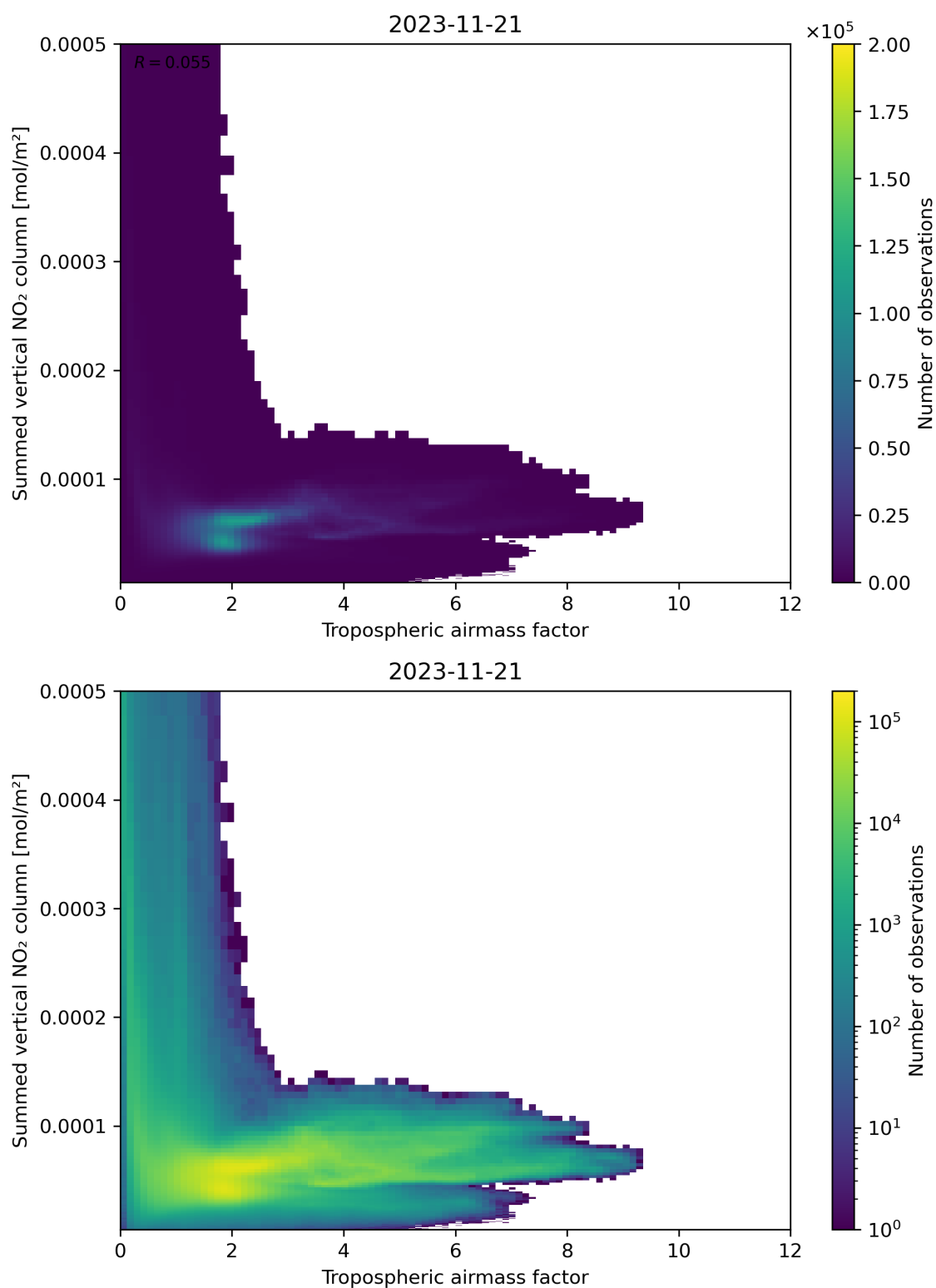
Figure 75: Scatter density plot of “Tropospheric airmass factor” against “Summed vertical NO 2 column” for 2023-11-20 to 2023-11-22.
