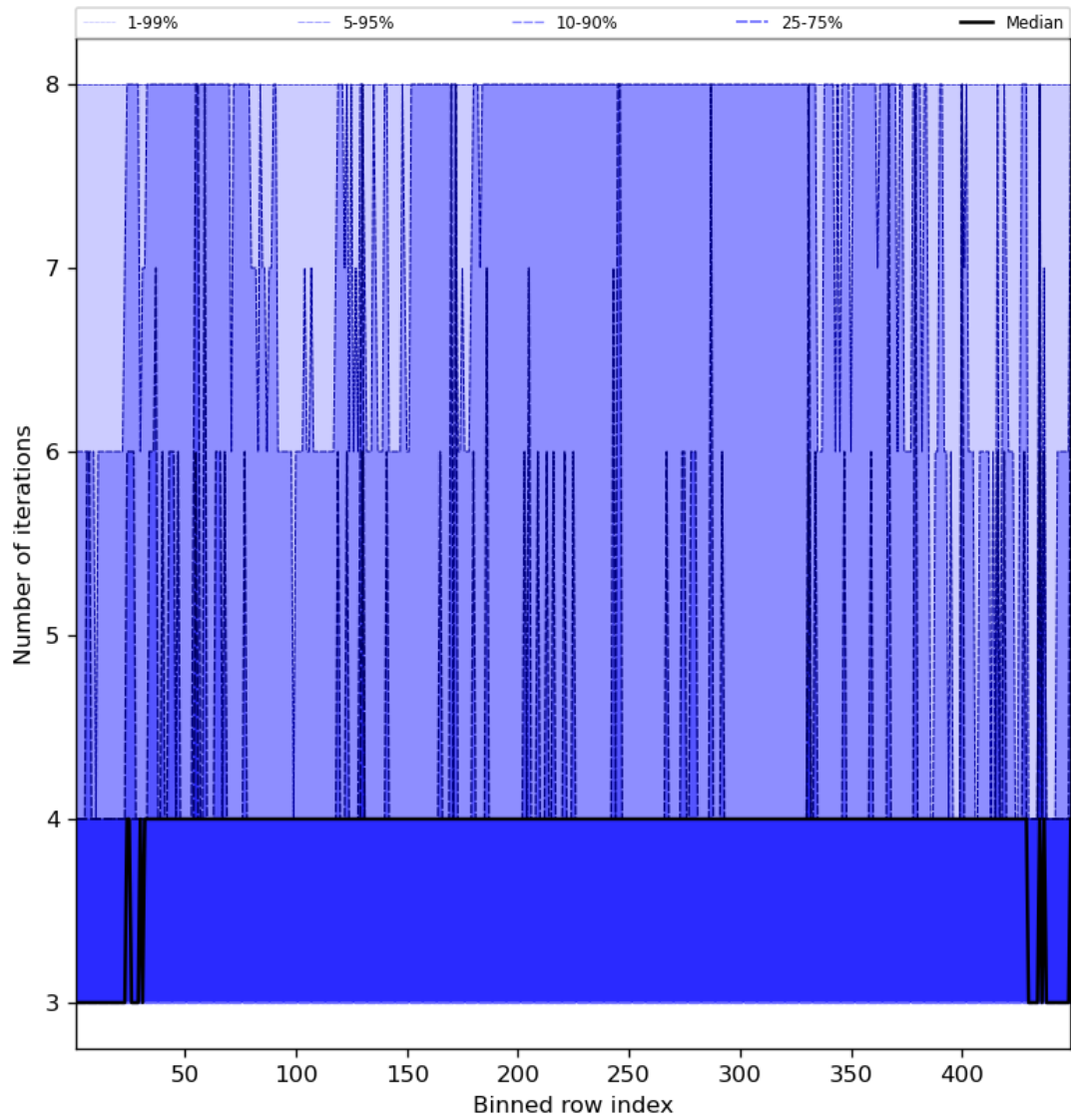
Figure 51: Along track statistics of “Number of iterations” for 2023-11-20 to 2023-11-22
