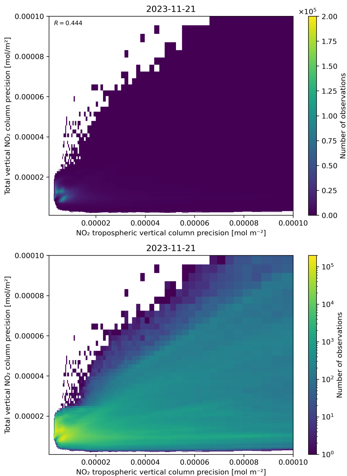
Figure 139: Scatter density plot of “NO 2 tropospheric vertical column precision” against “Total vertical NO 2 column precision” for 2023-11-20 to 2023-11-22.
