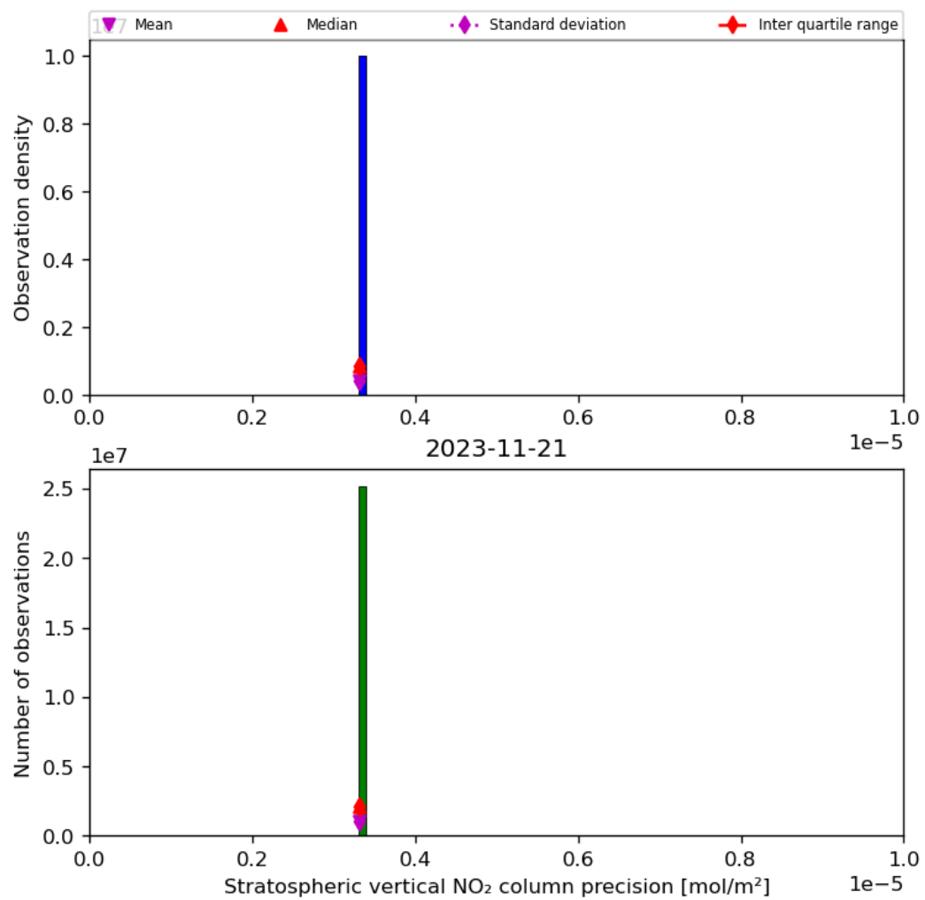
Figure 37: Histogram of “Stratospheric vertical NO 2 column precision” for 2023-11-20 to 2023-11-22
