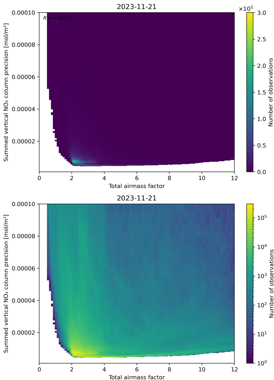
Figure 66: Scatter density plot of “Total airmass factor” against “Summed vertical NO 2 column precision” for 2023-11-20 to 2023-11-22.
