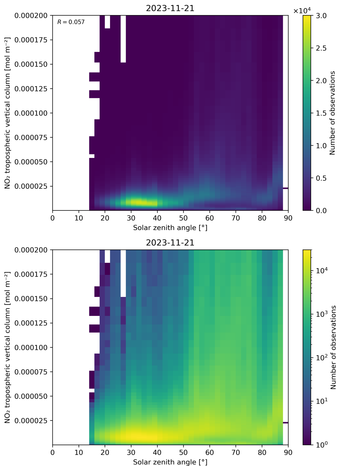
Figure 155: Scatter density plot of “Solar zenith angle” against “NO 2 tropospheric vertical column” for 2023-11-20 to 2023-11-22.
