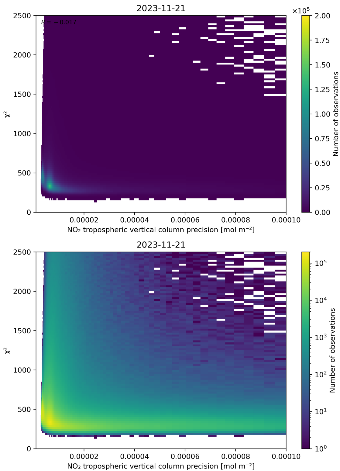
Figure 134: Scatter density plot of “NO 2 tropospheric vertical column precision” against “ \chi^2 ” for 2023-11-20 to 2023-11-22.
