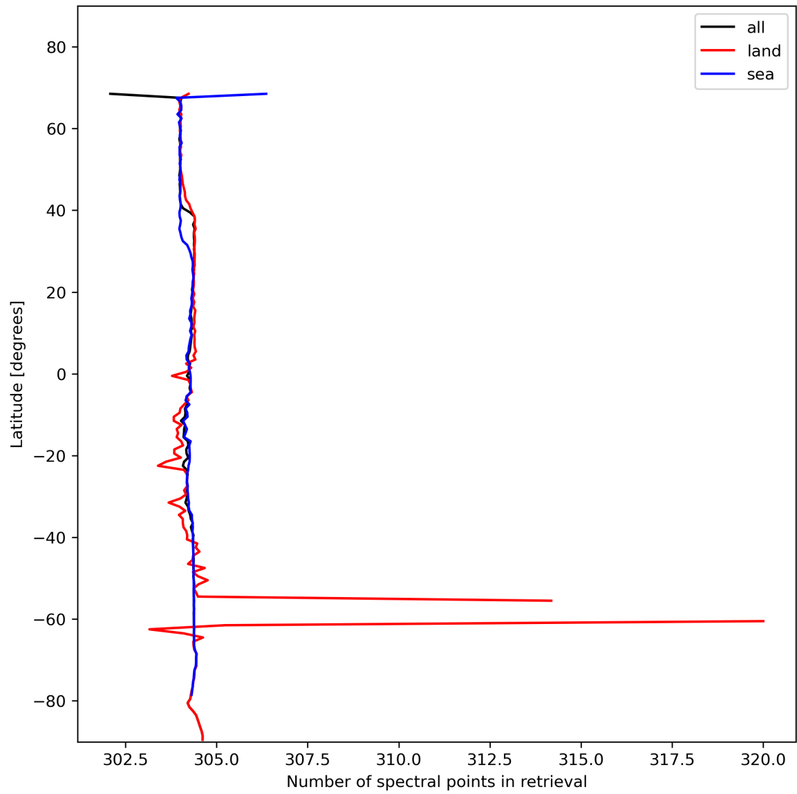
Figure 16: Zonal average of “Number of spectral points in retrieval” for 2023-11-20 to 2023-11-22.
