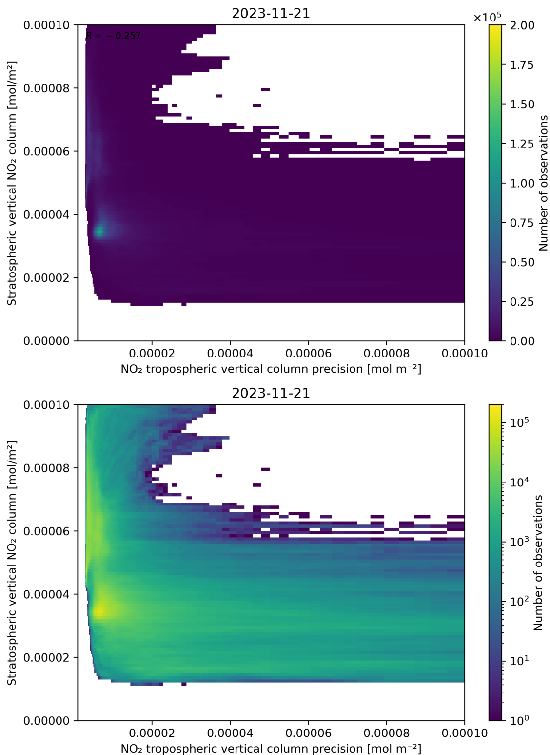
Figure 135: Scatter density plot of “NO 2 tropospheric vertical column precision” against “Stratospheric vertical NO 2 column” for 2023-11-20 to 2023-11-22.
