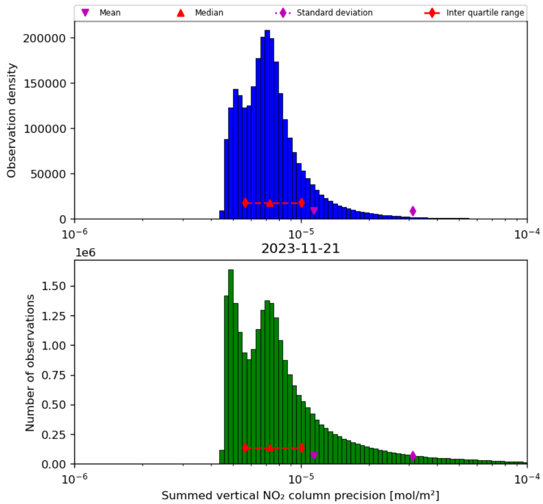
Figure 41: Histogram of “Summed vertical NO 2 column precision” for 2023-11-20 to 2023-11-22
