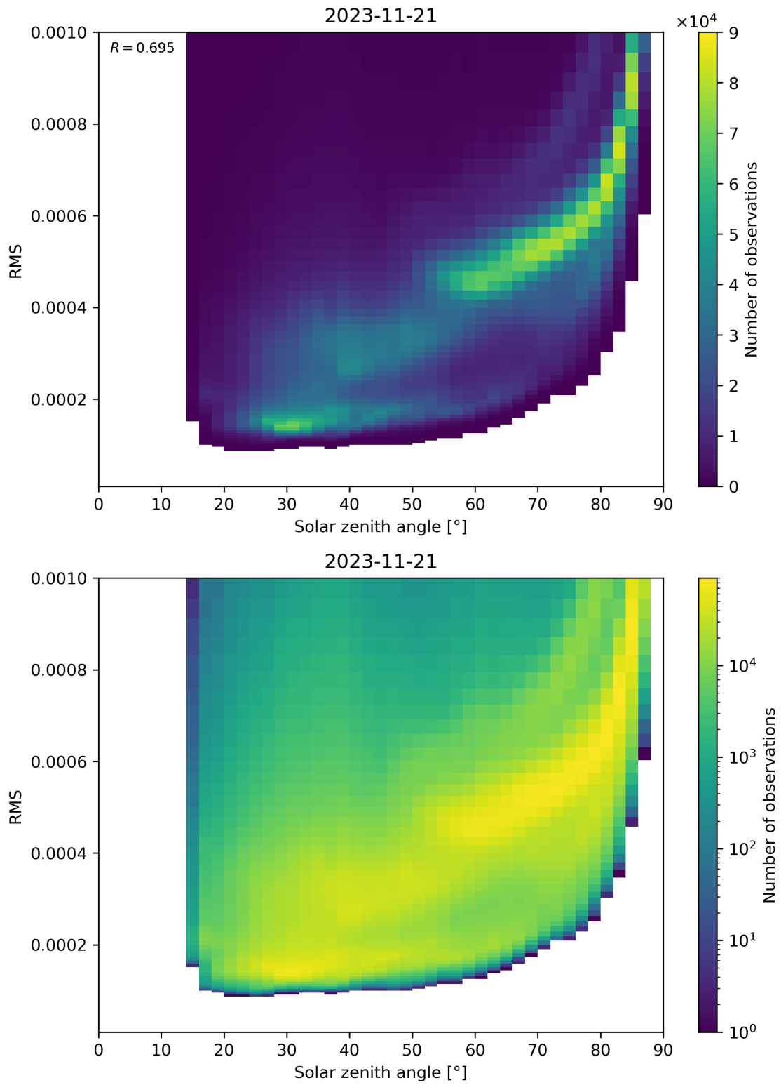
Figure 157: Scatter density plot of “Solar zenith angle” against “RMS” for 2023-11-20 to 2023-11-22.
