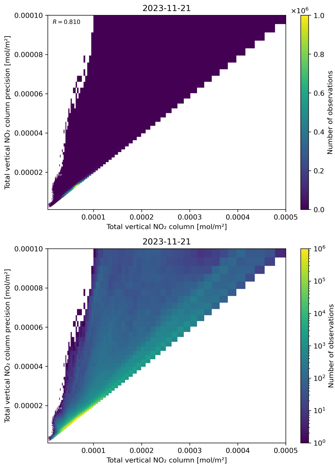
Figure 114: Scatter density plot of “Total vertical NO 2 column” against “Total vertical NO 2 column precision” for 2023-11-20 to 2023-11-22.
