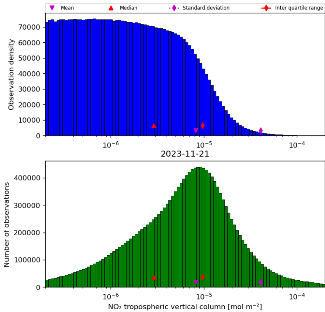
Figure 29: Histogram of “NO 2 tropospheric vertical column” for 2023-11-20 to 2023-11-22
