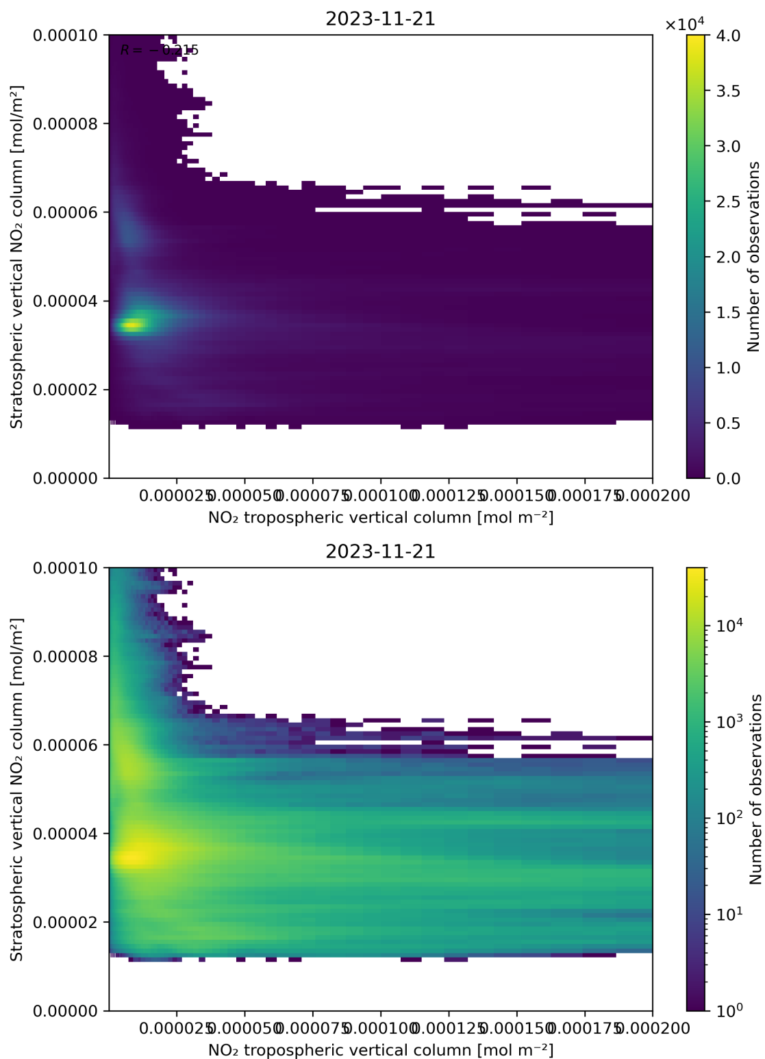
Figure 125: Scatter density plot of “NO 2 tropospheric vertical column” against “Stratospheric vertical NO 2 column” for 2023-11-20 to 2023-11-22.
