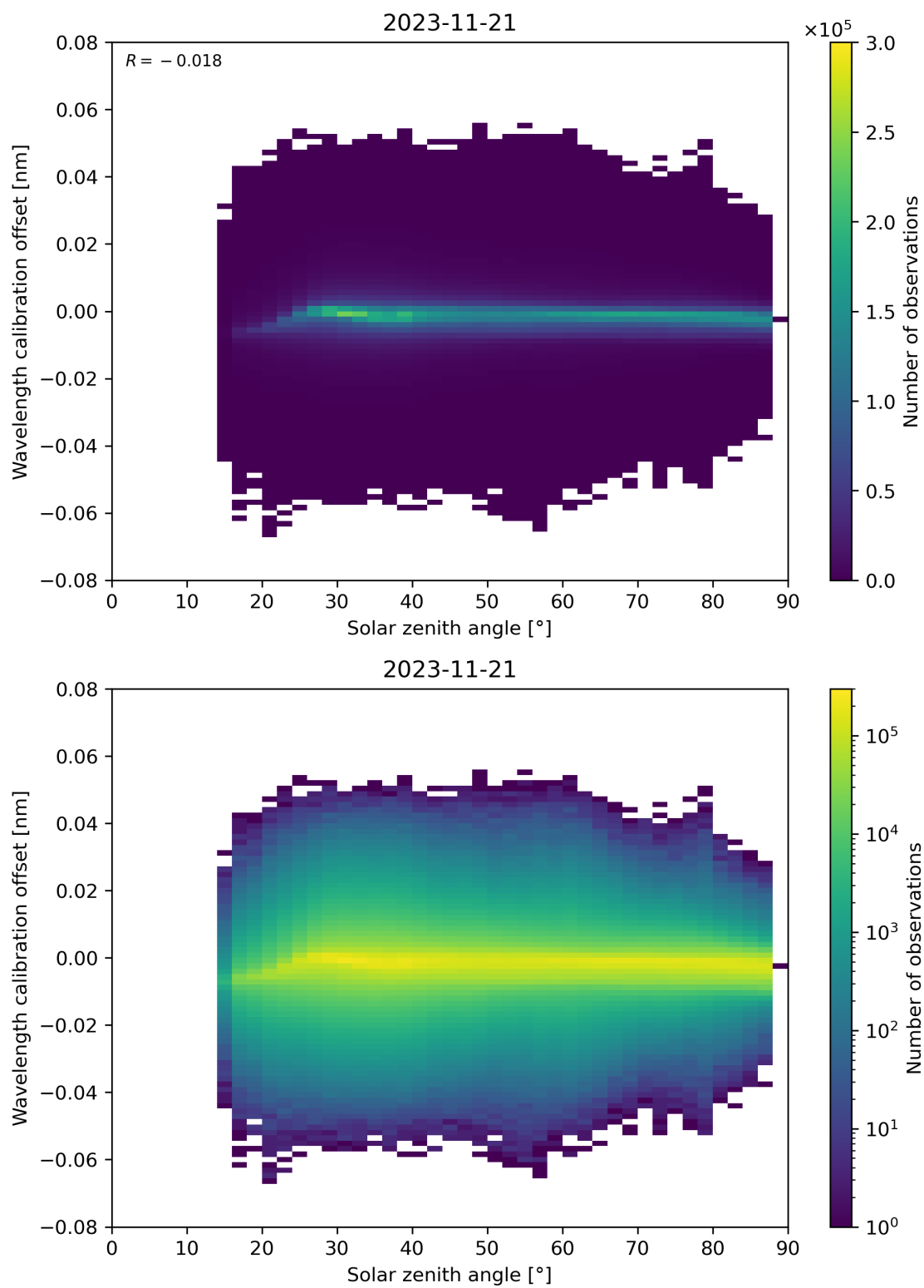
Figure 158: Scatter density plot of “Solar zenith angle” against “Wavelength calibration offset” for 2023-11-20 to 2023-11-22.
