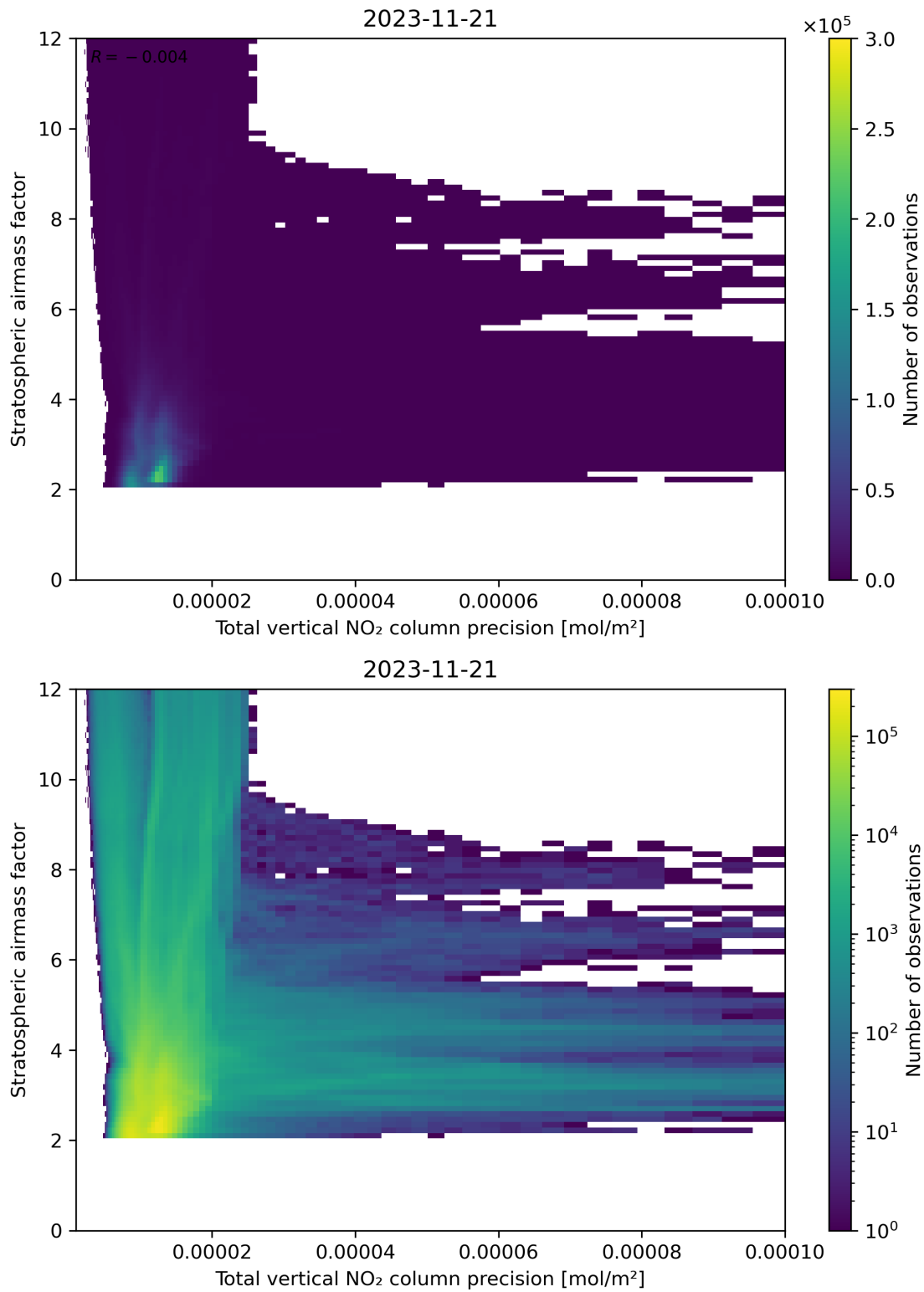
Figure 115: Scatter density plot of “Total vertical NO 2 column precision” against “Stratospheric air mass factor” for 2023-11-20 to 2023-11-22.
