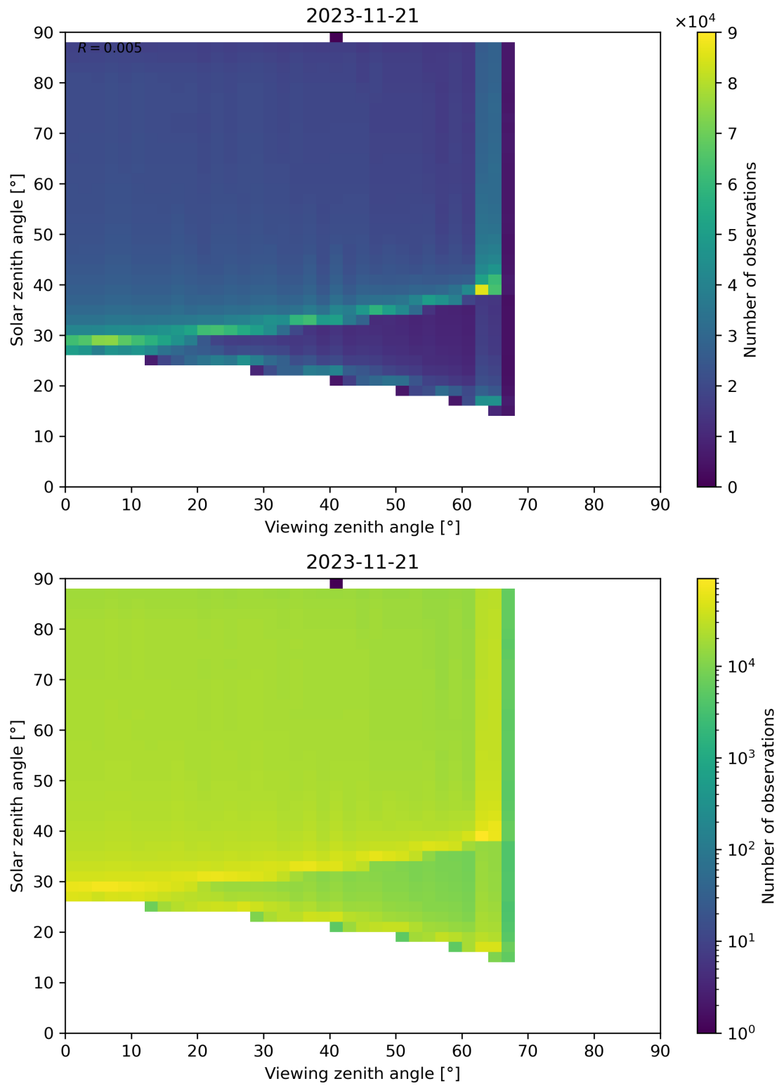
Figure 172: Scatter density plot of “Viewing zenith angle” against “Solar zenith angle” for 2023-11-20 to 2023-11-22.
