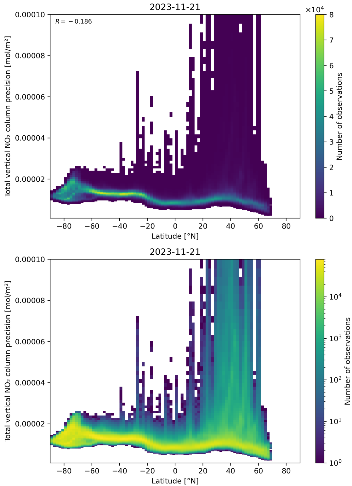
Figure 91: Scatter density plot of “Latitude” against “Total vertical NO 2 column precision” for 2023-11-20 to 2023-11-22.
