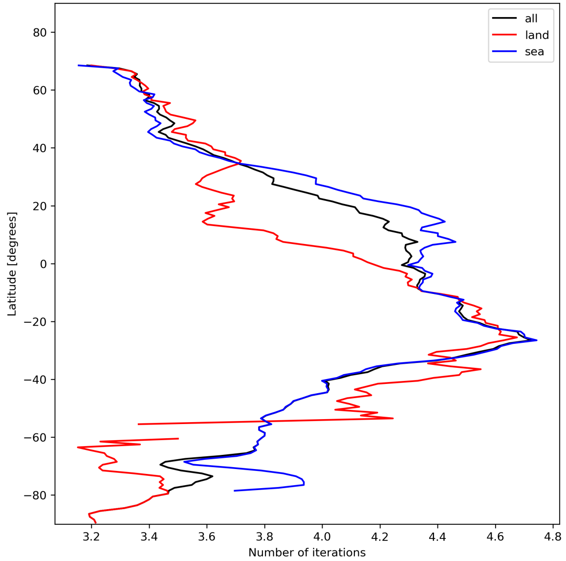
Figure 17: Zonal average of “Number of iterations” for 2023-11-20 to 2023-11-22.
