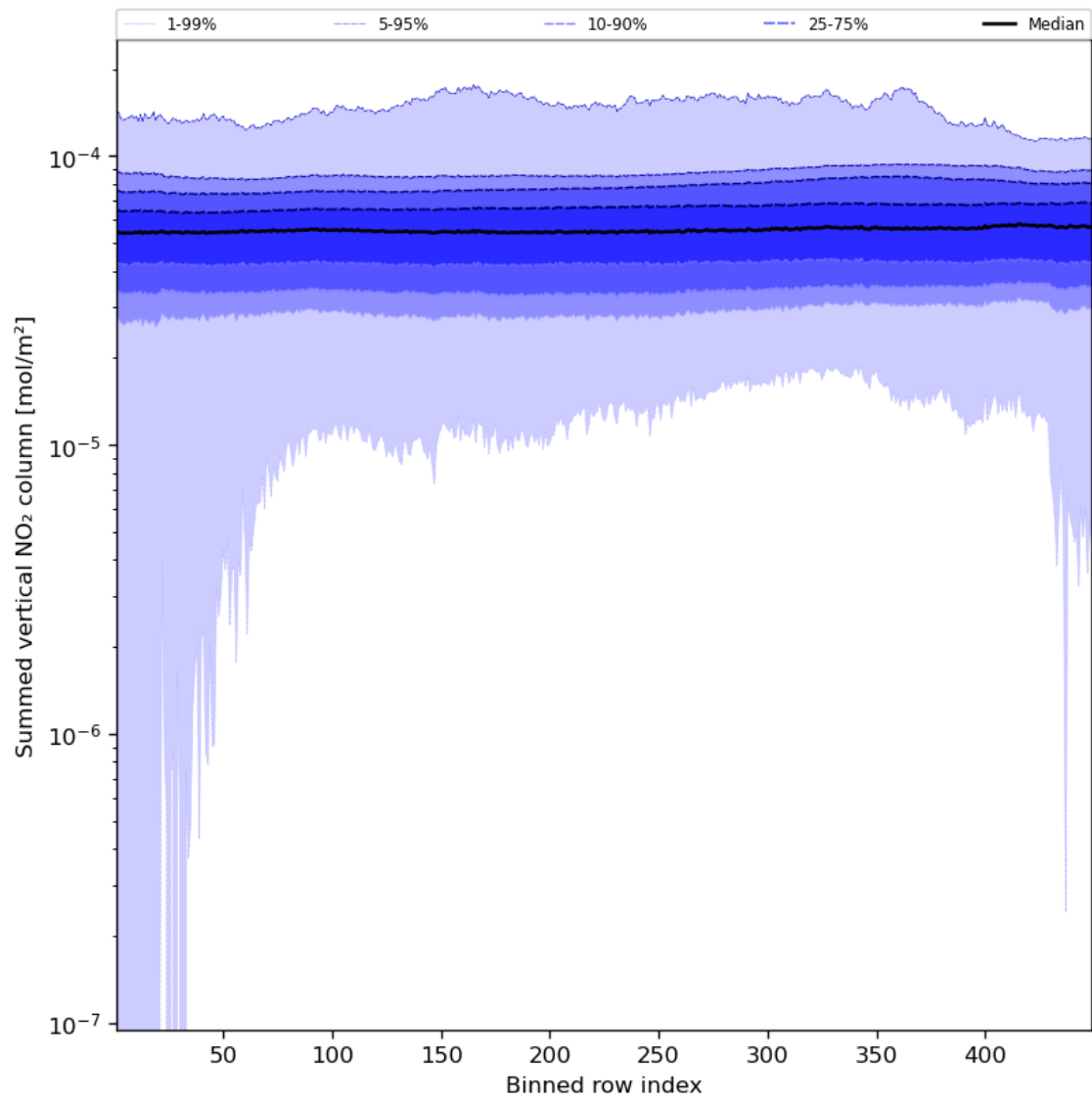
Figure 57: Along track statistics of “Summed vertical NO 2 column” for 2023-11-20 to 2023-11-22
