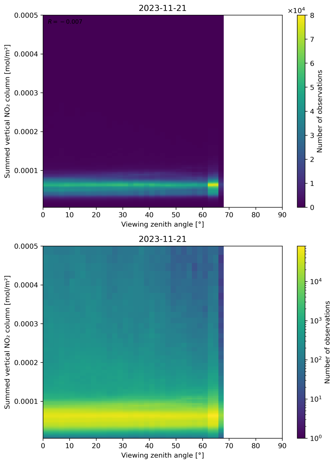
Figure 165: Scatter density plot of “Viewing zenith angle” against “Summed vertical NO 2 column” for 2023-11-20 to 2023-11-22.
