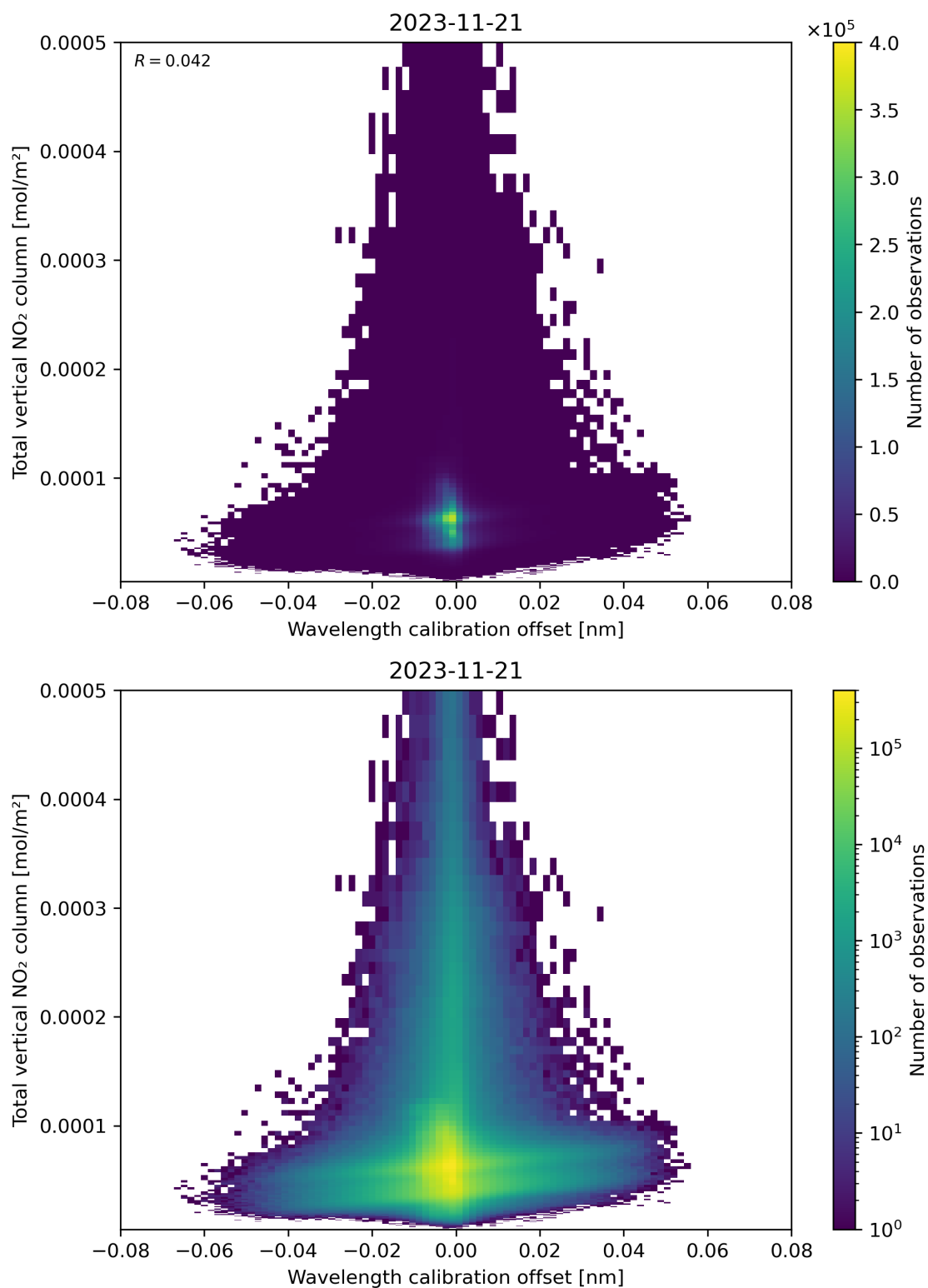
Figure 179: Scatter density plot of “Wavelength calibration offset” against “Total vertical NO 2 column” for 2023-11-20 to 2023-11-22.
