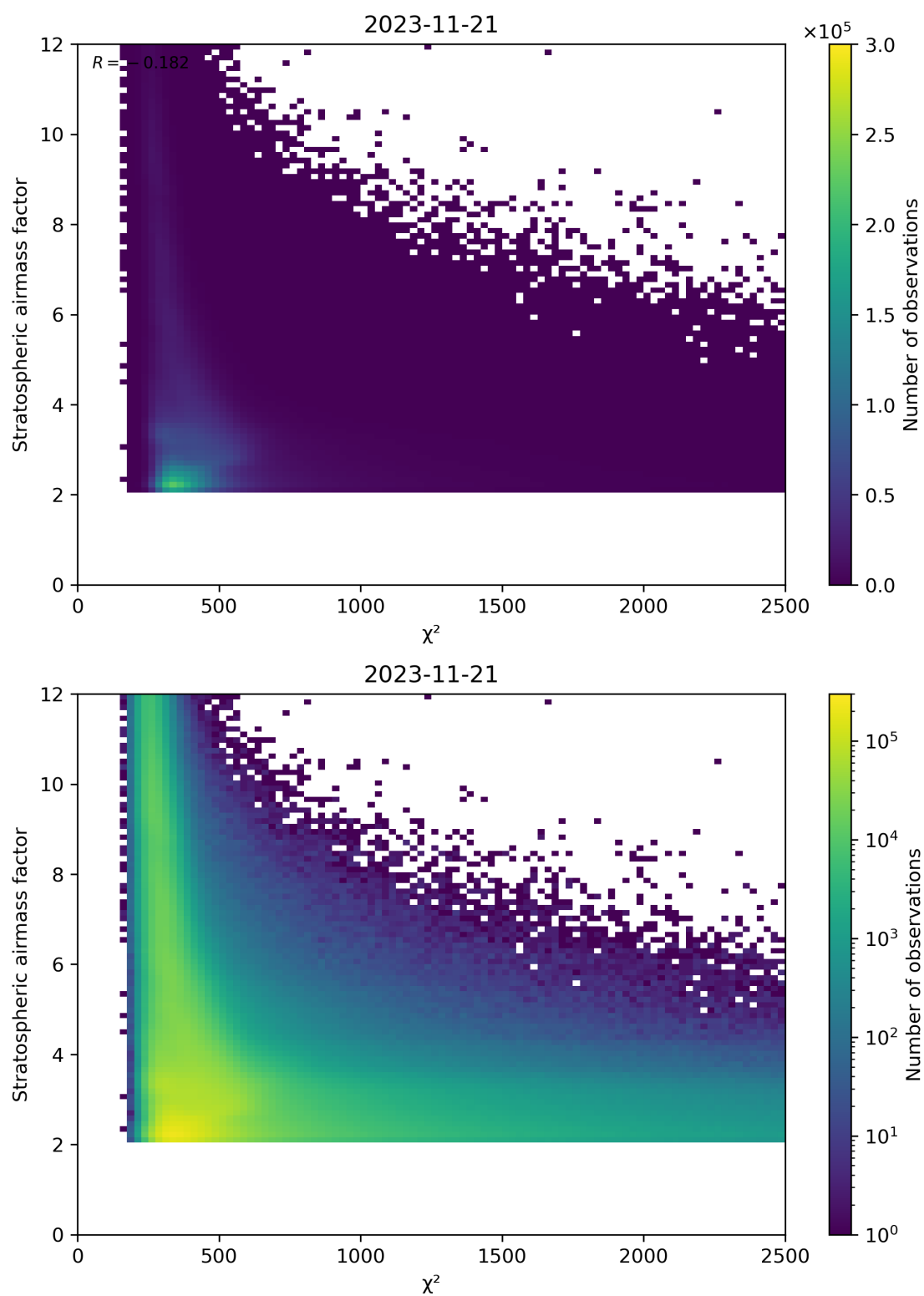
Figure 81: Scatter density plot of “ \chi^2 ” against “Stratospheric airmass factor” for 2023-11-20 to 2023-11-22.
