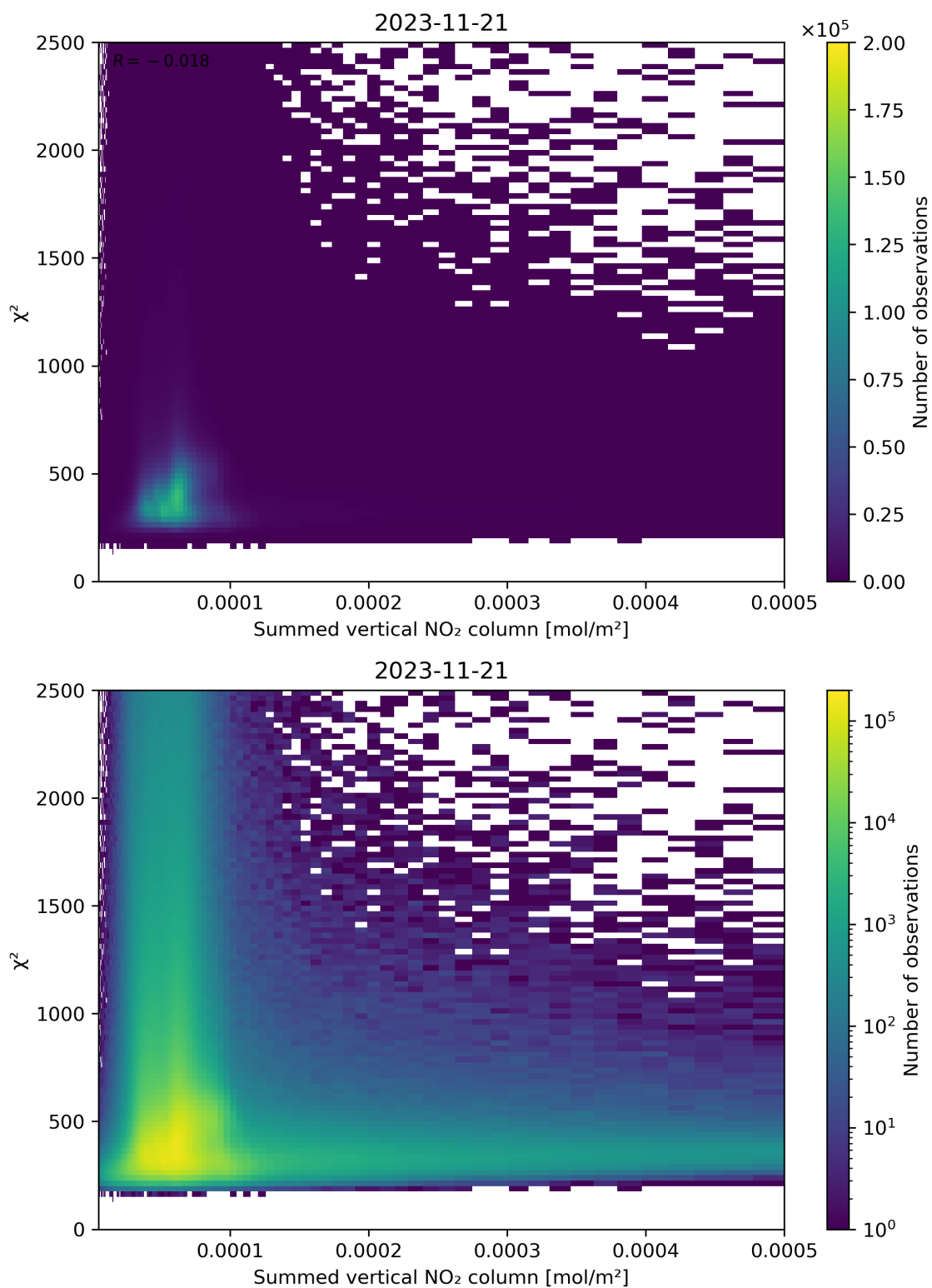
Figure 104: Scatter density plot of “Summed vertical NO 2 column” against “ \chi^2 ” for 2023-11-20 to 2023-11-22.
