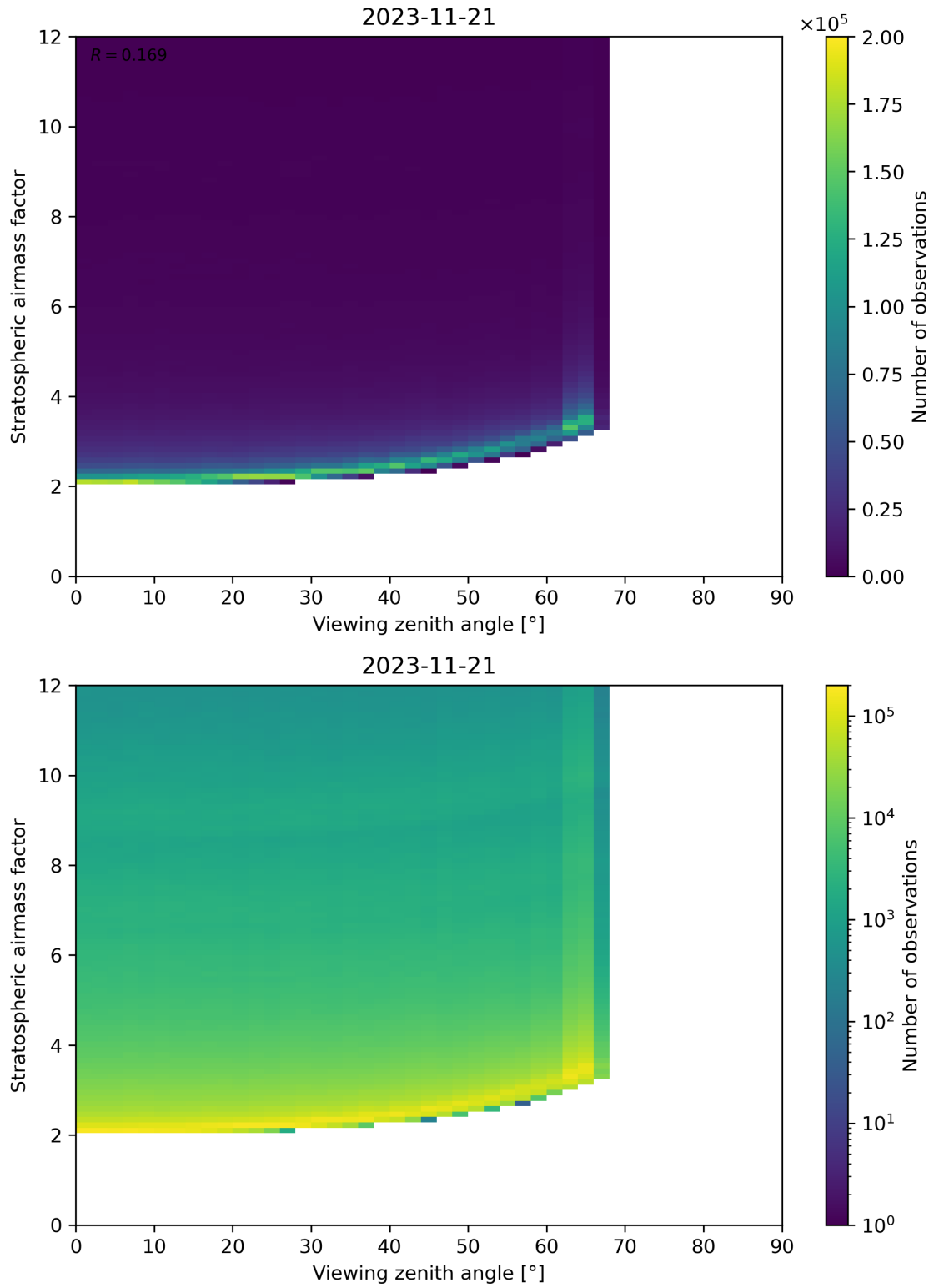
Figure 159: Scatter density plot of “Viewing zenith angle” against “Stratospheric airmass factor” for 2023-11-20 to 2023-11-22.
