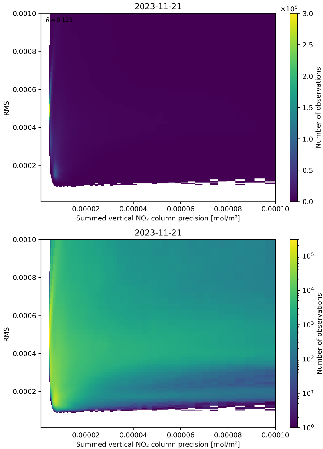
Figure 108: Scatter density plot of “Summed vertical NO 2 column precision” against “RMS” for 2023-11-20 to 2023-11-22.
