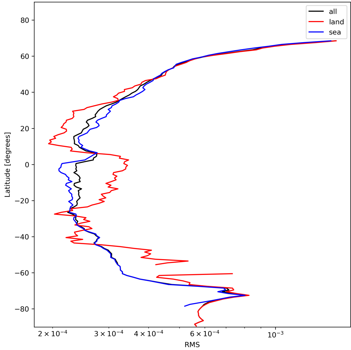
Figure 26: Zonal average of “RMS” for 2023-11-20 to 2023-11-22.
