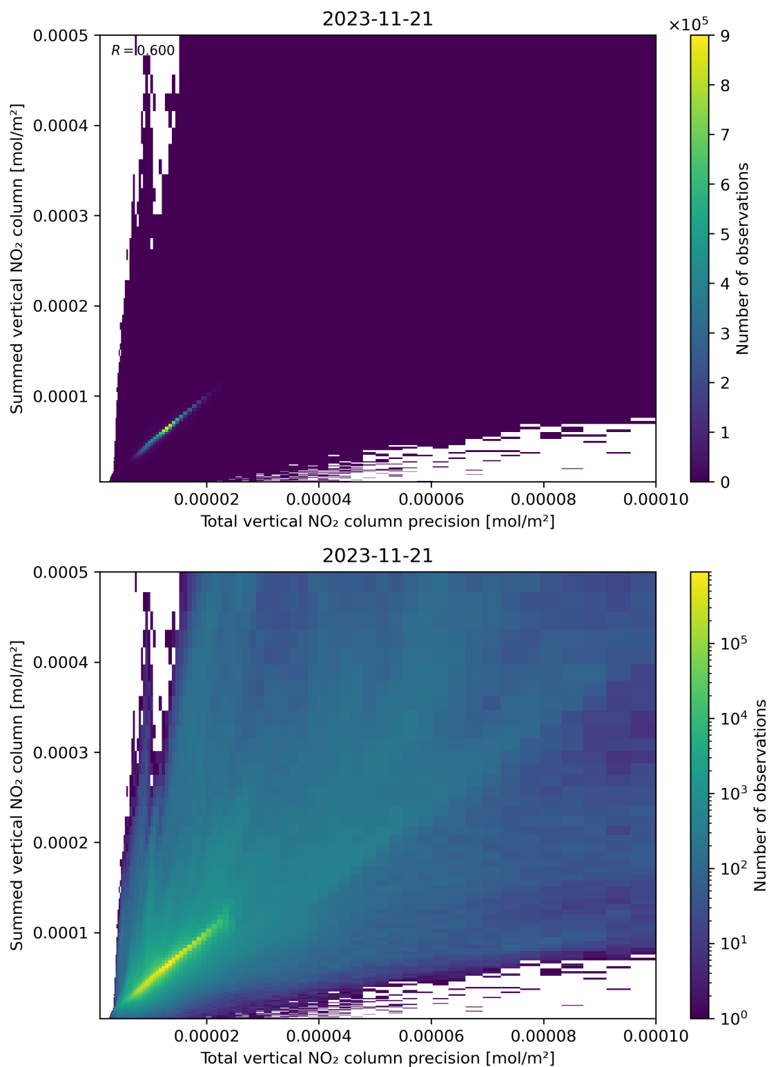
Figure 117: Scatter density plot of “Total vertical NO 2 column precision” against “Summed vertical NO 2 column” for 2023-11-20 to 2023-11-22.
