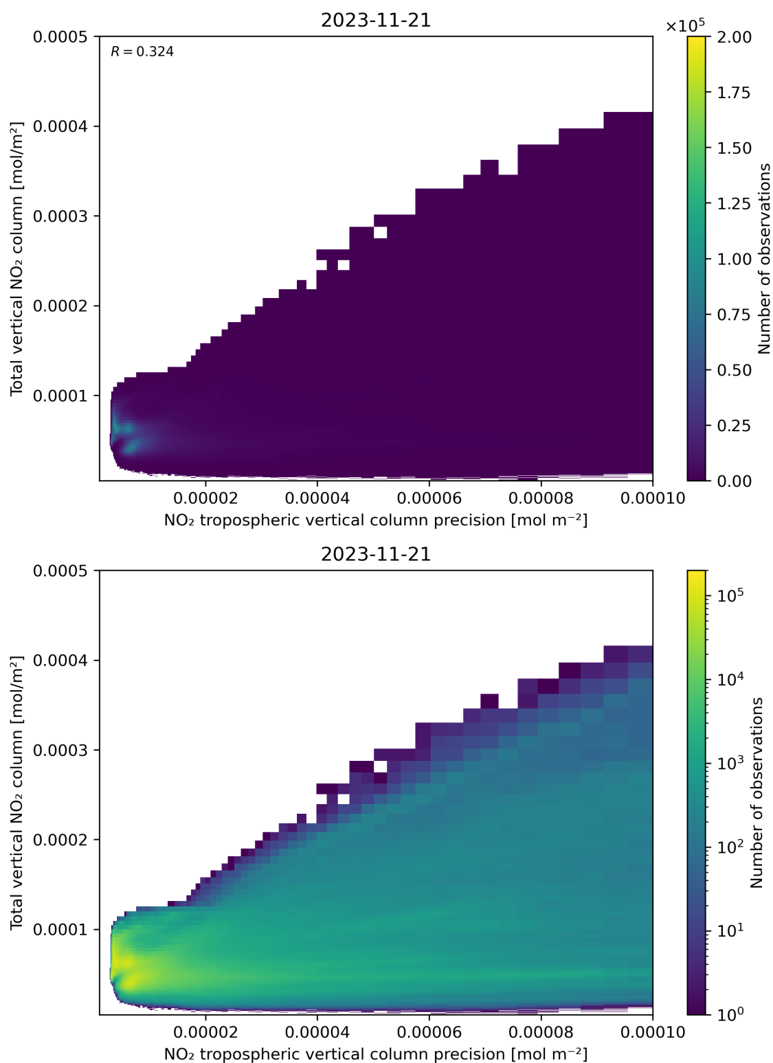
Figure 138: Scatter density plot of “NO 2 tropospheric vertical column precision” against “Total vertical NO 2 column” for 2023-11-20 to 2023-11-22.
