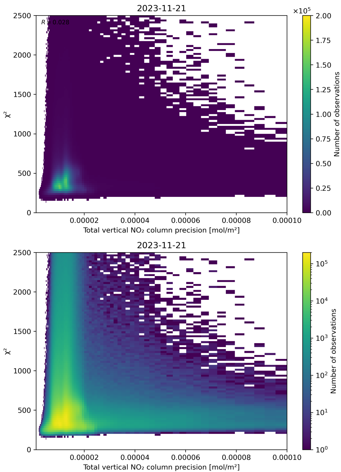
Figure 116: Scatter density plot of “Total vertical NO 2 column precision” against “ \chi^2 ” for 2023-11-20 to 2023-11-22.
