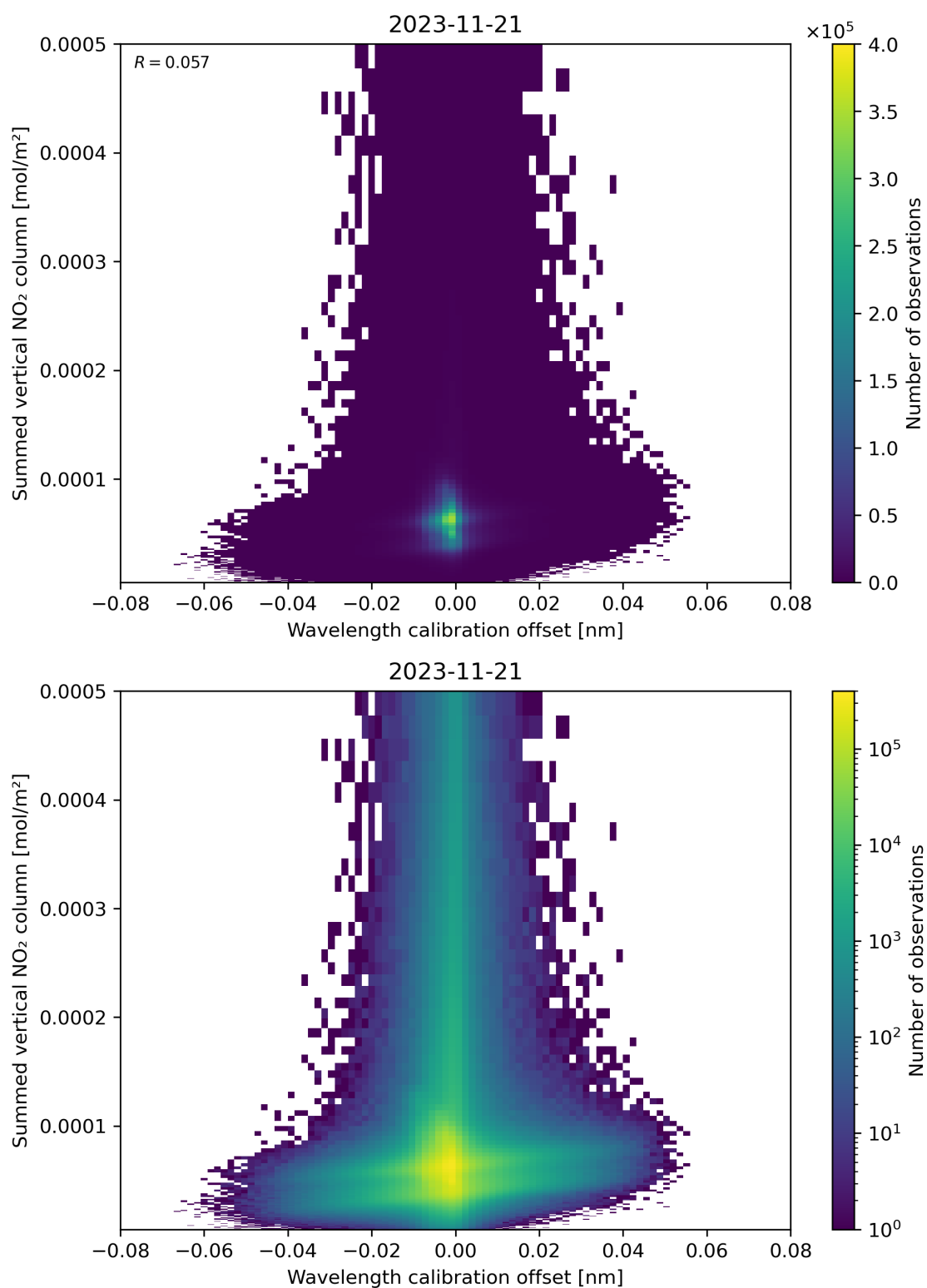
Figure 177: Scatter density plot of “Wavelength calibration offset” against “Summed vertical NO 2 column” for 2023-11-20 to 2023-11-22.
