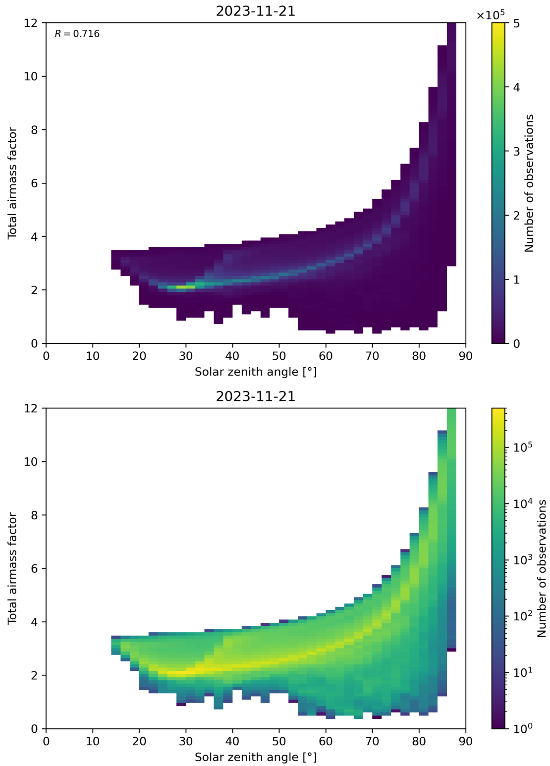
Figure 146: Scatter density plot of “Solar zenith angle” against “Total air mass factor” for 2023-11-20 to 2023-11-22.
