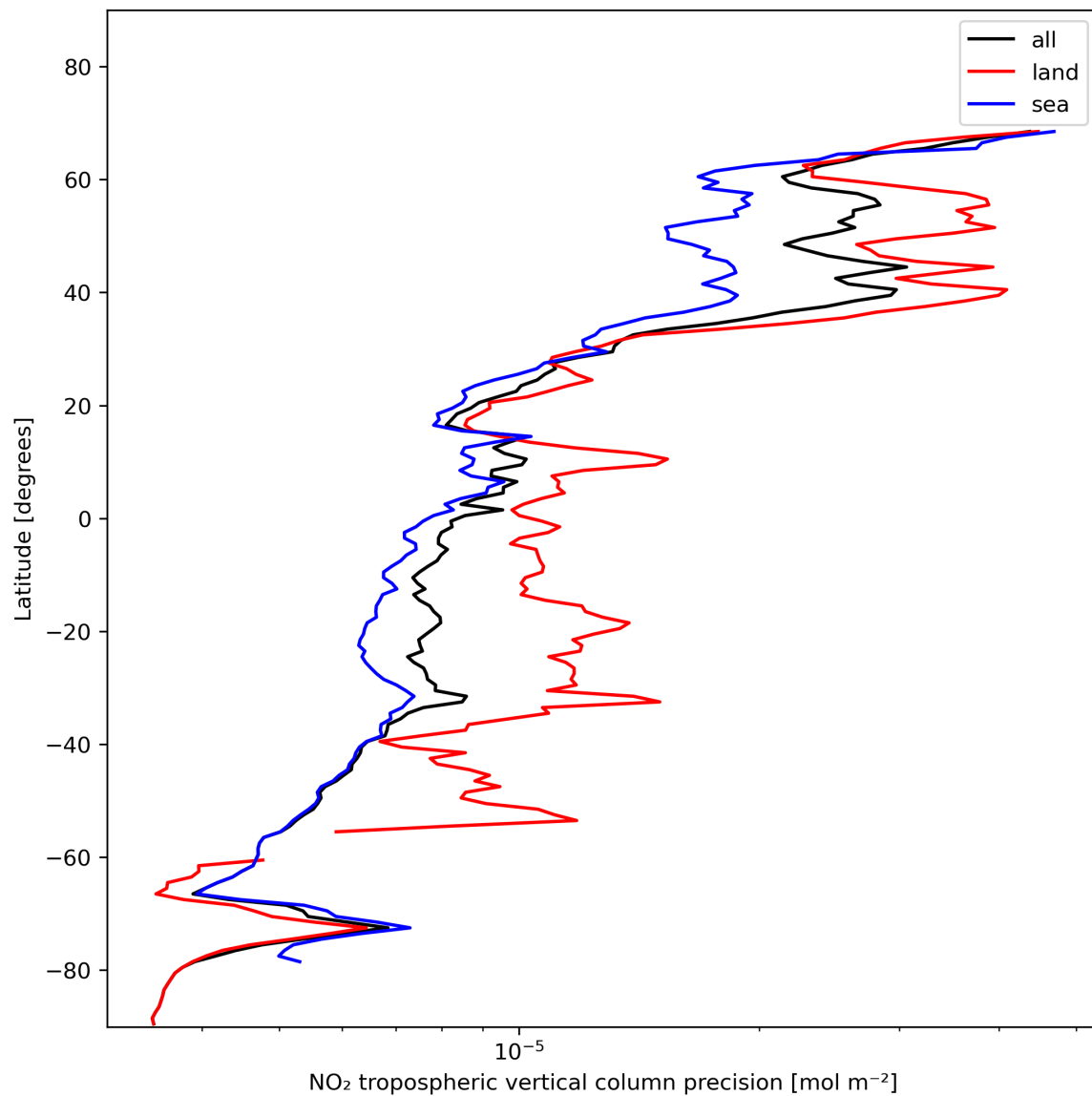
Figure 13: Zonal average of “NO 2 tropospheric vertical column precision” for 2023-11-20 to 2023-11-22.
