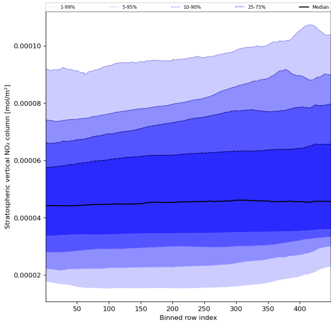
Figure 53: Along track statistics of “Stratospheric vertical NO 2 column” for 2023-11-20 to 2023-11-22
