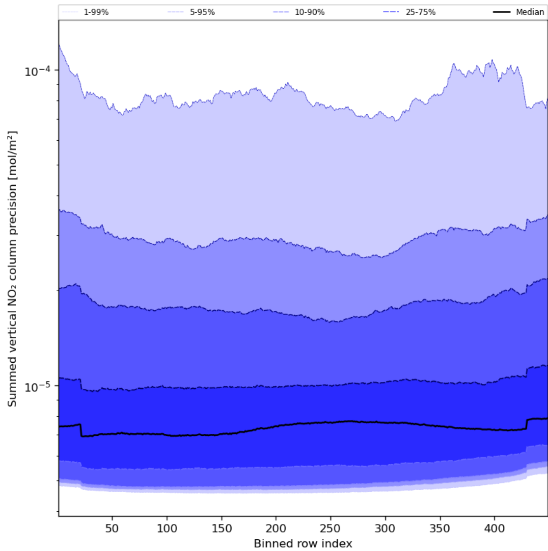
Figure 58: Along track statistics of “Summed vertical NO 2 column precision” for 2023-11-20 to 2023-11-22
