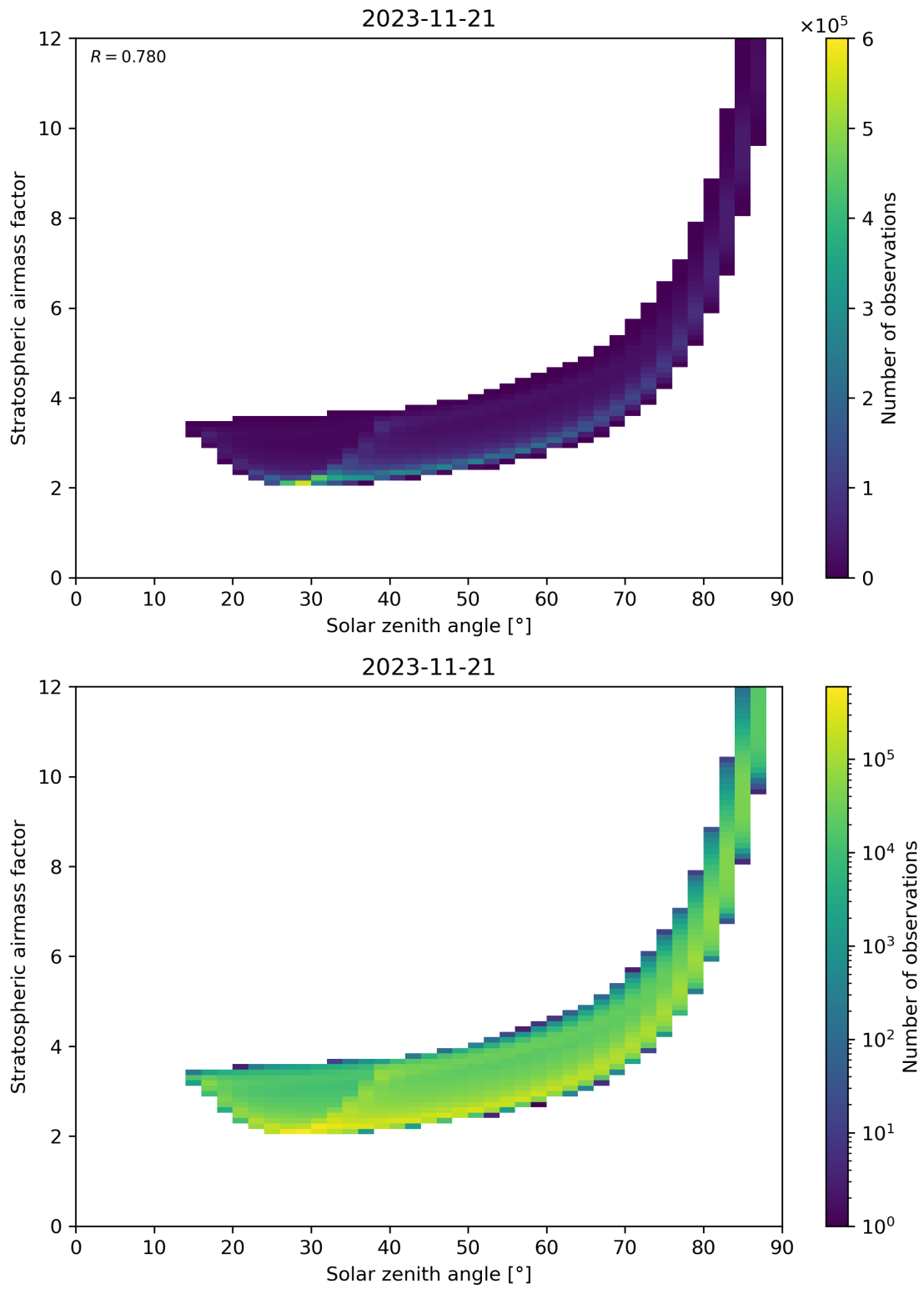
Figure 145: Scatter density plot of “Solar zenith angle” against “Stratospheric airmass factor” for 2023-11-20 to 2023-11-22.
