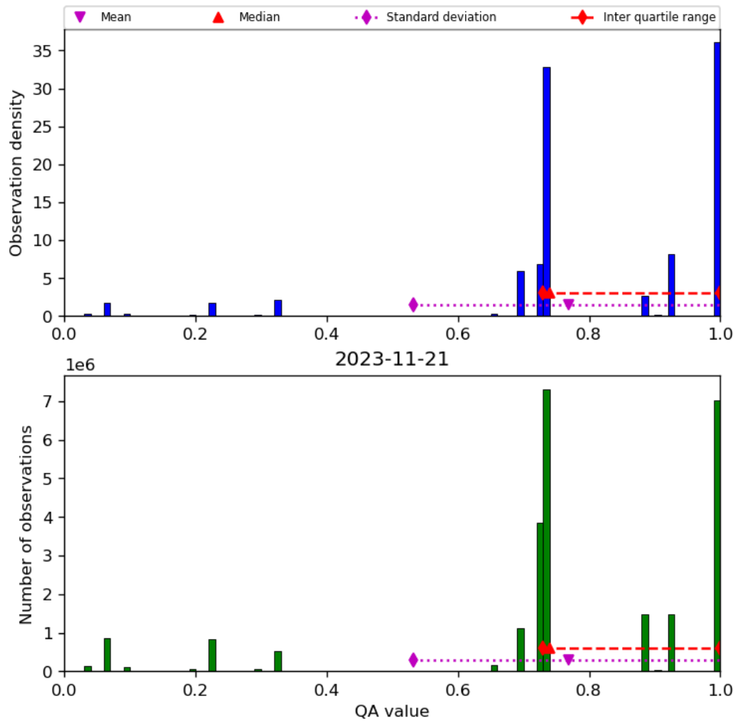
Figure 28: Histogram of “QA value” for 2023-11-20 to 2023-11-22
