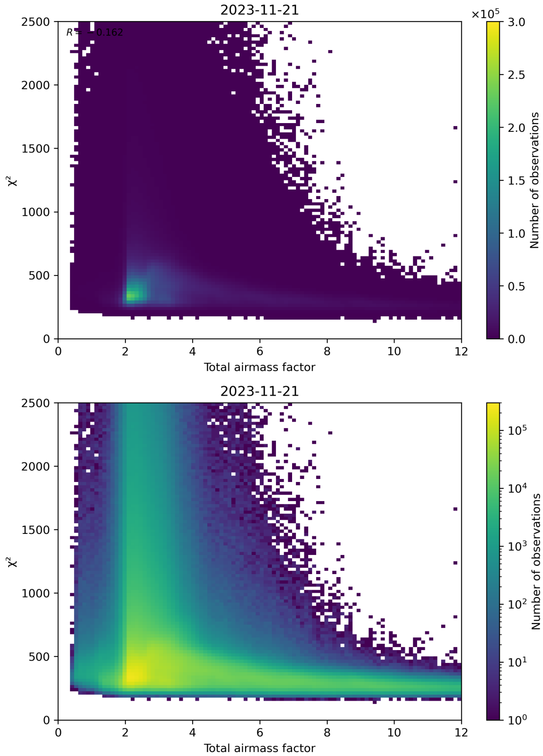
Figure 63: Scatter density plot of “Total airmass factor” against “ \chi^2 ” for 2023-11-20 to 2023-11-22.
