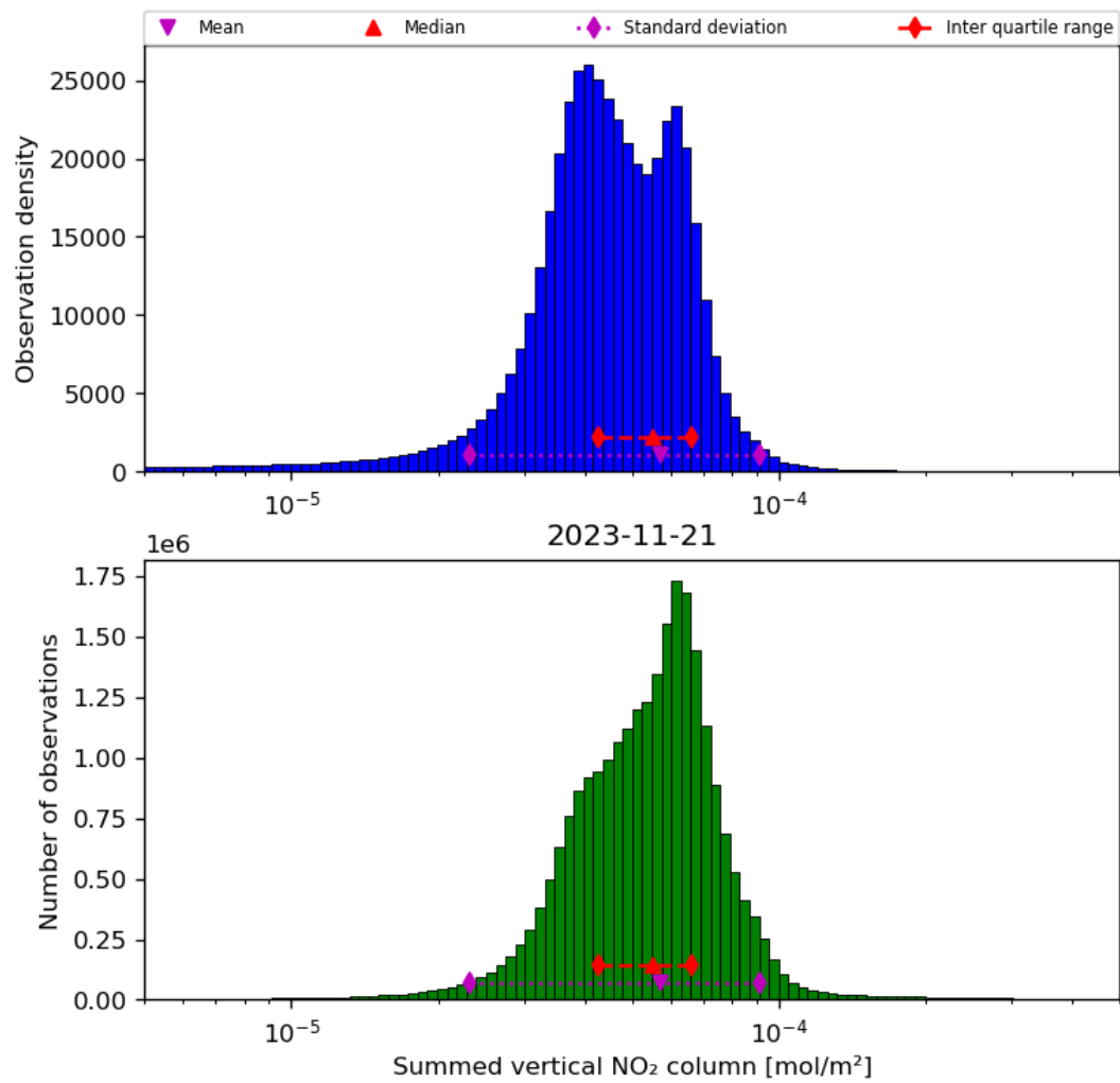
Figure 40: Histogram of “Summed vertical NO 2 column” for 2023-11-20 to 2023-11-22
