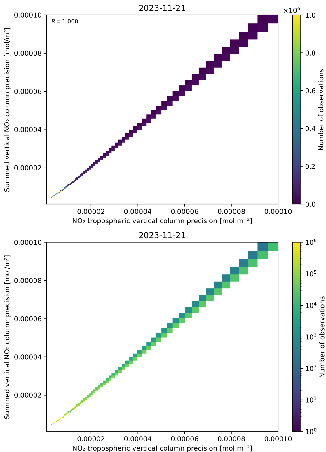
Figure 137: Scatter density plot of “NO 2 tropospheric vertical column precision” against “Summed vertical NO 2 column precision” for 2023-11-20 to 2023-11-22.
