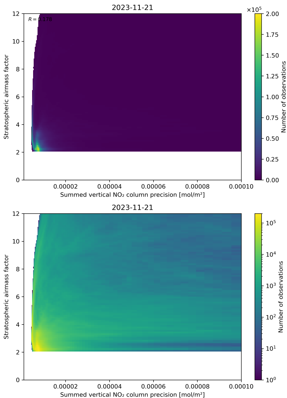
Figure 106: Scatter density plot of “Summed vertical NO 2 column precision” against “Stratospheric airmass factor” for 2023-11-20 to 2023-11-22.
