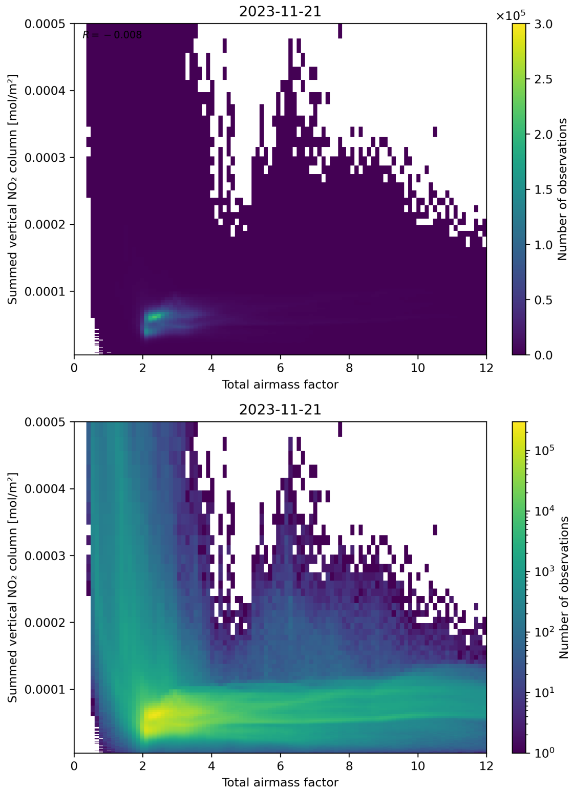
Figure 65: Scatter density plot of “Total airmass factor” against “Summed vertical NO 2 column” for 2023-11-20 to 2023-11-22.
