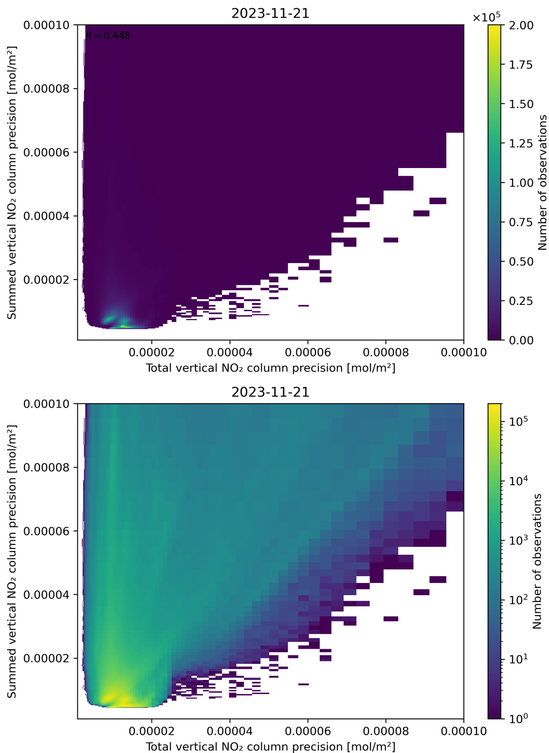
Figure 118: Scatter density plot of “Total vertical NO 2 column precision” against “Summed vertical NO 2 column precision” for 2023-11-20 to 2023-11-22.
