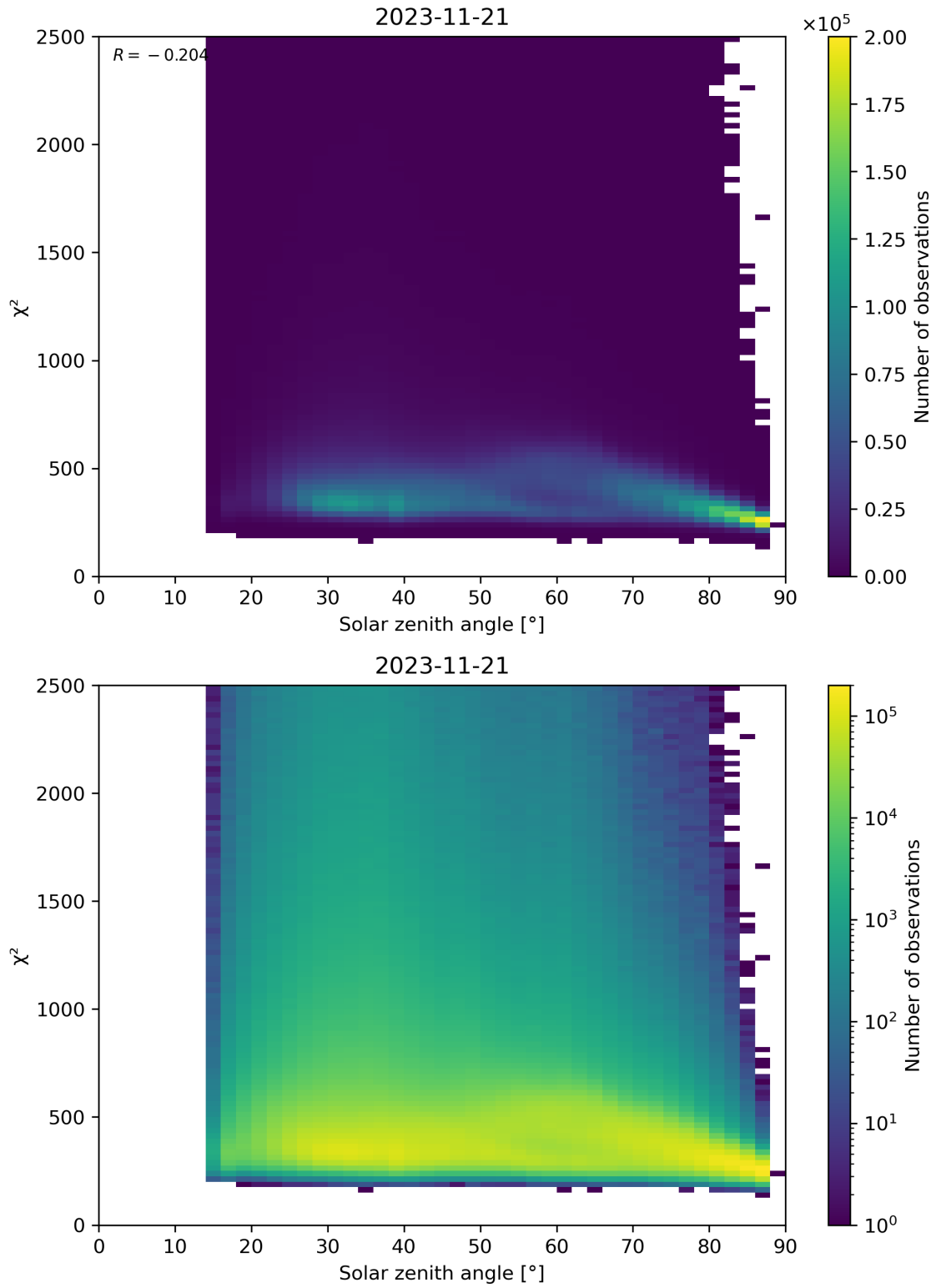
Figure 148: Scatter density plot of “Solar zenith angle” against “ \chi^2 ” for 2023-11-20 to 2023-11-22.
