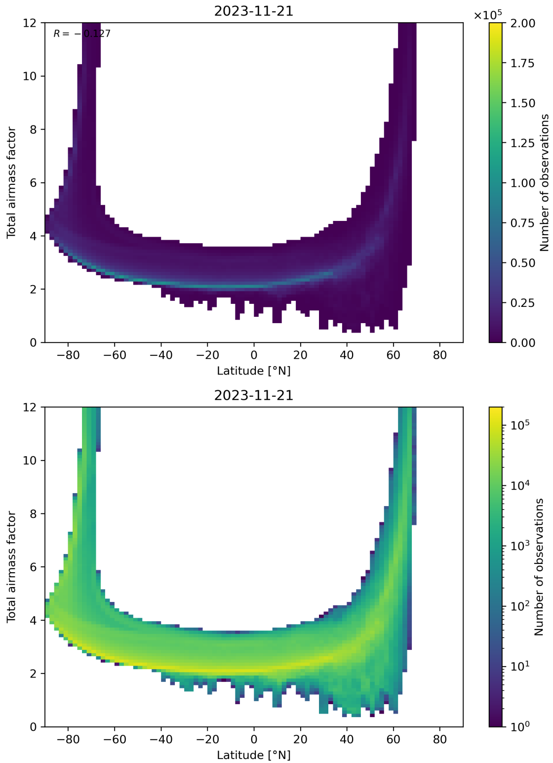
Figure 84: Scatter density plot of “Latitude” against “Total airmass factor” for 2023-11-20 to 2023-11-22.
