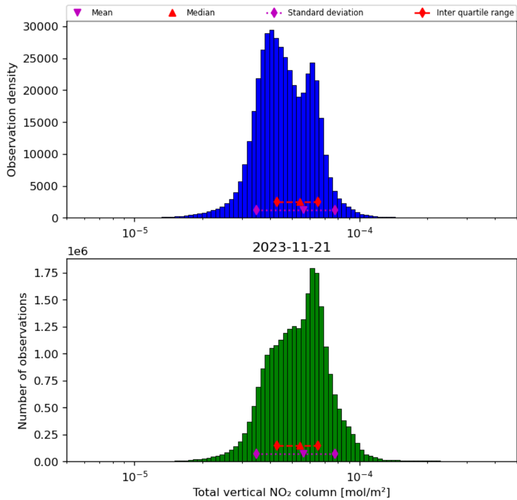
Figure 38: Histogram of “Total vertical NO 2 column” for 2023-11-20 to 2023-11-22
