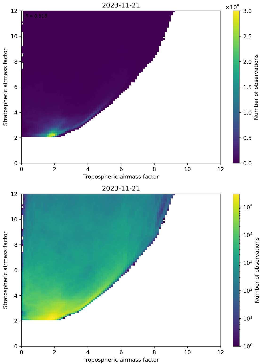
Figure 71: Scatter density plot of “Tropospheric airmass factor” against “Stratospheric airmass factor” for 2023-11-20 to 2023-11-22.
