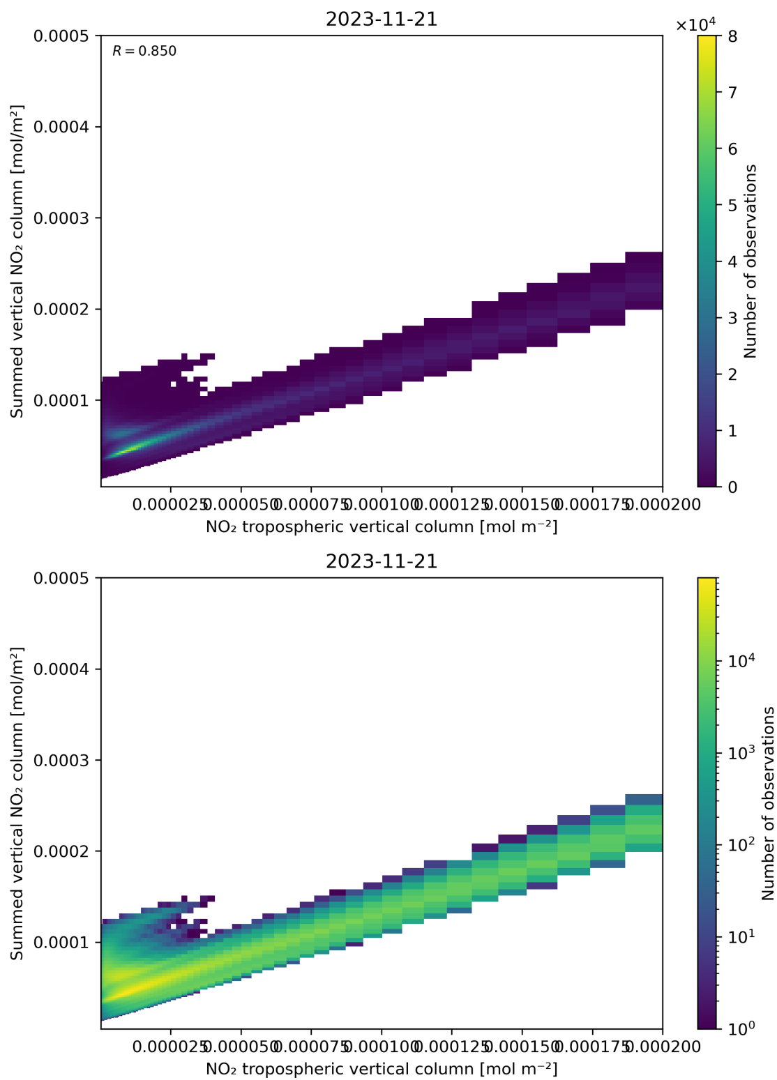
Figure 126: Scatter density plot of “NO 2 tropospheric vertical column” against “Summed vertical NO 2 column” for 2023-11-20 to 2023-11-22.
