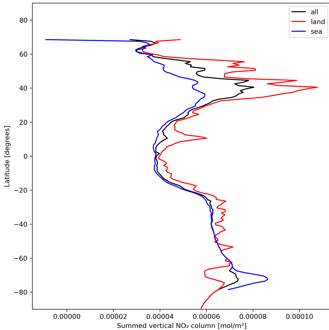
Figure 23: Zonal average of “Summed vertical NO 2 column” for 2023-11-20 to 2023-11-22.
