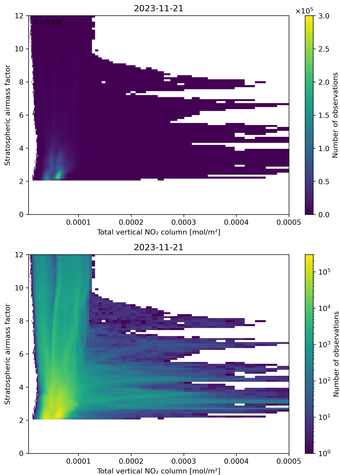
Figure 110: Scatter density plot of “Total vertical NO 2 column” against “Stratospheric air mass factor” for 2023-11-20 to 2023-11-22.
