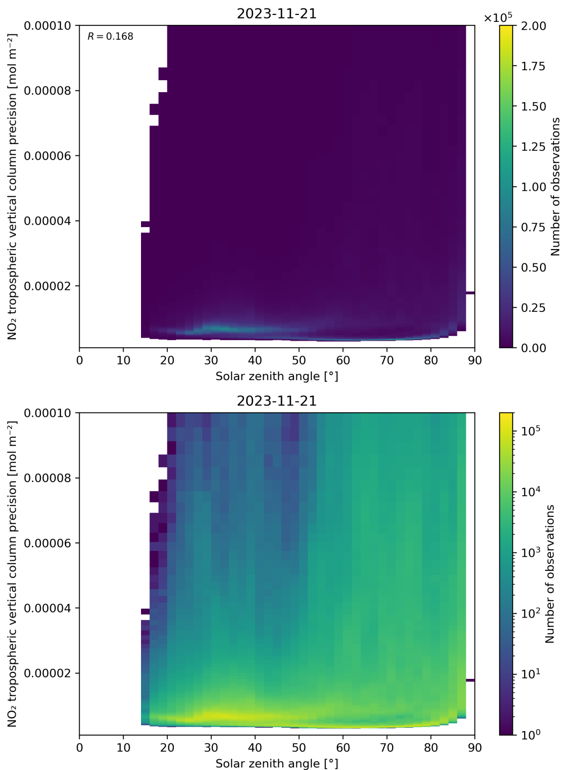
Figure 156: Scatter density plot of “Solar zenith angle” against “NO 2 tropospheric vertical column precision” for 2023-11-20 to 2023-11-22.
