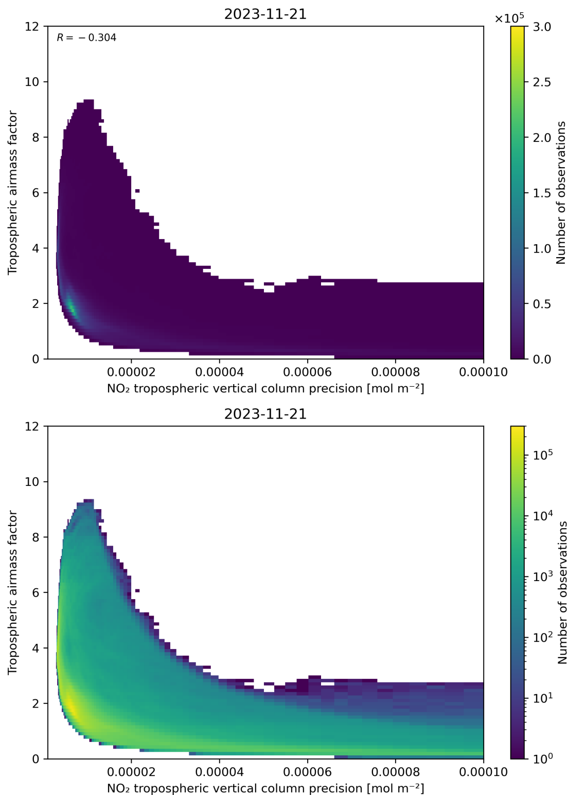
Figure 133: Scatter density plot of “NO 2 tropospheric vertical column precision” against “Tropospheric airmass factor” for 2023-11-20 to 2023-11-22.
