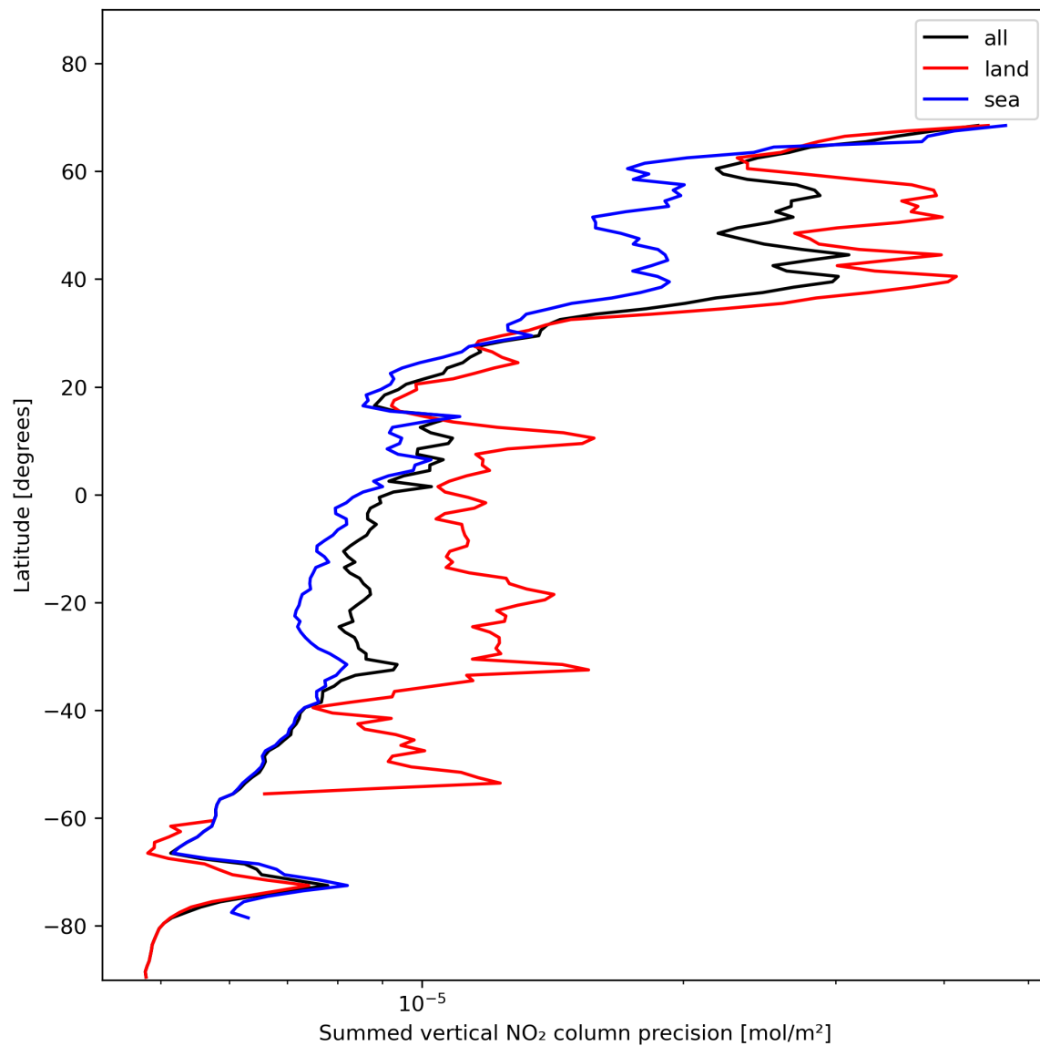
Figure 24: Zonal average of “Summed vertical NO 2 column precision” for 2023-11-20 to 2023-11-22.
