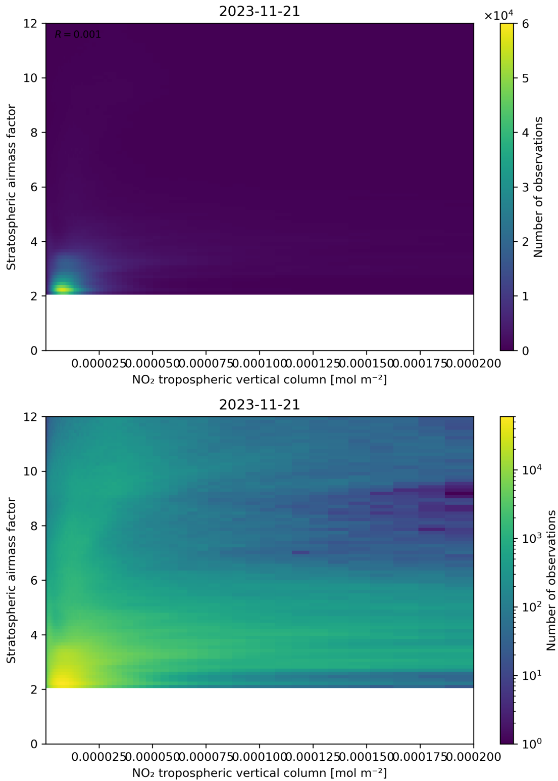
Figure 121: Scatter density plot of “NO 2 tropospheric vertical column” against “Stratospheric airmass factor” for 2023-11-20 to 2023-11-22.
