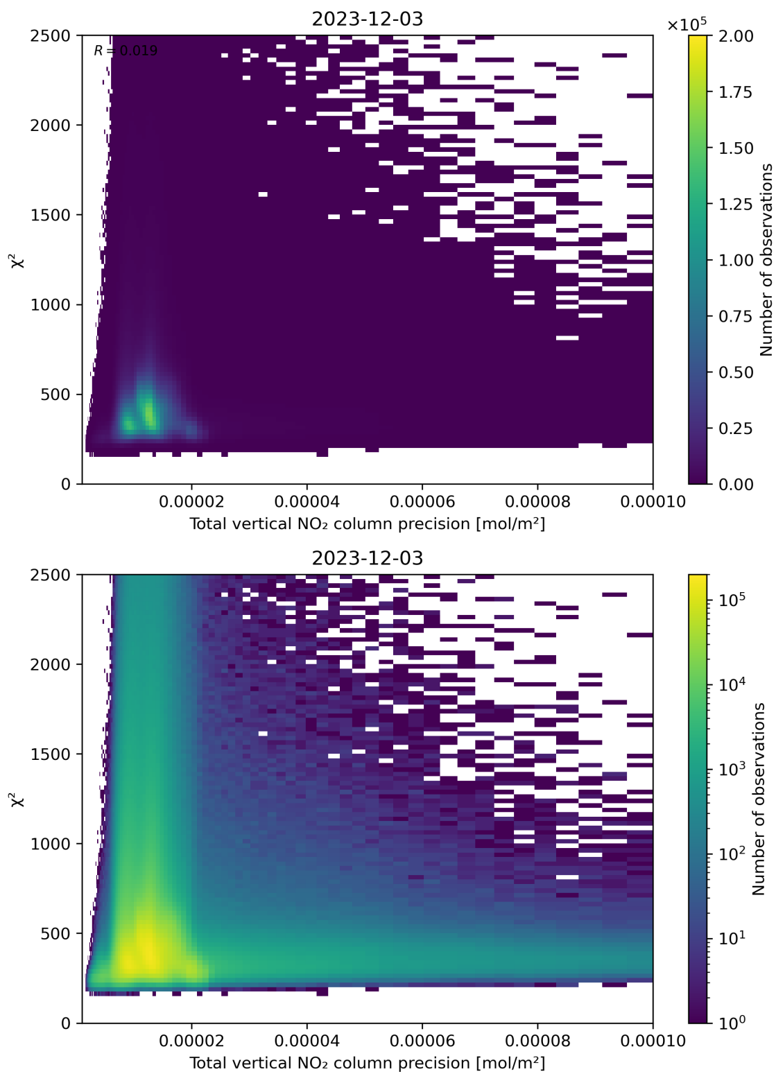
Figure 116: Scatter density plot of “Total vertical NO 2 column precision” against “ \chi^2 ” for 2023-12-02 to 2023-12-04.
