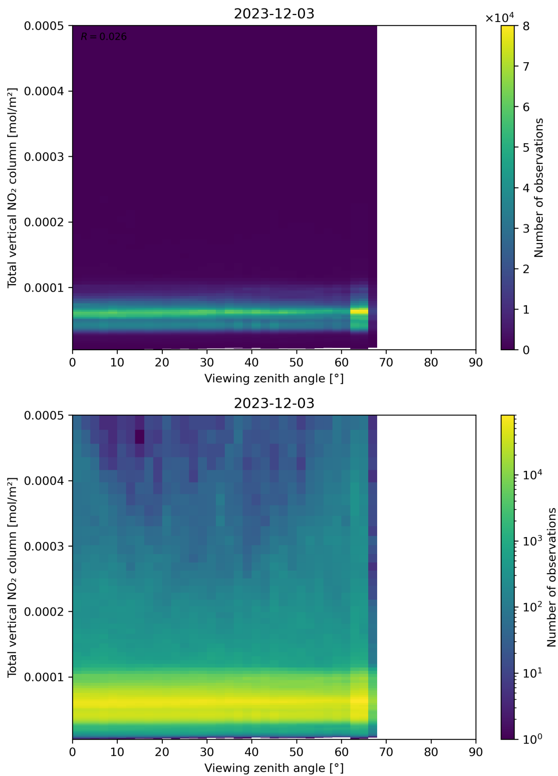
Figure 167: Scatter density plot of “Viewing zenith angle” against “Total vertical NO 2 column” for 2023-12-02 to 2023-12-04.
