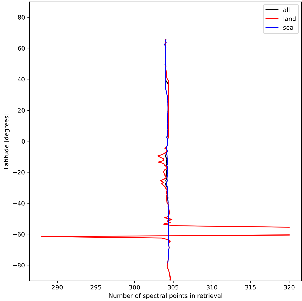
Figure 16: Zonal average of “Number of spectral points in retrieval” for 2023-12-02 to 2023-12-04.
