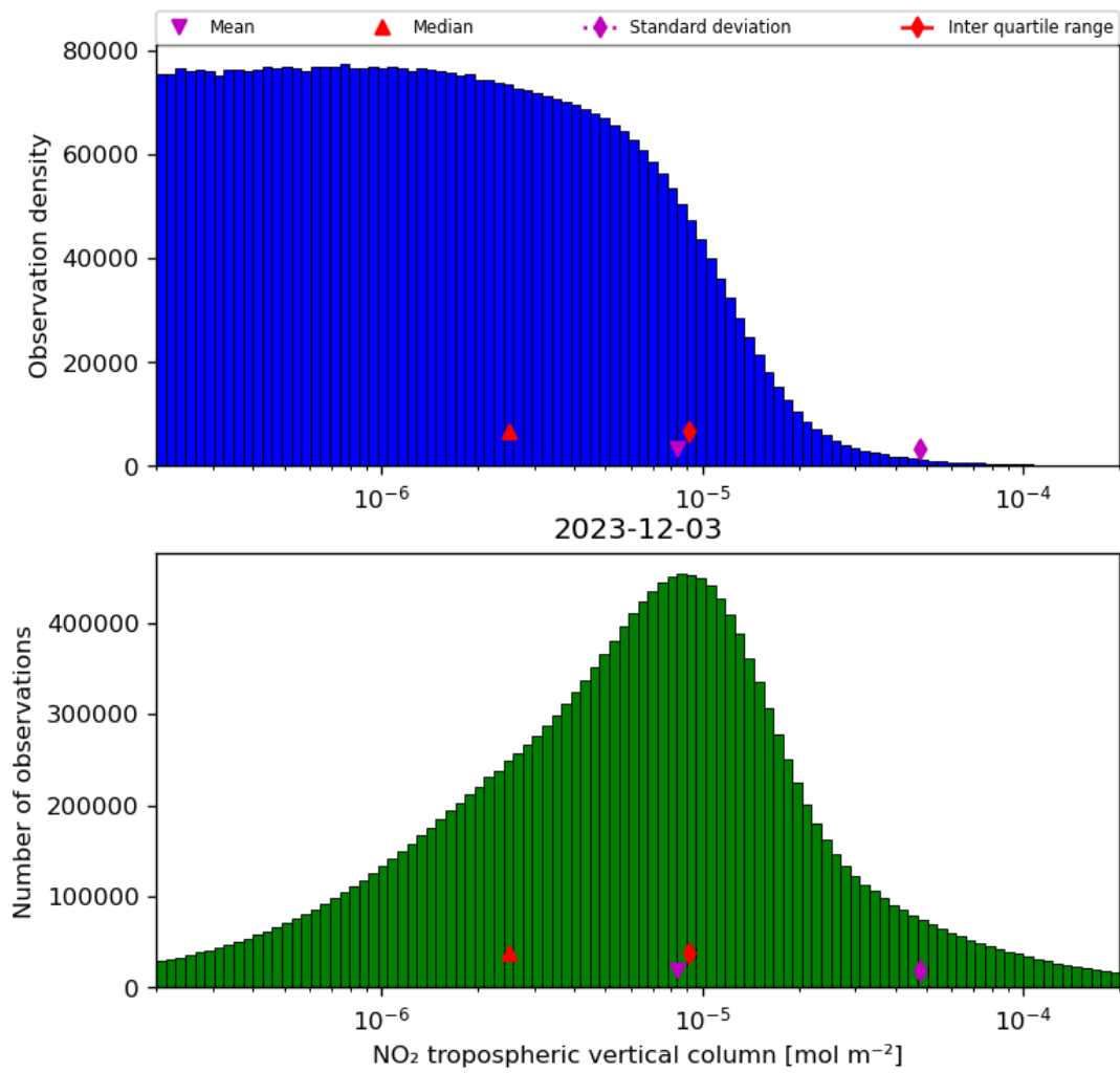
Figure 29: Histogram of “NO 2 tropospheric vertical column” for 2023-12-02 to 2023-12-04
