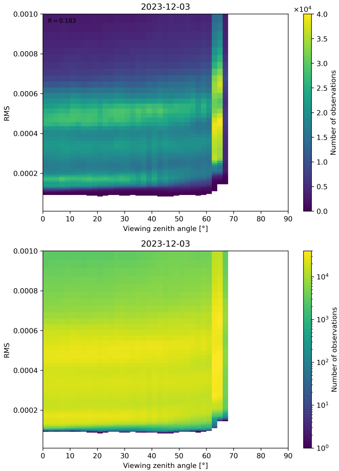
Figure 171: Scatter density plot of “Viewing zenith angle” against “RMS” for 2023-12-02 to 2023-12-04.
