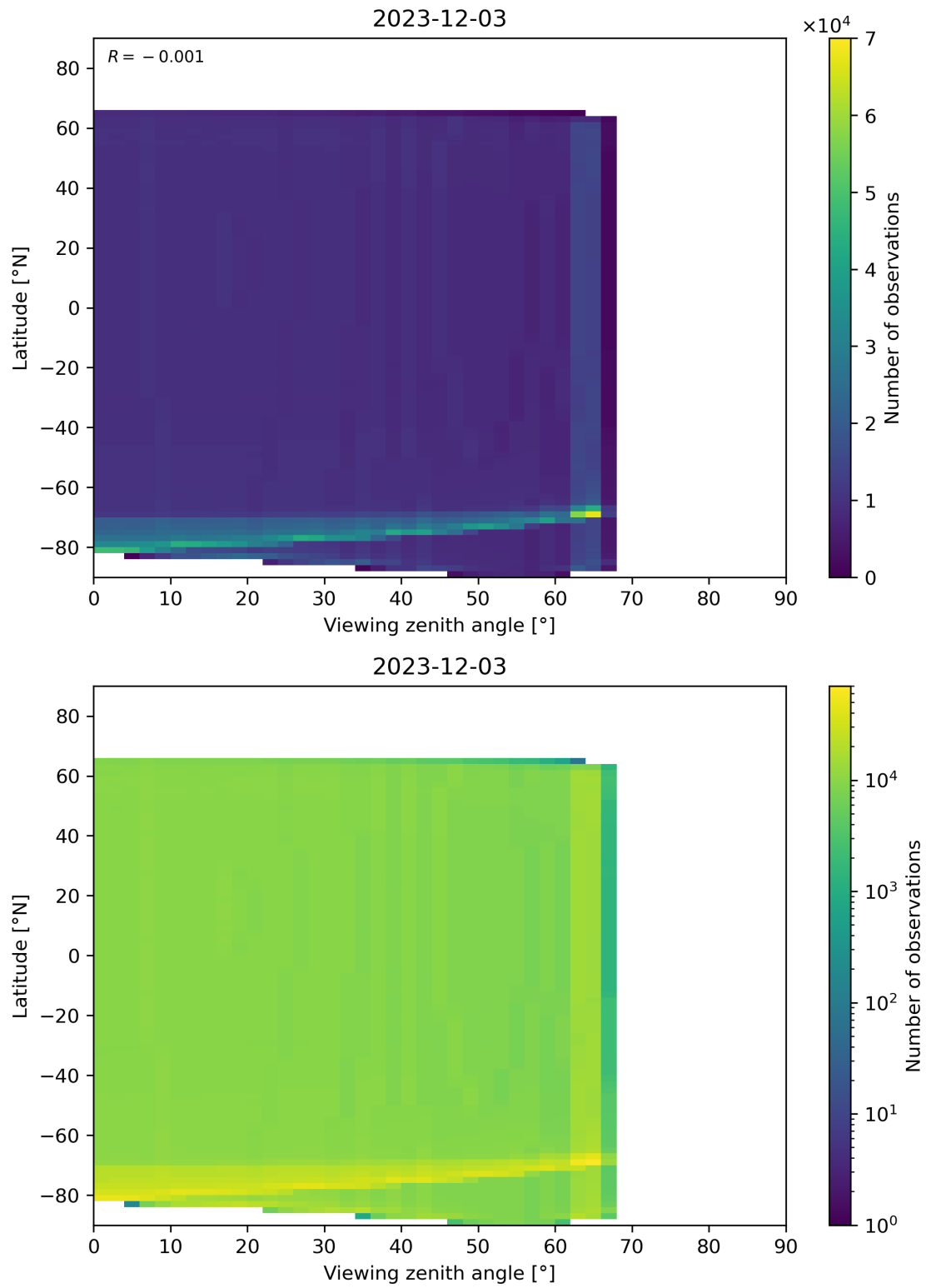
Figure 163: Scatter density plot of “Viewing zenith angle” against “Latitude” for 2023-12-02 to 2023-12-04.
