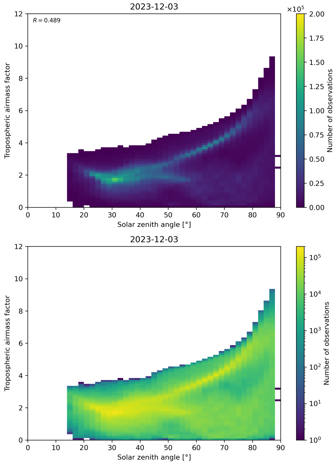
Figure 147: Scatter density plot of “Solar zenith angle” against “Tropospheric airmass factor” for 2023-12-02 to 2023-12-04.
