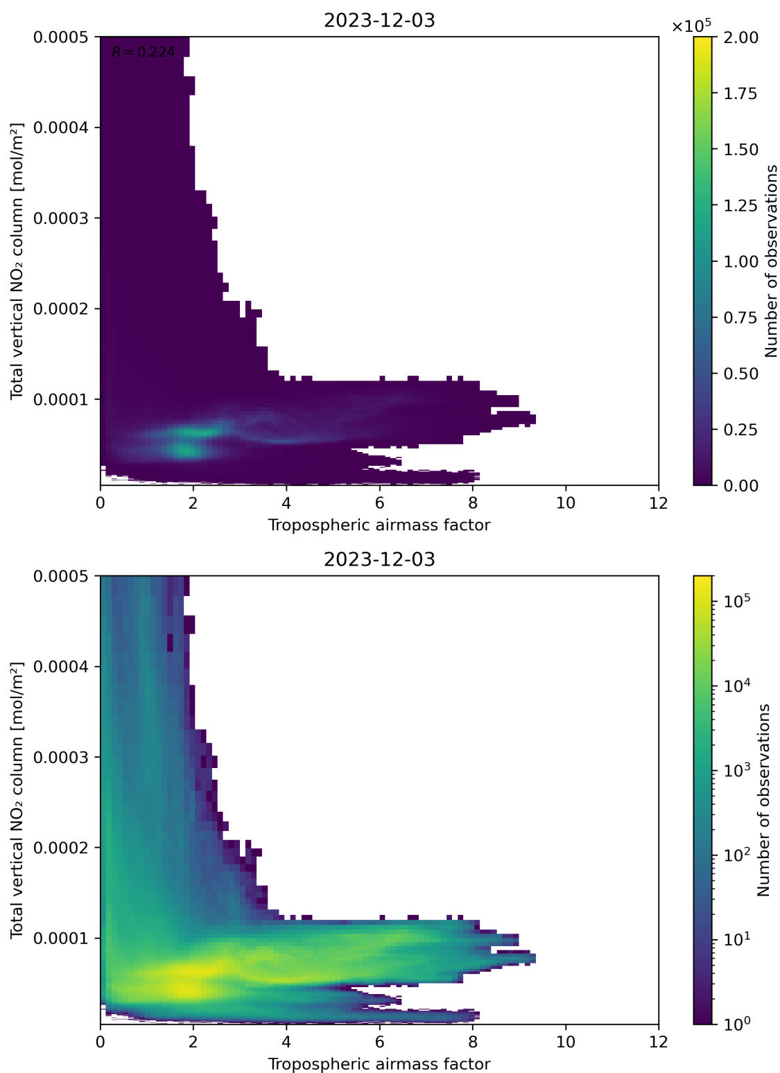
Figure 77: Scatter density plot of “Tropospheric airmass factor” against “Total vertical NO 2 column” for 2023-12-02 to 2023-12-04.
