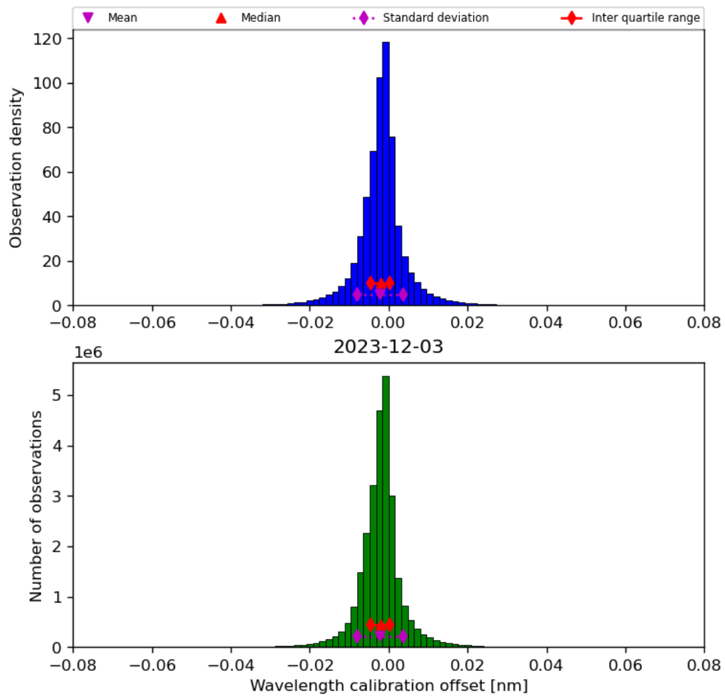
Figure 35: Histogram of “Wavelength calibration offset” for 2023-12-02 to 2023-12-04
