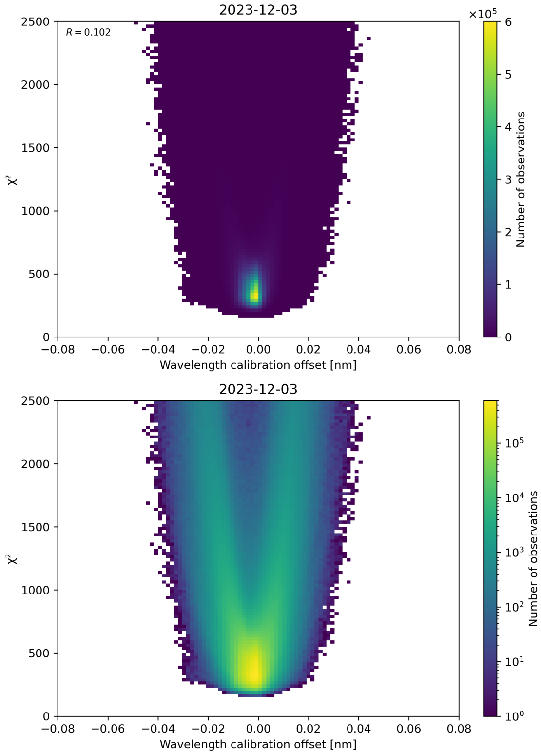
Figure 175: Scatter density plot of “Wavelength calibration offset” against “ \chi^2 ” for 2023-12-02 to 2023-12-04.
