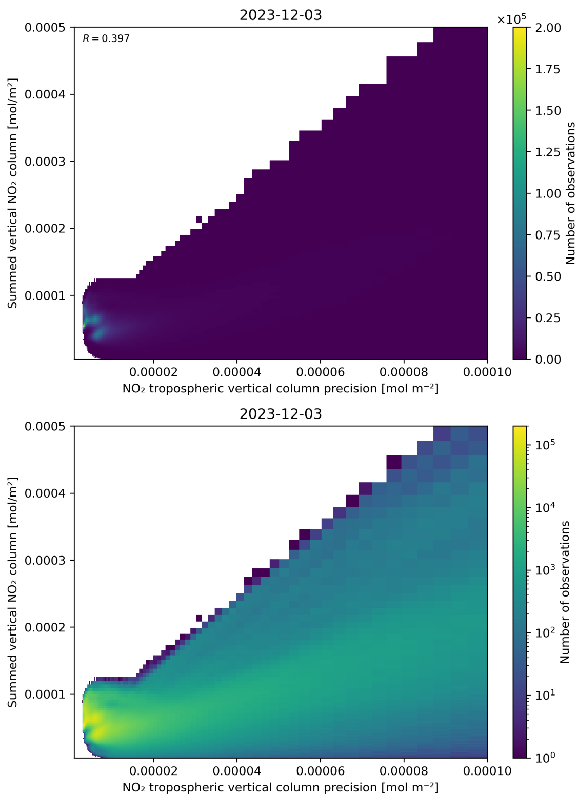
Figure 136: Scatter density plot of “NO 2 tropospheric vertical column precision” against “Summed vertical NO 2 column” for 2023-12-02 to 2023-12-04.
