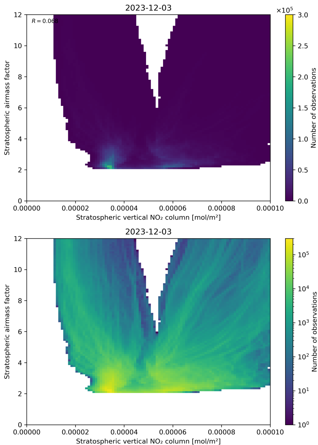
Figure 96: Scatter density plot of “Stratospheric vertical NO 2 column” against “Stratospheric airmass factor” for 2023-12-02 to 2023-12-04.
