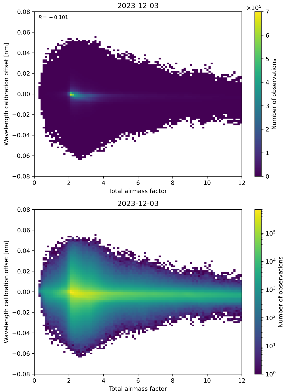
Figure 70: Scatter density plot of “Total airmass factor” against “Wavelength calibration offset” for 2023-12-02 to 2023-12-04.
