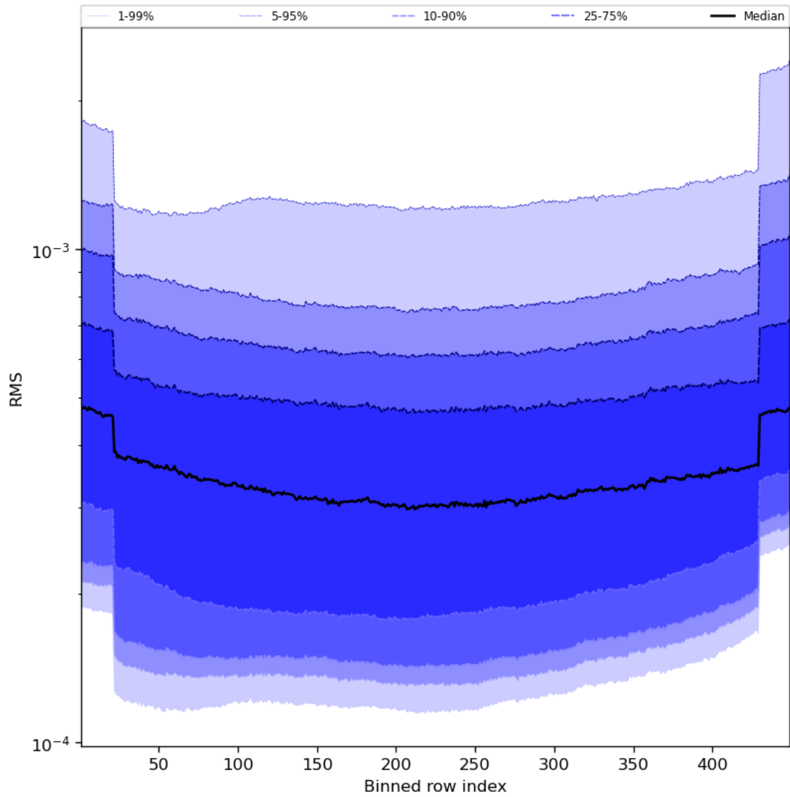
Figure 60: Along track statistics of “RMS” for 2023-12-02 to 2023-12-04
