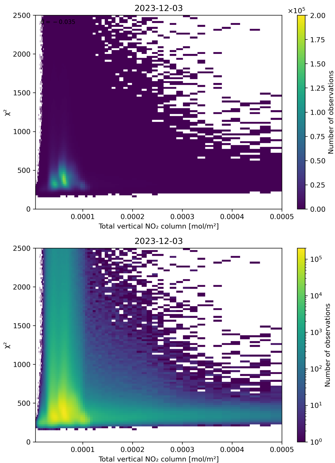
Figure 111: Scatter density plot of “Total vertical NO 2 column” against “ \chi^2 ” for 2023-12-02 to 2023-12-04.
