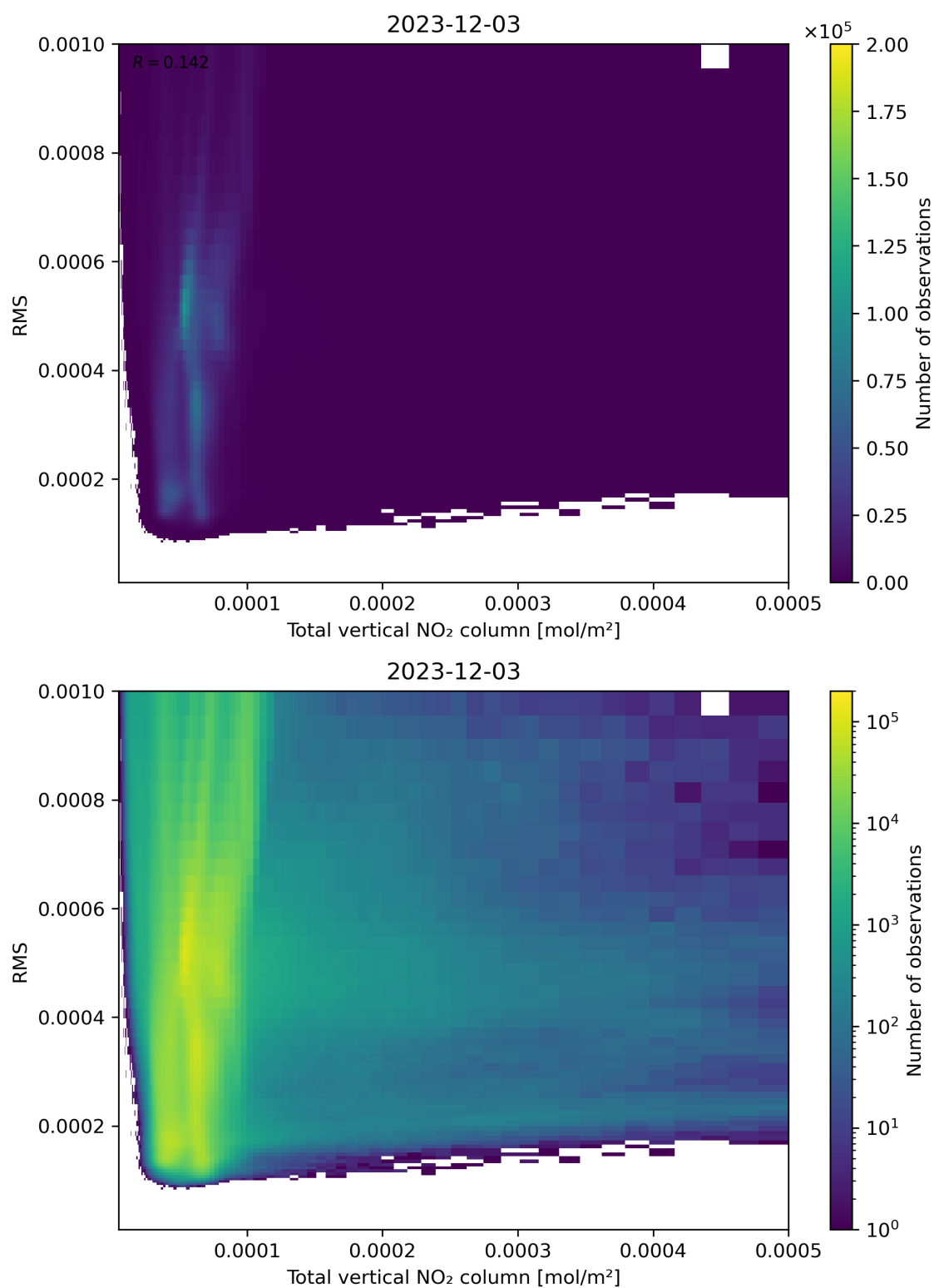
Figure 120: Scatter density plot of “Total vertical NO 2 column” against “RMS” for 2023-12-02 to 2023-12-04.
