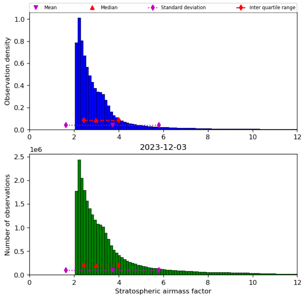
Figure 44: Histogram of “Stratospheric airmass factor” for 2023-12-02 to 2023-12-04
