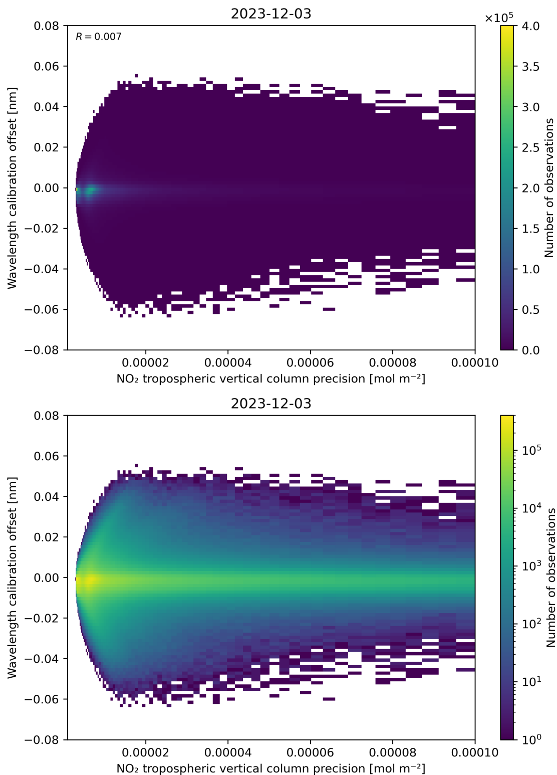
Figure 141: Scatter density plot of “NO 2 tropospheric vertical column precision” against “Wavelength calibration offset” for 2023-12-02 to 2023-12-04.
