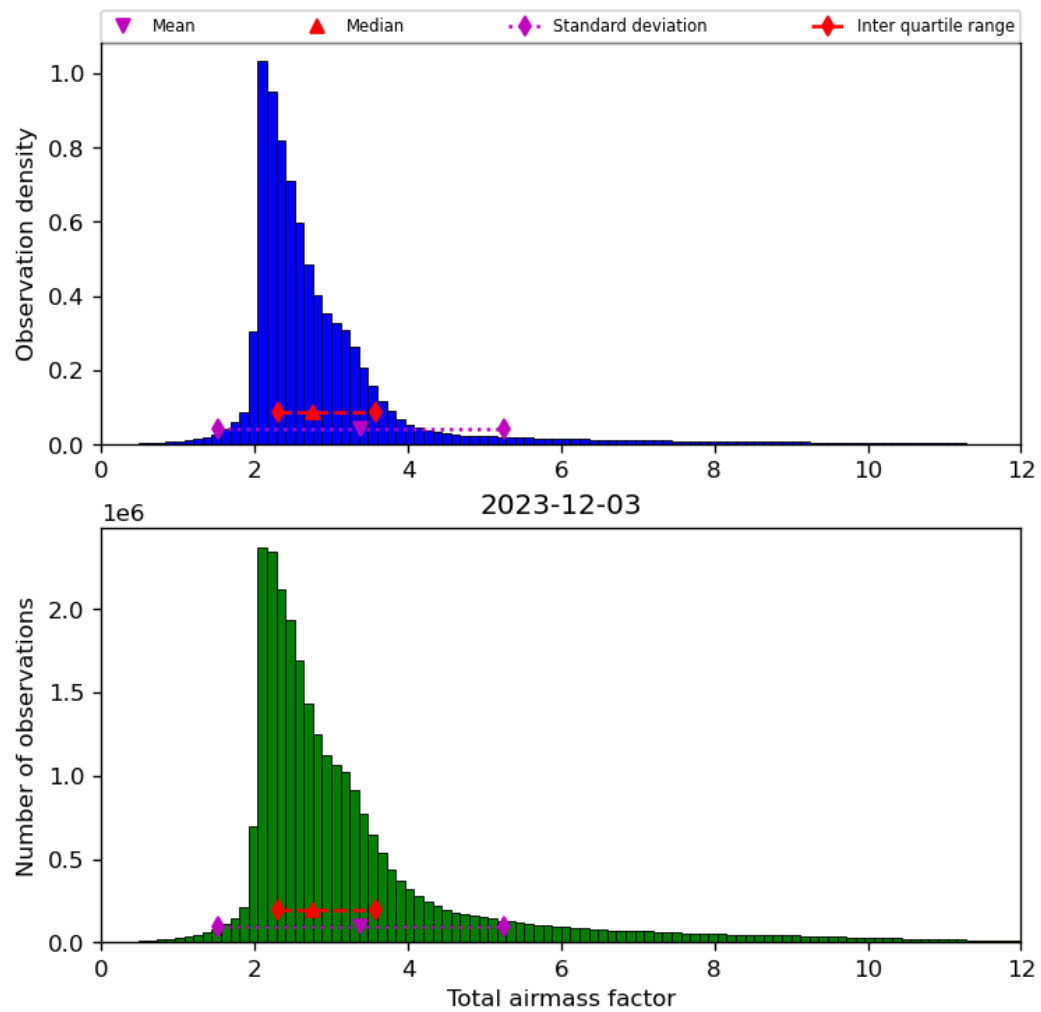
Figure 32: Histogram of “Total airmass factor” for 2023-12-02 to 2023-12-04
