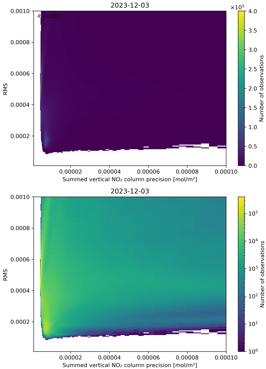
Figure 108: Scatter density plot of “Summed vertical NO 2 column precision” against “RMS” for 2023-12-02 to 2023-12-04.
