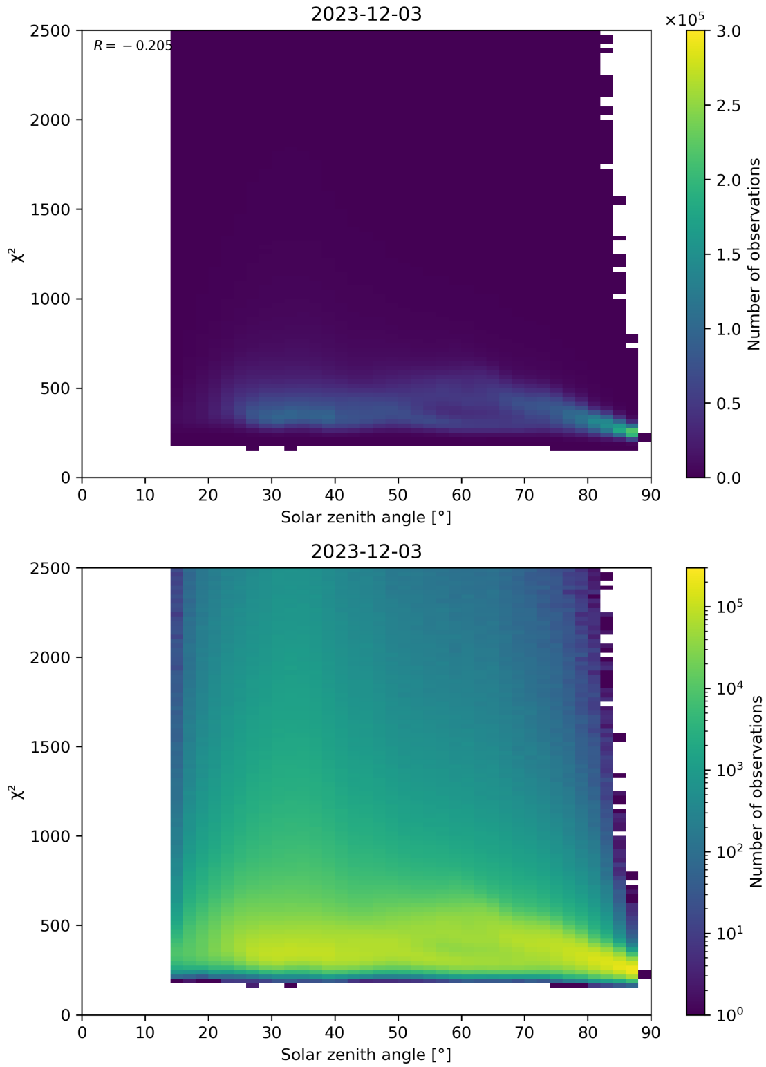
Figure 148: Scatter density plot of “Solar zenith angle” against “ \chi^2 ” for 2023-12-02 to 2023-12-04.
