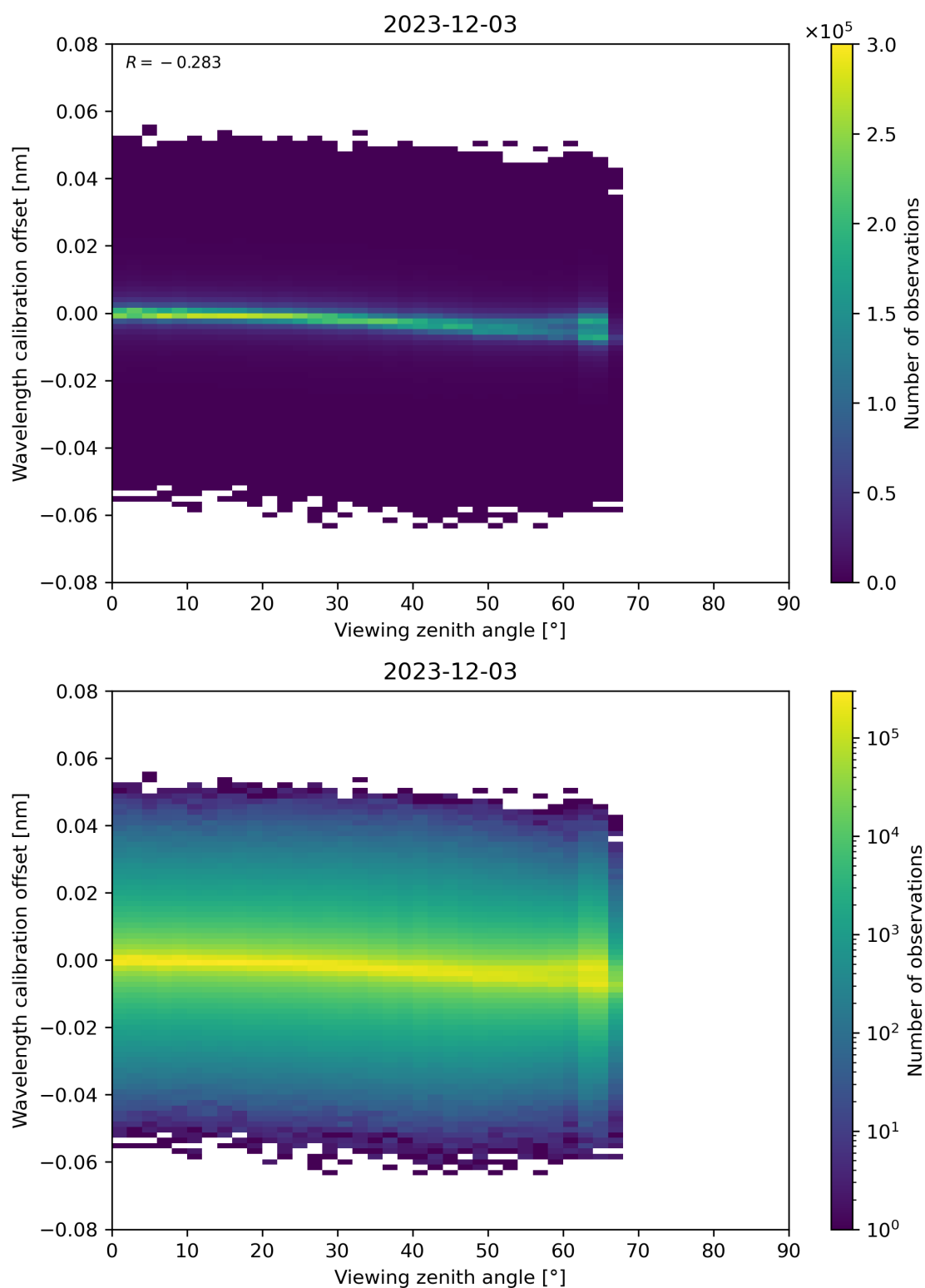
Figure 173: Scatter density plot of “Viewing zenith angle” against “Wavelength calibration offset” for 2023-12-02 to 2023-12-04.
