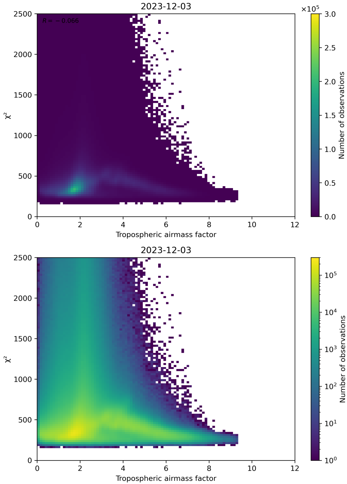
Figure 73: Scatter density plot of “Tropospheric airmass factor” against “ \chi^2 ” for 2023-12-02 to 2023-12-04.
