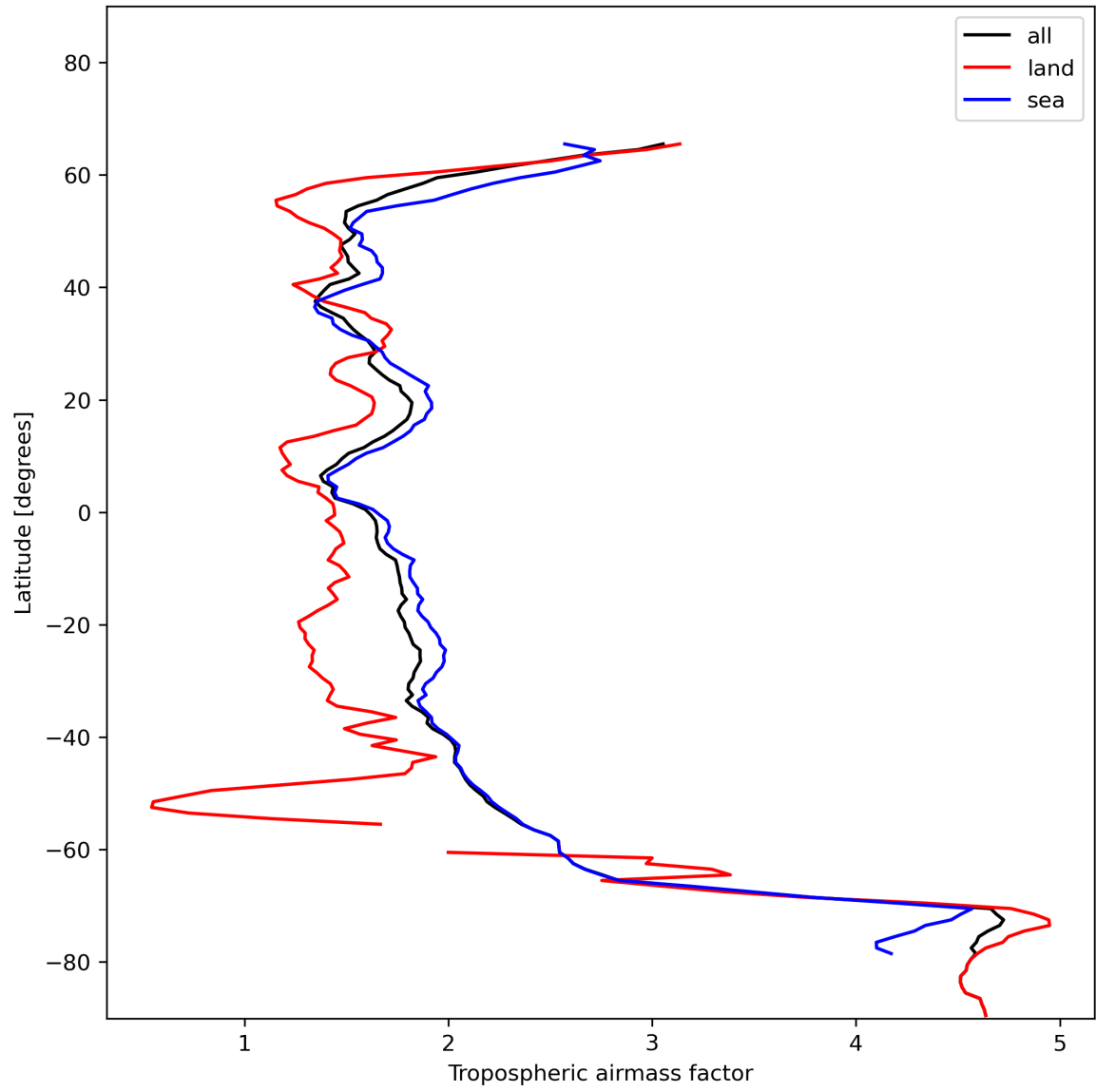
Figure 14: Zonal average of “Tropospheric air mass factor” for 2023-12-02 to 2023-12-04.
