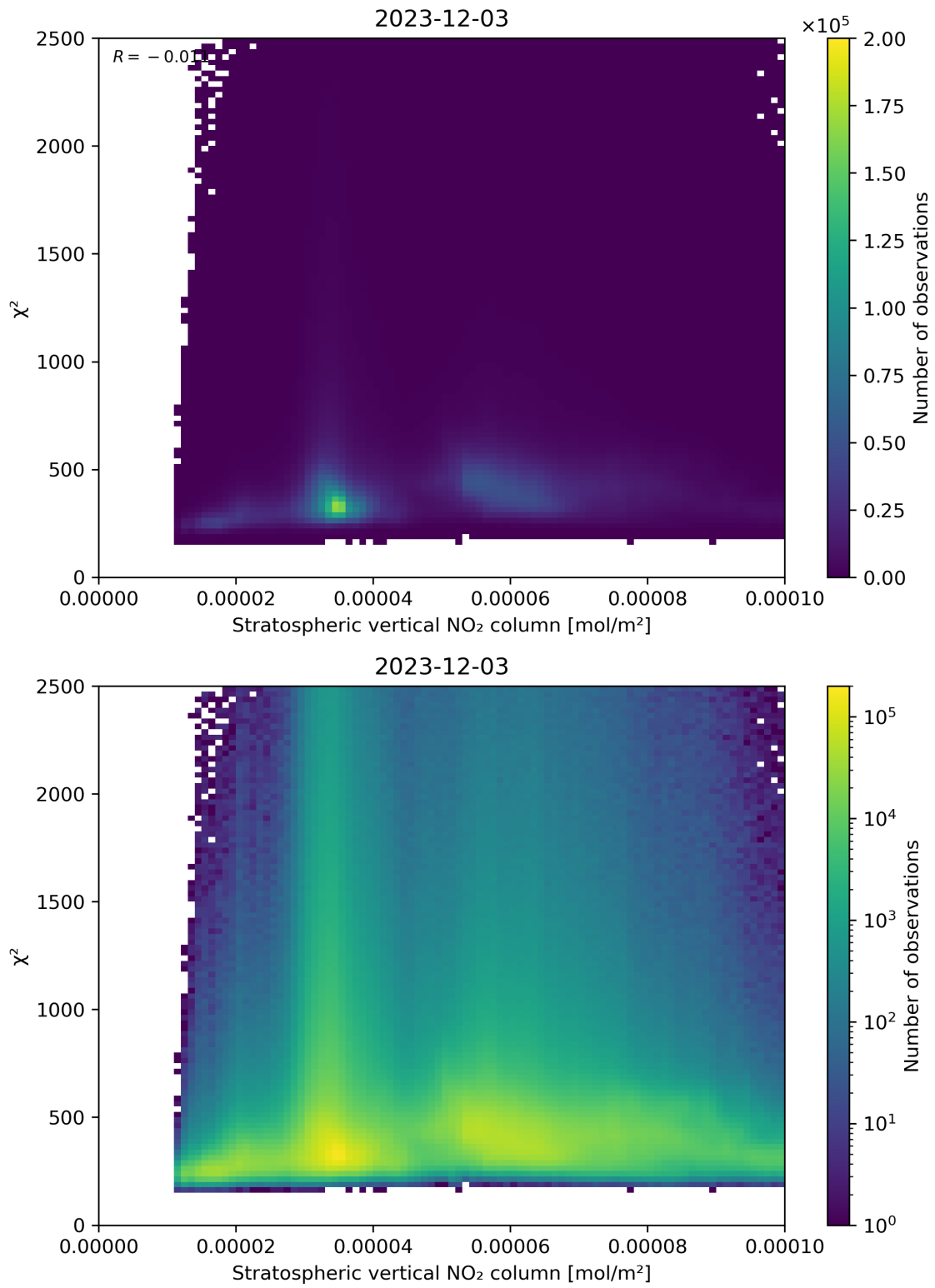
Figure 97: Scatter density plot of “Stratospheric vertical NO 2 column” against “ \chi^2 ” for 2023-12-02 to 2023-12-04.
