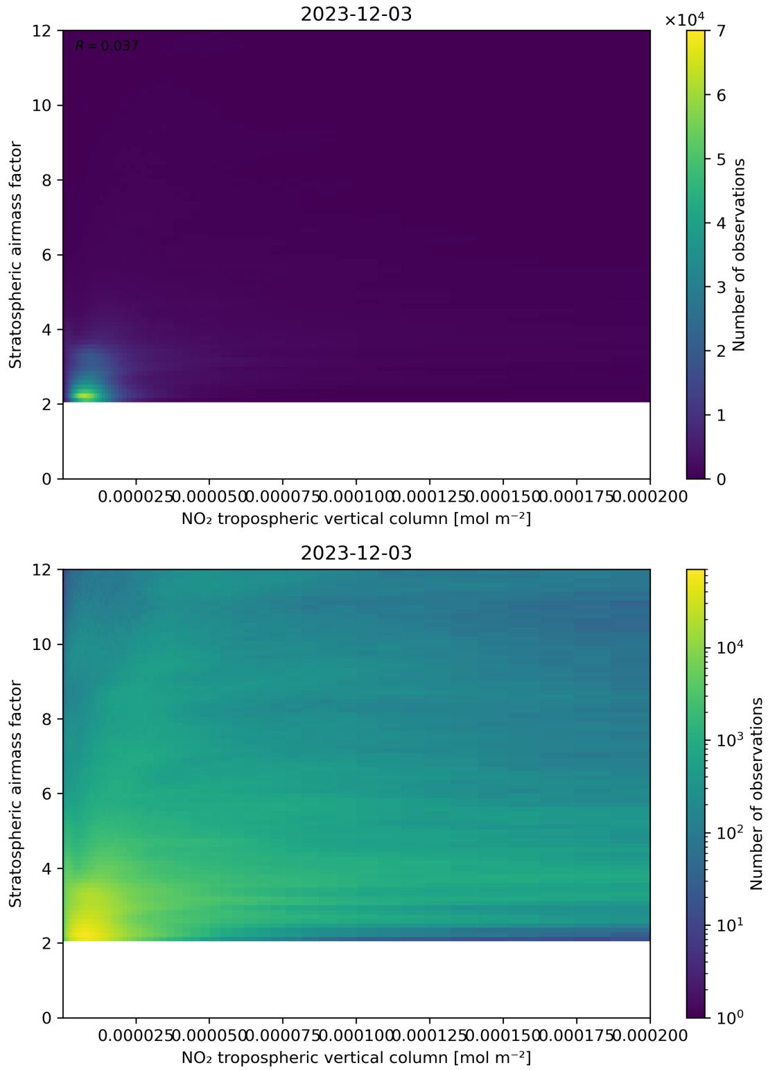
Figure 121: Scatter density plot of “NO 2 tropospheric vertical column” against “Stratospheric air mass factor” for 2023-12-02 to 2023-12-04.
