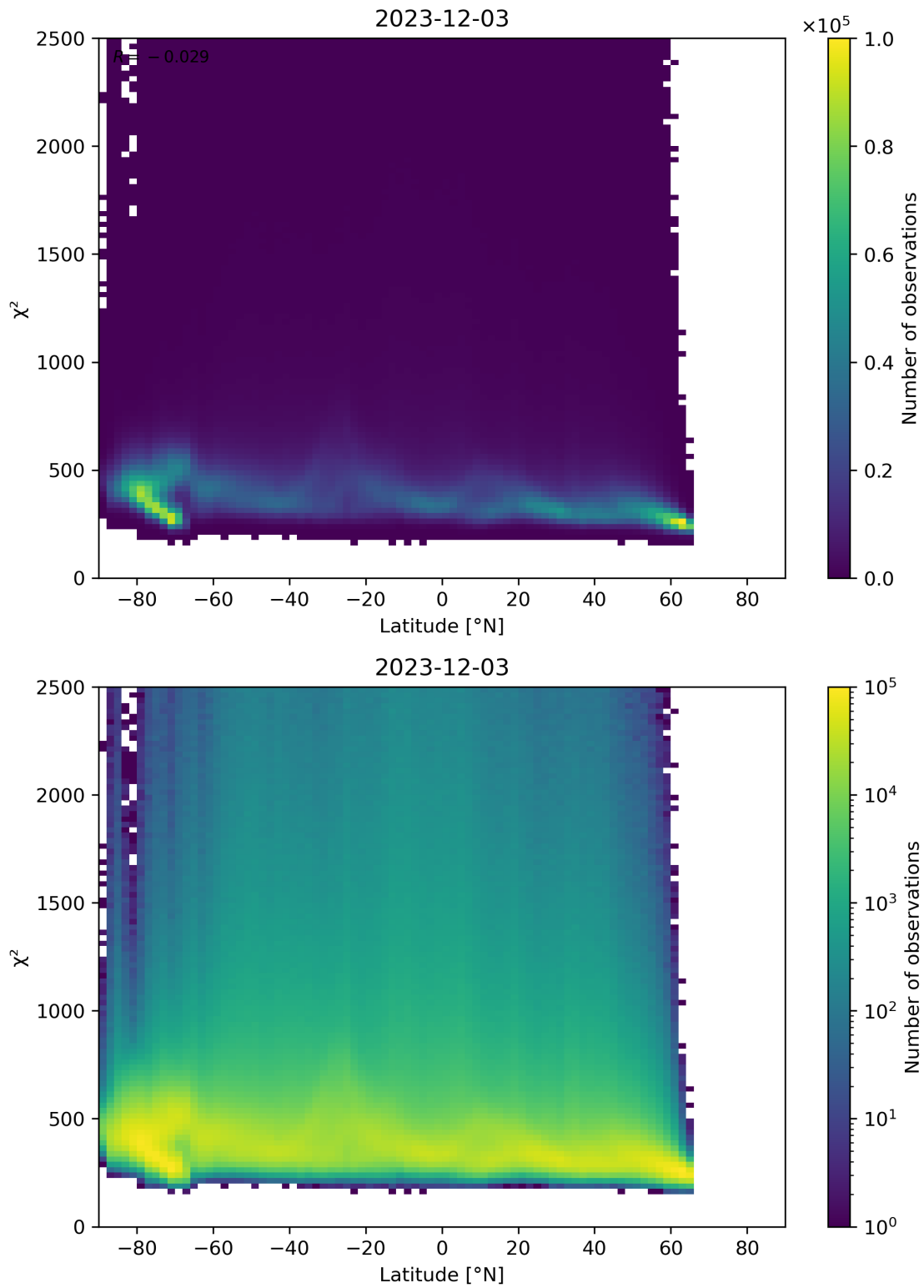
Figure 86: Scatter density plot of “Latitude” against “ \chi^2 ” for 2023-12-02 to 2023-12-04.
