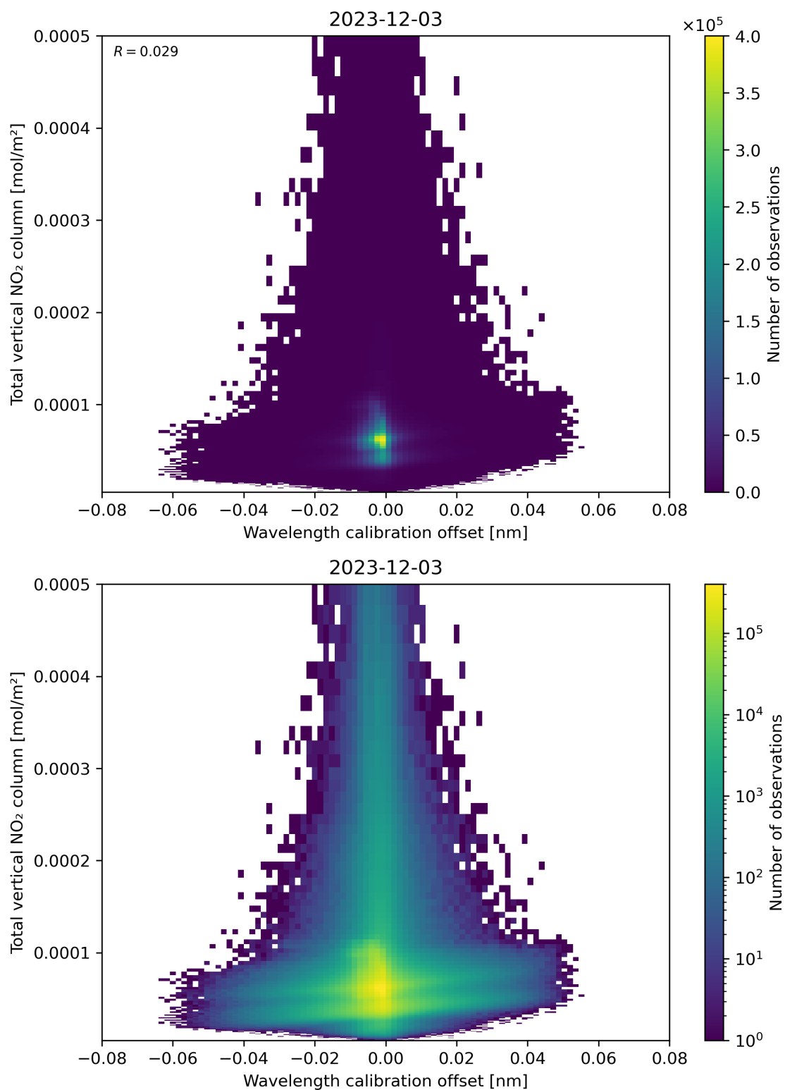
Figure 179: Scatter density plot of “Wavelength calibration offset” against “Total vertical NO 2 column” for 2023-12-02 to 2023-12-04.
