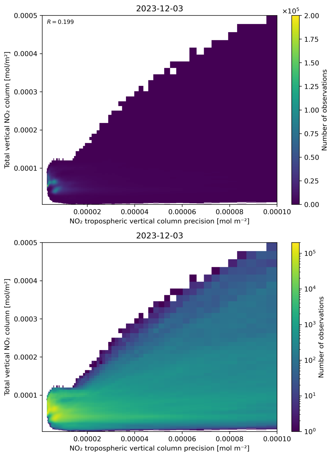
Figure 138: Scatter density plot of “NO 2 tropospheric vertical column precision” against “Total vertical NO 2 column” for 2023-12-02 to 2023-12-04.
