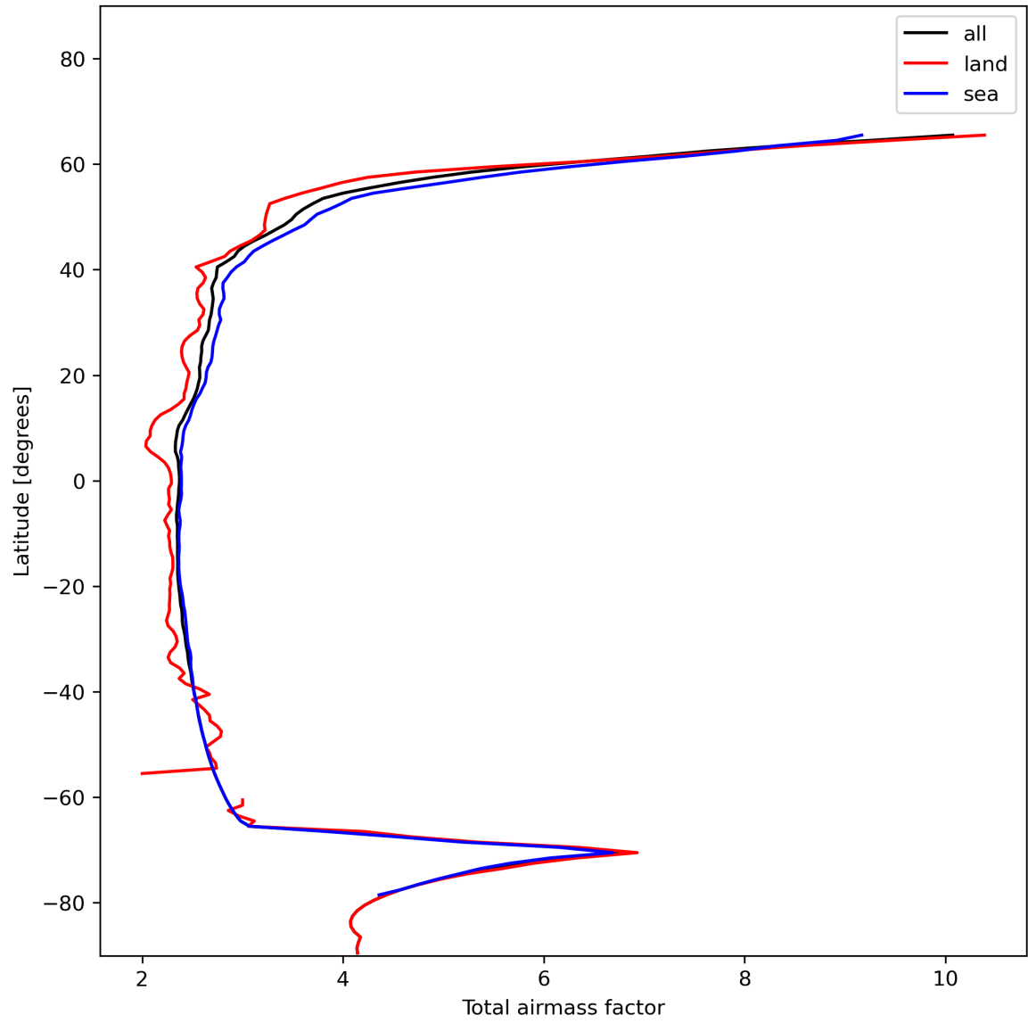
Figure 15: Zonal average of “Total airmass factor” for 2023-12-02 to 2023-12-04.
