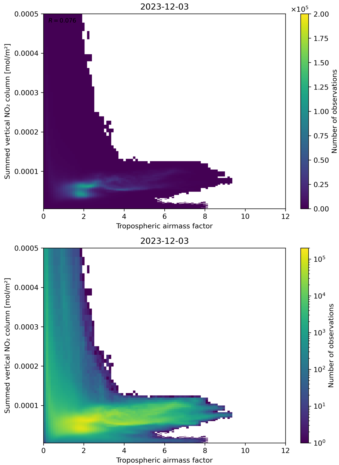
Figure 75: Scatter density plot of “Tropospheric airmass factor” against “Summed vertical NO 2 column” for 2023-12-02 to 2023-12-04.
