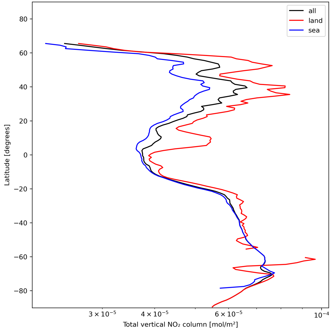
Figure 21: Zonal average of “Total vertical NO 2 column” for 2023-12-02 to 2023-12-04.
