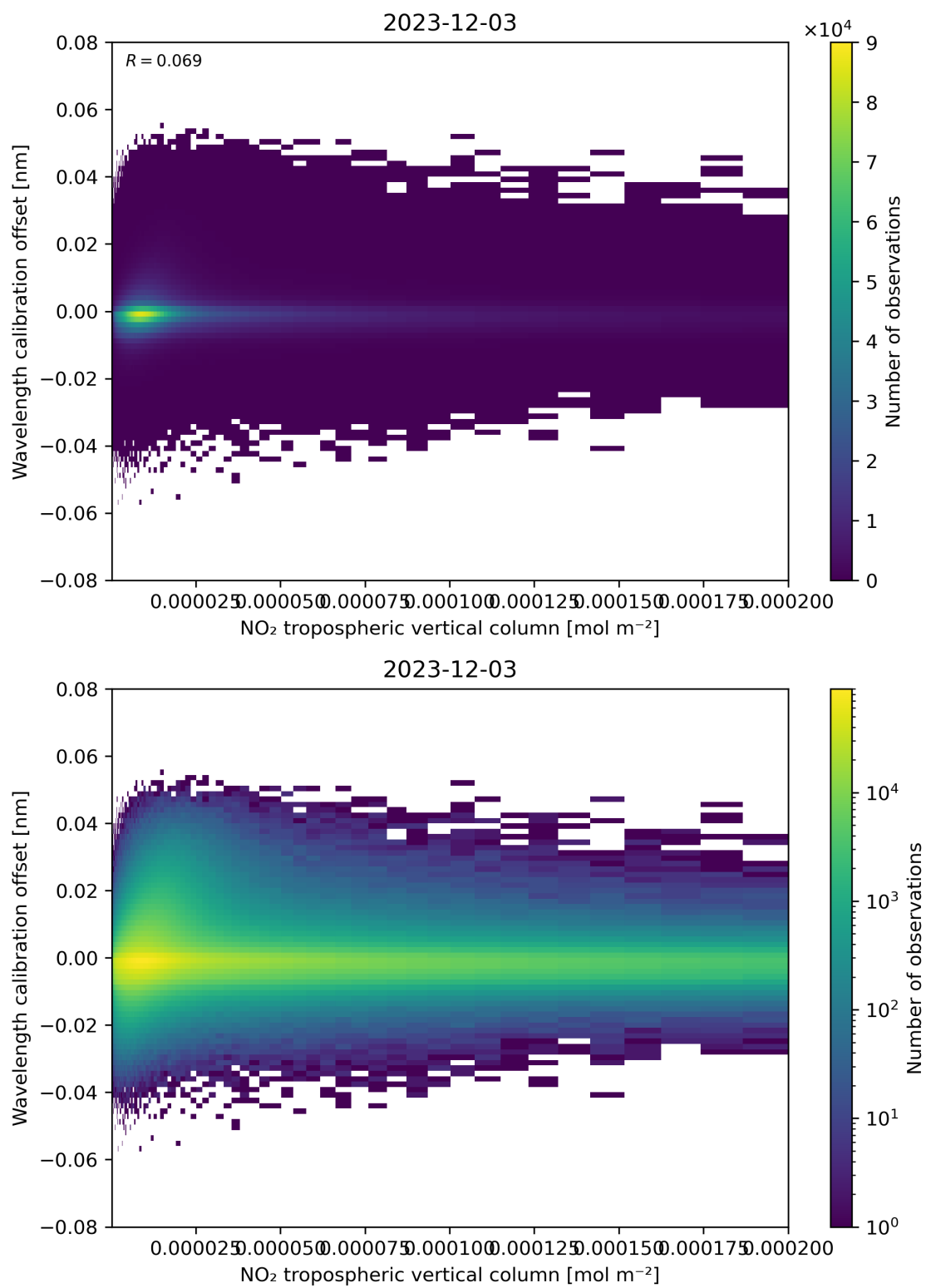
Figure 143: Scatter density plot of “NO 2 tropospheric vertical column” against “Wavelength calibration offset” for 2023-12-02 to 2023-12-04.
