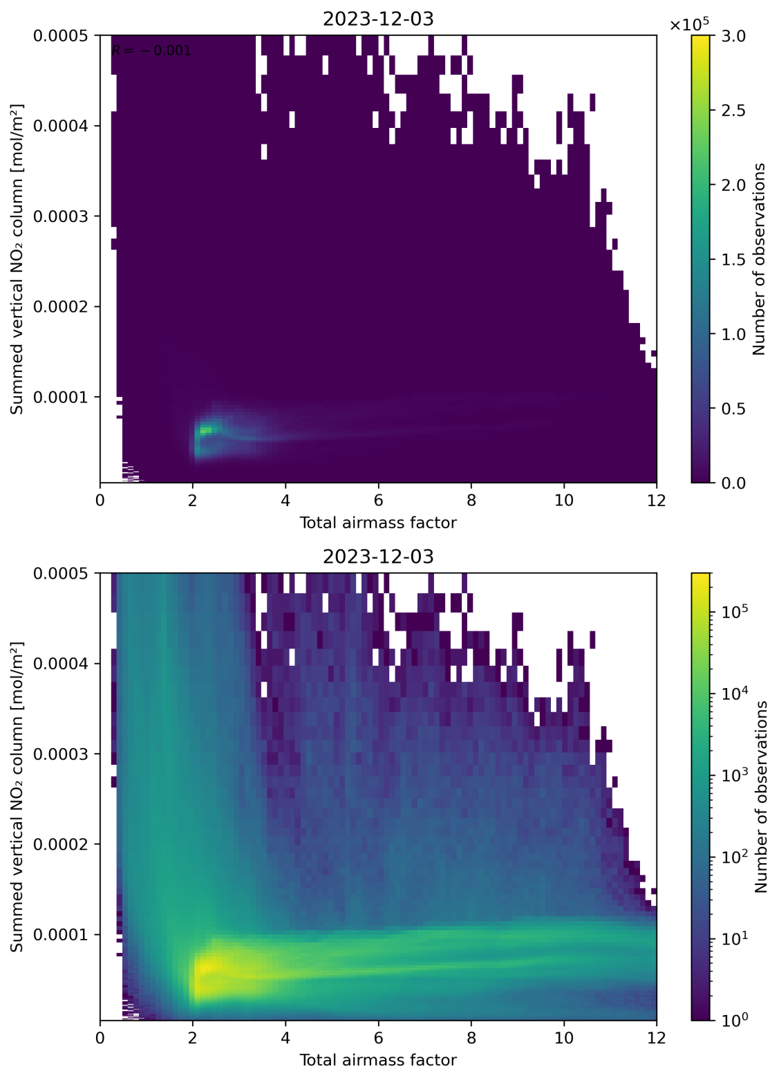
Figure 65: Scatter density plot of “Total airmass factor” against “Summed vertical NO 2 column” for 2023-12-02 to 2023-12-04.
