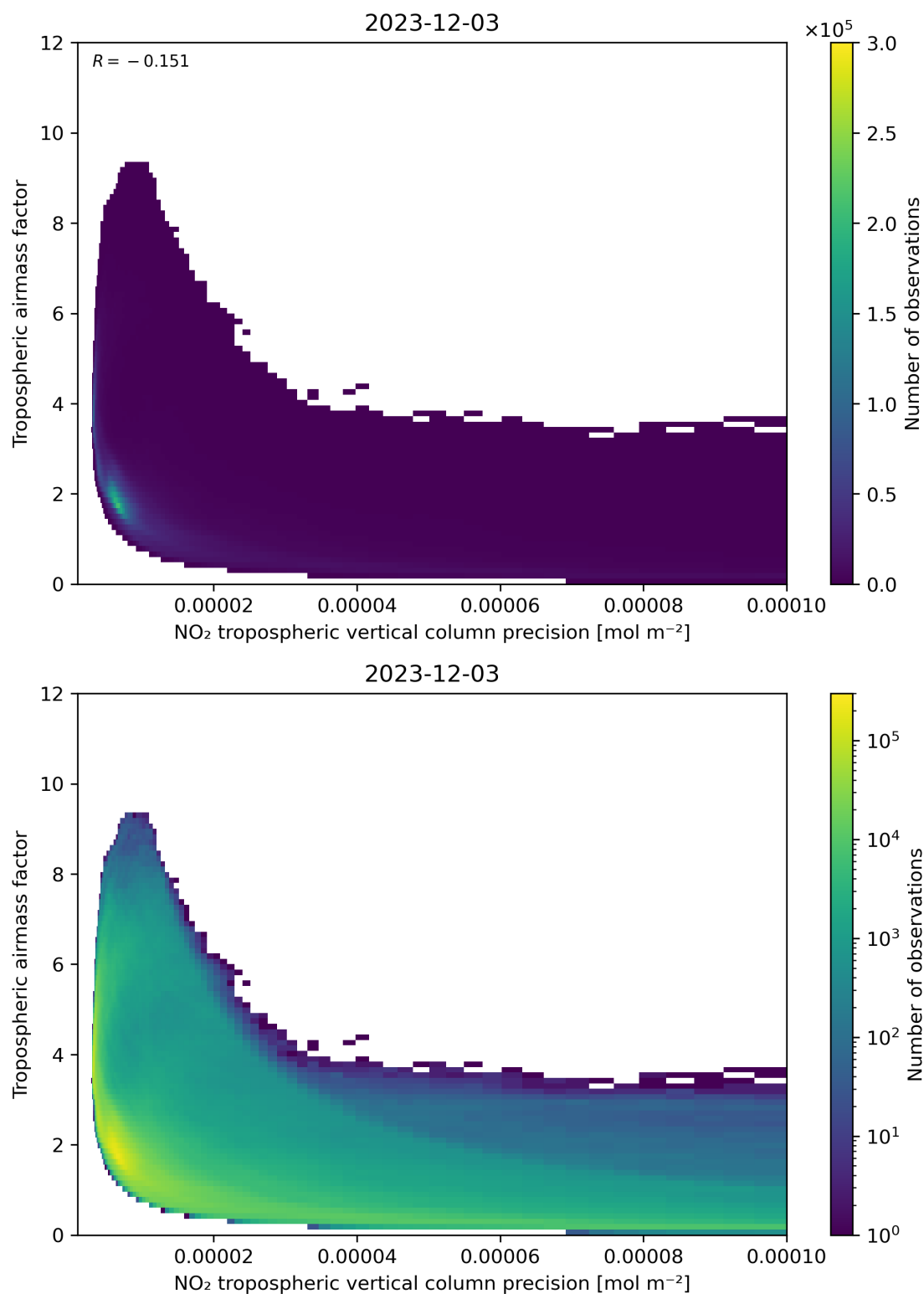
Figure 133: Scatter density plot of “NO 2 tropospheric vertical column precision” against “Tropospheric airmass factor” for 2023-12-02 to 2023-12-04.
