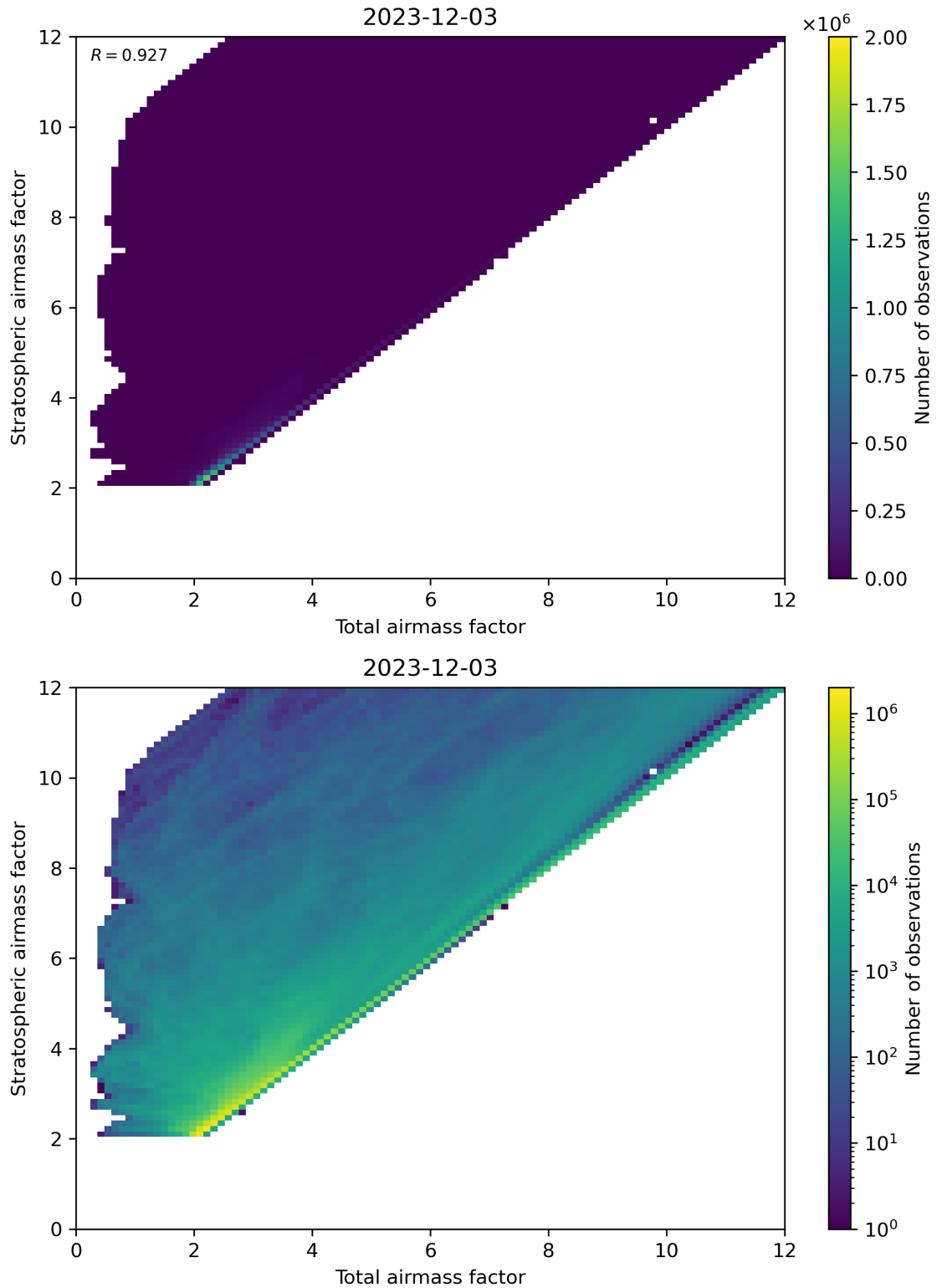
Figure 62: Scatter density plot of “Total airmass factor” against “Stratospheric airmass factor” for 2023-12-02 to 2023-12-04.
