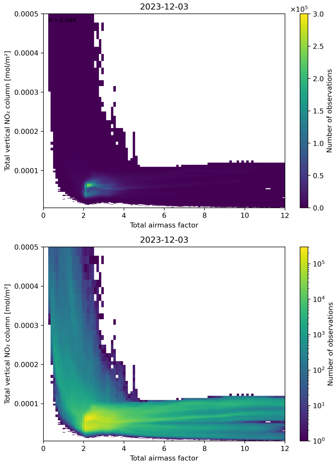
Figure 67: Scatter density plot of “Total airmass factor” against “Total vertical NO 2 column” for 2023-12-02 to 2023-12-04.
