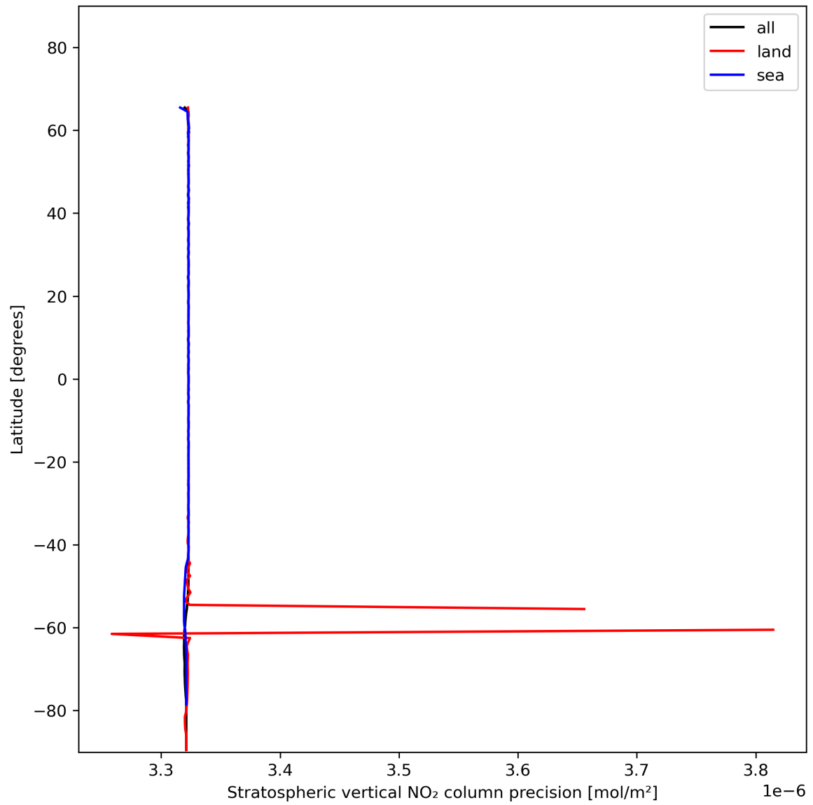
Figure 20: Zonal average of “Stratospheric vertical NO 2 column precision” for 2023-12-02 to 2023-12-04.
