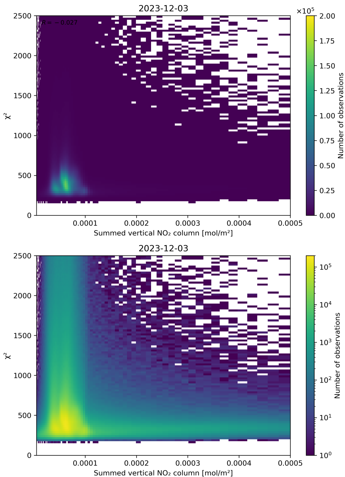
Figure 104: Scatter density plot of “Summed vertical NO 2 column” against “ \chi^2 ” for 2023-12-02 to 2023-12-04.
