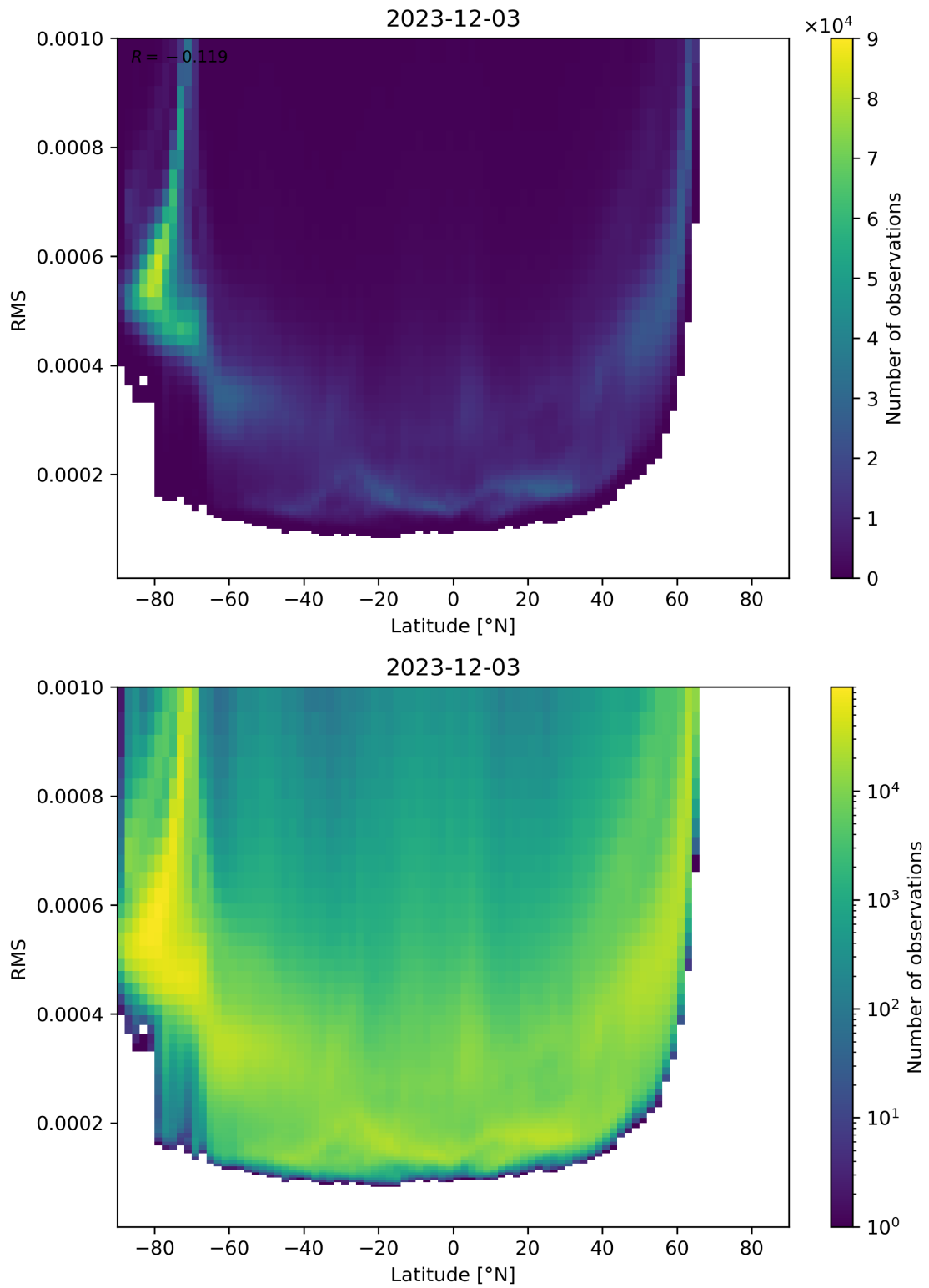
Figure 94: Scatter density plot of “Latitude” against “RMS” for 2023-12-02 to 2023-12-04.
