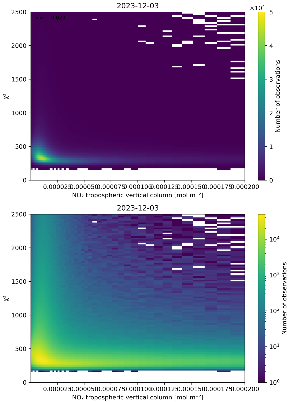
Figure 124: Scatter density plot of “NO 2 tropospheric vertical column” against “ \chi^2 ” for 2023-12-02 to 2023-12-04.
