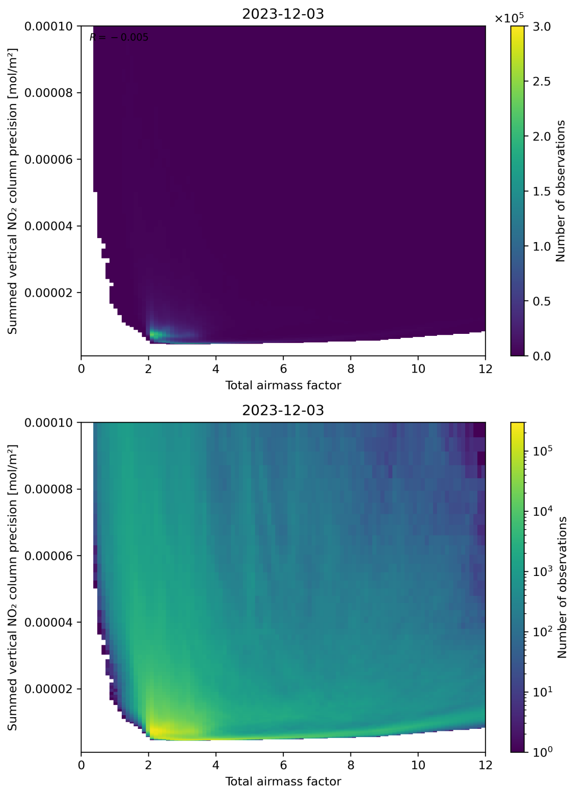
Figure 66: Scatter density plot of “Total airmass factor” against “Summed vertical NO 2 column precision” for 2023-12-02 to 2023-12-04.
