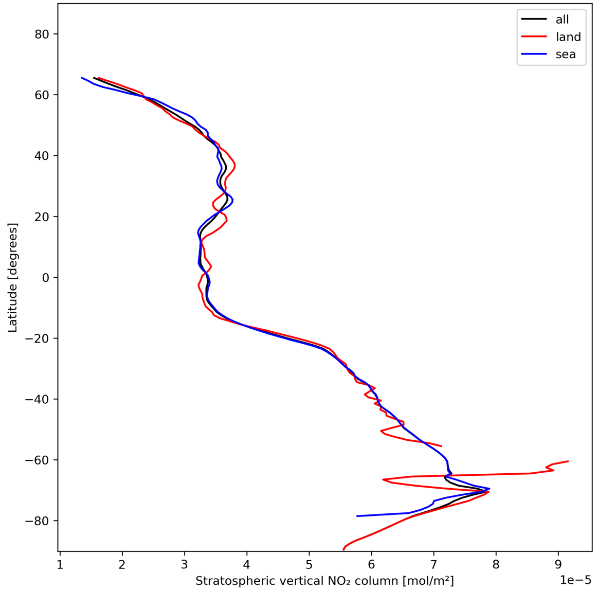
Figure 19: Zonal average of “Stratospheric vertical NO 2 column” for 2023-12-02 to 2023-12-04.
