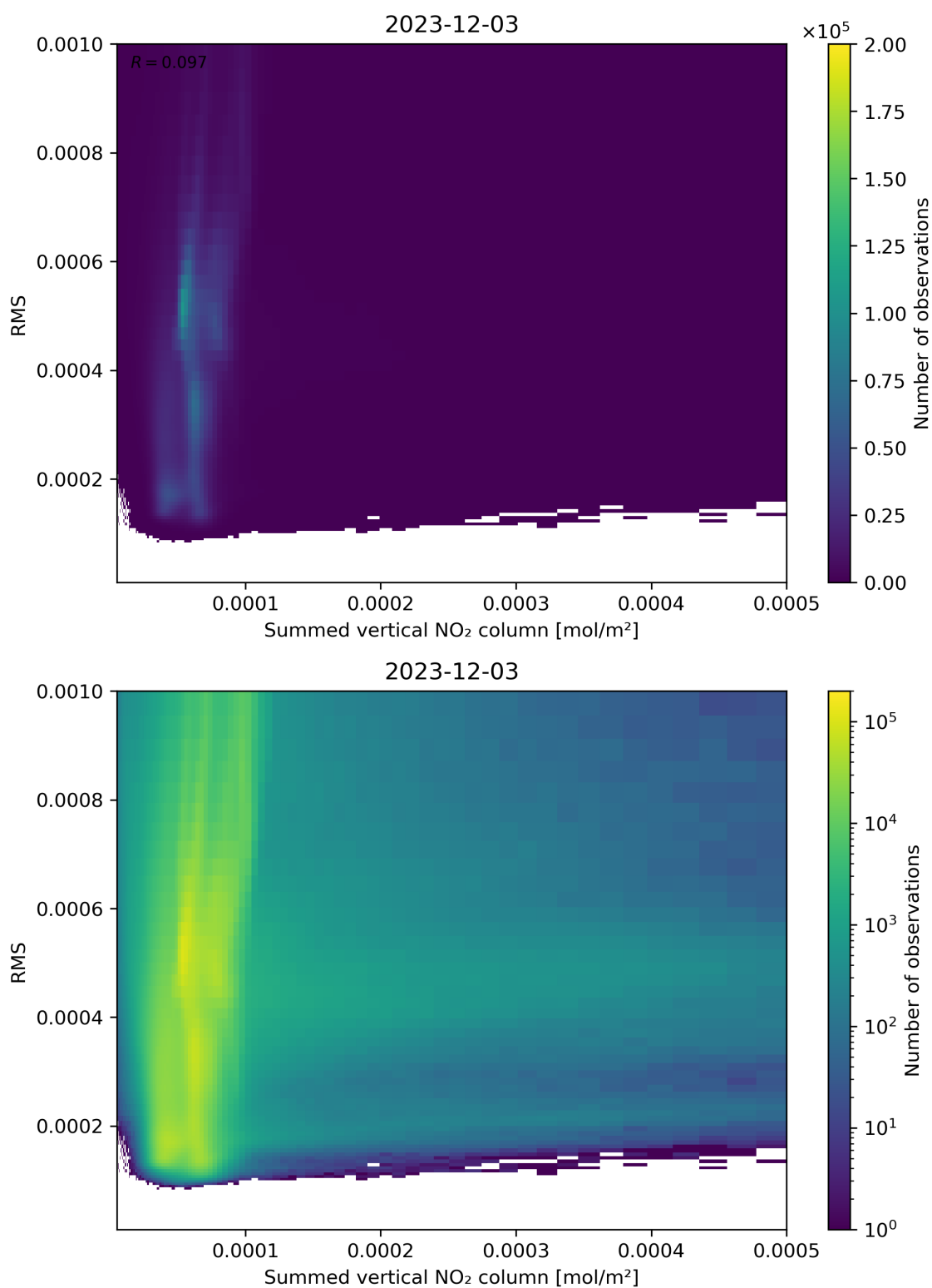
Figure 109: Scatter density plot of “Summed vertical NO 2 column” against “RMS” for 2023-12-02 to 2023-12-04.
