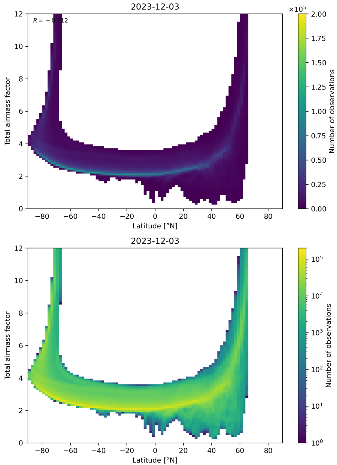
Figure 84: Scatter density plot of “Latitude” against “Total airmass factor” for 2023-12-02 to 2023-12-04.
