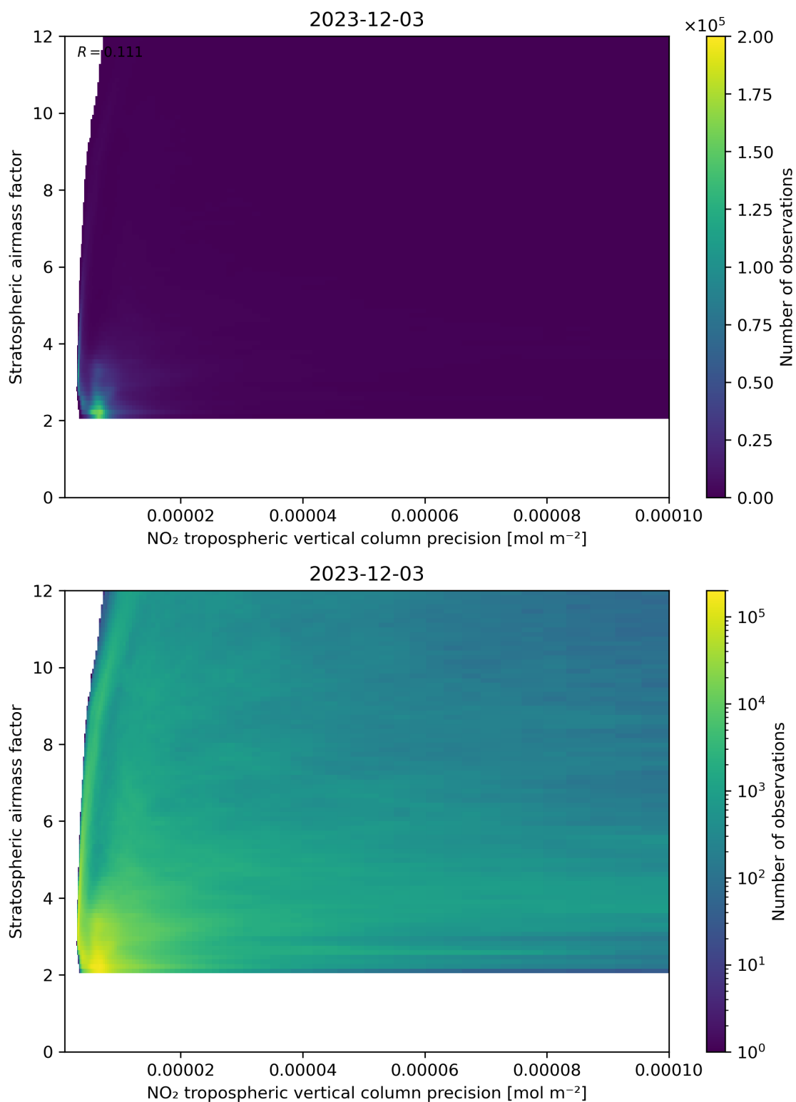
Figure 131: Scatter density plot of “NO 2 tropospheric vertical column precision” against “Stratospheric airmass factor” for 2023-12-02 to 2023-12-04.
