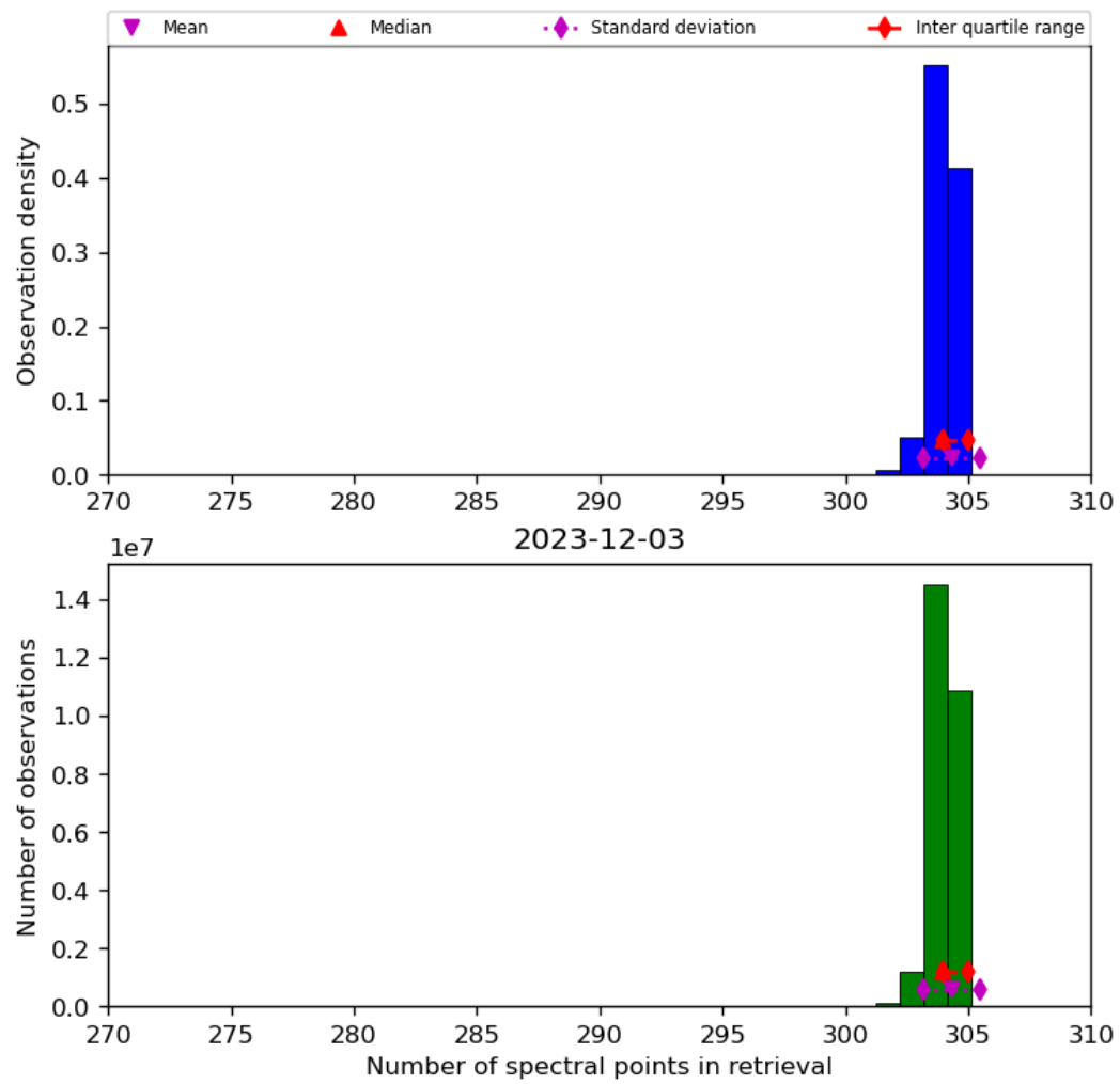
Figure 33: Histogram of “Number of spectral points in retrieval” for 2023-12-02 to 2023-12-04
