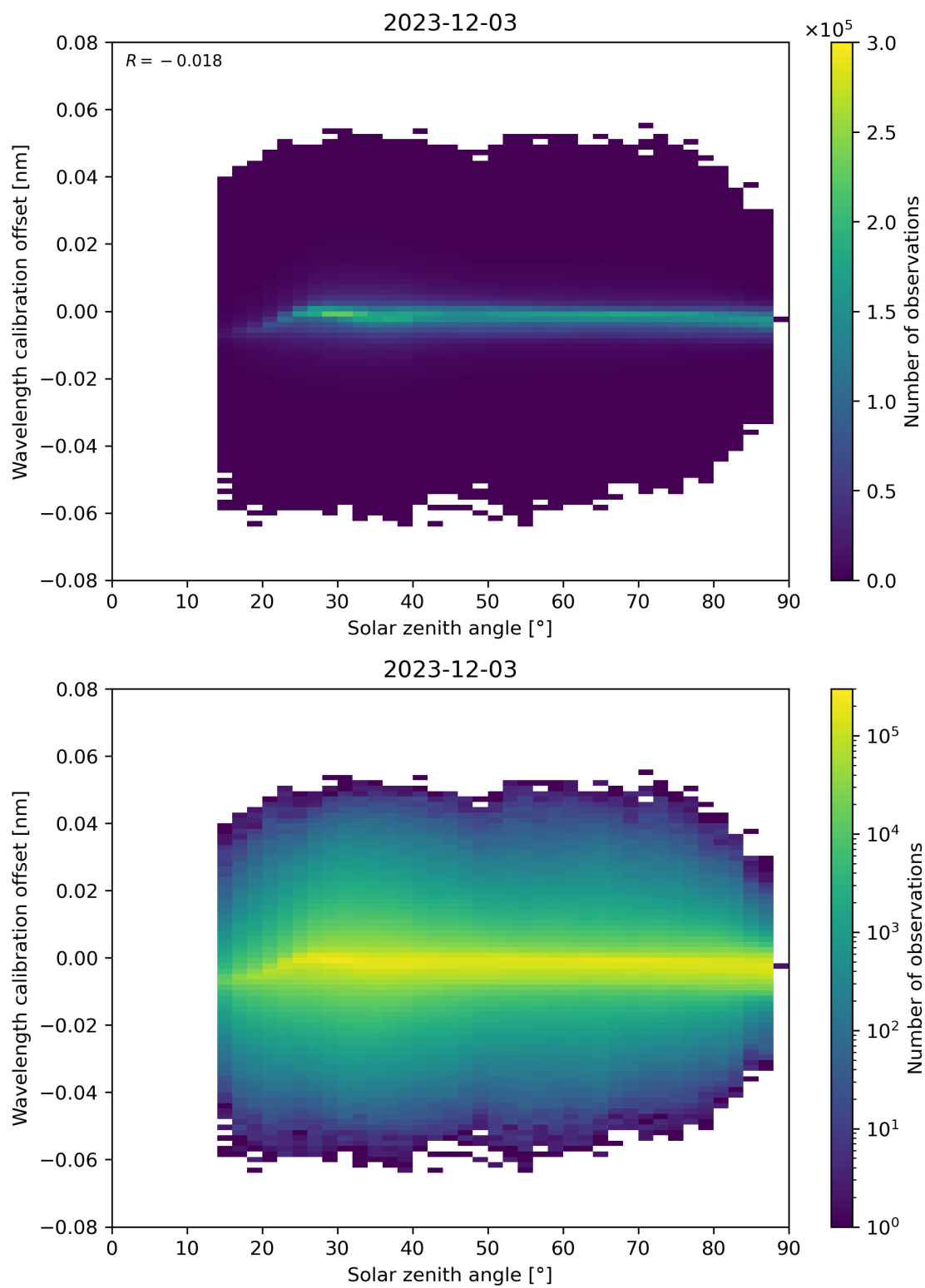
Figure 158: Scatter density plot of “Solar zenith angle” against “Wavelength calibration offset” for 2023-12-02 to 2023-12-04.
