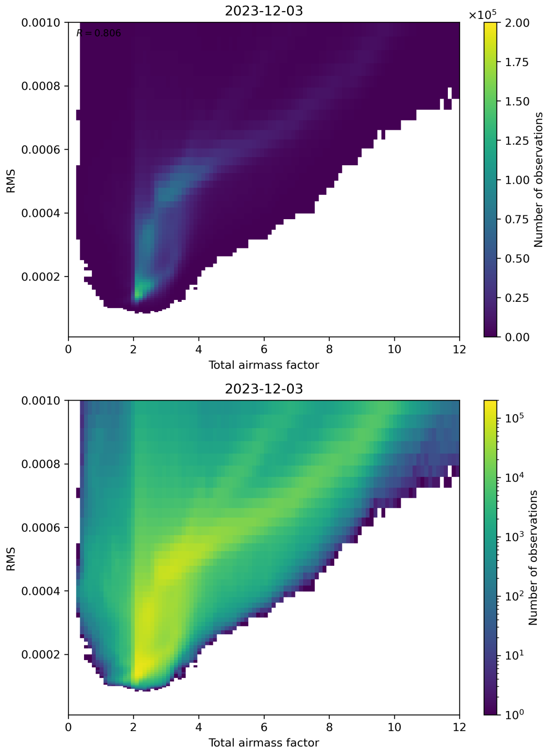
Figure 69: Scatter density plot of “Total airmass factor” against “RMS” for 2023-12-02 to 2023-12-04.
