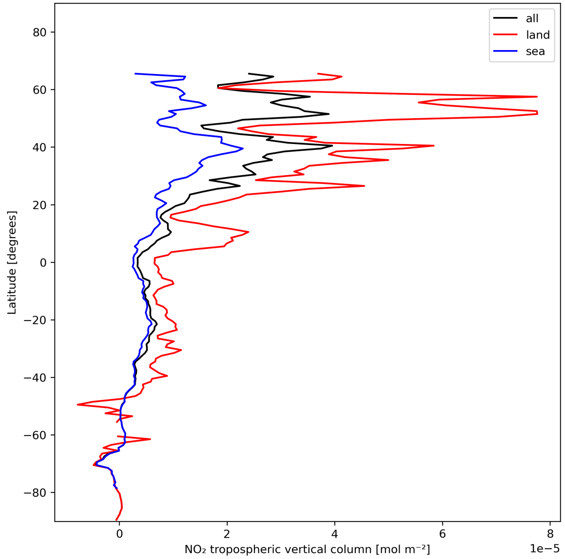
Figure 12: Zonal average of “NO 2 tropospheric vertical column” for 2023-12-02 to 2023-12-04.
