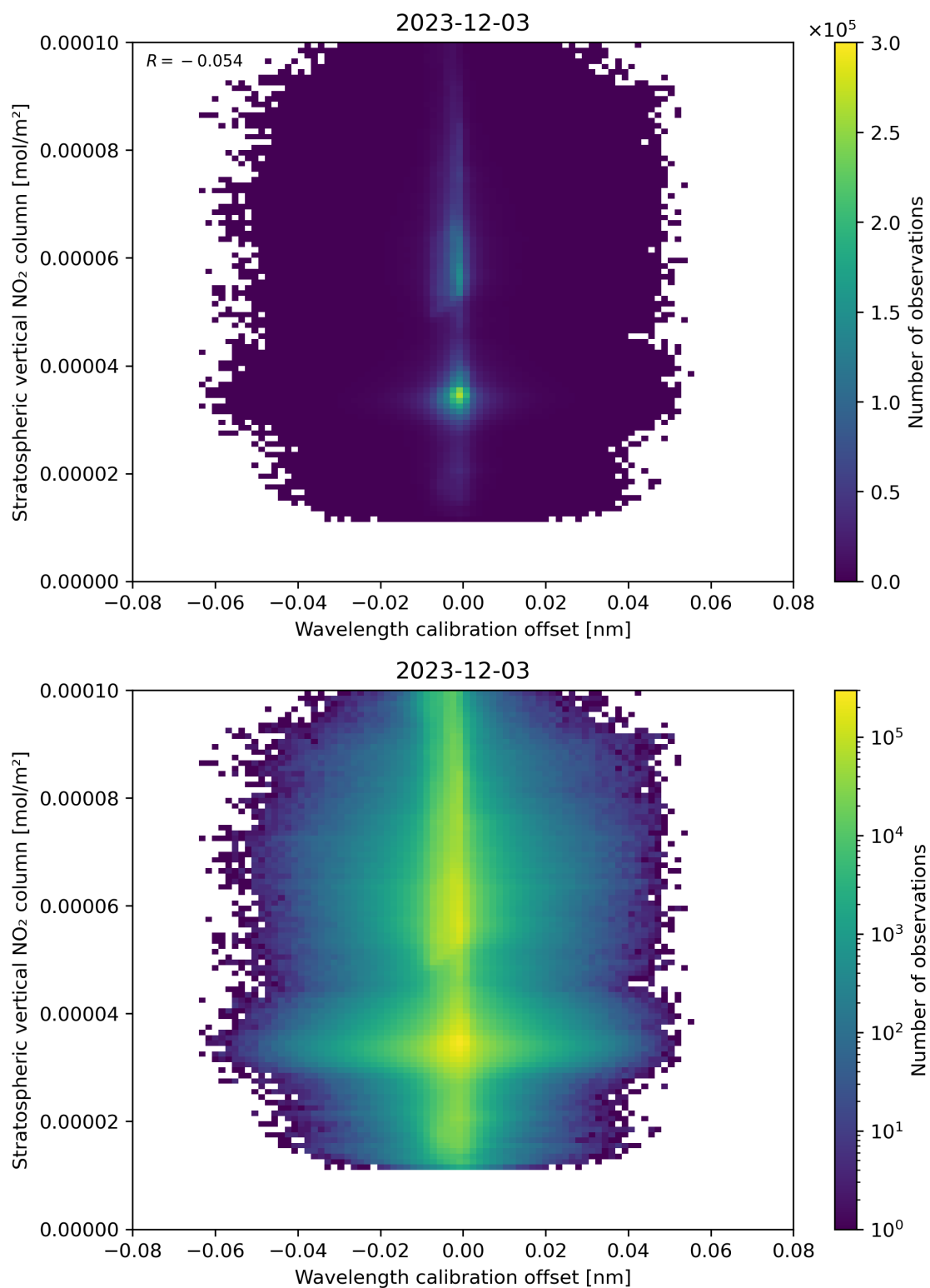
Figure 176: Scatter density plot of “Wavelength calibration offset” against “Stratospheric vertical NO 2 column” for 2023-12-02 to 2023-12-04.
