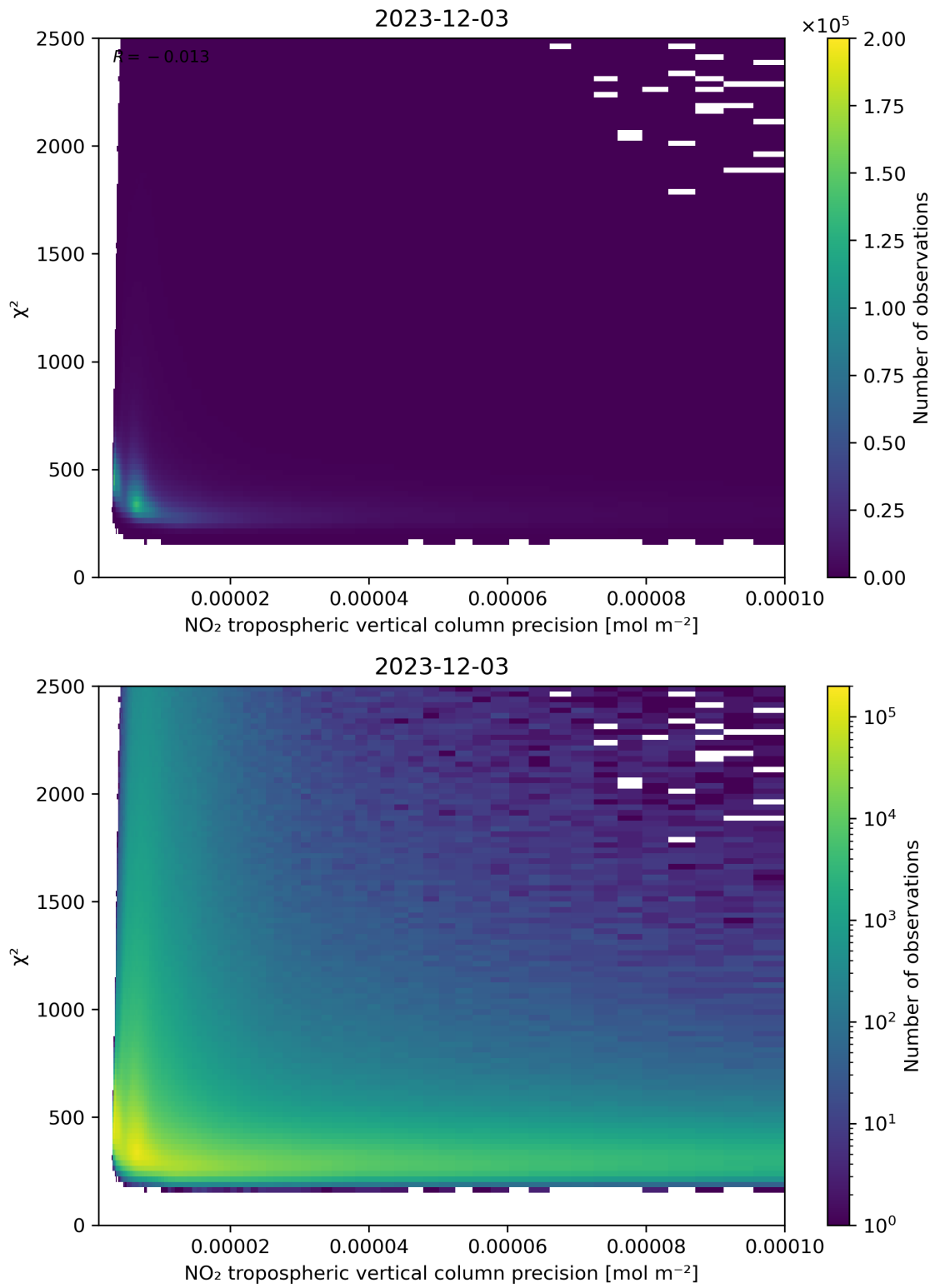
Figure 134: Scatter density plot of “NO 2 tropospheric vertical column precision” against “ \chi^2 ” for 2023-12-02 to 2023-12-04.
