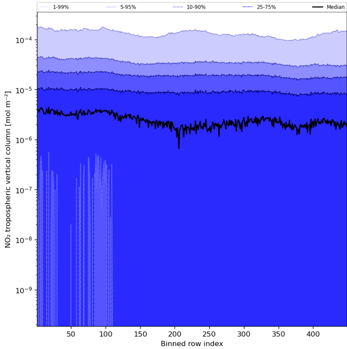
Figure 46: Along track statistics of “NO 2 tropospheric vertical column” for 2023-12-02 to 2023-12-04
