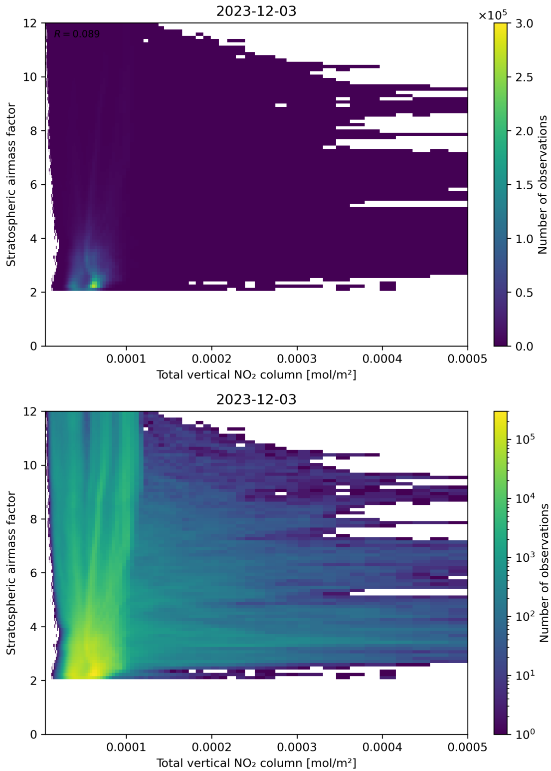
Figure 110: Scatter density plot of “Total vertical NO 2 column” against “Stratospheric air mass factor” for 2023-12-02 to 2023-12-04.
