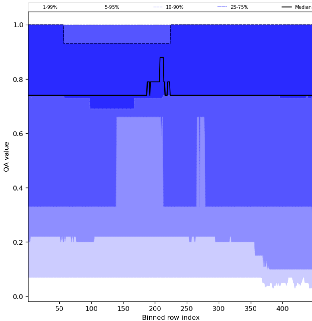
Figure 45: Along track statistics of “QA value” for 2023-12-02 to 2023-12-04
