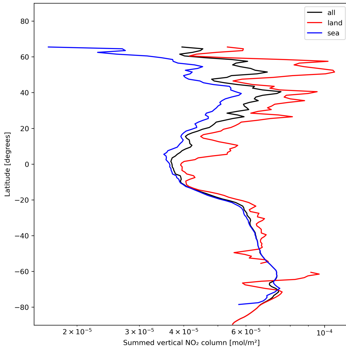
Figure 23: Zonal average of “Summed vertical NO 2 column” for 2023-12-02 to 2023-12-04.
