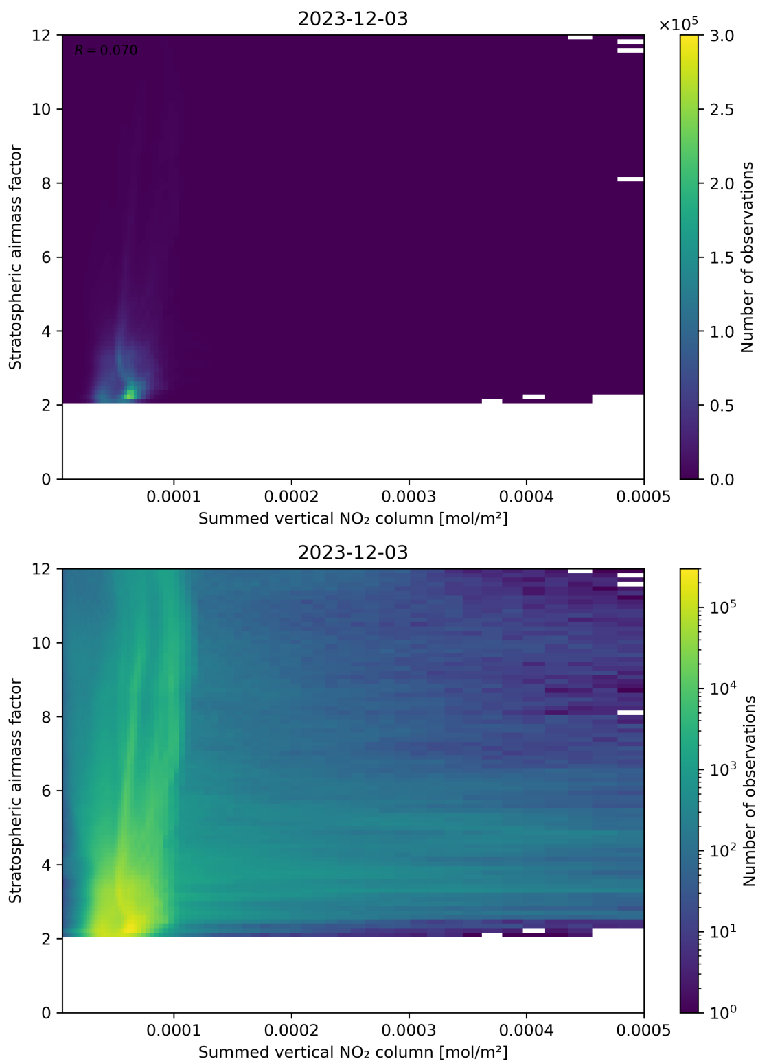
Figure 103: Scatter density plot of “Summed vertical NO 2 column” against “Stratospheric airmass factor” for 2023-12-02 to 2023-12-04.
