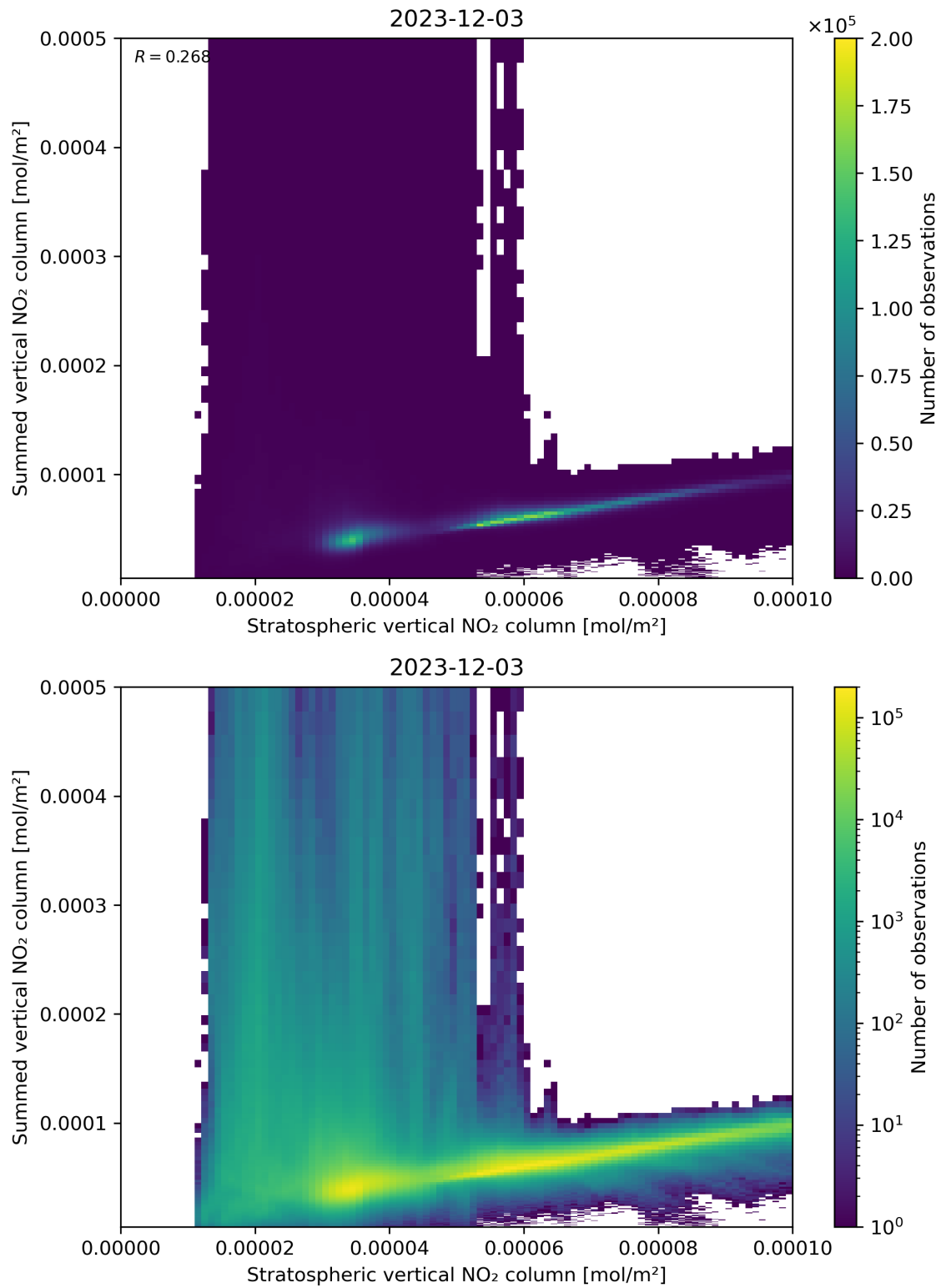
Figure 98: Scatter density plot of “Stratospheric vertical NO 2 column” against “Summed vertical NO 2 column” for 2023-12-02 to 2023-12-04.
