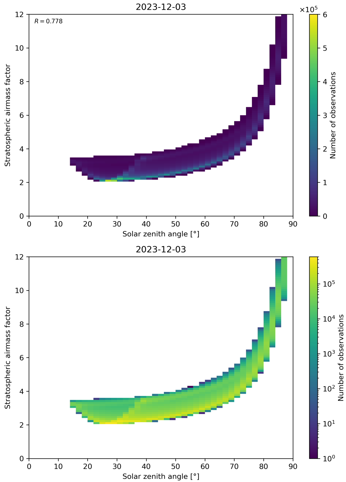
Figure 145: Scatter density plot of “Solar zenith angle” against “Stratospheric airmass factor” for 2023-12-02 to 2023-12-04.
