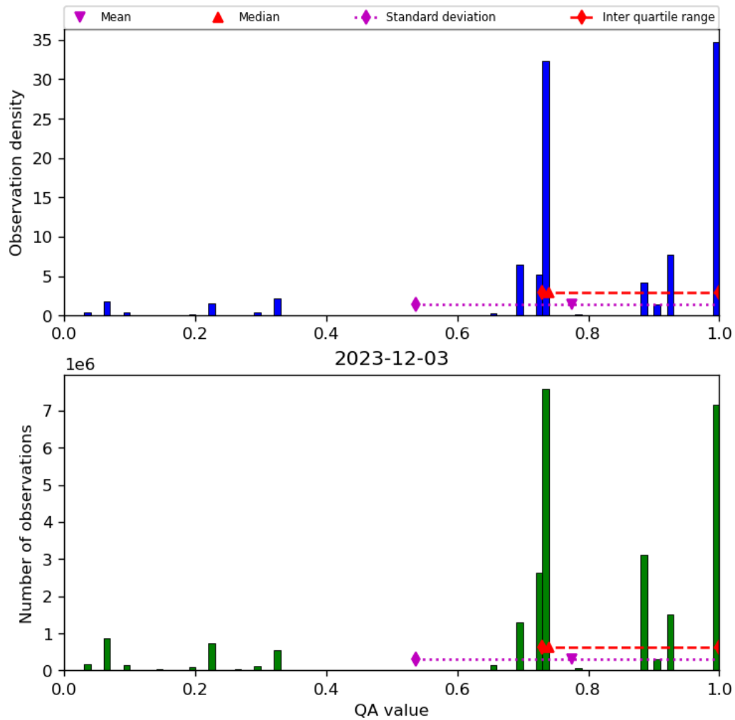
Figure 28: Histogram of “QA value” for 2023-12-02 to 2023-12-04
