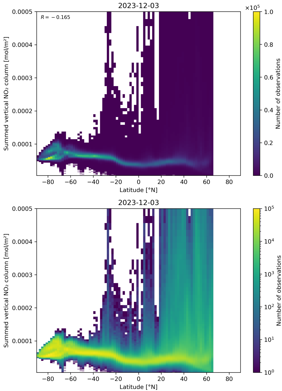
Figure 88: Scatter density plot of “Latitude” against “Summed vertical NO 2 column” for 2023-12-02 to 2023-12-04.
