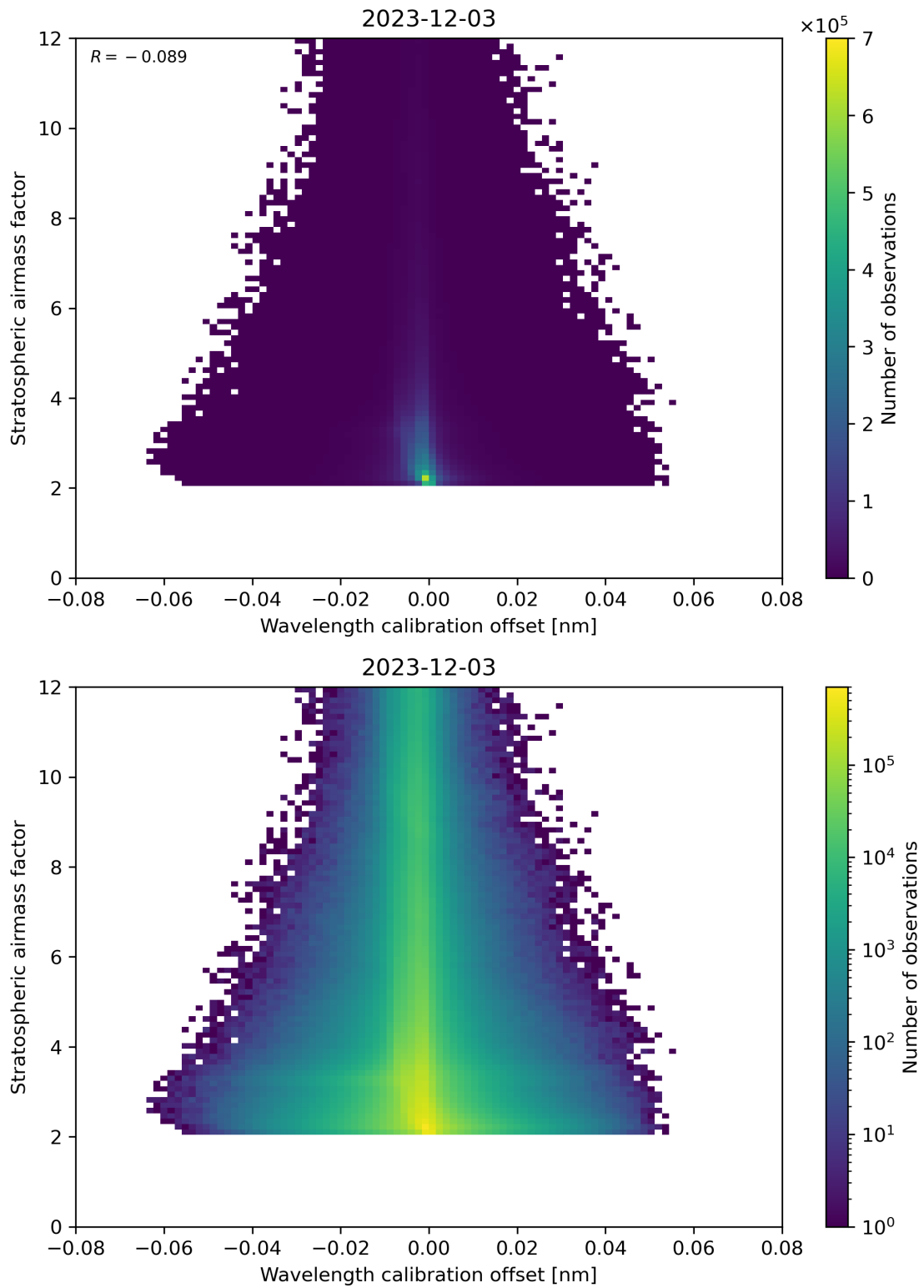
Figure 174: Scatter density plot of “Wavelength calibration offset” against “Stratospheric air mass factor” for 2023-12-02 to 2023-12-04.
