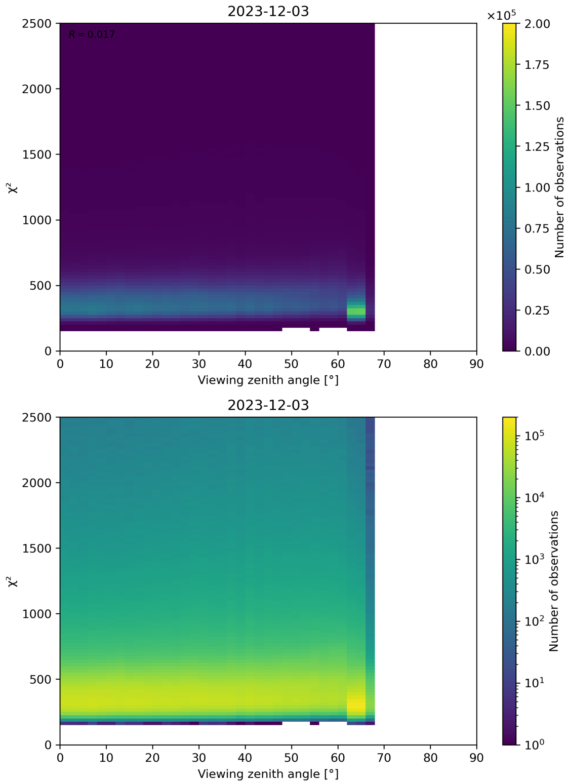
Figure 162: Scatter density plot of “Viewing zenith angle” against “ \chi^2 ” for 2023-12-02 to 2023-12-04.
