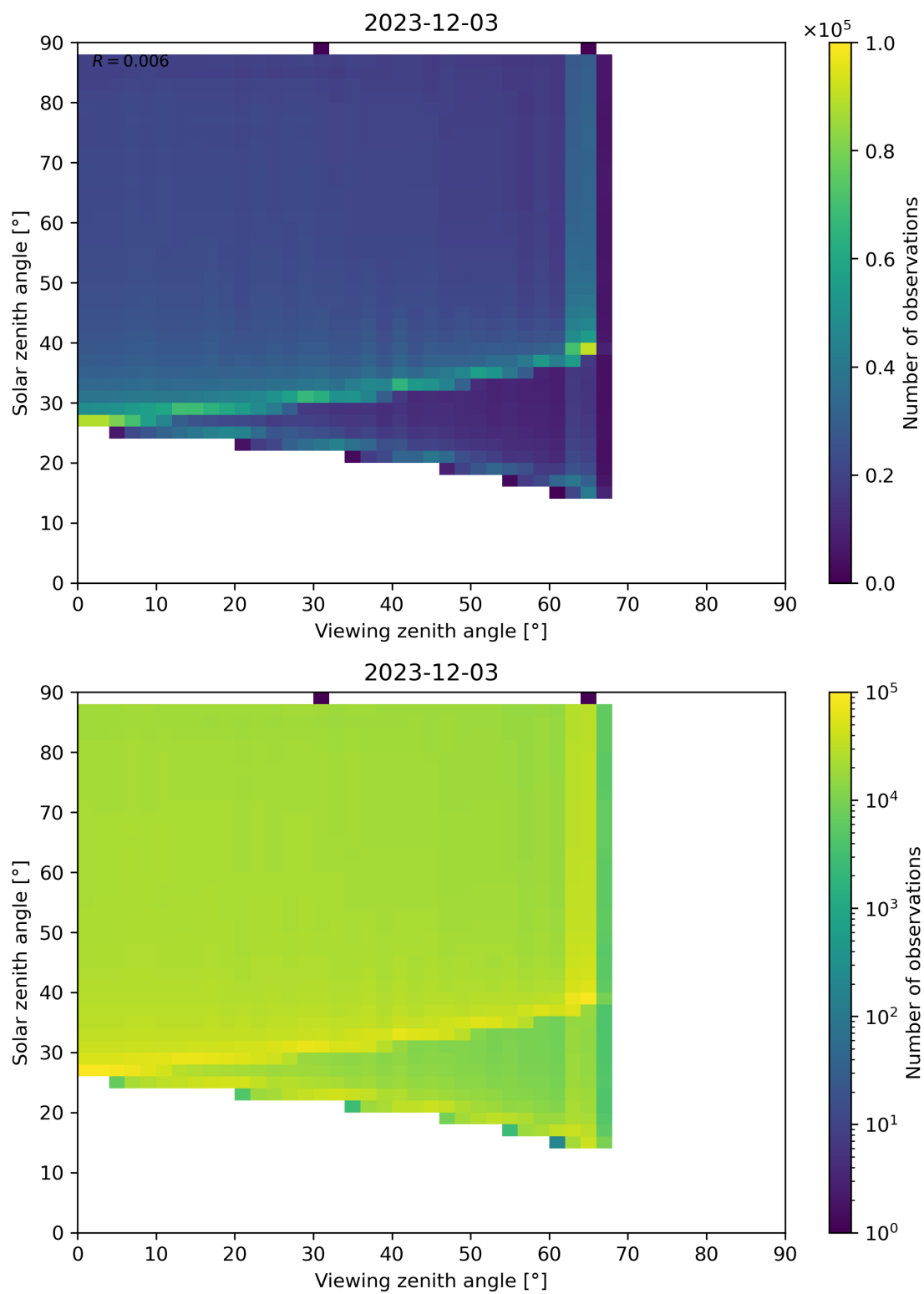
Figure 172: Scatter density plot of “Viewing zenith angle” against “Solar zenith angle” for 2023-12-02 to 2023-12-04.
