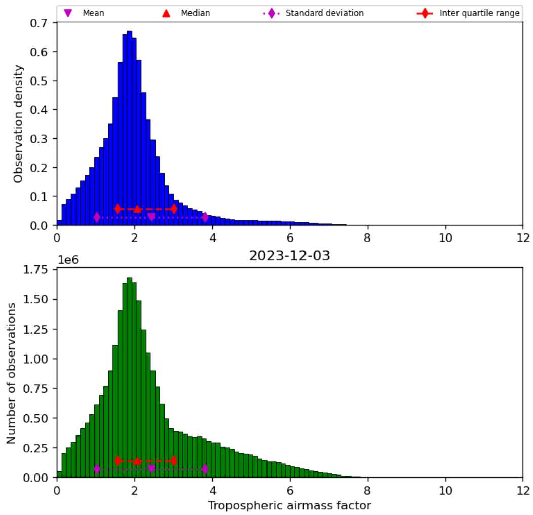
Figure 31: Histogram of “Tropospheric airmass factor” for 2023-12-02 to 2023-12-04
