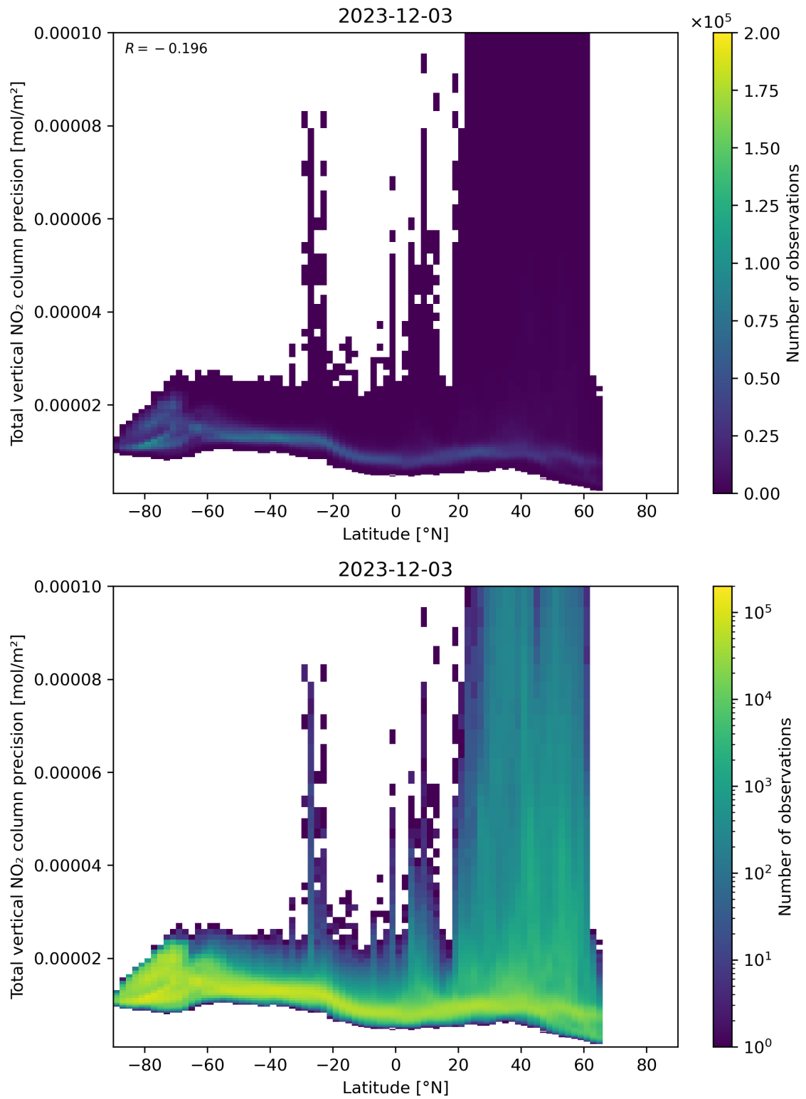
Figure 91: Scatter density plot of “Latitude” against “Total vertical NO 2 column precision” for 2023-12-02 to 2023-12-04.
