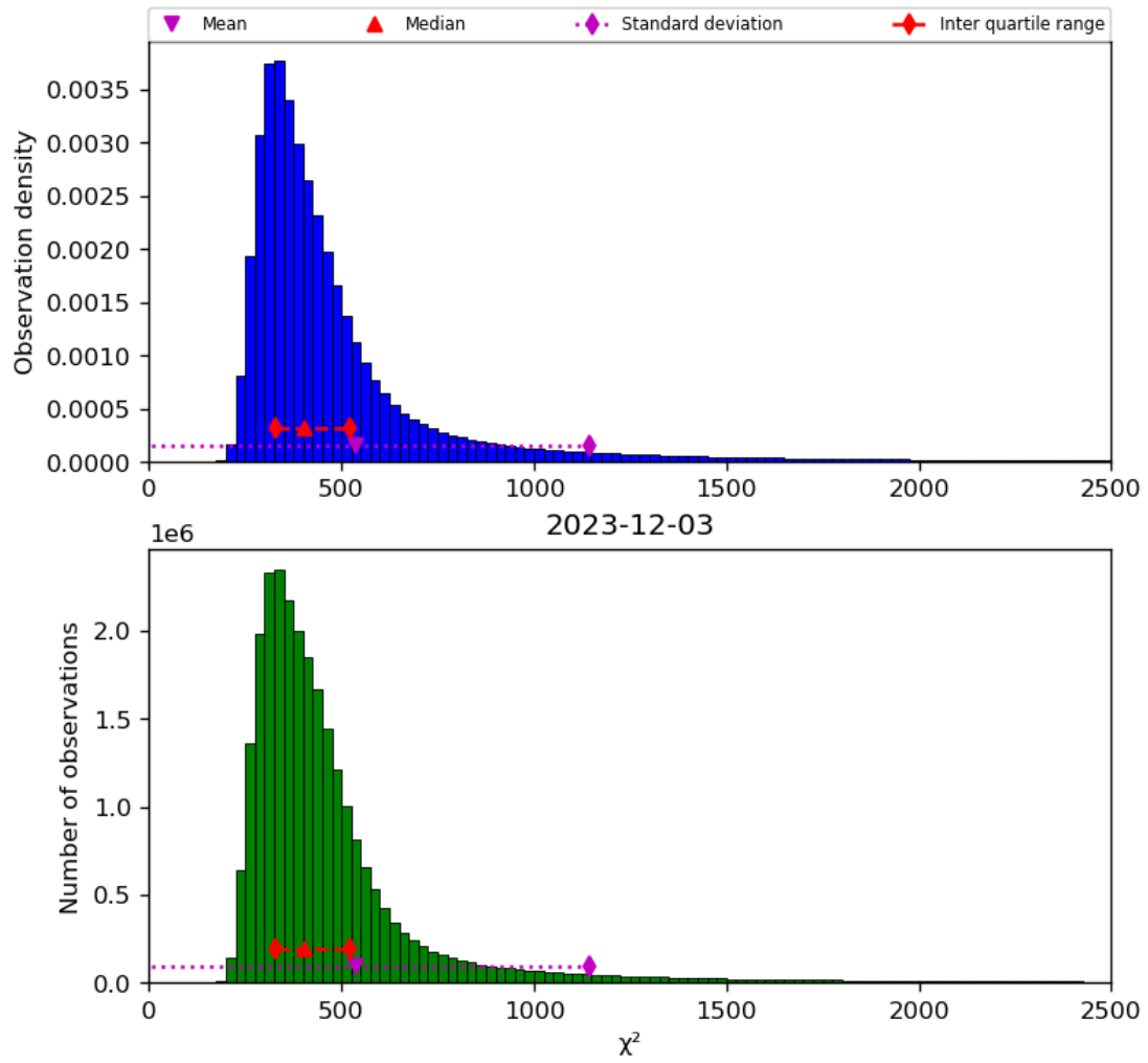
Figure 42: Histogram of “ \chi^2 ” for 2023-12-02 to 2023-12-04
