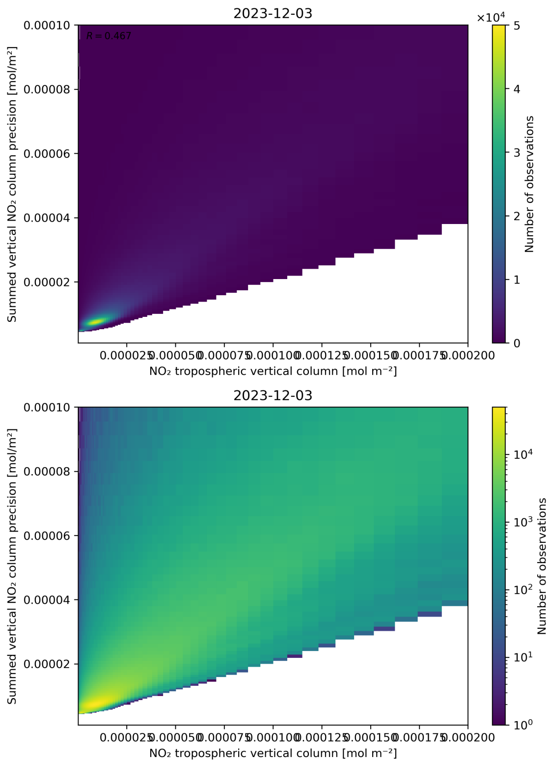
Figure 127: Scatter density plot of “NO 2 tropospheric vertical column” against “Summed vertical NO 2 column precision” for 2023-12-02 to 2023-12-04.
