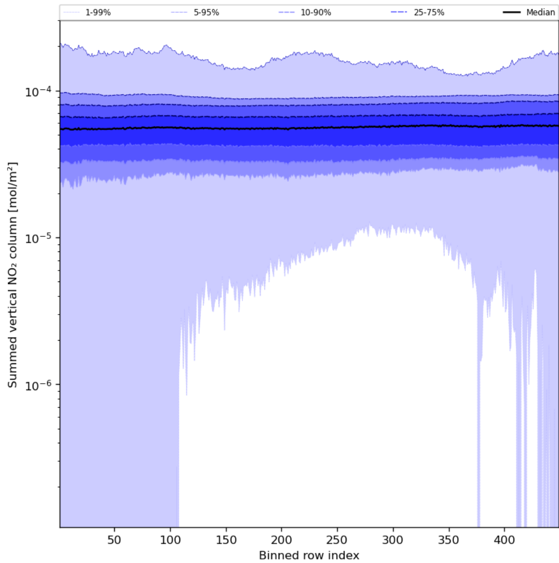
Figure 57: Along track statistics of “Summed vertical NO 2 column” for 2023-12-02 to 2023-12-04
