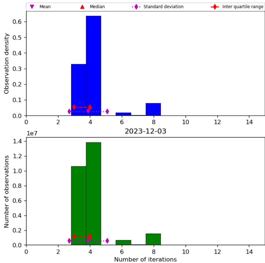
Figure 34: Histogram of “Number of iterations” for 2023-12-02 to 2023-12-04
