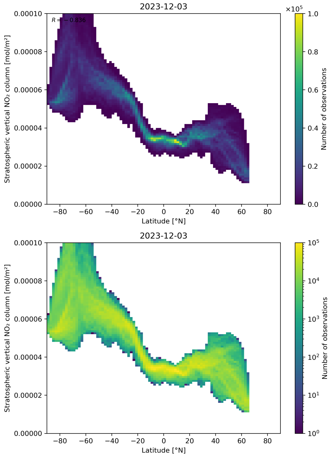
Figure 87: Scatter density plot of “Latitude” against “Stratospheric vertical NO 2 column” for 2023-12-02 to 2023-12-04.
