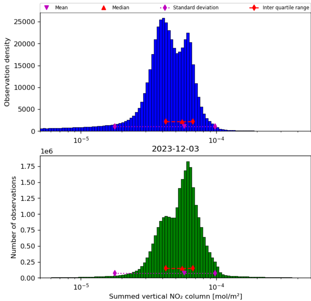
Figure 40: Histogram of "Summed vertical NO 2 column" for 2023-12-02 to 2023-12-04
