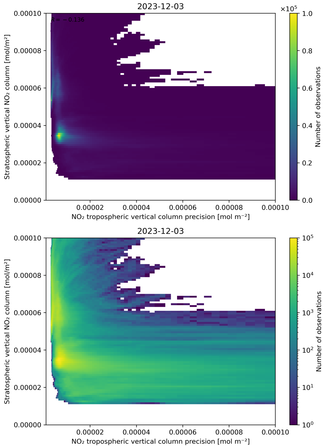
Figure 135: Scatter density plot of “NO 2 tropospheric vertical column precision” against “Stratospheric vertical NO 2 column” for 2023-12-02 to 2023-12-04.
