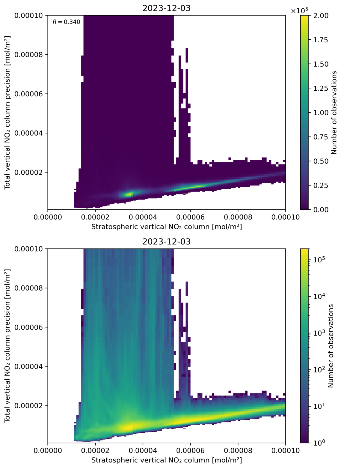
Figure 101: Scatter density plot of “Stratospheric vertical NO 2 column” against “Total vertical NO 2 column precision” for 2023-12-02 to 2023-12-04.
