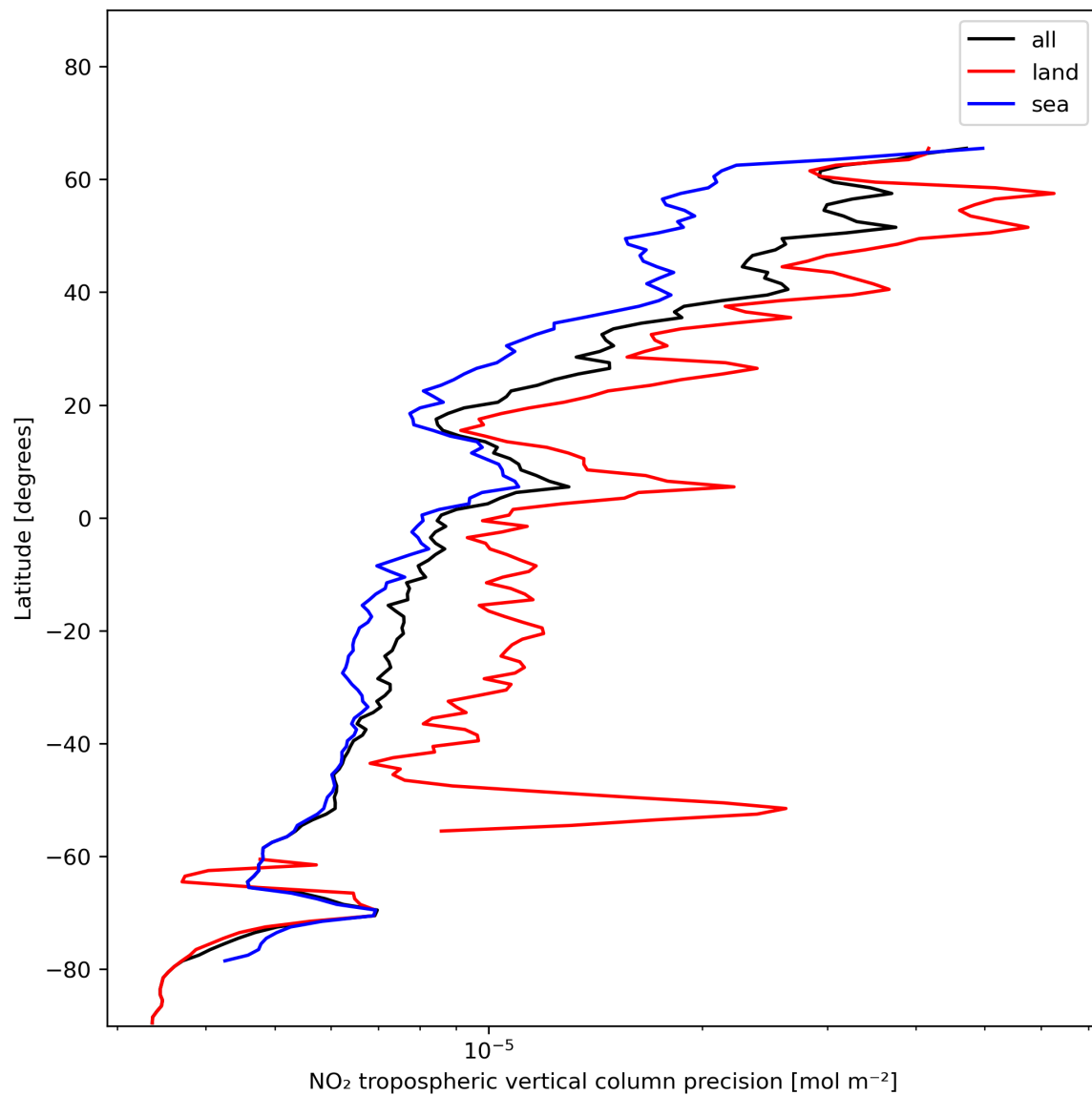
Figure 13: Zonal average of “NO 2 tropospheric vertical column precision” for 2023-12-02 to 2023-12-04.
