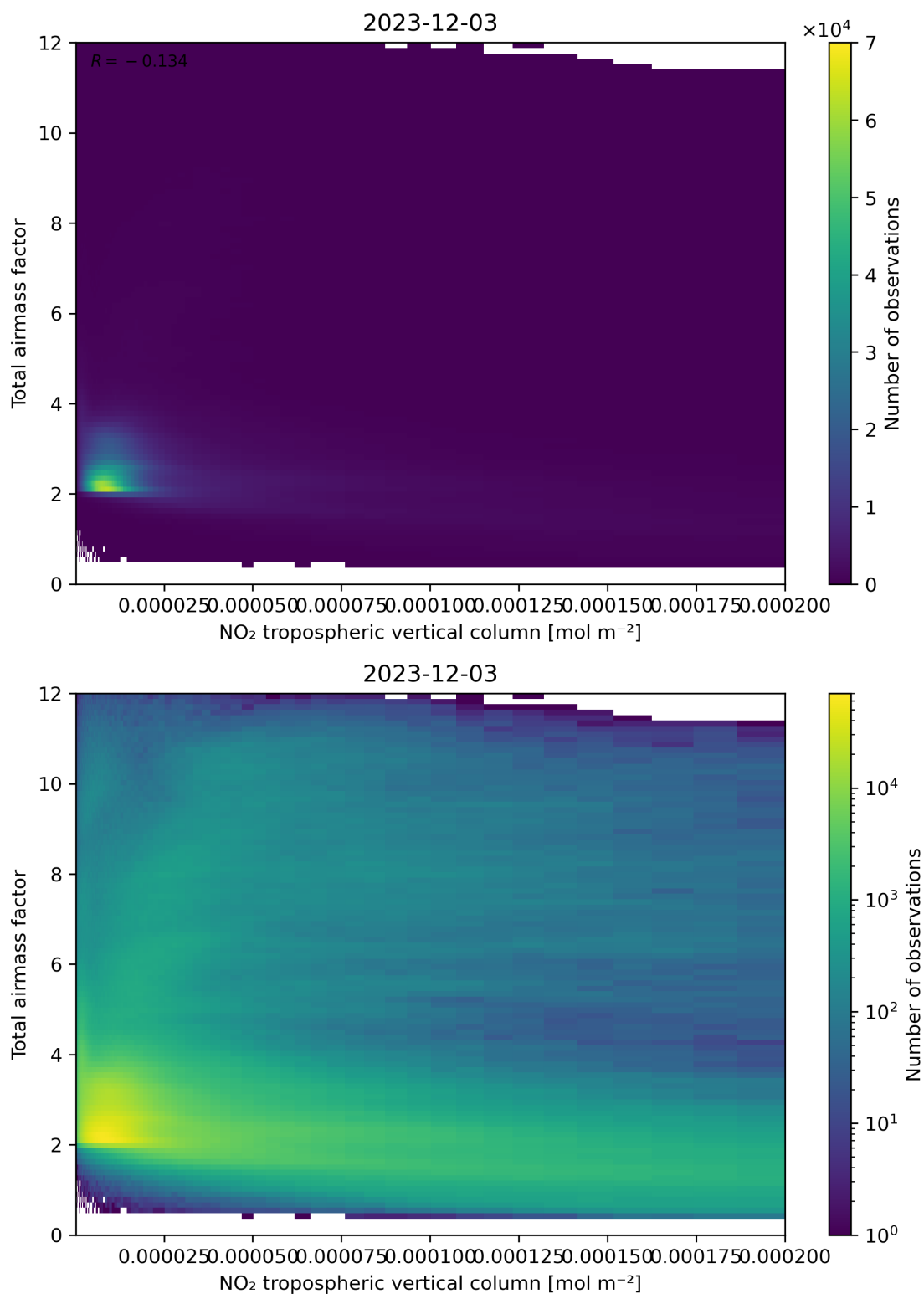
Figure 122: Scatter density plot of “NO 2 tropospheric vertical column” against “Total air mass factor” for 2023-12-02 to 2023-12-04.
