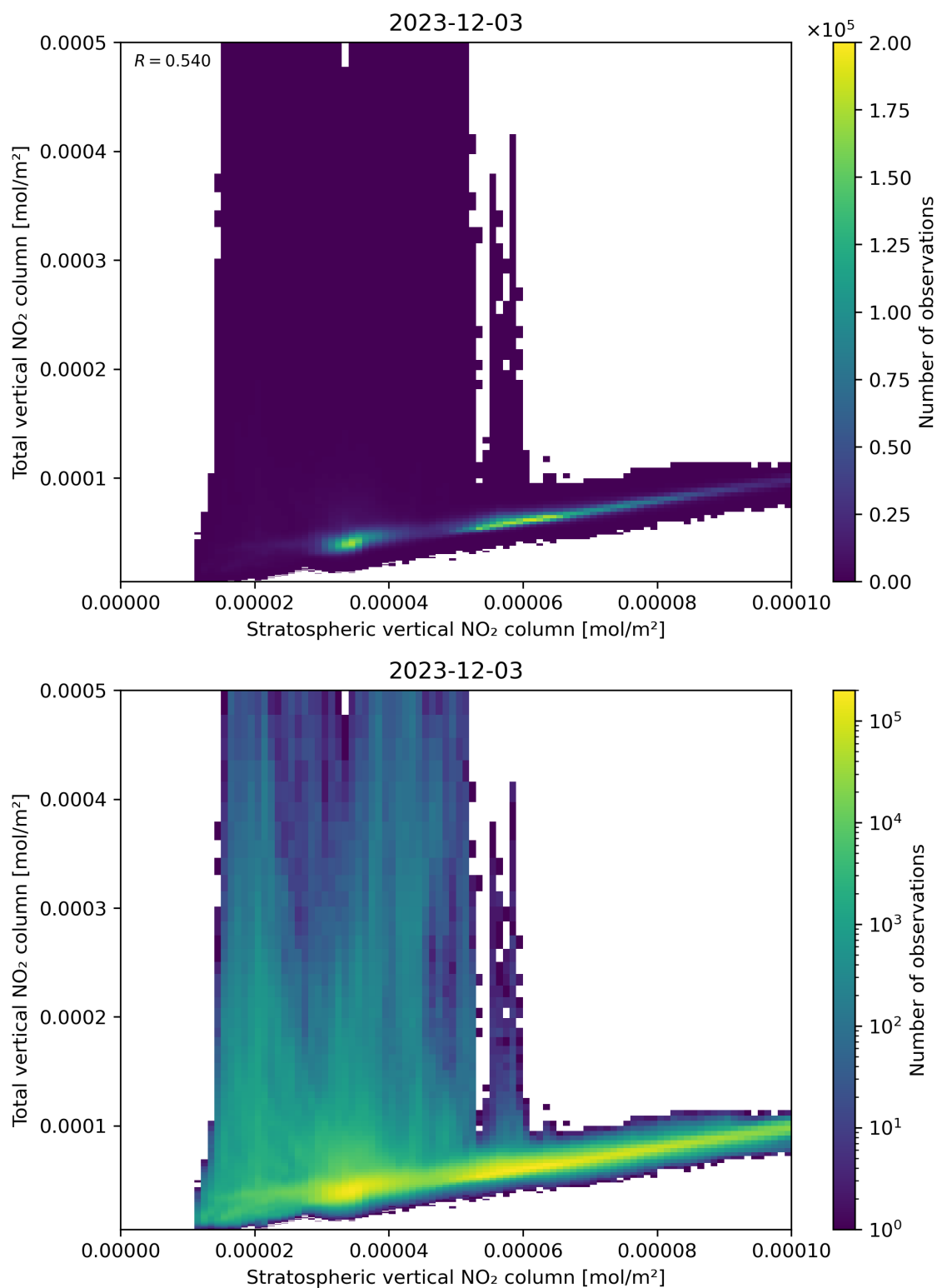
Figure 100: Scatter density plot of “Stratospheric vertical NO 2 column” against “Total vertical NO 2 column” for 2023-12-02 to 2023-12-04.
