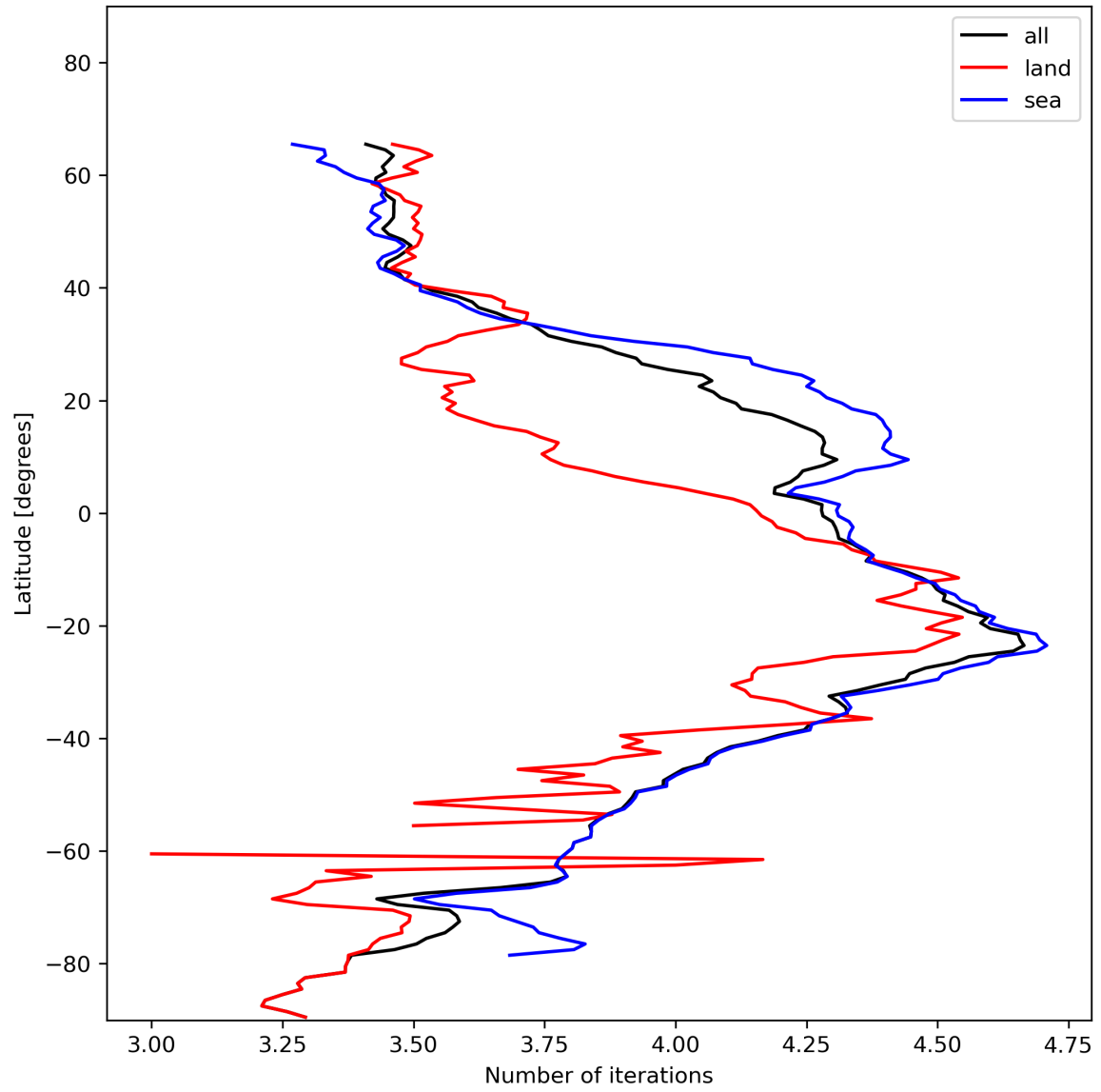
Figure 17: Zonal average of “Number of iterations” for 2023-12-02 to 2023-12-04.
