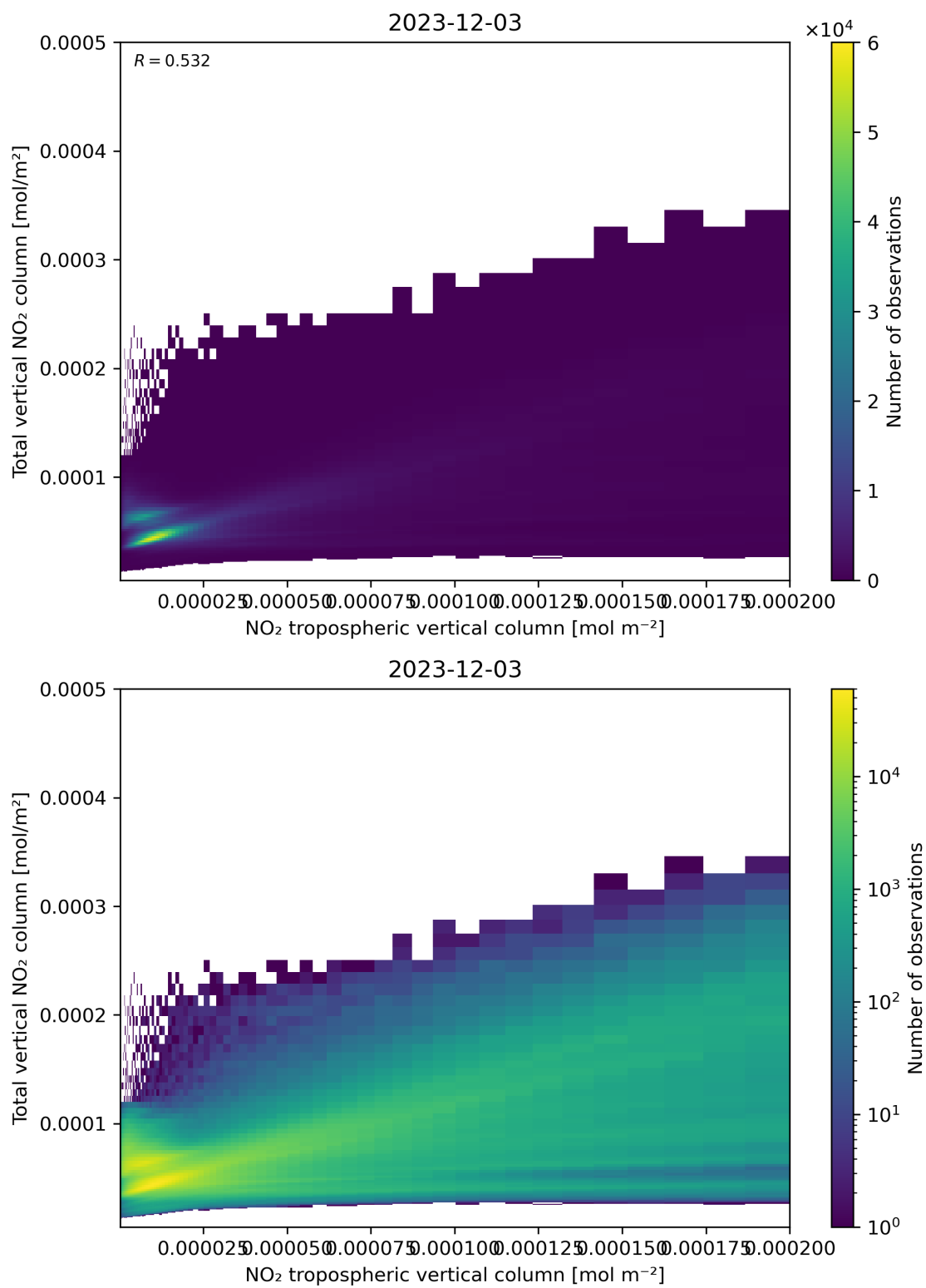
Figure 128: Scatter density plot of “NO 2 tropospheric vertical column” against “Total vertical NO 2 column” for 2023-12-02 to 2023-12-04.
