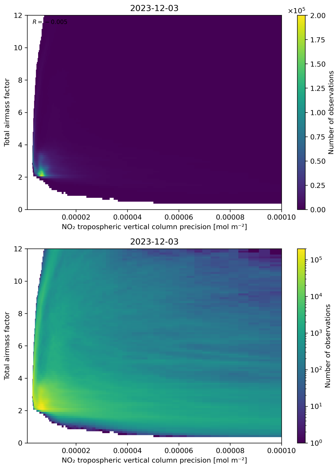
Figure 132: Scatter density plot of “NO 2 tropospheric vertical column precision” against “Total air mass factor” for 2023-12-02 to 2023-12-04.
