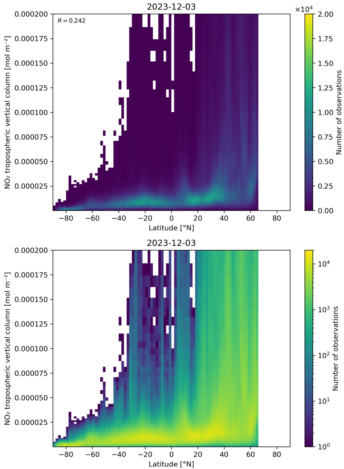
Figure 92: Scatter density plot of “Latitude” against “NO 2 tropospheric vertical column” for 2023-12-02 to 2023-12-04.
