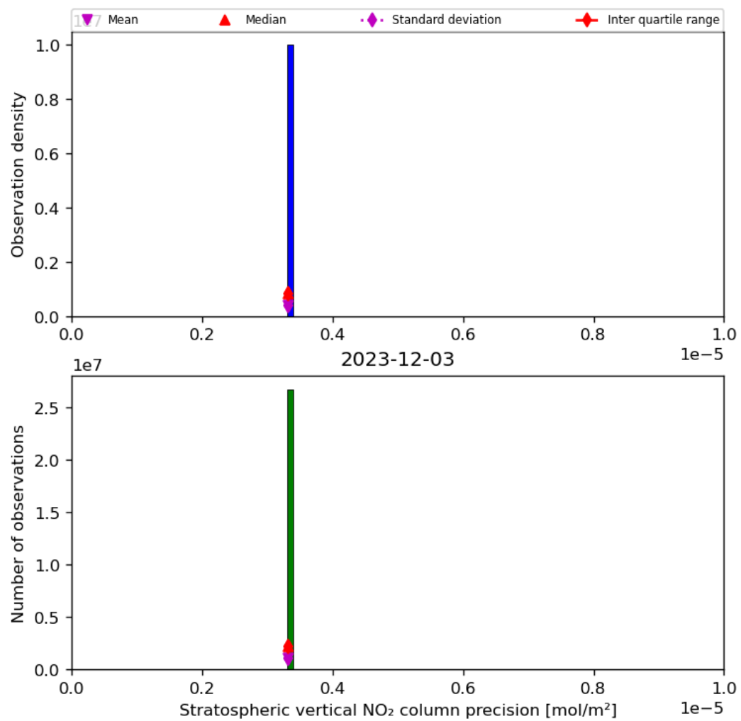
Figure 37: Histogram of “Stratospheric vertical NO 2 column precision” for 2023-12-02 to 2023-12-04
