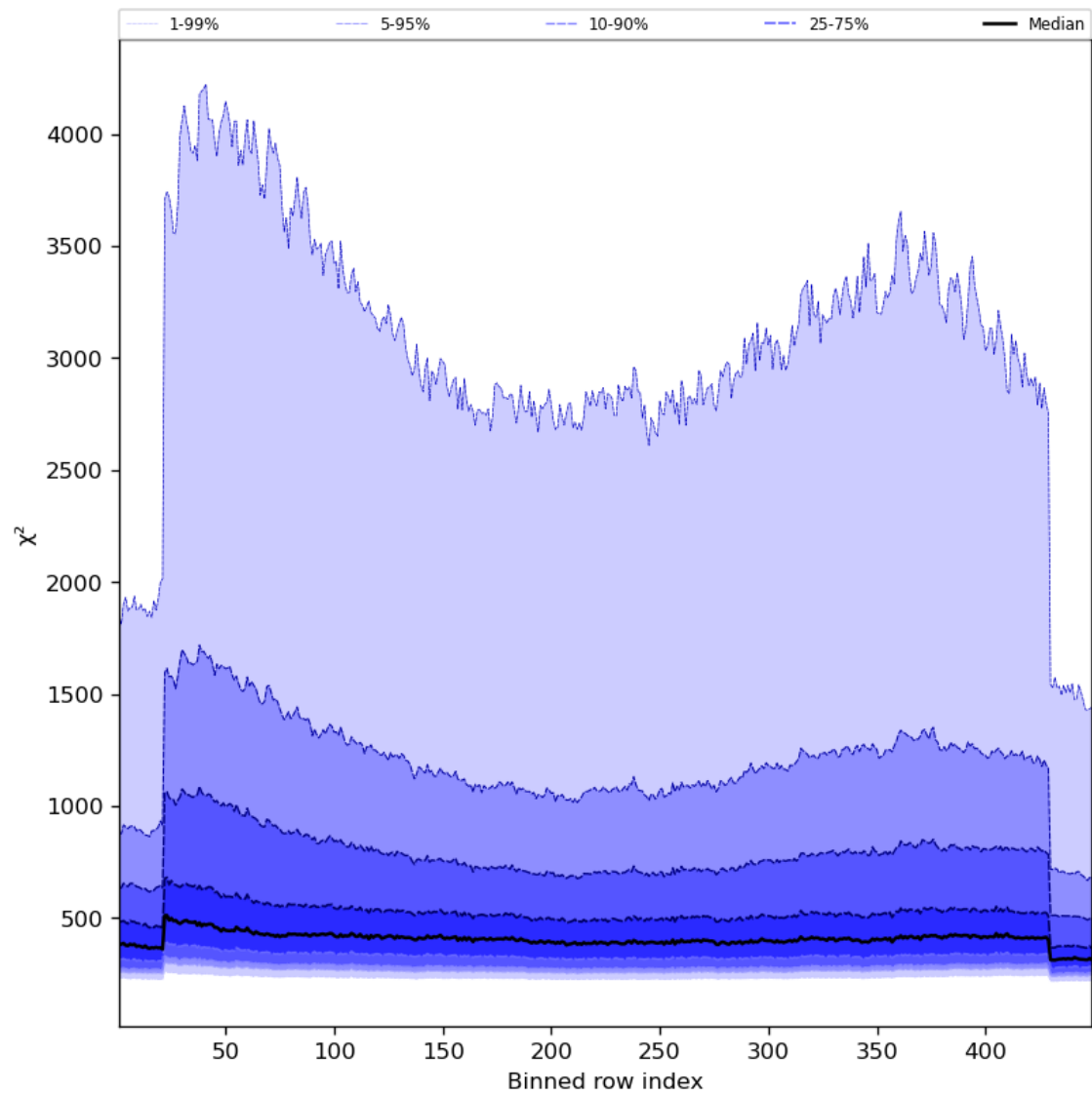
Figure 59: Along track statistics of “ \chi^2 ” for 2023-12-02 to 2023-12-04
