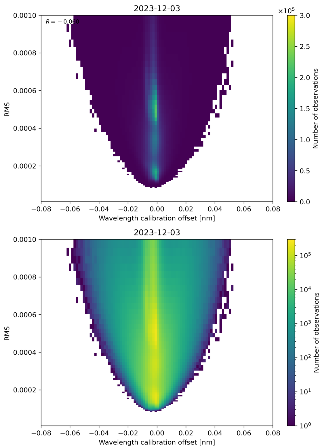
Figure 181: Scatter density plot of “Wavelength calibration offset” against “RMS” for 2023-12-02 to 2023-12-04.
