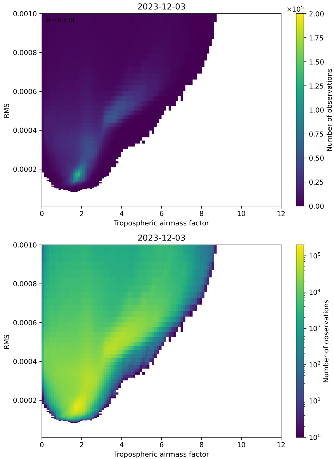
Figure 79: Scatter density plot of “Tropospheric airmass factor” against “RMS” for 2023-12-02 to 2023-12-04.
