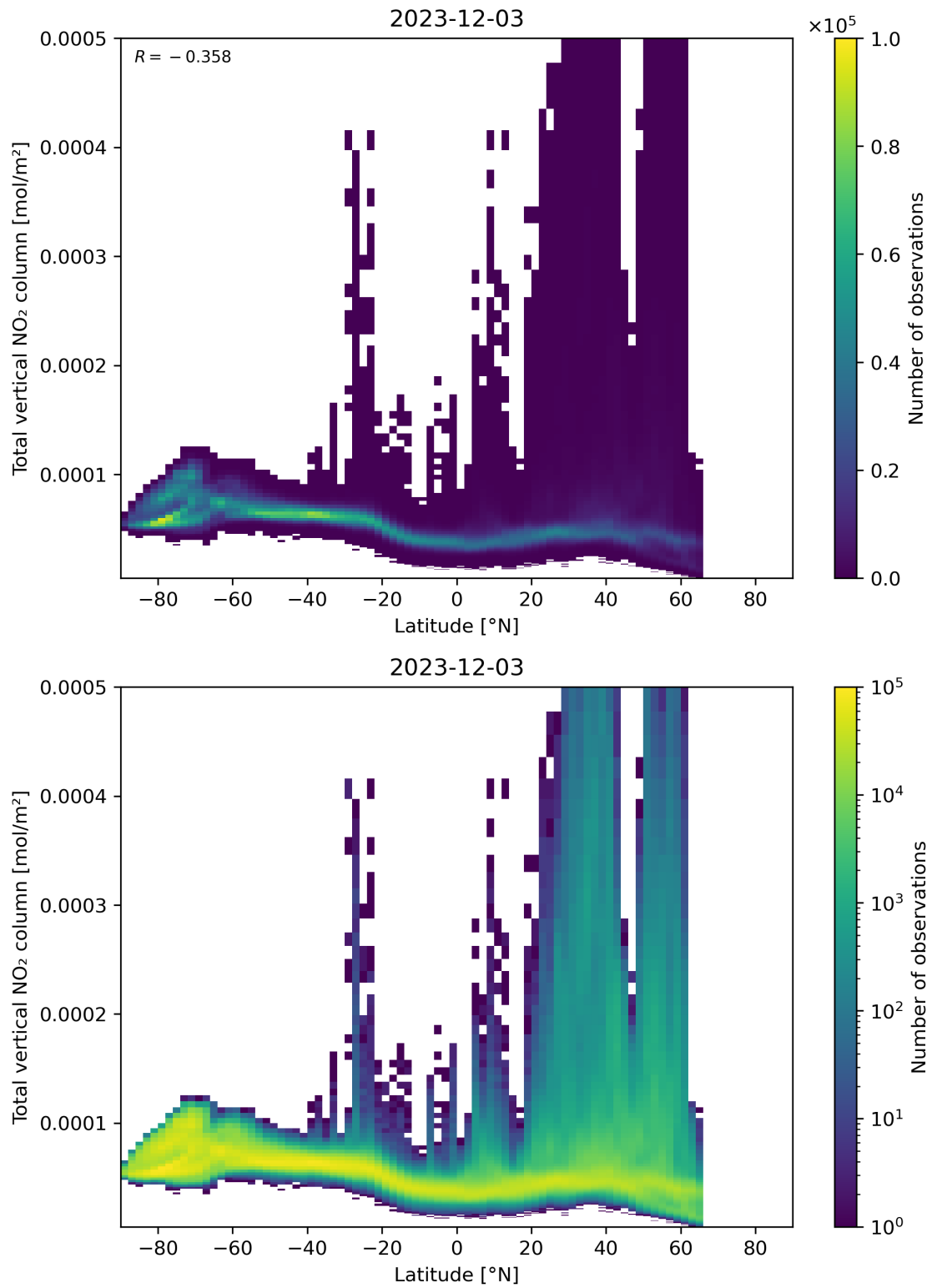
Figure 90: Scatter density plot of “Latitude” against “Total vertical NO 2 column” for 2023-12-02 to 2023-12-04.
