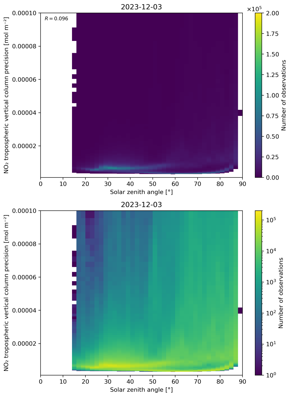
Figure 156: Scatter density plot of “Solar zenith angle” against “NO 2 tropospheric vertical column precision” for 2023-12-02 to 2023-12-04.
