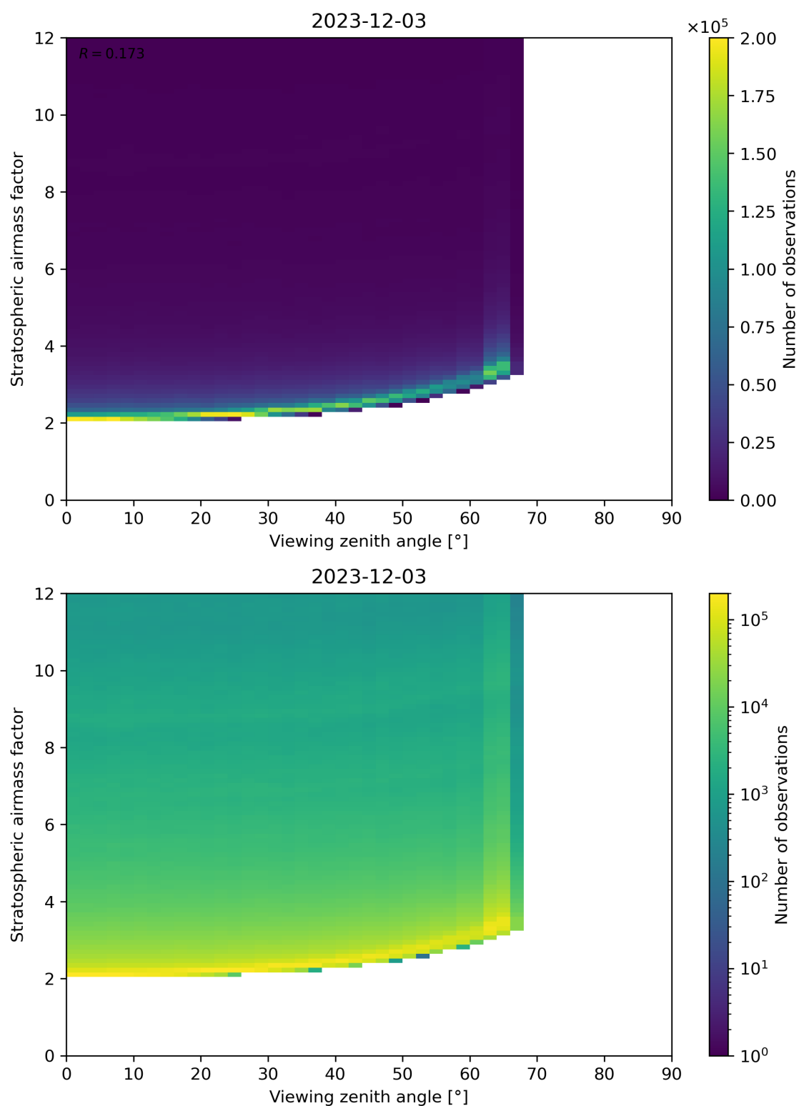
Figure 159: Scatter density plot of “Viewing zenith angle” against “Stratospheric airmass factor” for 2023-12-02 to 2023-12-04.
