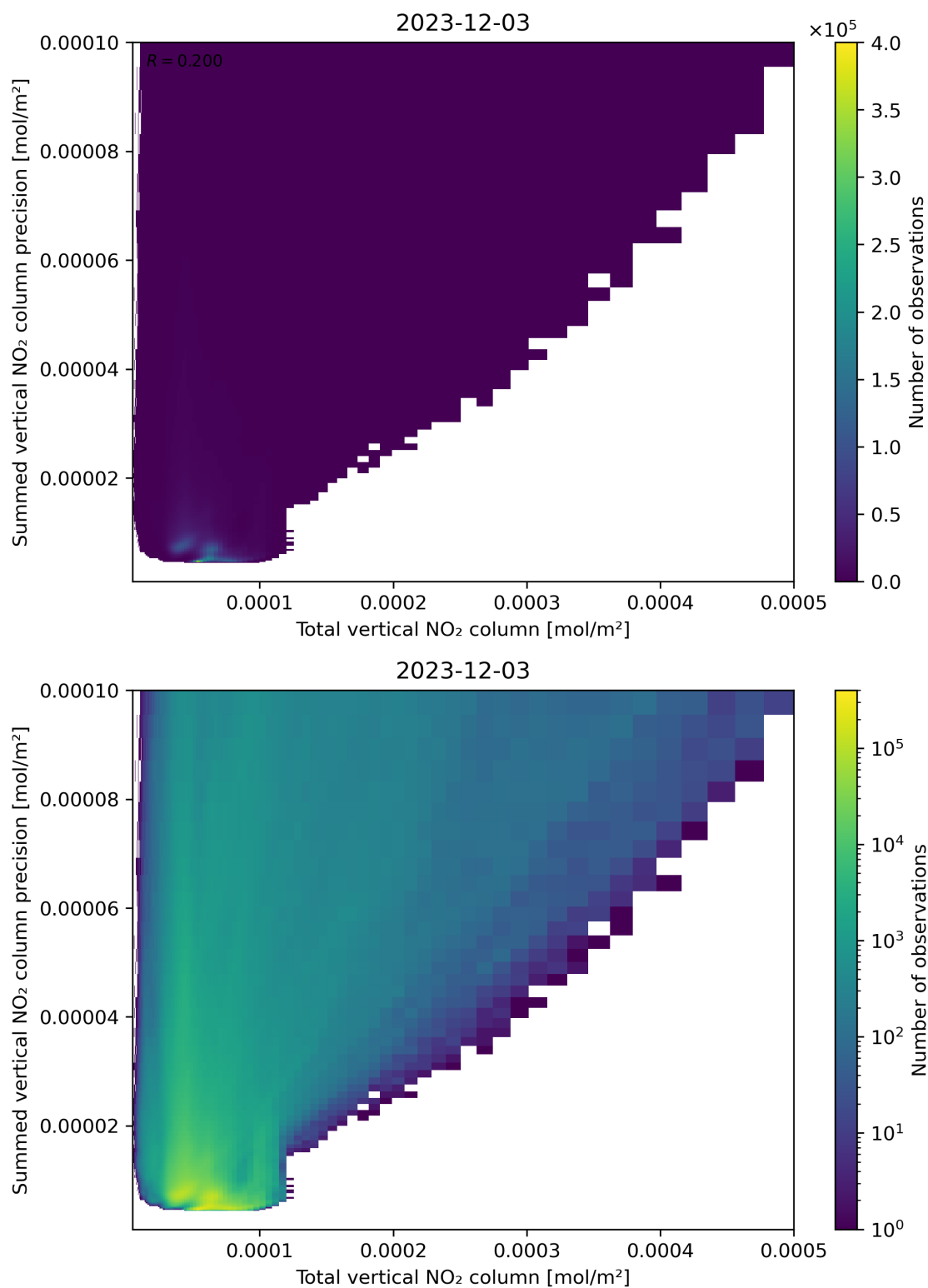
Figure 113: Scatter density plot of “Total vertical NO 2 column” against “Summed vertical NO 2 column precision” for 2023-12-02 to 2023-12-04.
