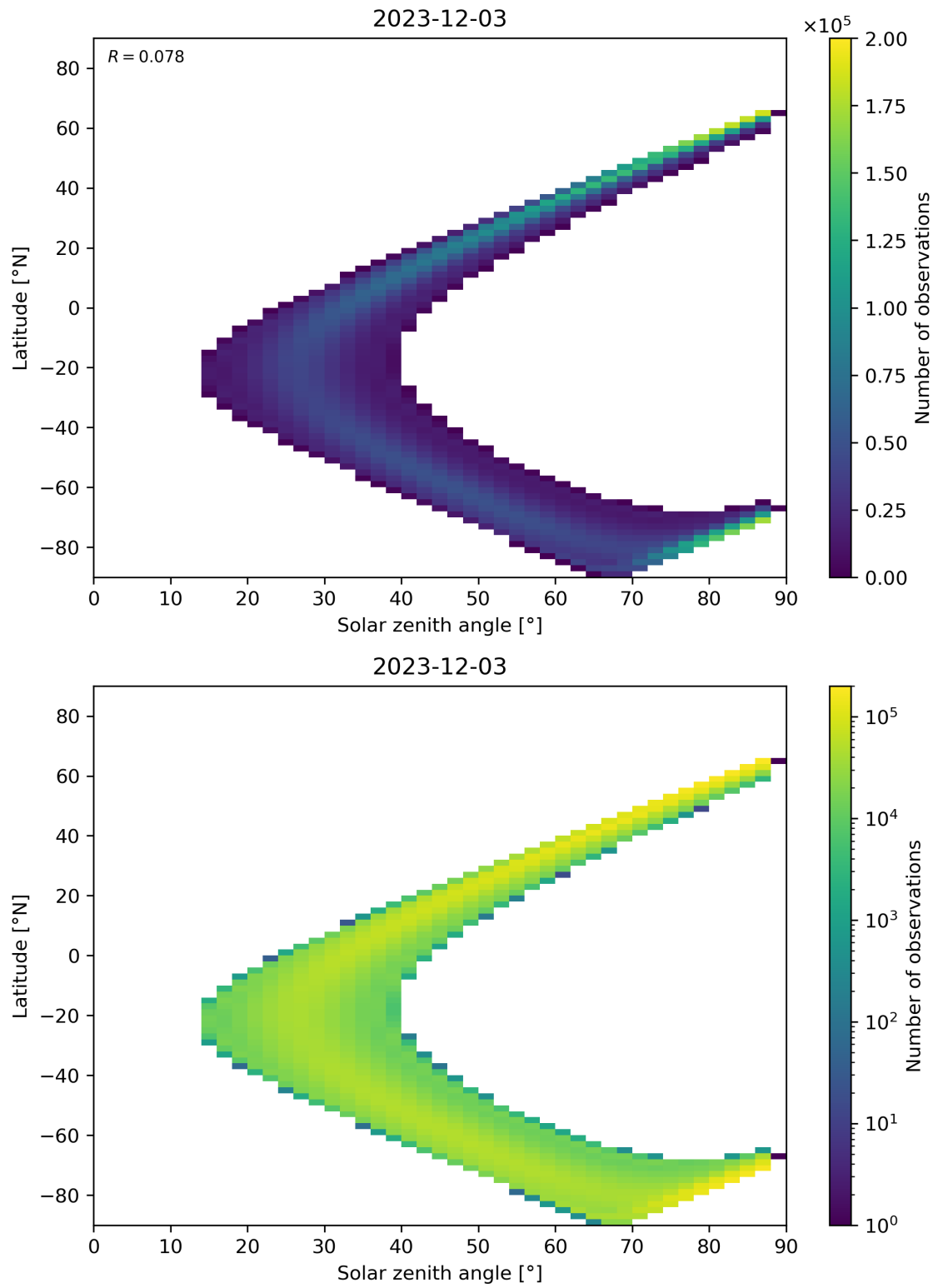
Figure 149: Scatter density plot of “Solar zenith angle” against “Latitude” for 2023-12-02 to 2023-12-04.
