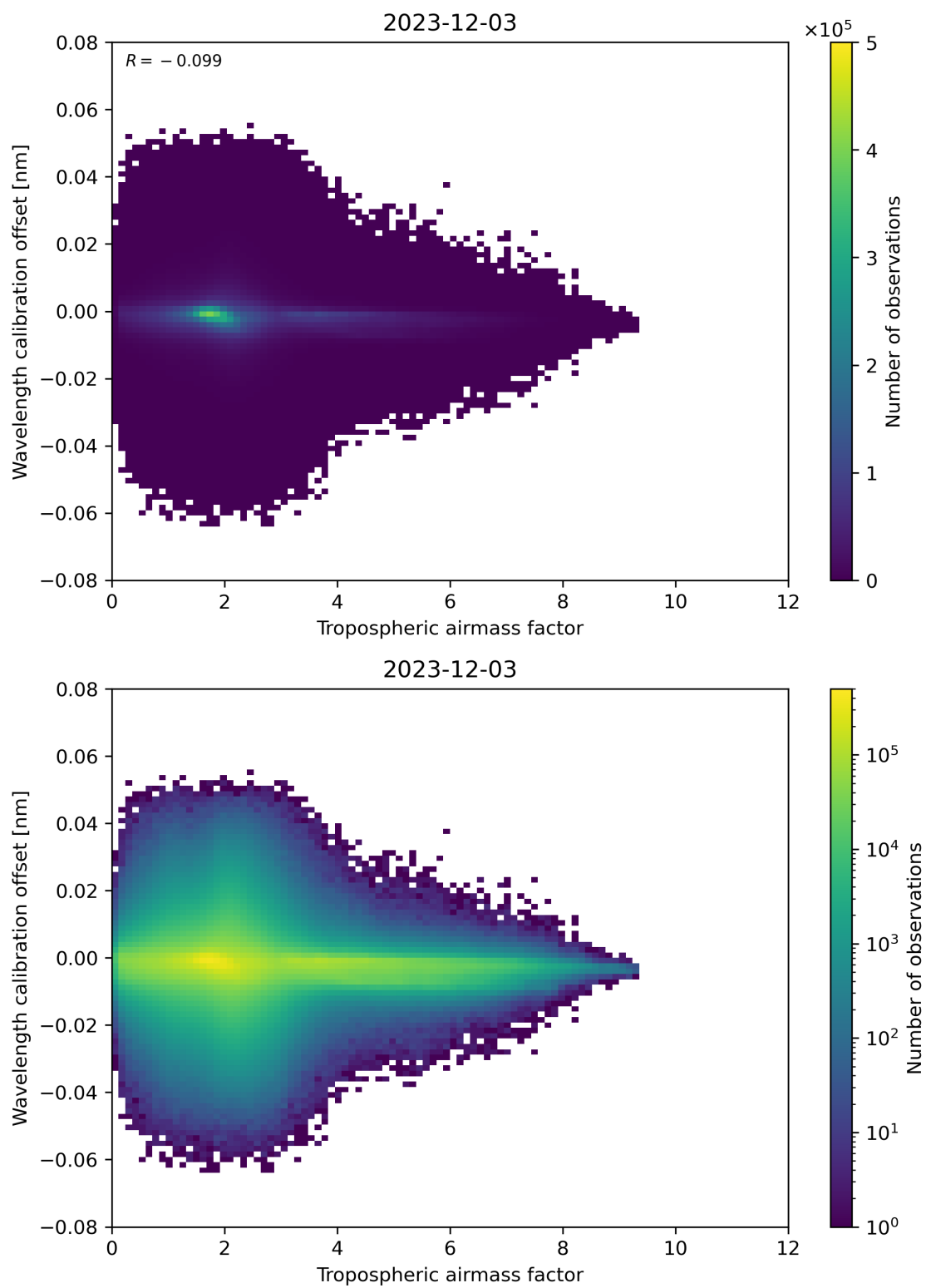
Figure 80: Scatter density plot of “Tropospheric air mass factor” against “Wavelength calibration offset” for 2023-12-02 to 2023-12-04.
