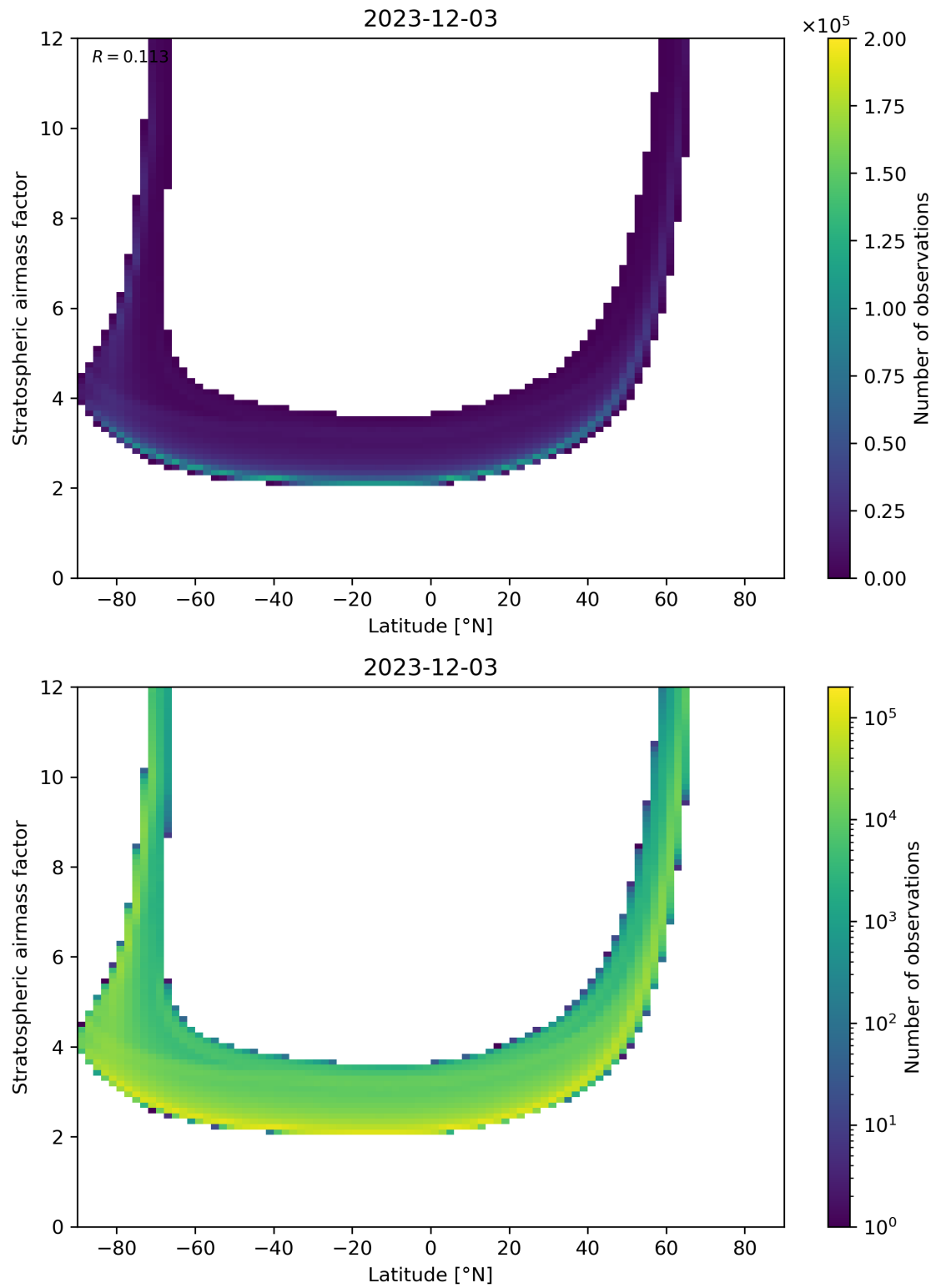
Figure 83: Scatter density plot of “Latitude” against “Stratospheric air mass factor” for 2023-12-02 to 2023-12-04.
