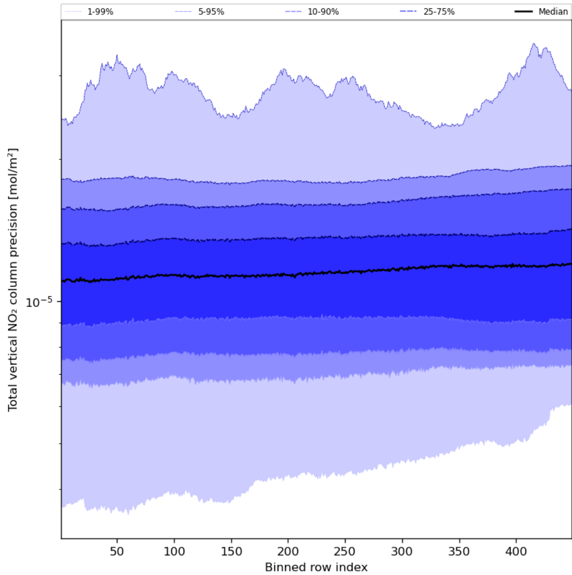
Figure 56: Along track statistics of “Total vertical NO 2 column precision” for 2023-12-02 to 2023-12-04
