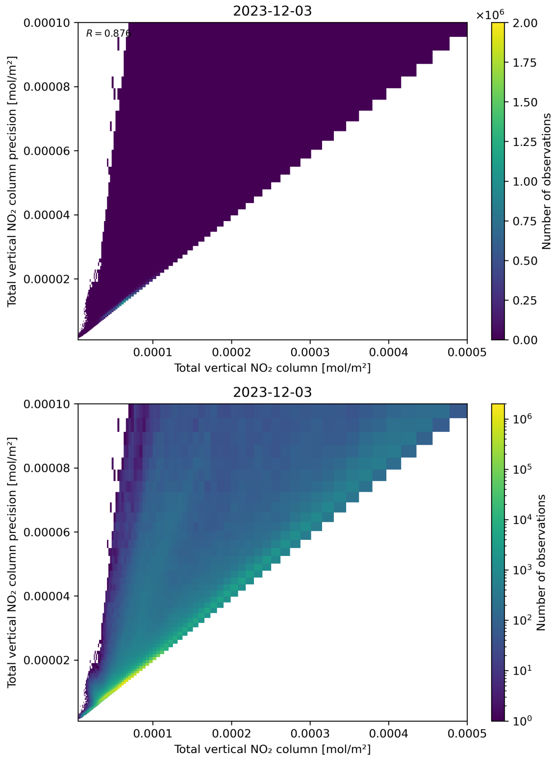
Figure 114: Scatter density plot of “Total vertical NO 2 column” against “Total vertical NO 2 column precision” for 2023-12-02 to 2023-12-04.
