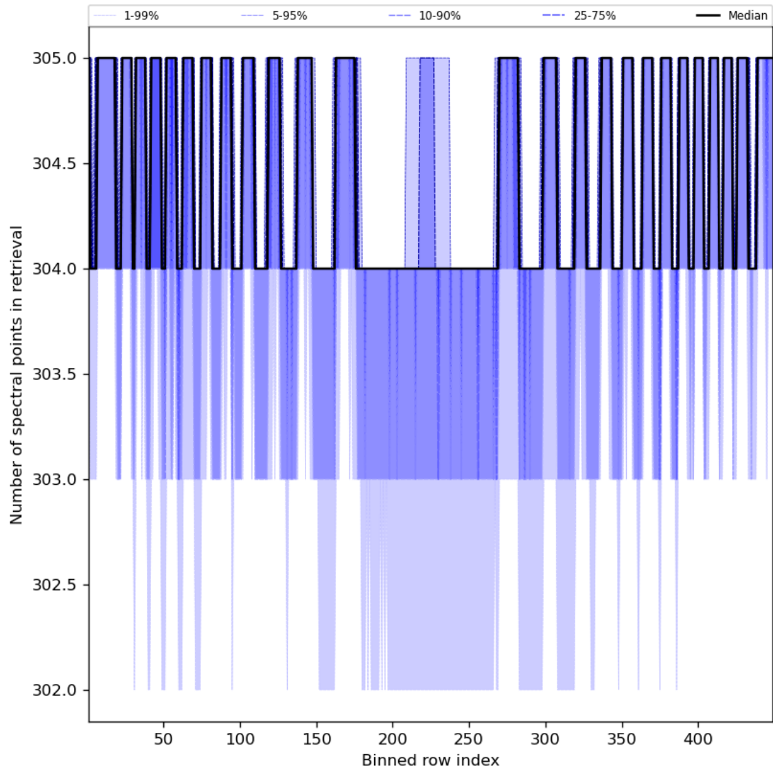
Figure 50: Along track statistics of “Number of spectral points in retrieval” for 2023-12-02 to 2023-12-04
