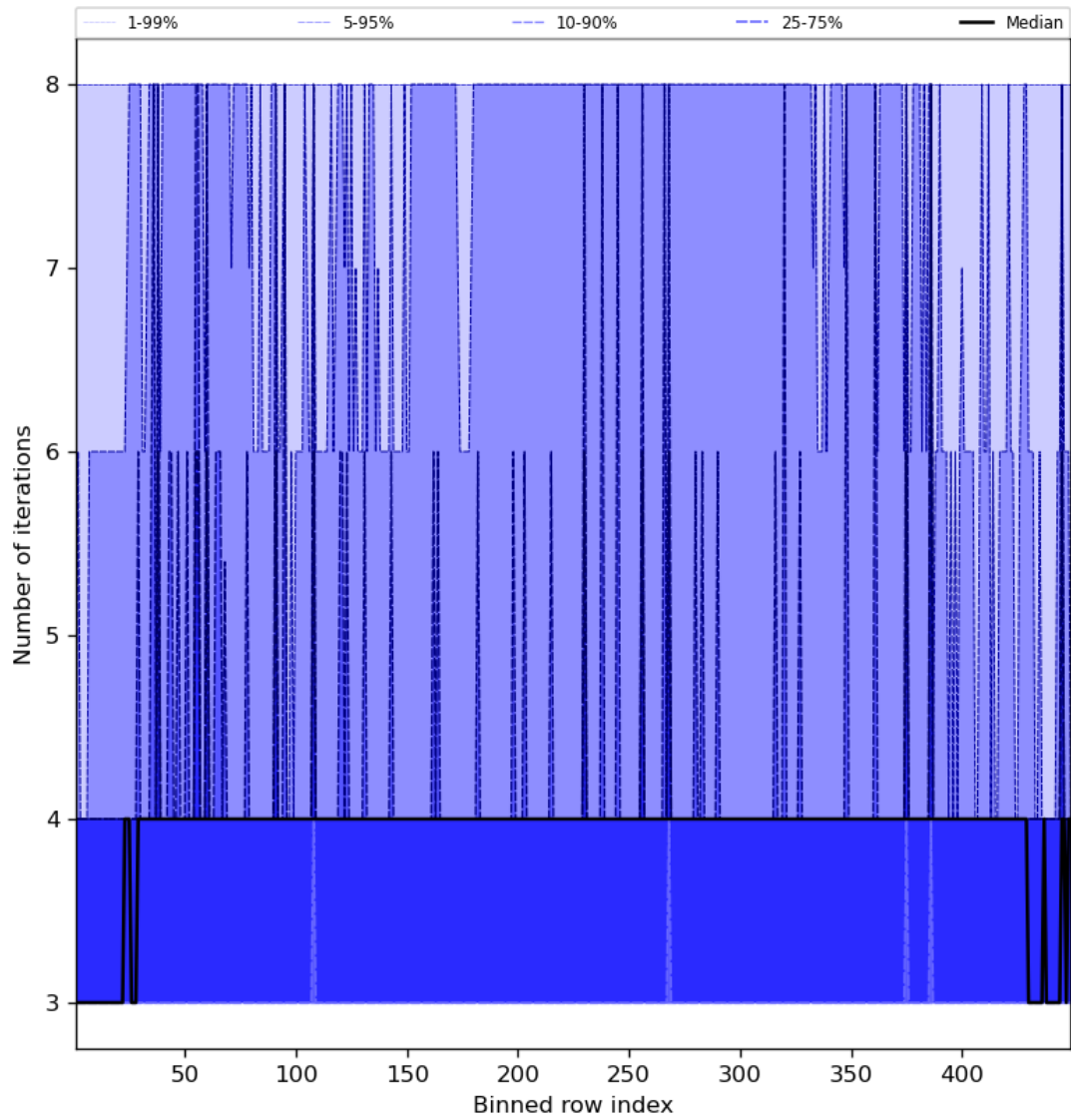
Figure 51: Along track statistics of “Number of iterations” for 2023-12-02 to 2023-12-04
