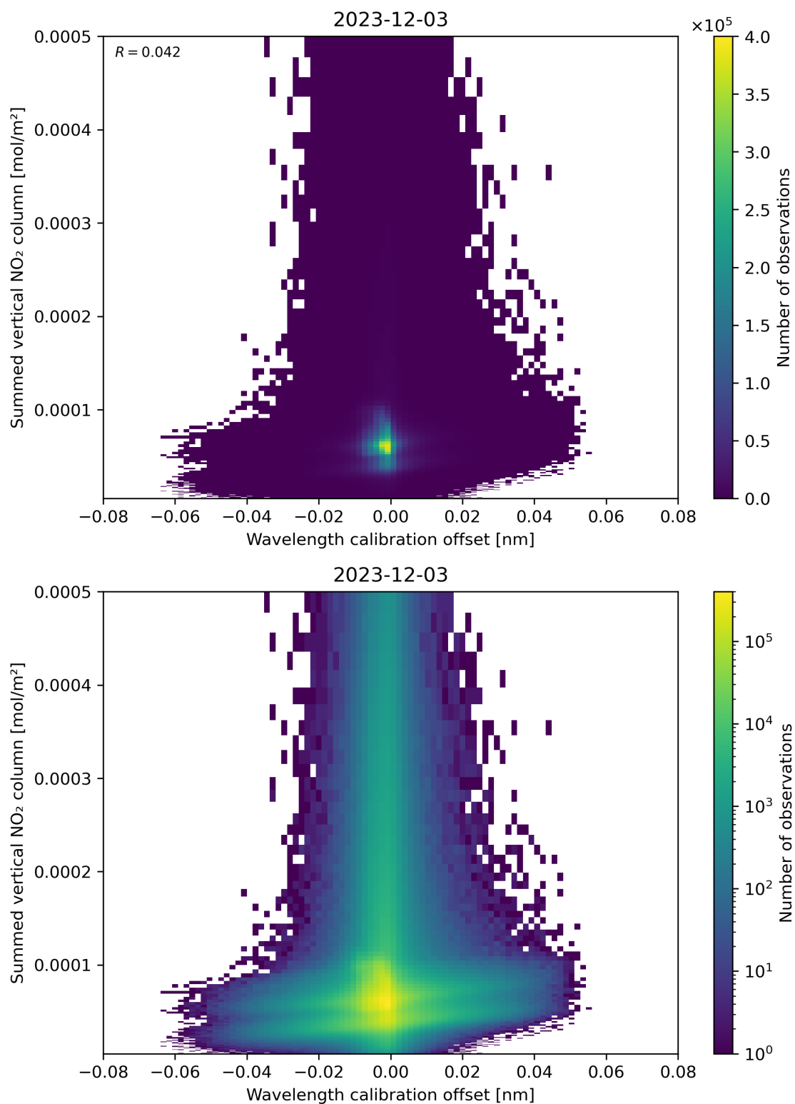
Figure 177: Scatter density plot of “Wavelength calibration offset” against “Summed vertical NO 2 column” for 2023-12-02 to 2023-12-04.
