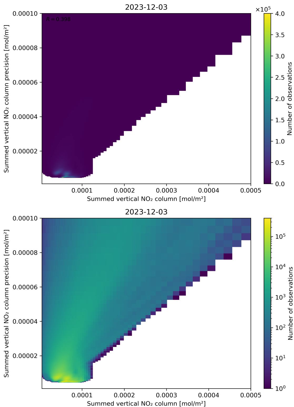
Figure 105: Scatter density plot of “Summed vertical NO 2 column” against “Summed vertical NO 2 column precision” for 2023-12-02 to 2023-12-04.
