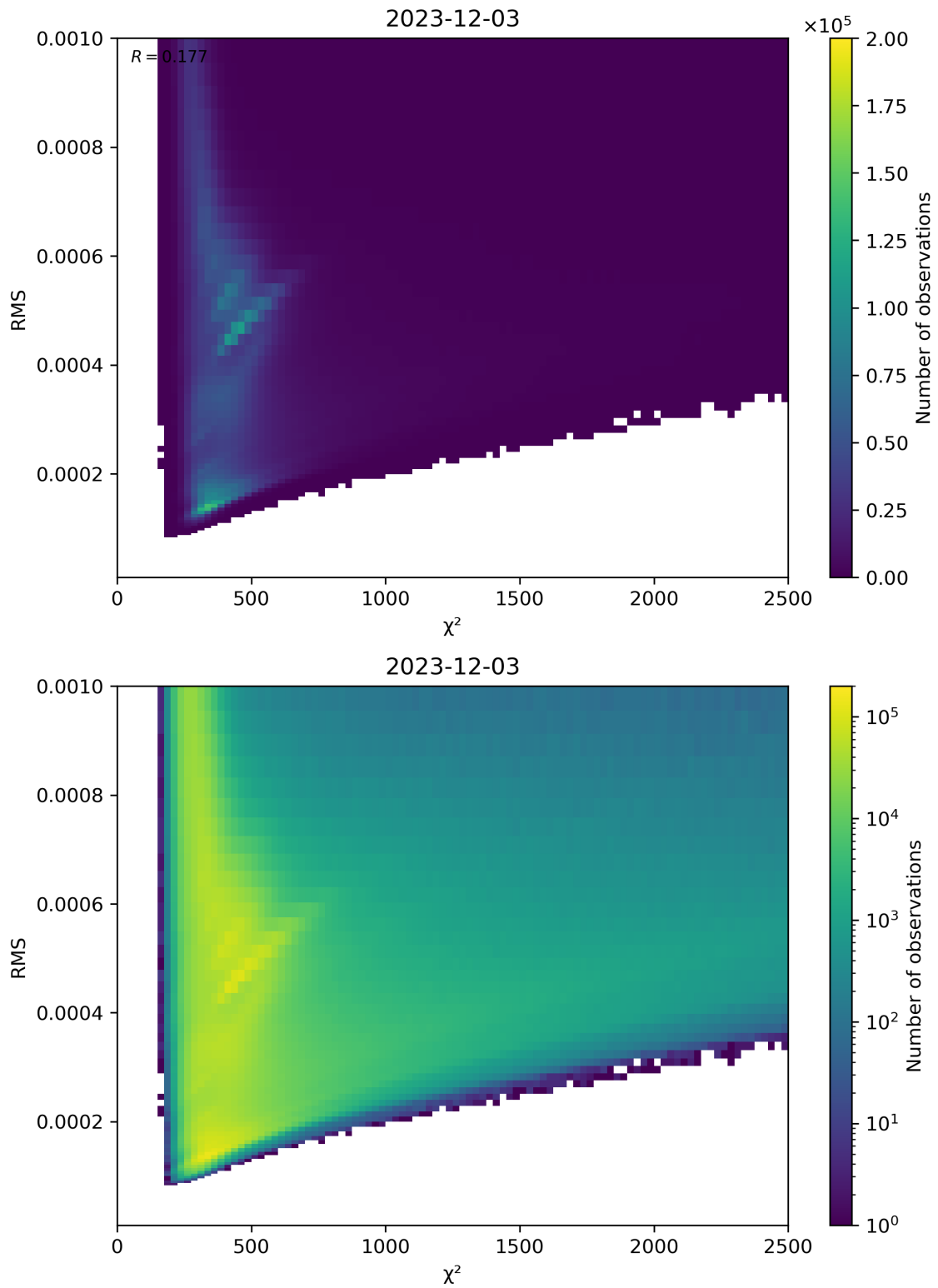
Figure 82: Scatter density plot of “ \chi^2 ” against “RMS” for 2023-12-02 to 2023-12-04.
