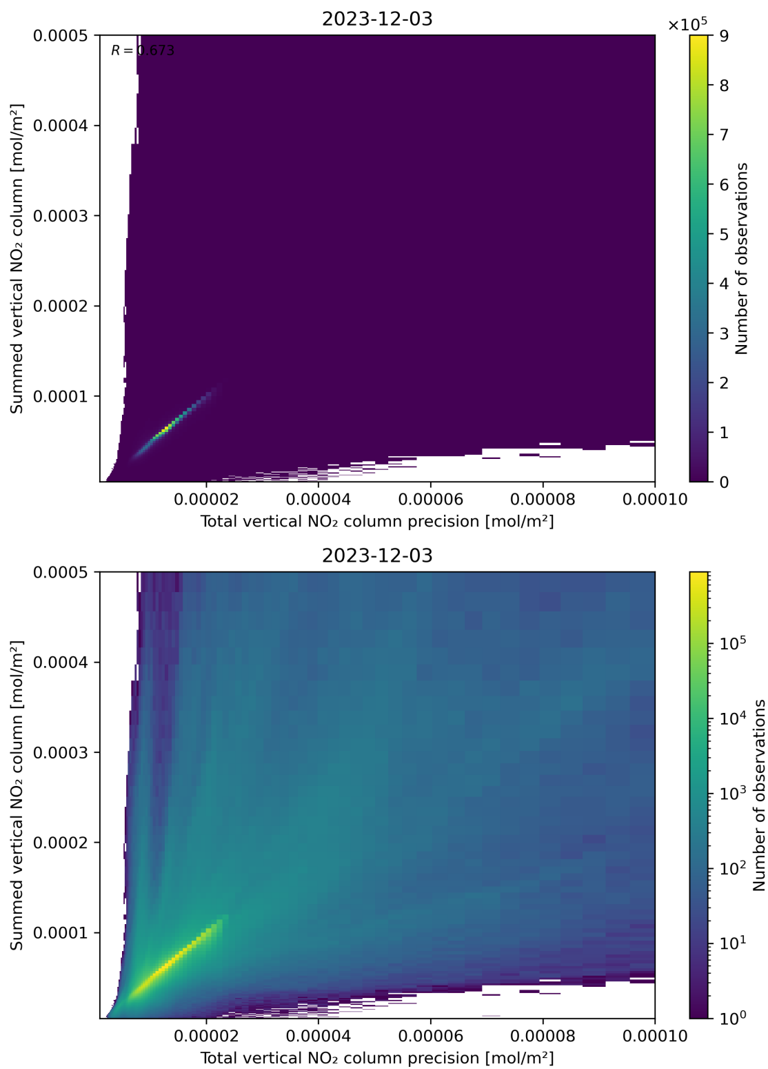
Figure 117: Scatter density plot of “Total vertical NO 2 column precision” against “Summed vertical NO 2 column” for 2023-12-02 to 2023-12-04.
