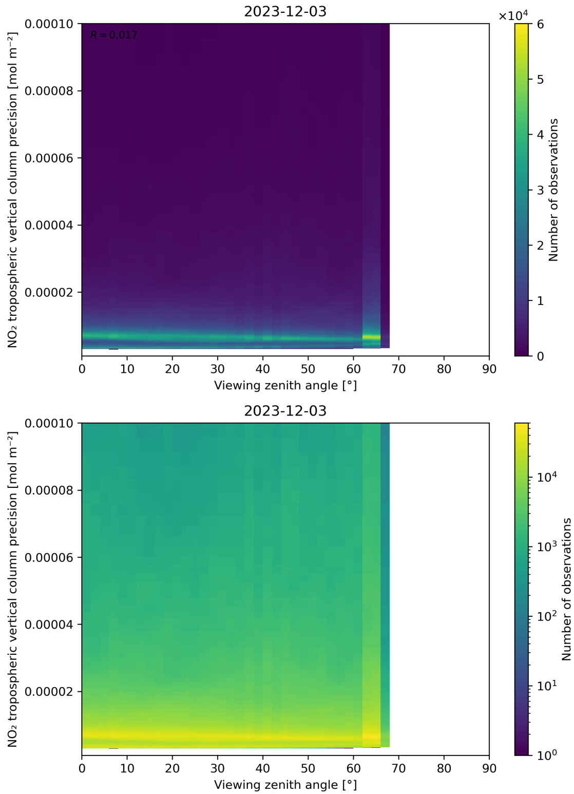
Figure 170: Scatter density plot of “Viewing zenith angle” against “NO 2 tropospheric vertical column precision” for 2023-12-02 to 2023-12-04.
