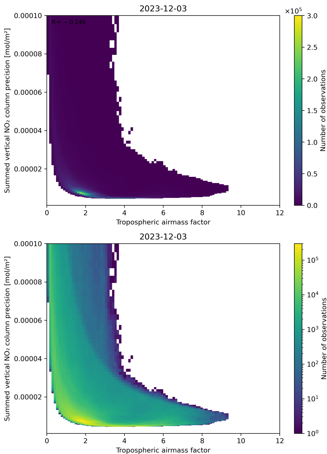
Figure 76: Scatter density plot of “Tropospheric air mass factor” against “Summed vertical NO 2 column precision” for 2023-12-02 to 2023-12-04.
