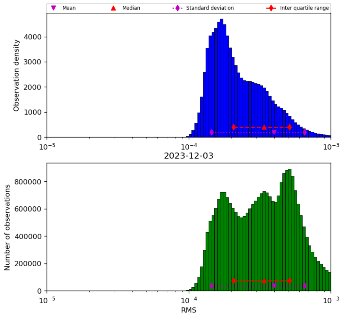
Figure 43: Histogram of “RMS” for 2023-12-02 to 2023-12-04
