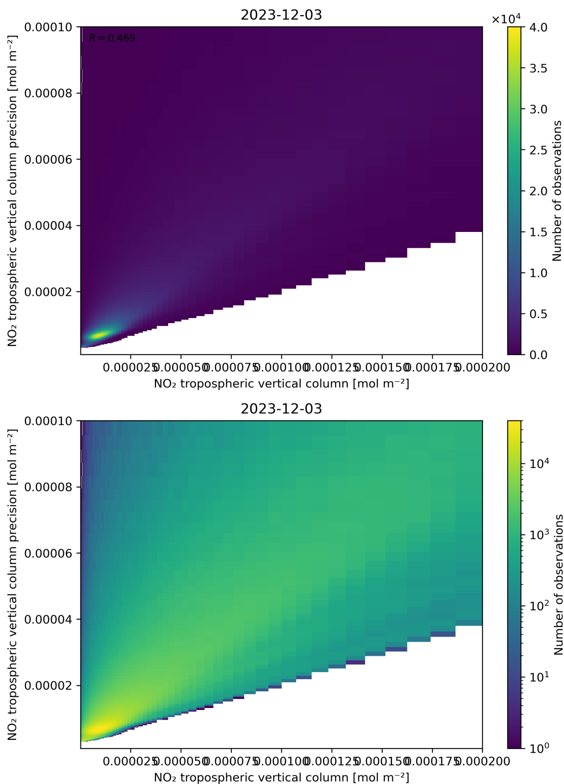
Figure 130: Scatter density plot of “NO 2 tropospheric vertical column” against “NO 2 tropospheric vertical column precision” for 2023-12-02 to 2023-12-04.
