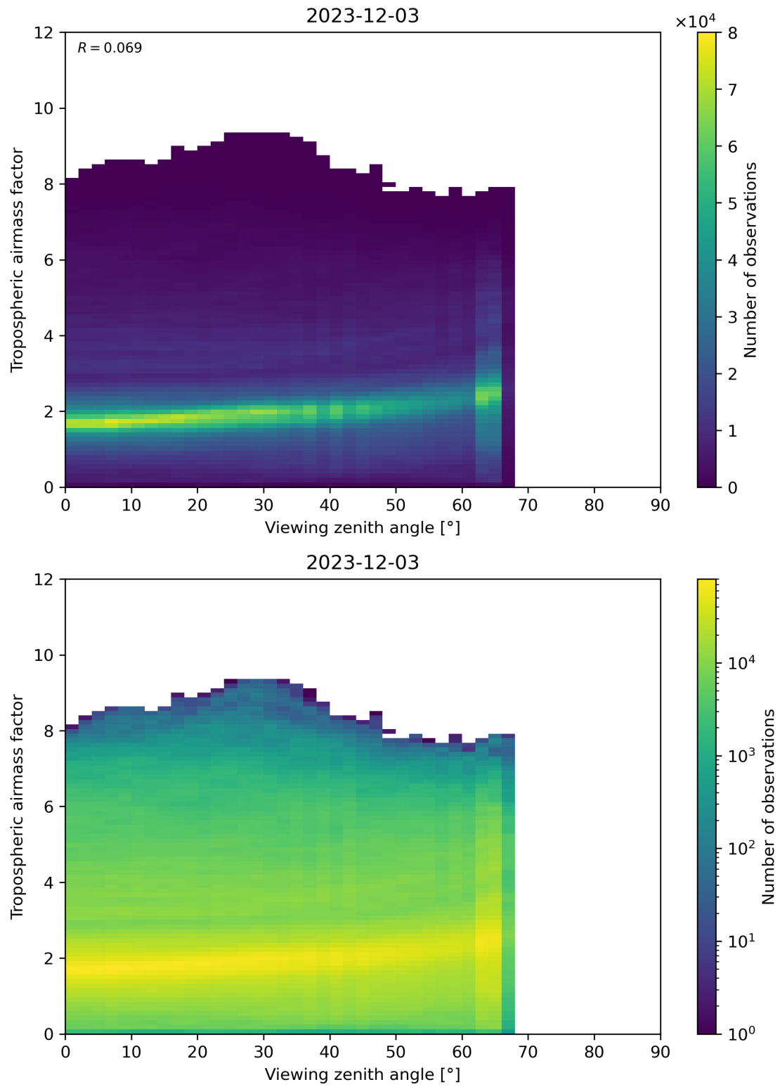
Figure 161: Scatter density plot of “Viewing zenith angle” against “Tropospheric airmass factor” for 2023-12-02 to 2023-12-04.
