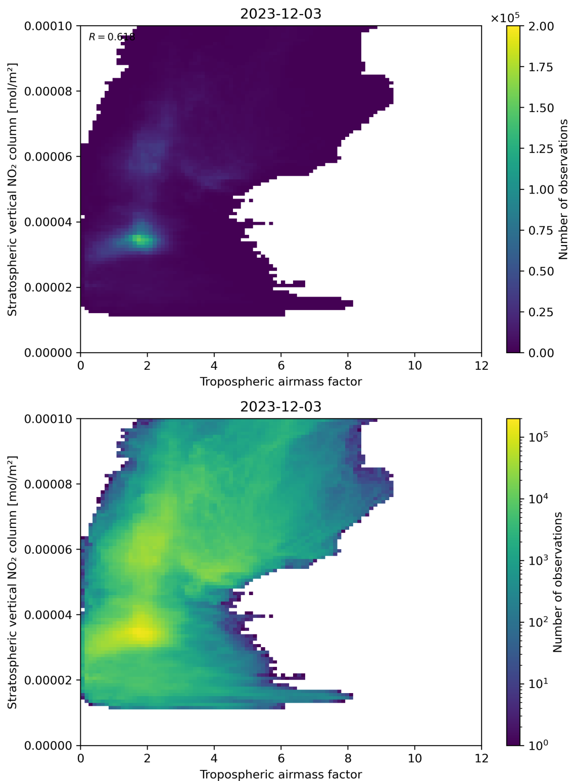
Figure 74: Scatter density plot of “Tropospheric air mass factor” against “Stratospheric vertical NO 2 column” for 2023-12-02 to 2023-12-04.
