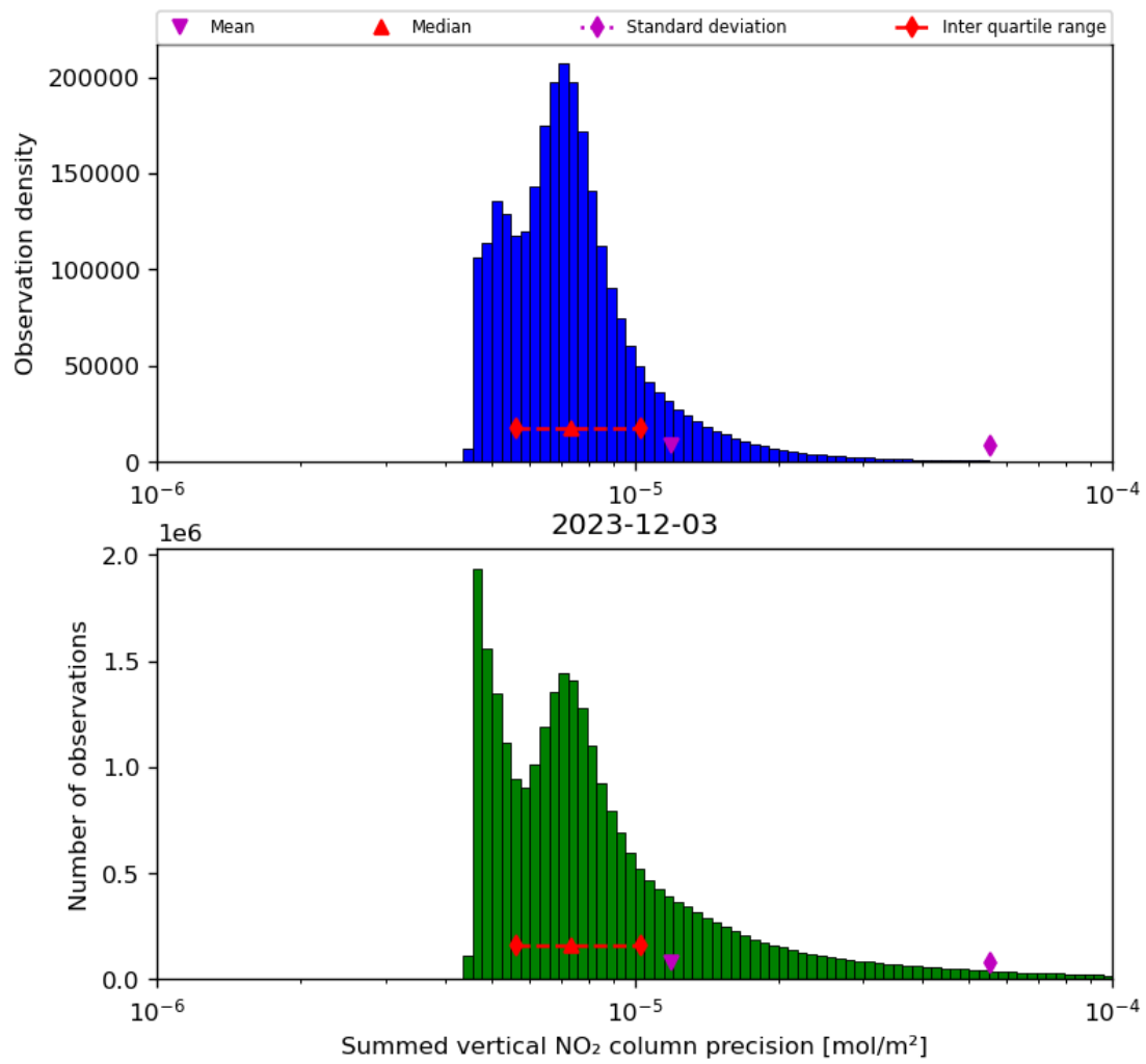
Figure 41: Histogram of "Summed vertical NO 2 column precision" for 2023-12-02 to 2023-12-04
