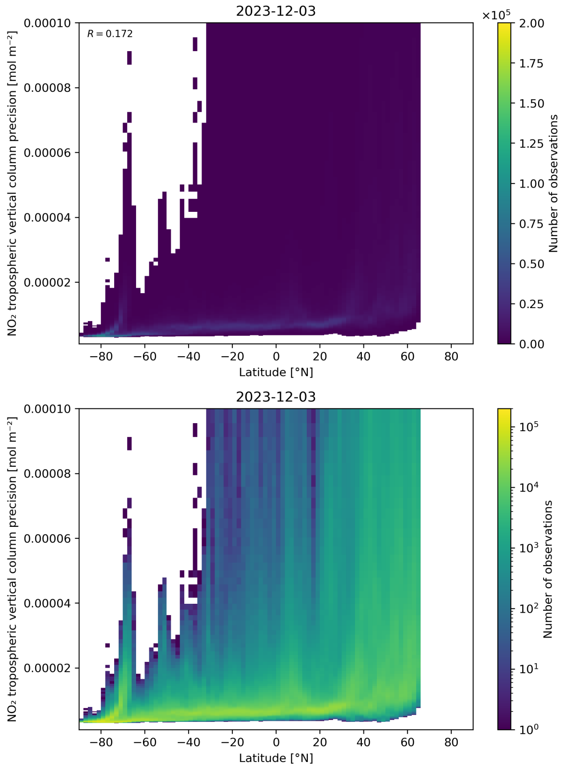
Figure 93: Scatter density plot of “Latitude” against “NO 2 tropospheric vertical column precision” for 2023-12-02 to 2023-12-04.
