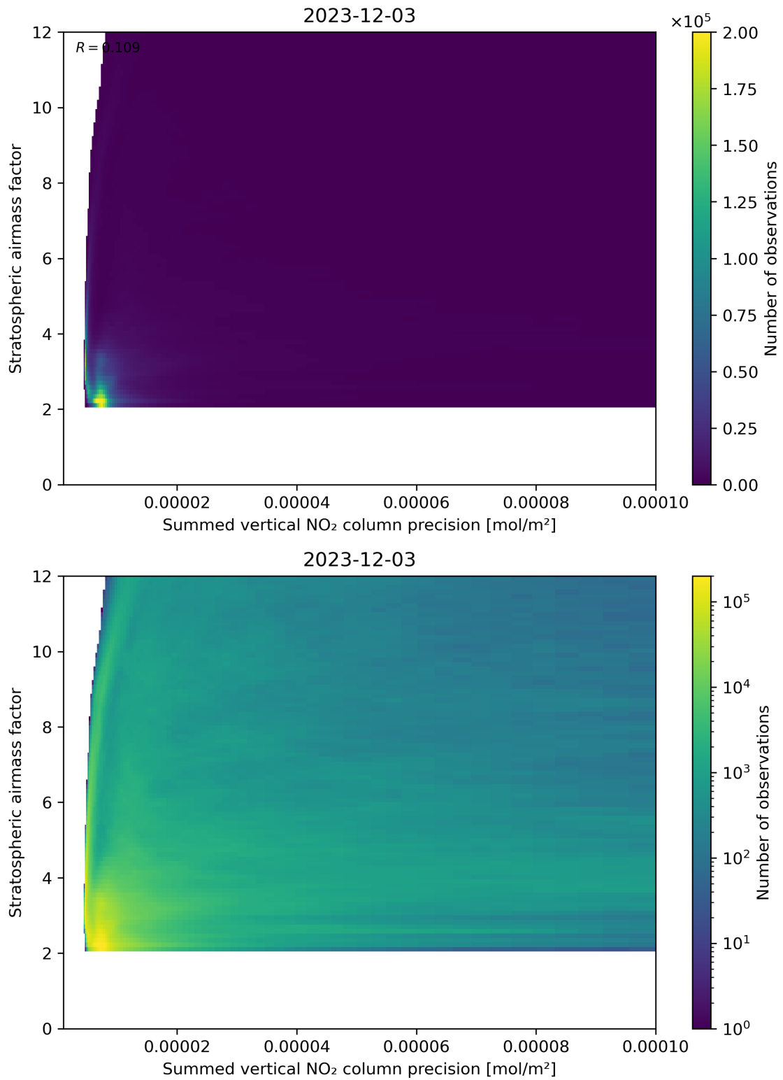
Figure 106: Scatter density plot of “Summed vertical NO 2 column precision” against “Stratospheric airmass factor” for 2023-12-02 to 2023-12-04.
