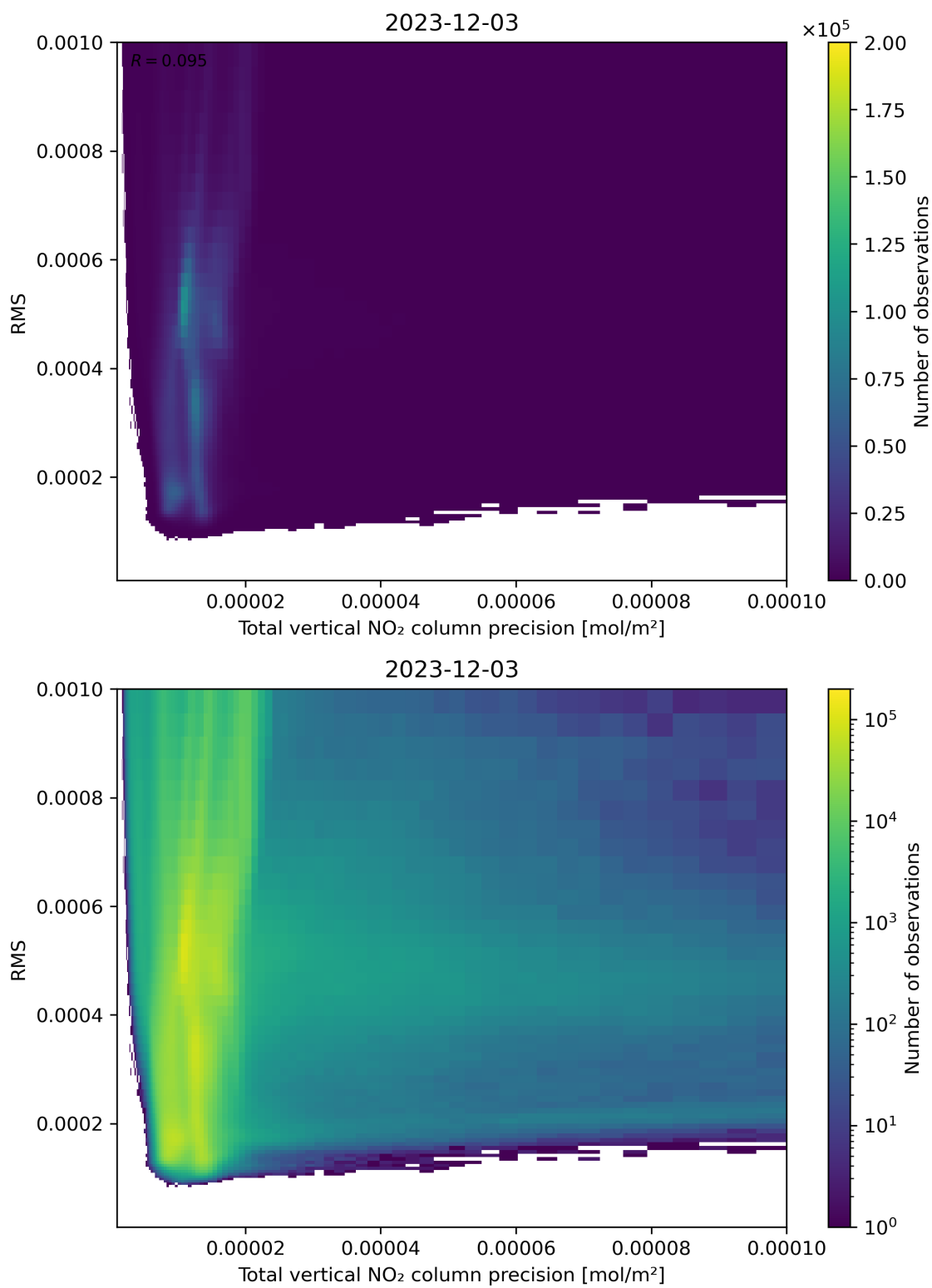
Figure 119: Scatter density plot of “Total vertical NO 2 column precision” against “RMS” for 2023-12-02 to 2023-12-04.
