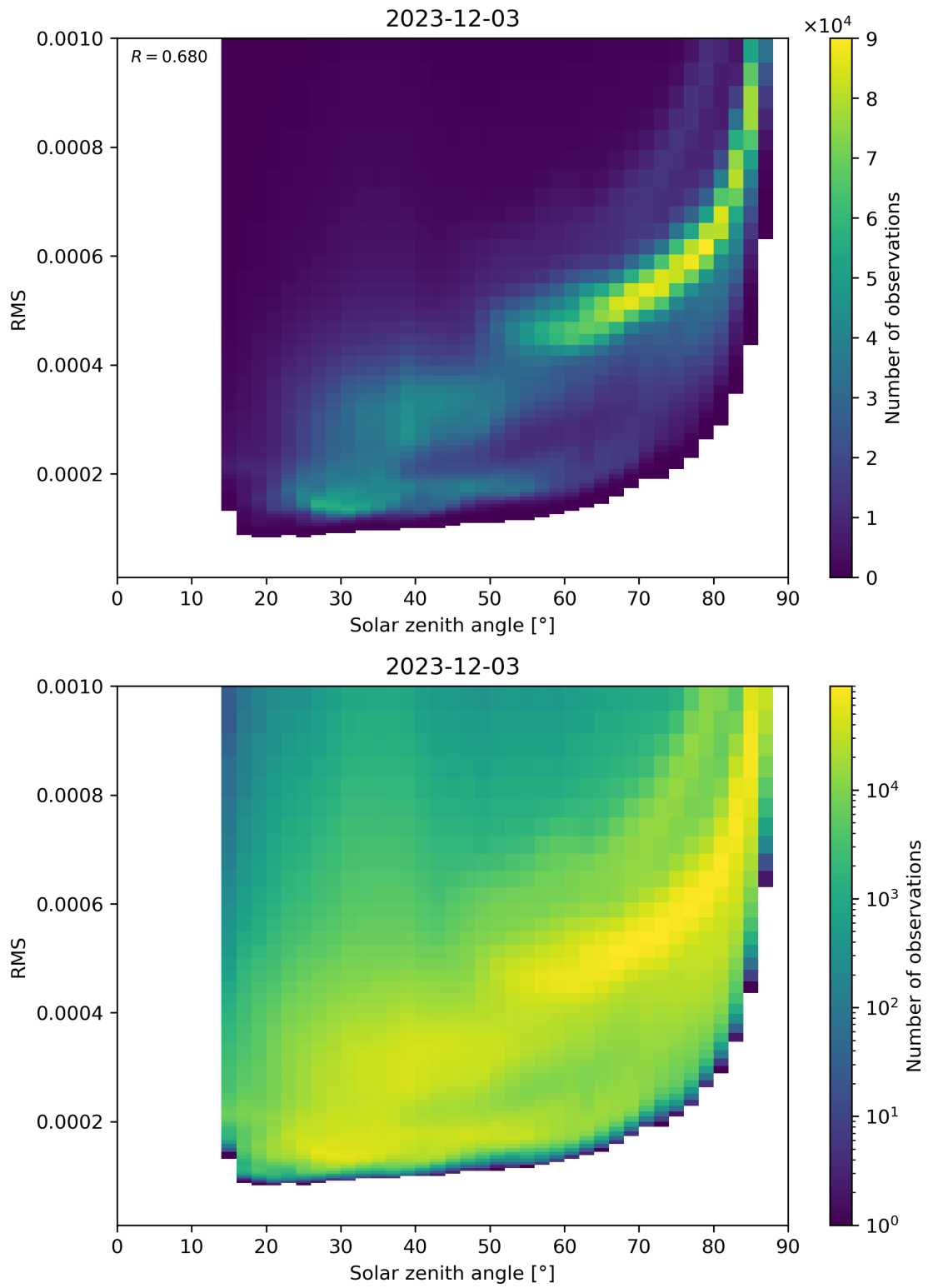
Figure 157: Scatter density plot of “Solar zenith angle” against “RMS” for 2023-12-02 to 2023-12-04.
