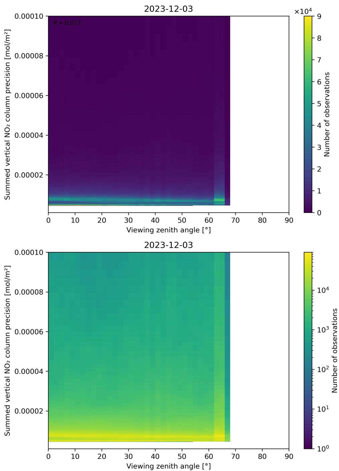
Figure 166: Scatter density plot of “Viewing zenith angle” against “Summed vertical NO 2 column precision” for 2023-12-02 to 2023-12-04.
