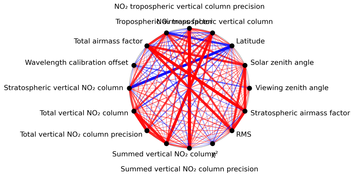
Figure 1: Map of correlation graph for 2023-12-02 to 2023-12-04.
