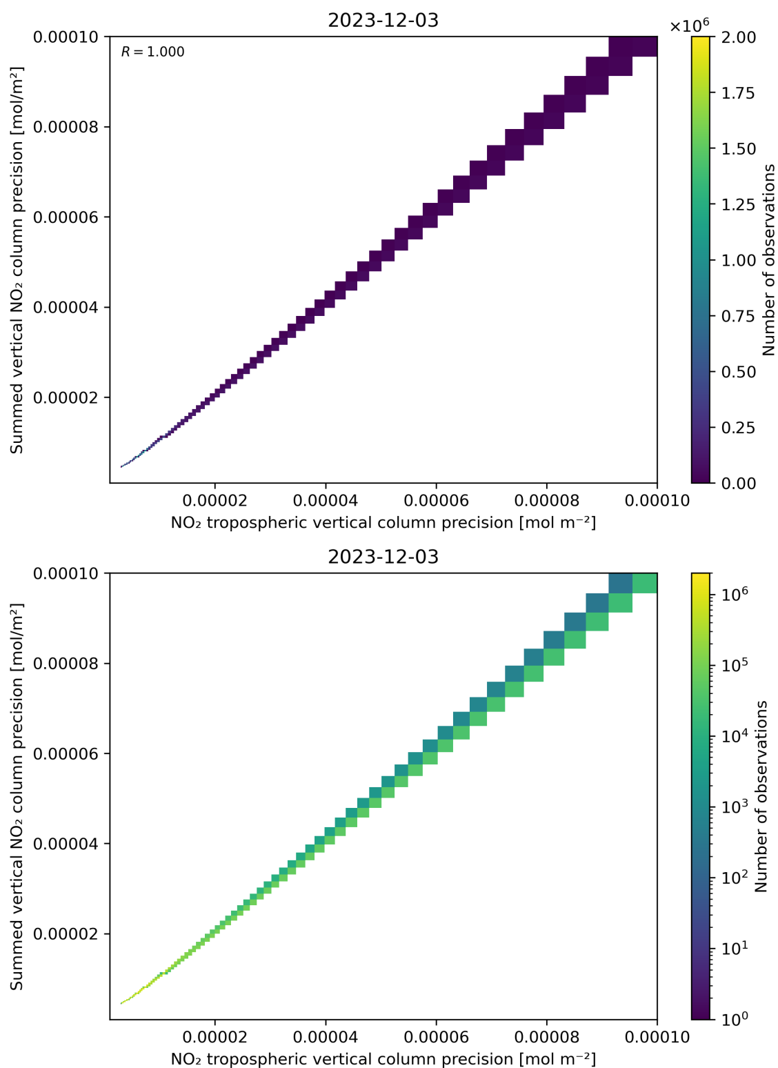
Figure 137: Scatter density plot of “NO 2 tropospheric vertical column precision” against “Summed vertical NO 2 column precision” for 2023-12-02 to 2023-12-04.
