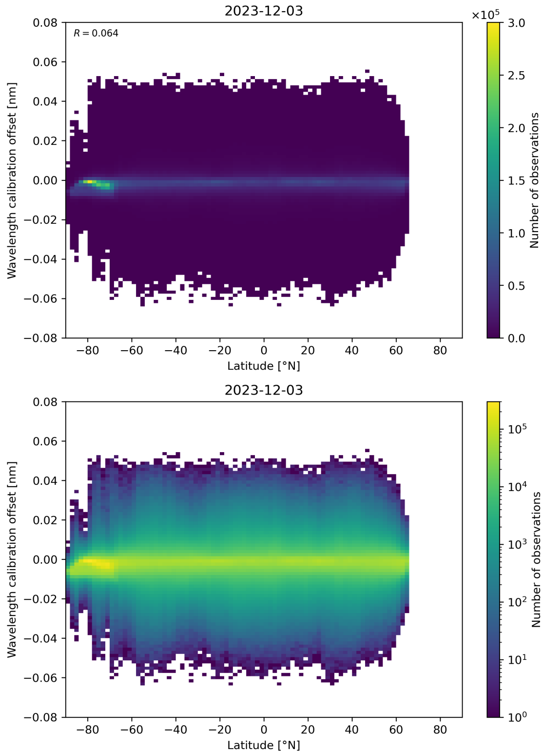
Figure 95: Scatter density plot of “Latitude” against “Wavelength calibration offset” for 2023-12-02 to 2023-12-04.
