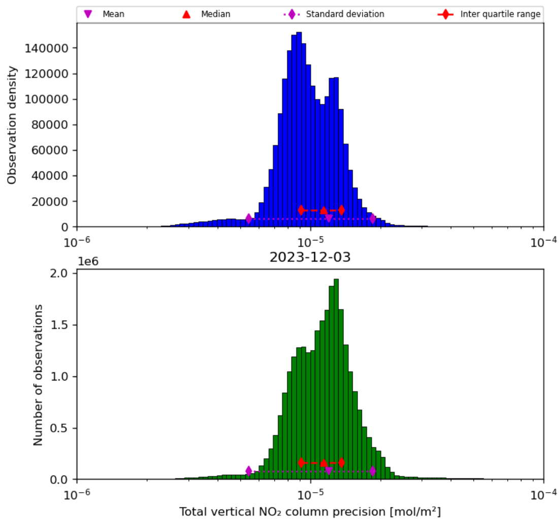
Figure 39: Histogram of “Total vertical NO 2 column precision” for 2023-12-02 to 2023-12-04
