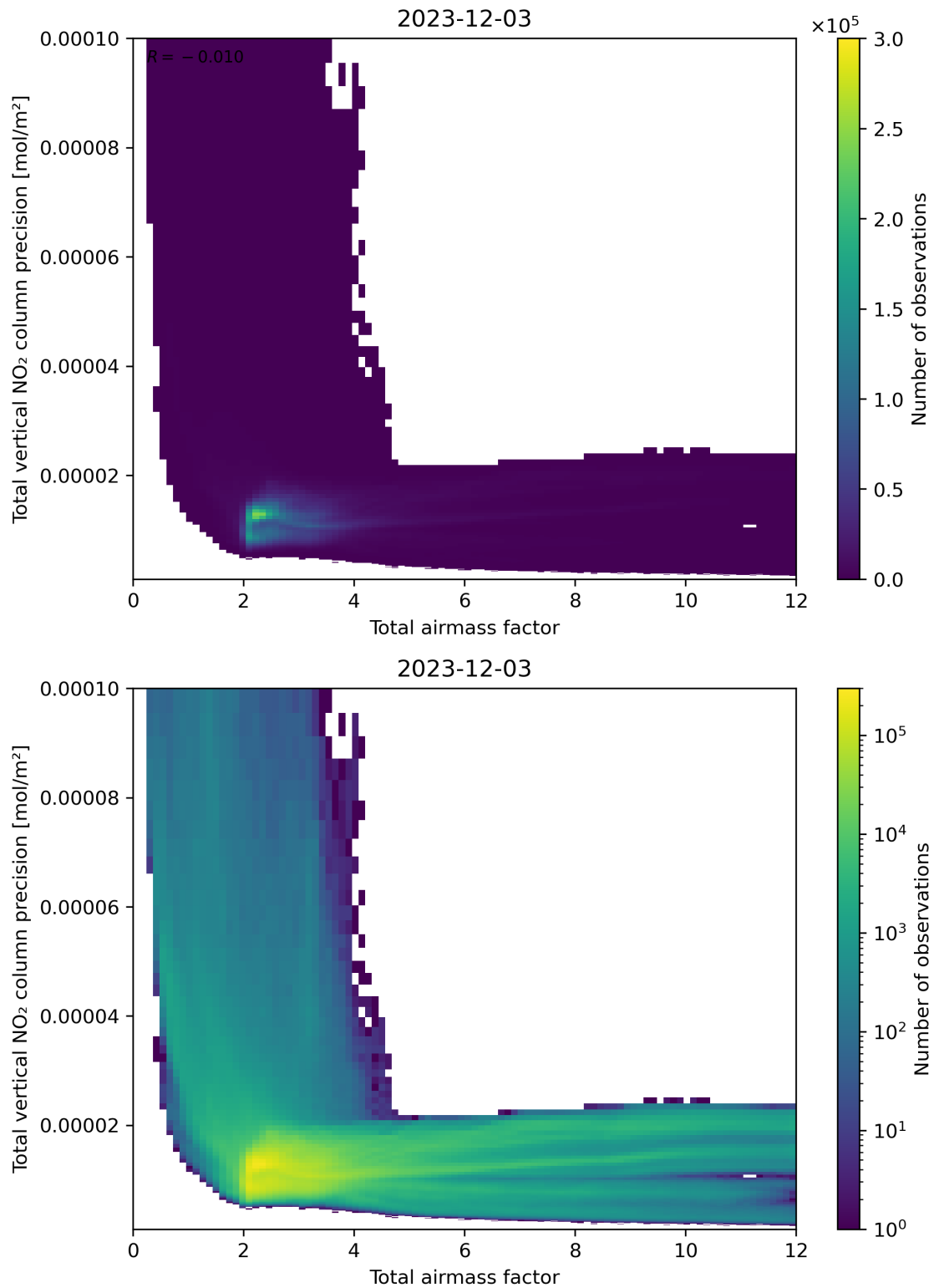
Figure 68: Scatter density plot of “Total airmass factor” against “Total vertical NO 2 column precision” for 2023-12-02 to 2023-12-04.
