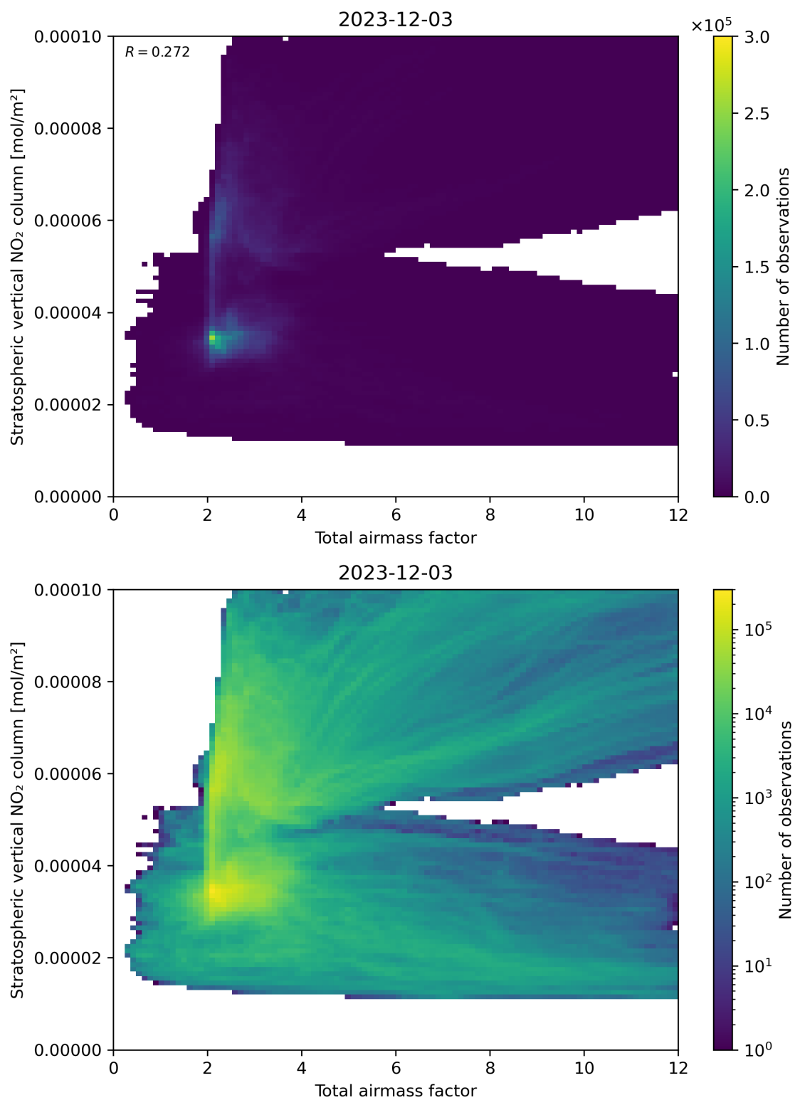
Figure 64: Scatter density plot of “Total airmass factor” against “Stratospheric vertical NO 2 column” for 2023-12-02 to 2023-12-04.
