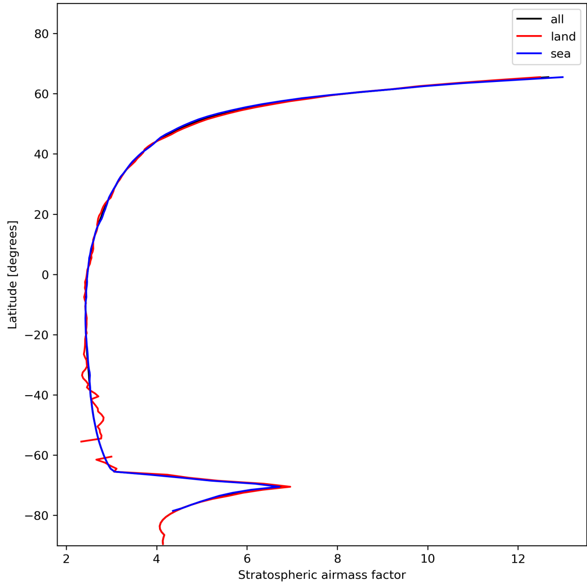
Figure 27: Zonal average of “Stratospheric air mass factor” for 2023-12-02 to 2023-12-04.
