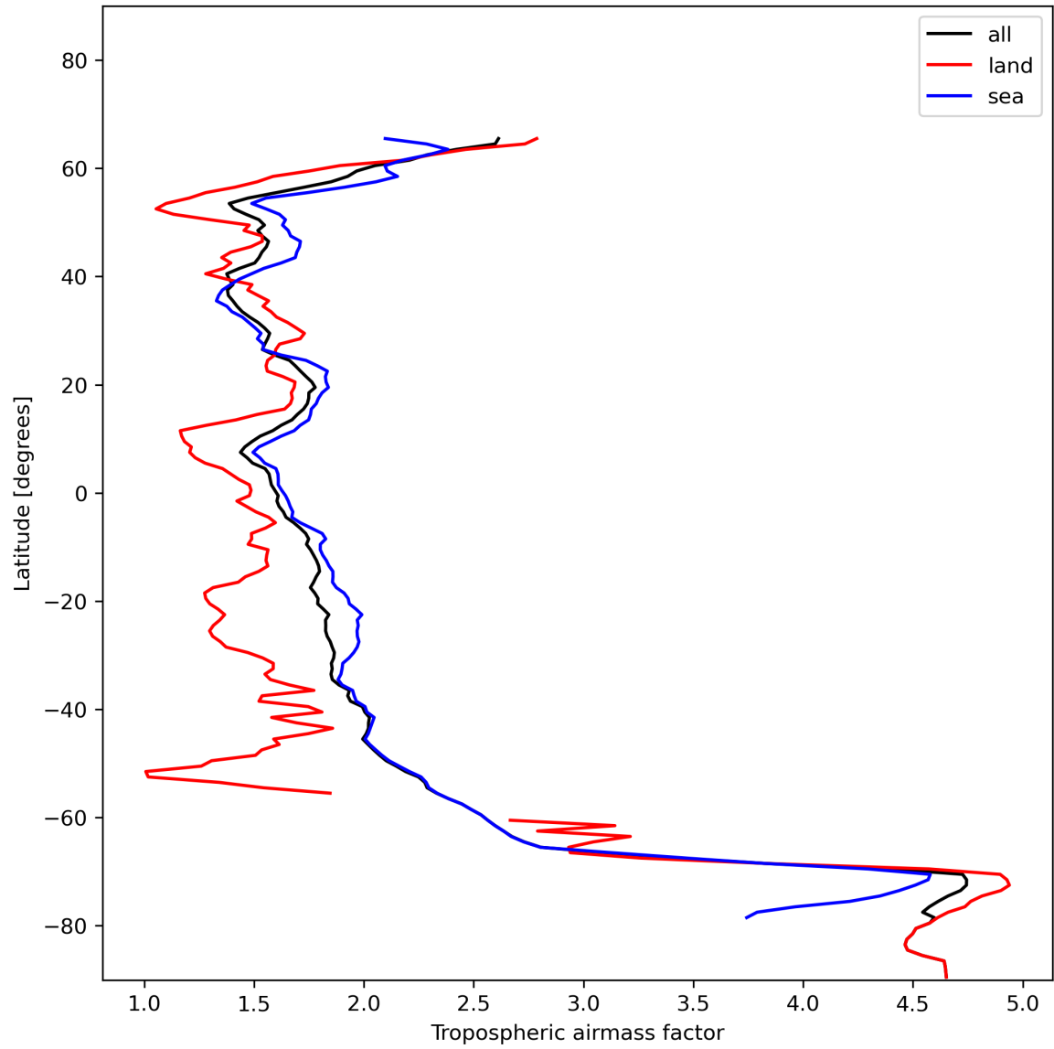
Figure 14: Zonal average of “Tropospheric airmass factor” for 2023-12-04 to 2023-12-05.
