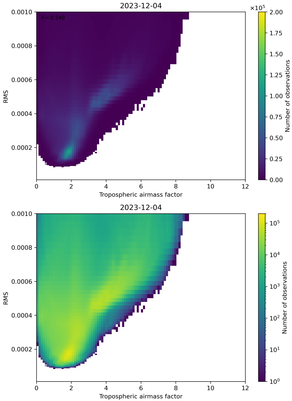
Figure 79: Scatter density plot of “Tropospheric airmass factor” against “RMS” for 2023-12-04 to 2023-12-05.
