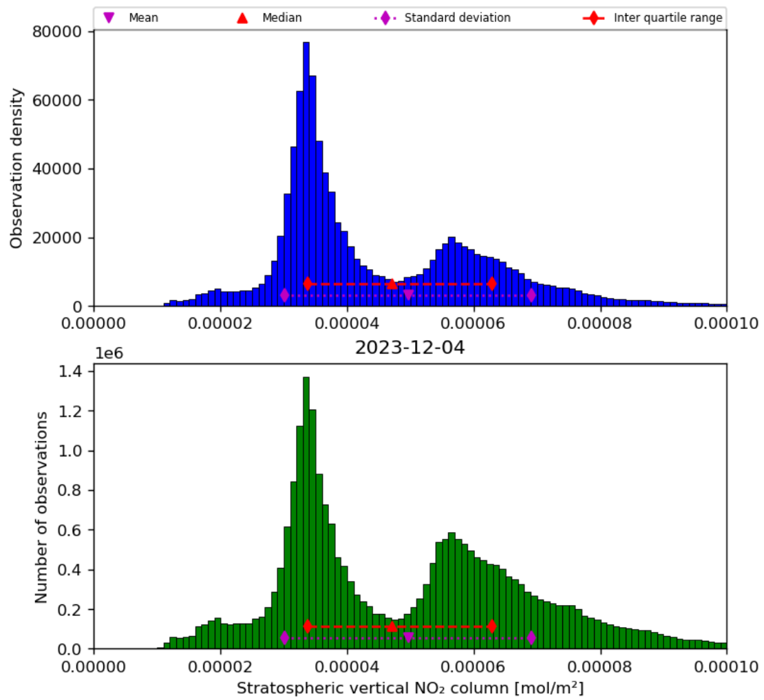
Figure 36: Histogram of “Stratospheric vertical NO 2 column” for 2023-12-04 to 2023-12-05
