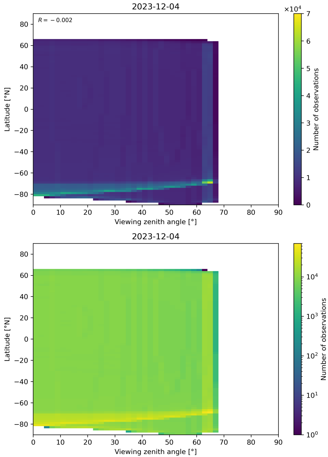
Figure 163: Scatter density plot of “Viewing zenith angle” against “Latitude” for 2023-12-04 to 2023-12-05.
