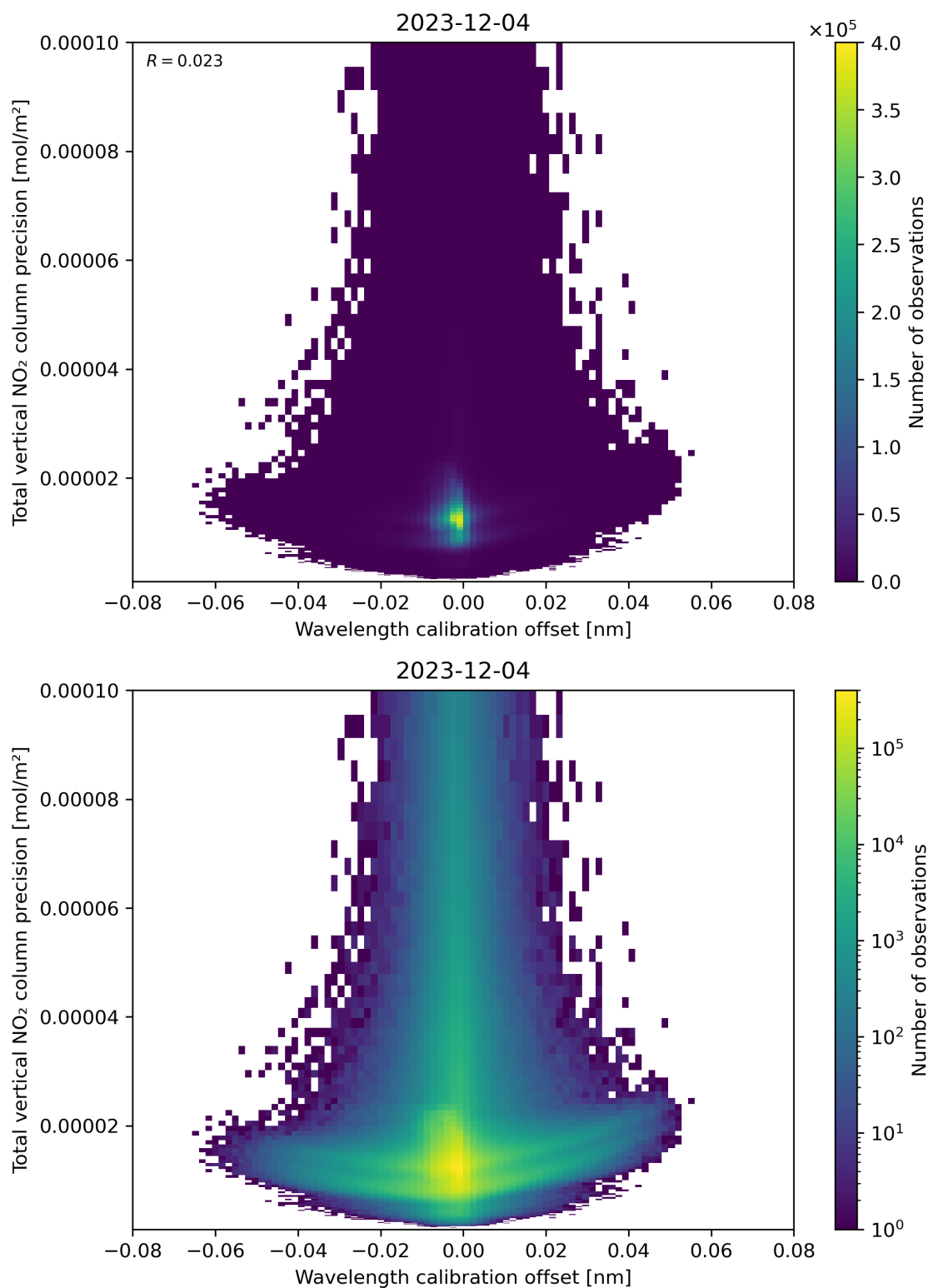
Figure 180: Scatter density plot of “Wavelength calibration offset” against “Total vertical NO 2 column precision” for 2023-12-04 to 2023-12-05.
