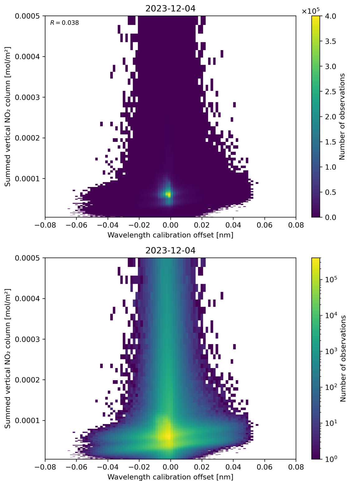
Figure 177: Scatter density plot of “Wavelength calibration offset” against “Summed vertical NO 2 column” for 2023-12-04 to 2023-12-05.
