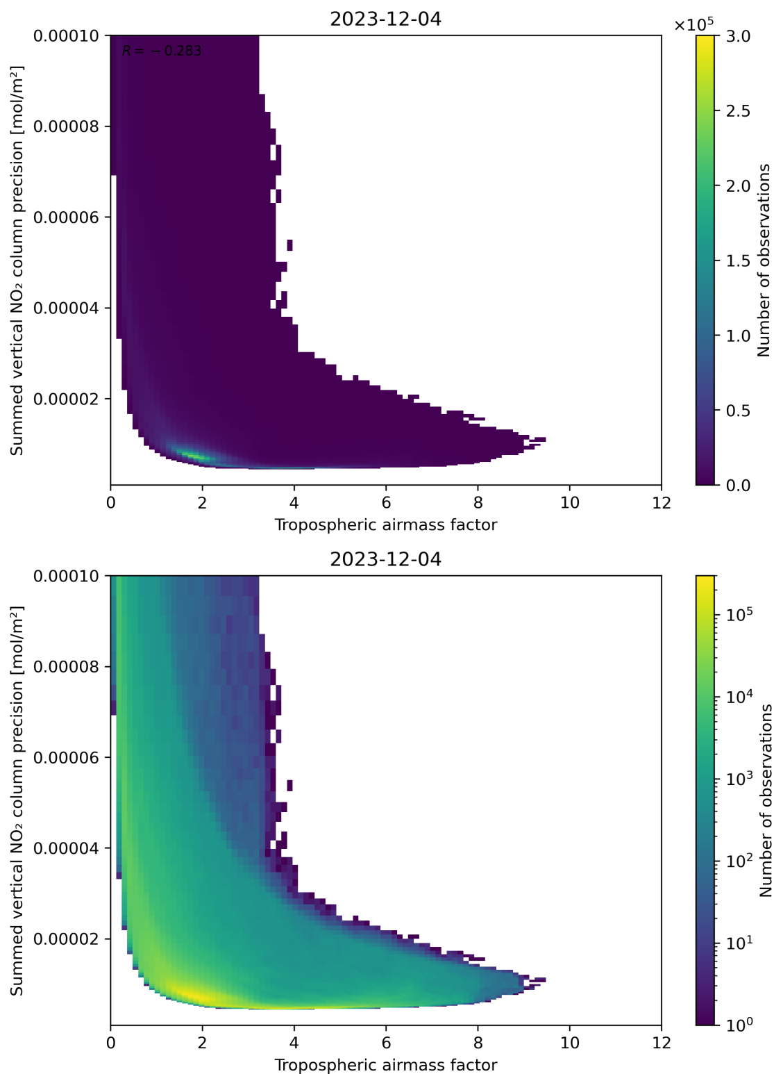
Figure 76: Scatter density plot of “Tropospheric air mass factor” against “Summed vertical NO 2 column precision” for 2023-12-04 to 2023-12-05.
