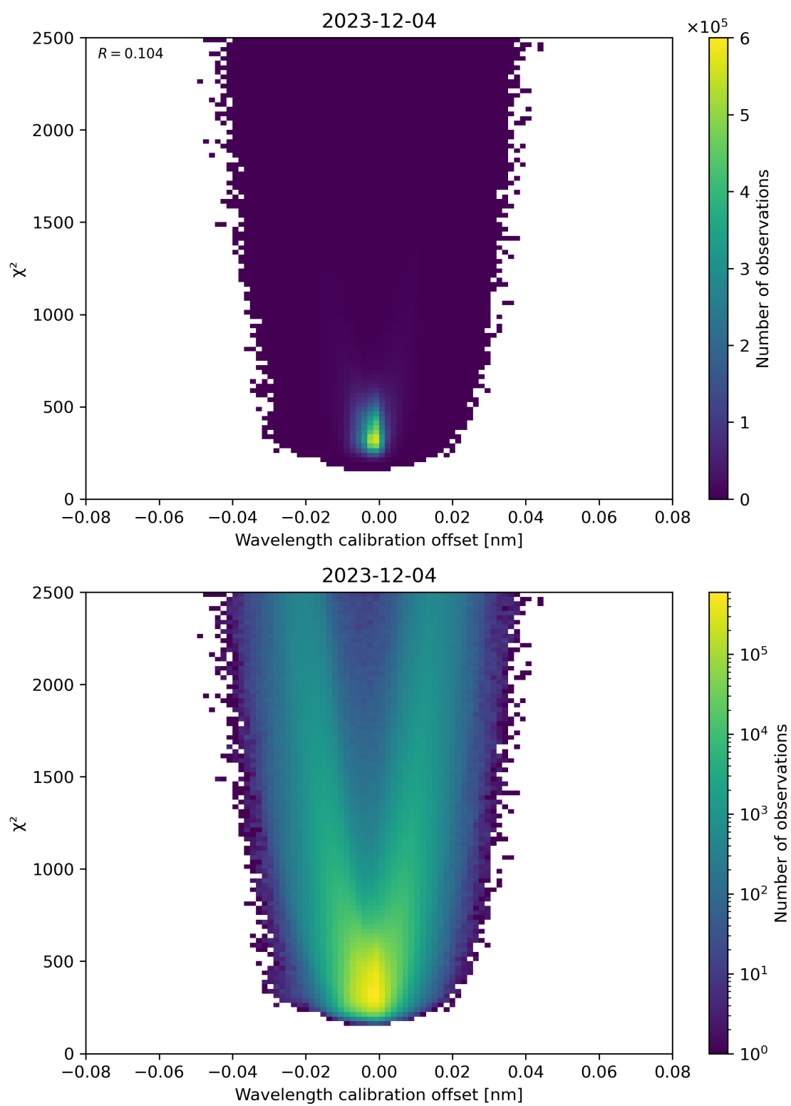
Figure 175: Scatter density plot of “Wavelength calibration offset” against “ \chi^2 ” for 2023-12-04 to 2023-12-05.
