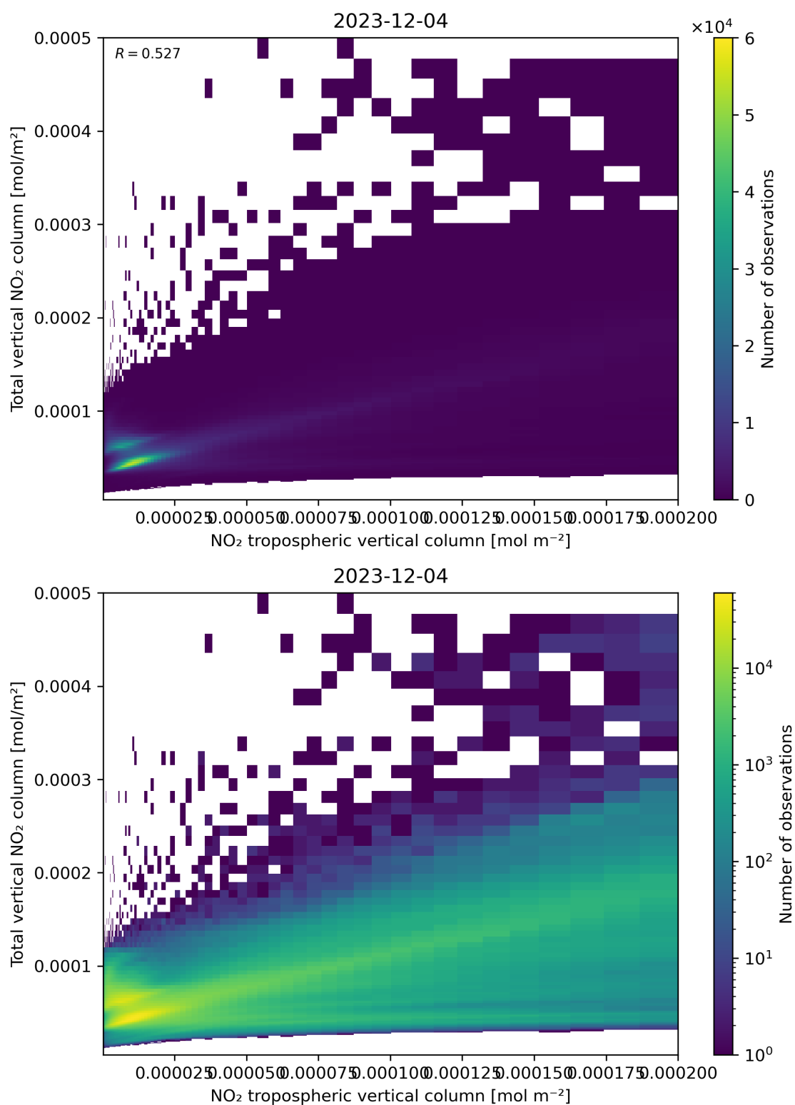
Figure 128: Scatter density plot of “NO 2 tropospheric vertical column” against “Total vertical NO 2 column” for 2023-12-04 to 2023-12-05.
