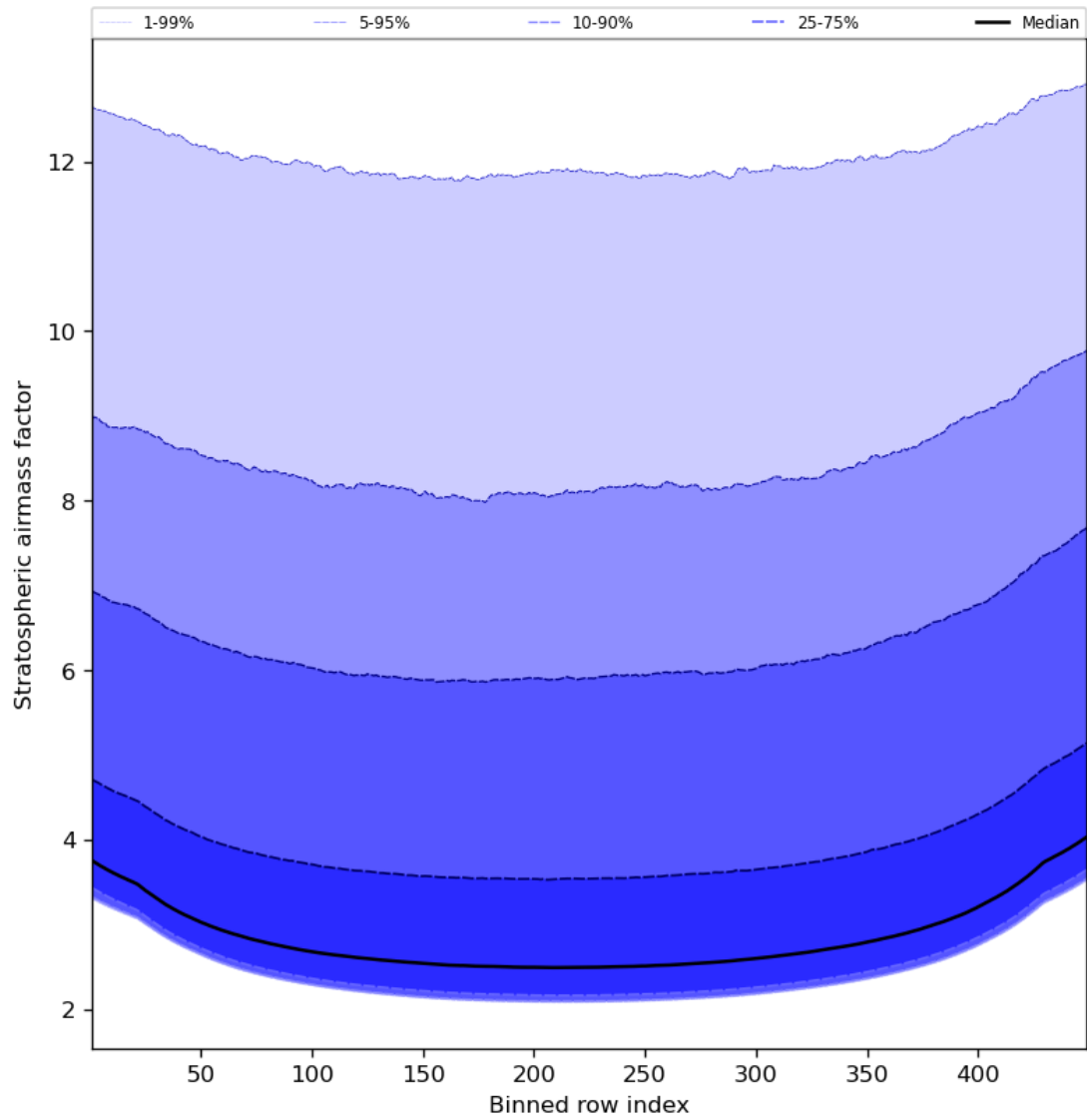
Figure 61: Along track statistics of “Stratospheric airmass factor” for 2023-12-04 to 2023-12-05
