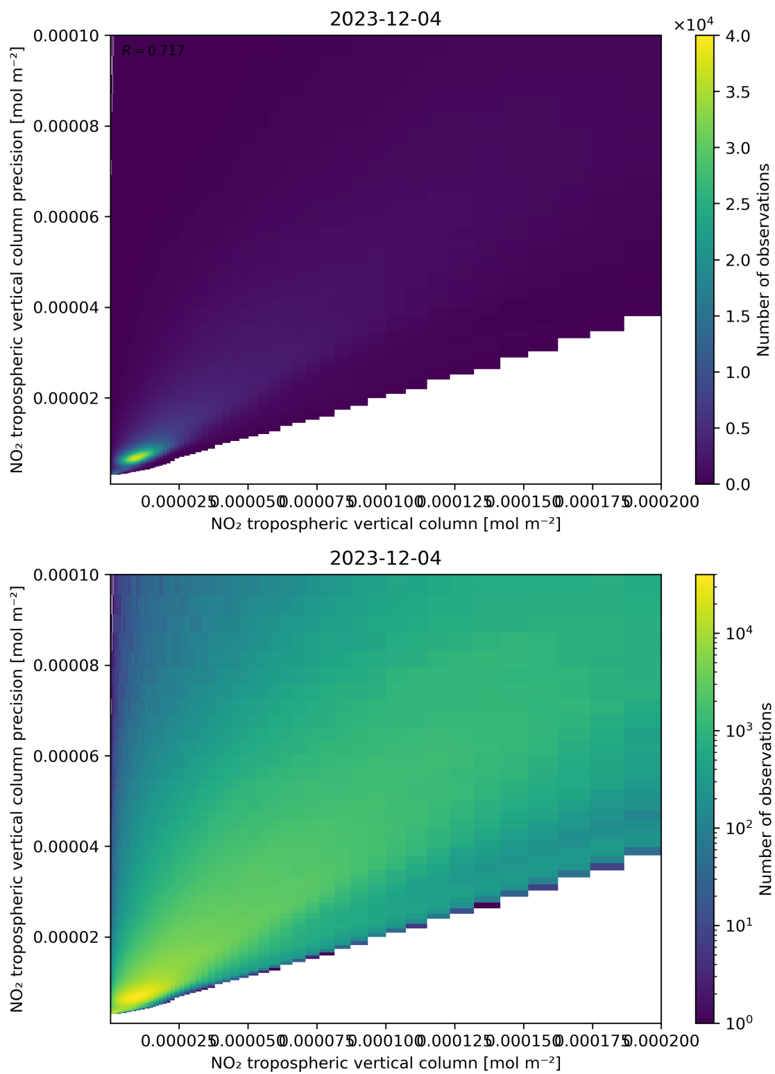
Figure 130: Scatter density plot of “NO 2 tropospheric vertical column” against “NO 2 tropospheric vertical column precision” for 2023-12-04 to 2023-12-05.
