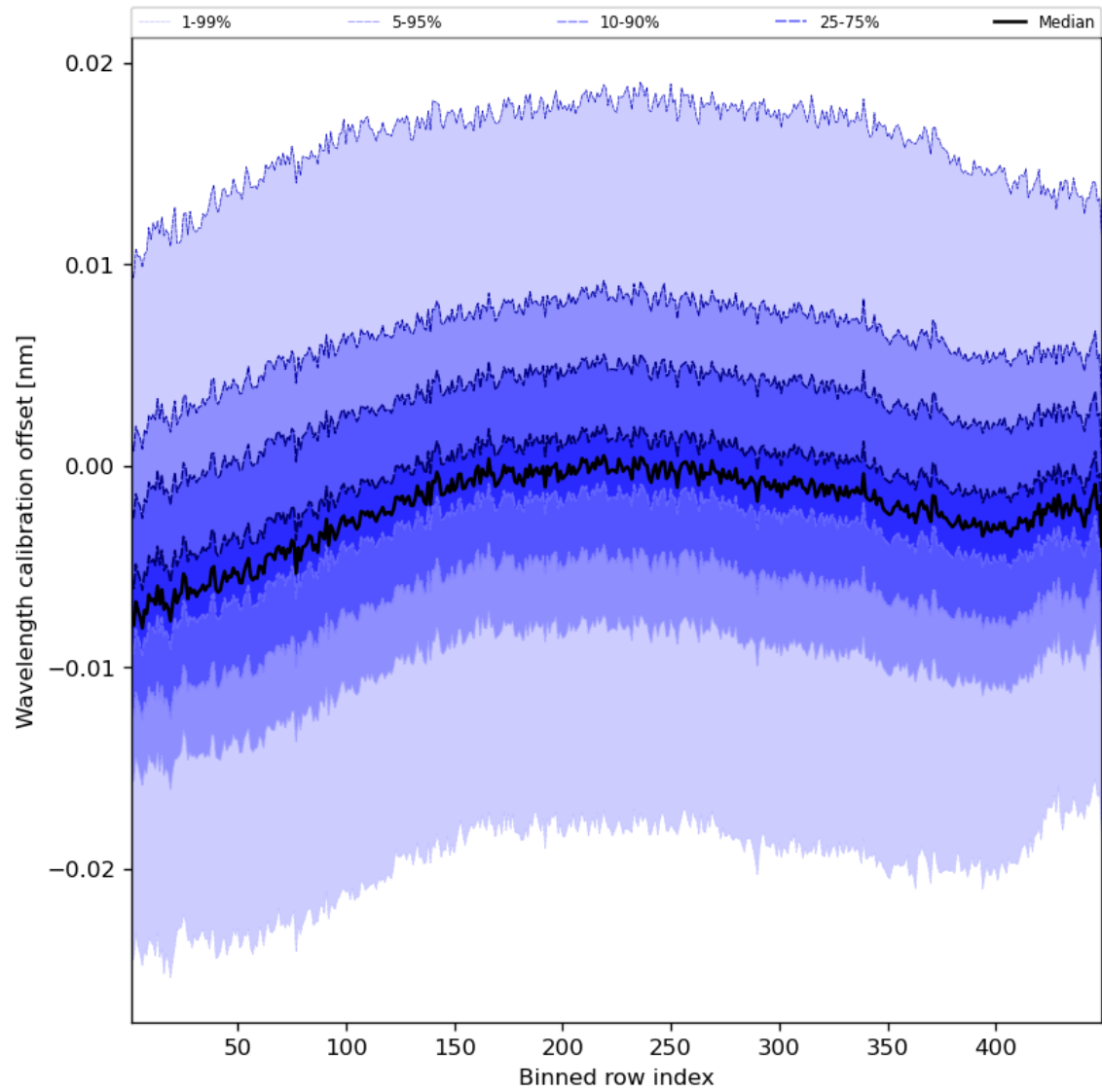
Figure 52: Along track statistics of “Wavelength calibration offset” for 2023-12-04 to 2023-12-05
