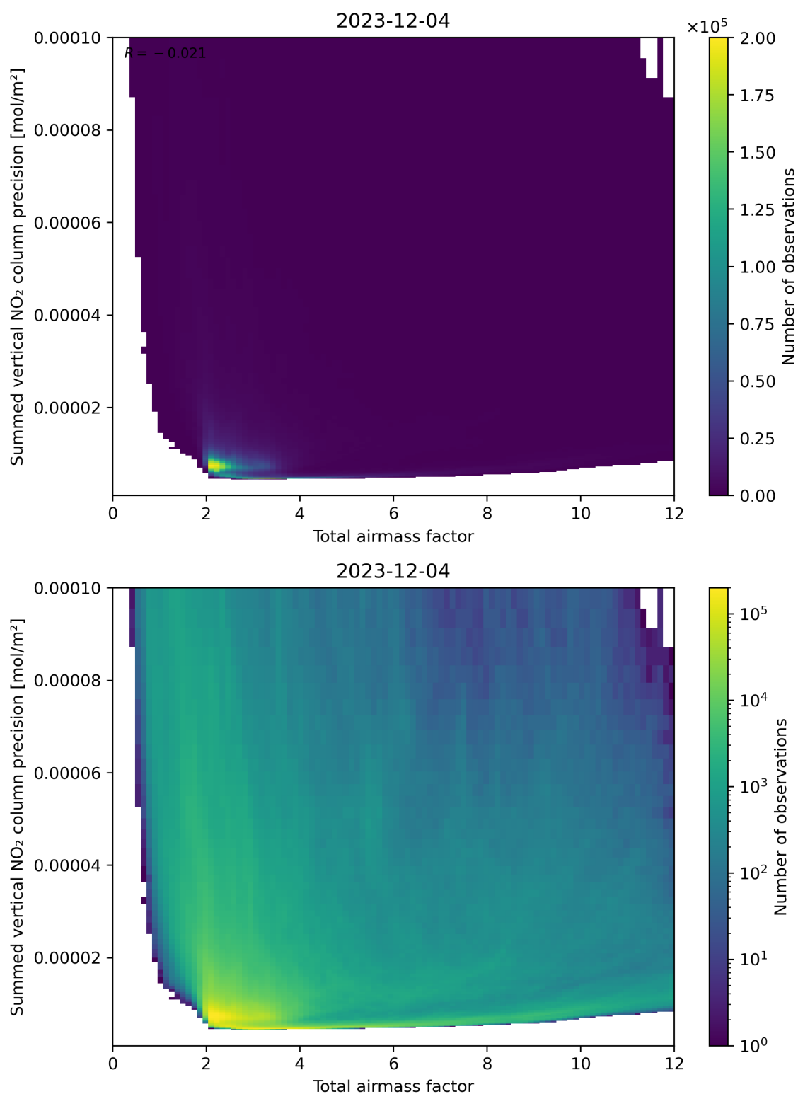
Figure 66: Scatter density plot of “Total airmass factor” against “Summed vertical NO 2 column precision” for 2023-12-04 to 2023-12-05.
