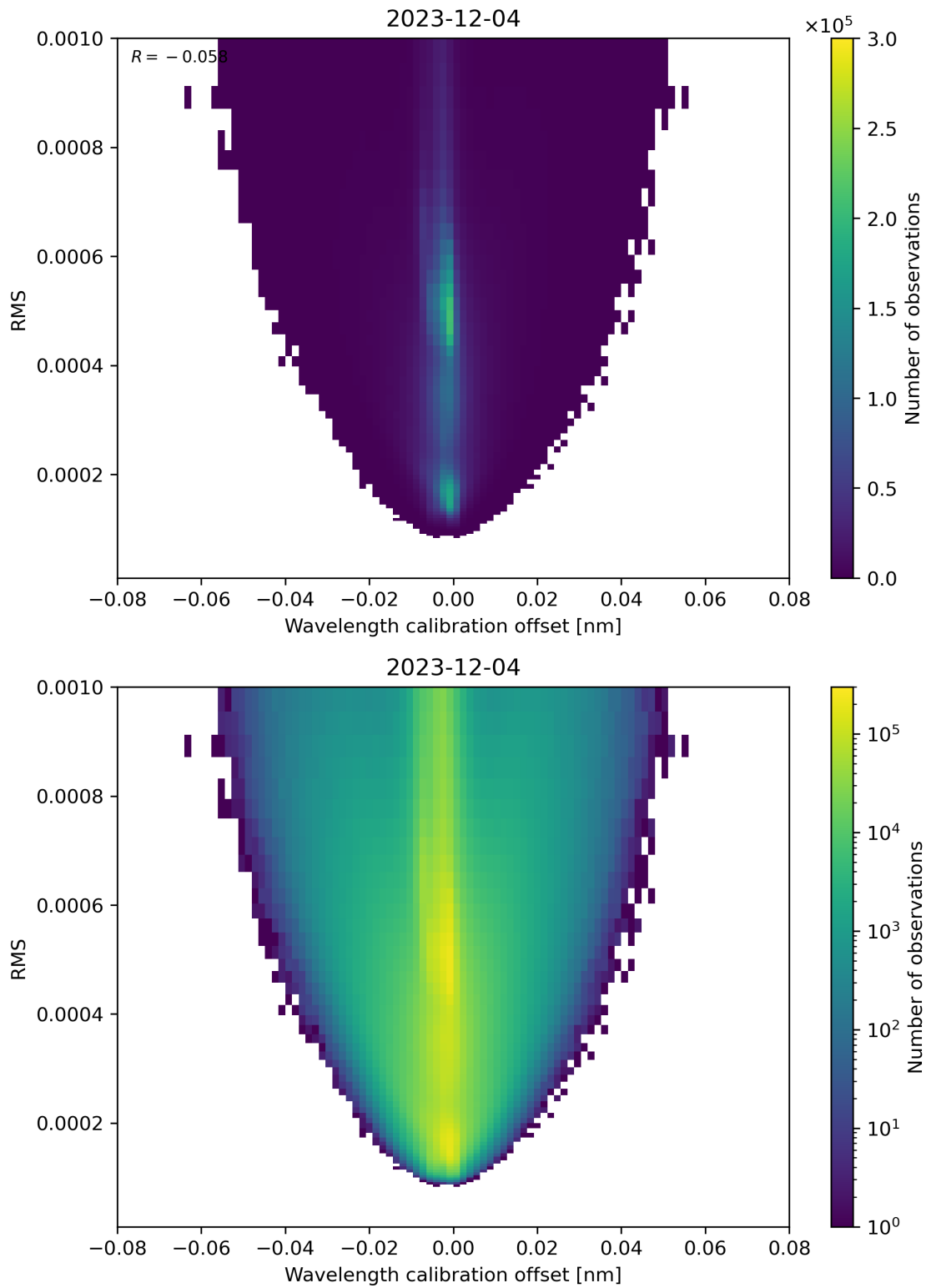
Figure 181: Scatter density plot of “Wavelength calibration offset” against “RMS” for 2023-12-04 to 2023-12-05.
