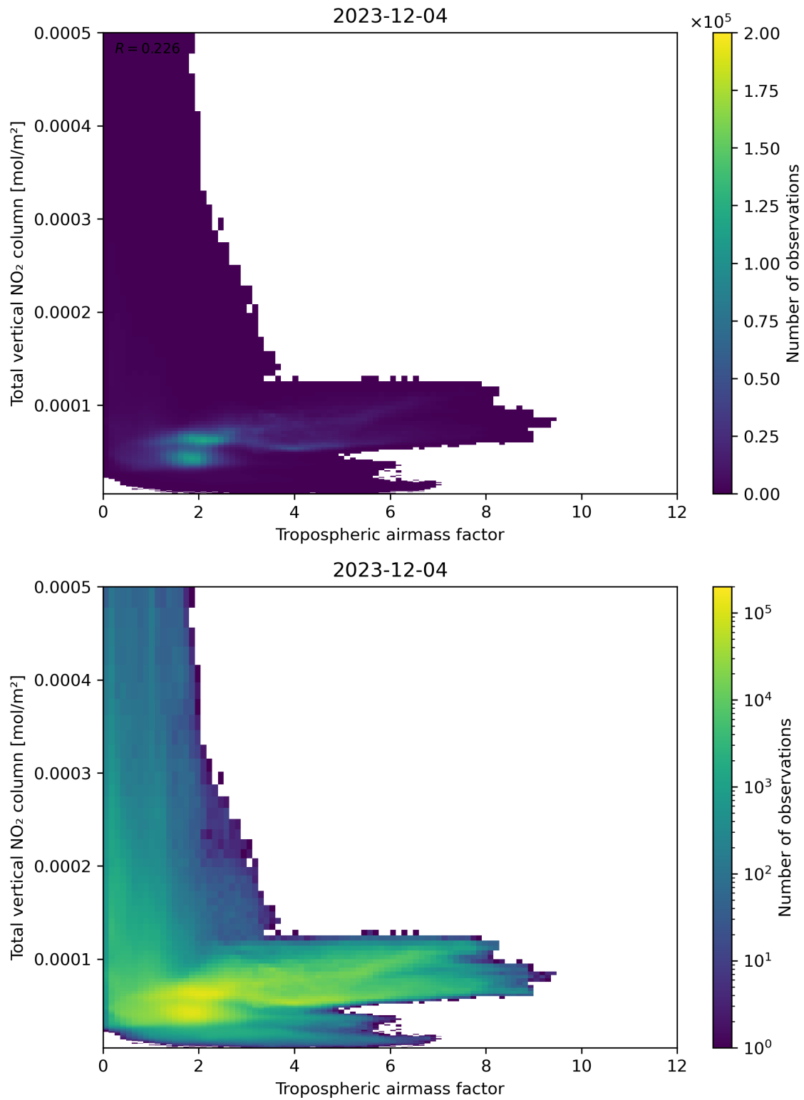
Figure 77: Scatter density plot of “Tropospheric airmass factor” against “Total vertical NO 2 column” for 2023-12-04 to 2023-12-05.
