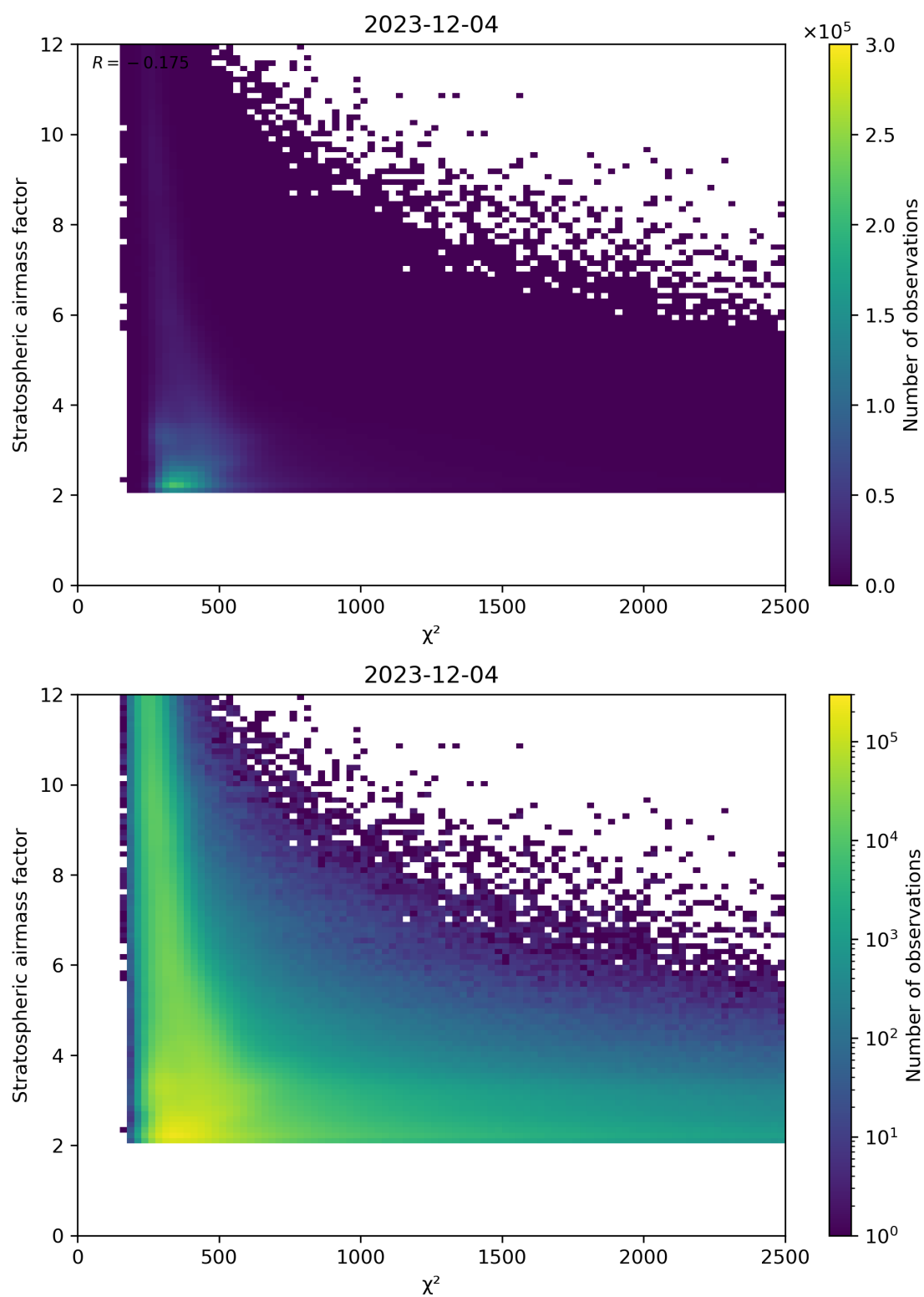
Figure 81: Scatter density plot of “ \chi^2 ” against “Stratospheric airmass factor” for 2023-12-04 to 2023-12-05.
