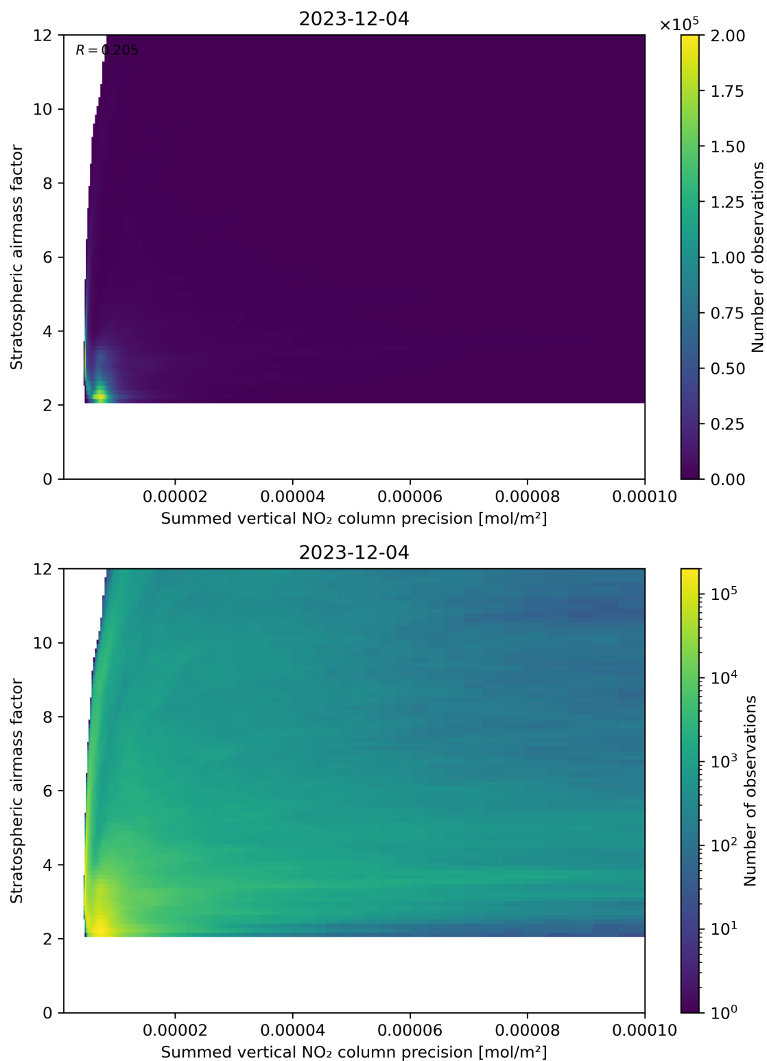
Figure 106: Scatter density plot of “Summed vertical NO 2 column precision” against “Stratospheric airmass factor” for 2023-12-04 to 2023-12-05.
