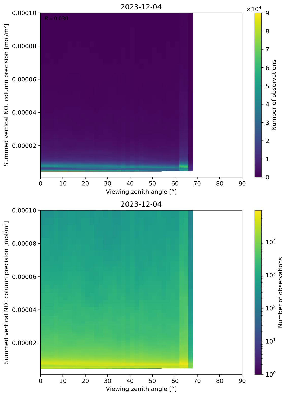
Figure 166: Scatter density plot of “Viewing zenith angle” against “Summed vertical NO 2 column precision” for 2023-12-04 to 2023-12-05.
