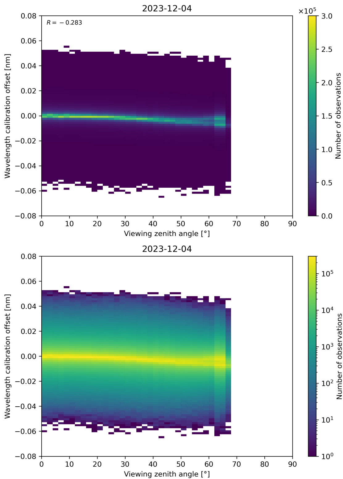
Figure 173: Scatter density plot of “Viewing zenith angle” against “Wavelength calibration offset” for 2023-12-04 to 2023-12-05.
