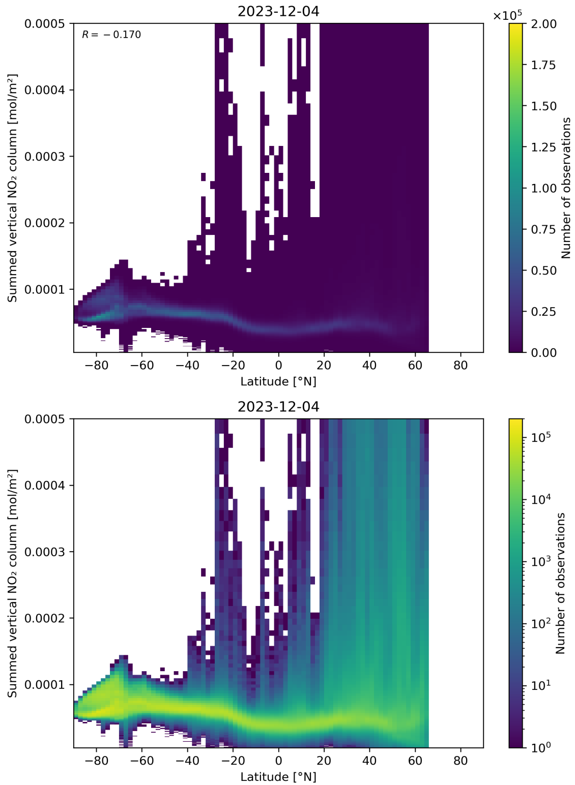
Figure 88: Scatter density plot of “Latitude” against “Summed vertical NO 2 column” for 2023-12-04 to 2023-12-05.
