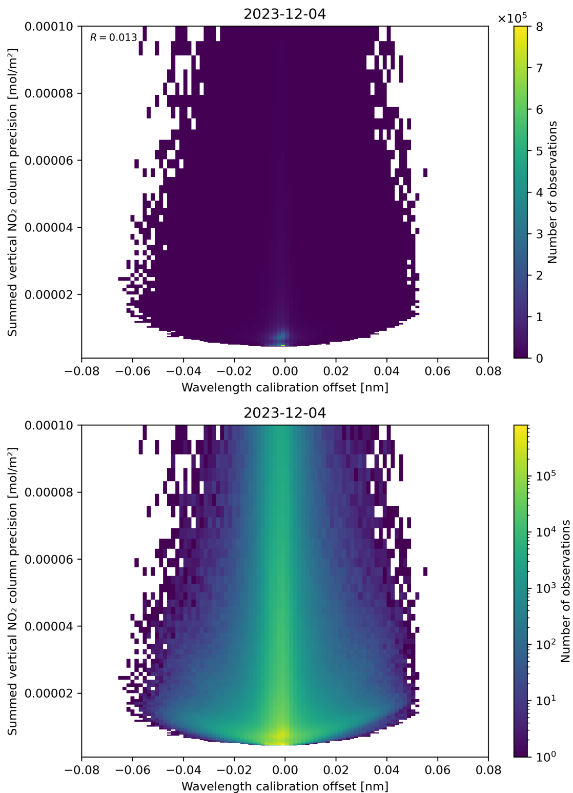
Figure 178: Scatter density plot of “Wavelength calibration offset” against “Summed vertical NO 2 column precision” for 2023-12-04 to 2023-12-05.
