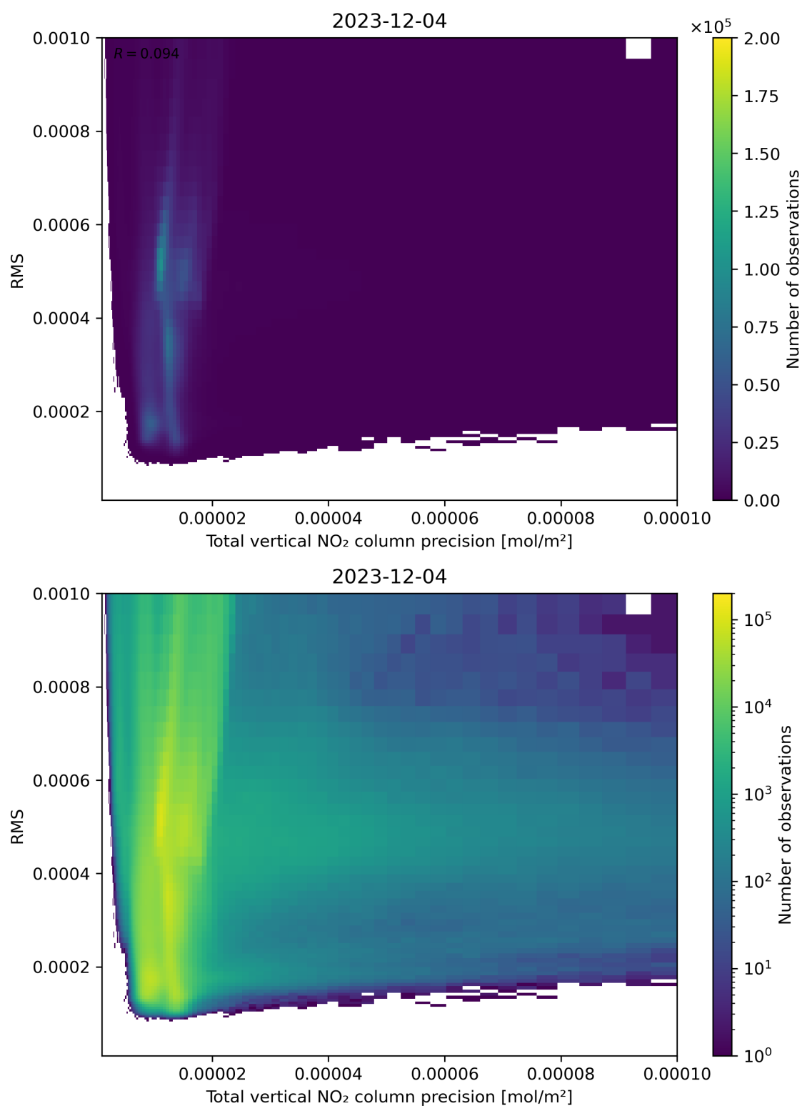
Figure 119: Scatter density plot of “Total vertical NO 2 column precision” against “RMS” for 2023-12-04 to 2023-12-05.
