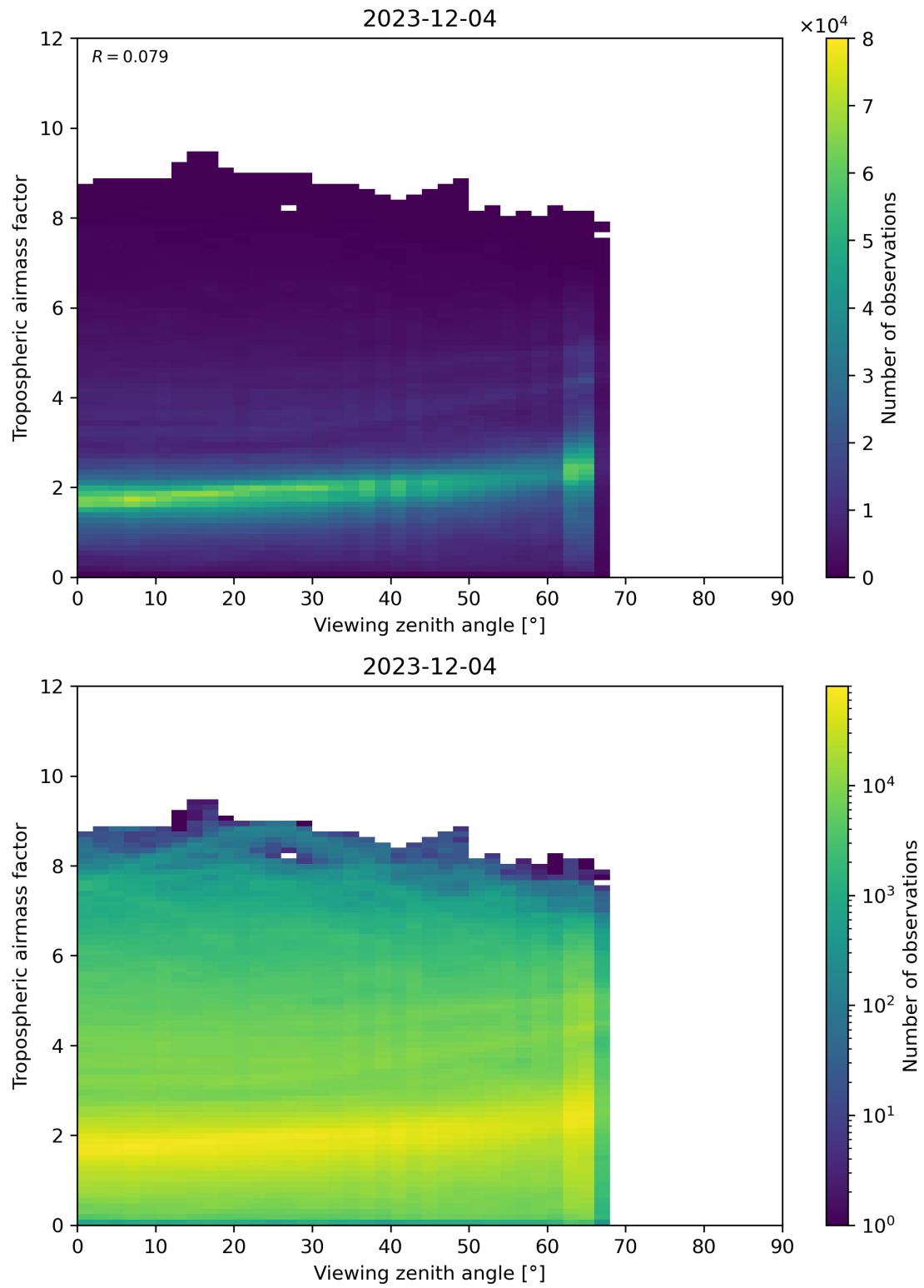
Figure 161: Scatter density plot of “Viewing zenith angle” against “Tropospheric airmass factor” for 2023-12-04 to 2023-12-05.
