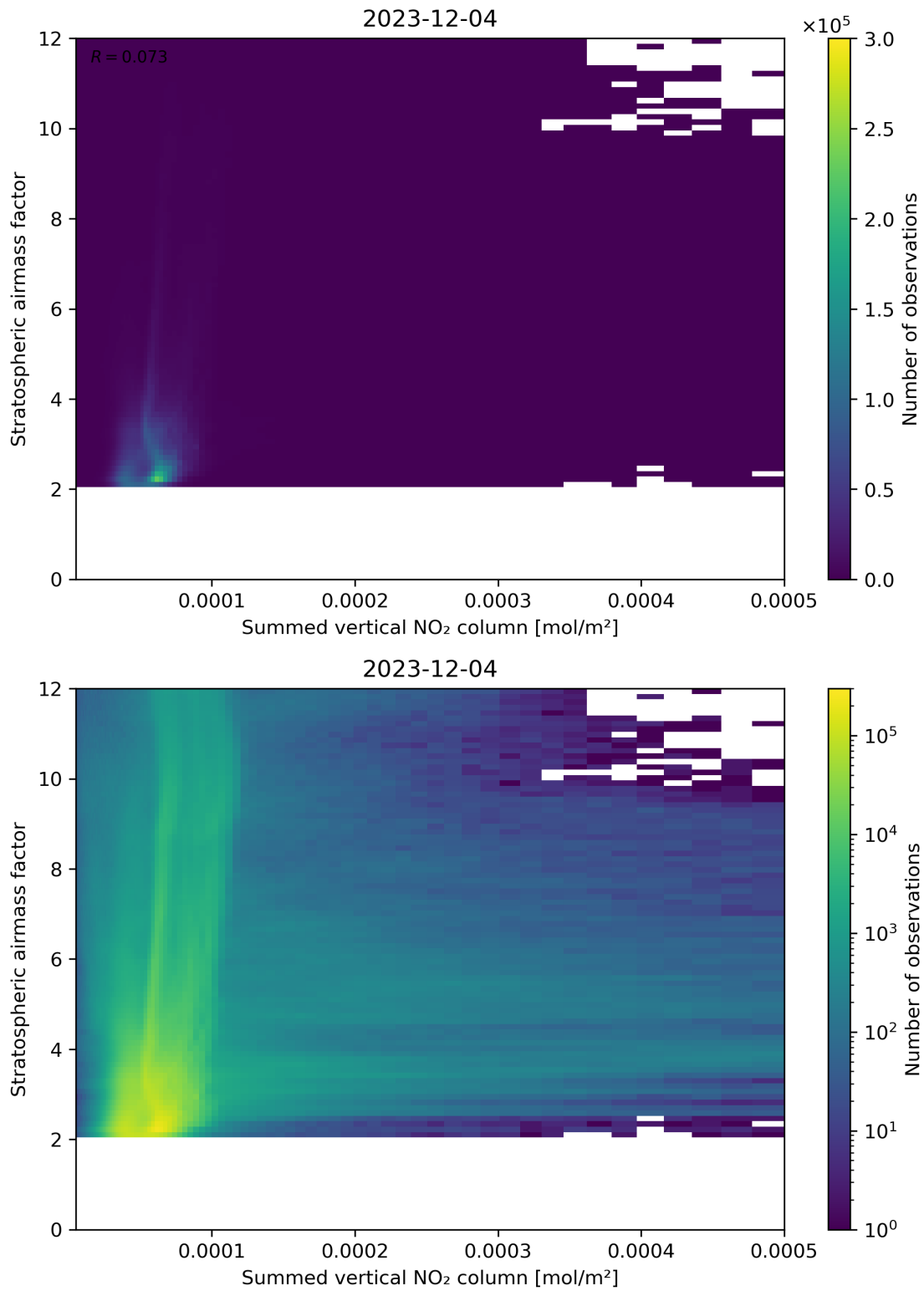
Figure 103: Scatter density plot of “Summed vertical NO 2 column” against “Stratospheric airmass factor” for 2023-12-04 to 2023-12-05.
