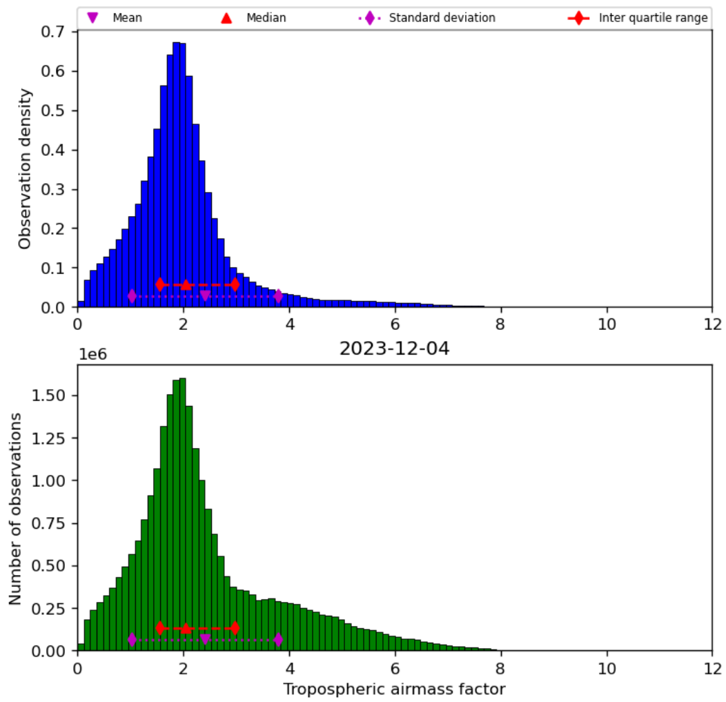
Figure 31: Histogram of “Tropospheric airmass factor” for 2023-12-04 to 2023-12-05
