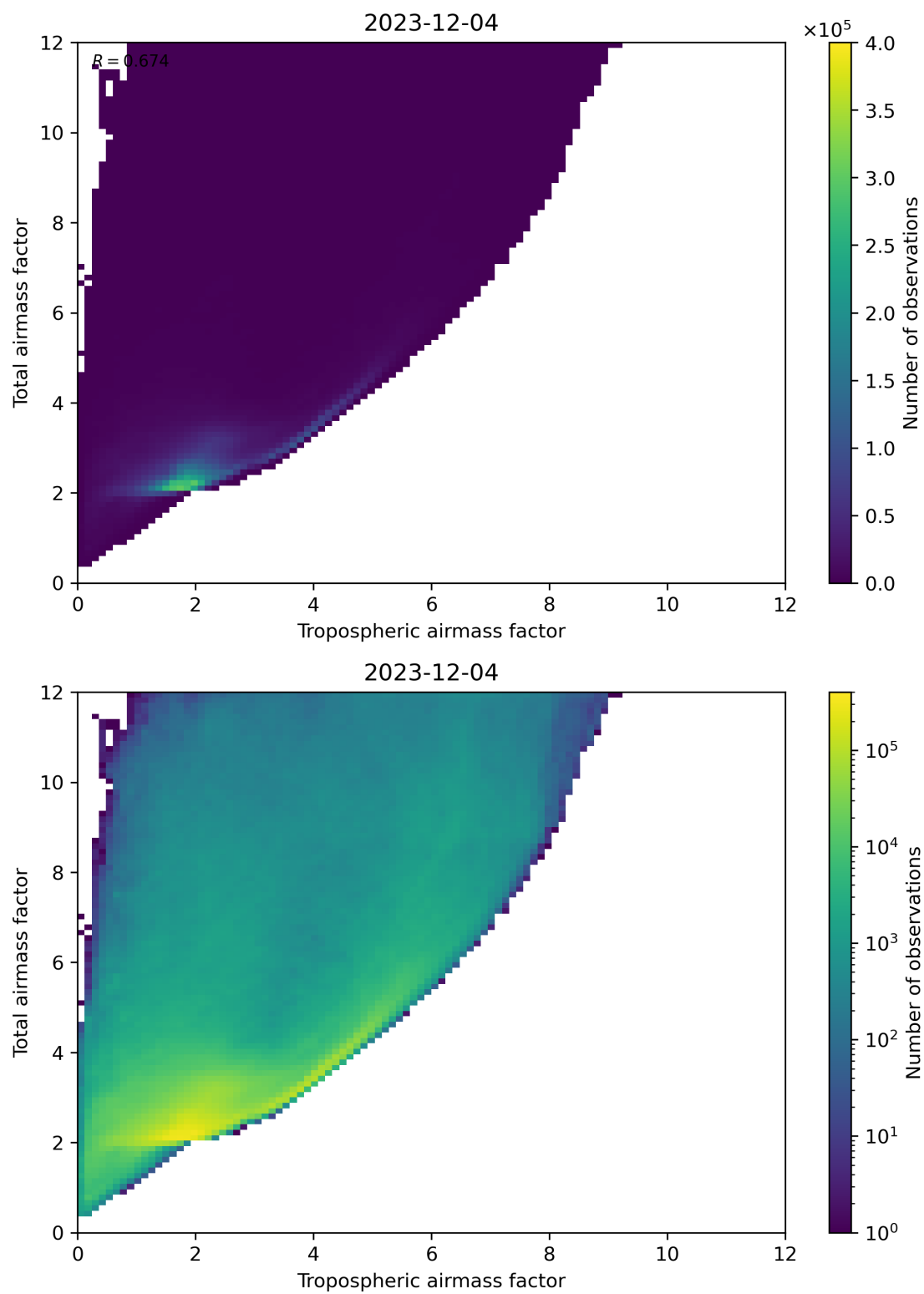
Figure 72: Scatter density plot of “Tropospheric airmass factor” against “Total airmass factor” for 2023-12-04 to 2023-12-05.
