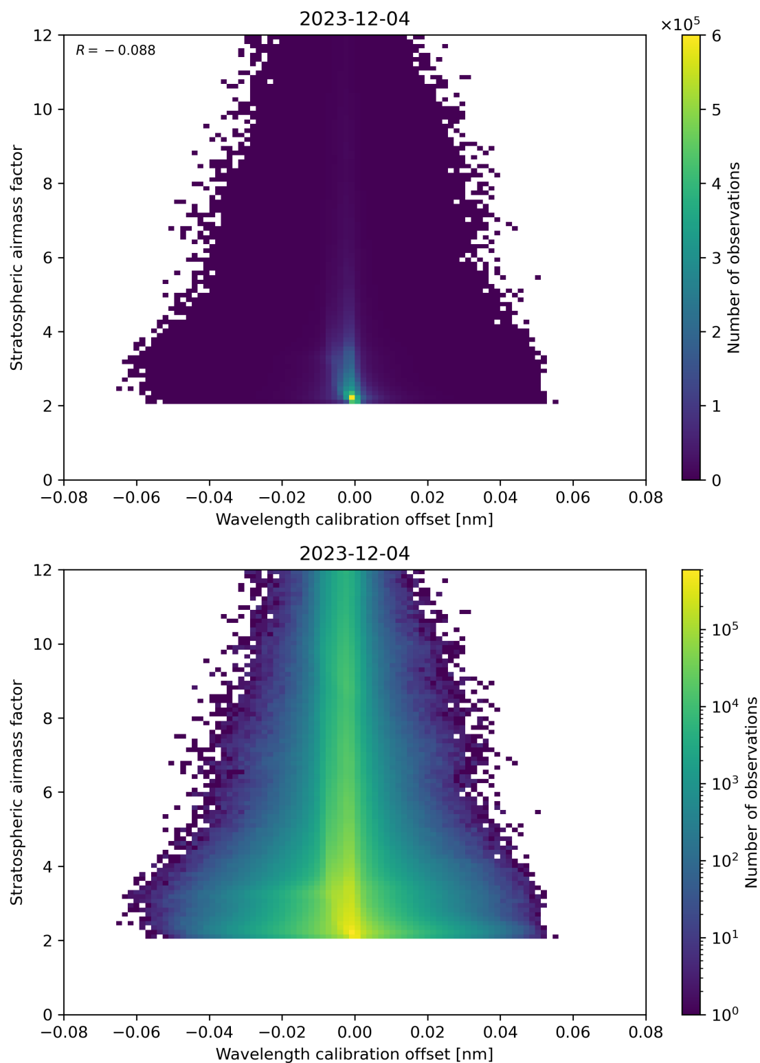
Figure 174: Scatter density plot of “Wavelength calibration offset” against “Stratospheric airmass factor” for 2023-12-04 to 2023-12-05.
