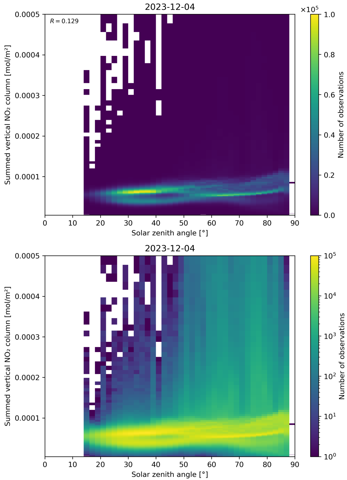
Figure 151: Scatter density plot of “Solar zenith angle” against “Summed vertical NO 2 column” for 2023-12-04 to 2023-12-05.
