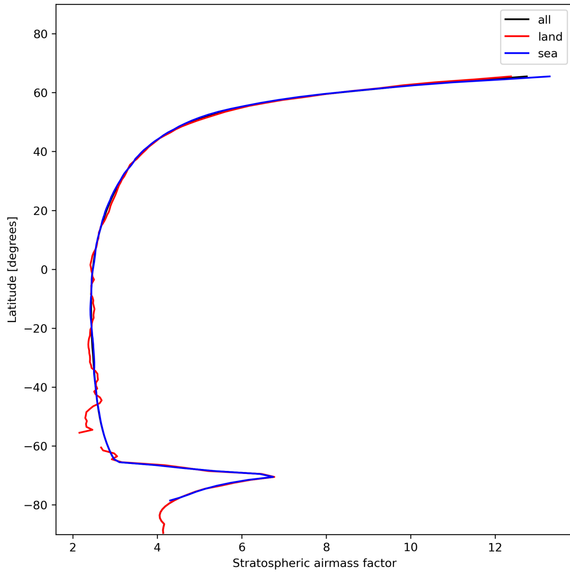
Figure 27: Zonal average of “Stratospheric air mass factor” for 2023-12-04 to 2023-12-05.
