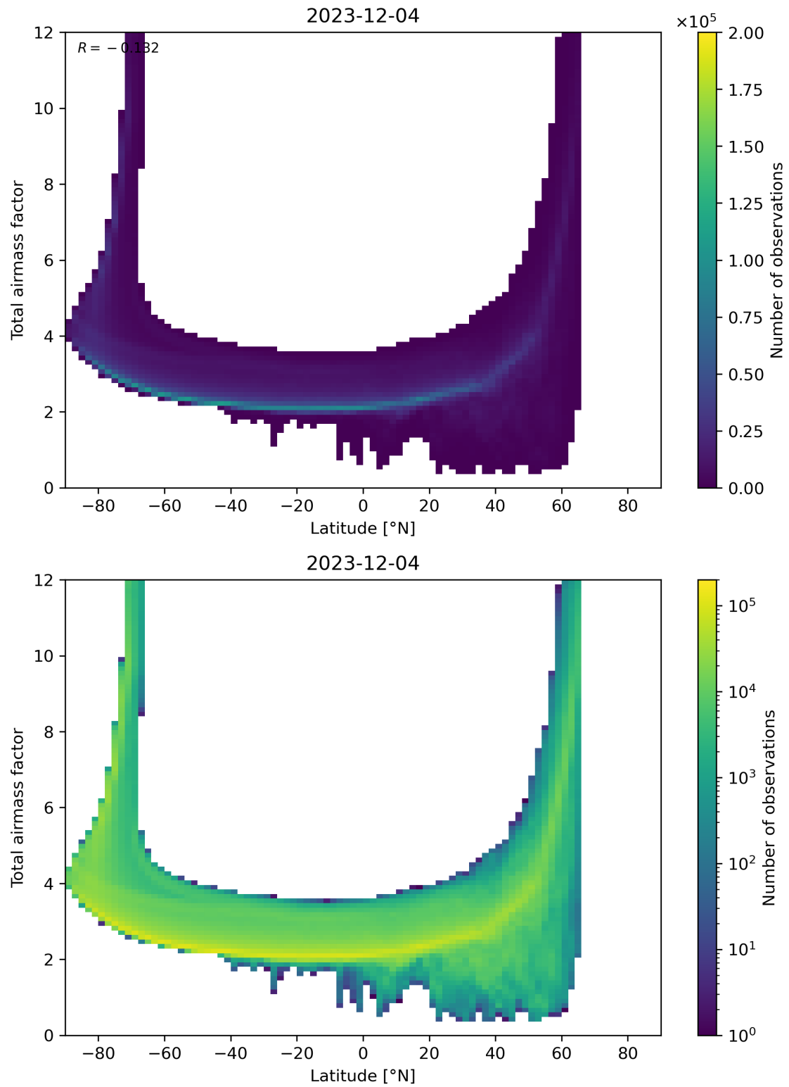
Figure 84: Scatter density plot of “Latitude” against “Total airmass factor” for 2023-12-04 to 2023-12-05.
