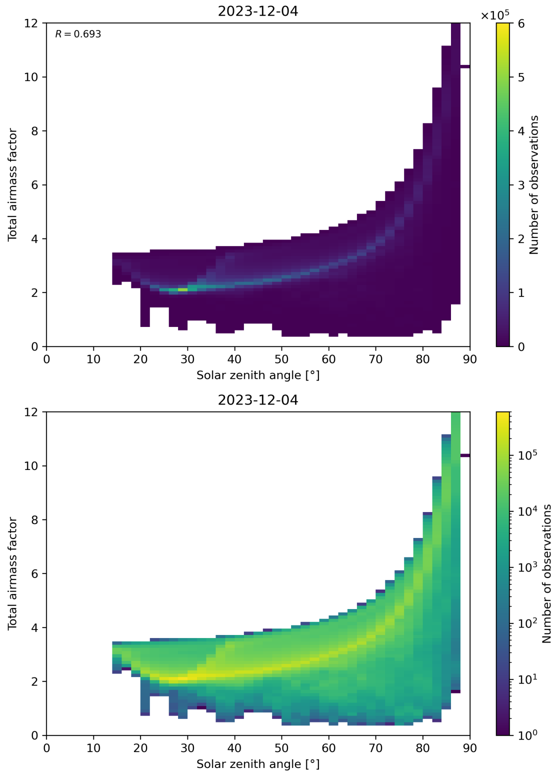
Figure 146: Scatter density plot of “Solar zenith angle” against “Total air mass factor” for 2023-12-04 to 2023-12-05.
