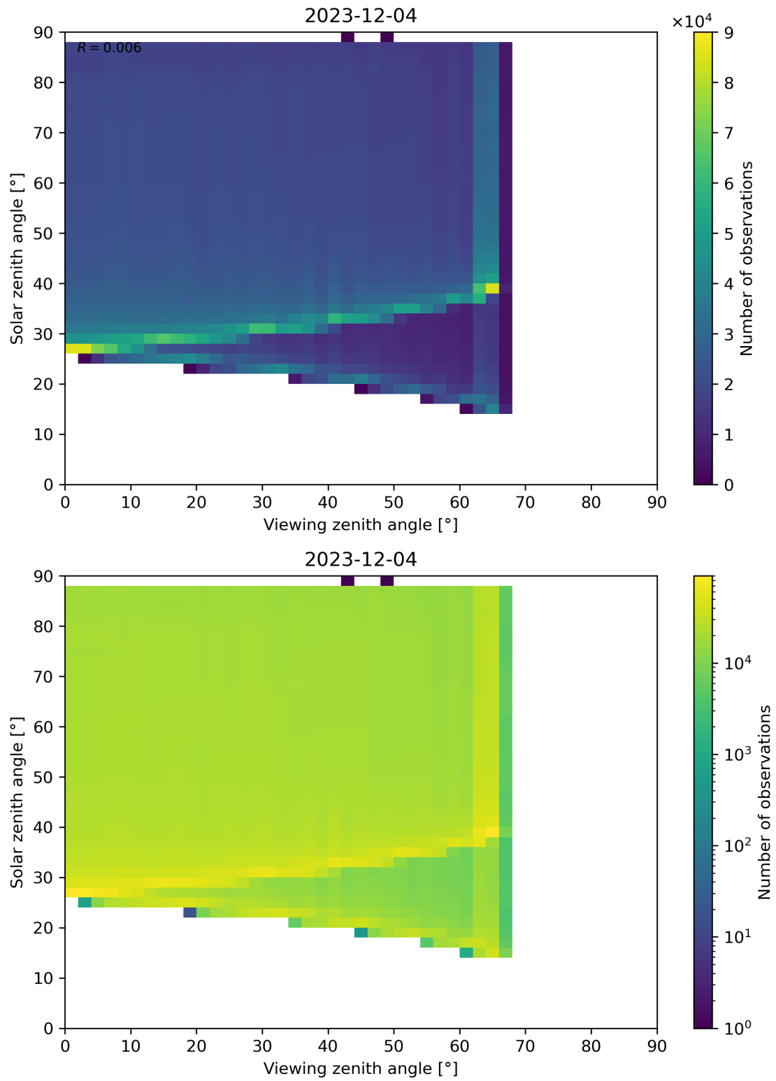
Figure 172: Scatter density plot of “Viewing zenith angle” against “Solar zenith angle” for 2023-12-04 to 2023-12-05.
