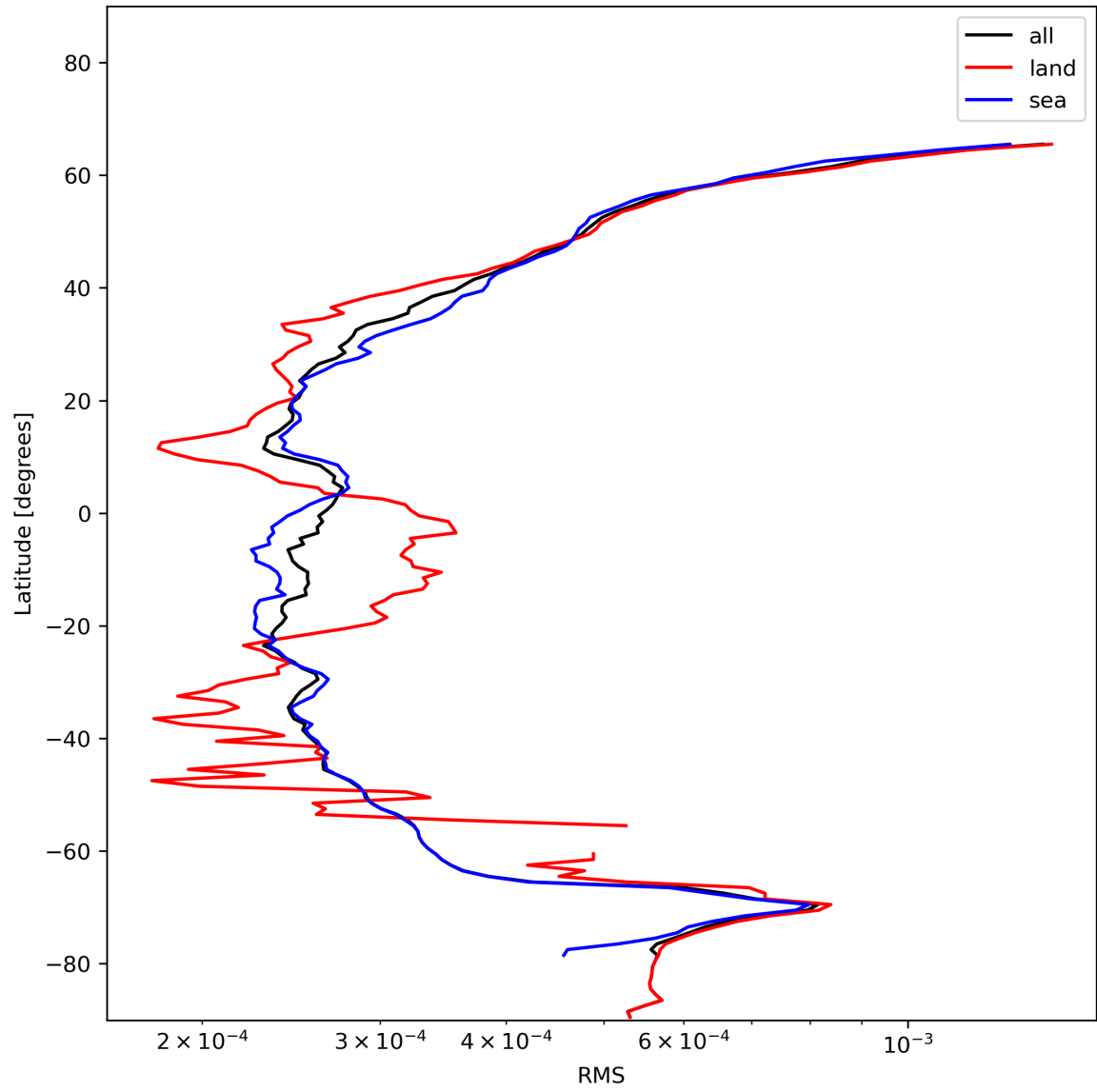
Figure 26: Zonal average of “RMS” for 2023-12-04 to 2023-12-05.
