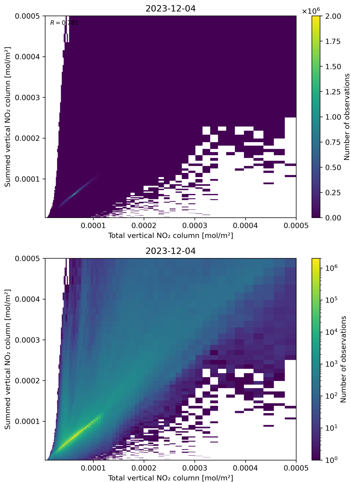
Figure 112: Scatter density plot of “Total vertical NO 2 column” against “Summed vertical NO 2 column” for 2023-12-04 to 2023-12-05.
