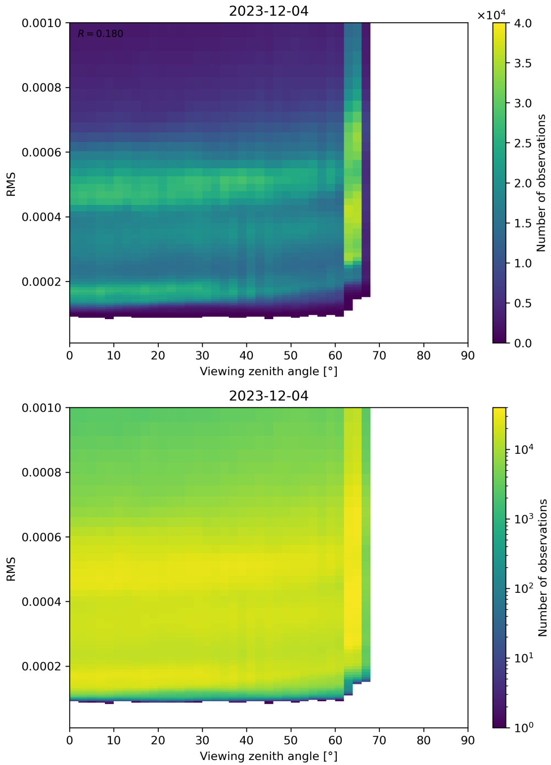
Figure 171: Scatter density plot of “Viewing zenith angle” against “RMS” for 2023-12-04 to 2023-12-05.
