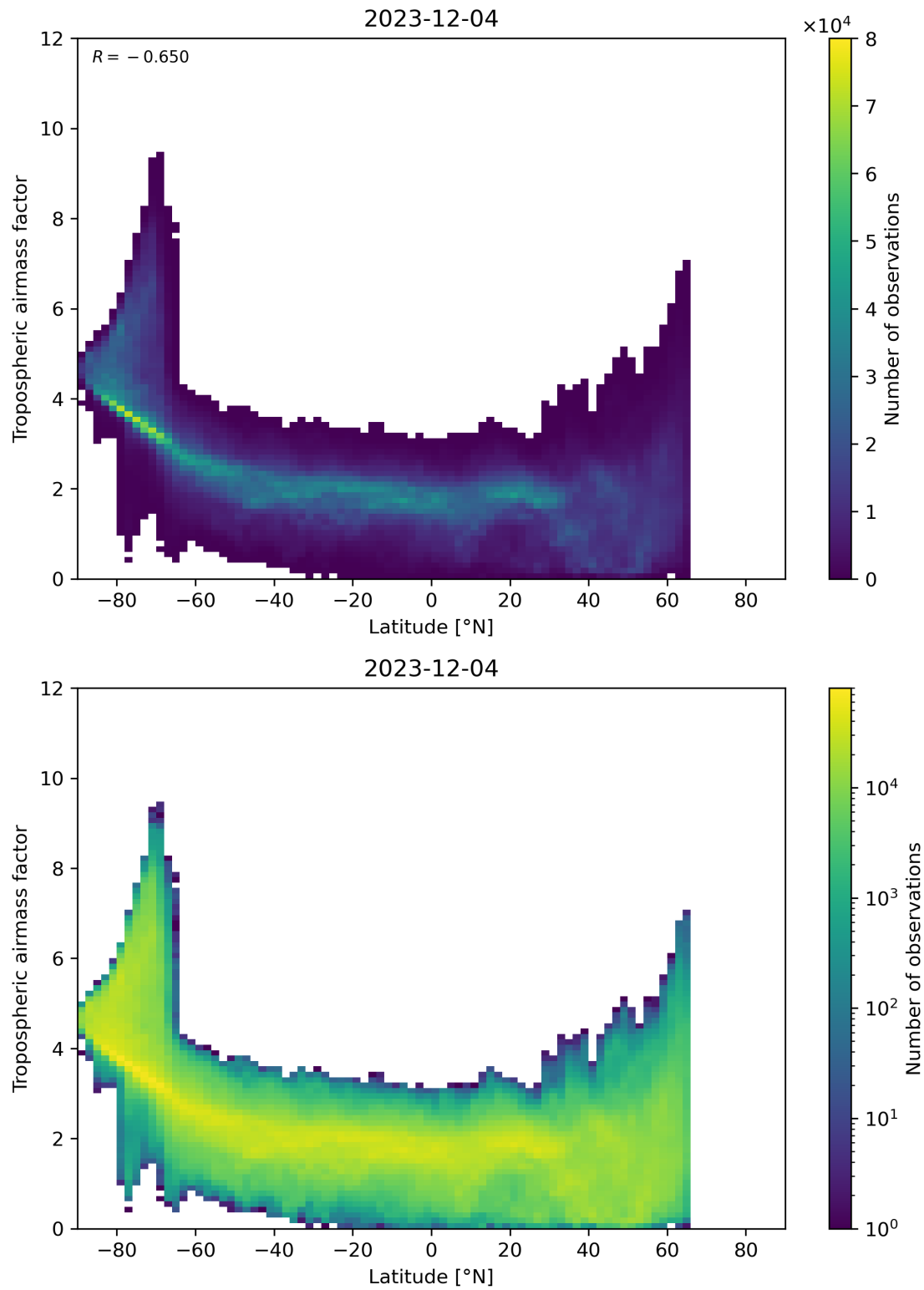
Figure 85: Scatter density plot of “Latitude” against “Tropospheric airmass factor” for 2023-12-04 to 2023-12-05.
