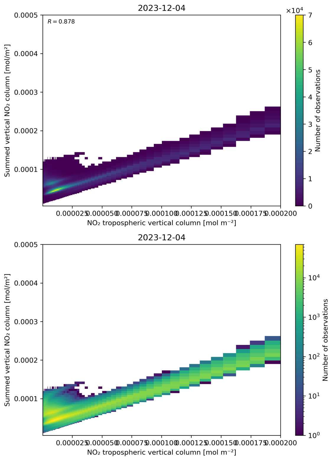
Figure 126: Scatter density plot of “NO 2 tropospheric vertical column” against “Summed vertical NO 2 column” for 2023-12-04 to 2023-12-05.
