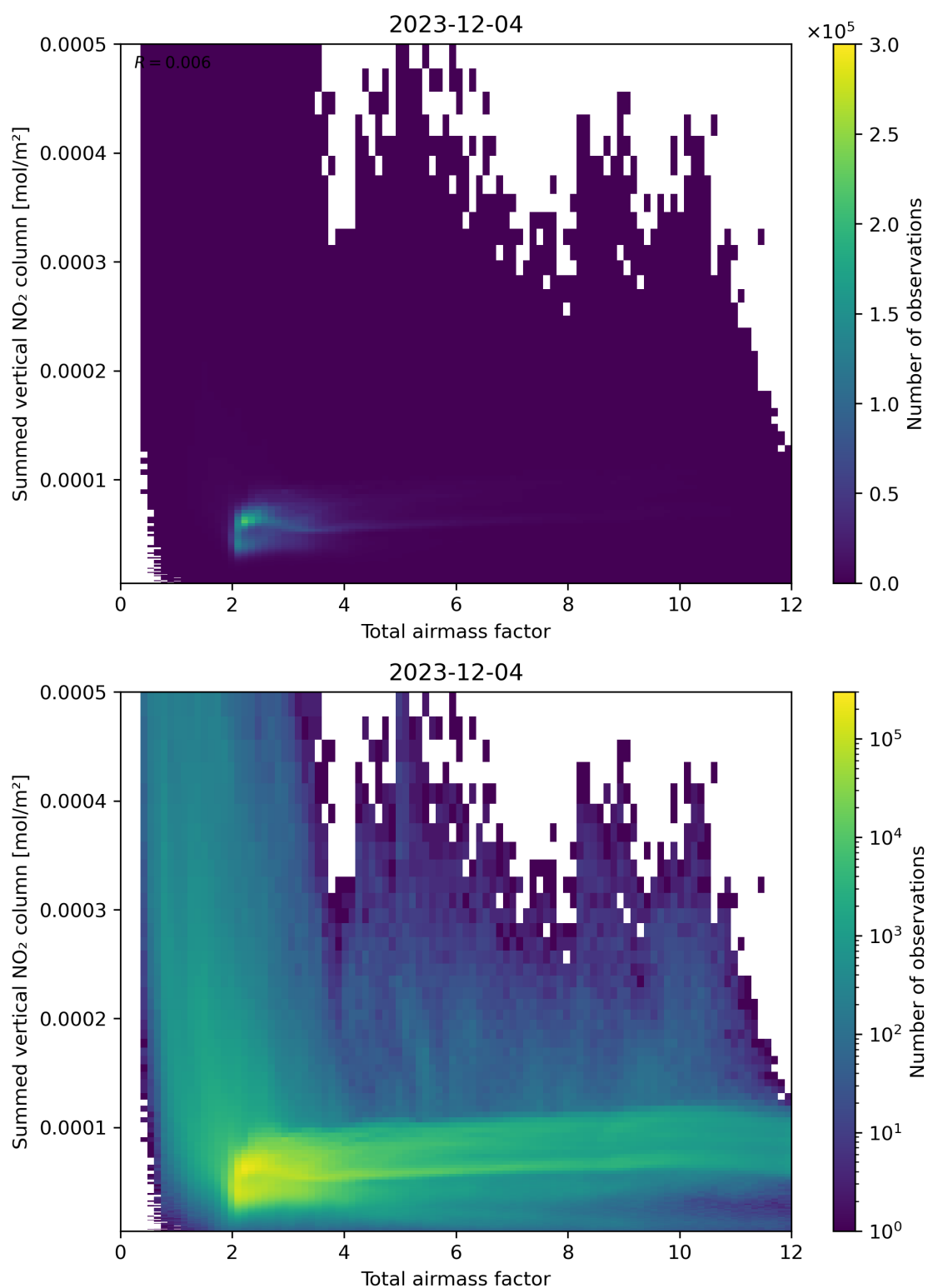
Figure 65: Scatter density plot of “Total air mass factor” against “Summed vertical NO 2 column” for 2023-12-04 to 2023-12-05.
