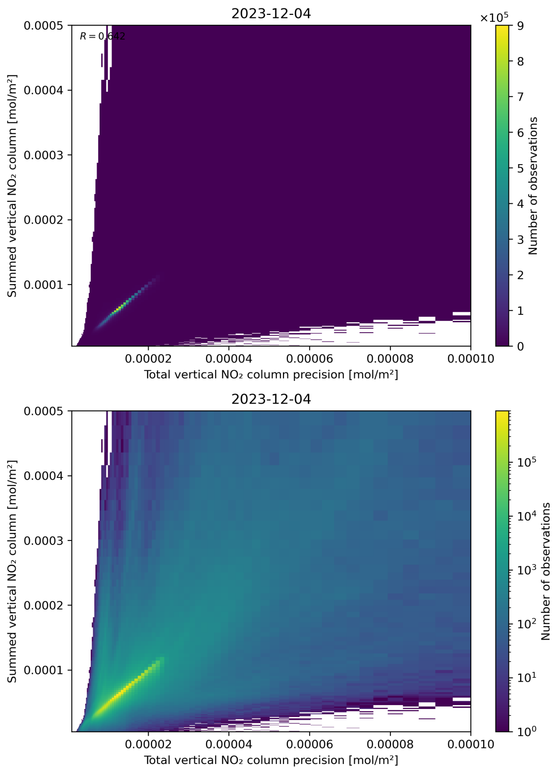
Figure 117: Scatter density plot of “Total vertical NO 2 column precision” against “Summed vertical NO 2 column” for 2023-12-04 to 2023-12-05.
