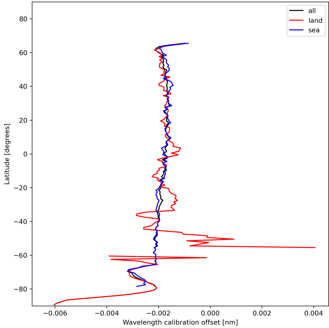
Figure 18: Zonal average of “Wavelength calibration offset” for 2023-12-04 to 2023-12-05.
