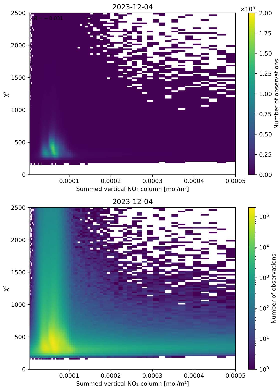
Figure 104: Scatter density plot of “Summed vertical NO 2 column” against “ \chi^2 ” for 2023-12-04 to 2023-12-05.
