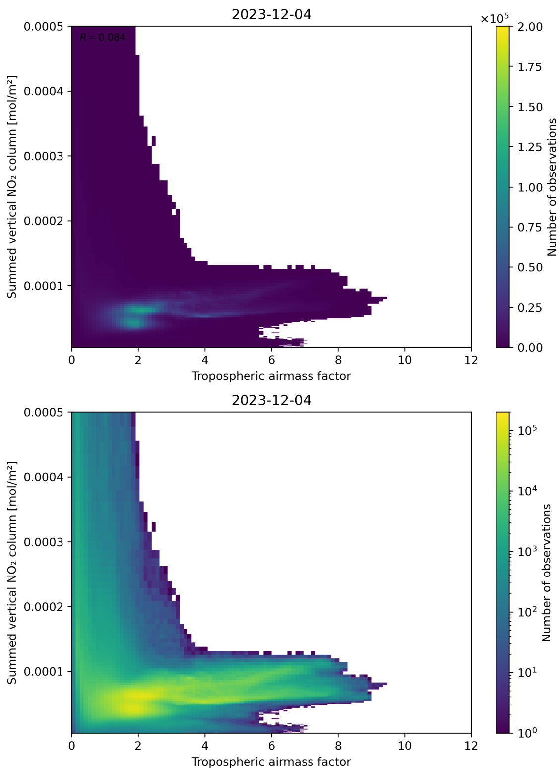
Figure 75: Scatter density plot of “Tropospheric airmass factor” against “Summed vertical NO 2 column” for 2023-12-04 to 2023-12-05.
