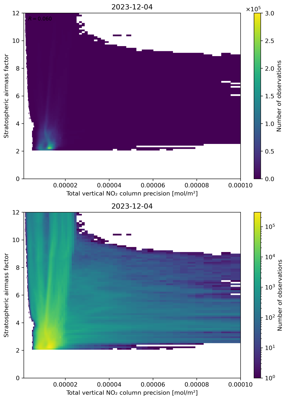
Figure 115: Scatter density plot of “Total vertical NO 2 column precision” against “Stratospheric air mass factor” for 2023-12-04 to 2023-12-05.
