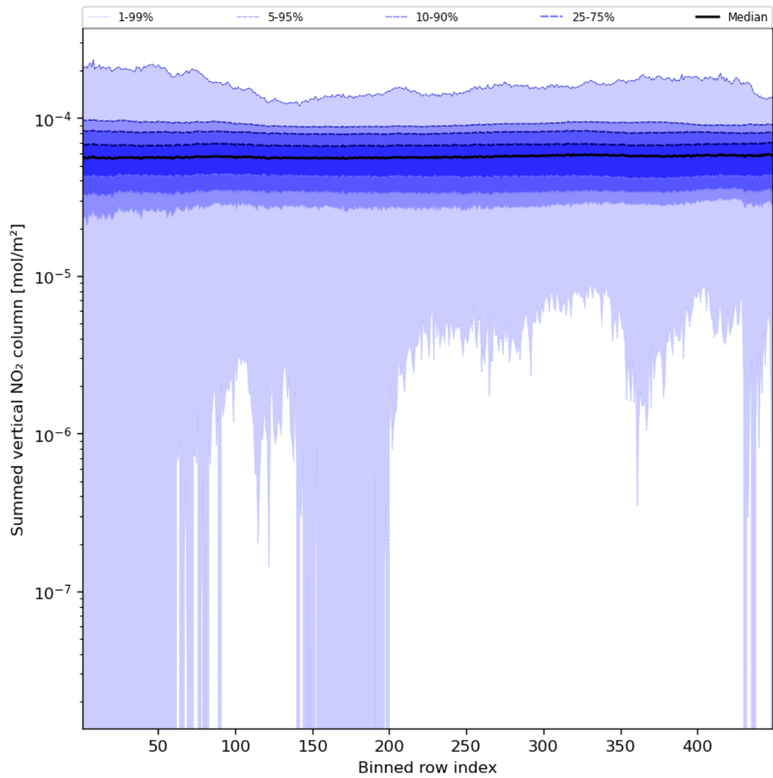
Figure 57: Along track statistics of “Summed vertical NO 2 column” for 2023-12-04 to 2023-12-05
