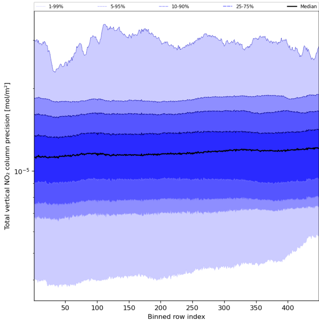
Figure 56: Along track statistics of “Total vertical NO 2 column precision” for 2023-12-04 to 2023-12-05
