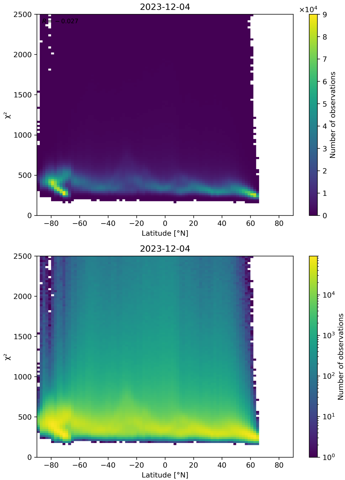
Figure 86: Scatter density plot of “Latitude” against “ \chi^2 ” for 2023-12-04 to 2023-12-05.
