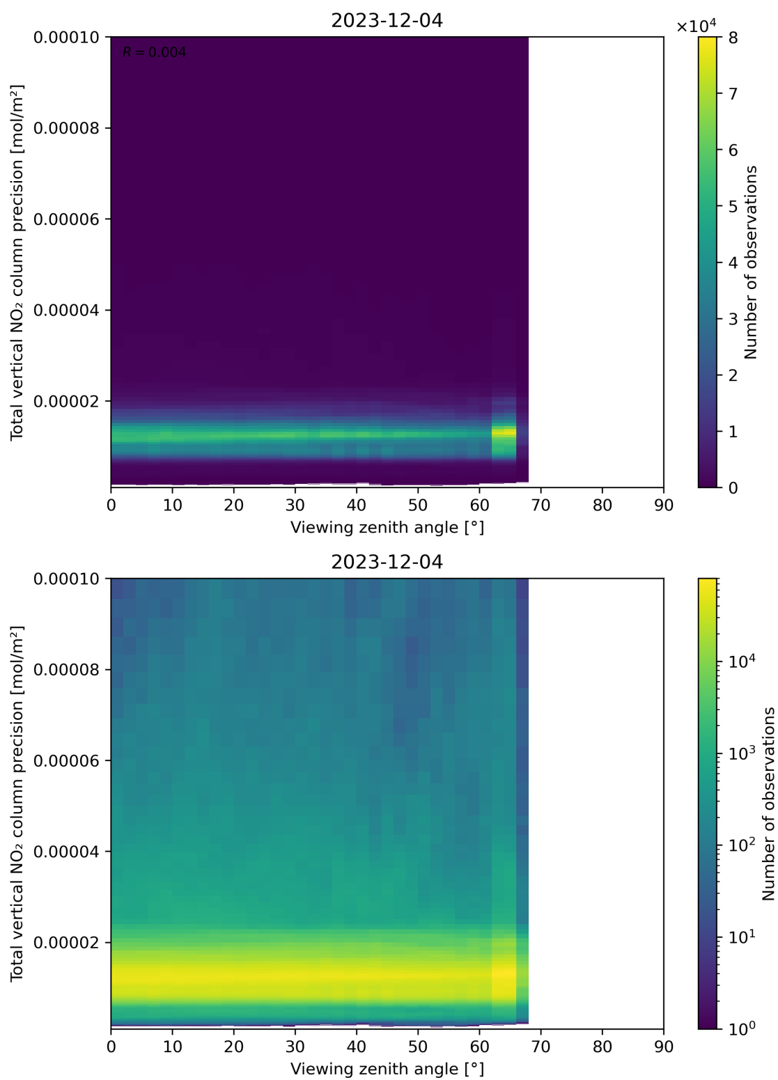
Figure 168: Scatter density plot of “Viewing zenith angle” against “Total vertical NO 2 column precision” for 2023-12-04 to 2023-12-05.
