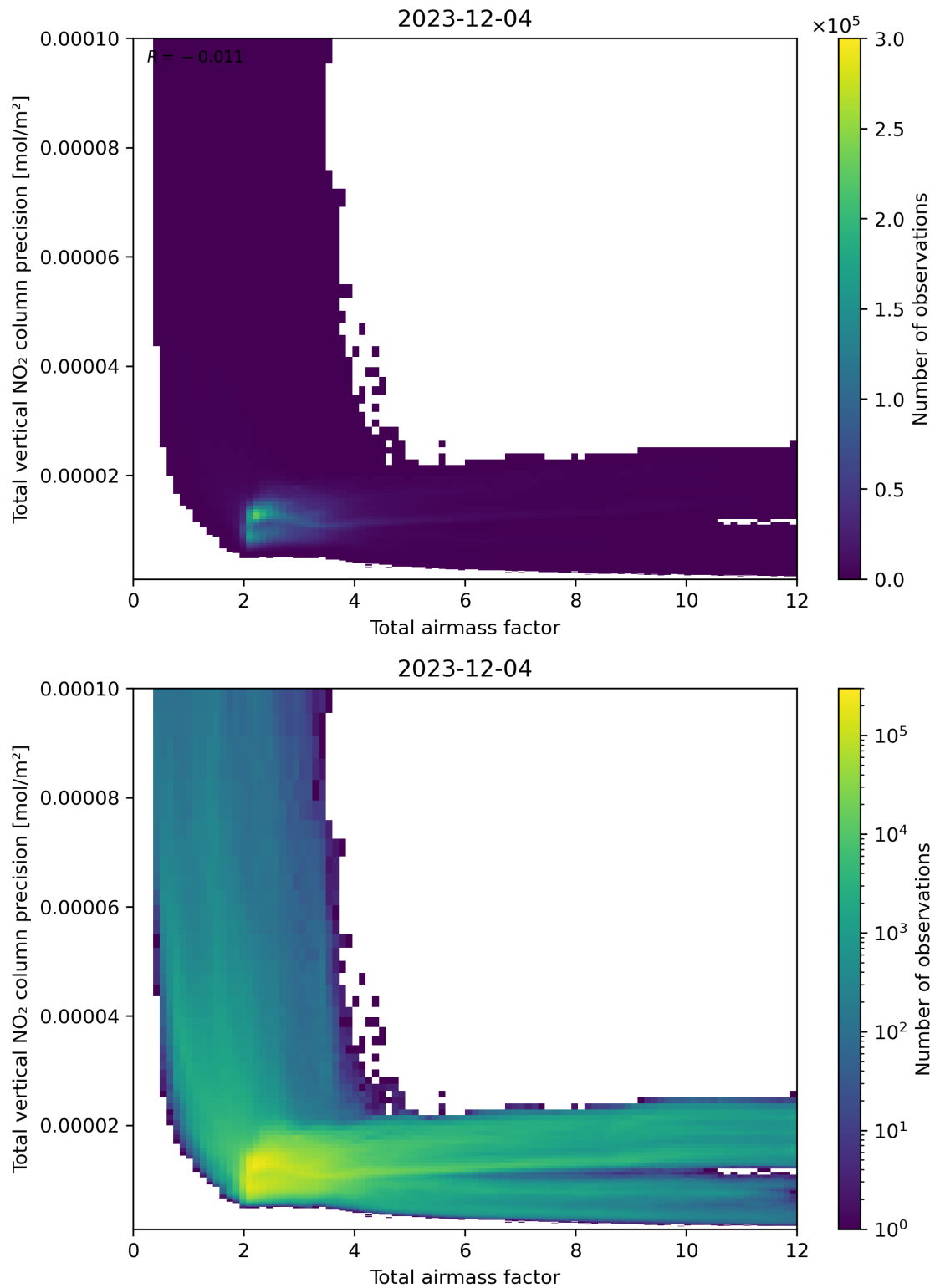
Figure 68: Scatter density plot of “Total airmass factor” against “Total vertical NO 2 column precision” for 2023-12-04 to 2023-12-05.
