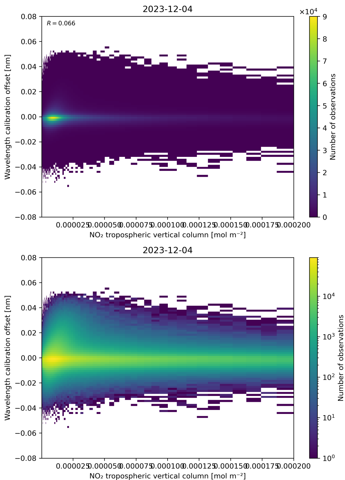
Figure 143: Scatter density plot of “NO 2 tropospheric vertical column” against “Wavelength calibration offset” for 2023-12-04 to 2023-12-05.
