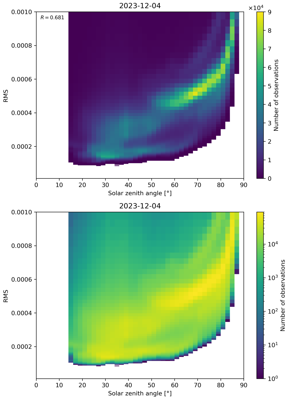
Figure 157: Scatter density plot of “Solar zenith angle” against “RMS” for 2023-12-04 to 2023-12-05.
