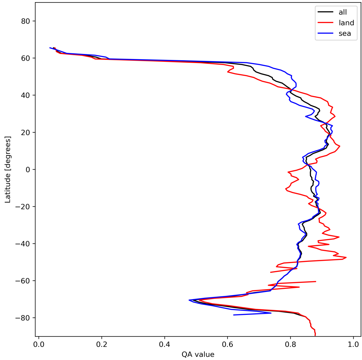
Figure 11: Zonal average of “QA value” for 2023-12-04 to 2023-12-05.
