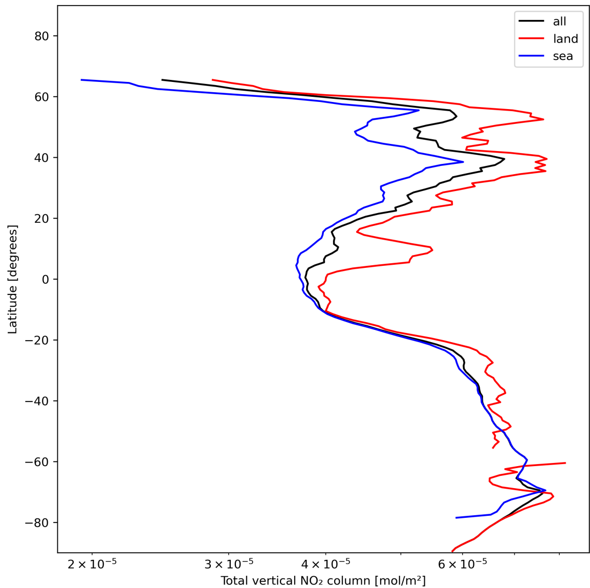
Figure 21: Zonal average of “Total vertical NO 2 column” for 2023-12-04 to 2023-12-05.
