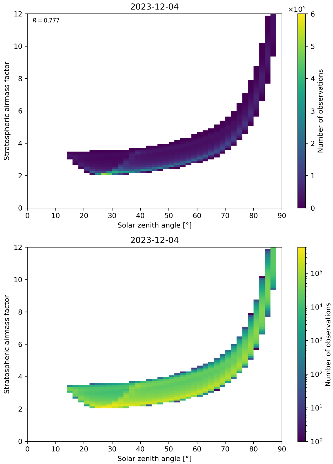
Figure 145: Scatter density plot of “Solar zenith angle” against “Stratospheric airmass factor” for 2023-12-04 to 2023-12-05.
