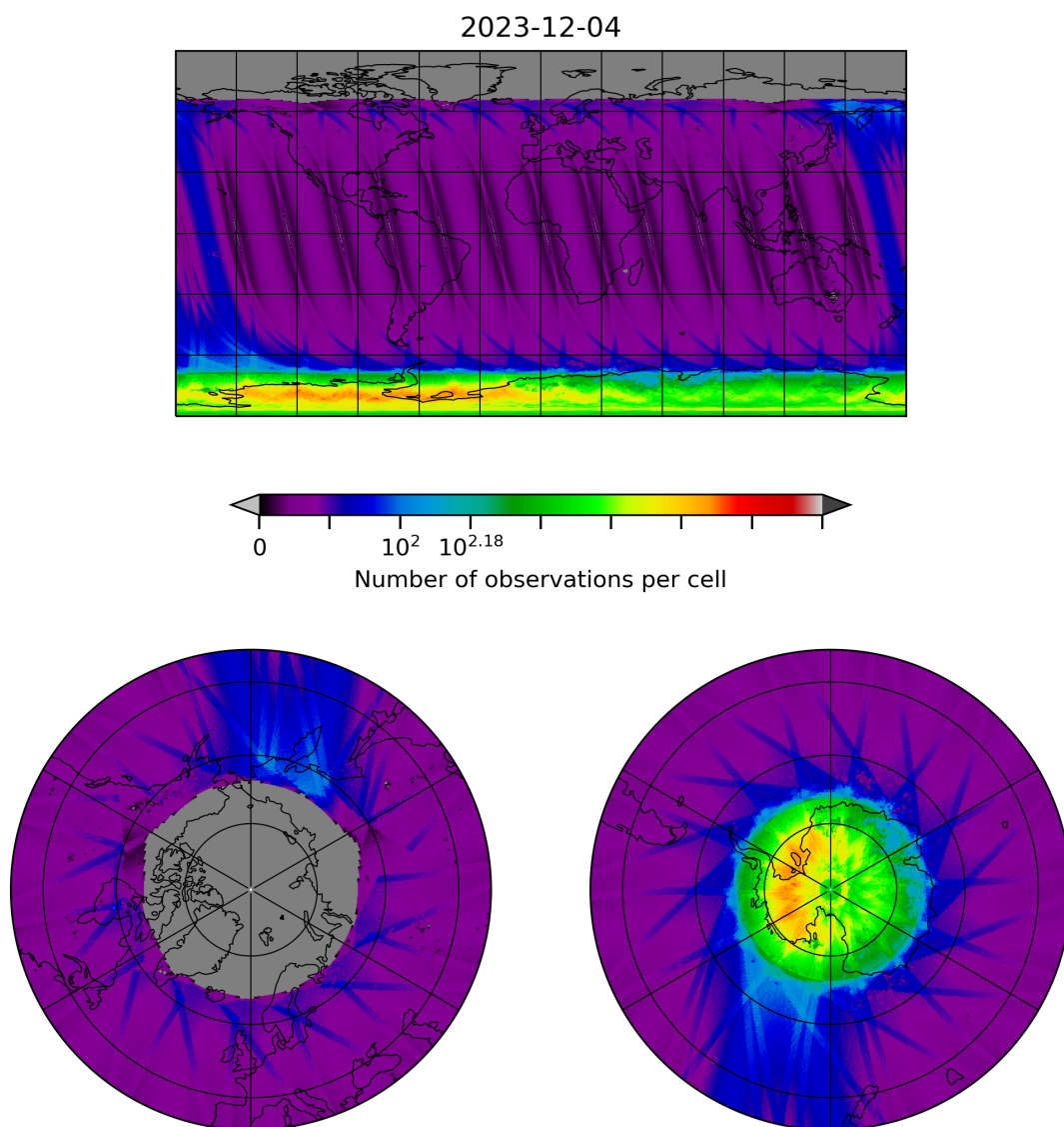
Figure 10: Map of the number of observations for 2023-12-04 to 2023-12-05
