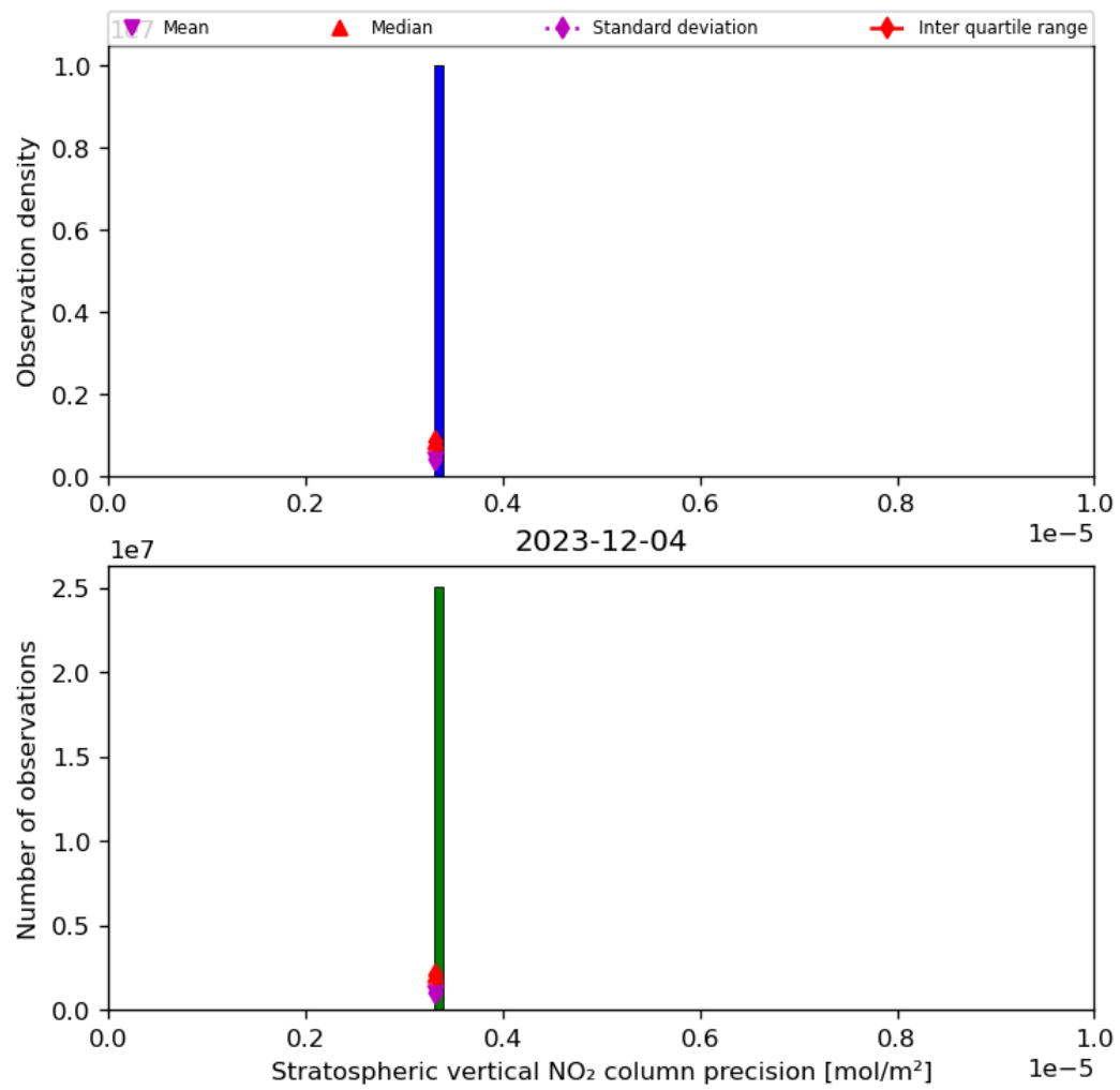
Figure 37: Histogram of “Stratospheric vertical NO 2 column precision” for 2023-12-04 to 2023-12-05
