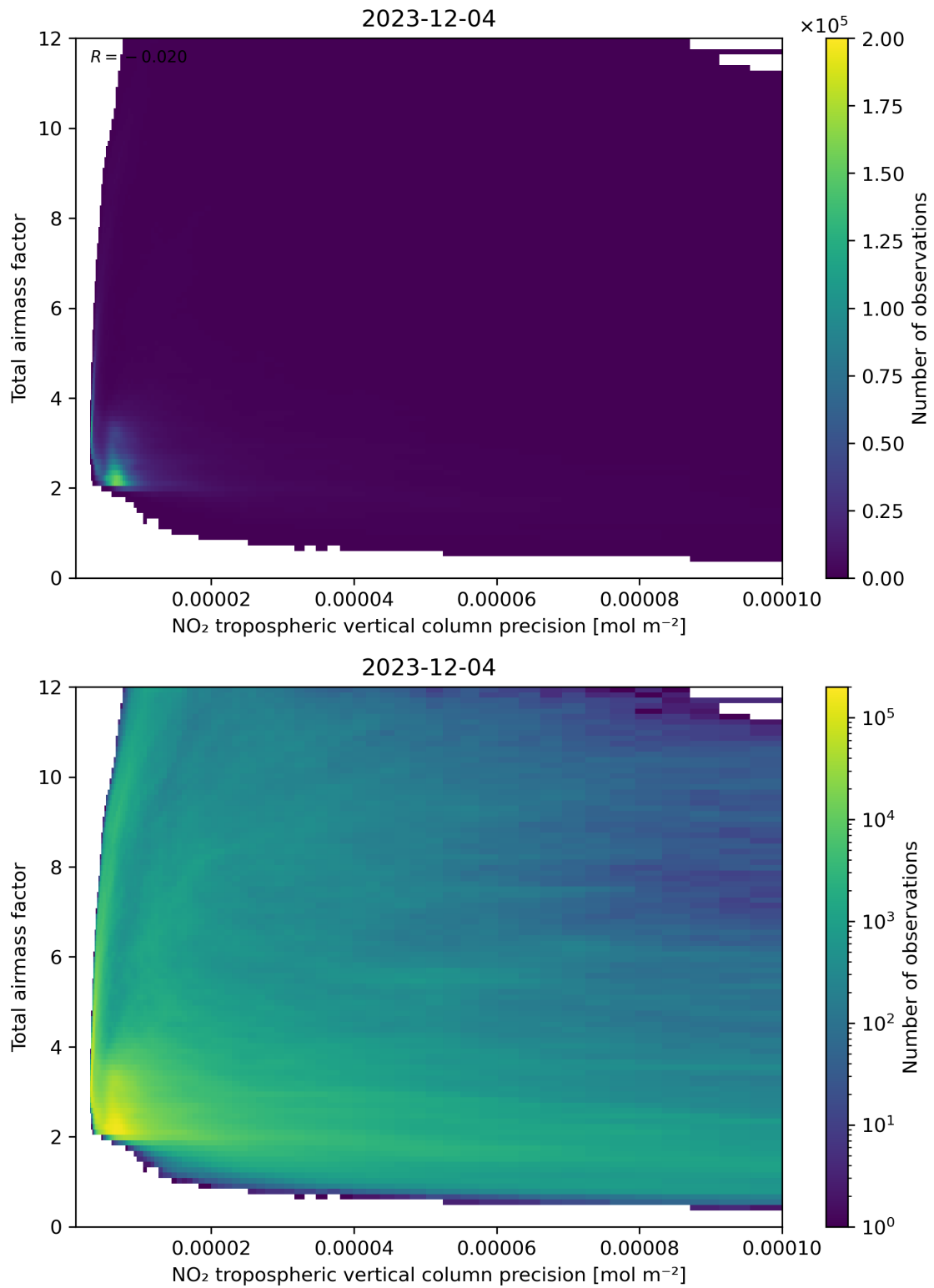
Figure 132: Scatter density plot of “NO 2 tropospheric vertical column precision” against “Total air mass factor” for 2023-12-04 to 2023-12-05.
