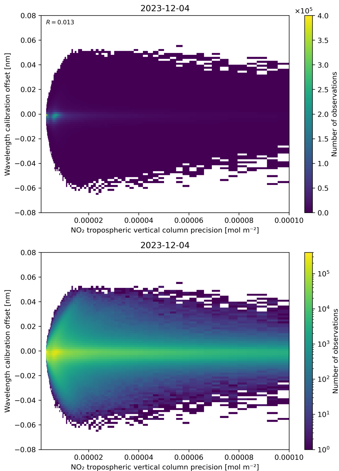
Figure 141: Scatter density plot of “NO 2 tropospheric vertical column precision” against “Wavelength calibration offset” for 2023-12-04 to 2023-12-05.
