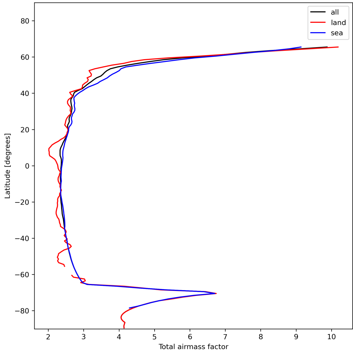
Figure 15: Zonal average of “Total airmass factor” for 2023-12-04 to 2023-12-05.
