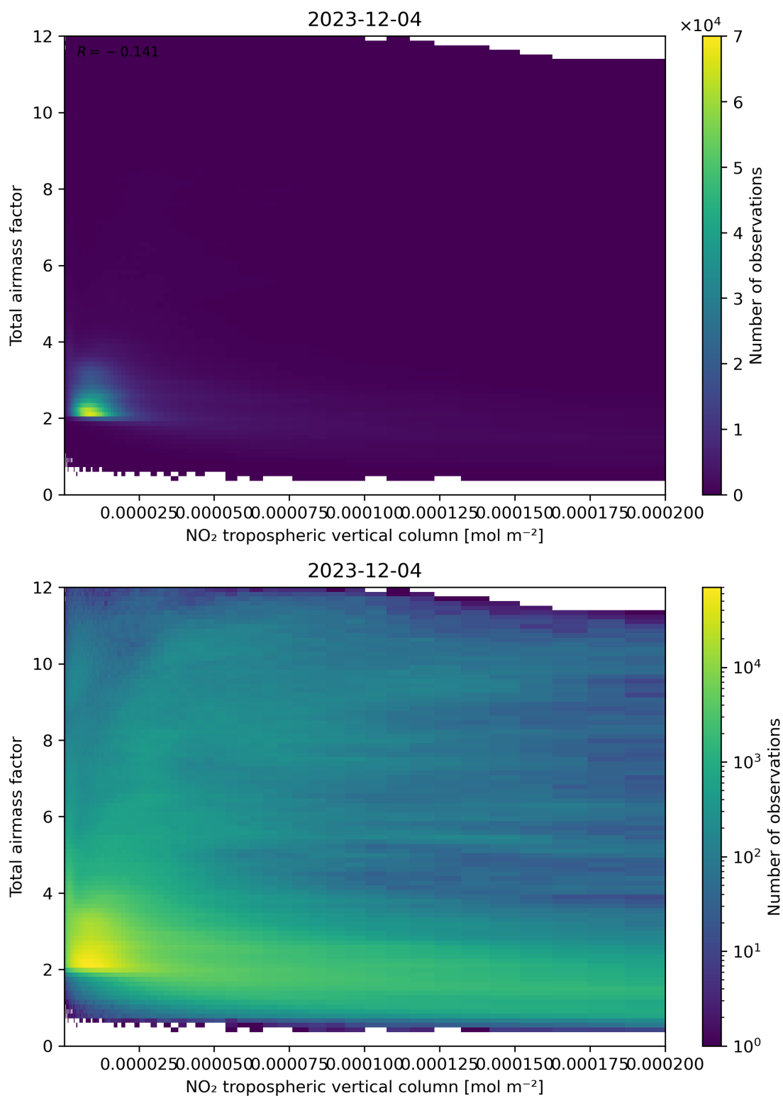
Figure 122: Scatter density plot of “NO 2 tropospheric vertical column” against “Total air mass factor” for 2023-12-04 to 2023-12-05.
