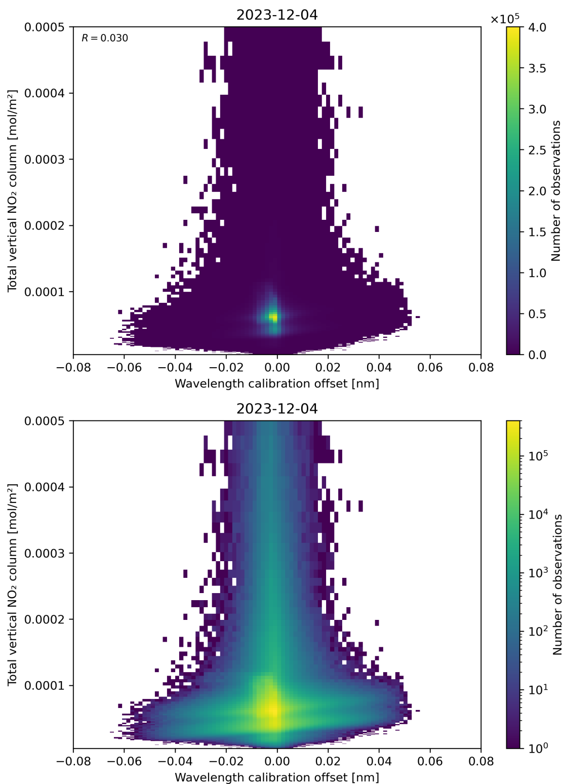
Figure 179: Scatter density plot of “Wavelength calibration offset” against “Total vertical NO 2 column” for 2023-12-04 to 2023-12-05.
