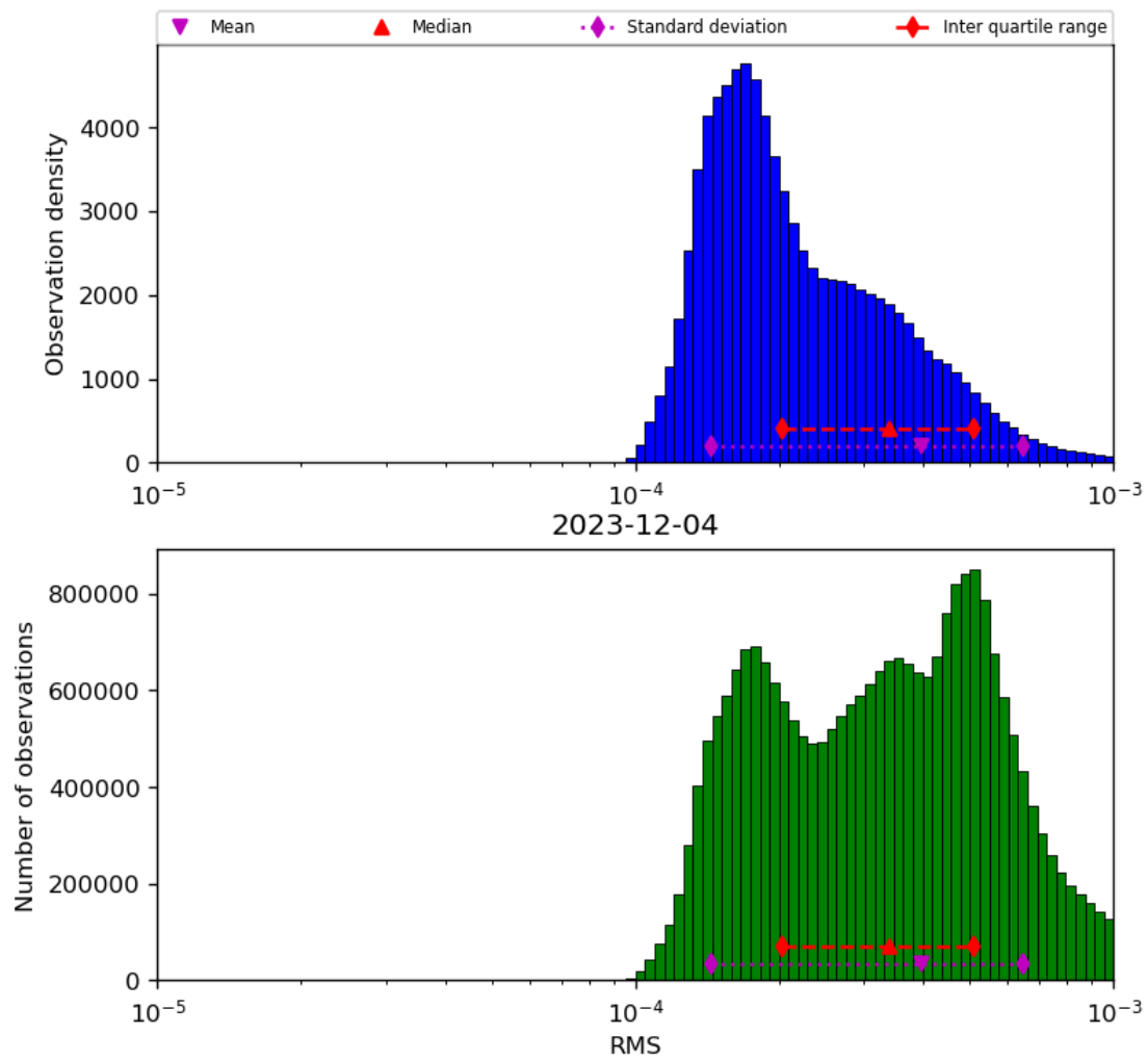
Figure 43: Histogram of “RMS” for 2023-12-04 to 2023-12-05
