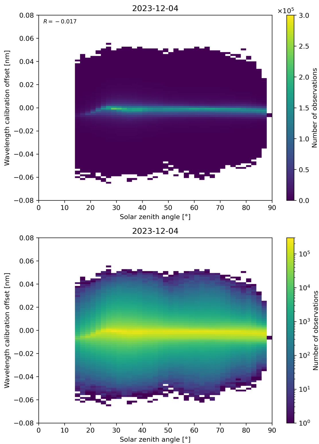
Figure 158: Scatter density plot of “Solar zenith angle” against “Wavelength calibration offset” for 2023-12-04 to 2023-12-05.
