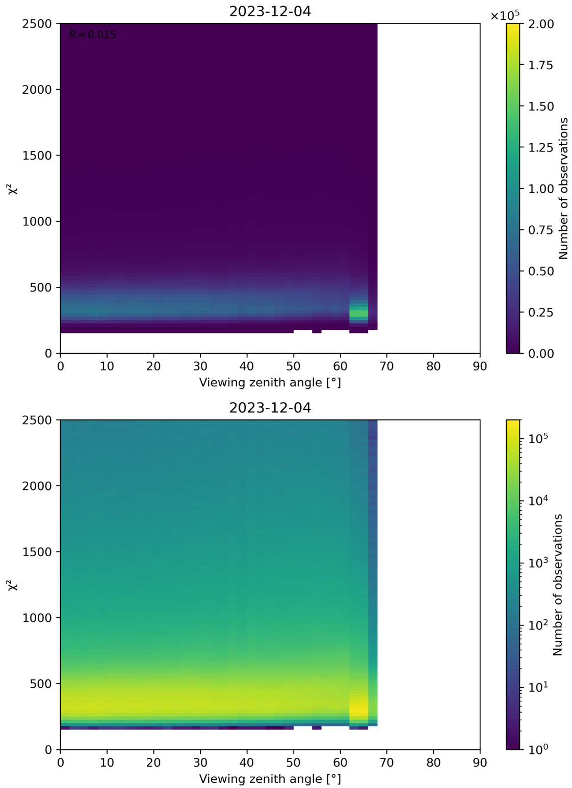
Figure 162: Scatter density plot of “Viewing zenith angle” against “ \chi^2 ” for 2023-12-04 to 2023-12-05.
