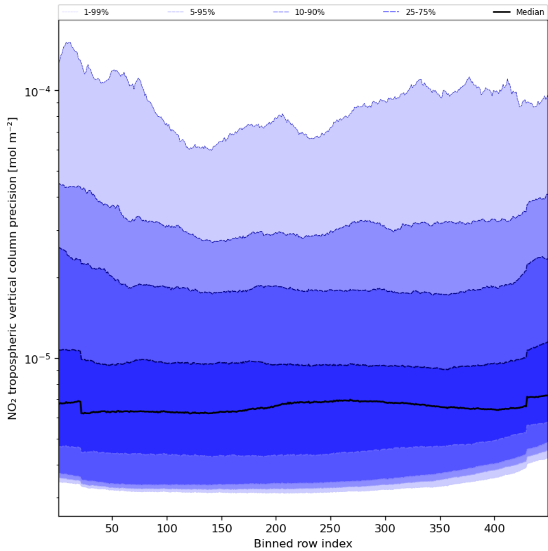
Figure 47: Along track statistics of “NO 2 tropospheric vertical column precision” for 2023-12-04 to 2023-12-05
