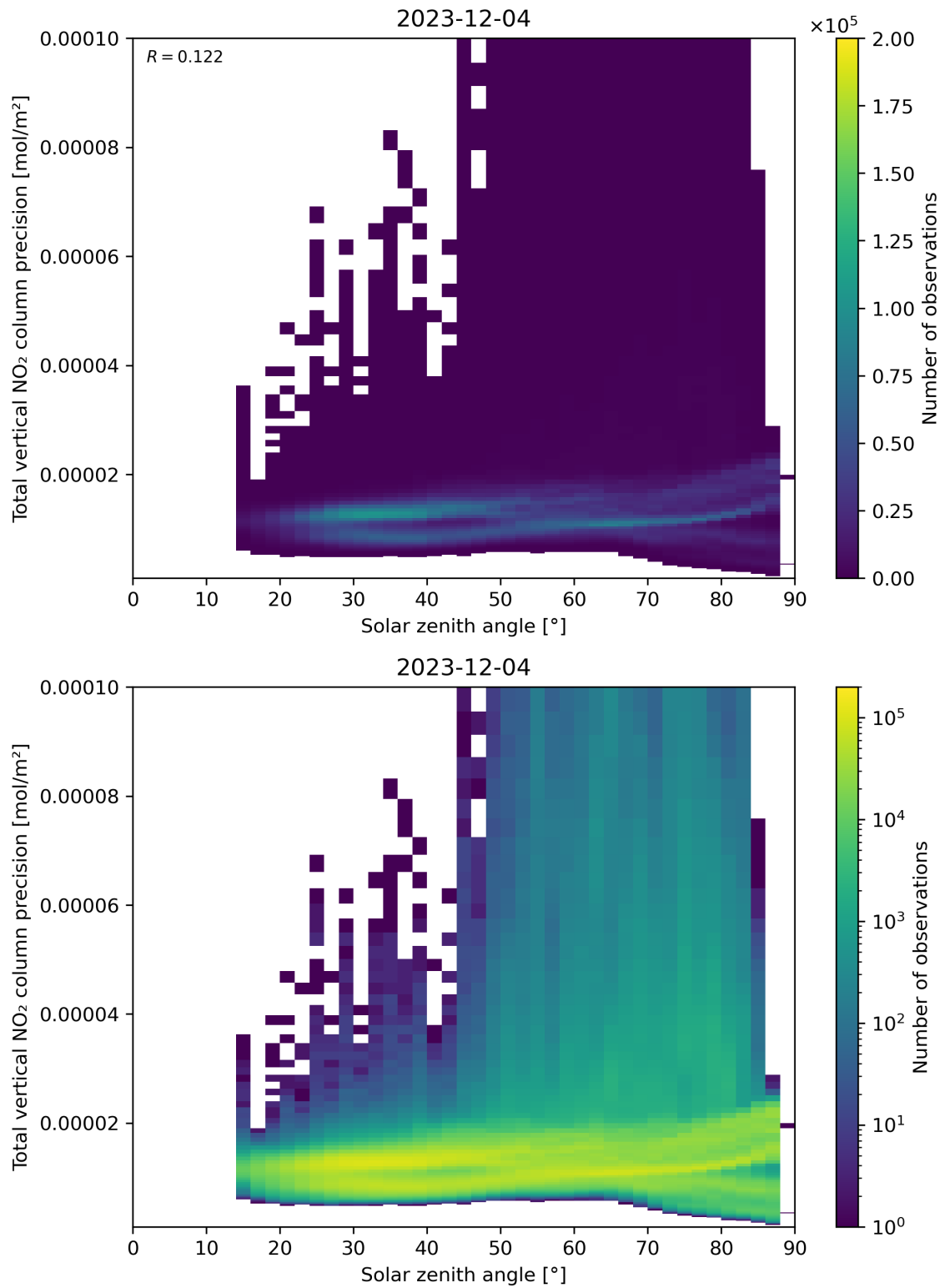
Figure 154: Scatter density plot of “Solar zenith angle” against “Total vertical NO 2 column precision” for 2023-12-04 to 2023-12-05.
