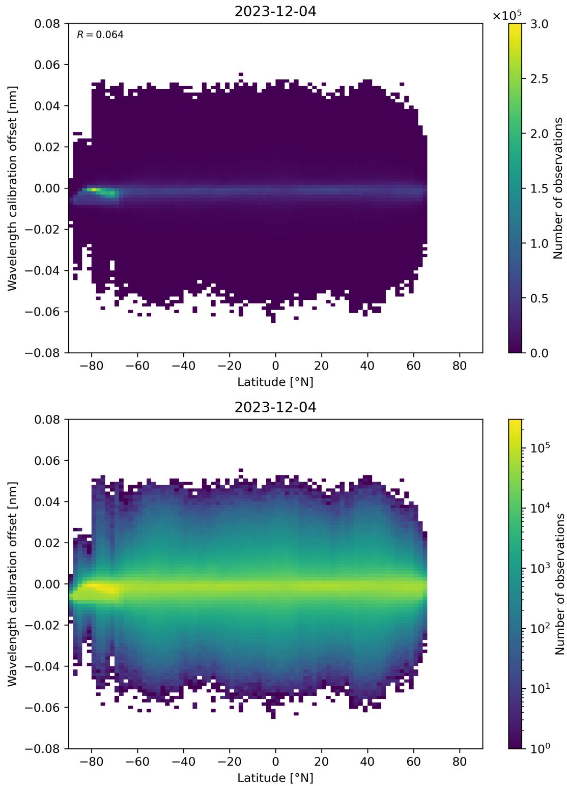
Figure 95: Scatter density plot of “Latitude” against “Wavelength calibration offset” for 2023-12-04 to 2023-12-05.
