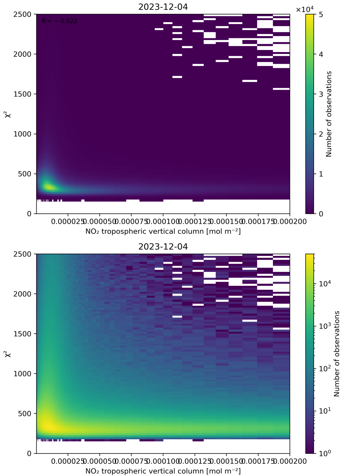
Figure 124: Scatter density plot of “NO 2 tropospheric vertical column” against “ \chi^2 ” for 2023-12-04 to 2023-12-05.
