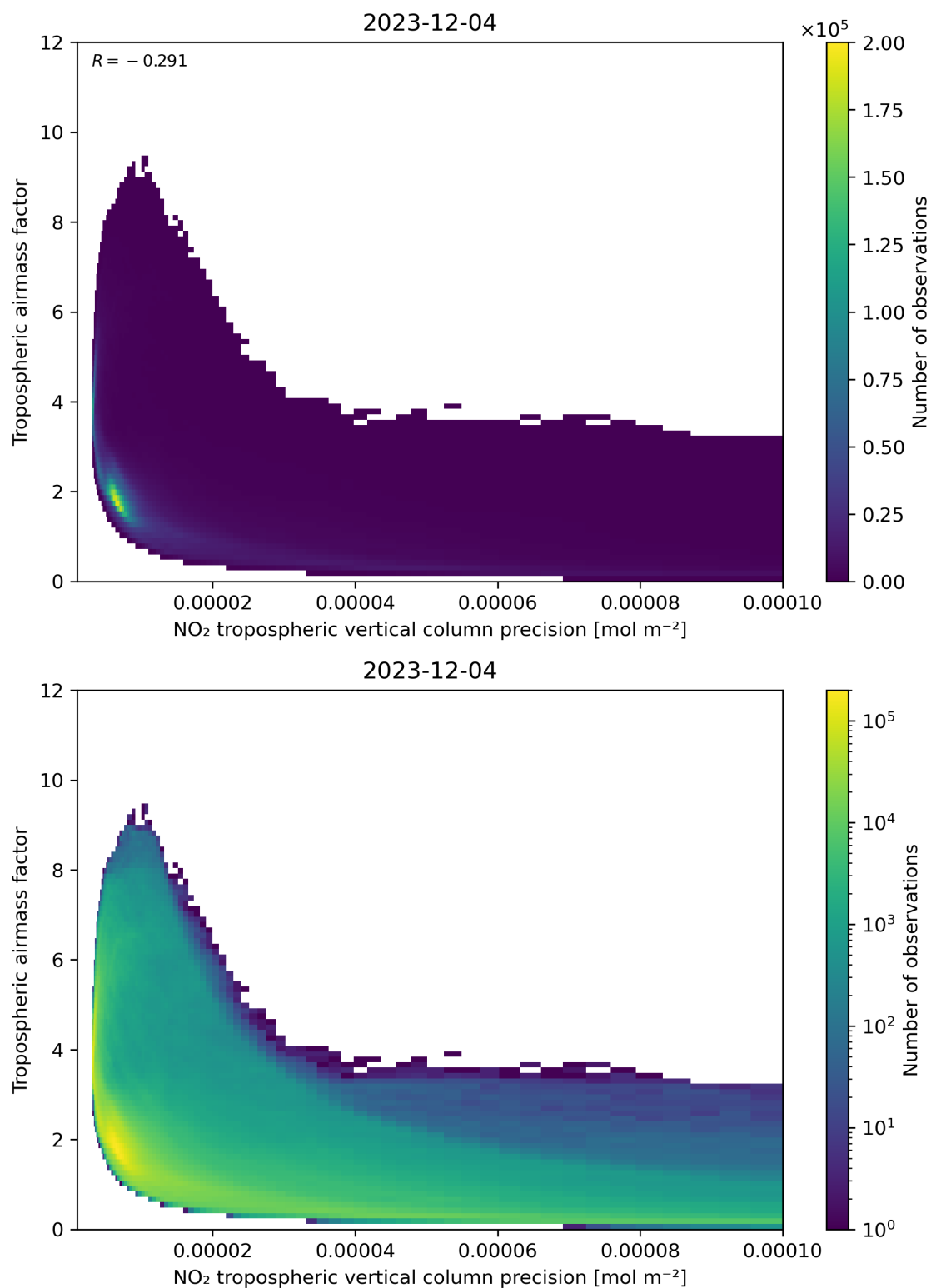
Figure 133: Scatter density plot of “NO 2 tropospheric vertical column precision” against “Tropospheric airmass factor” for 2023-12-04 to 2023-12-05.
