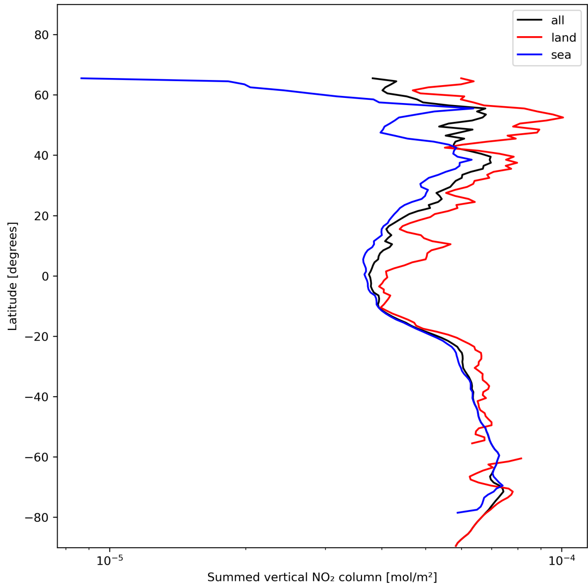
Figure 23: Zonal average of “Summed vertical NO 2 column” for 2023-12-04 to 2023-12-05.
