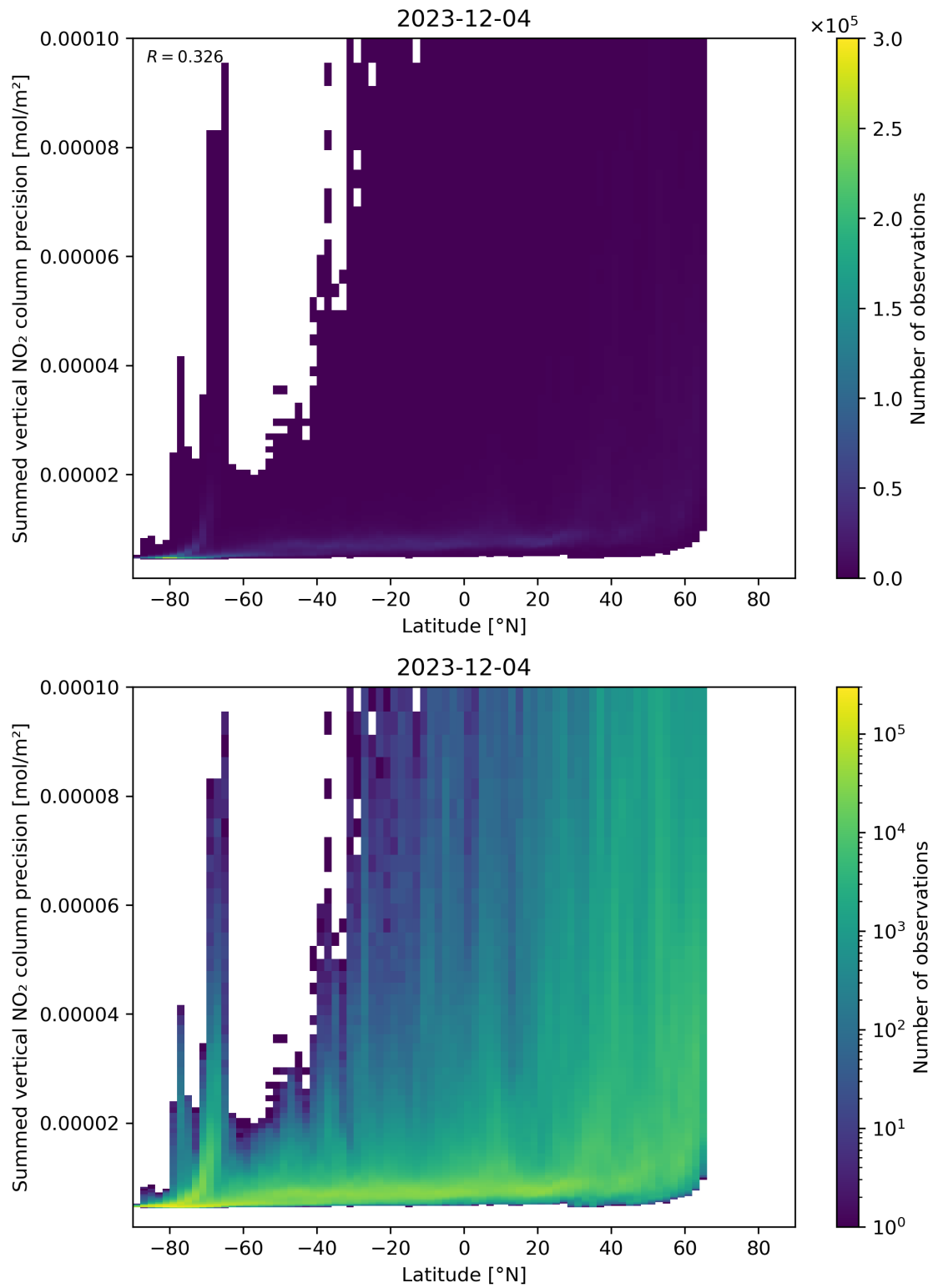
Figure 89: Scatter density plot of “Latitude” against “Summed vertical NO 2 column precision” for 2023-12-04 to 2023-12-05.
