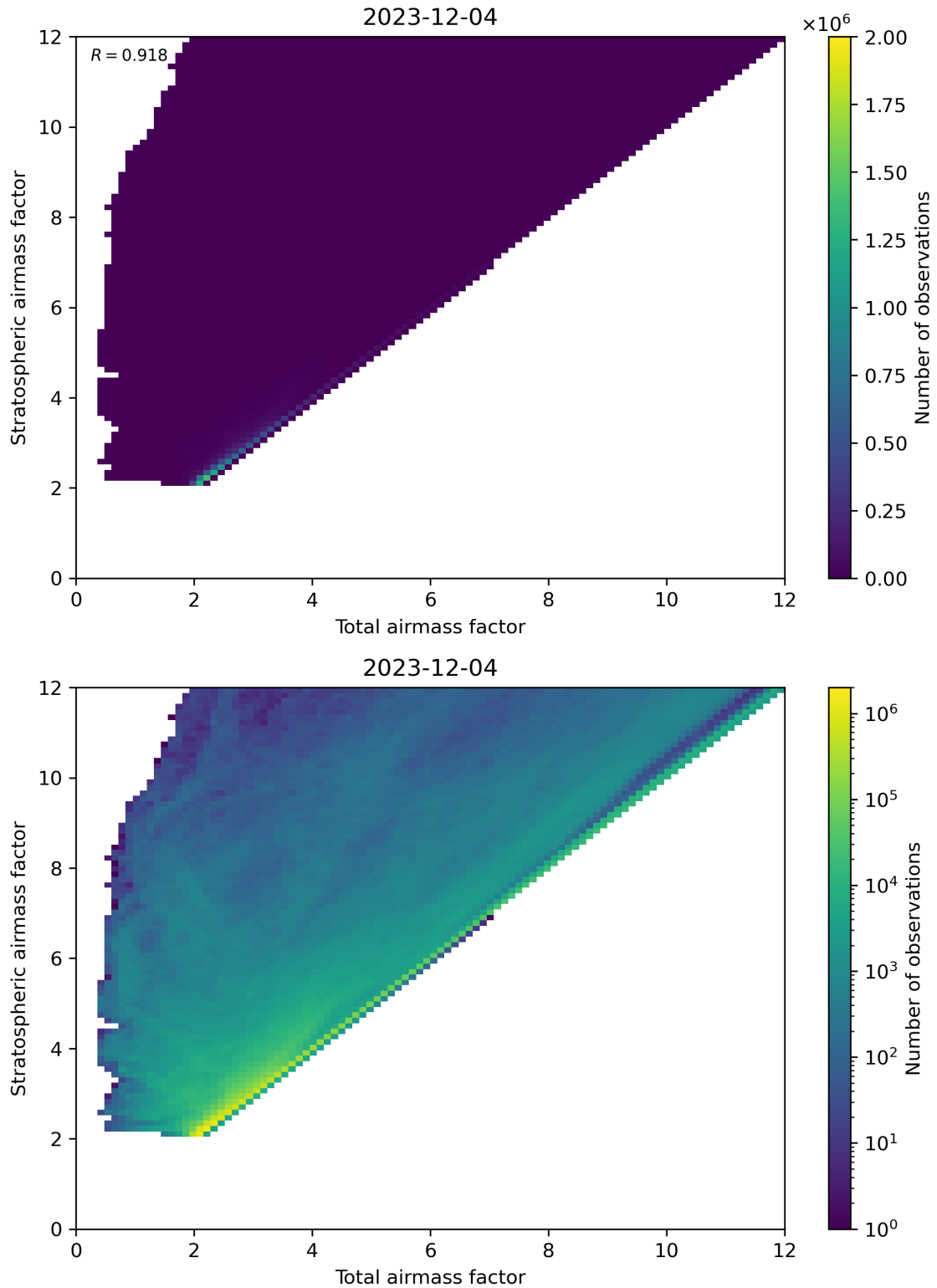
Figure 62: Scatter density plot of “Total airmass factor” against “Stratospheric airmass factor” for 2023-12-04 to 2023-12-05.
