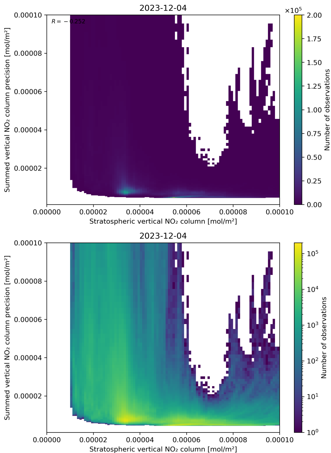
Figure 99: Scatter density plot of “Stratospheric vertical NO 2 column” against “Summed vertical NO 2 column precision” for 2023-12-04 to 2023-12-05.
