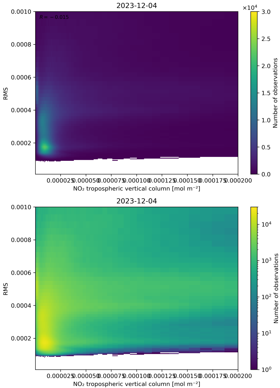
Figure 142: Scatter density plot of “NO 2 tropospheric vertical column” against “RMS” for 2023-12-04 to 2023-12-05.
