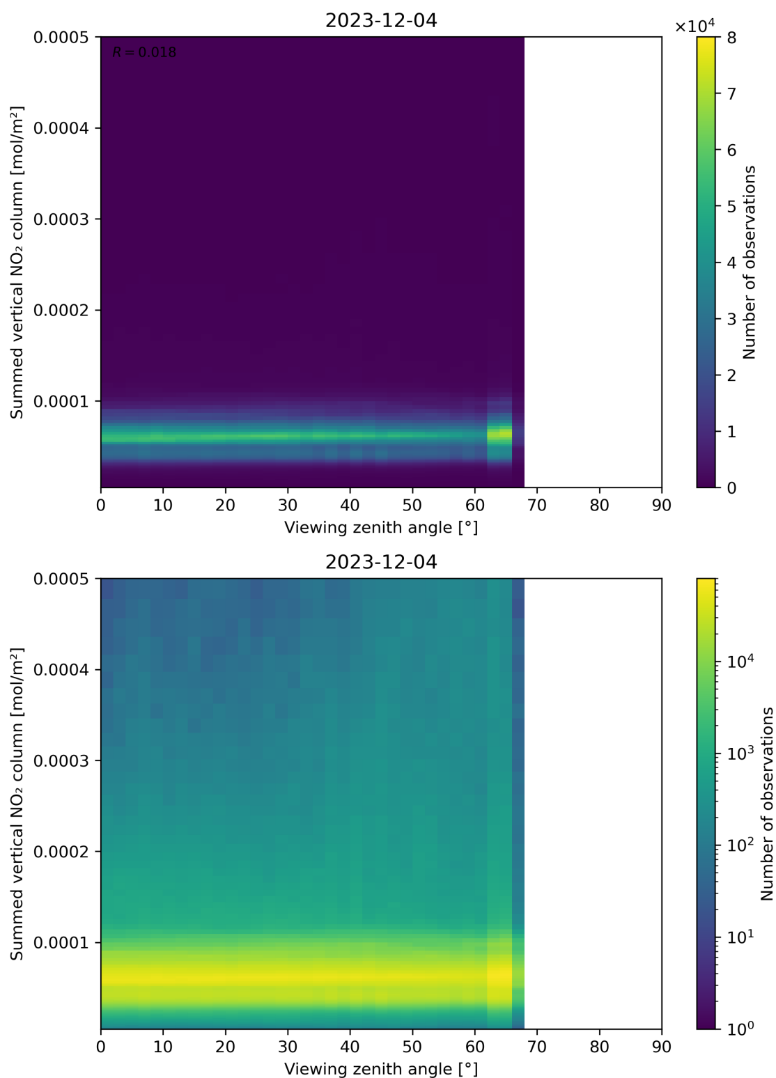
Figure 165: Scatter density plot of “Viewing zenith angle” against “Summed vertical NO 2 column” for 2023-12-04 to 2023-12-05.
