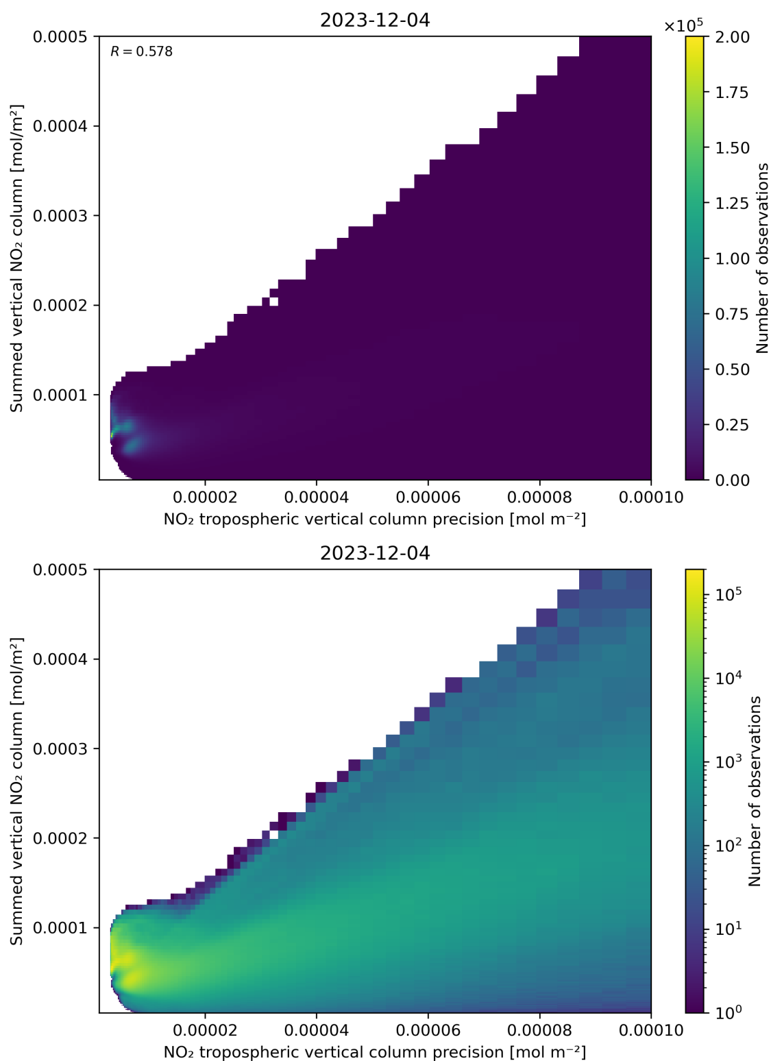
Figure 136: Scatter density plot of “NO 2 tropospheric vertical column precision” against “Summed vertical NO 2 column” for 2023-12-04 to 2023-12-05.
