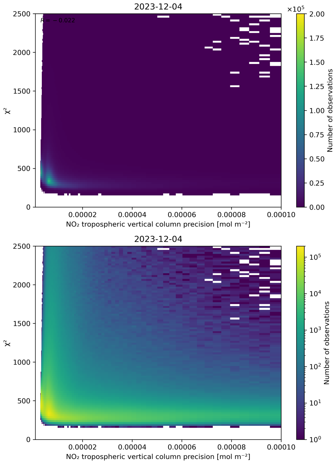
Figure 134: Scatter density plot of “NO 2 tropospheric vertical column precision” against “ \chi^2 ” for 2023-12-04 to 2023-12-05.
