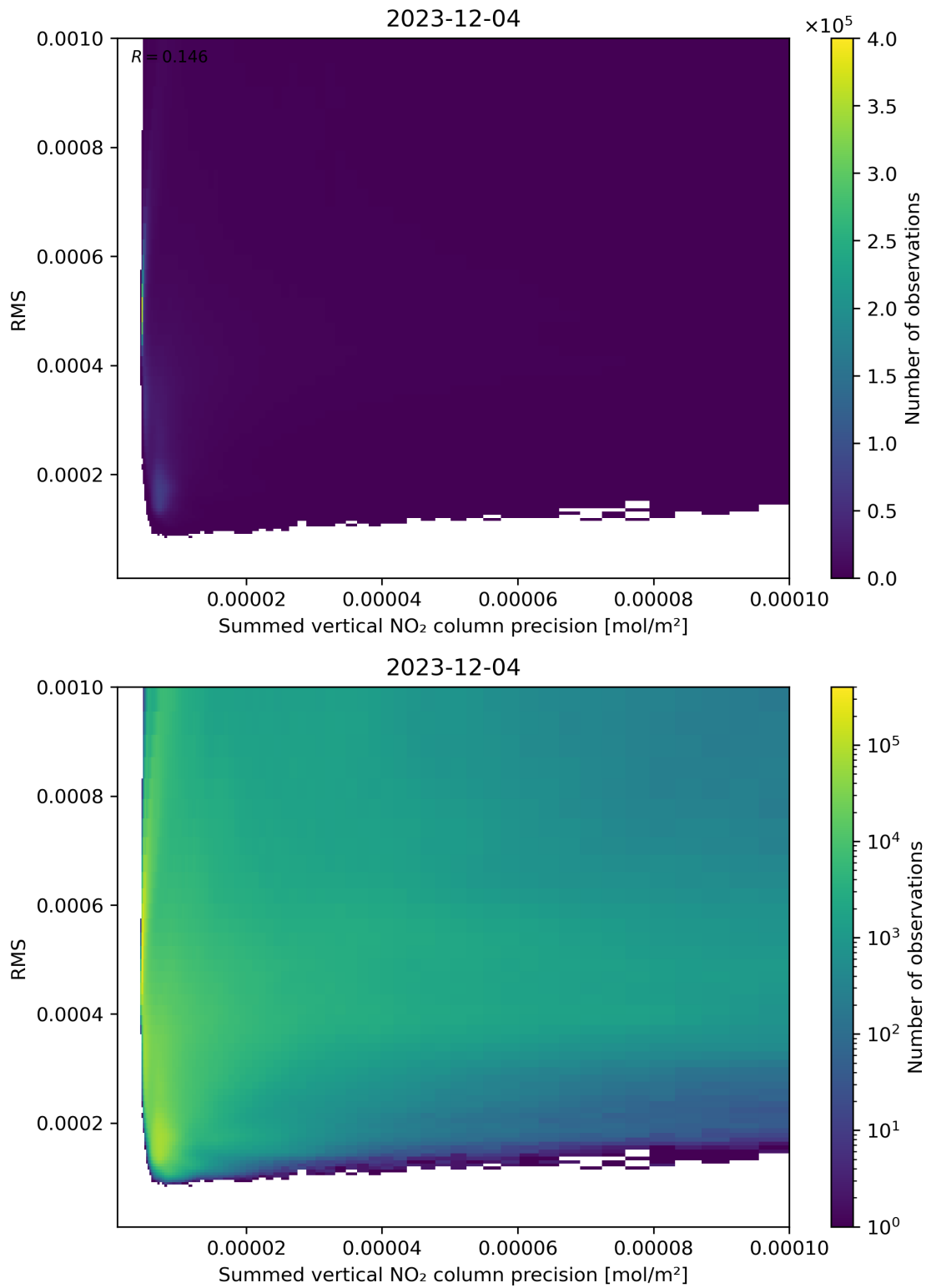
Figure 108: Scatter density plot of “Summed vertical NO 2 column precision” against “RMS” for 2023-12-04 to 2023-12-05.
