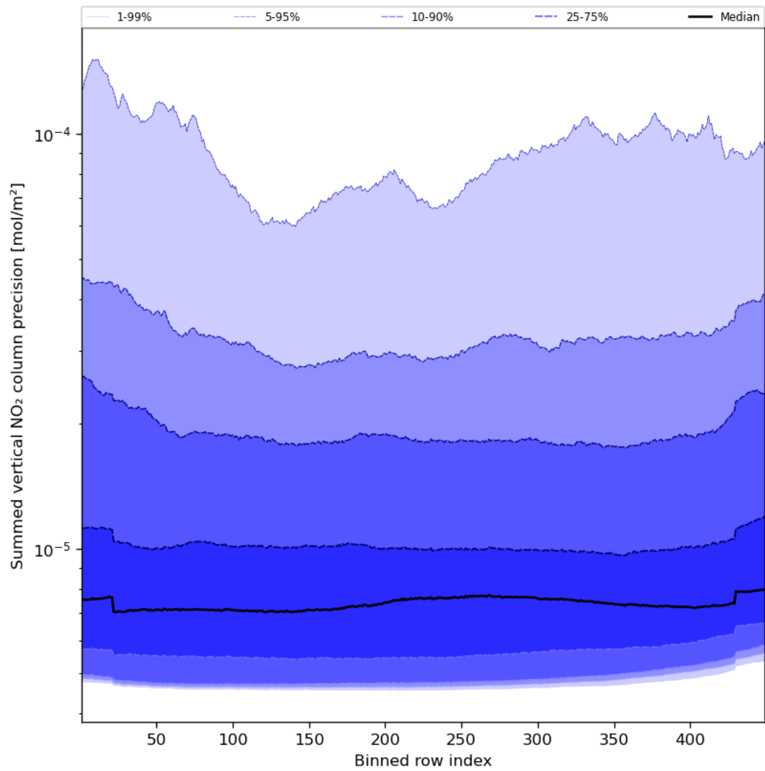
Figure 58: Along track statistics of “Summed vertical NO 2 column precision” for 2023-12-04 to 2023-12-05
