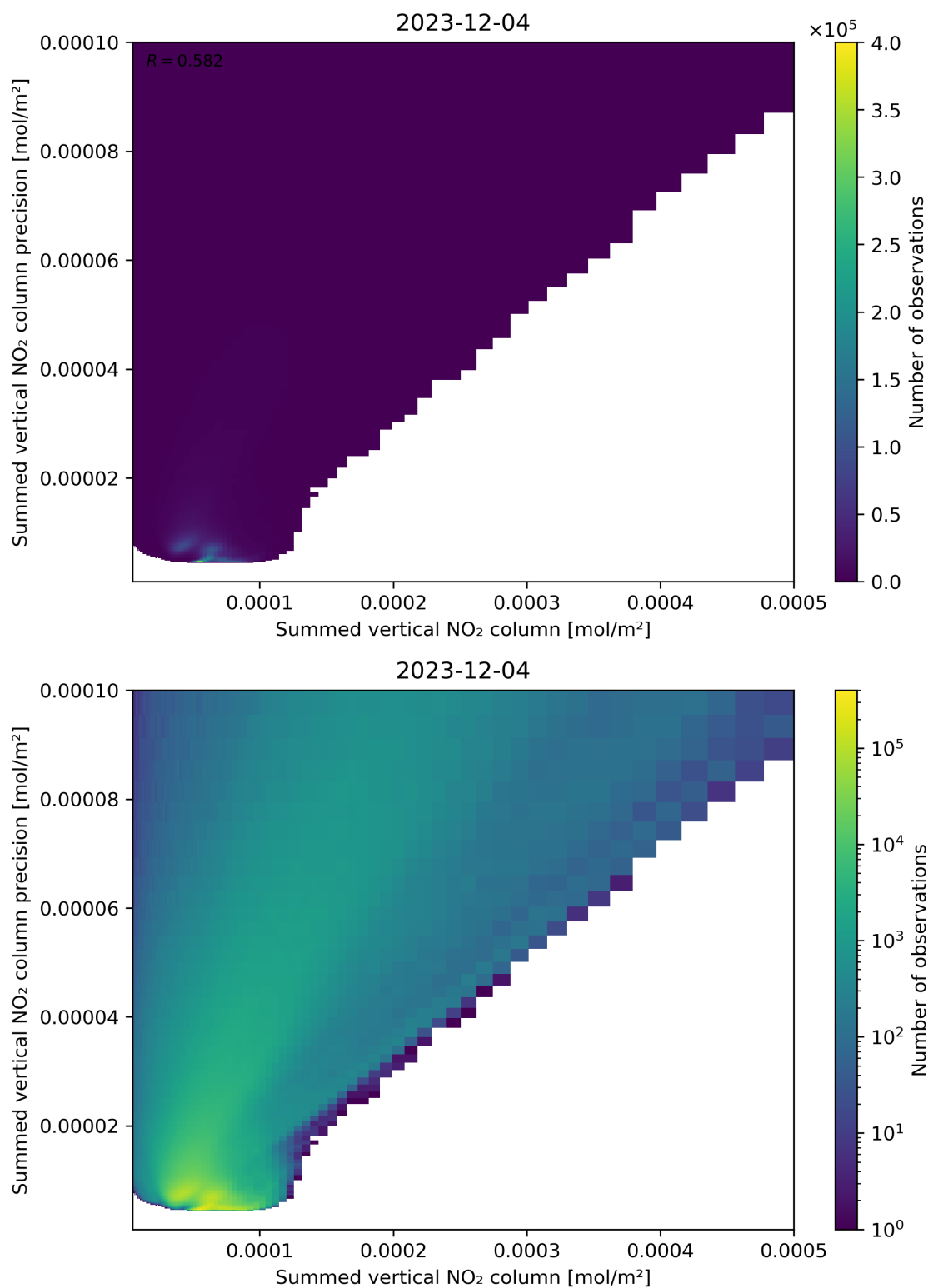
Figure 105: Scatter density plot of “Summed vertical NO 2 column” against “Summed vertical NO 2 column precision” for 2023-12-04 to 2023-12-05.
