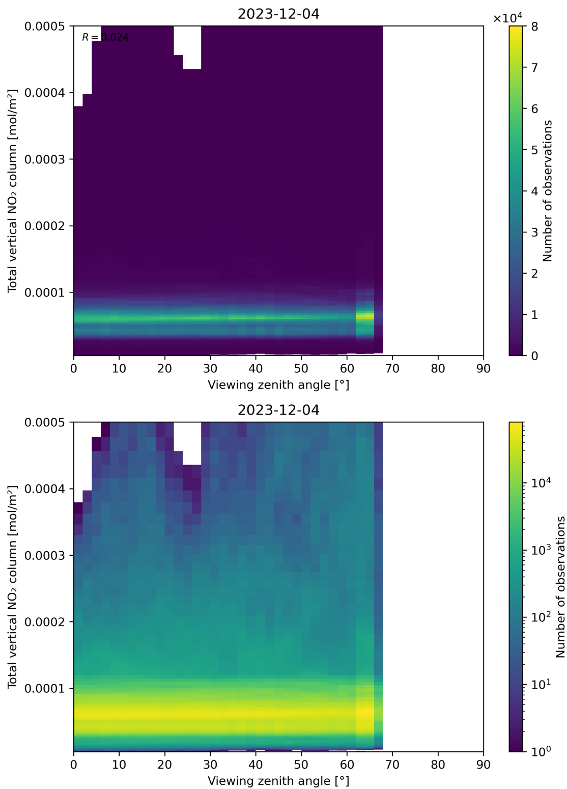
Figure 167: Scatter density plot of “Viewing zenith angle” against “Total vertical NO 2 column” for 2023-12-04 to 2023-12-05.
