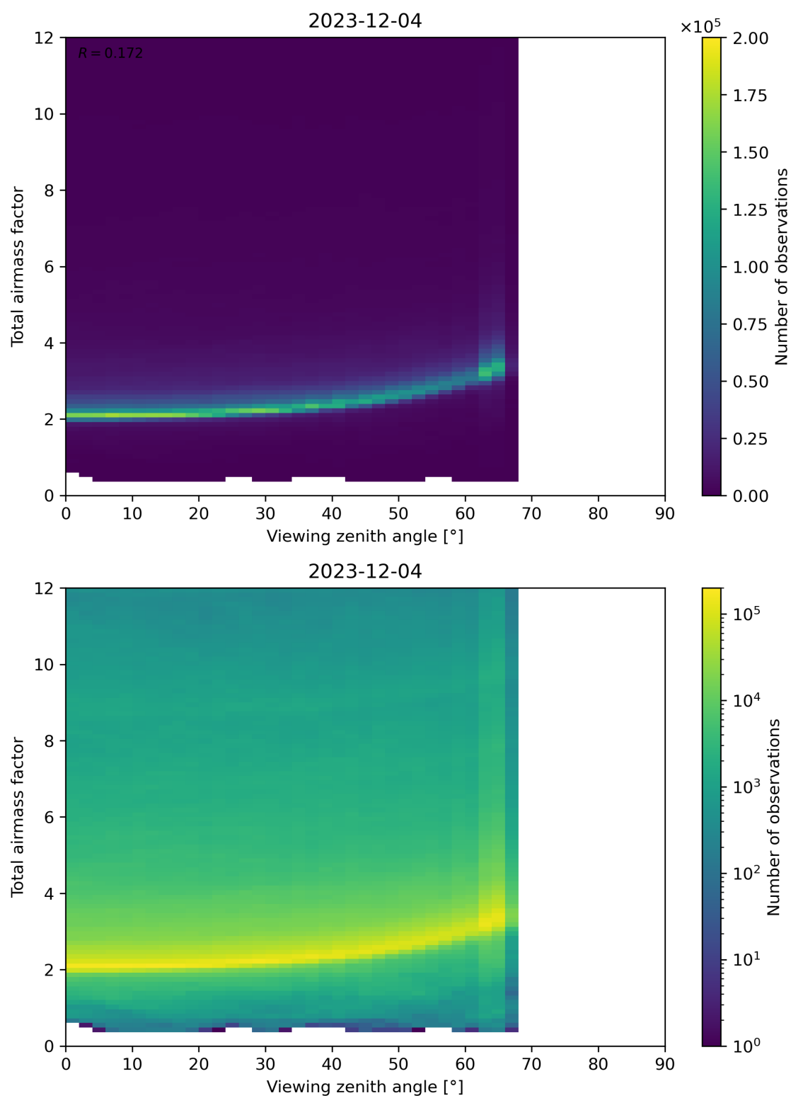
Figure 160: Scatter density plot of “Viewing zenith angle” against “Total airmass factor” for 2023-12-04 to 2023-12-05.
