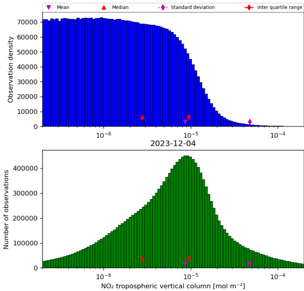
Figure 29: Histogram of “NO 2 tropospheric vertical column” for 2023-12-04 to 2023-12-05
