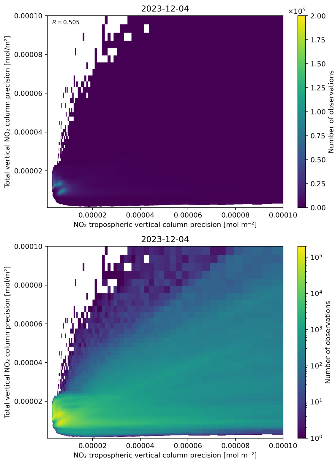
Figure 139: Scatter density plot of “NO 2 tropospheric vertical column precision” against “Total vertical NO 2 column precision” for 2023-12-04 to 2023-12-05.
