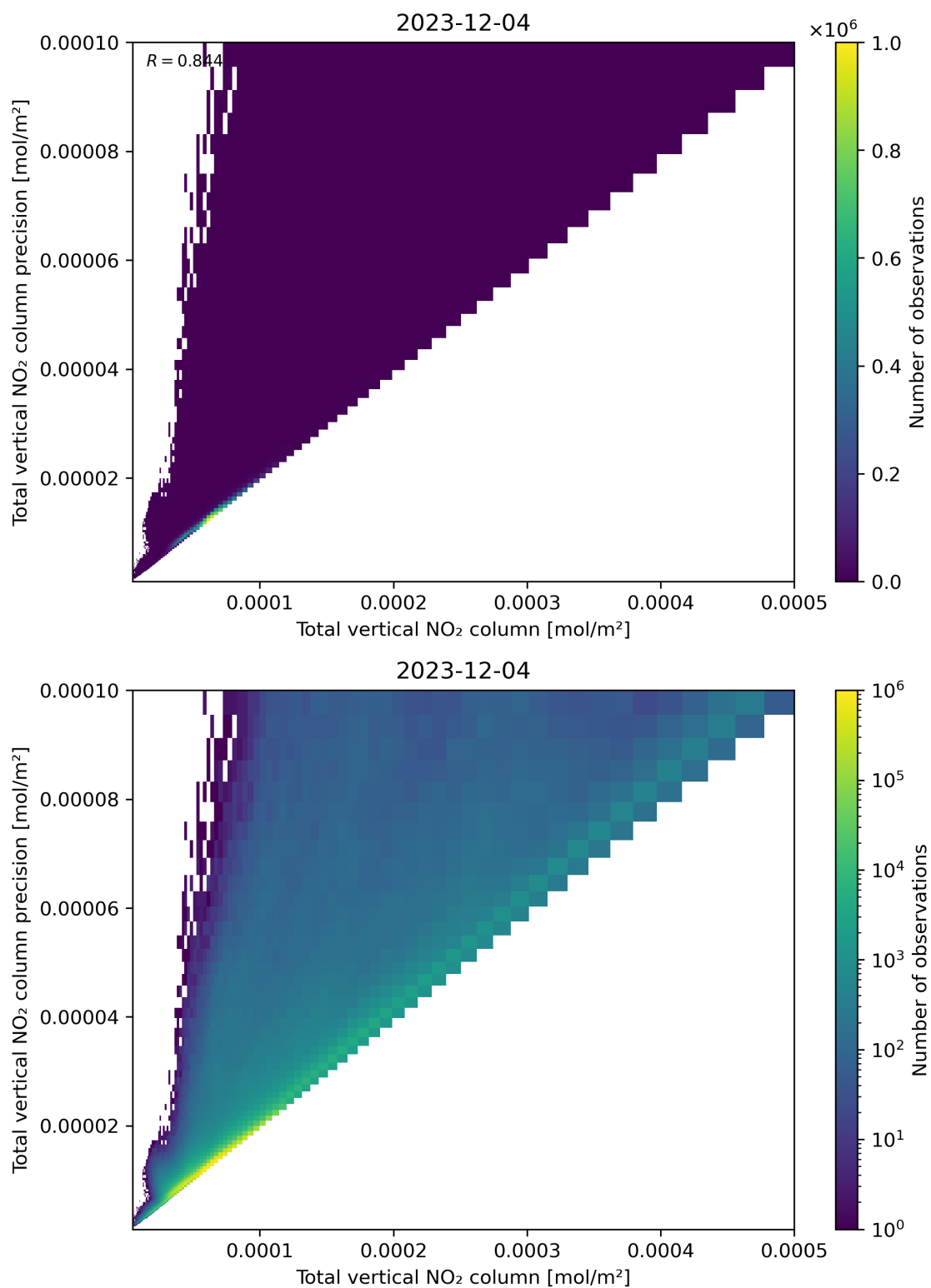
Figure 114: Scatter density plot of “Total vertical NO 2 column” against “Total vertical NO 2 column precision” for 2023-12-04 to 2023-12-05.
