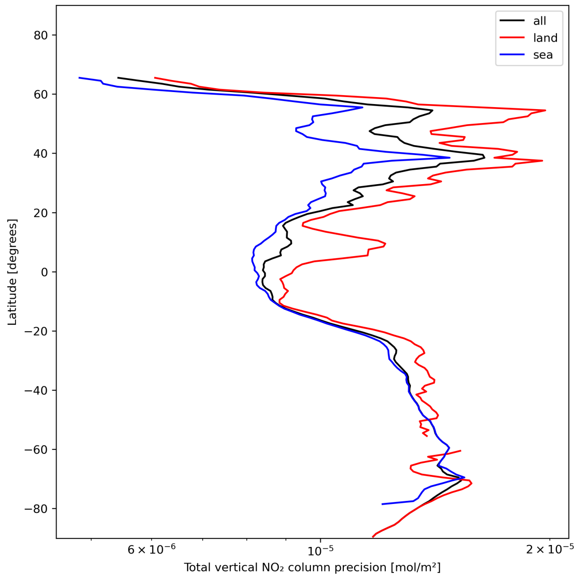
Figure 22: Zonal average of “Total vertical NO 2 column precision” for 2023-12-04 to 2023-12-05.
