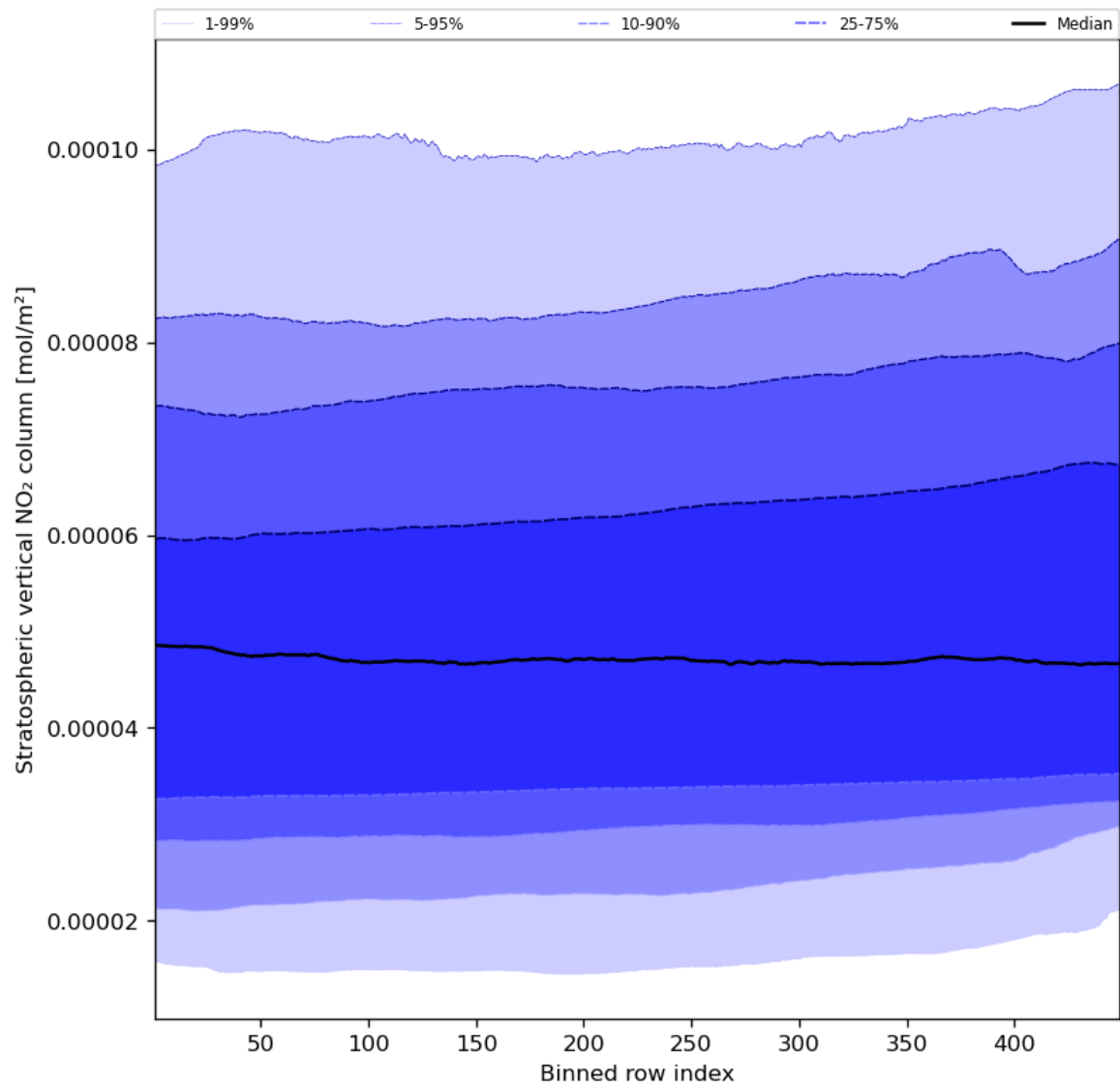
Figure 53: Along track statistics of “Stratospheric vertical NO 2 column” for 2023-12-04 to 2023-12-05
