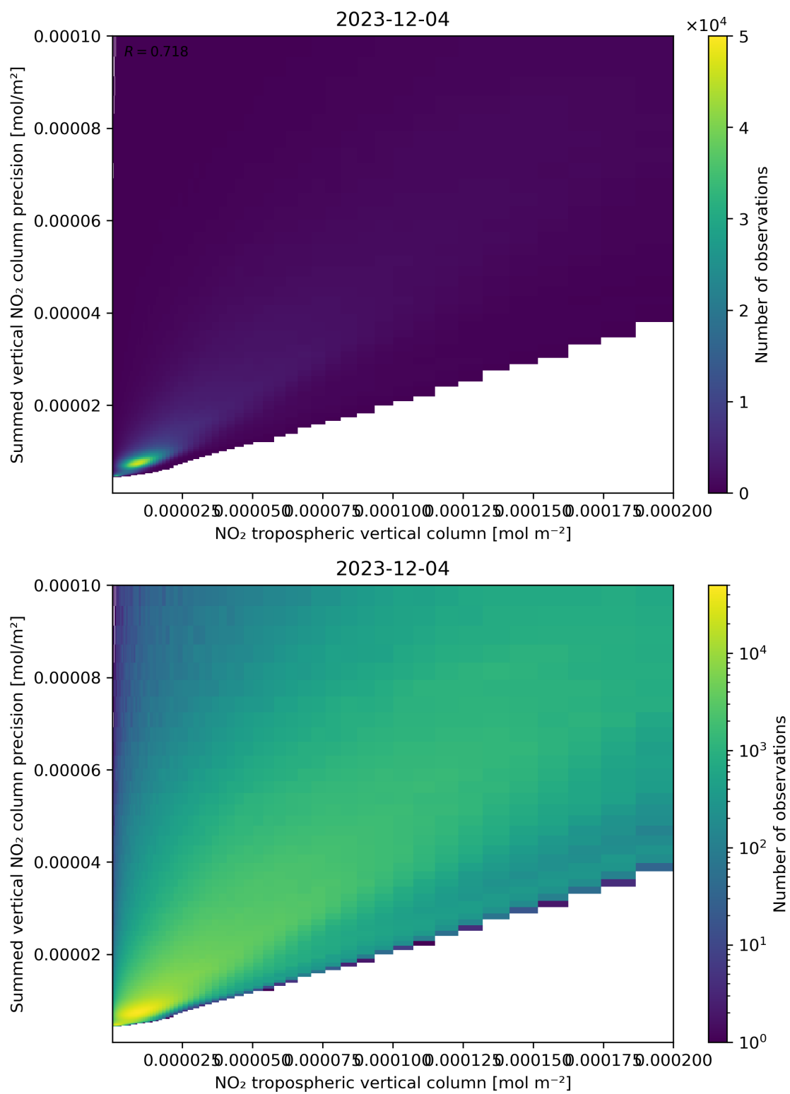
Figure 127: Scatter density plot of “NO 2 tropospheric vertical column” against “Summed vertical NO 2 column precision” for 2023-12-04 to 2023-12-05.
