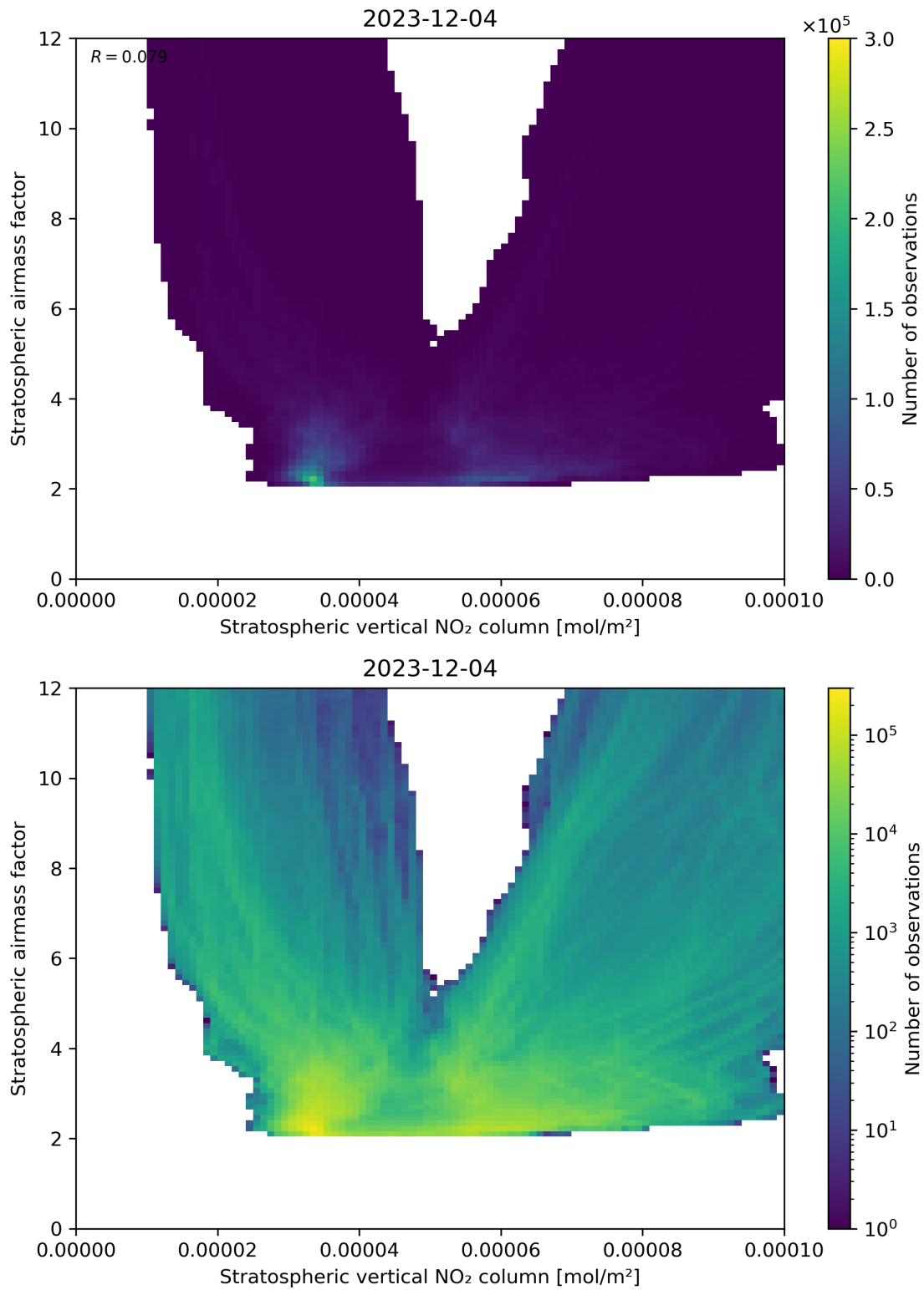
Figure 96: Scatter density plot of “Stratospheric vertical NO 2 column” against “Stratospheric airmass factor” for 2023-12-04 to 2023-12-05.
