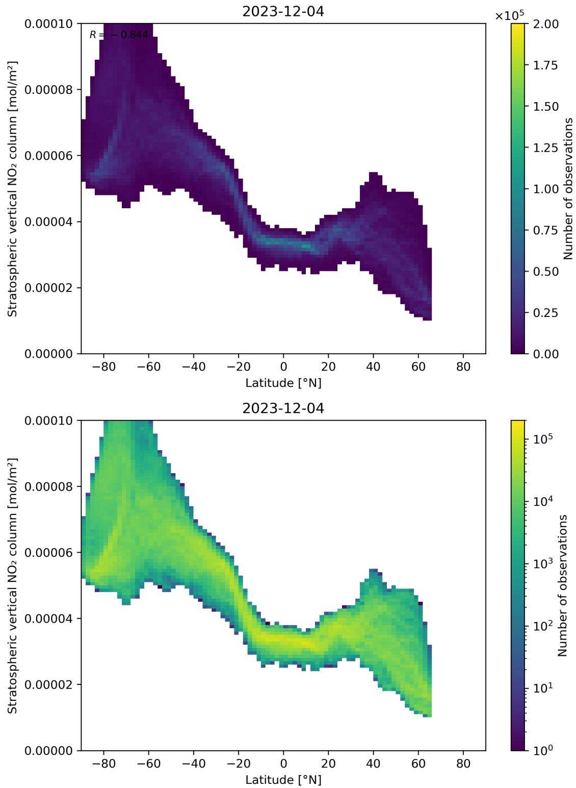
Figure 87: Scatter density plot of “Latitude” against “Stratospheric vertical NO 2 column” for 2023-12-04 to 2023-12-05.
