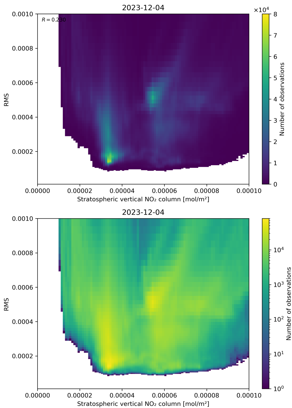
Figure 102: Scatter density plot of “Stratospheric vertical NO 2 column” against “RMS” for 2023-12-04 to 2023-12-05.
