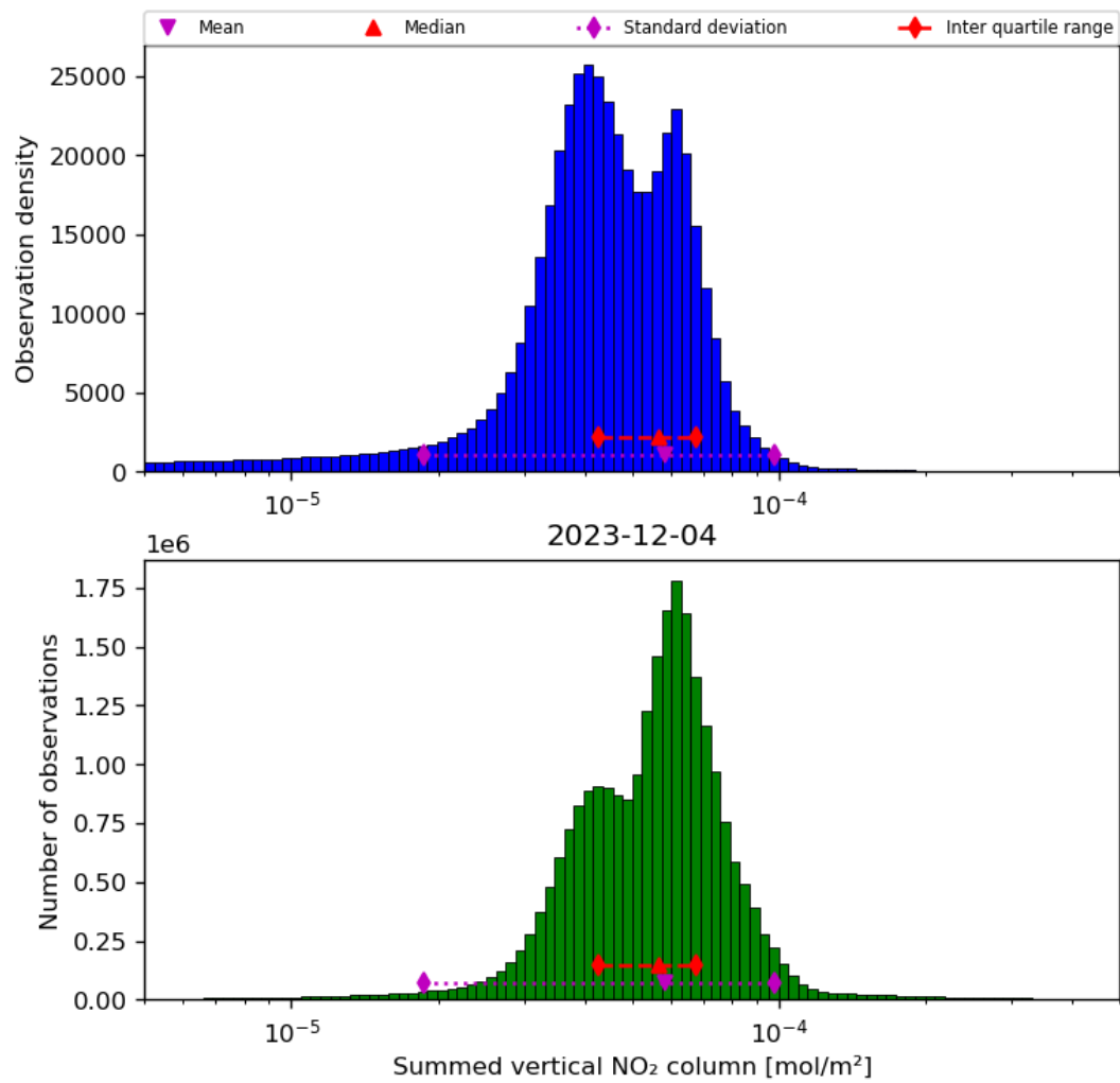
Figure 40: Histogram of "Summed vertical NO 2 column" for 2023-12-04 to 2023-12-05
