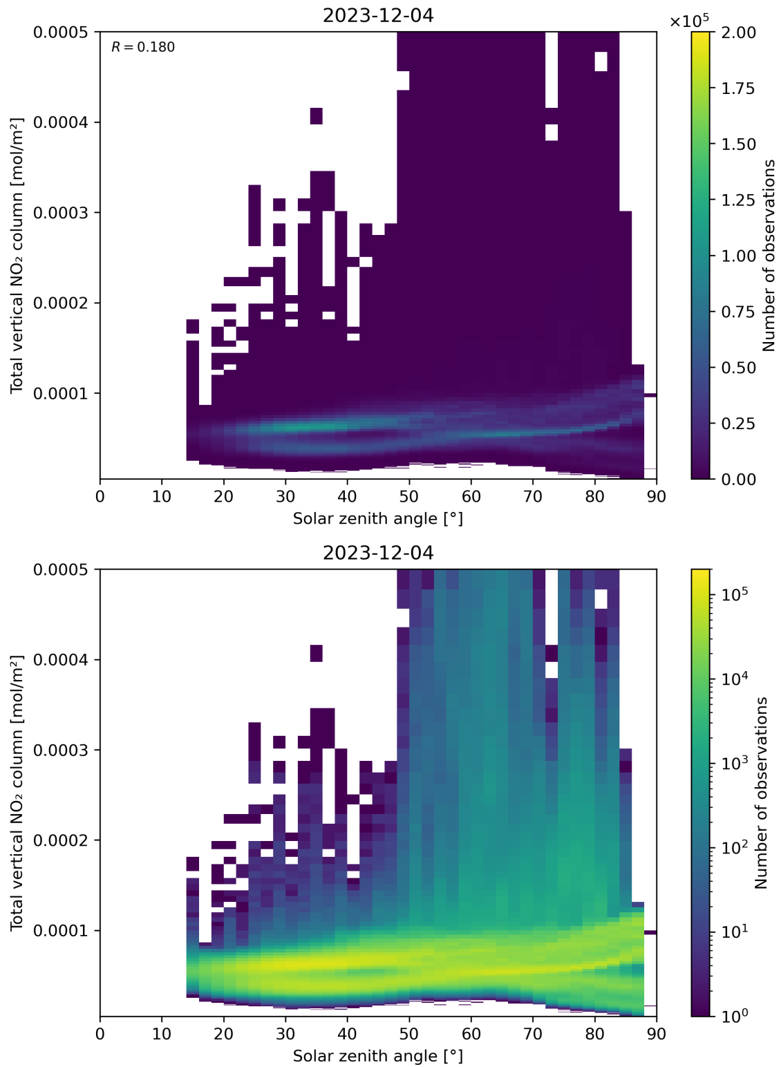
Figure 153: Scatter density plot of “Solar zenith angle” against “Total vertical \text{NO}_2 column” for 2023-12-04 to 2023-12-05.
