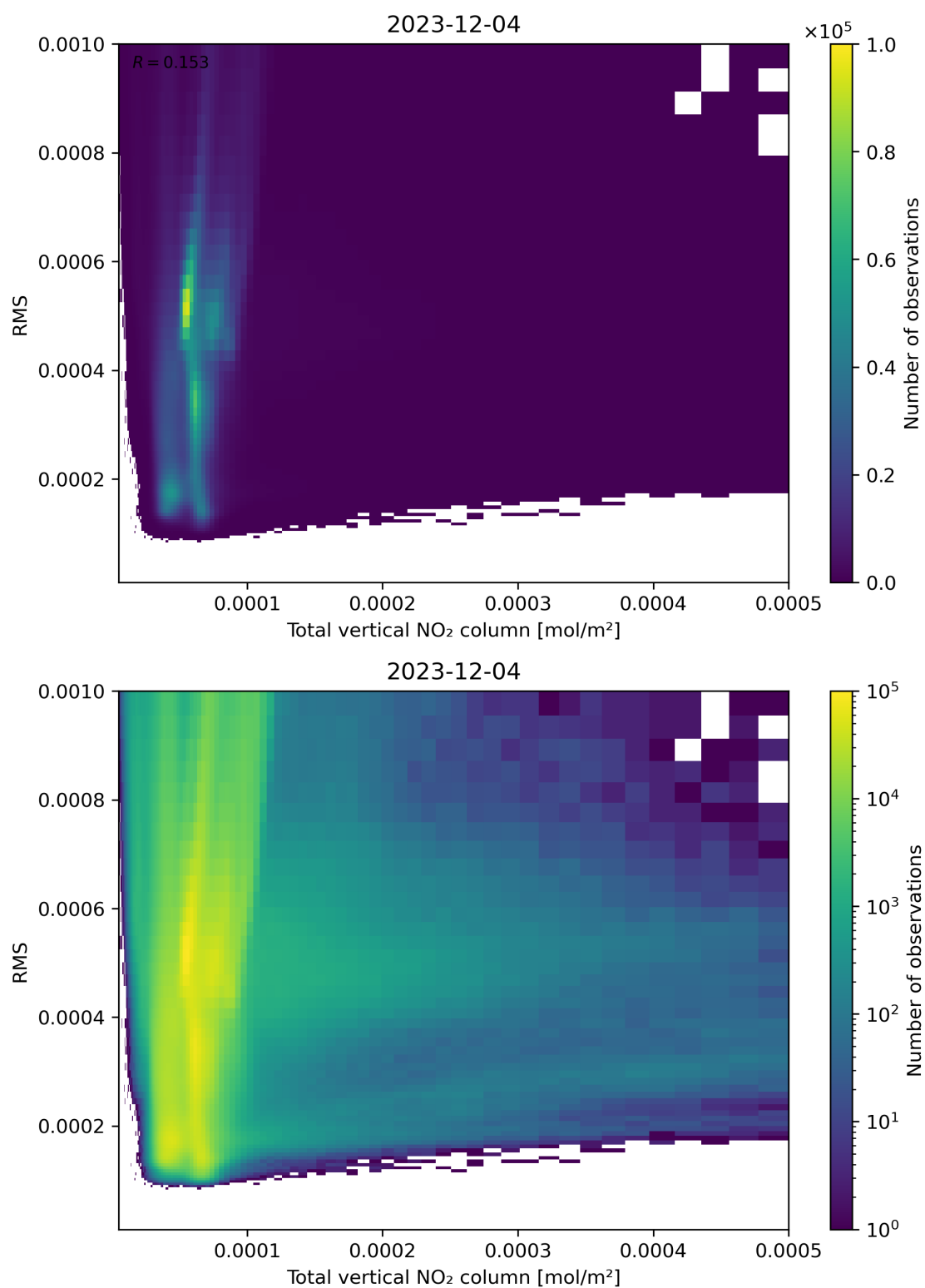
Figure 120: Scatter density plot of “Total vertical NO 2 column” against “RMS” for 2023-12-04 to 2023-12-05.
