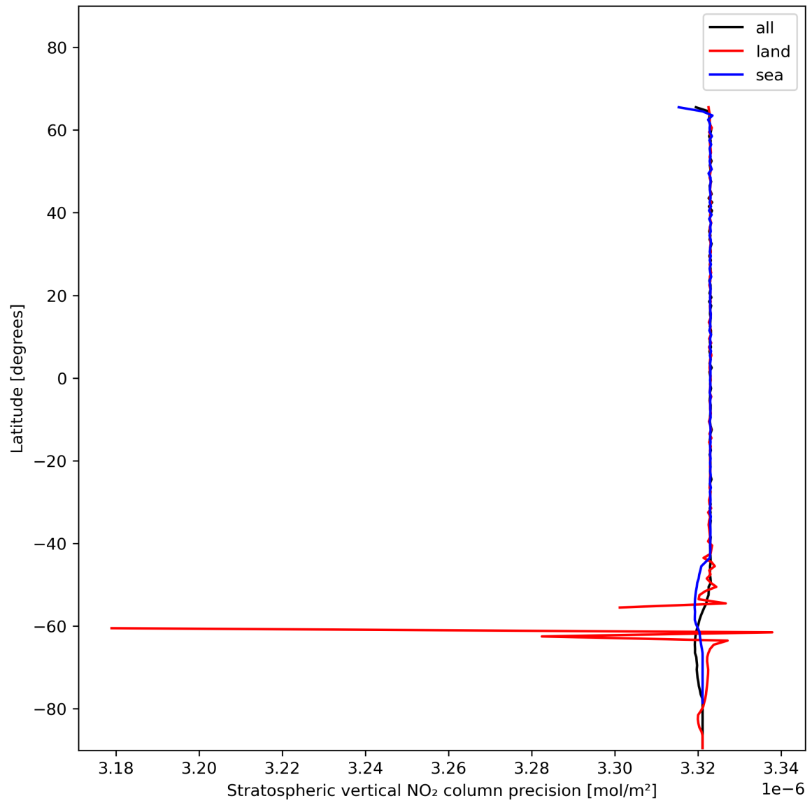
Figure 20: Zonal average of “Stratospheric vertical NO 2 column precision” for 2023-12-04 to 2023-12-05.
