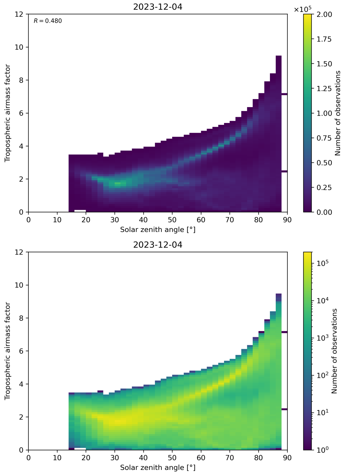
Figure 147: Scatter density plot of “Solar zenith angle” against “Tropospheric airmass factor” for 2023-12-04 to 2023-12-05.
