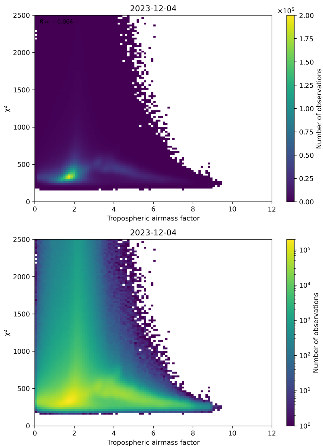
Figure 73: Scatter density plot of “Tropospheric airmass factor” against “ \chi^2 ” for 2023-12-04 to 2023-12-05.
