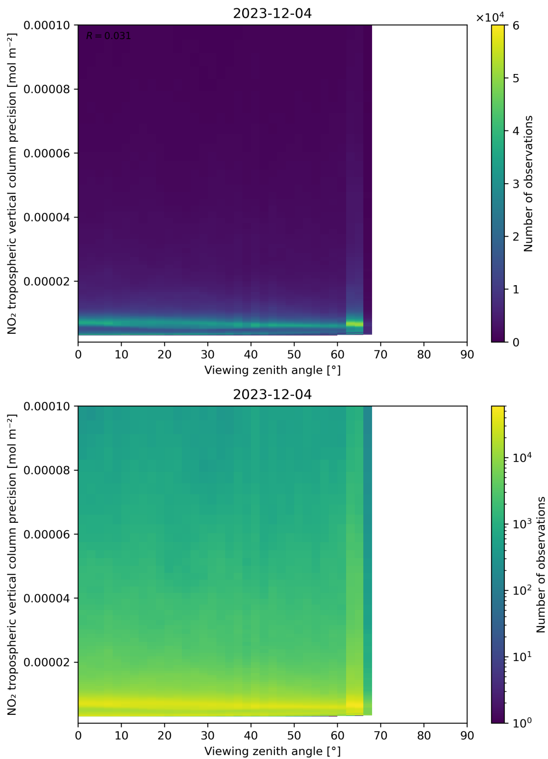
Figure 170: Scatter density plot of “Viewing zenith angle” against “NO 2 tropospheric vertical column precision” for 2023-12-04 to 2023-12-05.
