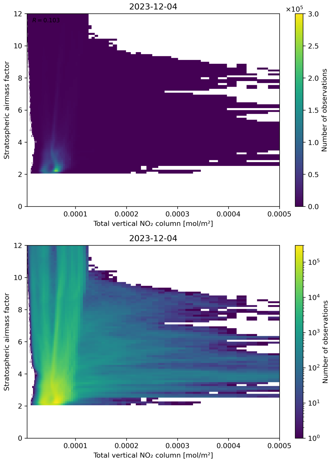
Figure 110: Scatter density plot of “Total vertical NO 2 column” against “Stratospheric air mass factor” for 2023-12-04 to 2023-12-05.
