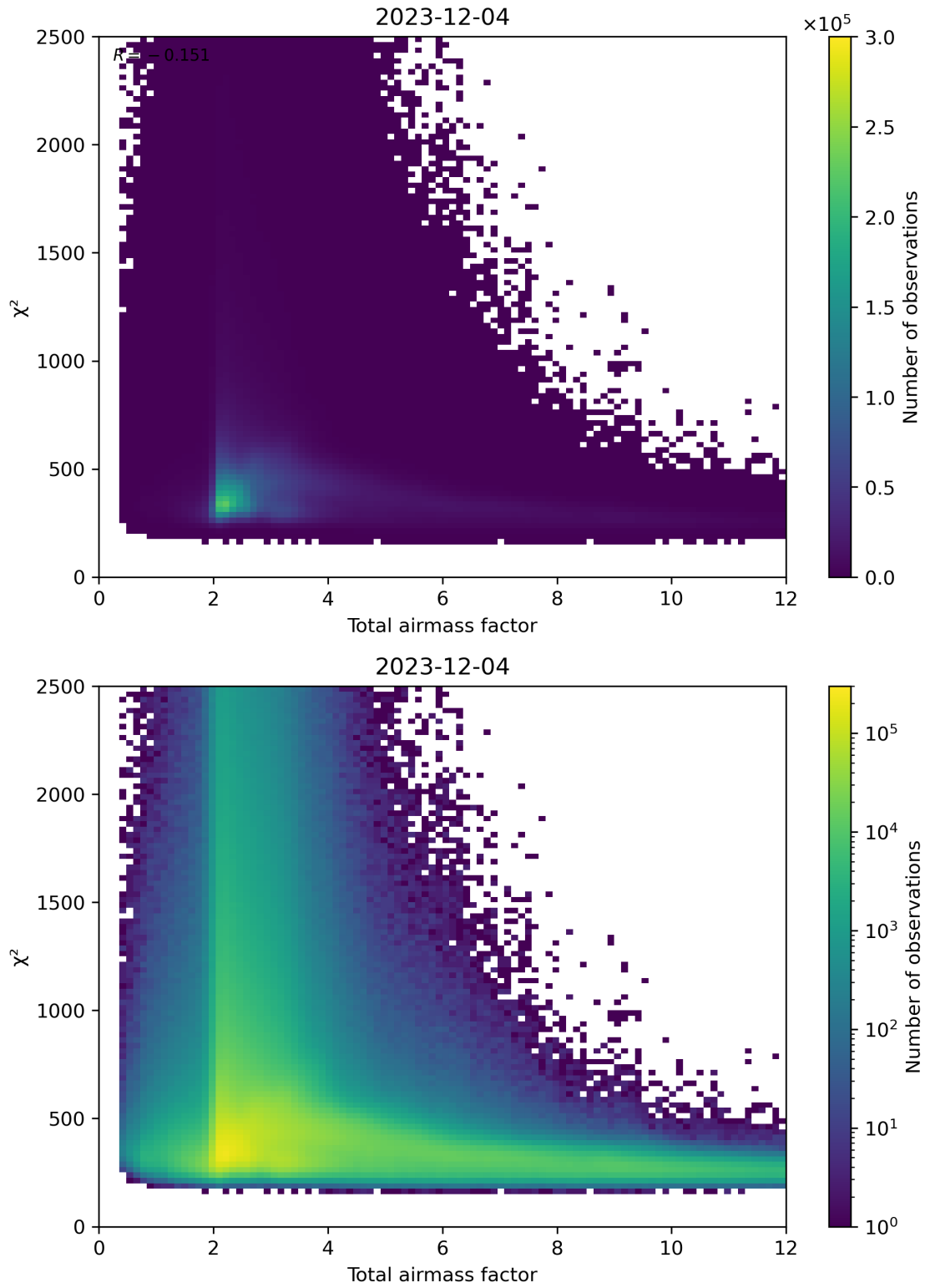
Figure 63: Scatter density plot of “Total airmass factor” against “ \chi^2 ” for 2023-12-04 to 2023-12-05.
