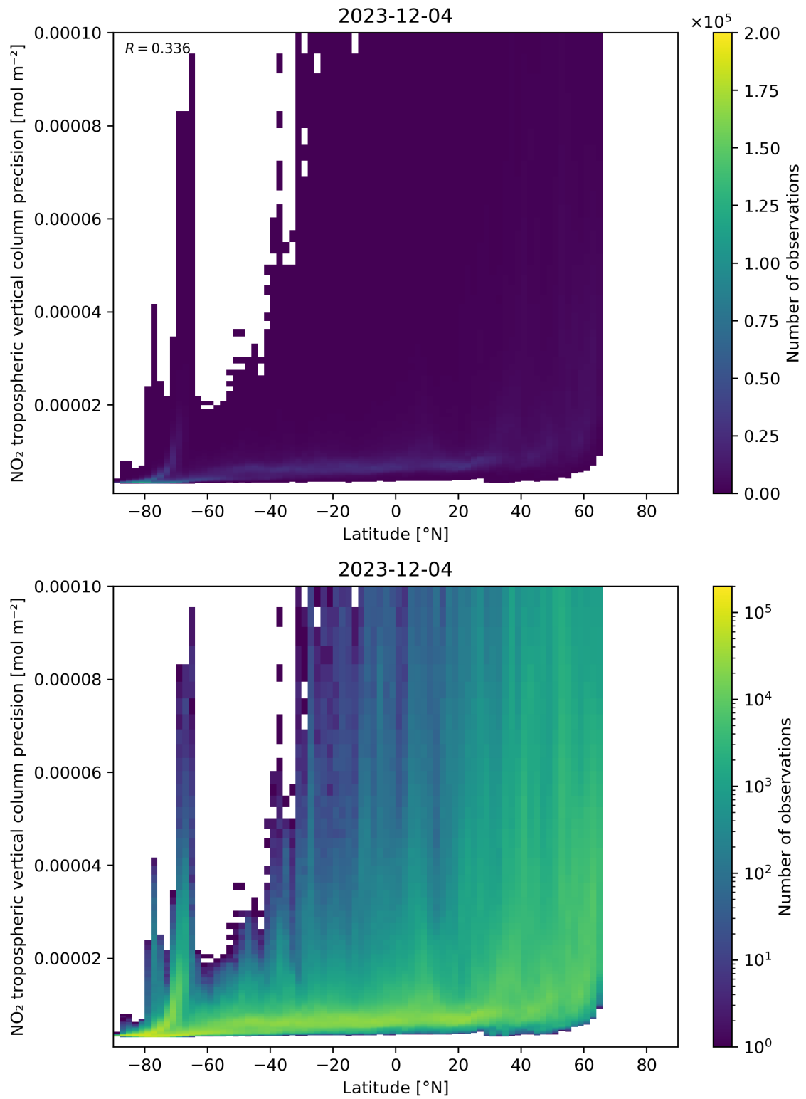
Figure 93: Scatter density plot of “Latitude” against “NO 2 tropospheric vertical column precision” for 2023-12-04 to 2023-12-05.
