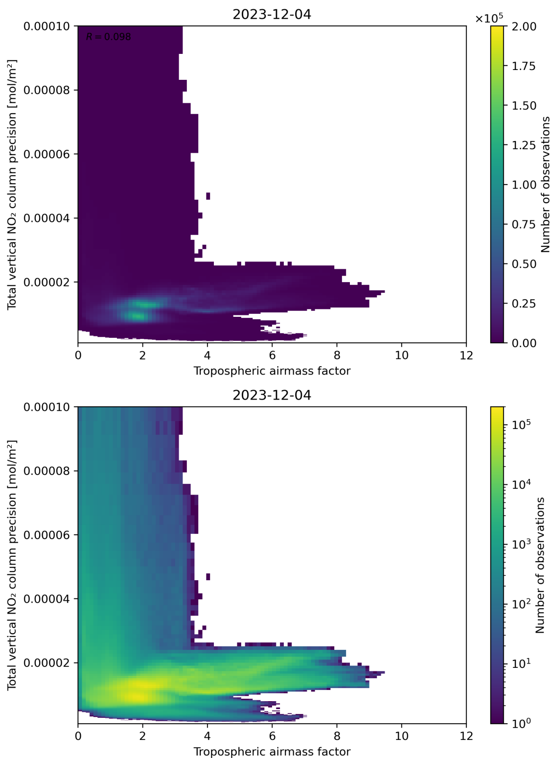
Figure 78: Scatter density plot of “Tropospheric air mass factor” against “Total vertical NO 2 column precision” for 2023-12-04 to 2023-12-05.
