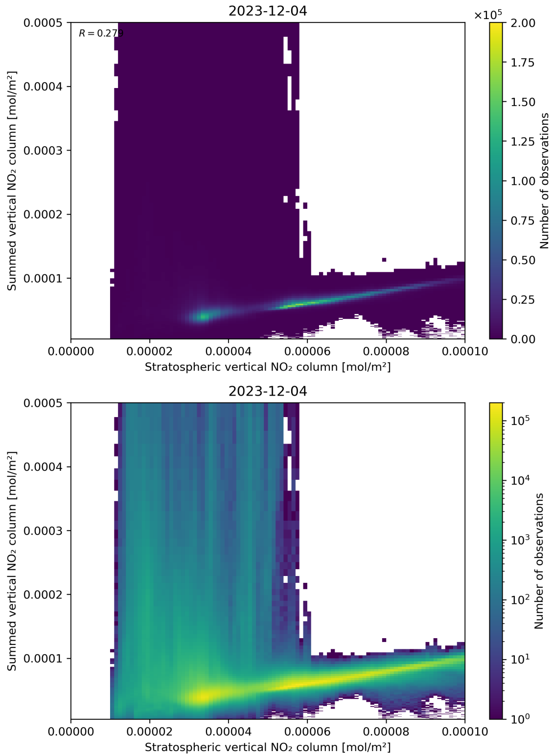
Figure 98: Scatter density plot of “Stratospheric vertical NO 2 column” against “Summed vertical NO 2 column” for 2023-12-04 to 2023-12-05.
