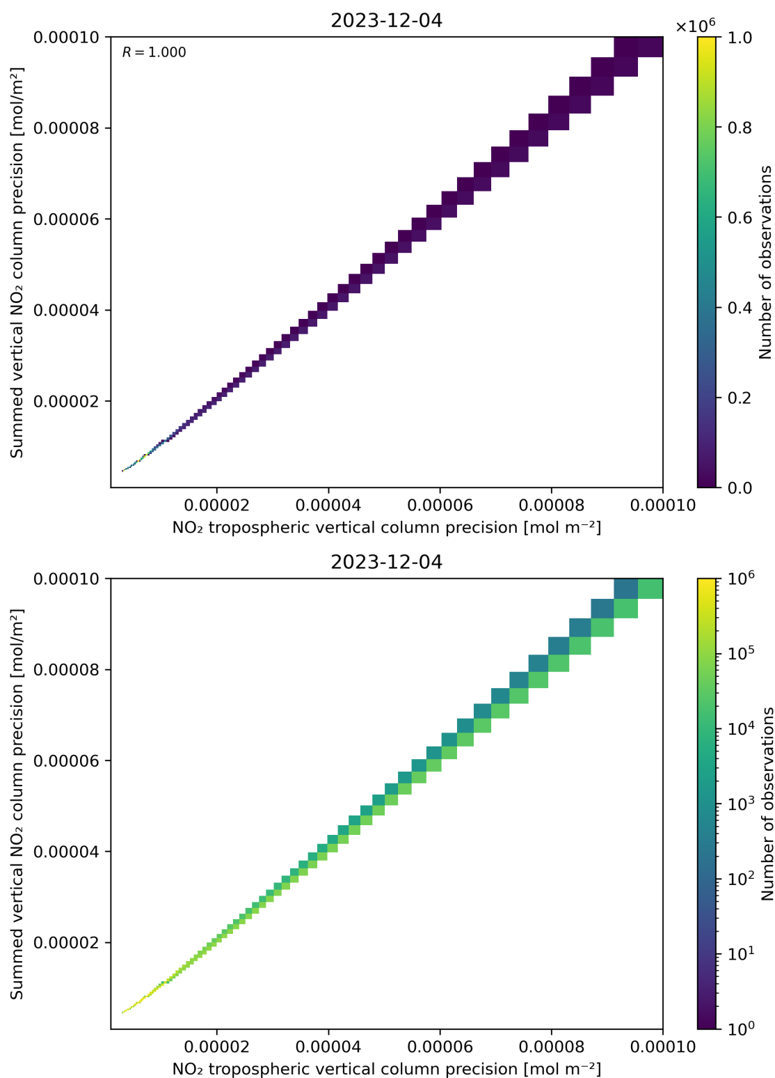
Figure 137: Scatter density plot of “NO 2 tropospheric vertical column precision” against “Summed vertical NO 2 column precision” for 2023-12-04 to 2023-12-05.
