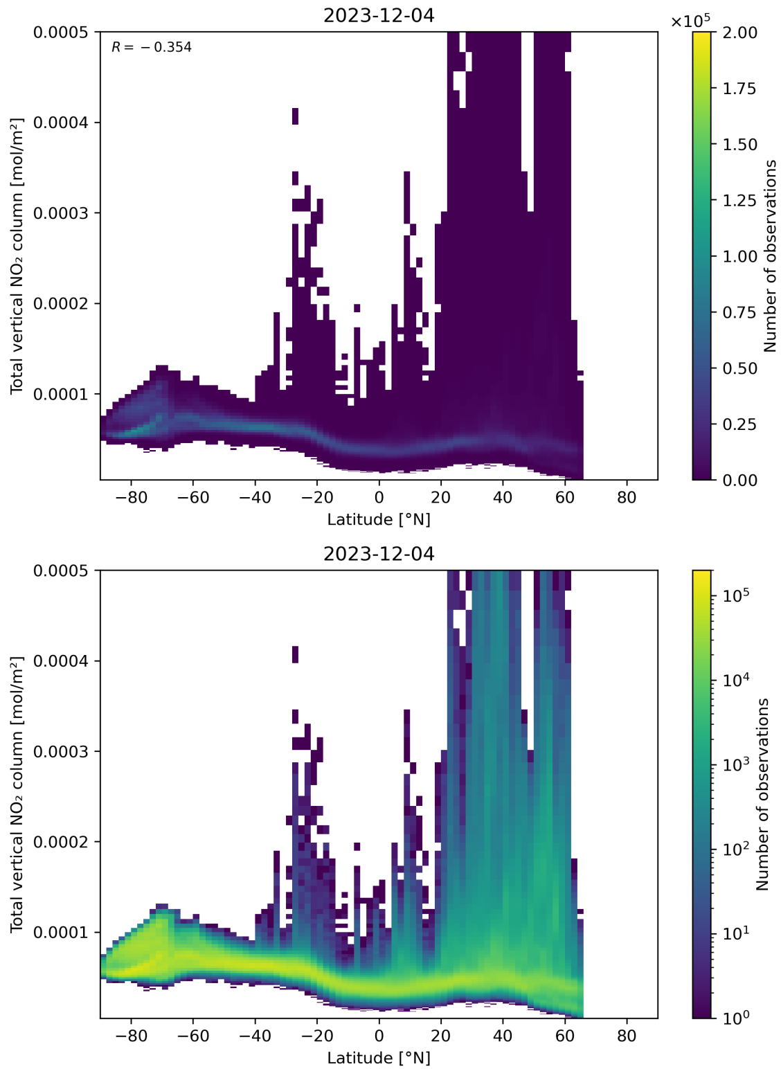
Figure 90: Scatter density plot of “Latitude” against “Total vertical NO 2 column” for 2023-12-04 to 2023-12-05.
