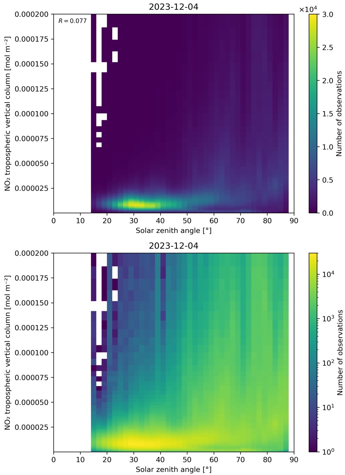
Figure 155: Scatter density plot of “Solar zenith angle” against “NO 2 tropospheric vertical column” for 2023-12-04 to 2023-12-05.
