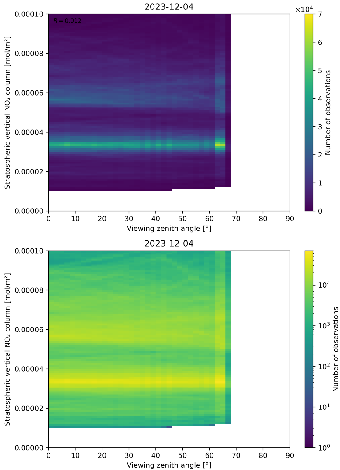
Figure 164: Scatter density plot of “Viewing zenith angle” against “Stratospheric vertical NO 2 column” for 2023-12-04 to 2023-12-05.
