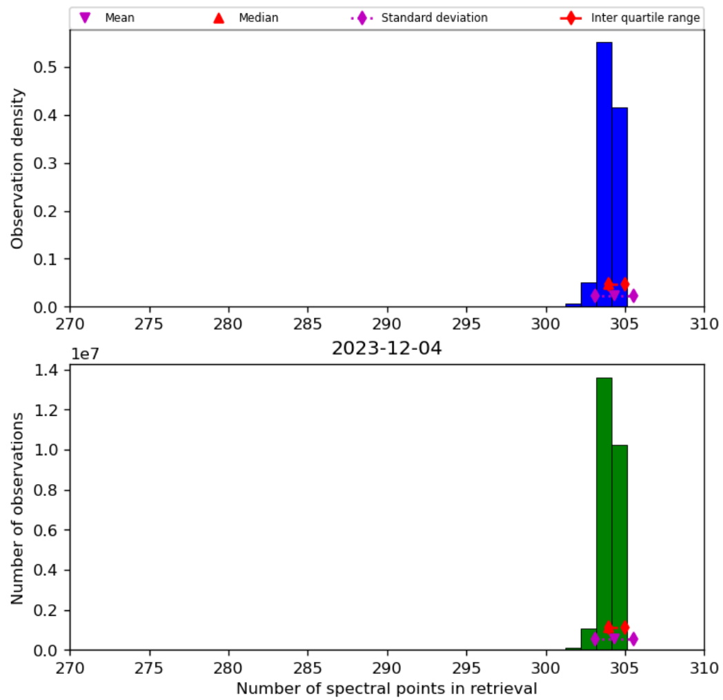
Figure 33: Histogram of “Number of spectral points in retrieval” for 2023-12-04 to 2023-12-05
