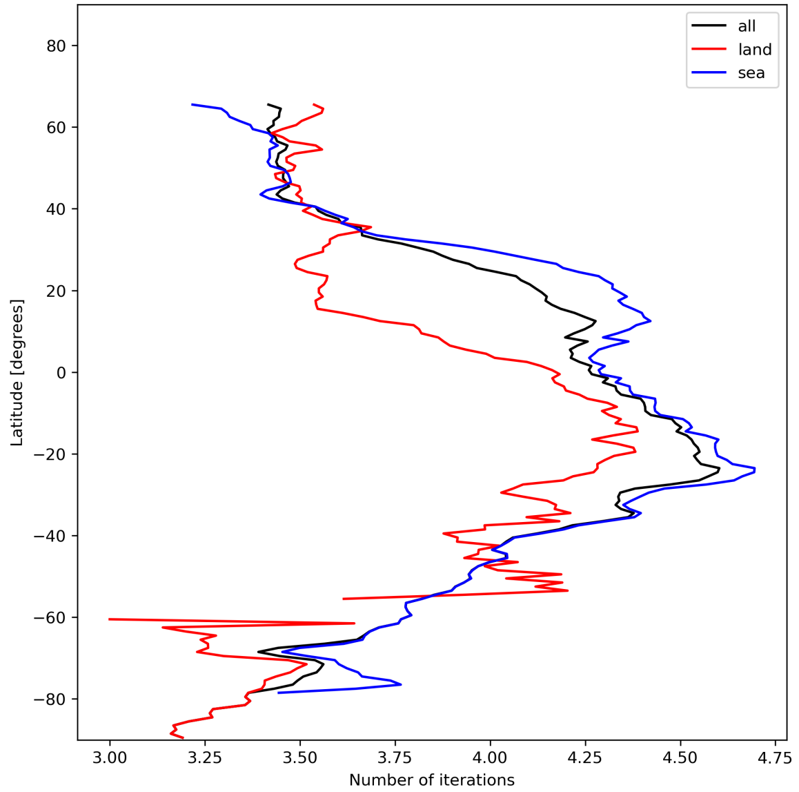
Figure 17: Zonal average of “Number of iterations” for 2023-12-04 to 2023-12-05.
