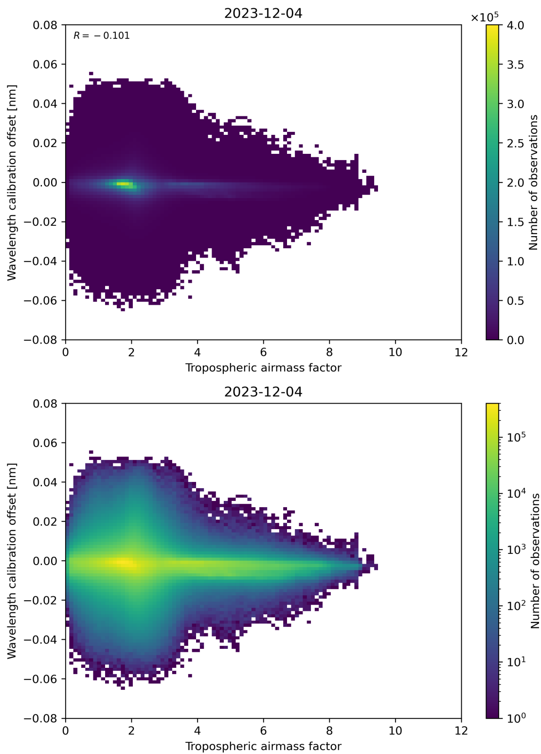
Figure 80: Scatter density plot of “Tropospheric air mass factor” against “Wavelength calibration offset” for 2023-12-04 to 2023-12-05.
