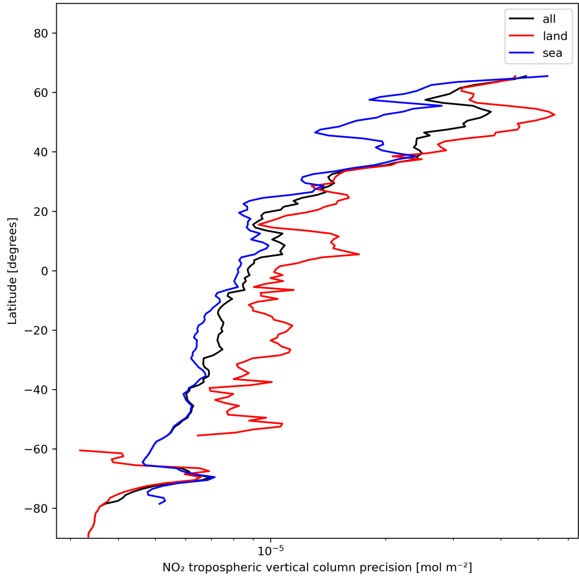
Figure 13: Zonal average of “NO 2 tropospheric vertical column precision” for 2023-12-04 to 2023-12-05.
