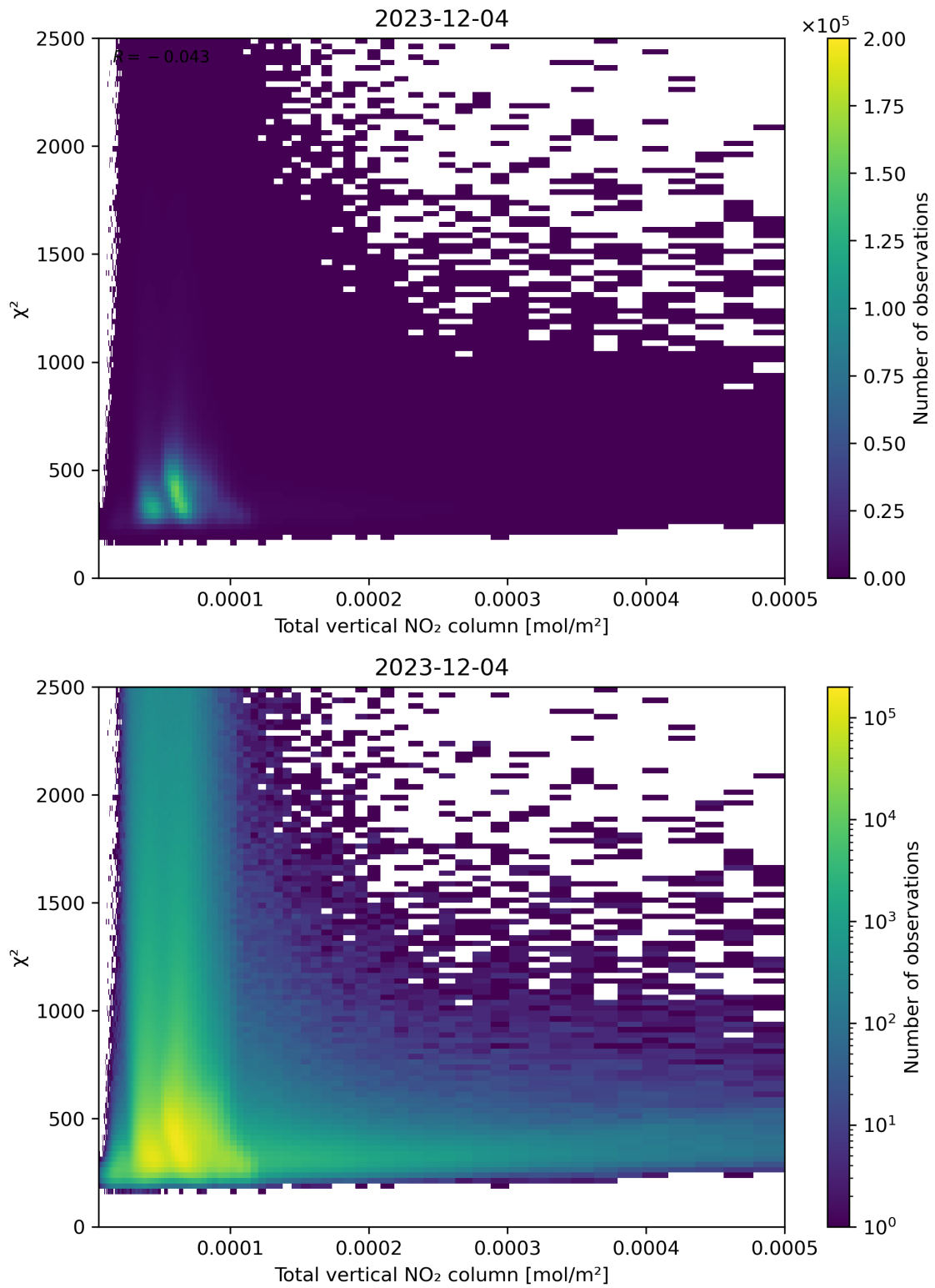
Figure 111: Scatter density plot of “Total vertical NO 2 column” against “ \chi^2 ” for 2023-12-04 to 2023-12-05.
