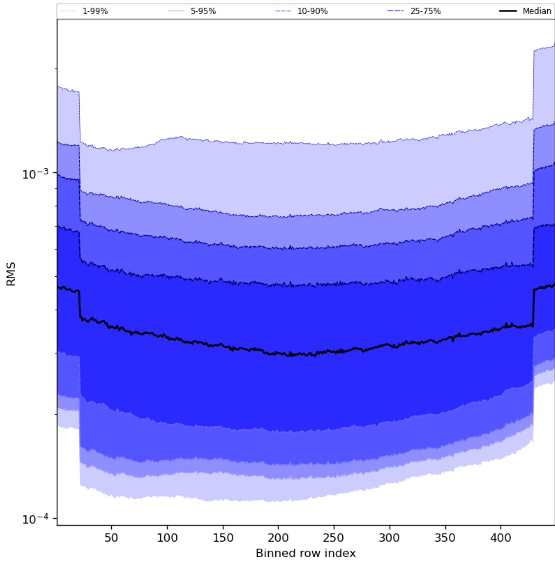
Figure 60: Along track statistics of “RMS” for 2023-12-04 to 2023-12-05
