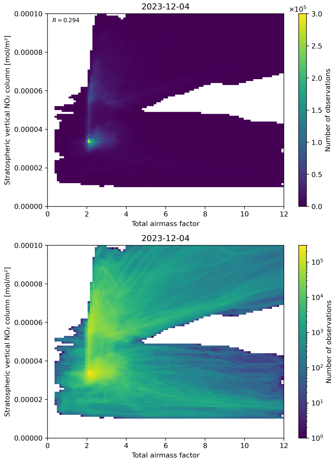
Figure 64: Scatter density plot of “Total airmass factor” against “Stratospheric vertical NO 2 column” for 2023-12-04 to 2023-12-05.
