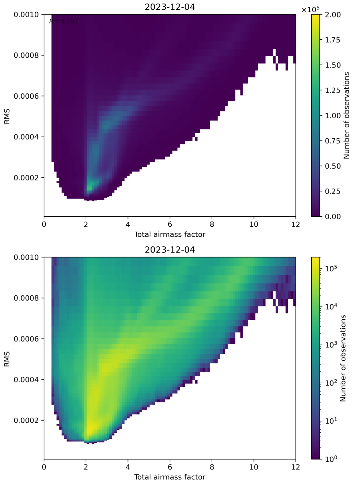
Figure 69: Scatter density plot of “Total airmass factor” against “RMS” for 2023-12-04 to 2023-12-05.
