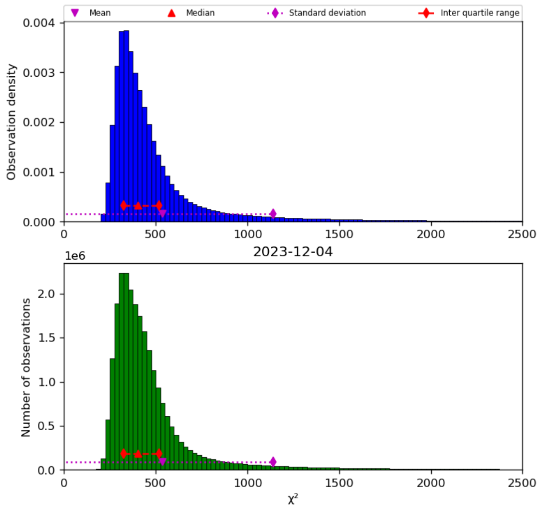
Figure 42: Histogram of “ \chi^2 ” for 2023-12-04 to 2023-12-05
