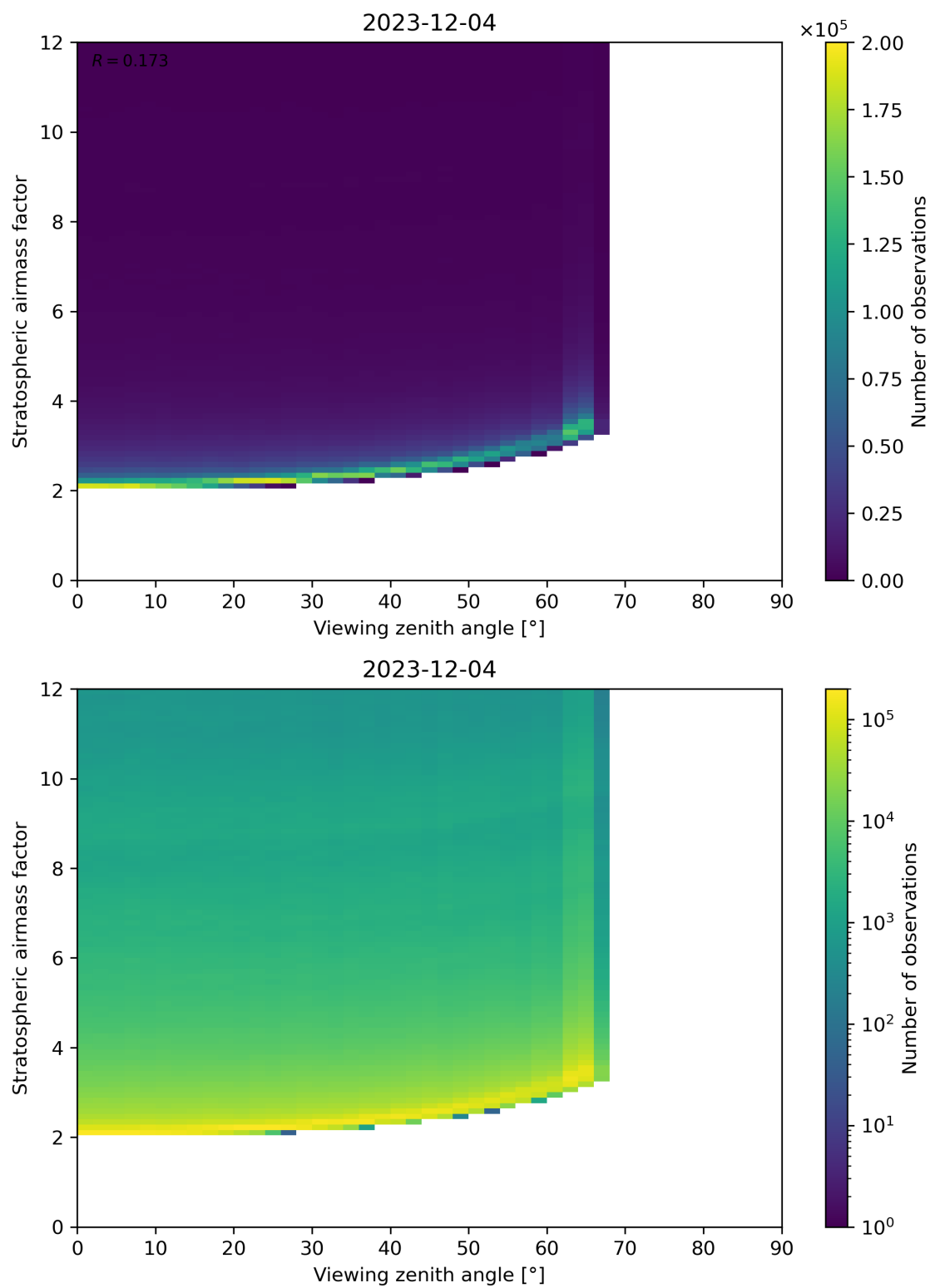
Figure 159: Scatter density plot of “Viewing zenith angle” against “Stratospheric airmass factor” for 2023-12-04 to 2023-12-05.
