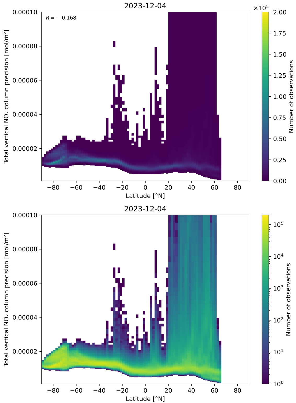
Figure 91: Scatter density plot of “Latitude” against “Total vertical NO 2 column precision” for 2023-12-04 to 2023-12-05.
