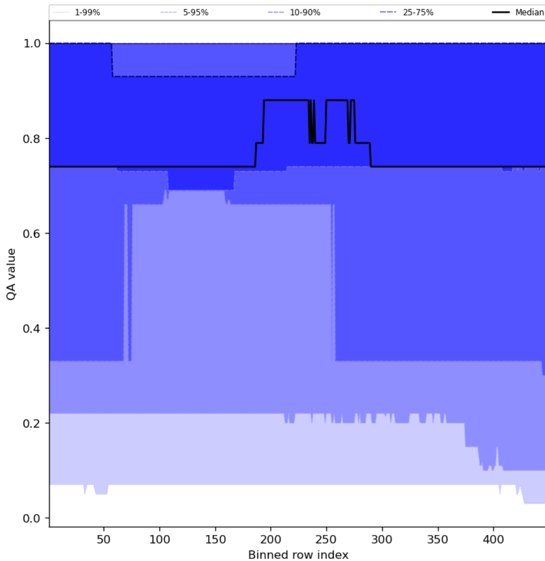
Figure 45: Along track statistics of “QA value” for 2023-12-04 to 2023-12-05
