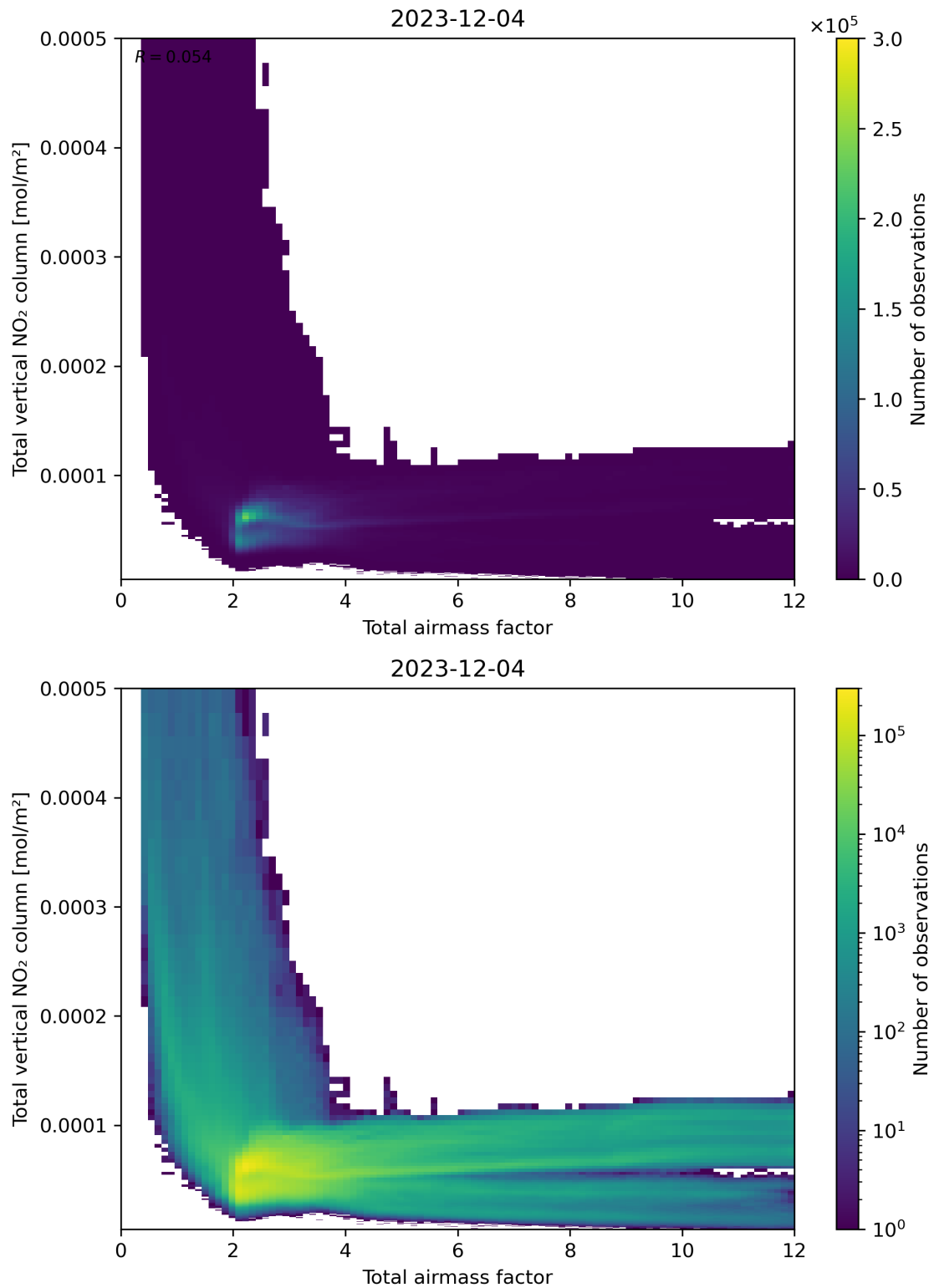
Figure 67: Scatter density plot of “Total airmass factor” against “Total vertical NO 2 column” for 2023-12-04 to 2023-12-05.
