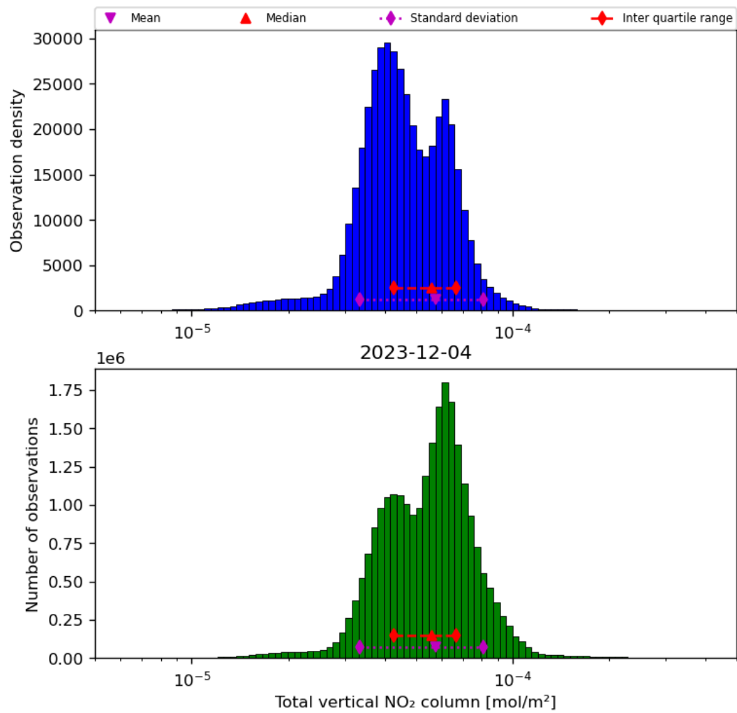
Figure 38: Histogram of “Total vertical NO 2 column” for 2023-12-04 to 2023-12-05
