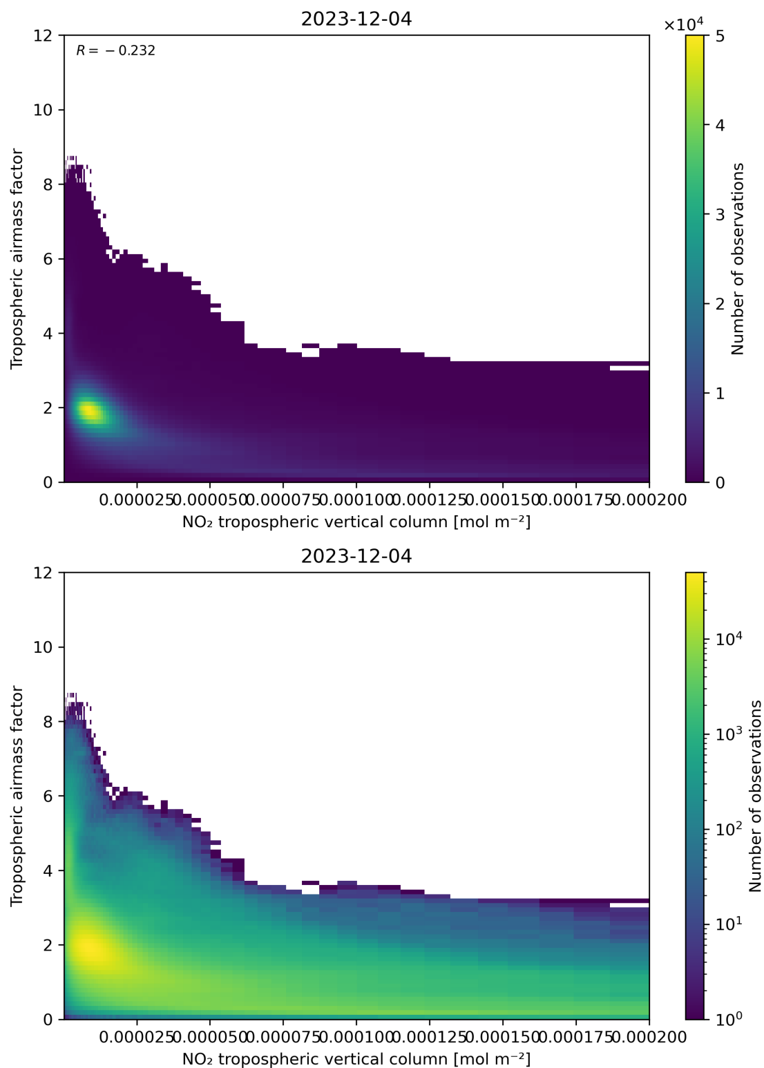
Figure 123: Scatter density plot of “NO 2 tropospheric vertical column” against “Tropospheric air mass factor” for 2023-12-04 to 2023-12-05.
