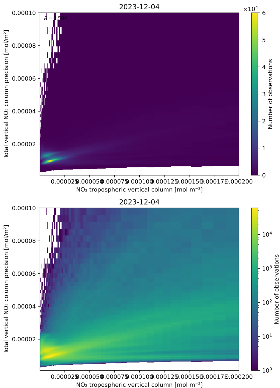
Figure 129: Scatter density plot of “NO 2 tropospheric vertical column” against “Total vertical NO 2 column precision” for 2023-12-04 to 2023-12-05.
