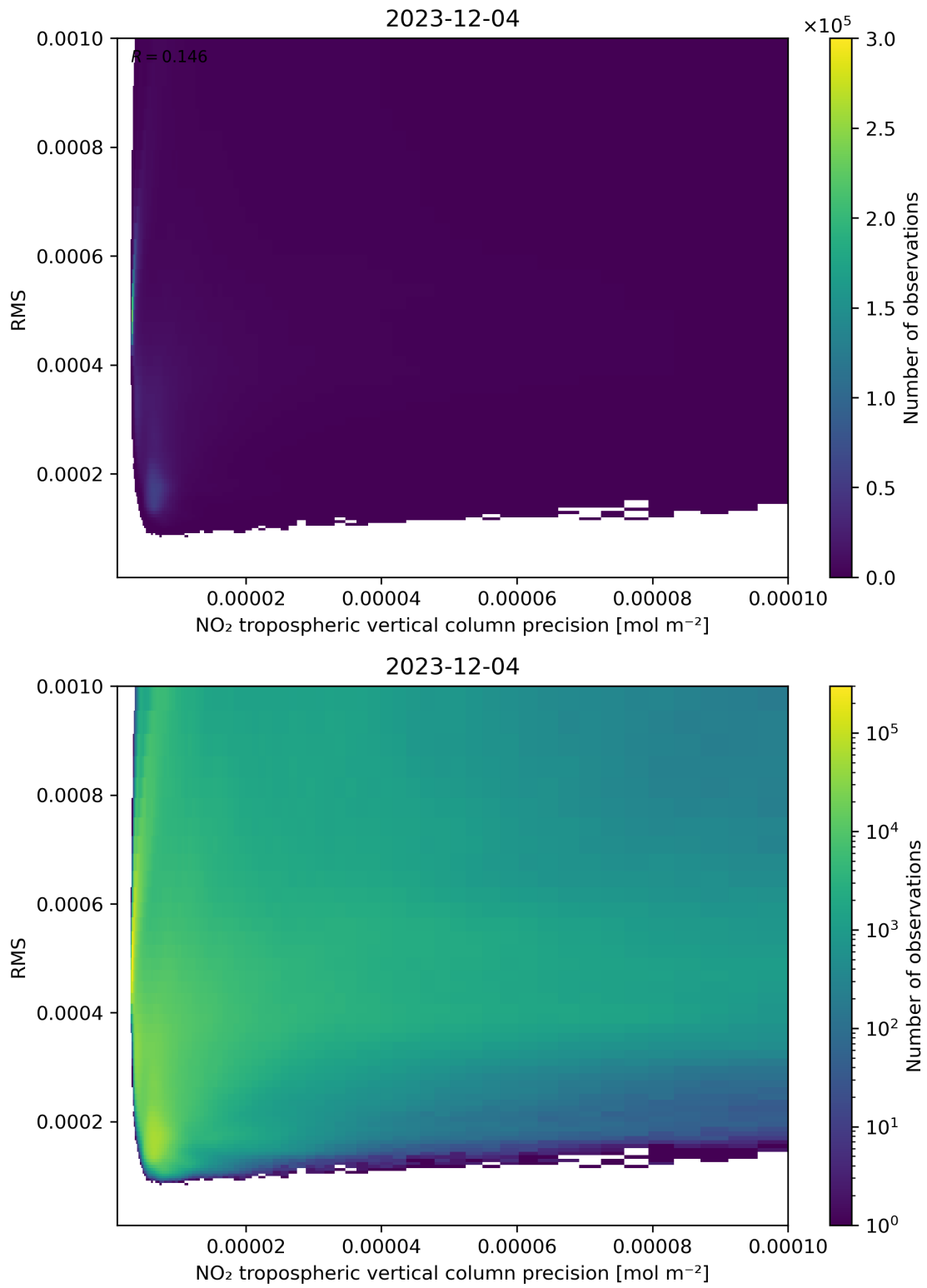
Figure 140: Scatter density plot of “NO 2 tropospheric vertical column precision” against “RMS” for 2023-12-04 to 2023-12-05.
