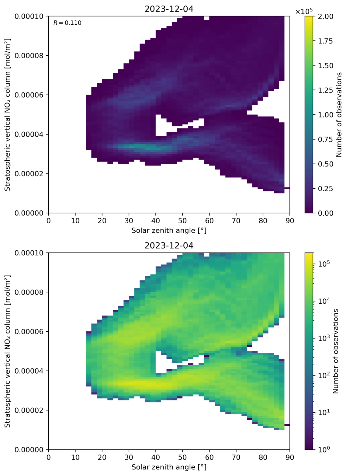
Figure 150: Scatter density plot of “Solar zenith angle” against “Stratospheric vertical NO 2 column” for 2023-12-04 to 2023-12-05.
