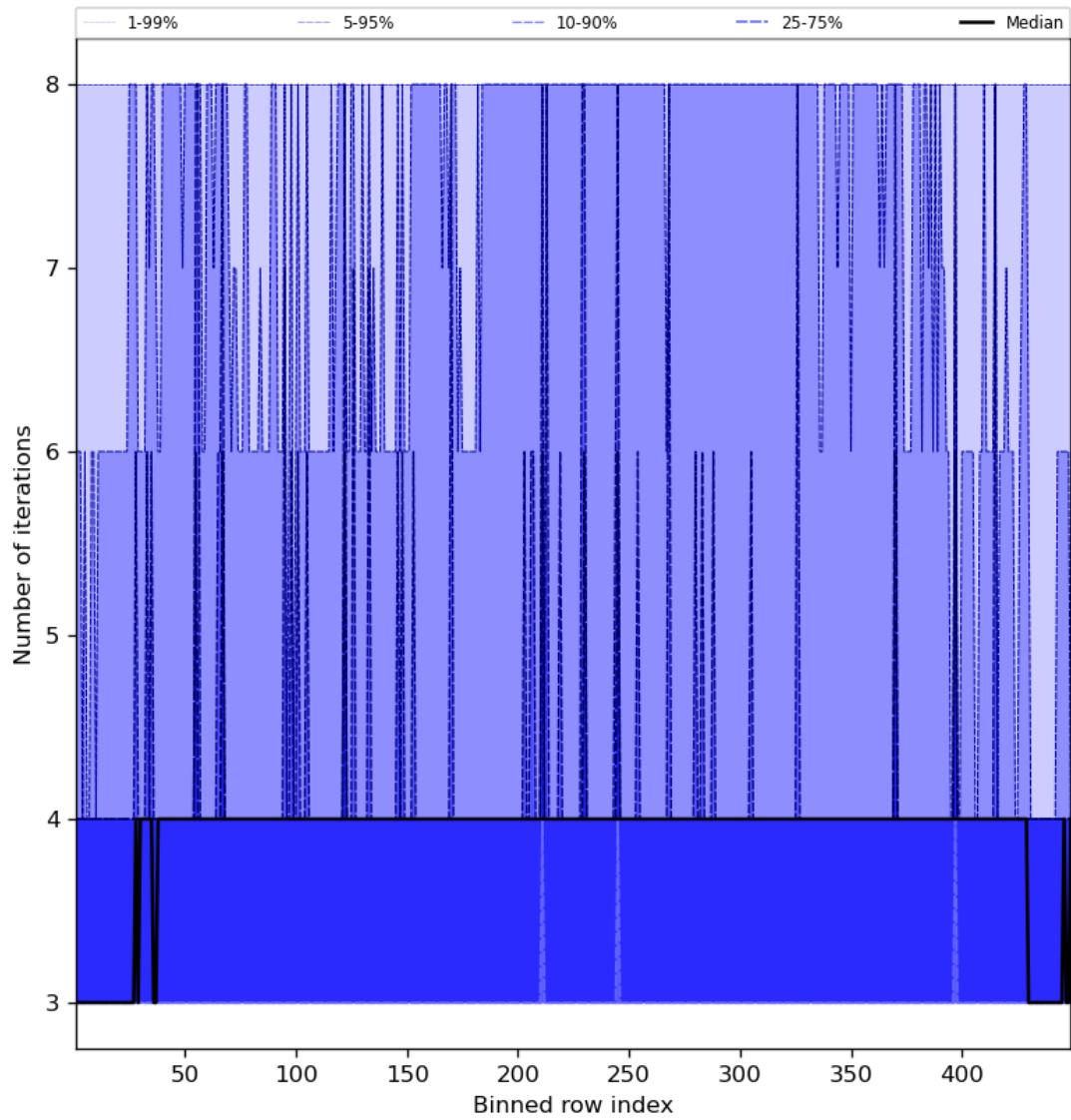
Figure 51: Along track statistics of “Number of iterations” for 2023-12-04 to 2023-12-05
