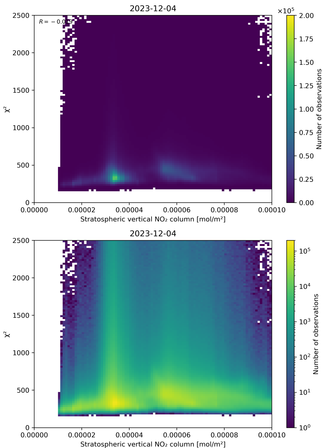
Figure 97: Scatter density plot of “Stratospheric vertical NO 2 column” against “ \chi^2 ” for 2023-12-04 to 2023-12-05.
