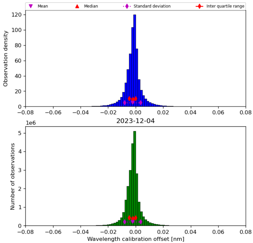
Figure 35: Histogram of “Wavelength calibration offset” for 2023-12-04 to 2023-12-05
