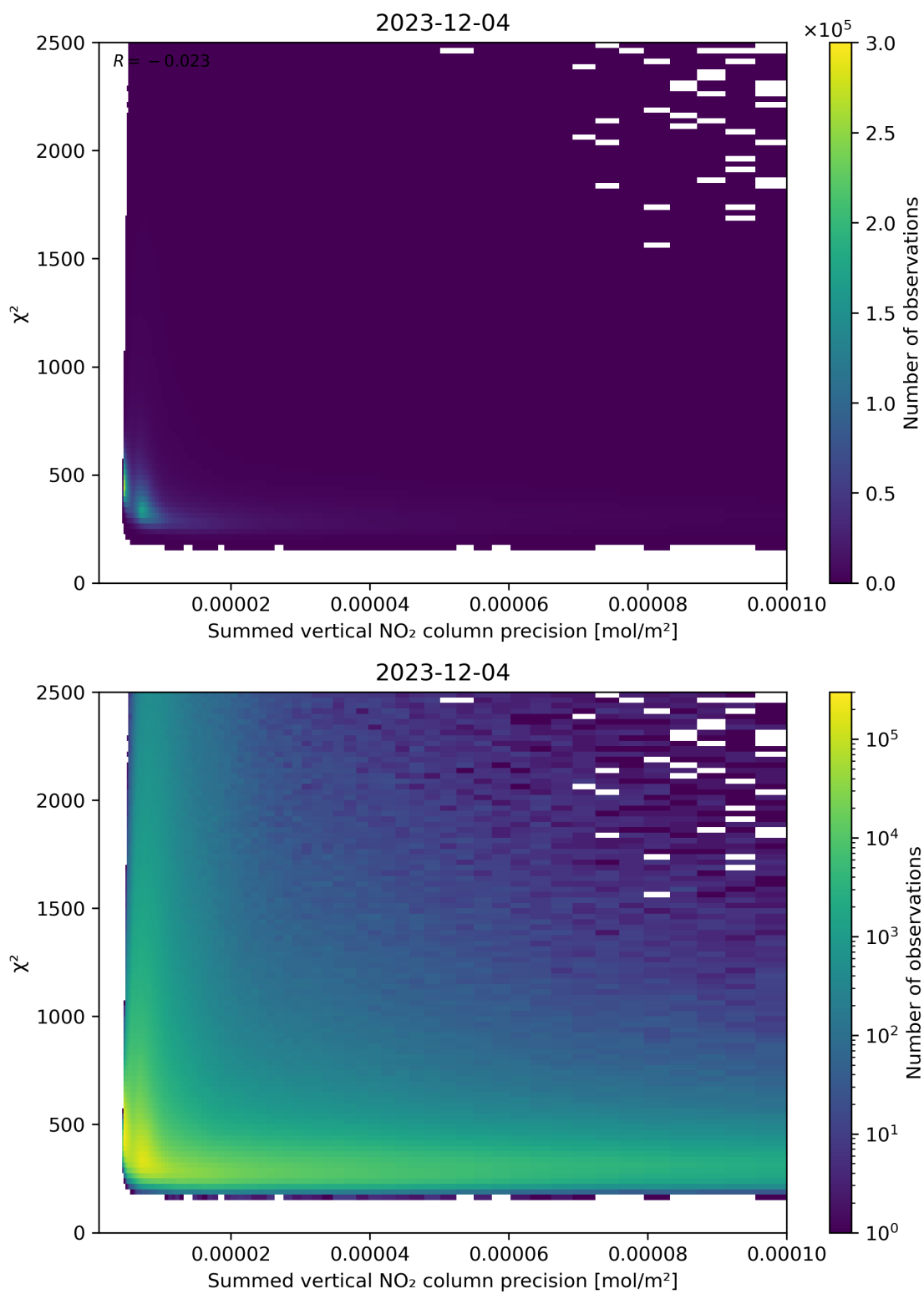
Figure 107: Scatter density plot of “Summed vertical NO 2 column precision” against “ \chi^2 ” for 2023-12-04 to 2023-12-05.
