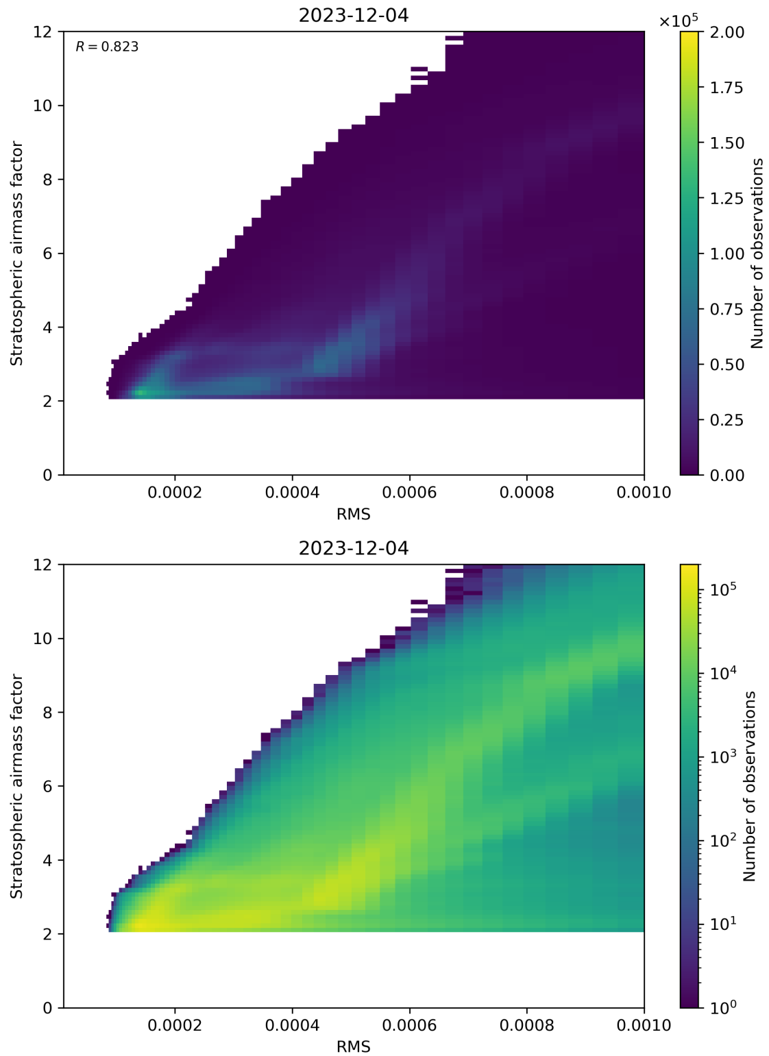
Figure 144: Scatter density plot of “RMS” against “Stratospheric airmass factor” for 2023-12-04 to 2023-12-05.
