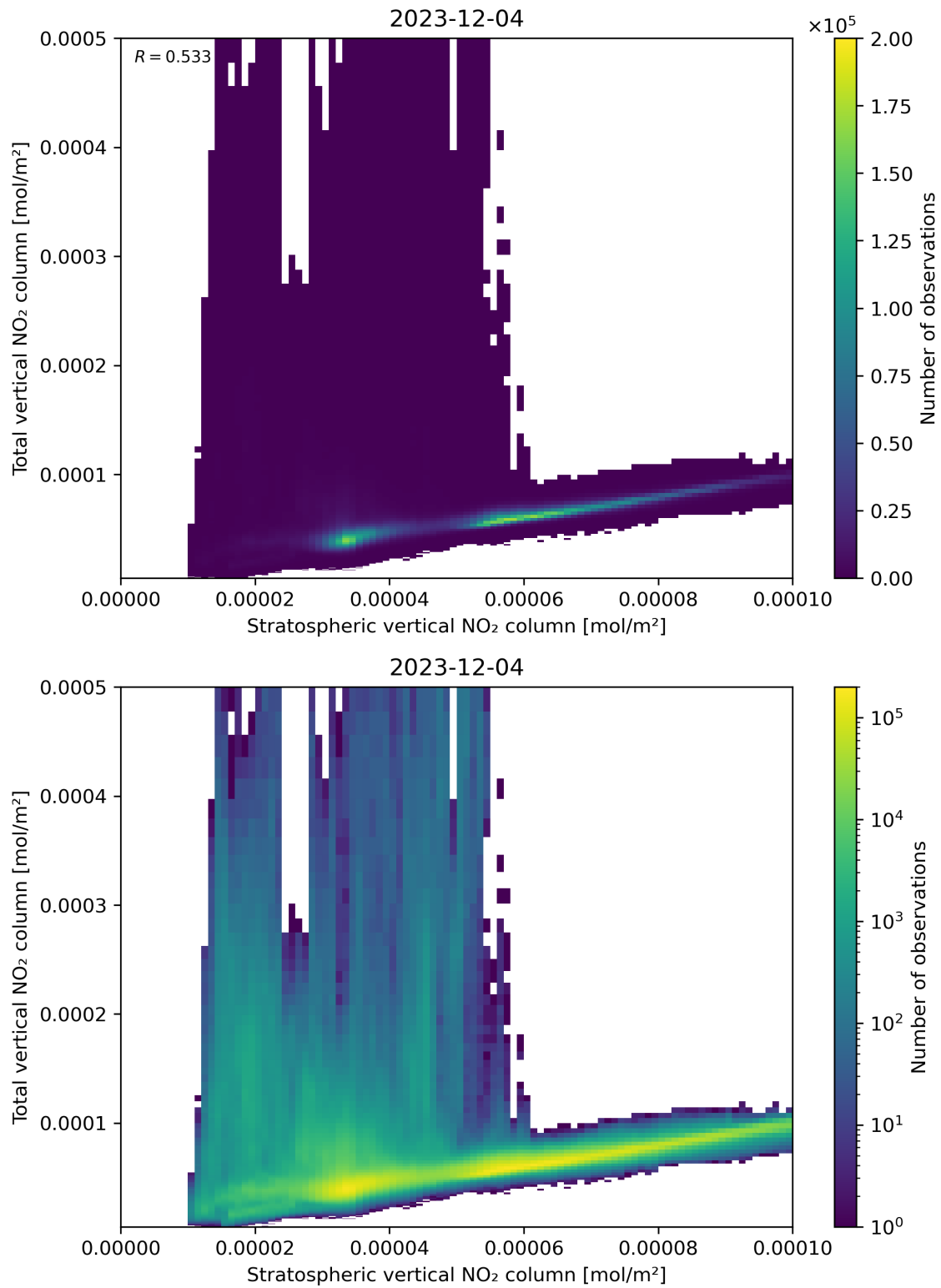
Figure 100: Scatter density plot of “Stratospheric vertical NO 2 column” against “Total vertical NO 2 column” for 2023-12-04 to 2023-12-05.
