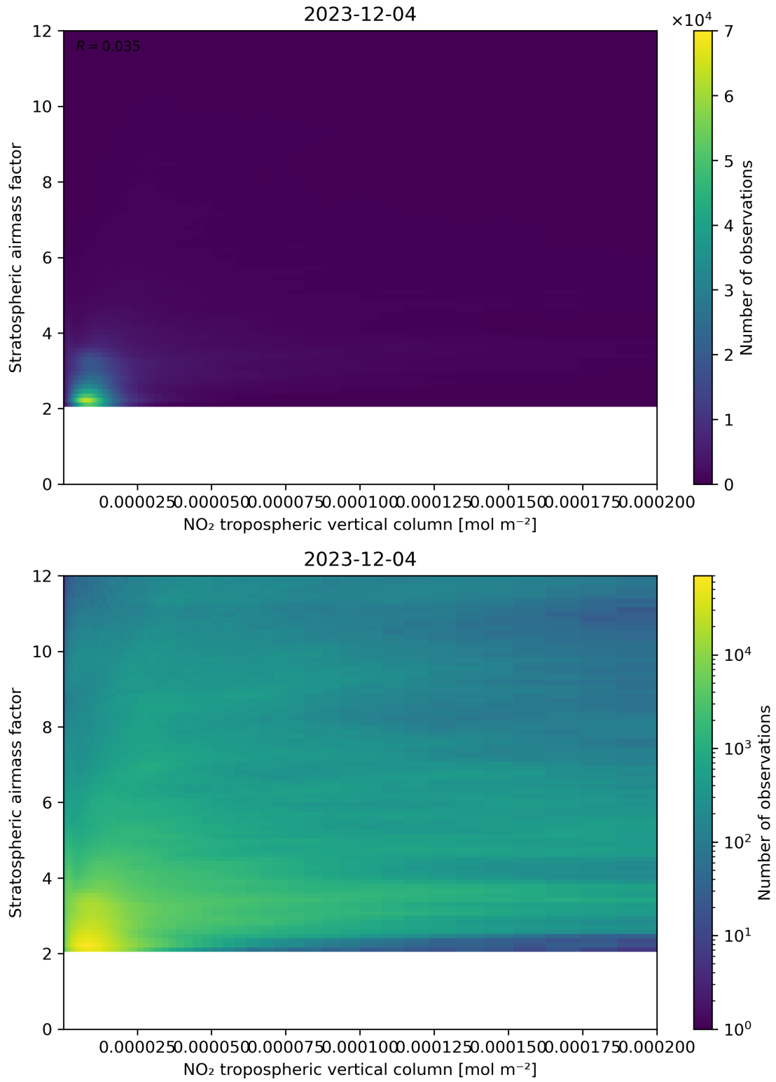
Figure 121: Scatter density plot of “NO 2 tropospheric vertical column” against “Stratospheric airmass factor” for 2023-12-04 to 2023-12-05.
