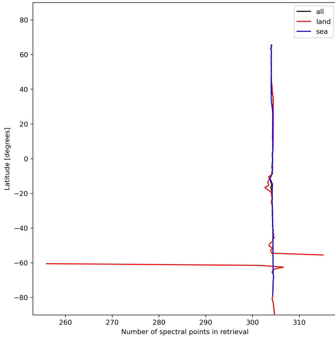
Figure 16: Zonal average of “Number of spectral points in retrieval” for 2023-12-04 to 2023-12-05.
