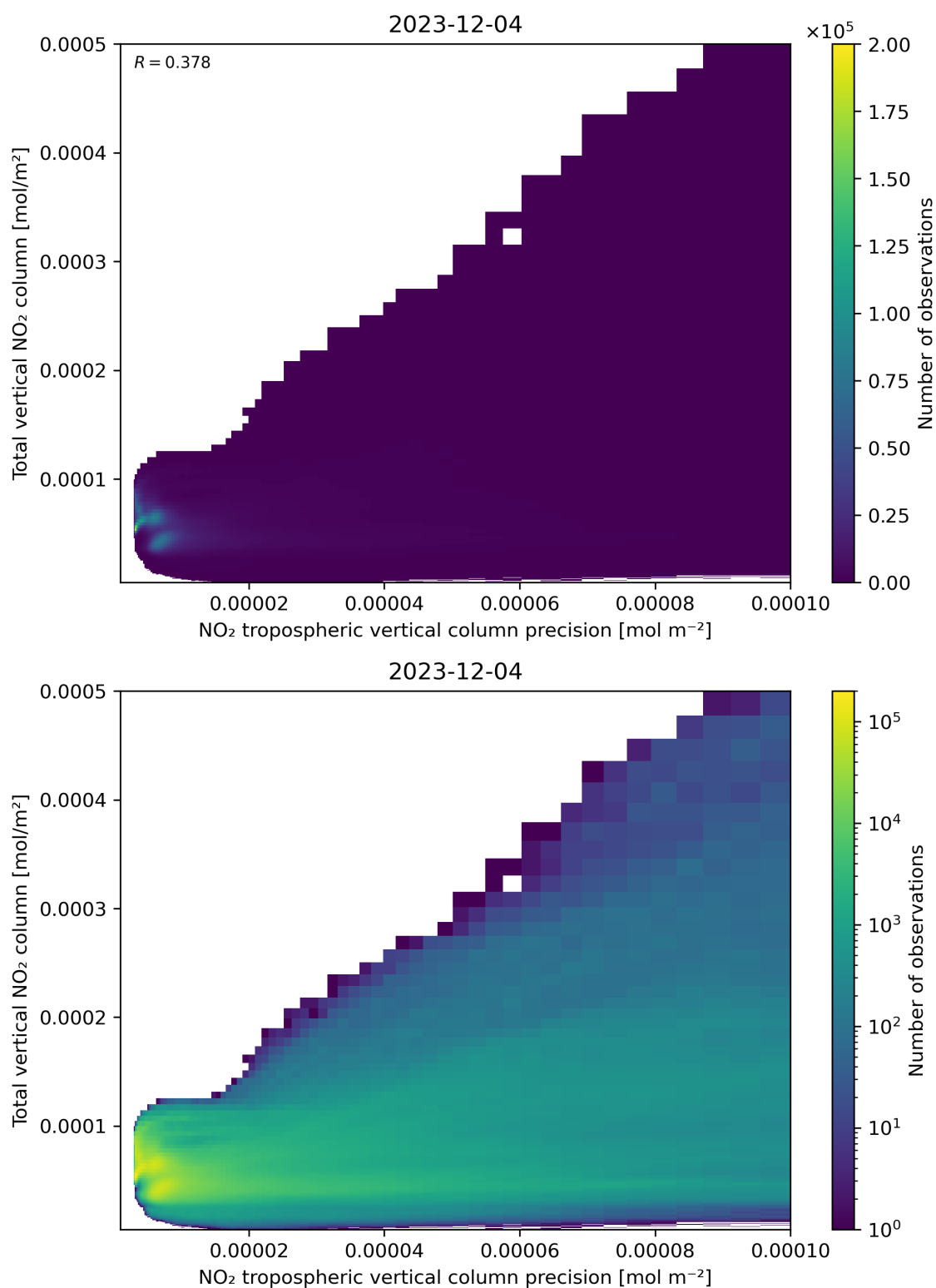
Figure 138: Scatter density plot of “NO 2 tropospheric vertical column precision” against “Total vertical NO 2 column” for 2023-12-04 to 2023-12-05.
