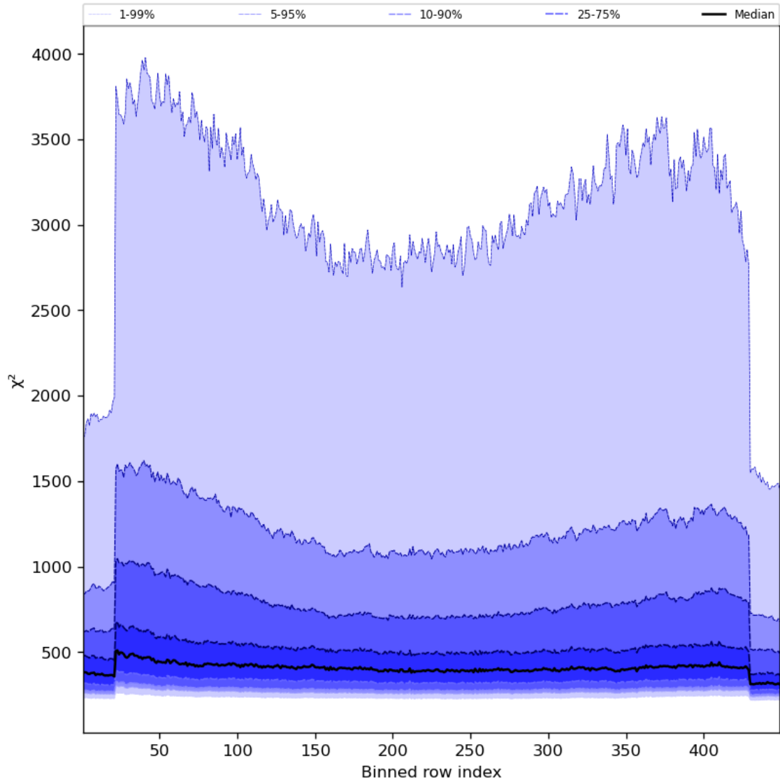
Figure 59: Along track statistics of “ \chi^2 ” for 2023-12-04 to 2023-12-05
