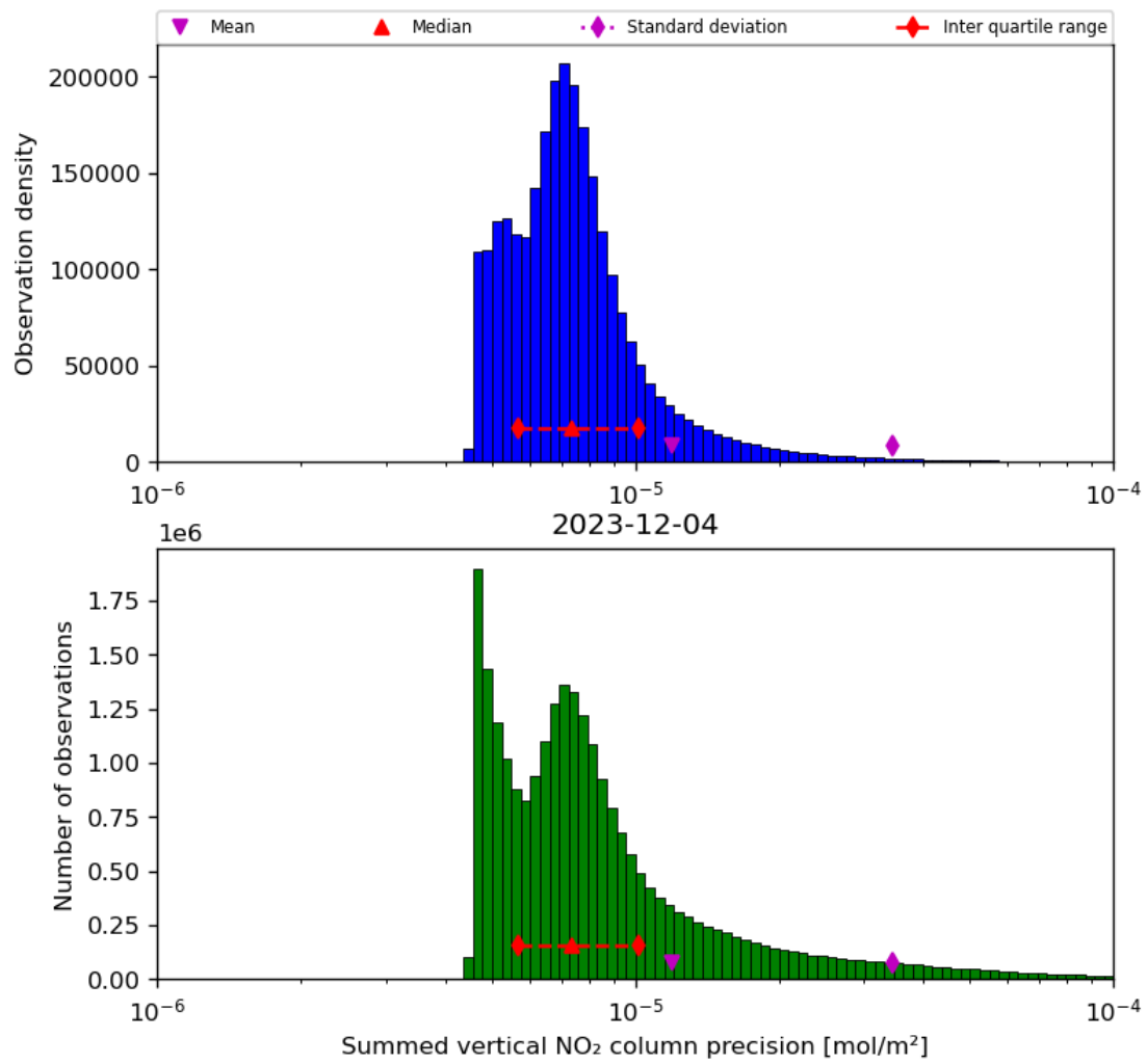
Figure 41: Histogram of “Summed vertical NO 2 column precision” for 2023-12-04 to 2023-12-05
