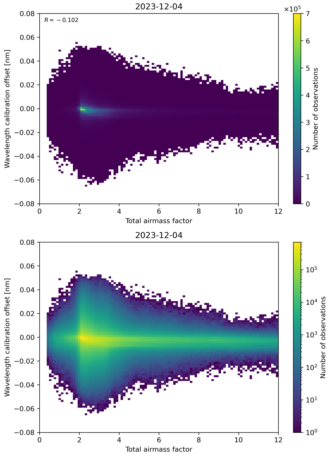
Figure 70: Scatter density plot of “Total airmass factor” against “Wavelength calibration offset” for 2023-12-04 to 2023-12-05.
