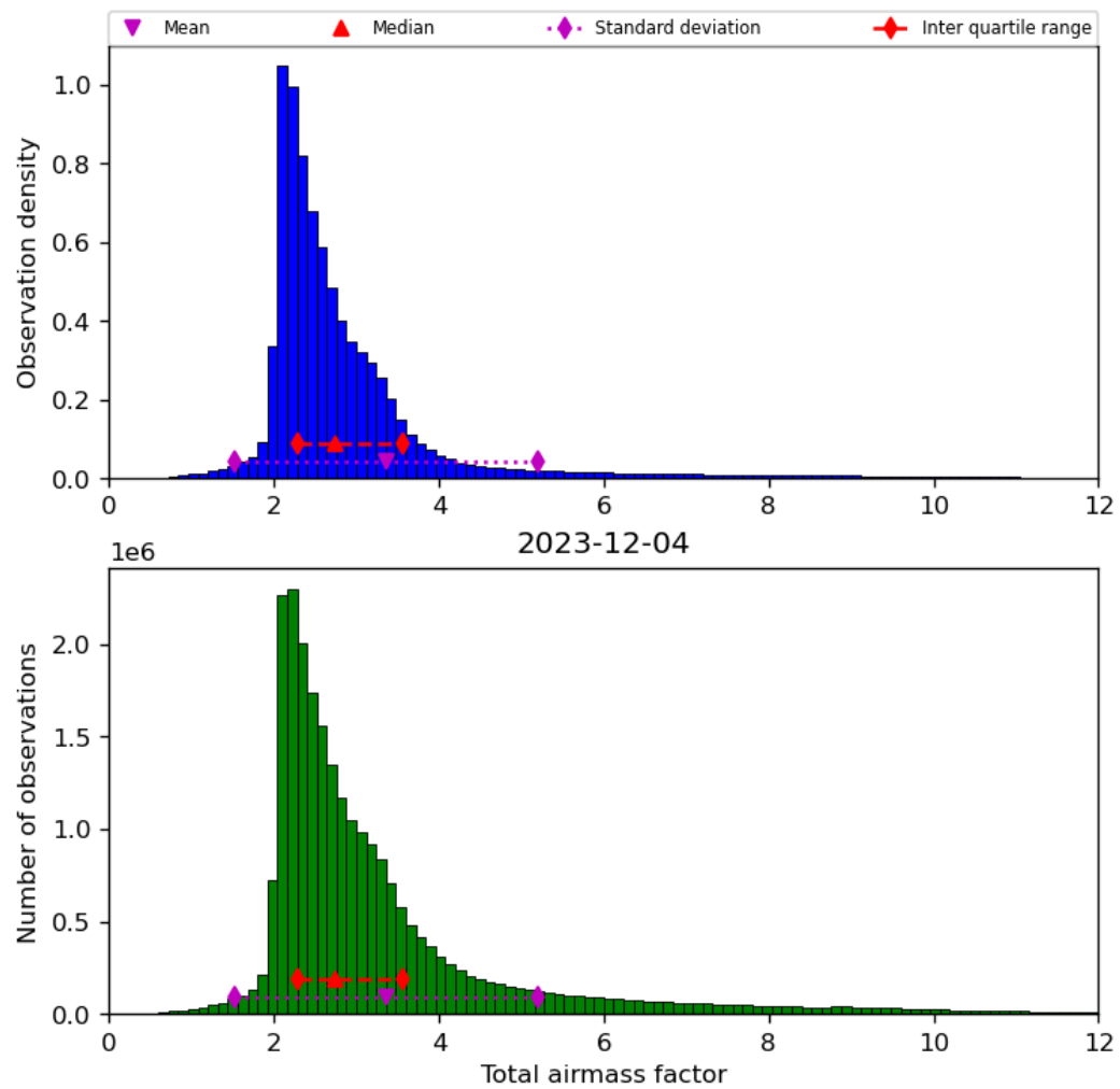
Figure 32: Histogram of “Total airmass factor” for 2023-12-04 to 2023-12-05
