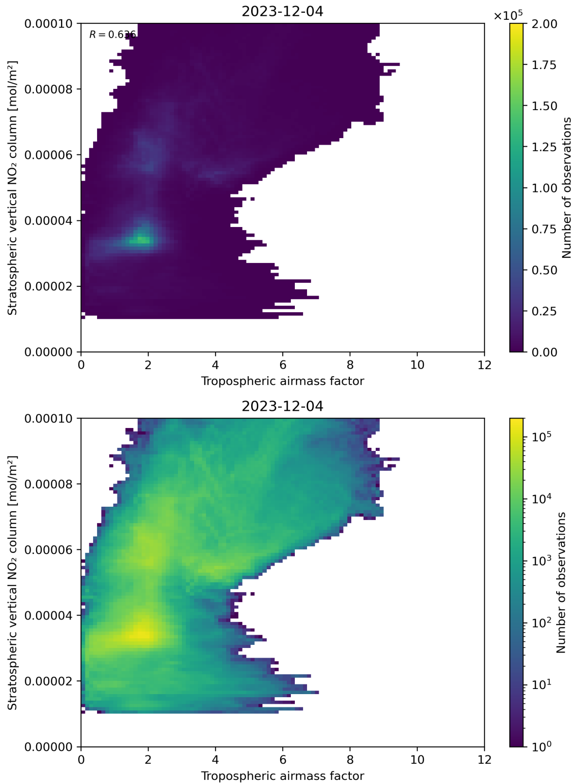
Figure 74: Scatter density plot of “Tropospheric air mass factor” against “Stratospheric vertical NO 2 column” for 2023-12-04 to 2023-12-05.
