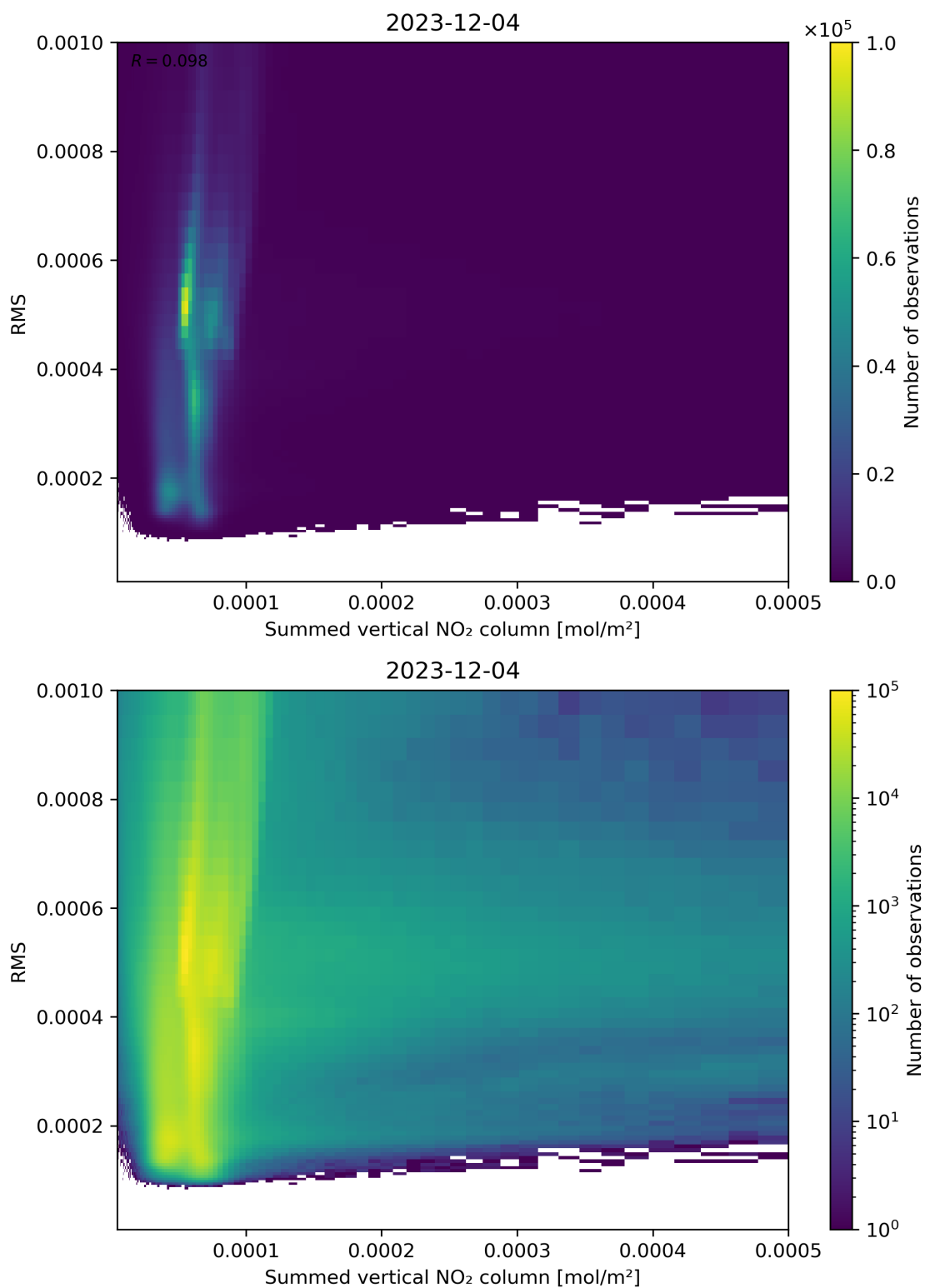
Figure 109: Scatter density plot of “Summed vertical NO 2 column” against “RMS” for 2023-12-04 to 2023-12-05.
