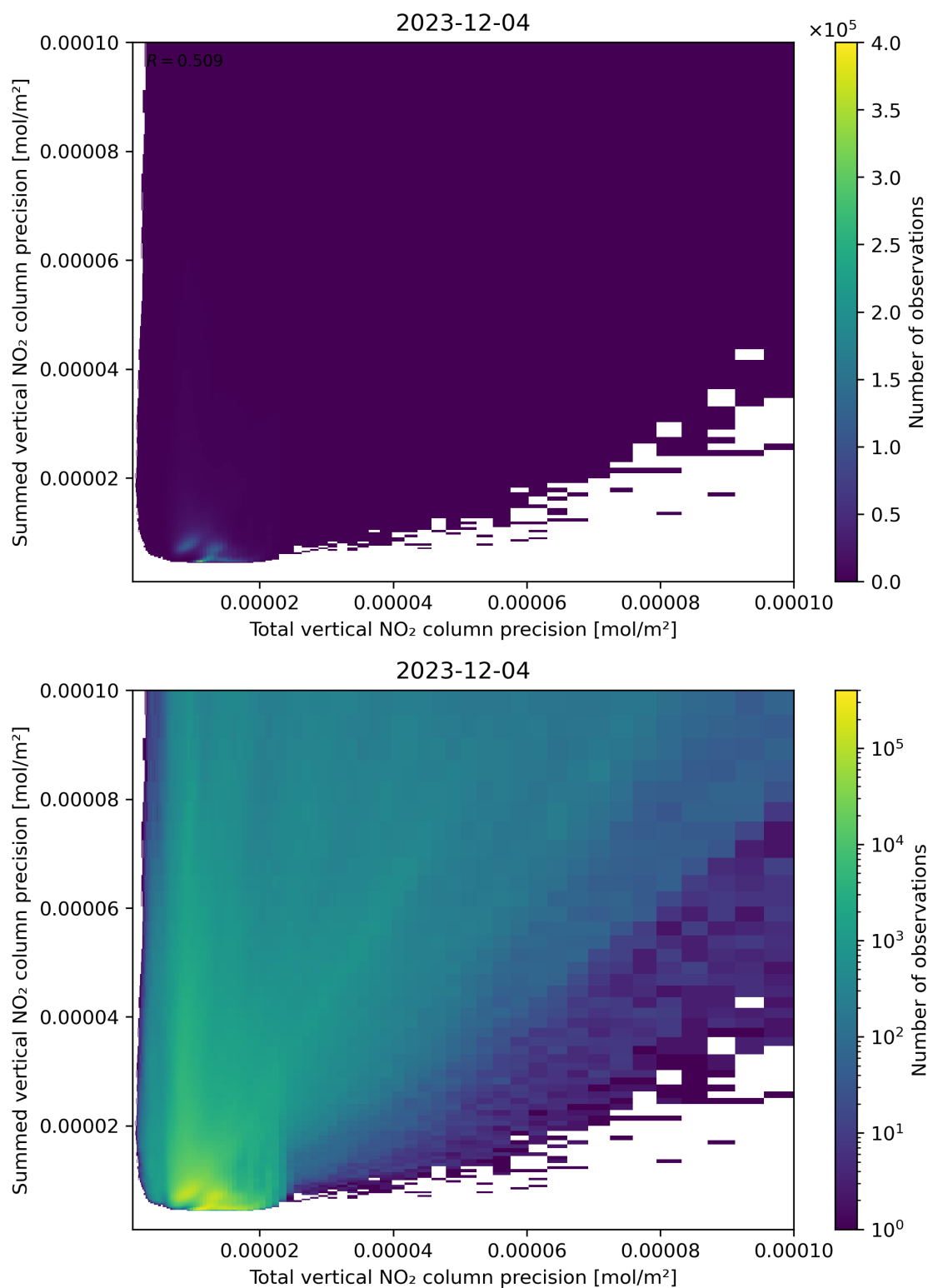
Figure 118: Scatter density plot of “Total vertical NO 2 column precision” against “Summed vertical NO 2 column precision” for 2023-12-04 to 2023-12-05.
