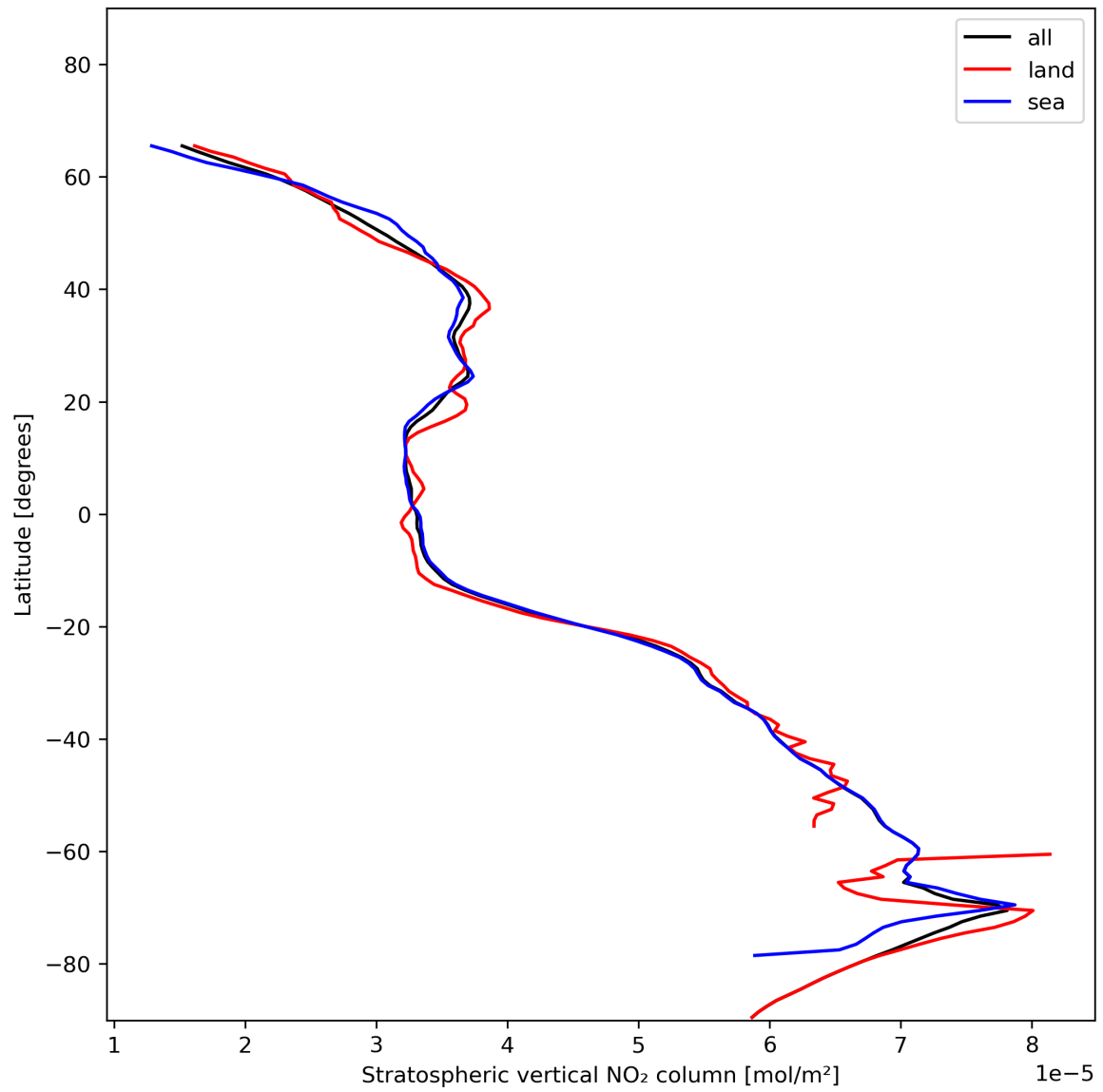
Figure 19: Zonal average of “Stratospheric vertical NO 2 column” for 2023-12-04 to 2023-12-05.
