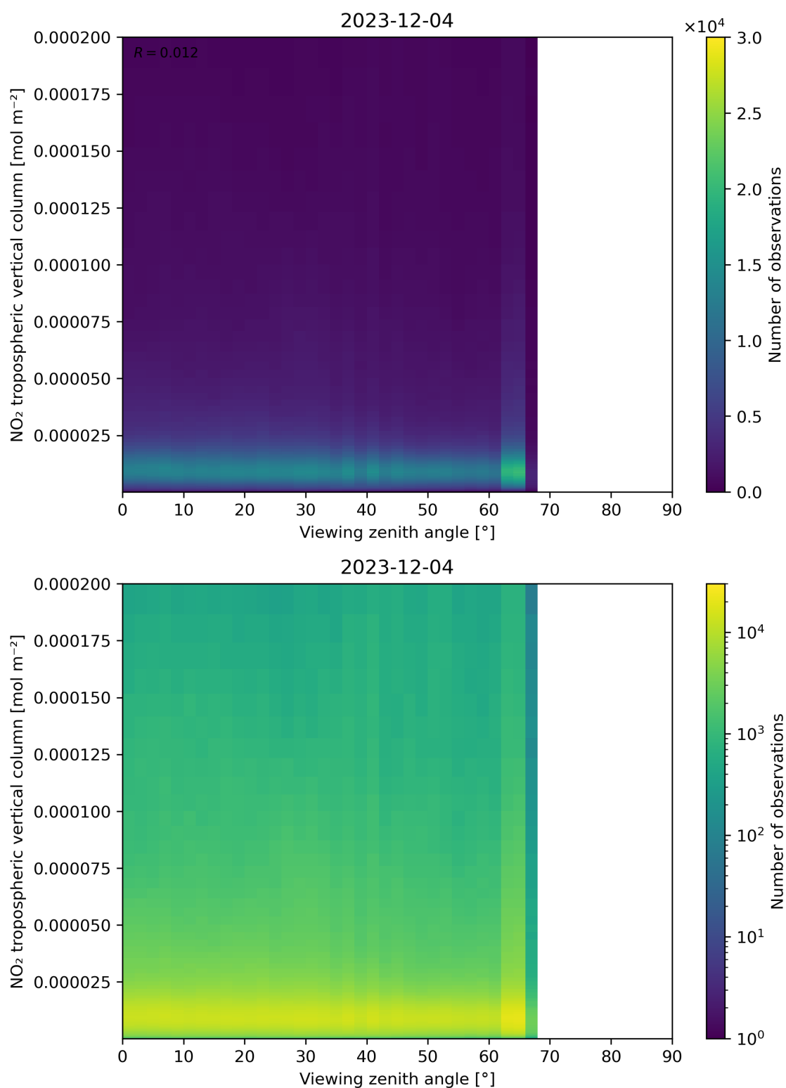
Figure 169: Scatter density plot of “Viewing zenith angle” against “NO 2 tropospheric vertical column” for 2023-12-04 to 2023-12-05.
