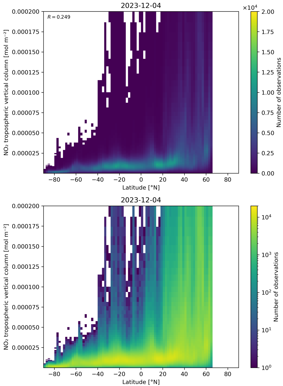
Figure 92: Scatter density plot of “Latitude” against “NO 2 tropospheric vertical column” for 2023-12-04 to 2023-12-05.
