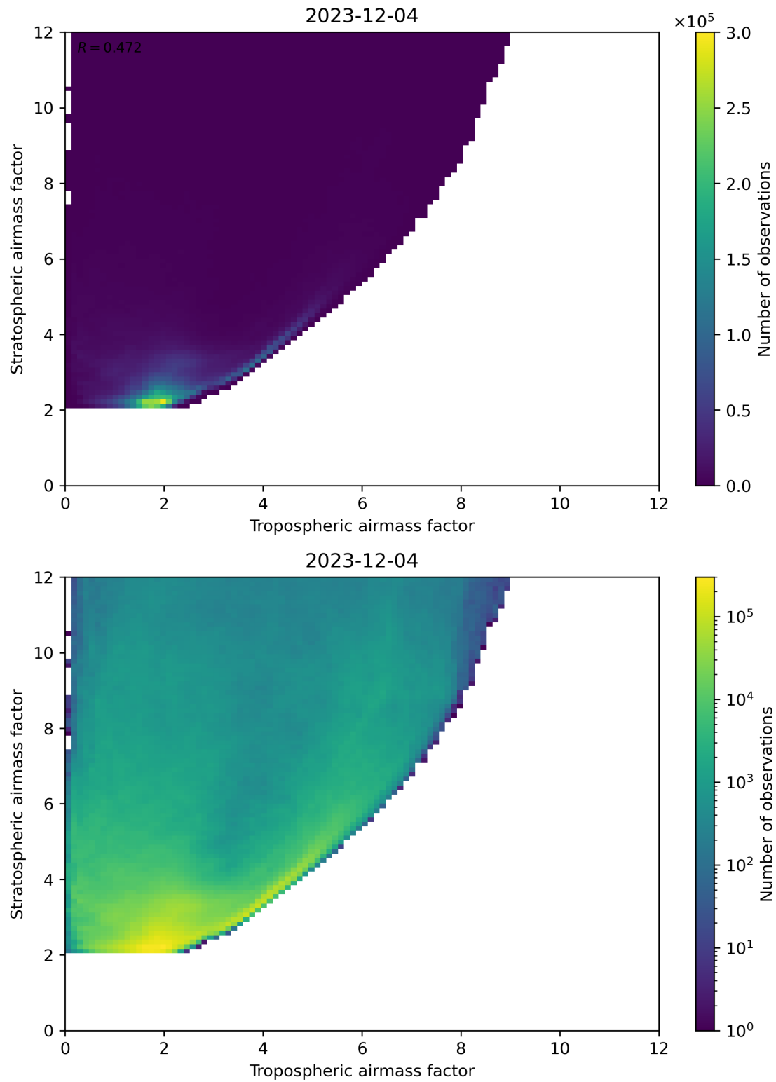
Figure 71: Scatter density plot of “Tropospheric airmass factor” against “Stratospheric airmass factor” for 2023-12-04 to 2023-12-05.
