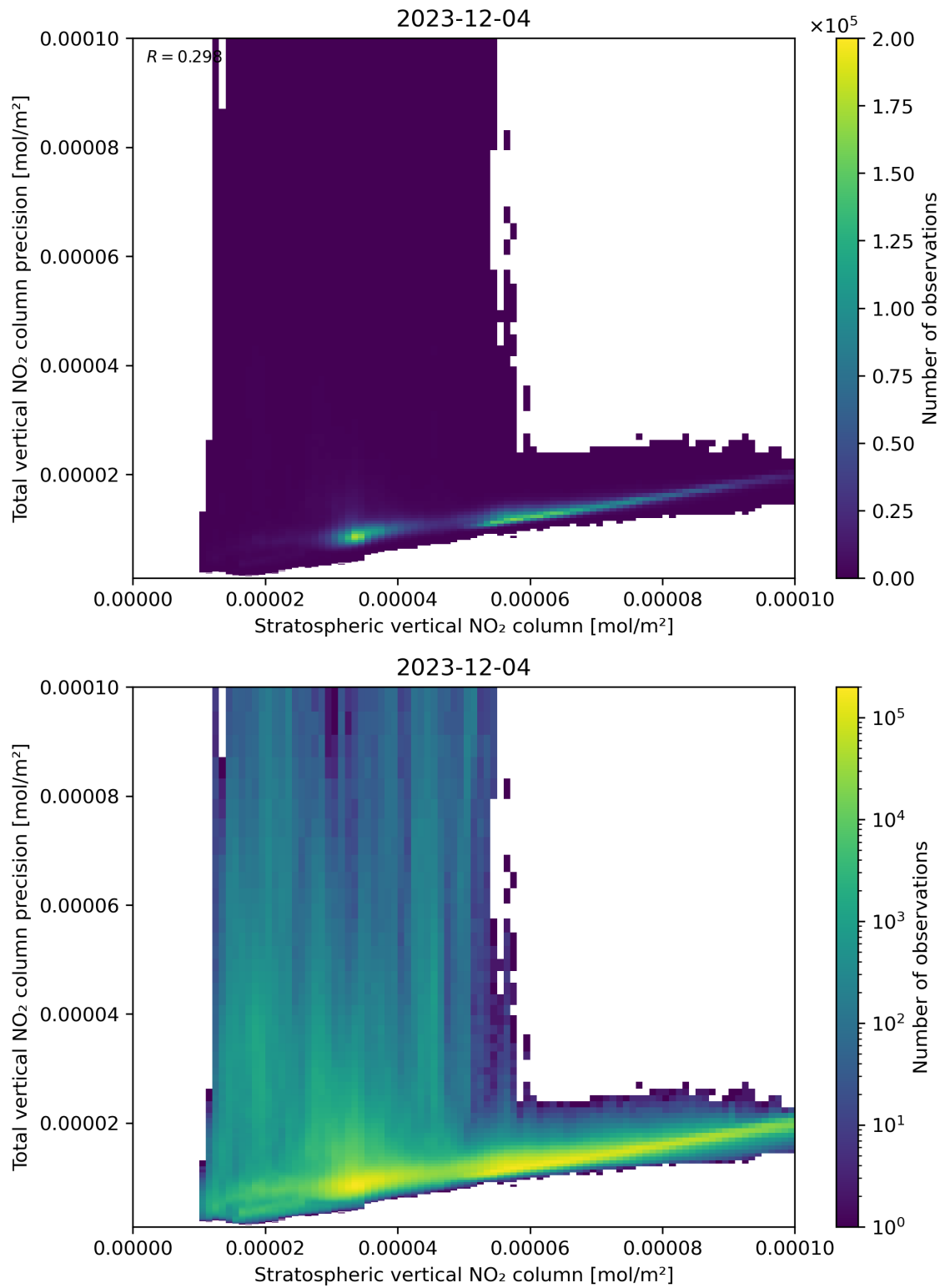
Figure 101: Scatter density plot of “Stratospheric vertical NO 2 column” against “Total vertical NO 2 column precision” for 2023-12-04 to 2023-12-05.
