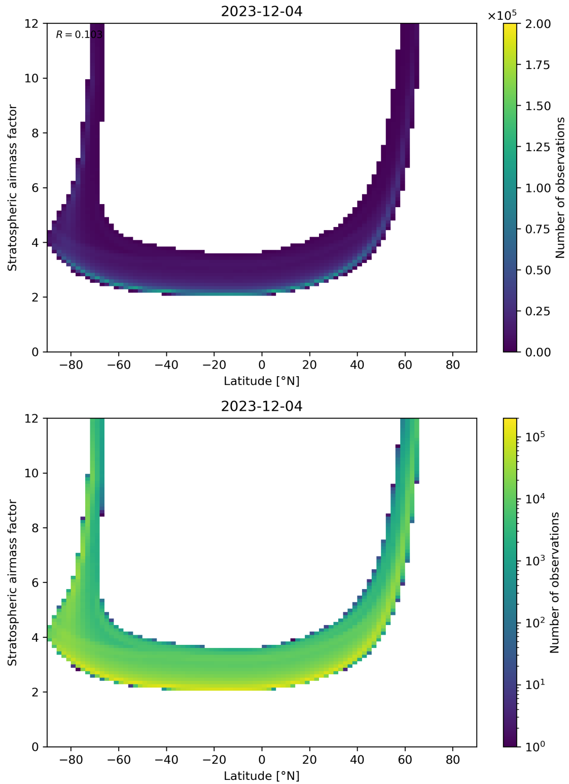
Figure 83: Scatter density plot of “Latitude” against “Stratospheric airmass factor” for 2023-12-04 to 2023-12-05.
