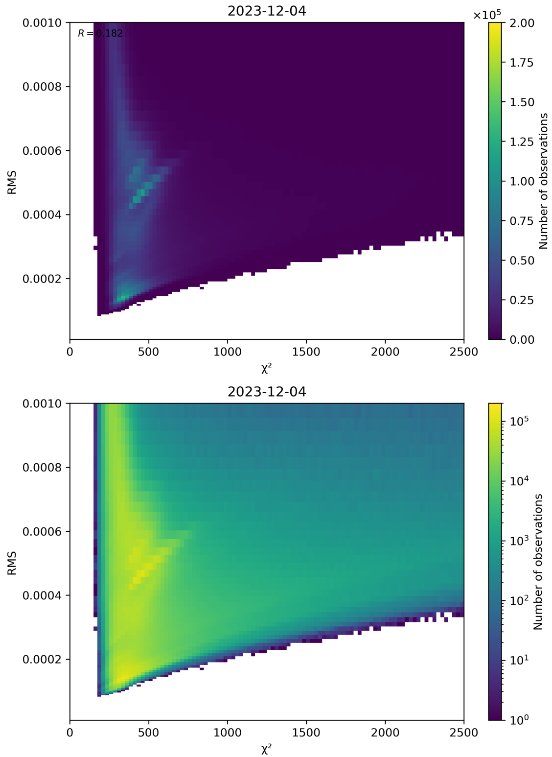
Figure 82: Scatter density plot of “ \chi^2 ” against “RMS” for 2023-12-04 to 2023-12-05.
