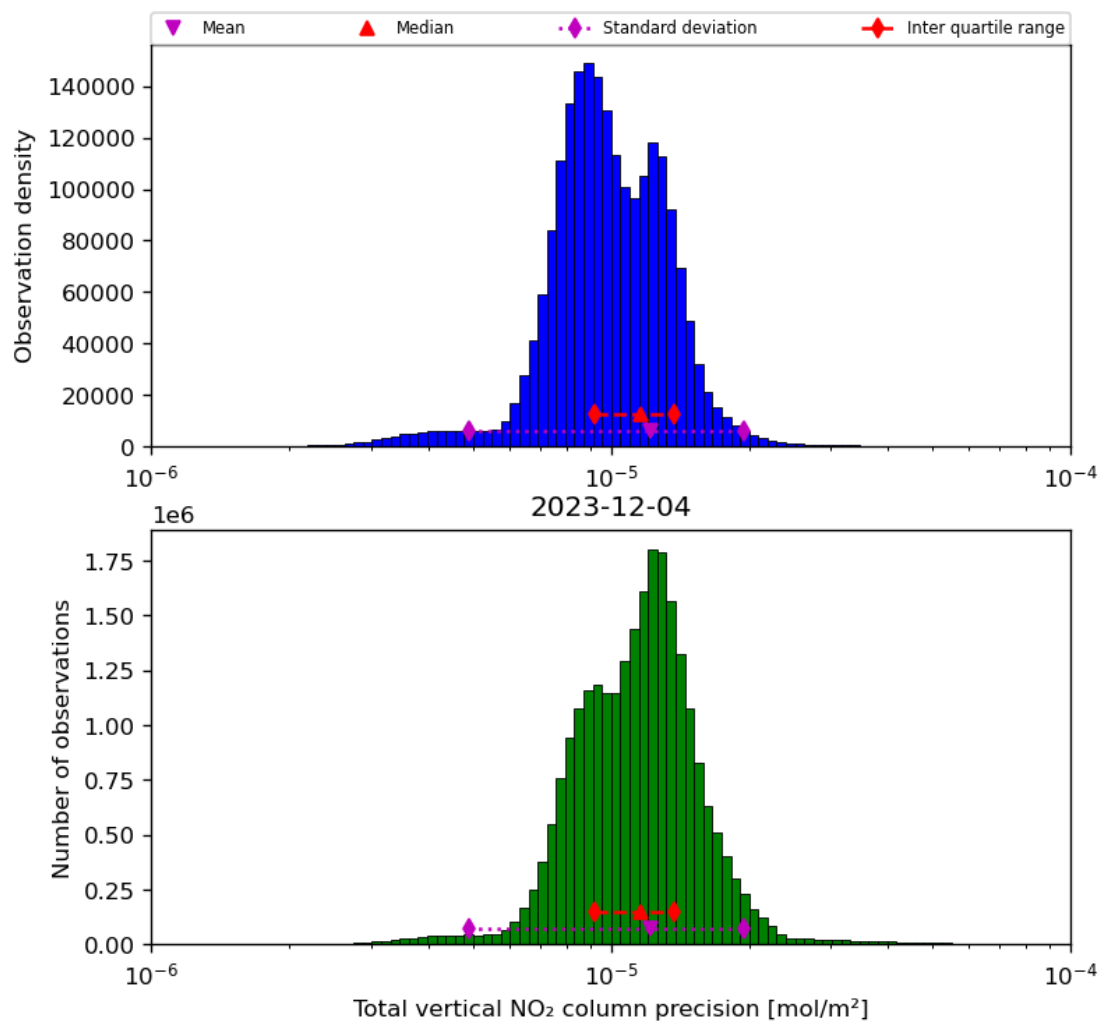
Figure 39: Histogram of “Total vertical NO 2 column precision” for 2023-12-04 to 2023-12-05
