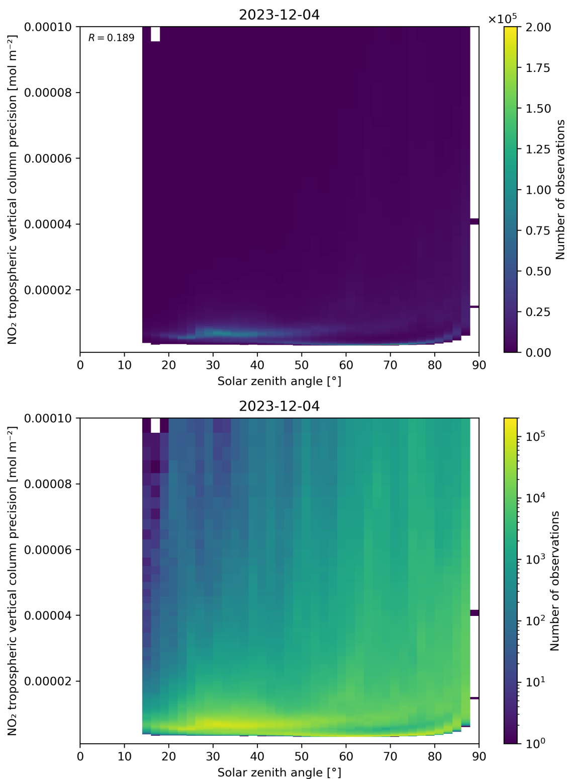
Figure 156: Scatter density plot of “Solar zenith angle” against “NO 2 tropospheric vertical column precision” for 2023-12-04 to 2023-12-05.
