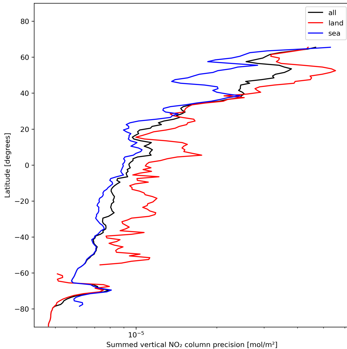
Figure 24: Zonal average of “Summed vertical NO 2 column precision” for 2023-12-04 to 2023-12-05.
