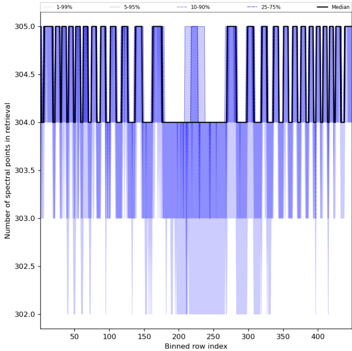
Figure 50: Along track statistics of “Number of spectral points in retrieval” for 2023-12-04 to 2023-12-05
