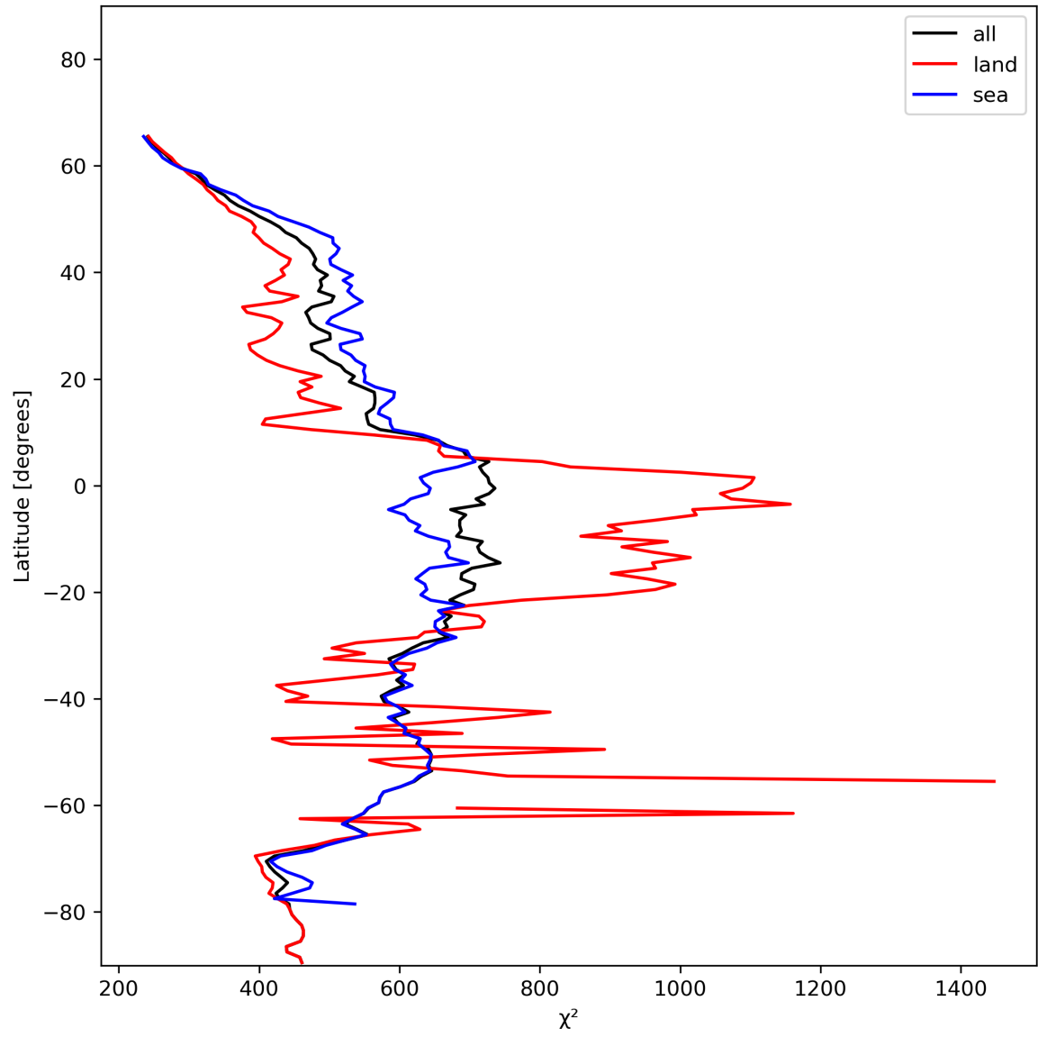
Figure 25: Zonal average of “ \chi^2 ” for 2023-12-04 to 2023-12-05.
