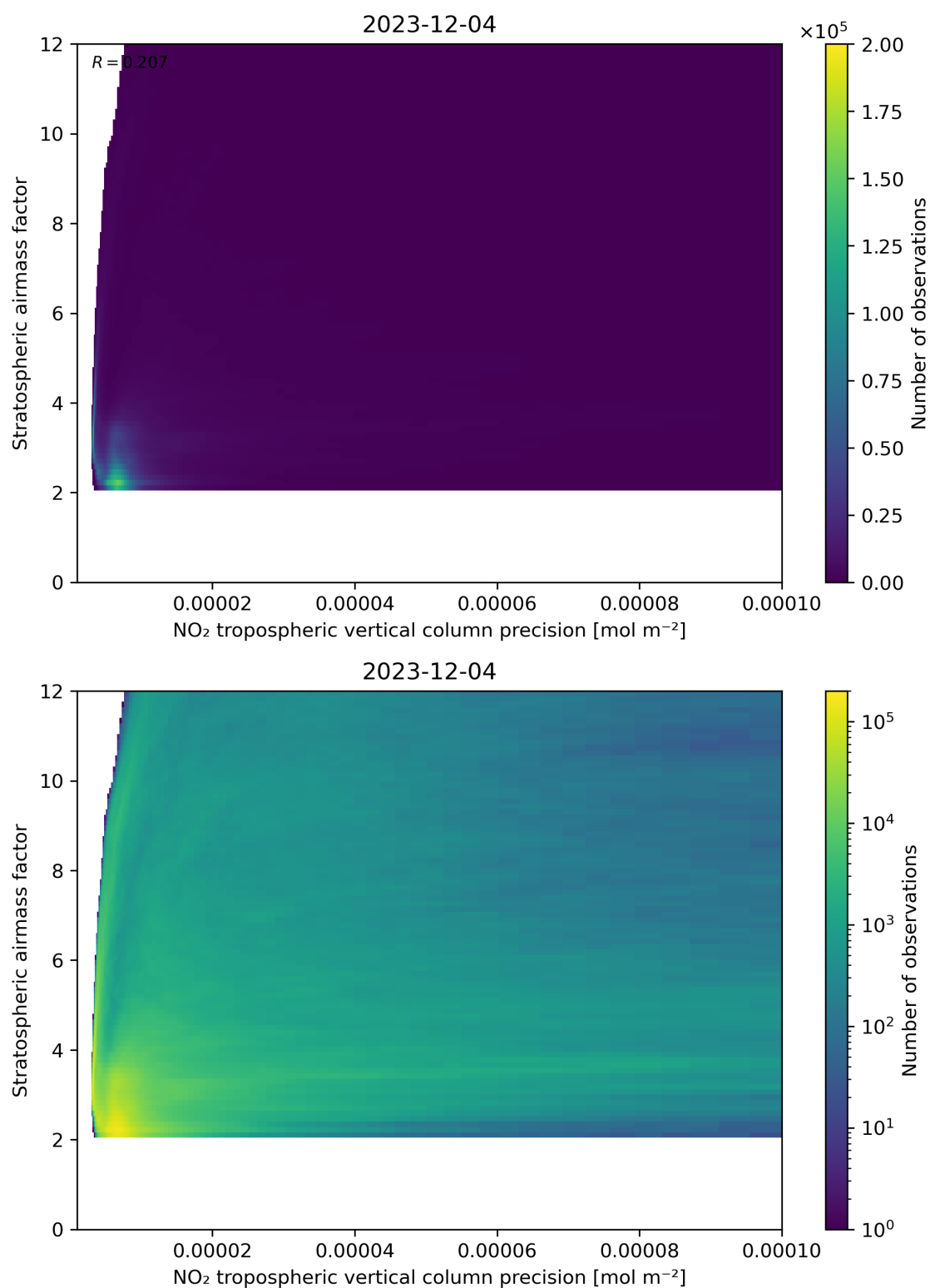
Figure 131: Scatter density plot of “NO 2 tropospheric vertical column precision” against “Stratospheric airmass factor” for 2023-12-04 to 2023-12-05.
