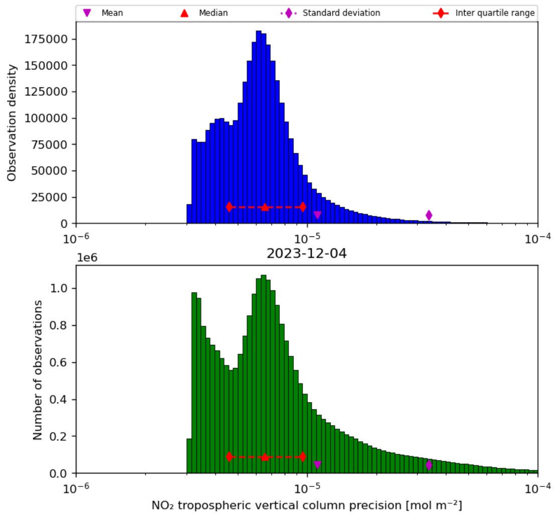
Figure 30: Histogram of “NO 2 tropospheric vertical column precision” for 2023-12-04 to 2023-12-05
