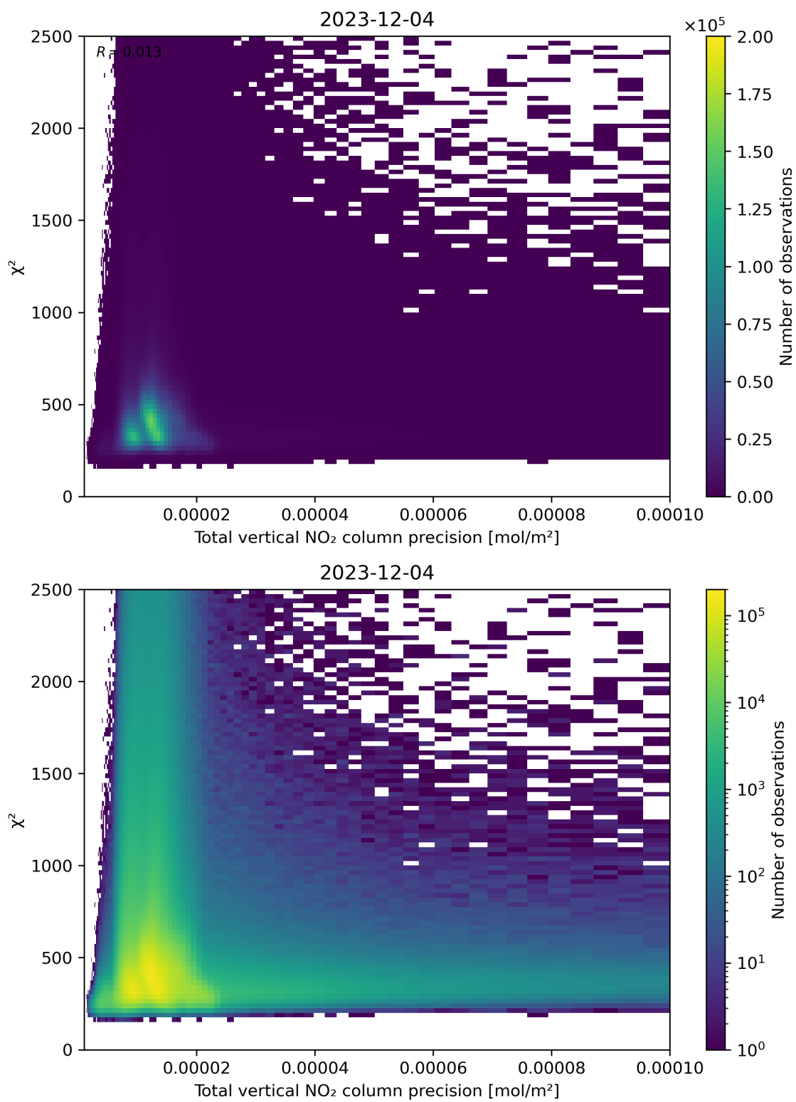
Figure 116: Scatter density plot of “Total vertical NO 2 column precision” against “ \chi^2 ” for 2023-12-04 to 2023-12-05.
