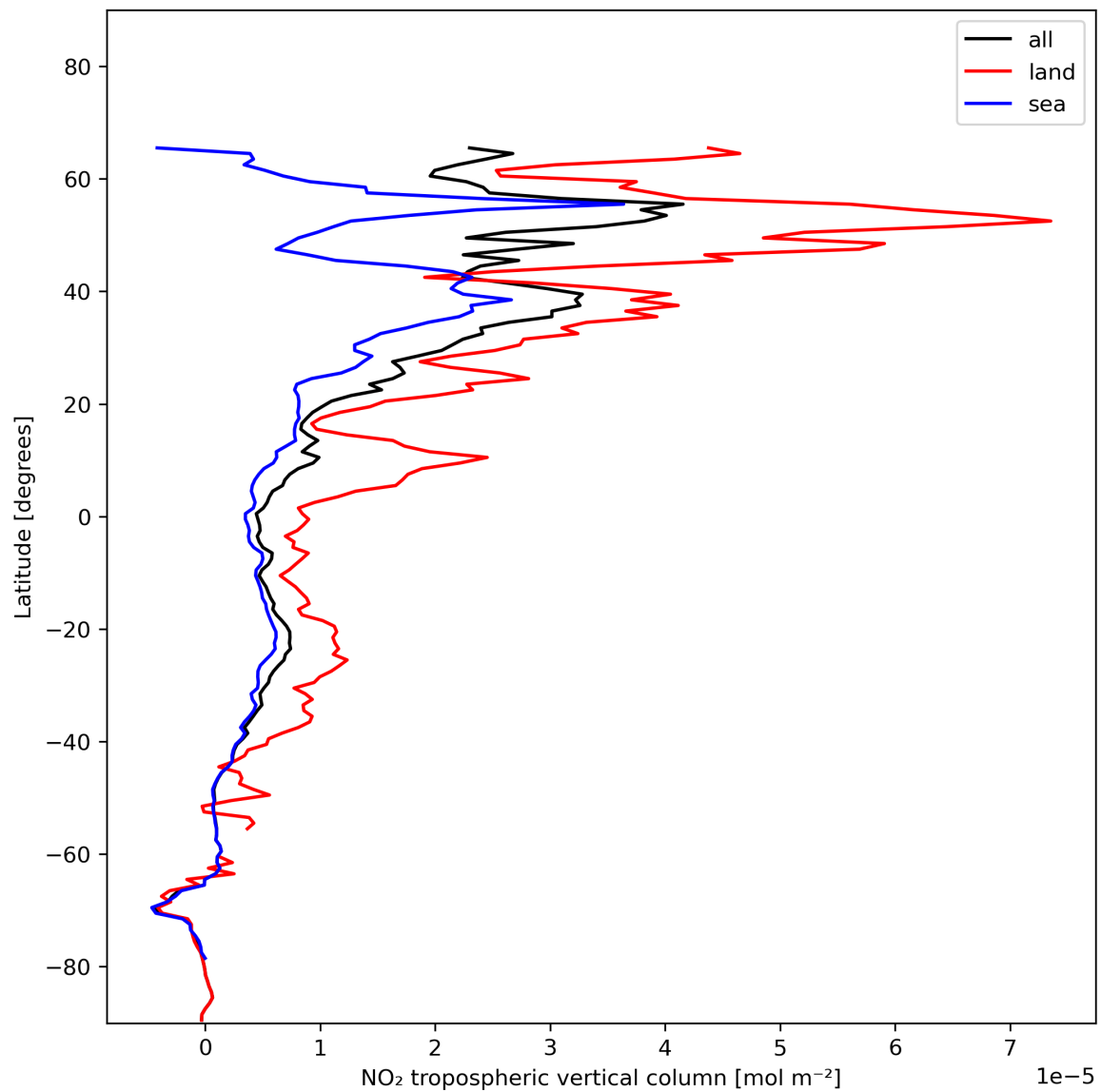
Figure 12: Zonal average of “NO 2 tropospheric vertical column” for 2023-12-04 to 2023-12-05.
