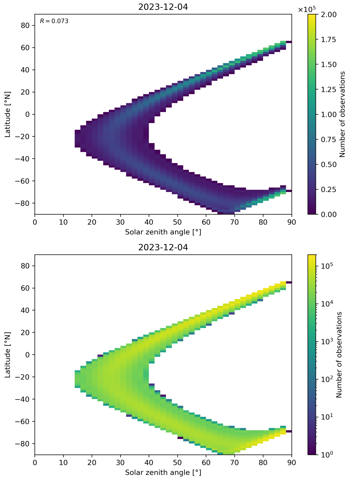
Figure 149: Scatter density plot of “Solar zenith angle” against “Latitude” for 2023-12-04 to 2023-12-05.
