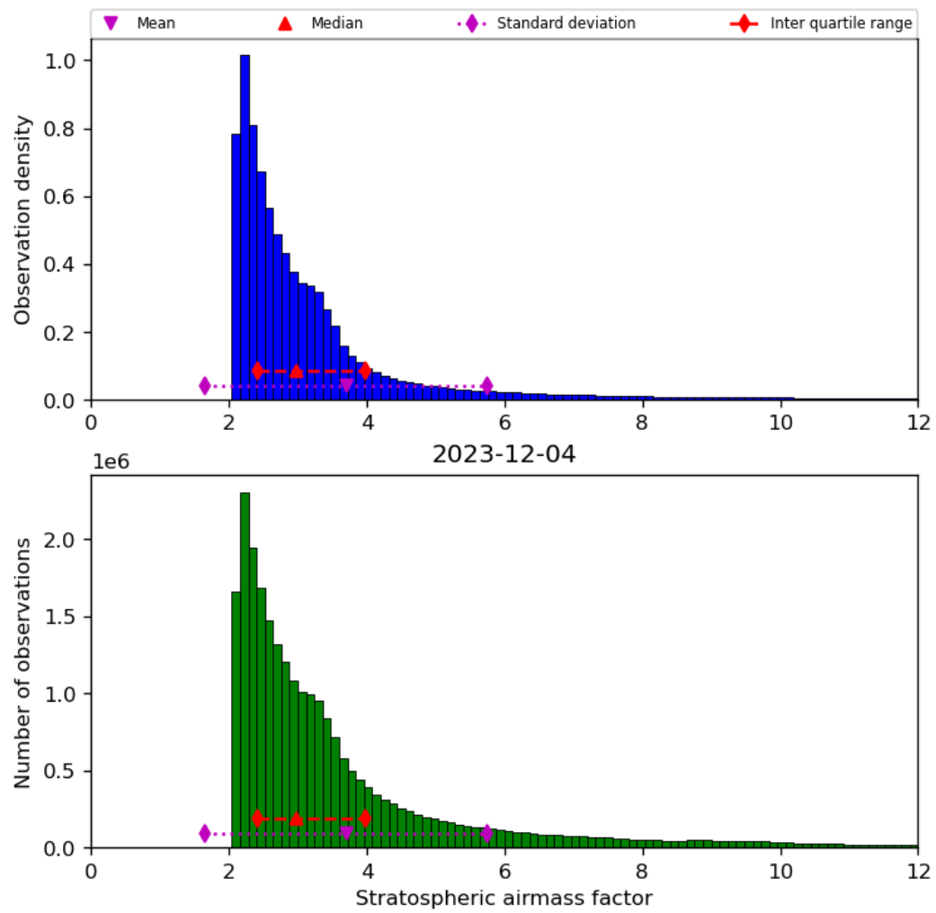
Figure 44: Histogram of “Stratospheric airmass factor” for 2023-12-04 to 2023-12-05
