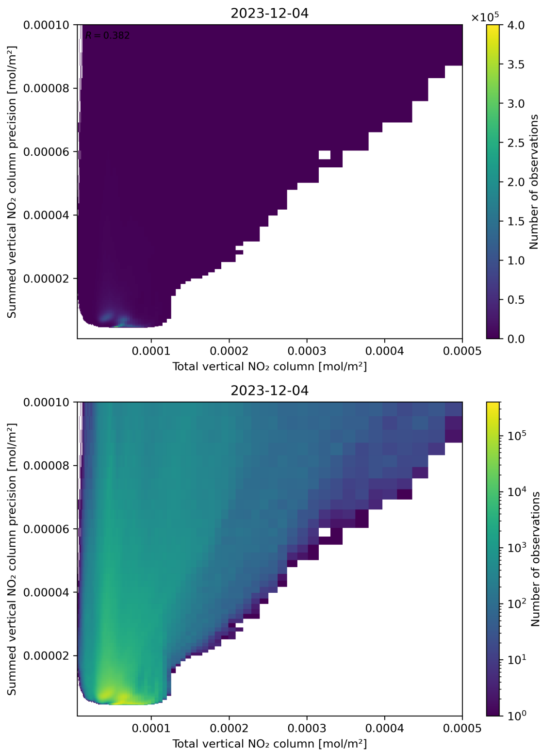
Figure 113: Scatter density plot of “Total vertical NO 2 column” against “Summed vertical NO 2 column precision” for 2023-12-04 to 2023-12-05.
