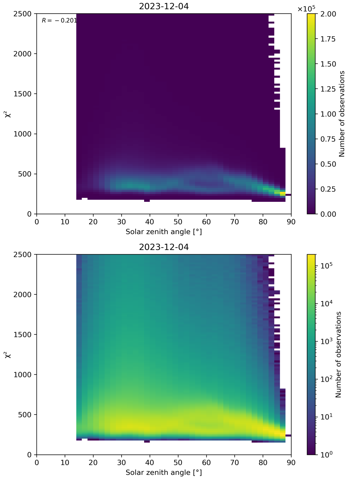
Figure 148: Scatter density plot of “Solar zenith angle” against “ \chi^2 ” for 2023-12-04 to 2023-12-05.
