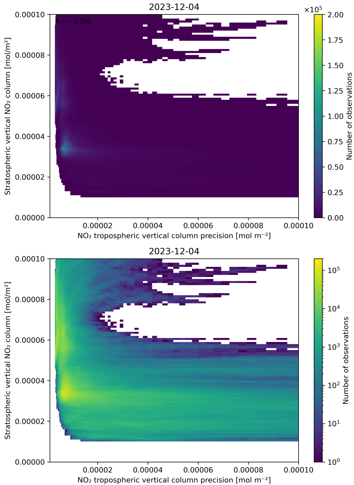
Figure 135: Scatter density plot of “NO 2 tropospheric vertical column precision” against “Stratospheric vertical NO 2 column” for 2023-12-04 to 2023-12-05.
