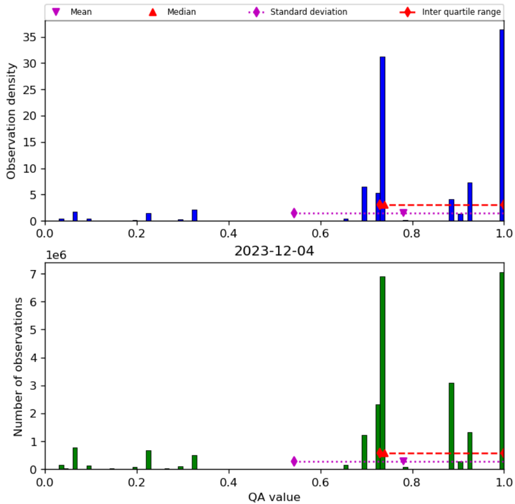
Figure 28: Histogram of “QA value” for 2023-12-04 to 2023-12-05
