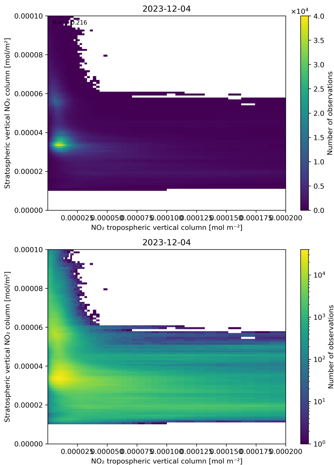
Figure 125: Scatter density plot of “NO 2 tropospheric vertical column” against “Stratospheric vertical NO 2 column” for 2023-12-04 to 2023-12-05.
