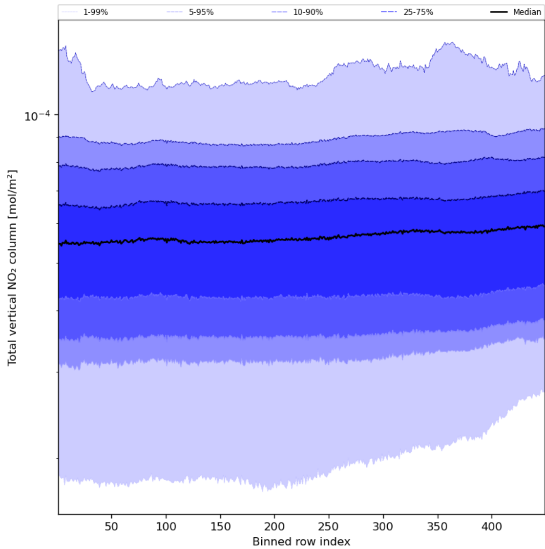
Figure 55: Along track statistics of “Total vertical NO 2 column” for 2023-12-04 to 2023-12-05
