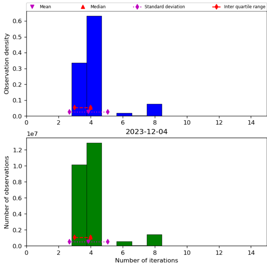
Figure 34: Histogram of “Number of iterations” for 2023-12-04 to 2023-12-05
