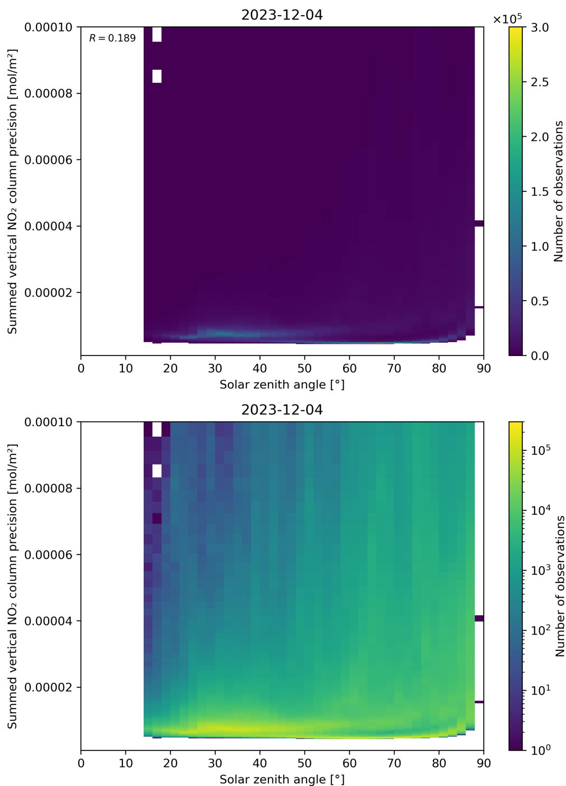
Figure 152: Scatter density plot of “Solar zenith angle” against “Summed vertical NO 2 column precision” for 2023-12-04 to 2023-12-05.
