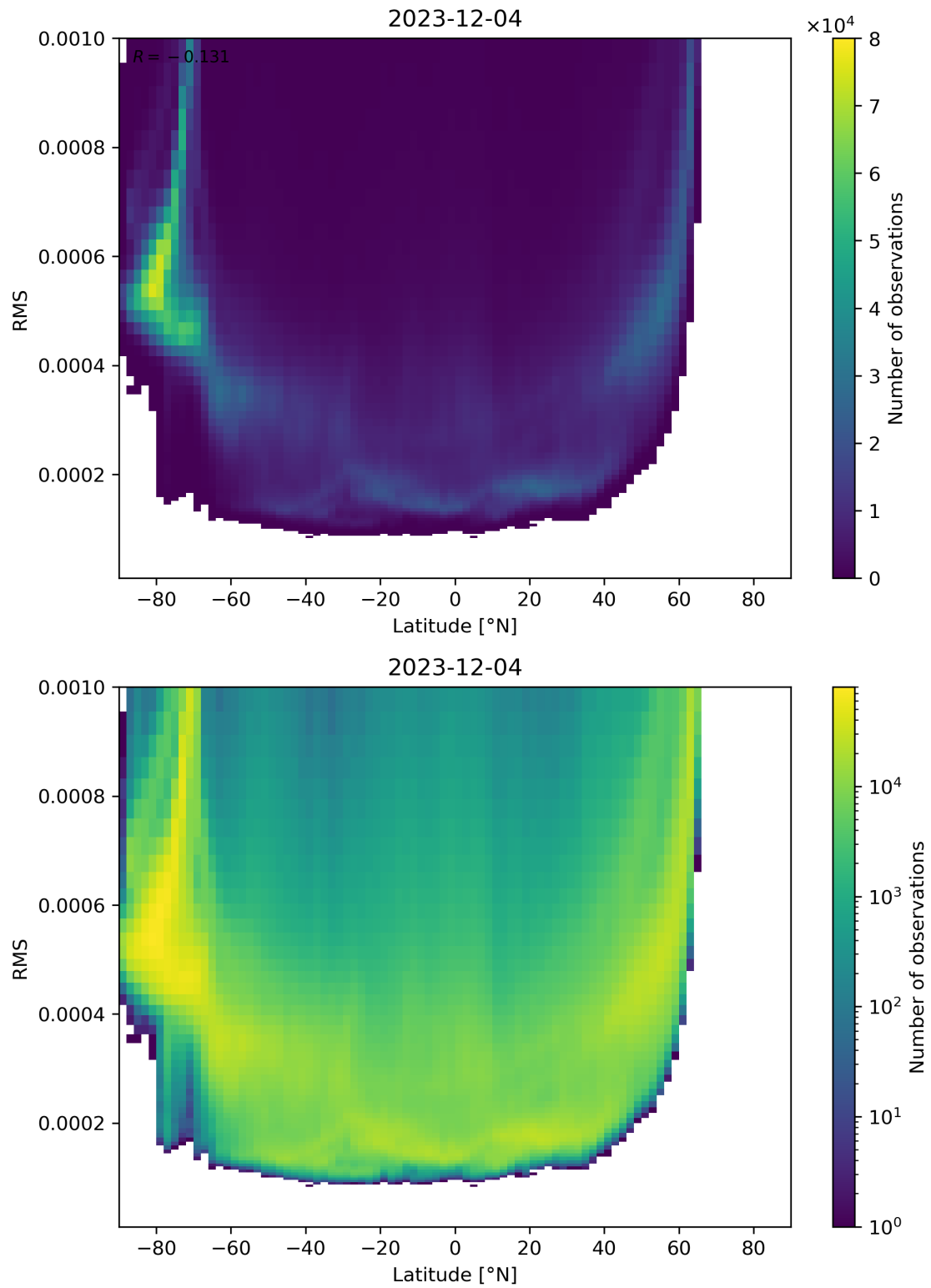
Figure 94: Scatter density plot of “Latitude” against “RMS” for 2023-12-04 to 2023-12-05.
