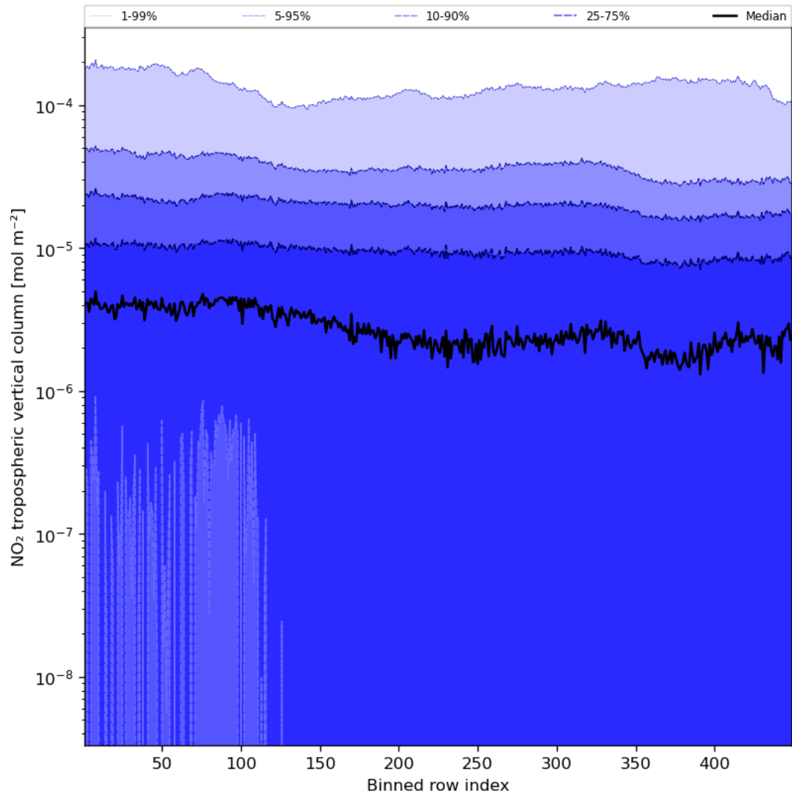
Figure 46: Along track statistics of “NO 2 tropospheric vertical column” for 2023-12-04 to 2023-12-05
