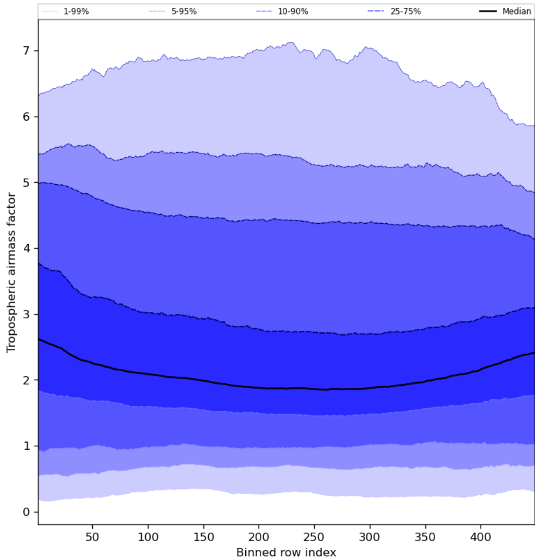
Figure 48: Along track statistics of “Tropospheric air mass factor” for 2023-12-04 to 2023-12-05
