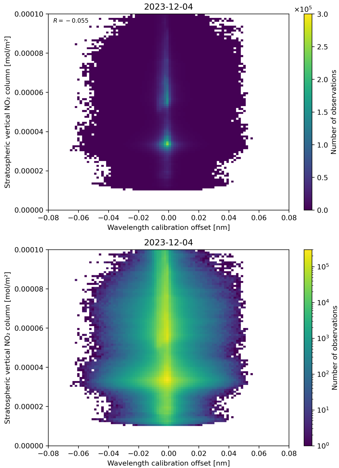
Figure 176: Scatter density plot of “Wavelength calibration offset” against “Stratospheric vertical NO 2 column” for 2023-12-04 to 2023-12-05.
