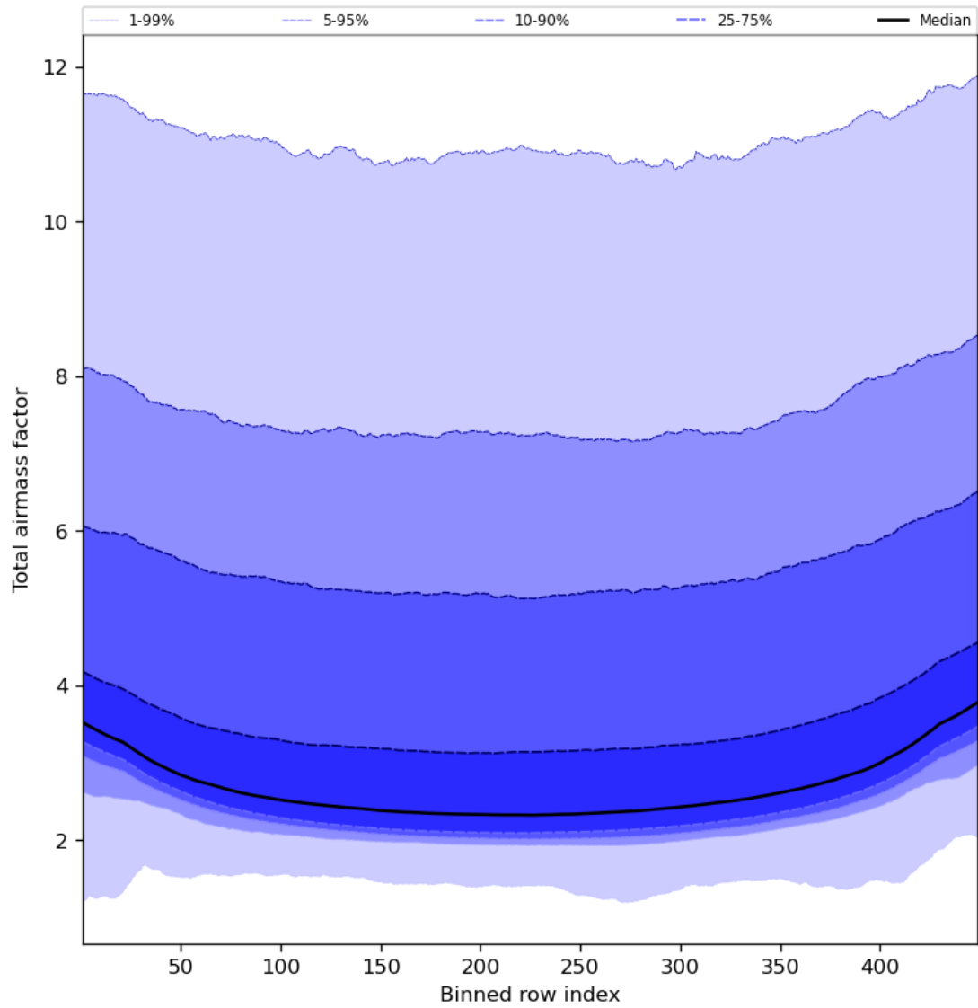
Figure 49: Along track statistics of “Total airmass factor” for 2023-12-04 to 2023-12-05
