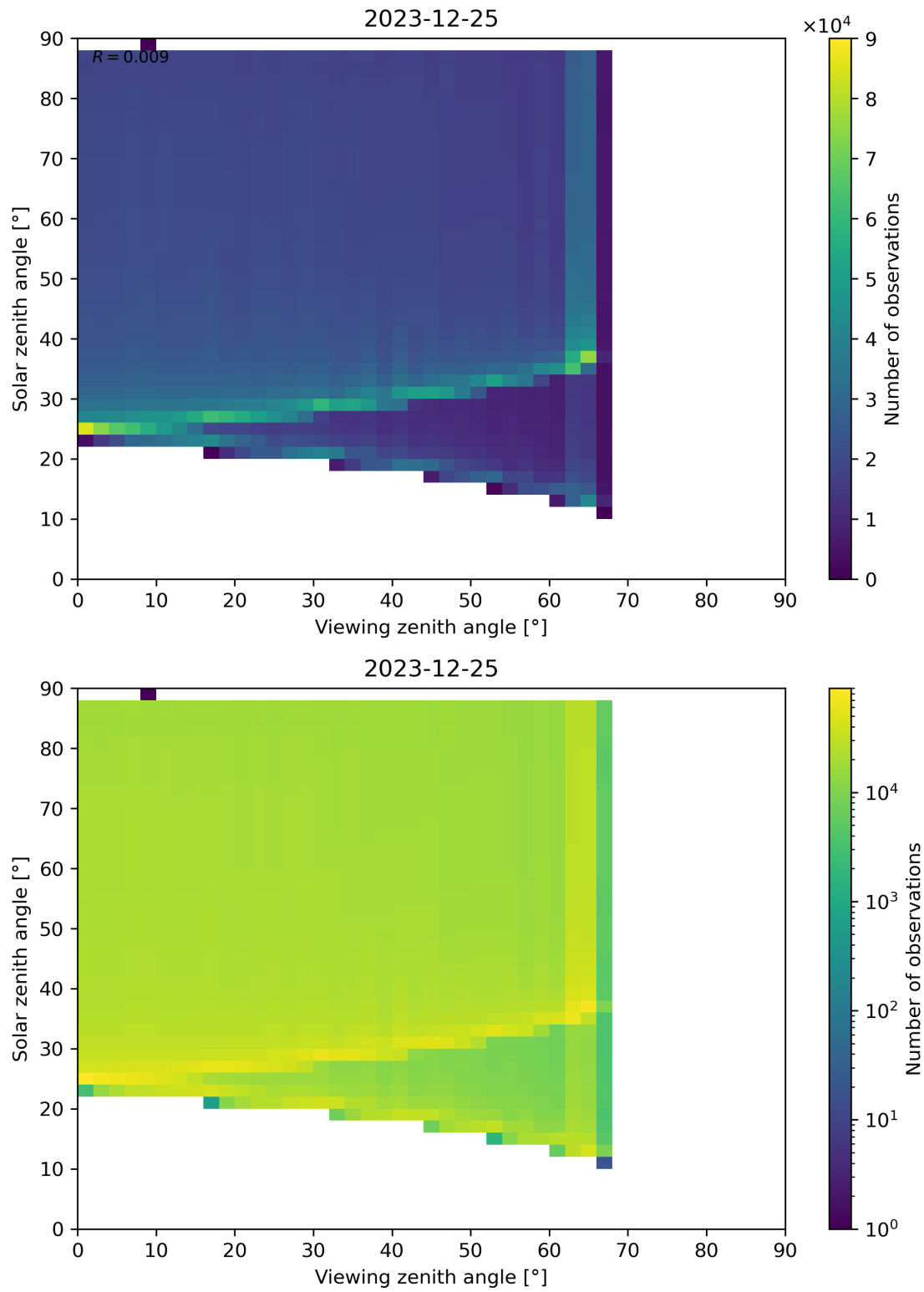
Figure 172: Scatter density plot of “Viewing zenith angle” against “Solar zenith angle” for 2023-12-25 to 2023-12-26.
