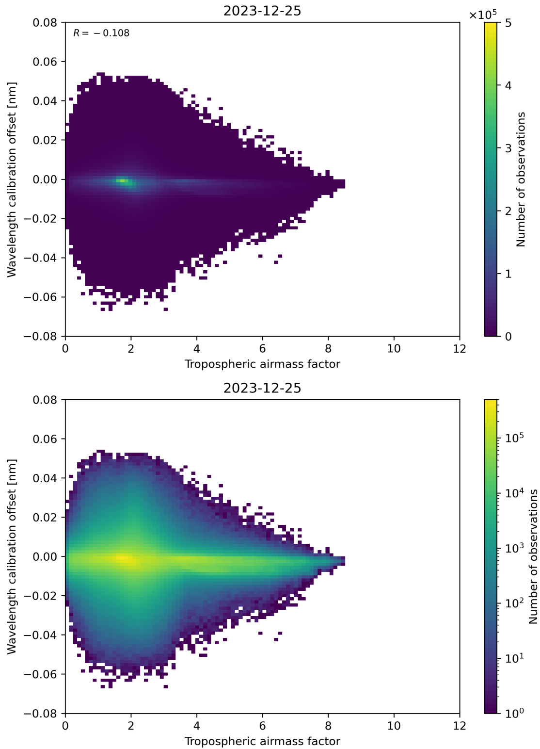
Figure 80: Scatter density plot of “Tropospheric airmass factor” against “Wavelength calibration offset” for 2023-12-25 to 2023-12-26.
