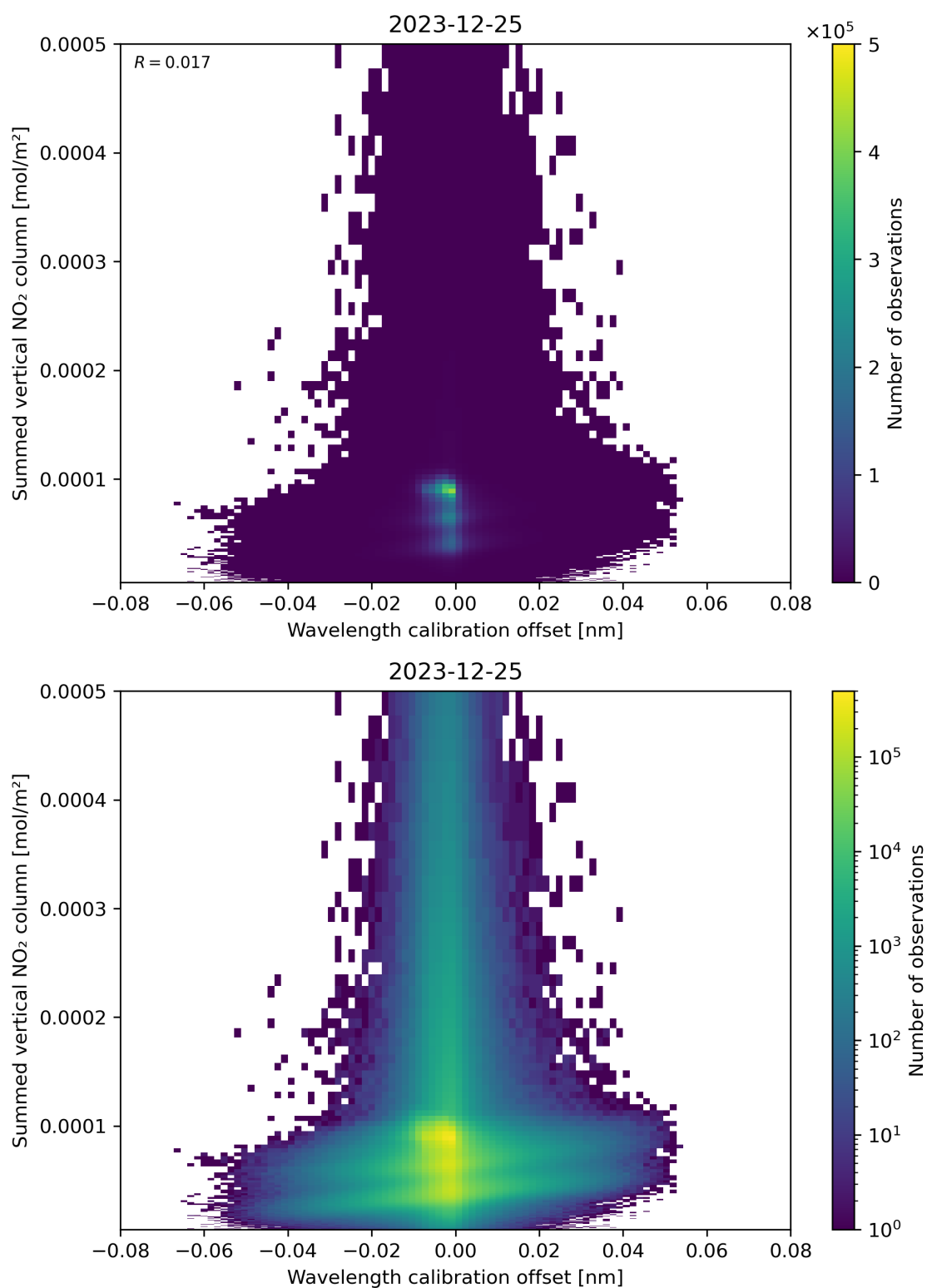
Figure 177: Scatter density plot of “Wavelength calibration offset” against “Summed vertical NO 2 column” for 2023-12-25 to 2023-12-26.
