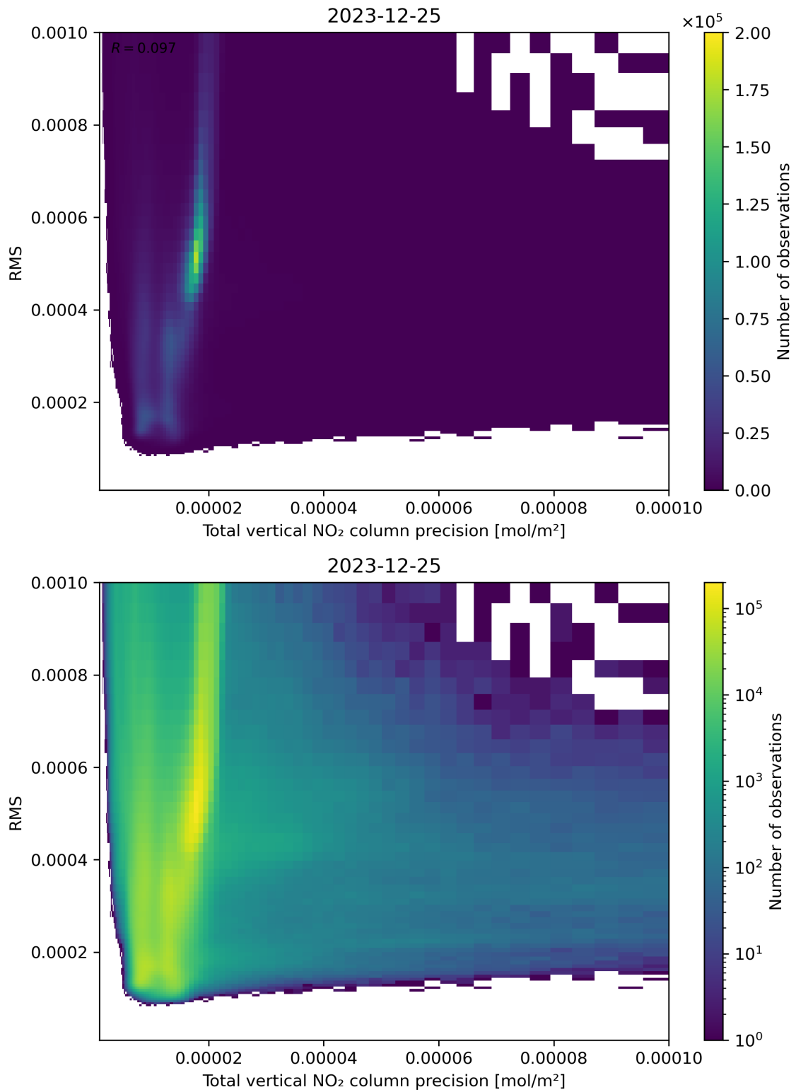
Figure 119: Scatter density plot of “Total vertical NO 2 column precision” against “RMS” for 2023-12-25 to 2023-12-26.
