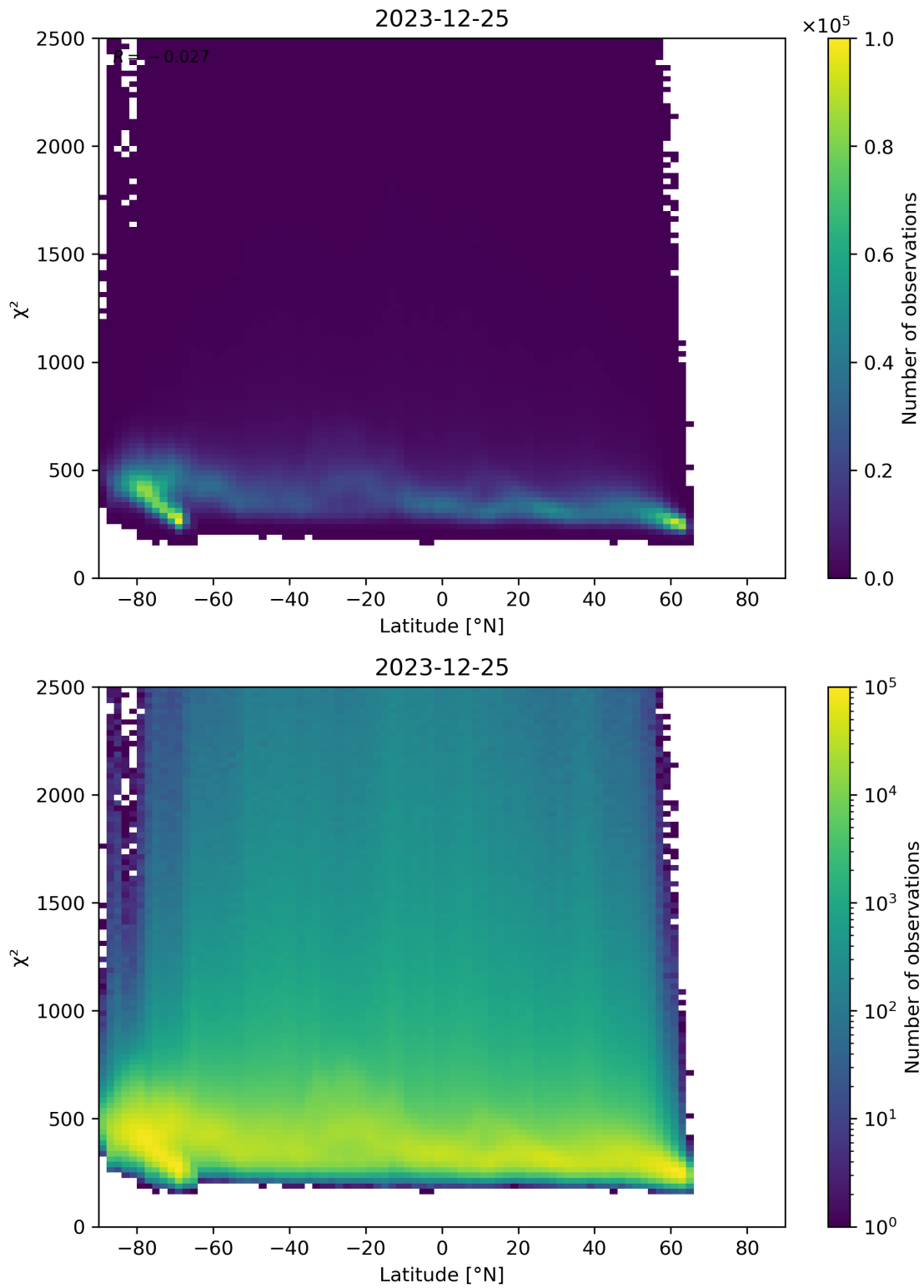
Figure 86: Scatter density plot of “Latitude” against “ \chi^2 ” for 2023-12-25 to 2023-12-26.
