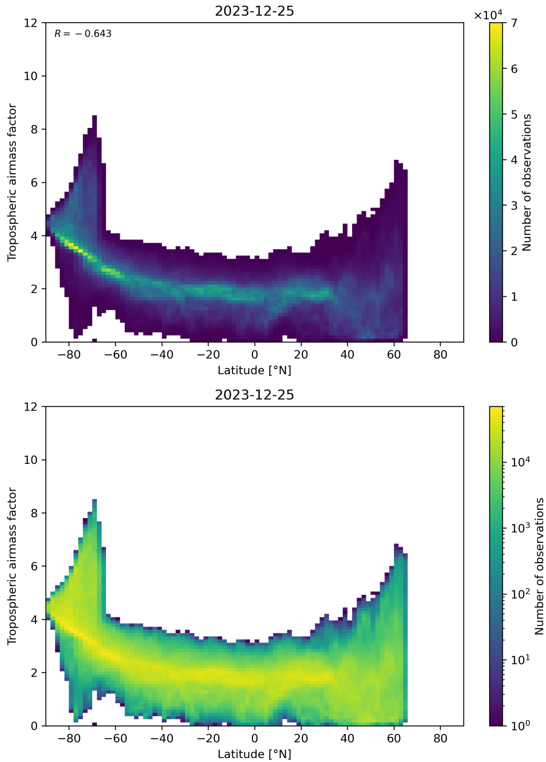
Figure 85: Scatter density plot of “Latitude” against “Tropospheric airmass factor” for 2023-12-25 to 2023-12-26.
