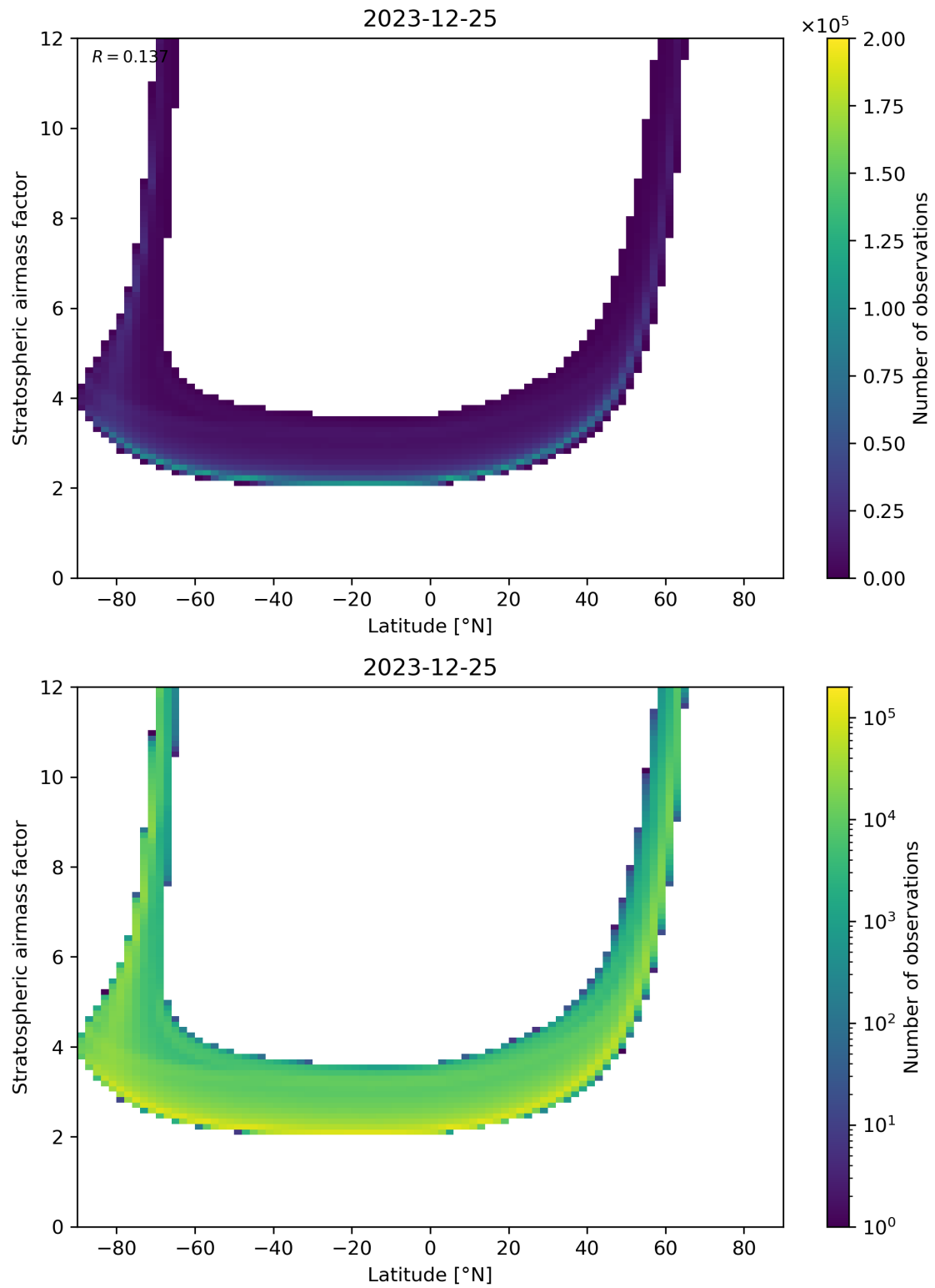
Figure 83: Scatter density plot of “Latitude” against “Stratospheric air mass factor” for 2023-12-25 to 2023-12-26.
