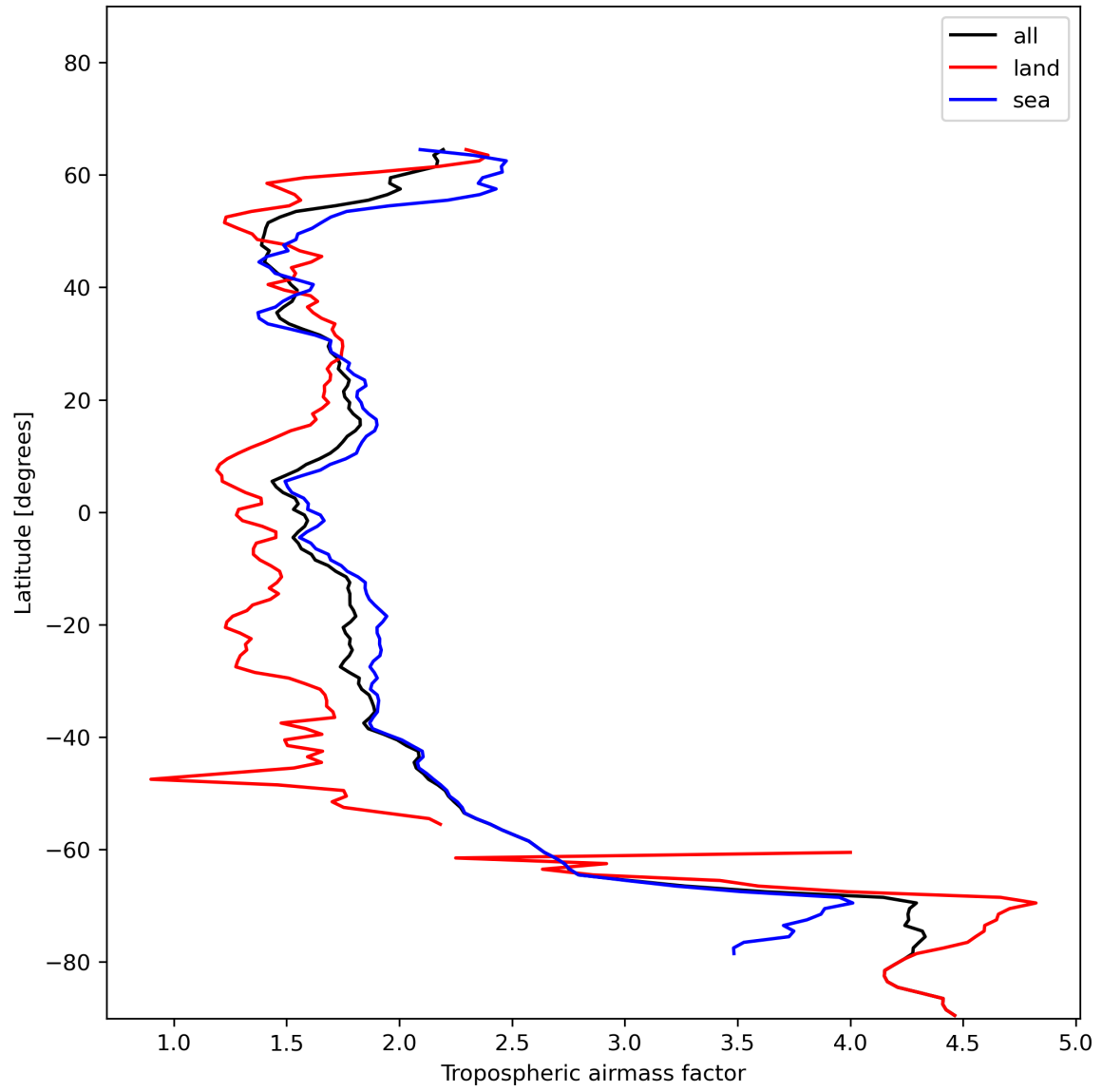
Figure 14: Zonal average of “Tropospheric air mass factor” for 2023-12-25 to 2023-12-26.
