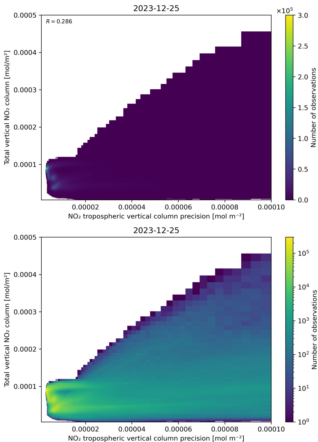
Figure 138: Scatter density plot of “NO 2 tropospheric vertical column precision” against “Total vertical NO 2 column” for 2023-12-25 to 2023-12-26.
