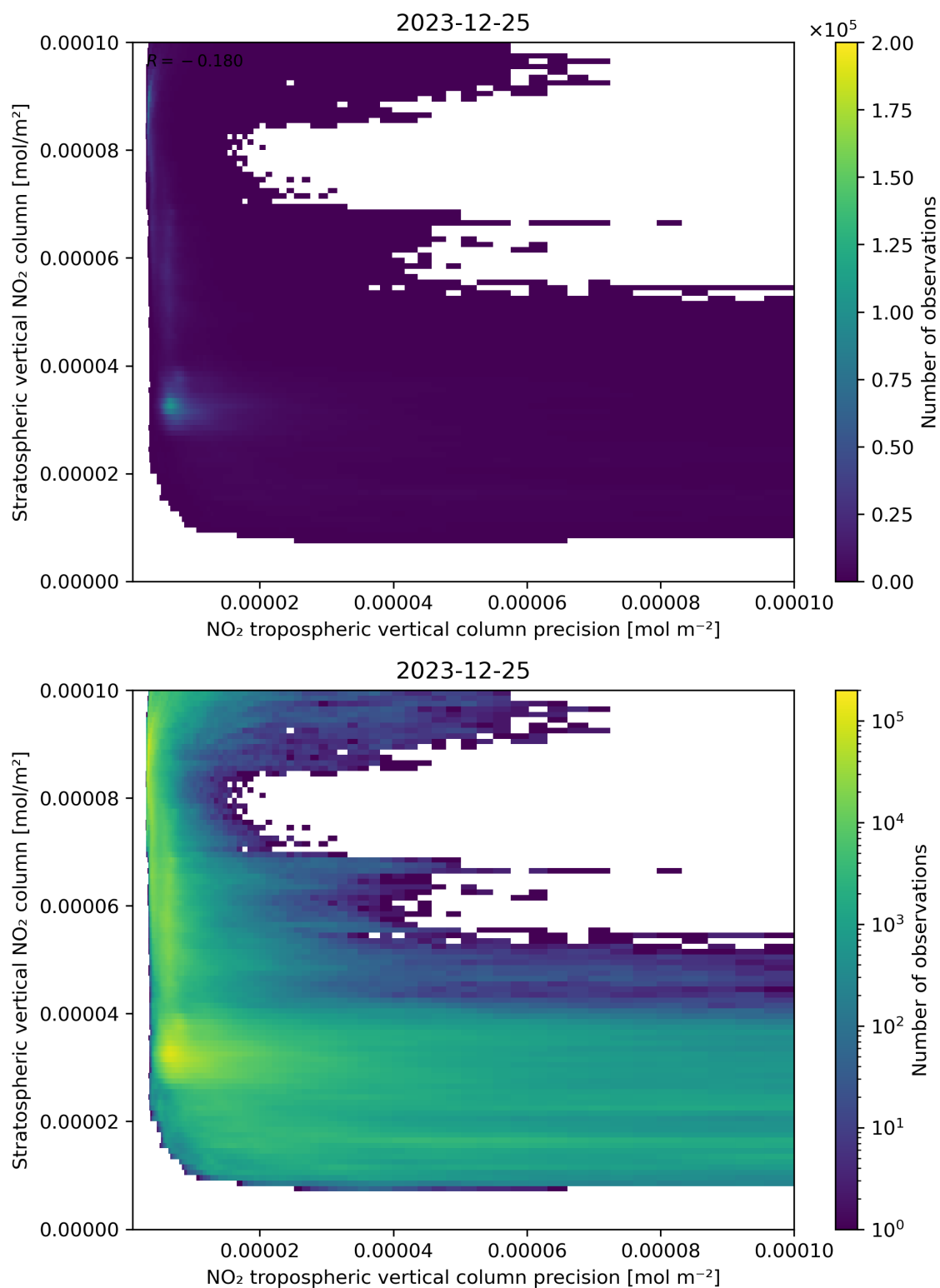
Figure 135: Scatter density plot of “NO 2 tropospheric vertical column precision” against “Stratospheric vertical NO 2 column” for 2023-12-25 to 2023-12-26.
