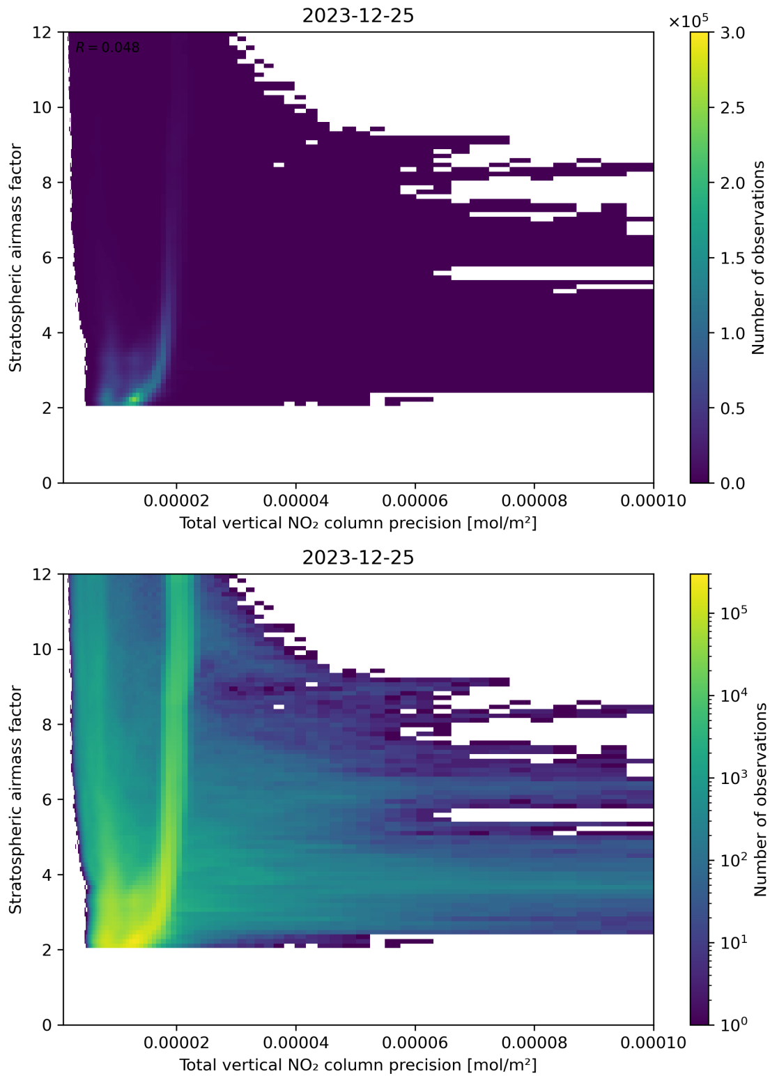
Figure 115: Scatter density plot of “Total vertical NO 2 column precision” against “Stratospheric air mass factor” for 2023-12-25 to 2023-12-26.
