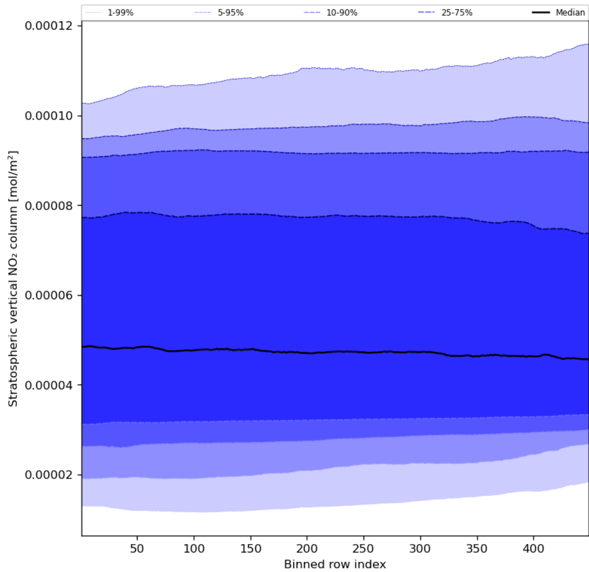
Figure 53: Along track statistics of “Stratospheric vertical NO 2 column” for 2023-12-25 to 2023-12-26
