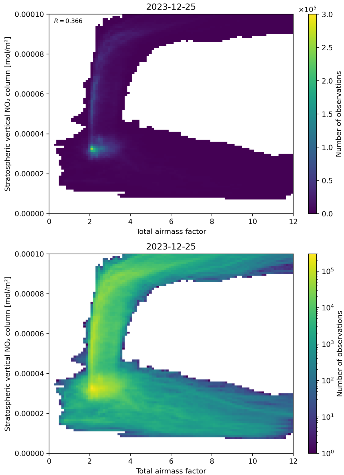
Figure 64: Scatter density plot of “Total airmass factor” against “Stratospheric vertical NO 2 column” for 2023-12-25 to 2023-12-26.
