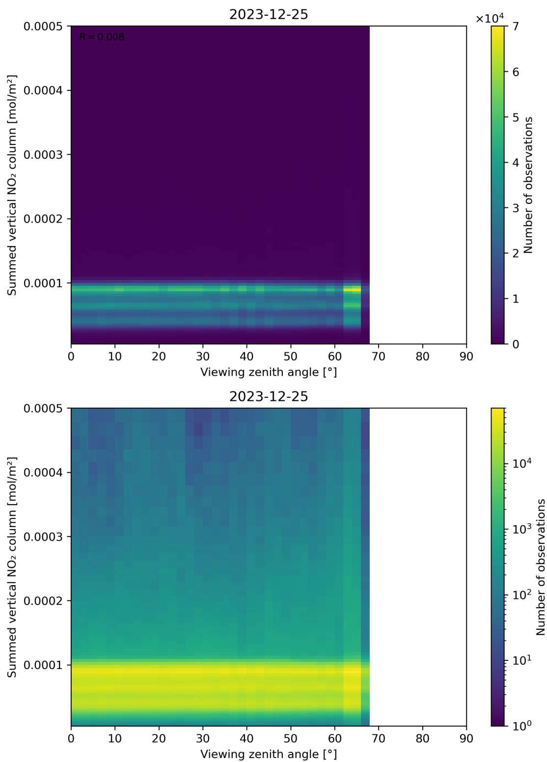
Figure 165: Scatter density plot of “Viewing zenith angle” against “Summed vertical NO 2 column” for 2023-12-25 to 2023-12-26.
