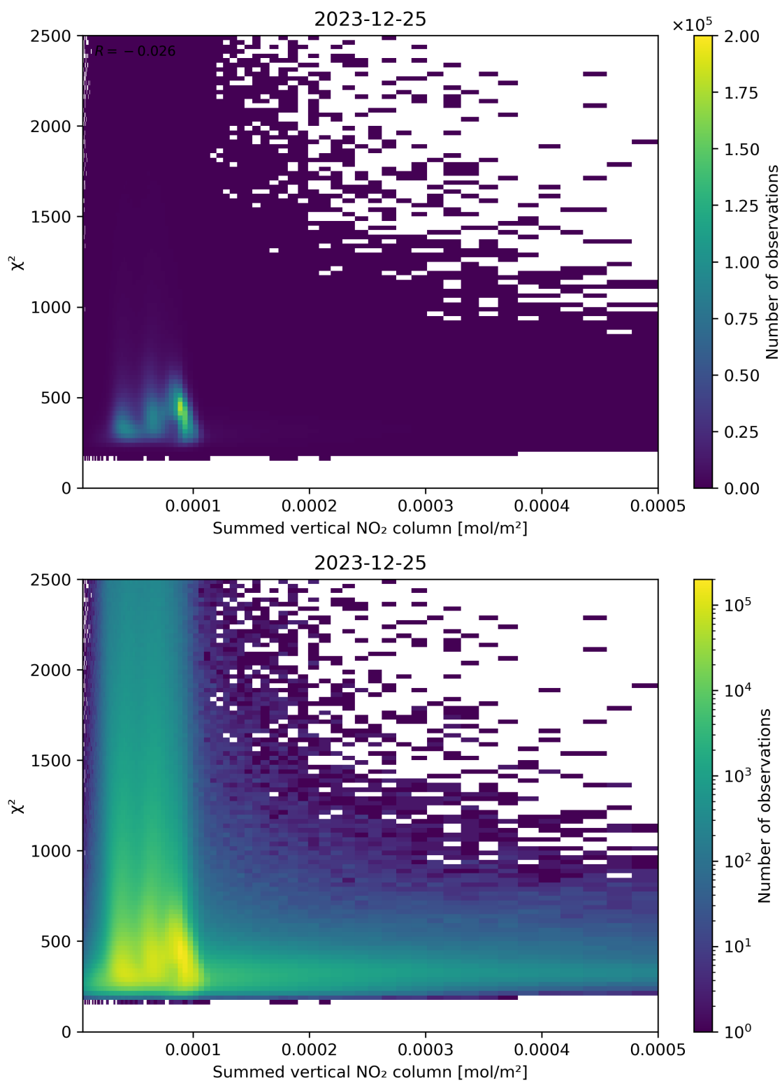
Figure 104: Scatter density plot of “Summed vertical NO 2 column” against “ \chi^2 ” for 2023-12-25 to 2023-12-26.
