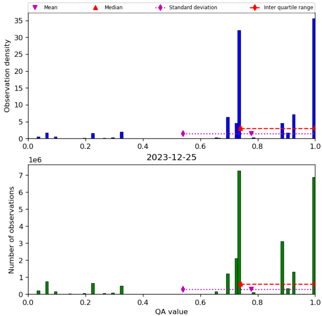
Figure 28: Histogram of “QA value” for 2023-12-25 to 2023-12-26
