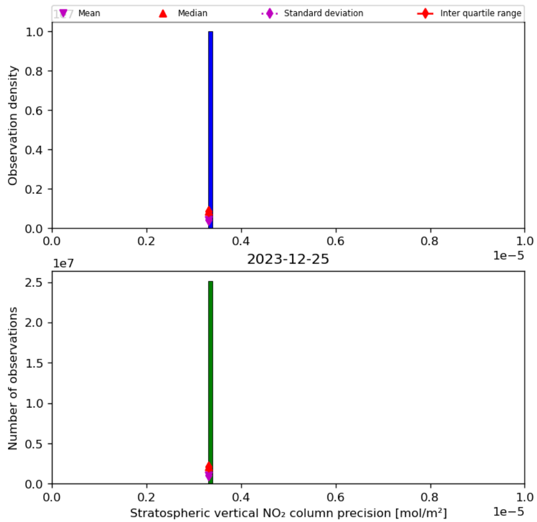
Figure 37: Histogram of “Stratospheric vertical NO 2 column precision” for 2023-12-25 to 2023-12-26
