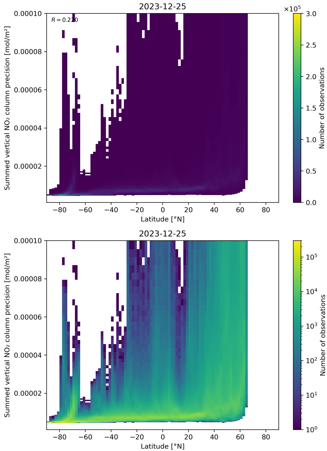
Figure 89: Scatter density plot of “Latitude” against “Summed vertical NO 2 column precision” for 2023-12-25 to 2023-12-26.
