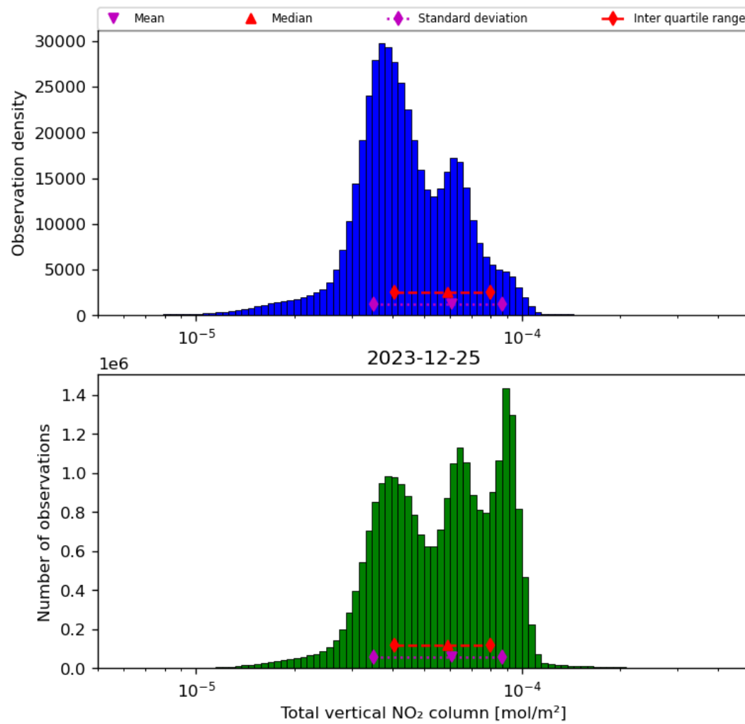
Figure 38: Histogram of “Total vertical NO 2 column” for 2023-12-25 to 2023-12-26
