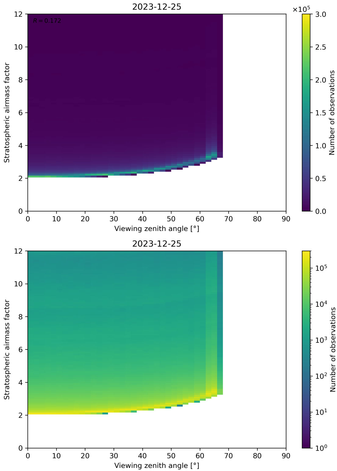
Figure 159: Scatter density plot of “Viewing zenith angle” against “Stratospheric airmass factor” for 2023-12-25 to 2023-12-26.
