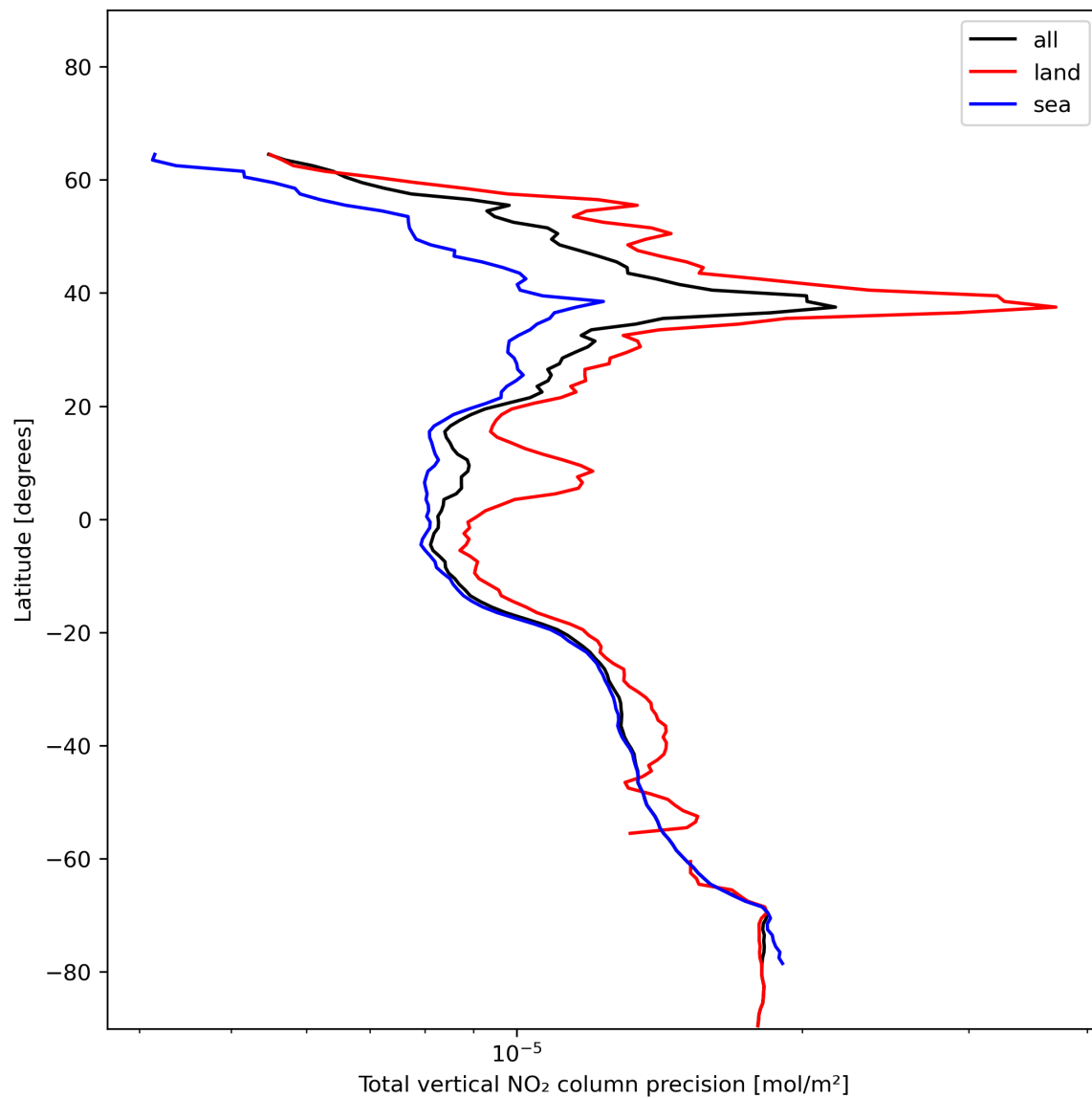
Figure 22: Zonal average of “Total vertical NO 2 column precision” for 2023-12-25 to 2023-12-26.
