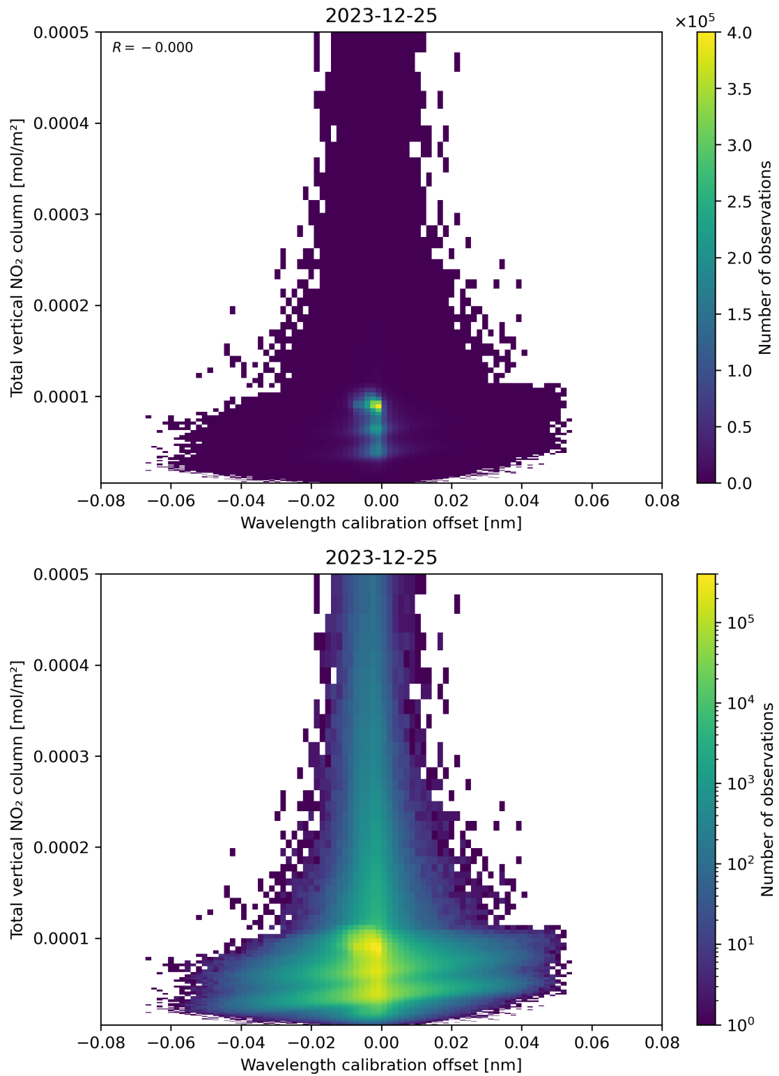
Figure 179: Scatter density plot of “Wavelength calibration offset” against “Total vertical NO 2 column” for 2023-12-25 to 2023-12-26.
