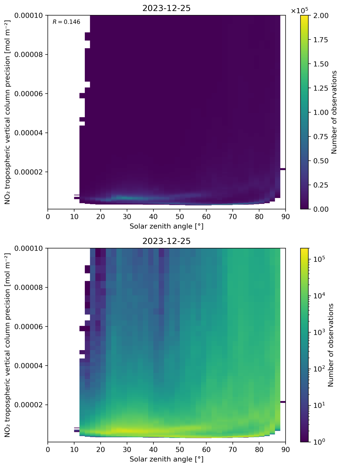
Figure 156: Scatter density plot of “Solar zenith angle” against “NO 2 tropospheric vertical column precision” for 2023-12-25 to 2023-12-26.
