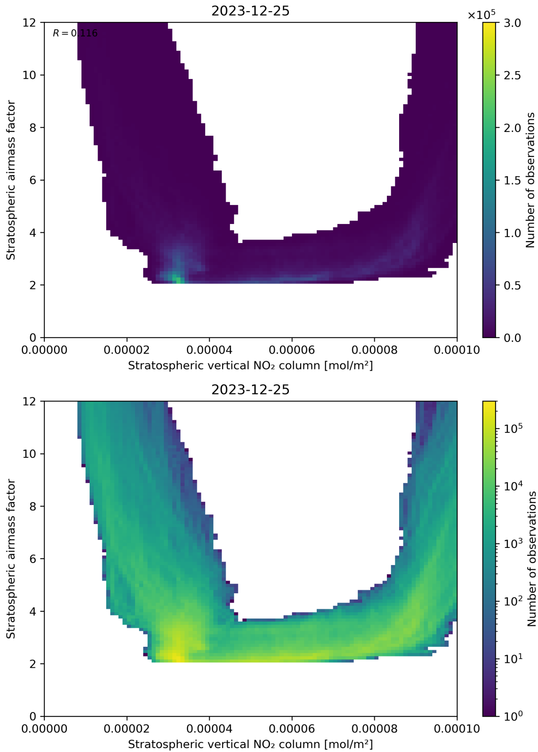
Figure 96: Scatter density plot of “Stratospheric vertical NO 2 column” against “Stratospheric airmass factor” for 2023-12-25 to 2023-12-26.
