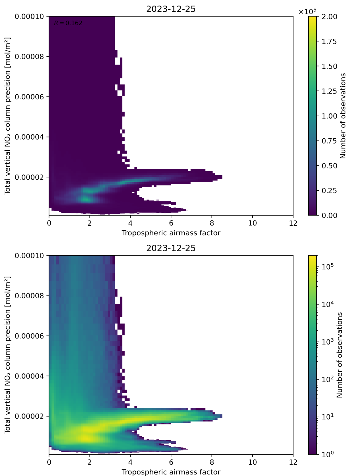
Figure 78: Scatter density plot of “Tropospheric air mass factor” against “Total vertical NO 2 column precision” for 2023-12-25 to 2023-12-26.
