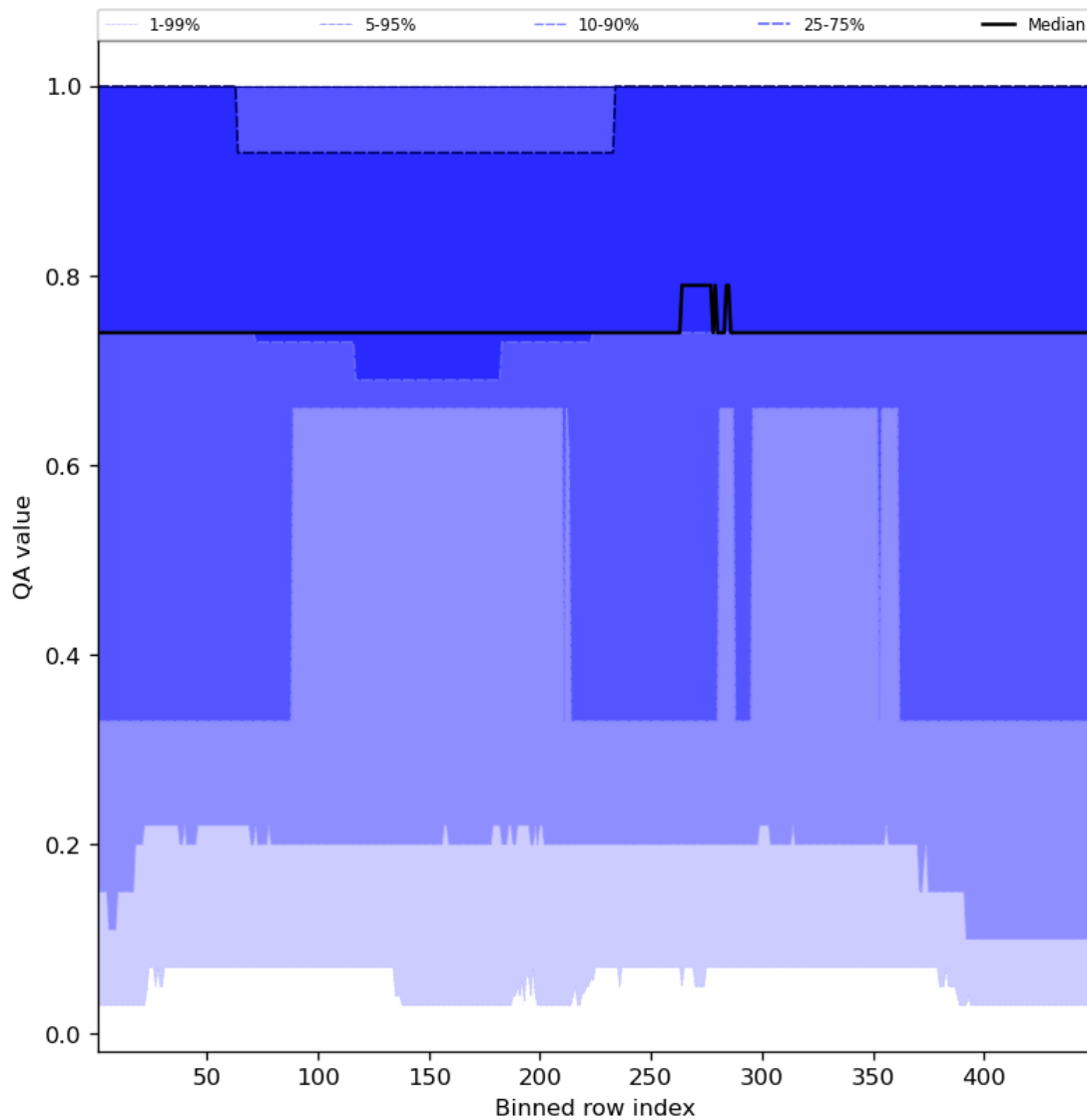
Figure 45: Along track statistics of “QA value” for 2023-12-25 to 2023-12-26
