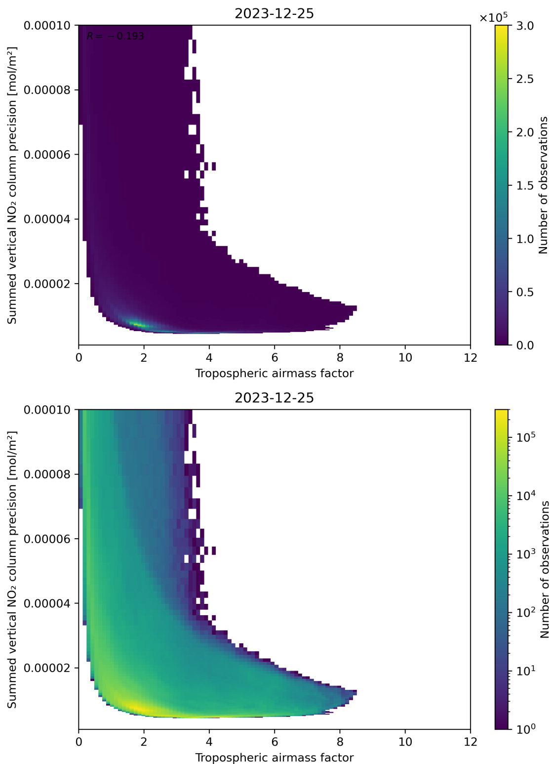
Figure 76: Scatter density plot of “Tropospheric air mass factor” against “Summed vertical NO 2 column precision” for 2023-12-25 to 2023-12-26.
