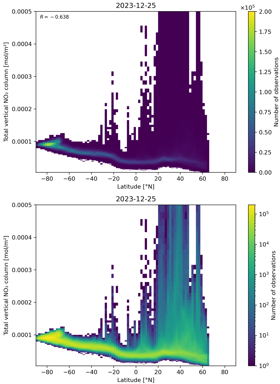
Figure 90: Scatter density plot of “Latitude” against “Total vertical NO 2 column” for 2023-12-25 to 2023-12-26.
