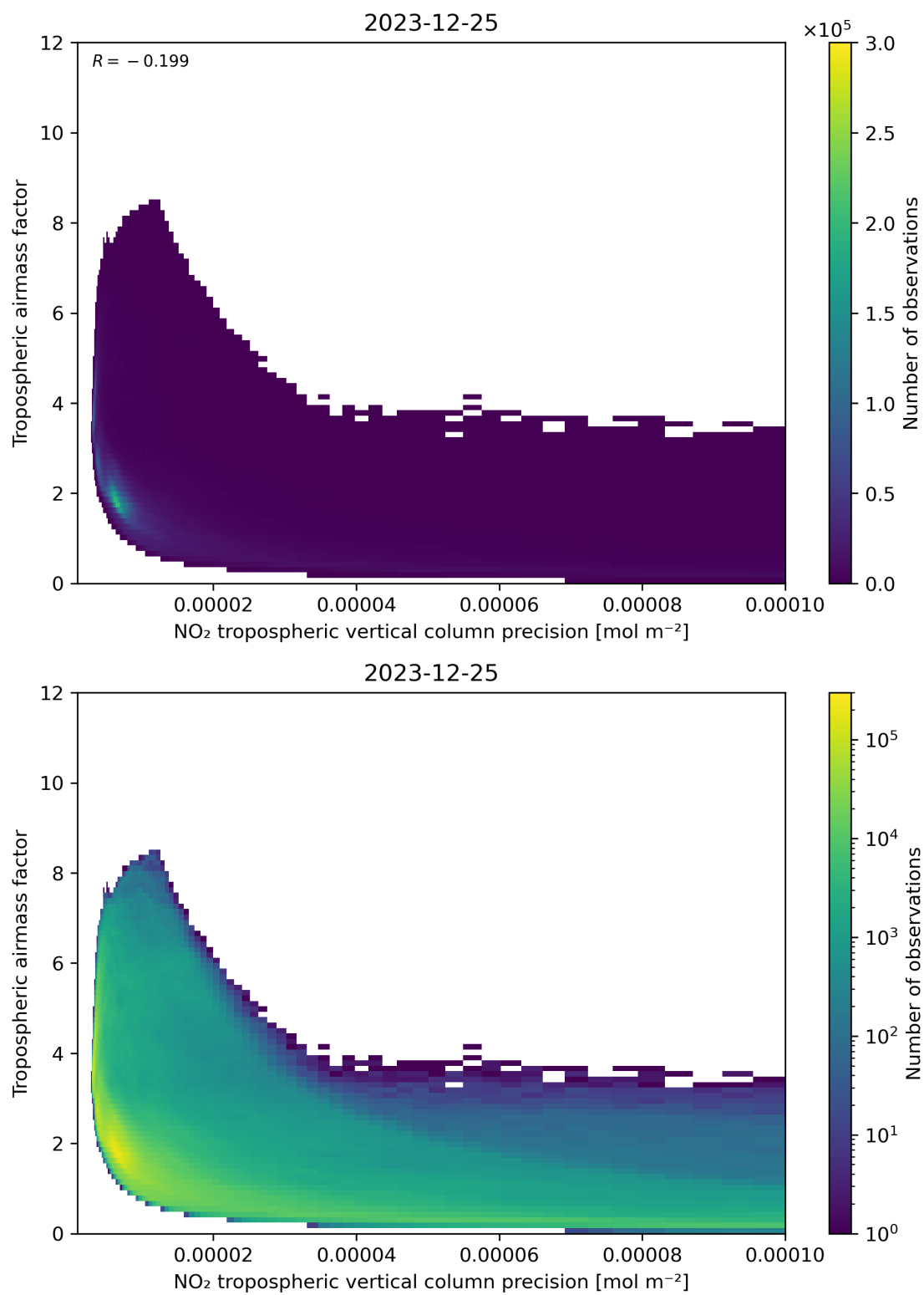
Figure 133: Scatter density plot of “NO 2 tropospheric vertical column precision” against “Tropospheric airmass factor” for 2023-12-25 to 2023-12-26.
