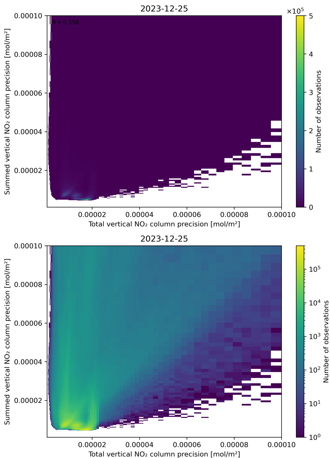
Figure 118: Scatter density plot of “Total vertical NO 2 column precision” against “Summed vertical NO 2 column precision” for 2023-12-25 to 2023-12-26.
