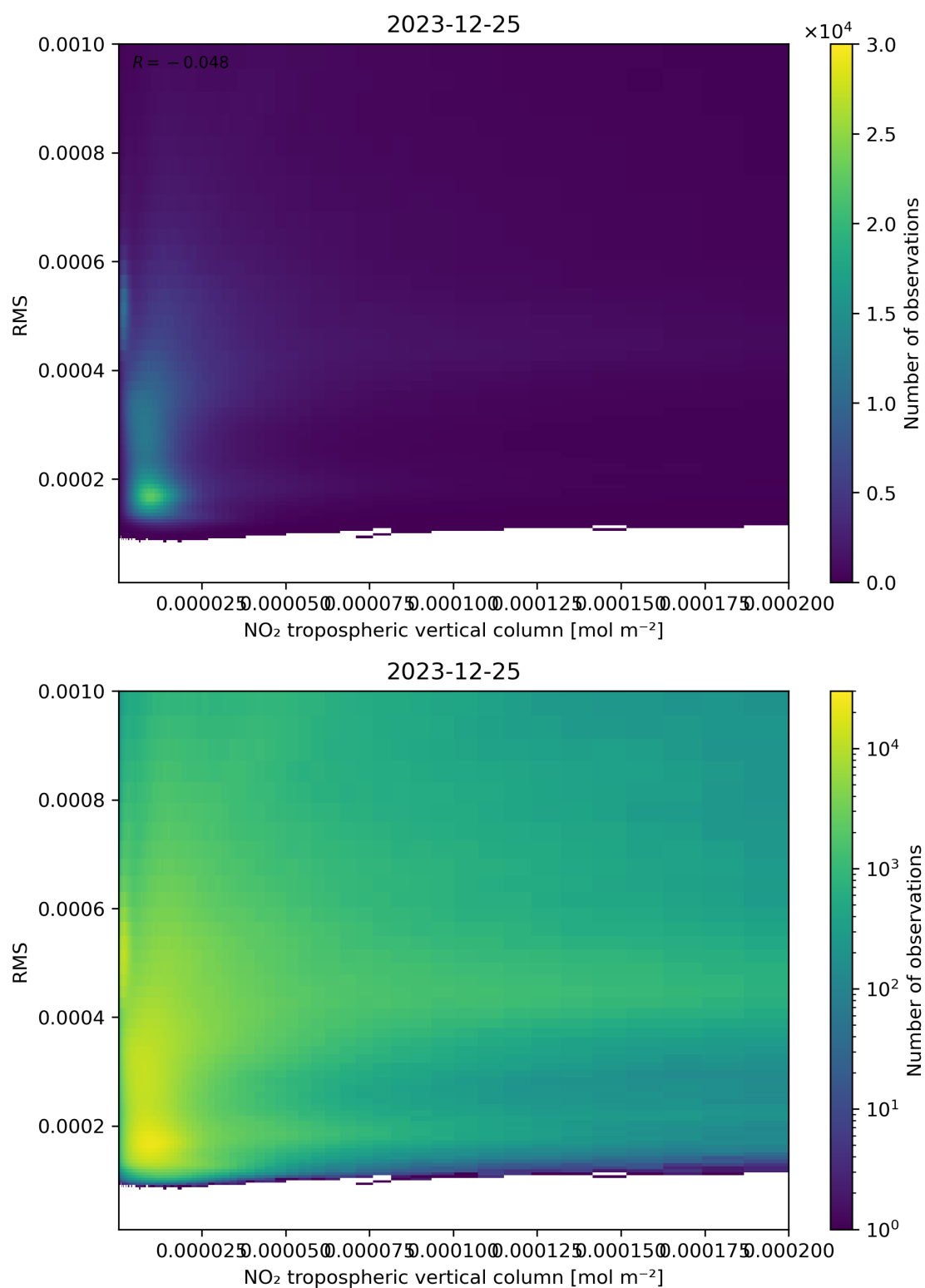
Figure 142: Scatter density plot of “NO 2 tropospheric vertical column” against “RMS” for 2023-12-25 to 2023-12-26.
