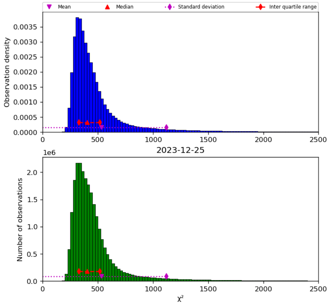
Figure 42: Histogram of “ \chi^2 ” for 2023-12-25 to 2023-12-26
