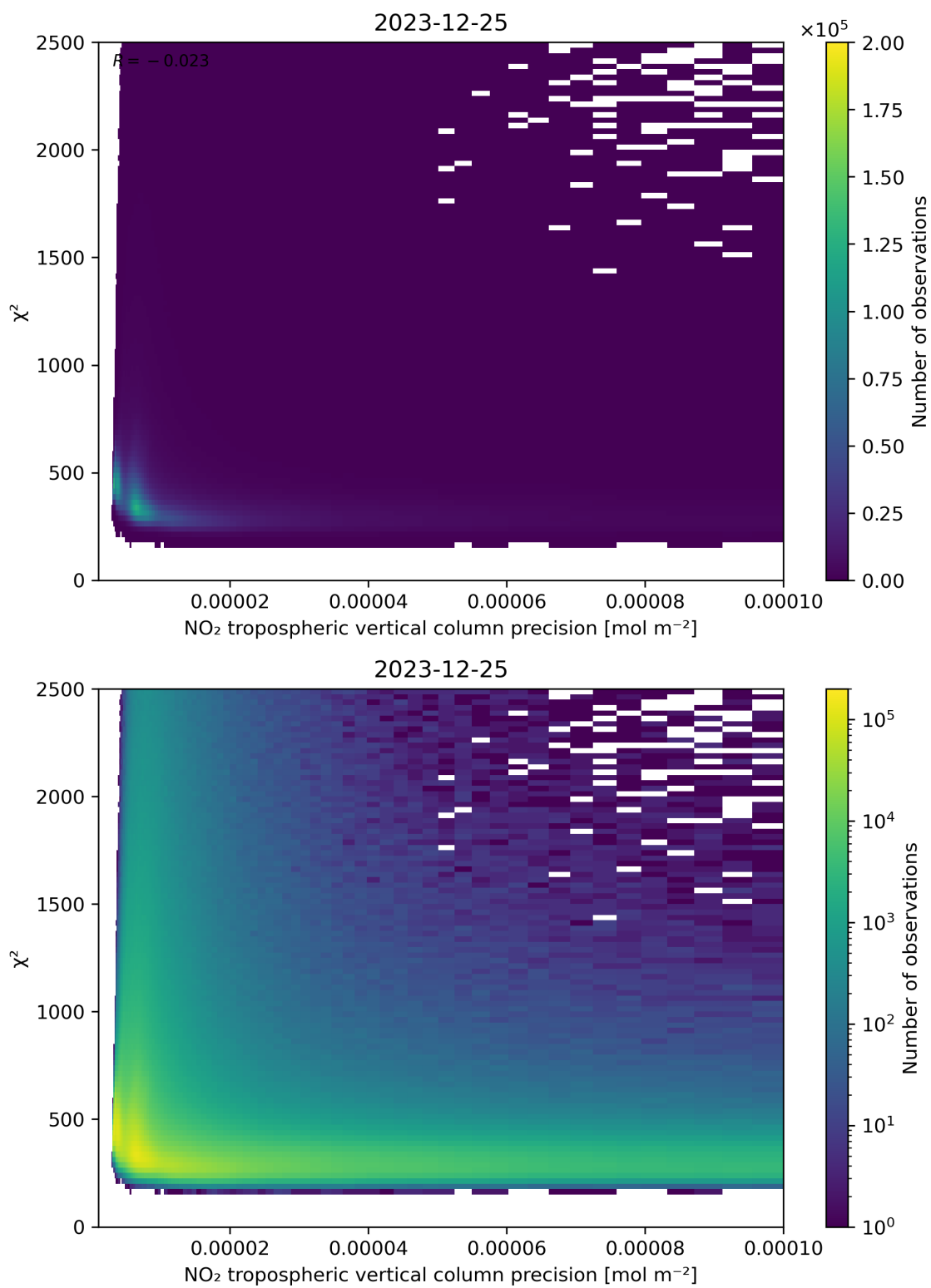
Figure 134: Scatter density plot of “NO 2 tropospheric vertical column precision” against “ \chi^2 ” for 2023-12-25 to 2023-12-26.
