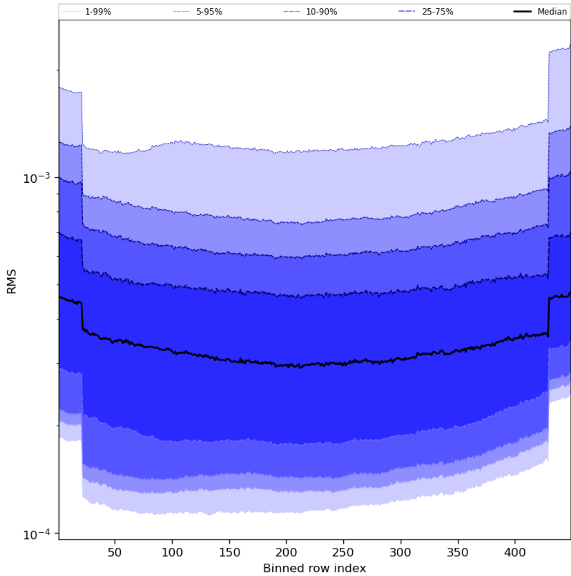
Figure 60: Along track statistics of “RMS” for 2023-12-25 to 2023-12-26
