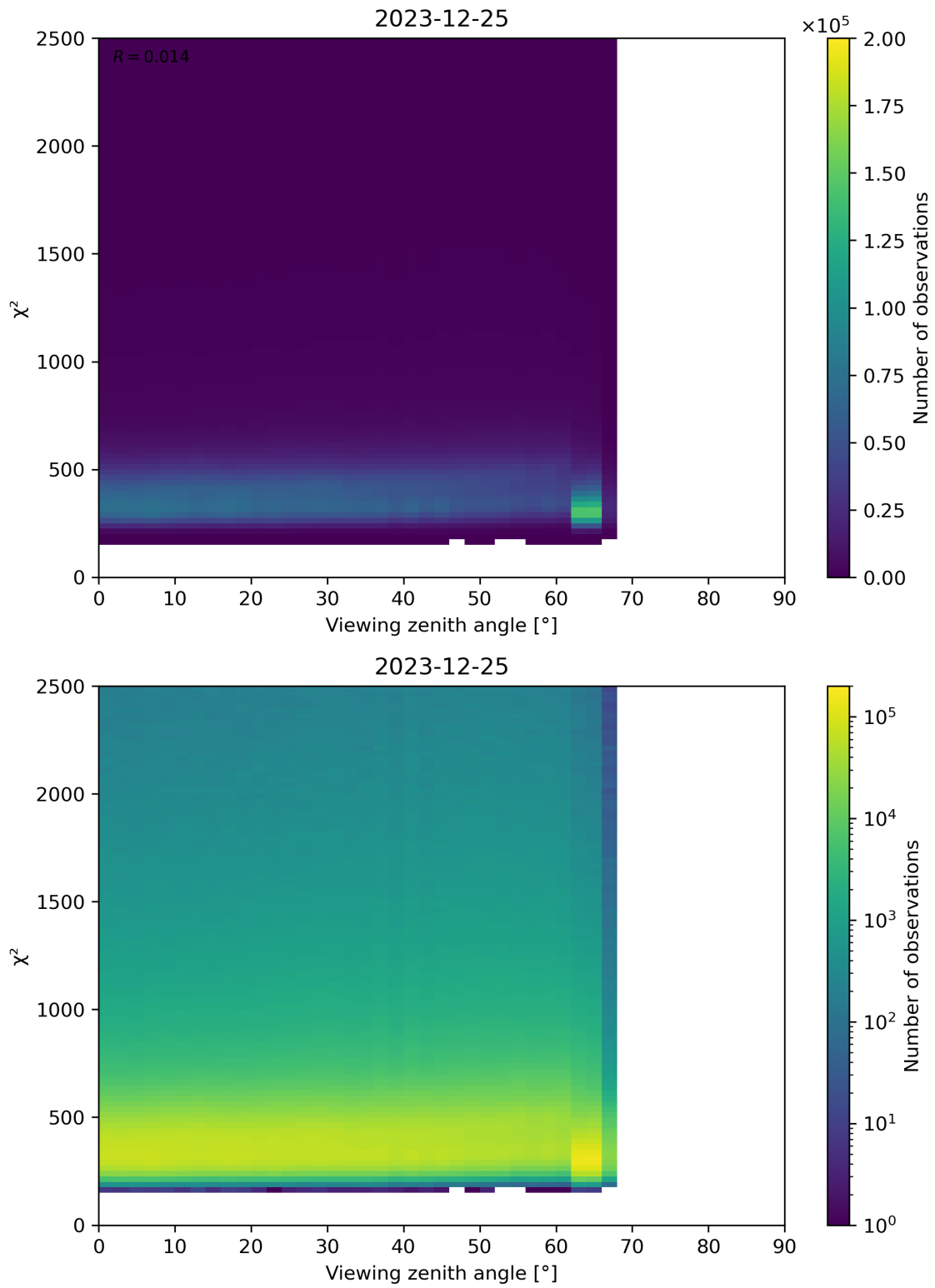
Figure 162: Scatter density plot of “Viewing zenith angle” against “ \chi^2 ” for 2023-12-25 to 2023-12-26.
