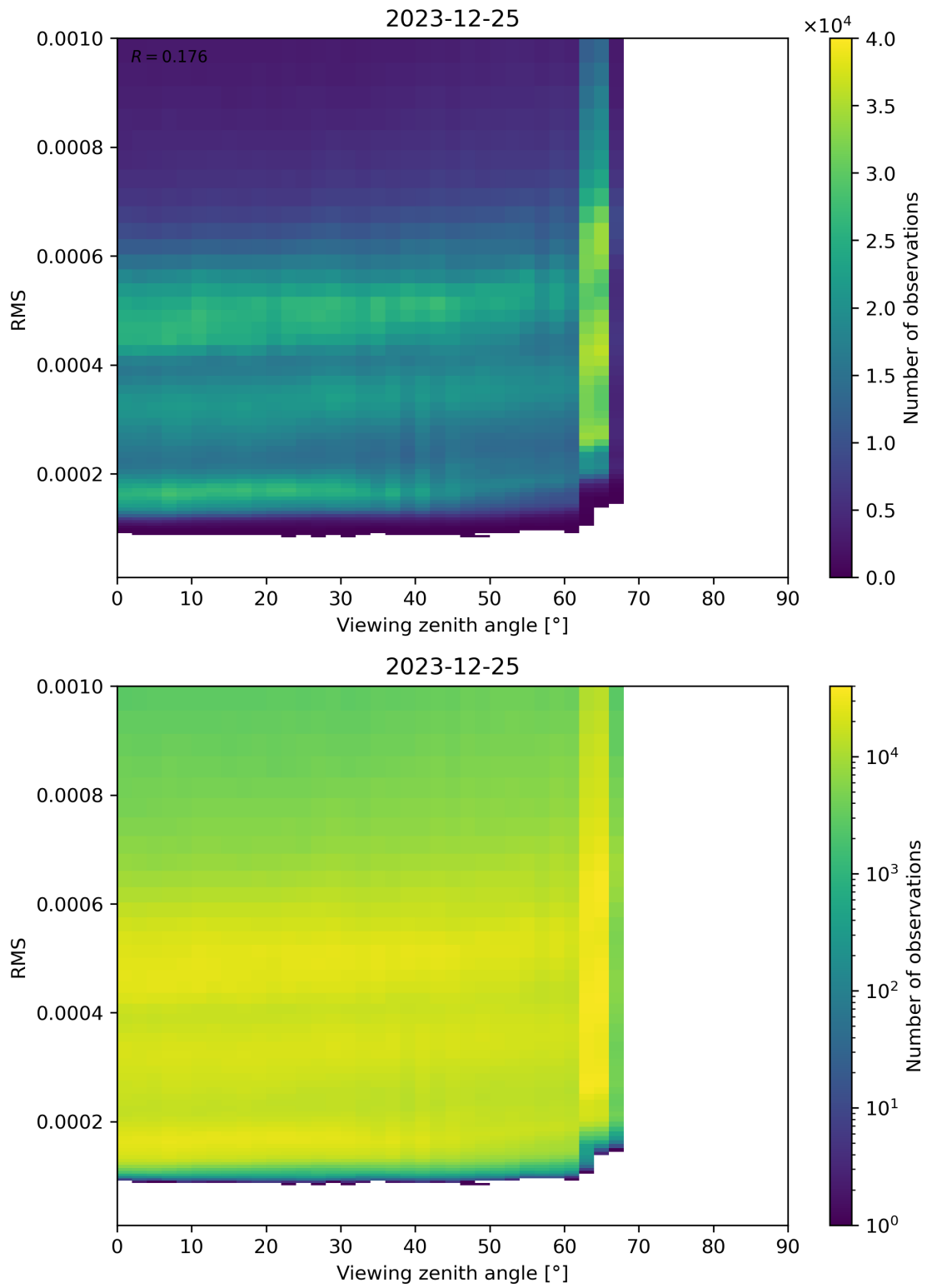
Figure 171: Scatter density plot of “Viewing zenith angle” against “RMS” for 2023-12-25 to 2023-12-26.
