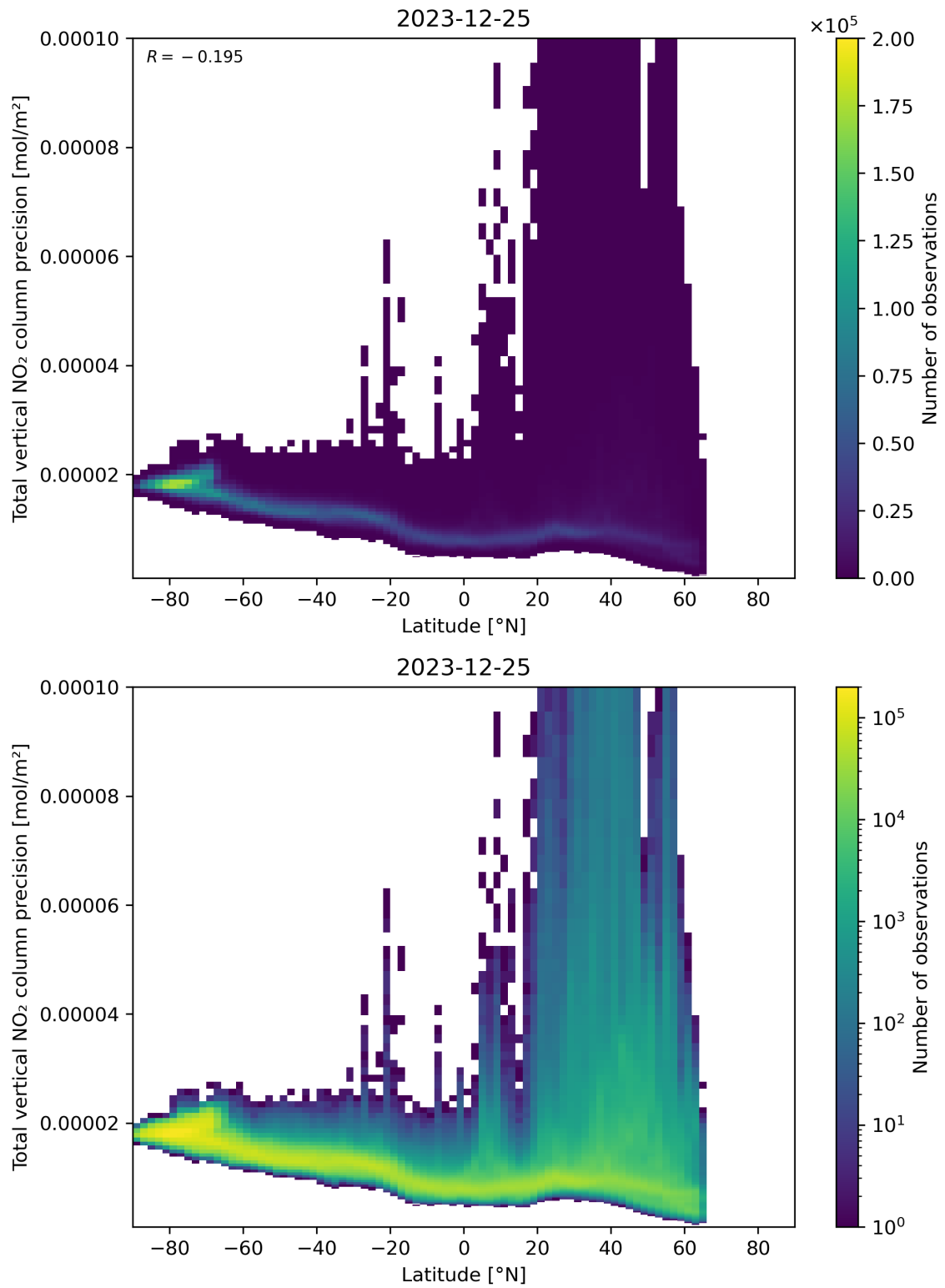
Figure 91: Scatter density plot of “Latitude” against “Total vertical NO 2 column precision” for 2023-12-25 to 2023-12-26.
