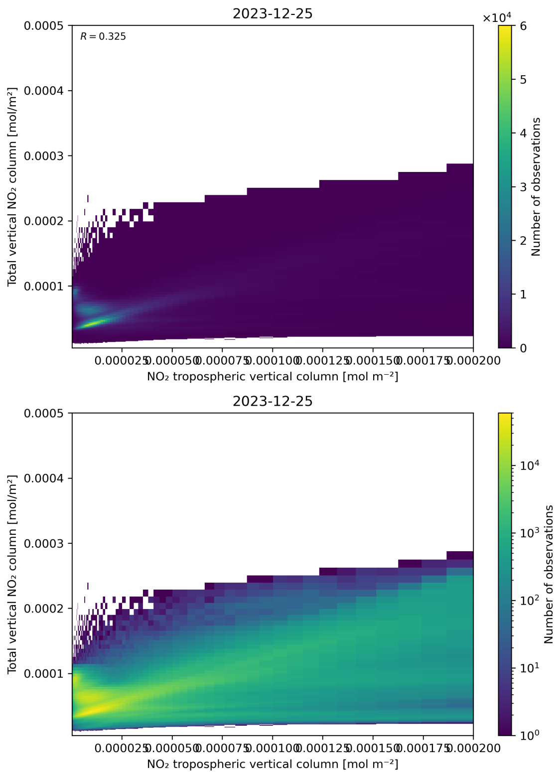
Figure 128: Scatter density plot of “NO 2 tropospheric vertical column” against “Total vertical NO 2 column” for 2023-12-25 to 2023-12-26.
