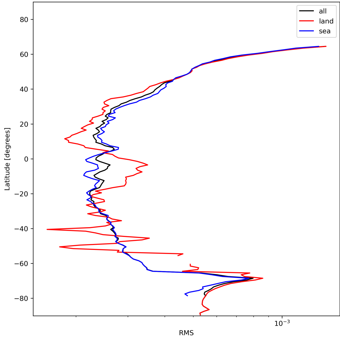
Figure 26: Zonal average of “RMS” for 2023-12-25 to 2023-12-26.
