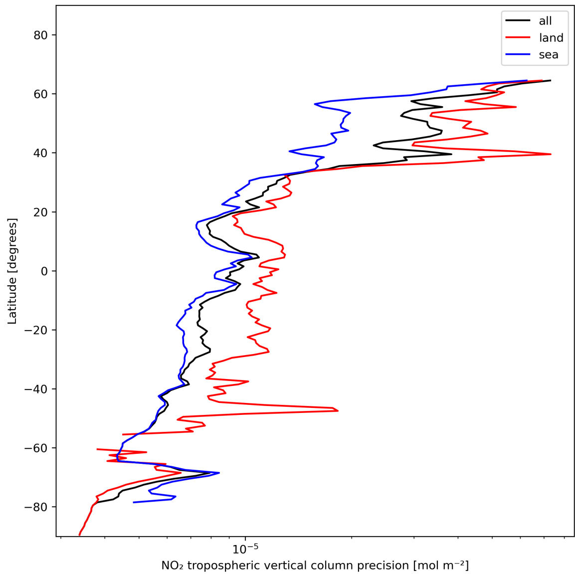
Figure 13: Zonal average of “NO 2 tropospheric vertical column precision” for 2023-12-25 to 2023-12-26.
