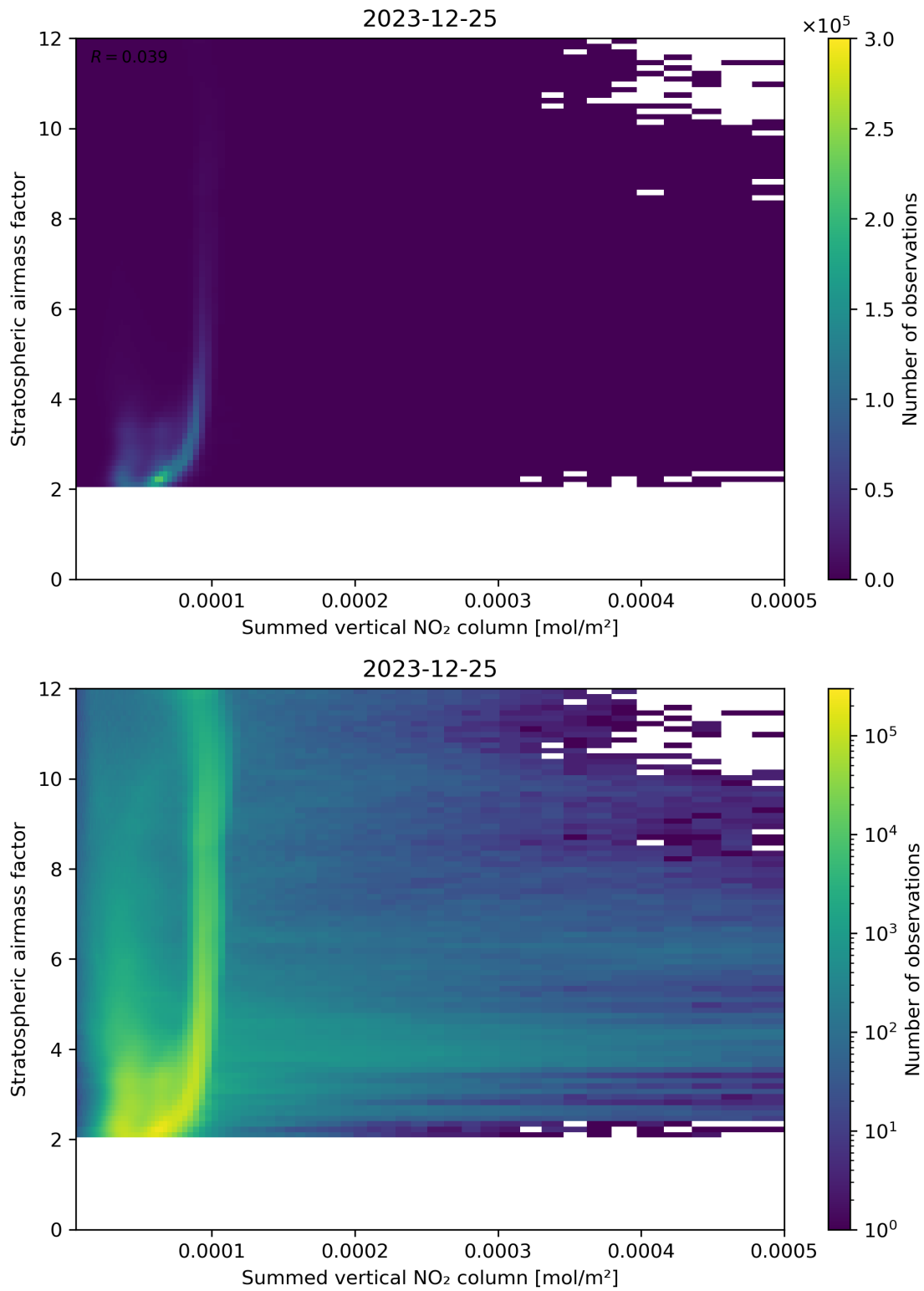
Figure 103: Scatter density plot of “Summed vertical NO 2 column” against “Stratospheric air mass factor” for 2023-12-25 to 2023-12-26.
