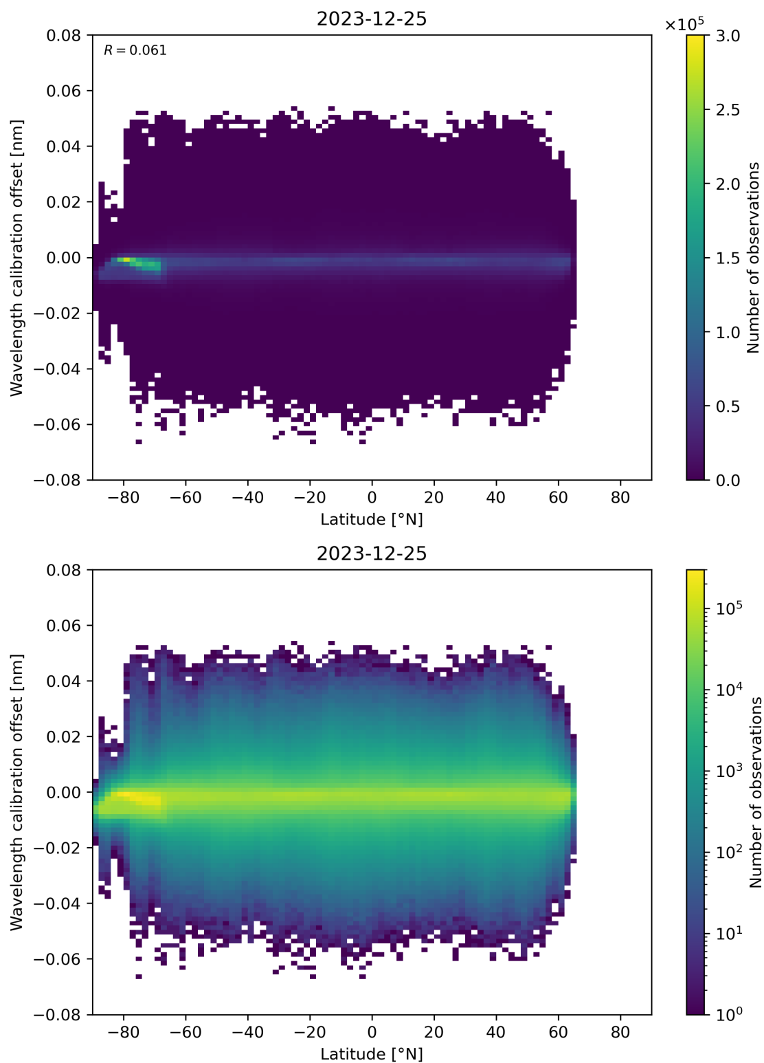
Figure 95: Scatter density plot of “Latitude” against “Wavelength calibration offset” for 2023-12-25 to 2023-12-26.
