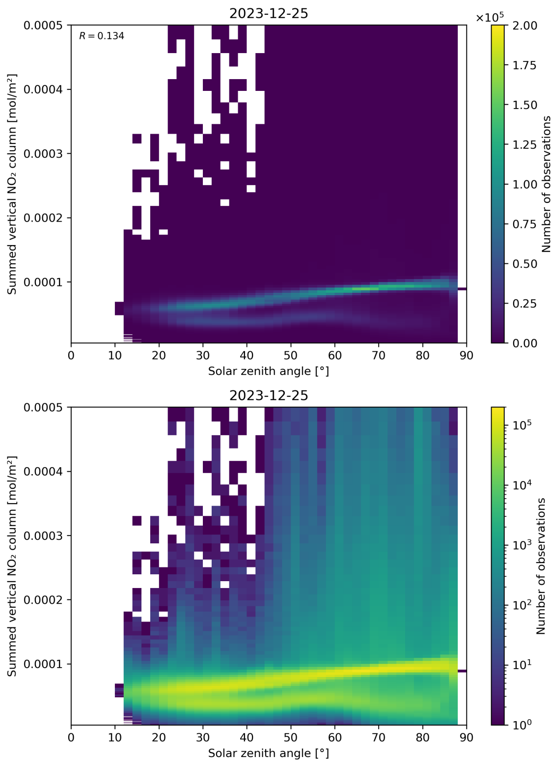
Figure 151: Scatter density plot of “Solar zenith angle” against “Summed vertical NO 2 column” for 2023-12-25 to 2023-12-26.
