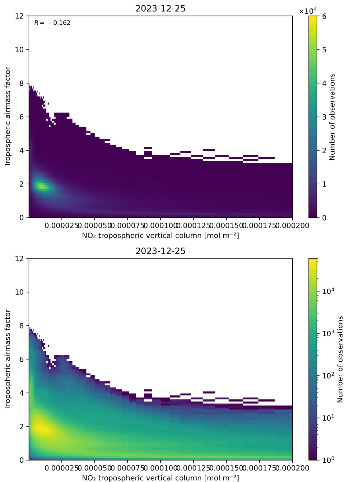
Figure 123: Scatter density plot of “NO 2 tropospheric vertical column” against “Tropospheric air mass factor” for 2023-12-25 to 2023-12-26.
