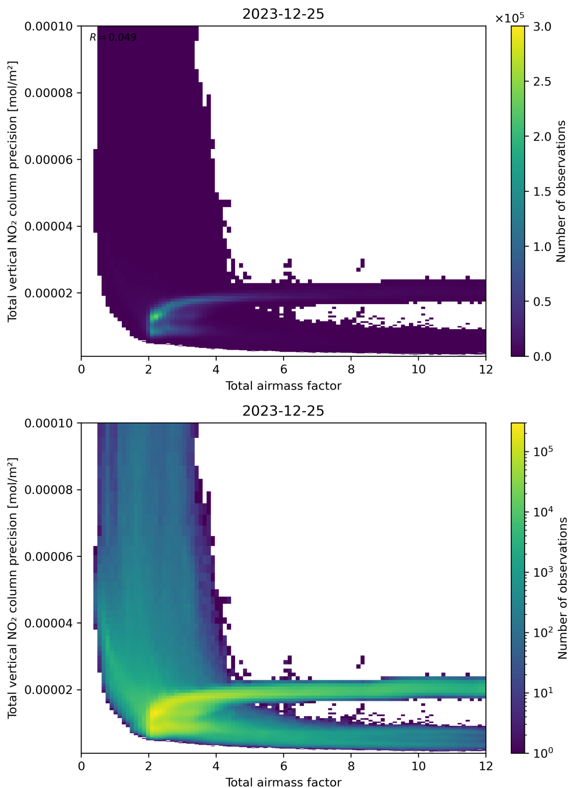
Figure 68: Scatter density plot of “Total airmass factor” against “Total vertical NO 2 column precision” for 2023-12-25 to 2023-12-26.
