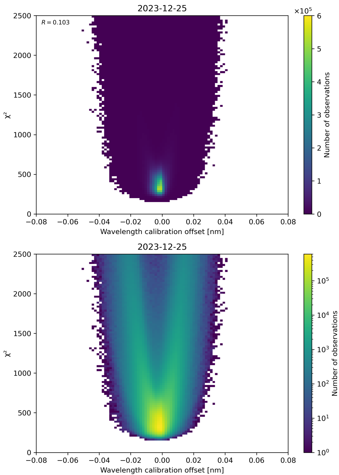
Figure 175: Scatter density plot of “Wavelength calibration offset” against “ \chi^2 ” for 2023-12-25 to 2023-12-26.
