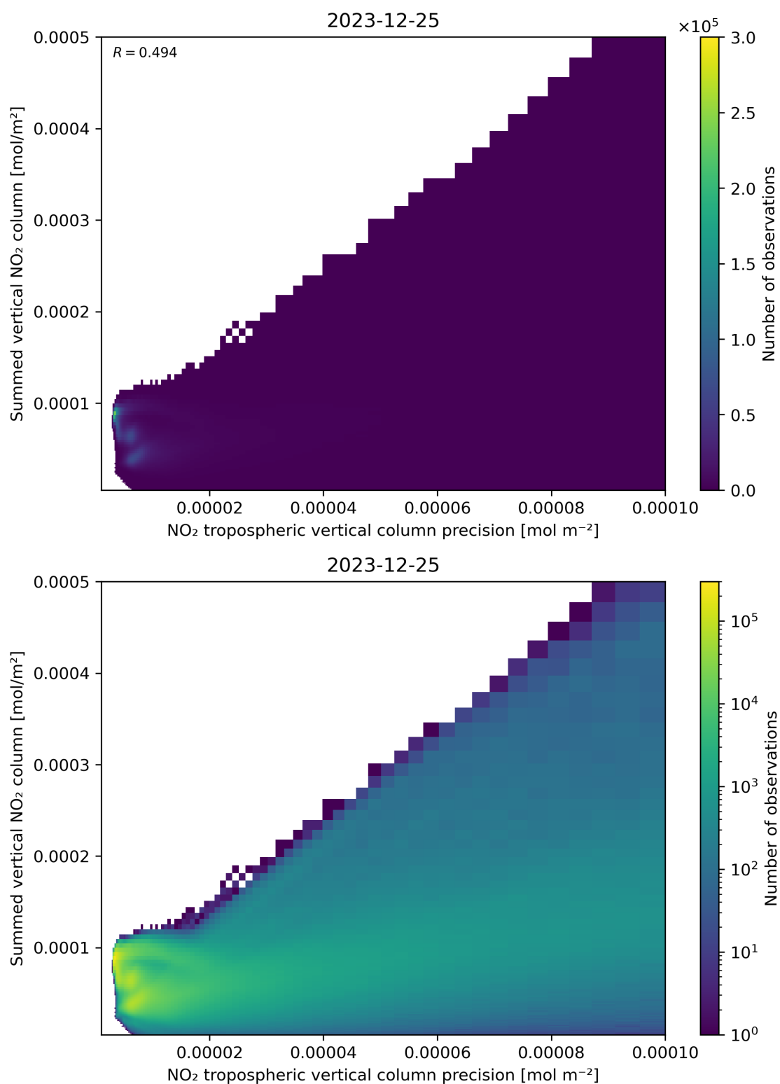
Figure 136: Scatter density plot of “NO 2 tropospheric vertical column precision” against “Summed vertical NO 2 column” for 2023-12-25 to 2023-12-26.
