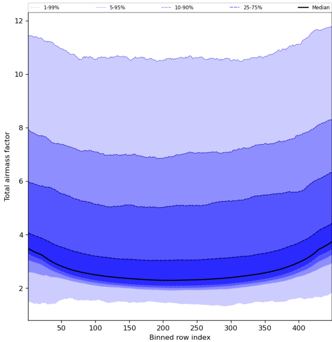
Figure 49: Along track statistics of “Total airmass factor” for 2023-12-25 to 2023-12-26
