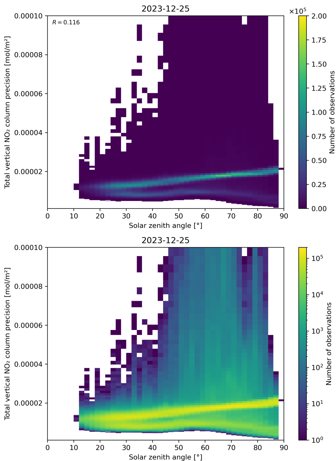
Figure 154: Scatter density plot of “Solar zenith angle” against “Total vertical NO 2 column precision” for 2023-12-25 to 2023-12-26.
