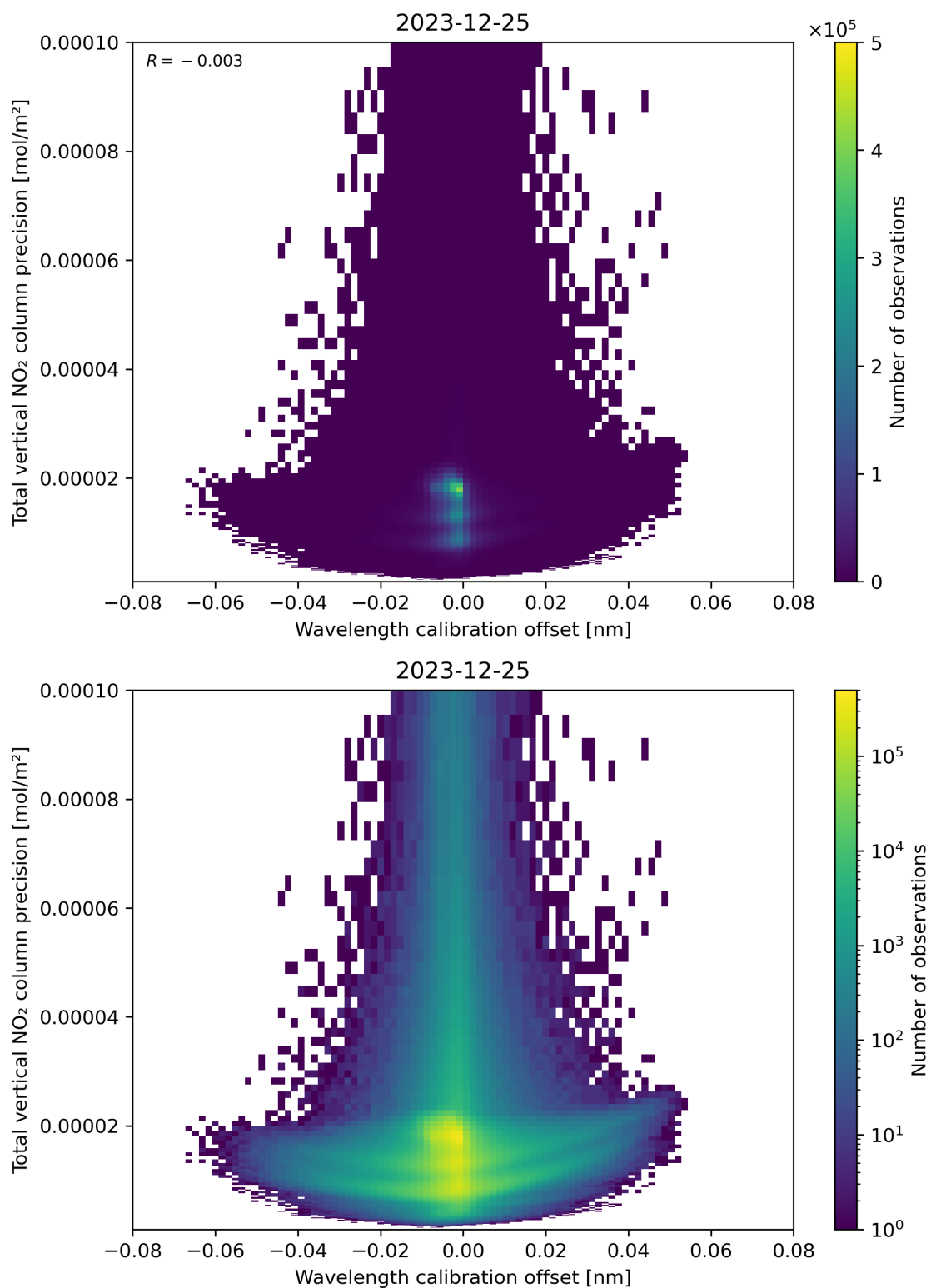
Figure 180: Scatter density plot of “Wavelength calibration offset” against “Total vertical NO 2 column precision” for 2023-12-25 to 2023-12-26.
