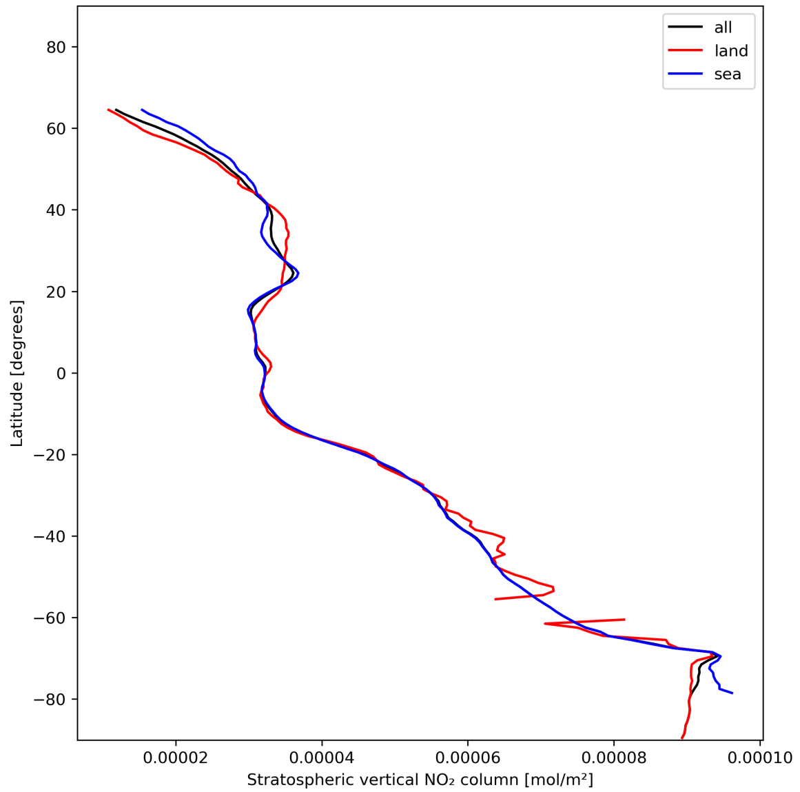
Figure 19: Zonal average of “Stratospheric vertical NO 2 column” for 2023-12-25 to 2023-12-26.
