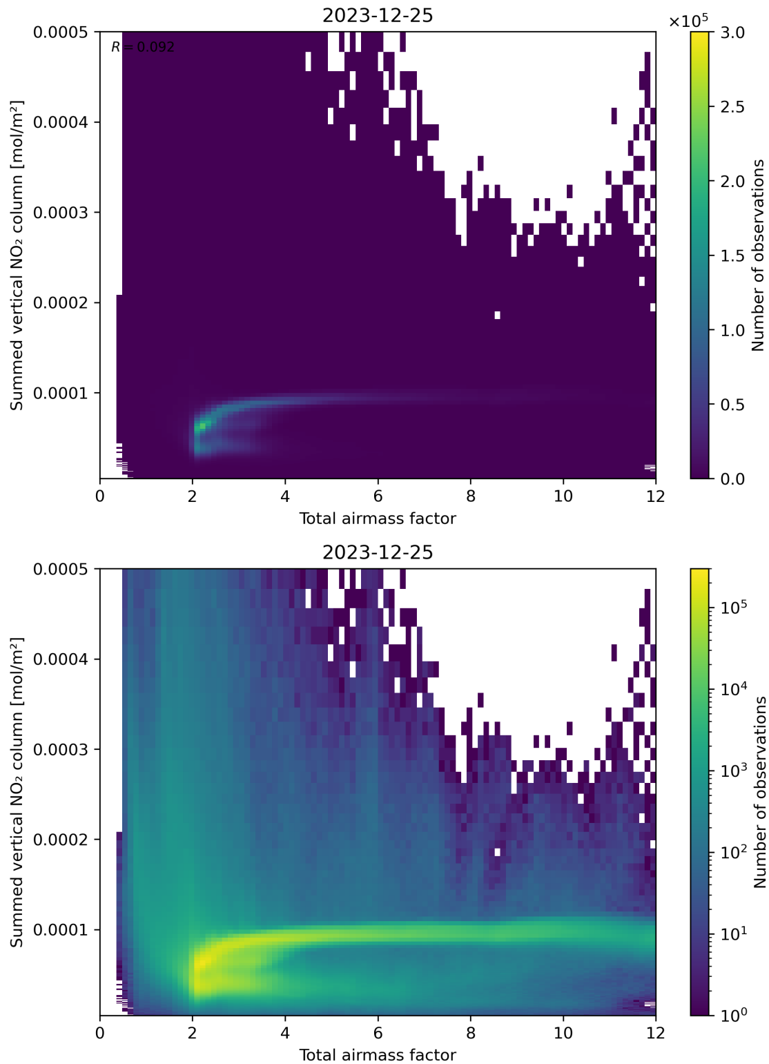
Figure 65: Scatter density plot of “Total airmass factor” against “Summed vertical NO 2 column” for 2023-12-25 to 2023-12-26.
