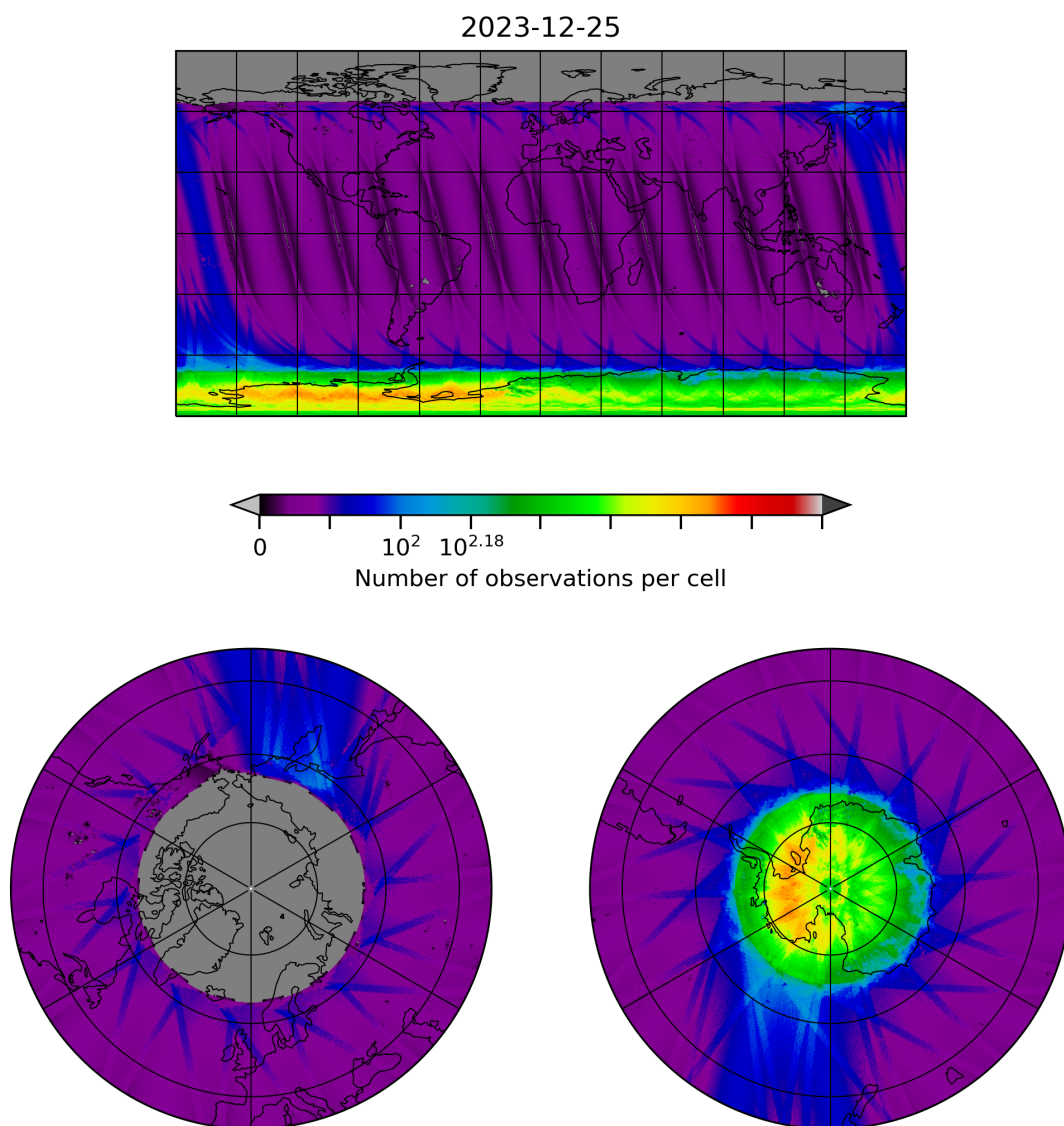
Figure 10: Map of the number of observations for 2023-12-25 to 2023-12-26
