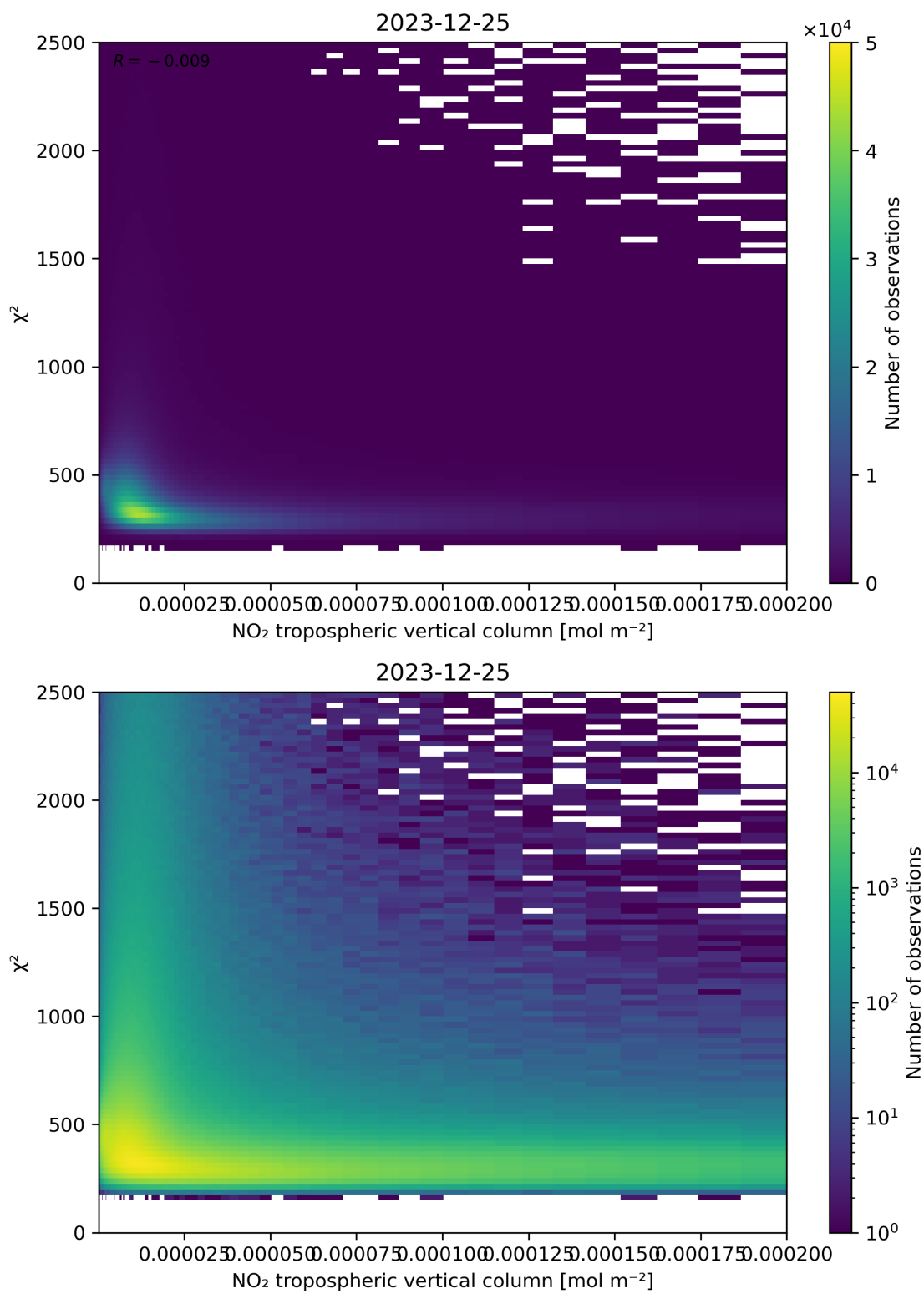
Figure 124: Scatter density plot of “NO 2 tropospheric vertical column” against “ \chi^2 ” for 2023-12-25 to 2023-12-26.
