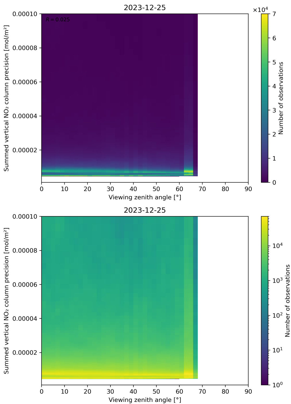
Figure 166: Scatter density plot of “Viewing zenith angle” against “Summed vertical NO 2 column precision” for 2023-12-25 to 2023-12-26.
