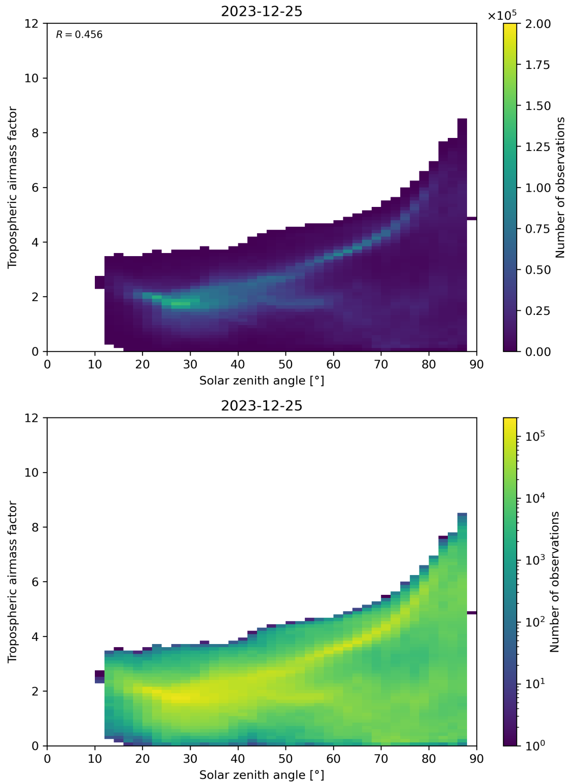
Figure 147: Scatter density plot of “Solar zenith angle” against “Tropospheric airmass factor” for 2023-12-25 to 2023-12-26.
