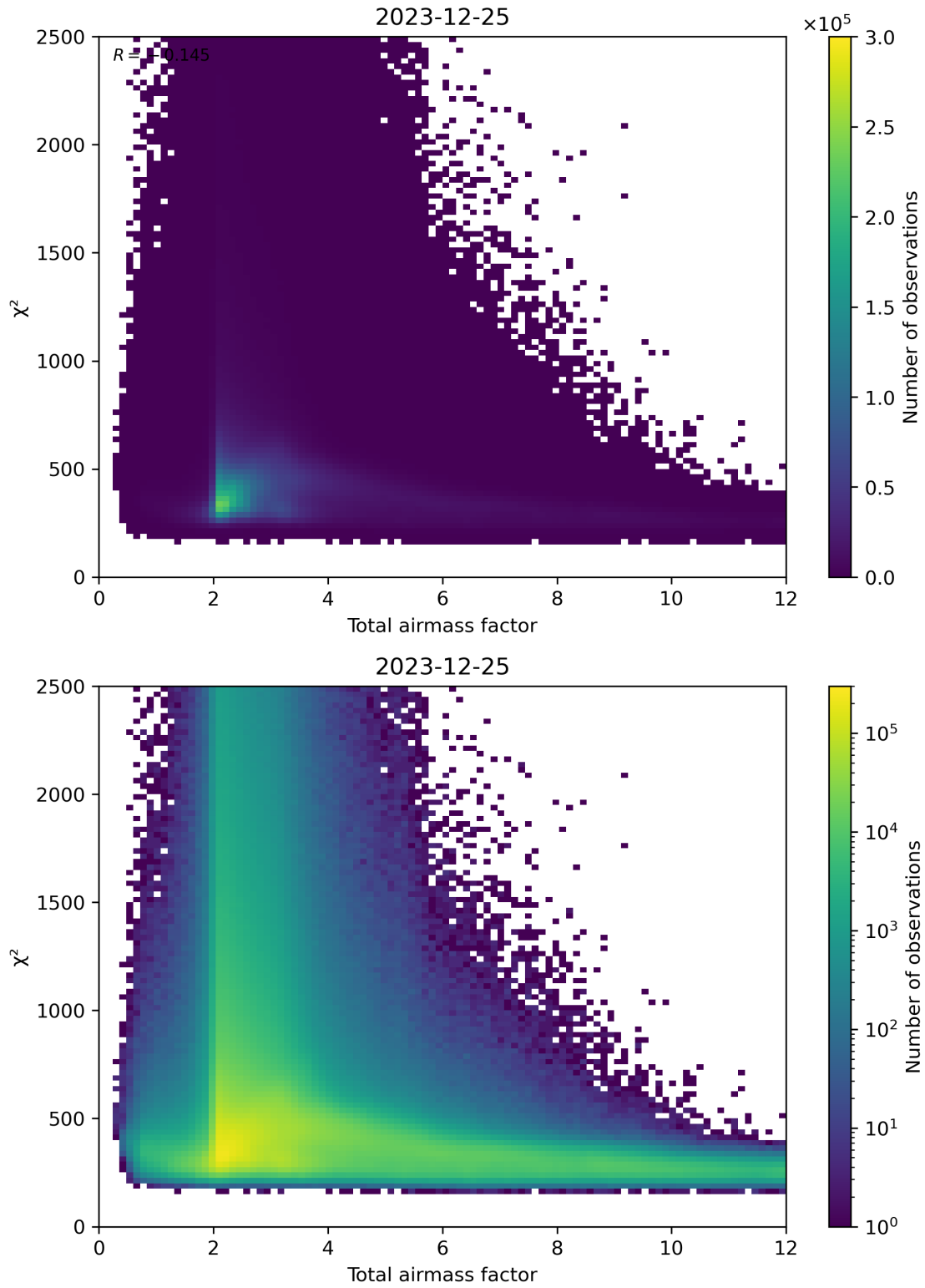
Figure 63: Scatter density plot of “Total airmass factor” against “ \chi^2 ” for 2023-12-25 to 2023-12-26.
