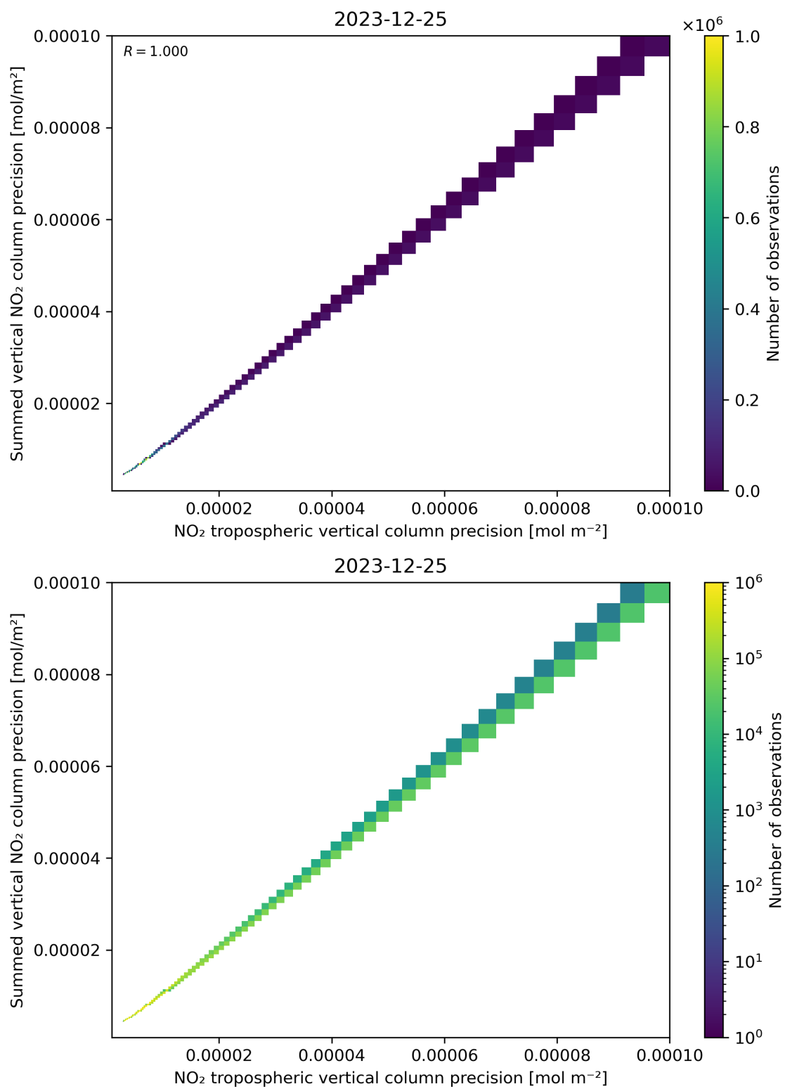
Figure 137: Scatter density plot of “NO 2 tropospheric vertical column precision” against “Summed vertical NO 2 column precision” for 2023-12-25 to 2023-12-26.
