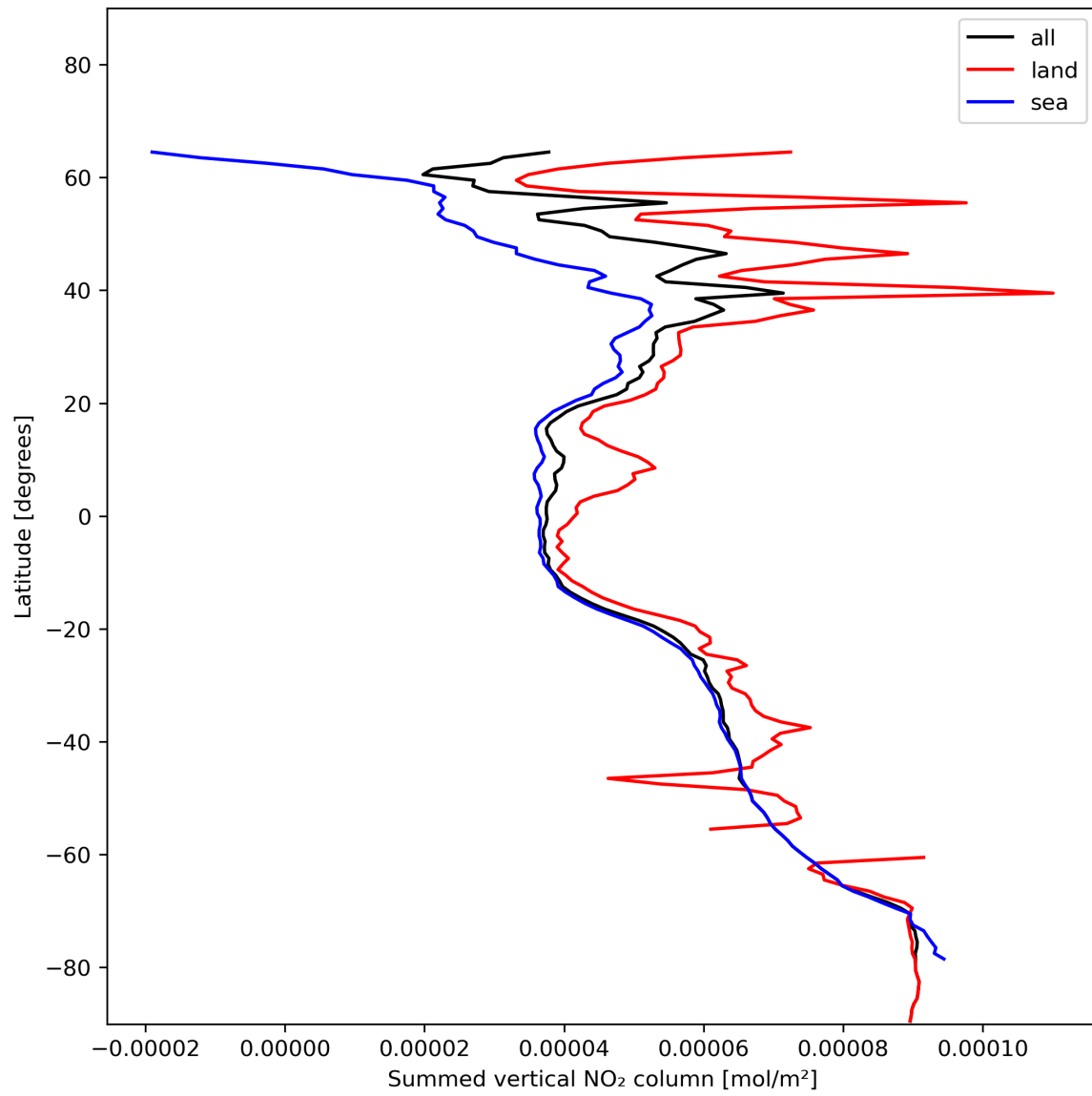
Figure 23: Zonal average of “Summed vertical NO 2 column” for 2023-12-25 to 2023-12-26.
