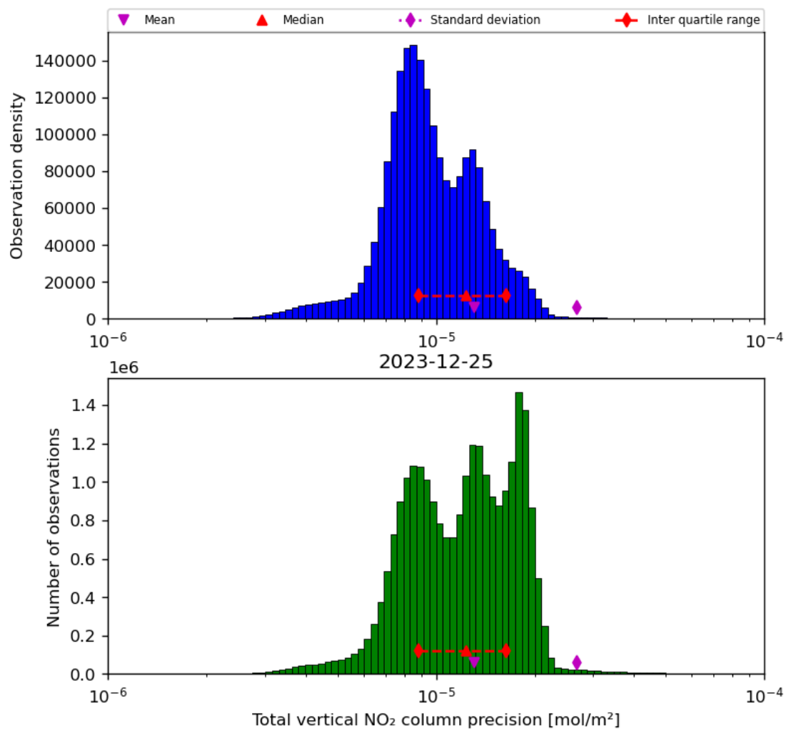
Figure 39: Histogram of “Total vertical NO 2 column precision” for 2023-12-25 to 2023-12-26
