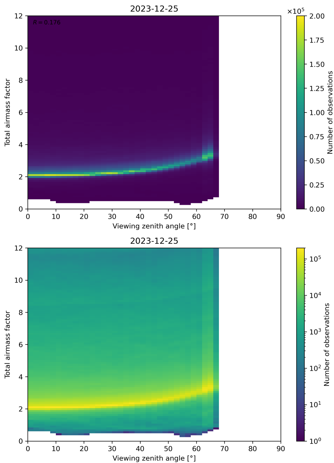
Figure 160: Scatter density plot of “Viewing zenith angle” against “Total airmass factor” for 2023-12-25 to 2023-12-26.
