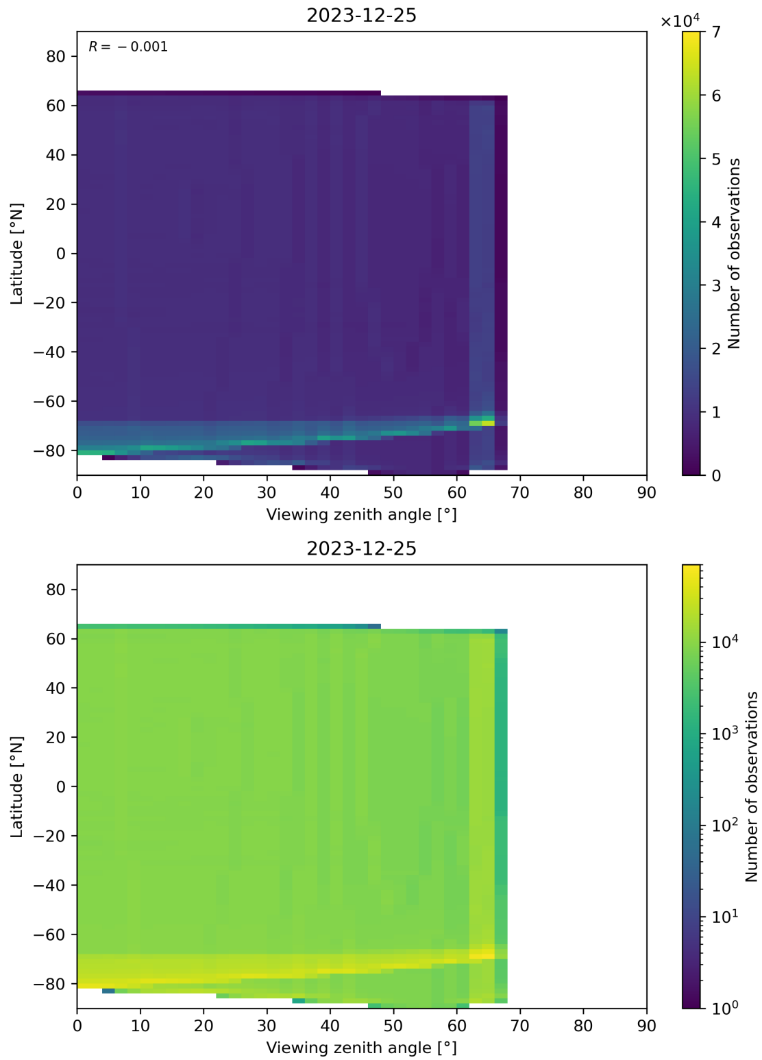
Figure 163: Scatter density plot of “Viewing zenith angle” against “Latitude” for 2023-12-25 to 2023-12-26.
