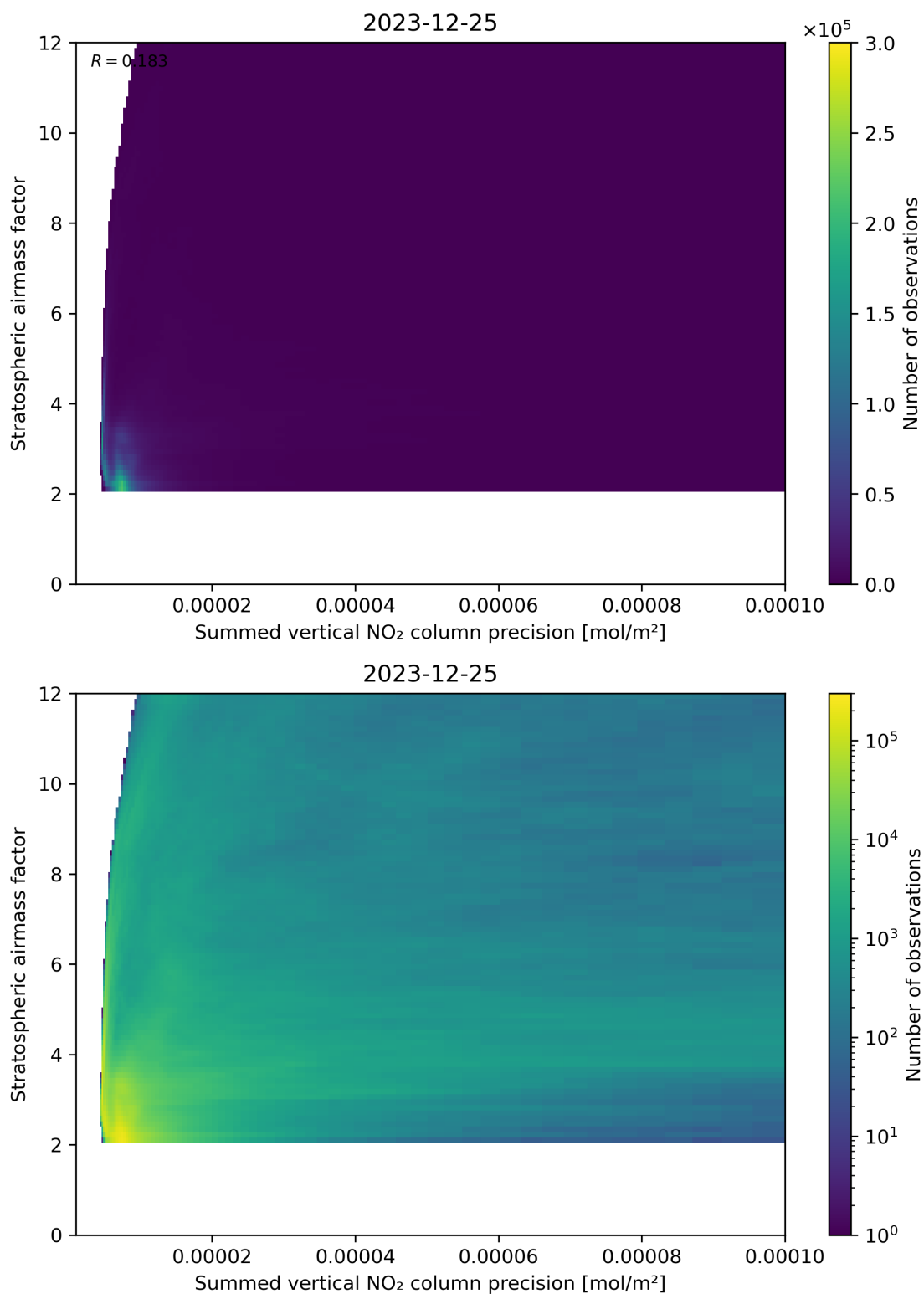
Figure 106: Scatter density plot of “Summed vertical NO 2 column precision” against “Stratospheric airmass factor” for 2023-12-25 to 2023-12-26.
