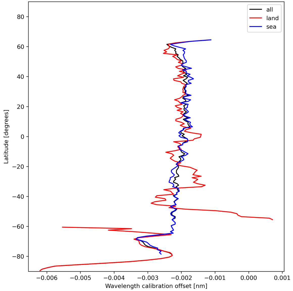
Figure 18: Zonal average of “Wavelength calibration offset” for 2023-12-25 to 2023-12-26.
