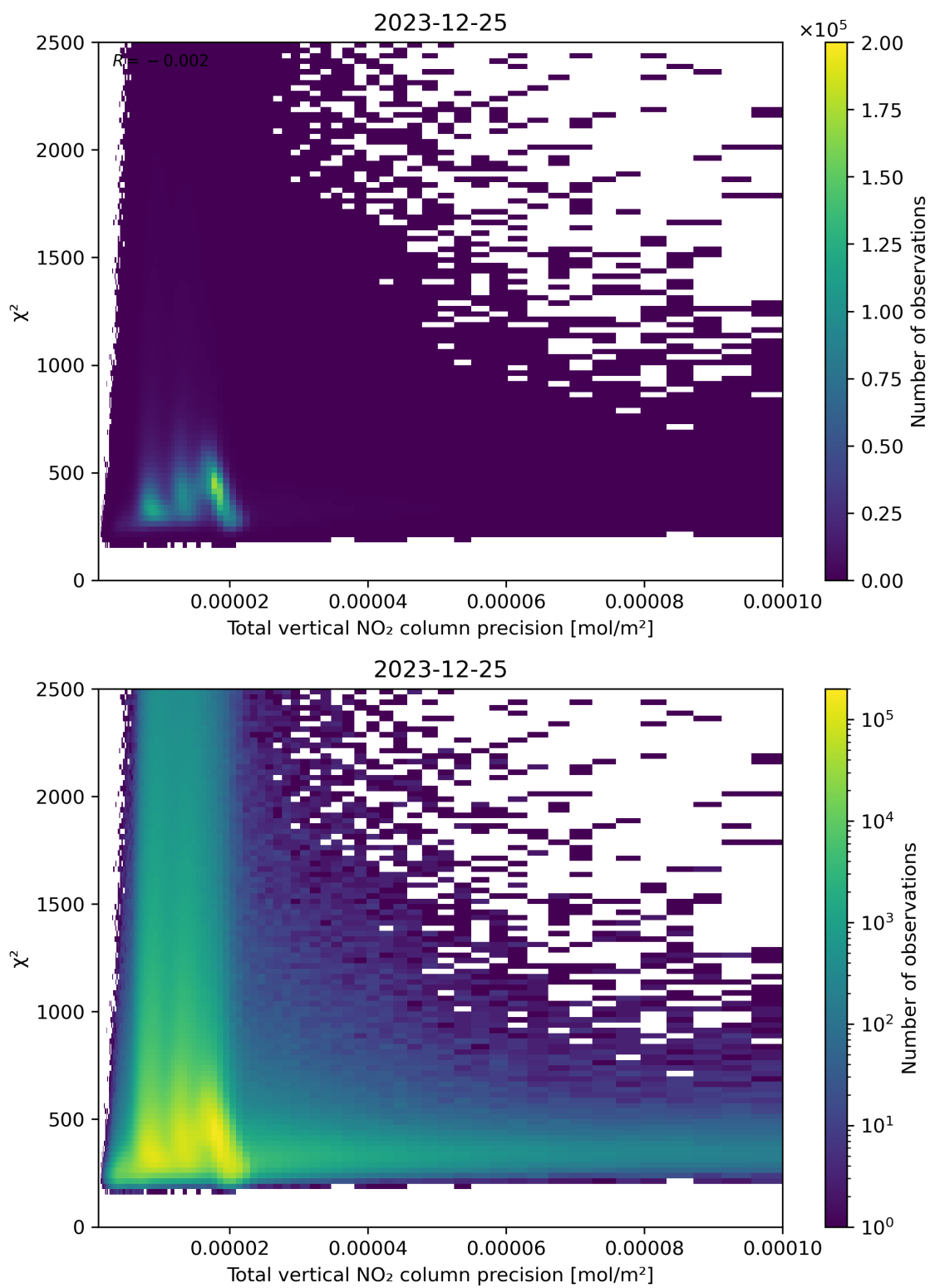
Figure 116: Scatter density plot of “Total vertical NO 2 column precision” against “ \chi^2 ” for 2023-12-25 to 2023-12-26.
