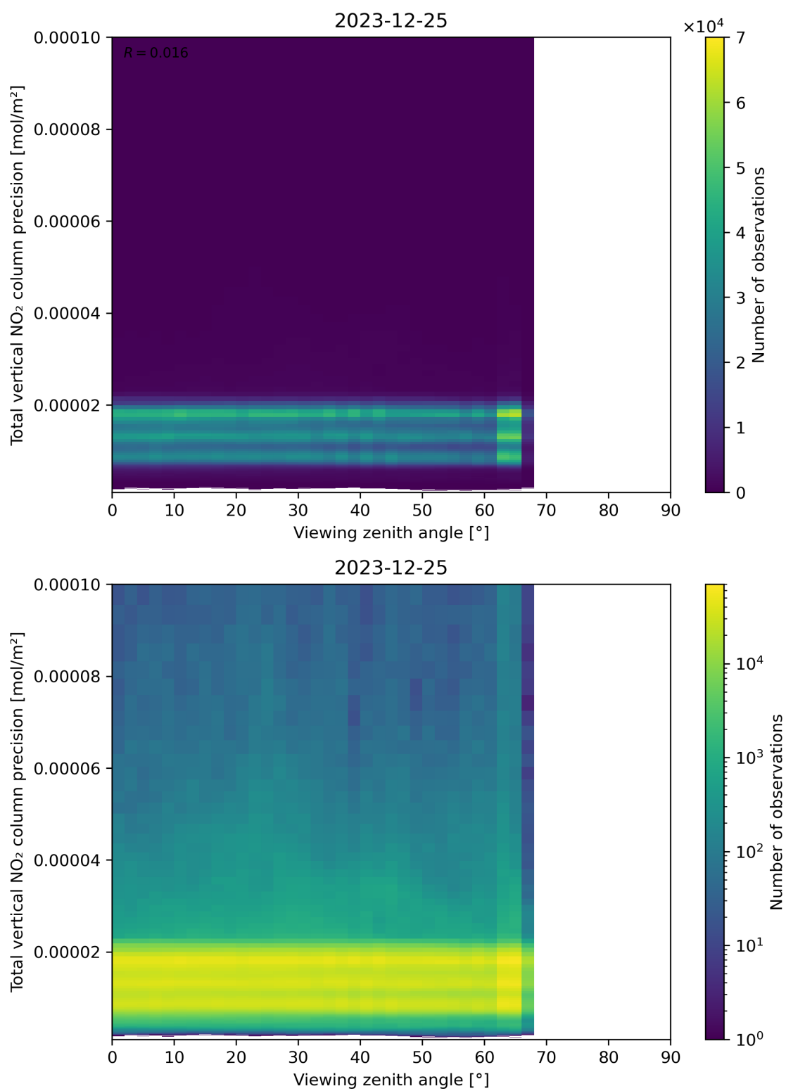
Figure 168: Scatter density plot of “Viewing zenith angle” against “Total vertical NO 2 column precision” for 2023-12-25 to 2023-12-26.
