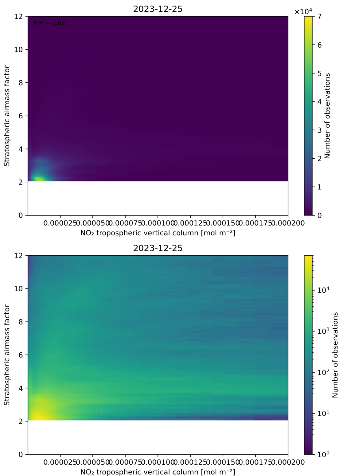
Figure 121: Scatter density plot of “NO 2 tropospheric vertical column” against “Stratospheric airmass factor” for 2023-12-25 to 2023-12-26.
