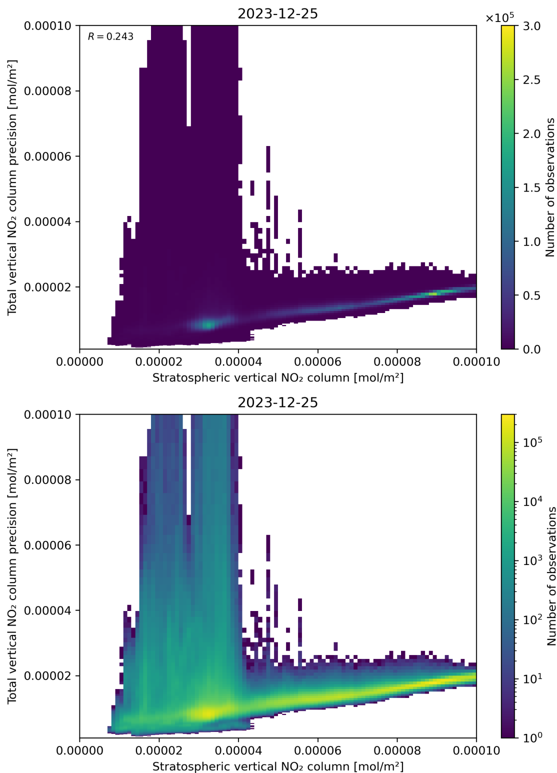
Figure 101: Scatter density plot of “Stratospheric vertical NO 2 column” against “Total vertical NO 2 column precision” for 2023-12-25 to 2023-12-26.
