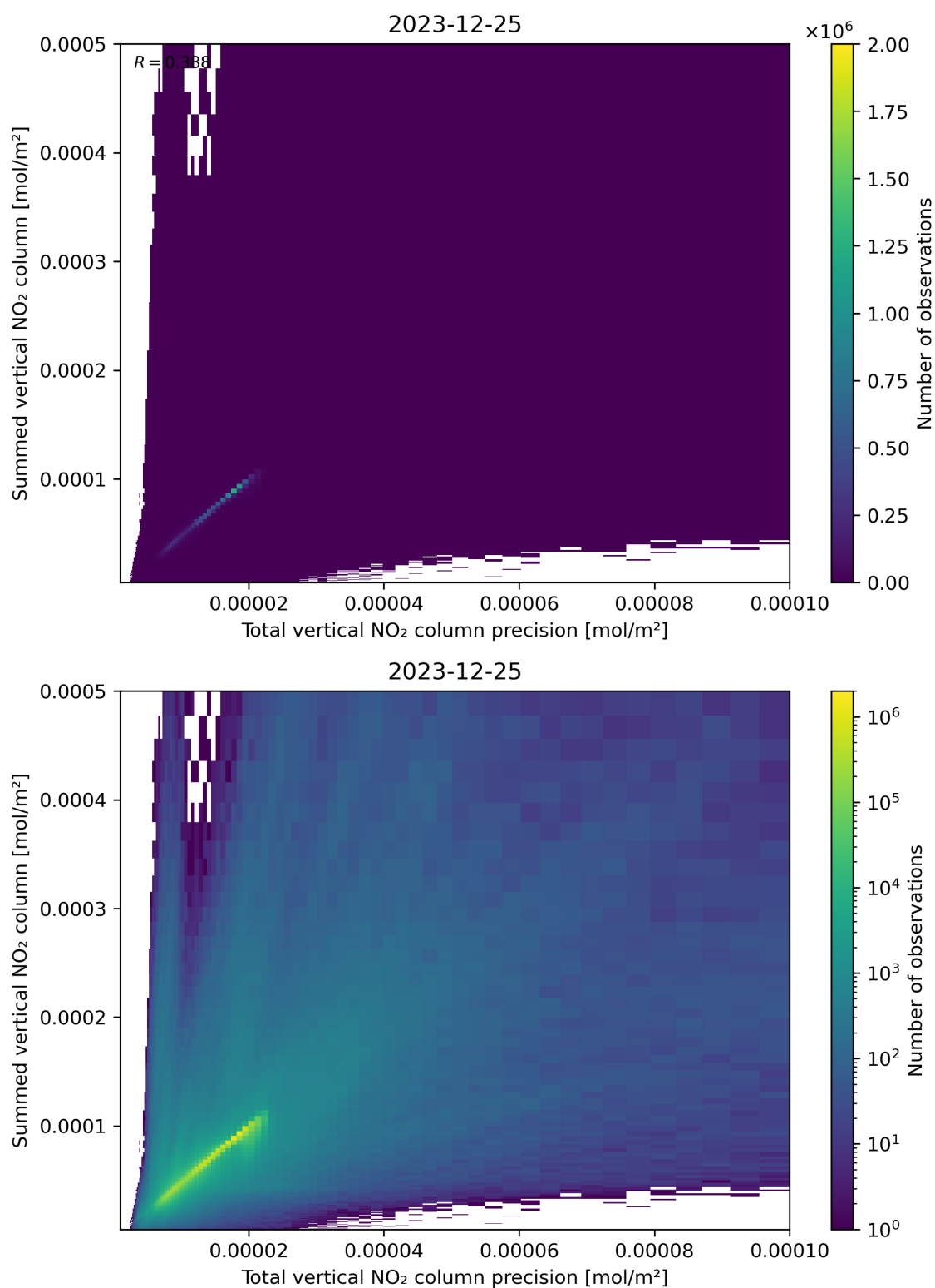
Figure 117: Scatter density plot of “Total vertical NO 2 column precision” against “Summed vertical NO 2 column” for 2023-12-25 to 2023-12-26.
