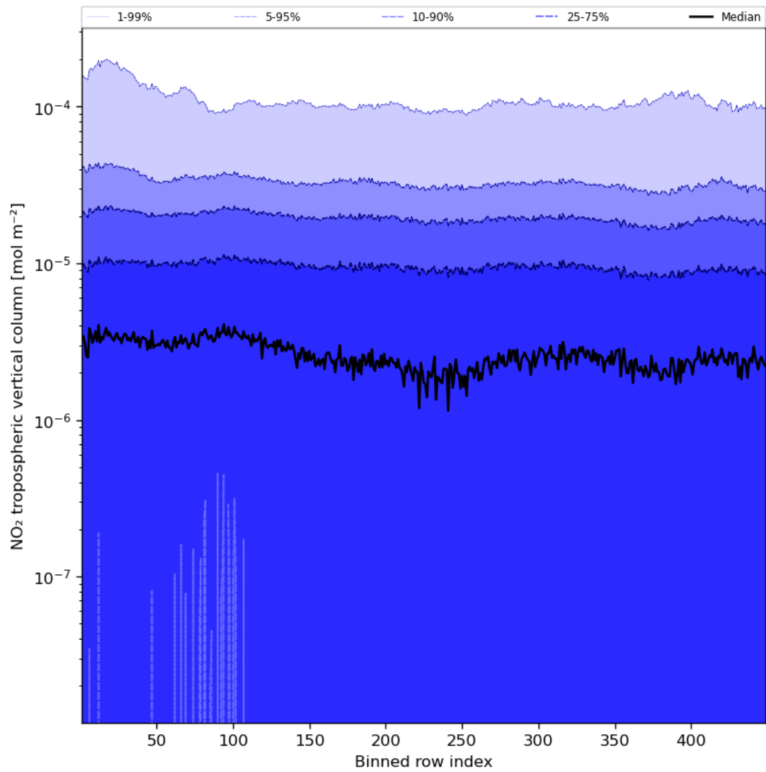
Figure 46: Along track statistics of “NO 2 tropospheric vertical column” for 2023-12-25 to 2023-12-26
