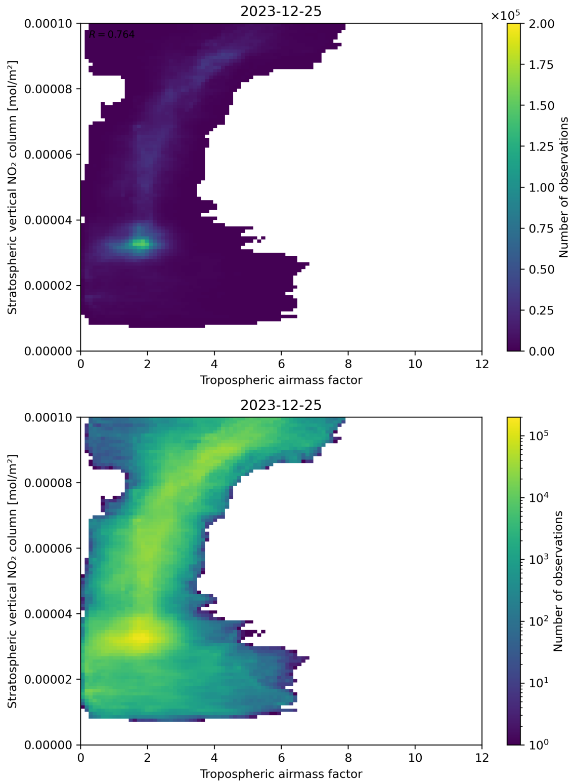
Figure 74: Scatter density plot of “Tropospheric air mass factor” against “Stratospheric vertical NO 2 column” for 2023-12-25 to 2023-12-26.
