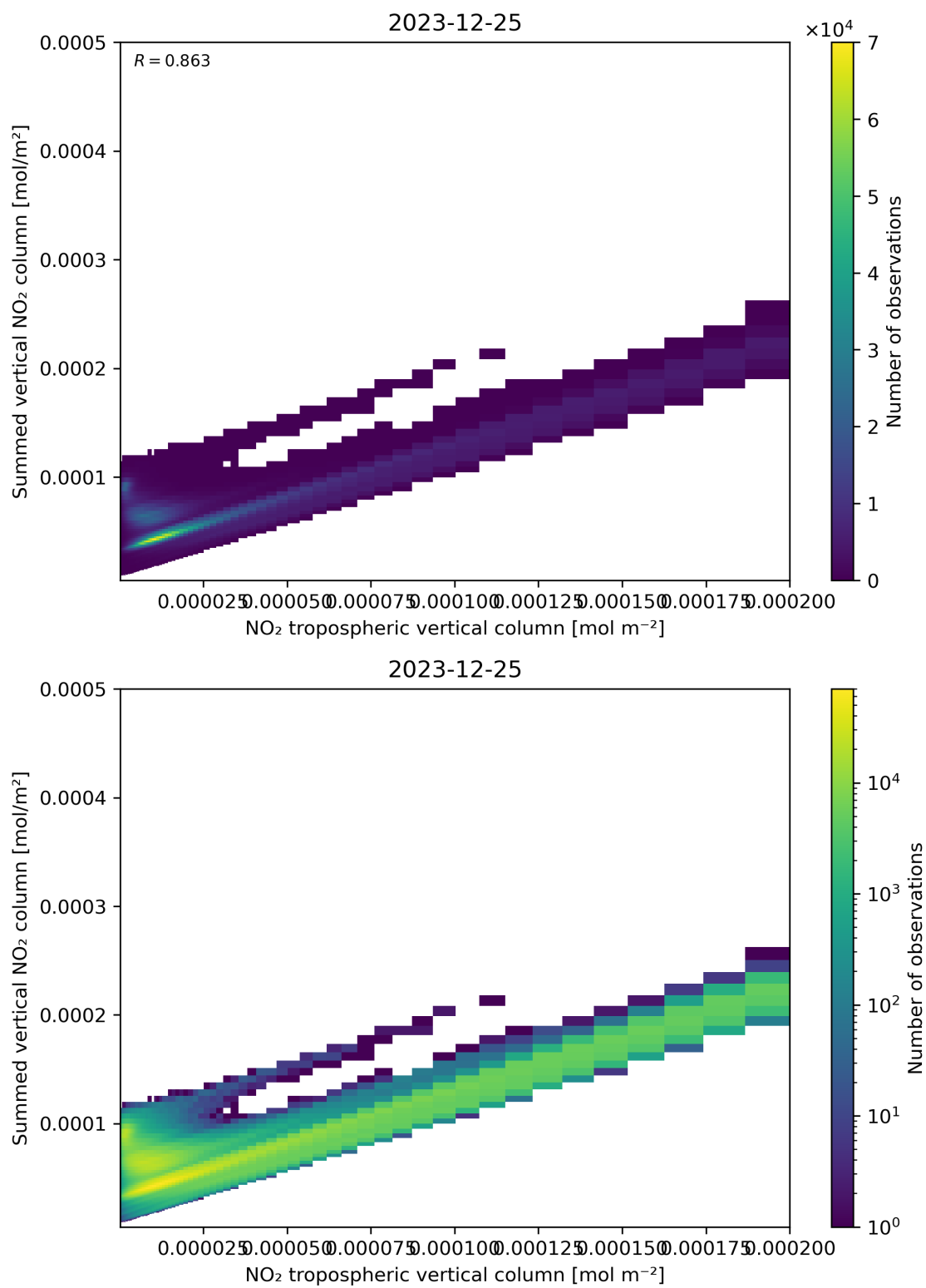
Figure 126: Scatter density plot of “NO 2 tropospheric vertical column” against “Summed vertical NO 2 column” for 2023-12-25 to 2023-12-26.
