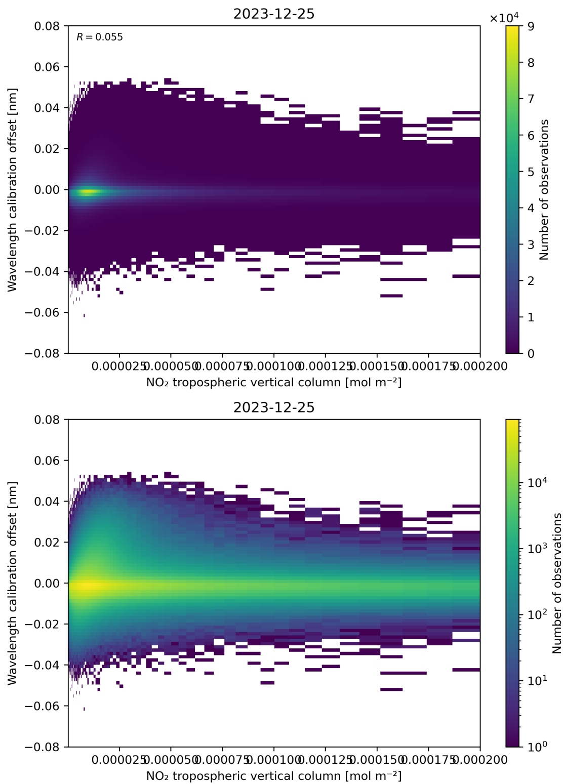
Figure 143: Scatter density plot of “NO 2 tropospheric vertical column” against “Wavelength calibration offset” for 2023-12-25 to 2023-12-26.
