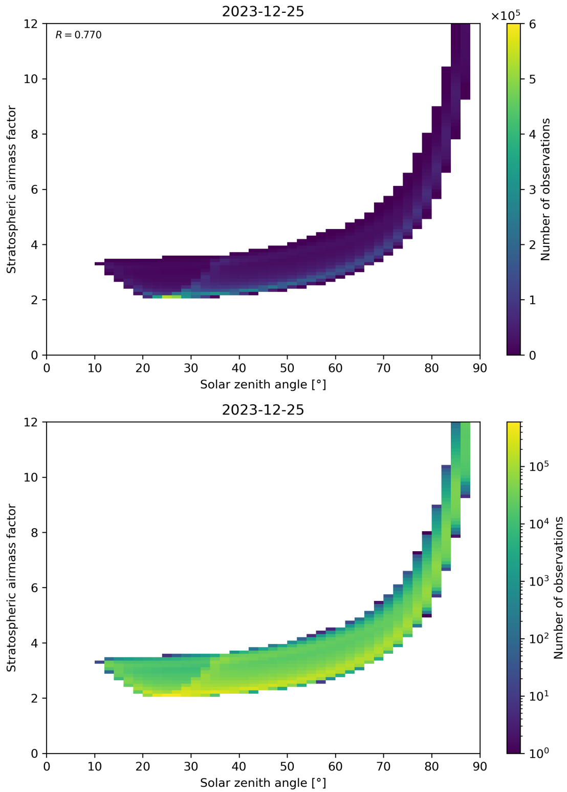
Figure 145: Scatter density plot of “Solar zenith angle” against “Stratospheric airmass factor” for 2023-12-25 to 2023-12-26.
