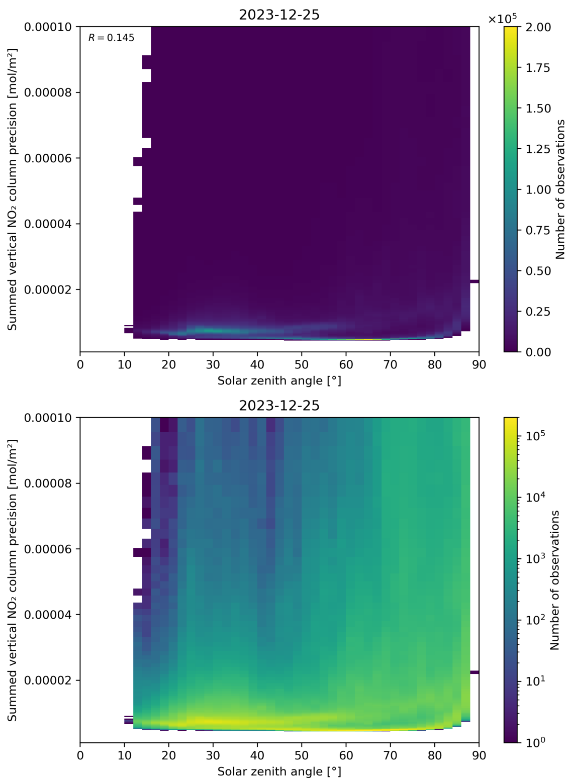
Figure 152: Scatter density plot of “Solar zenith angle” against “Summed vertical NO 2 column precision” for 2023-12-25 to 2023-12-26.
