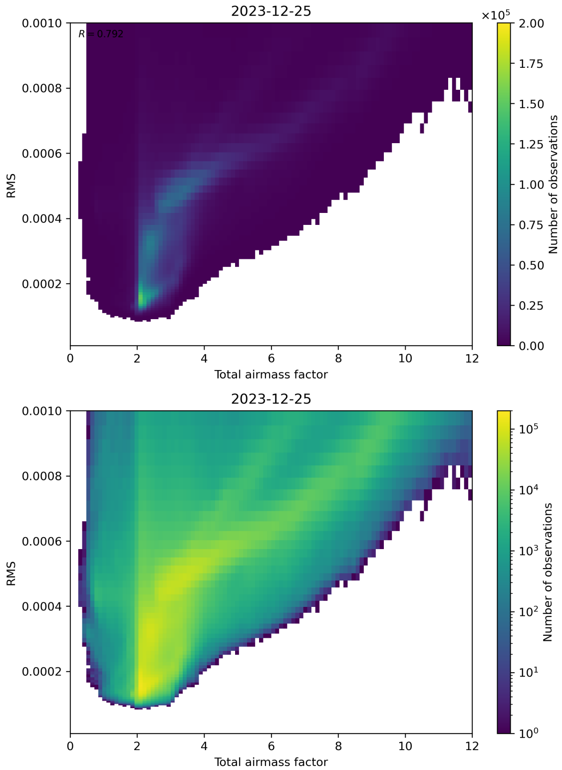
Figure 69: Scatter density plot of “Total airmass factor” against “RMS” for 2023-12-25 to 2023-12-26.
