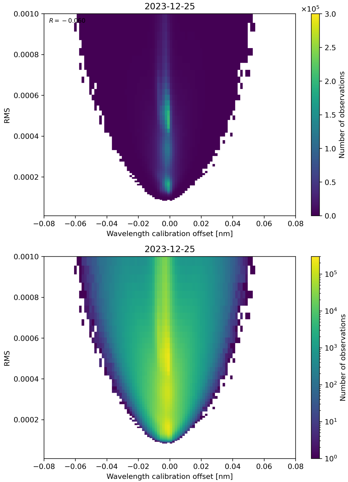
Figure 181: Scatter density plot of “Wavelength calibration offset” against “RMS” for 2023-12-25 to 2023-12-26.
