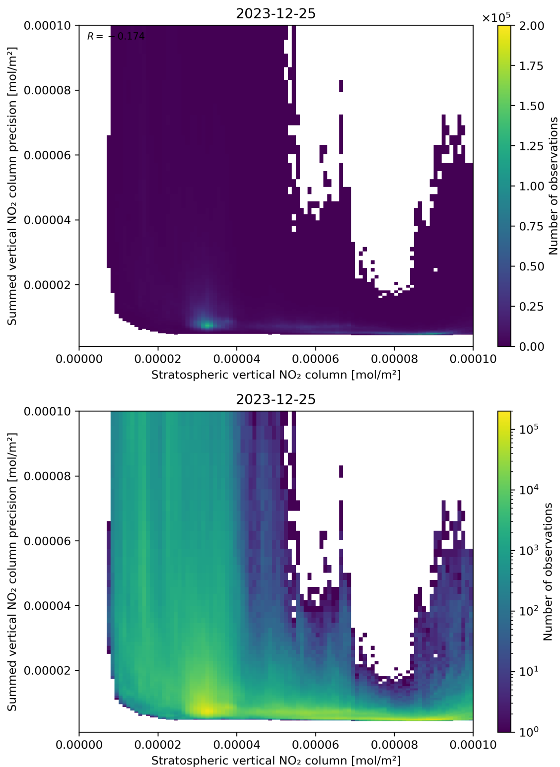
Figure 99: Scatter density plot of “Stratospheric vertical NO 2 column” against “Summed vertical NO 2 column precision” for 2023-12-25 to 2023-12-26.
