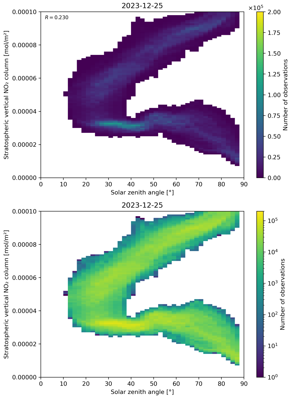
Figure 150: Scatter density plot of “Solar zenith angle” against “Stratospheric vertical NO 2 column” for 2023-12-25 to 2023-12-26.
