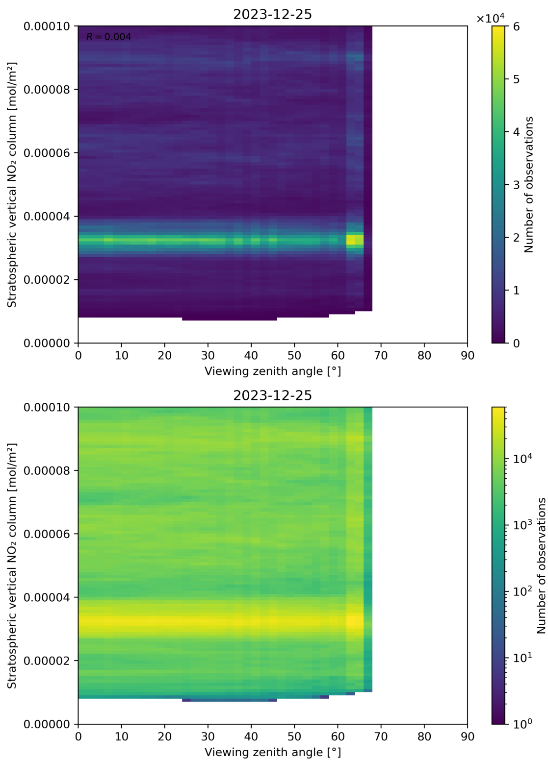
Figure 164: Scatter density plot of “Viewing zenith angle” against “Stratospheric vertical NO 2 column” for 2023-12-25 to 2023-12-26.
