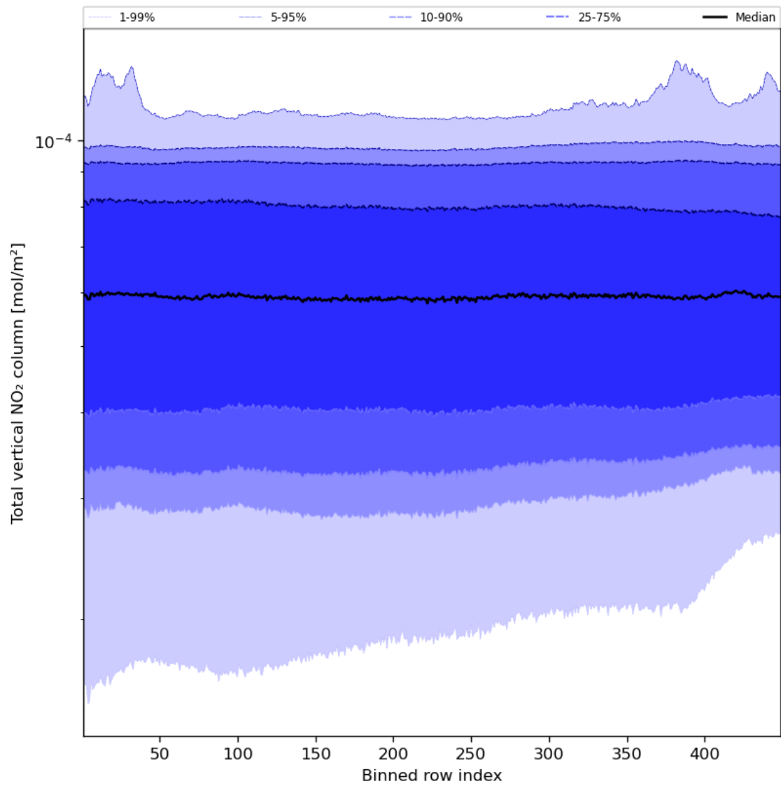
Figure 55: Along track statistics of “Total vertical NO 2 column” for 2023-12-25 to 2023-12-26
