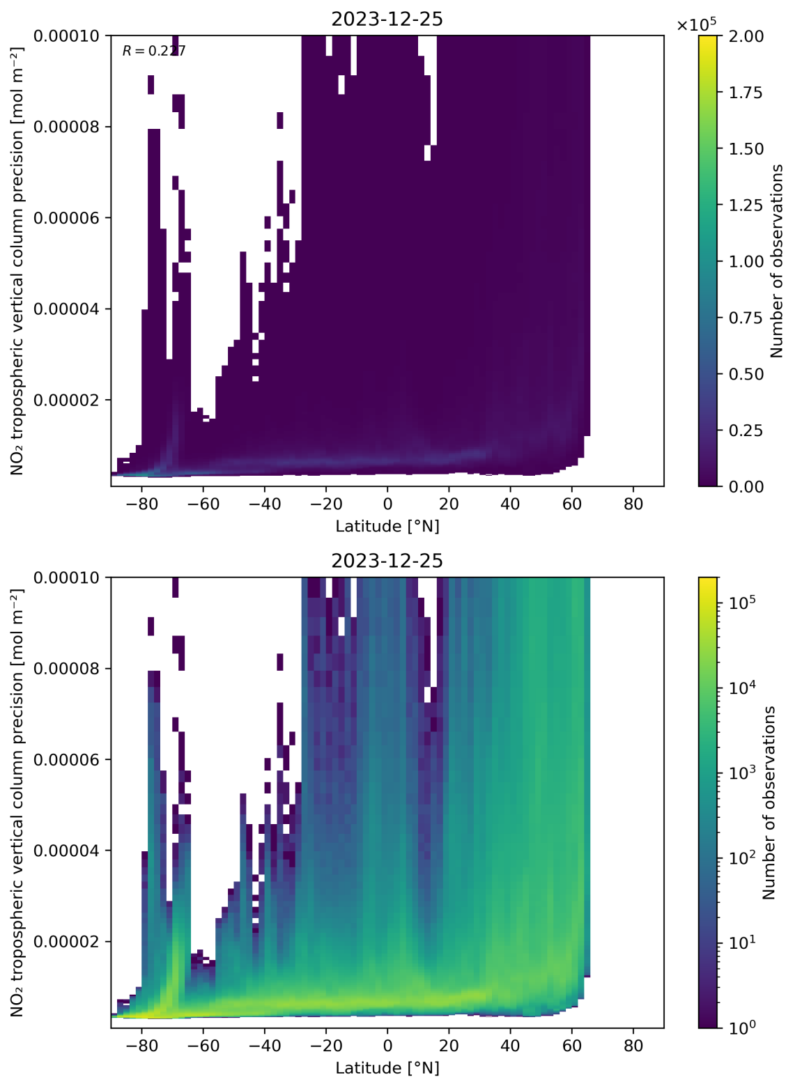
Figure 93: Scatter density plot of “Latitude” against “NO 2 tropospheric vertical column precision” for 2023-12-25 to 2023-12-26.
