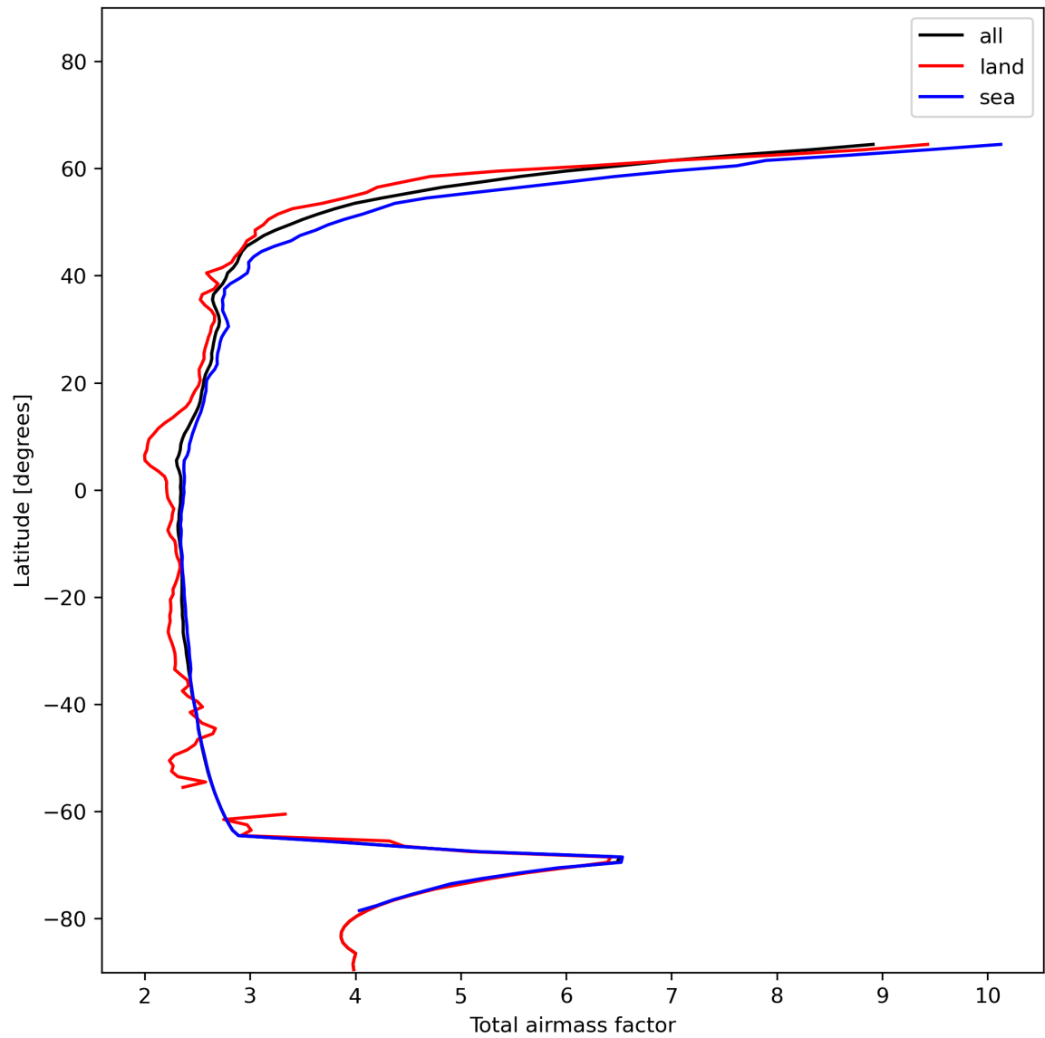
Figure 15: Zonal average of “Total airmass factor” for 2023-12-25 to 2023-12-26.
