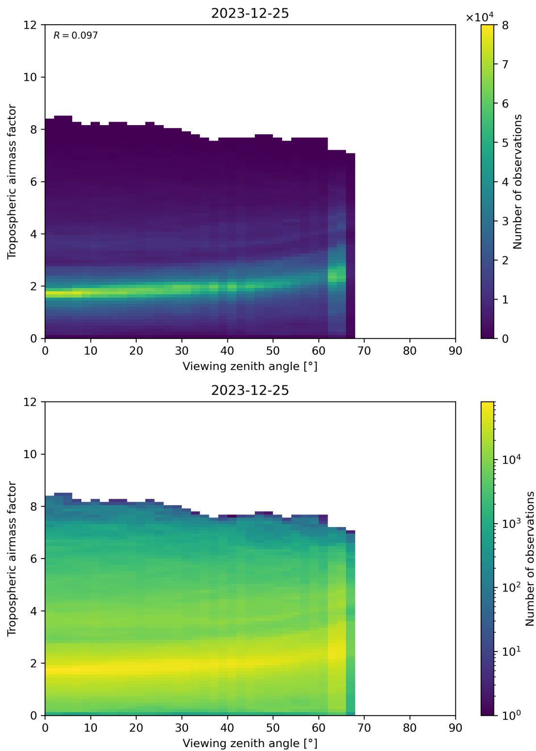
Figure 161: Scatter density plot of “Viewing zenith angle” against “Tropospheric airmass factor” for 2023-12-25 to 2023-12-26.
