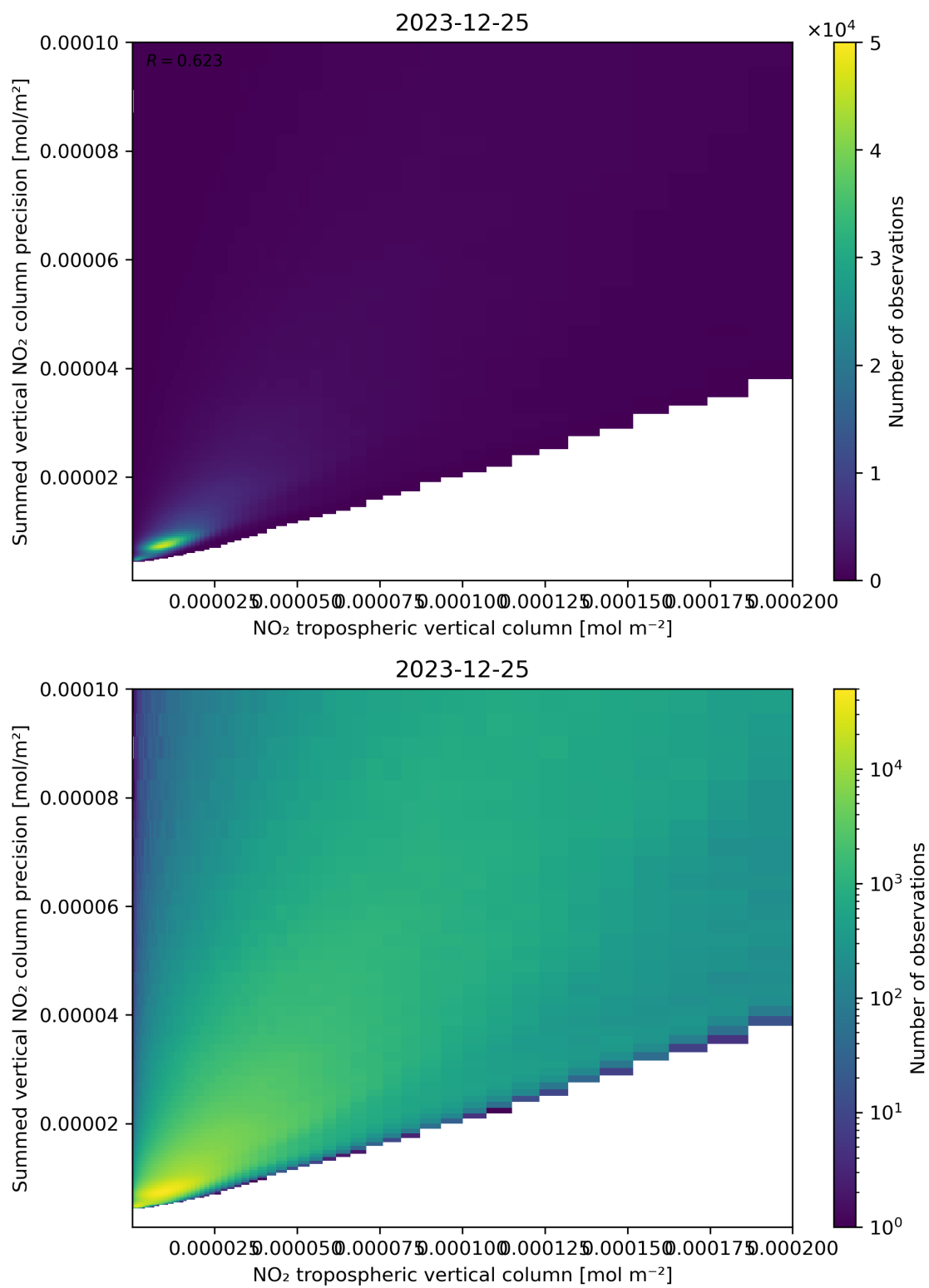
Figure 127: Scatter density plot of “NO 2 tropospheric vertical column” against “Summed vertical NO 2 column precision” for 2023-12-25 to 2023-12-26.
