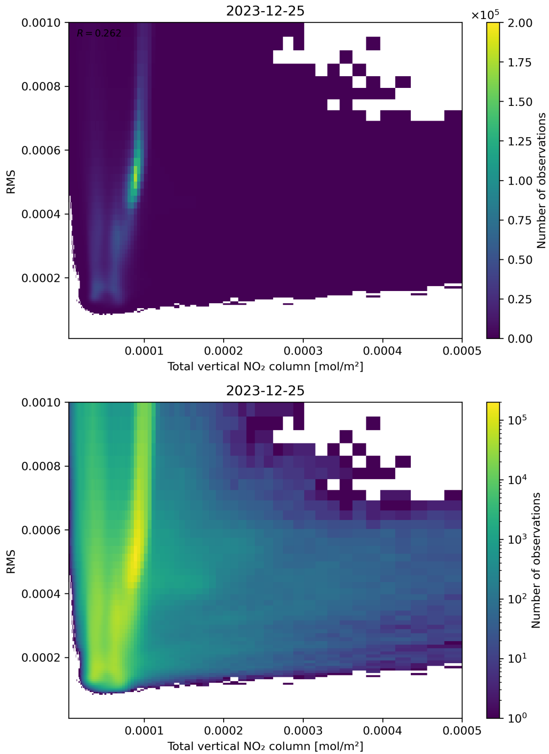
Figure 120: Scatter density plot of “Total vertical NO 2 column” against “RMS” for 2023-12-25 to 2023-12-26.
