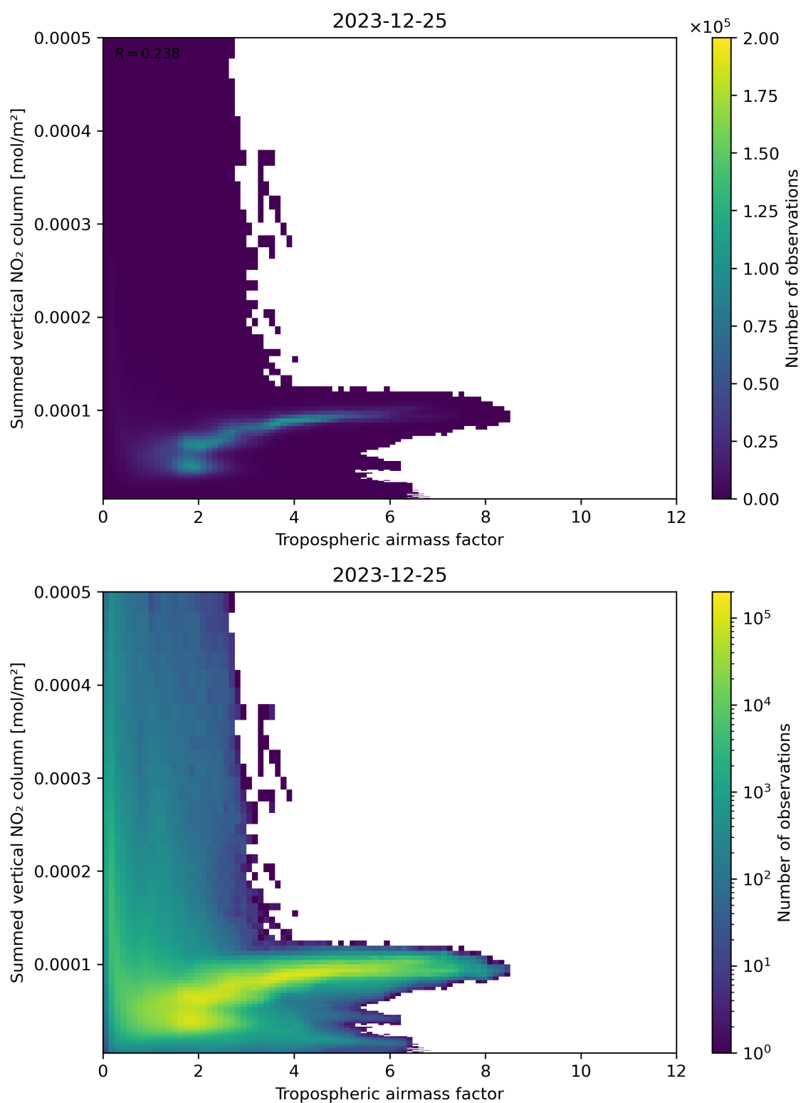
Figure 75: Scatter density plot of “Tropospheric airmass factor” against “Summed vertical NO 2 column” for 2023-12-25 to 2023-12-26.
