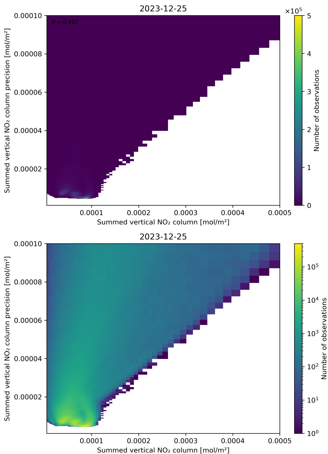
Figure 105: Scatter density plot of “Summed vertical NO 2 column” against “Summed vertical NO 2 column precision” for 2023-12-25 to 2023-12-26.
