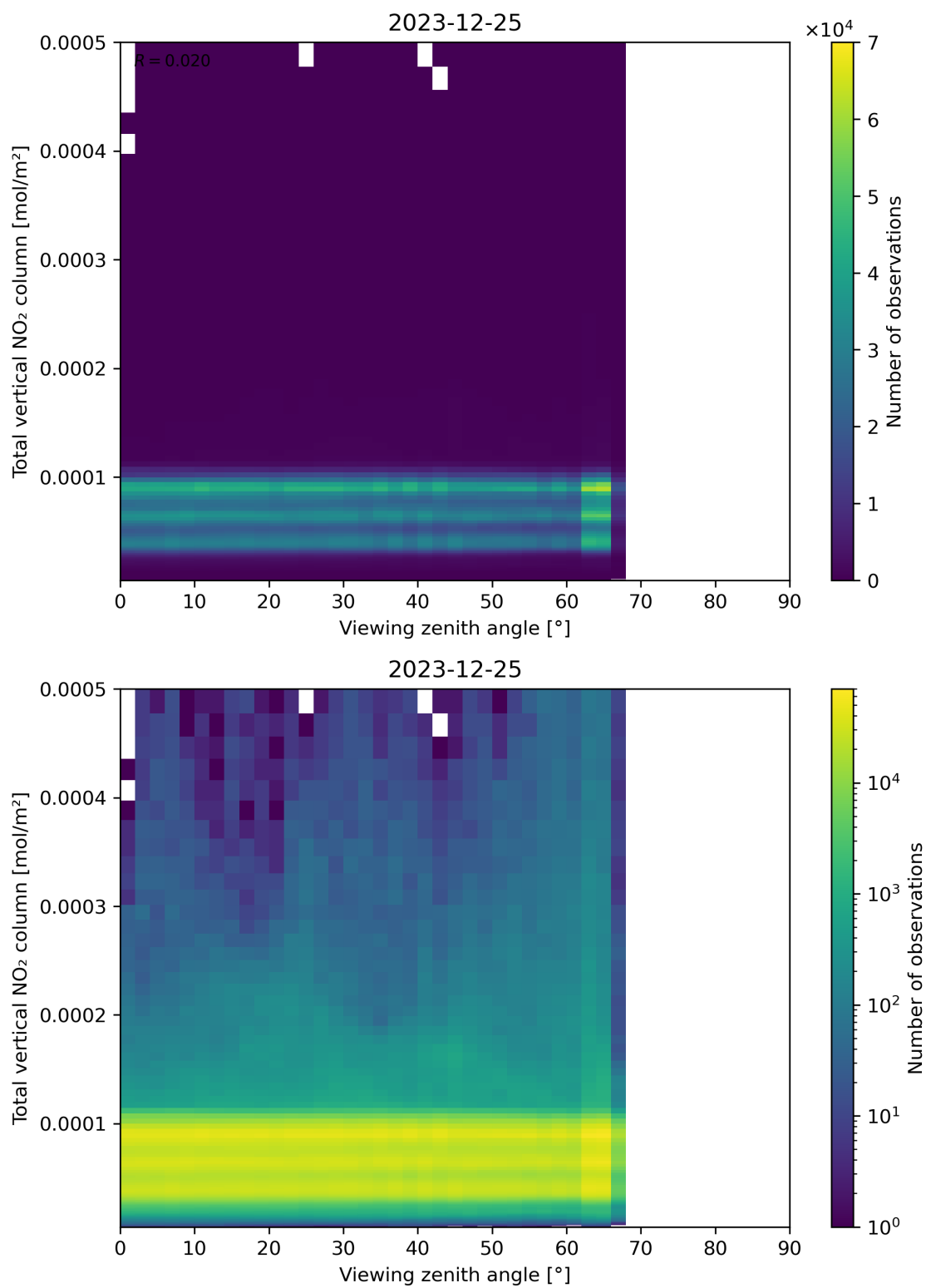
Figure 167: Scatter density plot of “Viewing zenith angle” against “Total vertical NO 2 column” for 2023-12-25 to 2023-12-26.
