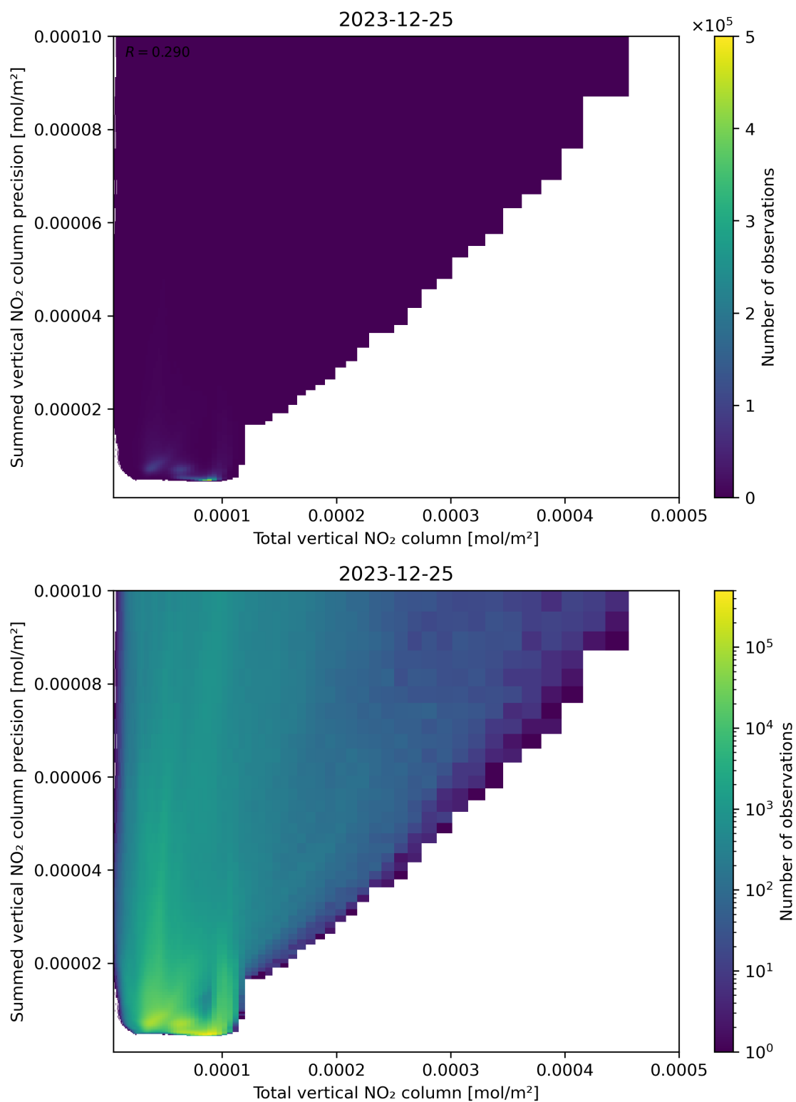
Figure 113: Scatter density plot of “Total vertical NO 2 column” against “Summed vertical NO 2 column precision” for 2023-12-25 to 2023-12-26.
