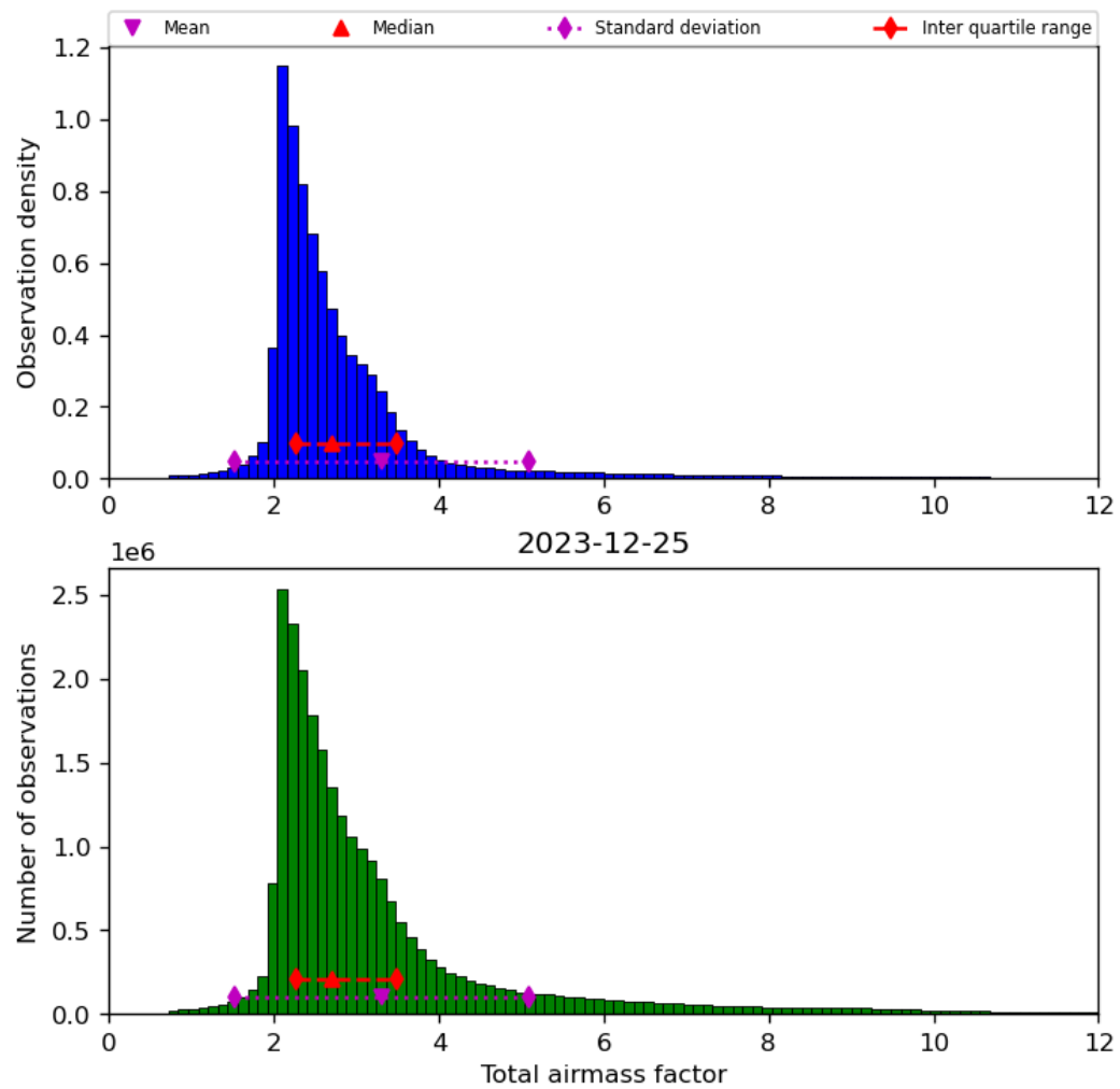
Figure 32: Histogram of “Total airmass factor” for 2023-12-25 to 2023-12-26
