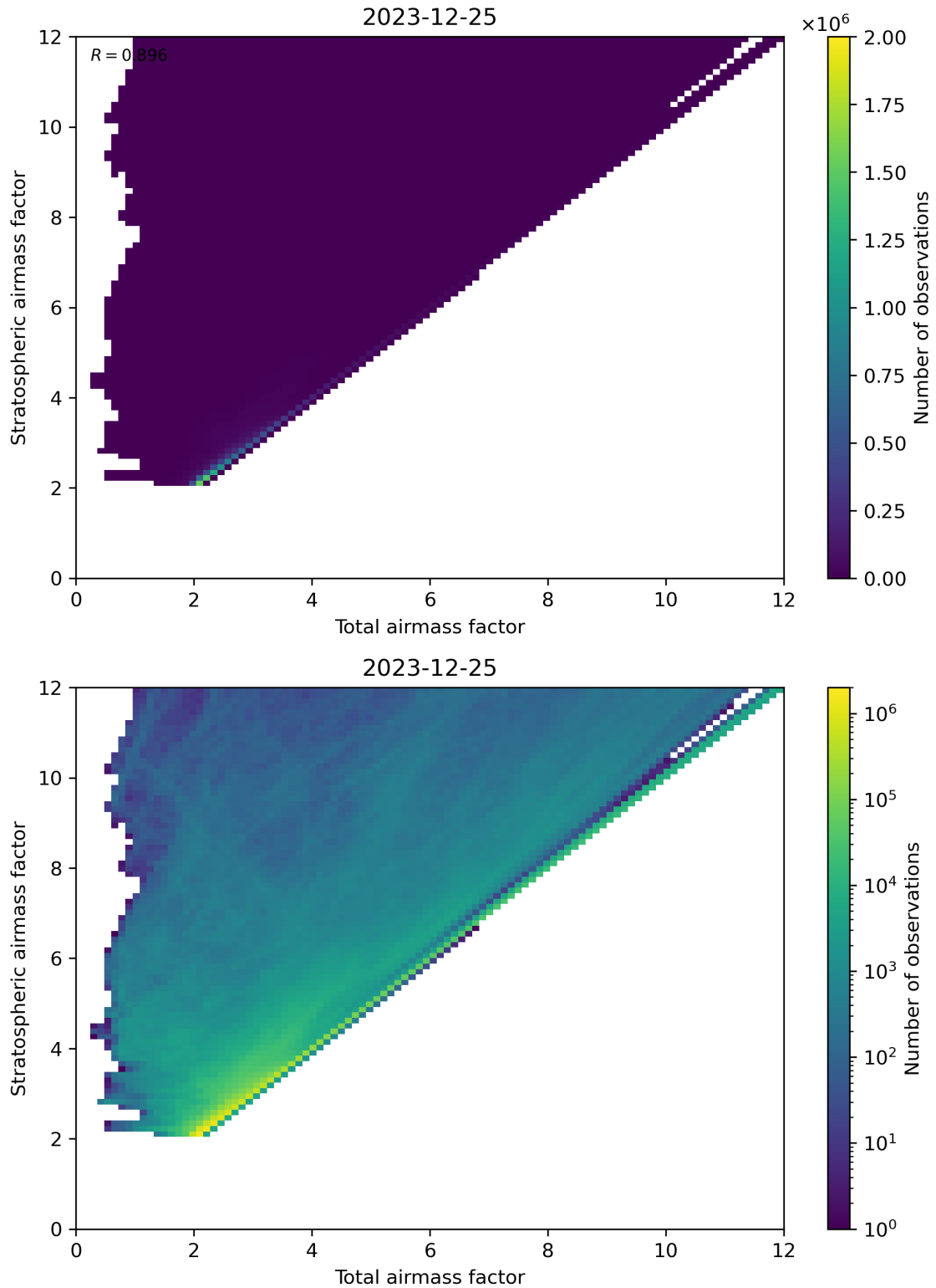
Figure 62: Scatter density plot of “Total airmass factor” against “Stratospheric airmass factor” for 2023-12-25 to 2023-12-26.
