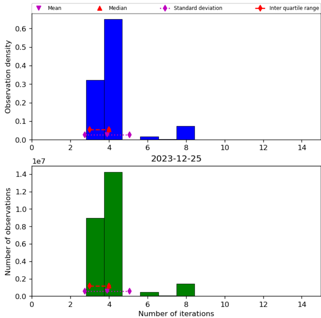
Figure 34: Histogram of “Number of iterations” for 2023-12-25 to 2023-12-26
