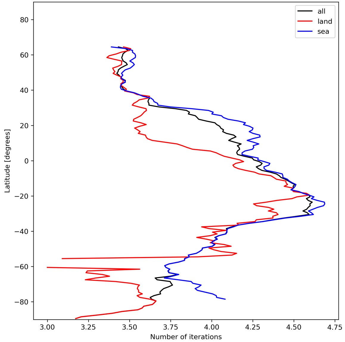
Figure 17: Zonal average of “Number of iterations” for 2023-12-25 to 2023-12-26.
