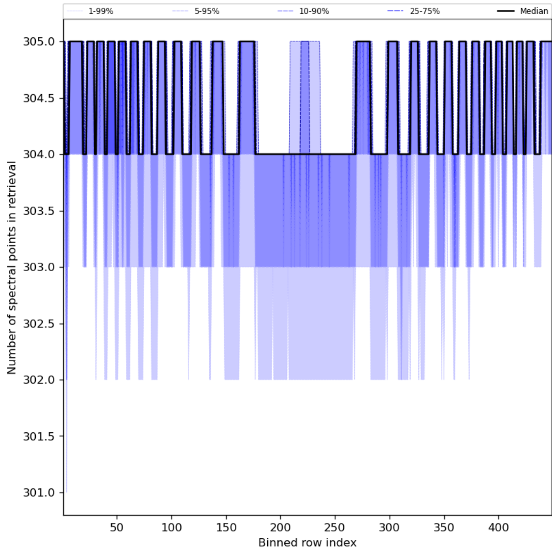
Figure 50: Along track statistics of “Number of spectral points in retrieval” for 2023-12-25 to 2023-12-26
