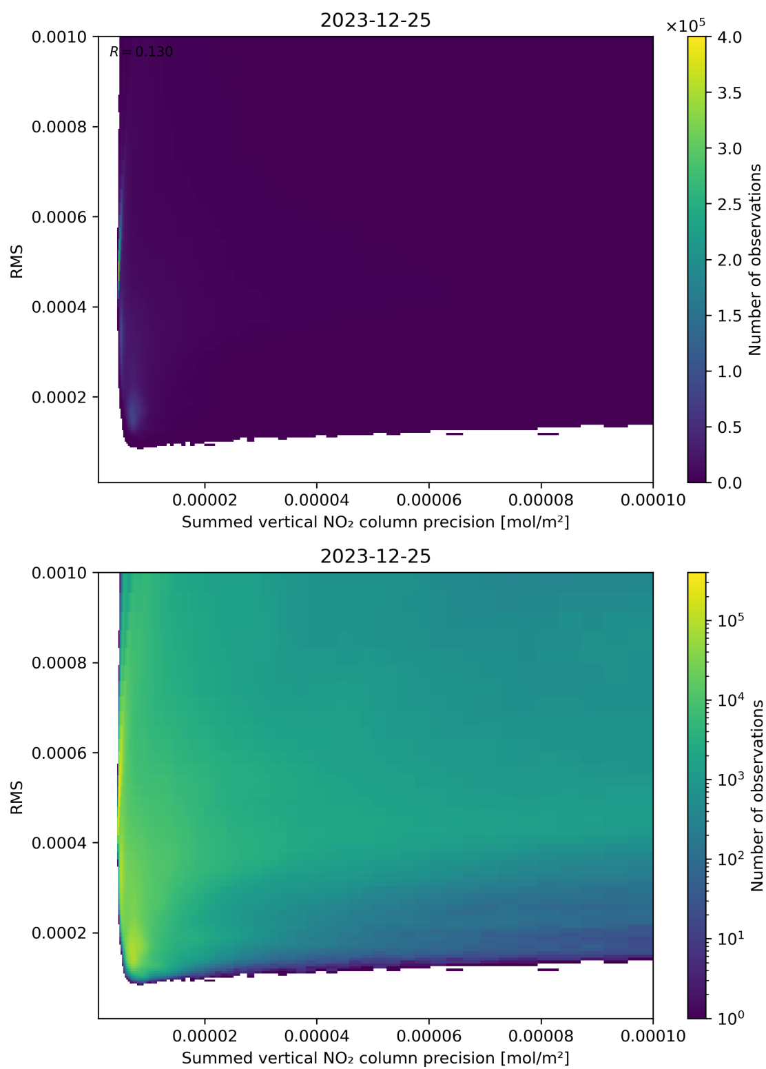
Figure 108: Scatter density plot of “Summed vertical NO 2 column precision” against “RMS” for 2023-12-25 to 2023-12-26.
