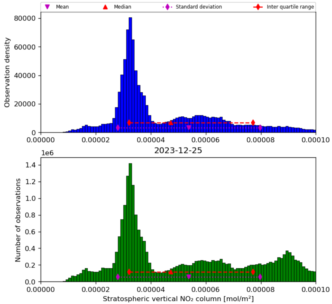
Figure 36: Histogram of “Stratospheric vertical NO 2 column” for 2023-12-25 to 2023-12-26
