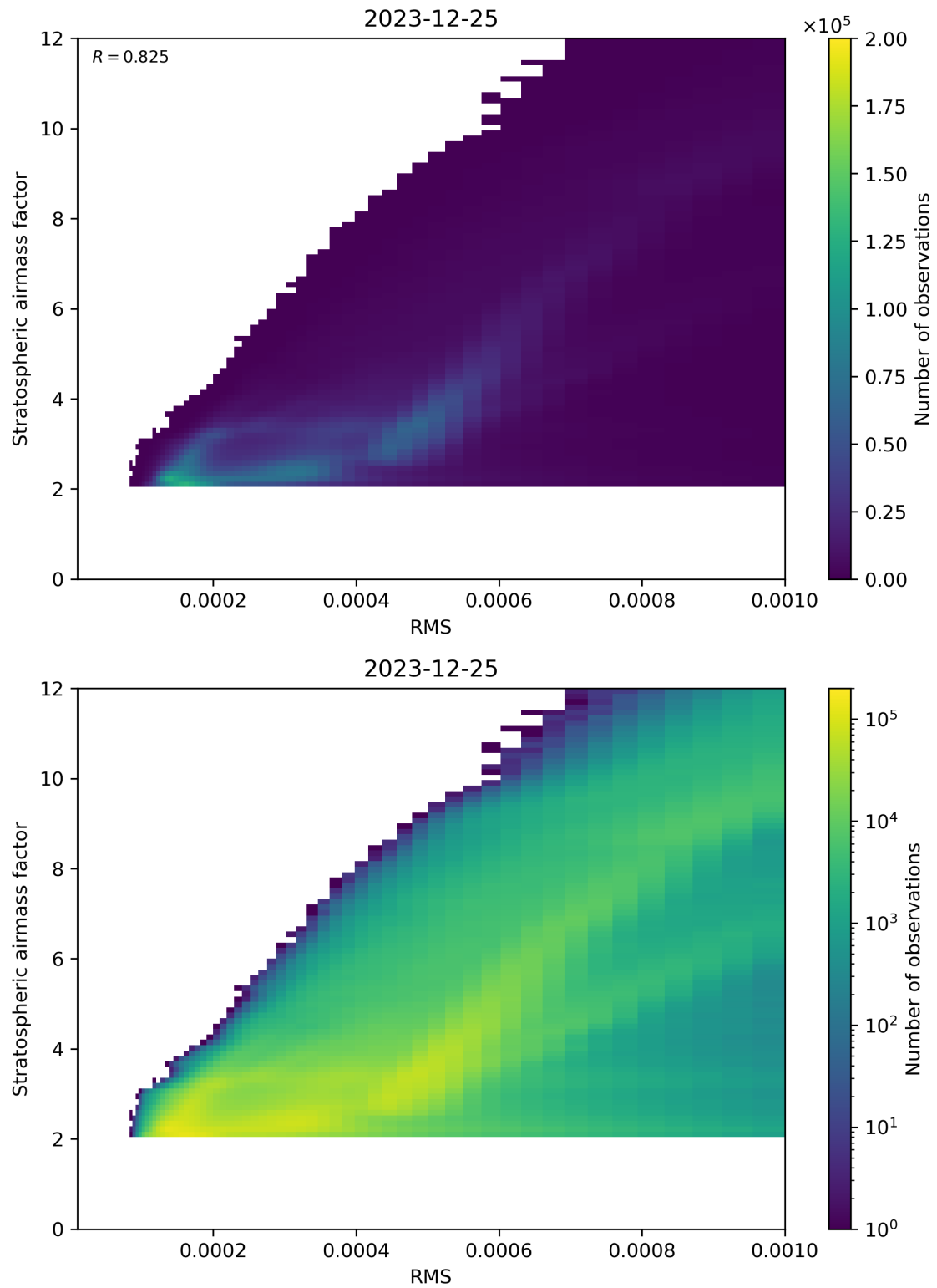
Figure 144: Scatter density plot of “RMS” against “Stratospheric airmass factor” for 2023-12-25 to 2023-12-26.
