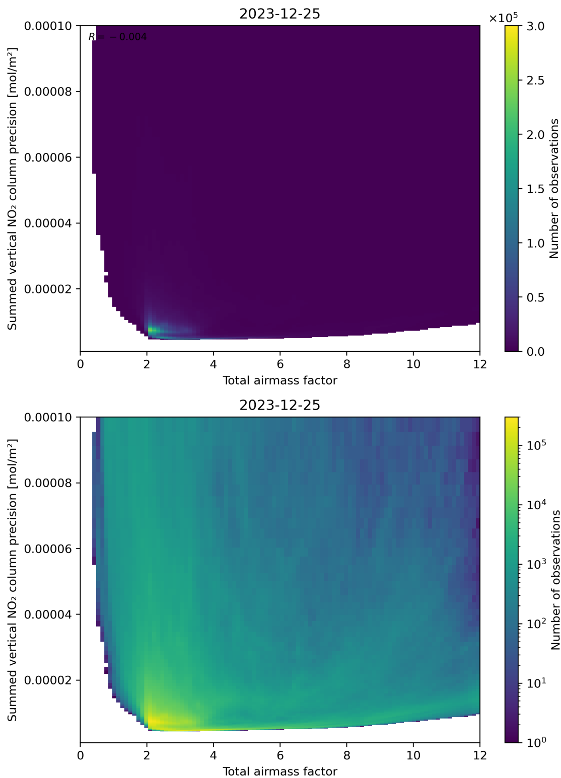
Figure 66: Scatter density plot of “Total airmass factor” against “Summed vertical NO 2 column precision” for 2023-12-25 to 2023-12-26.
