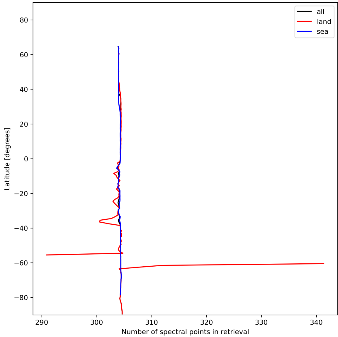
Figure 16: Zonal average of “Number of spectral points in retrieval” for 2023-12-25 to 2023-12-26.
