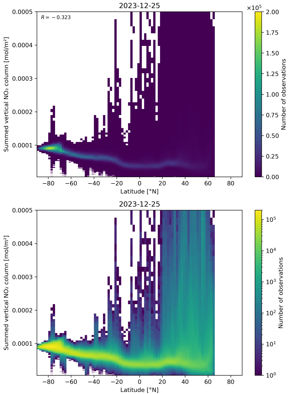
Figure 88: Scatter density plot of “Latitude” against “Summed vertical NO 2 column” for 2023-12-25 to 2023-12-26.
