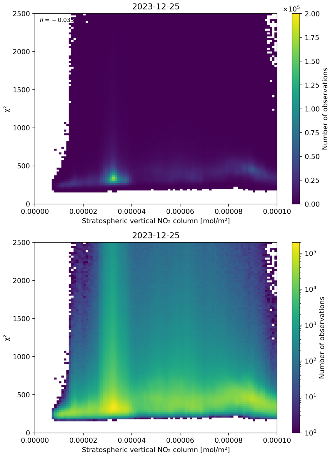
Figure 97: Scatter density plot of “Stratospheric vertical NO 2 column” against “ \chi^2 ” for 2023-12-25 to 2023-12-26.
