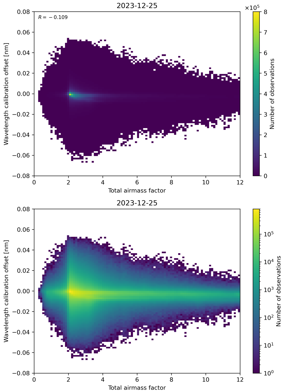
Figure 70: Scatter density plot of “Total airmass factor” against “Wavelength calibration offset” for 2023-12-25 to 2023-12-26.
