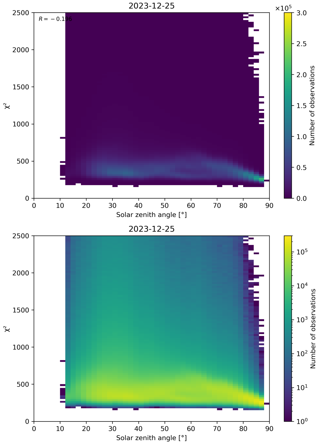
Figure 148: Scatter density plot of “Solar zenith angle” against “ \chi^2 ” for 2023-12-25 to 2023-12-26.
