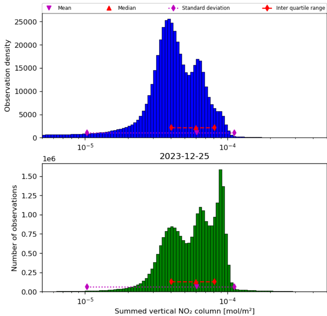
Figure 40: Histogram of “Summed vertical NO 2 column” for 2023-12-25 to 2023-12-26
