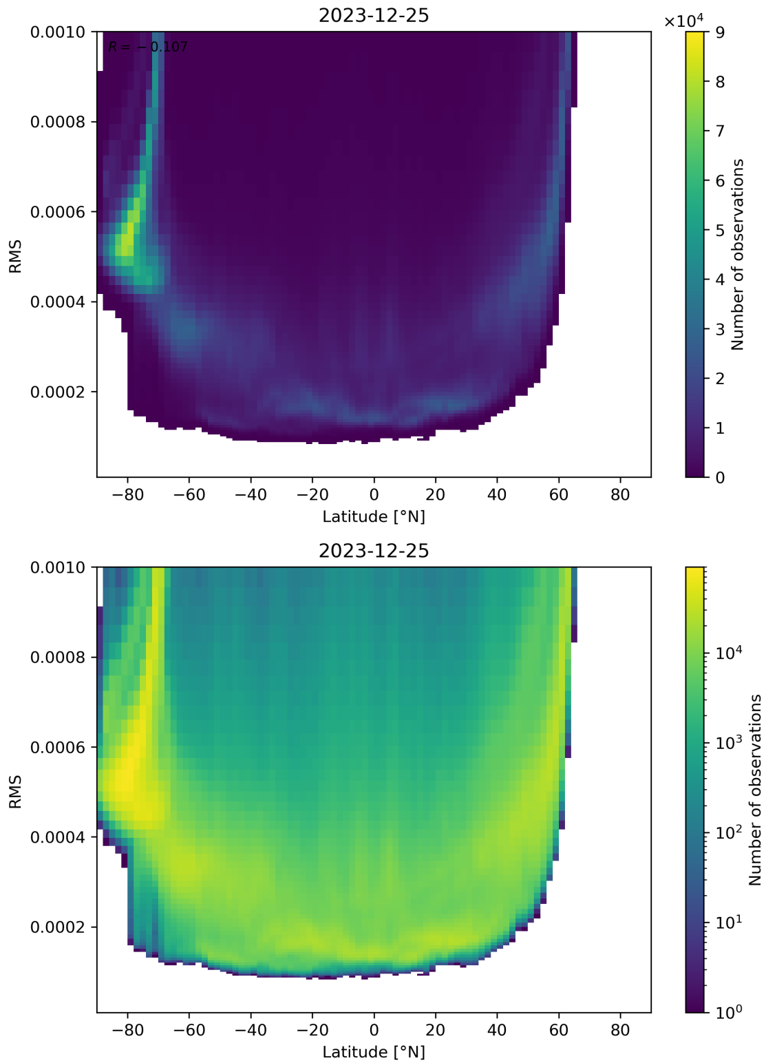
Figure 94: Scatter density plot of “Latitude” against “RMS” for 2023-12-25 to 2023-12-26.
