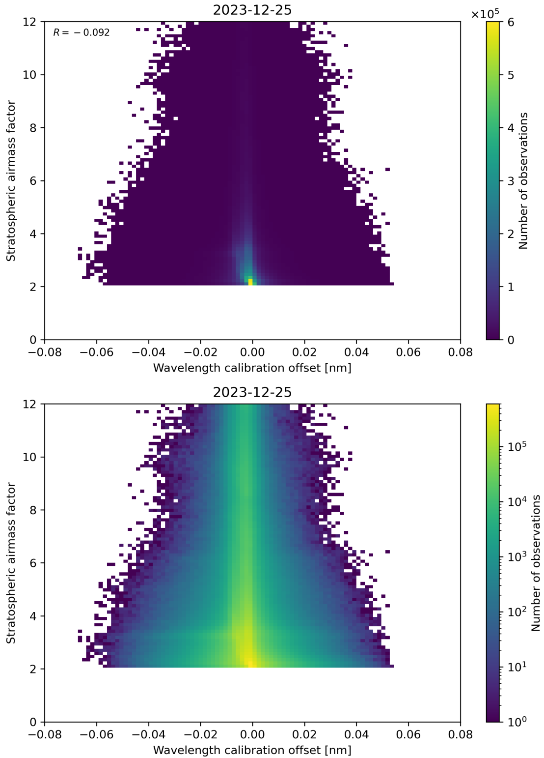
Figure 174: Scatter density plot of “Wavelength calibration offset” against “Stratospheric airmass factor” for 2023-12-25 to 2023-12-26.
