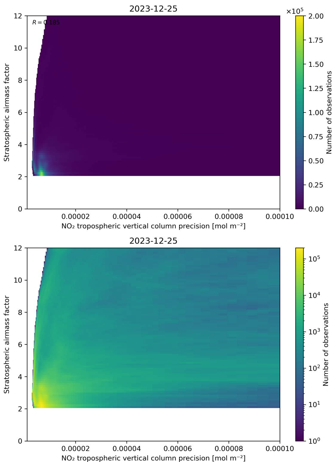
Figure 131: Scatter density plot of “NO 2 tropospheric vertical column precision” against “Stratospheric airmass factor” for 2023-12-25 to 2023-12-26.
