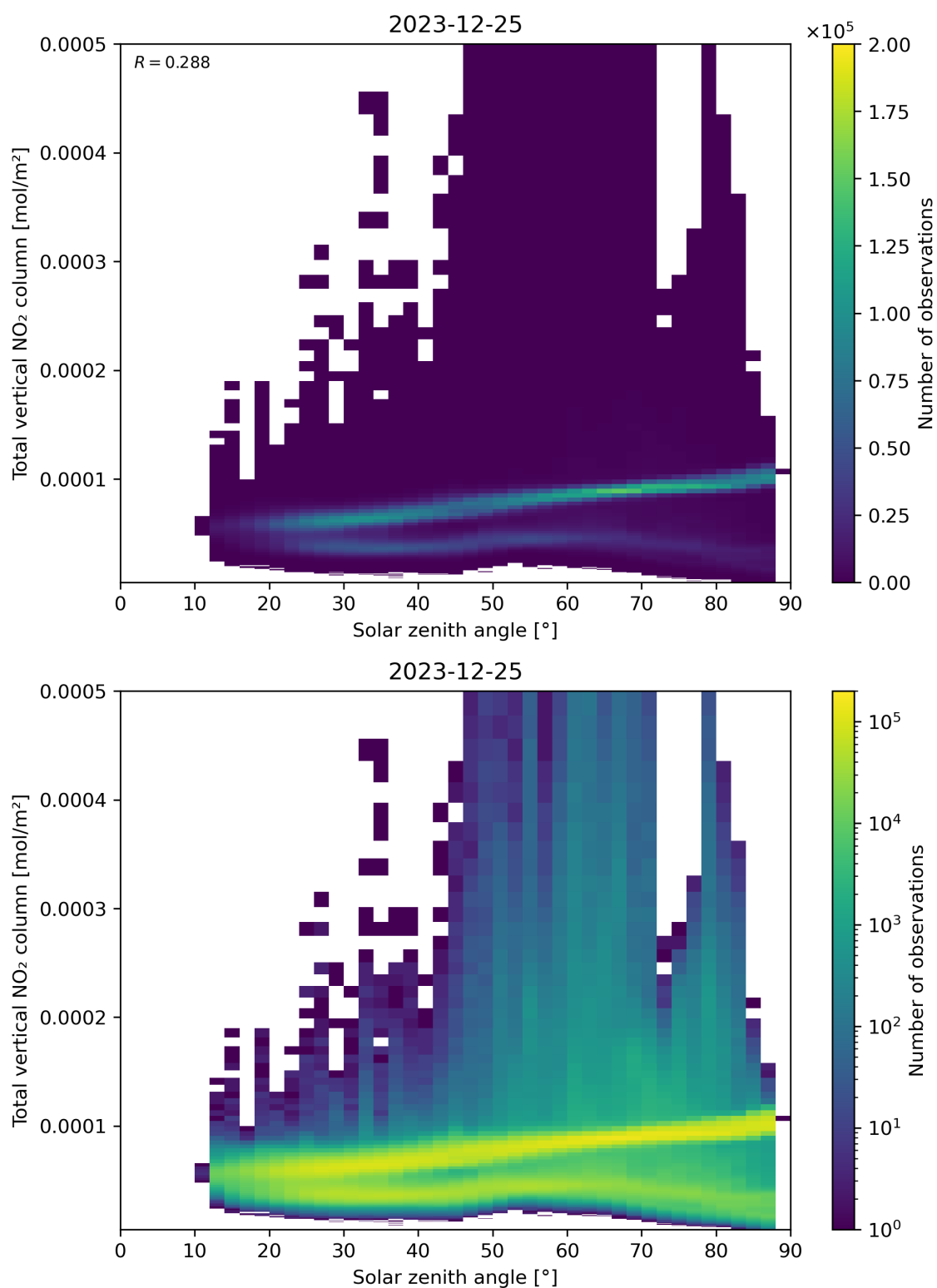
Figure 153: Scatter density plot of “Solar zenith angle” against “Total vertical NO 2 column” for 2023-12-25 to 2023-12-26.
