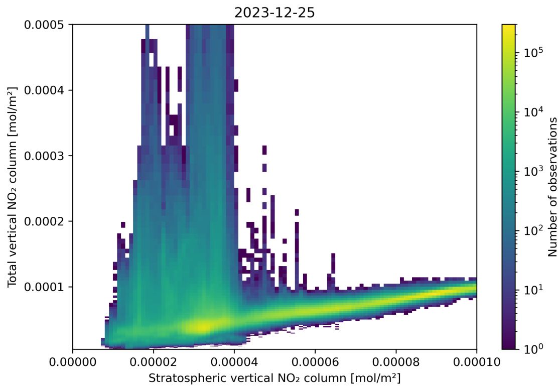
Figure 100: Scatter density plot of “Stratospheric vertical NO 2 column” against “Total vertical NO 2 column” for 2023-12-25 to 2023-12-26.
