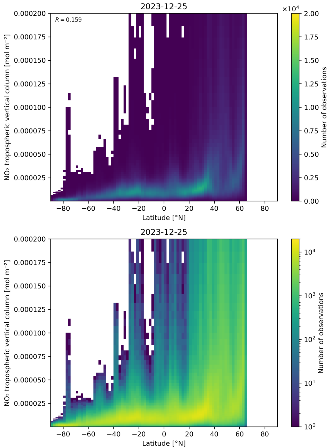
Figure 92: Scatter density plot of “Latitude” against “NO 2 tropospheric vertical column” for 2023-12-25 to 2023-12-26.
