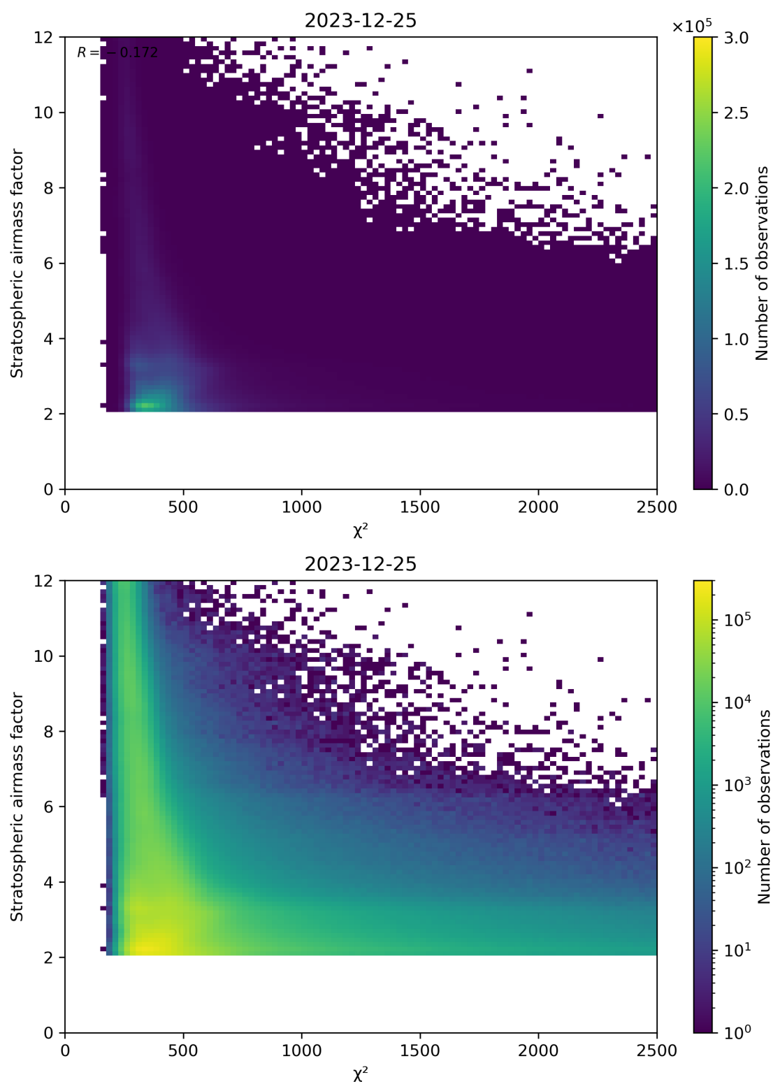
Figure 81: Scatter density plot of “ \chi^2 ” against “Stratospheric airmass factor” for 2023-12-25 to 2023-12-26.
