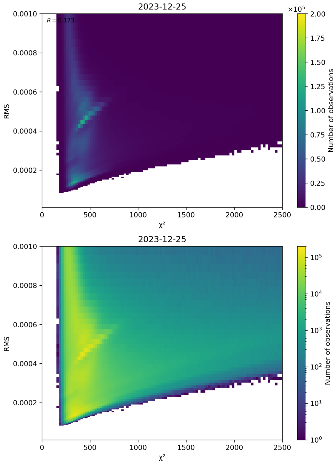
Figure 82: Scatter density plot of “ \chi^2 ” against “RMS” for 2023-12-25 to 2023-12-26.
