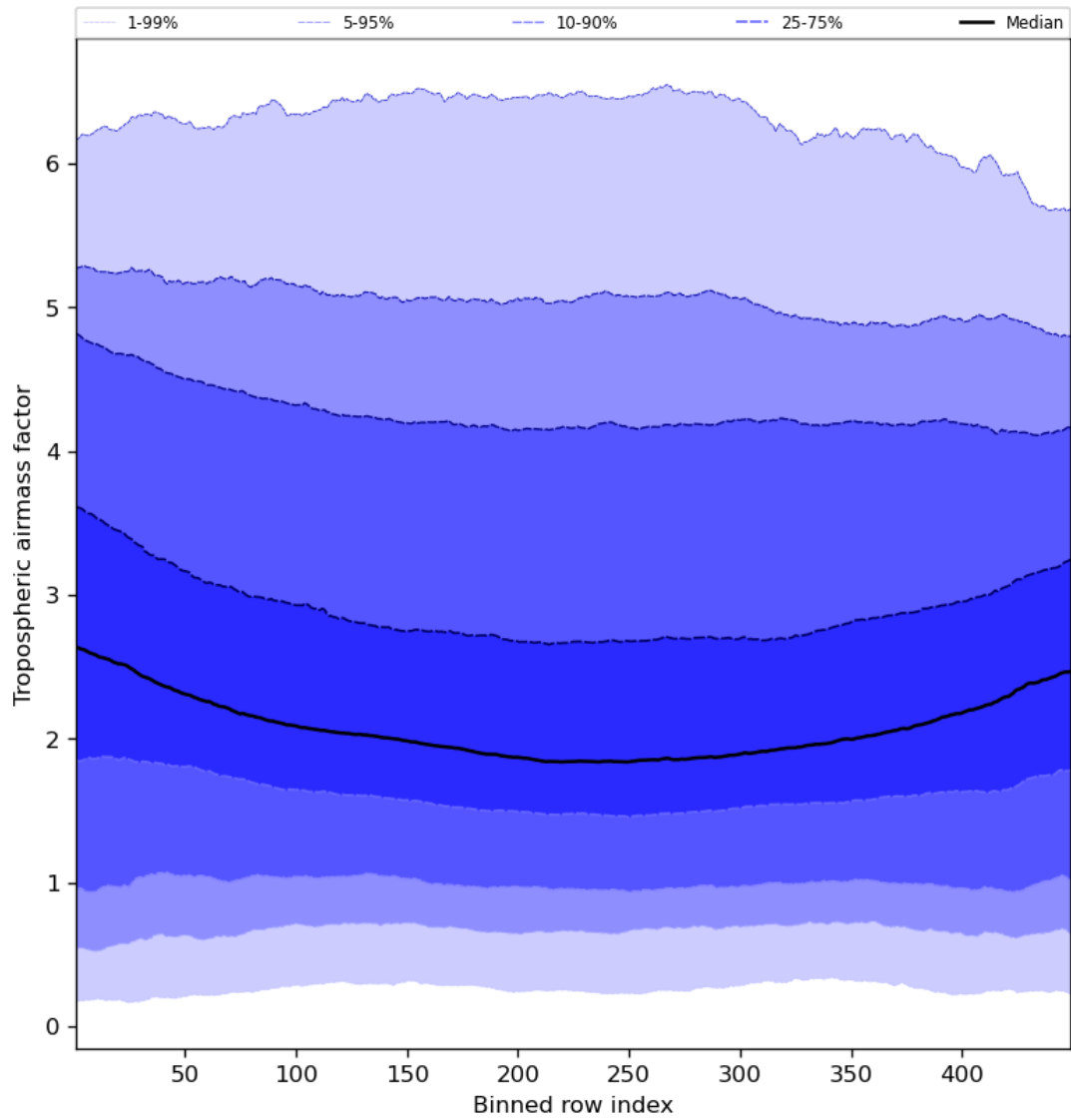
Figure 48: Along track statistics of “Tropospheric airmass factor” for 2023-12-25 to 2023-12-26
