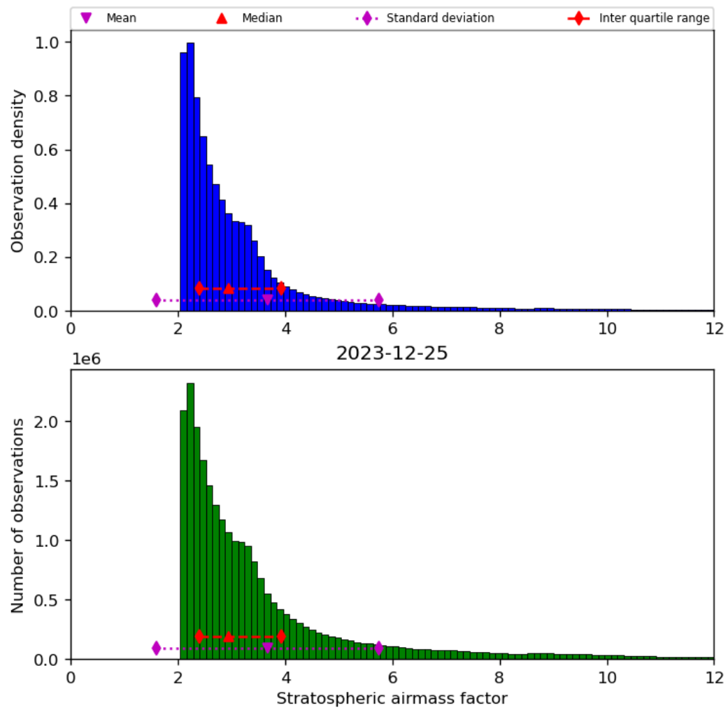
Figure 44: Histogram of “Stratospheric airmass factor” for 2023-12-25 to 2023-12-26
