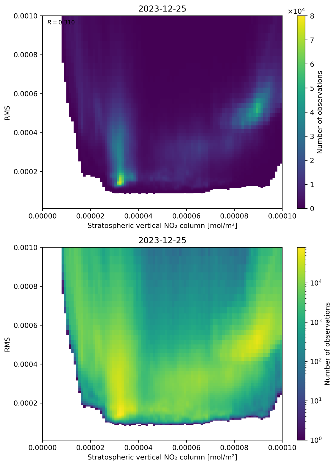
Figure 102: Scatter density plot of “Stratospheric vertical NO 2 column” against “RMS” for 2023-12-25 to 2023-12-26.
