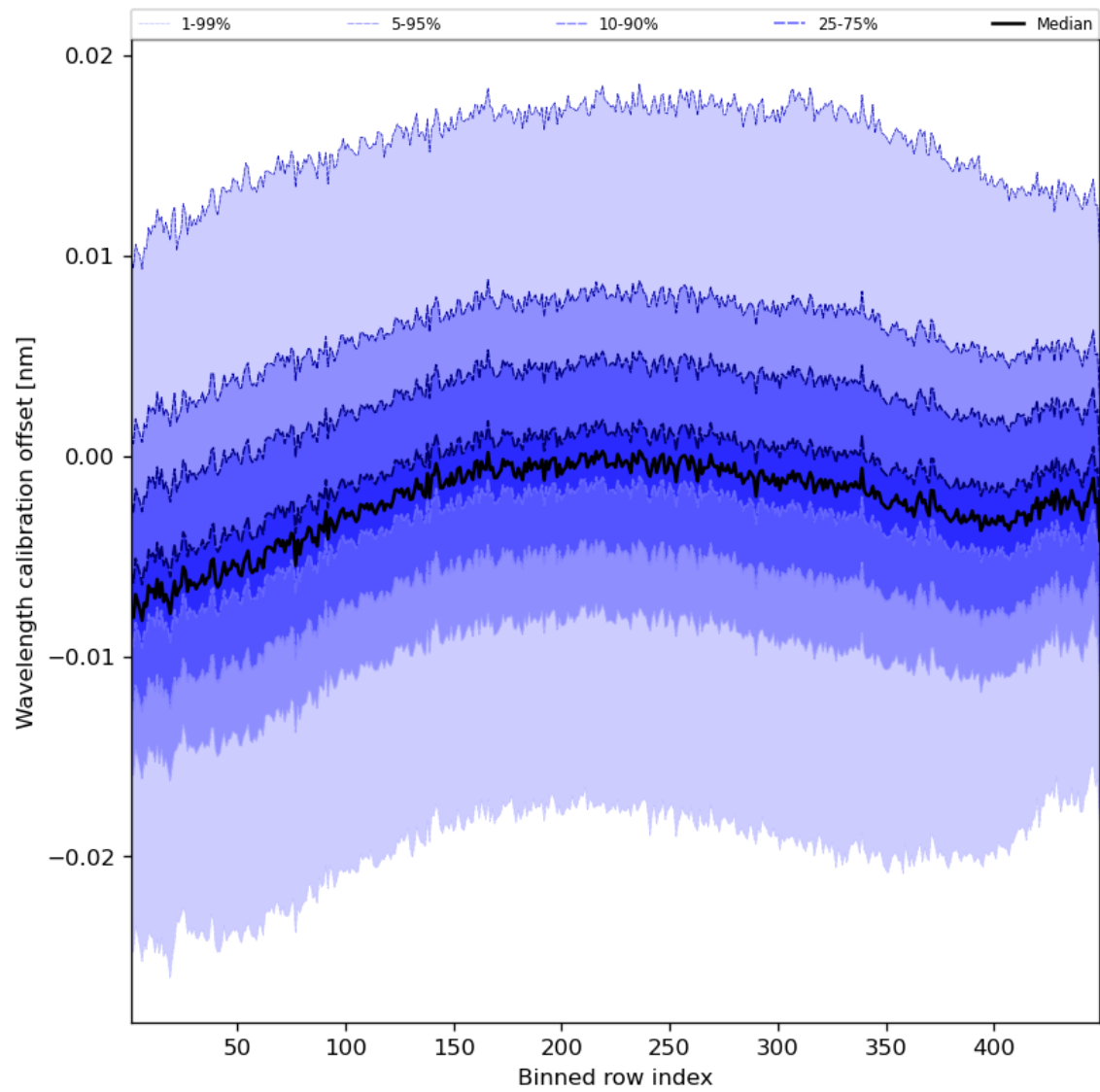
Figure 52: Along track statistics of “Wavelength calibration offset” for 2023-12-25 to 2023-12-26
