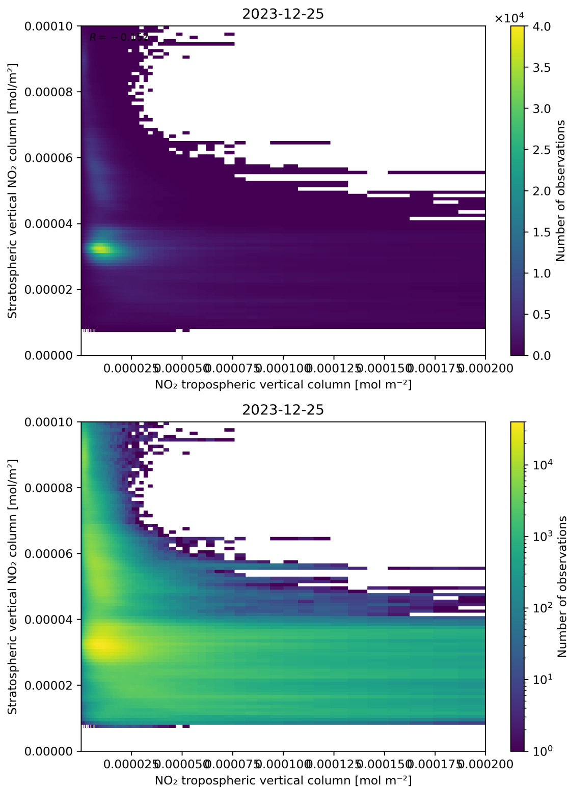
Figure 125: Scatter density plot of “NO 2 tropospheric vertical column” against “Stratospheric vertical NO 2 column” for 2023-12-25 to 2023-12-26.
