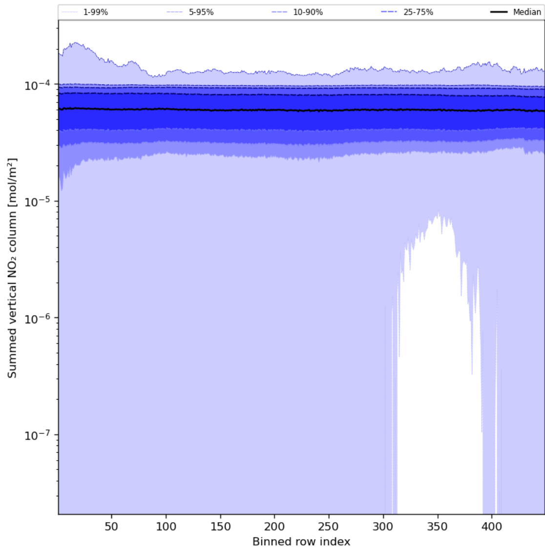
Figure 57: Along track statistics of “Summed vertical NO 2 column” for 2023-12-25 to 2023-12-26
