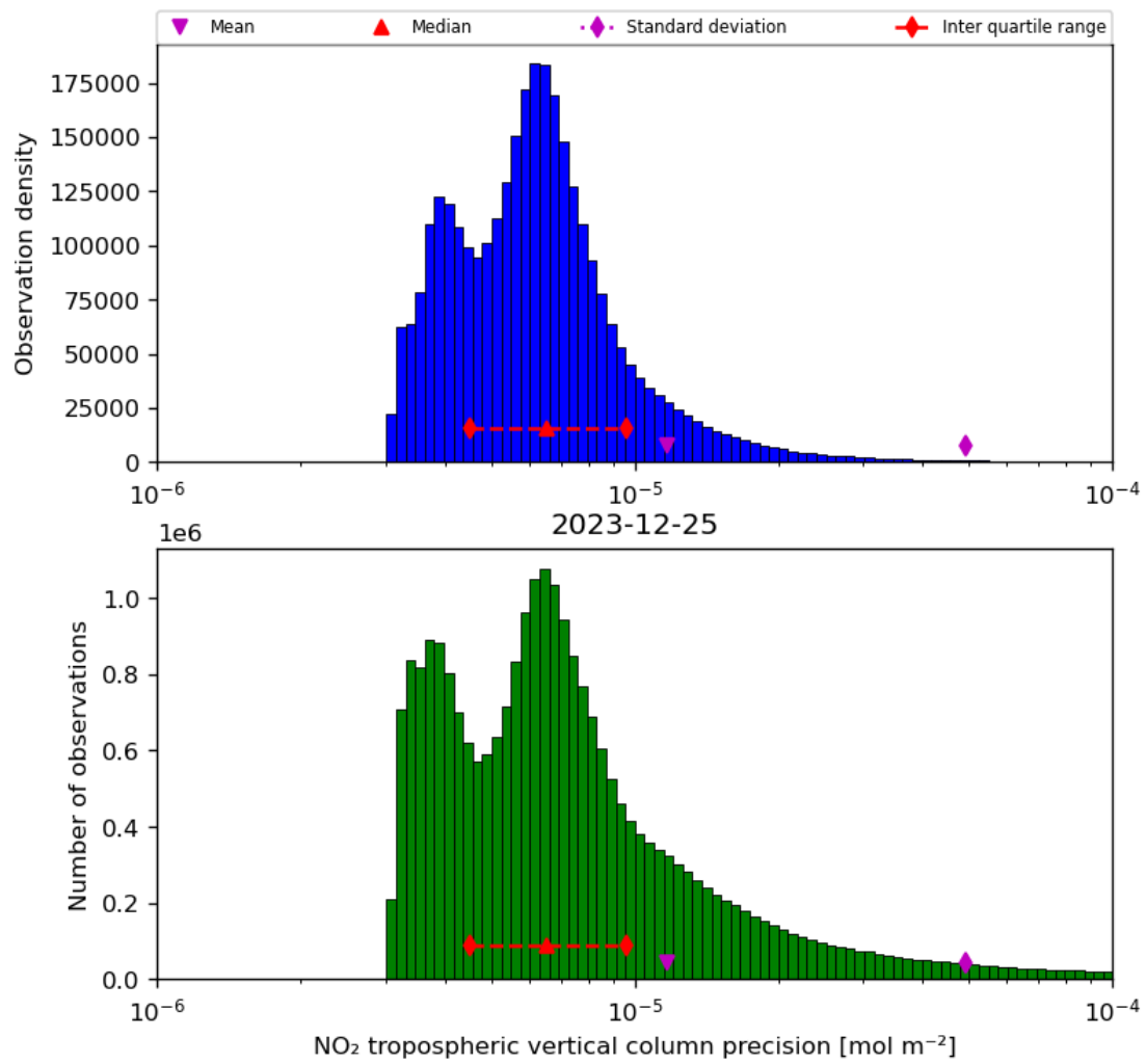
Figure 30: Histogram of "NO 2 tropospheric vertical column precision" for 2023-12-25 to 2023-12-26
