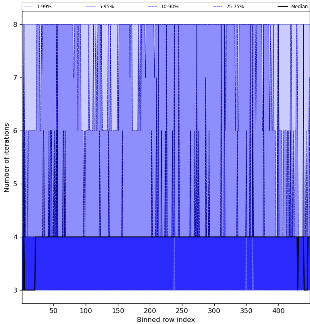
Figure 51: Along track statistics of “Number of iterations” for 2023-12-25 to 2023-12-26
