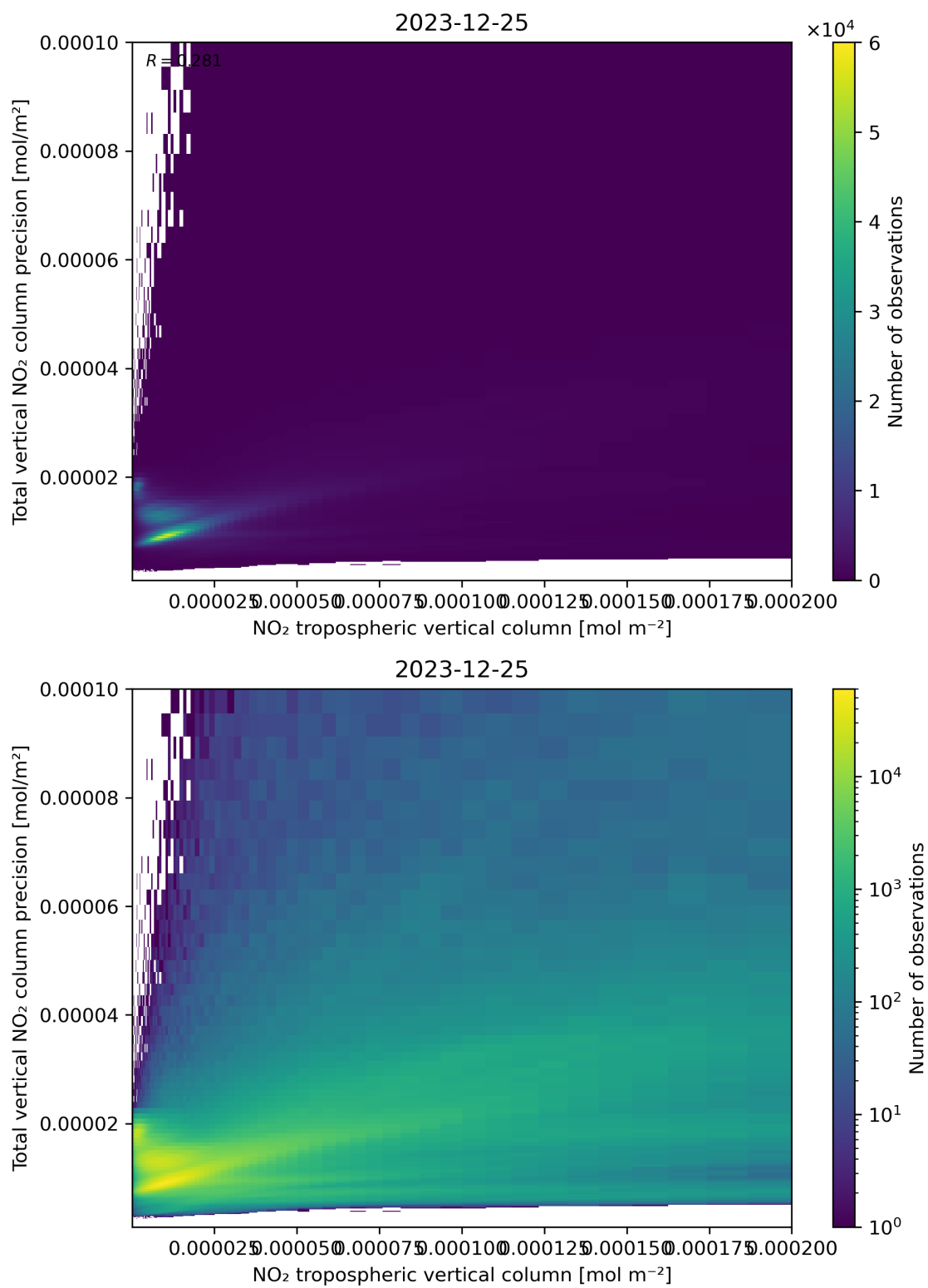
Figure 129: Scatter density plot of “NO 2 tropospheric vertical column” against “Total vertical NO 2 column precision” for 2023-12-25 to 2023-12-26.
