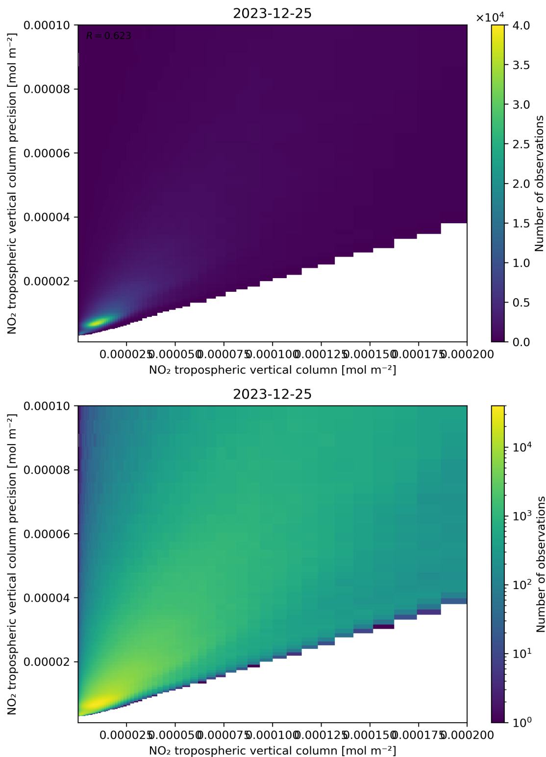
Figure 130: Scatter density plot of “NO 2 tropospheric vertical column” against “NO 2 tropospheric vertical column precision” for 2023-12-25 to 2023-12-26.
