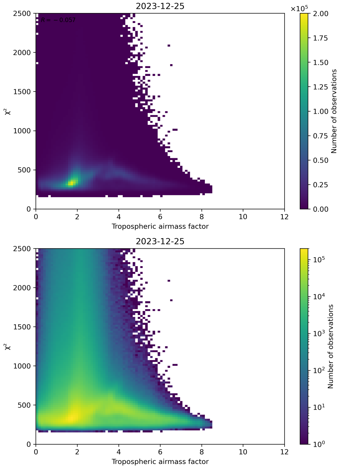
Figure 73: Scatter density plot of “Tropospheric airmass factor” against “ \chi^2 ” for 2023-12-25 to 2023-12-26.
