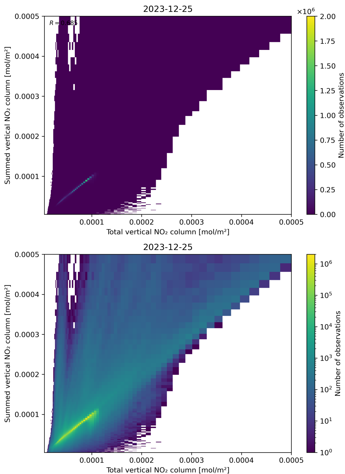
Figure 112: Scatter density plot of “Total vertical NO 2 column” against “Summed vertical NO 2 column” for 2023-12-25 to 2023-12-26.
