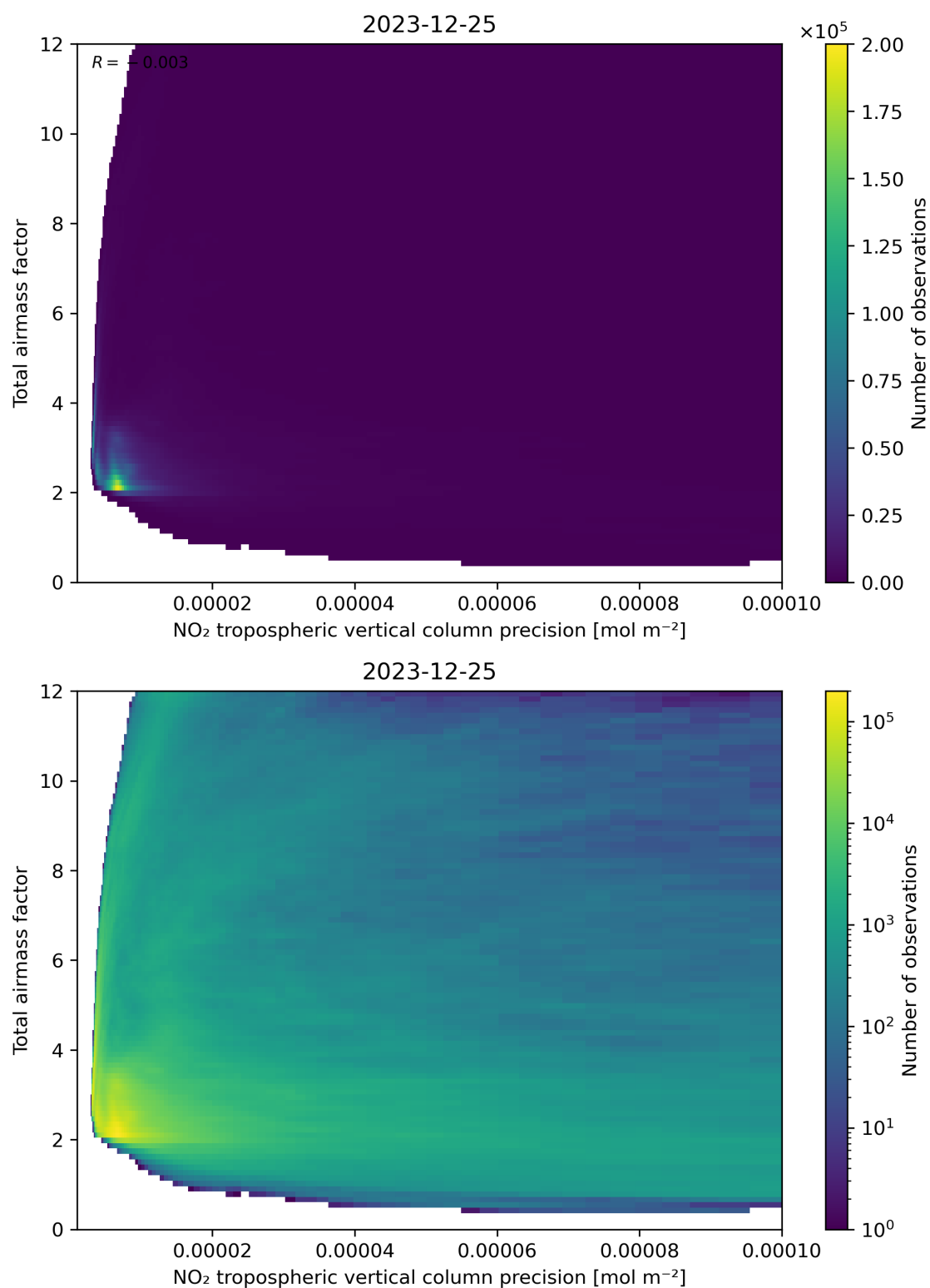
Figure 132: Scatter density plot of “NO 2 tropospheric vertical column precision” against “Total airmass factor” for 2023-12-25 to 2023-12-26.
