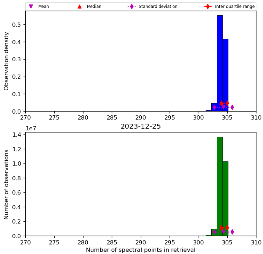
Figure 33: Histogram of “Number of spectral points in retrieval” for 2023-12-25 to 2023-12-26
