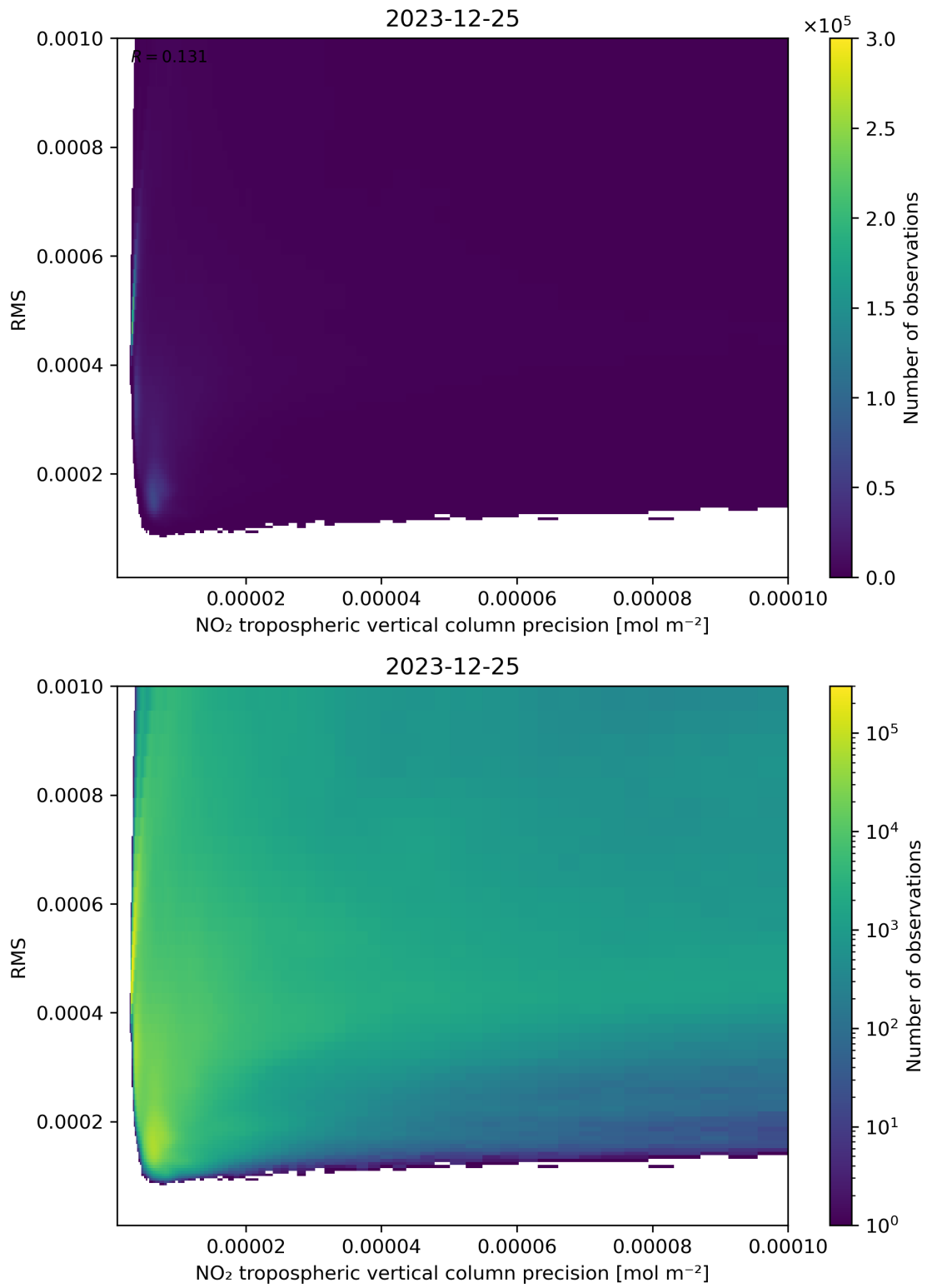
Figure 140: Scatter density plot of “NO 2 tropospheric vertical column precision” against “RMS” for 2023-12-25 to 2023-12-26.
