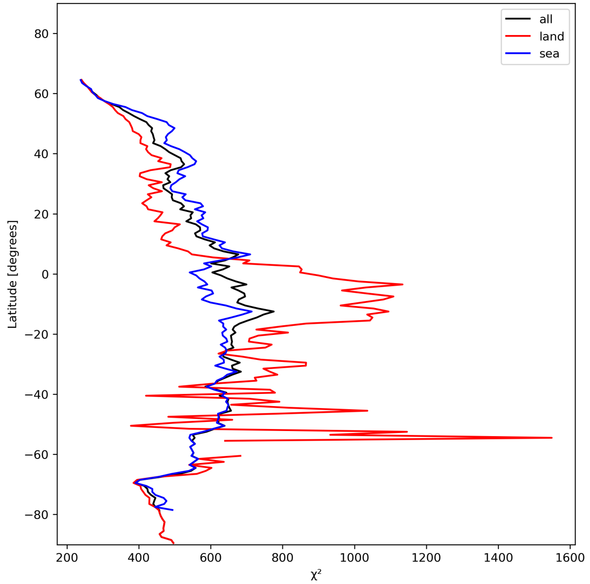
Figure 25: Zonal average of “ \chi^2 ” for 2023-12-25 to 2023-12-26.
