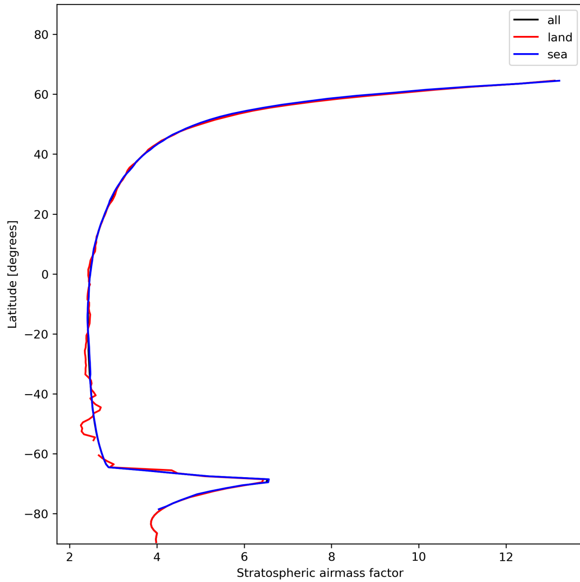
Figure 27: Zonal average of “Stratospheric air mass factor” for 2023-12-25 to 2023-12-26.
