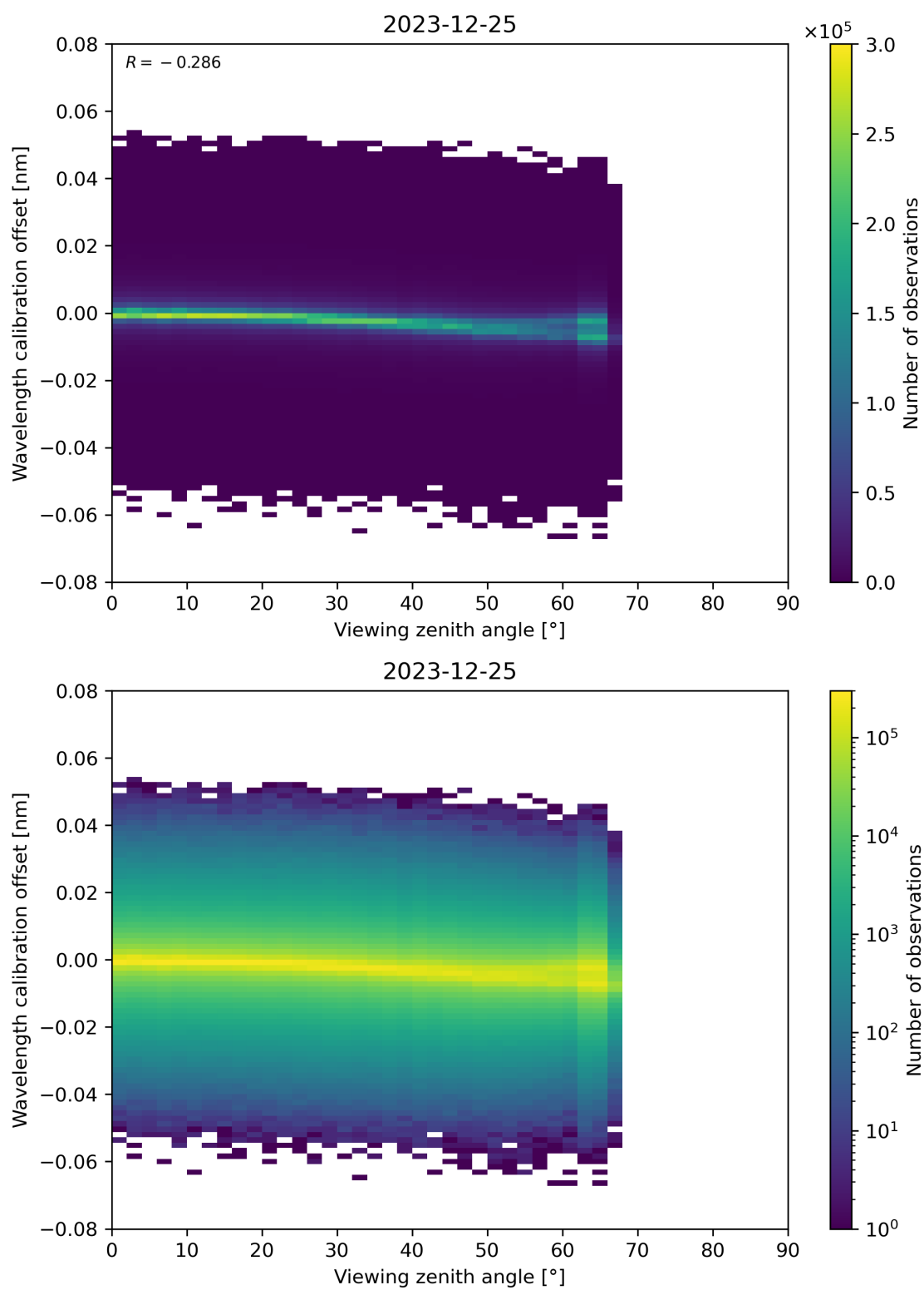
Figure 173: Scatter density plot of “Viewing zenith angle” against “Wavelength calibration offset” for 2023-12-25 to 2023-12-26.
