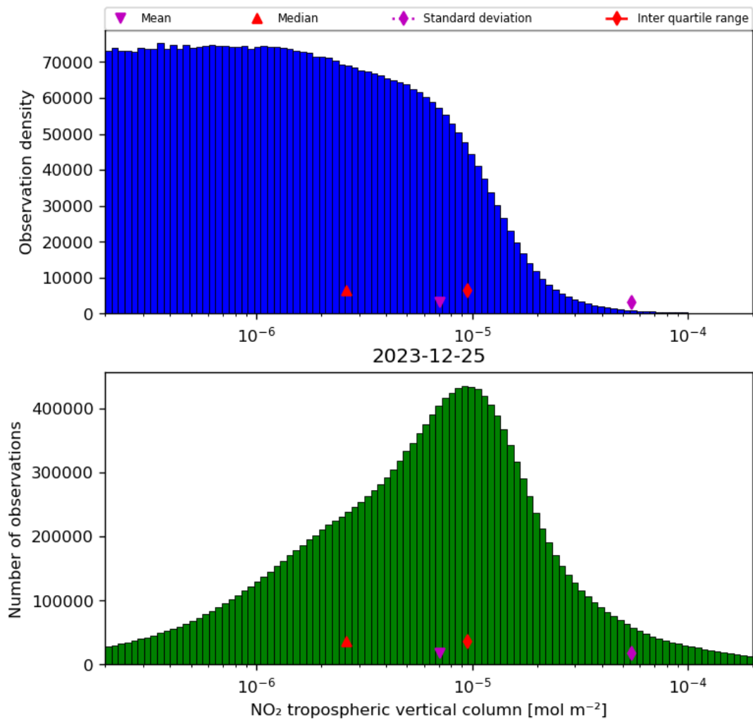
Figure 29: Histogram of “NO 2 tropospheric vertical column” for 2023-12-25 to 2023-12-26
