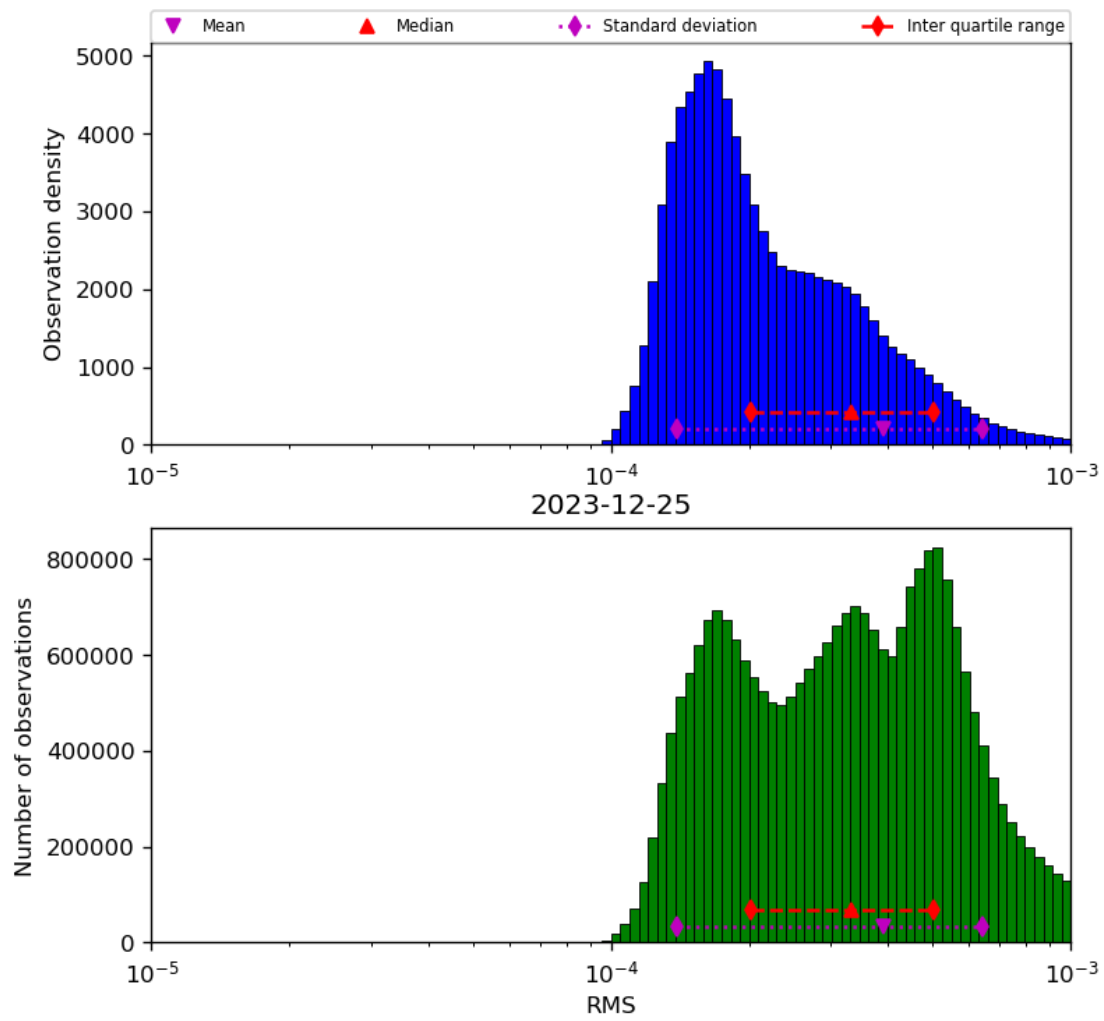
Figure 43: Histogram of “RMS” for 2023-12-25 to 2023-12-26
