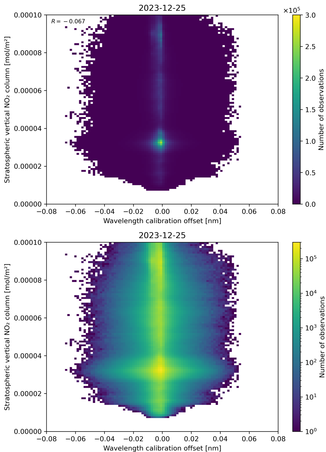
Figure 176: Scatter density plot of “Wavelength calibration offset” against “Stratospheric vertical NO 2 column” for 2023-12-25 to 2023-12-26.
