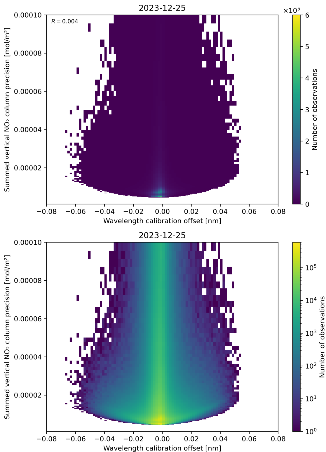
Figure 178: Scatter density plot of “Wavelength calibration offset” against “Summed vertical NO 2 column precision” for 2023-12-25 to 2023-12-26.
