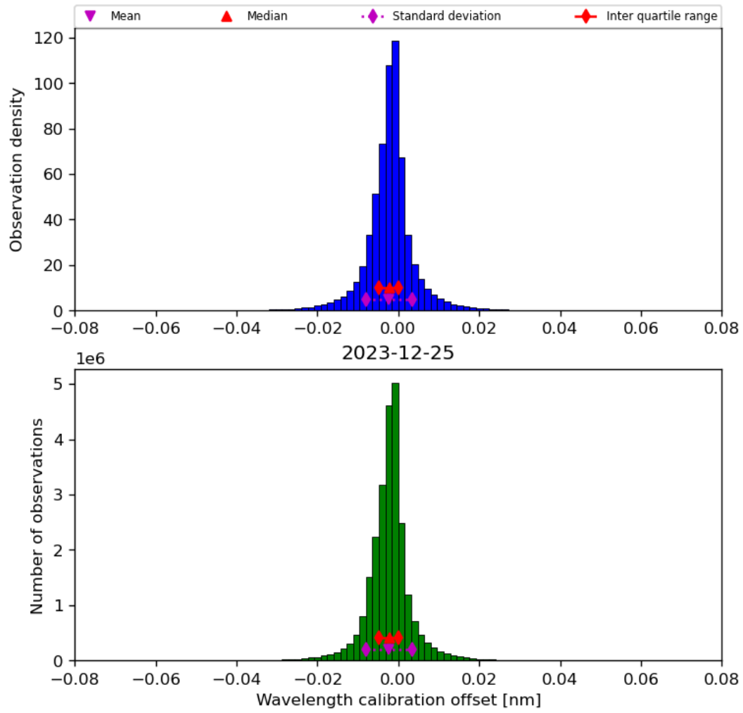
Figure 35: Histogram of “Wavelength calibration offset” for 2023-12-25 to 2023-12-26
