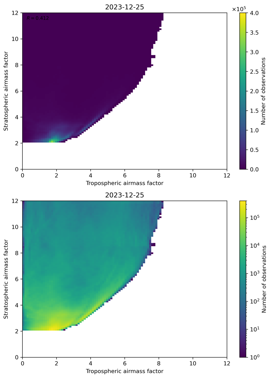
Figure 71: Scatter density plot of “Tropospheric airmass factor” against “Stratospheric airmass factor” for 2023-12-25 to 2023-12-26.
