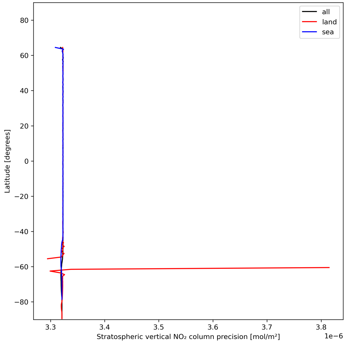
Figure 20: Zonal average of “Stratospheric vertical NO 2 column precision” for 2023-12-25 to 2023-12-26.
