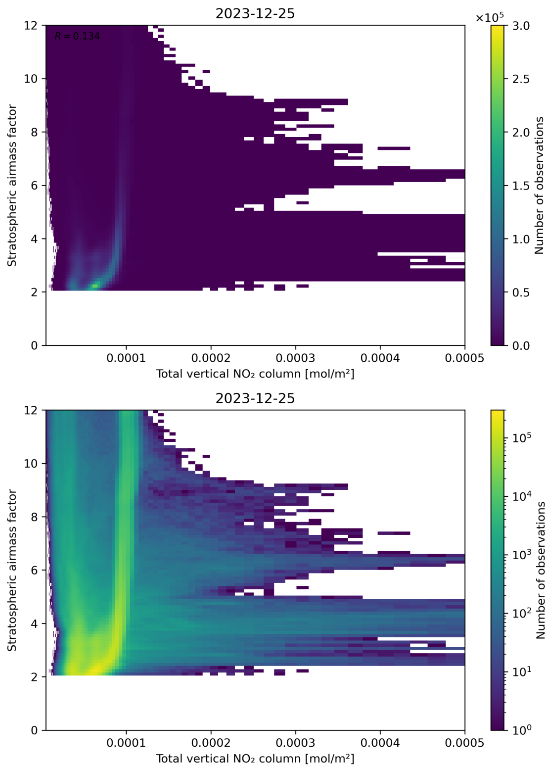
Figure 110: Scatter density plot of “Total vertical NO 2 column” against “Stratospheric airmass factor” for 2023-12-25 to 2023-12-26.
