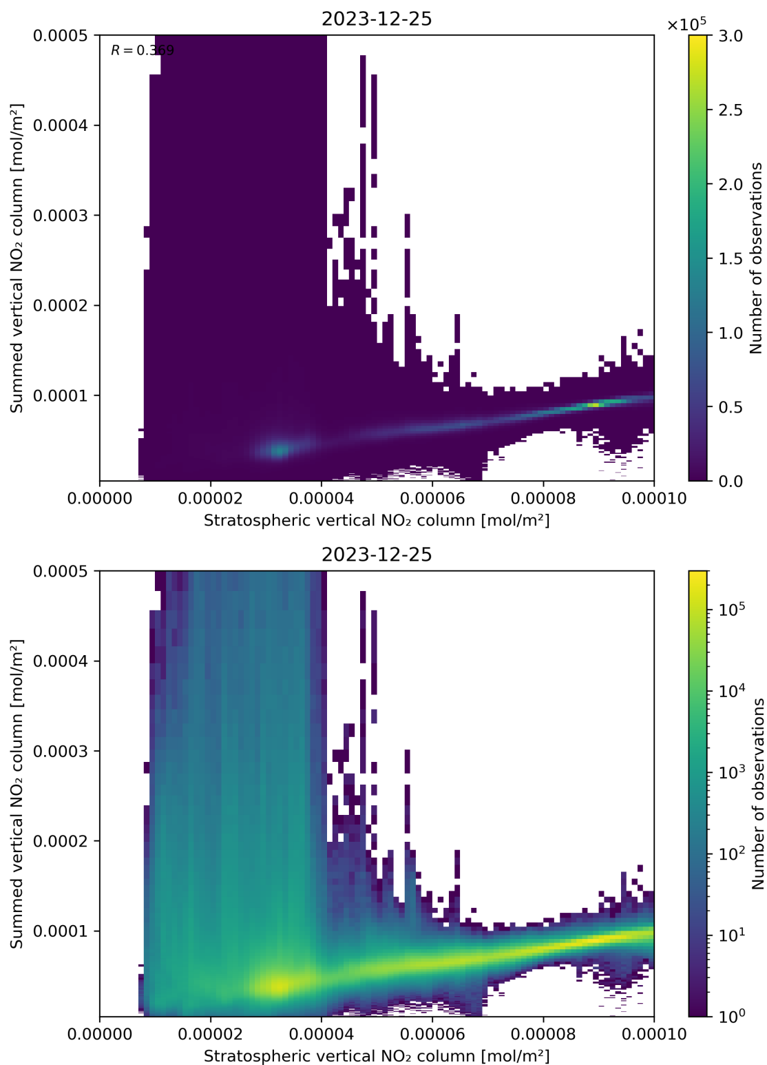
Figure 98: Scatter density plot of “Stratospheric vertical NO 2 column” against “Summed vertical NO 2 column” for 2023-12-25 to 2023-12-26.
