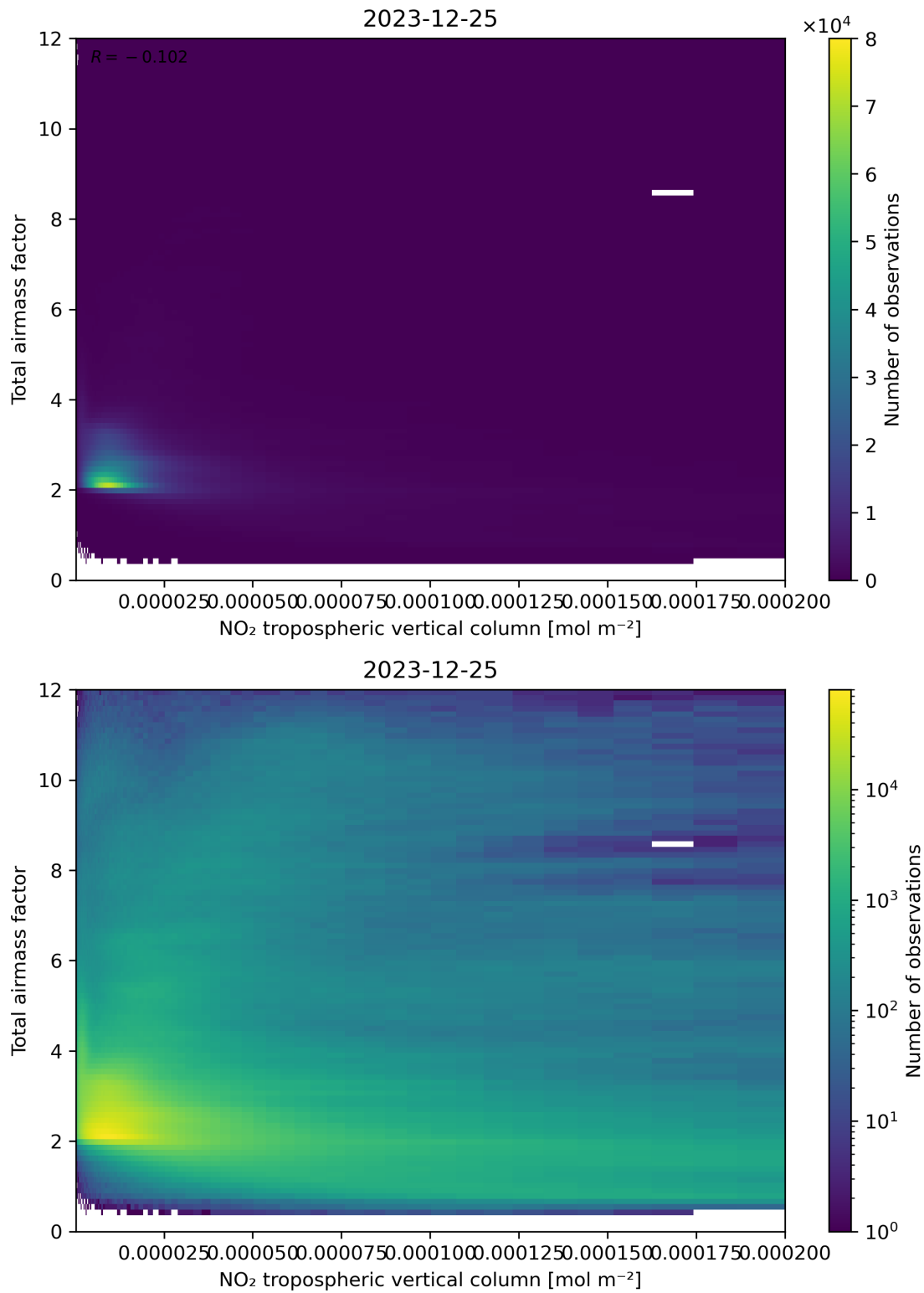
Figure 122: Scatter density plot of “NO 2 tropospheric vertical column” against “Total air mass factor” for 2023-12-25 to 2023-12-26.
