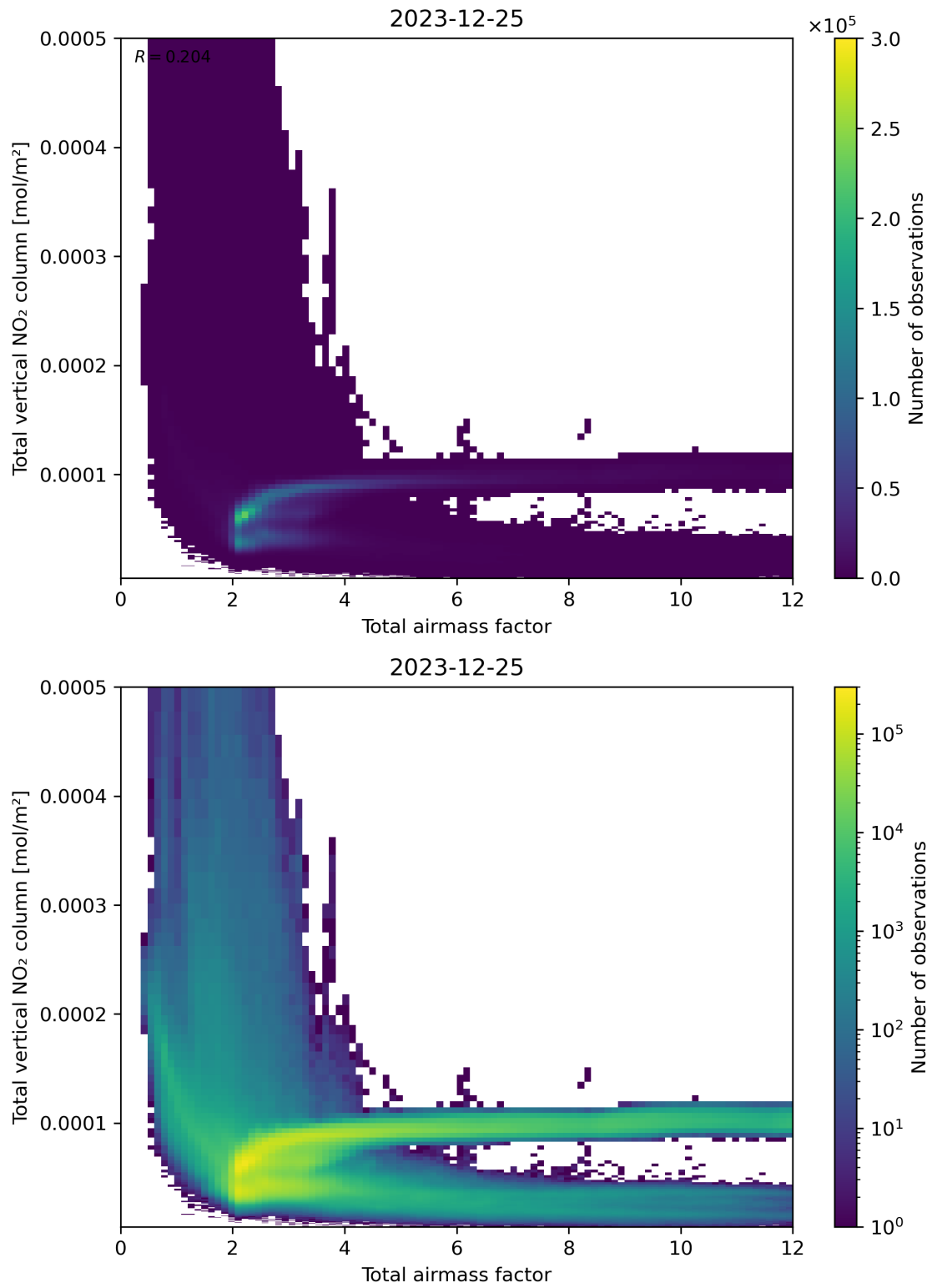
Figure 67: Scatter density plot of “Total airmass factor” against “Total vertical NO 2 column” for 2023-12-25 to 2023-12-26.
