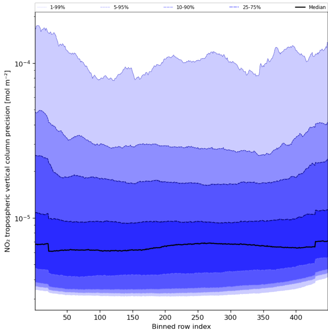
Figure 47: Along track statistics of “NO 2 tropospheric vertical column precision” for 2023-12-25 to 2023-12-26
