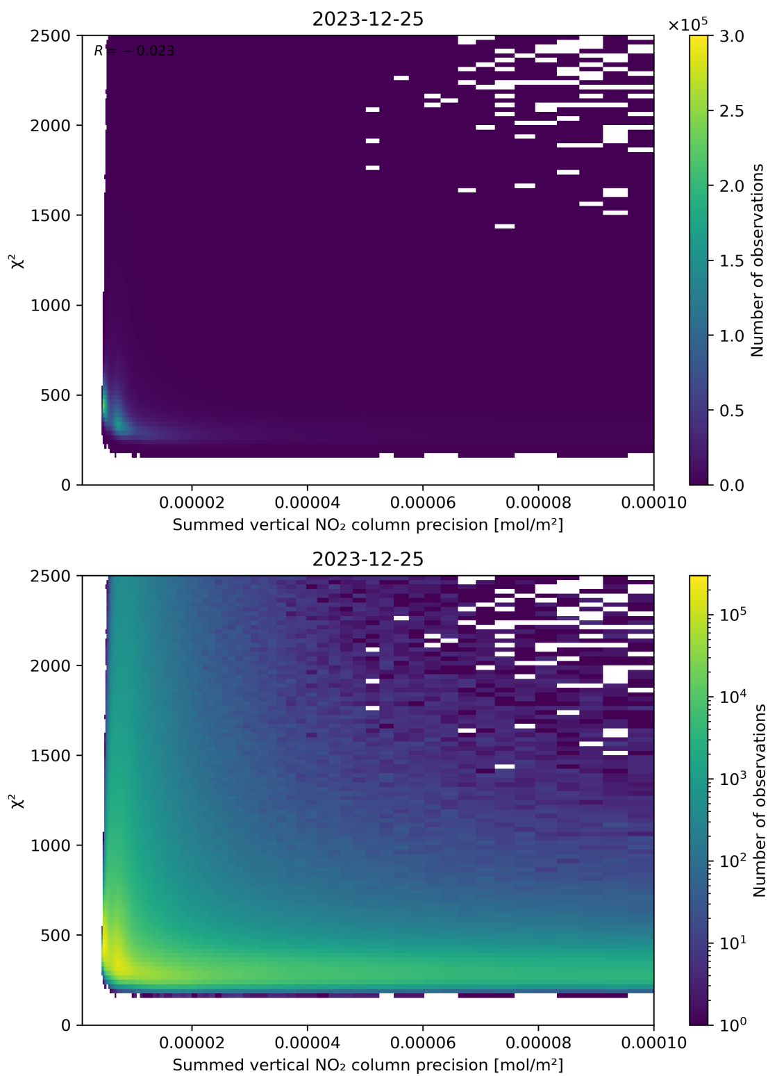
Figure 107: Scatter density plot of “Summed vertical NO 2 column precision” against “ \chi^2 ” for 2023-12-25 to 2023-12-26.
