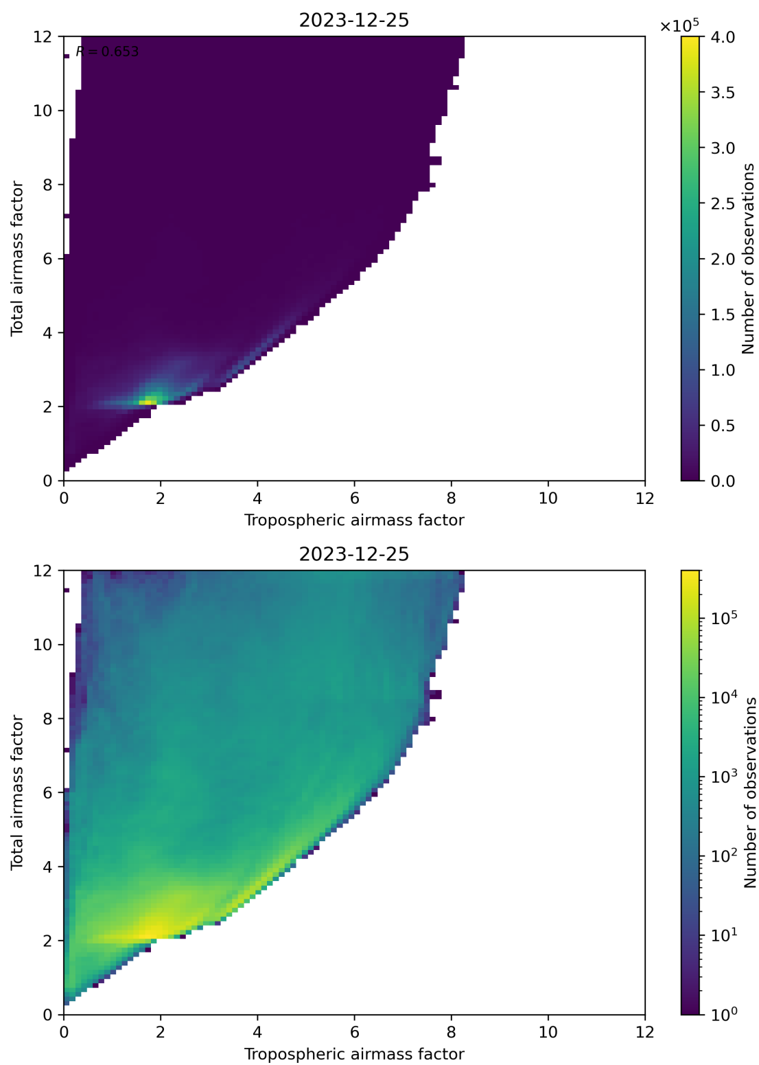
Figure 72: Scatter density plot of “Tropospheric airmass factor” against “Total airmass factor” for 2023-12-25 to 2023-12-26.
