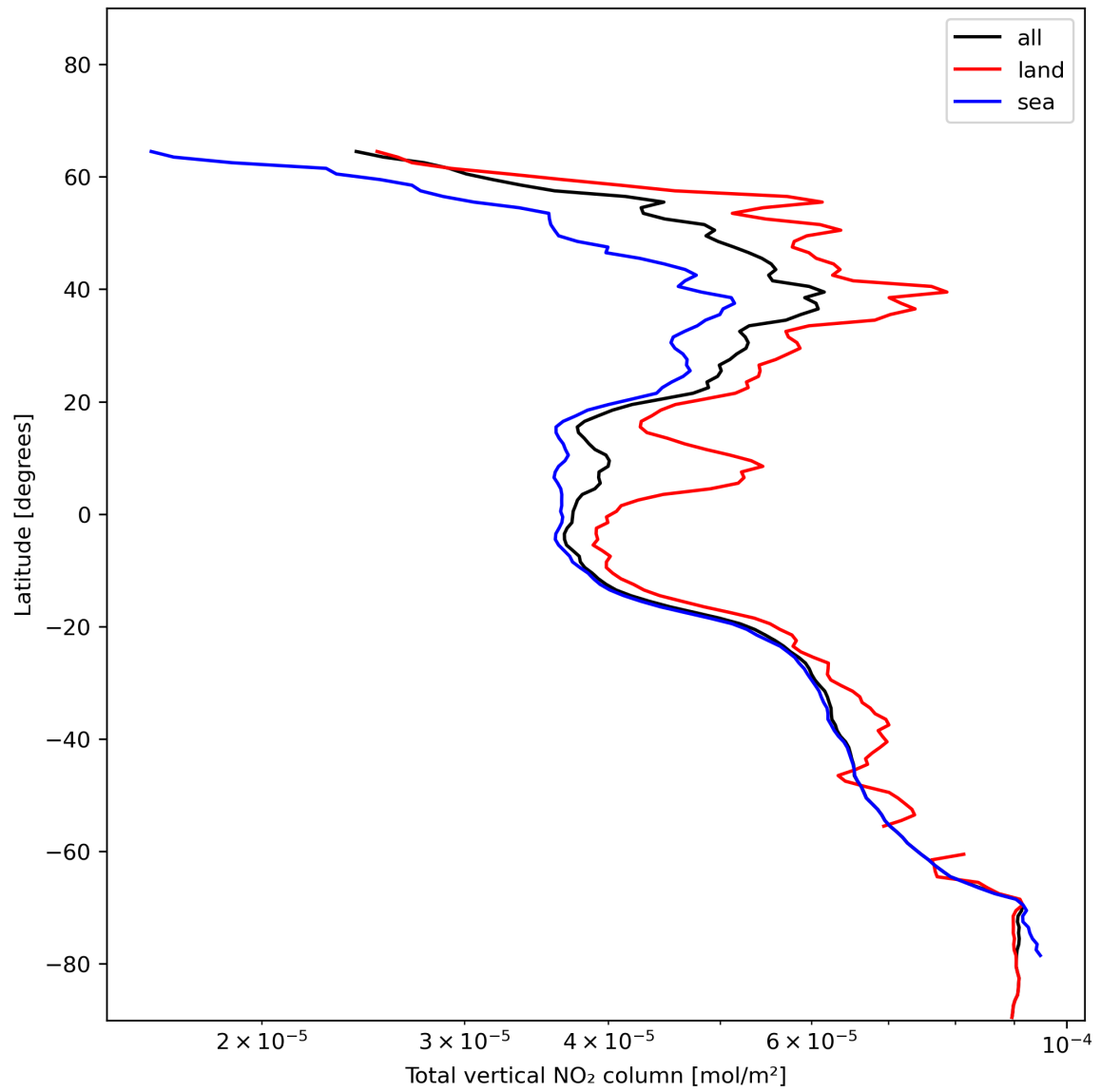
Figure 21: Zonal average of “Total vertical NO 2 column” for 2023-12-25 to 2023-12-26.
