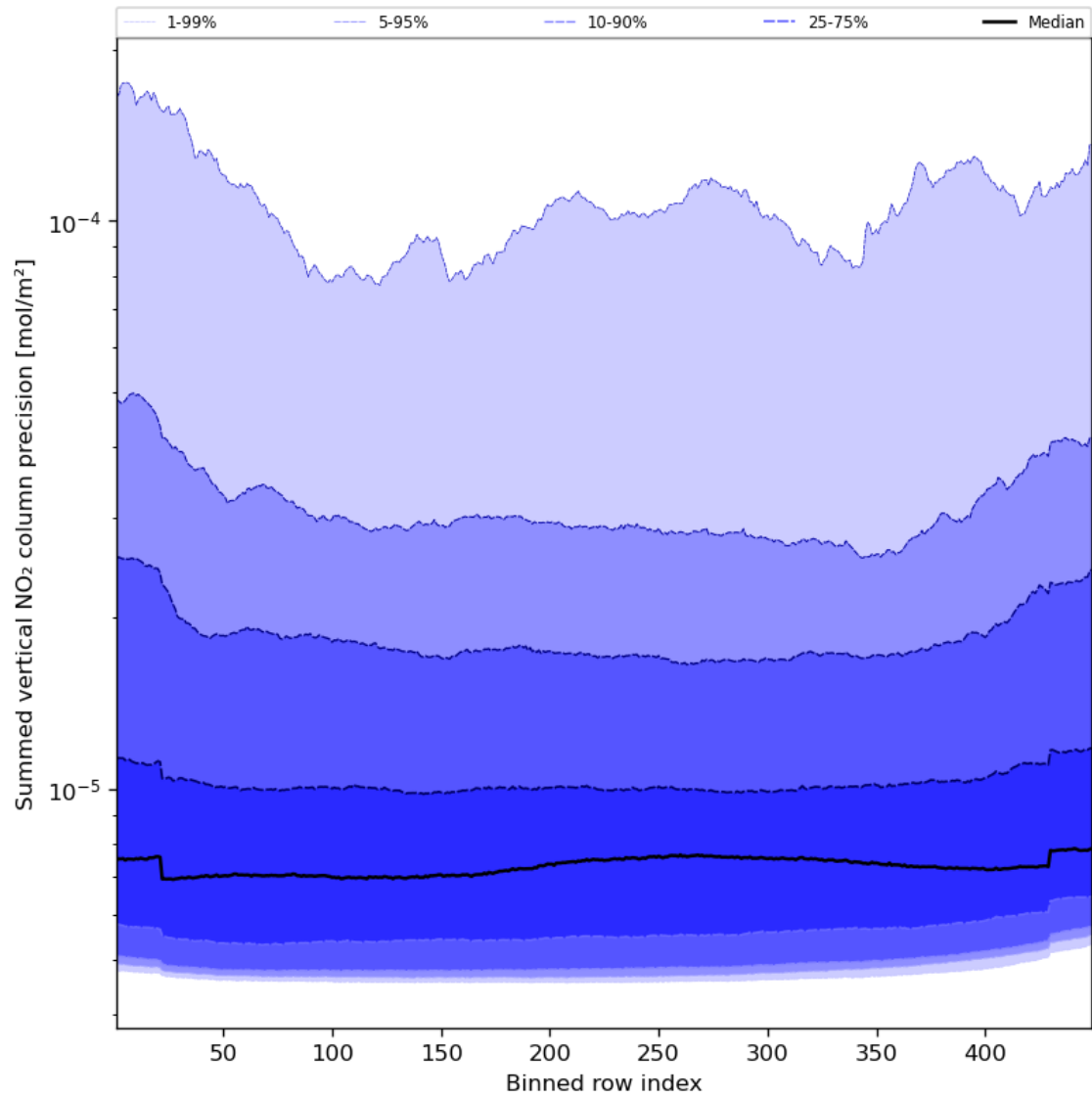
Figure 58: Along track statistics of “Summed vertical NO 2 column precision” for 2023-12-25 to 2023-12-26
