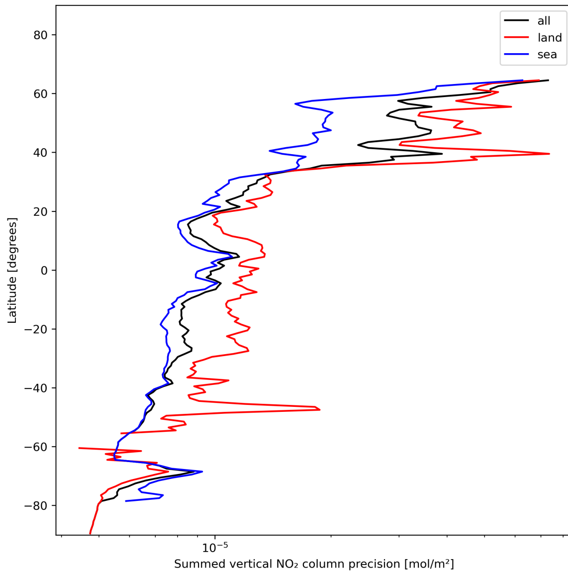
Figure 24: Zonal average of “Summed vertical NO 2 column precision” for 2023-12-25 to 2023-12-26.
