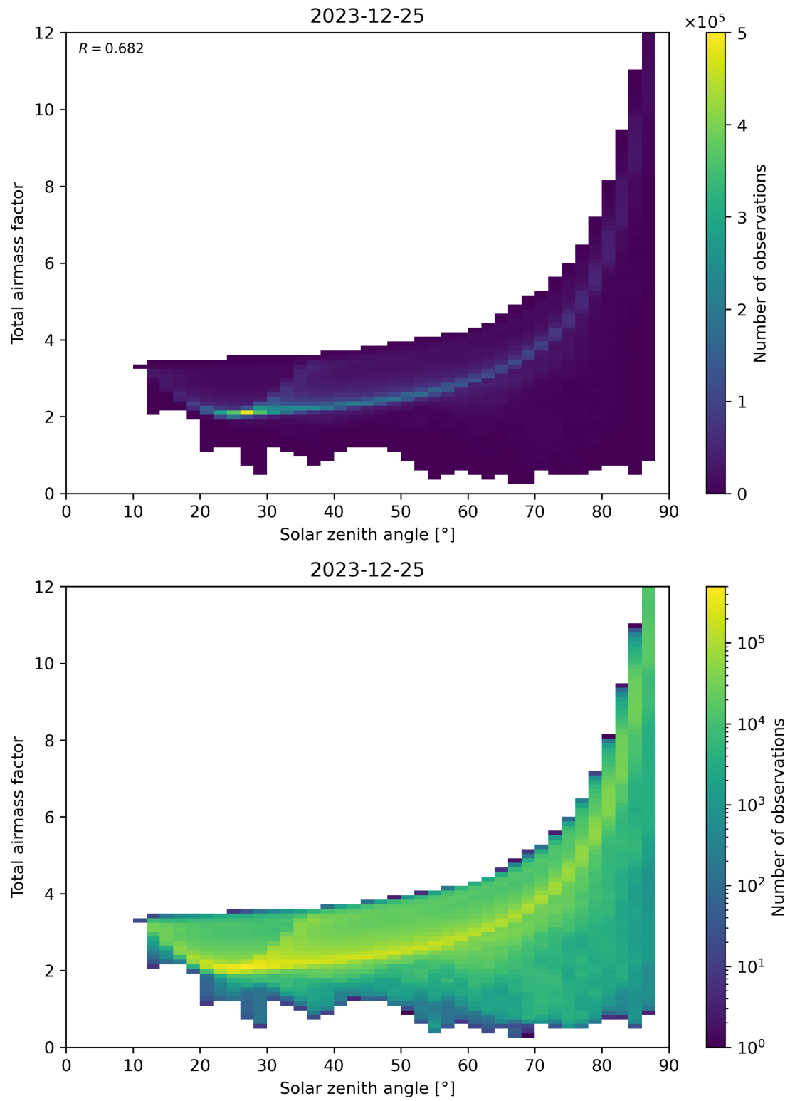
Figure 146: Scatter density plot of “Solar zenith angle” against “Total air mass factor” for 2023-12-25 to 2023-12-26.
