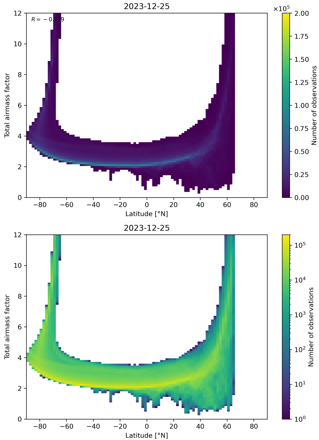
Figure 84: Scatter density plot of “Latitude” against “Total airmass factor” for 2023-12-25 to 2023-12-26.
