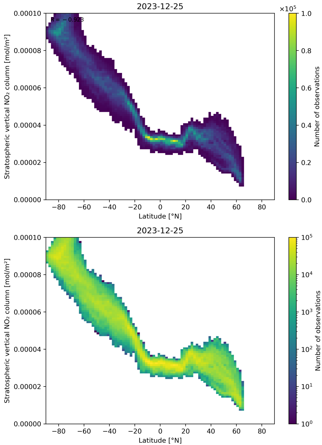
Figure 87: Scatter density plot of “Latitude” against “Stratospheric vertical NO 2 column” for 2023-12-25 to 2023-12-26.
