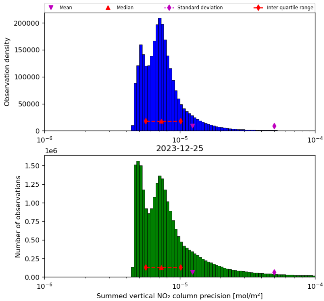
Figure 41: Histogram of “Summed vertical NO 2 column precision” for 2023-12-25 to 2023-12-26
