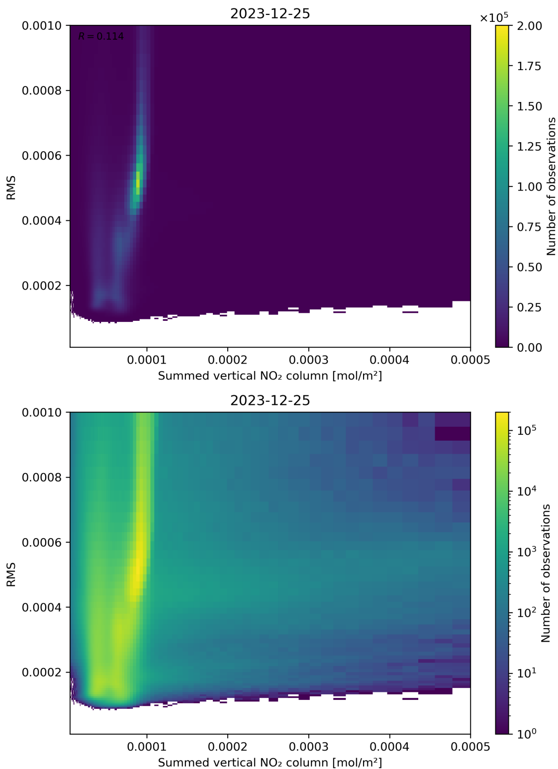
Figure 109: Scatter density plot of “Summed vertical NO 2 column” against “RMS” for 2023-12-25 to 2023-12-26.
