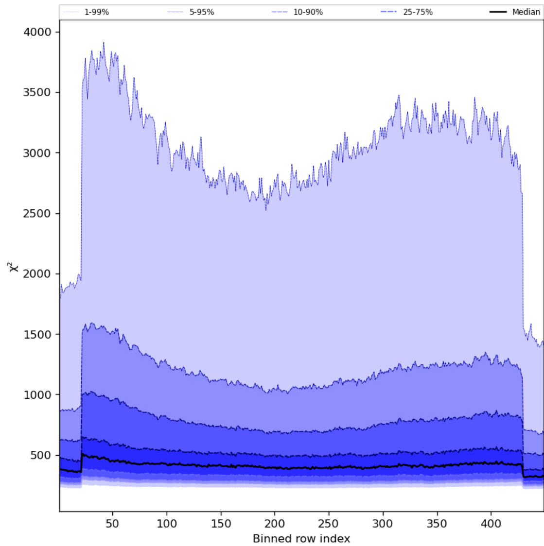
Figure 59: Along track statistics of “ \chi^2 ” for 2023-12-25 to 2023-12-26
