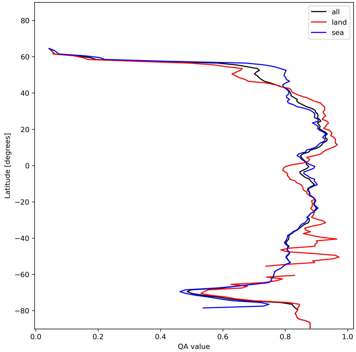
Figure 11: Zonal average of “QA value” for 2023-12-25 to 2023-12-26.
