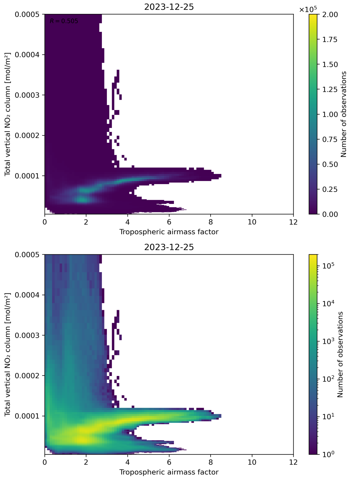
Figure 77: Scatter density plot of “Tropospheric airmass factor” against “Total vertical NO 2 column” for 2023-12-25 to 2023-12-26.
