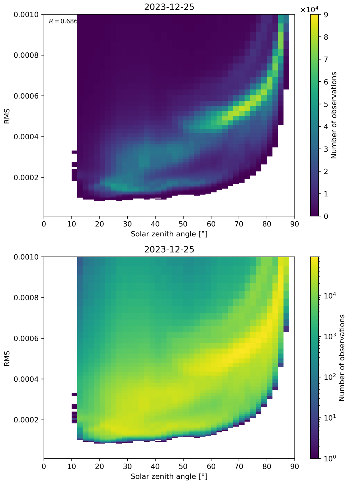
Figure 157: Scatter density plot of “Solar zenith angle” against “RMS” for 2023-12-25 to 2023-12-26.
