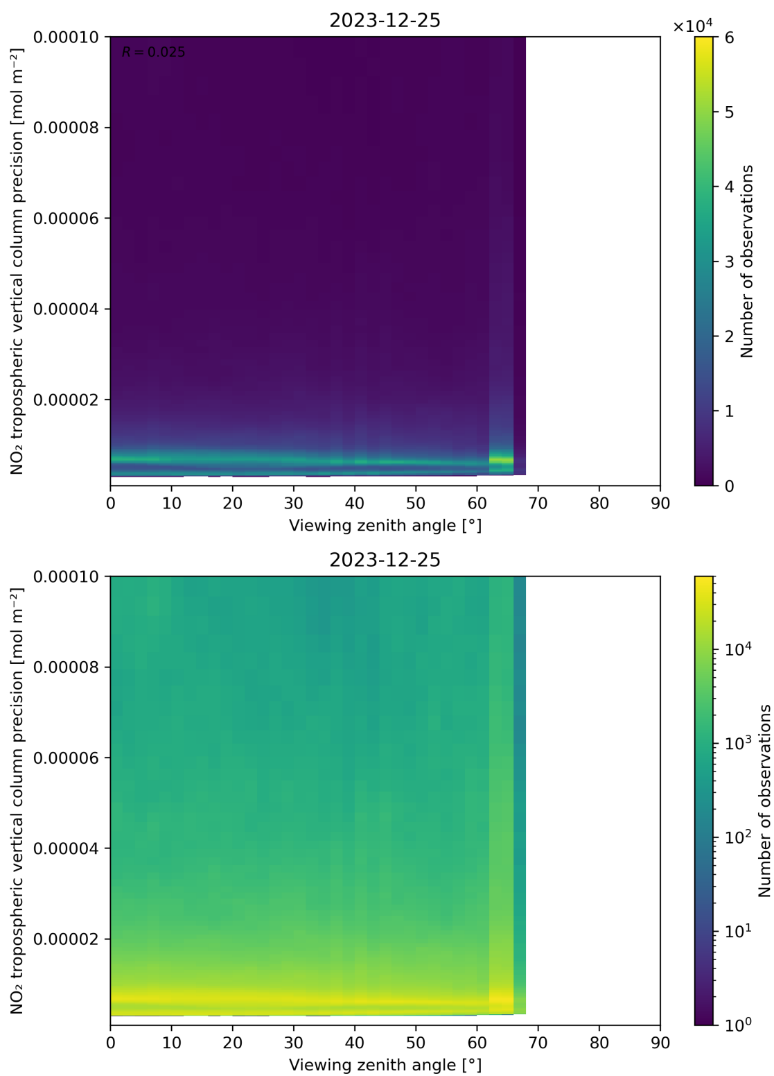
Figure 170: Scatter density plot of “Viewing zenith angle” against “NO 2 tropospheric vertical column precision” for 2023-12-25 to 2023-12-26.
