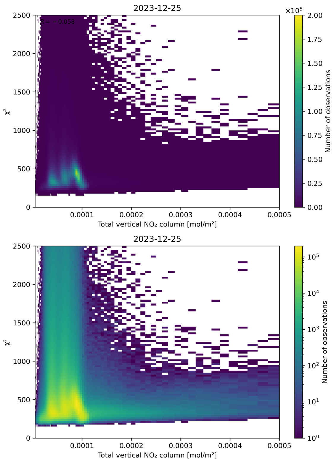
Figure 111: Scatter density plot of “Total vertical NO 2 column” against “ \chi^2 ” for 2023-12-25 to 2023-12-26.
