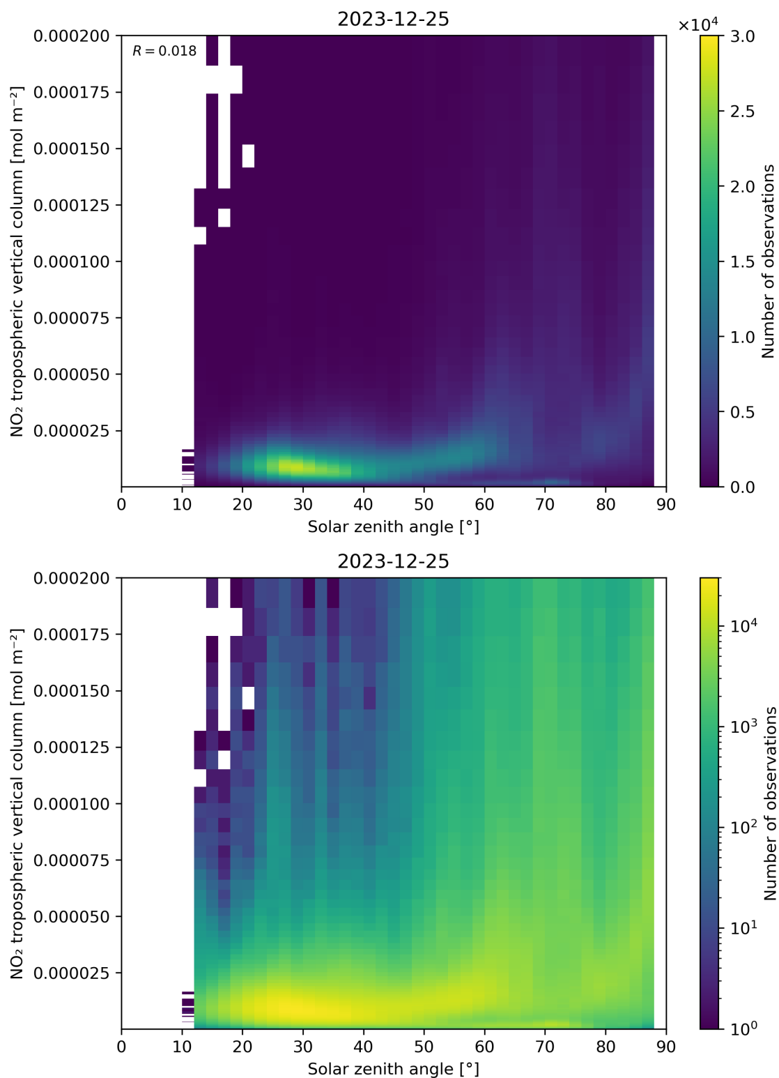
Figure 155: Scatter density plot of “Solar zenith angle” against “NO 2 tropospheric vertical column” for 2023-12-25 to 2023-12-26.
