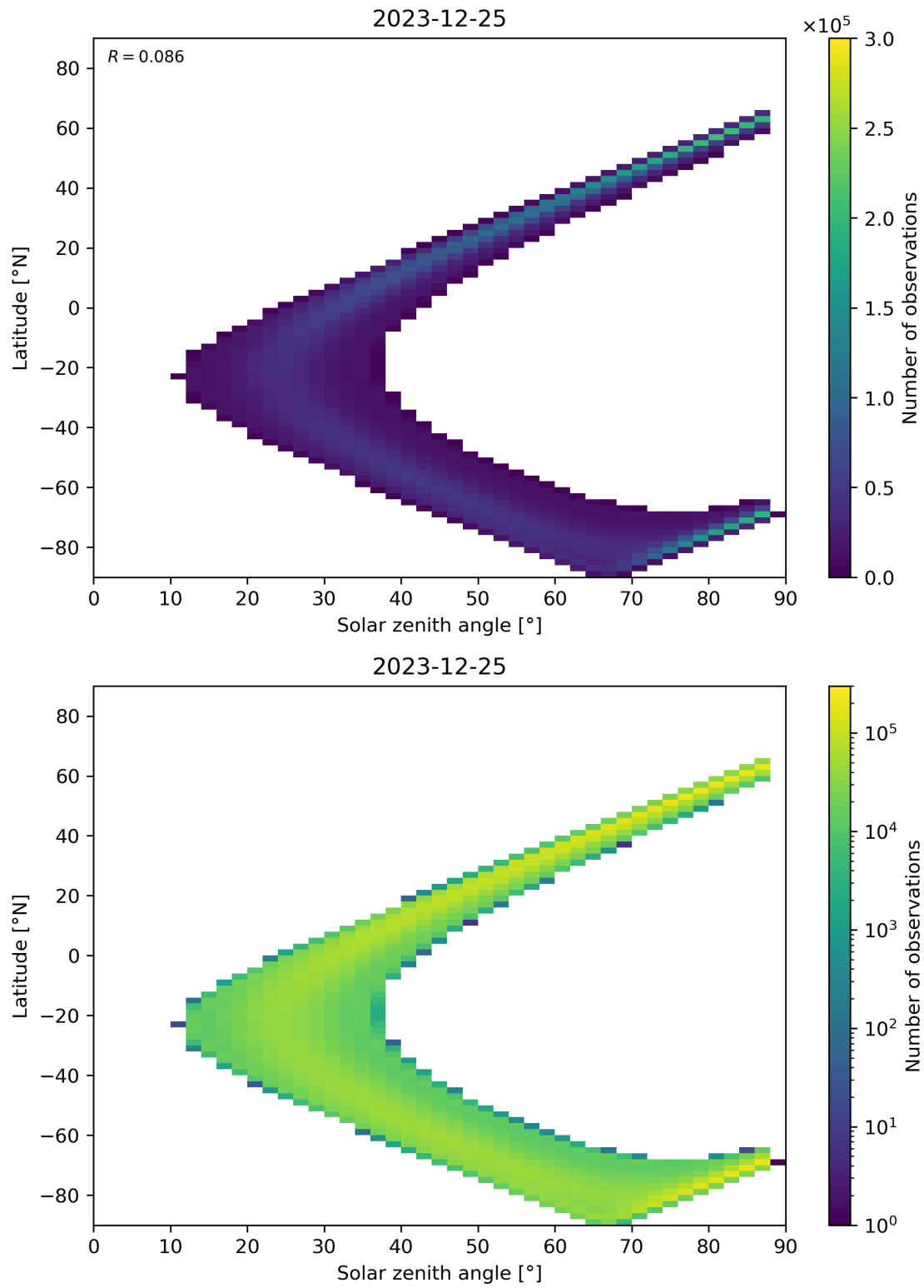
Figure 149: Scatter density plot of “Solar zenith angle” against “Latitude” for 2023-12-25 to 2023-12-26.
