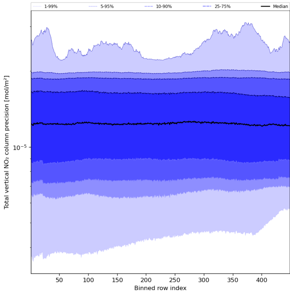
Figure 56: Along track statistics of “Total vertical NO 2 column precision” for 2023-12-25 to 2023-12-26
