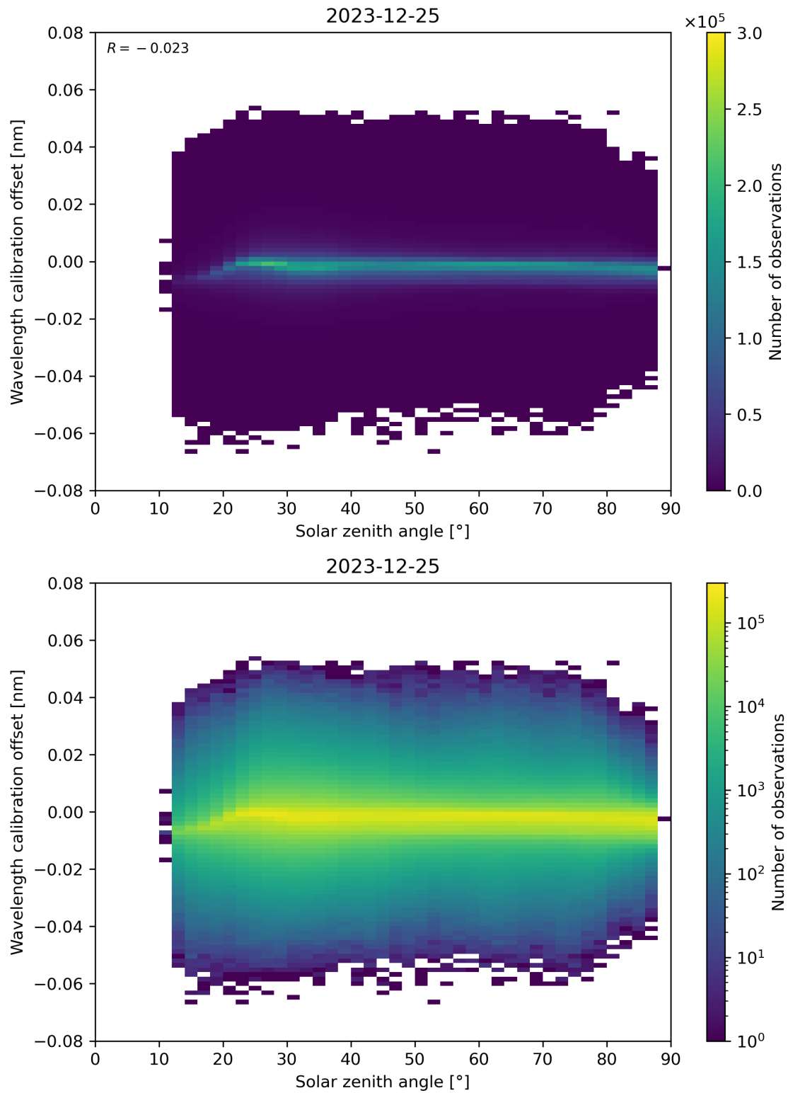
Figure 158: Scatter density plot of “Solar zenith angle” against “Wavelength calibration offset” for 2023-12-25 to 2023-12-26.
