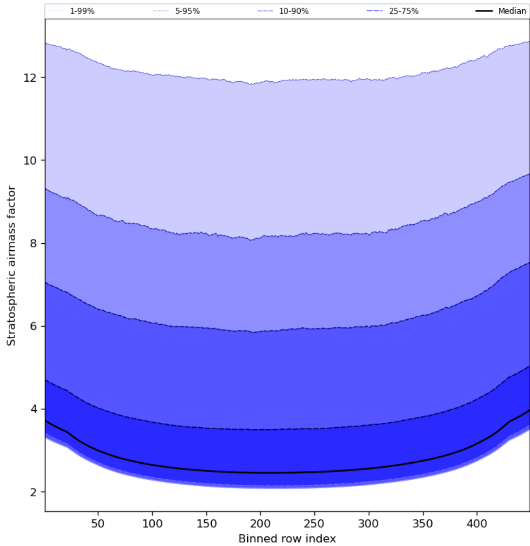
Figure 61: Along track statistics of “Stratospheric airmass factor” for 2023-12-25 to 2023-12-26
