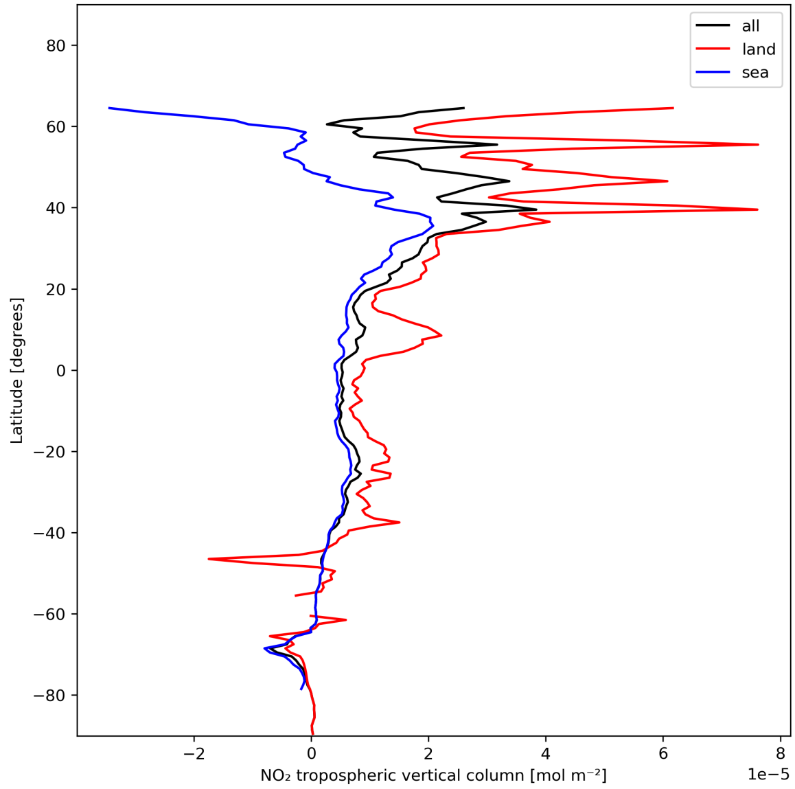
Figure 12: Zonal average of “NO 2 tropospheric vertical column” for 2023-12-25 to 2023-12-26.
