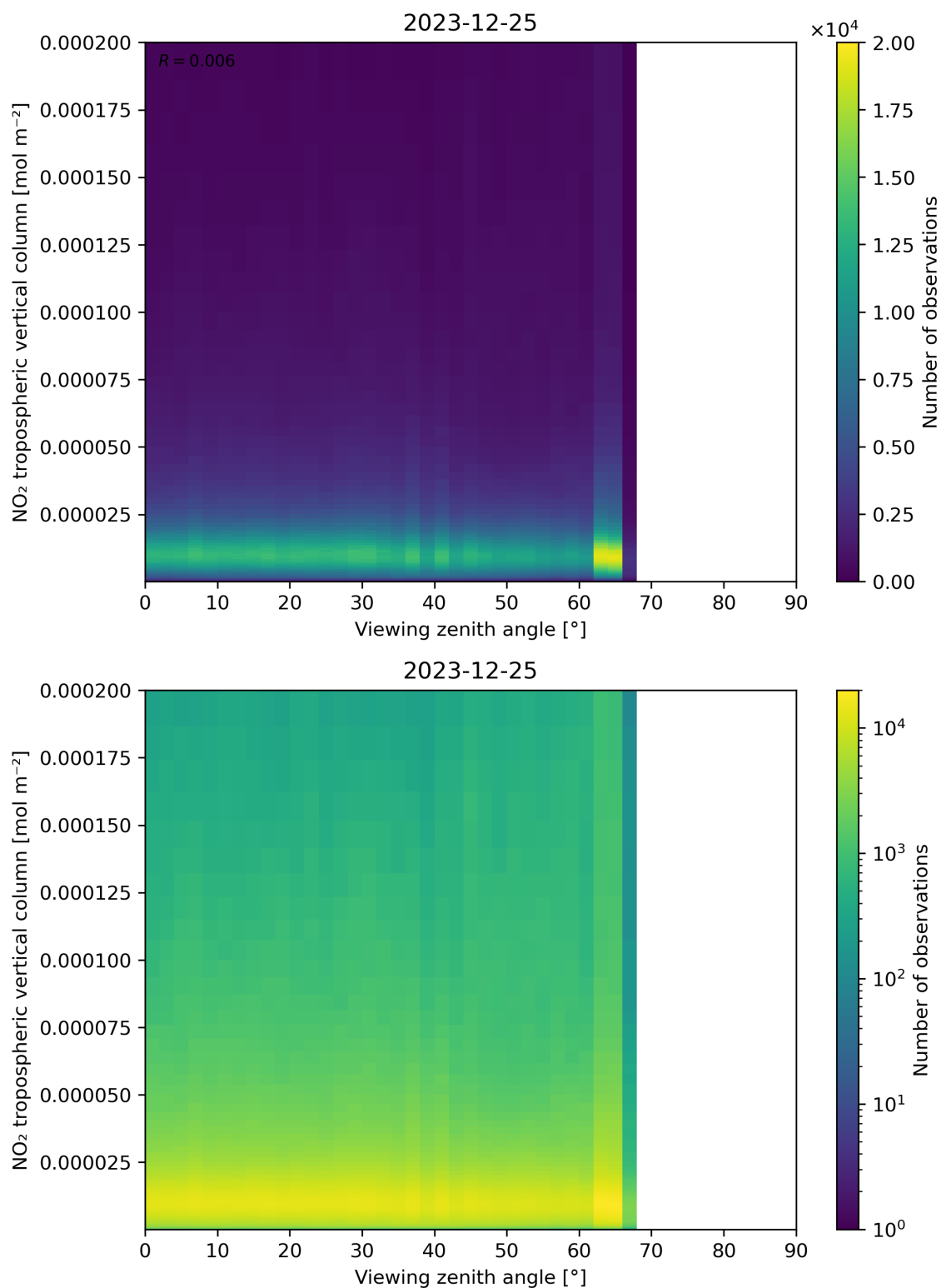
Figure 169: Scatter density plot of “Viewing zenith angle” against “NO 2 tropospheric vertical column” for 2023-12-25 to 2023-12-26.
