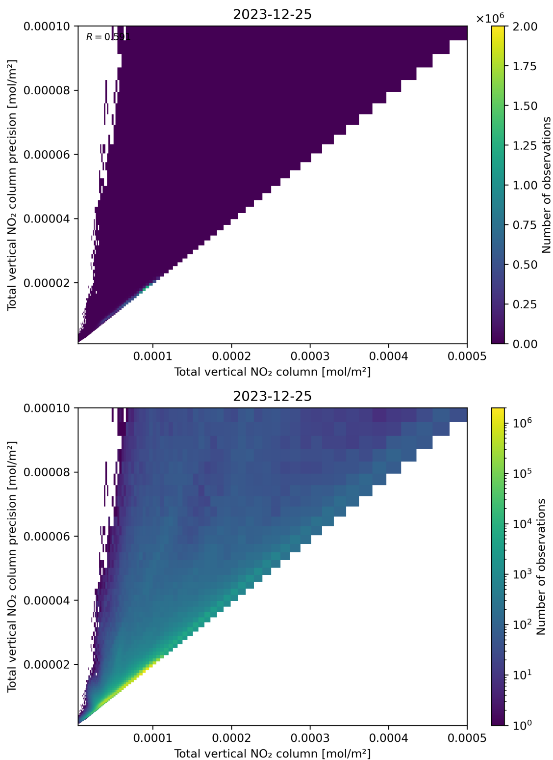
Figure 114: Scatter density plot of “Total vertical NO 2 column” against “Total vertical NO 2 column precision” for 2023-12-25 to 2023-12-26.
