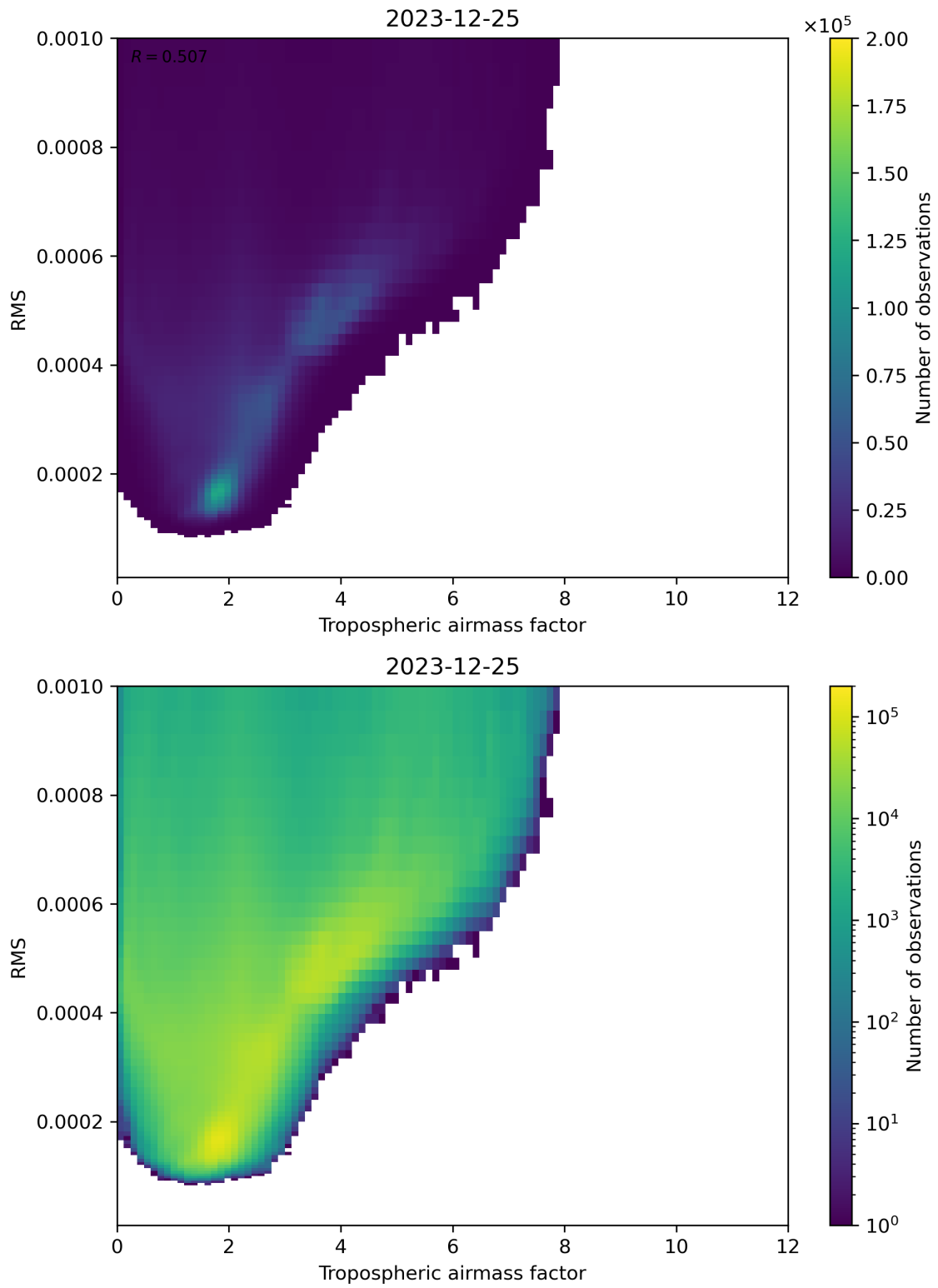
Figure 79: Scatter density plot of “Tropospheric airmass factor” against “RMS” for 2023-12-25 to 2023-12-26.
