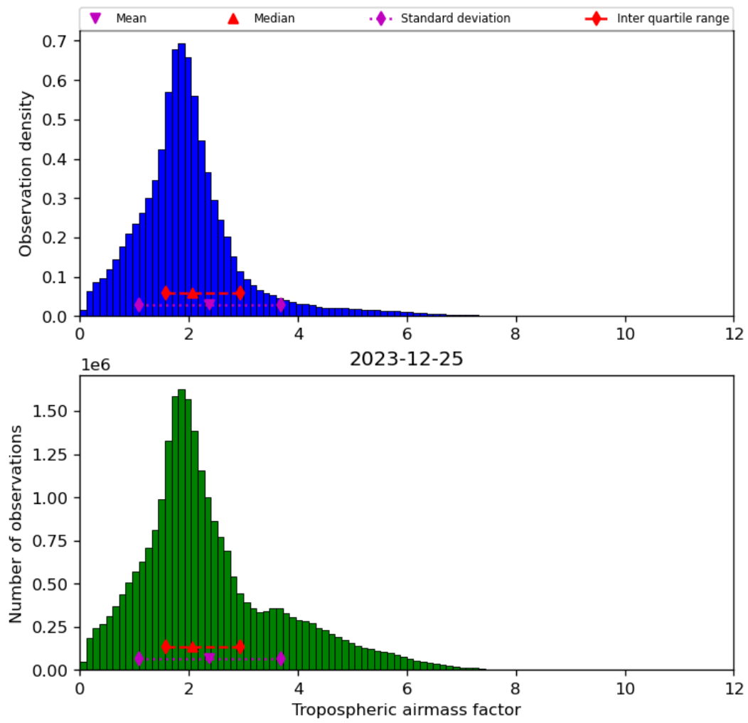
Figure 31: Histogram of “Tropospheric airmass factor” for 2023-12-25 to 2023-12-26
