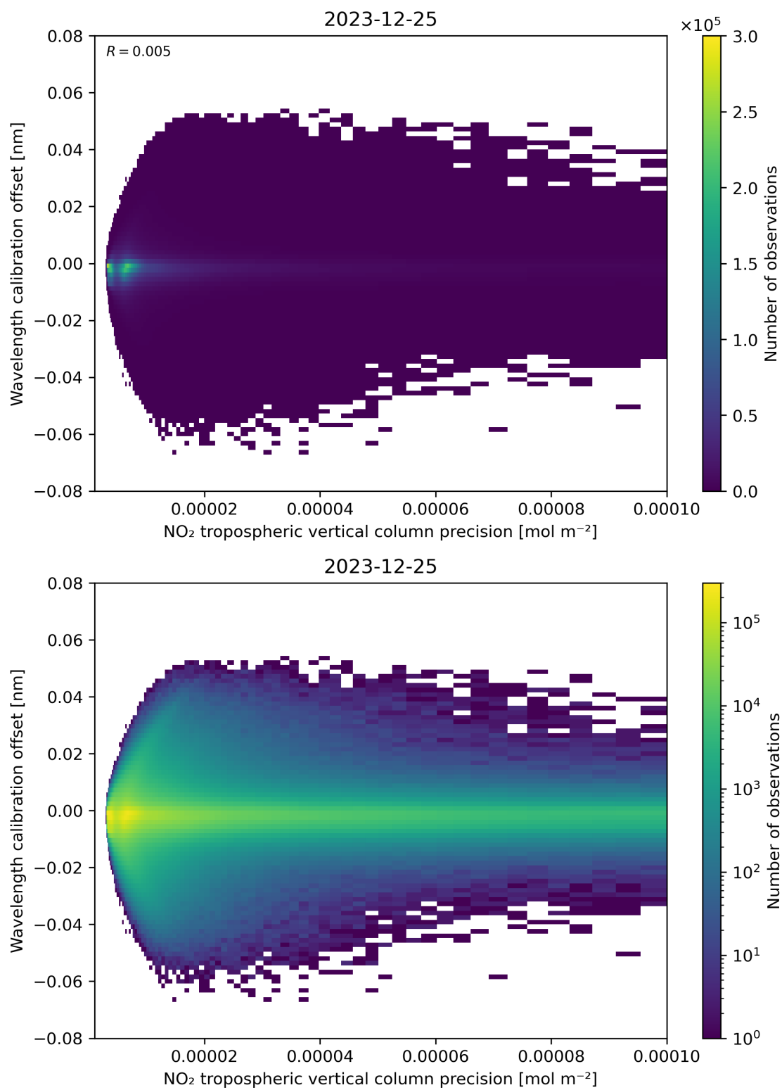
Figure 141: Scatter density plot of “NO 2 tropospheric vertical column precision” against “Wavelength calibration offset” for 2023-12-25 to 2023-12-26.
