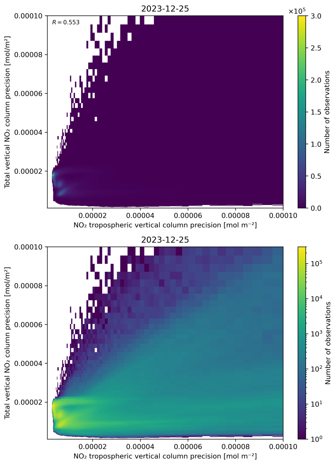
Figure 139: Scatter density plot of “NO 2 tropospheric vertical column precision” against “Total vertical NO 2 column precision” for 2023-12-25 to 2023-12-26.
