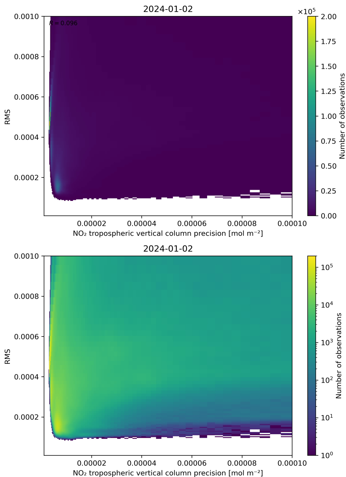
Figure 140: Scatter density plot of “NO 2 tropospheric vertical column precision” against “RMS” for 2024-01-01 to 2024-01-03.
