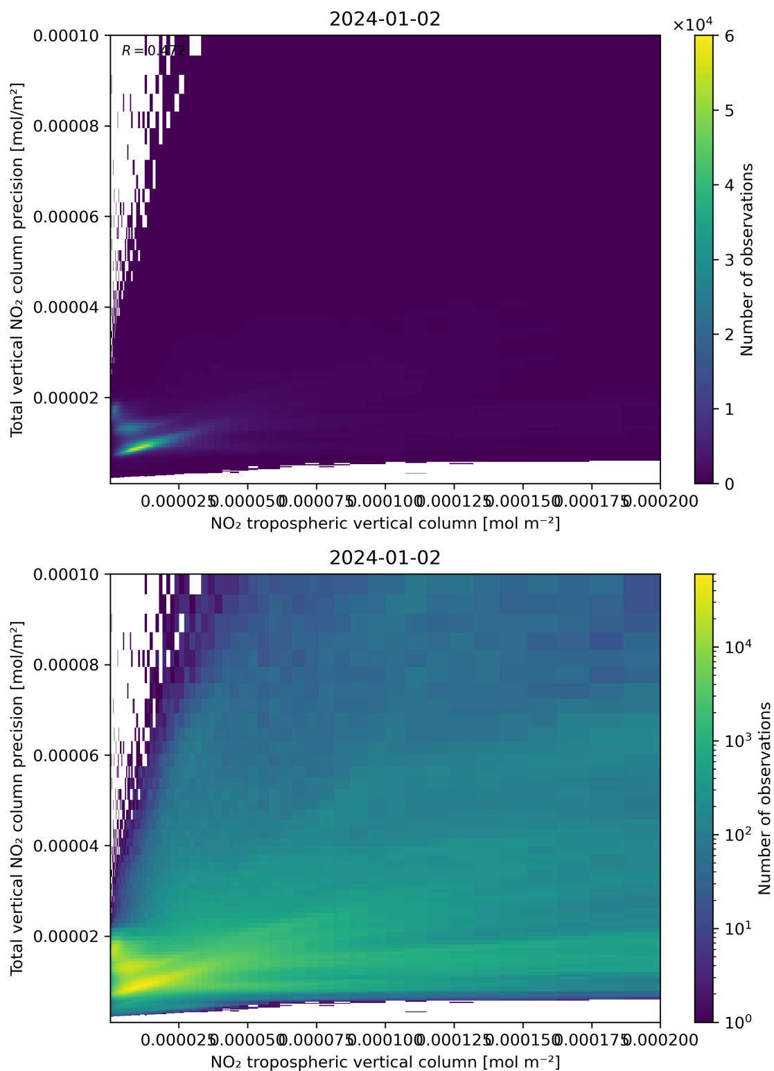
Figure 129: Scatter density plot of “NO 2 tropospheric vertical column” against “Total vertical NO 2 column precision” for 2024-01-01 to 2024-01-03.
