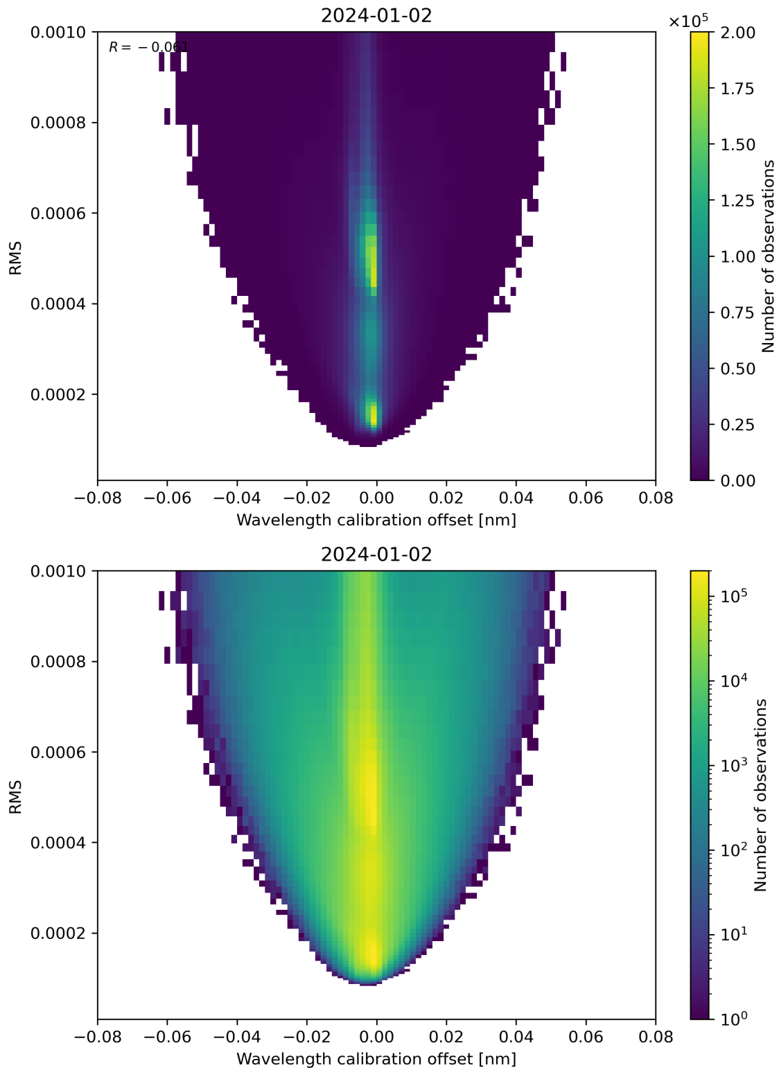
Figure 181: Scatter density plot of “Wavelength calibration offset” against “RMS” for 2024-01-01 to 2024-01-03.
