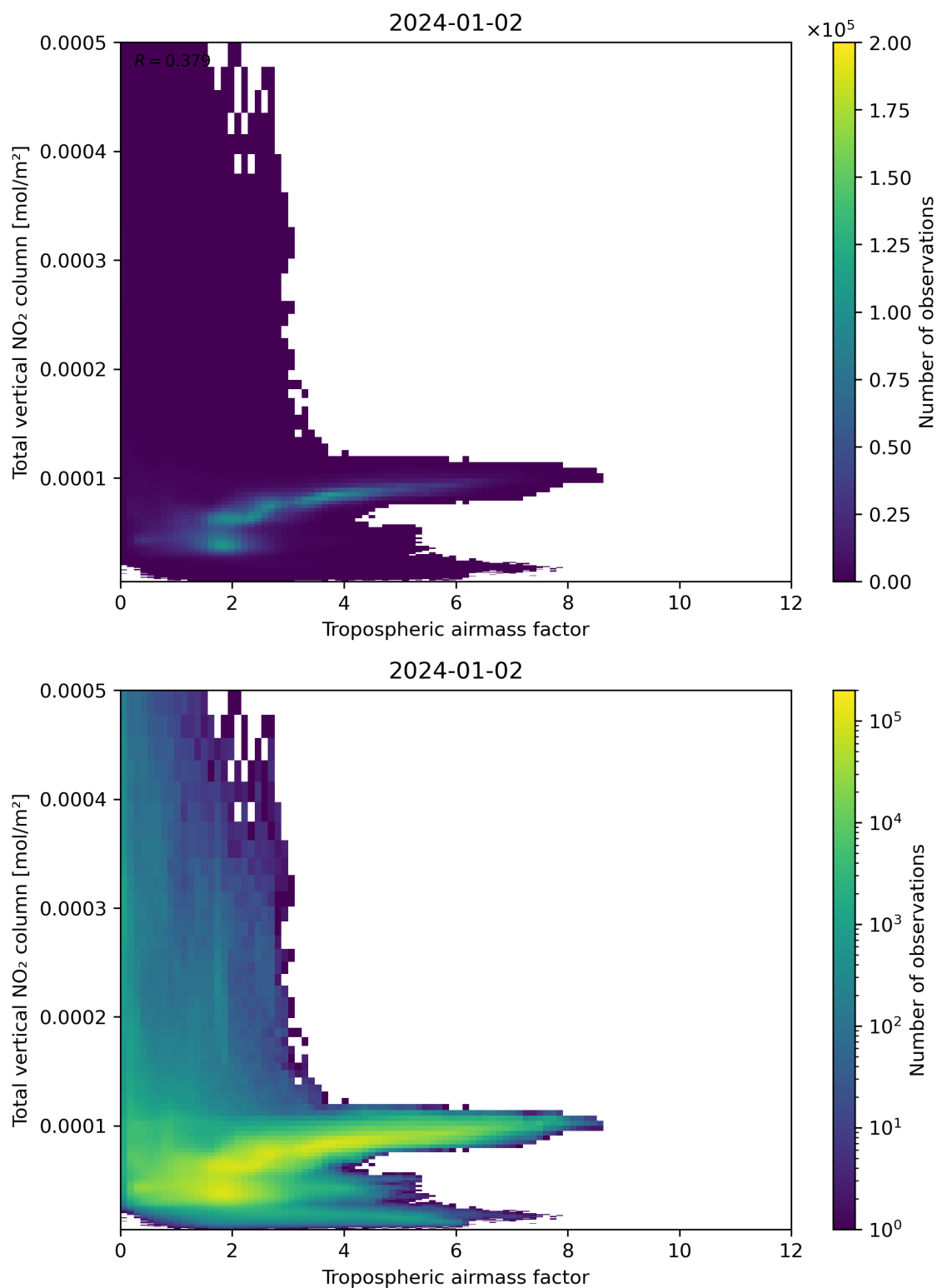
Figure 77: Scatter density plot of “Tropospheric airmass factor” against “Total vertical NO 2 column” for 2024-01-01 to 2024-01-03.
