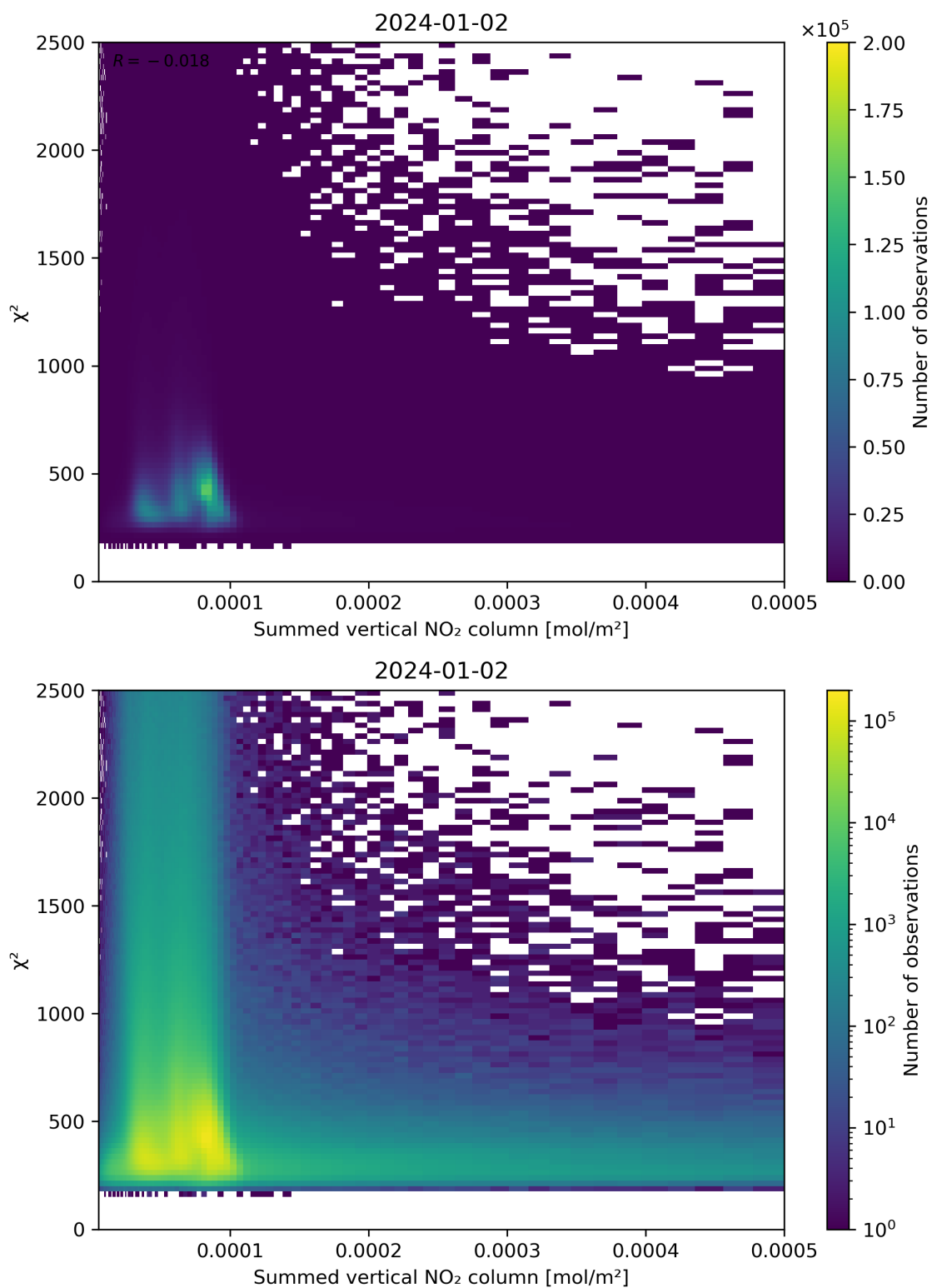
Figure 104: Scatter density plot of “Summed vertical NO 2 column” against “ \chi^2 ” for 2024-01-01 to 2024-01-03.
