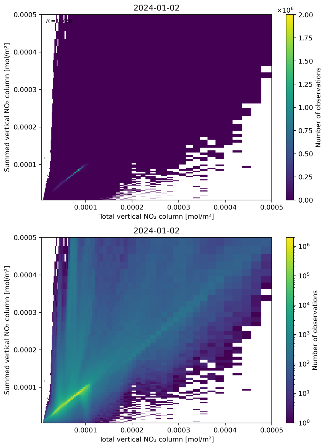
Figure 112: Scatter density plot of “Total vertical NO 2 column” against “Summed vertical NO 2 column” for 2024-01-01 to 2024-01-03.
