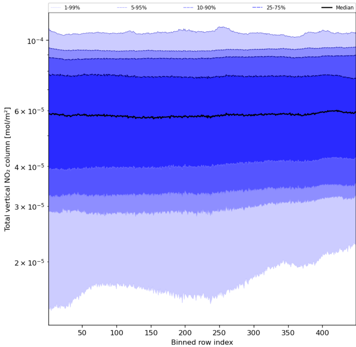
Figure 55: Along track statistics of “Total vertical NO 2 column” for 2024-01-01 to 2024-01-03
