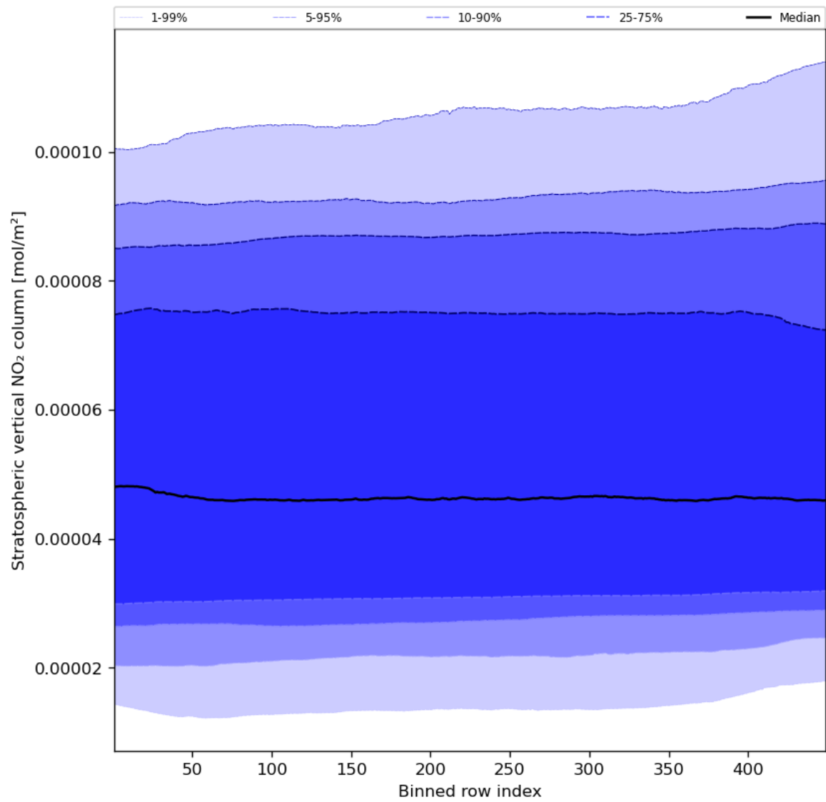
Figure 53: Along track statistics of “Stratospheric vertical NO 2 column” for 2024-01-01 to 2024-01-03
