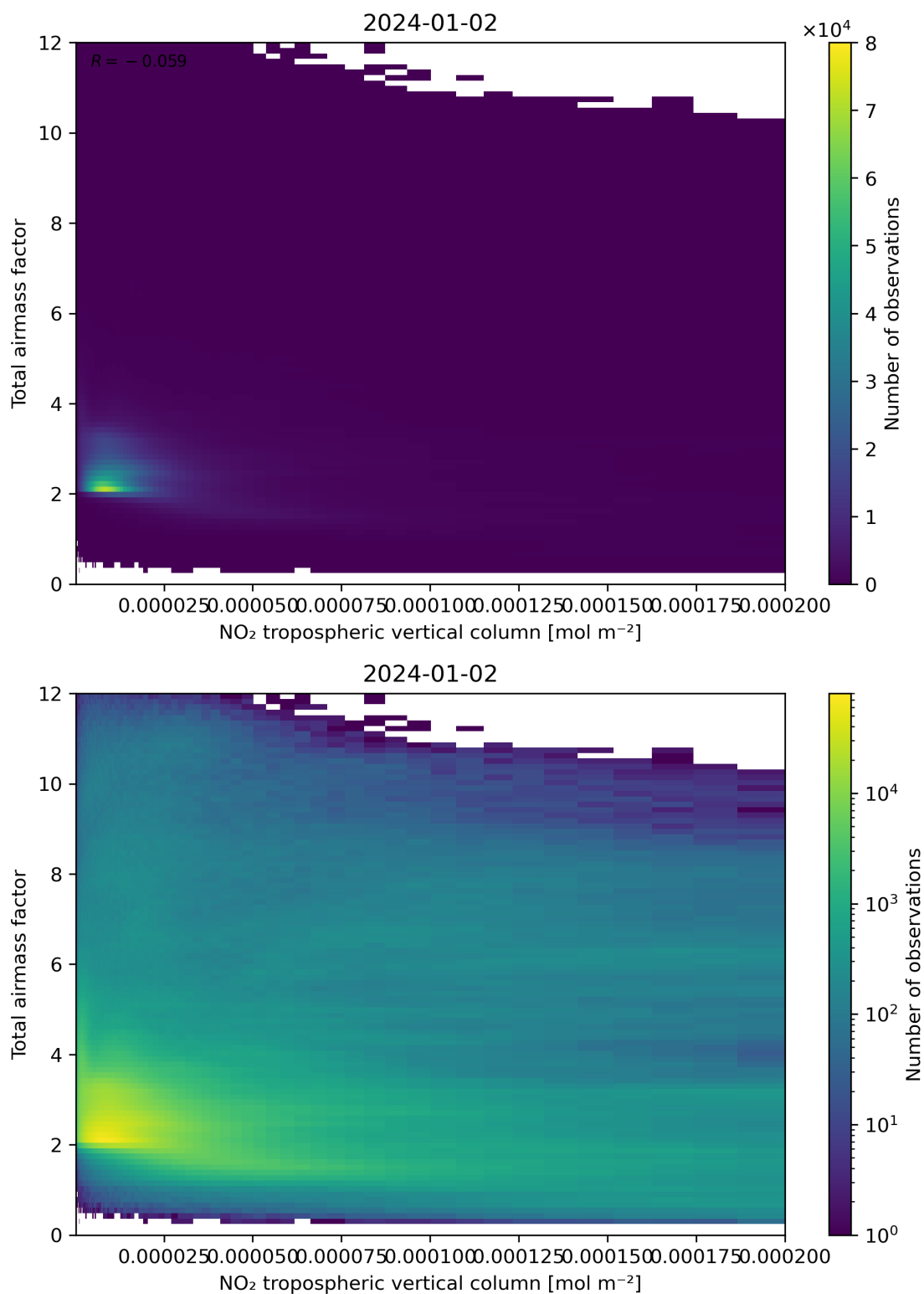
Figure 122: Scatter density plot of “NO 2 tropospheric vertical column” against “Total air mass factor” for 2024-01-01 to 2024-01-03.
