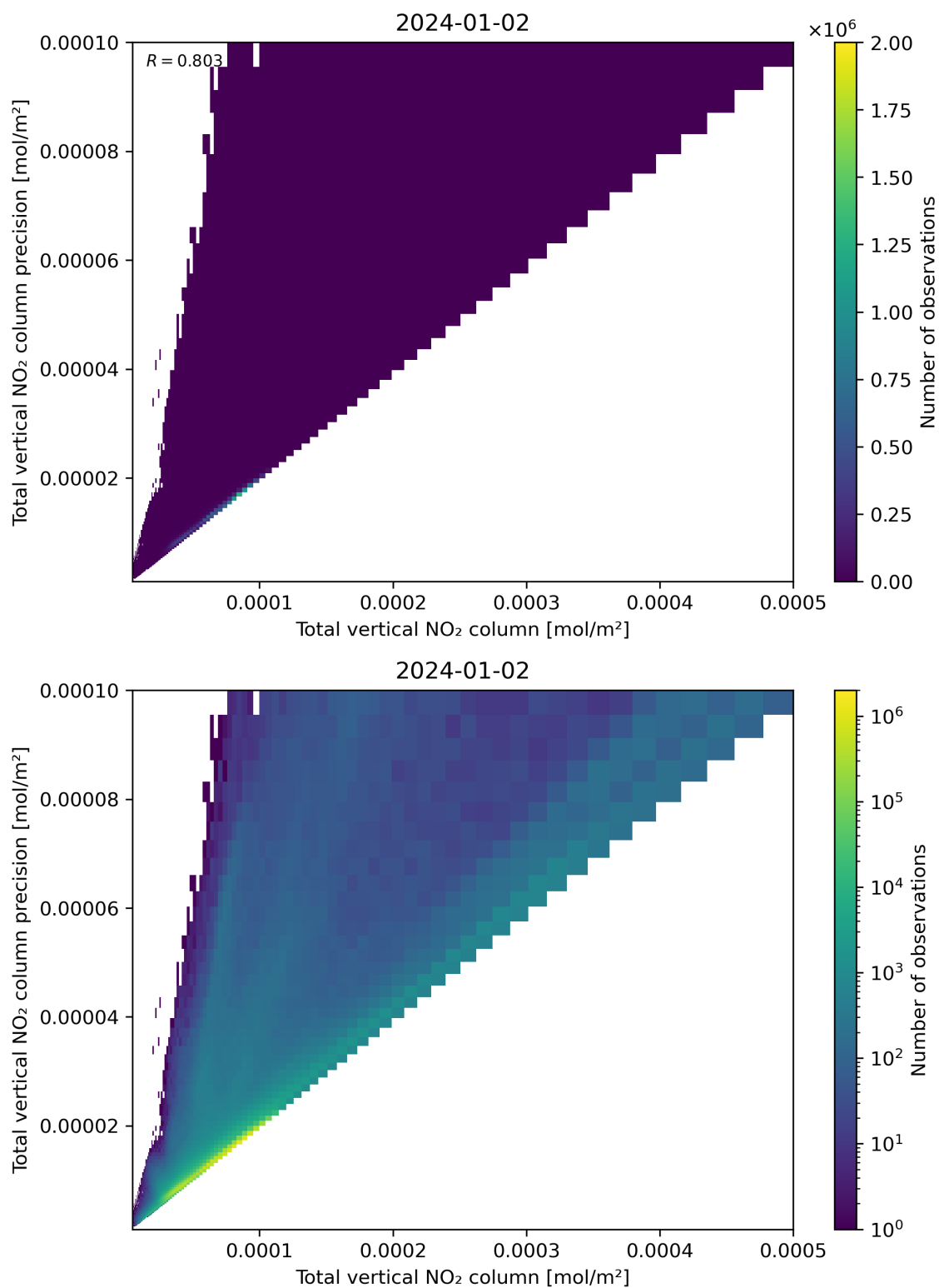
Figure 114: Scatter density plot of “Total vertical NO 2 column” against “Total vertical NO 2 column precision” for 2024-01-01 to 2024-01-03.
