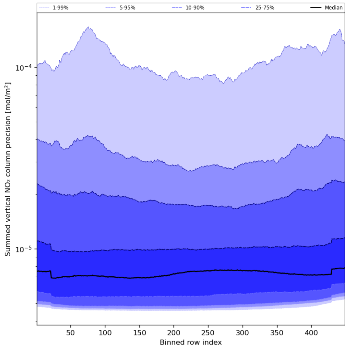
Figure 58: Along track statistics of “Summed vertical NO 2 column precision” for 2024-01-01 to 2024-01-03
