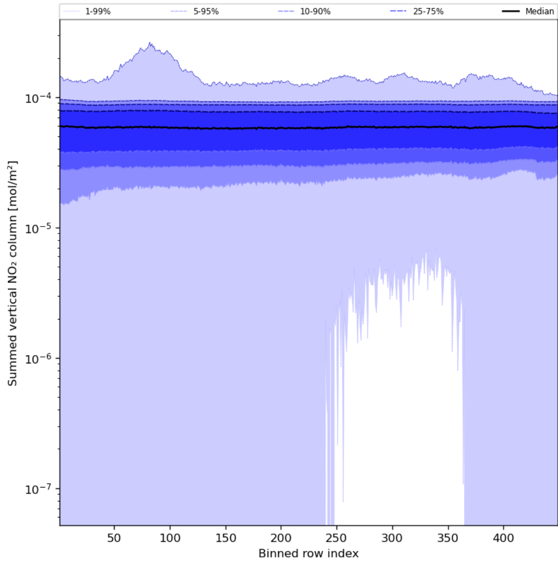
Figure 57: Along track statistics of “Summed vertical NO 2 column” for 2024-01-01 to 2024-01-03
