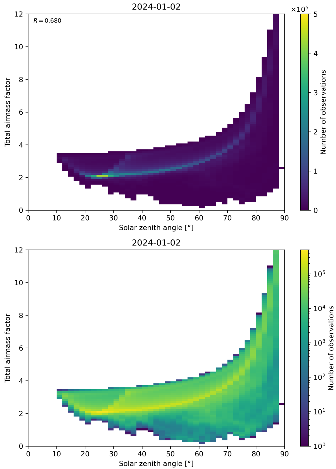
Figure 146: Scatter density plot of “Solar zenith angle” against “Total air mass factor” for 2024-01-01 to 2024-01-03.
