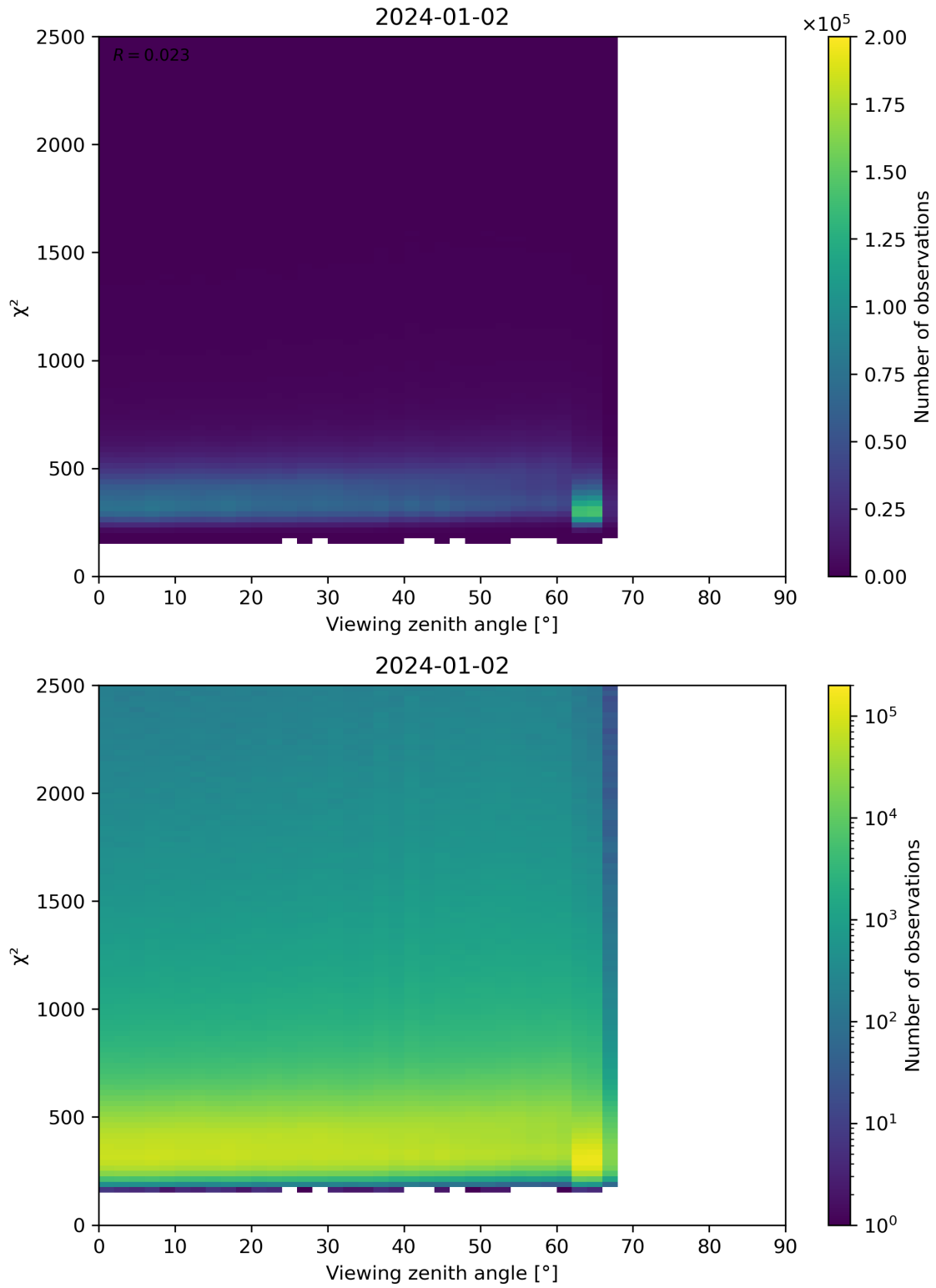
Figure 162: Scatter density plot of “Viewing zenith angle” against “ \chi^2 ” for 2024-01-01 to 2024-01-03.
