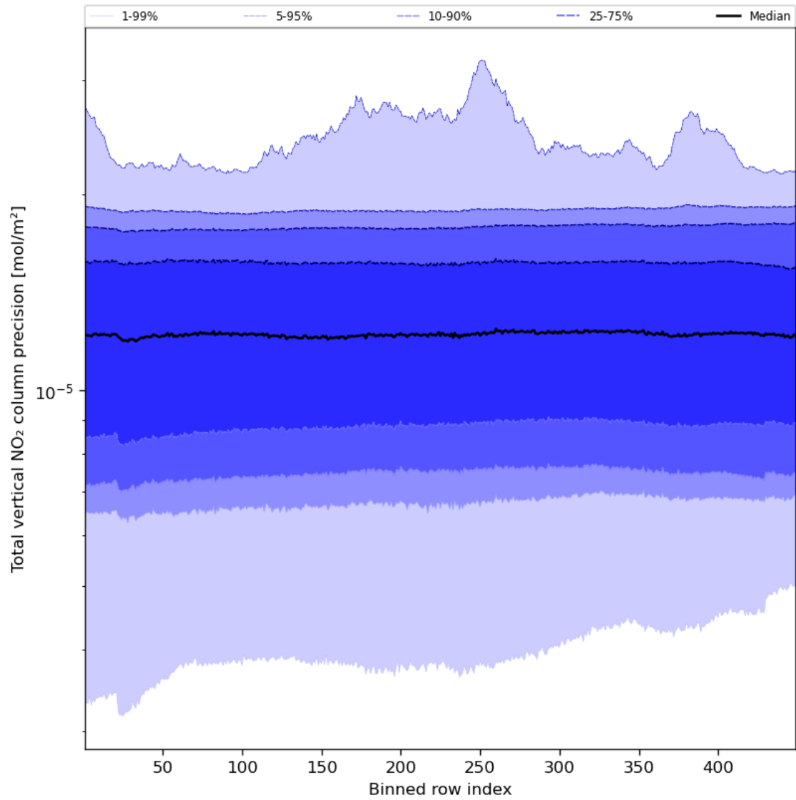
Figure 56: Along track statistics of “Total vertical NO 2 column precision” for 2024-01-01 to 2024-01-03
