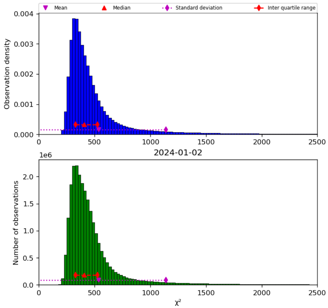
Figure 42: Histogram of “ \chi^2 ” for 2024-01-01 to 2024-01-03
