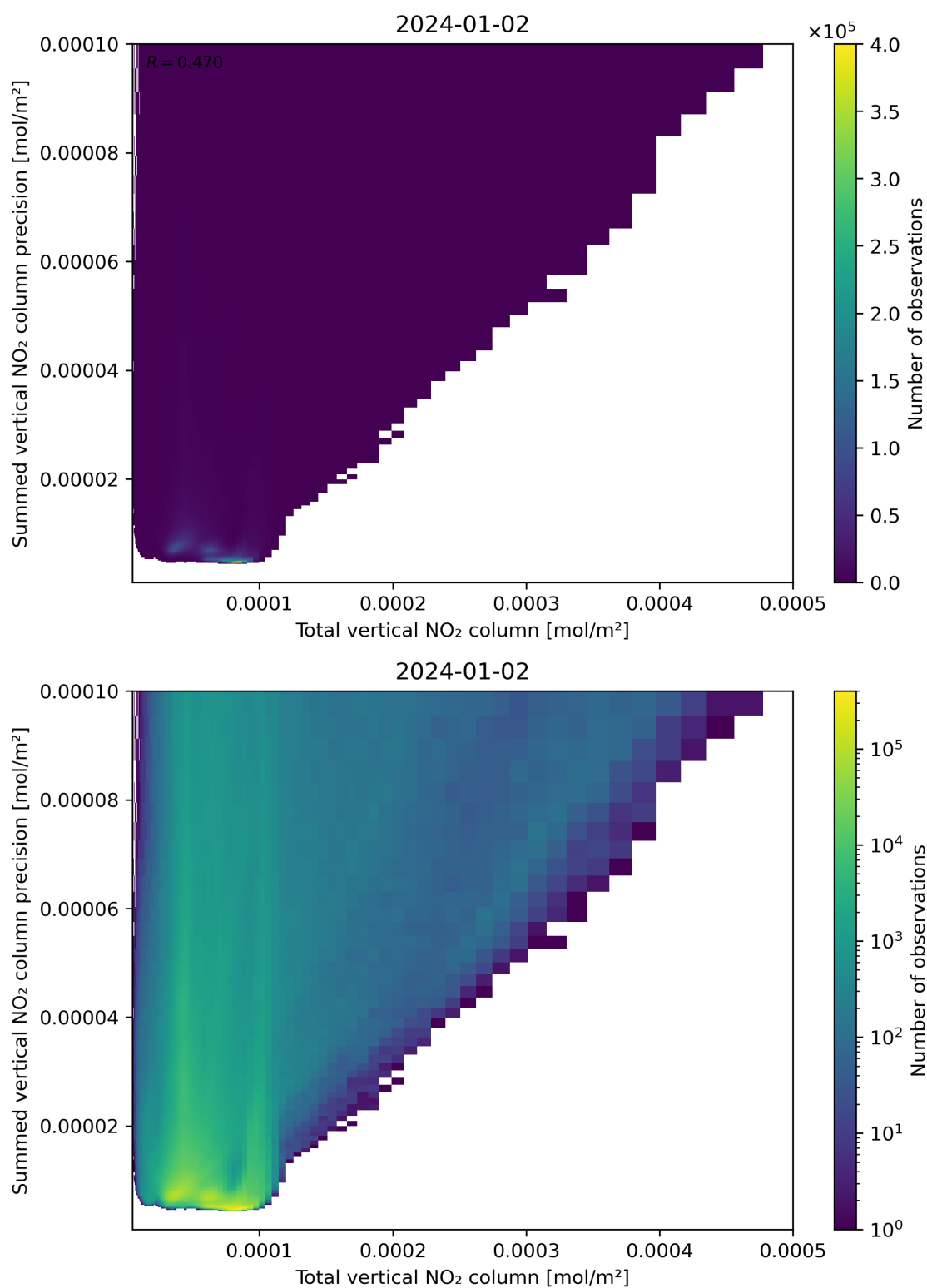
Figure 113: Scatter density plot of “Total vertical NO 2 column” against “Summed vertical NO 2 column precision” for 2024-01-01 to 2024-01-03.
