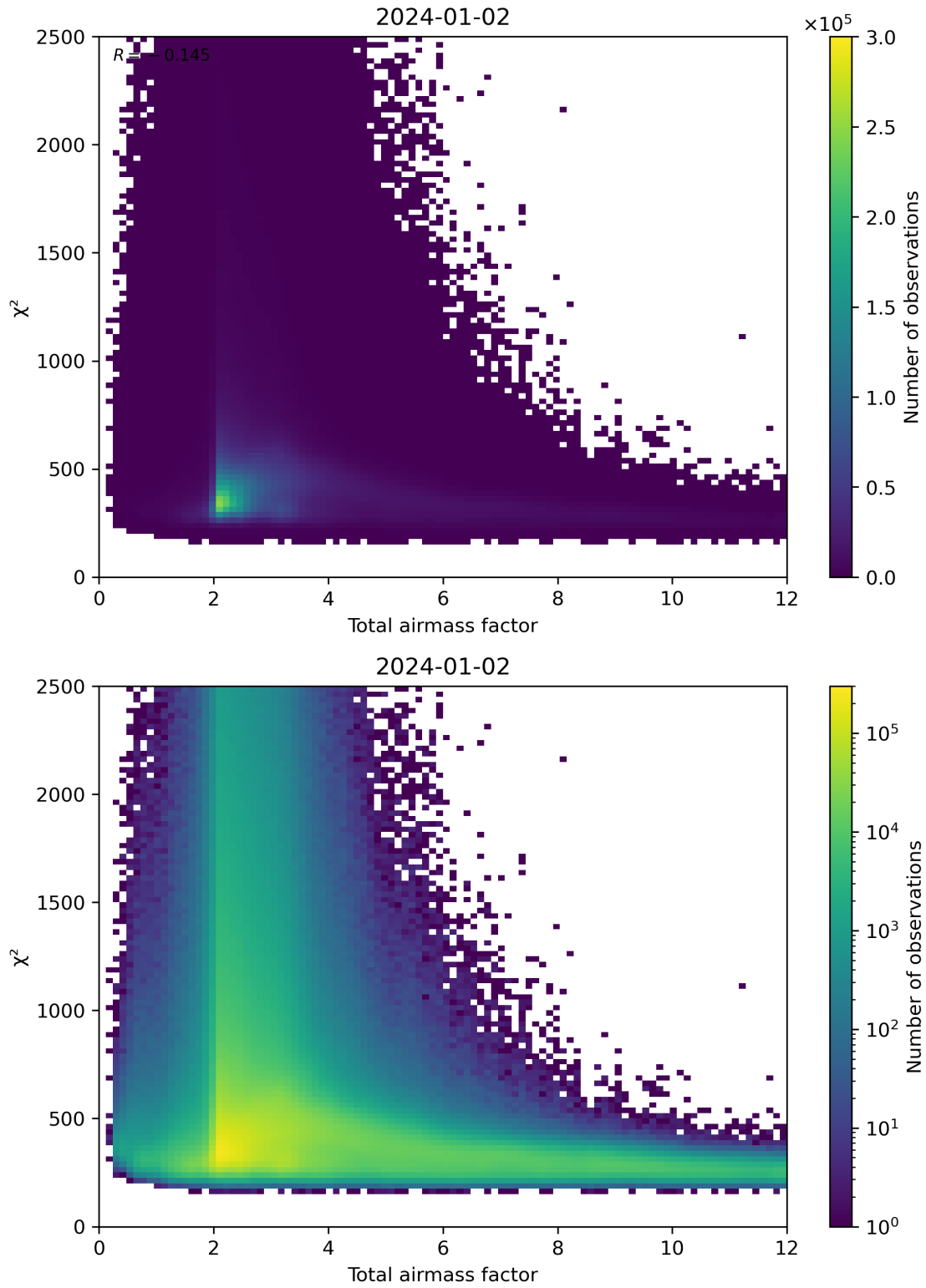
Figure 63: Scatter density plot of “Total airmass factor” against “ \chi^2 ” for 2024-01-01 to 2024-01-03.
