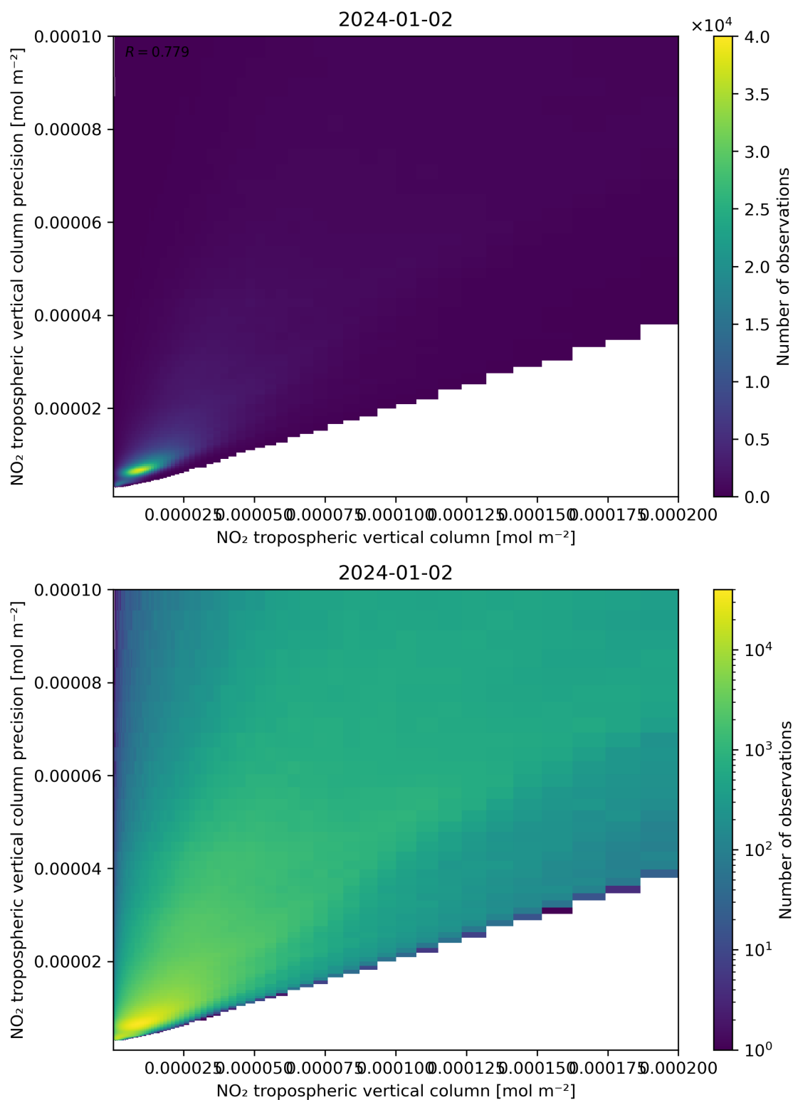
Figure 130: Scatter density plot of “NO 2 tropospheric vertical column” against “NO 2 tropospheric vertical column precision” for 2024-01-01 to 2024-01-03.
