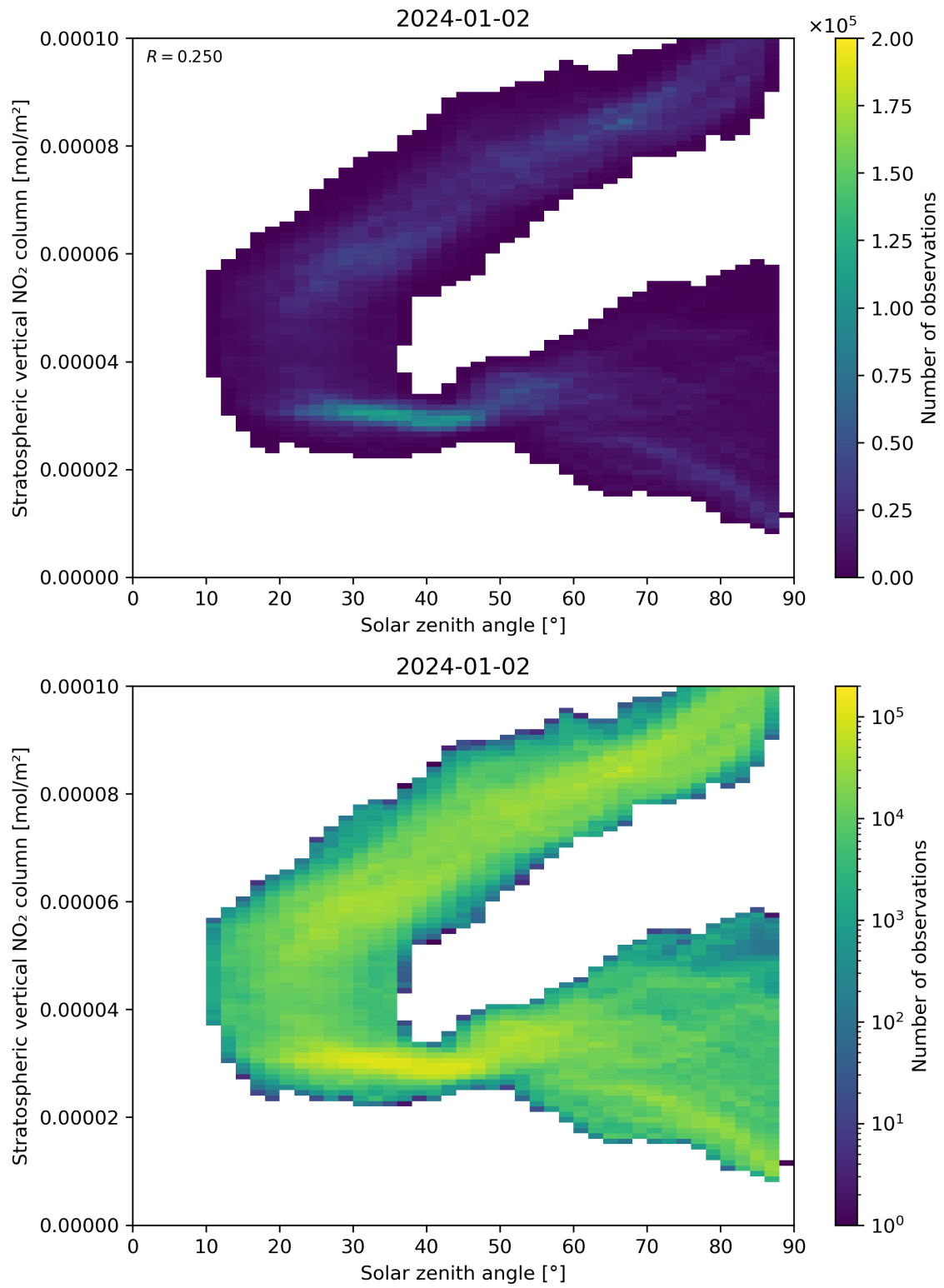
Figure 150: Scatter density plot of “Solar zenith angle” against “Stratospheric vertical NO 2 column” for 2024-01-01 to 2024-01-03.
