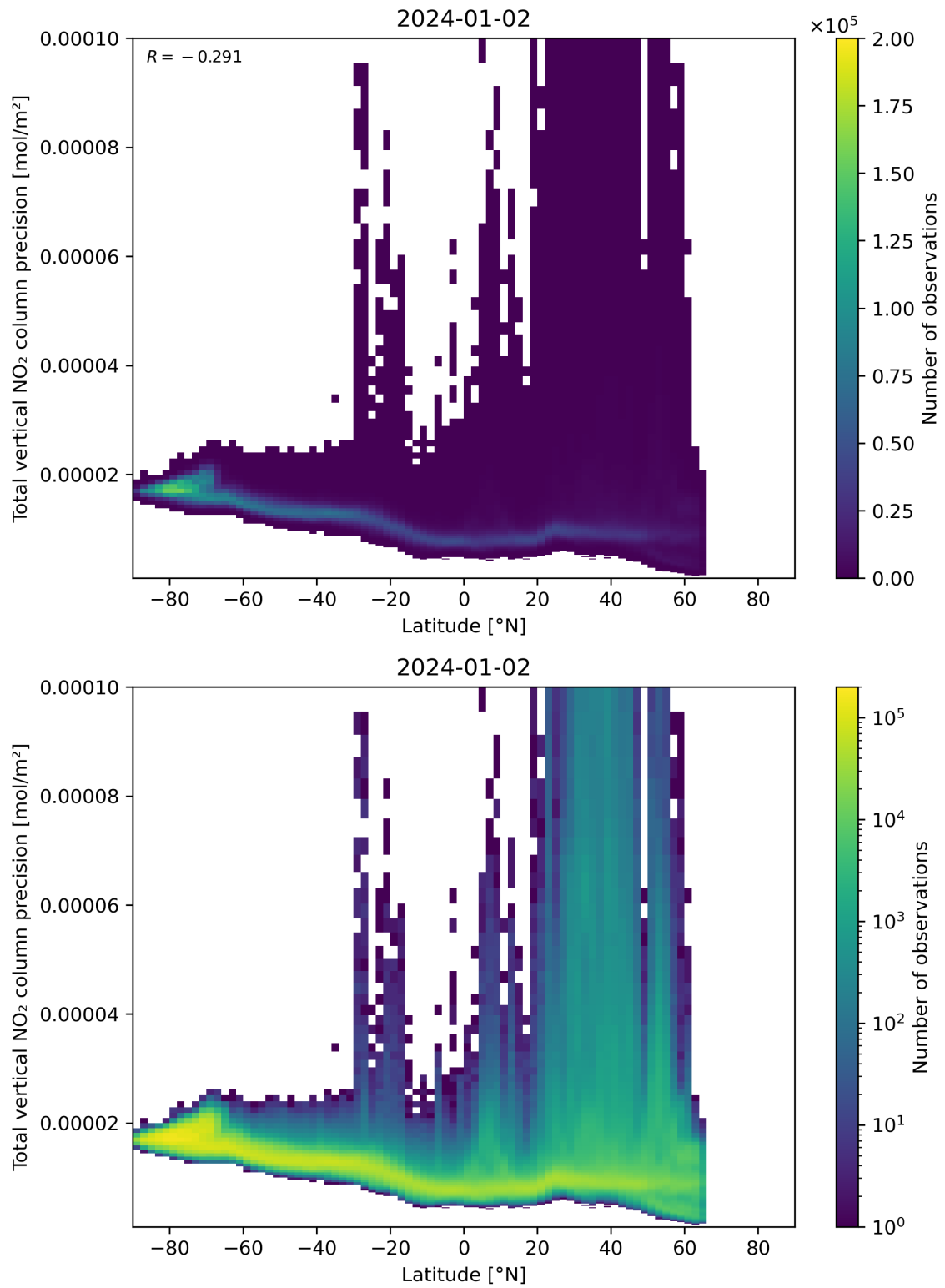
Figure 91: Scatter density plot of “Latitude” against “Total vertical NO 2 column precision” for 2024-01-01 to 2024-01-03.
