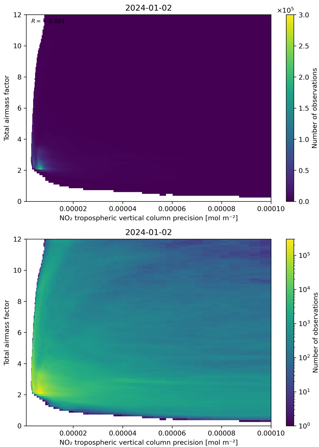
Figure 132: Scatter density plot of “NO 2 tropospheric vertical column precision” against “Total air mass factor” for 2024-01-01 to 2024-01-03.
