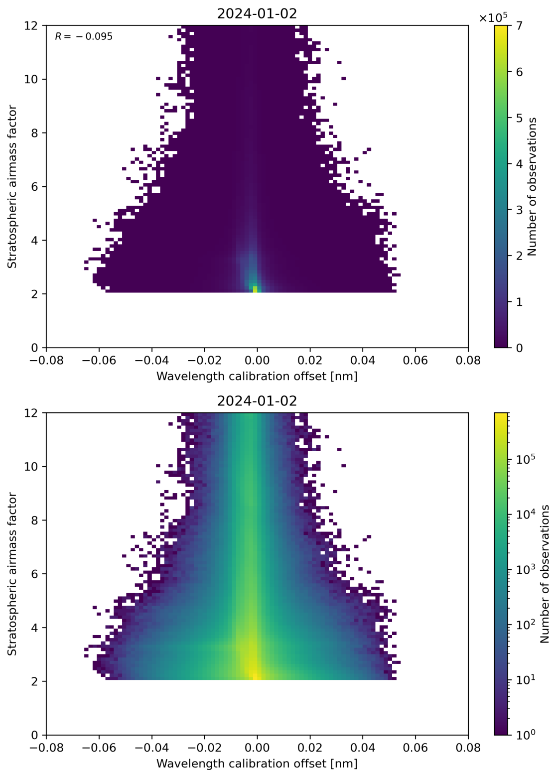
Figure 174: Scatter density plot of “Wavelength calibration offset” against “Stratospheric air mass factor” for 2024-01-01 to 2024-01-03.
