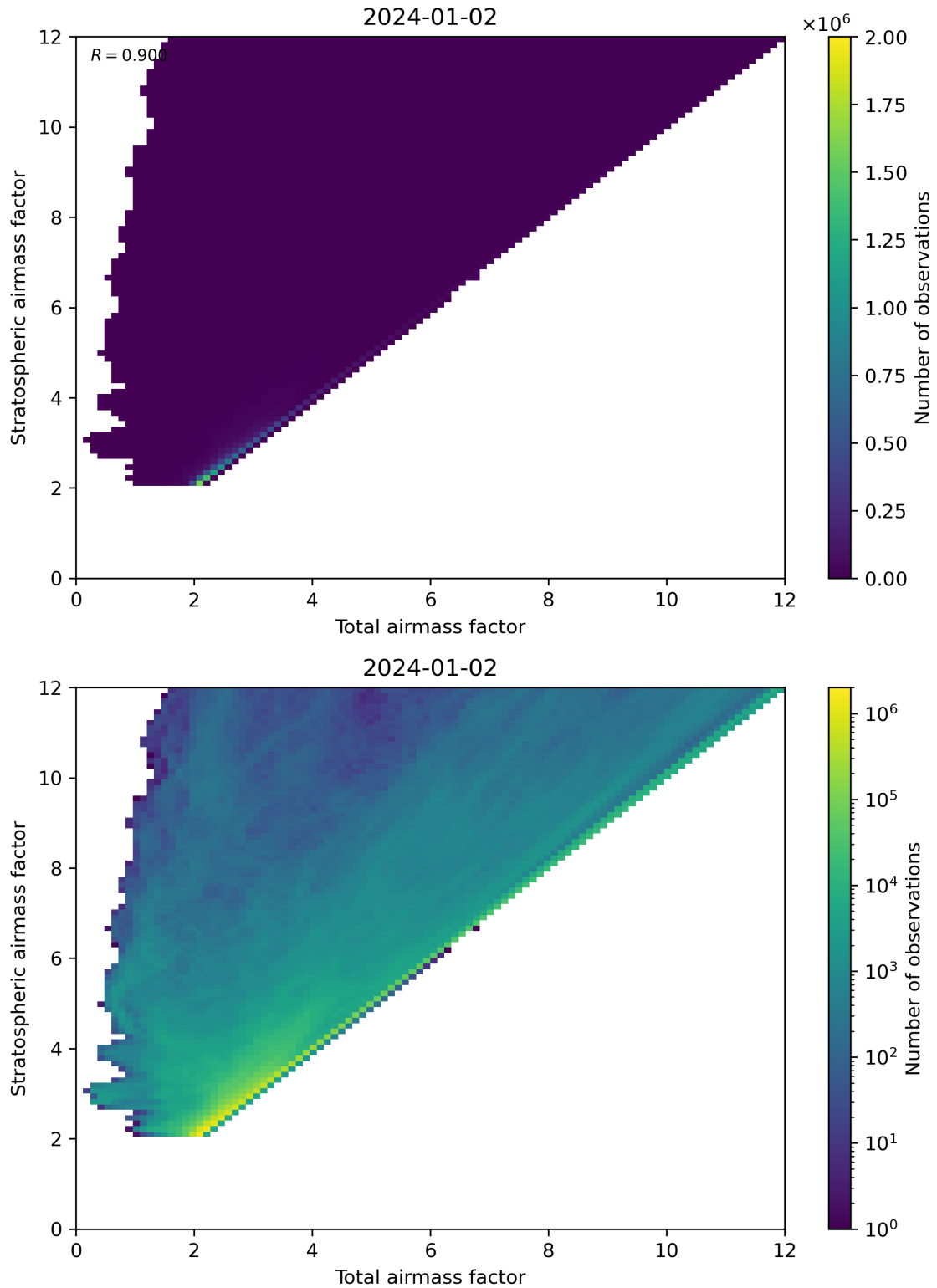
Figure 62: Scatter density plot of “Total airmass factor” against “Stratospheric airmass factor” for 2024-01-01 to 2024-01-03.
