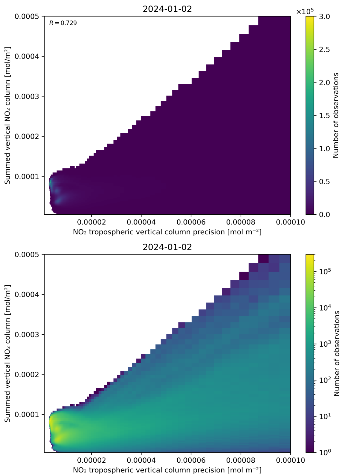
Figure 136: Scatter density plot of “NO 2 tropospheric vertical column precision” against “Summed vertical NO 2 column” for 2024-01-01 to 2024-01-03.
