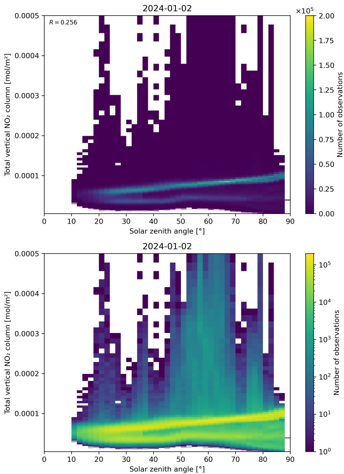
Figure 153: Scatter density plot of “Solar zenith angle” against “Total vertical NO 2 column” for 2024-01-01 to 2024-01-03.
