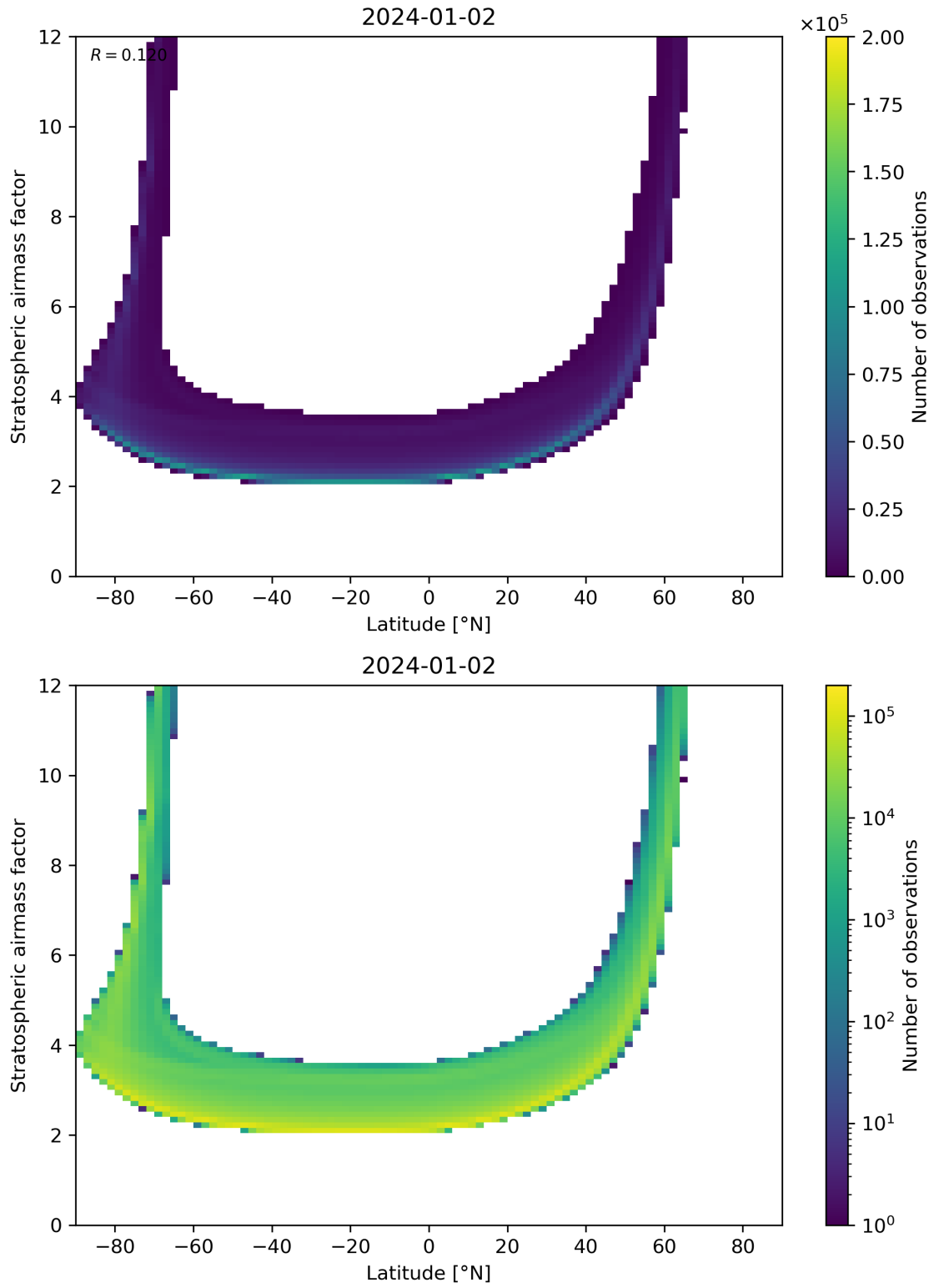
Figure 83: Scatter density plot of “Latitude” against “Stratospheric airmass factor” for 2024-01-01 to 2024-01-03.
