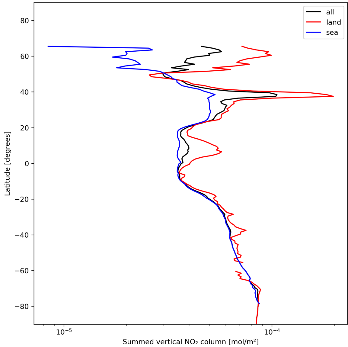
Figure 23: Zonal average of “Summed vertical NO 2 column” for 2024-01-01 to 2024-01-03.
