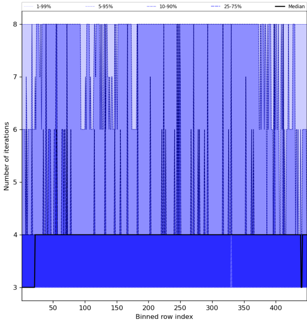
Figure 51: Along track statistics of “Number of iterations” for 2024-01-01 to 2024-01-03
