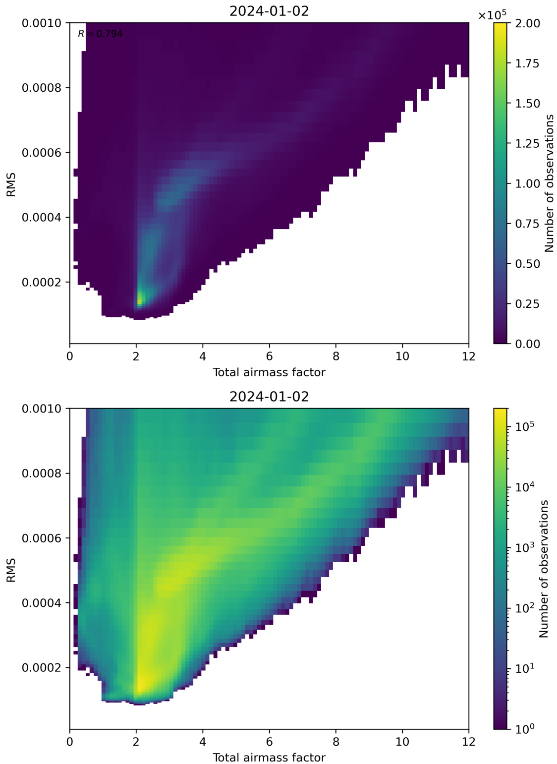
Figure 69: Scatter density plot of “Total airmass factor” against “RMS” for 2024-01-01 to 2024-01-03.
