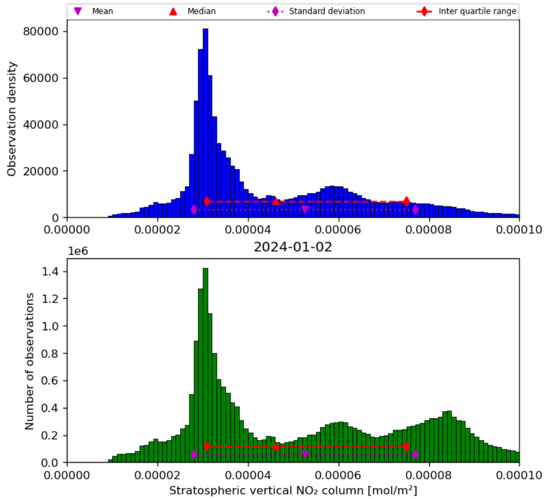
Figure 36: Histogram of “Stratospheric vertical NO 2 column” for 2024-01-01 to 2024-01-03
