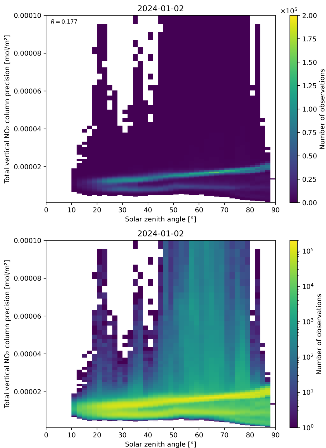
Figure 154: Scatter density plot of “Solar zenith angle” against “Total vertical NO 2 column precision” for 2024-01-01 to 2024-01-03.
