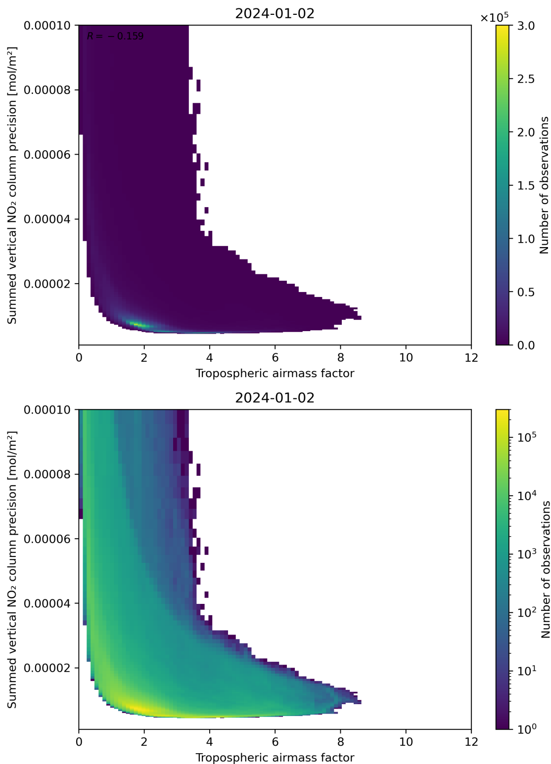
Figure 76: Scatter density plot of “Tropospheric air mass factor” against “Summed vertical NO 2 column precision” for 2024-01-01 to 2024-01-03.
