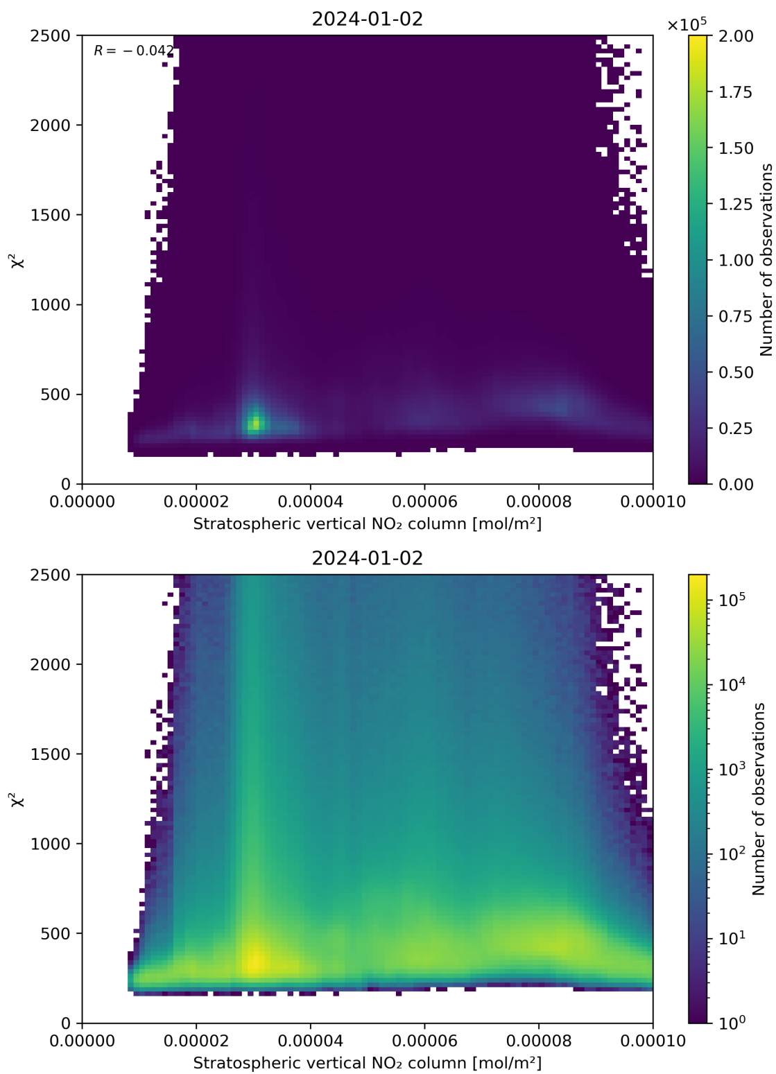
Figure 97: Scatter density plot of “Stratospheric vertical NO 2 column” against “ \chi^2 ” for 2024-01-01 to 2024-01-03.
