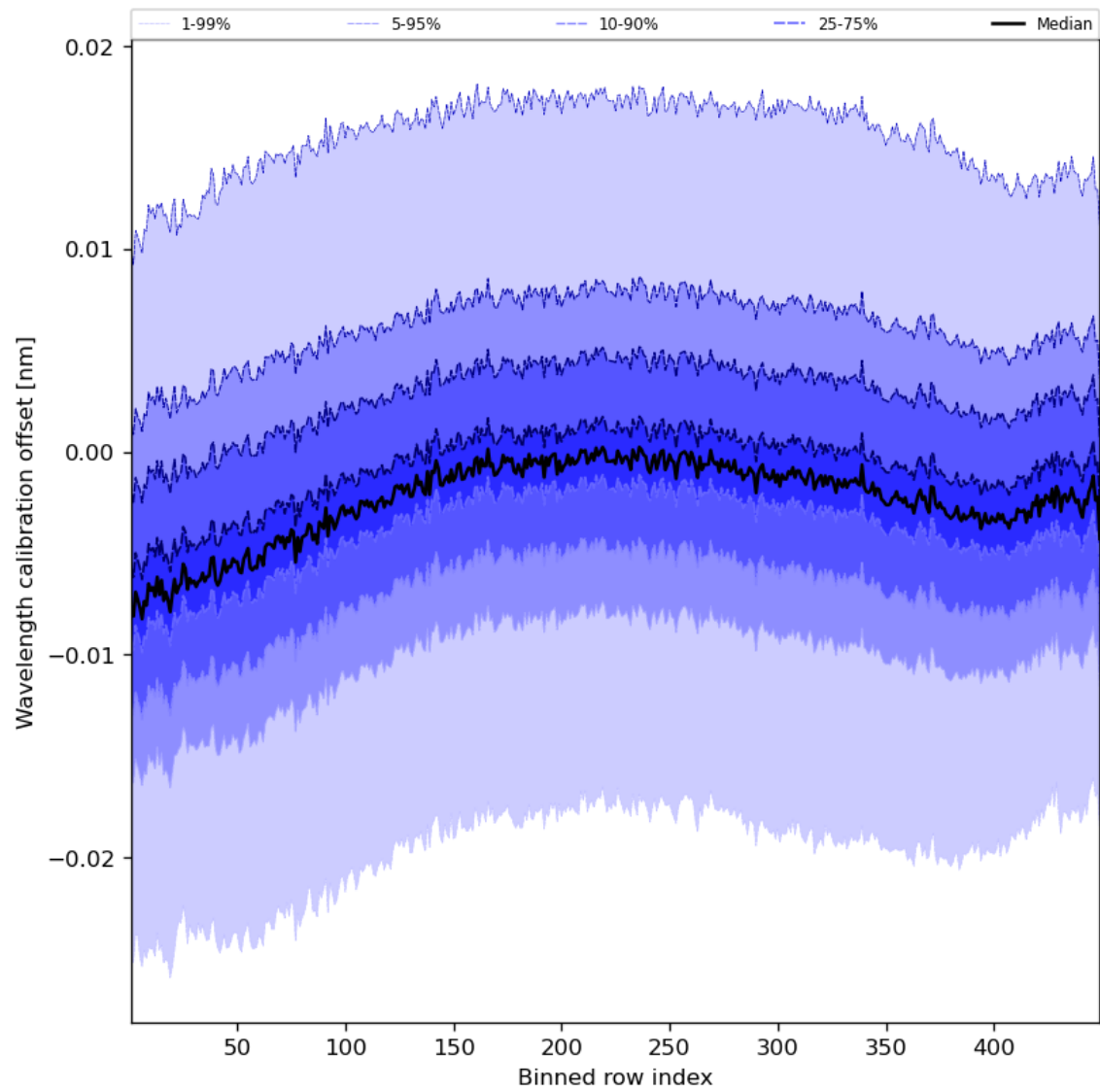
Figure 52: Along track statistics of “Wavelength calibration offset” for 2024-01-01 to 2024-01-03
