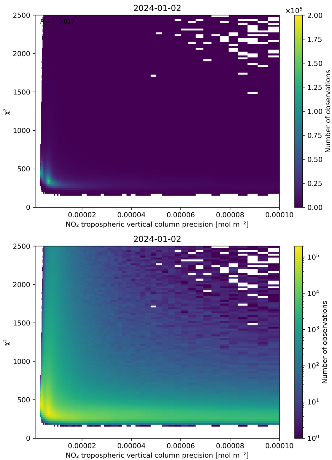
Figure 134: Scatter density plot of “NO 2 tropospheric vertical column precision” against “ \chi^2 ” for 2024-01-01 to 2024-01-03.
