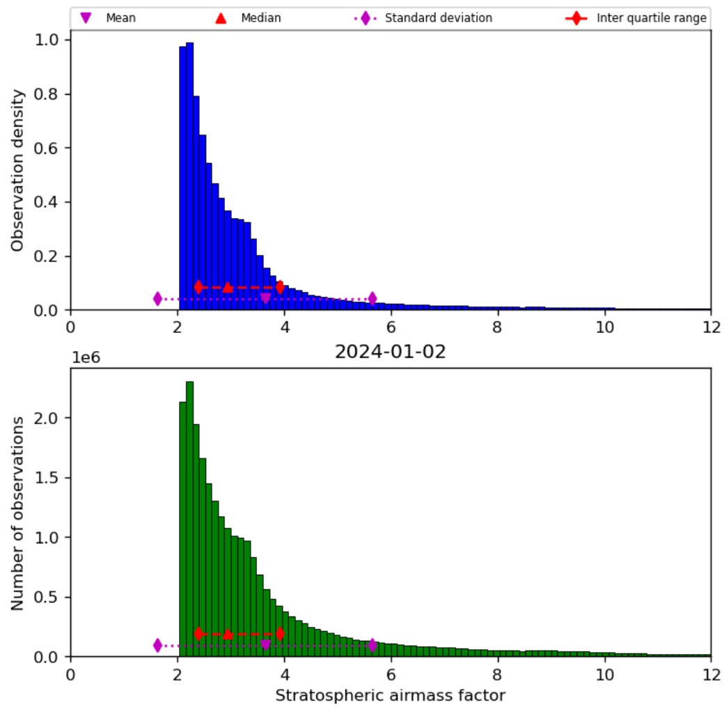
Figure 44: Histogram of “Stratospheric airmass factor” for 2024-01-01 to 2024-01-03
