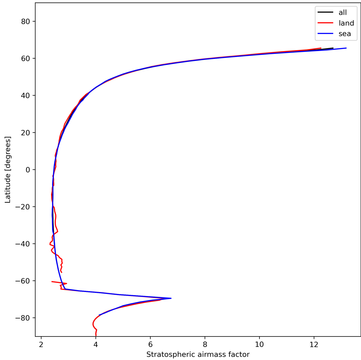
Figure 27: Zonal average of “Stratospheric airmass factor” for 2024-01-01 to 2024-01-03.
