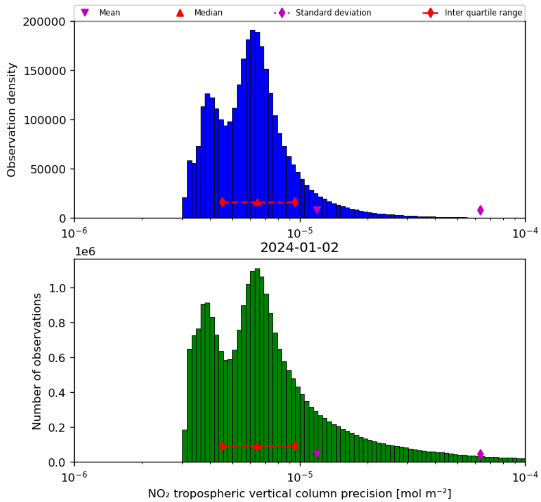
Figure 30: Histogram of “NO 2 tropospheric vertical column precision” for 2024-01-01 to 2024-01-03
