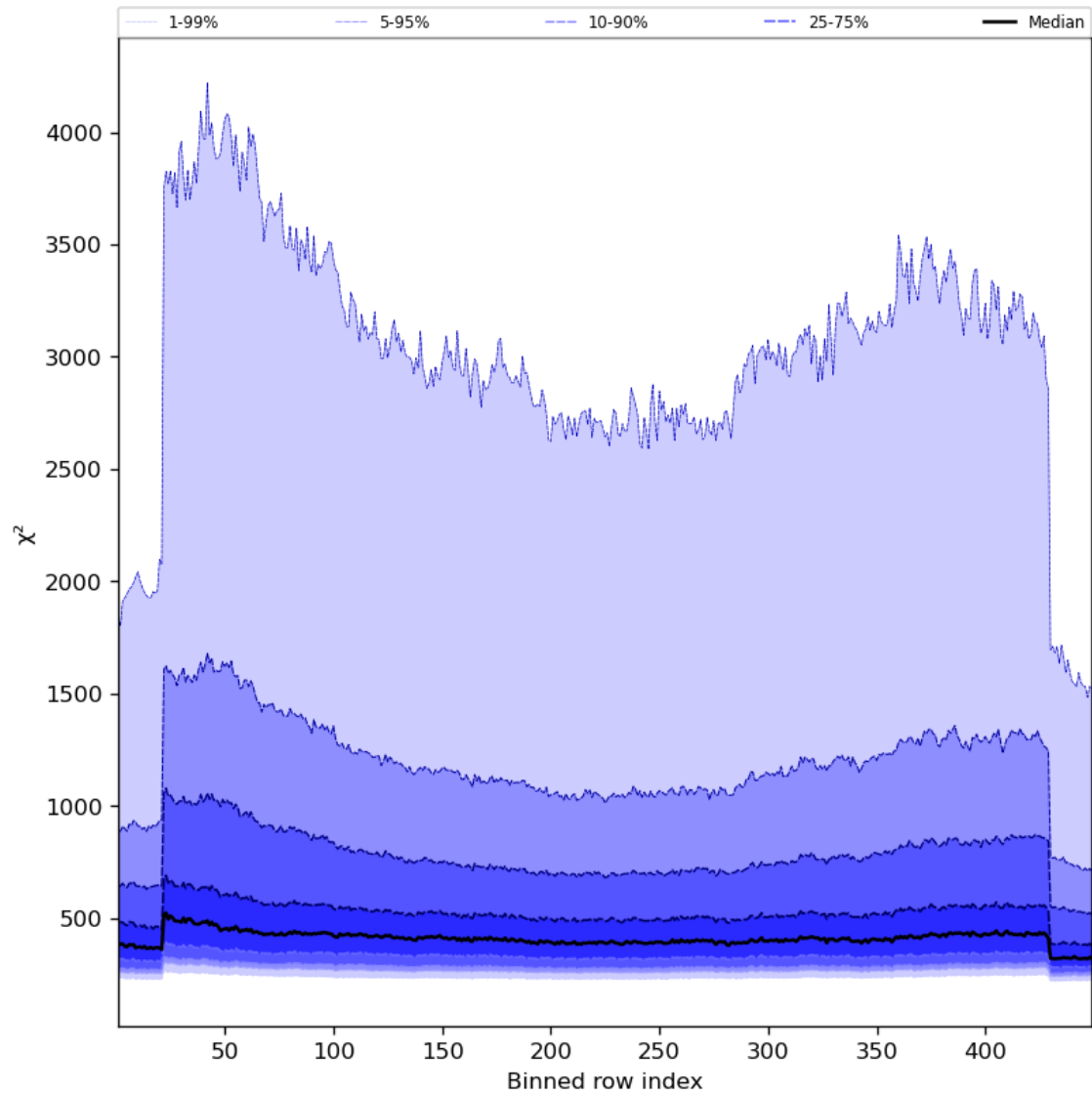
Figure 59: Along track statistics of “ \chi^2 ” for 2024-01-01 to 2024-01-03
