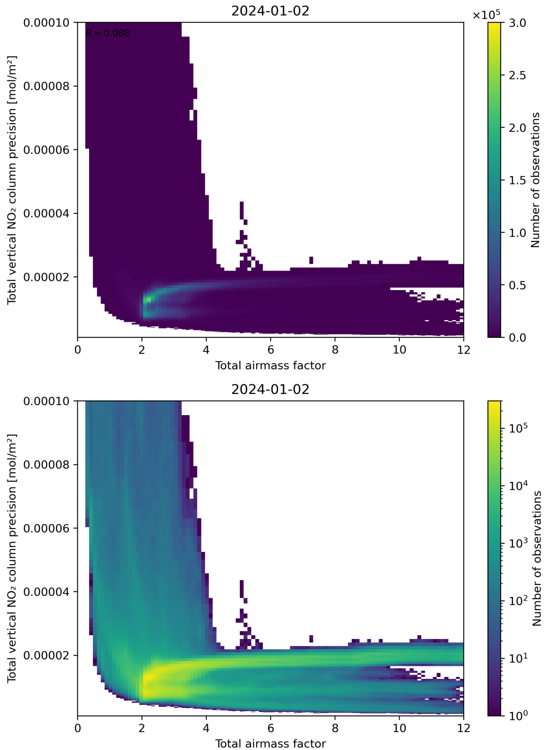
Figure 68: Scatter density plot of “Total airmass factor” against “Total vertical NO 2 column precision” for 2024-01-01 to 2024-01-03.
