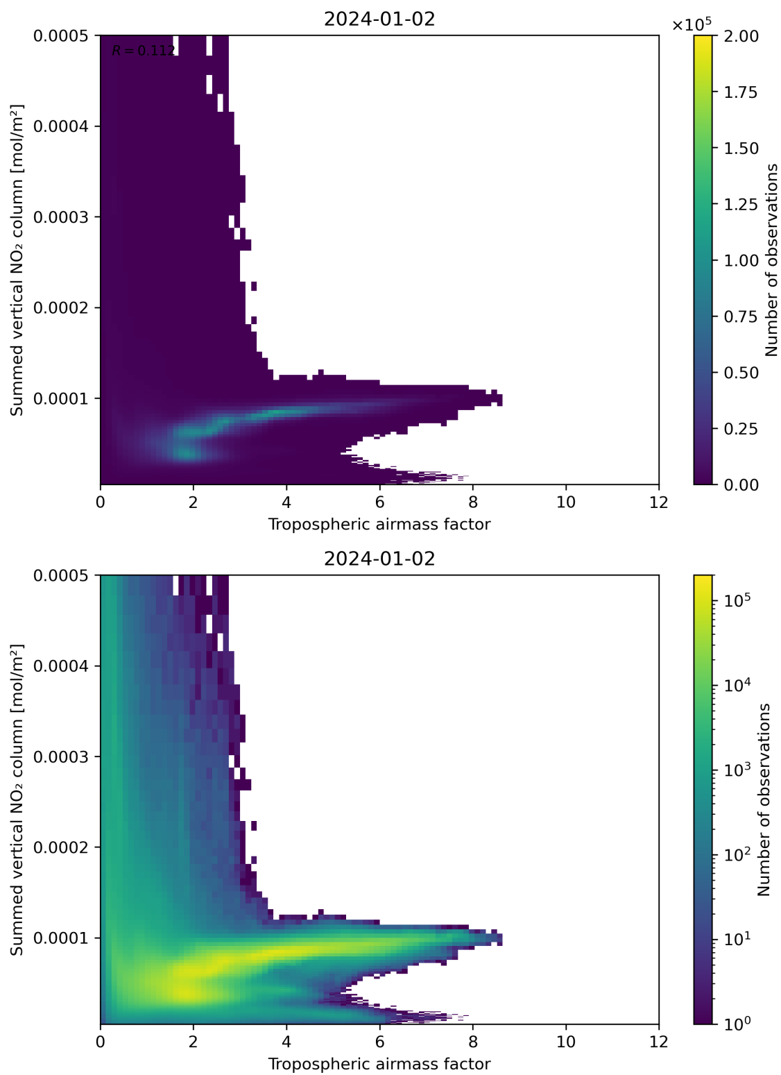
Figure 75: Scatter density plot of “Tropospheric airmass factor” against “Summed vertical NO 2 column” for 2024-01-01 to 2024-01-03.
