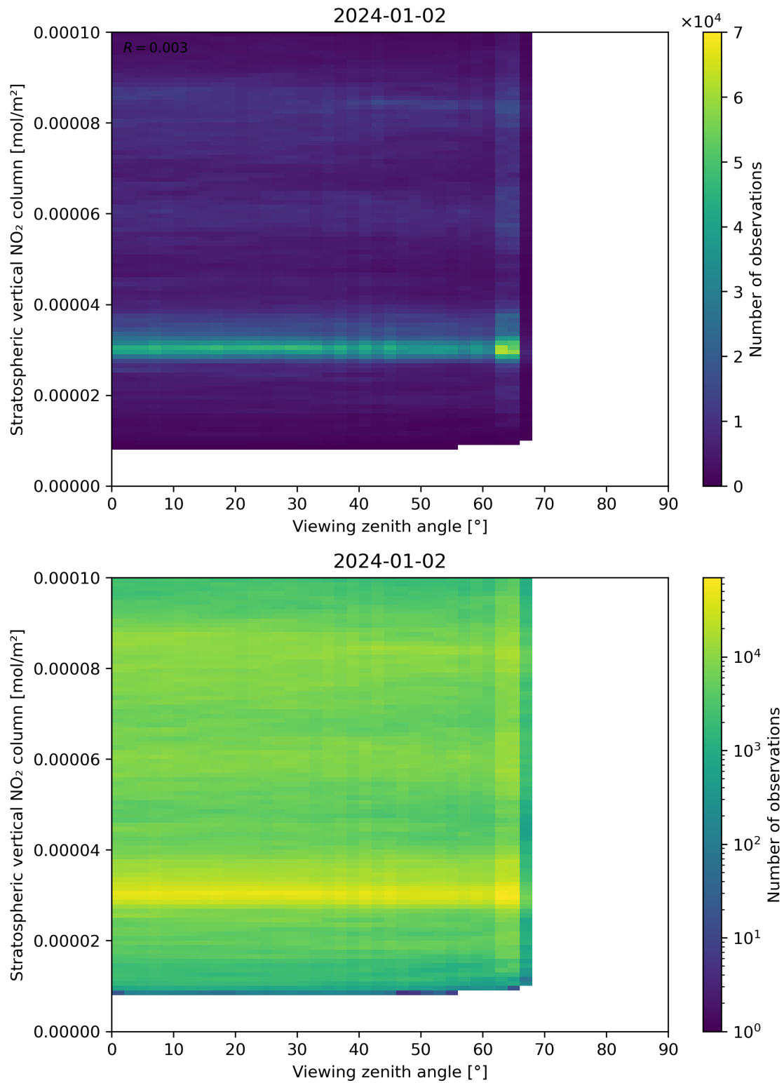
Figure 164: Scatter density plot of “Viewing zenith angle” against “Stratospheric vertical NO 2 column” for 2024-01-01 to 2024-01-03.
