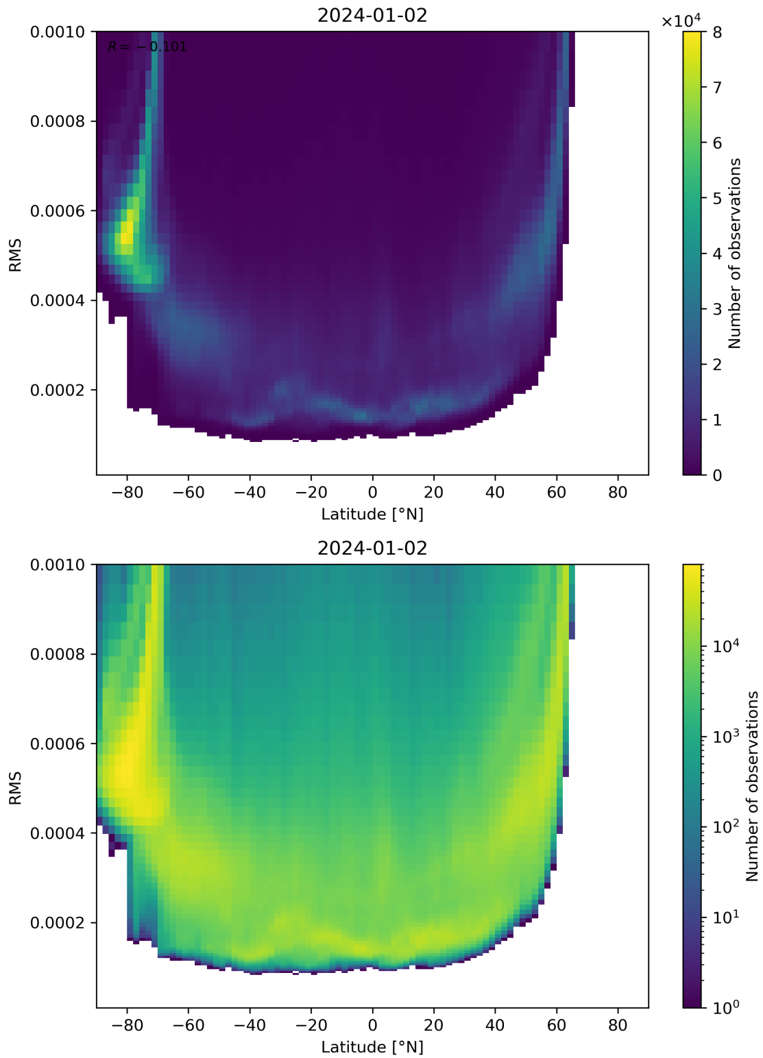
Figure 94: Scatter density plot of “Latitude” against “RMS” for 2024-01-01 to 2024-01-03.
