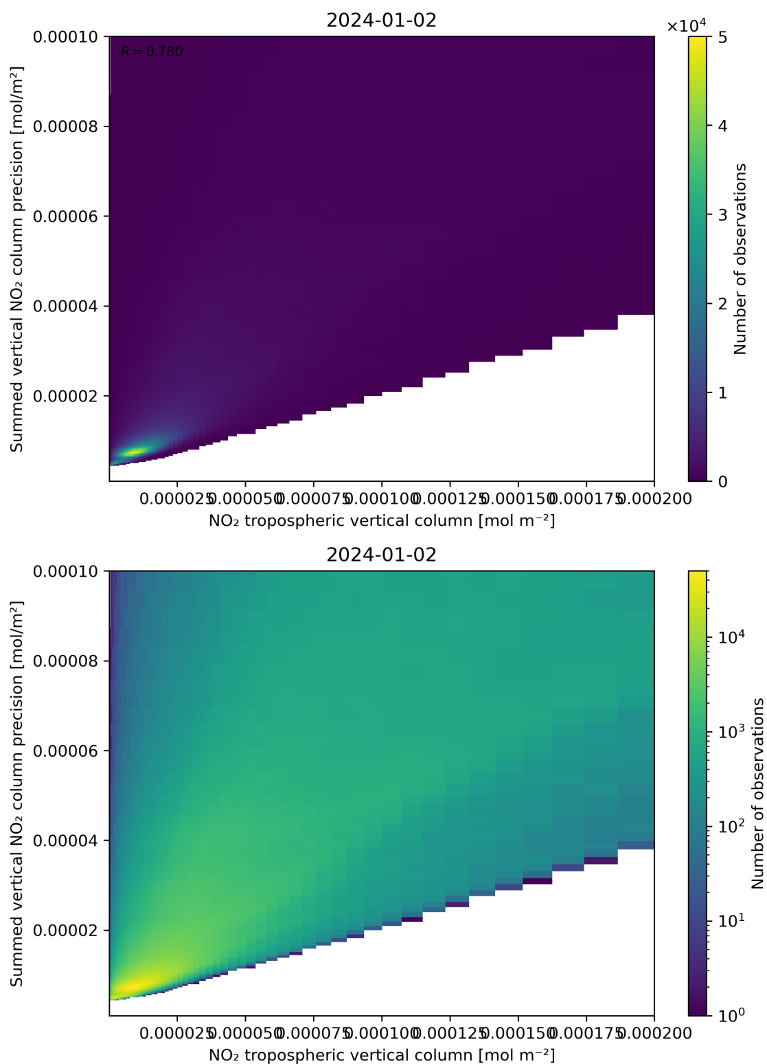
Figure 127: Scatter density plot of “NO 2 tropospheric vertical column” against “Summed vertical NO 2 column precision” for 2024-01-01 to 2024-01-03.
