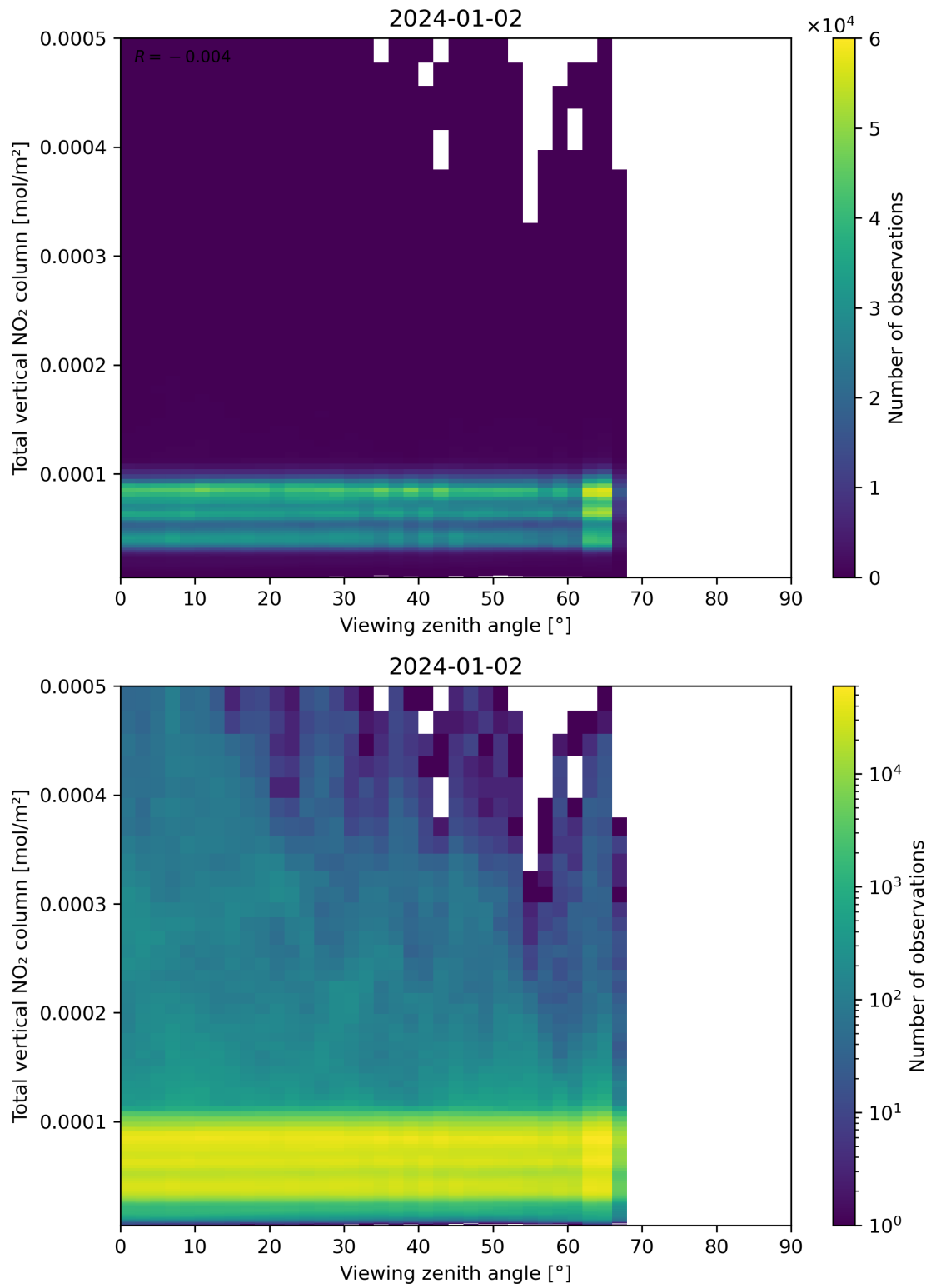
Figure 167: Scatter density plot of “Viewing zenith angle” against “Total vertical NO 2 column” for 2024-01-01 to 2024-01-03.
