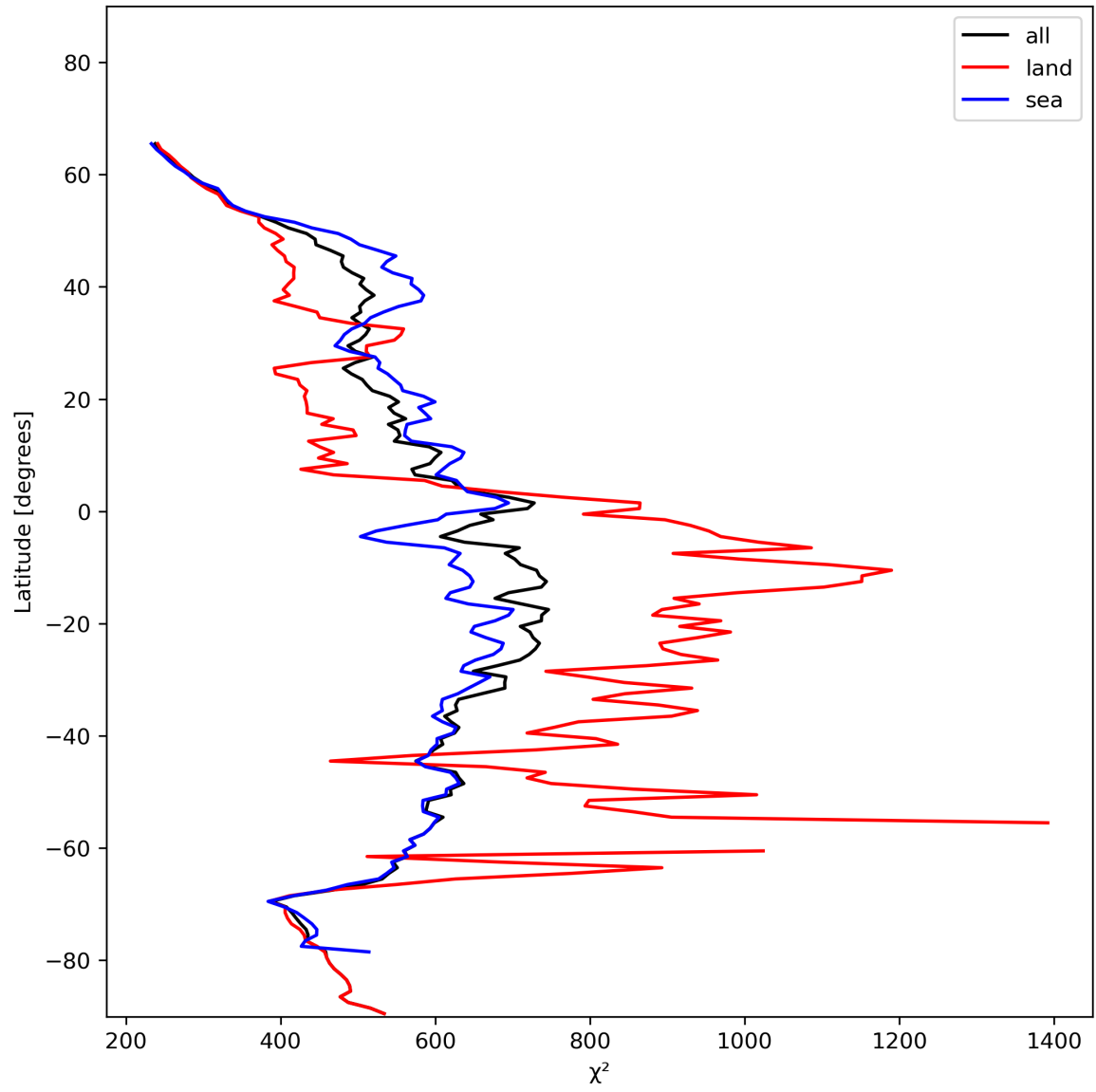
Figure 25: Zonal average of “ \chi^2 ” for 2024-01-01 to 2024-01-03.
