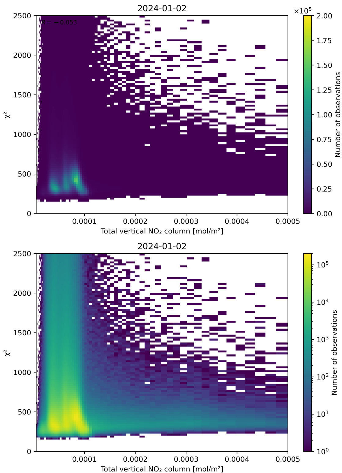
Figure 111: Scatter density plot of “Total vertical NO 2 column” against “ \chi^2 ” for 2024-01-01 to 2024-01-03.
