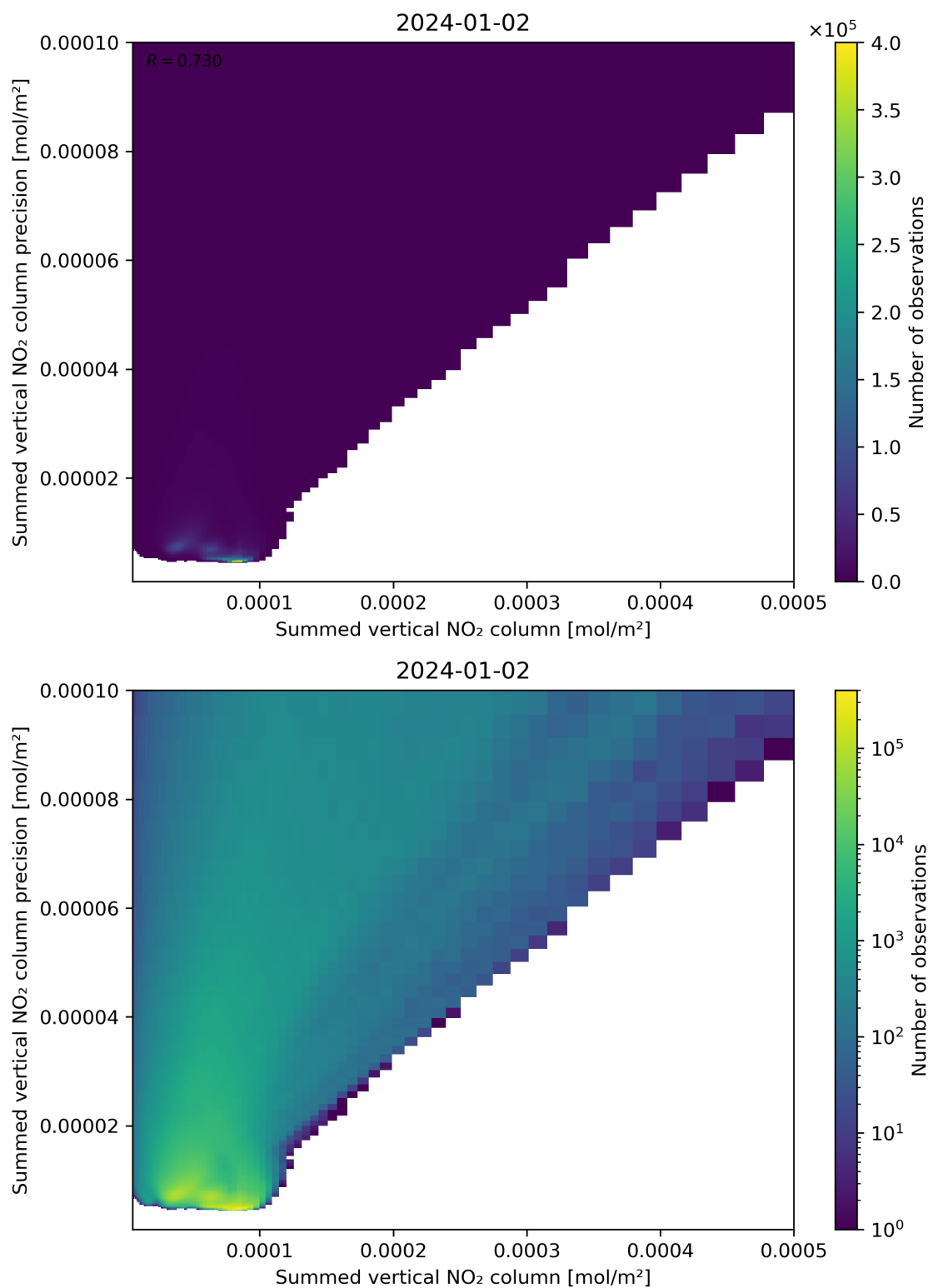
Figure 105: Scatter density plot of “Summed vertical NO 2 column” against “Summed vertical NO 2 column precision” for 2024-01-01 to 2024-01-03.
