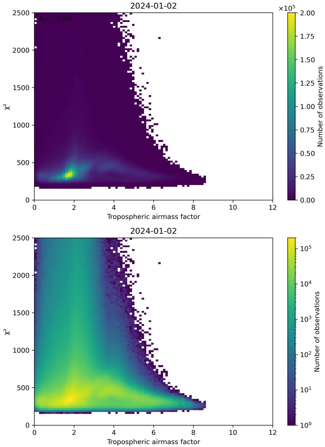
Figure 73: Scatter density plot of “Tropospheric airmass factor” against “ \chi^2 ” for 2024-01-01 to 2024-01-03.
