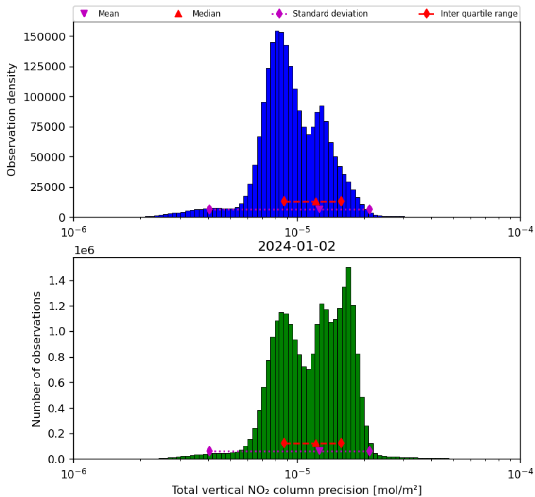
Figure 39: Histogram of “Total vertical NO 2 column precision” for 2024-01-01 to 2024-01-03
