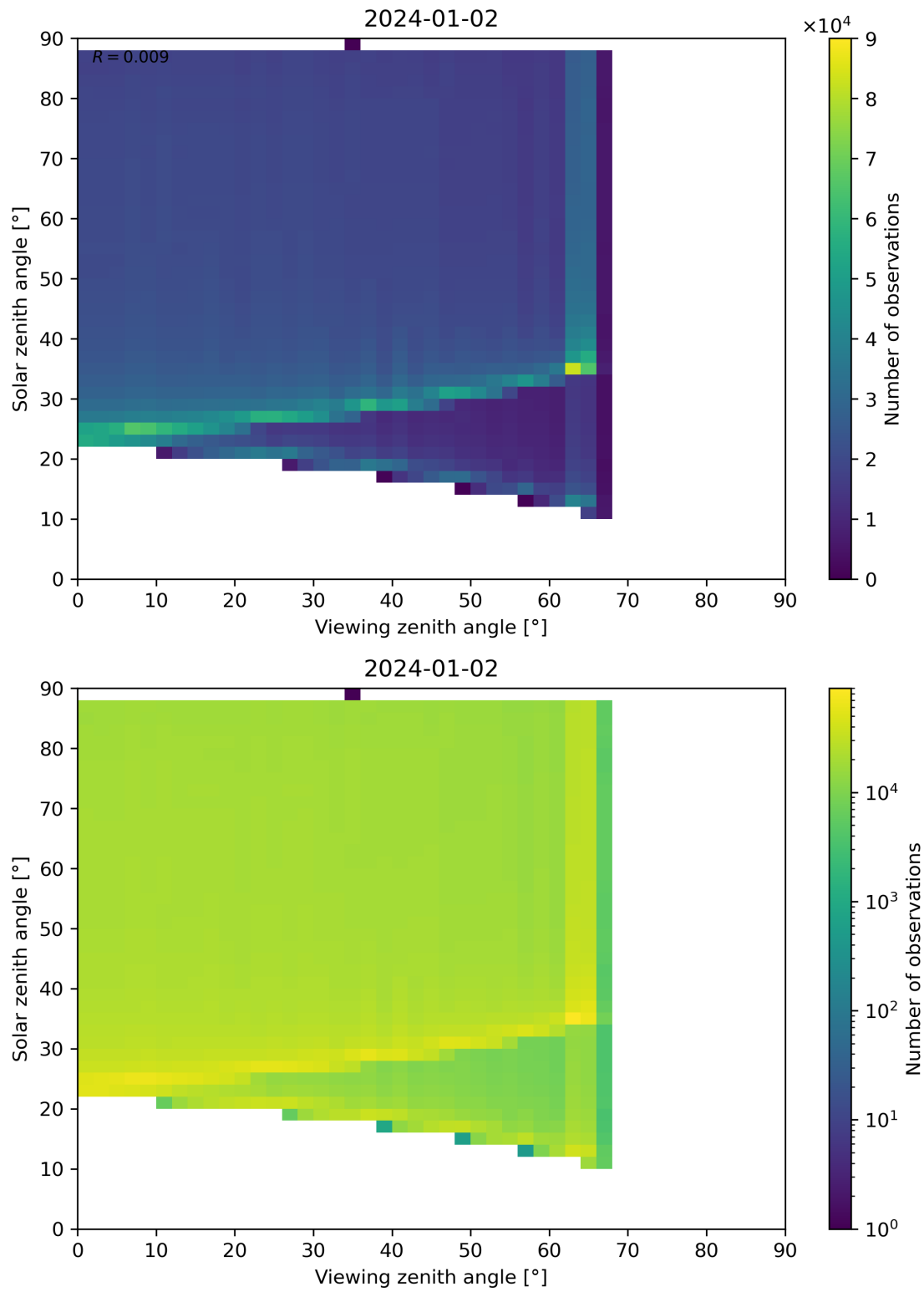
Figure 172: Scatter density plot of “Viewing zenith angle” against “Solar zenith angle” for 2024-01-01 to 2024-01-03.
