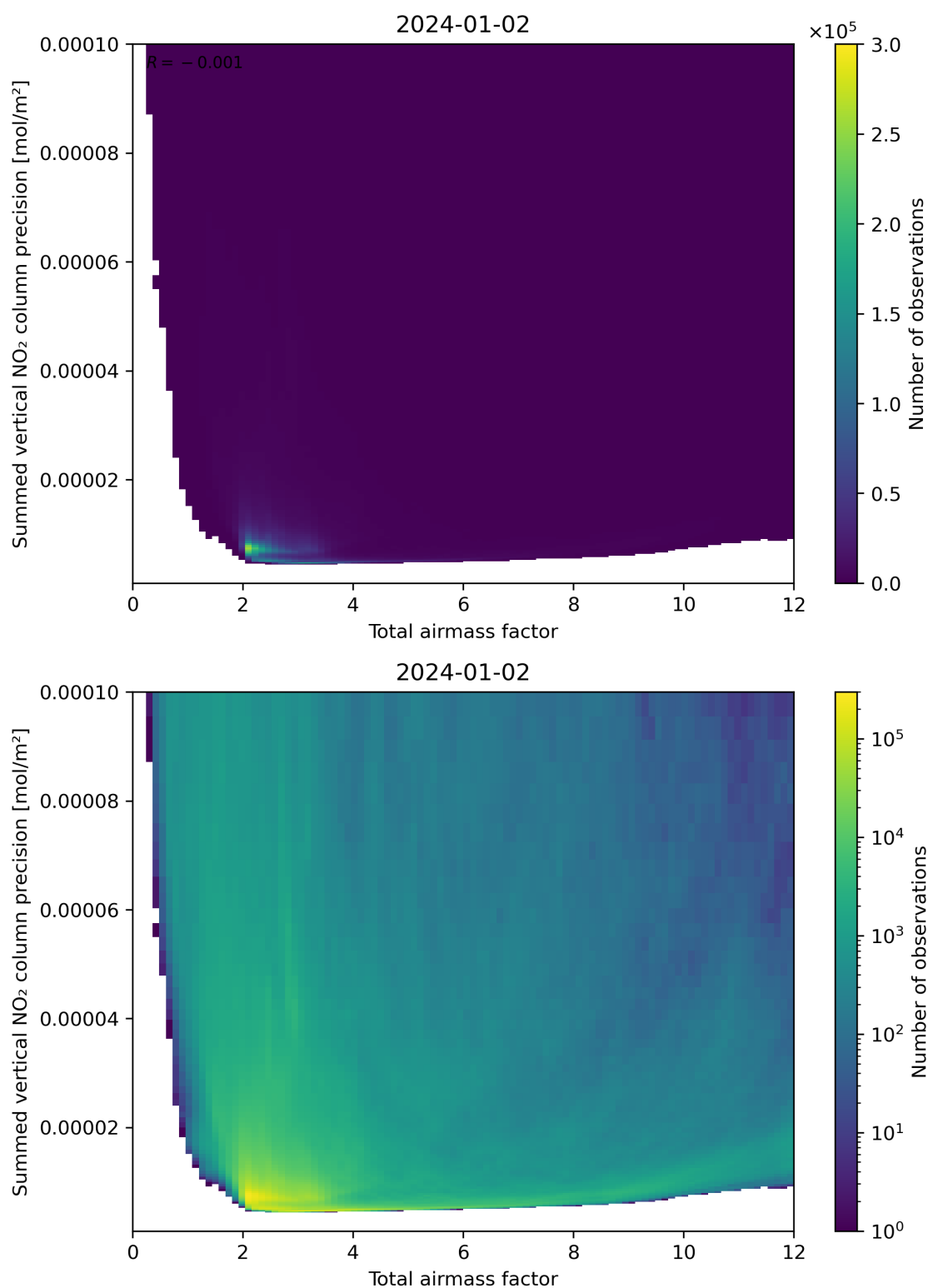
Figure 66: Scatter density plot of “Total airmass factor” against “Summed vertical NO 2 column precision” for 2024-01-01 to 2024-01-03.
