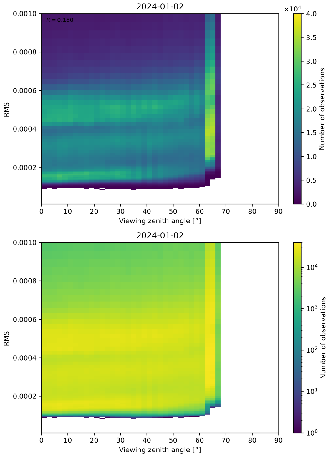
Figure 171: Scatter density plot of “Viewing zenith angle” against “RMS” for 2024-01-01 to 2024-01-03.
