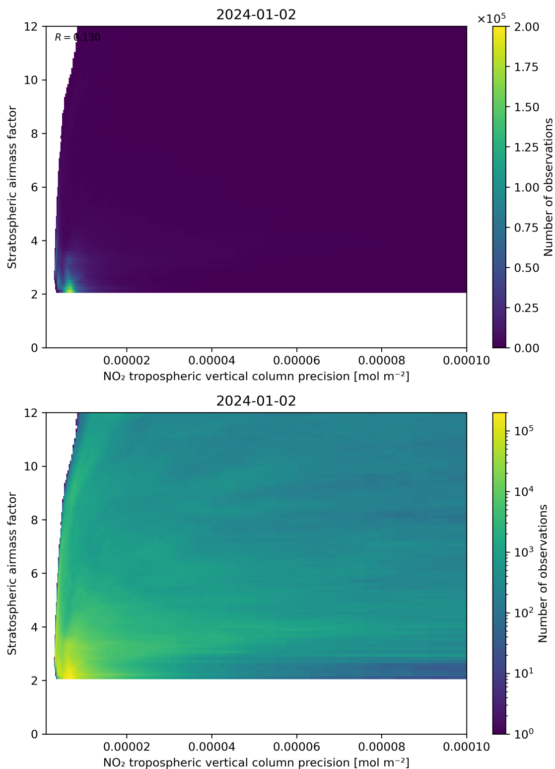
Figure 131: Scatter density plot of “NO 2 tropospheric vertical column precision” against “Stratospheric airmass factor” for 2024-01-01 to 2024-01-03.
