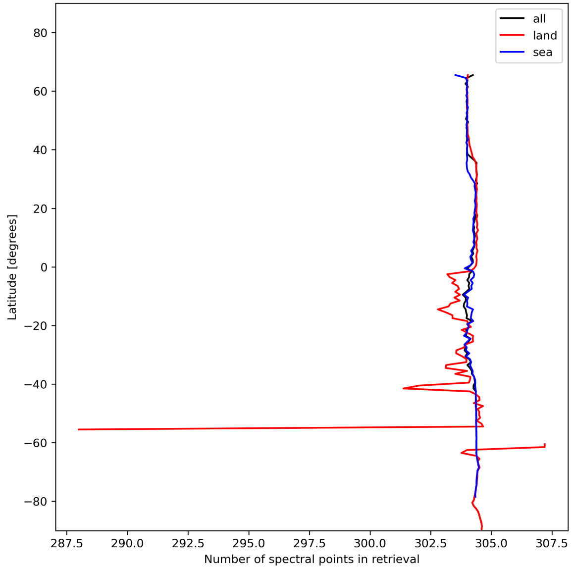
Figure 16: Zonal average of “Number of spectral points in retrieval” for 2024-01-01 to 2024-01-03.
