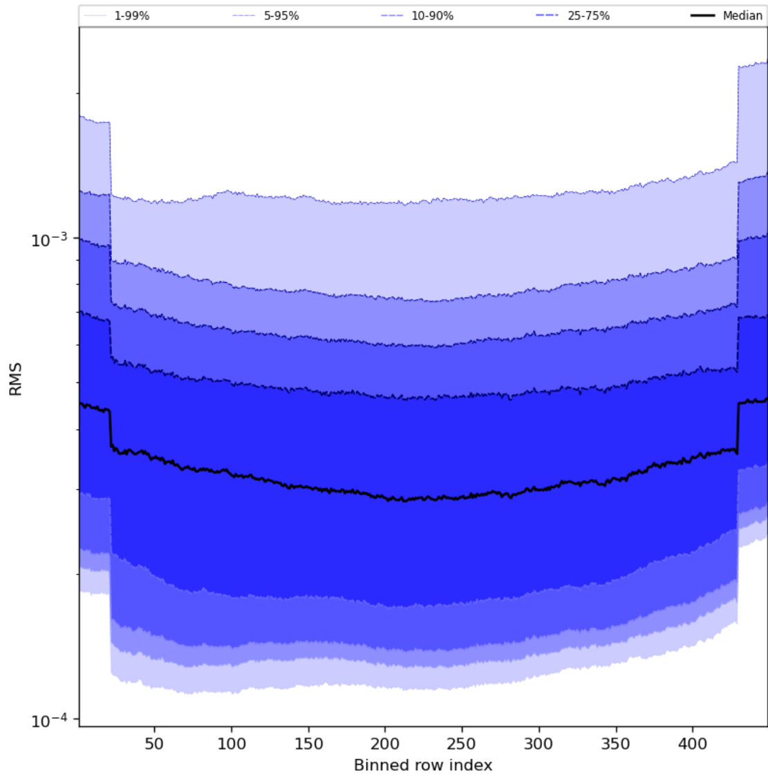
Figure 60: Along track statistics of “RMS” for 2024-01-01 to 2024-01-03
