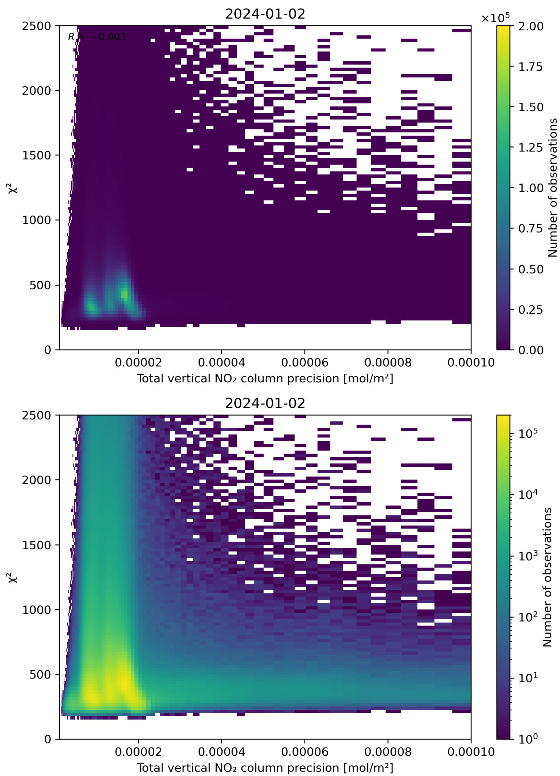
Figure 116: Scatter density plot of “Total vertical NO 2 column precision” against “ \chi^2 ” for 2024-01-01 to 2024-01-03.
