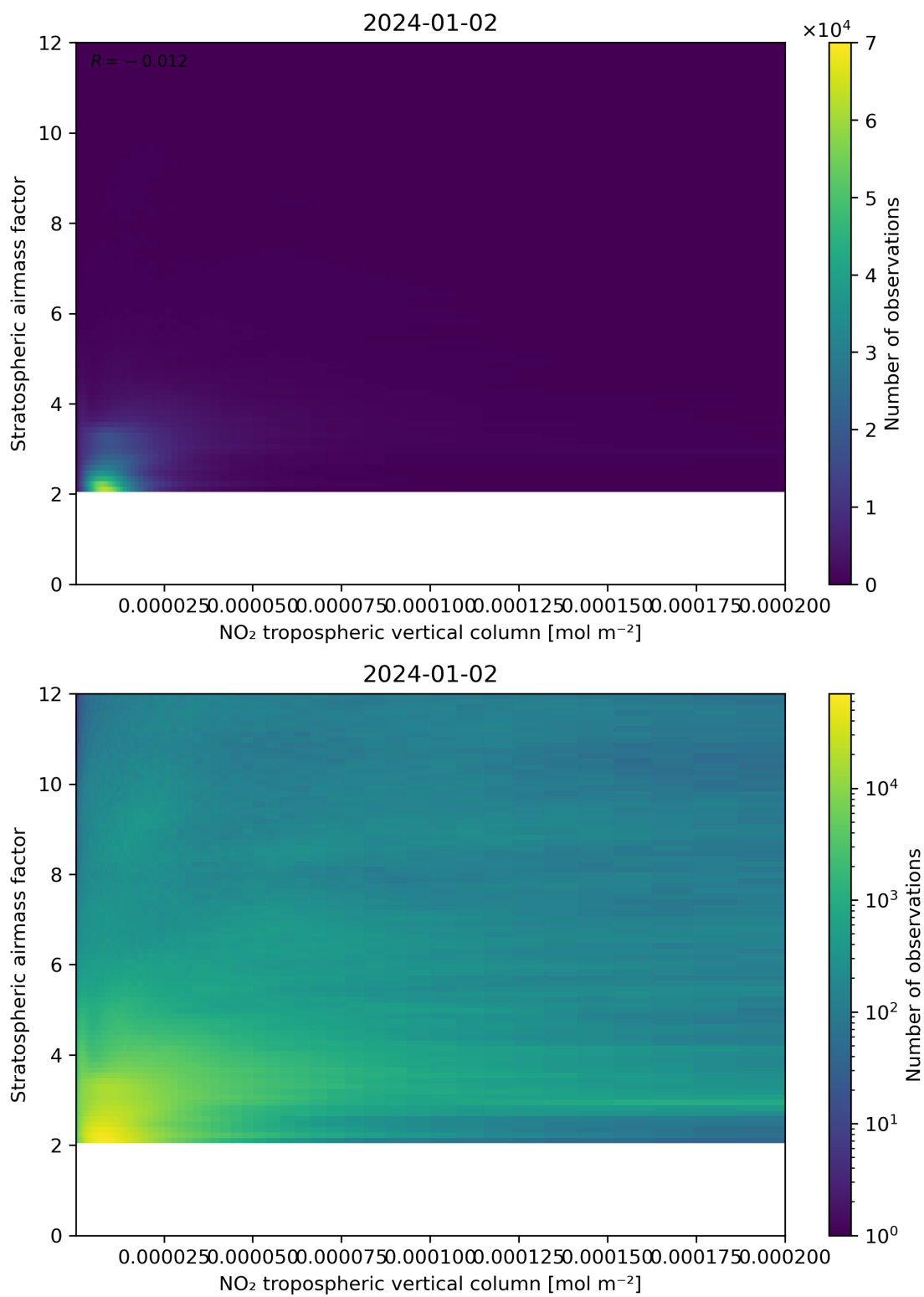
Figure 121: Scatter density plot of “NO 2 tropospheric vertical column” against “Stratospheric airmass factor” for 2024-01-01 to 2024-01-03.
