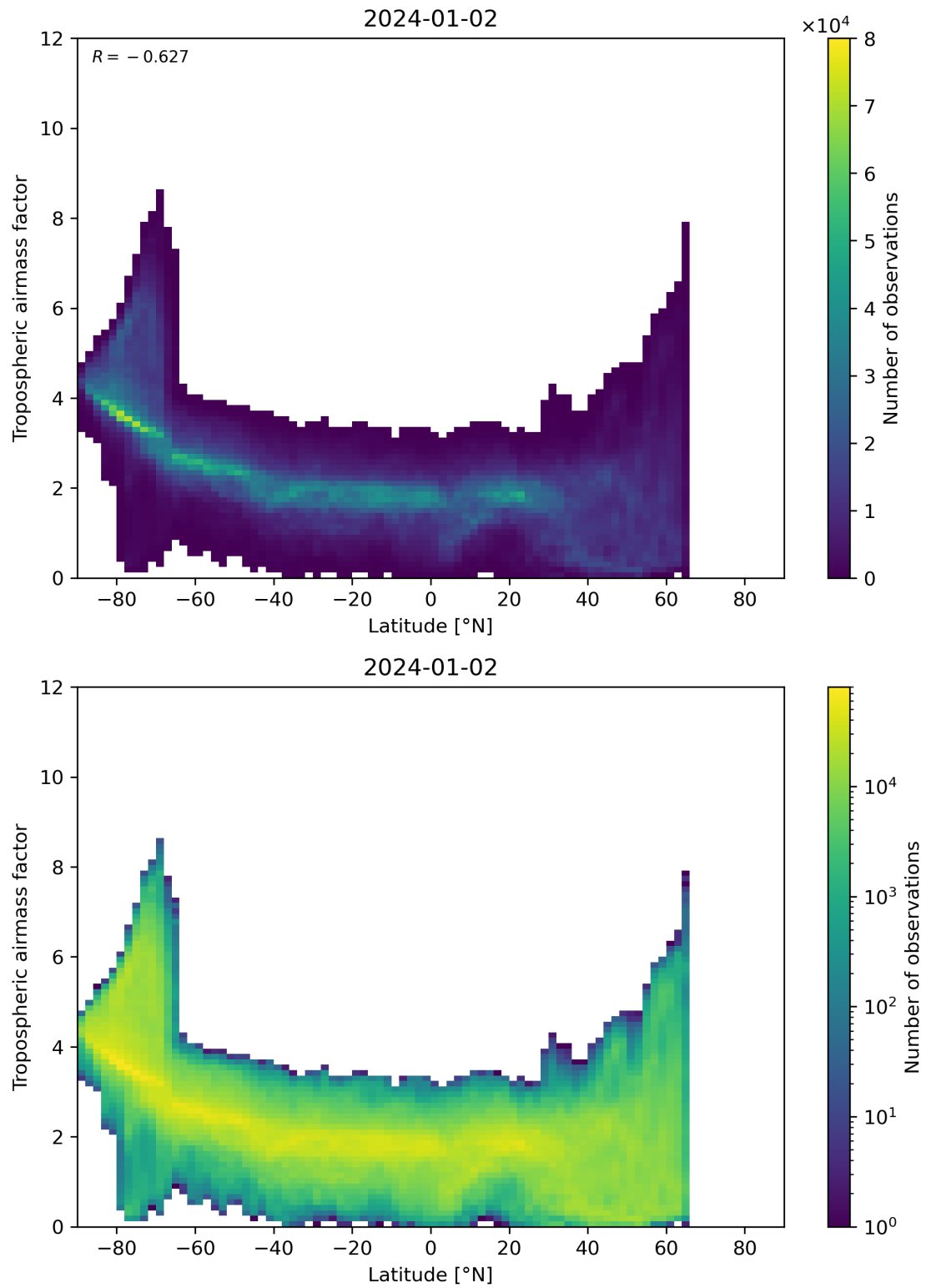
Figure 85: Scatter density plot of “Latitude” against “Tropospheric airmass factor” for 2024-01-01 to 2024-01-03.
