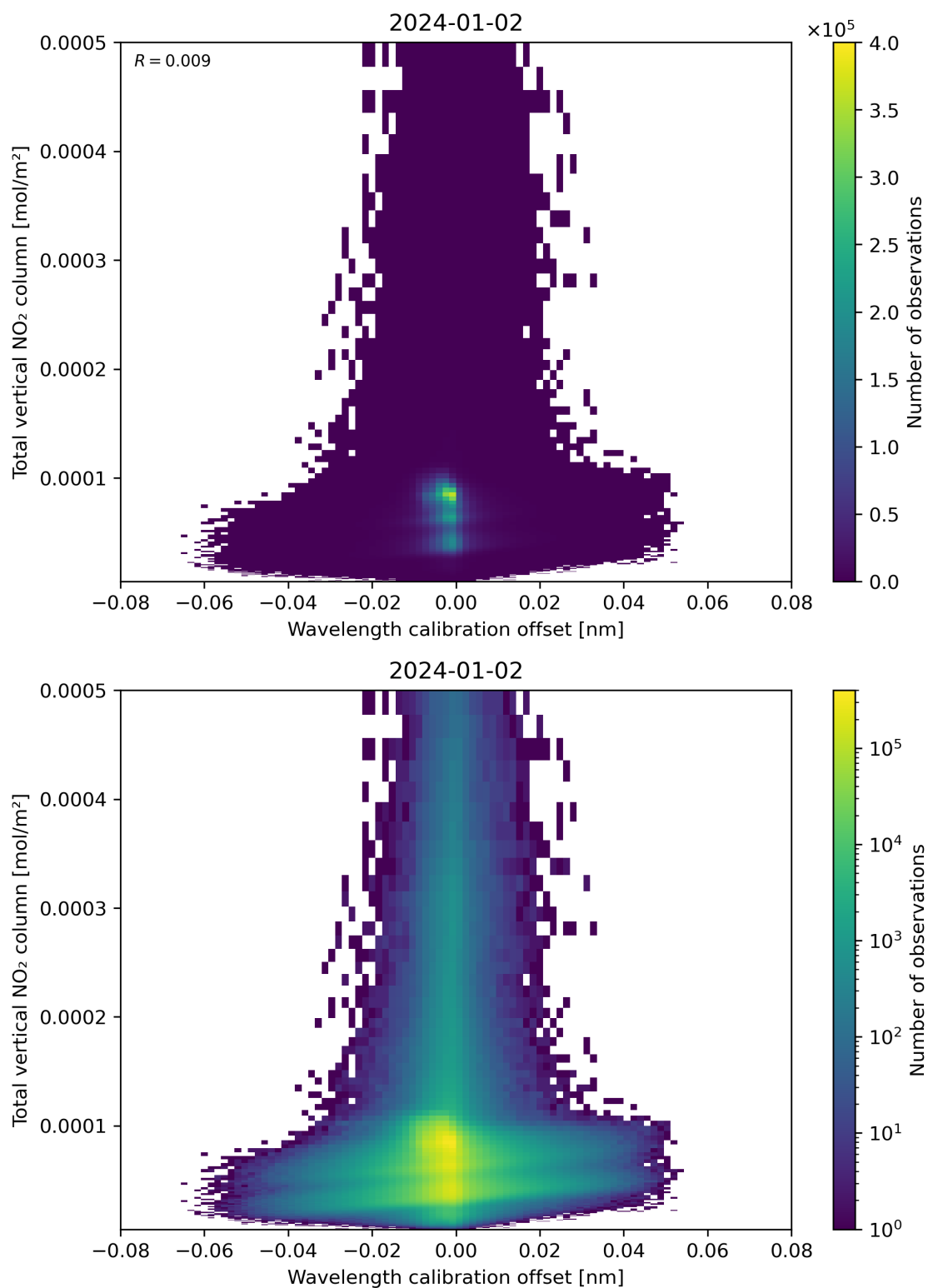
Figure 179: Scatter density plot of “Wavelength calibration offset” against “Total vertical NO 2 column” for 2024-01-01 to 2024-01-03.
