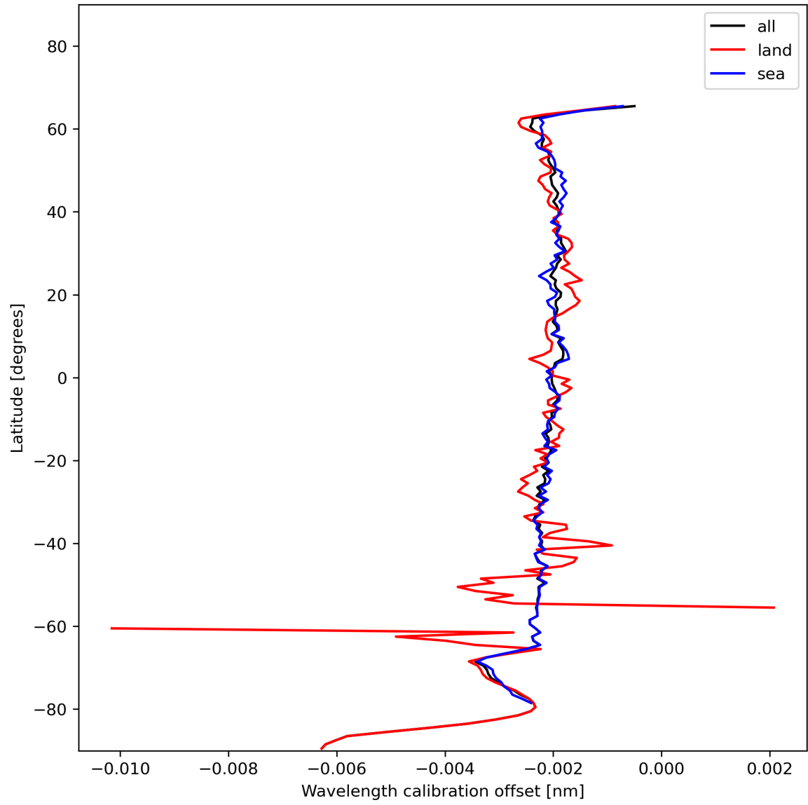
Figure 18: Zonal average of “Wavelength calibration offset” for 2024-01-01 to 2024-01-03.
