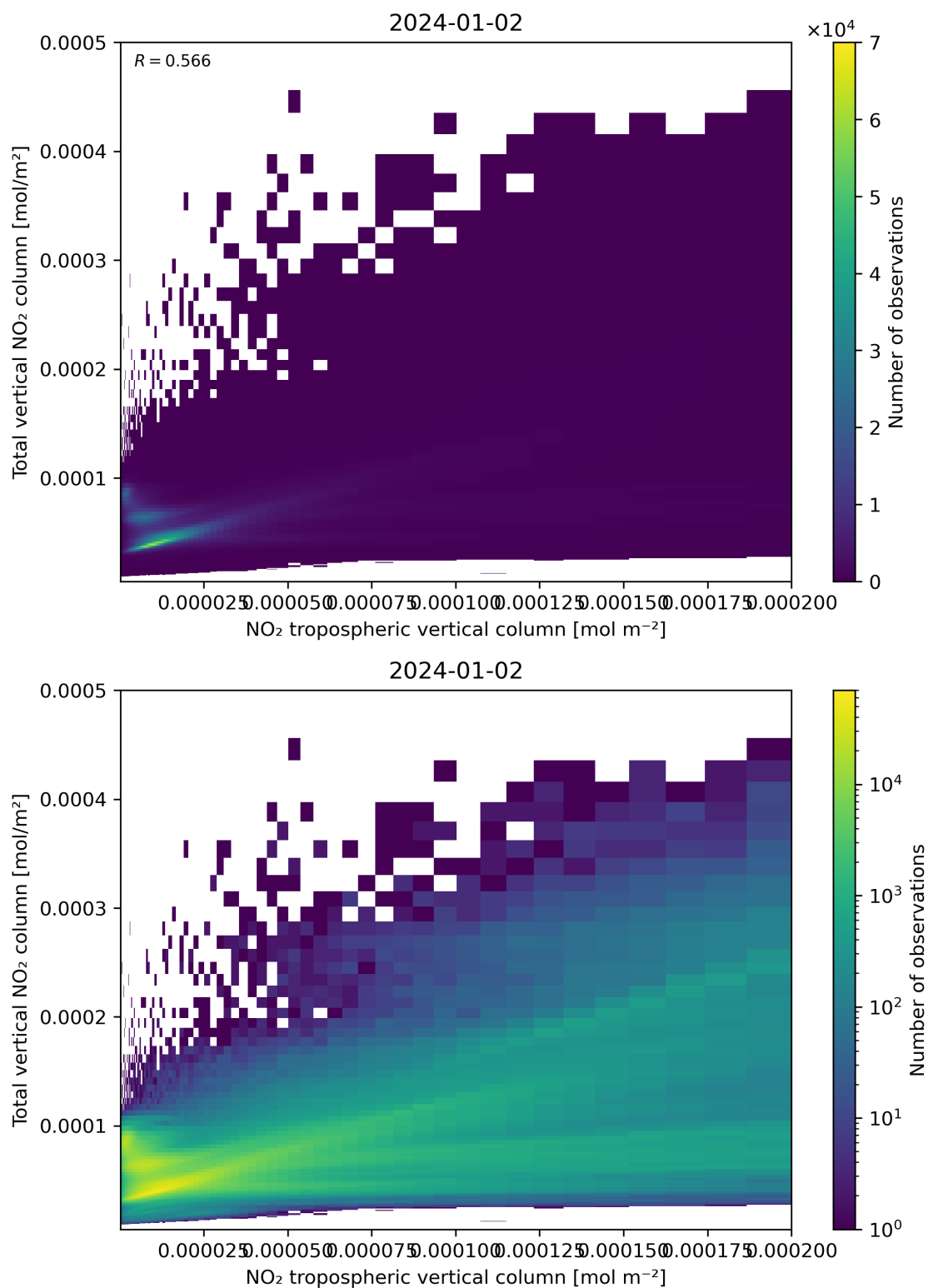
Figure 128: Scatter density plot of “NO 2 tropospheric vertical column” against “Total vertical NO 2 column” for 2024-01-01 to 2024-01-03.
