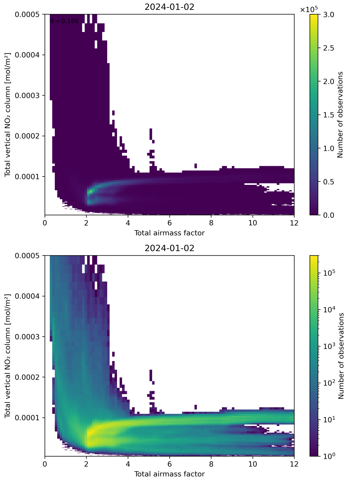
Figure 67: Scatter density plot of “Total airmass factor” against “Total vertical NO 2 column” for 2024-01-01 to 2024-01-03.
