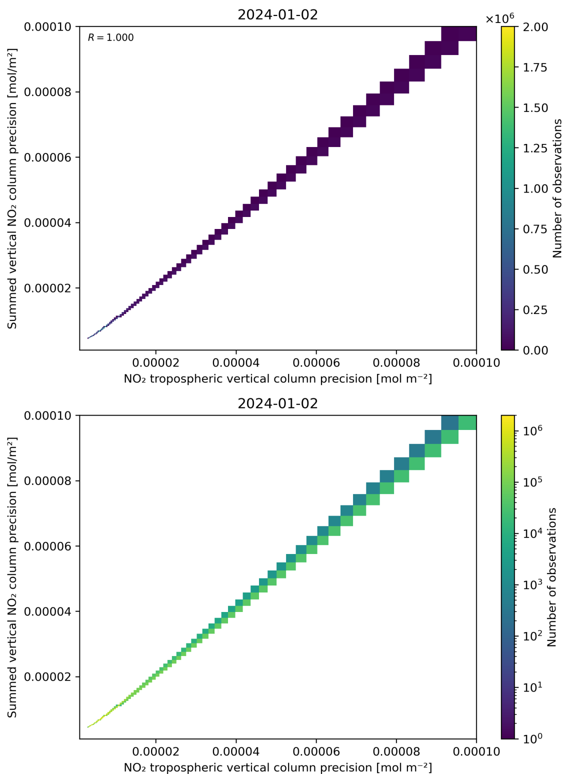
Figure 137: Scatter density plot of “NO 2 tropospheric vertical column precision” against “Summed vertical NO 2 column precision” for 2024-01-01 to 2024-01-03.
