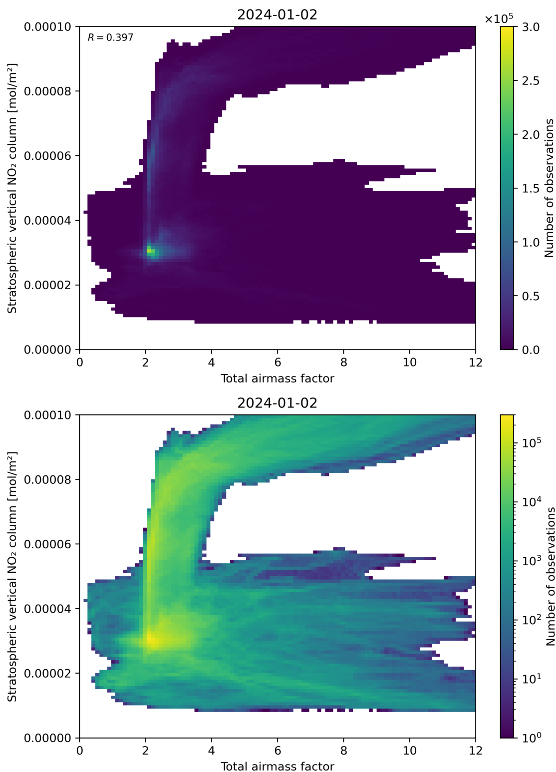
Figure 64: Scatter density plot of “Total airmass factor” against “Stratospheric vertical NO 2 column” for 2024-01-01 to 2024-01-03.
