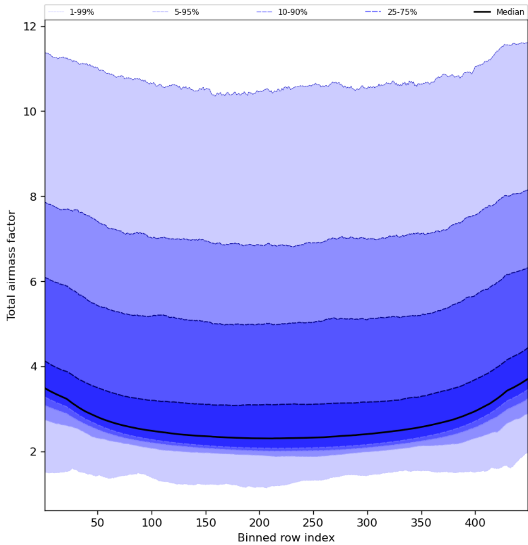
Figure 49: Along track statistics of “Total airmass factor” for 2024-01-01 to 2024-01-03
