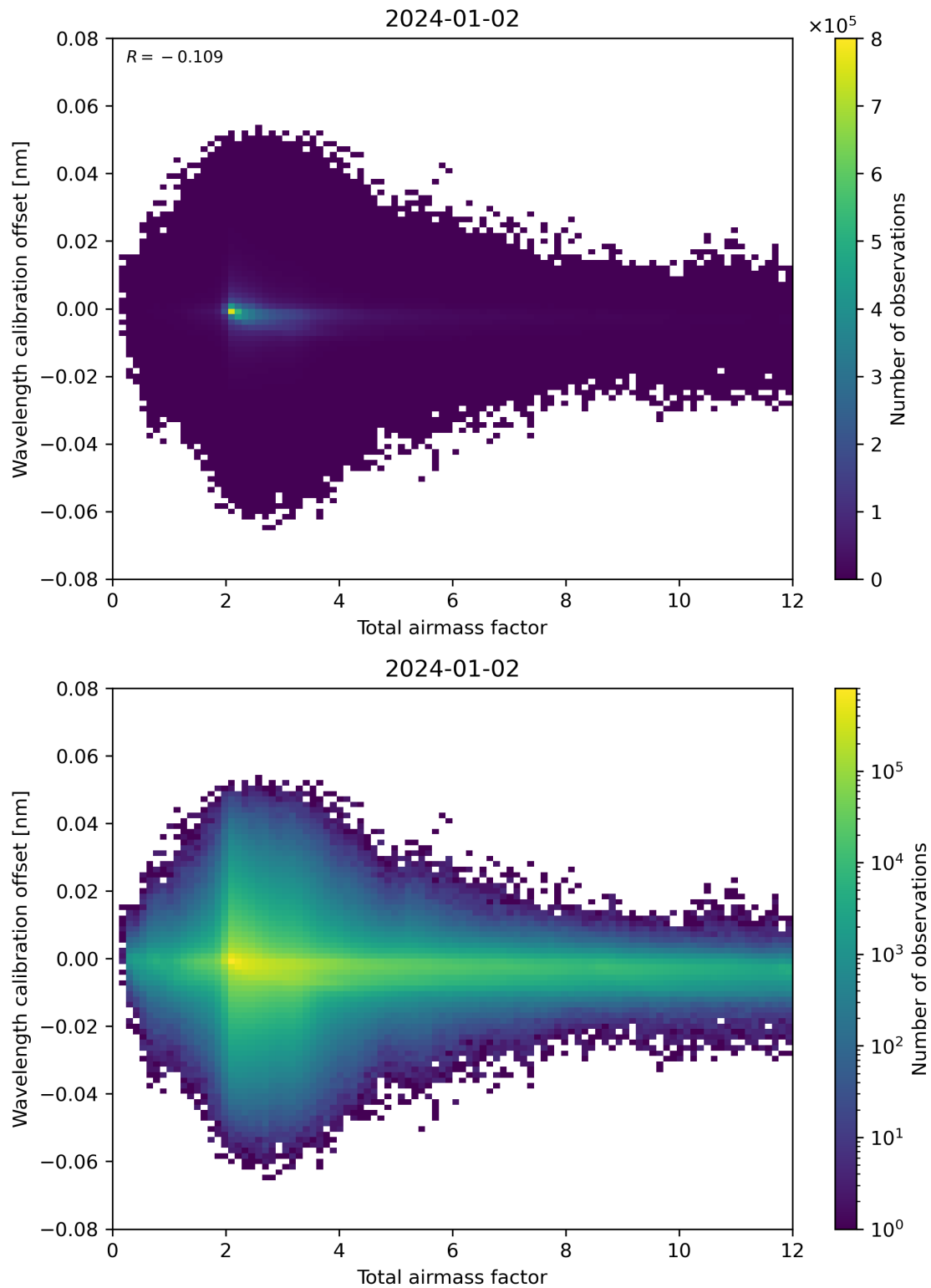
Figure 70: Scatter density plot of “Total airmass factor” against “Wavelength calibration offset” for 2024-01-01 to 2024-01-03.
