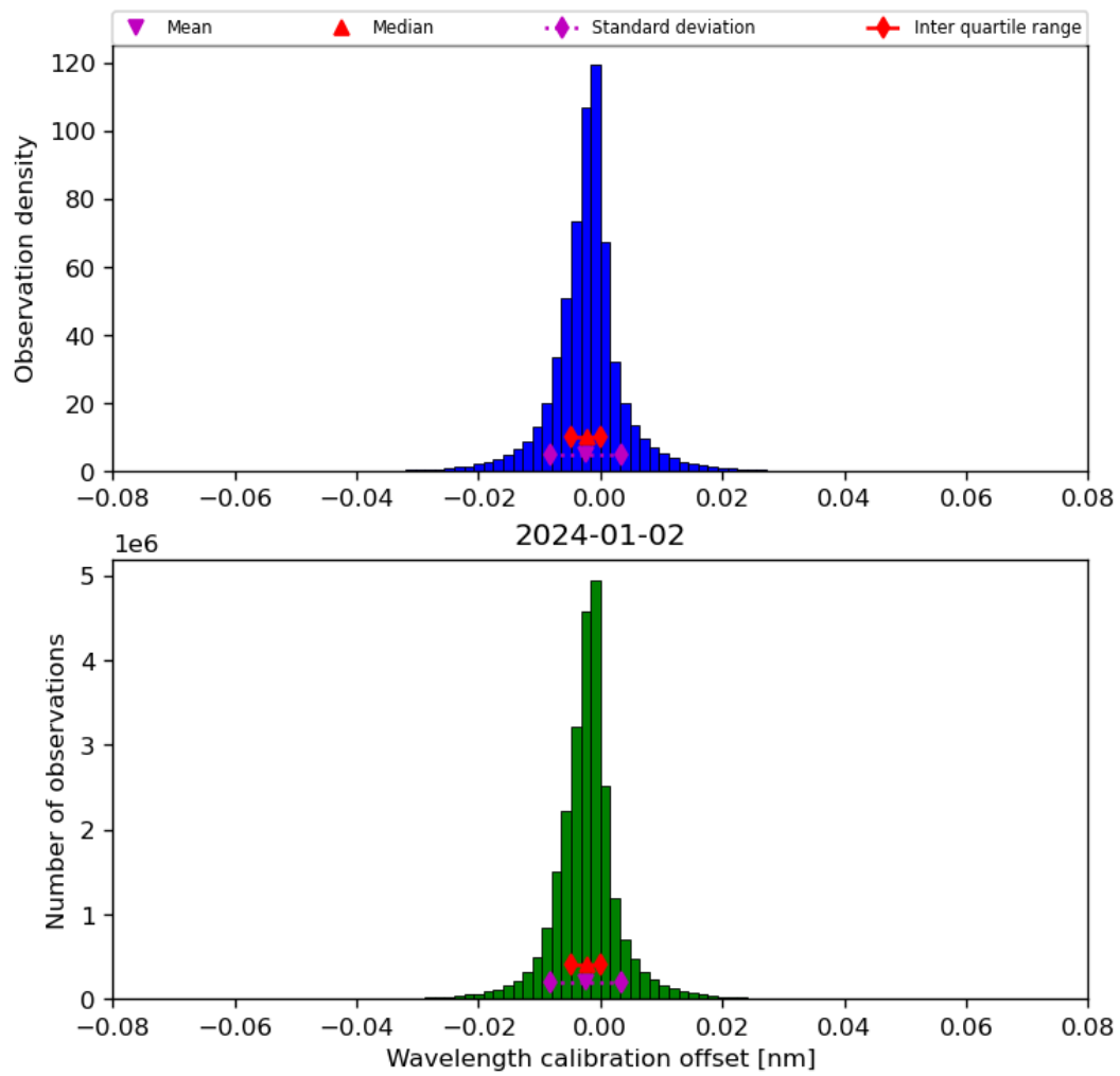
Figure 35: Histogram of “Wavelength calibration offset” for 2024-01-01 to 2024-01-03
