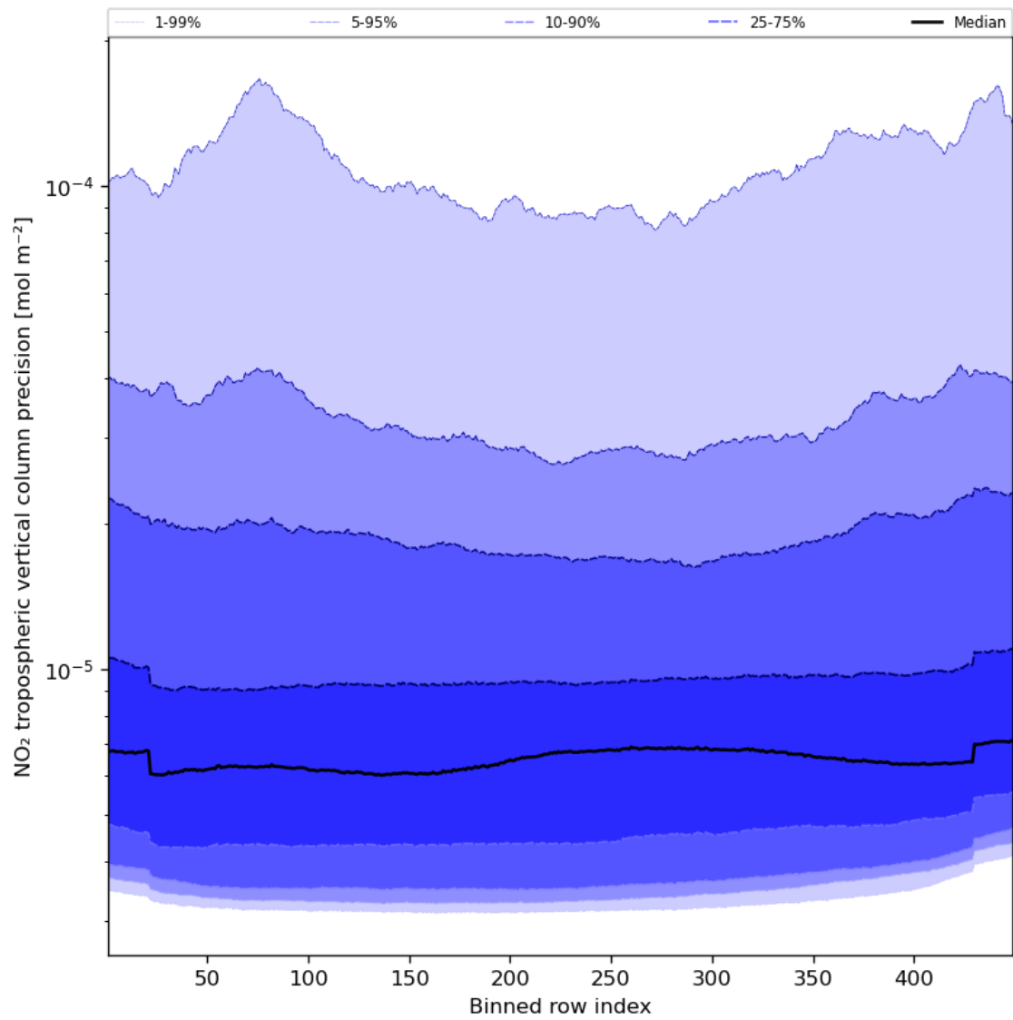
Figure 47: Along track statistics of “NO 2 tropospheric vertical column precision” for 2024-01-01 to 2024-01-03
