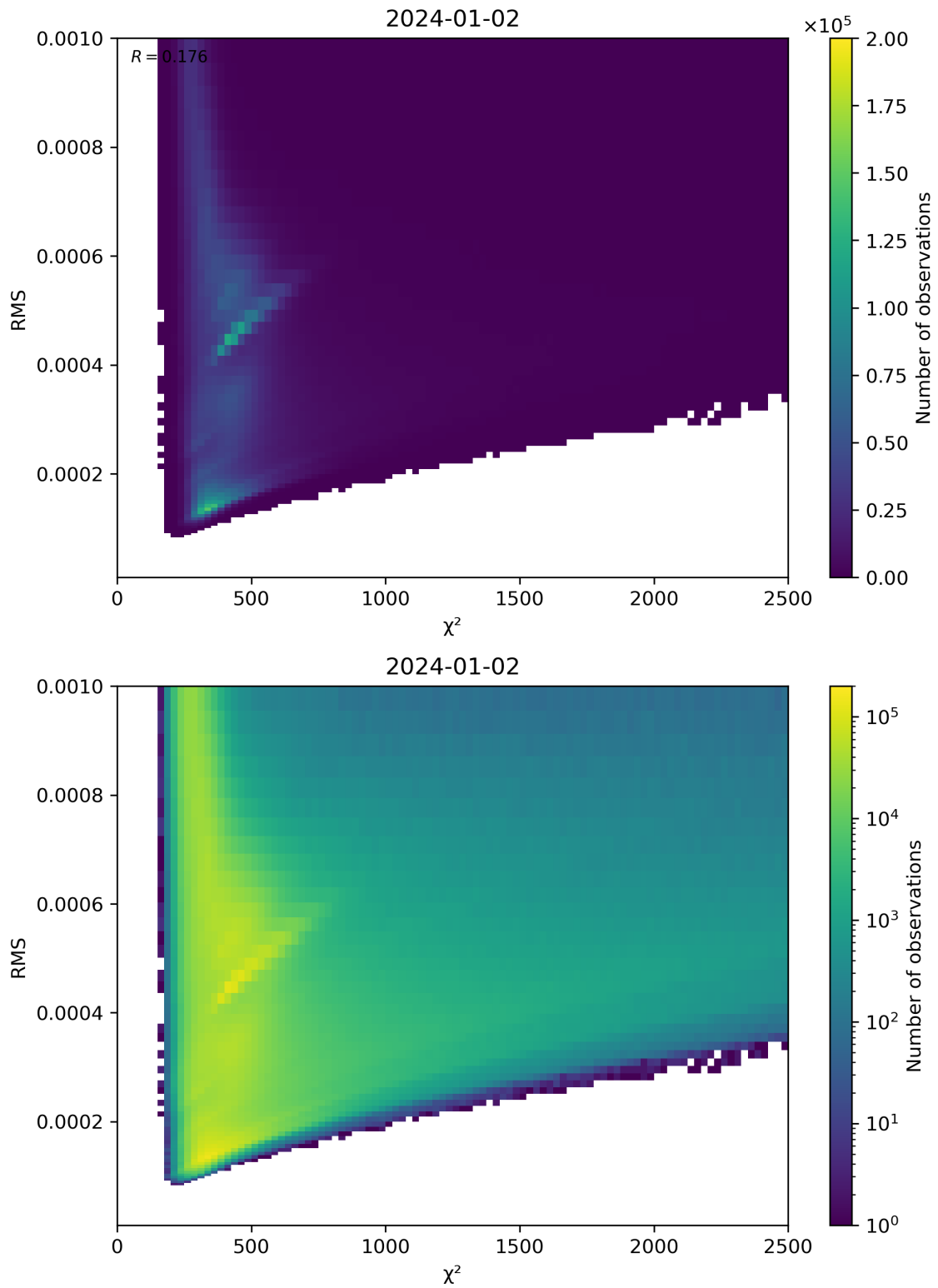
Figure 82: Scatter density plot of “ \chi^2 ” against “RMS” for 2024-01-01 to 2024-01-03.
