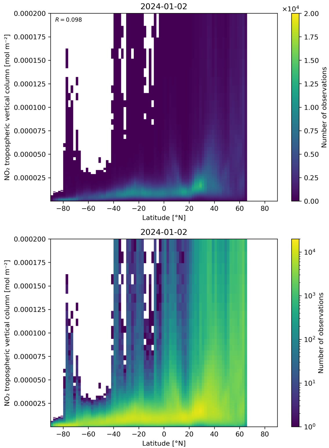
Figure 92: Scatter density plot of “Latitude” against “NO 2 tropospheric vertical column” for 2024-01-01 to 2024-01-03.
