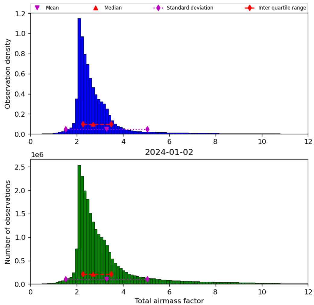
Figure 32: Histogram of “Total airmass factor” for 2024-01-01 to 2024-01-03
