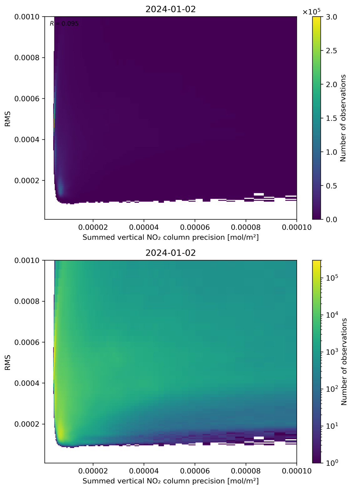
Figure 108: Scatter density plot of “Summed vertical NO 2 column precision” against “RMS” for 2024-01-01 to 2024-01-03.
