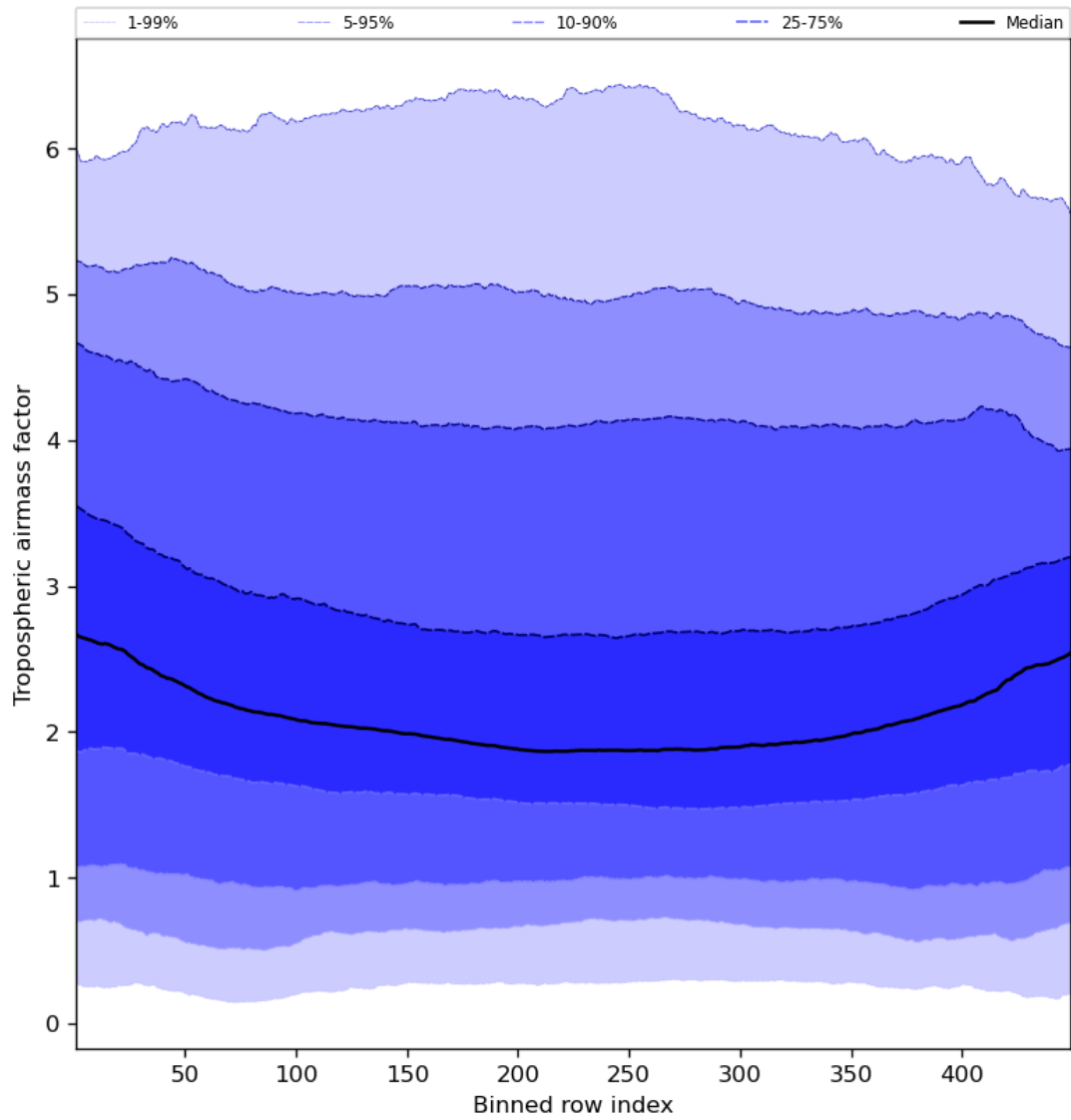
Figure 48: Along track statistics of “Tropospheric airmass factor” for 2024-01-01 to 2024-01-03
