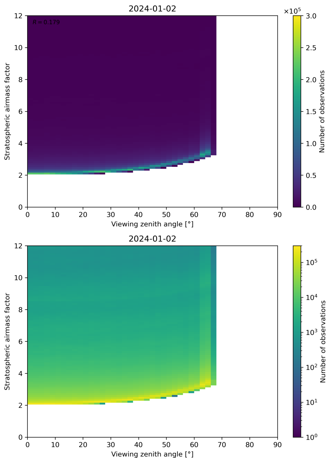
Figure 159: Scatter density plot of “Viewing zenith angle” against “Stratospheric airmass factor” for 2024-01-01 to 2024-01-03.
