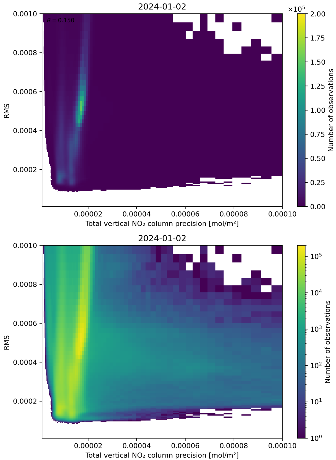
Figure 119: Scatter density plot of “Total vertical NO 2 column precision” against “RMS” for 2024-01-01 to 2024-01-03.
