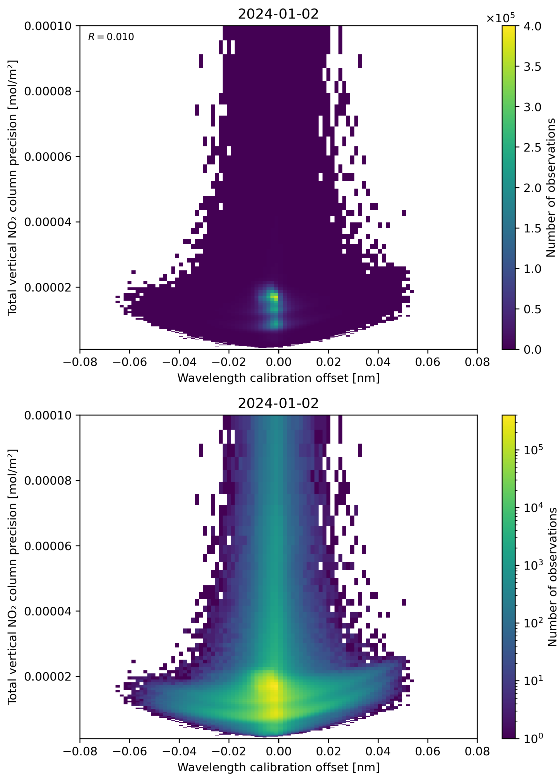
Figure 180: Scatter density plot of “Wavelength calibration offset” against “Total vertical NO 2 column precision” for 2024-01-01 to 2024-01-03.
