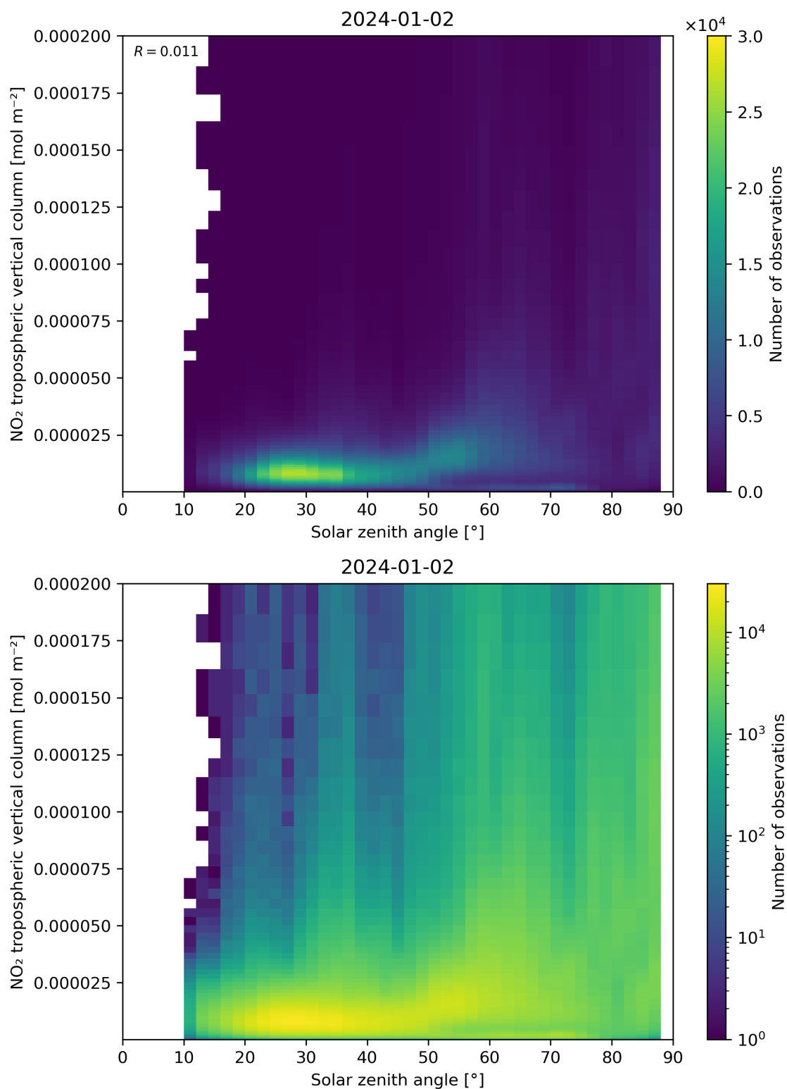
Figure 155: Scatter density plot of “Solar zenith angle” against “NO 2 tropospheric vertical column” for 2024-01-01 to 2024-01-03.
