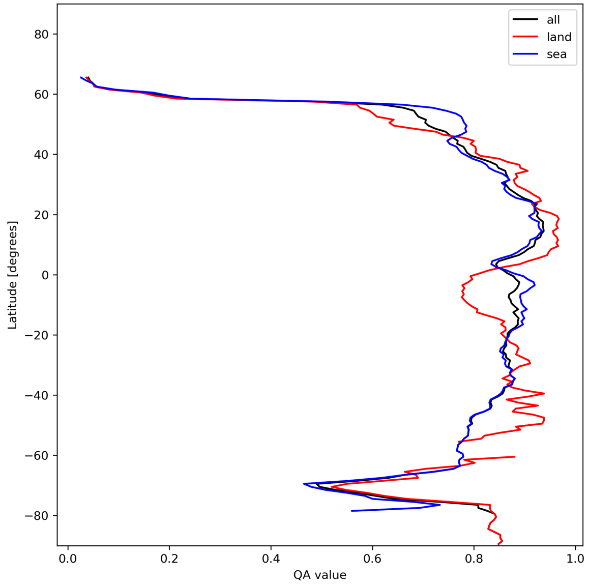
Figure 11: Zonal average of “QA value” for 2024-01-01 to 2024-01-03.
