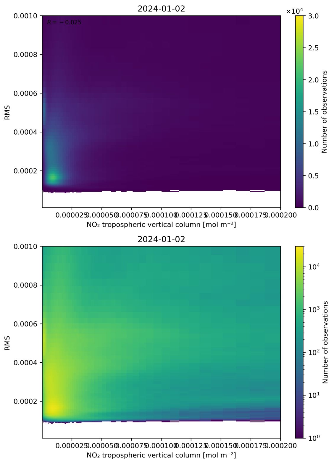
Figure 142: Scatter density plot of “NO 2 tropospheric vertical column” against “RMS” for 2024-01-01 to 2024-01-03.
