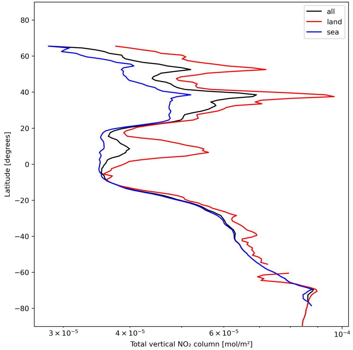
Figure 21: Zonal average of “Total vertical NO 2 column” for 2024-01-01 to 2024-01-03.
