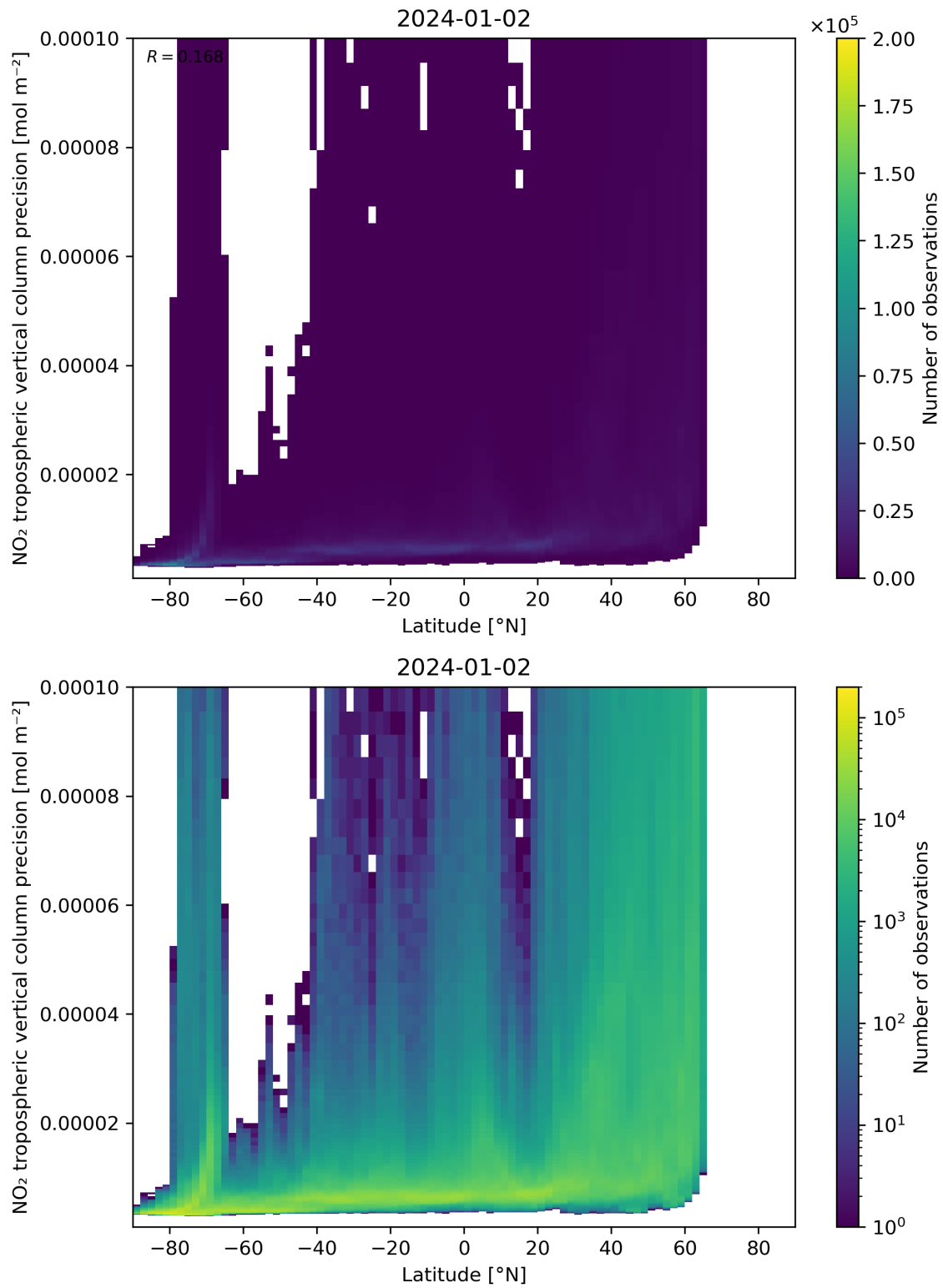
Figure 93: Scatter density plot of “Latitude” against “NO 2 tropospheric vertical column precision” for 2024-01-01 to 2024-01-03.
