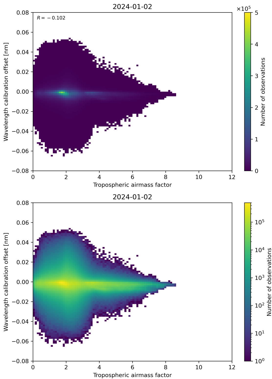
Figure 80: Scatter density plot of “Tropospheric air mass factor” against “Wavelength calibration offset” for 2024-01-01 to 2024-01-03.
