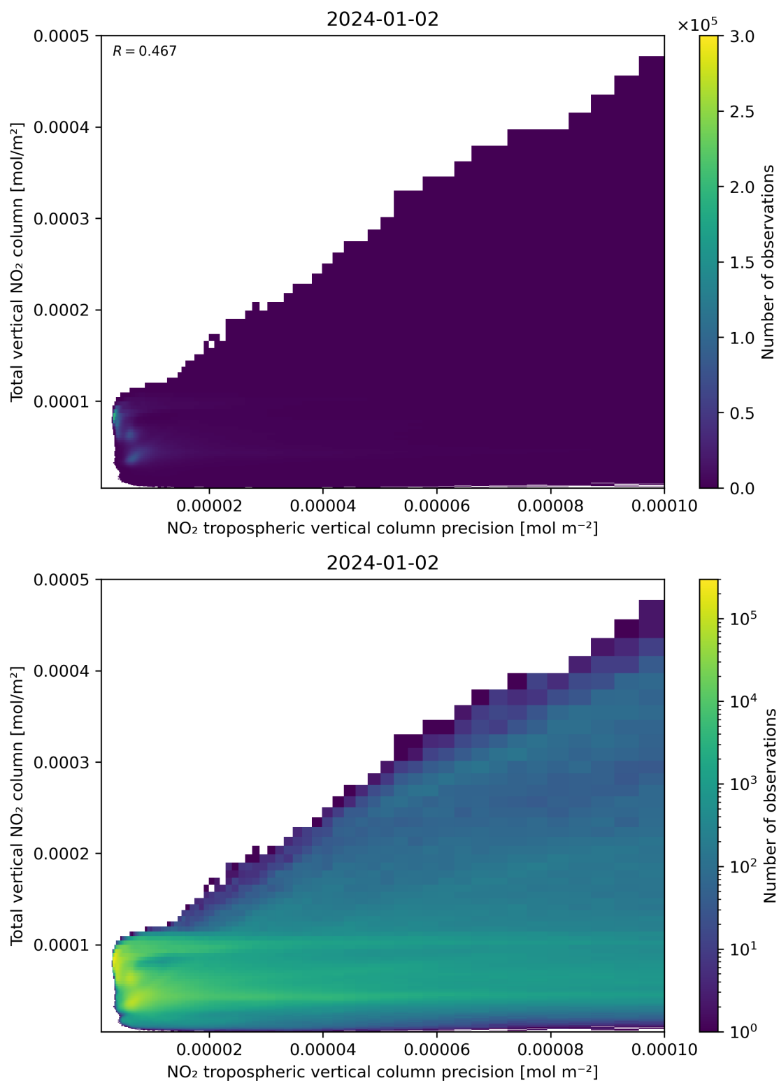
Figure 138: Scatter density plot of “NO 2 tropospheric vertical column precision” against “Total vertical NO 2 column” for 2024-01-01 to 2024-01-03.
