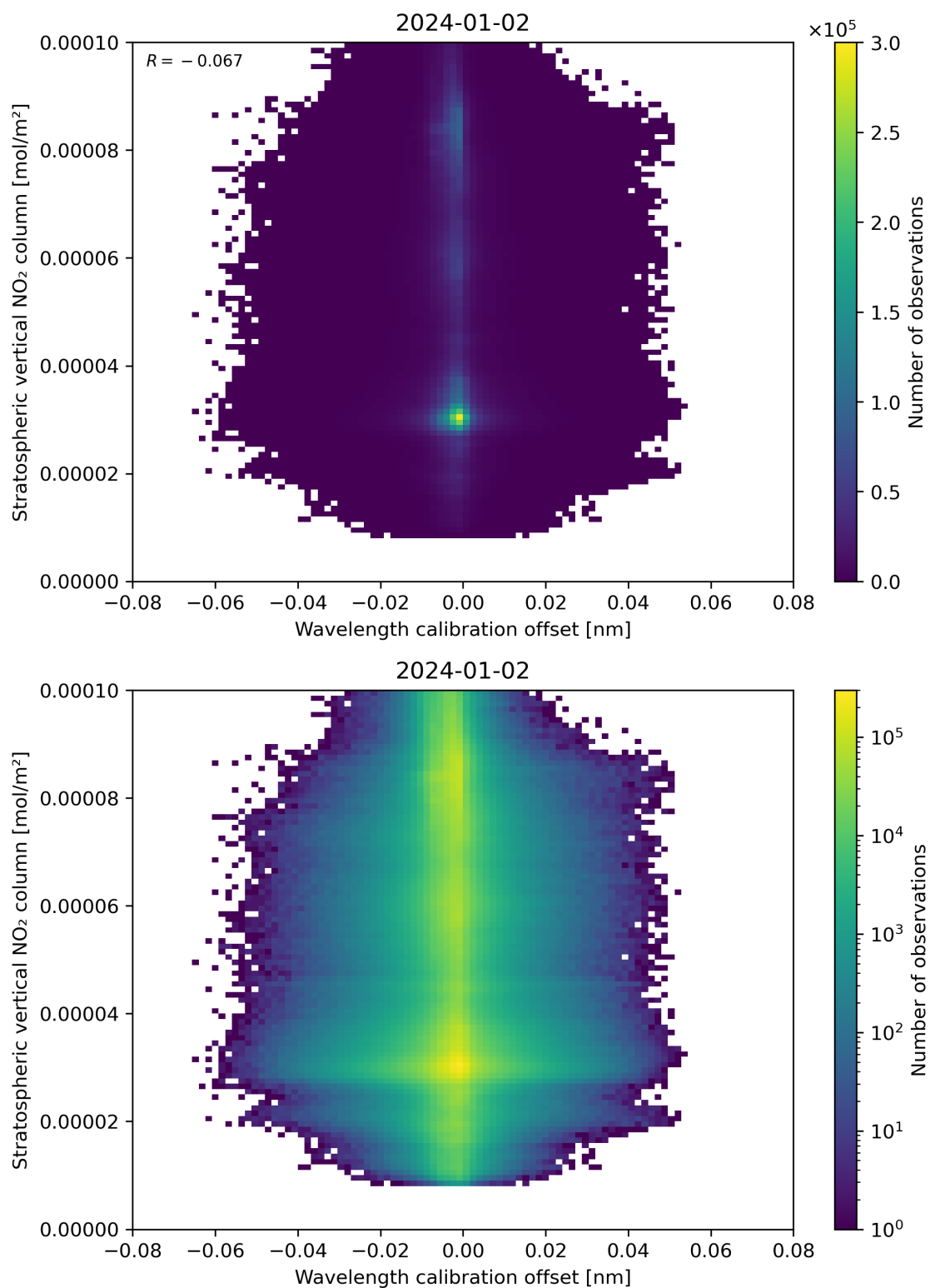
Figure 176: Scatter density plot of “Wavelength calibration offset” against “Stratospheric vertical NO 2 column” for 2024-01-01 to 2024-01-03.
