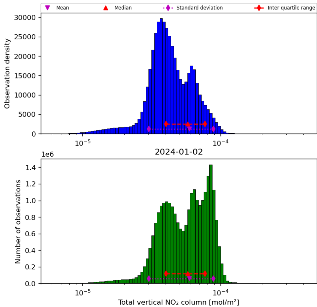
Figure 38: Histogram of “Total vertical NO 2 column” for 2024-01-01 to 2024-01-03
