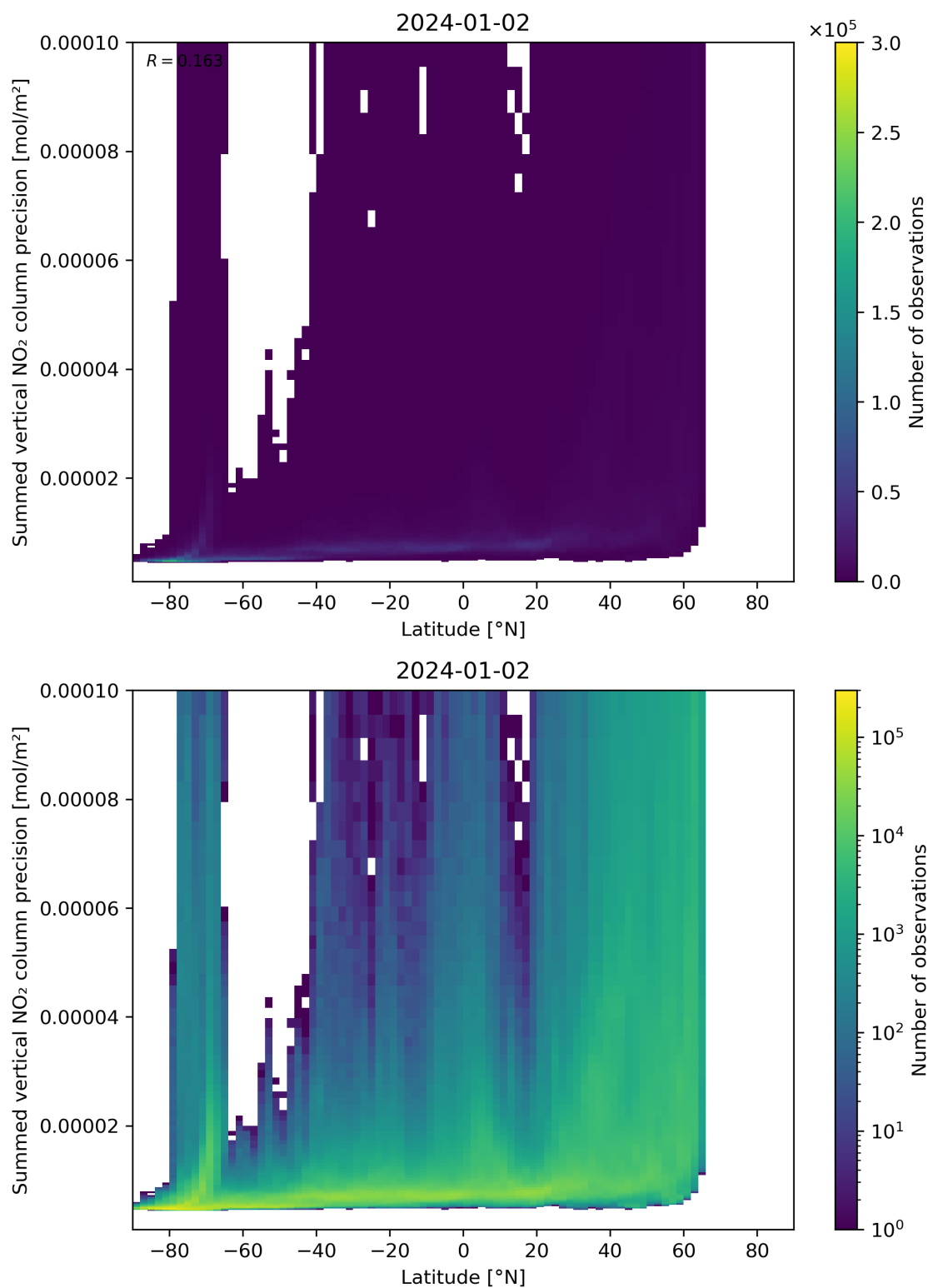
Figure 89: Scatter density plot of “Latitude” against “Summed vertical NO 2 column precision” for 2024-01-01 to 2024-01-03.
