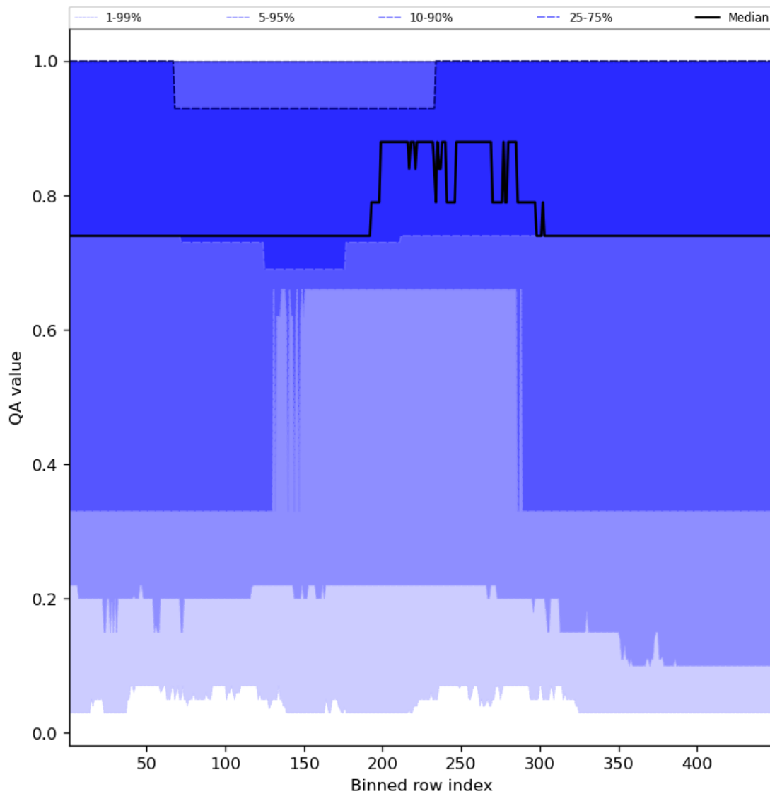
Figure 45: Along track statistics of “QA value” for 2024-01-01 to 2024-01-03
