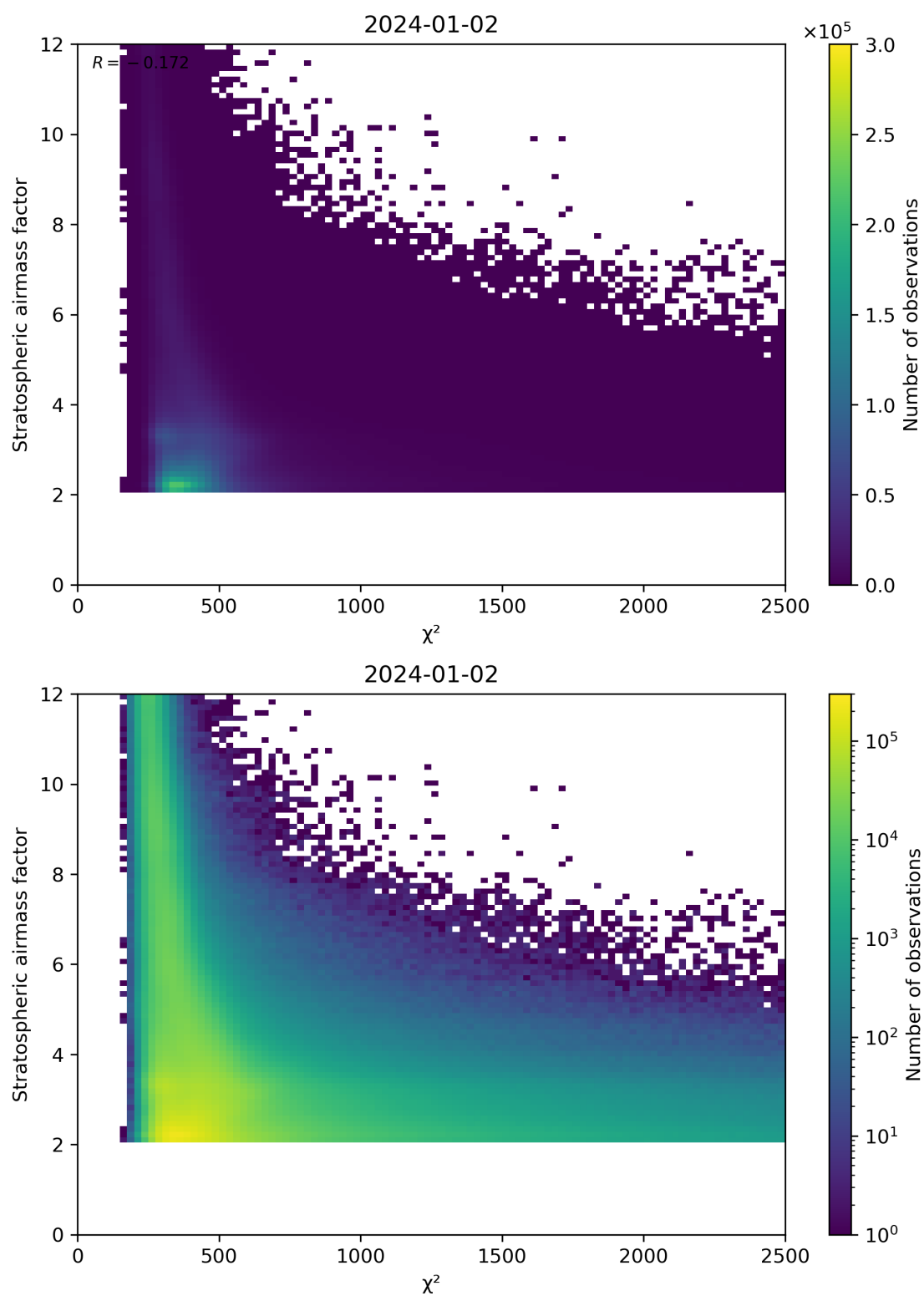
Figure 81: Scatter density plot of “ \chi^2 ” against “Stratospheric airmass factor” for 2024-01-01 to 2024-01-03.
