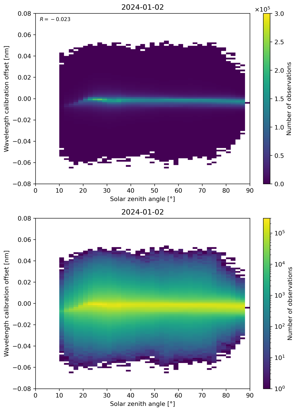
Figure 158: Scatter density plot of “Solar zenith angle” against “Wavelength calibration offset” for 2024-01-01 to 2024-01-03.
