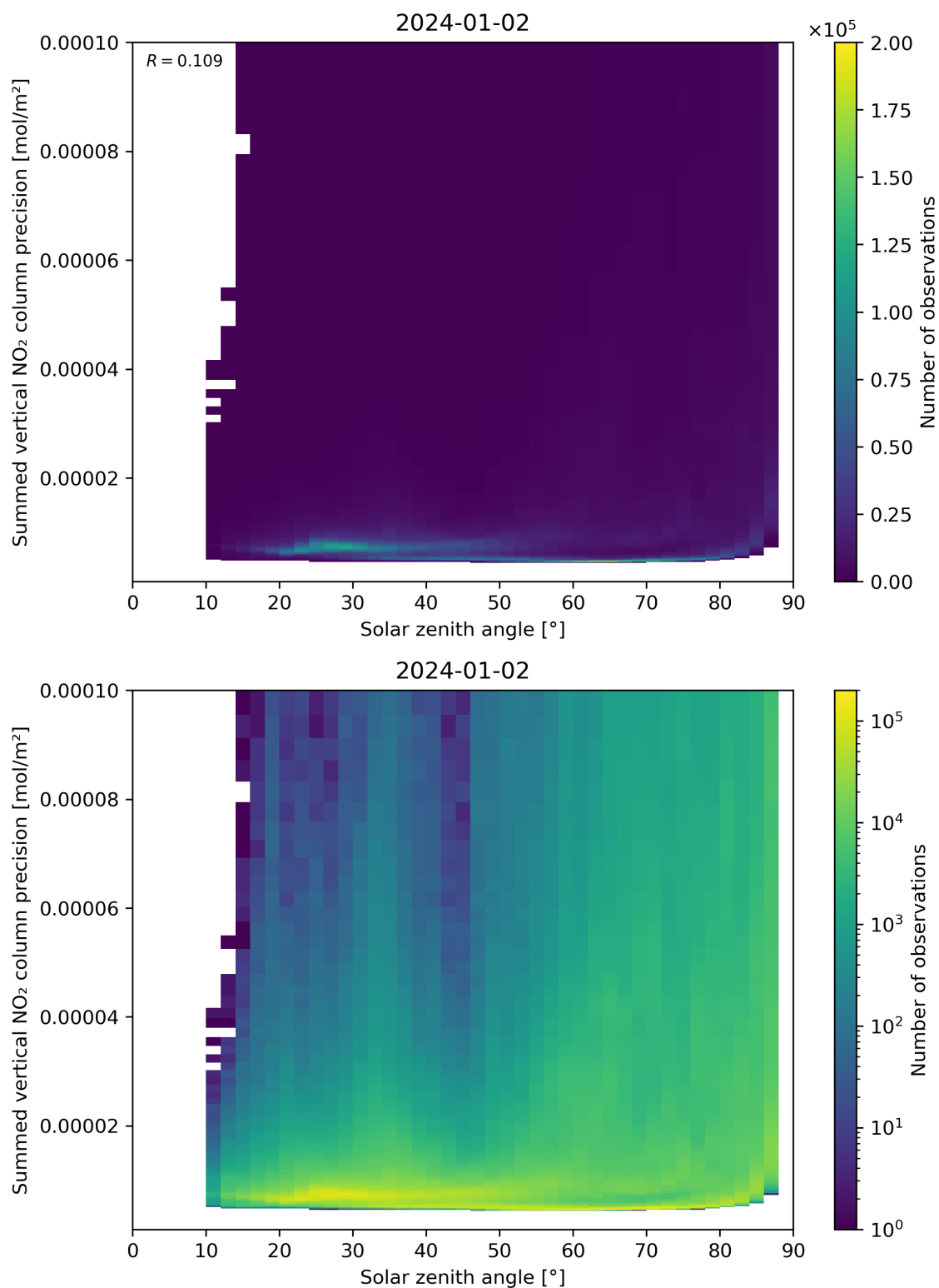
Figure 152: Scatter density plot of “Solar zenith angle” against “Summed vertical NO 2 column precision” for 2024-01-01 to 2024-01-03.
