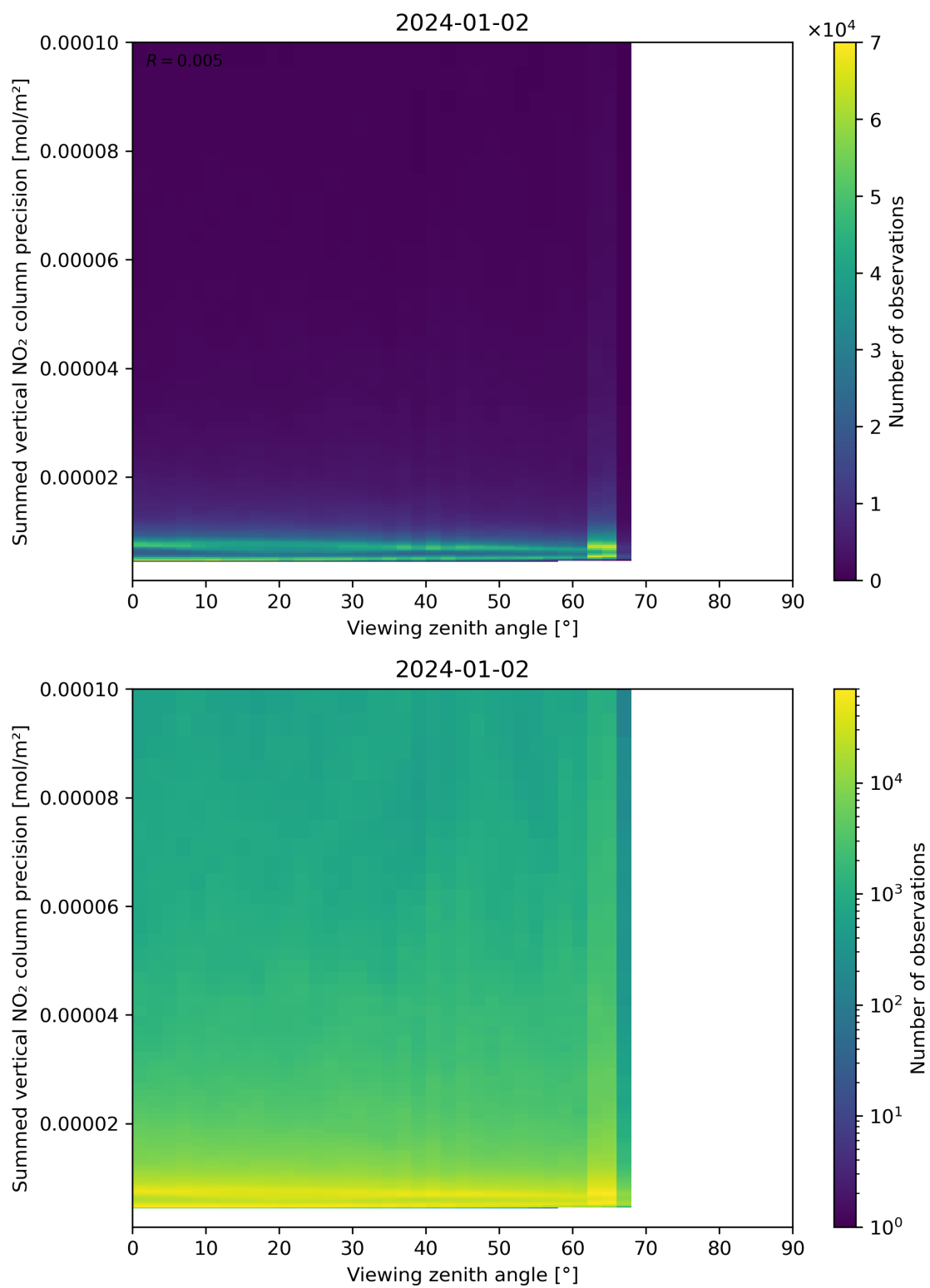
Figure 166: Scatter density plot of “Viewing zenith angle” against “Summed vertical NO 2 column precision” for 2024-01-01 to 2024-01-03.
