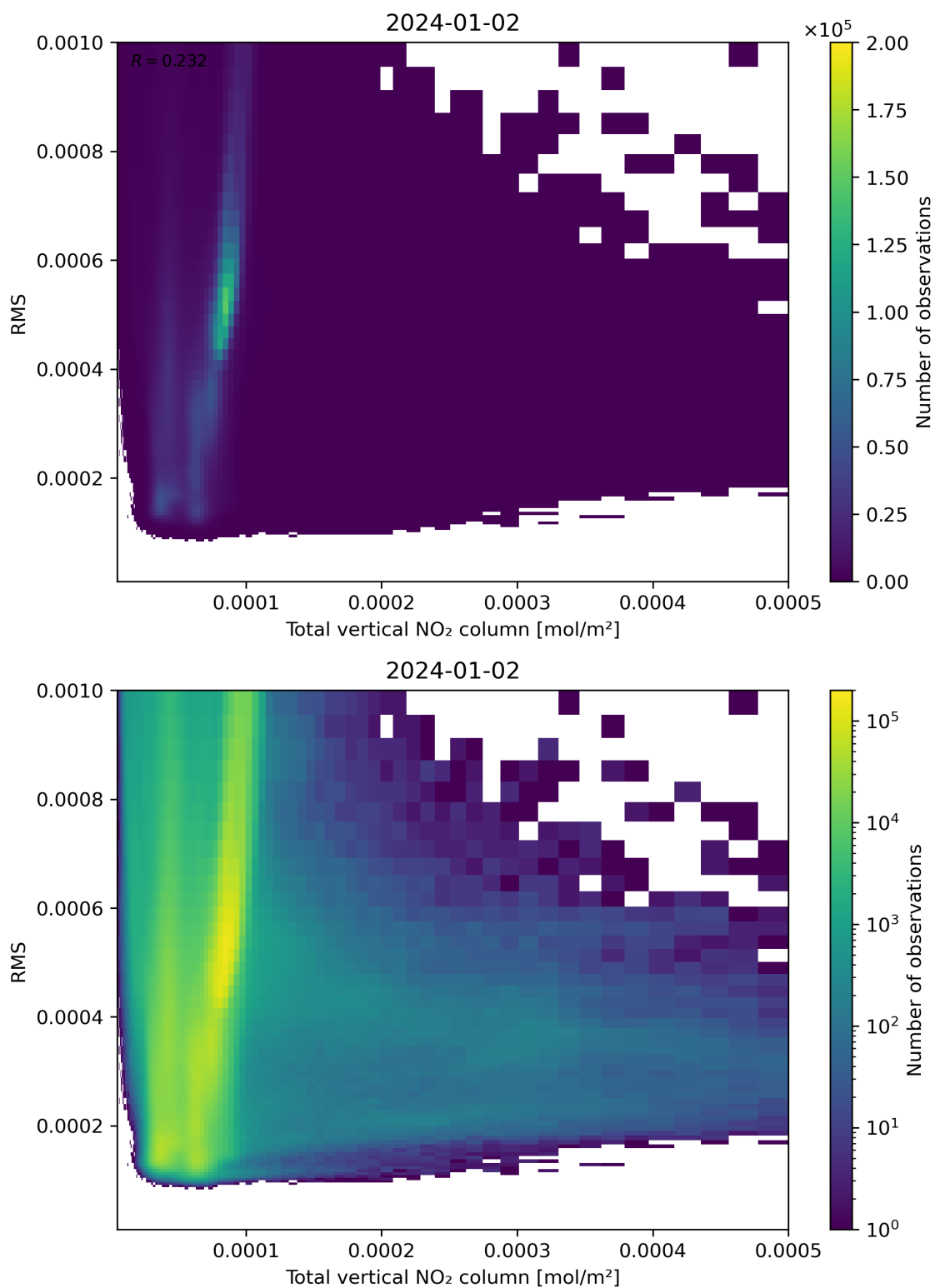
Figure 120: Scatter density plot of “Total vertical NO 2 column” against “RMS” for 2024-01-01 to 2024-01-03.
