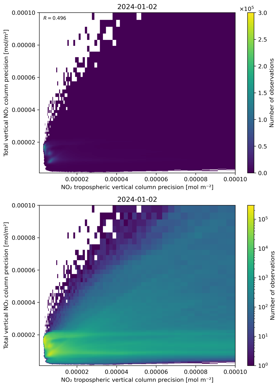
Figure 139: Scatter density plot of “NO 2 tropospheric vertical column precision” against “Total vertical NO 2 column precision” for 2024-01-01 to 2024-01-03.
