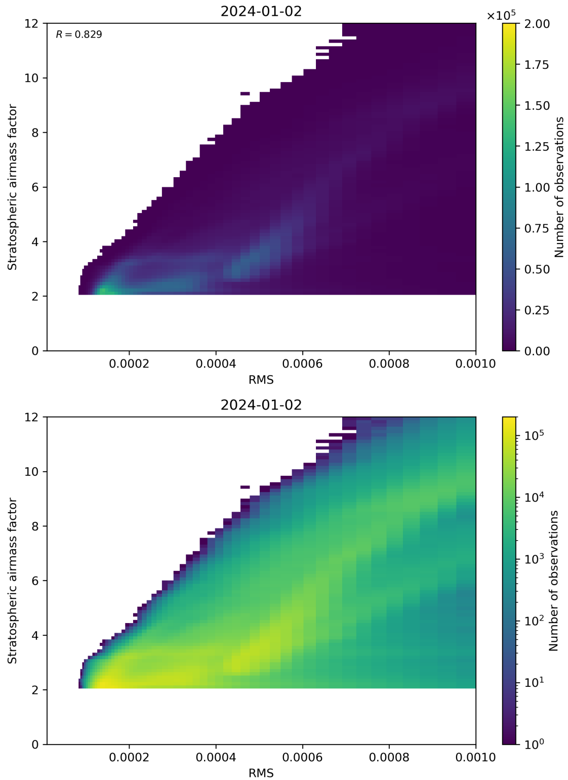
Figure 144: Scatter density plot of “RMS” against “Stratospheric airmass factor” for 2024-01-01 to 2024-01-03.
