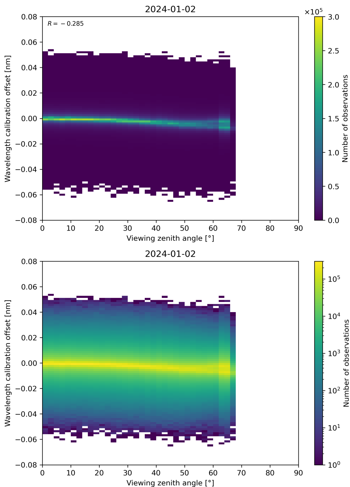
Figure 173: Scatter density plot of “Viewing zenith angle” against “Wavelength calibration offset” for 2024-01-01 to 2024-01-03.
