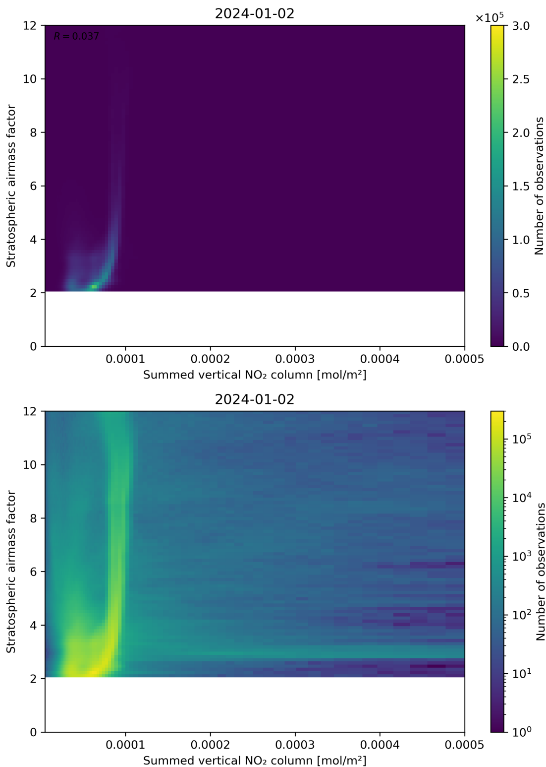
Figure 103: Scatter density plot of “Summed vertical NO 2 column” against “Stratospheric air mass factor” for 2024-01-01 to 2024-01-03.
