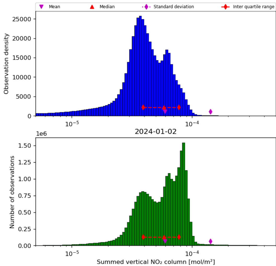
Figure 40: Histogram of “Summed vertical NO 2 column” for 2024-01-01 to 2024-01-03
