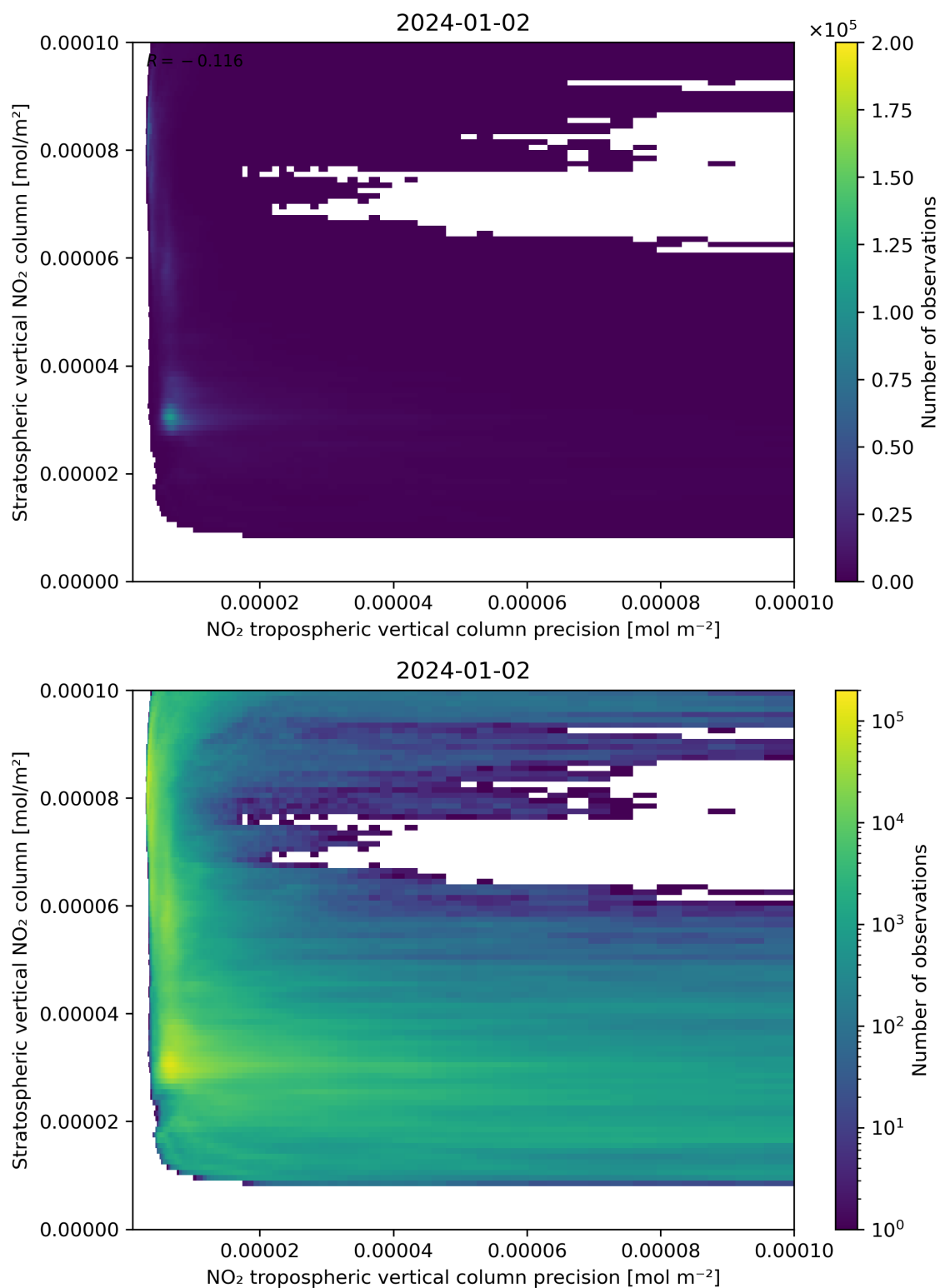
Figure 135: Scatter density plot of “NO 2 tropospheric vertical column precision” against “Stratospheric vertical NO 2 column” for 2024-01-01 to 2024-01-03.
