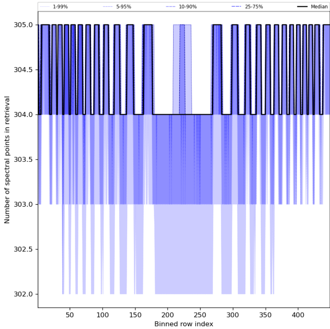
Figure 50: Along track statistics of “Number of spectral points in retrieval” for 2024-01-01 to 2024-01-03
