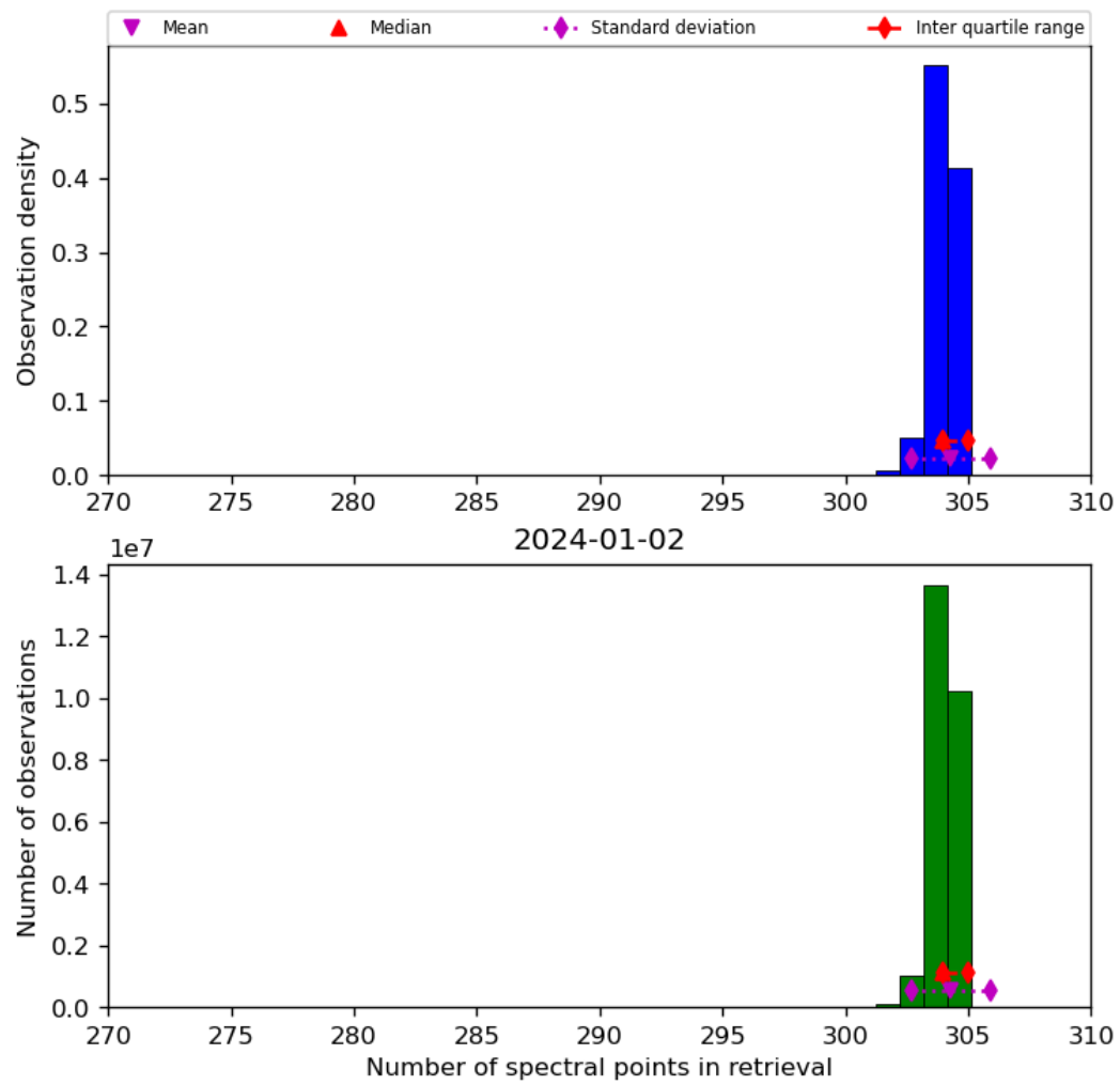
Figure 33: Histogram of “Number of spectral points in retrieval” for 2024-01-01 to 2024-01-03
