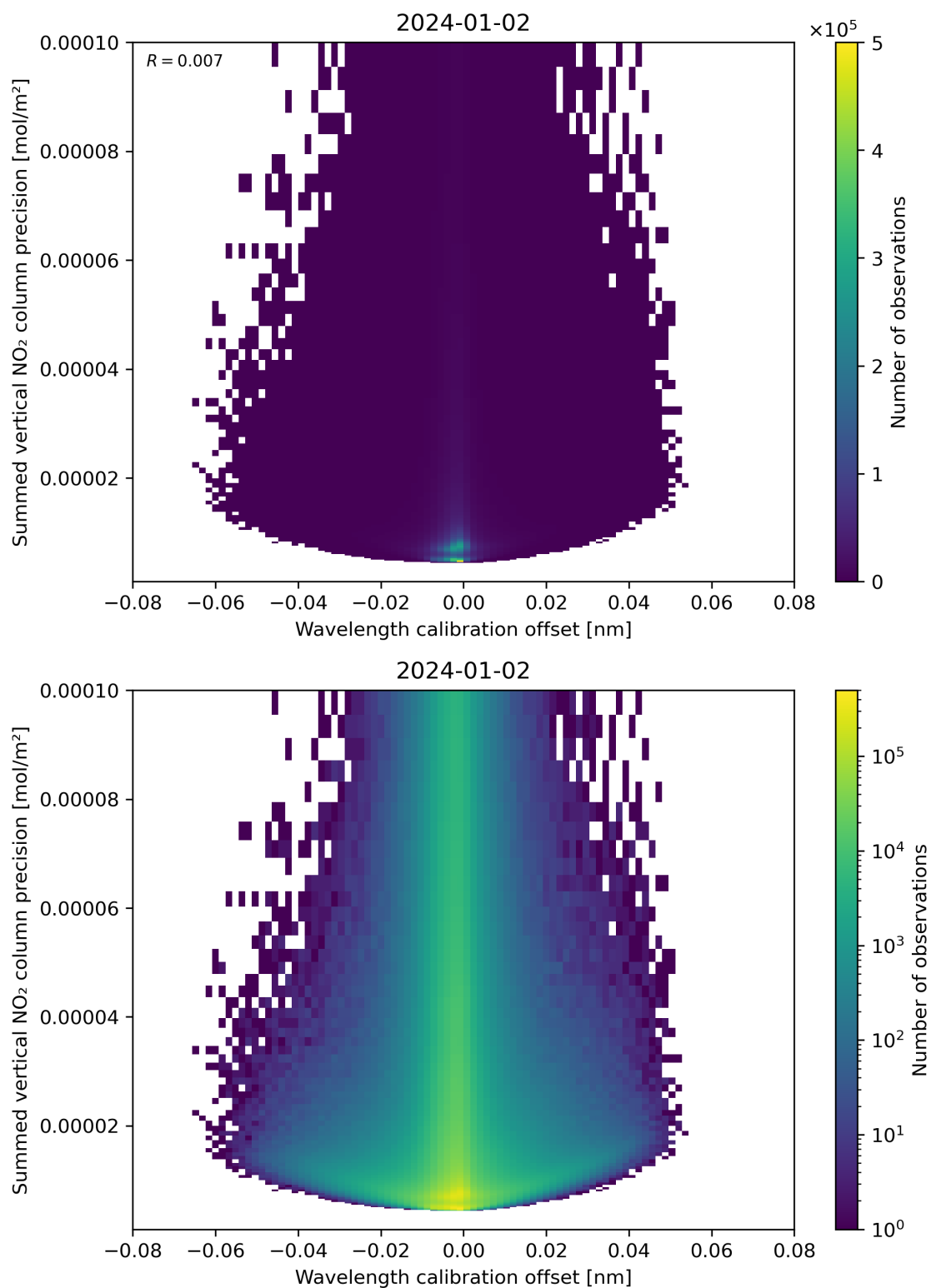
Figure 178: Scatter density plot of “Wavelength calibration offset” against “Summed vertical NO 2 column precision” for 2024-01-01 to 2024-01-03.
