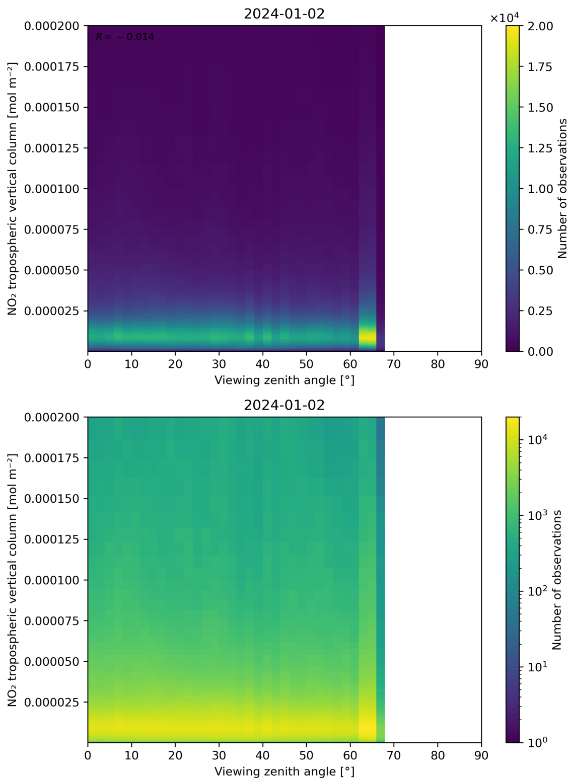
Figure 169: Scatter density plot of “Viewing zenith angle” against “NO 2 tropospheric vertical column” for 2024-01-01 to 2024-01-03.
