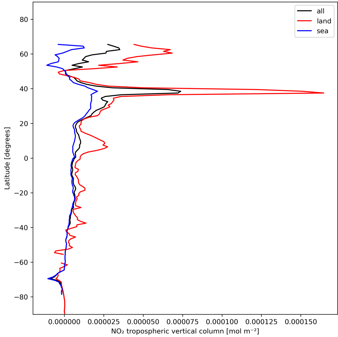
Figure 12: Zonal average of “NO 2 tropospheric vertical column” for 2024-01-01 to 2024-01-03.
