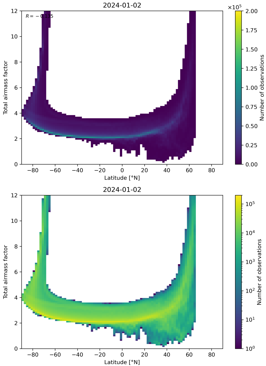
Figure 84: Scatter density plot of “Latitude” against “Total airmass factor” for 2024-01-01 to 2024-01-03.
