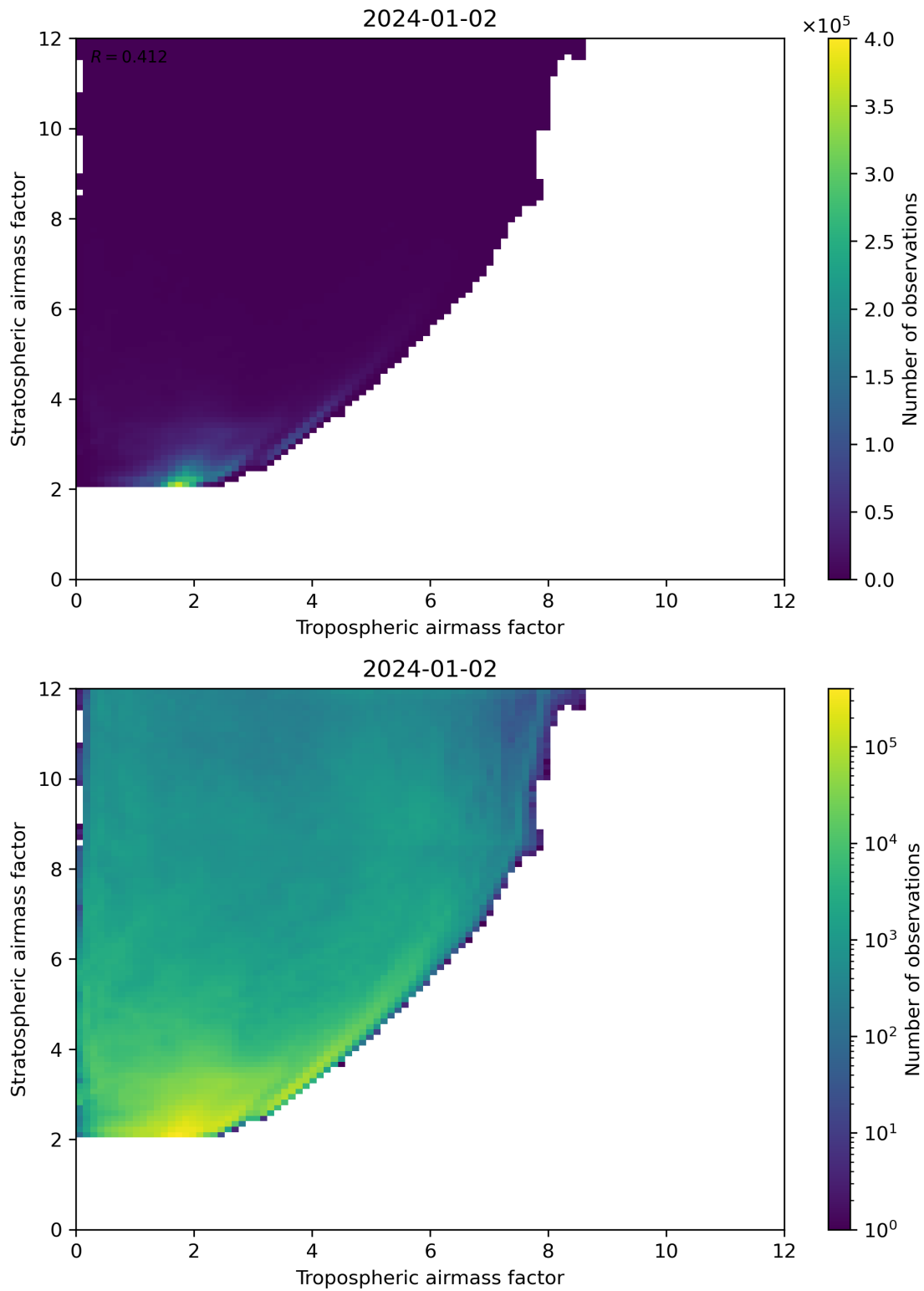
Figure 71: Scatter density plot of “Tropospheric airmass factor” against “Stratospheric airmass factor” for 2024-01-01 to 2024-01-03.
