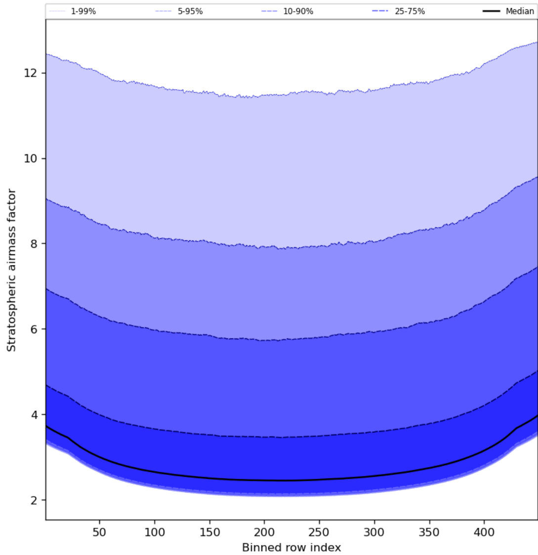
Figure 61: Along track statistics of “Stratospheric airmass factor” for 2024-01-01 to 2024-01-03
