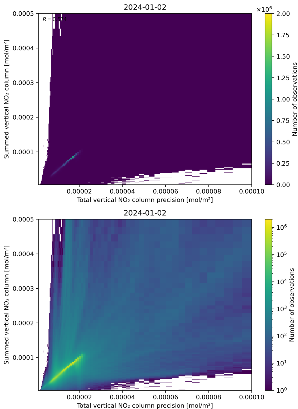
Figure 117: Scatter density plot of “Total vertical NO 2 column precision” against “Summed vertical NO 2 column” for 2024-01-01 to 2024-01-03.
