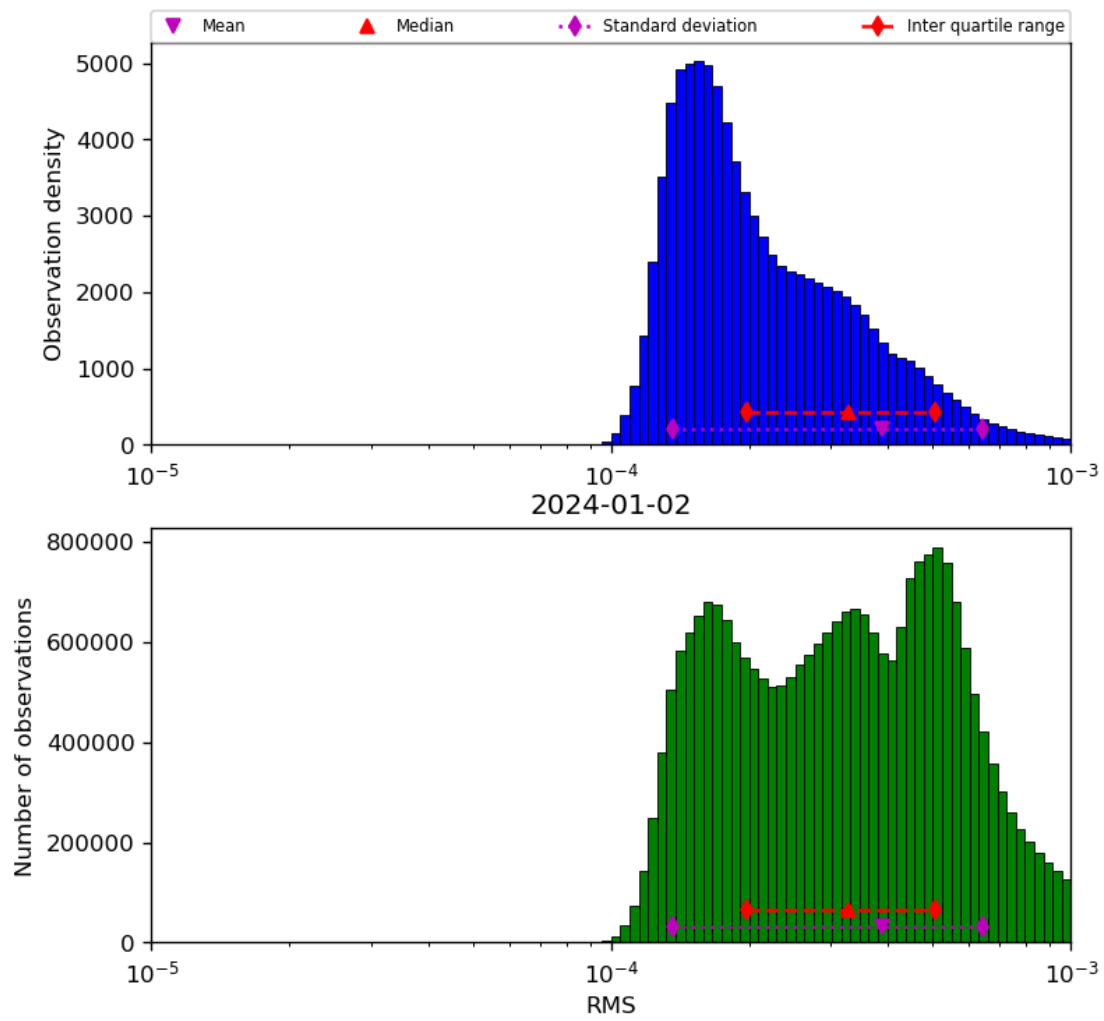
Figure 43: Histogram of “RMS” for 2024-01-01 to 2024-01-03
