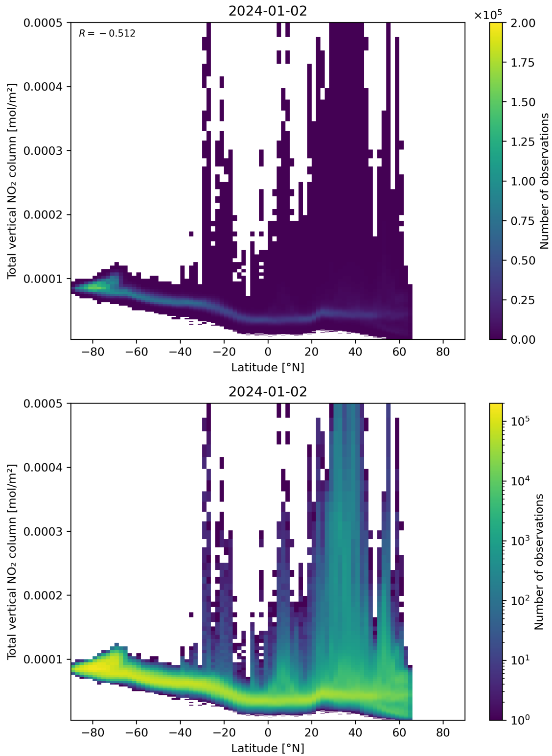
Figure 90: Scatter density plot of “Latitude” against “Total vertical NO 2 column” for 2024-01-01 to 2024-01-03.
