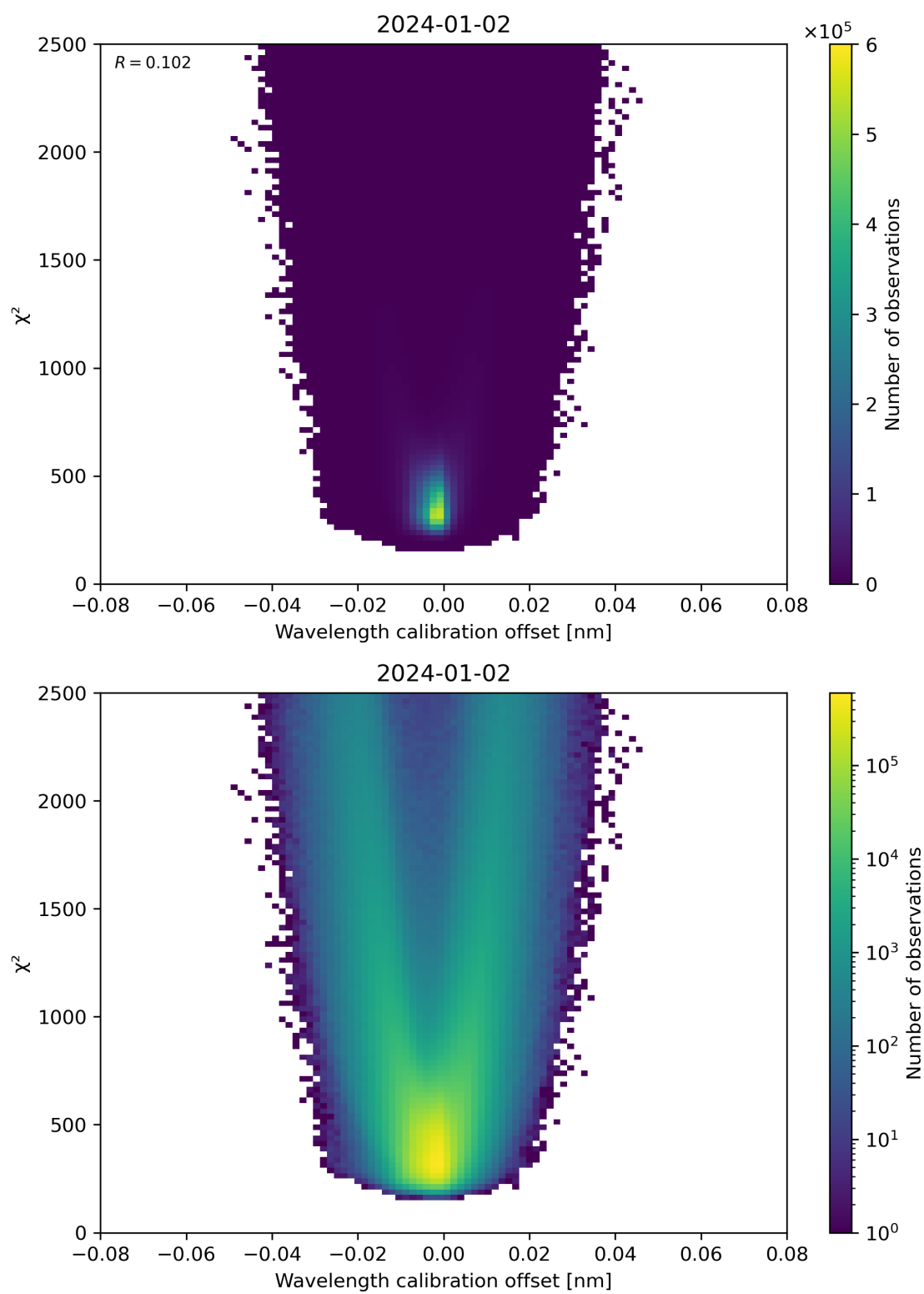
Figure 175: Scatter density plot of “Wavelength calibration offset” against “ \chi^2 ” for 2024-01-01 to 2024-01-03.
