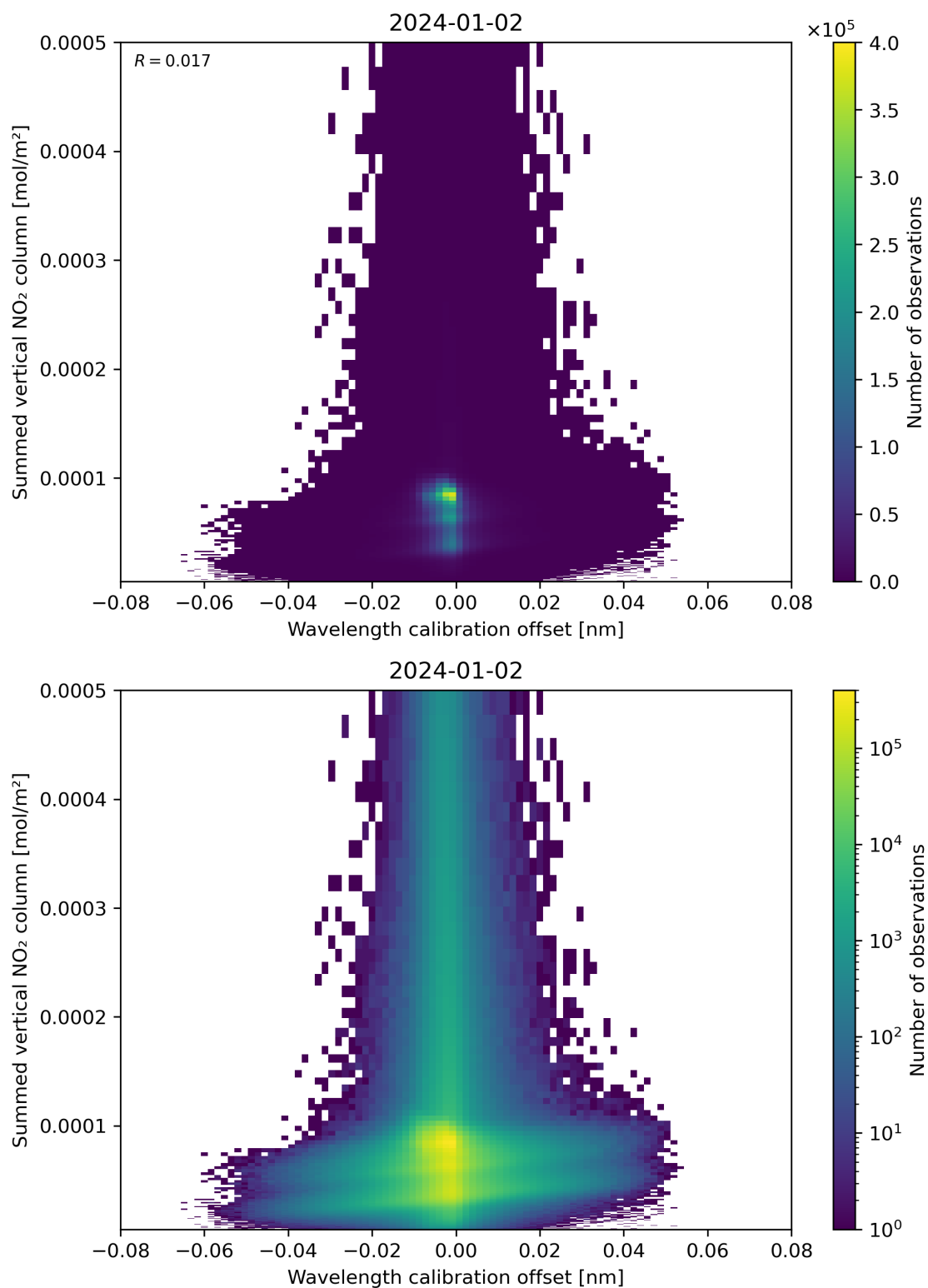
Figure 177: Scatter density plot of “Wavelength calibration offset” against “Summed vertical NO 2 column” for 2024-01-01 to 2024-01-03.
