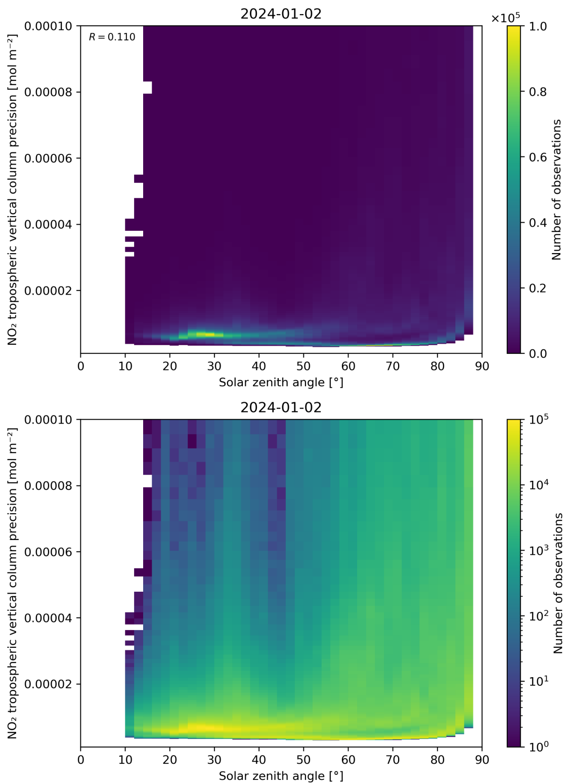
Figure 156: Scatter density plot of “Solar zenith angle” against “NO 2 tropospheric vertical column precision” for 2024-01-01 to 2024-01-03.
