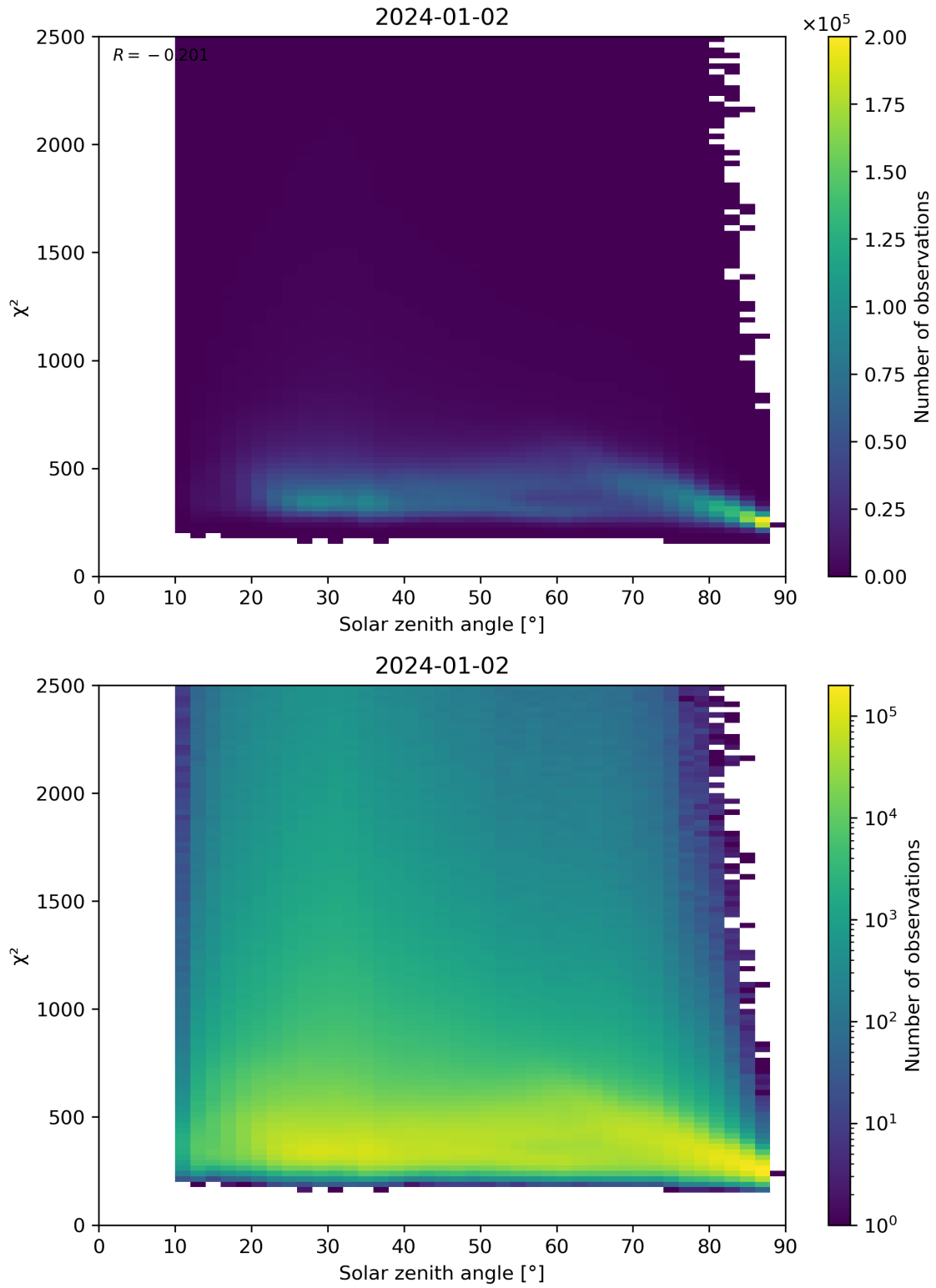
Figure 148: Scatter density plot of “Solar zenith angle” against “ \chi^2 ” for 2024-01-01 to 2024-01-03.
