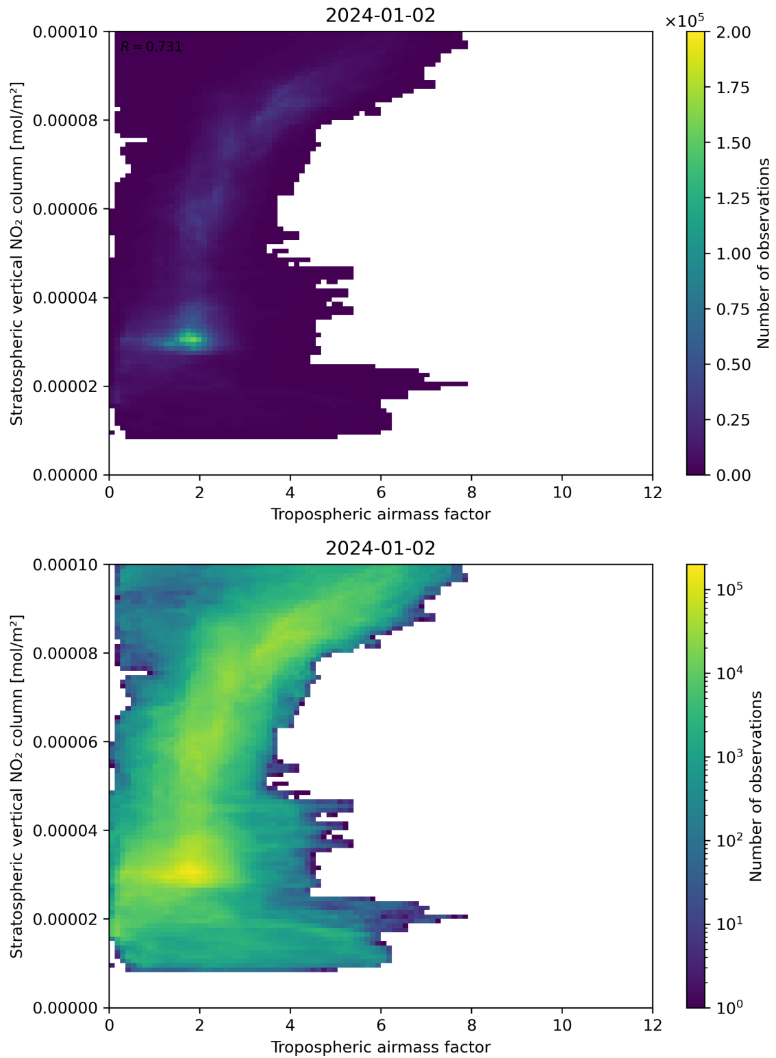
Figure 74: Scatter density plot of “Tropospheric air mass factor” against “Stratospheric vertical NO 2 column” for 2024-01-01 to 2024-01-03.
