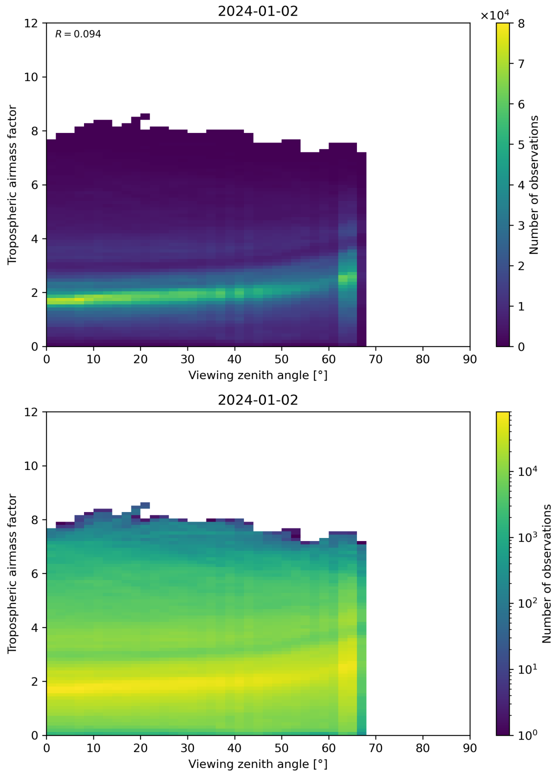
Figure 161: Scatter density plot of “Viewing zenith angle” against “Tropospheric airmass factor” for 2024-01-01 to 2024-01-03.
