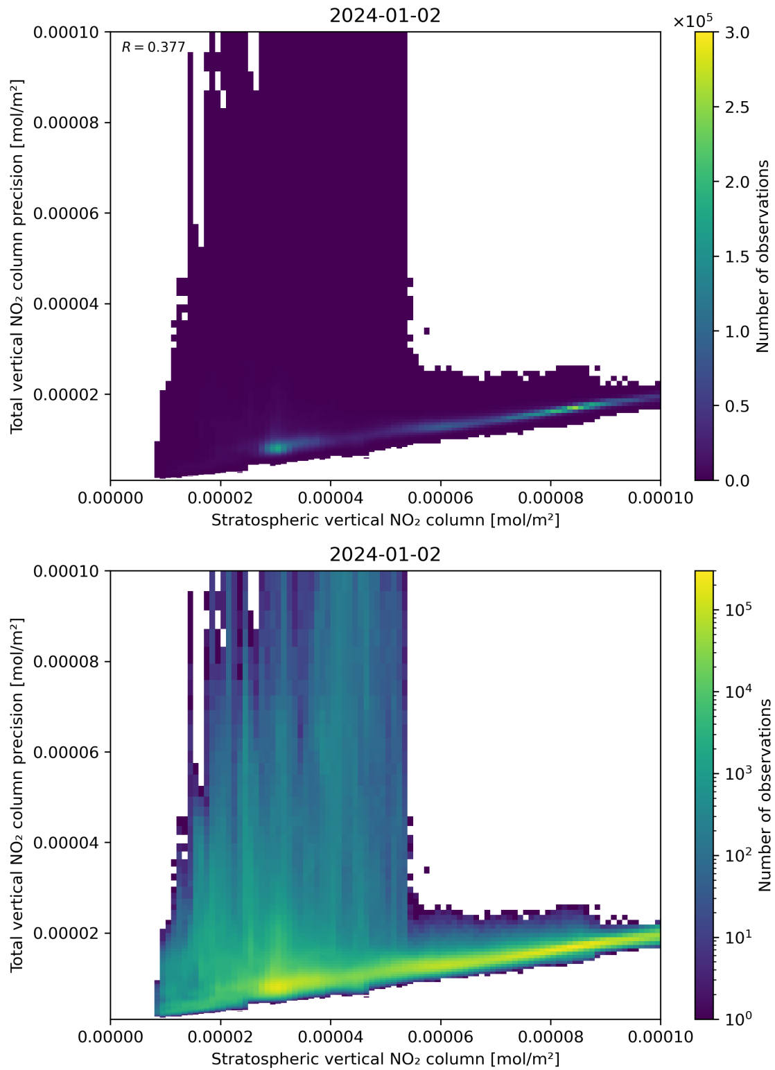
Figure 101: Scatter density plot of “Stratospheric vertical NO 2 column” against “Total vertical NO 2 column precision” for 2024-01-01 to 2024-01-03.
