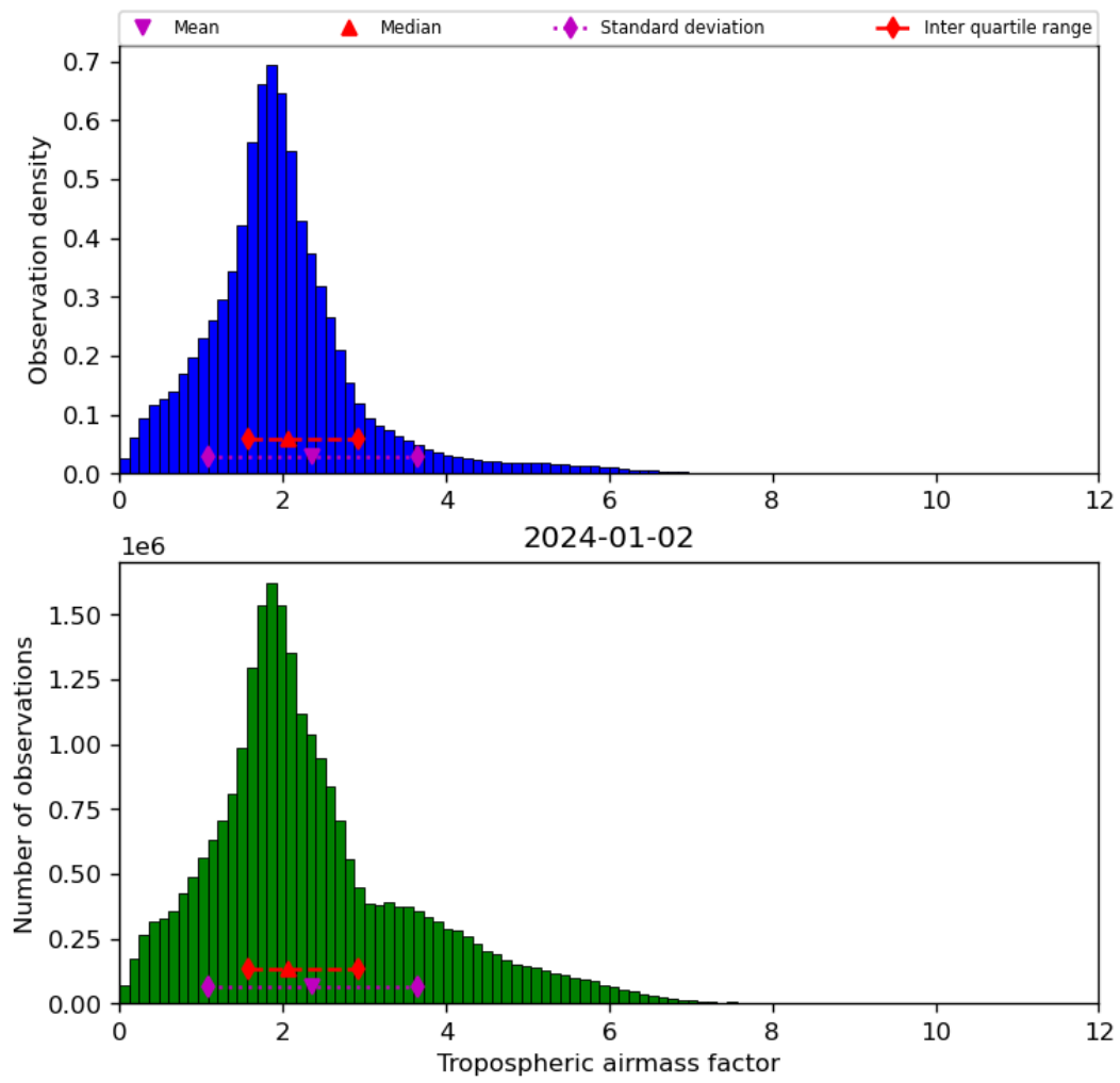
Figure 31: Histogram of “Tropospheric airmass factor” for 2024-01-01 to 2024-01-03
