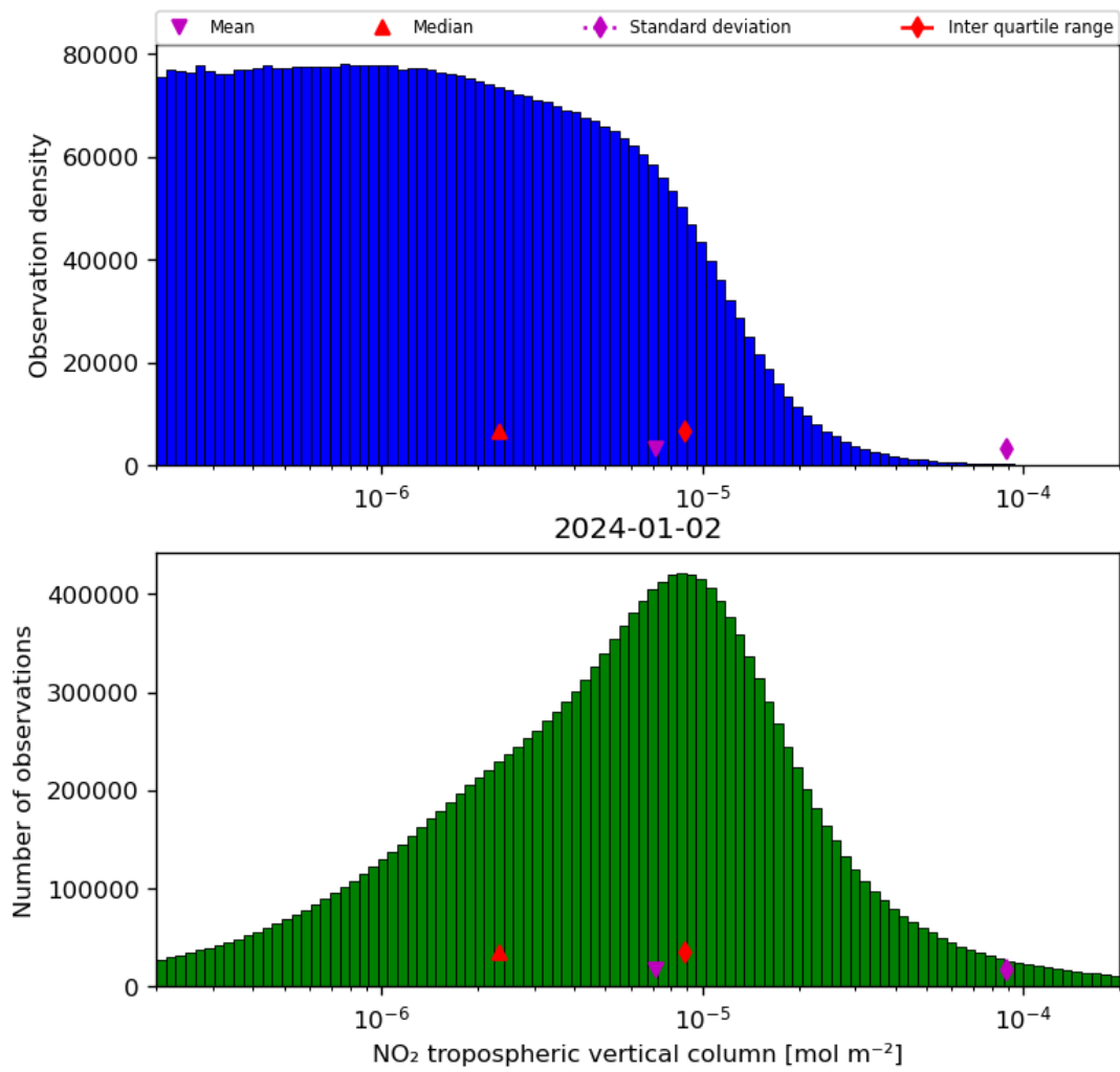
Figure 29: Histogram of “NO 2 tropospheric vertical column” for 2024-01-01 to 2024-01-03
