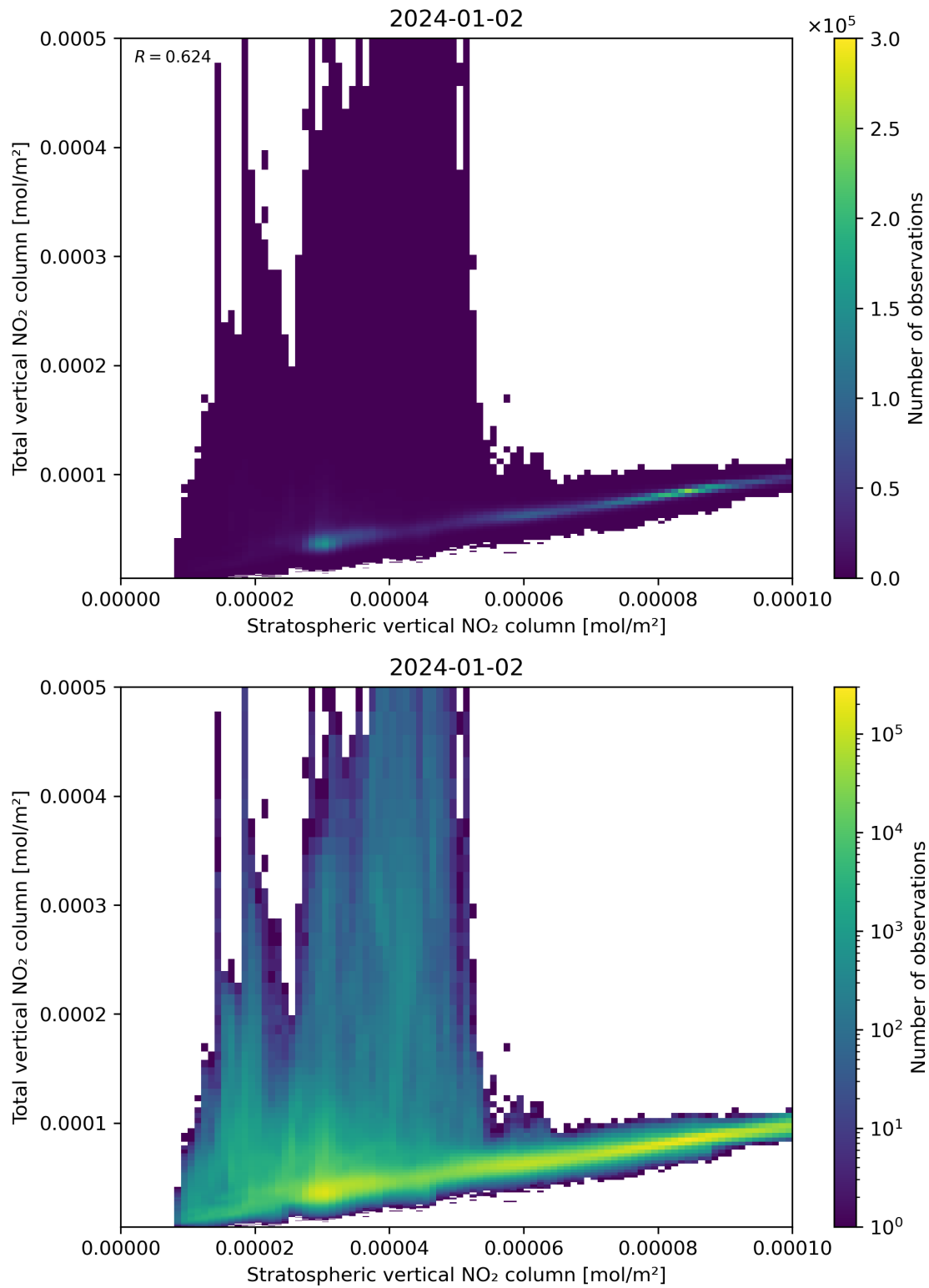
Figure 100: Scatter density plot of “Stratospheric vertical NO 2 column” against “Total vertical NO 2 column” for 2024-01-01 to 2024-01-03.
