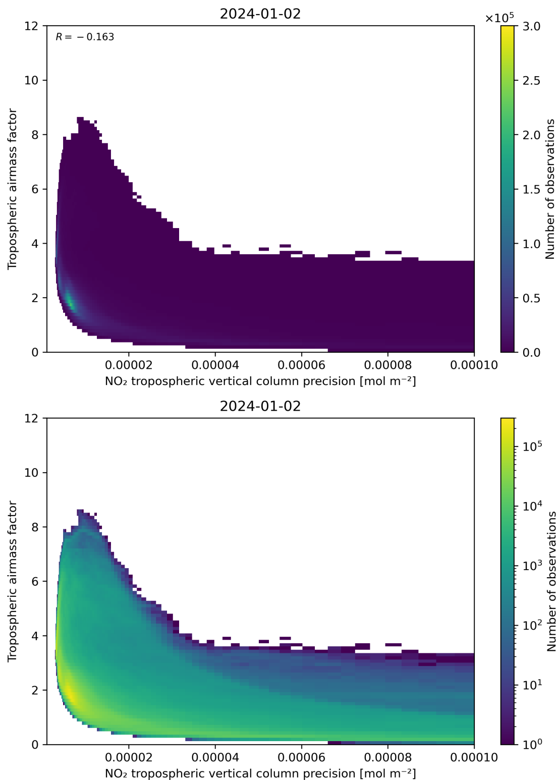
Figure 133: Scatter density plot of “NO 2 tropospheric vertical column precision” against “Tropospheric airmass factor” for 2024-01-01 to 2024-01-03.
