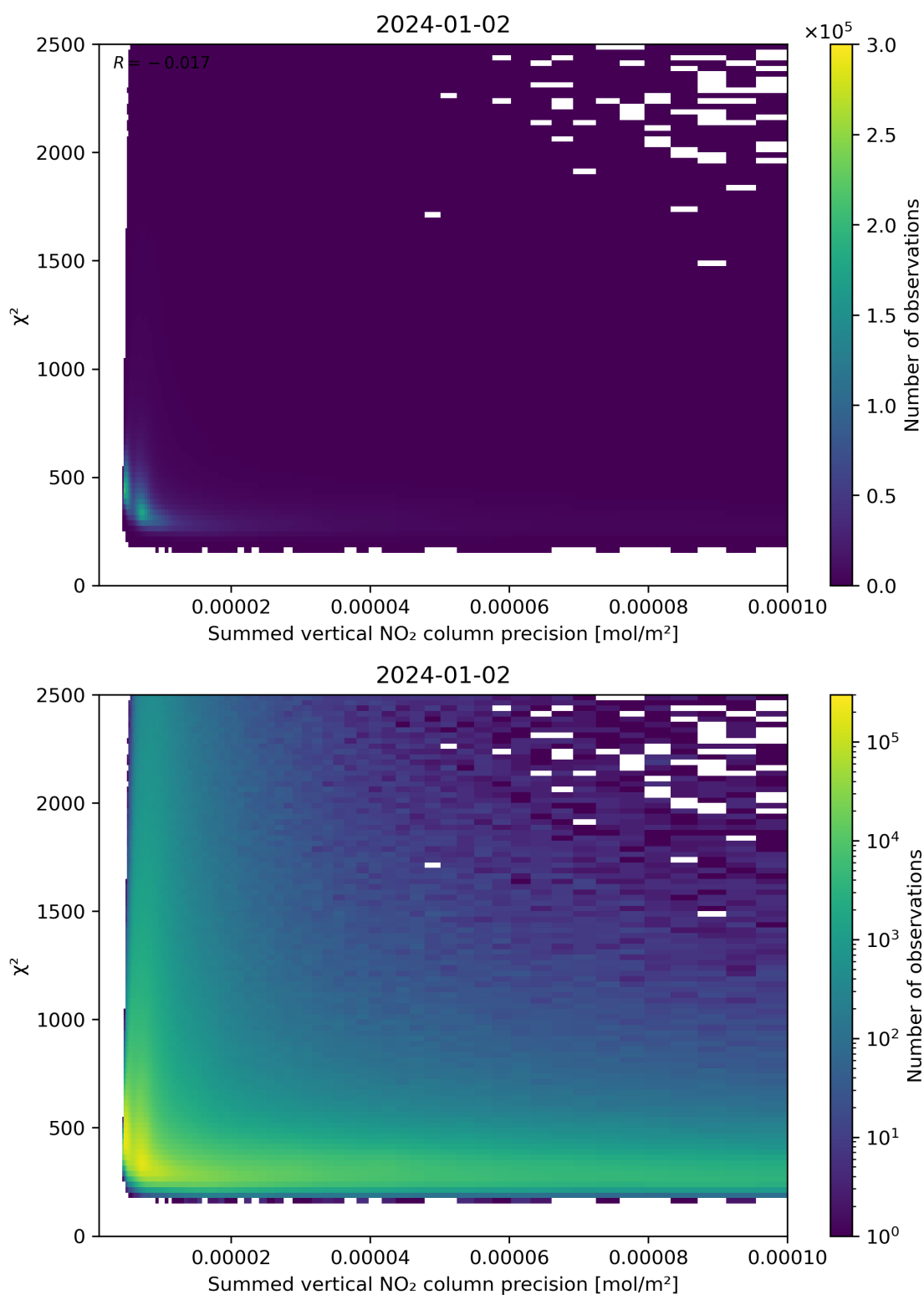
Figure 107: Scatter density plot of “Summed vertical NO 2 column precision” against “ \chi^2 ” for 2024-01-01 to 2024-01-03.
