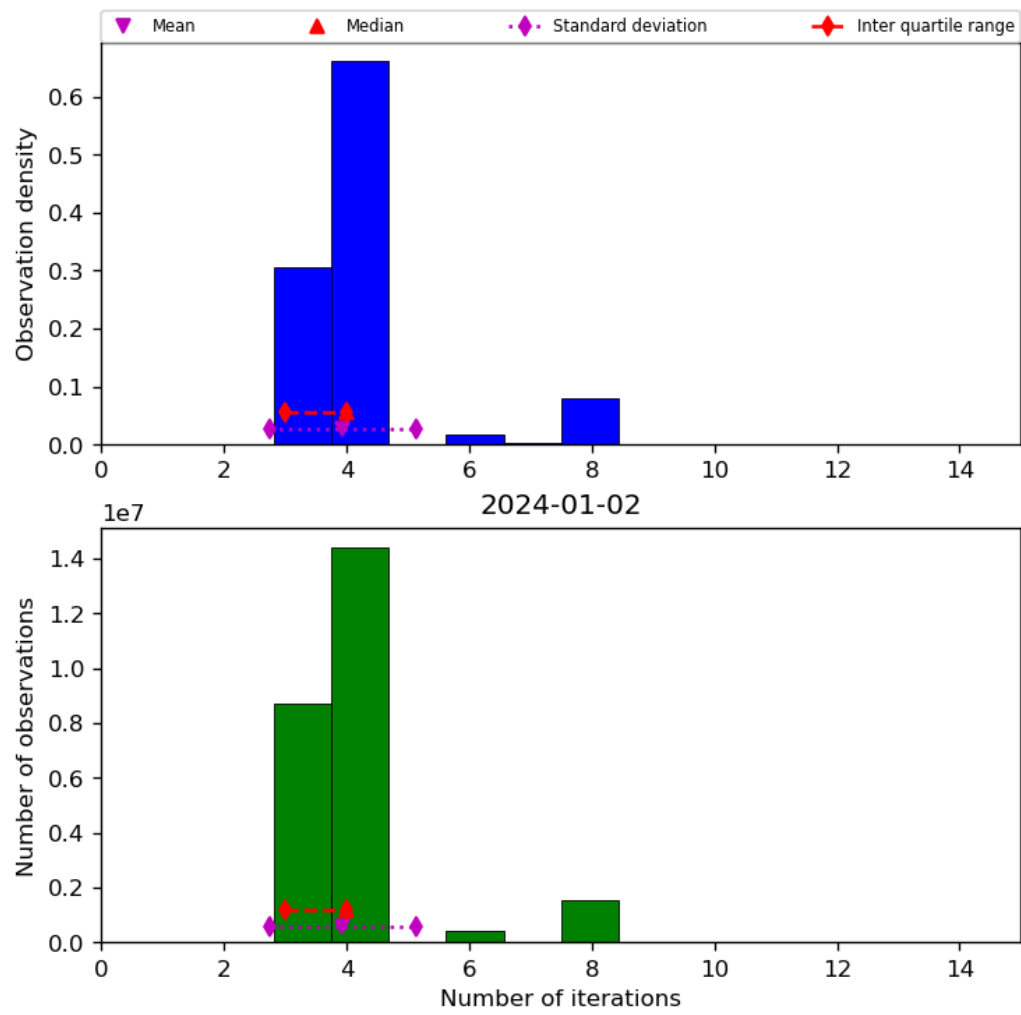
Figure 34: Histogram of “Number of iterations” for 2024-01-01 to 2024-01-03
