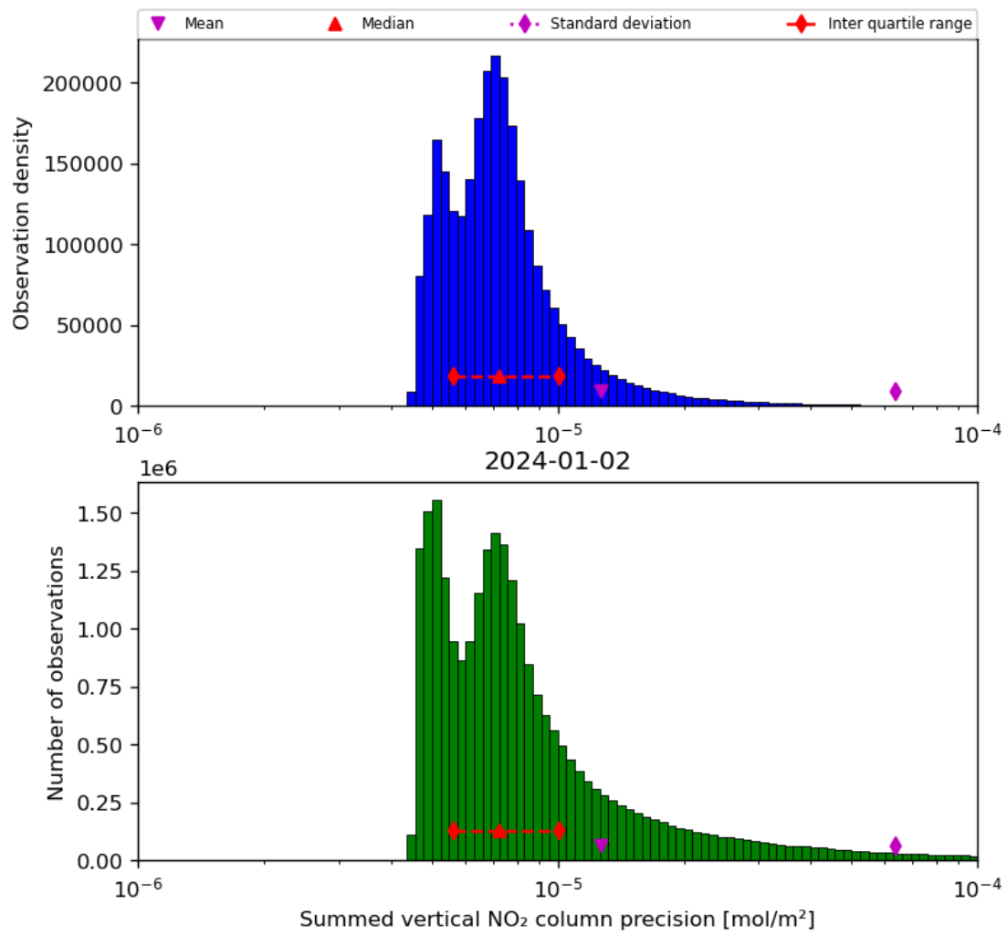
Figure 41: Histogram of “Summed vertical NO 2 column precision” for 2024-01-01 to 2024-01-03
