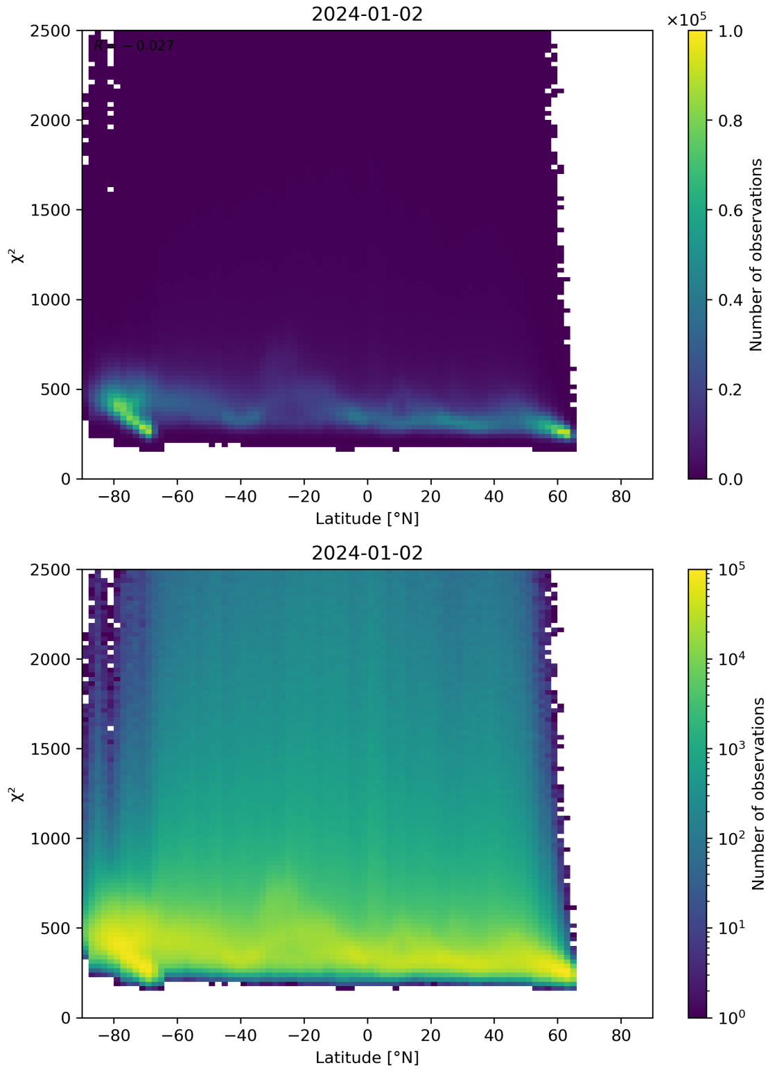
Figure 86: Scatter density plot of “Latitude” against “ \chi^2 ” for 2024-01-01 to 2024-01-03.
