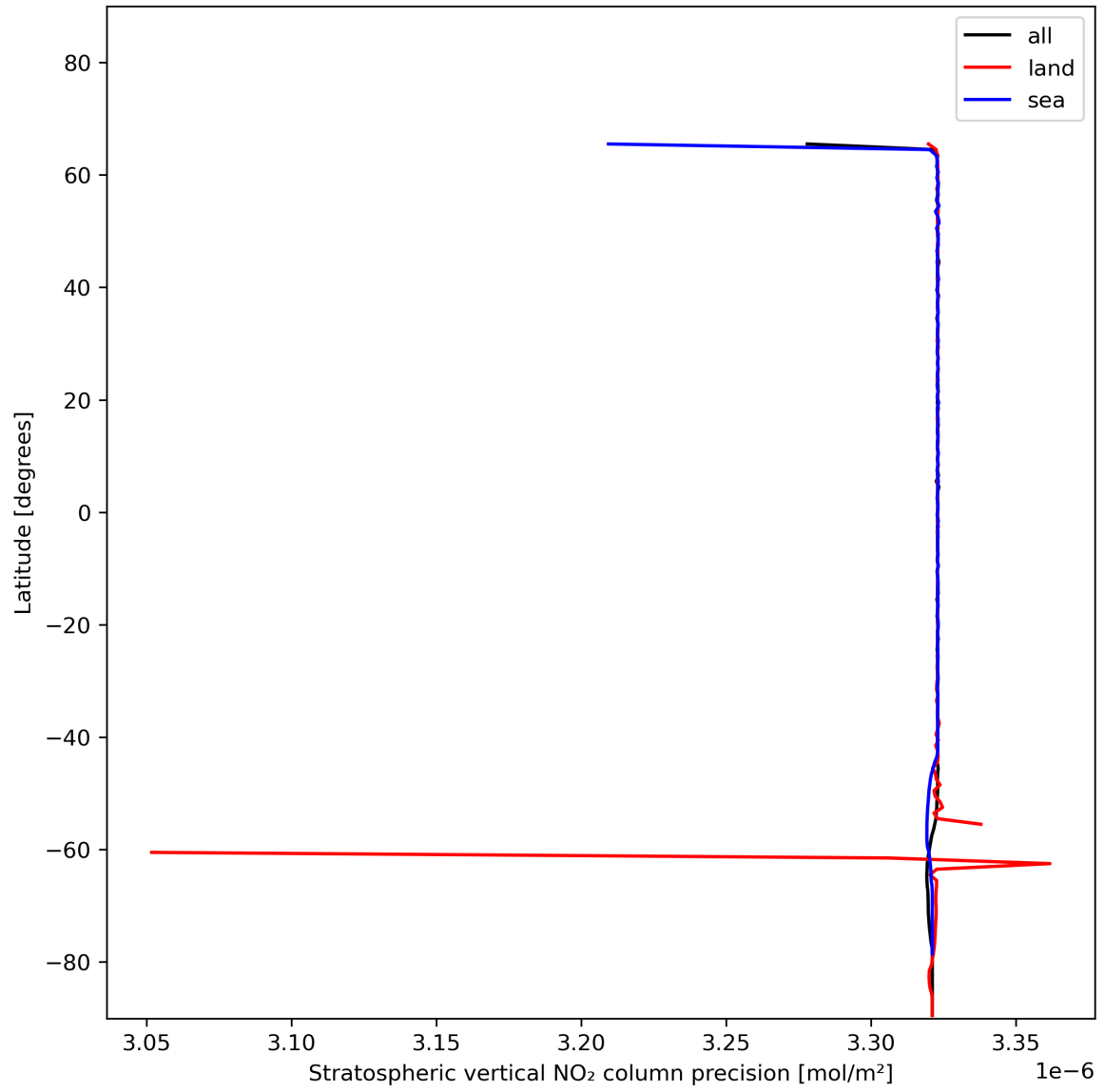
Figure 20: Zonal average of “Stratospheric vertical NO 2 column precision” for 2024-01-01 to 2024-01-03.
