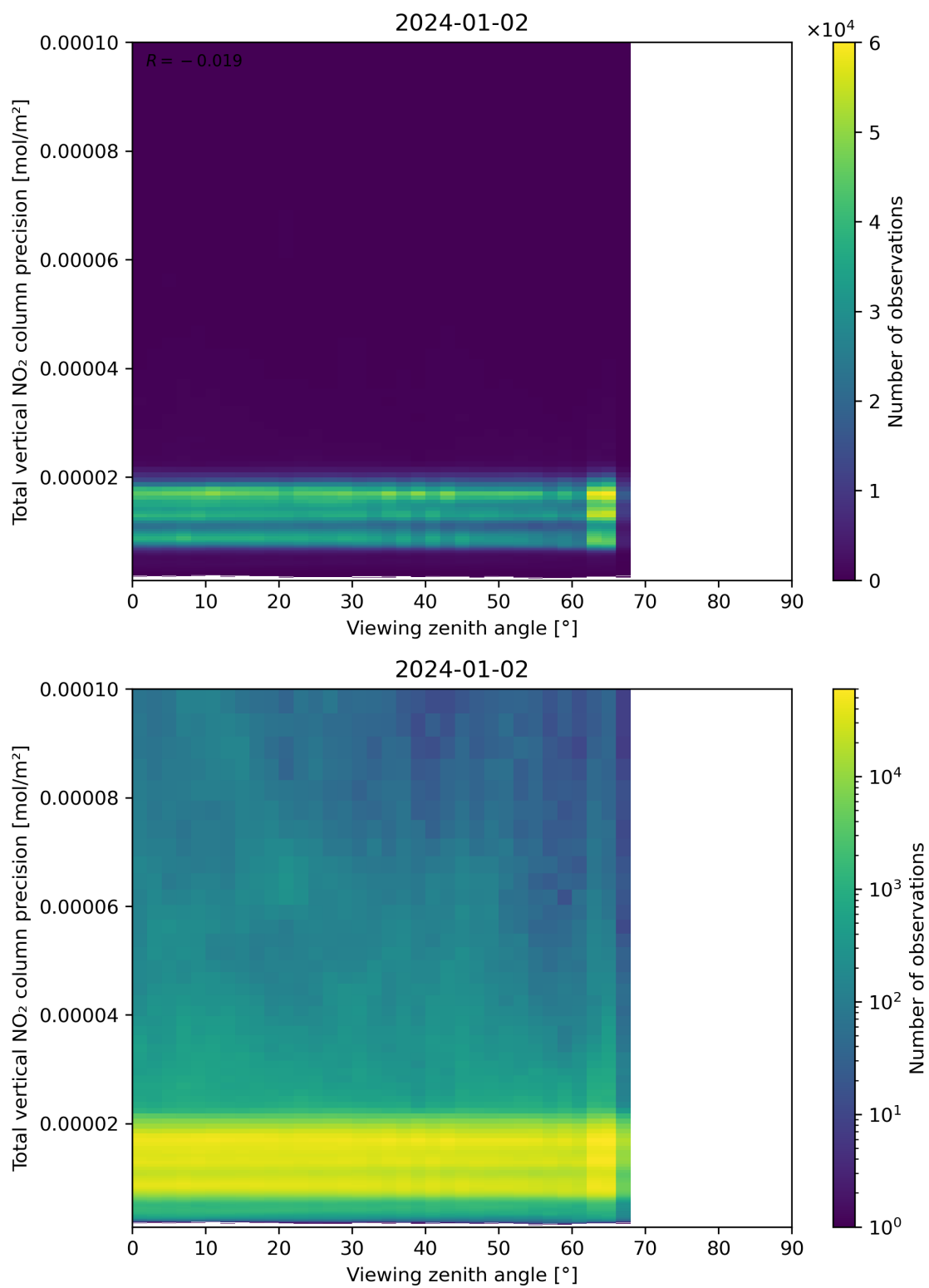
Figure 168: Scatter density plot of “Viewing zenith angle” against “Total vertical NO 2 column precision” for 2024-01-01 to 2024-01-03.
