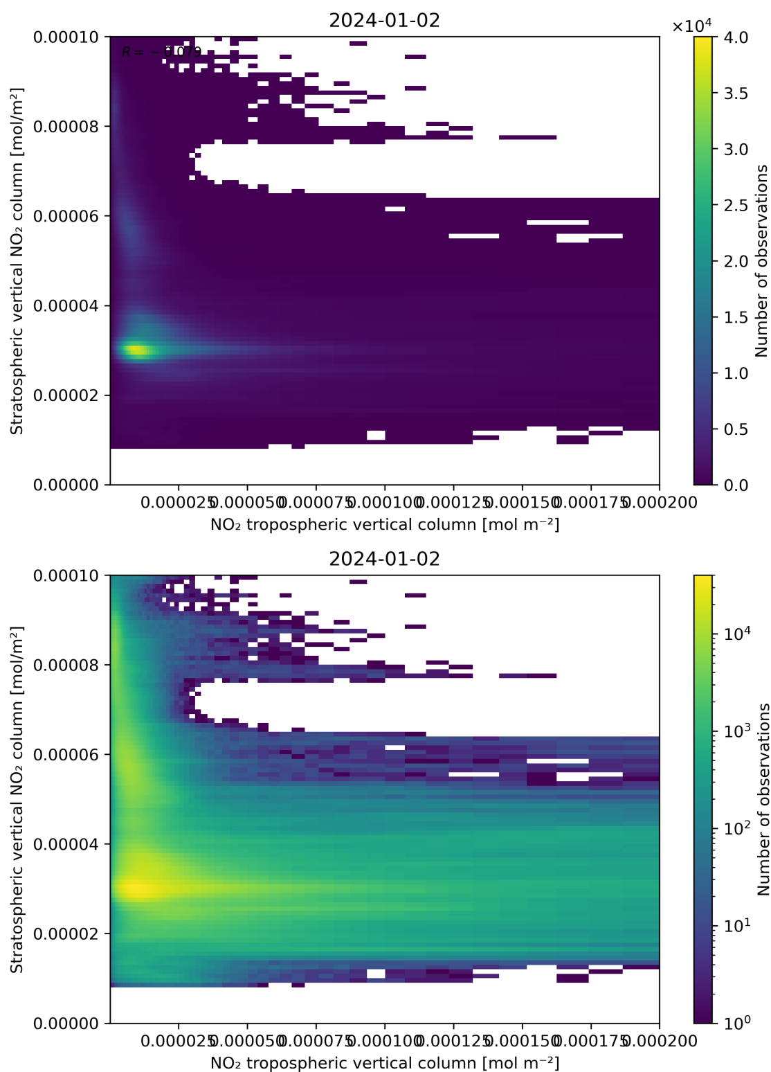
Figure 125: Scatter density plot of “NO 2 tropospheric vertical column” against “Stratospheric vertical NO 2 column” for 2024-01-01 to 2024-01-03.
