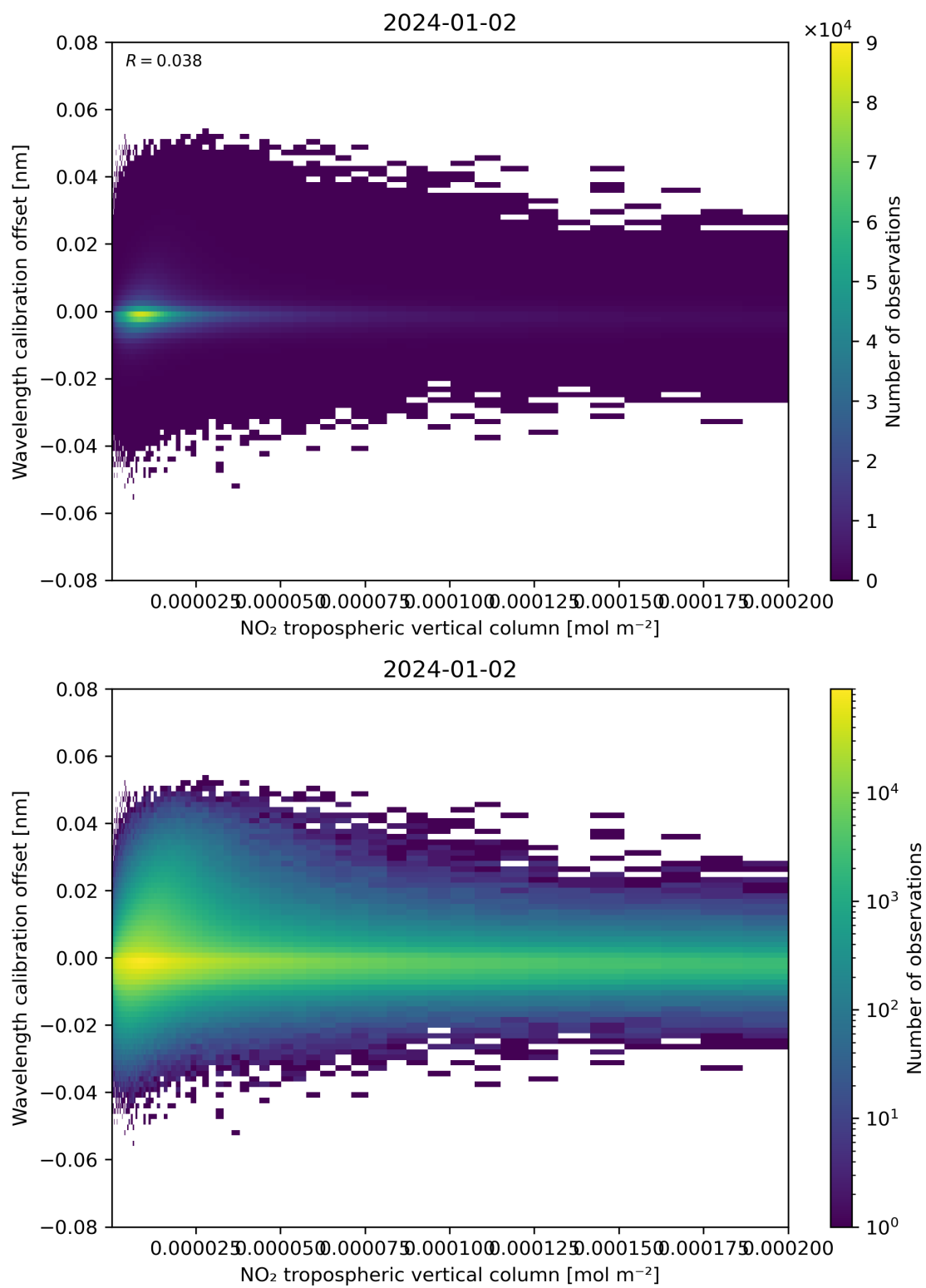
Figure 143: Scatter density plot of “NO 2 tropospheric vertical column” against “Wavelength calibration offset” for 2024-01-01 to 2024-01-03.
