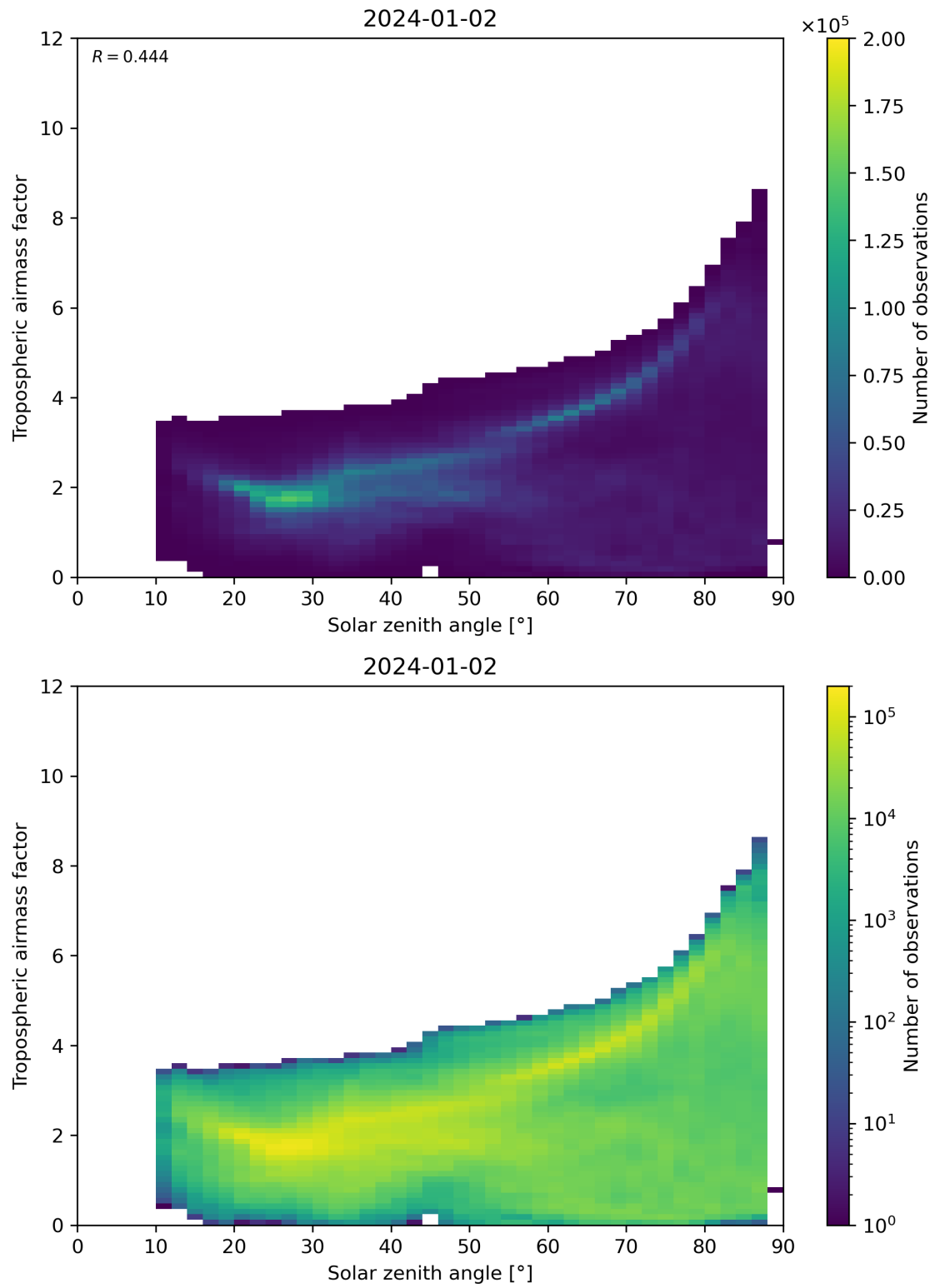
Figure 147: Scatter density plot of “Solar zenith angle” against “Tropospheric airmass factor” for 2024-01-01 to 2024-01-03.
