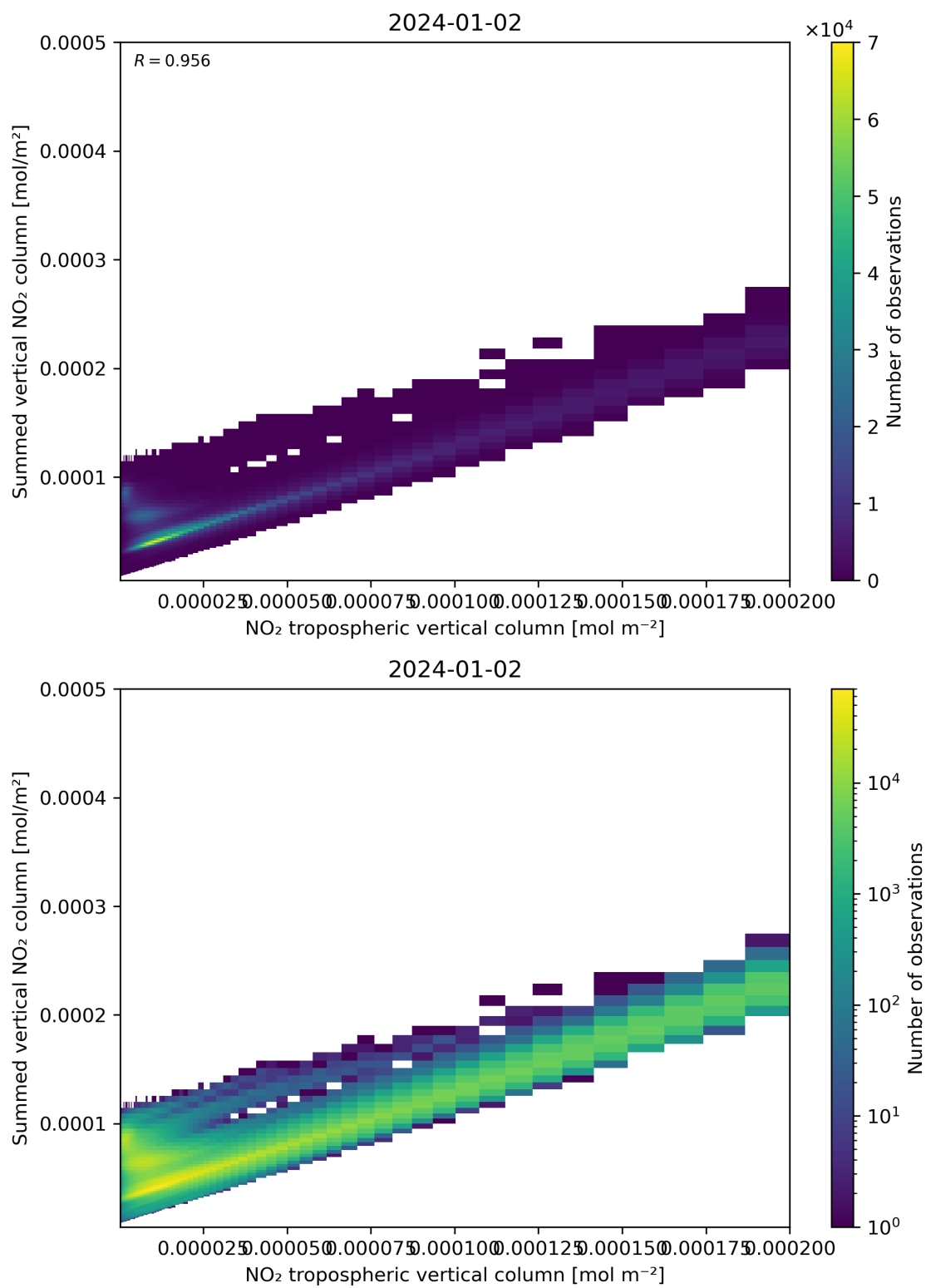
Figure 126: Scatter density plot of “NO 2 tropospheric vertical column” against “Summed vertical NO 2 column” for 2024-01-01 to 2024-01-03.
