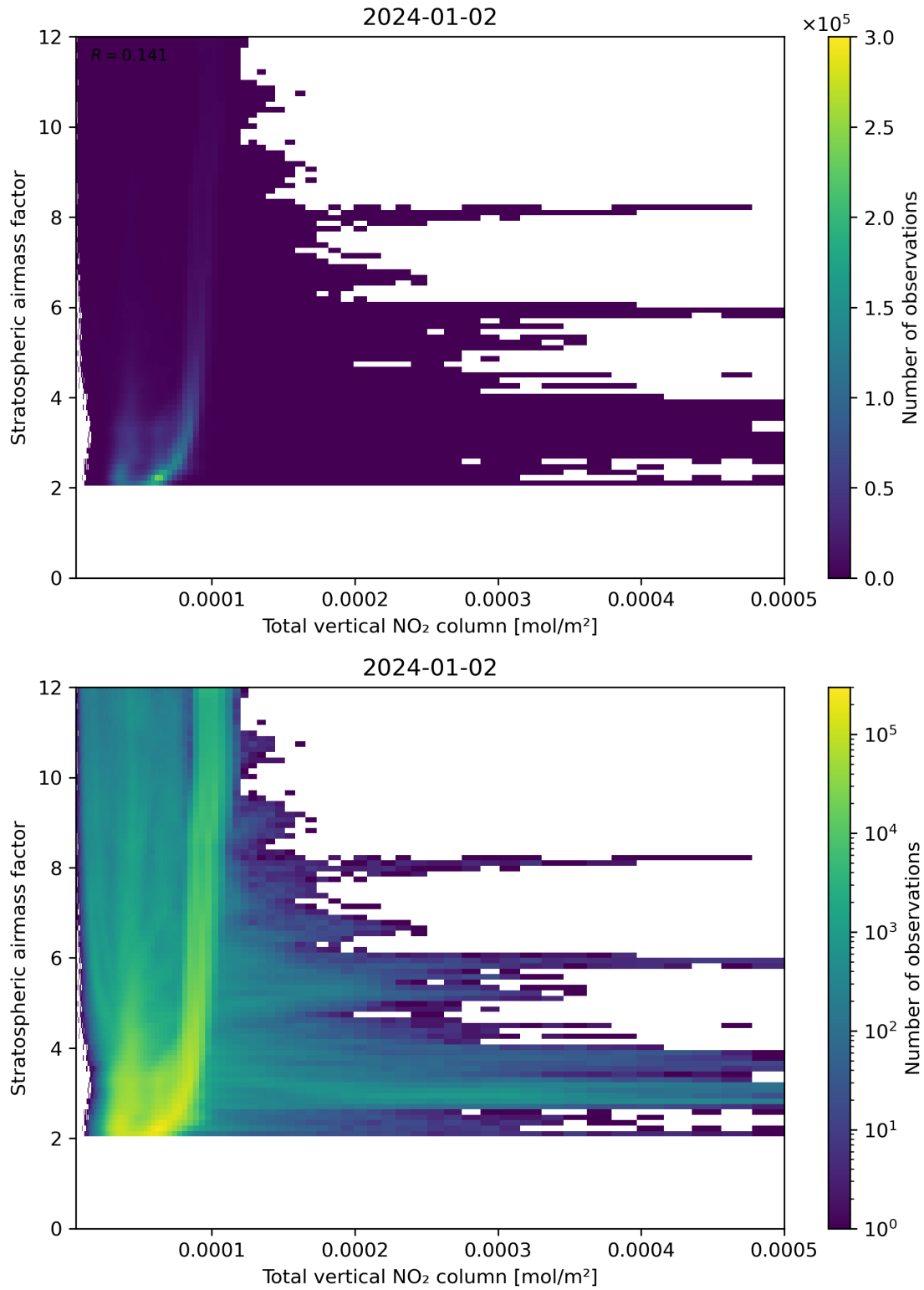
Figure 110: Scatter density plot of “Total vertical NO 2 column” against “Stratospheric airmass factor” for 2024-01-01 to 2024-01-03.
