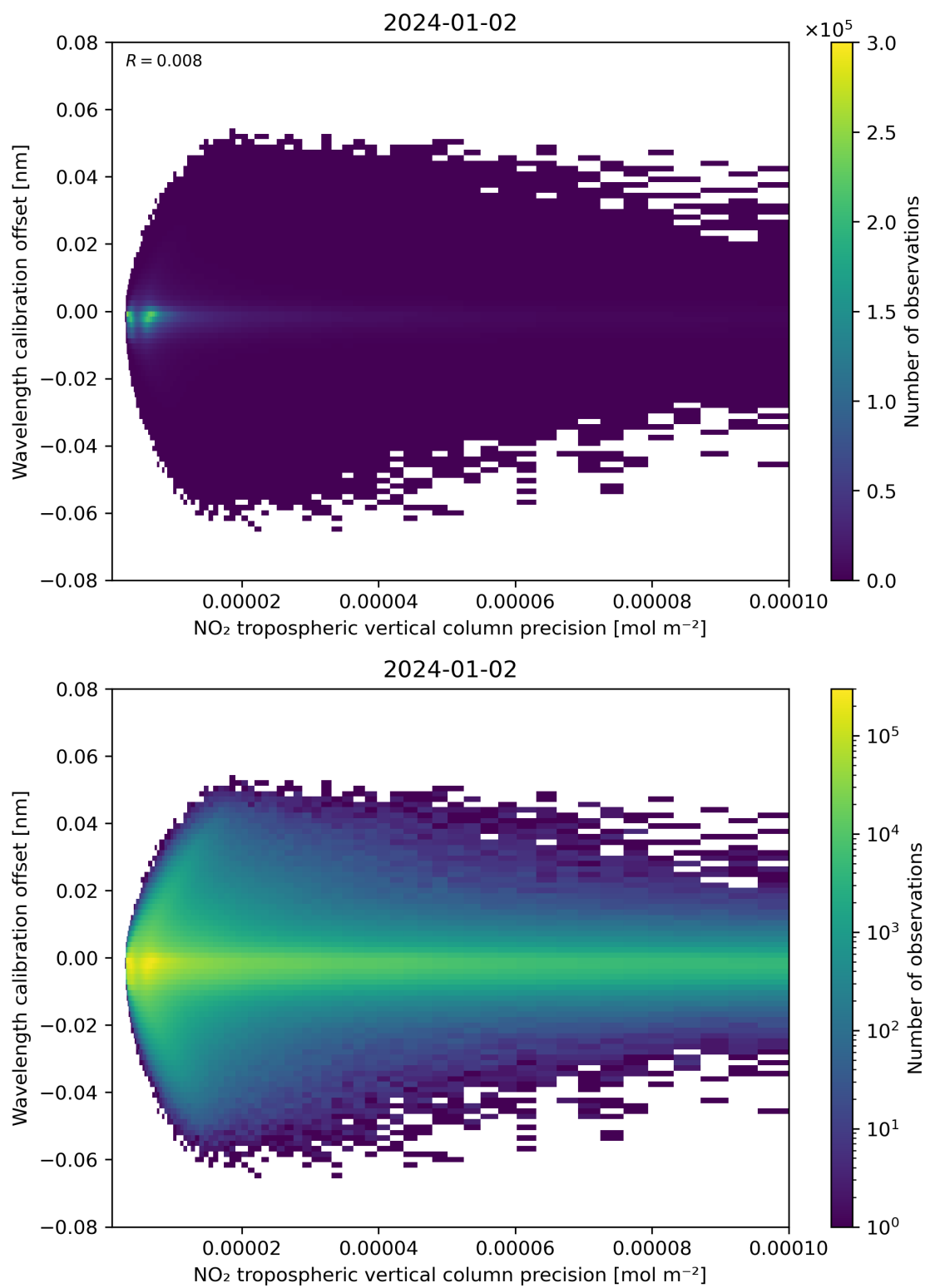
Figure 141: Scatter density plot of “NO 2 tropospheric vertical column precision” against “Wavelength calibration offset” for 2024-01-01 to 2024-01-03.
