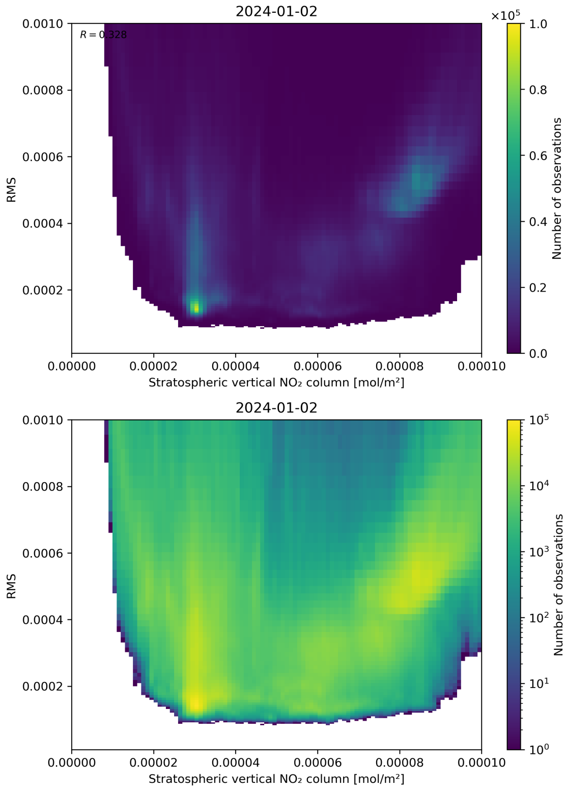
Figure 102: Scatter density plot of “Stratospheric vertical NO 2 column” against “RMS” for 2024-01-01 to 2024-01-03.
