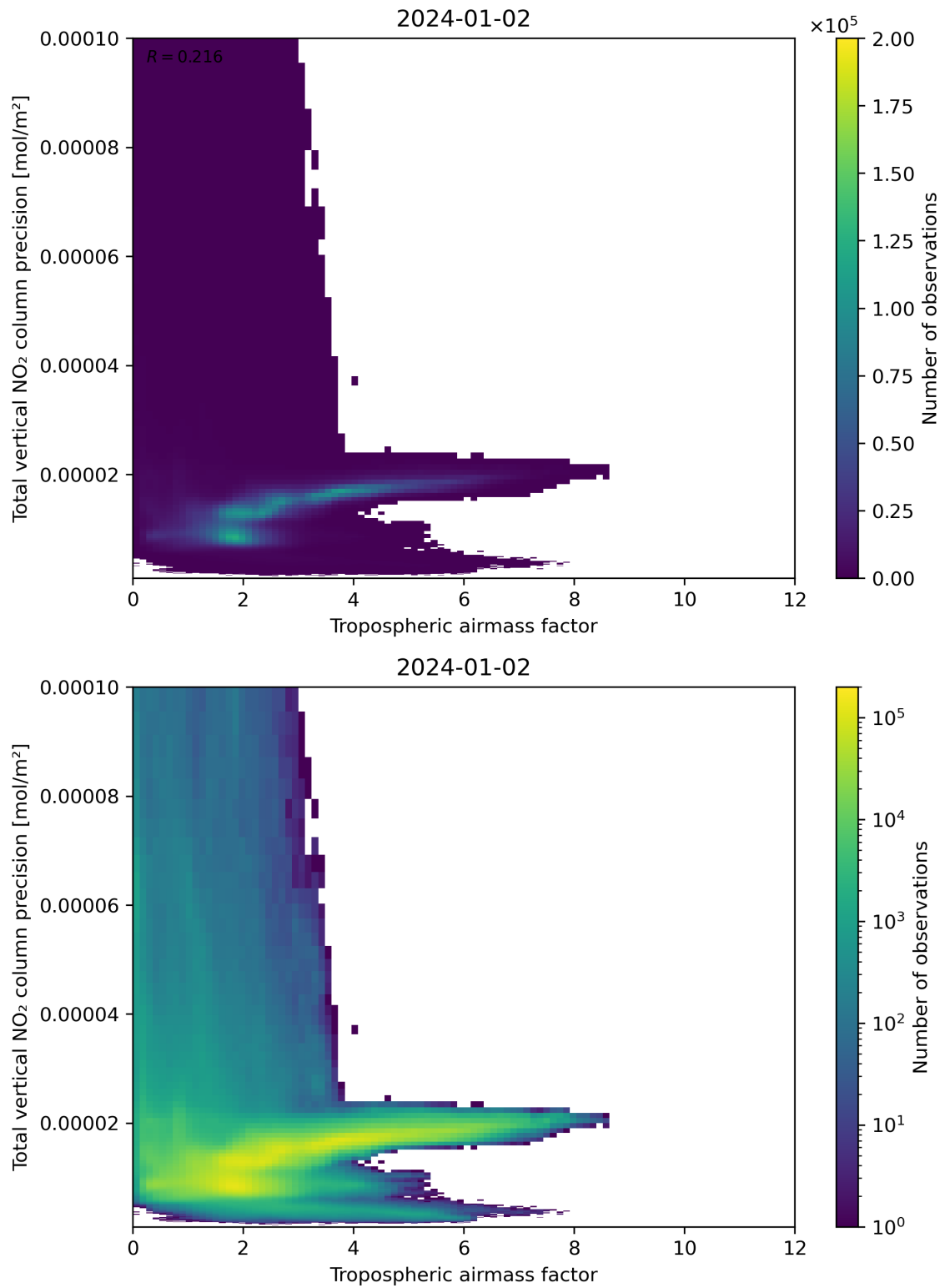
Figure 78: Scatter density plot of “Tropospheric air mass factor” against “Total vertical NO 2 column precision” for 2024-01-01 to 2024-01-03.
