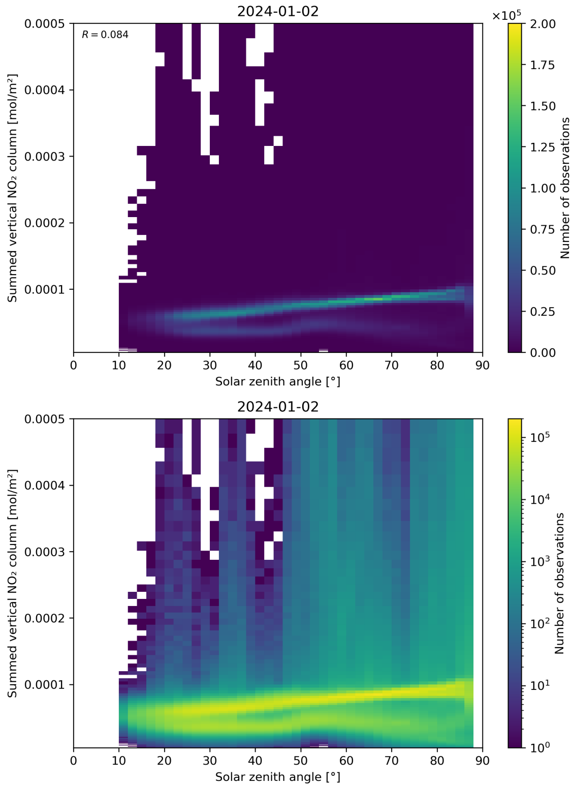
Figure 151: Scatter density plot of “Solar zenith angle” against “Summed vertical NO 2 column” for 2024-01-01 to 2024-01-03.
