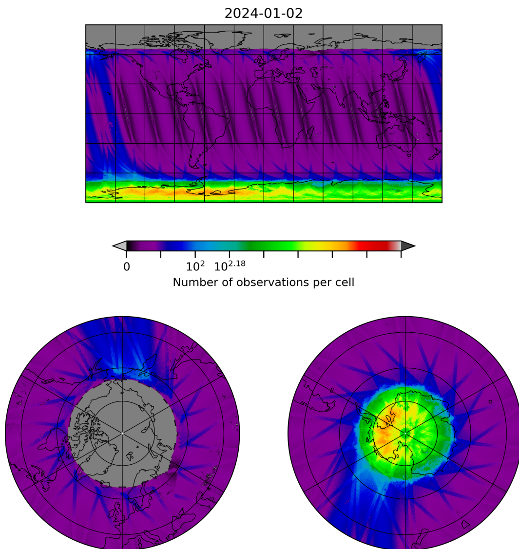
Figure 10: Map of the number of observations for 2024-01-01 to 2024-01-03
