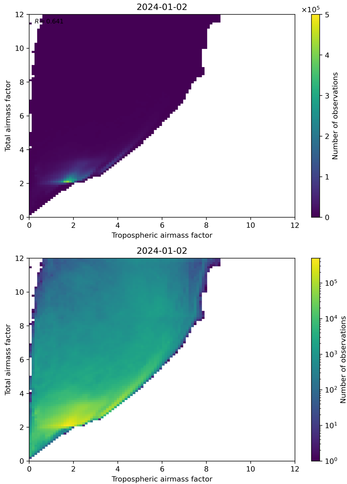
Figure 72: Scatter density plot of “Tropospheric airmass factor” against “Total airmass factor” for 2024-01-01 to 2024-01-03.
