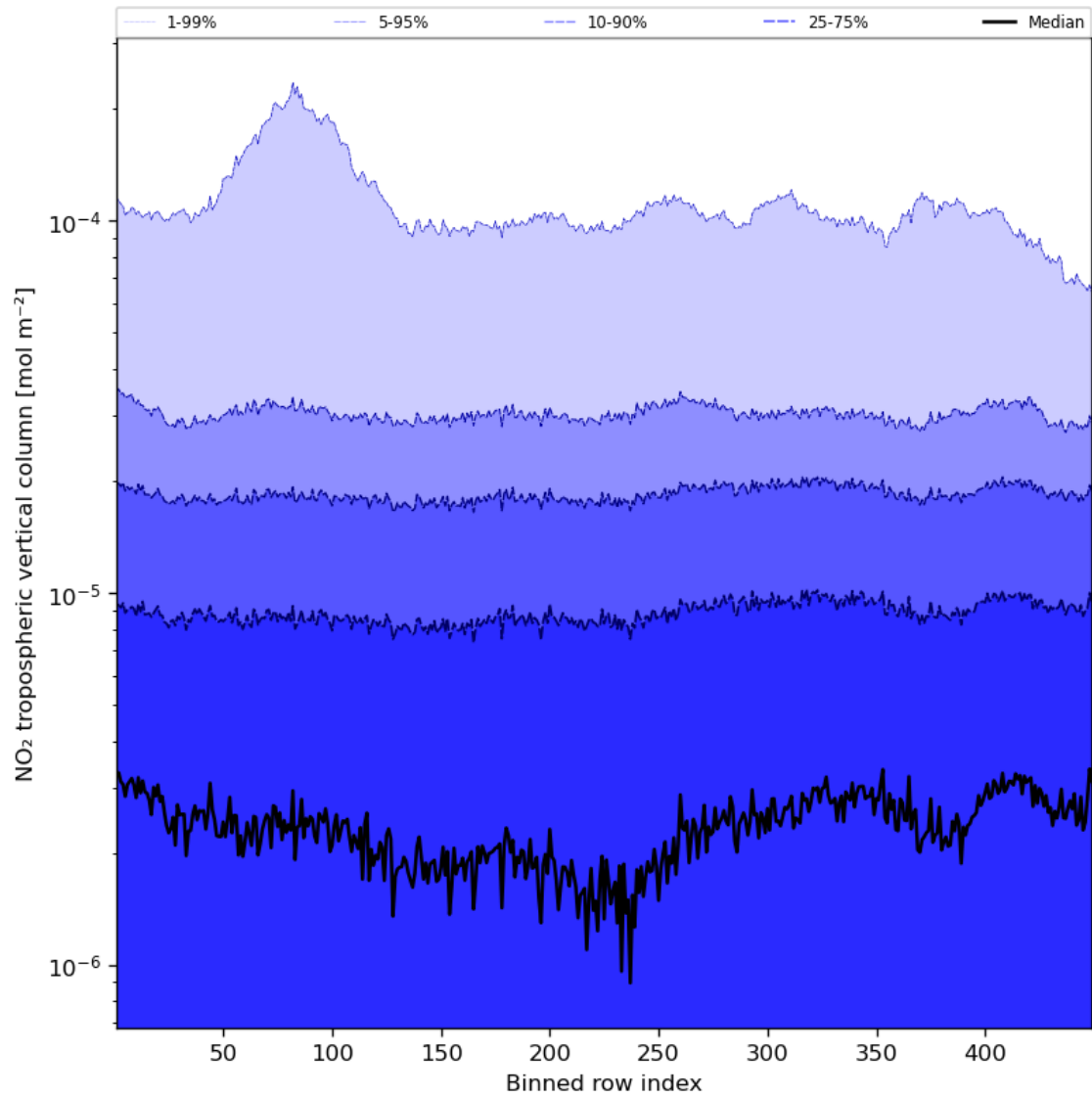
Figure 46: Along track statistics of “NO 2 tropospheric vertical column” for 2024-01-01 to 2024-01-03
