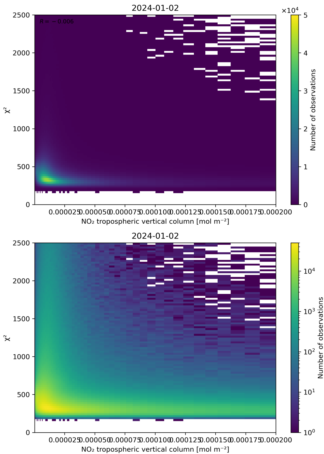
Figure 124: Scatter density plot of “NO 2 tropospheric vertical column” against “ \chi^2 ” for 2024-01-01 to 2024-01-03.
