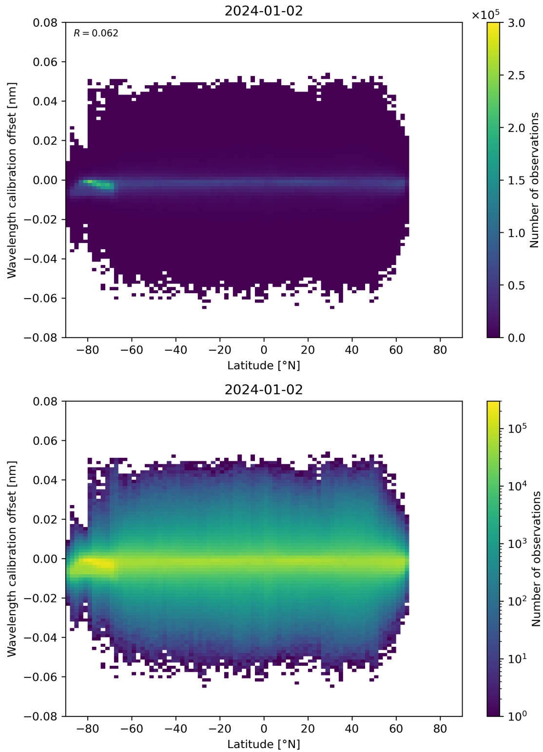
Figure 95: Scatter density plot of “Latitude” against “Wavelength calibration offset” for 2024-01-01 to 2024-01-03.
