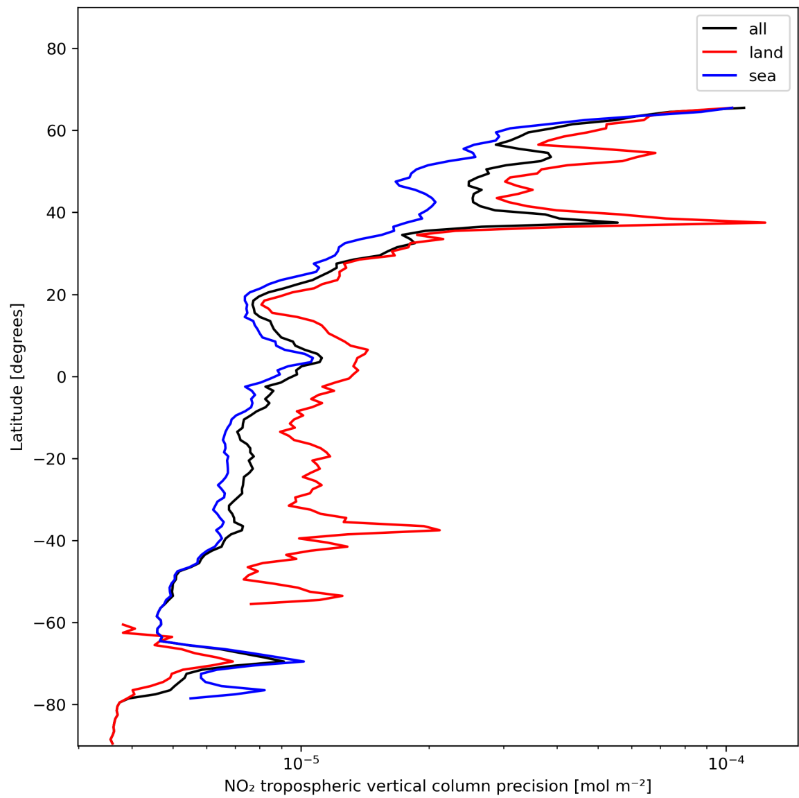
Figure 13: Zonal average of “NO 2 tropospheric vertical column precision” for 2024-01-01 to 2024-01-03.
