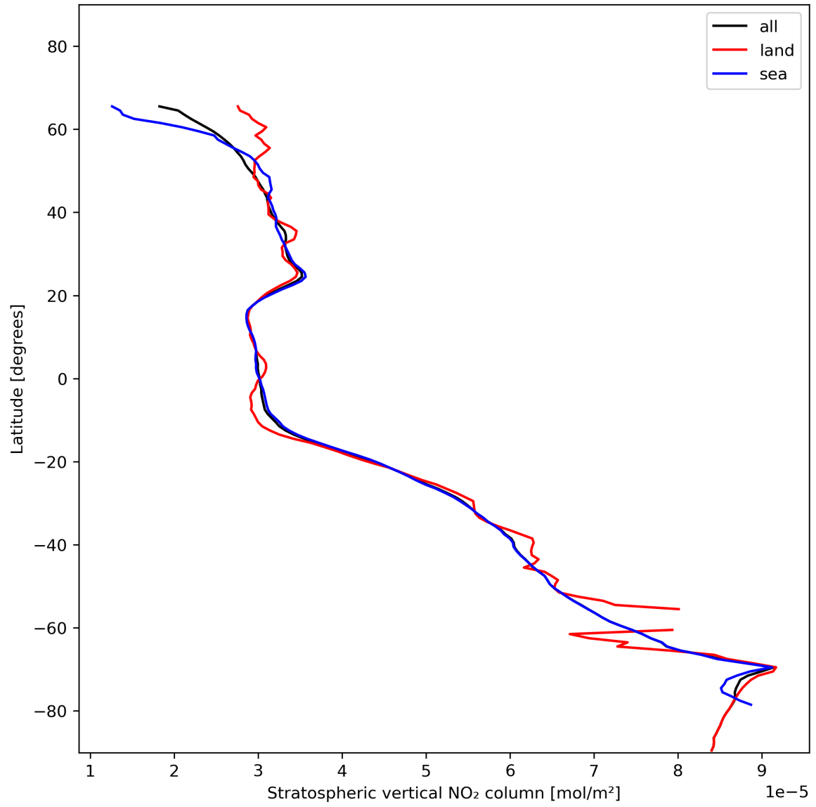
Figure 19: Zonal average of “Stratospheric vertical NO 2 column” for 2024-01-01 to 2024-01-03.
