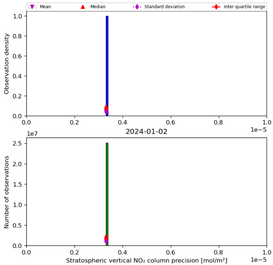
Figure 37: Histogram of “Stratospheric vertical NO 2 column precision” for 2024-01-01 to 2024-01-03
