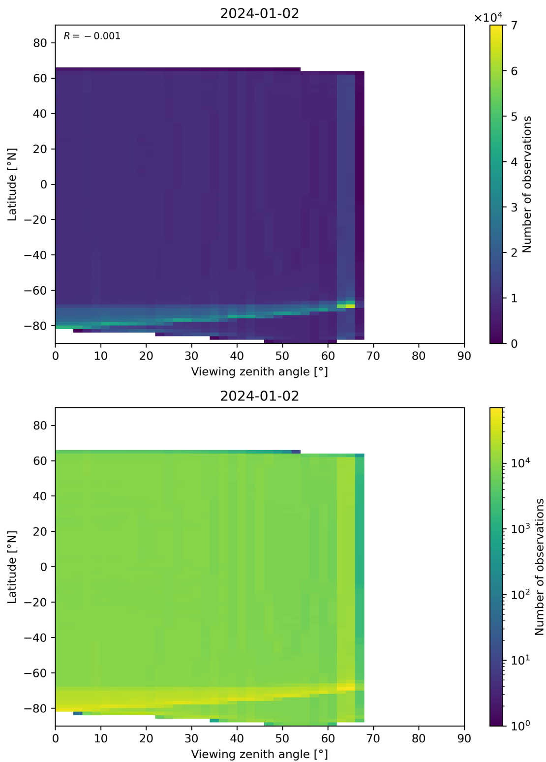
Figure 163: Scatter density plot of “Viewing zenith angle” against “Latitude” for 2024-01-01 to 2024-01-03.
