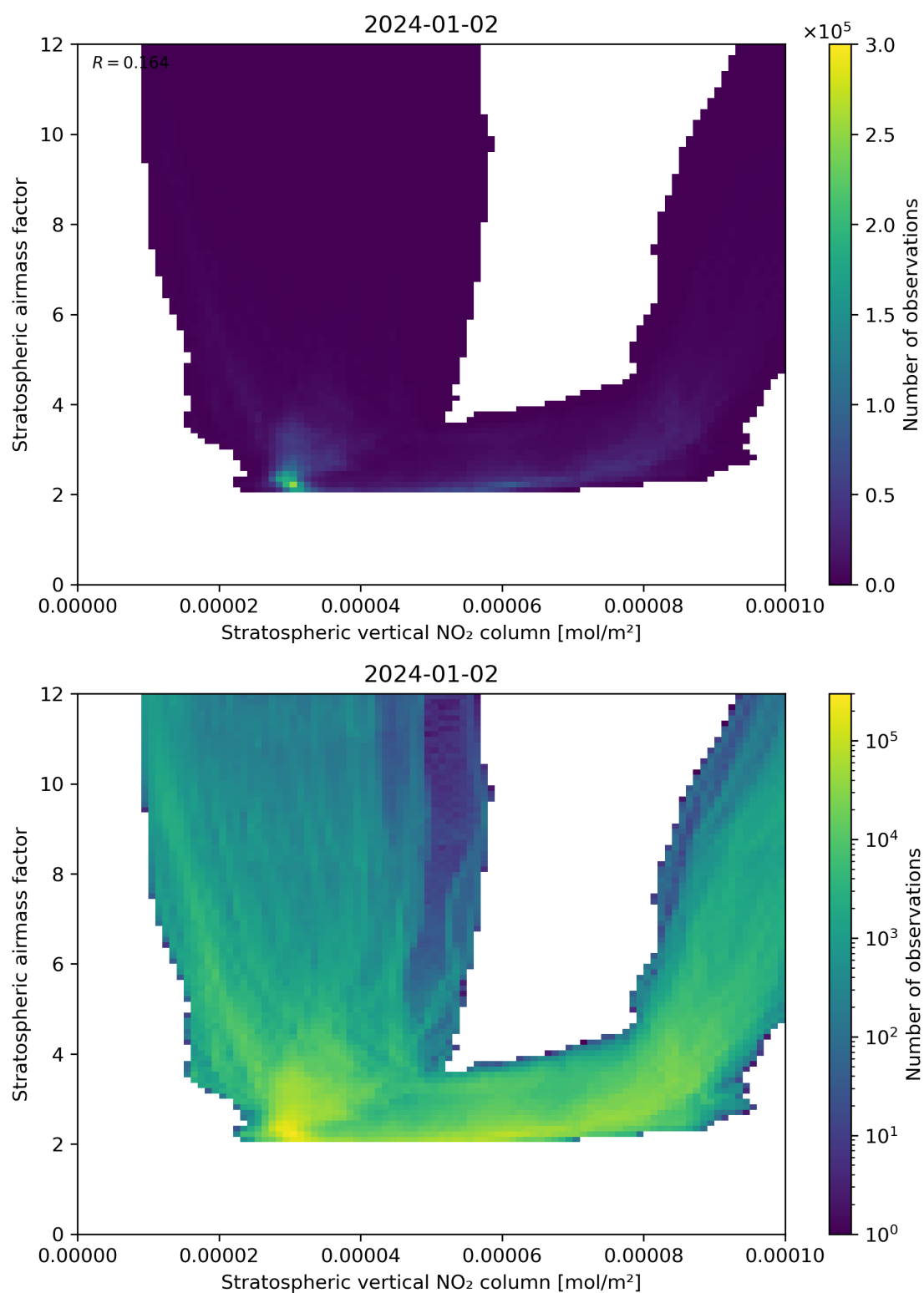
Figure 96: Scatter density plot of “Stratospheric vertical NO 2 column” against “Stratospheric airmass factor” for 2024-01-01 to 2024-01-03.
