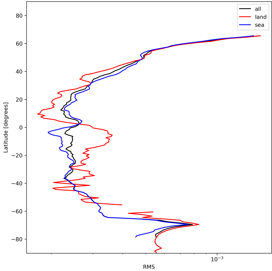
Figure 26: Zonal average of “RMS” for 2024-01-01 to 2024-01-03.
