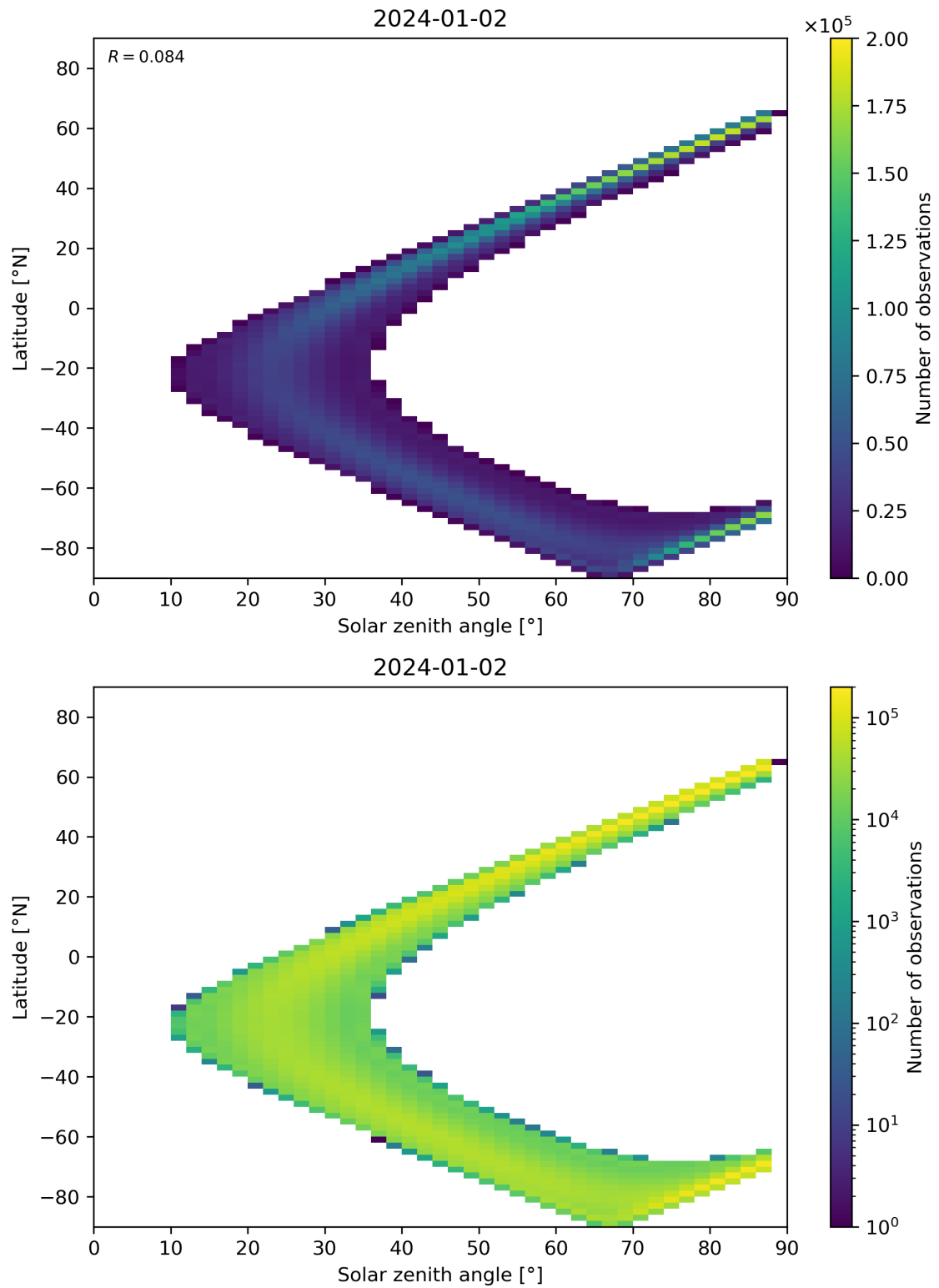
Figure 149: Scatter density plot of “Solar zenith angle” against “Latitude” for 2024-01-01 to 2024-01-03.
