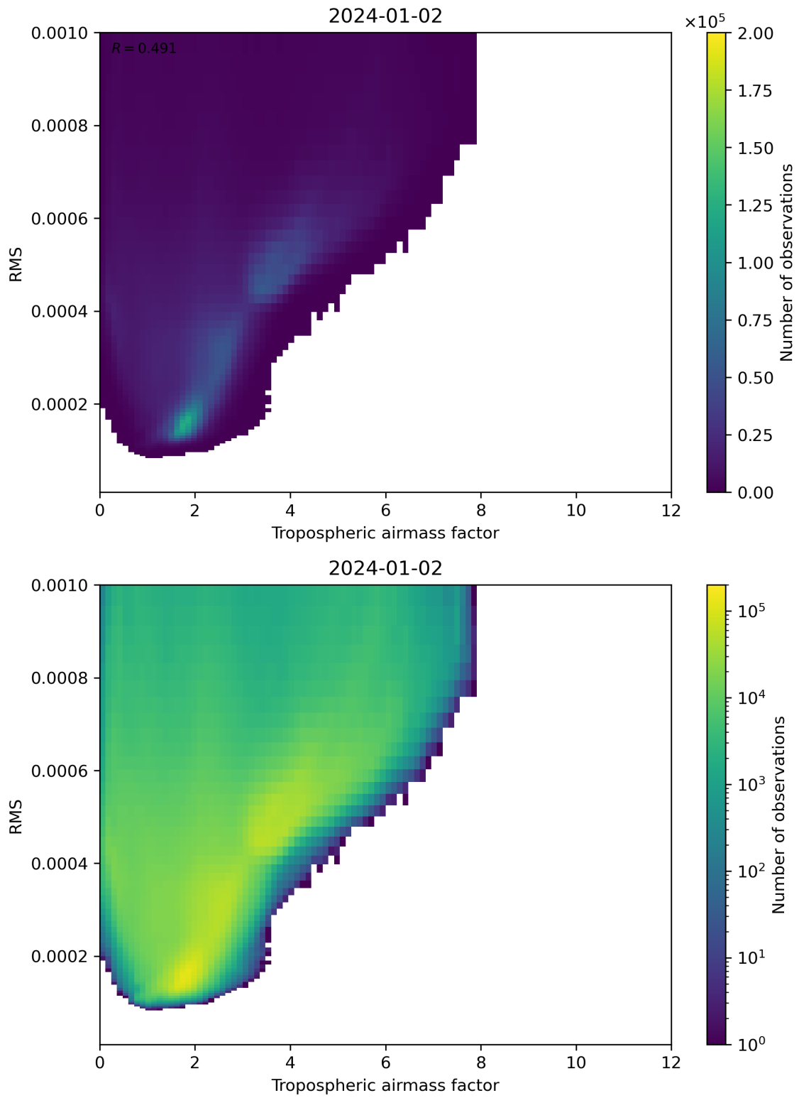
Figure 79: Scatter density plot of “Tropospheric airmass factor” against “RMS” for 2024-01-01 to 2024-01-03.
