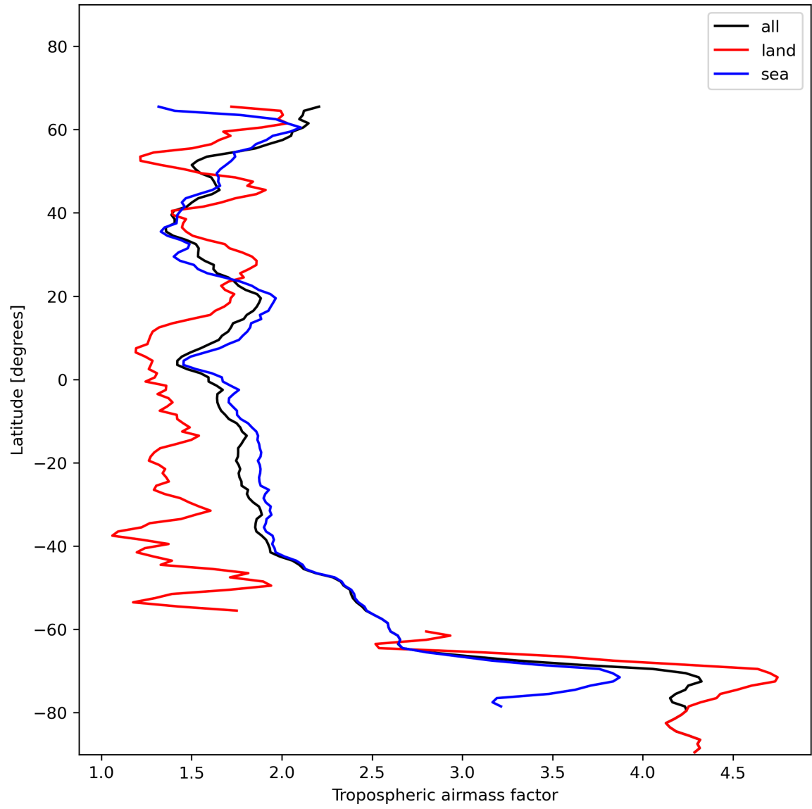
Figure 14: Zonal average of “Tropospheric airmass factor” for 2024-01-01 to 2024-01-03.
