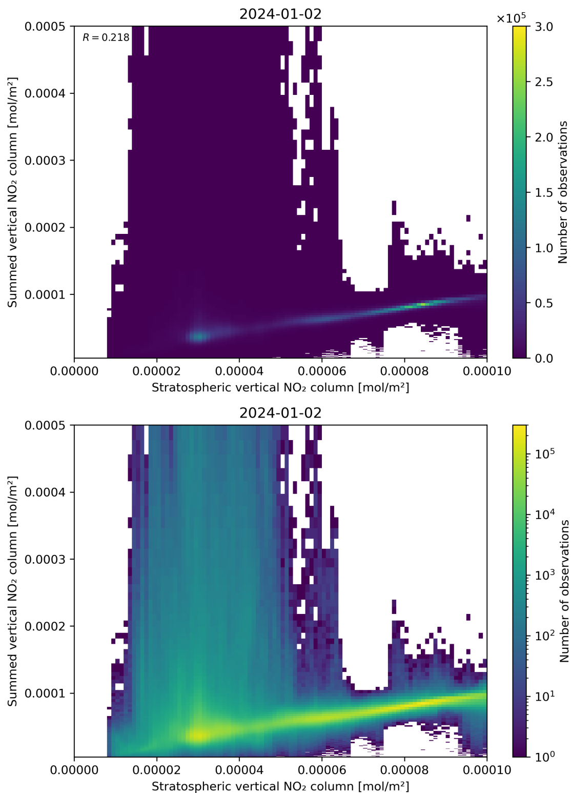
Figure 98: Scatter density plot of “Stratospheric vertical NO 2 column” against “Summed vertical NO 2 column” for 2024-01-01 to 2024-01-03.
