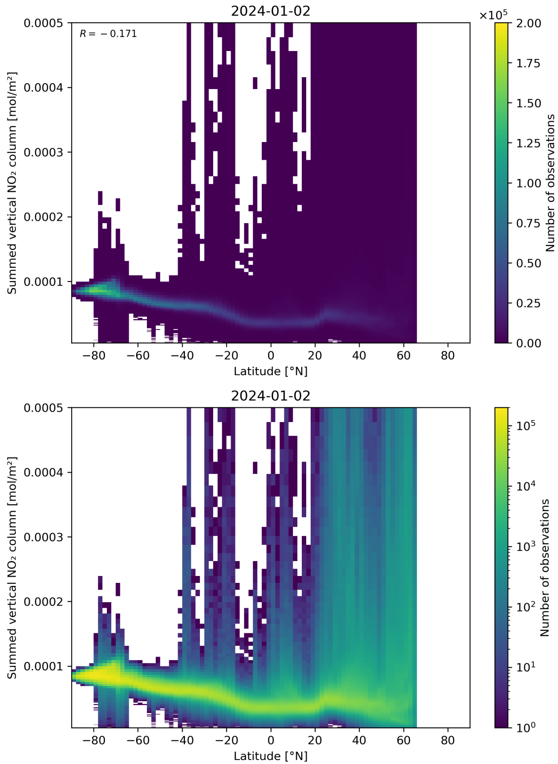
Figure 88: Scatter density plot of “Latitude” against “Summed vertical NO 2 column” for 2024-01-01 to 2024-01-03.
