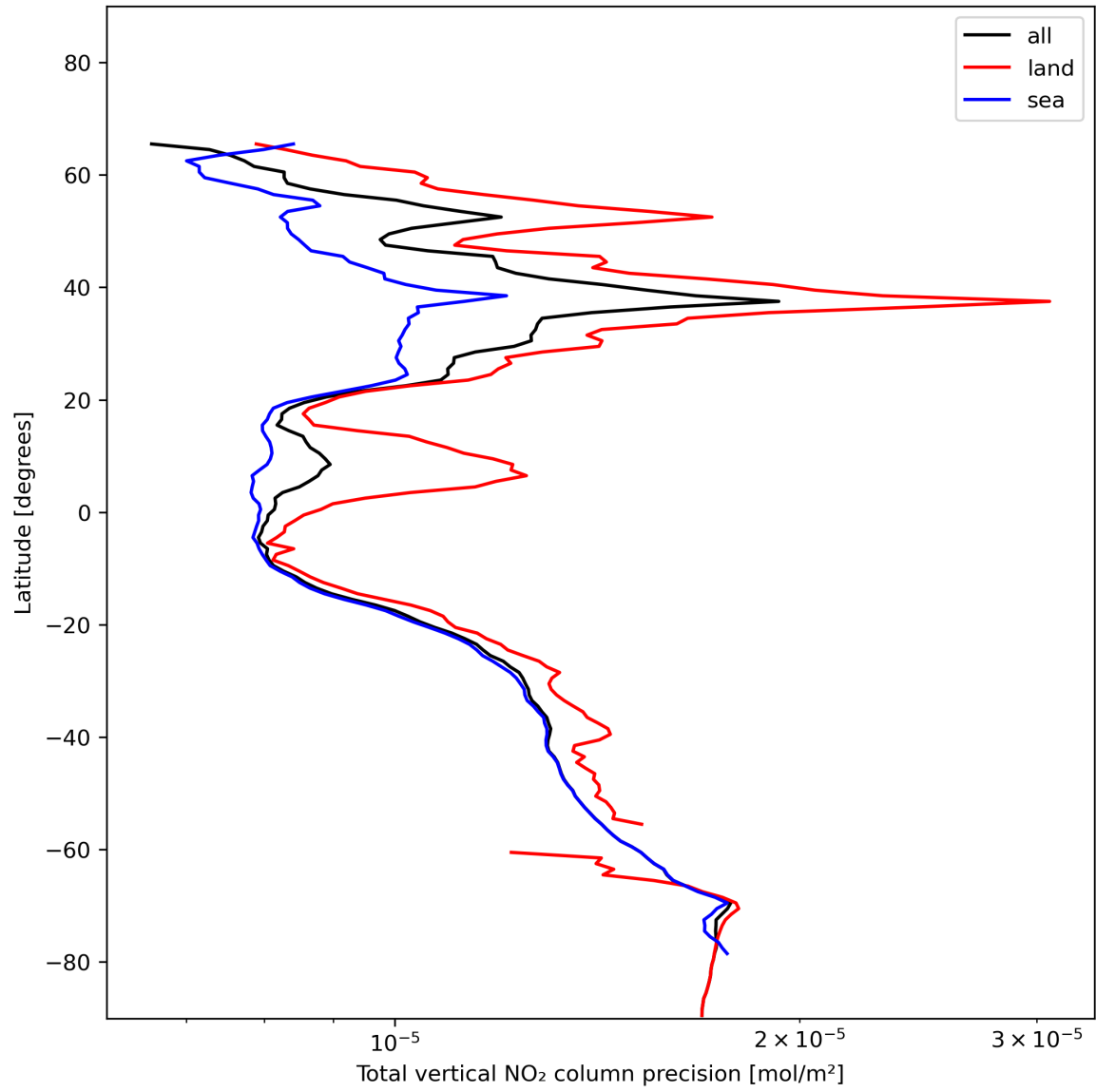
Figure 22: Zonal average of “Total vertical NO 2 column precision” for 2024-01-01 to 2024-01-03.
