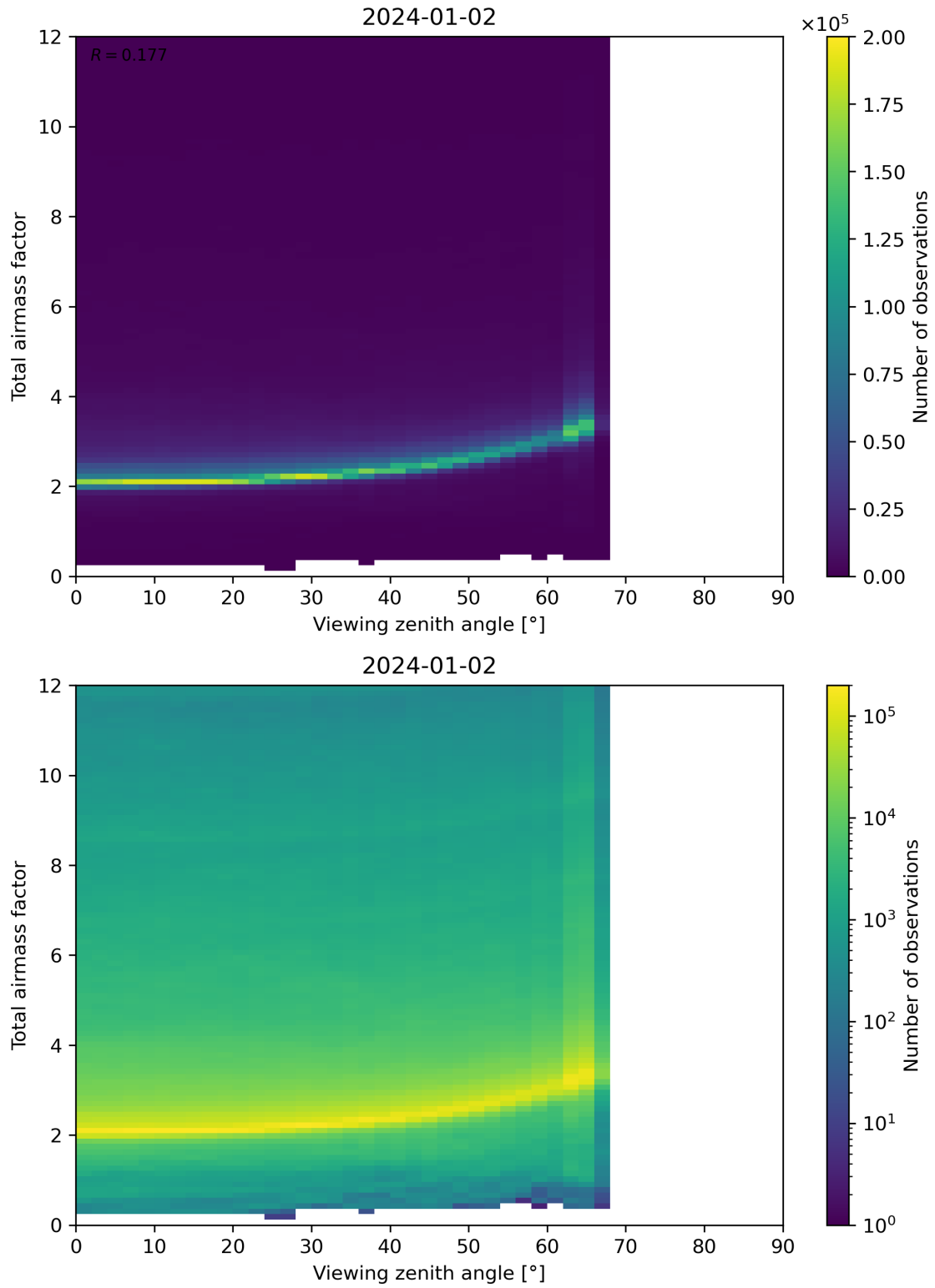
Figure 160: Scatter density plot of “Viewing zenith angle” against “Total airmass factor” for 2024-01-01 to 2024-01-03.
