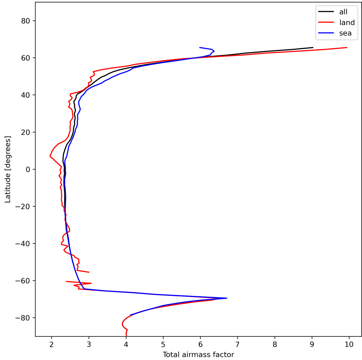
Figure 15: Zonal average of “Total airmass factor” for 2024-01-01 to 2024-01-03.
