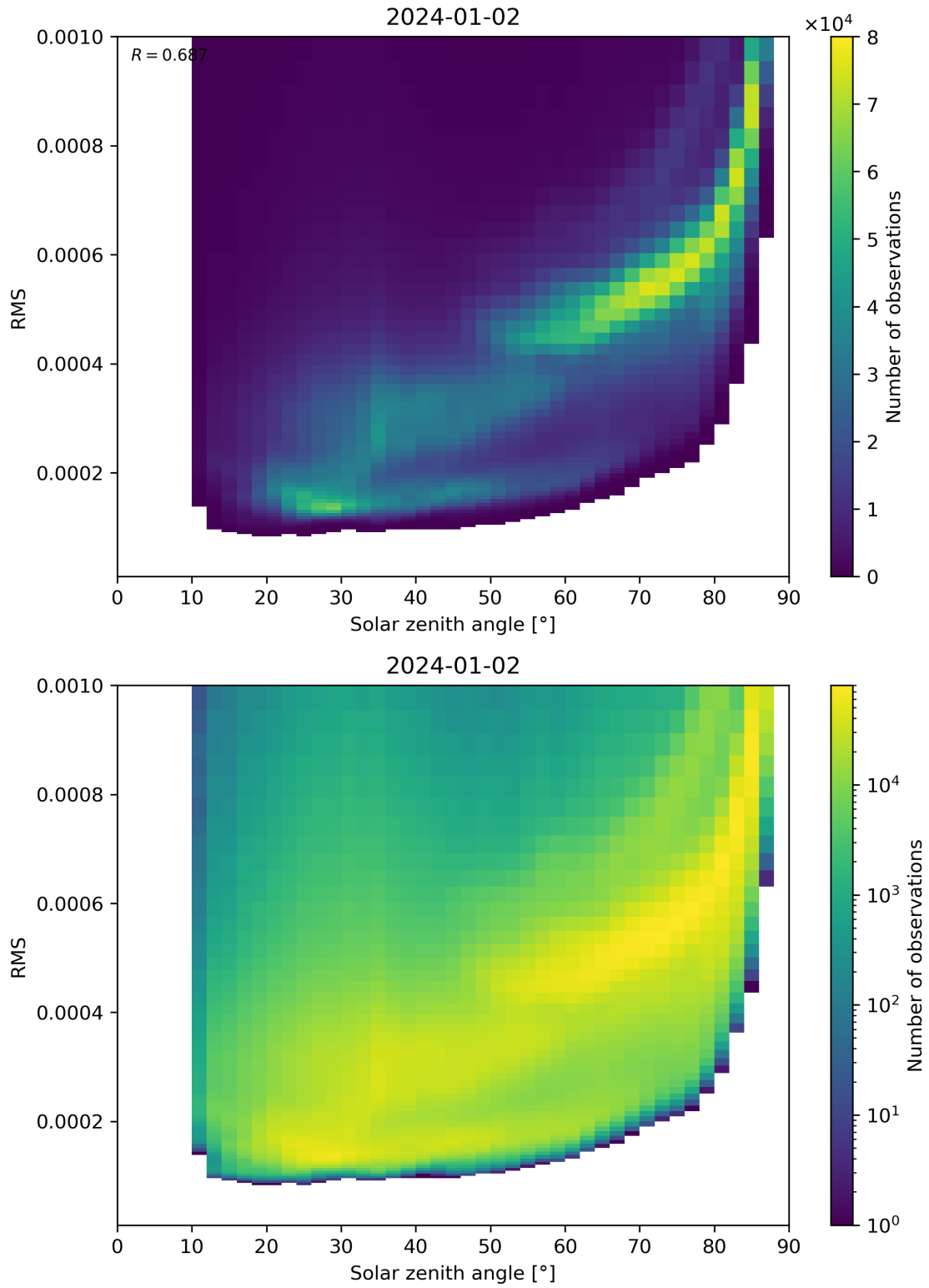
Figure 157: Scatter density plot of “Solar zenith angle” against “RMS” for 2024-01-01 to 2024-01-03.
