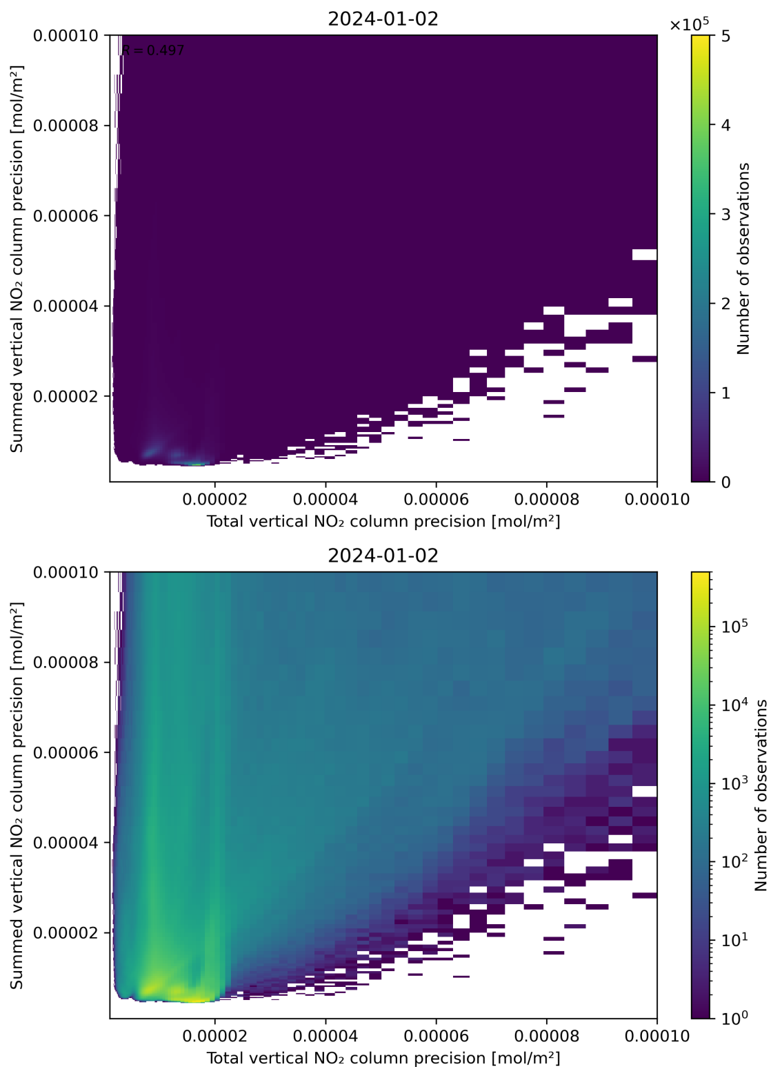
Figure 118: Scatter density plot of “Total vertical NO 2 column precision” against “Summed vertical NO 2 column precision” for 2024-01-01 to 2024-01-03.
