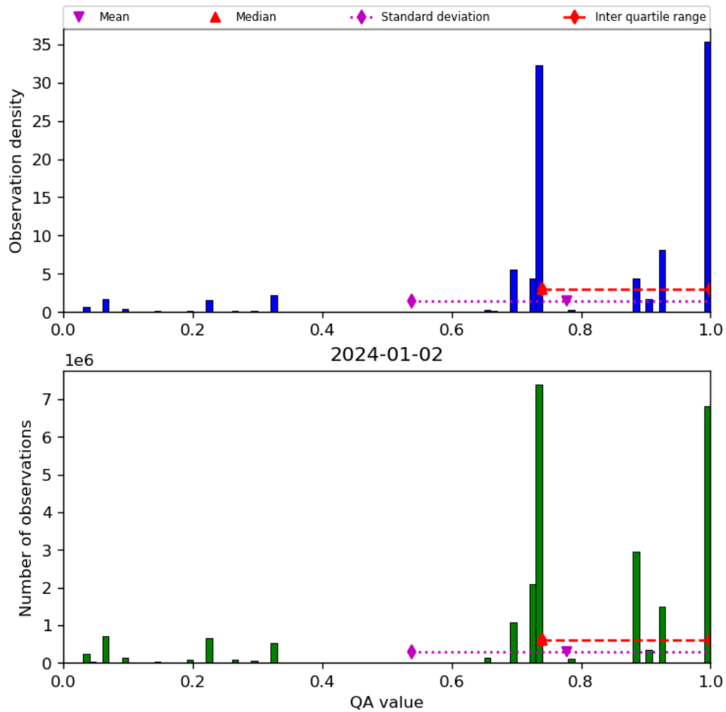
Figure 28: Histogram of “QA value” for 2024-01-01 to 2024-01-03
