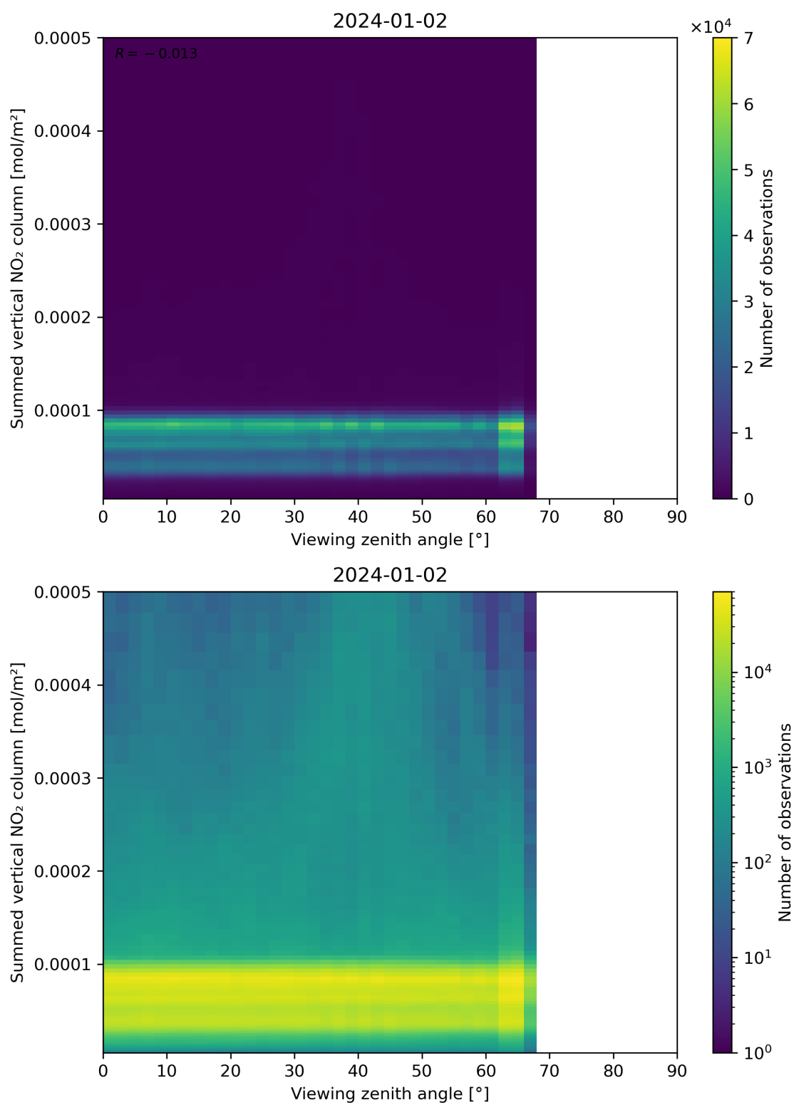
Figure 165: Scatter density plot of “Viewing zenith angle” against “Summed vertical NO 2 column” for 2024-01-01 to 2024-01-03.
