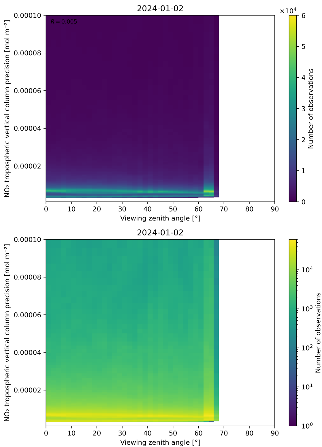
Figure 170: Scatter density plot of “Viewing zenith angle” against “NO 2 tropospheric vertical column precision” for 2024-01-01 to 2024-01-03.
