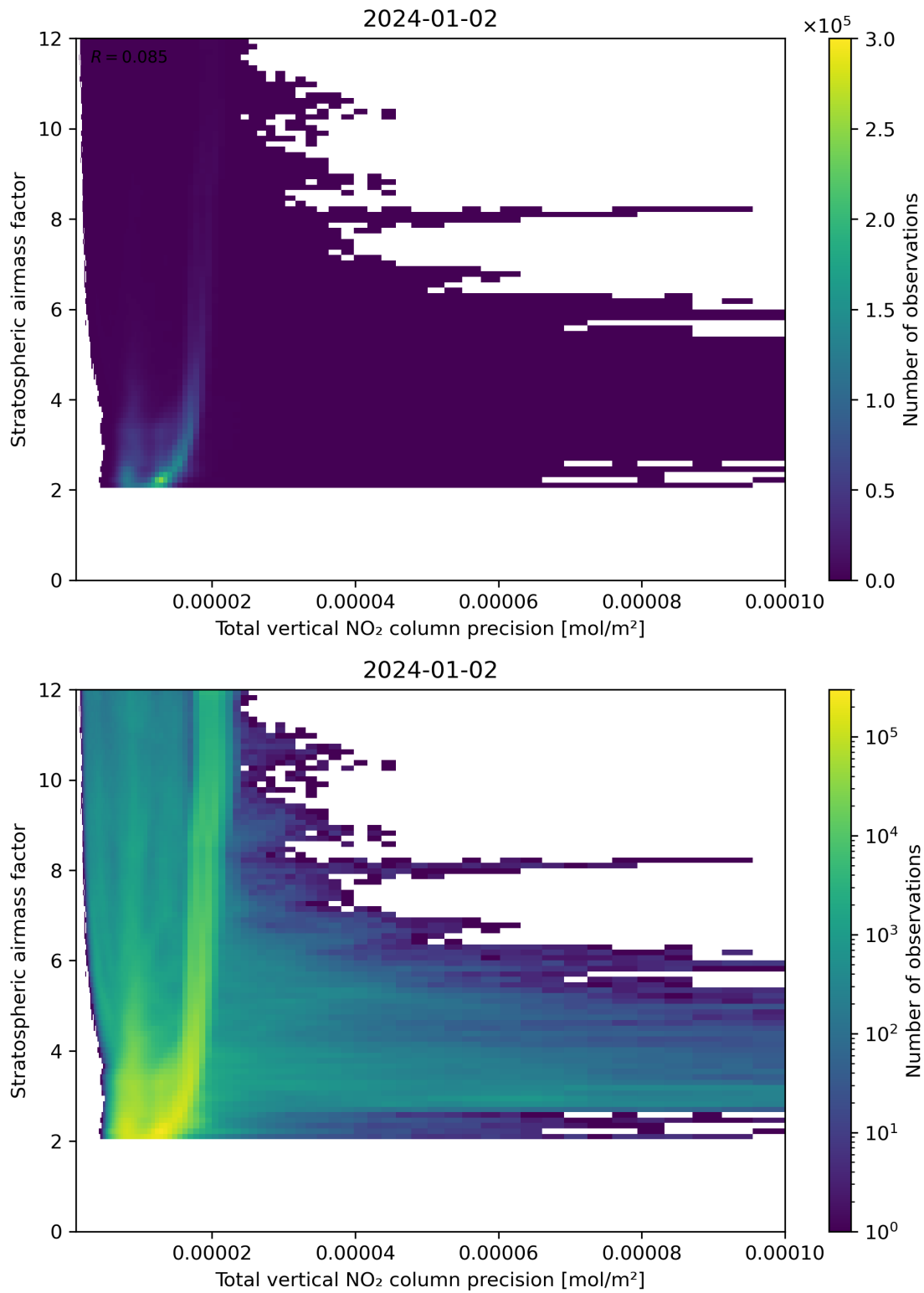
Figure 115: Scatter density plot of “Total vertical NO 2 column precision” against “Stratospheric air mass factor” for 2024-01-01 to 2024-01-03.
