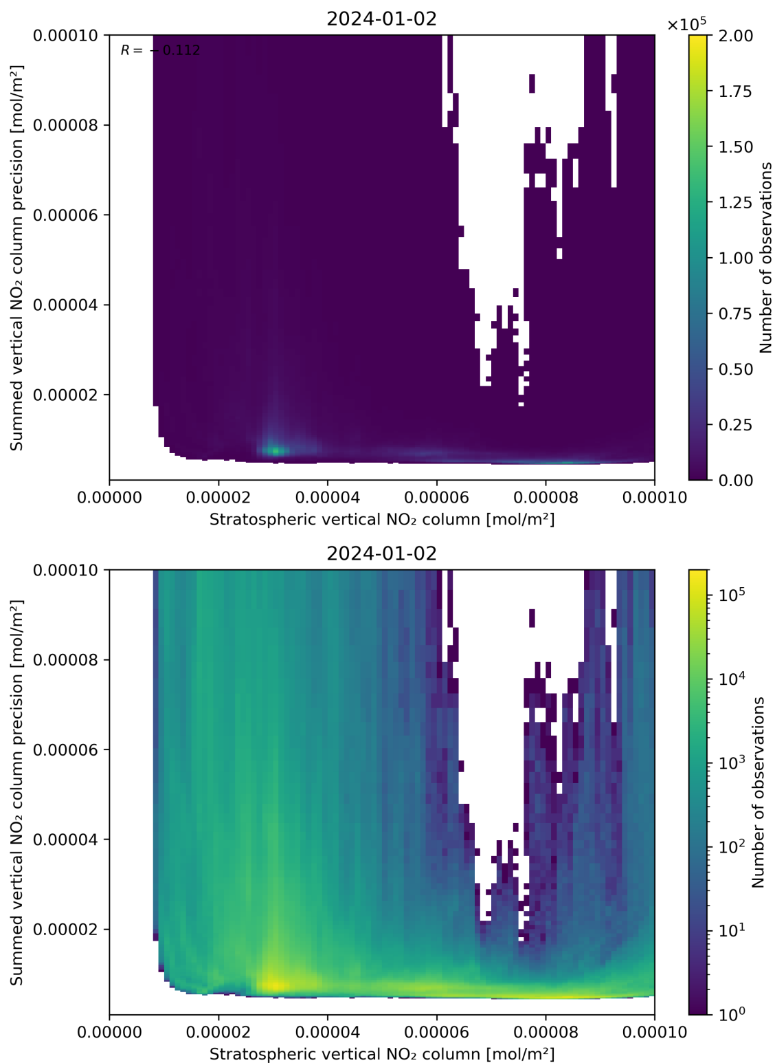
Figure 99: Scatter density plot of “Stratospheric vertical NO 2 column” against “Summed vertical NO 2 column precision” for 2024-01-01 to 2024-01-03.
