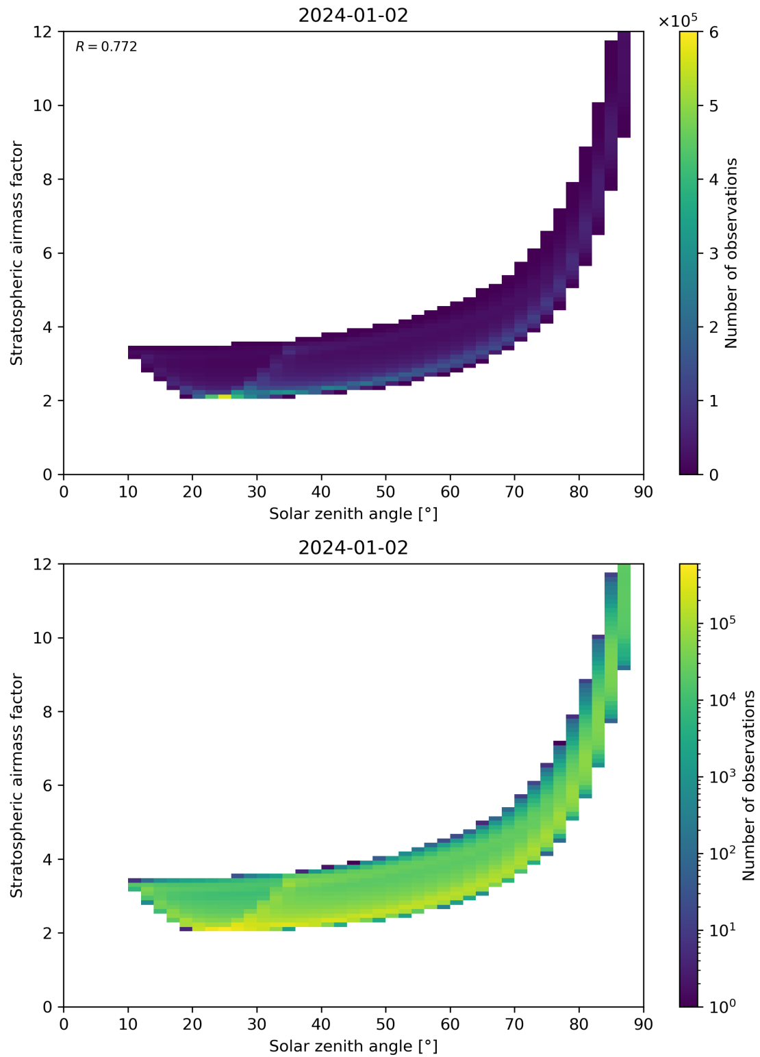
Figure 145: Scatter density plot of “Solar zenith angle” against “Stratospheric airmass factor” for 2024-01-01 to 2024-01-03.
