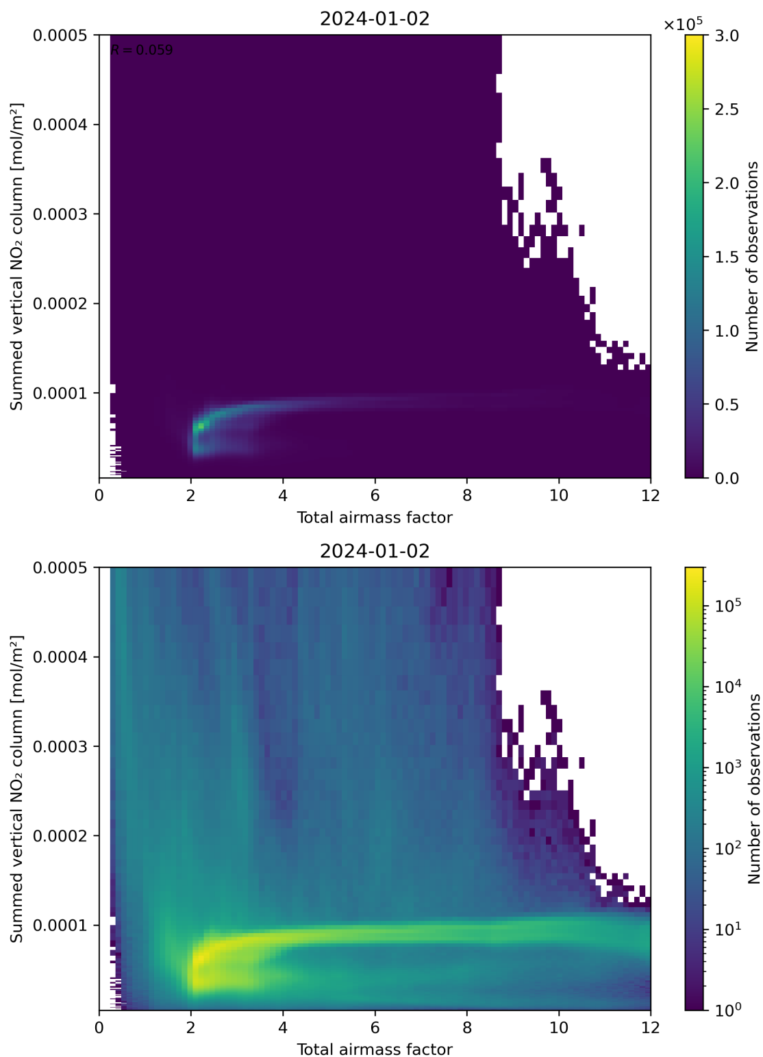
Figure 65: Scatter density plot of “Total airmass factor” against “Summed vertical NO 2 column” for 2024-01-01 to 2024-01-03.
