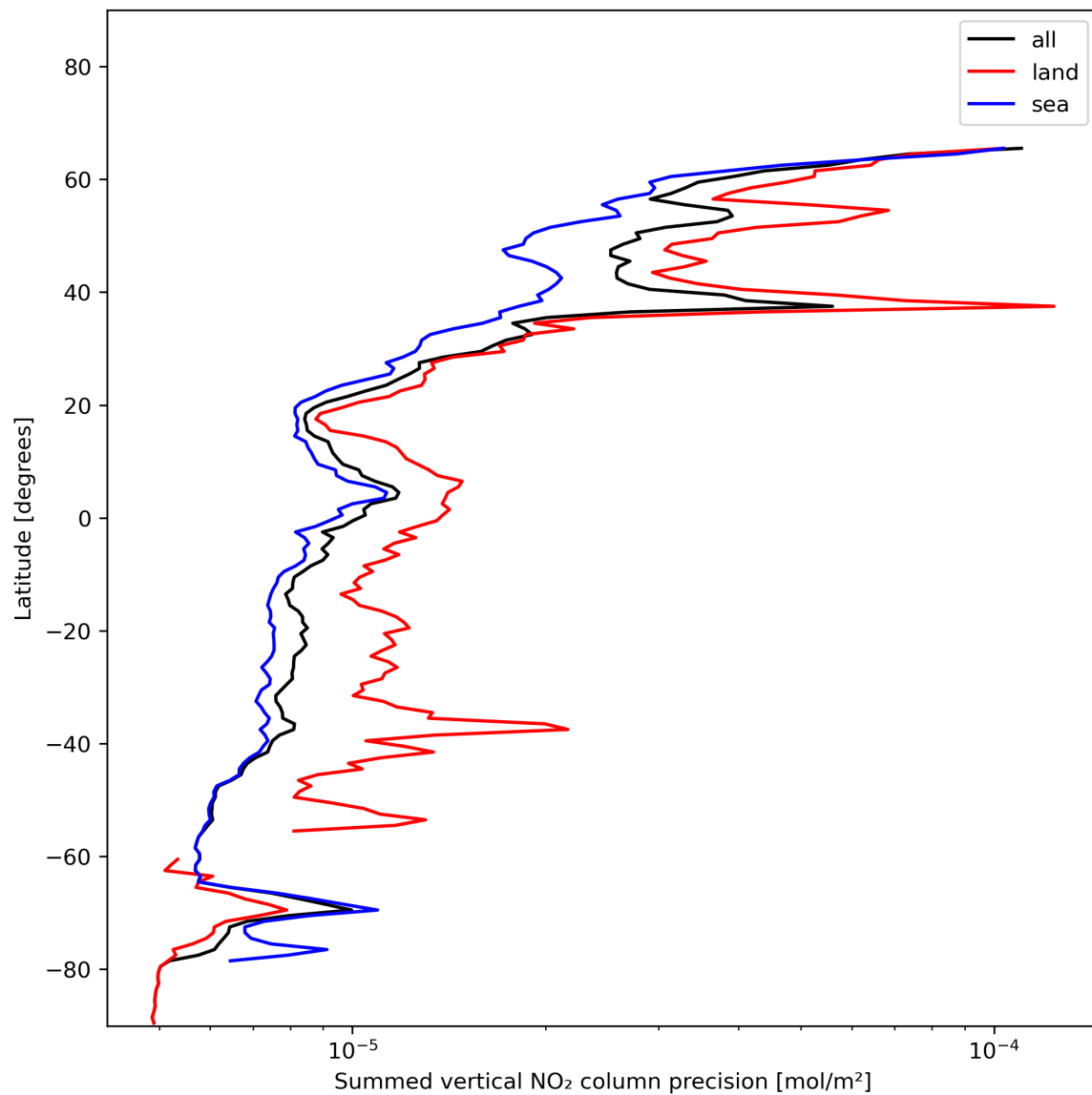
Figure 24: Zonal average of “Summed vertical NO 2 column precision” for 2024-01-01 to 2024-01-03.
