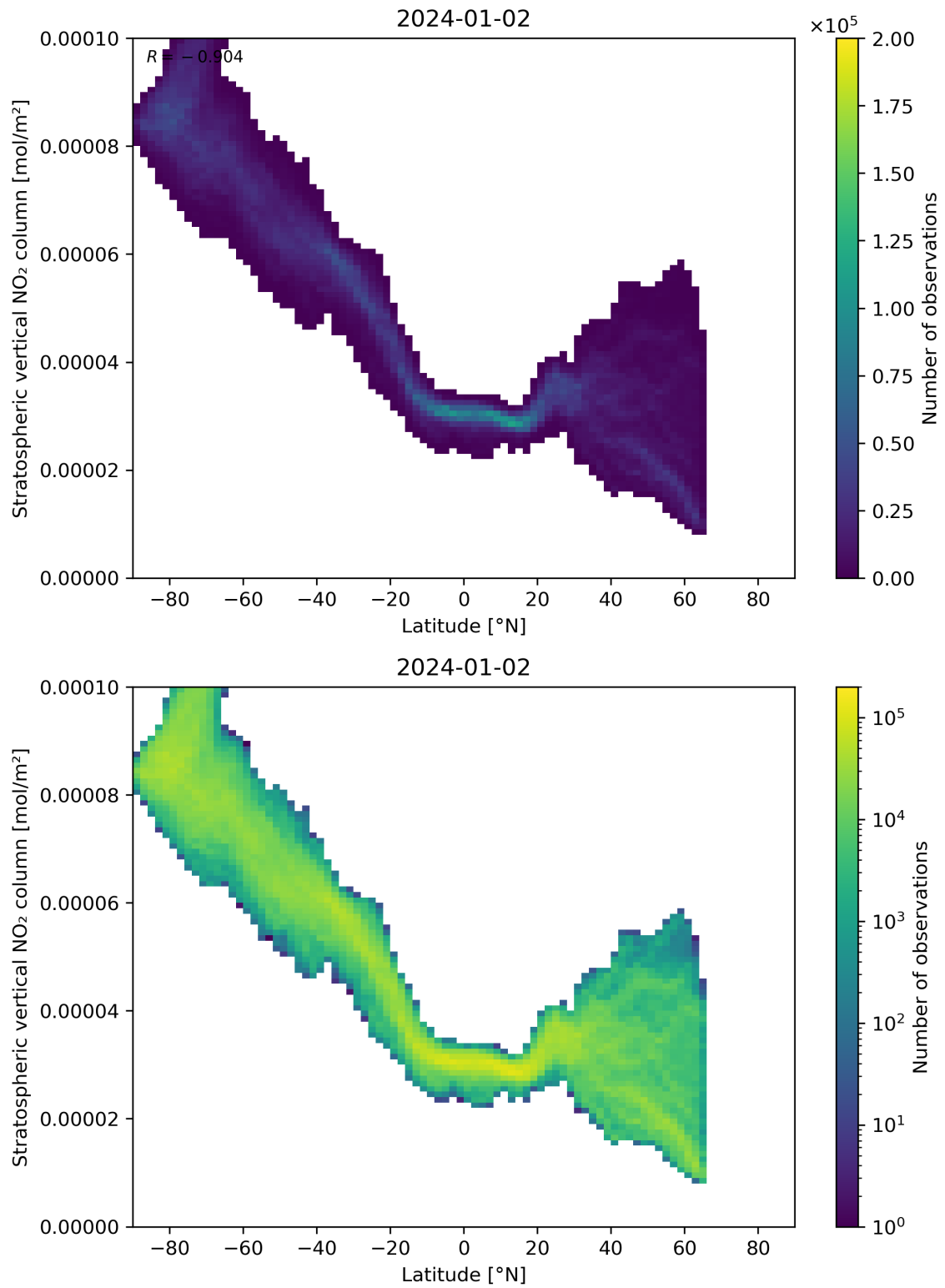
Figure 87: Scatter density plot of “Latitude” against “Stratospheric vertical NO 2 column” for 2024-01-01 to 2024-01-03.
