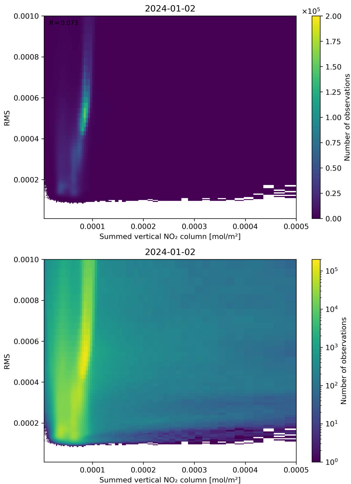
Figure 109: Scatter density plot of “Summed vertical NO 2 column” against “RMS” for 2024-01-01 to 2024-01-03.
