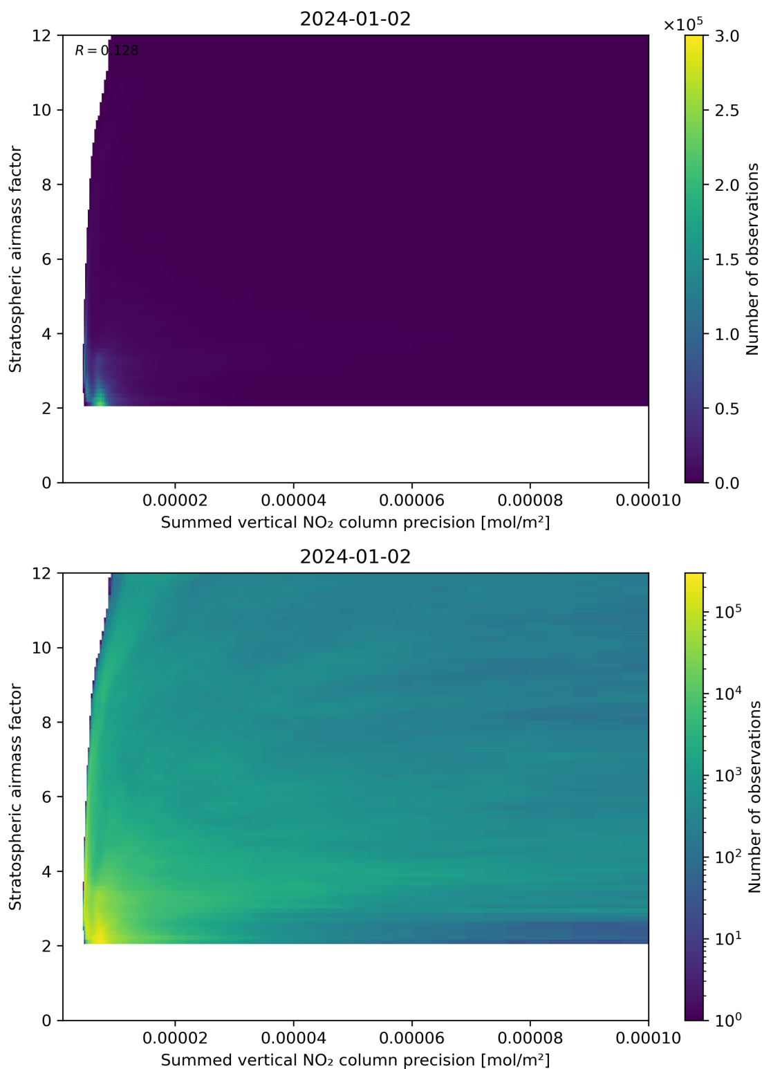
Figure 106: Scatter density plot of “Summed vertical NO 2 column precision” against “Stratospheric airmass factor” for 2024-01-01 to 2024-01-03.
