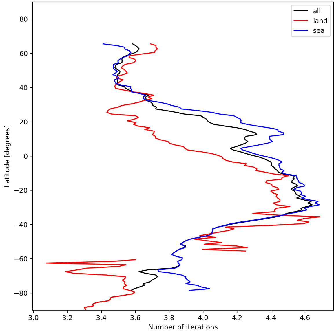
Figure 17: Zonal average of “Number of iterations” for 2024-01-01 to 2024-01-03.
