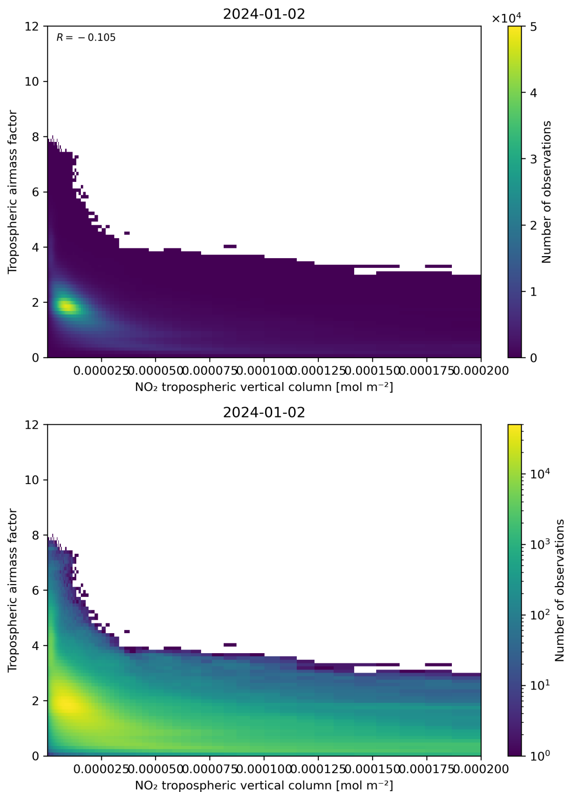
Figure 123: Scatter density plot of “NO 2 tropospheric vertical column” against “Tropospheric air mass factor” for 2024-01-01 to 2024-01-03.
