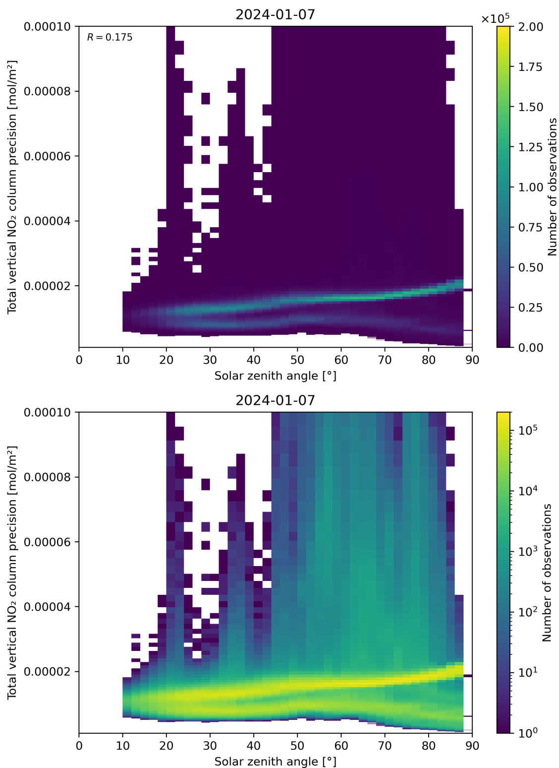
Figure 154: Scatter density plot of “Solar zenith angle” against “Total vertical NO 2 column precision” for 2024-01-06 to 2024-01-08.
