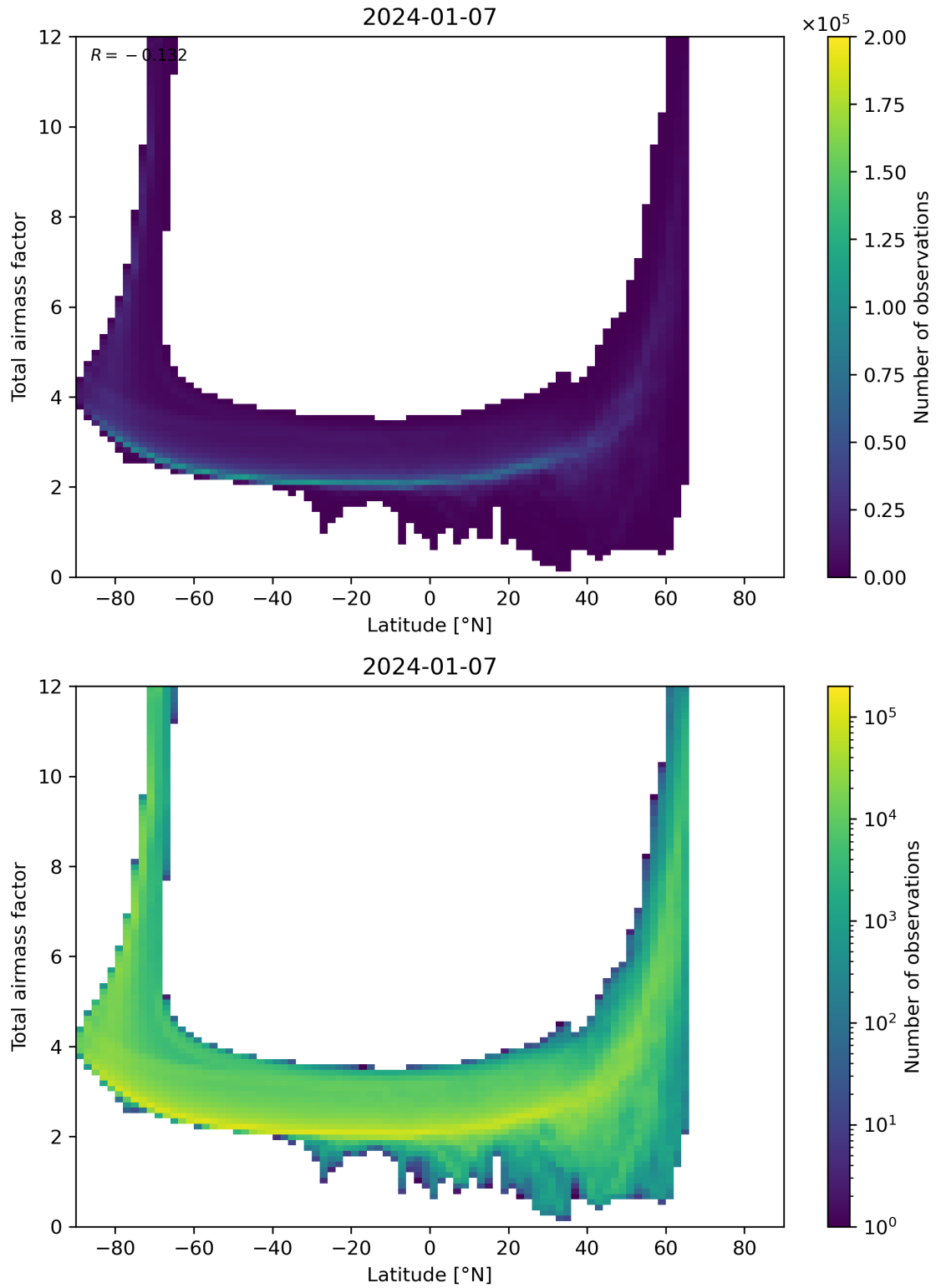
Figure 84: Scatter density plot of “Latitude” against “Total airmass factor” for 2024-01-06 to 2024-01-08.
