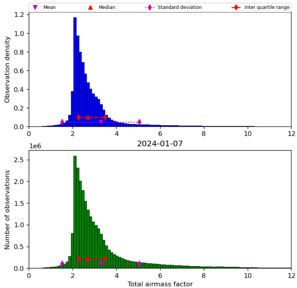
Figure 32: Histogram of “Total airmass factor” for 2024-01-06 to 2024-01-08
