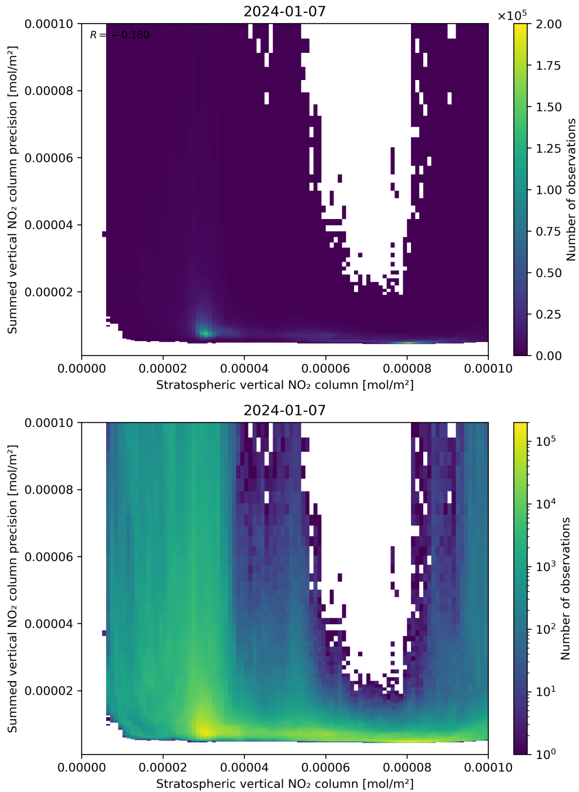
Figure 99: Scatter density plot of “Stratospheric vertical NO 2 column” against “Summed vertical NO 2 column precision” for 2024-01-06 to 2024-01-08.
