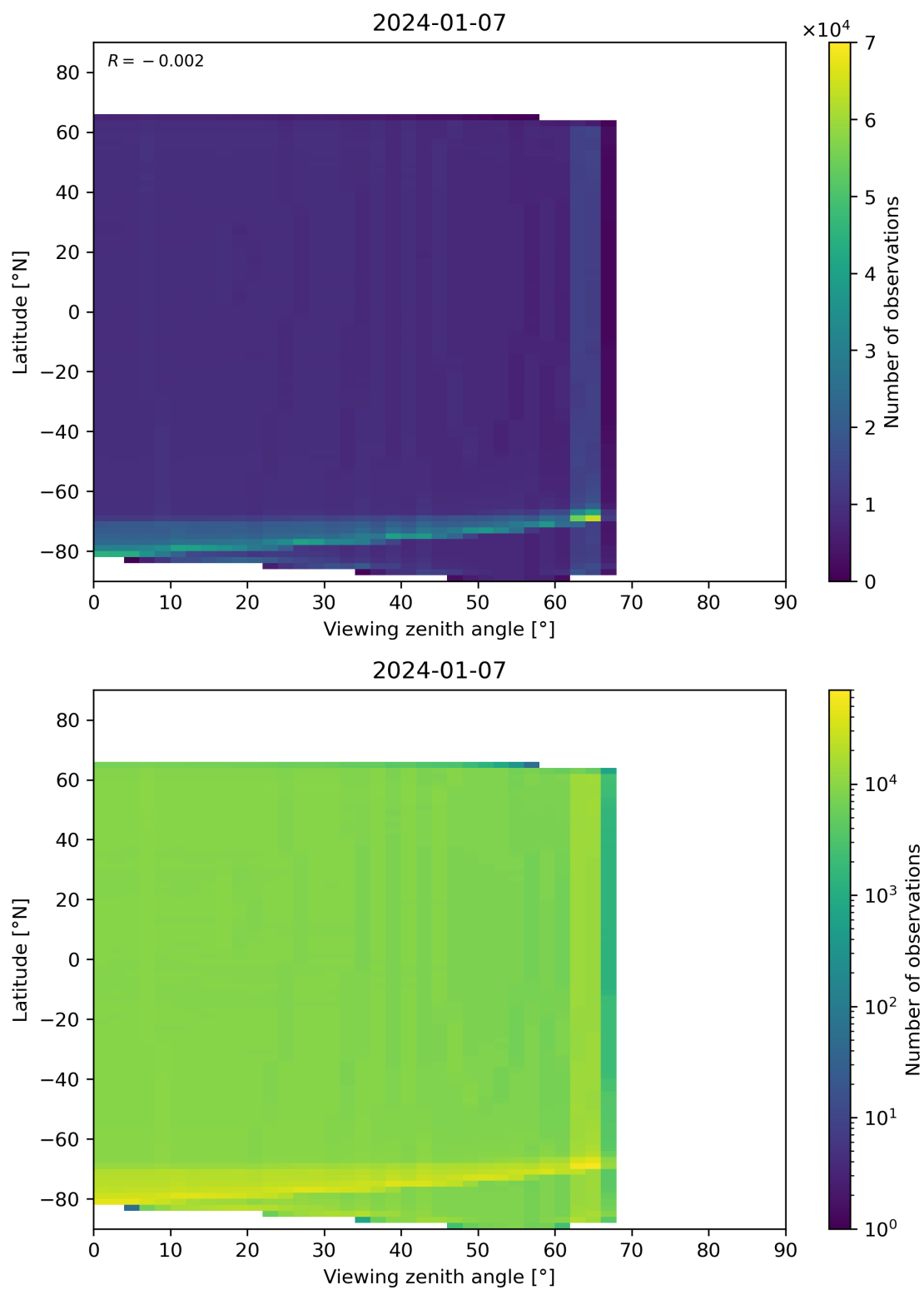
Figure 163: Scatter density plot of “Viewing zenith angle” against “Latitude” for 2024-01-06 to 2024-01-08.
