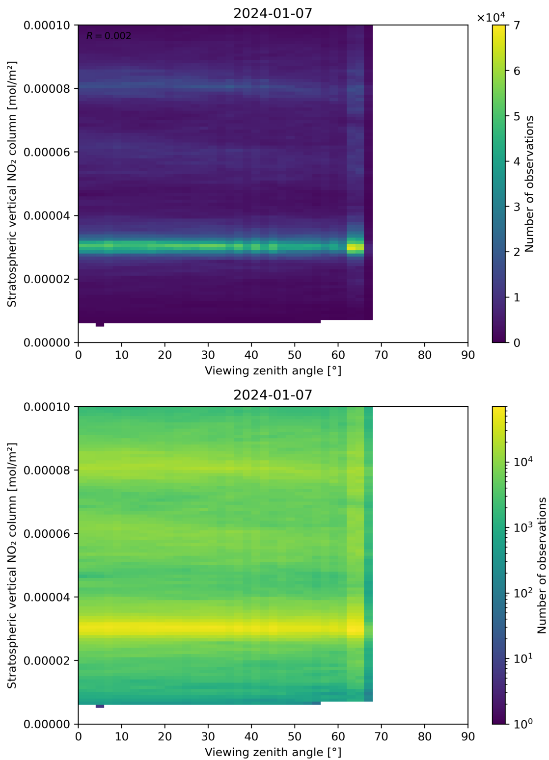
Figure 164: Scatter density plot of “Viewing zenith angle” against “Stratospheric vertical NO 2 column” for 2024-01-06 to 2024-01-08.
