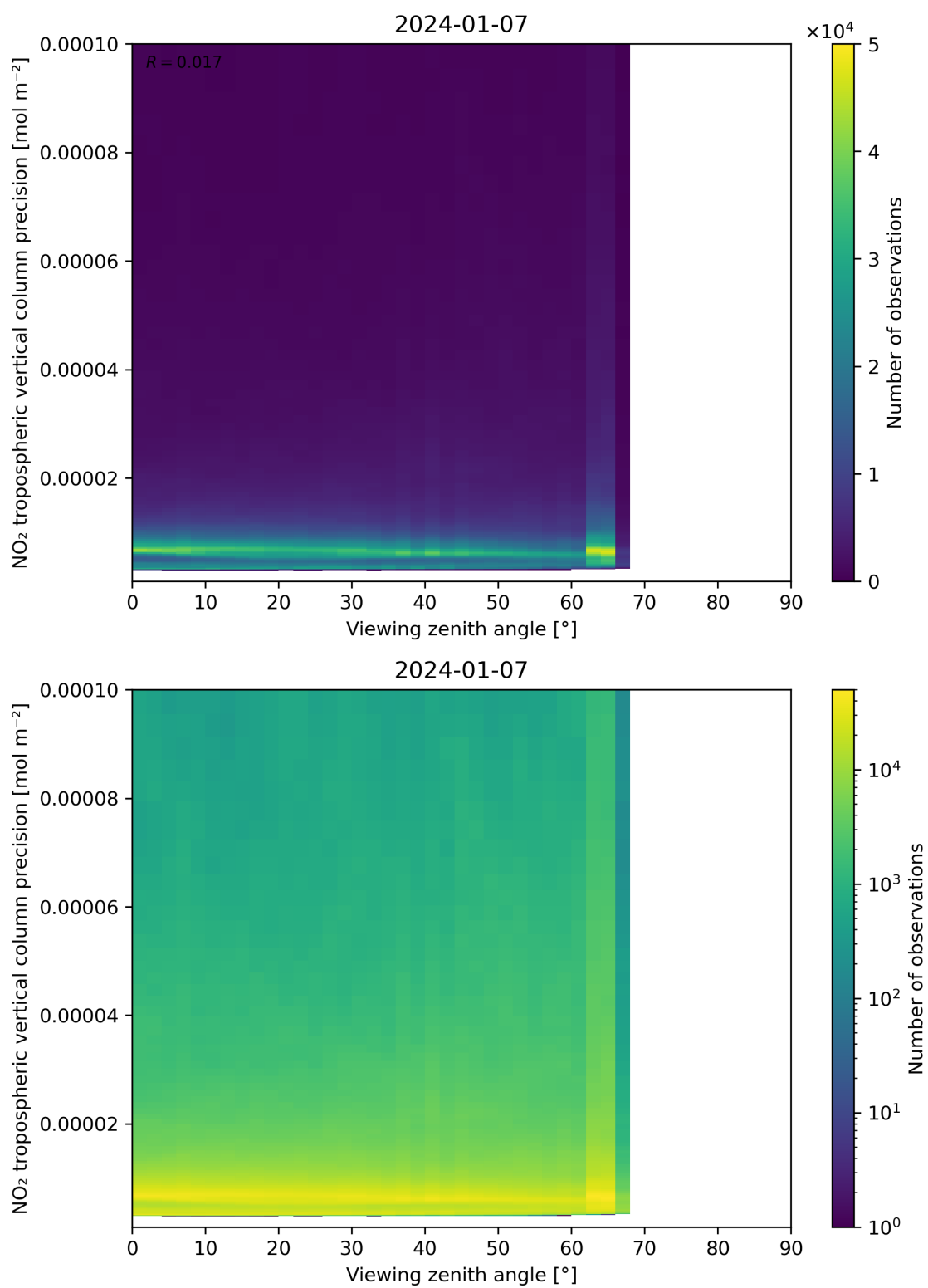
Figure 170: Scatter density plot of “Viewing zenith angle” against “NO 2 tropospheric vertical column precision” for 2024-01-06 to 2024-01-08.
