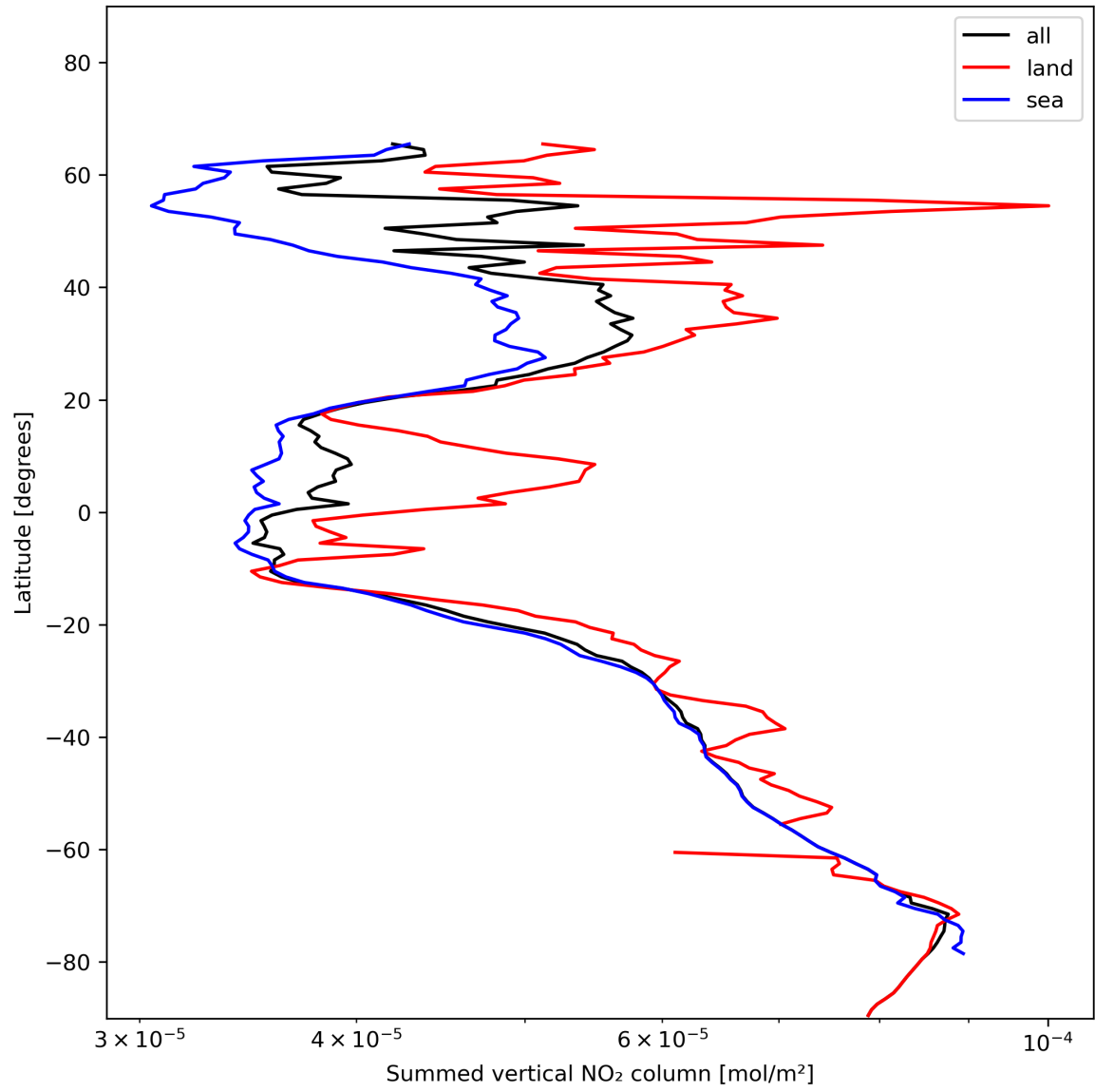
Figure 23: Zonal average of “Summed vertical NO 2 column” for 2024-01-06 to 2024-01-08.
