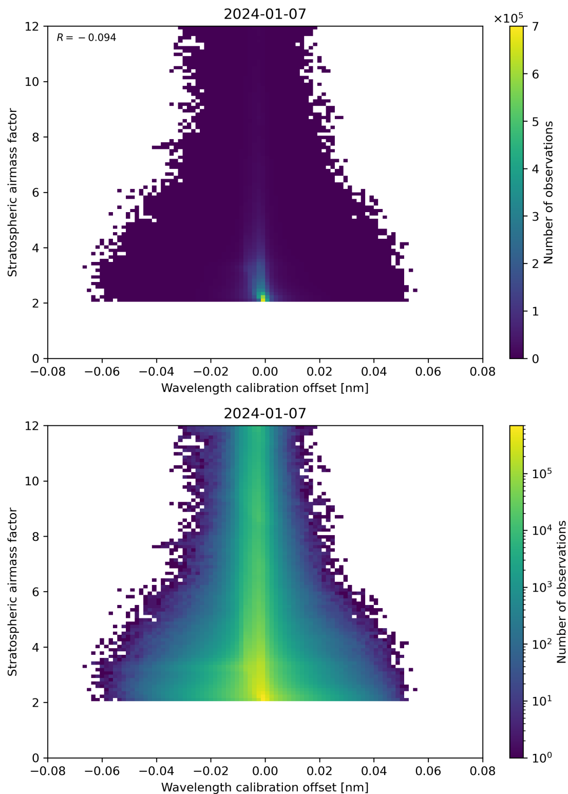
Figure 174: Scatter density plot of “Wavelength calibration offset” against “Stratospheric airmass factor” for 2024-01-06 to 2024-01-08.
