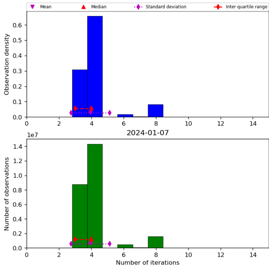
Figure 34: Histogram of “Number of iterations” for 2024-01-06 to 2024-01-08
