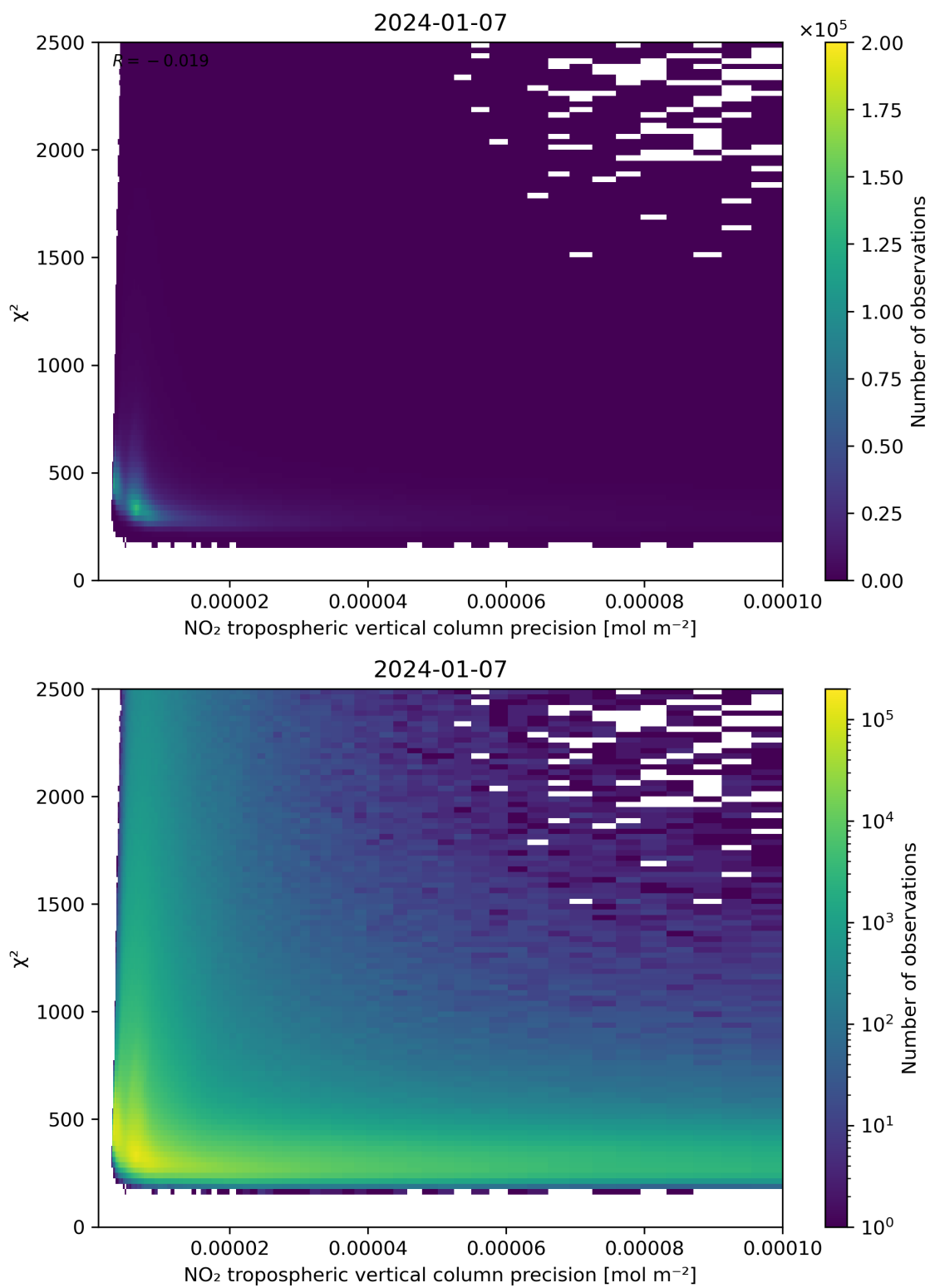
Figure 134: Scatter density plot of “NO 2 tropospheric vertical column precision” against “ \chi^2 ” for 2024-01-06 to 2024-01-08.
