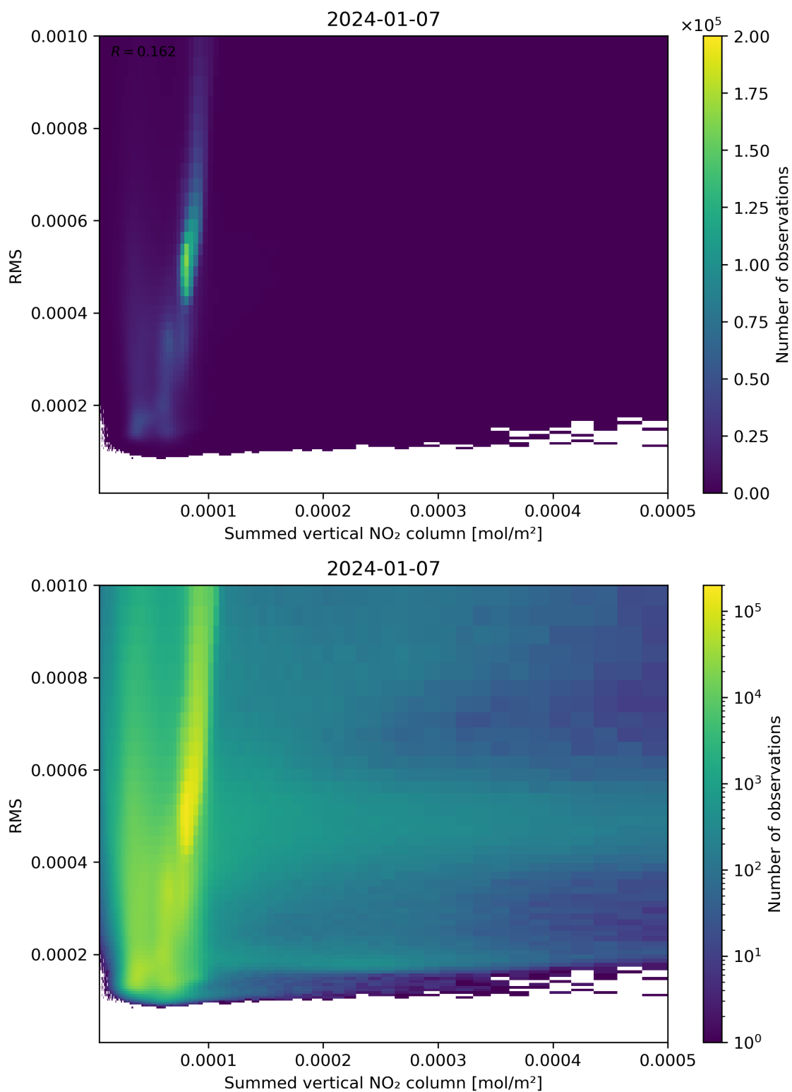
Figure 109: Scatter density plot of “Summed vertical NO 2 column” against “RMS” for 2024-01-06 to 2024-01-08.
