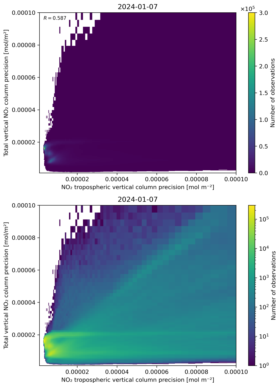
Figure 139: Scatter density plot of “NO 2 tropospheric vertical column precision” against “Total vertical NO 2 column precision” for 2024-01-06 to 2024-01-08.
