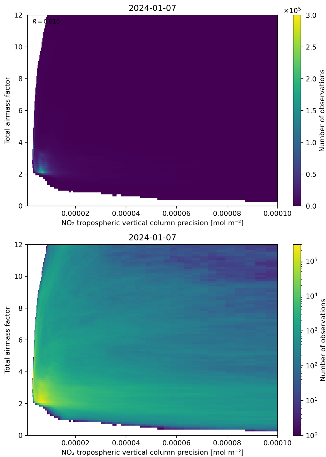
Figure 132: Scatter density plot of “NO 2 tropospheric vertical column precision” against “Total air mass factor” for 2024-01-06 to 2024-01-08.
