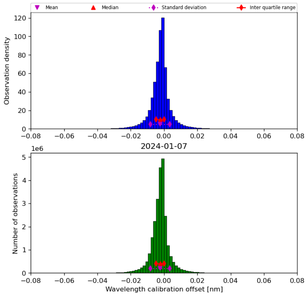
Figure 35: Histogram of “Wavelength calibration offset” for 2024-01-06 to 2024-01-08
