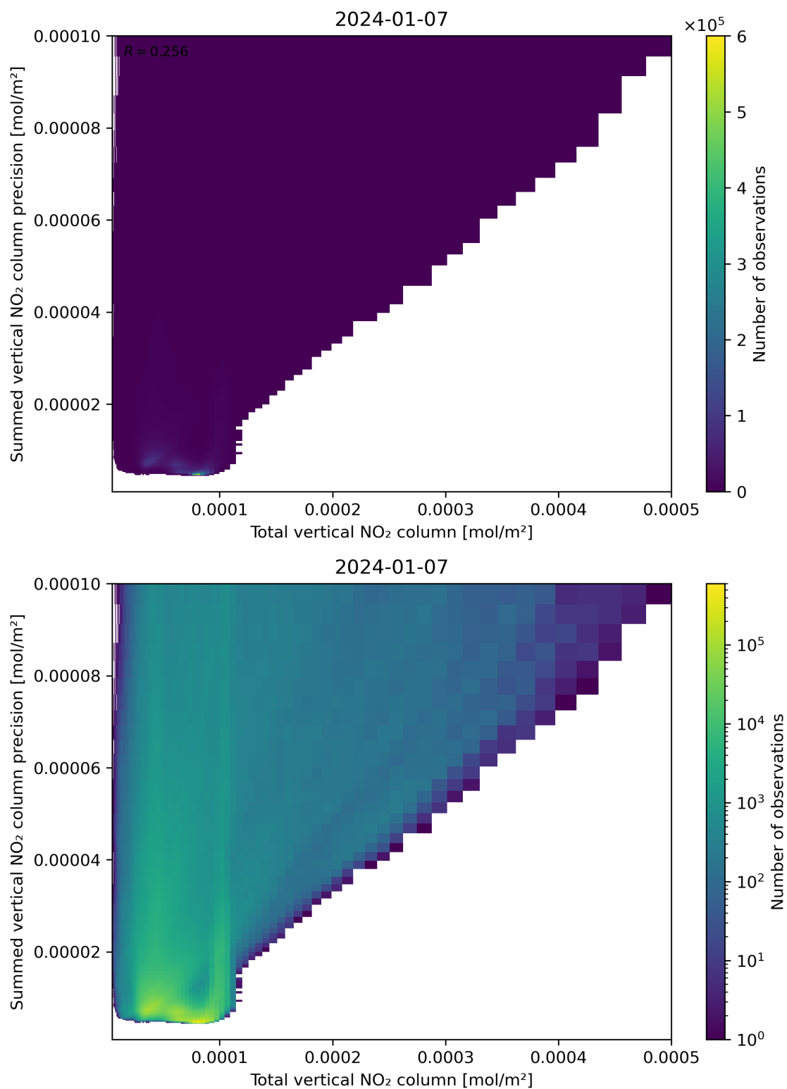
Figure 113: Scatter density plot of “Total vertical NO 2 column” against “Summed vertical NO 2 column precision” for 2024-01-06 to 2024-01-08.
