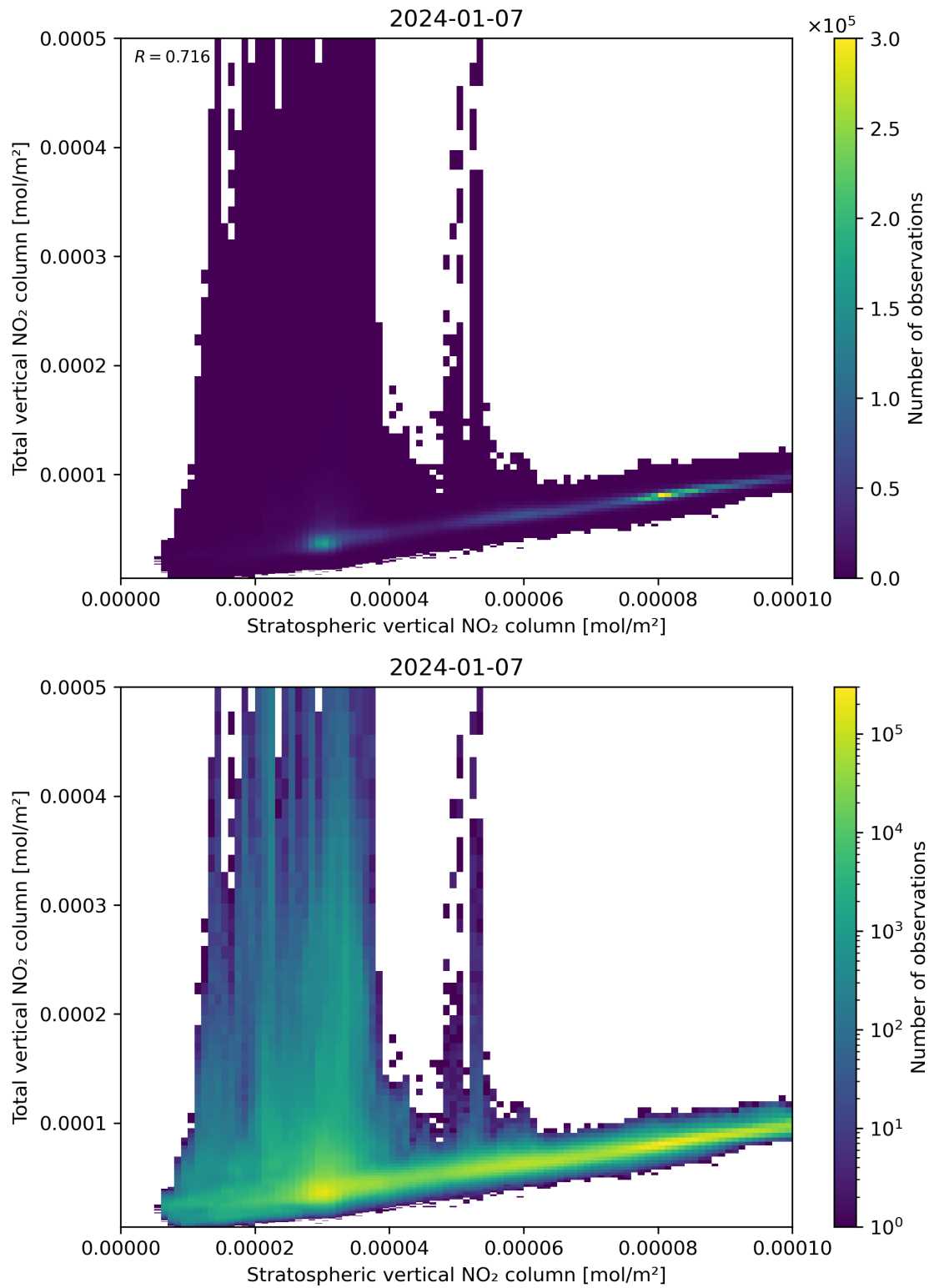
Figure 100: Scatter density plot of “Stratospheric vertical NO 2 column” against “Total vertical NO 2 column” for 2024-01-06 to 2024-01-08.
