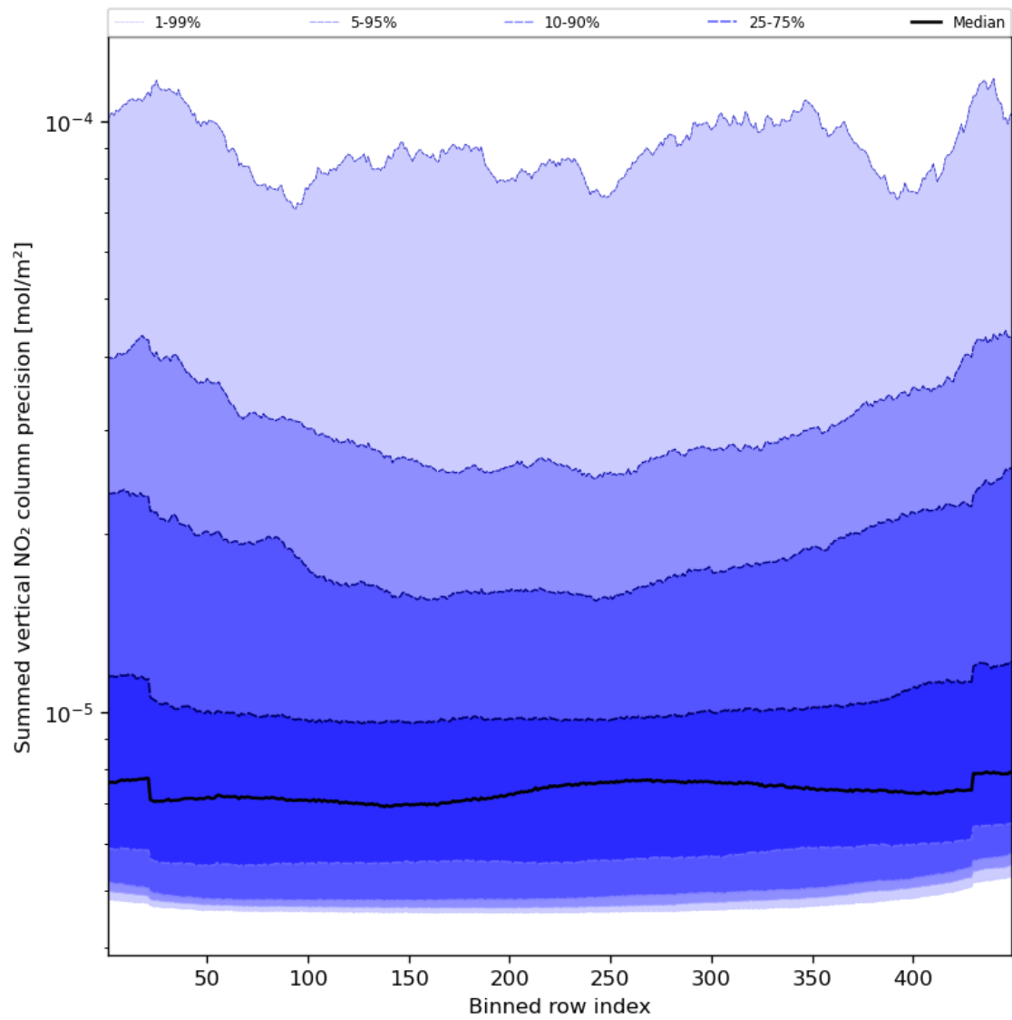
Figure 58: Along track statistics of “Summed vertical NO 2 column precision” for 2024-01-06 to 2024-01-08
