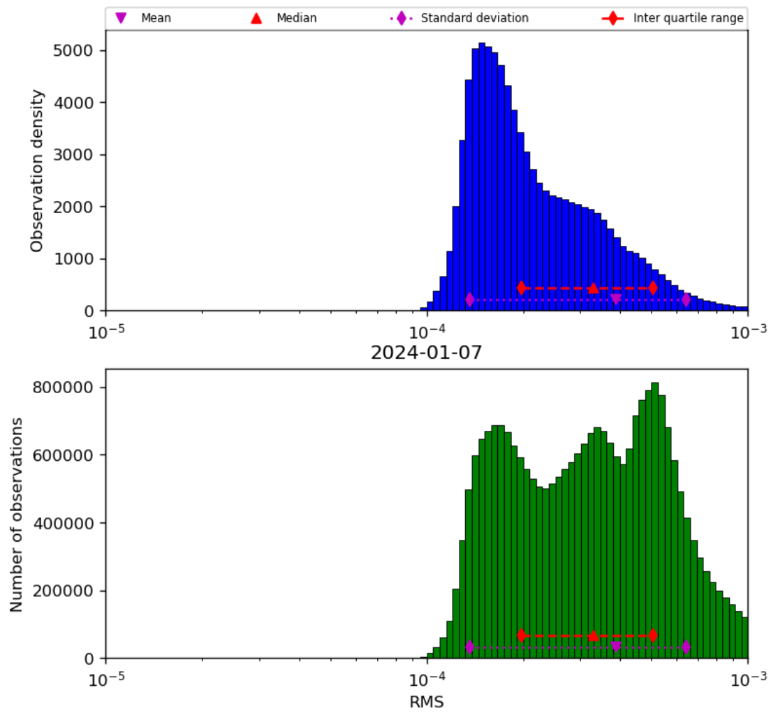
Figure 43: Histogram of “RMS” for 2024-01-06 to 2024-01-08
