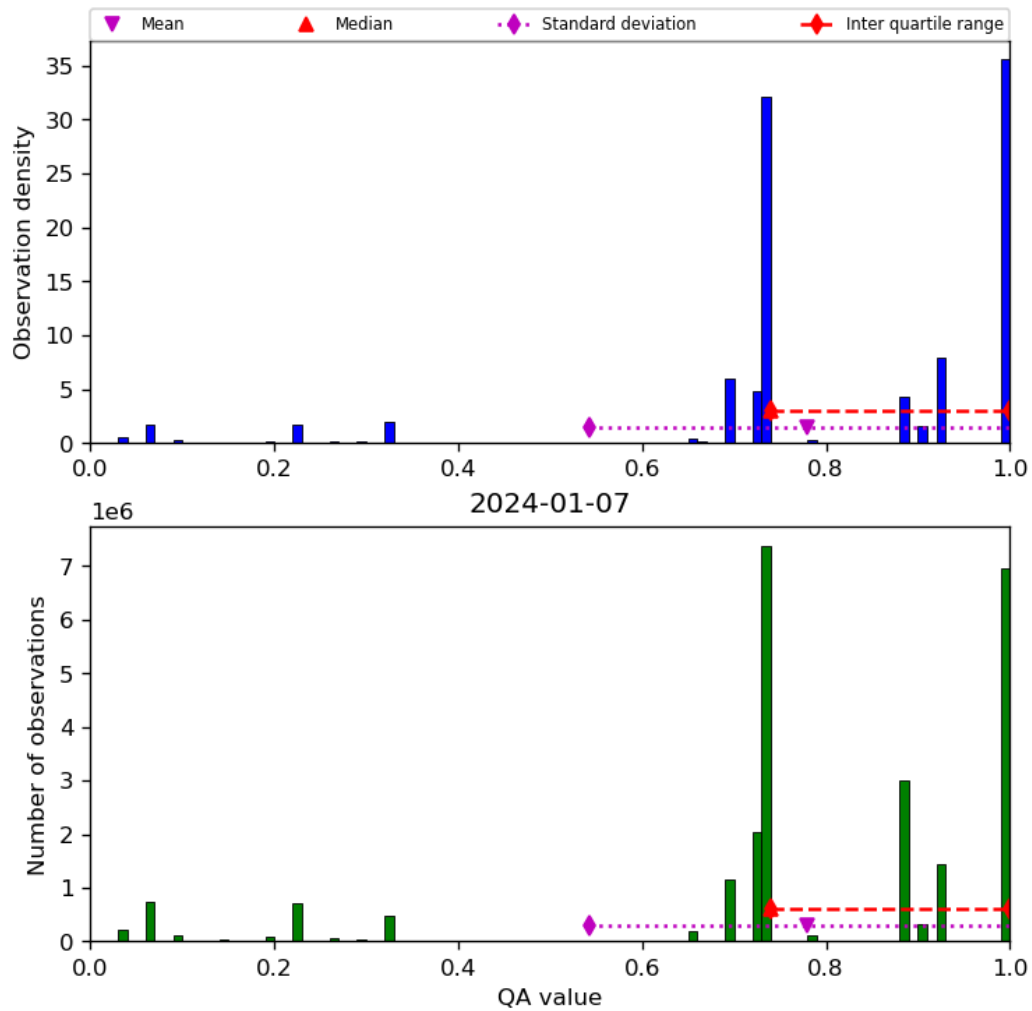
Figure 28: Histogram of “QA value” for 2024-01-06 to 2024-01-08
