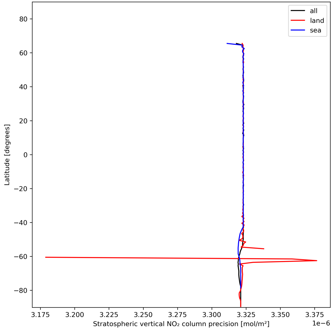
Figure 20: Zonal average of “Stratospheric vertical NO 2 column precision” for 2024-01-06 to 2024-01-08.
