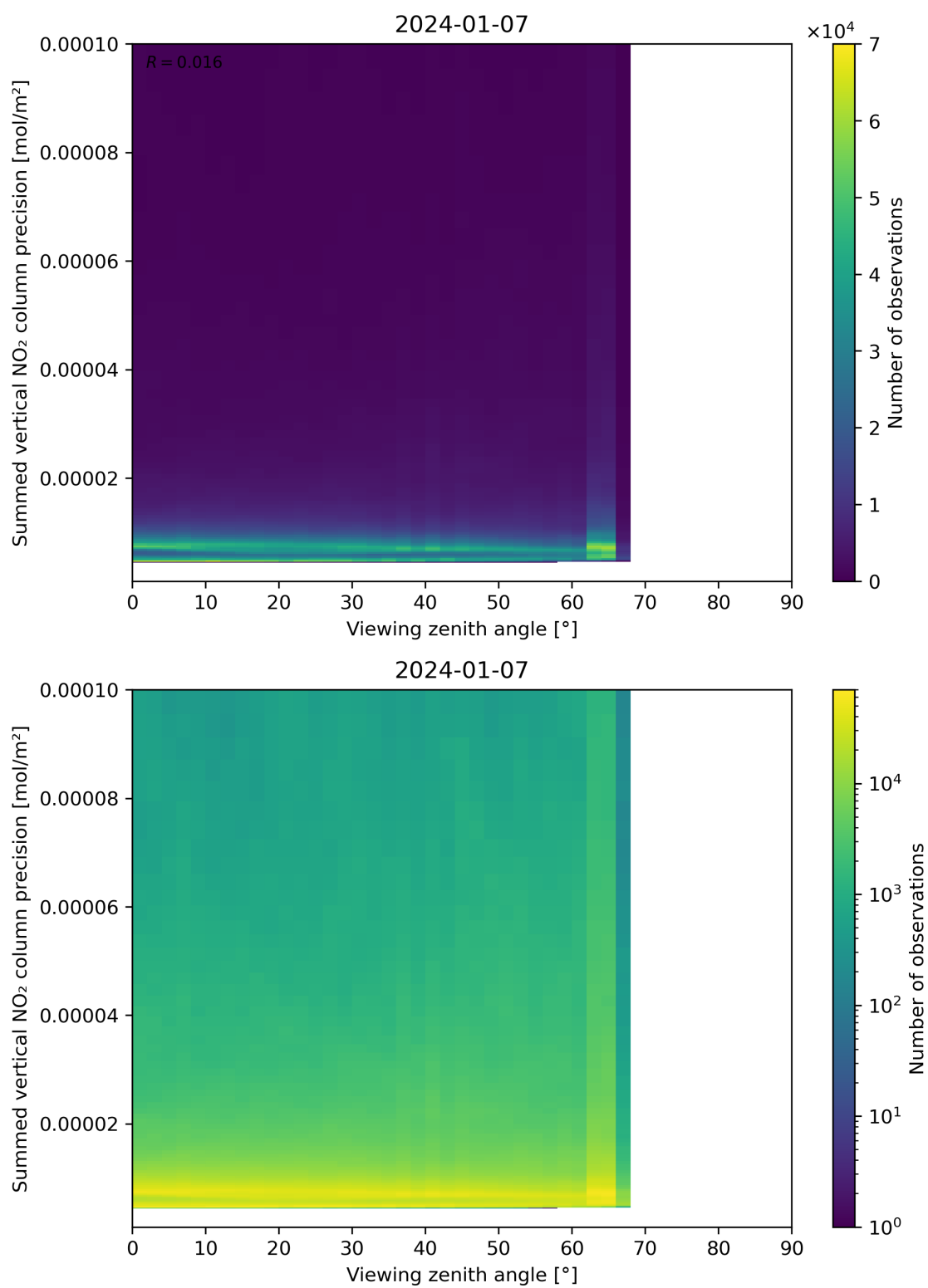
Figure 166: Scatter density plot of “Viewing zenith angle” against “Summed vertical NO 2 column precision” for 2024-01-06 to 2024-01-08.
