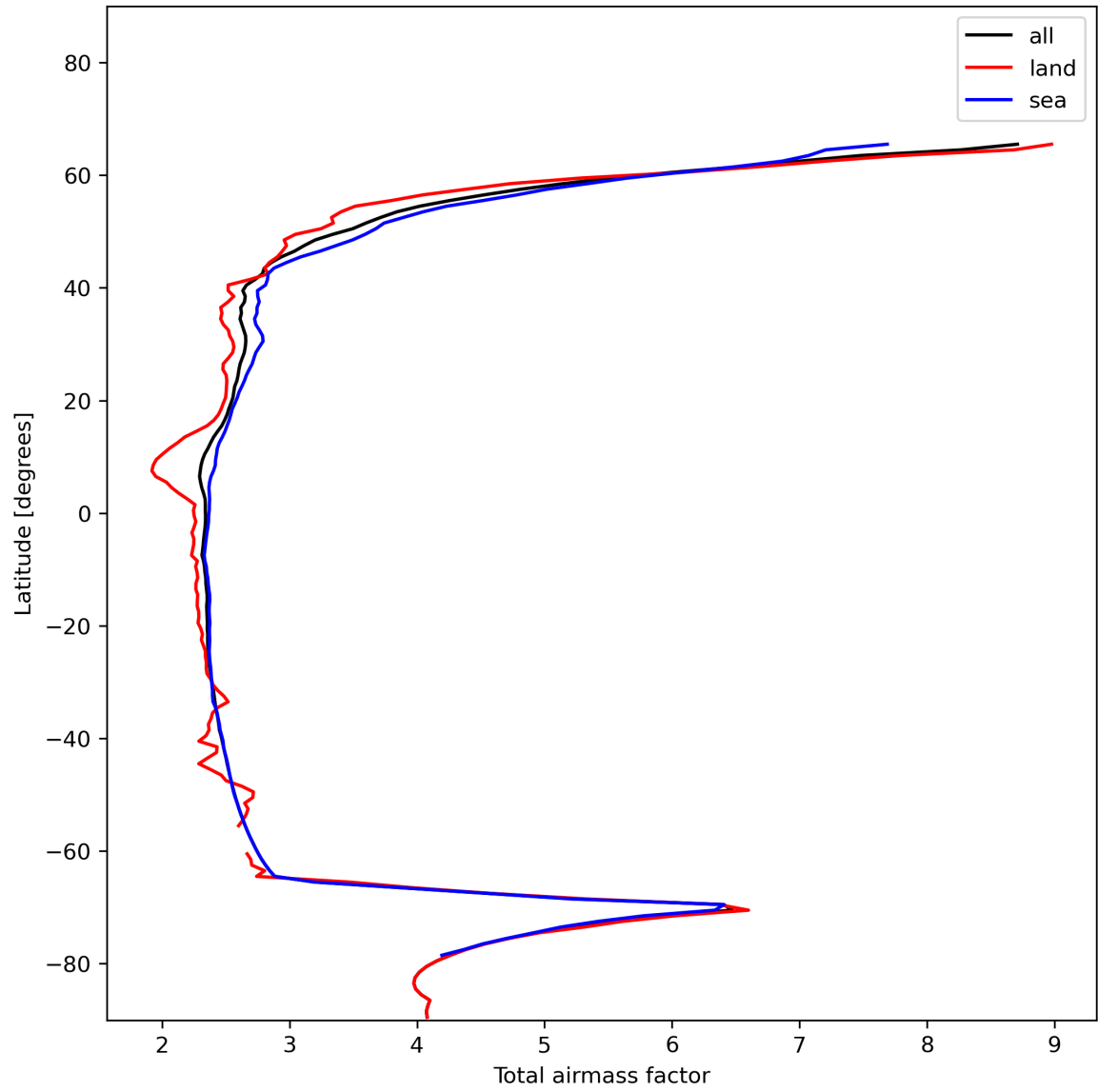
Figure 15: Zonal average of “Total airmass factor” for 2024-01-06 to 2024-01-08.
