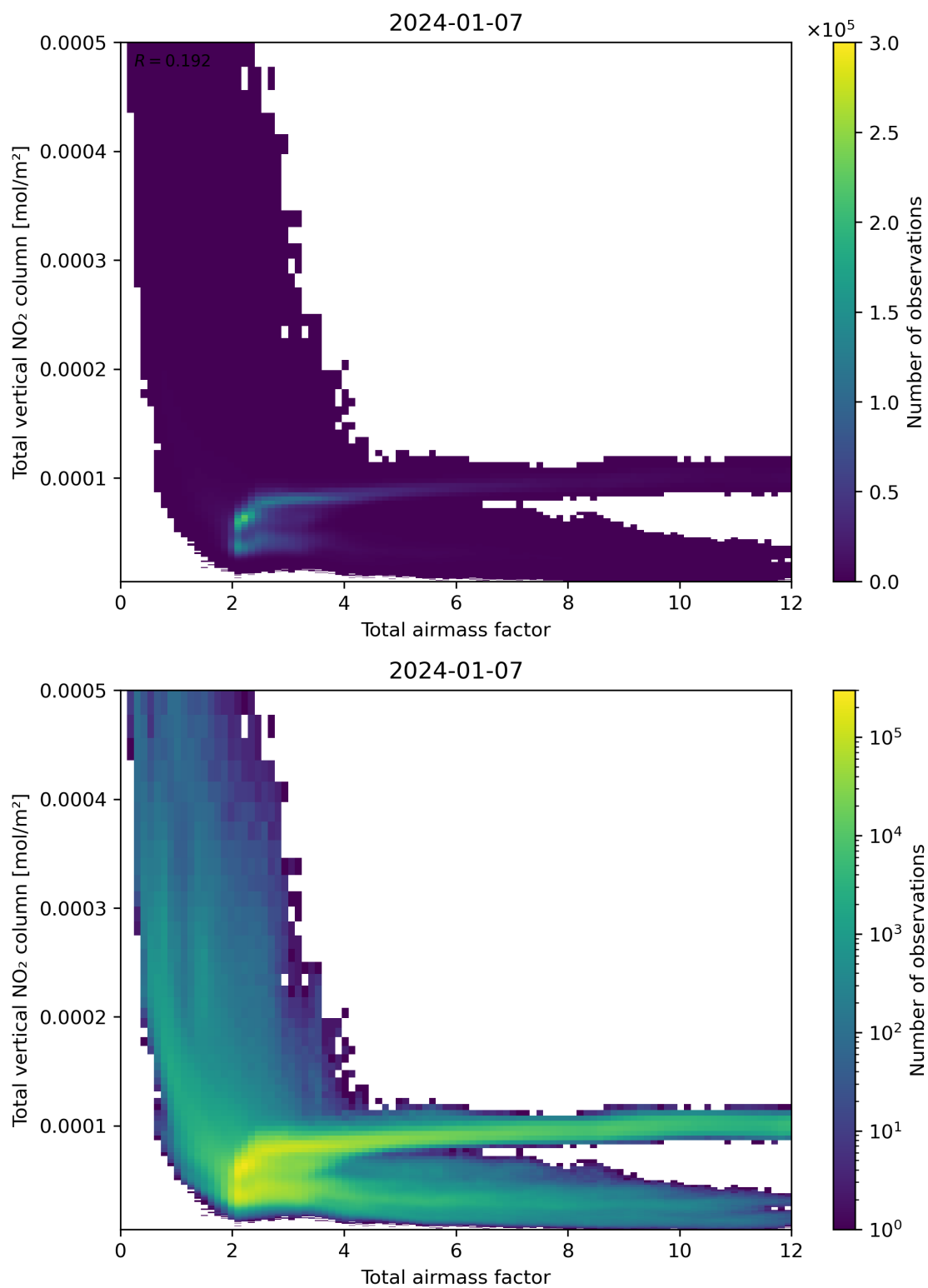
Figure 67: Scatter density plot of “Total airmass factor” against “Total vertical NO 2 column” for 2024-01-06 to 2024-01-08.
