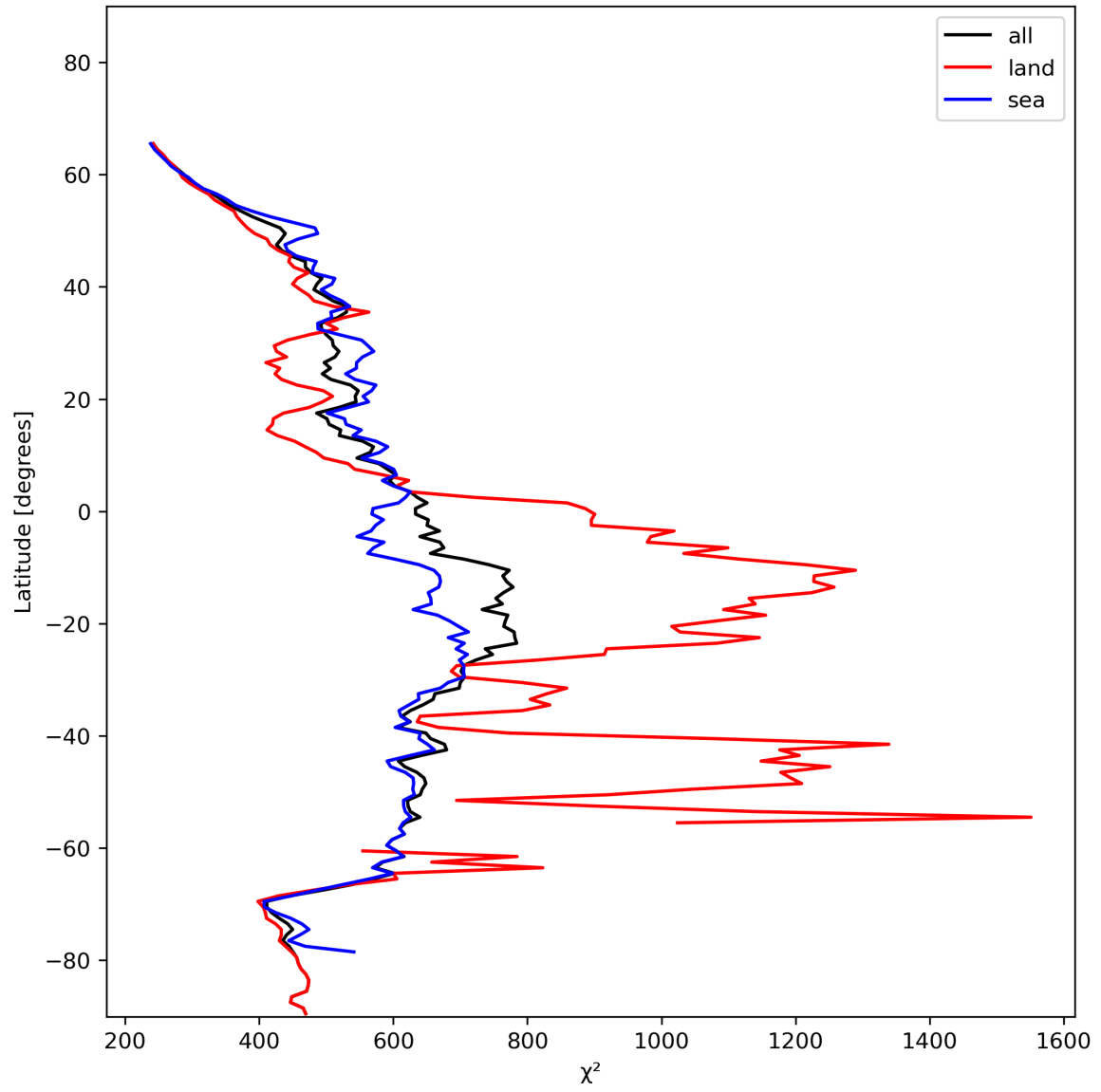
Figure 25: Zonal average of “ \chi^2 ” for 2024-01-06 to 2024-01-08.
