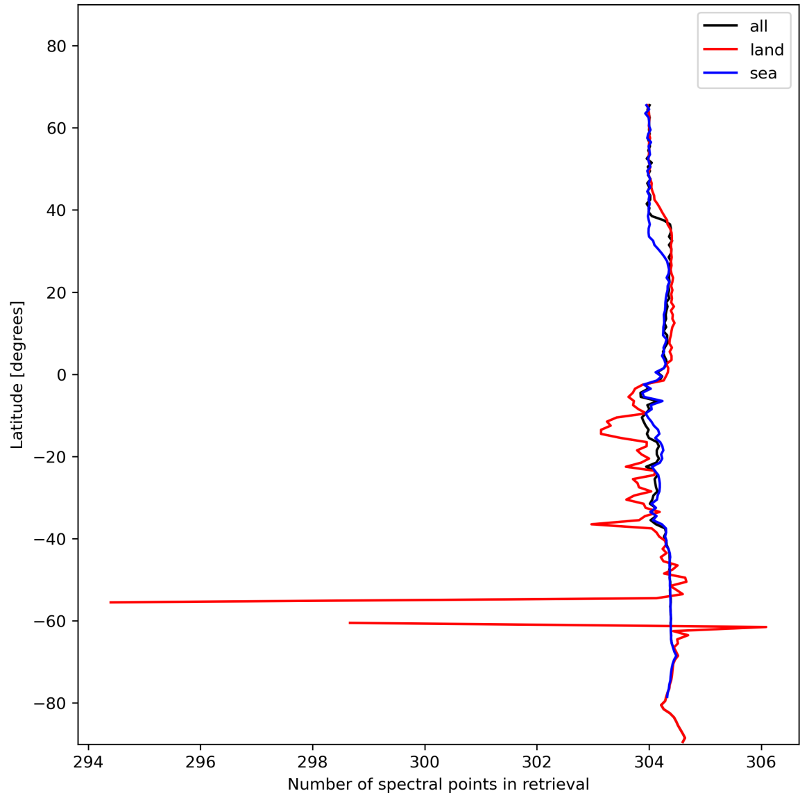
Figure 16: Zonal average of “Number of spectral points in retrieval” for 2024-01-06 to 2024-01-08.
