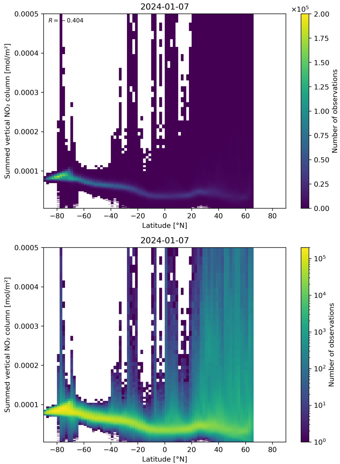
Figure 88: Scatter density plot of “Latitude” against “Summed vertical NO 2 column” for 2024-01-06 to 2024-01-08.
