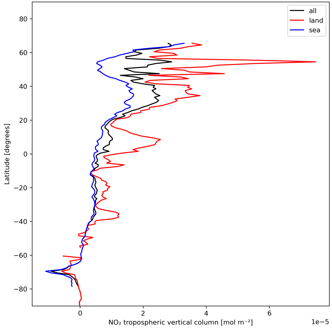
Figure 12: Zonal average of “NO 2 tropospheric vertical column” for 2024-01-06 to 2024-01-08.
