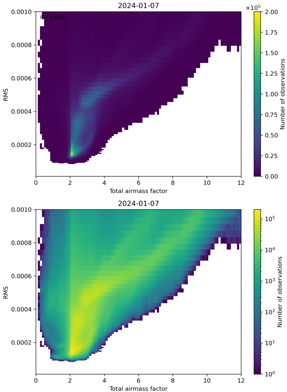
Figure 69: Scatter density plot of “Total airmass factor” against “RMS” for 2024-01-06 to 2024-01-08.
