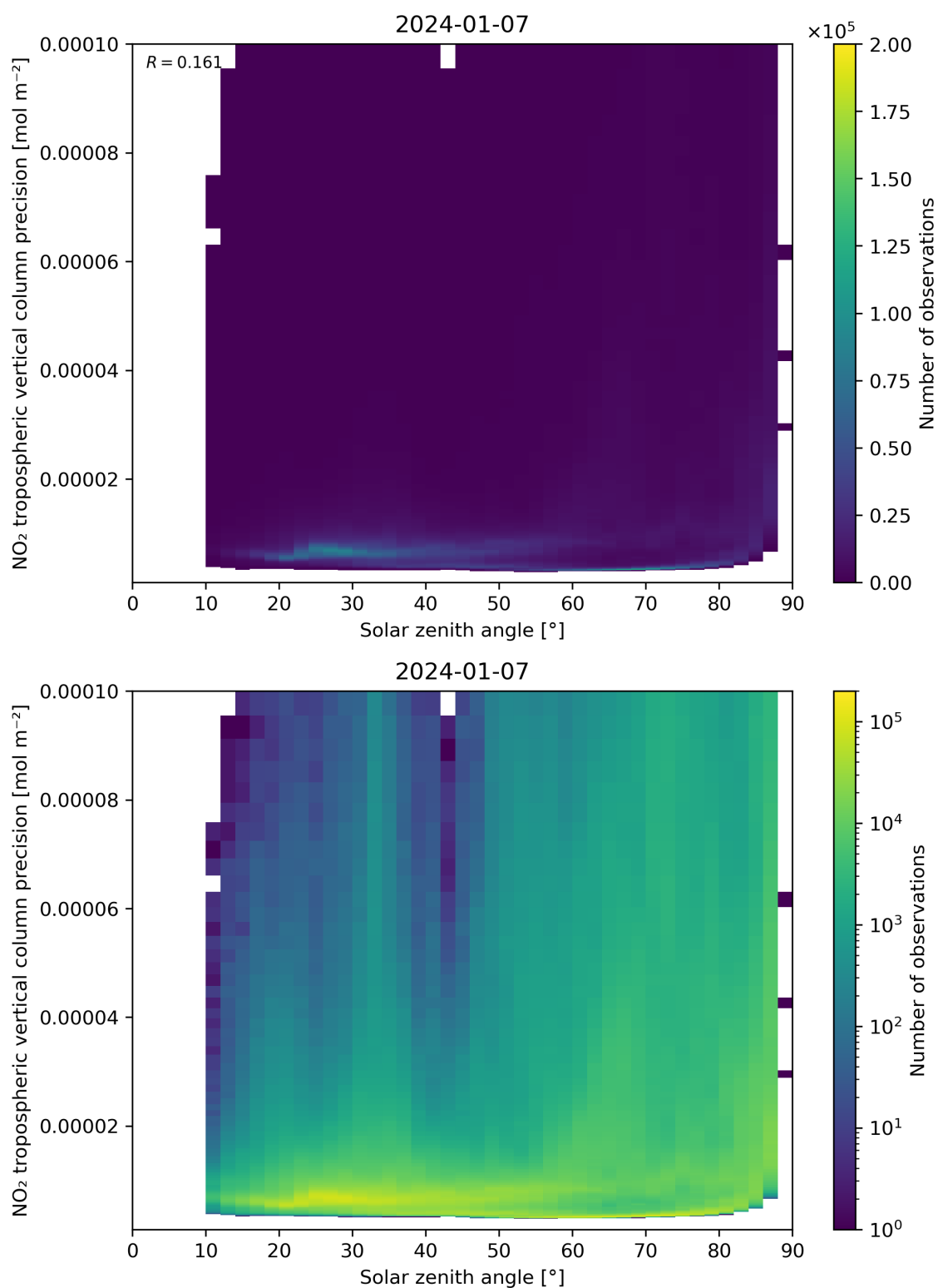
Figure 156: Scatter density plot of “Solar zenith angle” against “NO 2 tropospheric vertical column precision” for 2024-01-06 to 2024-01-08.
