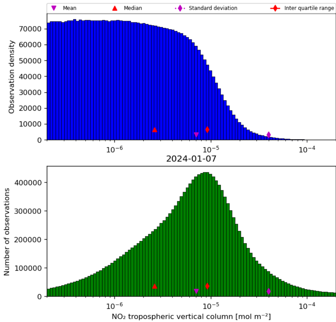
Figure 29: Histogram of “NO 2 tropospheric vertical column” for 2024-01-06 to 2024-01-08
