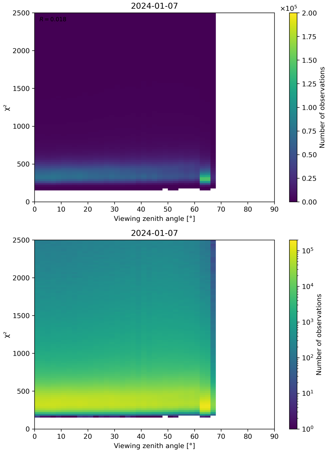
Figure 162: Scatter density plot of “Viewing zenith angle” against “ \chi^2 ” for 2024-01-06 to 2024-01-08.
