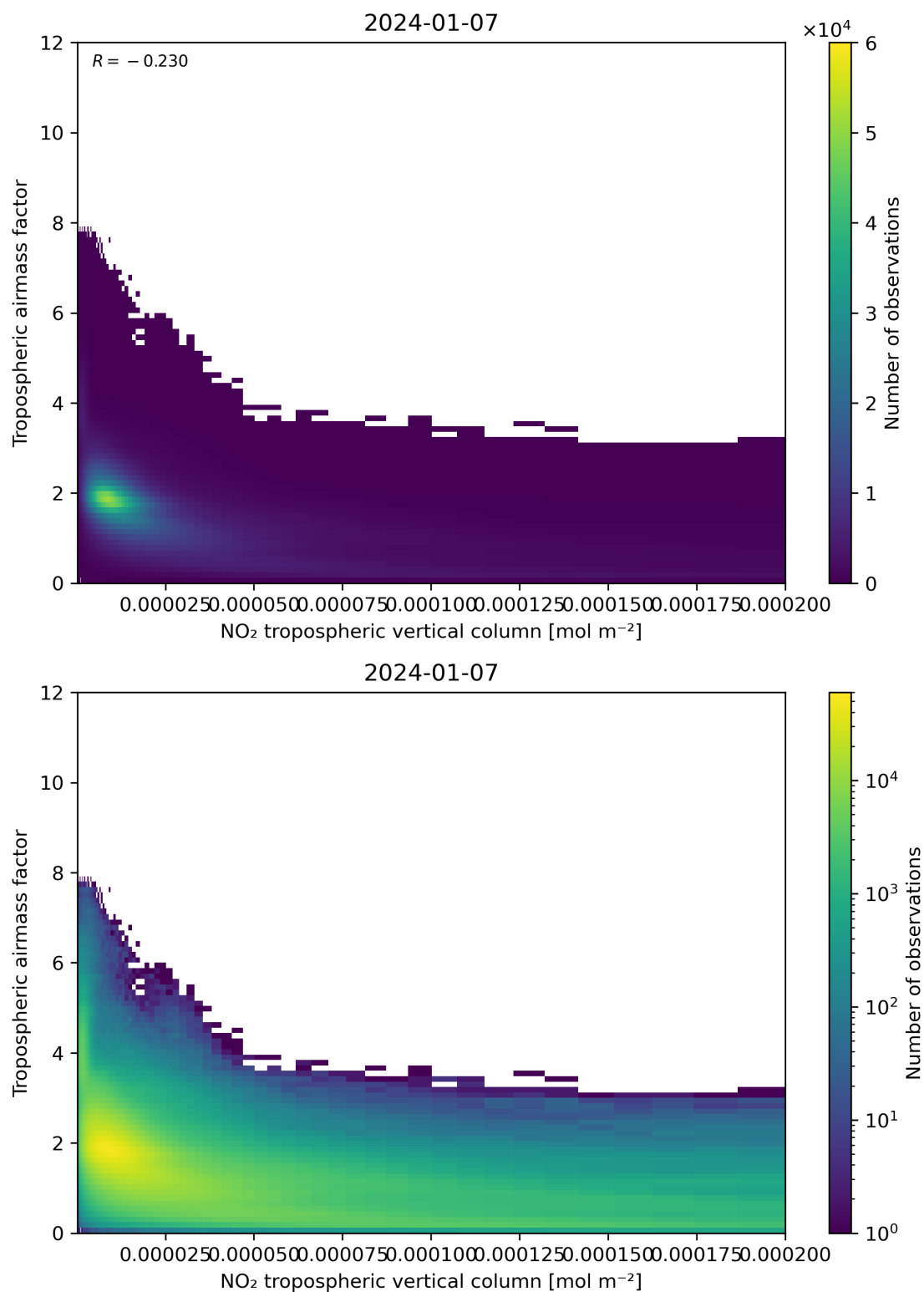
Figure 123: Scatter density plot of “NO 2 tropospheric vertical column” against “Tropospheric airmass factor” for 2024-01-06 to 2024-01-08.
