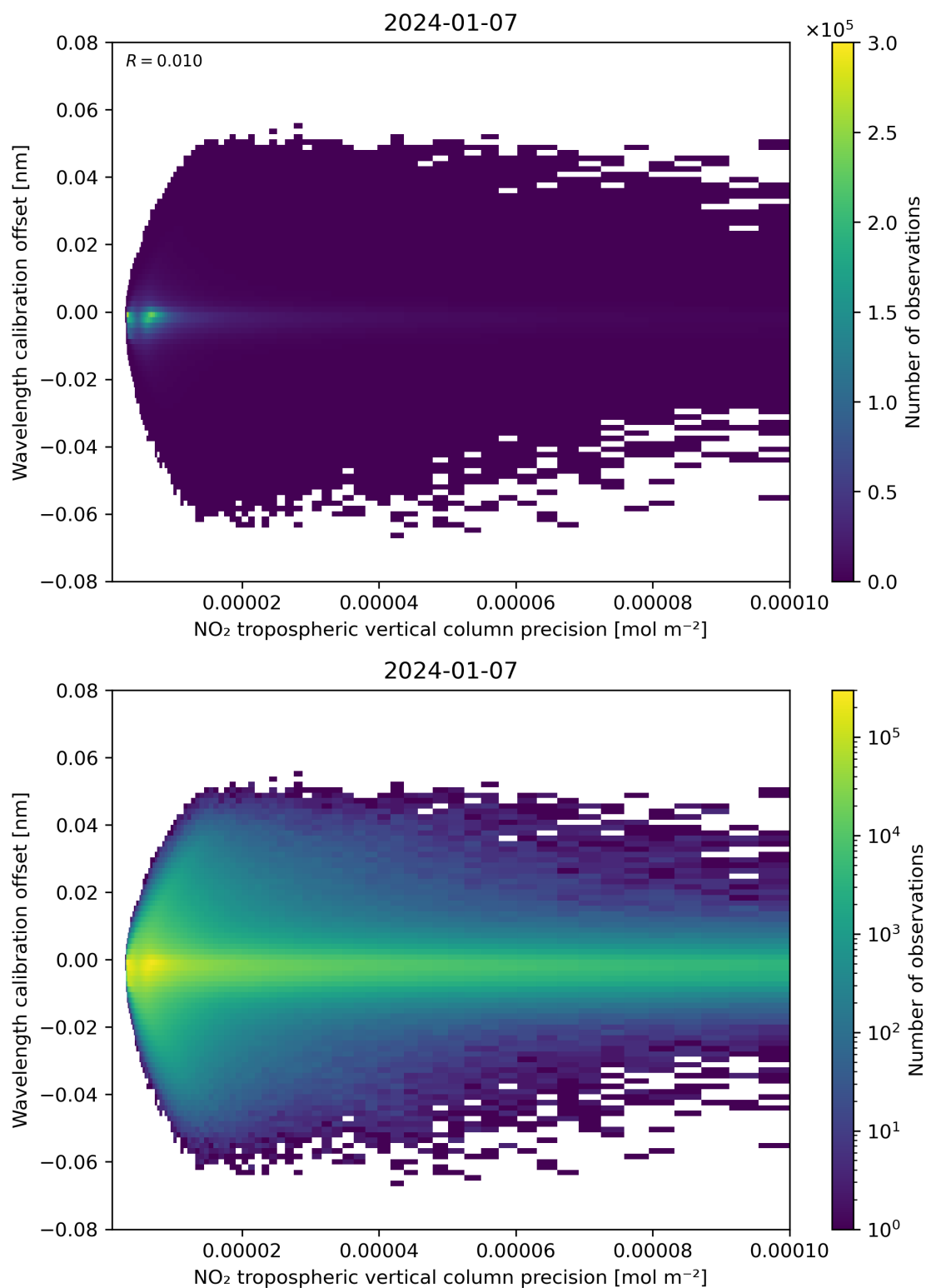
Figure 141: Scatter density plot of “NO 2 tropospheric vertical column precision” against “Wavelength calibration offset” for 2024-01-06 to 2024-01-08.
