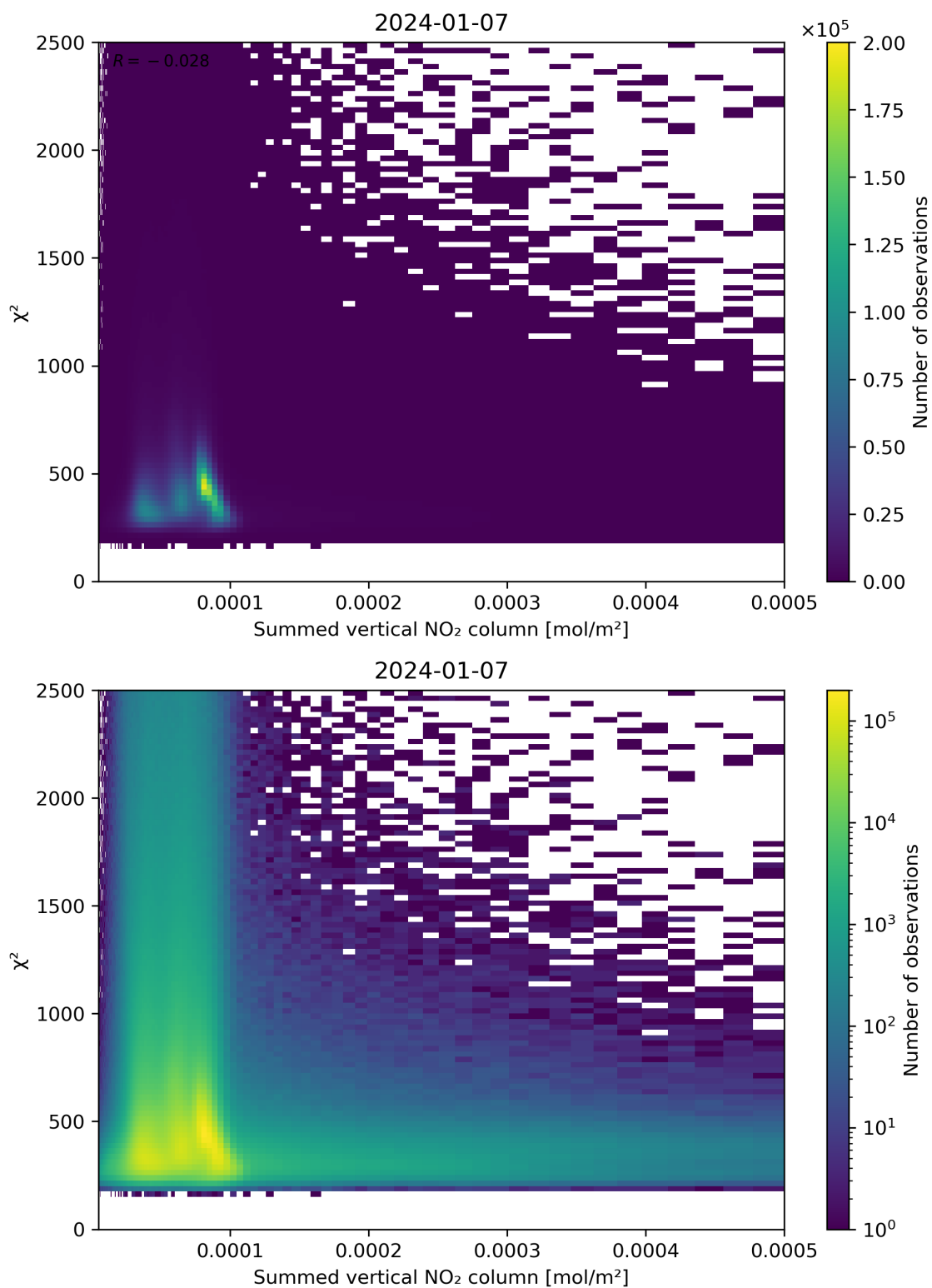
Figure 104: Scatter density plot of “Summed vertical NO 2 column” against “ \chi^2 ” for 2024-01-06 to 2024-01-08.
