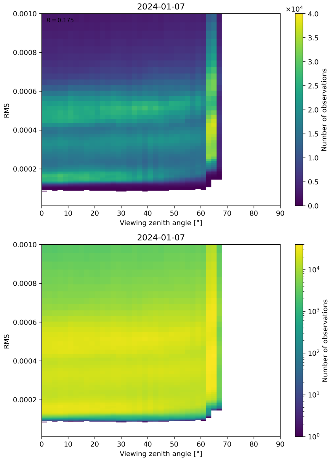
Figure 171: Scatter density plot of “Viewing zenith angle” against “RMS” for 2024-01-06 to 2024-01-08.
