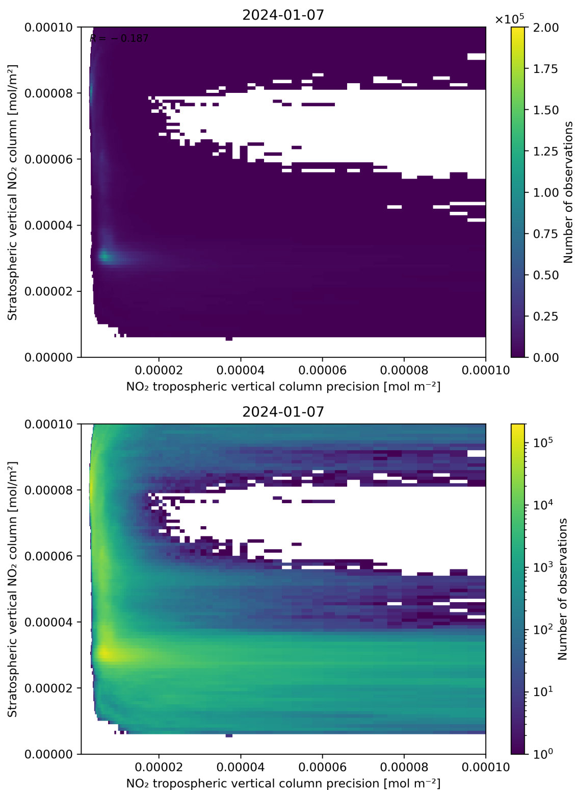
Figure 135: Scatter density plot of “NO 2 tropospheric vertical column precision” against “Stratospheric vertical NO 2 column” for 2024-01-06 to 2024-01-08.
