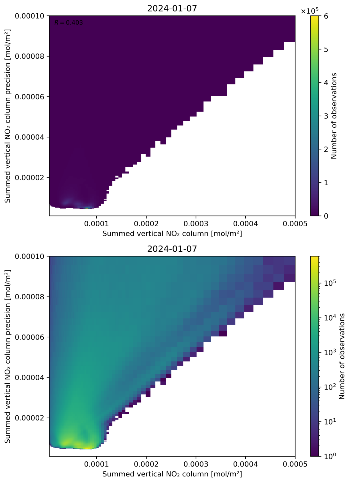
Figure 105: Scatter density plot of “Summed vertical NO 2 column” against “Summed vertical NO 2 column precision” for 2024-01-06 to 2024-01-08.
