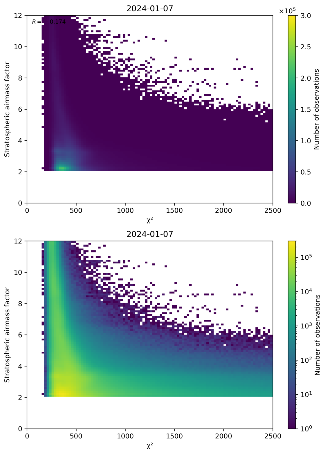
Figure 81: Scatter density plot of “ \chi^2 ” against “Stratospheric airmass factor” for 2024-01-06 to 2024-01-08.
