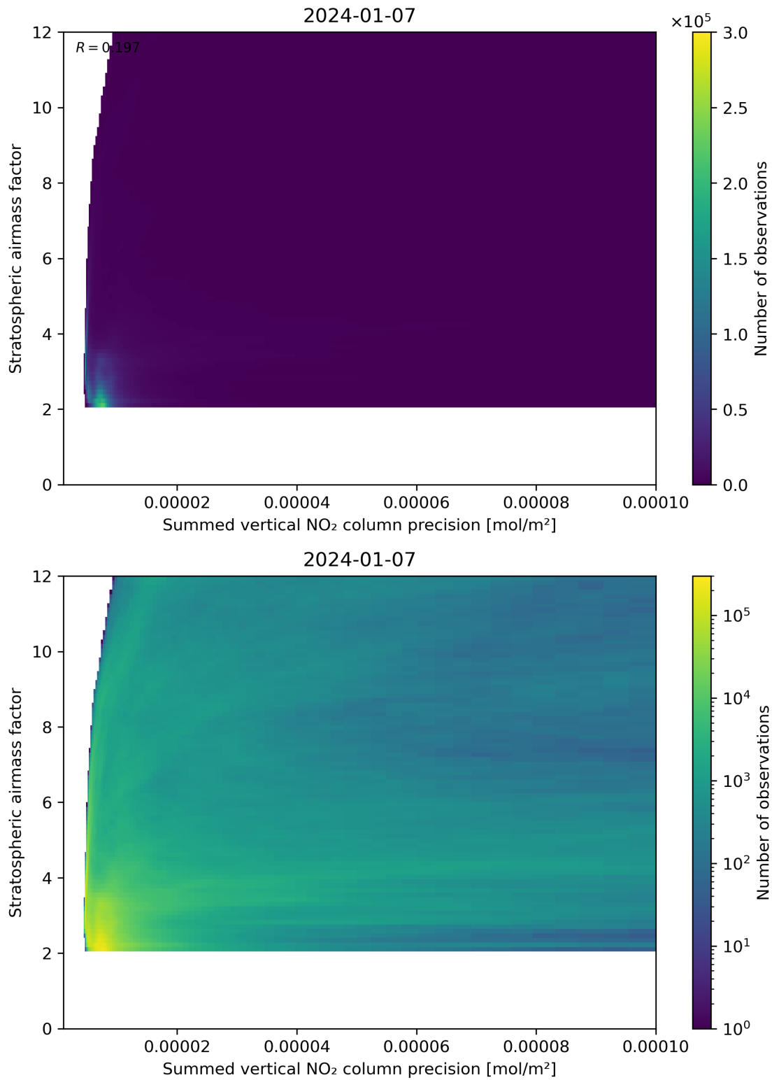
Figure 106: Scatter density plot of “Summed vertical NO 2 column precision” against “Stratospheric airmass factor” for 2024-01-06 to 2024-01-08.
