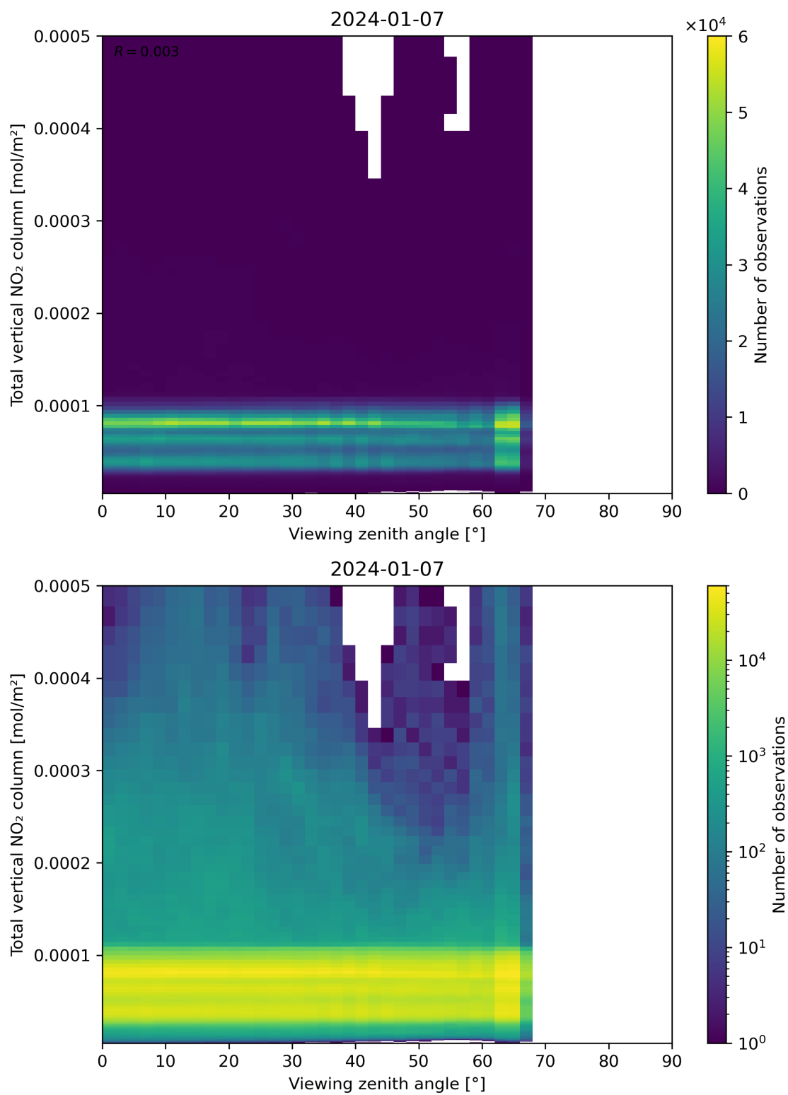
Figure 167: Scatter density plot of “Viewing zenith angle” against “Total vertical NO 2 column” for 2024-01-06 to 2024-01-08.
