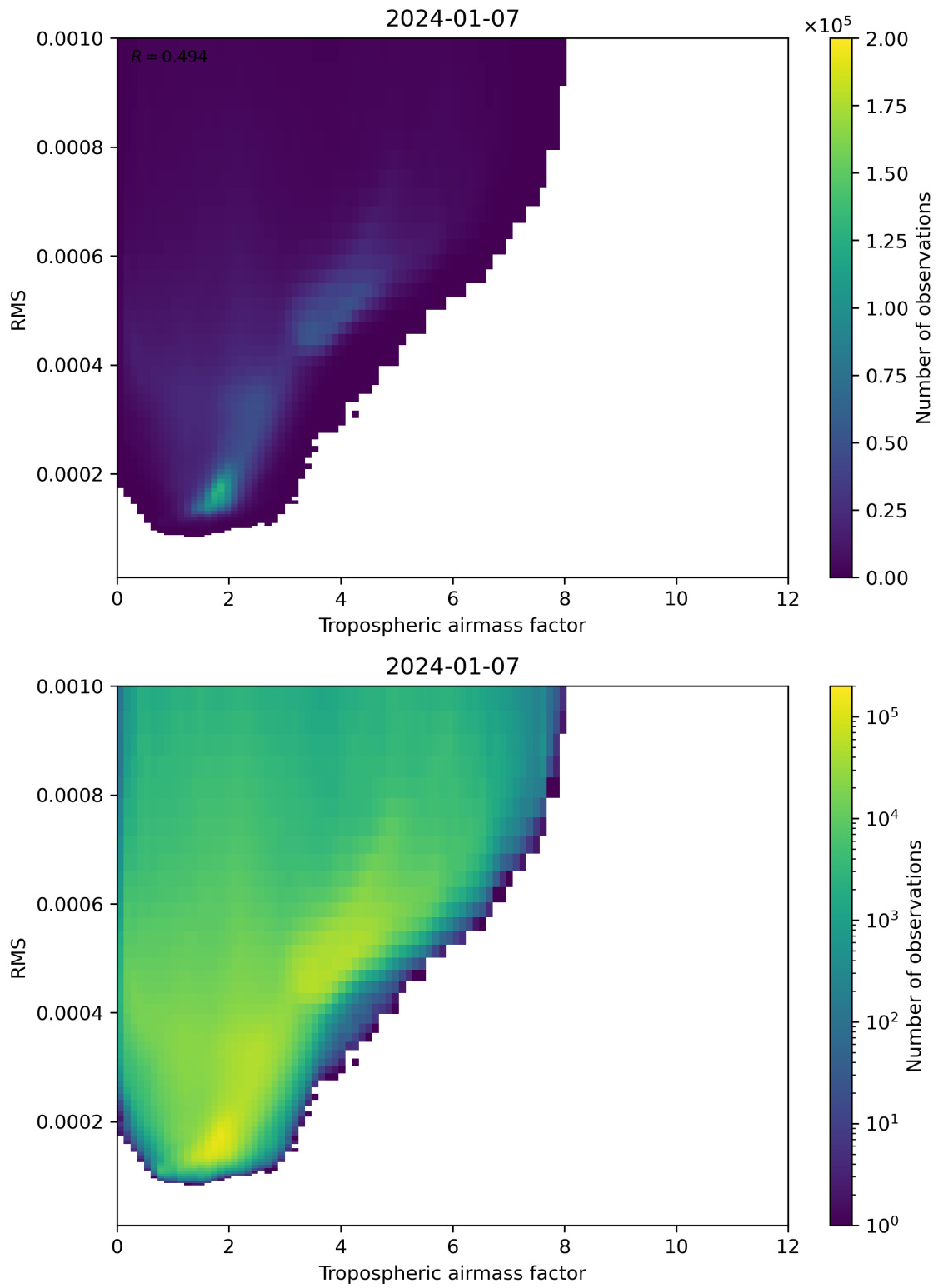
Figure 79: Scatter density plot of “Tropospheric airmass factor” against “RMS” for 2024-01-06 to 2024-01-08.
