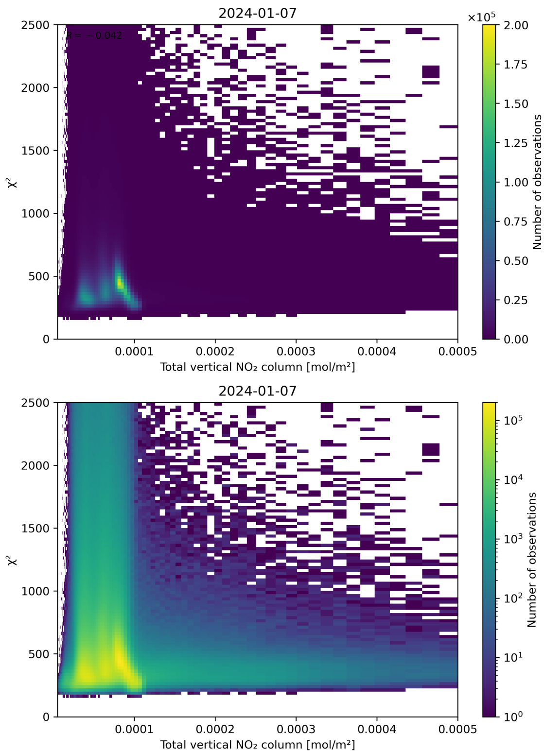
Figure 111: Scatter density plot of “Total vertical NO 2 column” against “ \chi^2 ” for 2024-01-06 to 2024-01-08.
