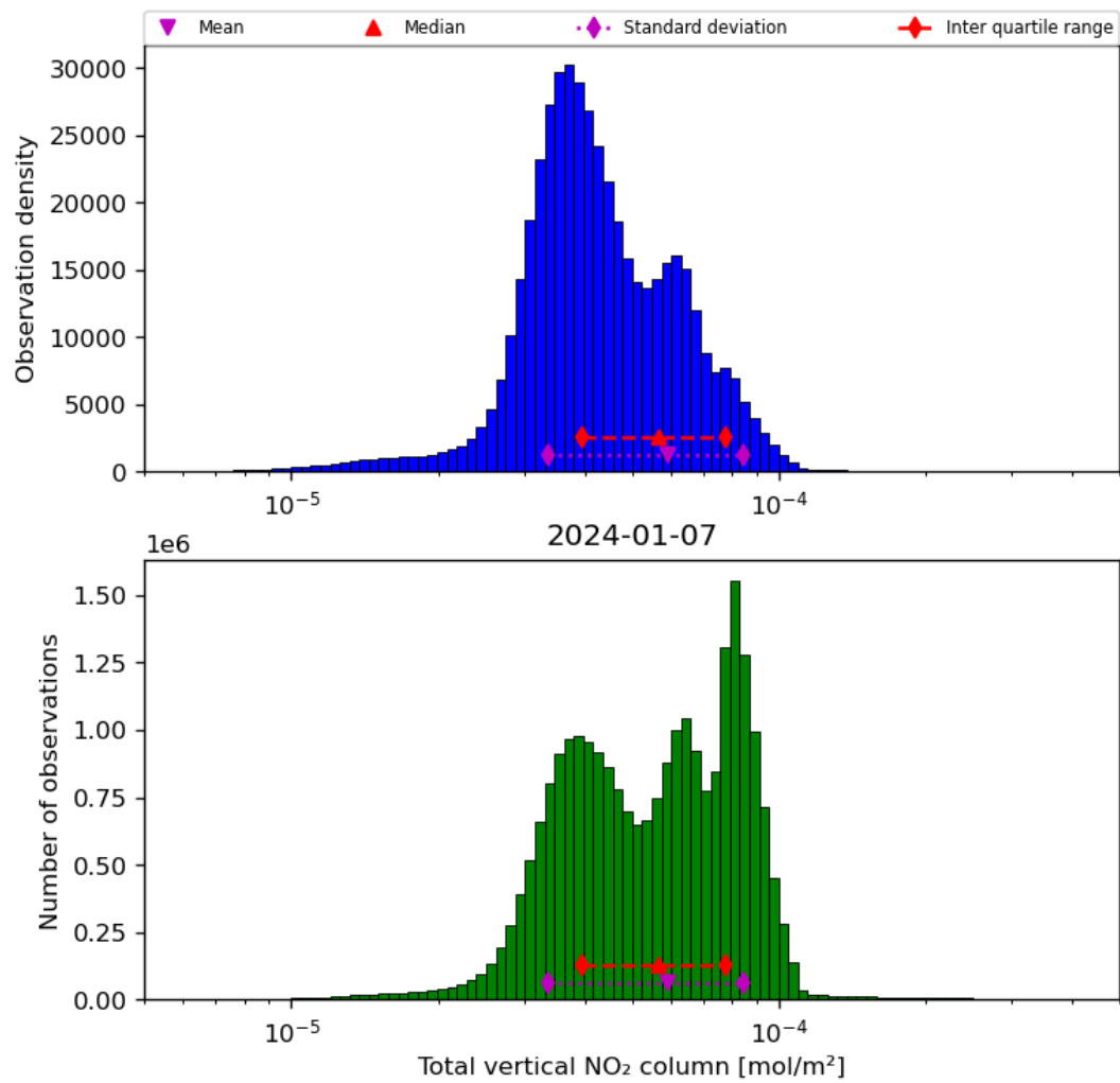
Figure 38: Histogram of “Total vertical NO 2 column” for 2024-01-06 to 2024-01-08
