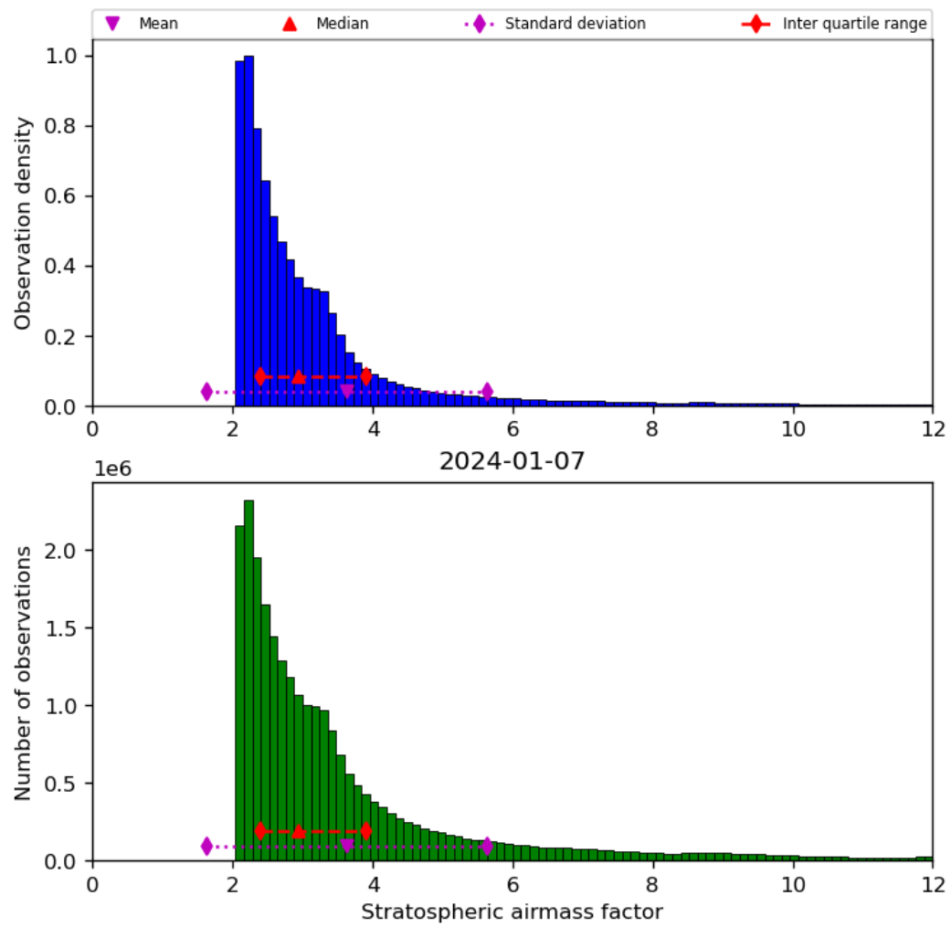
Figure 44: Histogram of “Stratospheric airmass factor” for 2024-01-06 to 2024-01-08
