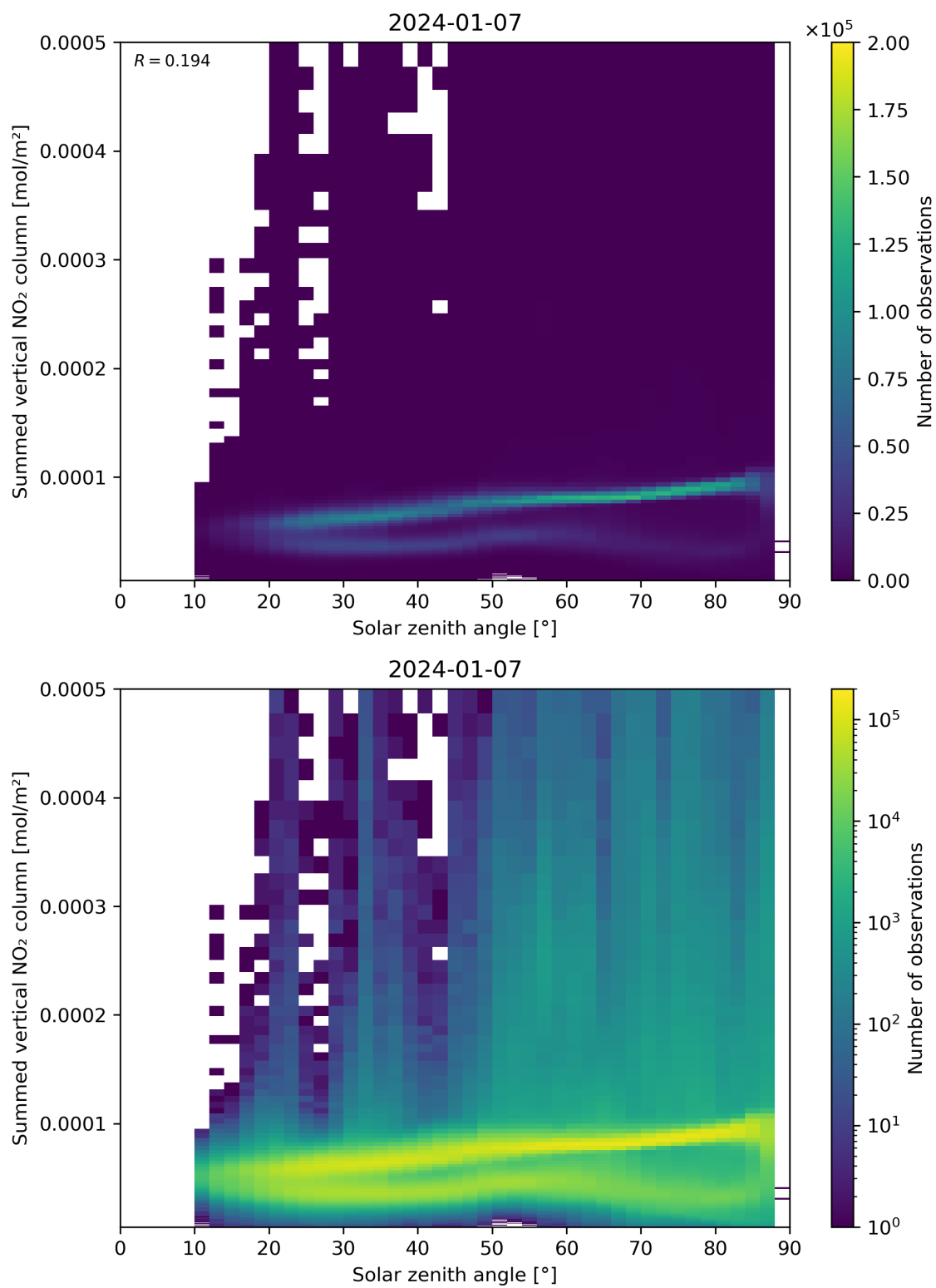
Figure 151: Scatter density plot of “Solar zenith angle” against “Summed vertical NO 2 column” for 2024-01-06 to 2024-01-08.
