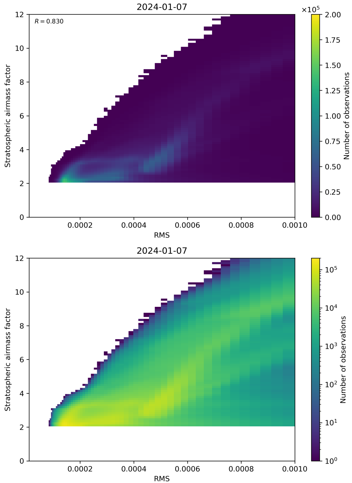
Figure 144: Scatter density plot of “RMS” against “Stratospheric airmass factor” for 2024-01-06 to 2024-01-08.
