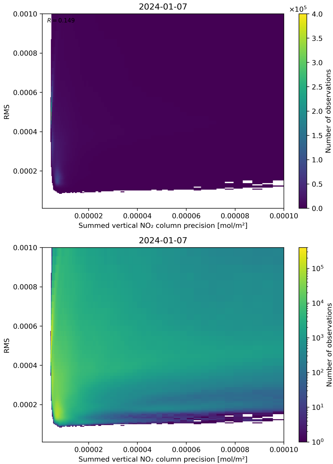
Figure 108: Scatter density plot of “Summed vertical NO 2 column precision” against “RMS” for 2024-01-06 to 2024-01-08.
