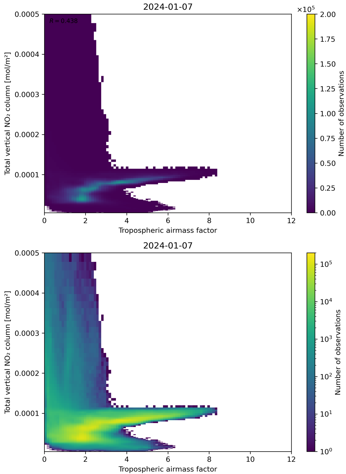
Figure 77: Scatter density plot of “Tropospheric airmass factor” against “Total vertical NO 2 column” for 2024-01-06 to 2024-01-08.
