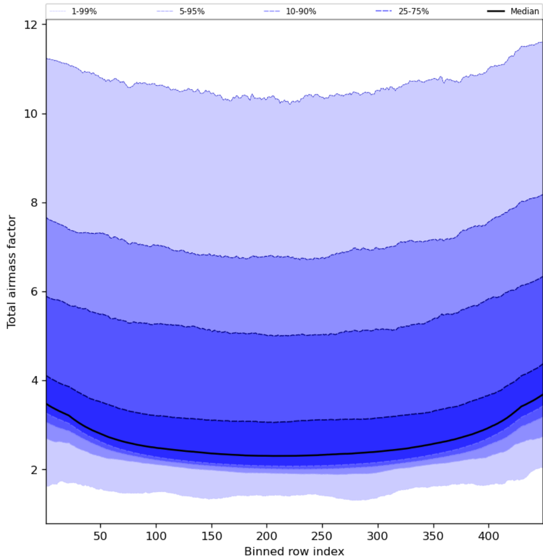
Figure 49: Along track statistics of “Total airmass factor” for 2024-01-06 to 2024-01-08
