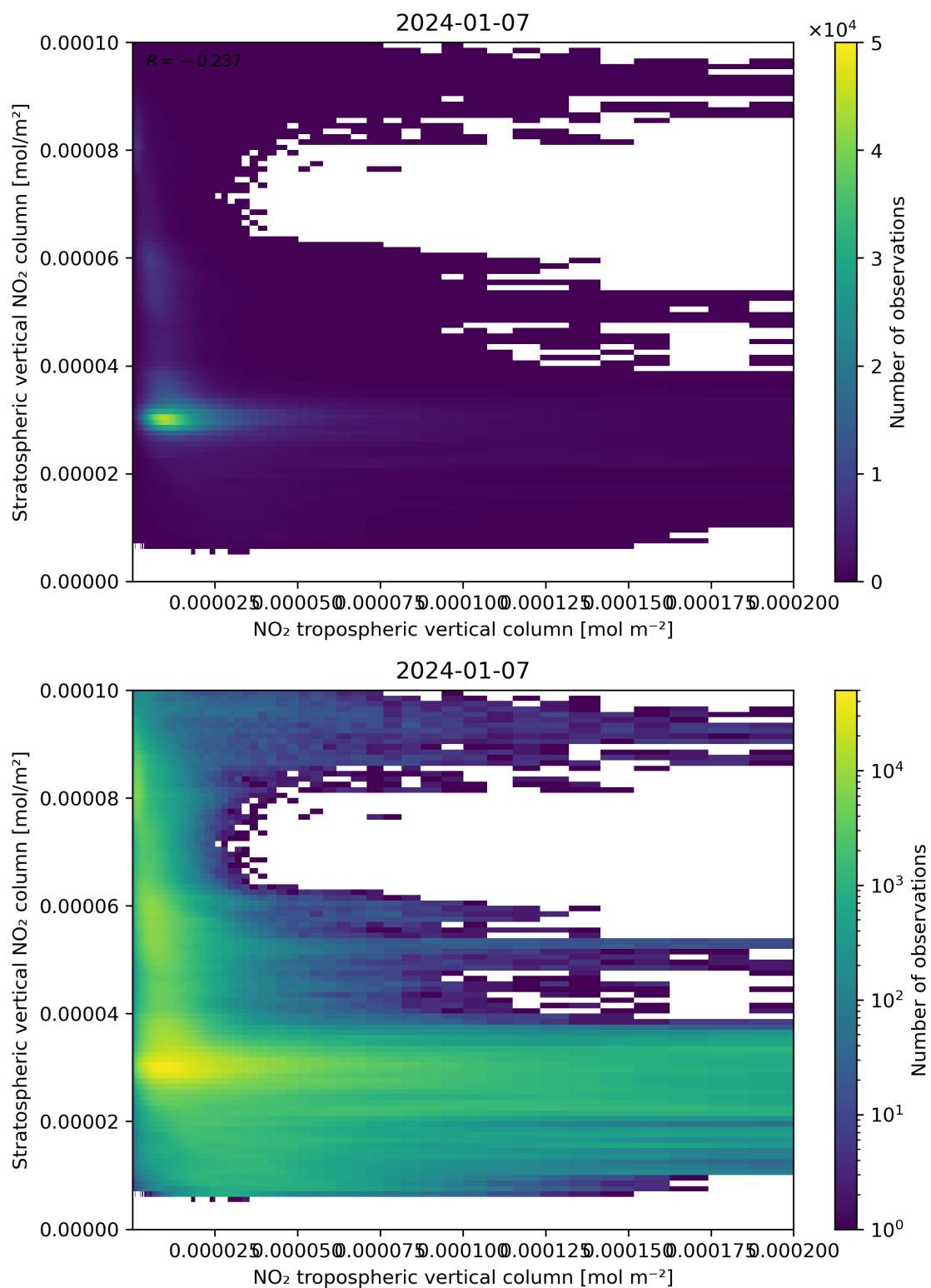
Figure 125: Scatter density plot of “NO 2 tropospheric vertical column” against “Stratospheric vertical NO 2 column” for 2024-01-06 to 2024-01-08.
