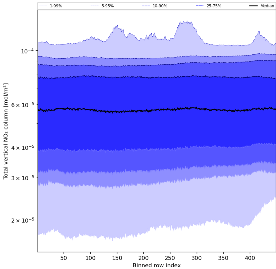
Figure 55: Along track statistics of “Total vertical NO 2 column” for 2024-01-06 to 2024-01-08
