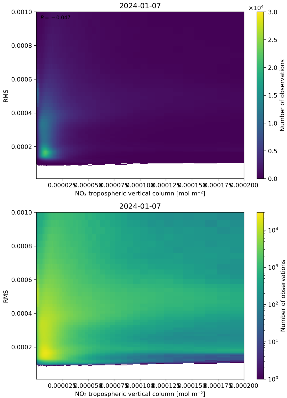
Figure 142: Scatter density plot of “NO 2 tropospheric vertical column” against “RMS” for 2024-01-06 to 2024-01-08.
