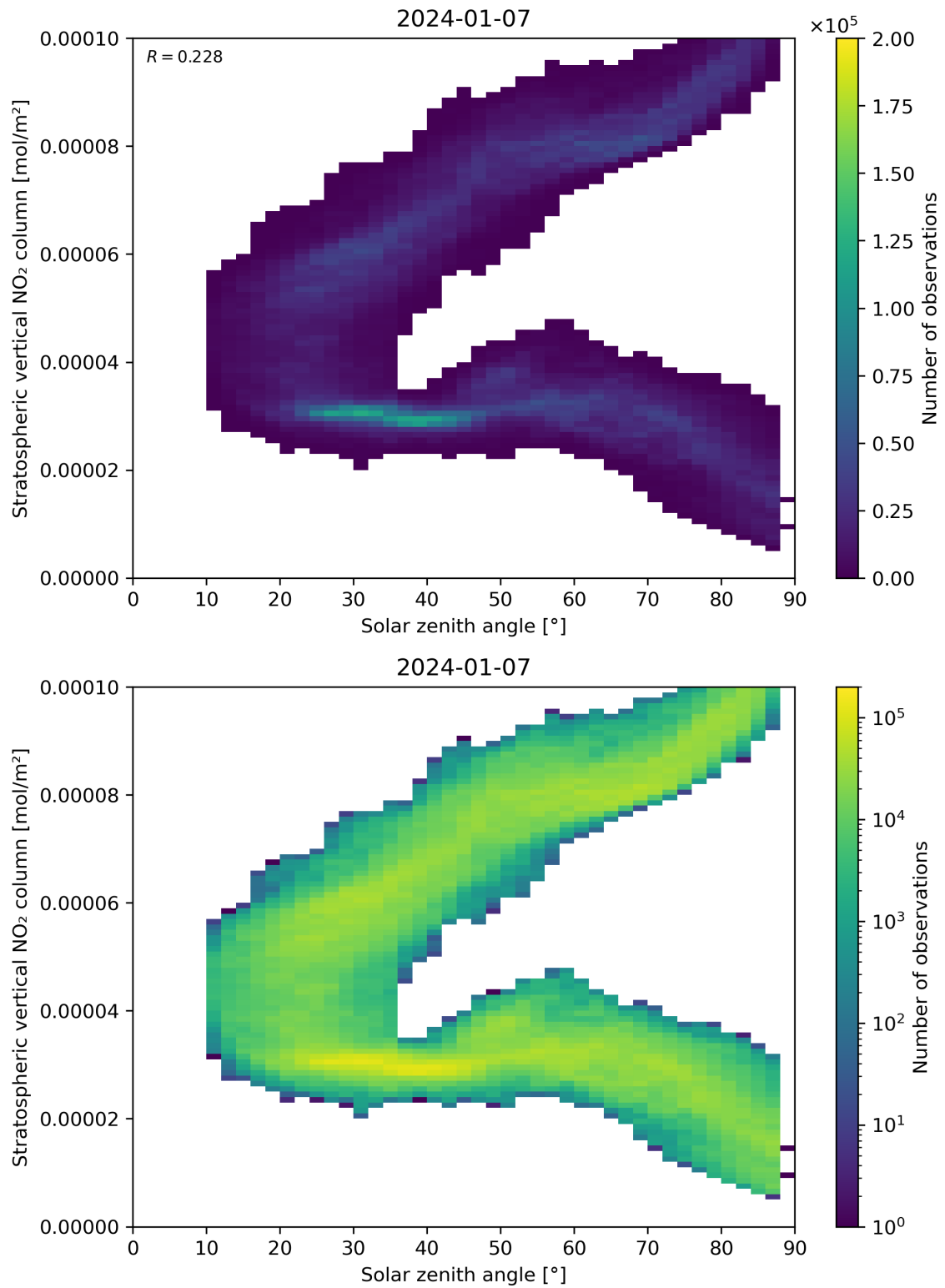
Figure 150: Scatter density plot of “Solar zenith angle” against “Stratospheric vertical NO 2 column” for 2024-01-06 to 2024-01-08.
