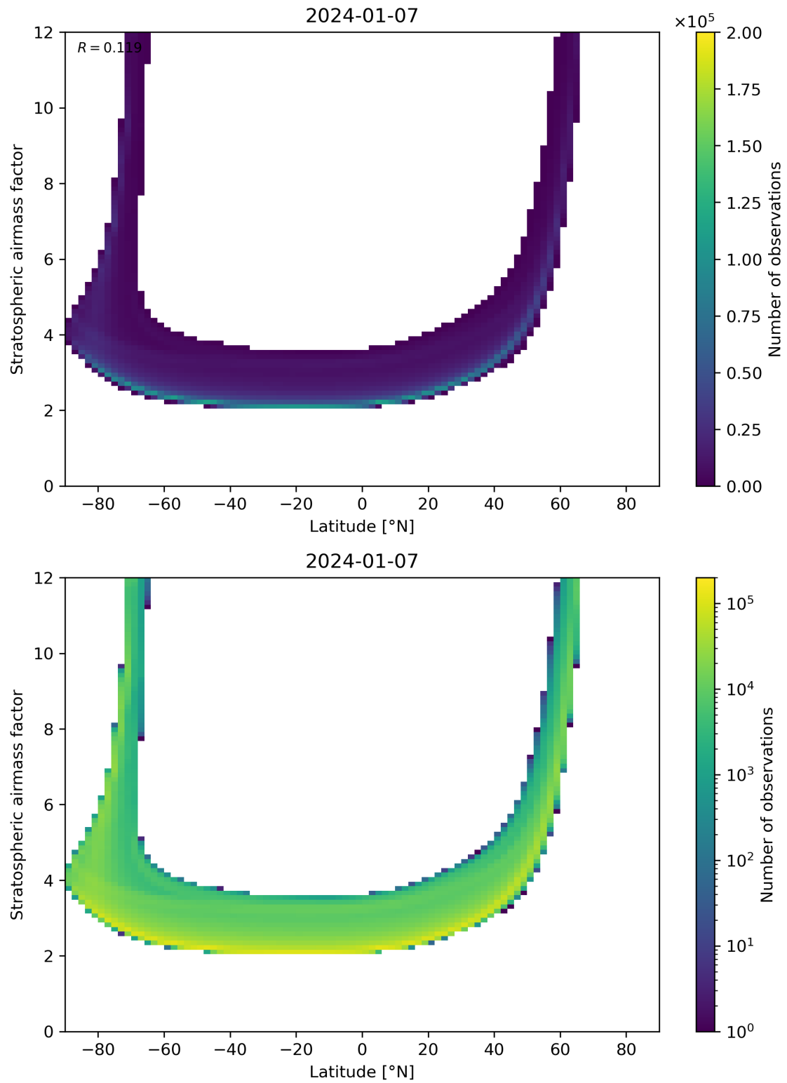
Figure 83: Scatter density plot of “Latitude” against “Stratospheric airmass factor” for 2024-01-06 to 2024-01-08.
