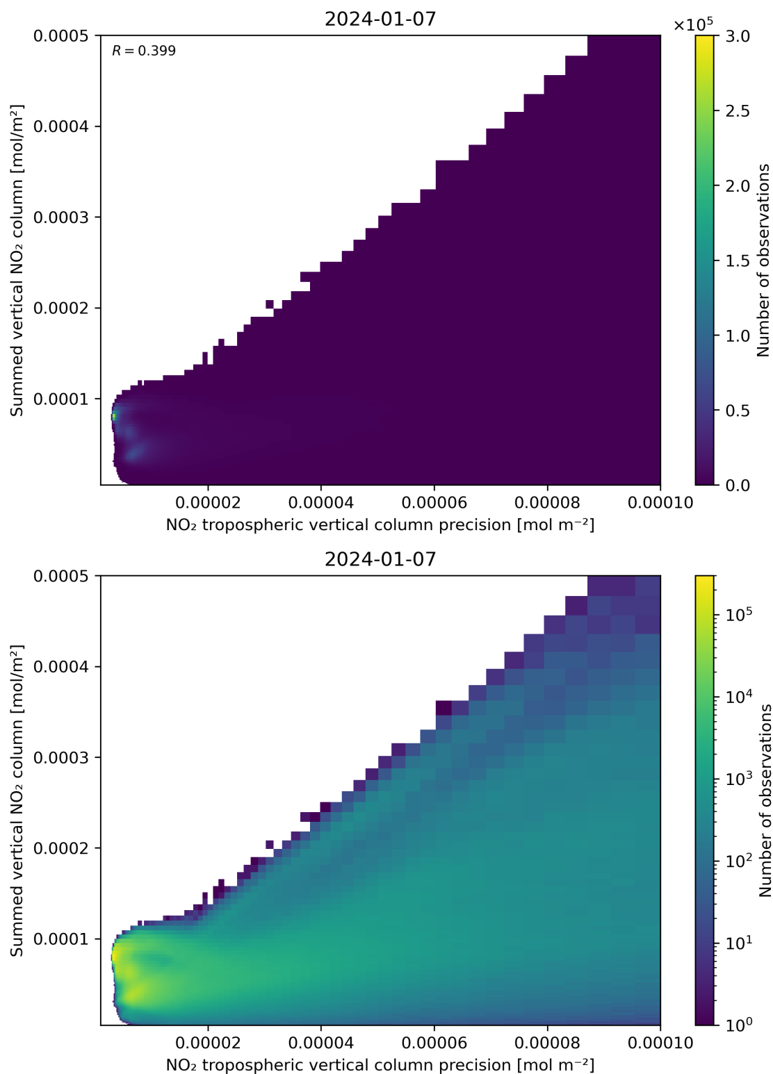
Figure 136: Scatter density plot of “NO 2 tropospheric vertical column precision” against “Summed vertical NO 2 column” for 2024-01-06 to 2024-01-08.
