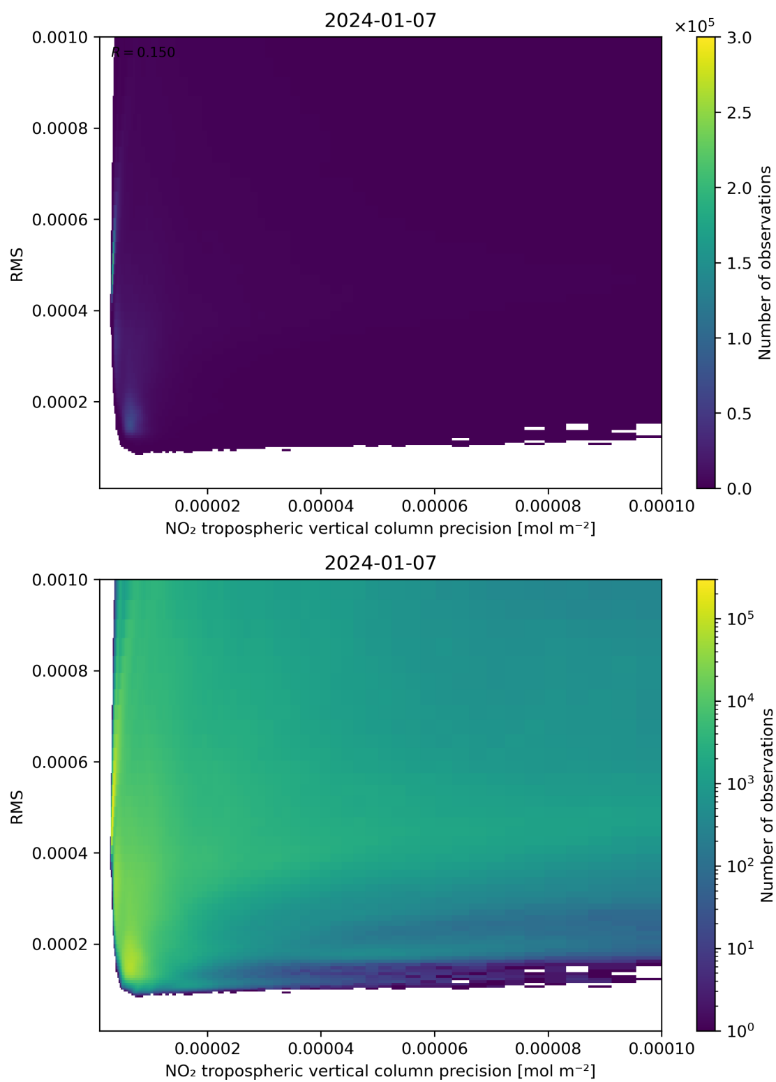
Figure 140: Scatter density plot of “NO 2 tropospheric vertical column precision” against “RMS” for 2024-01-06 to 2024-01-08.
