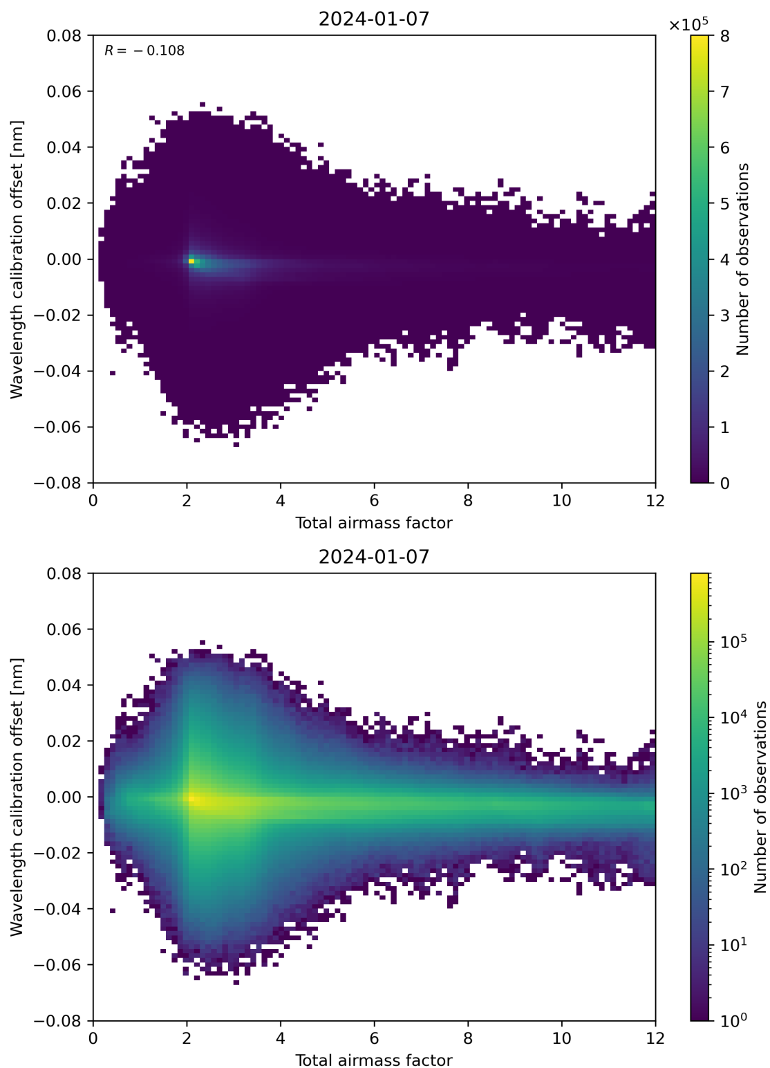
Figure 70: Scatter density plot of “Total airmass factor” against “Wavelength calibration offset” for 2024-01-06 to 2024-01-08.
