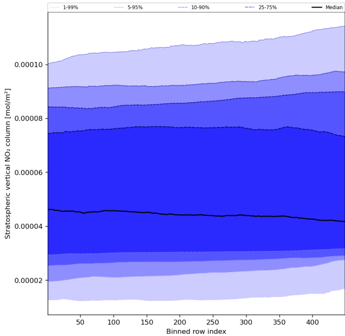
Figure 53: Along track statistics of “Stratospheric vertical NO 2 column” for 2024-01-06 to 2024-01-08
