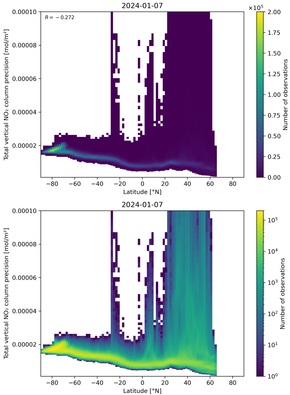
Figure 91: Scatter density plot of “Latitude” against “Total vertical NO 2 column precision” for 2024-01-06 to 2024-01-08.
