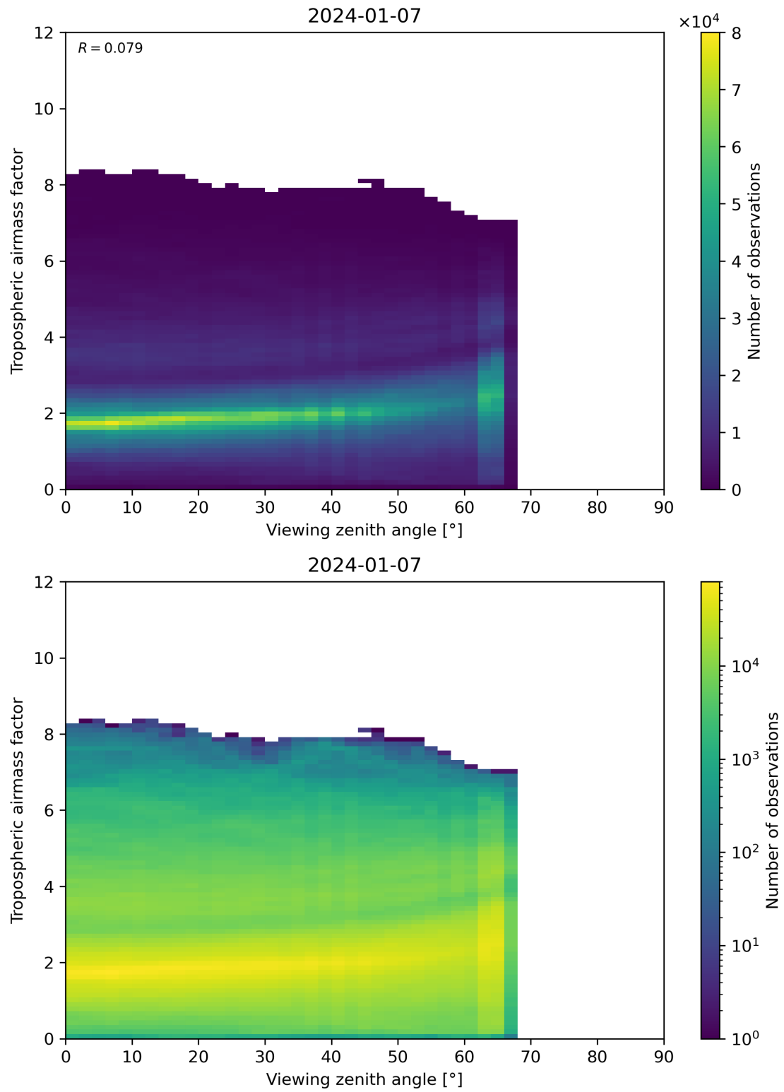
Figure 161: Scatter density plot of “Viewing zenith angle” against “Tropospheric airmass factor” for 2024-01-06 to 2024-01-08.
