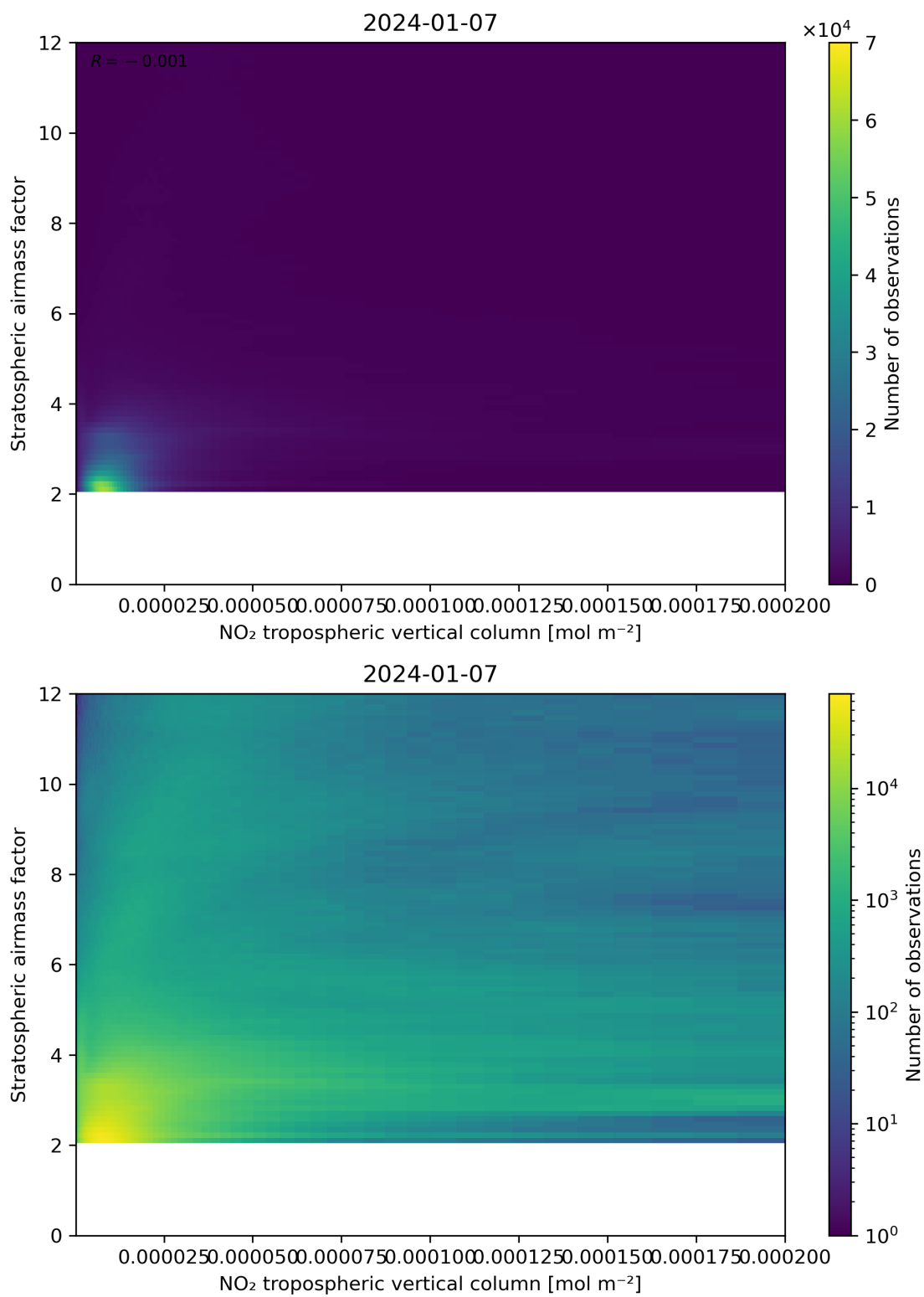
Figure 121: Scatter density plot of “NO 2 tropospheric vertical column” against “Stratospheric airmass factor” for 2024-01-06 to 2024-01-08.
