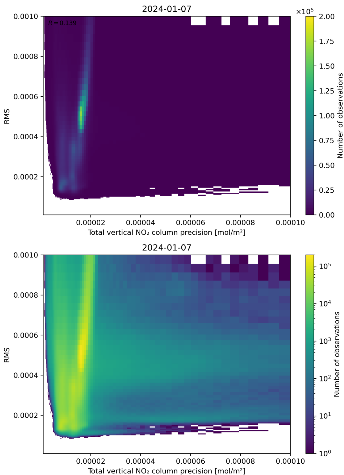
Figure 119: Scatter density plot of “Total vertical NO 2 column precision” against “RMS” for 2024-01-06 to 2024-01-08.
