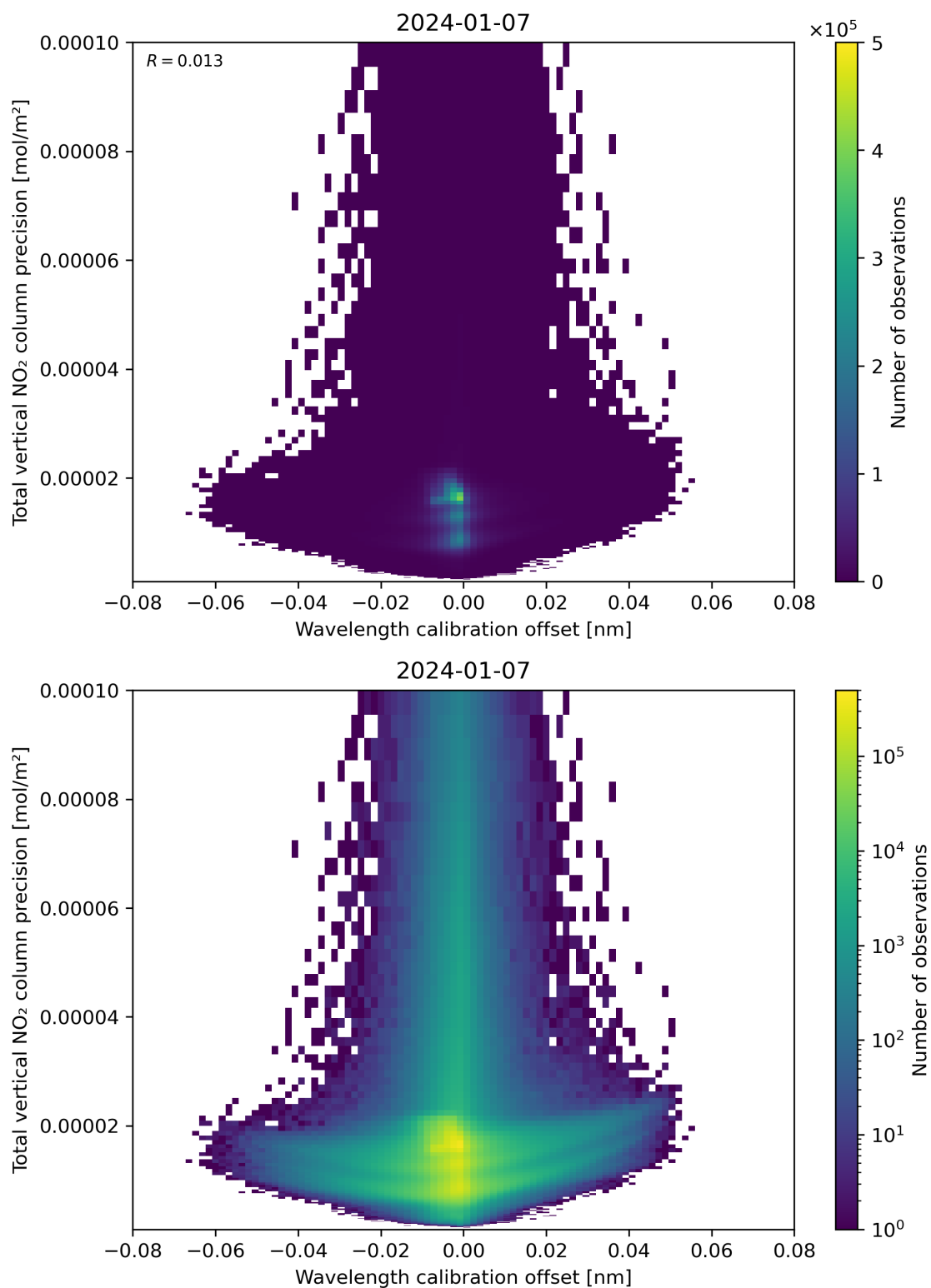
Figure 180: Scatter density plot of “Wavelength calibration offset” against “Total vertical NO 2 column precision” for 2024-01-06 to 2024-01-08.
