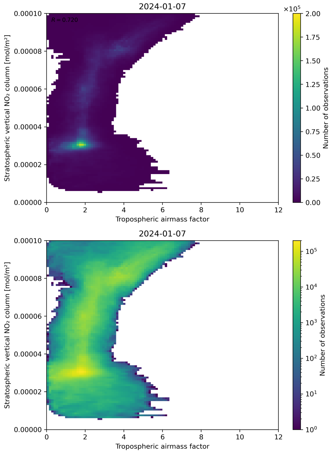
Figure 74: Scatter density plot of “Tropospheric air mass factor” against “Stratospheric vertical NO 2 column” for 2024-01-06 to 2024-01-08.
