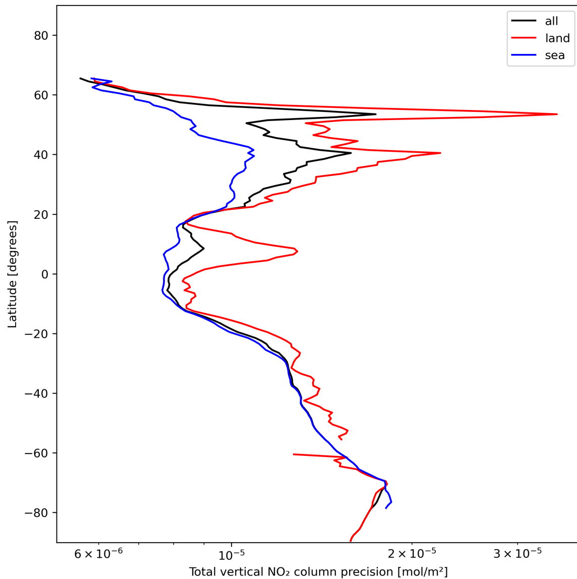
Figure 22: Zonal average of “Total vertical NO 2 column precision” for 2024-01-06 to 2024-01-08.
