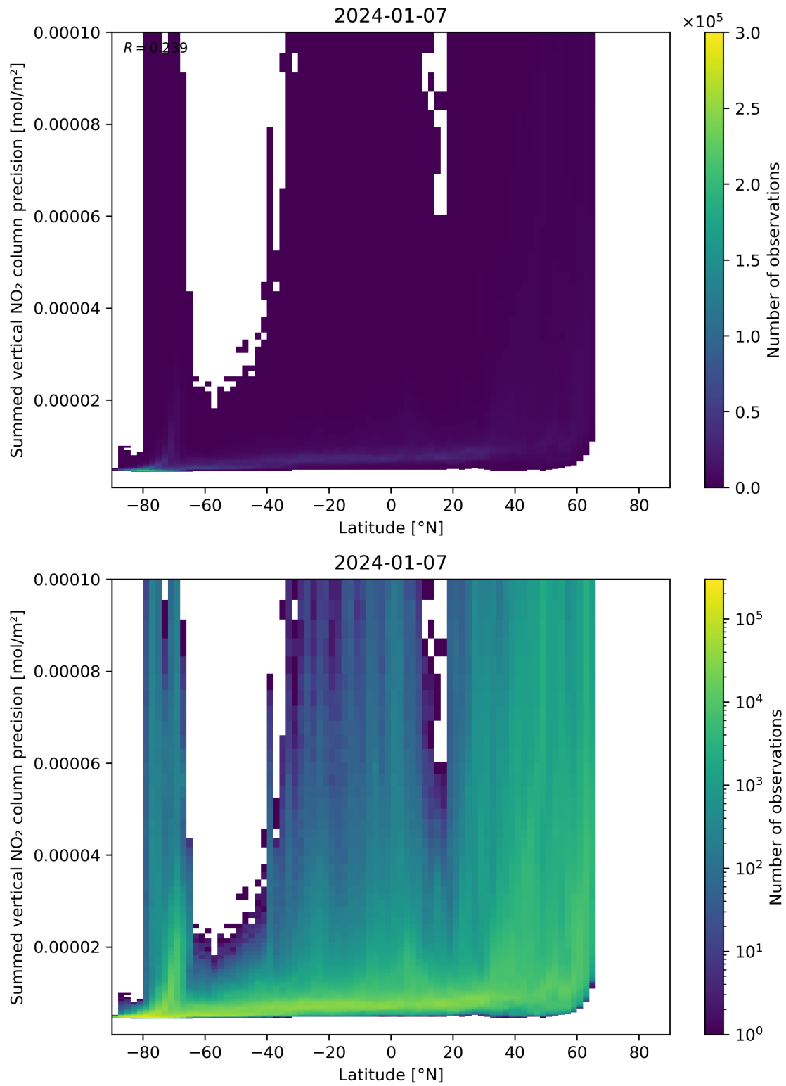
Figure 89: Scatter density plot of “Latitude” against “Summed vertical NO 2 column precision” for 2024-01-06 to 2024-01-08.
