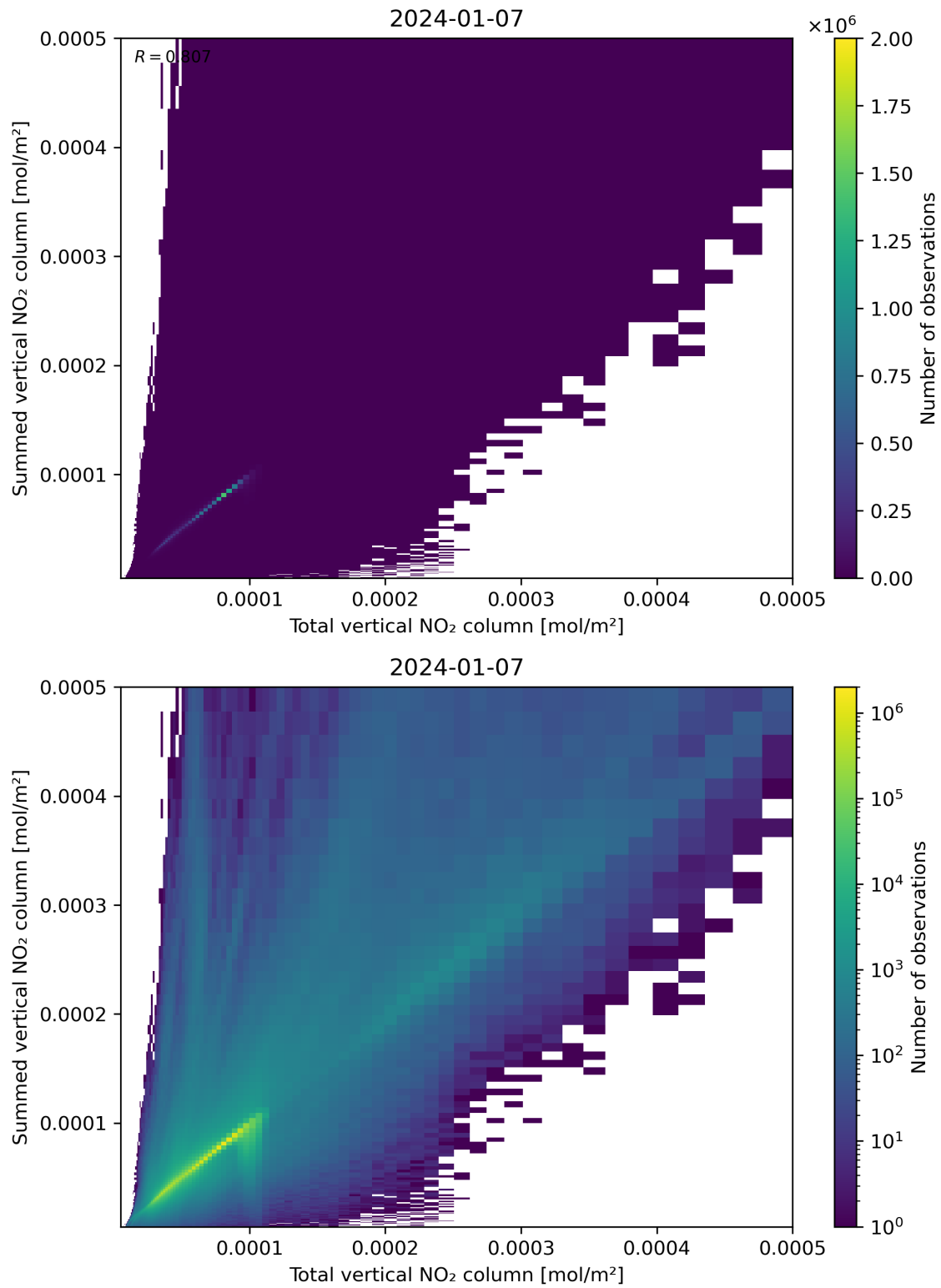
Figure 112: Scatter density plot of “Total vertical NO 2 column” against “Summed vertical NO 2 column” for 2024-01-06 to 2024-01-08.
