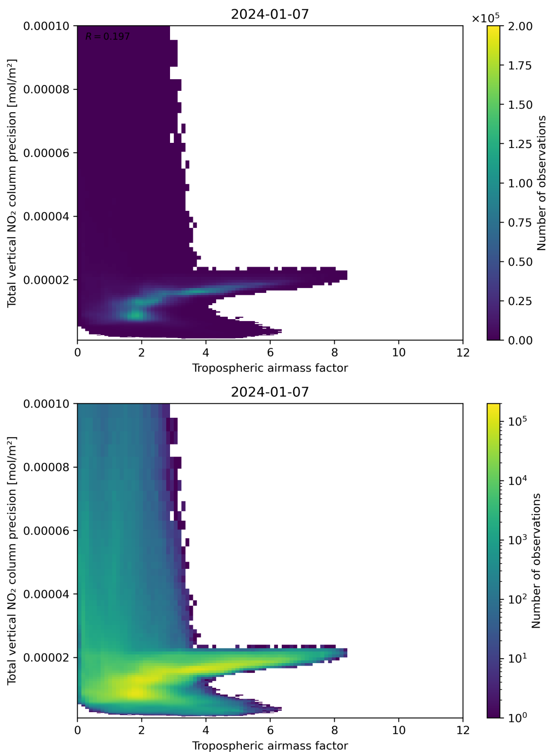
Figure 78: Scatter density plot of “Tropospheric air mass factor” against “Total vertical NO 2 column precision” for 2024-01-06 to 2024-01-08.
