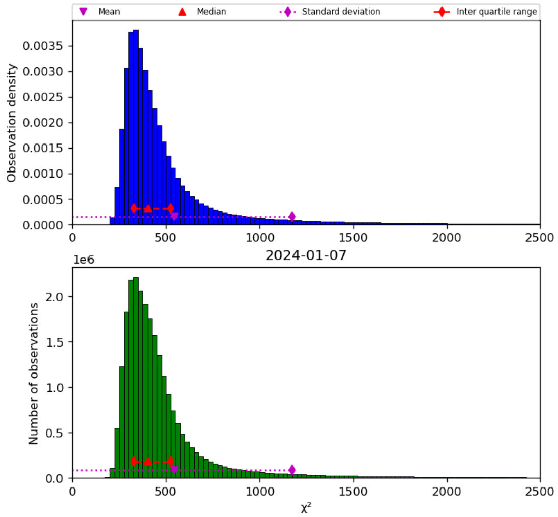
Figure 42: Histogram of " \chi^2 " for 2024-01-06 to 2024-01-08
