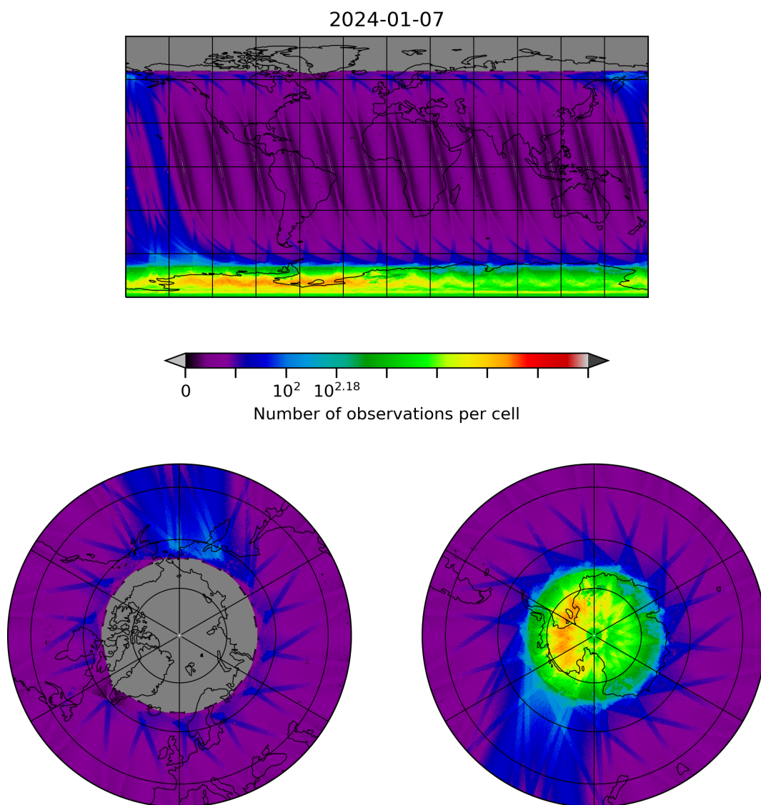
Figure 10: Map of the number of observations for 2024-01-06 to 2024-01-08
