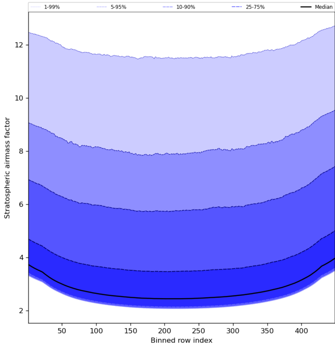
Figure 61: Along track statistics of “Stratospheric airmass factor” for 2024-01-06 to 2024-01-08
