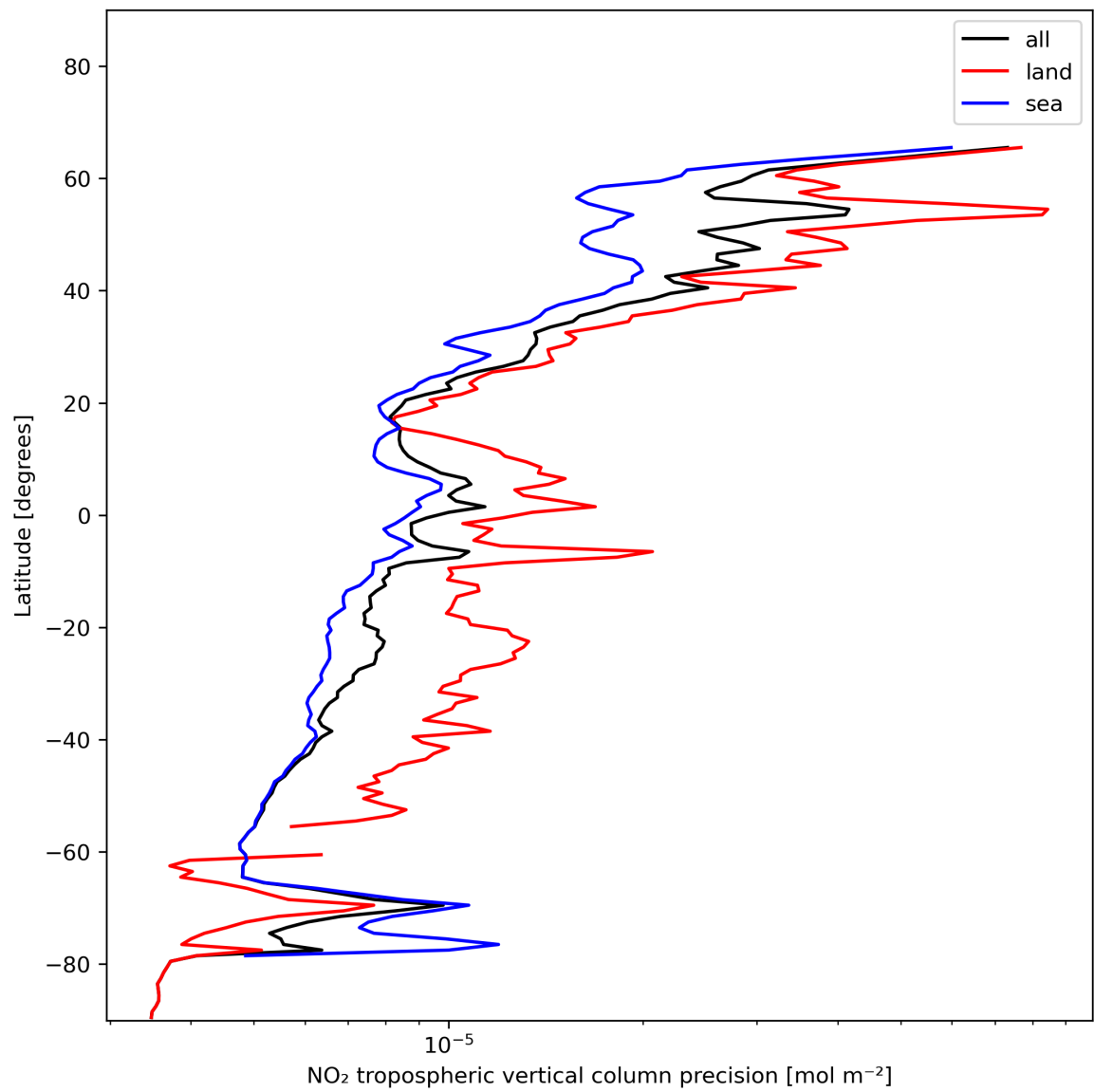
Figure 13: Zonal average of “NO 2 tropospheric vertical column precision” for 2024-01-06 to 2024-01-08.
