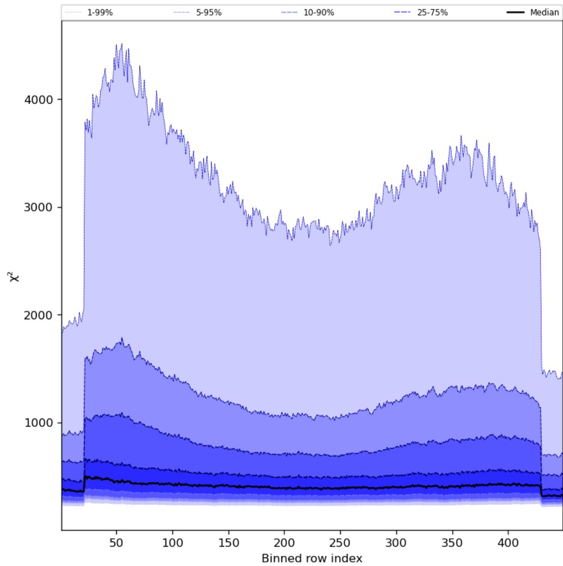
Figure 59: Along track statistics of “ \chi^2 ” for 2024-01-06 to 2024-01-08
