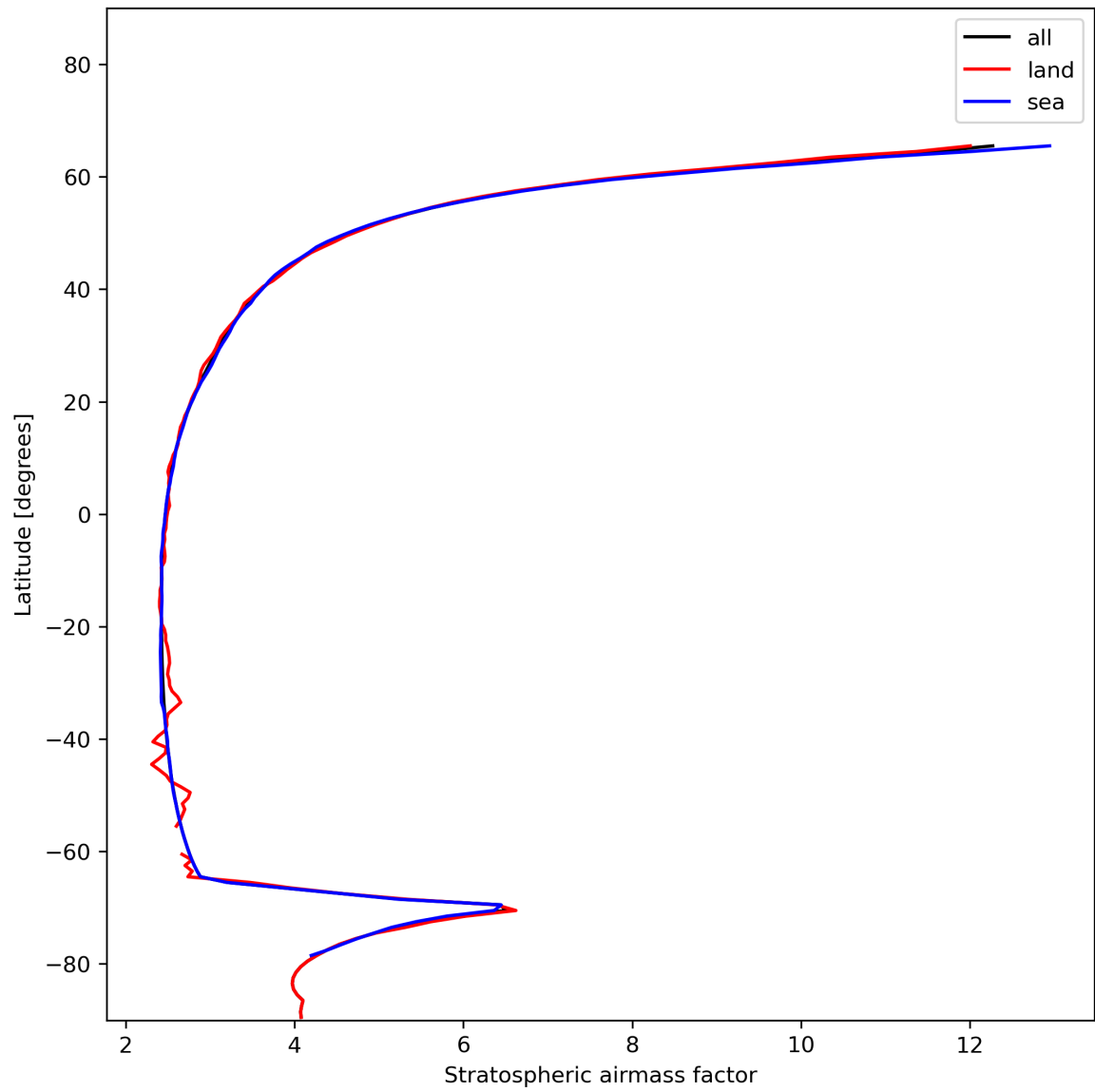
Figure 27: Zonal average of “Stratospheric airmass factor” for 2024-01-06 to 2024-01-08.
