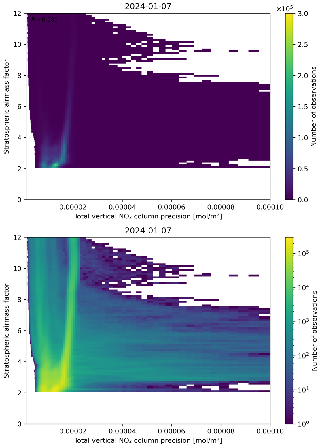
Figure 115: Scatter density plot of “Total vertical NO 2 column precision” against “Stratospheric air mass factor” for 2024-01-06 to 2024-01-08.
