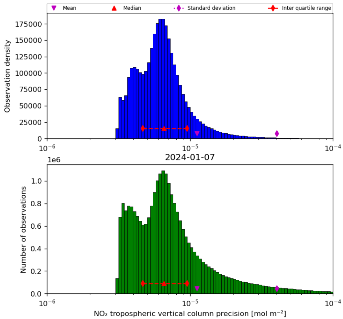
Figure 30: Histogram of “NO 2 tropospheric vertical column precision” for 2024-01-06 to 2024-01-08
