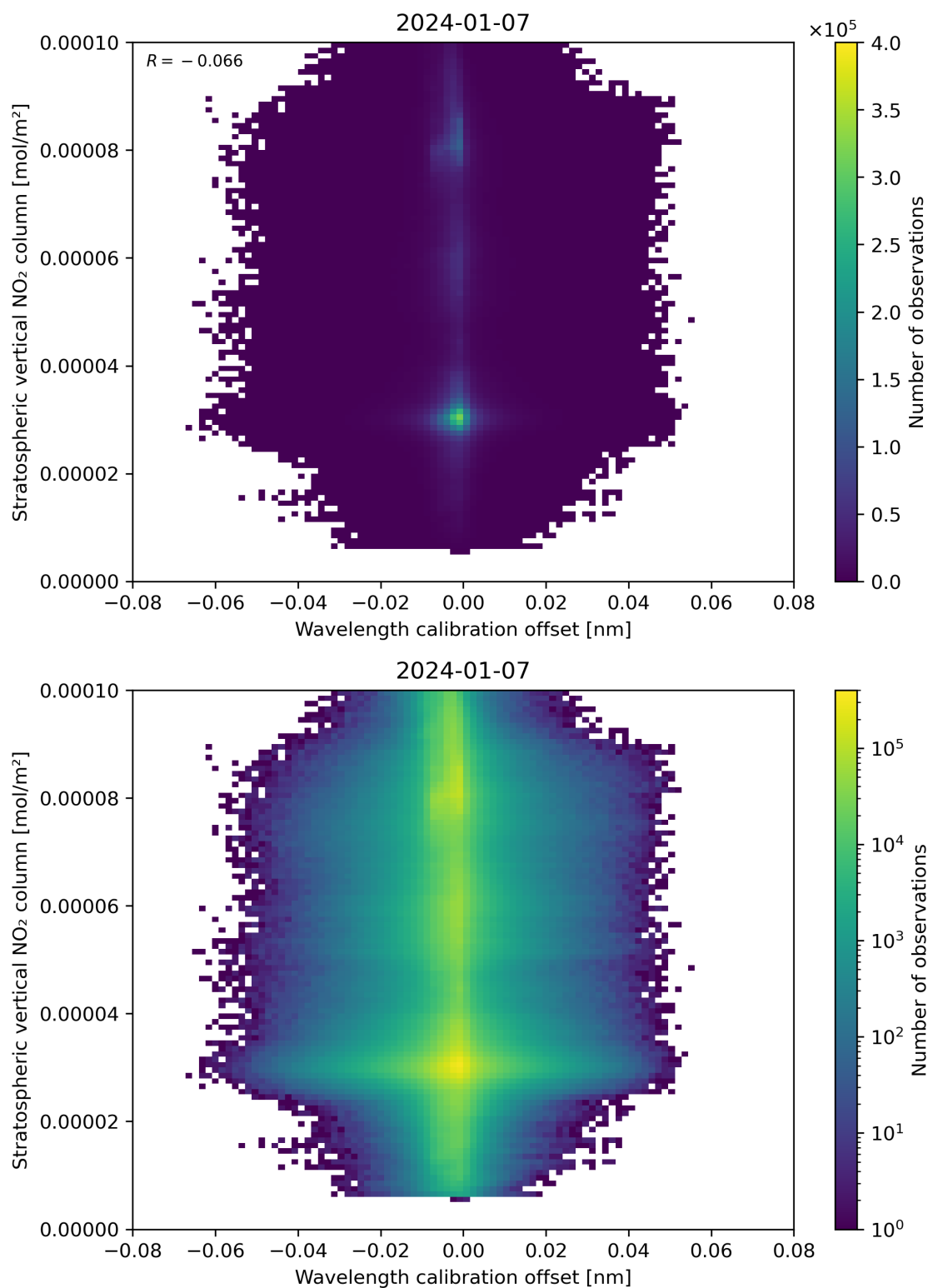
Figure 176: Scatter density plot of “Wavelength calibration offset” against “Stratospheric vertical NO 2 column” for 2024-01-06 to 2024-01-08.
