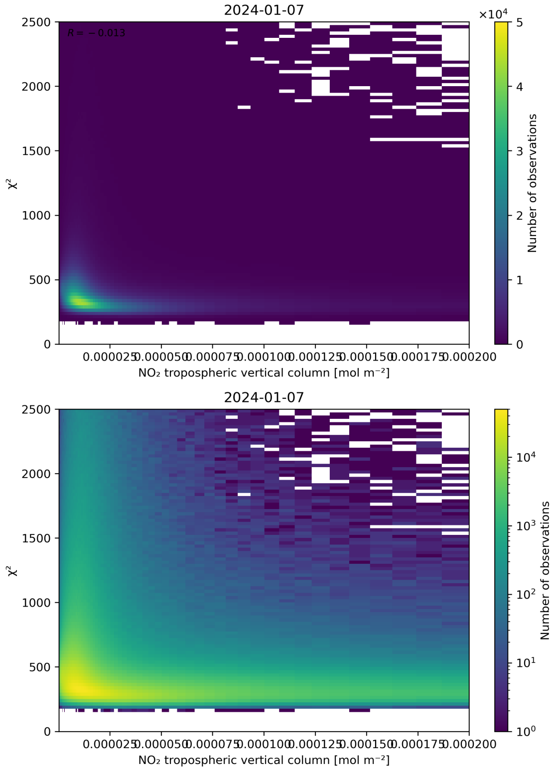
Figure 124: Scatter density plot of “NO 2 tropospheric vertical column” against “ \chi^2 ” for 2024-01-06 to 2024-01-08.
