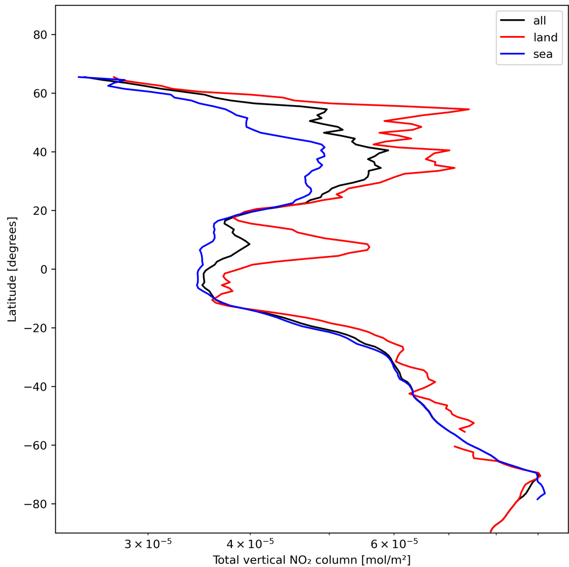
Figure 21: Zonal average of “Total vertical NO 2 column” for 2024-01-06 to 2024-01-08.
