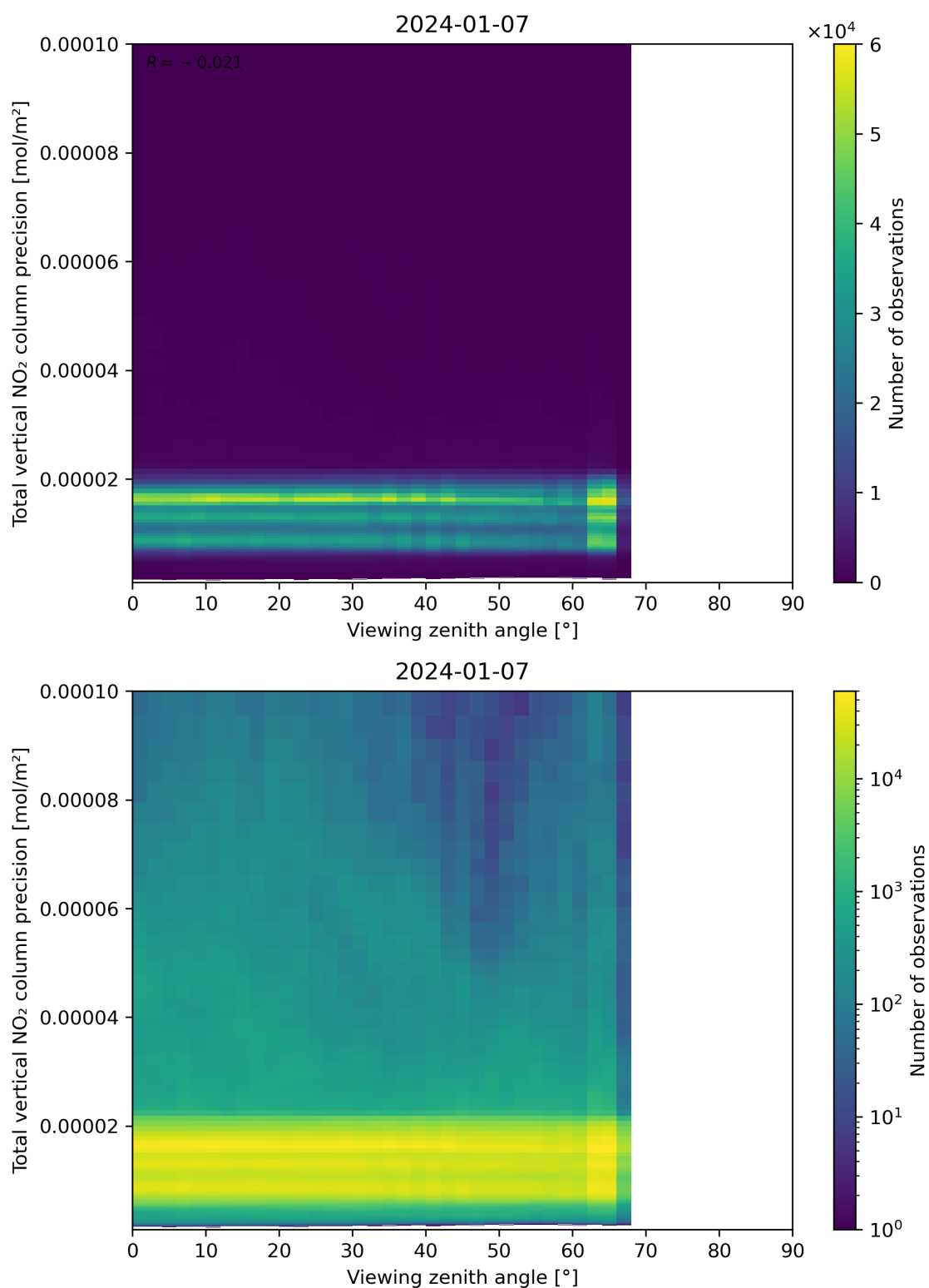
Figure 168: Scatter density plot of “Viewing zenith angle” against “Total vertical NO 2 column precision” for 2024-01-06 to 2024-01-08.
