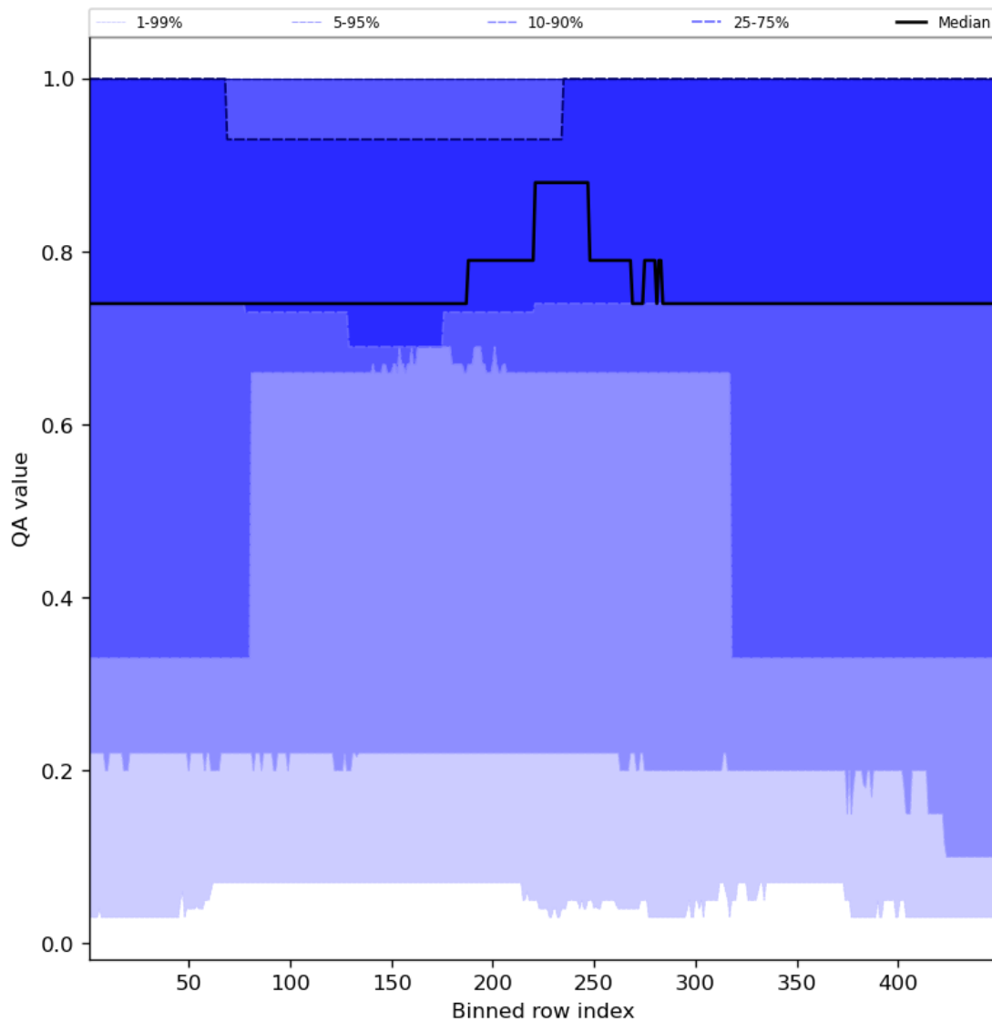
Figure 45: Along track statistics of “QA value” for 2024-01-06 to 2024-01-08
