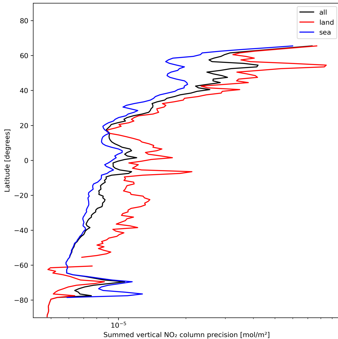
Figure 24: Zonal average of “Summed vertical NO 2 column precision” for 2024-01-06 to 2024-01-08.
