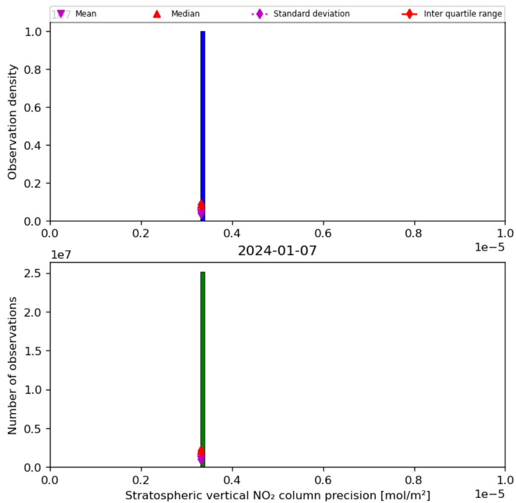
Figure 37: Histogram of “Stratospheric vertical NO 2 column precision” for 2024-01-06 to 2024-01-08
