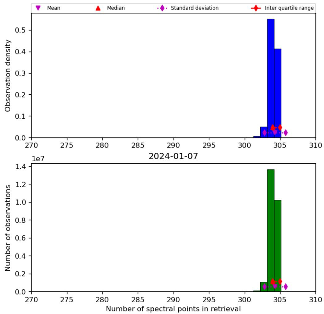
Figure 33: Histogram of “Number of spectral points in retrieval” for 2024-01-06 to 2024-01-08
