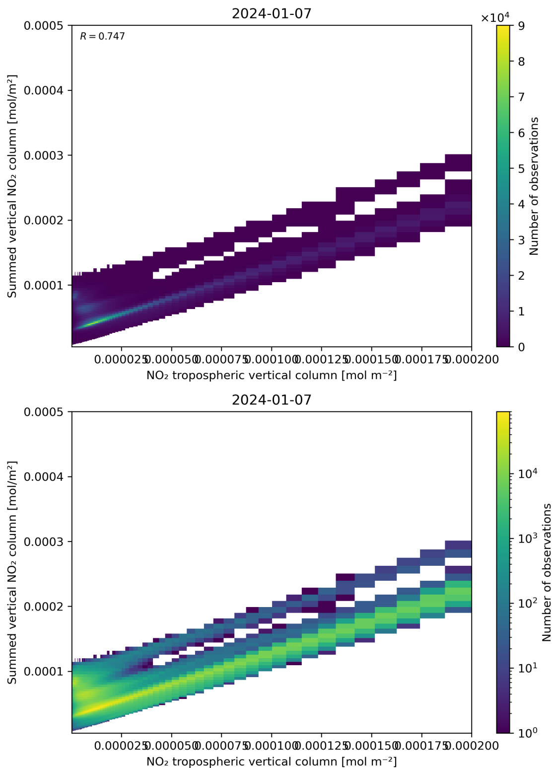
Figure 126: Scatter density plot of “NO 2 tropospheric vertical column” against “Summed vertical NO 2 column” for 2024-01-06 to 2024-01-08.
