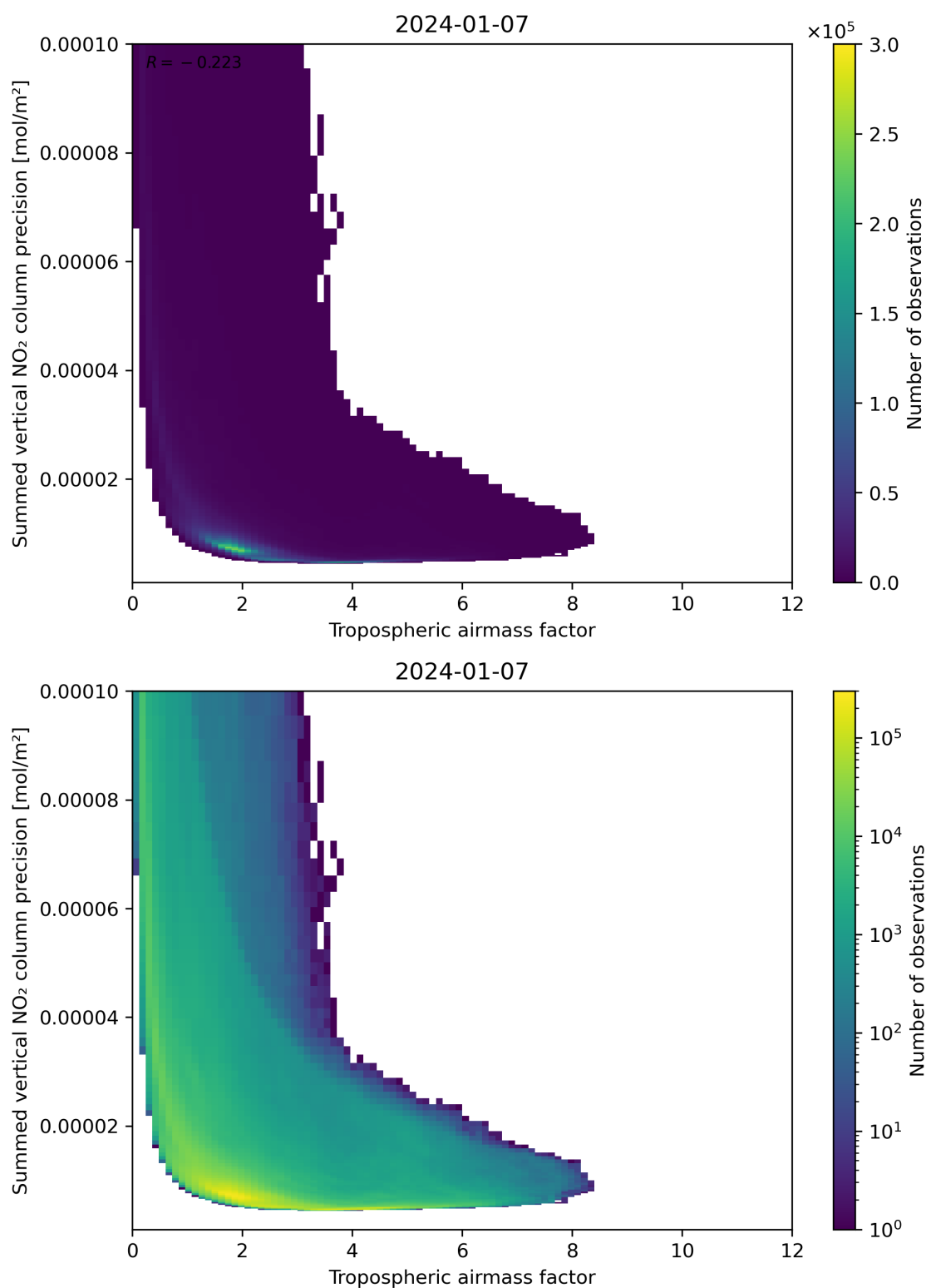
Figure 76: Scatter density plot of “Tropospheric air mass factor” against “Summed vertical NO 2 column precision” for 2024-01-06 to 2024-01-08.
