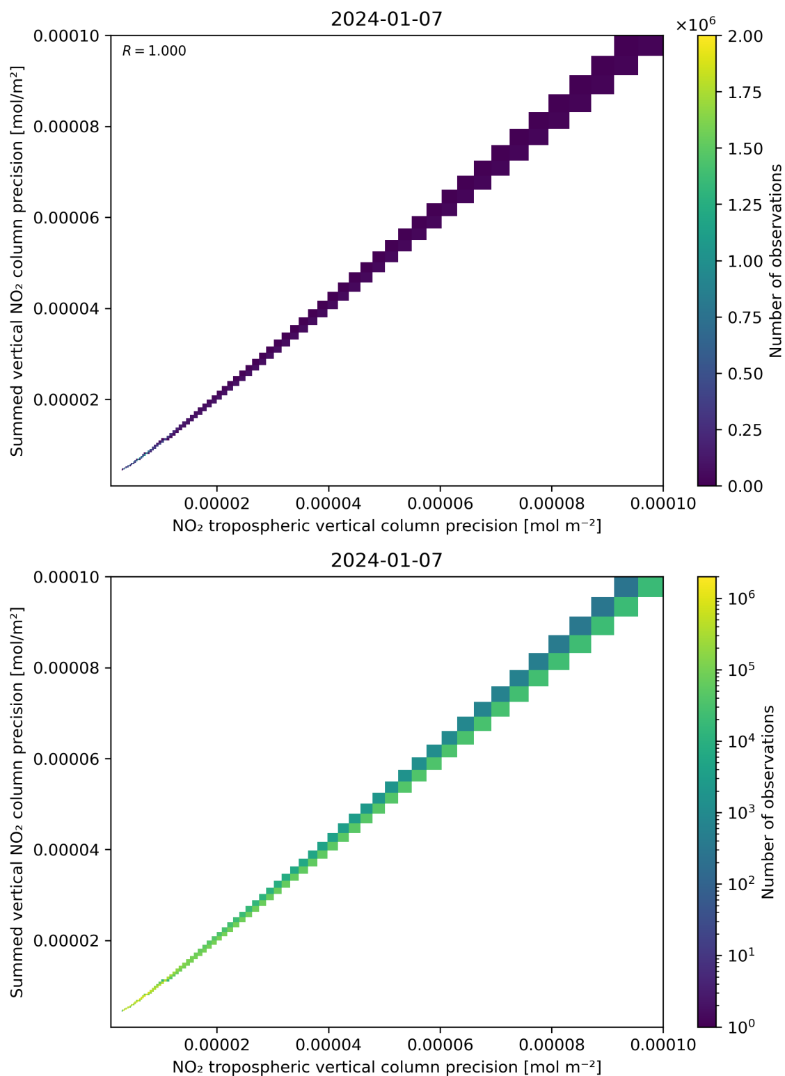
Figure 137: Scatter density plot of “NO 2 tropospheric vertical column precision” against “Summed vertical NO 2 column precision” for 2024-01-06 to 2024-01-08.
