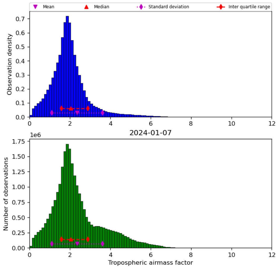
Figure 31: Histogram of “Tropospheric airmass factor” for 2024-01-06 to 2024-01-08
