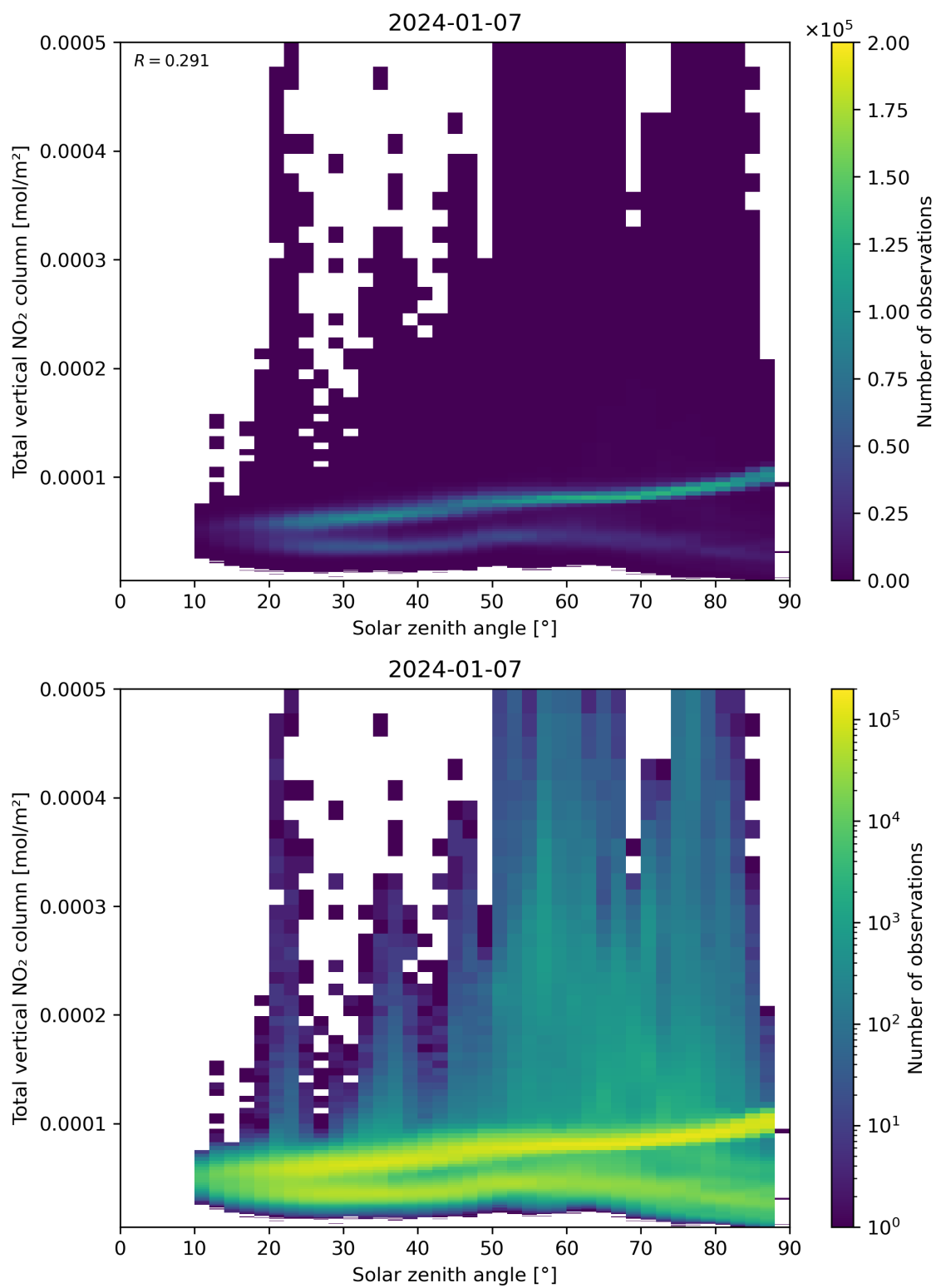
Figure 153: Scatter density plot of “Solar zenith angle” against “Total vertical \text{NO}_2 column” for 2024-01-06 to 2024-01-08.
