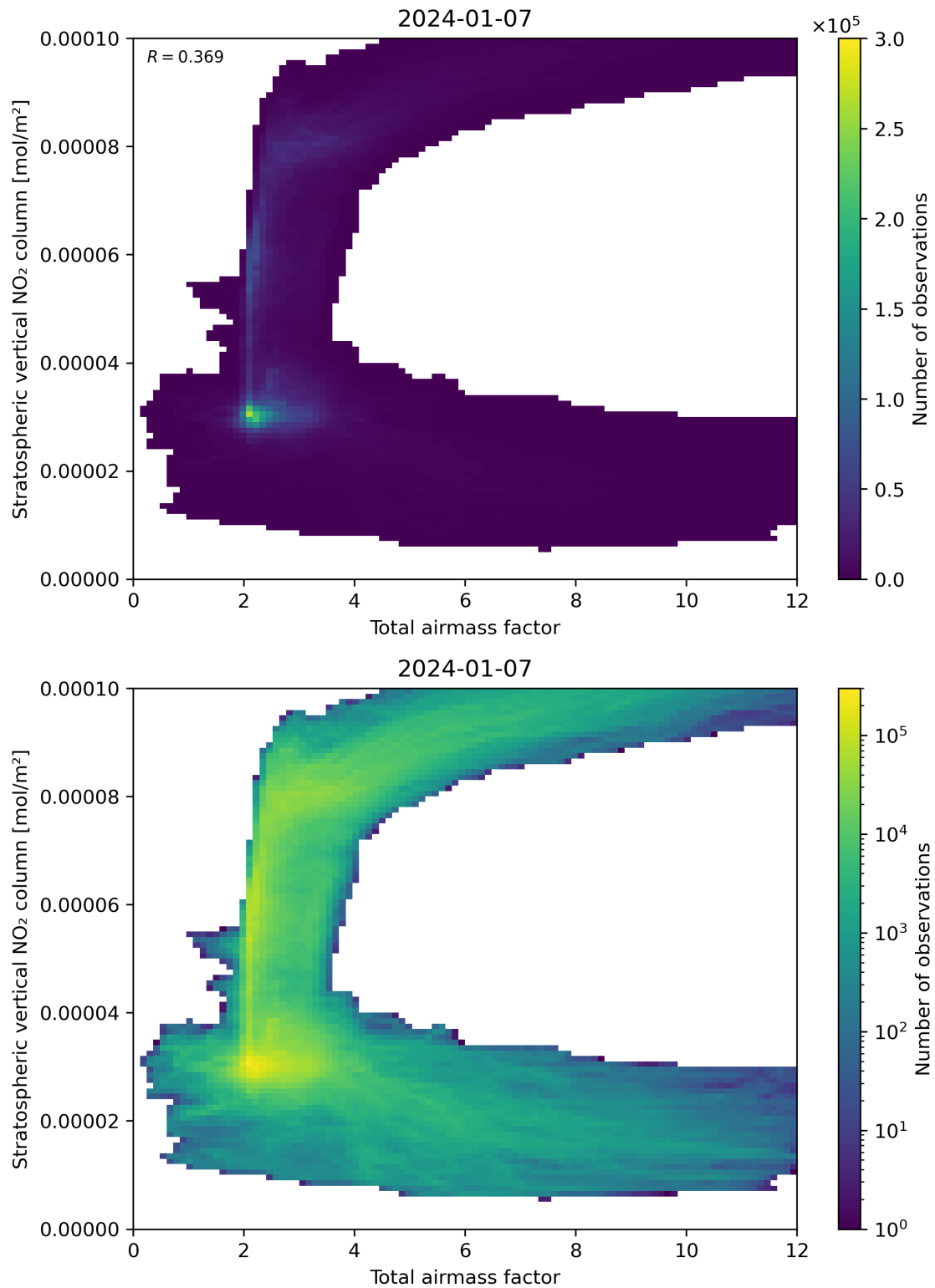
Figure 64: Scatter density plot of “Total airmass factor” against “Stratospheric vertical NO 2 column” for 2024-01-06 to 2024-01-08.
