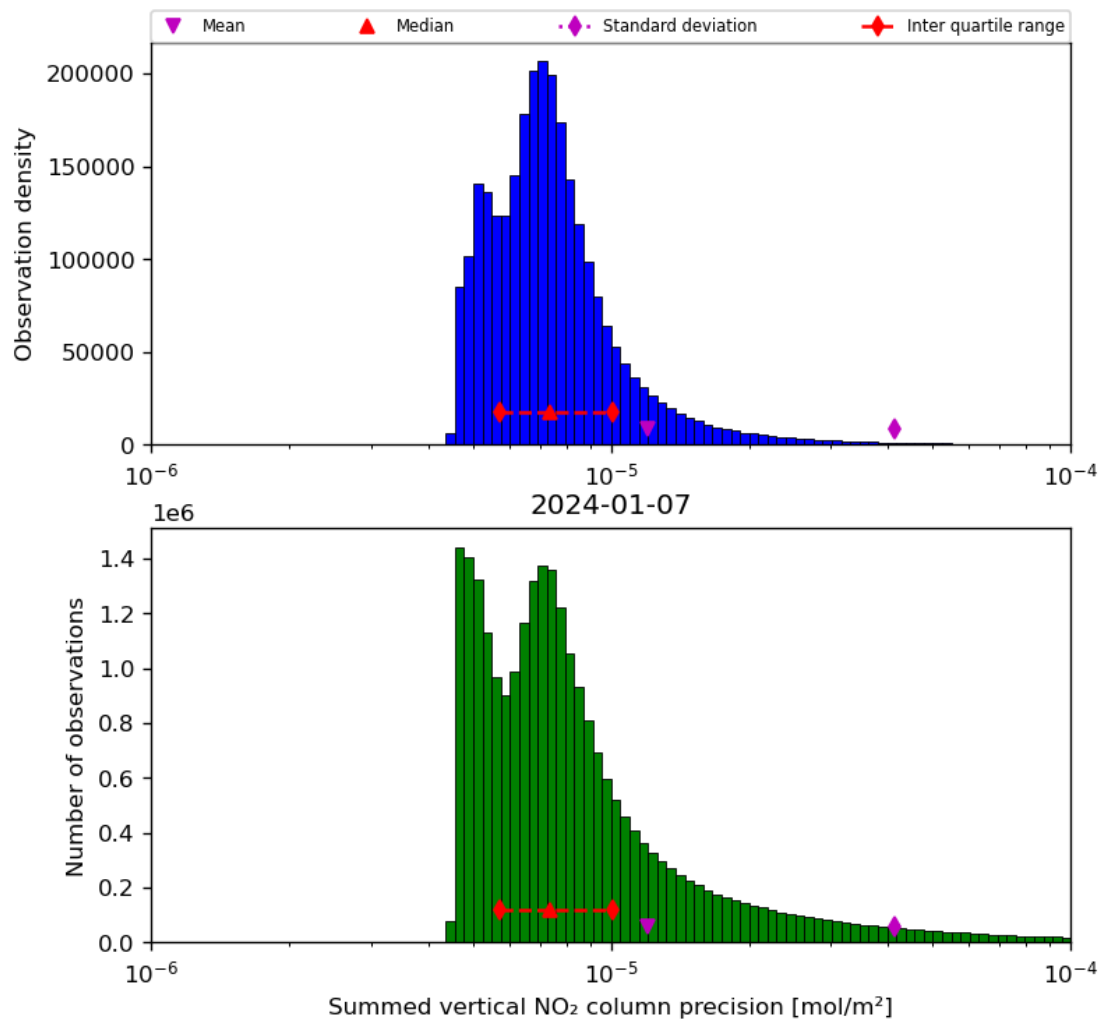
Figure 41: Histogram of “Summed vertical NO 2 column precision” for 2024-01-06 to 2024-01-08
