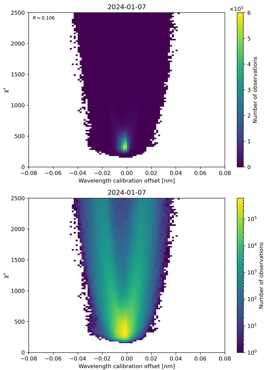
Figure 175: Scatter density plot of “Wavelength calibration offset” against “ \chi^2 ” for 2024-01-06 to 2024-01-08.
