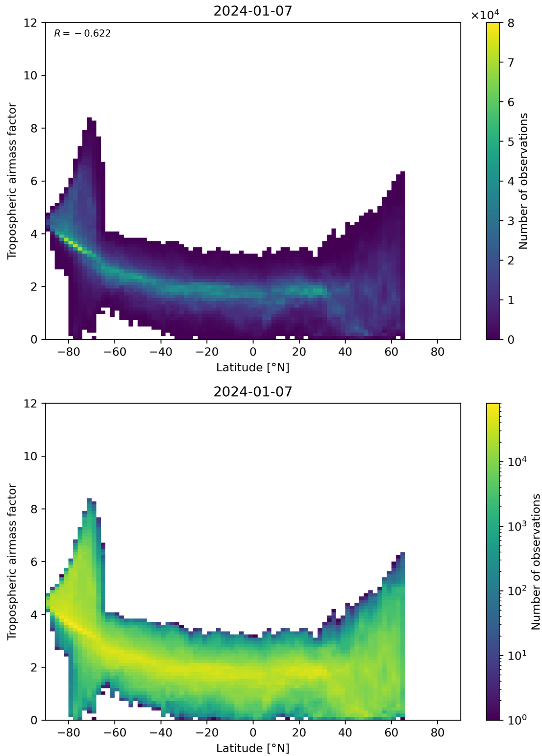
Figure 85: Scatter density plot of “Latitude” against “Tropospheric air mass factor” for 2024-01-06 to 2024-01-08.
