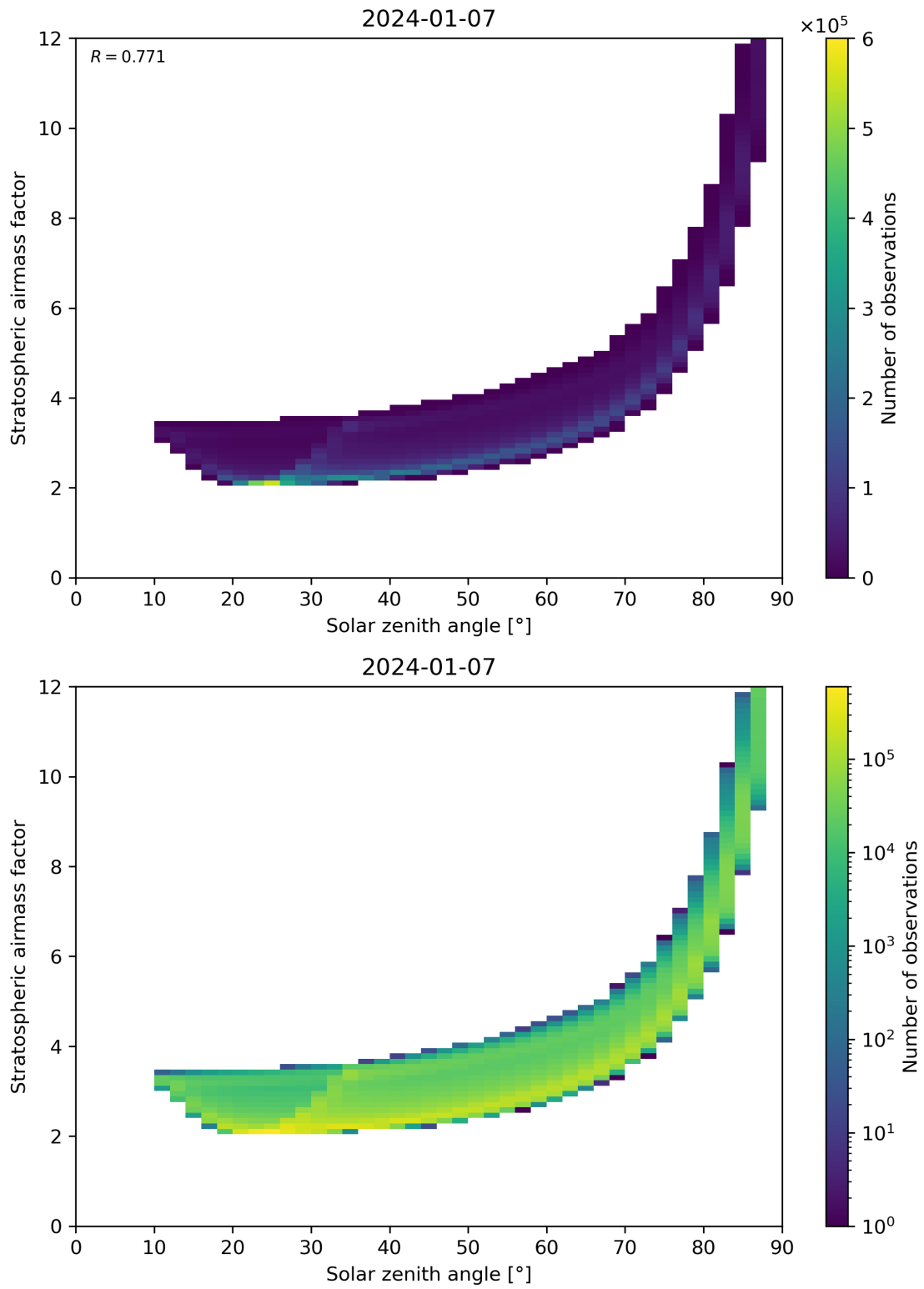
Figure 145: Scatter density plot of “Solar zenith angle” against “Stratospheric airmass factor” for 2024-01-06 to 2024-01-08.
