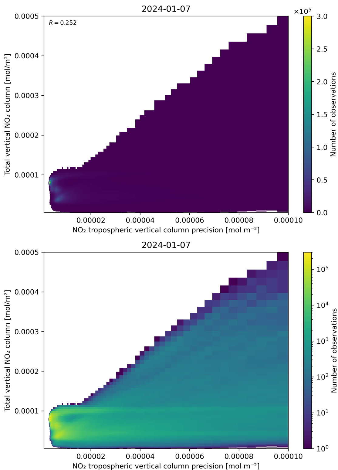
Figure 138: Scatter density plot of “NO 2 tropospheric vertical column precision” against “Total vertical NO 2 column” for 2024-01-06 to 2024-01-08.
