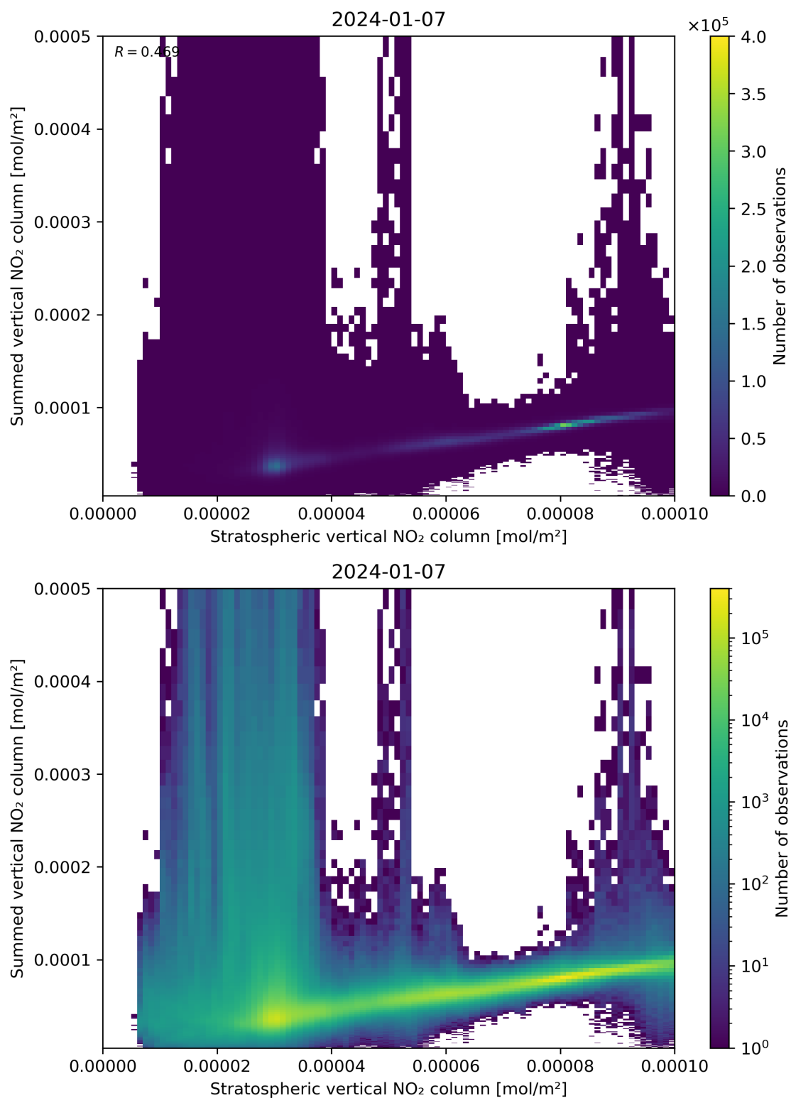
Figure 98: Scatter density plot of “Stratospheric vertical NO 2 column” against “Summed vertical NO 2 column” for 2024-01-06 to 2024-01-08.
