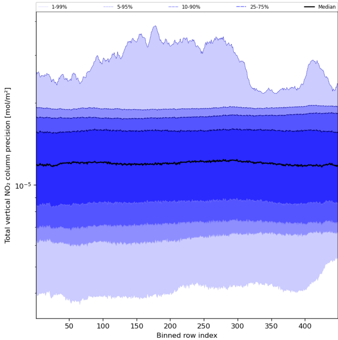
Figure 56: Along track statistics of “Total vertical NO 2 column precision” for 2024-01-06 to 2024-01-08
