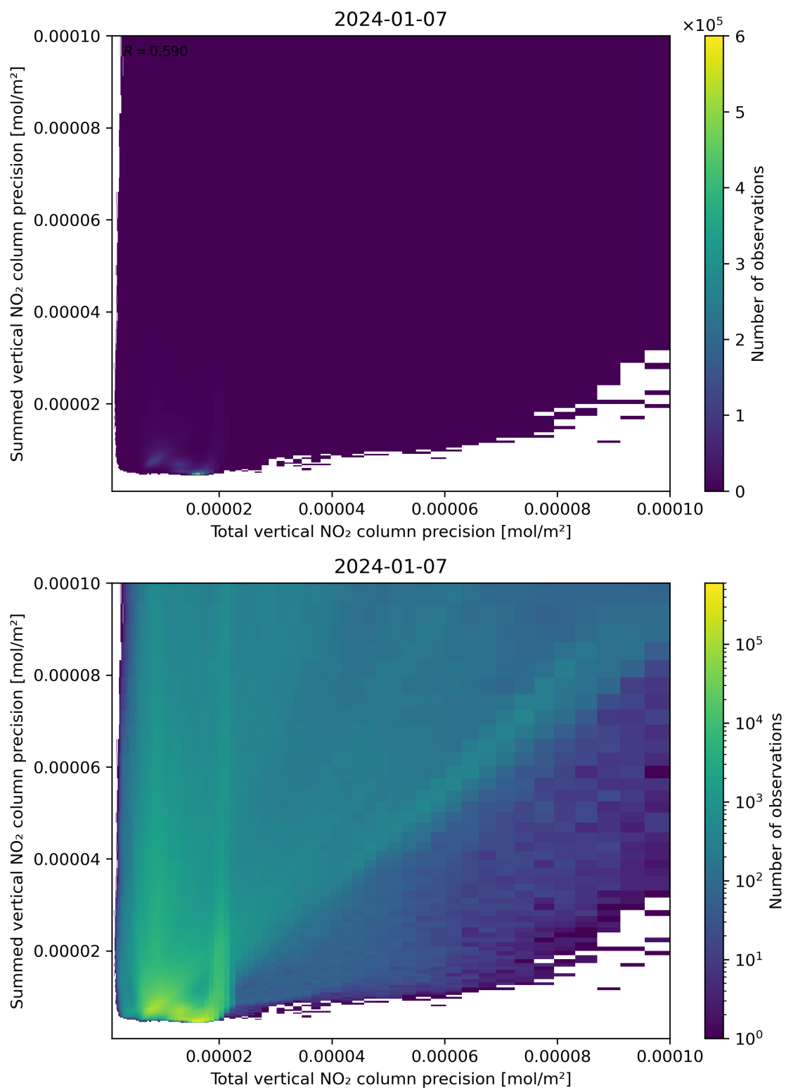
Figure 118: Scatter density plot of “Total vertical NO 2 column precision” against “Summed vertical NO 2 column precision” for 2024-01-06 to 2024-01-08.
