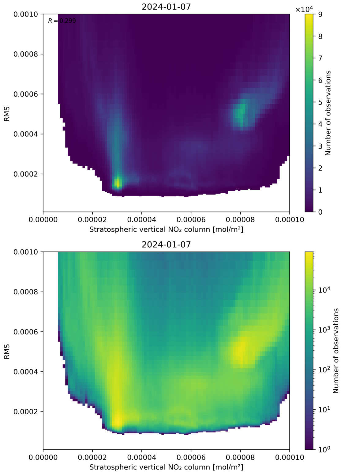
Figure 102: Scatter density plot of “Stratospheric vertical NO 2 column” against “RMS” for 2024-01-06 to 2024-01-08.
