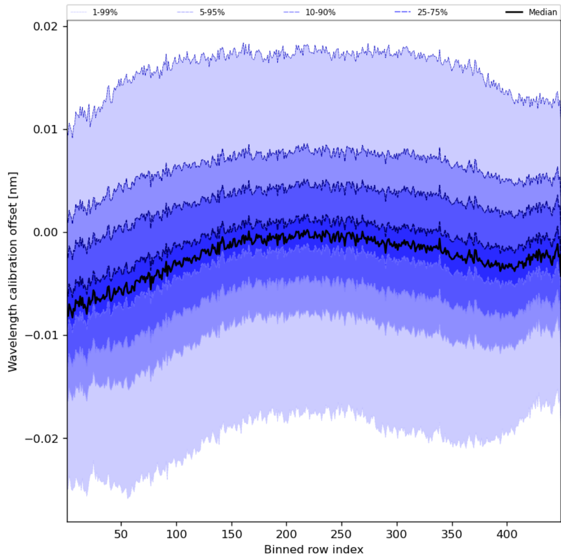
Figure 52: Along track statistics of “Wavelength calibration offset” for 2024-01-06 to 2024-01-08
