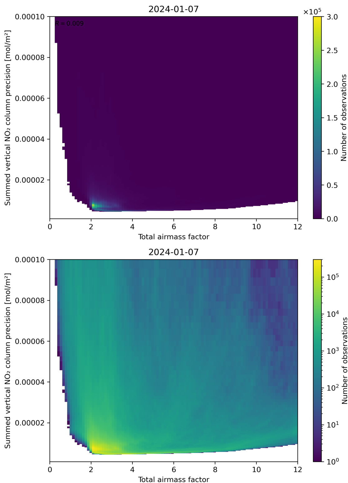
Figure 66: Scatter density plot of “Total airmass factor” against “Summed vertical NO 2 column precision” for 2024-01-06 to 2024-01-08.
