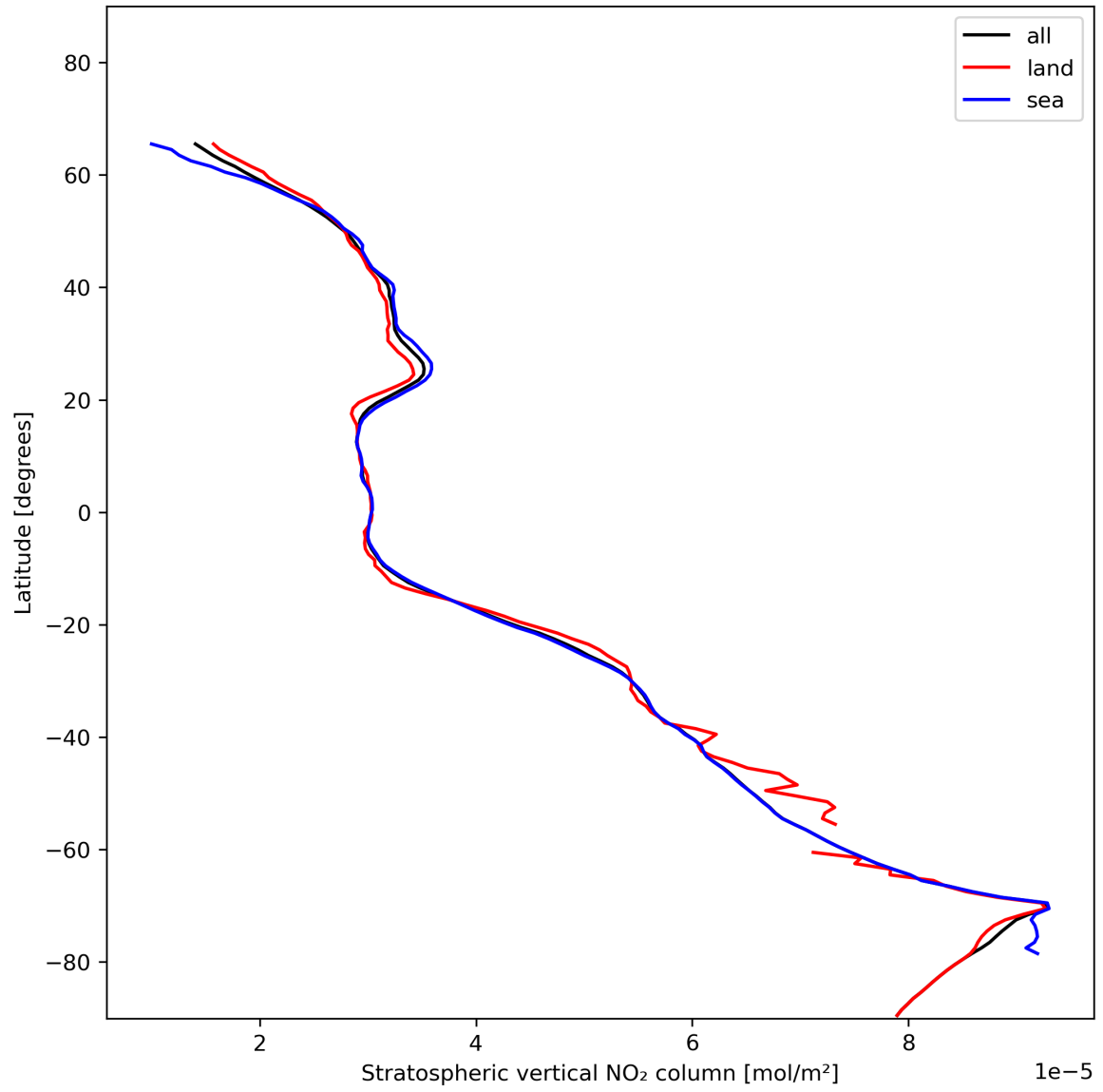
Figure 19: Zonal average of “Stratospheric vertical NO 2 column” for 2024-01-06 to 2024-01-08.
