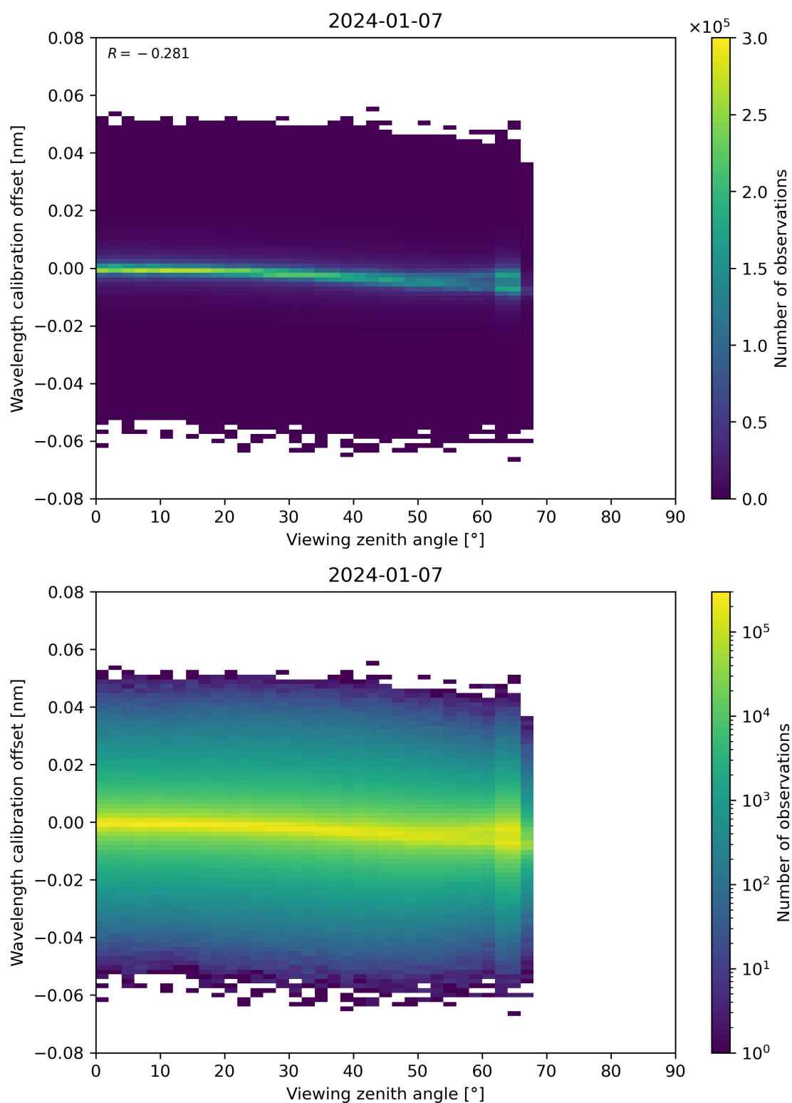
Figure 173: Scatter density plot of “Viewing zenith angle” against “Wavelength calibration offset” for 2024-01-06 to 2024-01-08.
