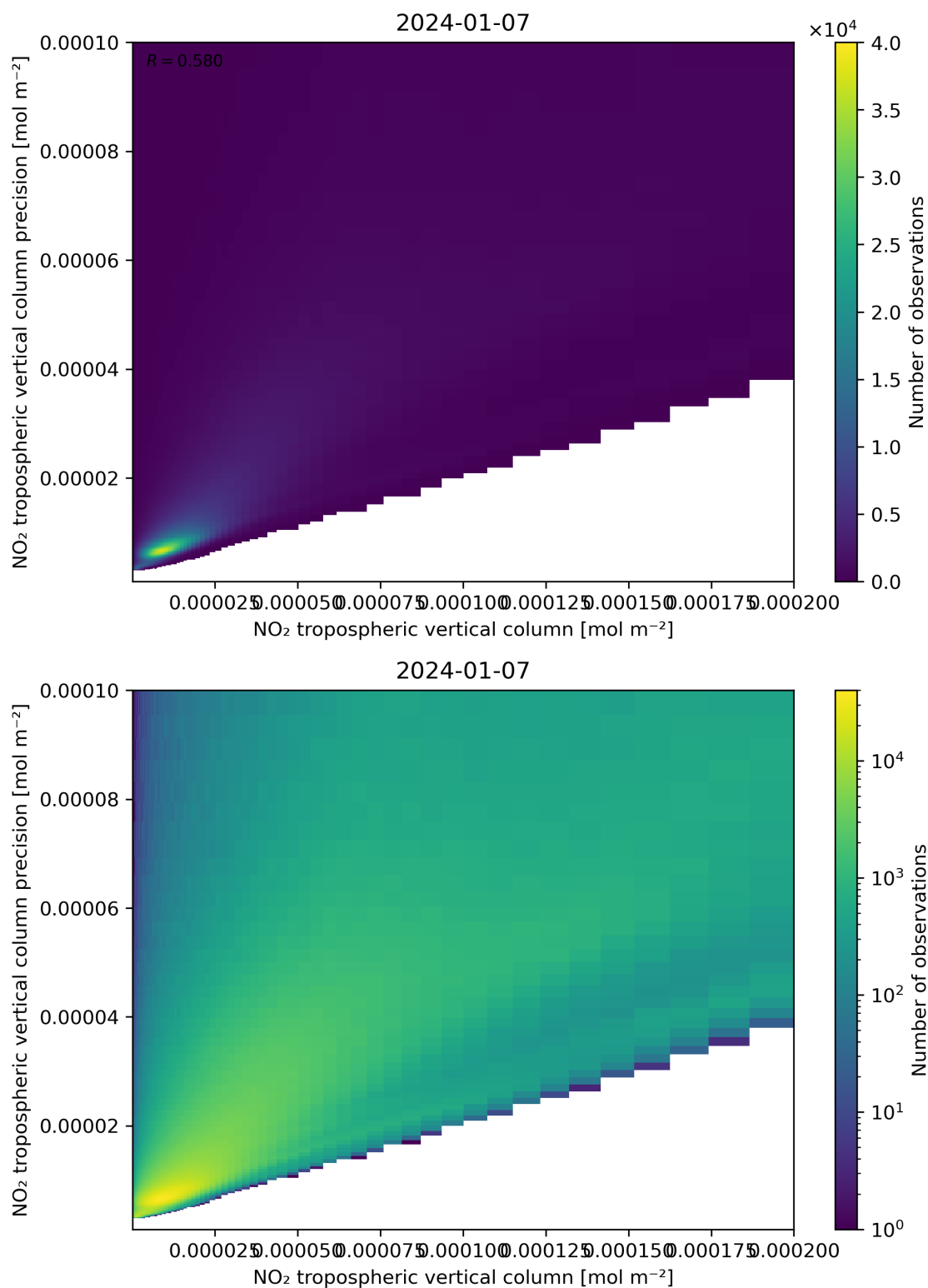
Figure 130: Scatter density plot of “NO 2 tropospheric vertical column” against “NO 2 tropospheric vertical column precision” for 2024-01-06 to 2024-01-08.
