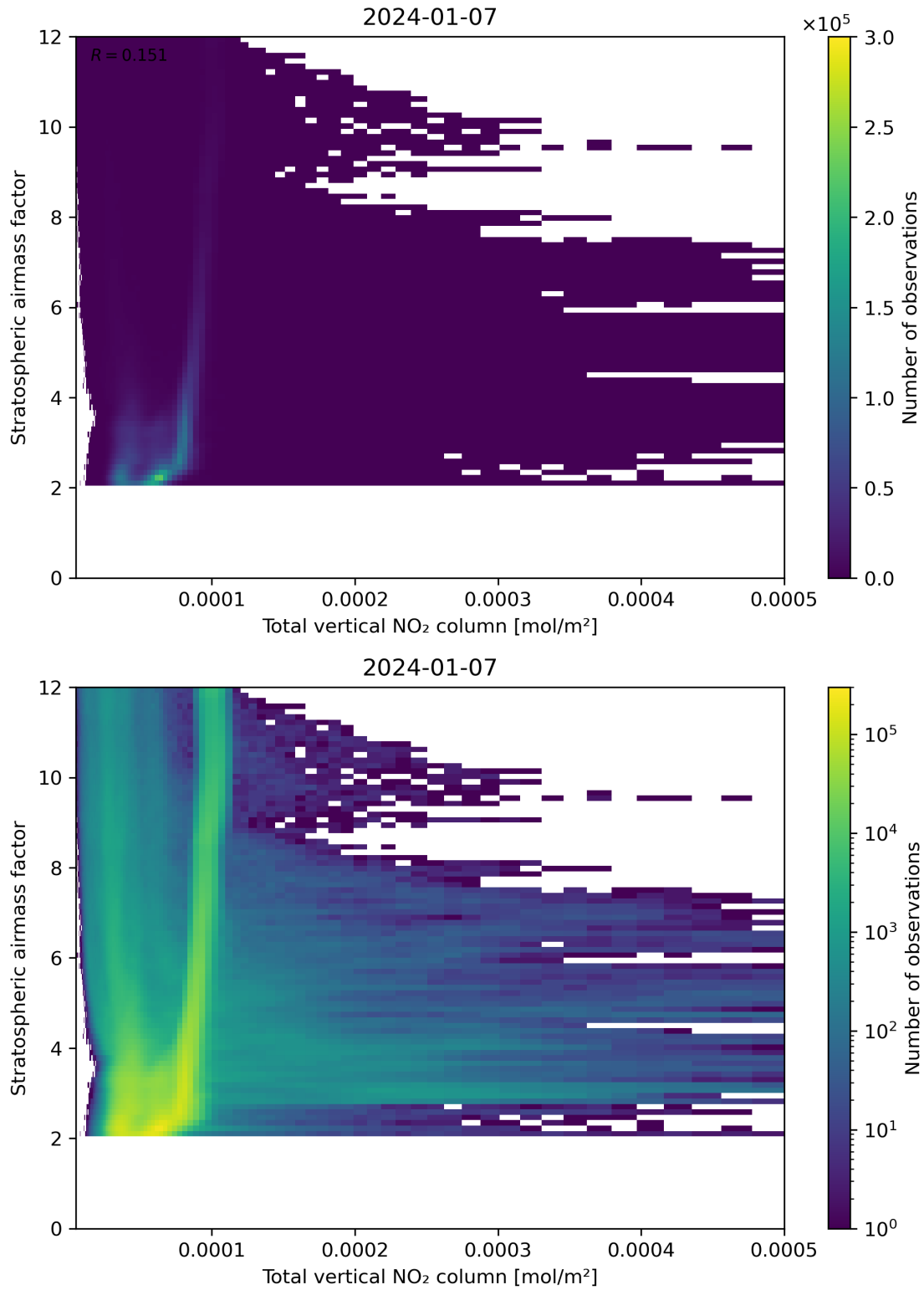
Figure 110: Scatter density plot of “Total vertical NO 2 column” against “Stratospheric airmass factor” for 2024-01-06 to 2024-01-08.
