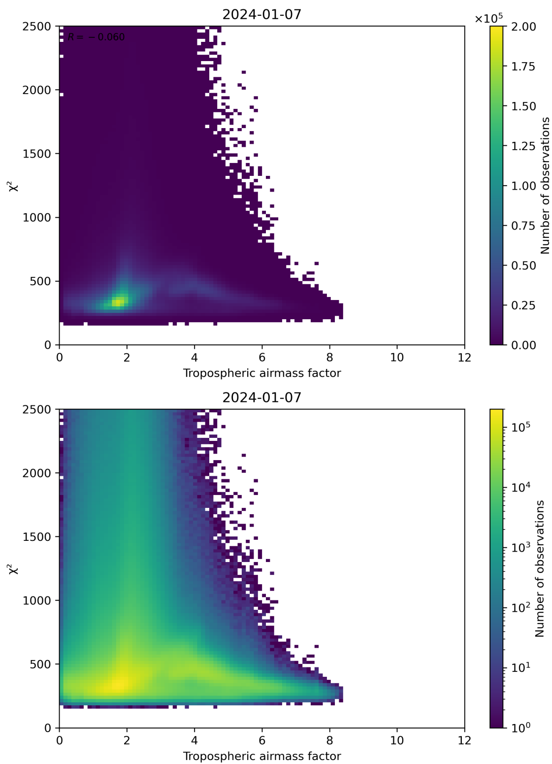
Figure 73: Scatter density plot of “Tropospheric airmass factor” against “ \chi^2 ” for 2024-01-06 to 2024-01-08.
