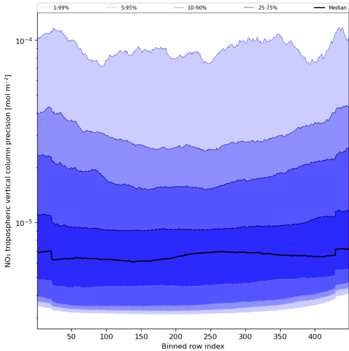
Figure 47: Along track statistics of “NO 2 tropospheric vertical column precision” for 2024-01-06 to 2024-01-08
