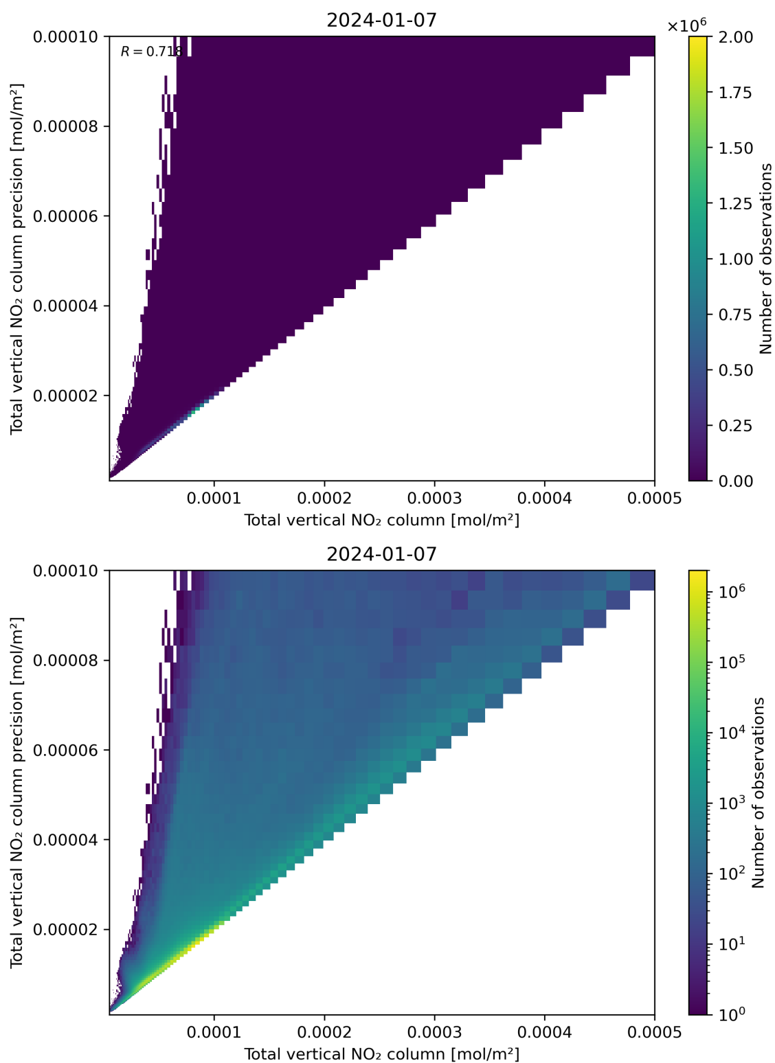
Figure 114: Scatter density plot of “Total vertical NO 2 column” against “Total vertical NO 2 column precision” for 2024-01-06 to 2024-01-08.
