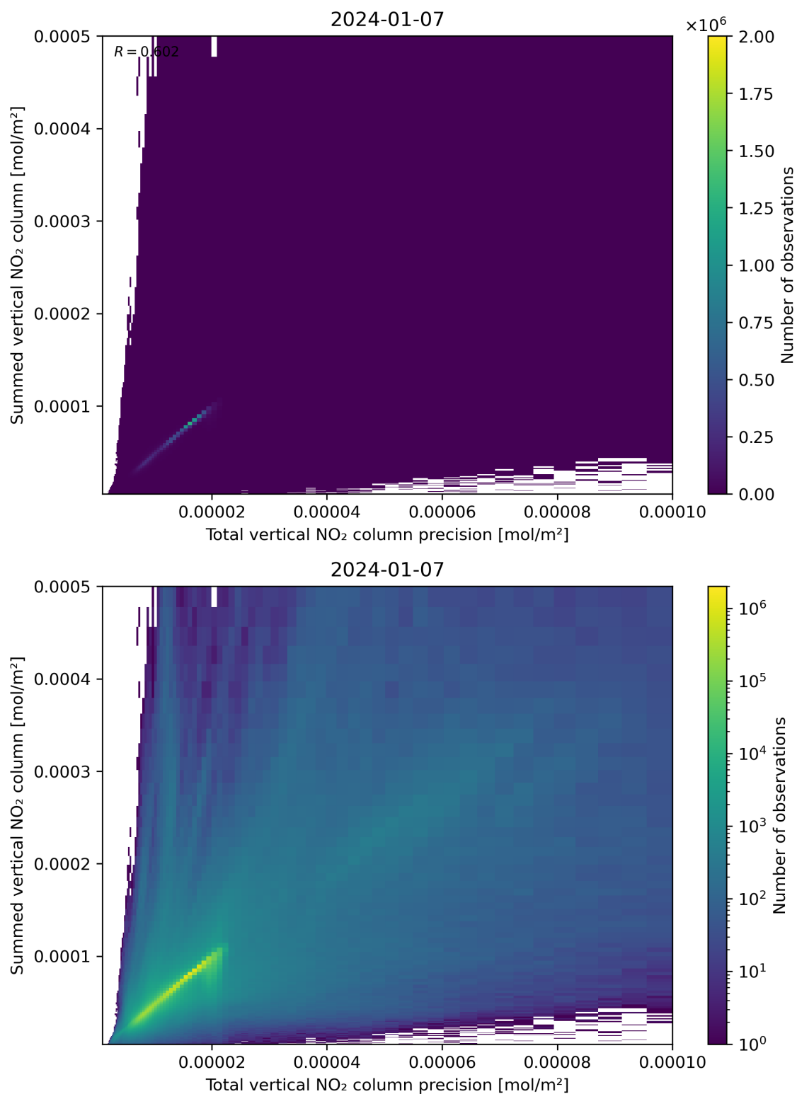
Figure 117: Scatter density plot of “Total vertical NO 2 column precision” against “Summed vertical NO 2 column” for 2024-01-06 to 2024-01-08.
