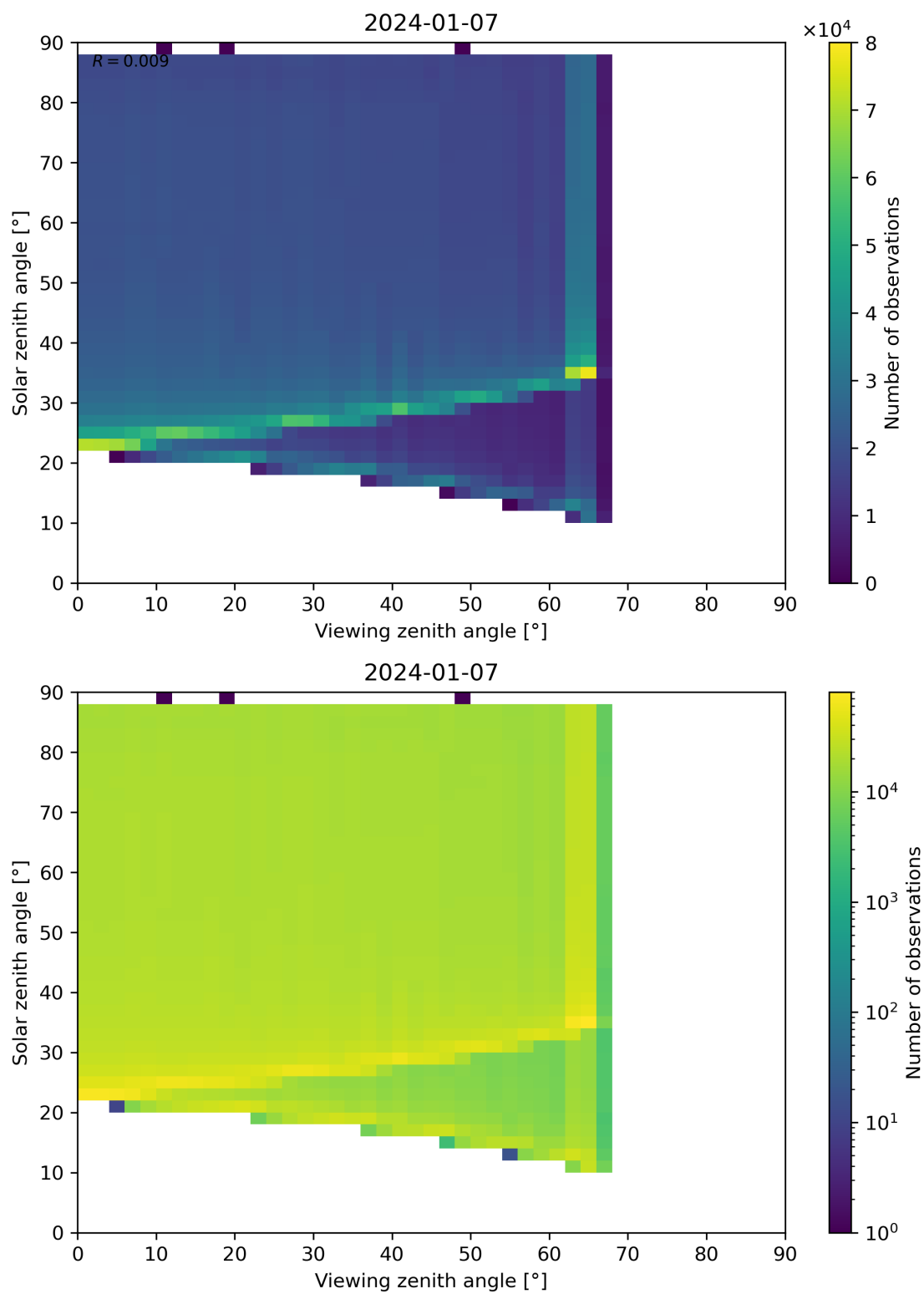
Figure 172: Scatter density plot of “Viewing zenith angle” against “Solar zenith angle” for 2024-01-06 to 2024-01-08.
