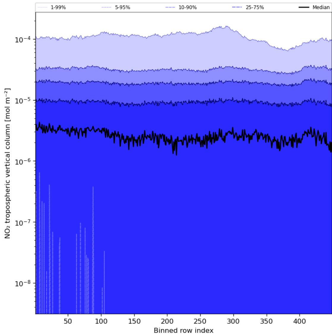
Figure 46: Along track statistics of “NO 2 tropospheric vertical column” for 2024-01-06 to 2024-01-08
