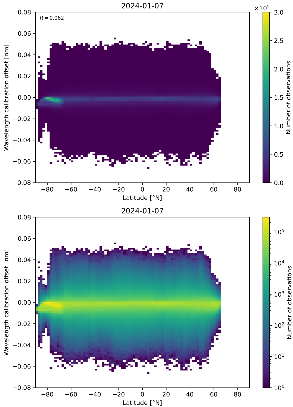
Figure 95: Scatter density plot of “Latitude” against “Wavelength calibration offset” for 2024-01-06 to 2024-01-08.
