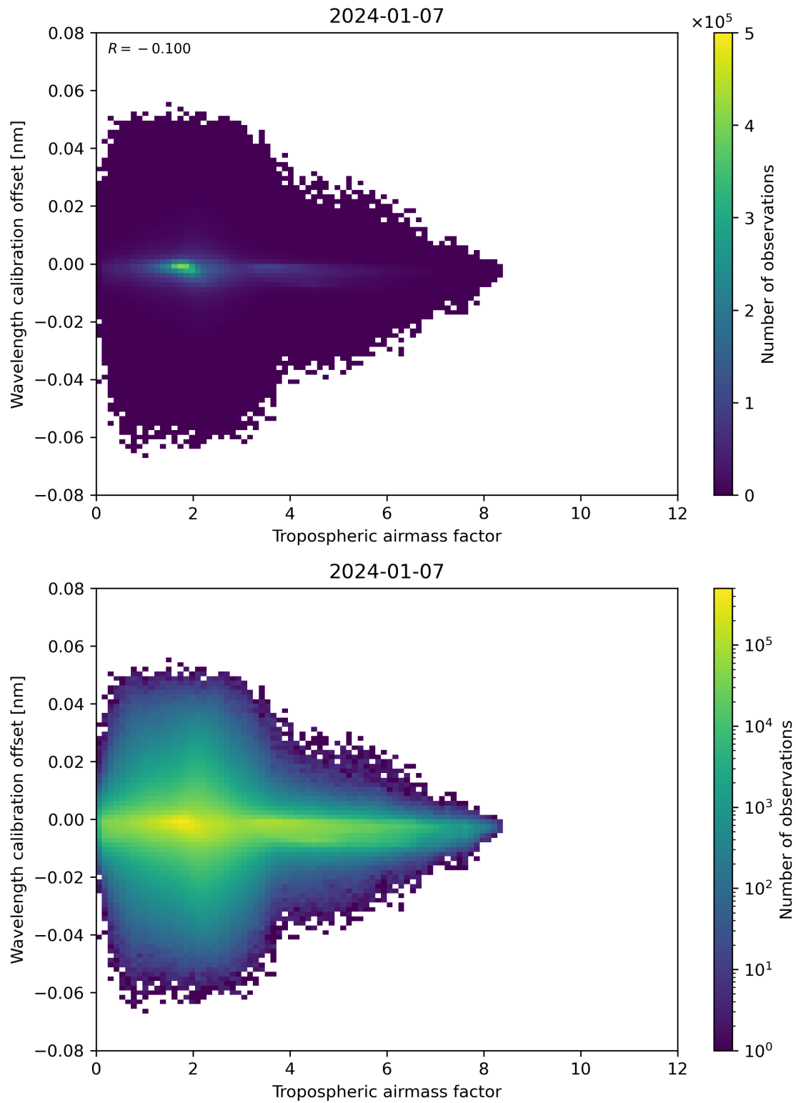
Figure 80: Scatter density plot of “Tropospheric air mass factor” against “Wavelength calibration offset” for 2024-01-06 to 2024-01-08.
