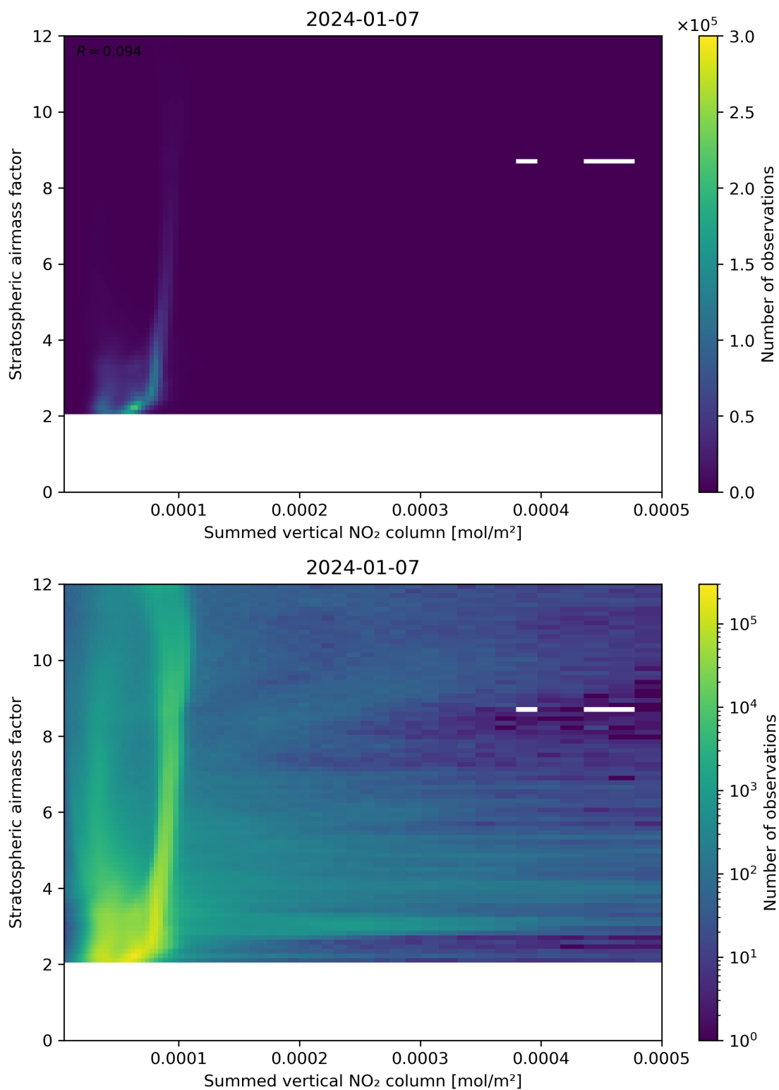
Figure 103: Scatter density plot of “Summed vertical NO 2 column” against “Stratospheric airmass factor” for 2024-01-06 to 2024-01-08.
