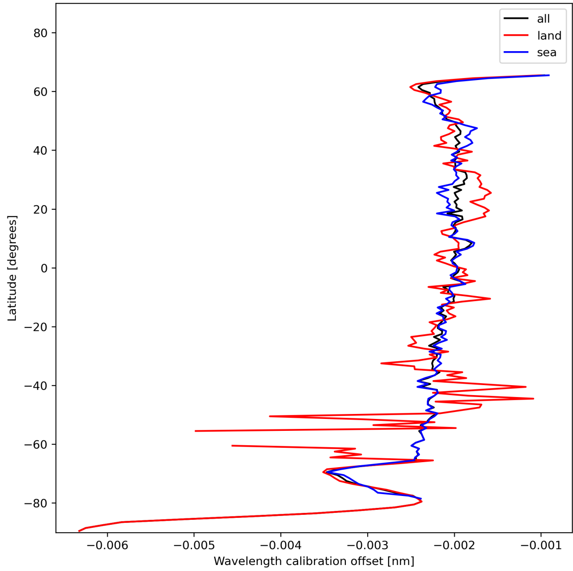
Figure 18: Zonal average of “Wavelength calibration offset” for 2024-01-06 to 2024-01-08.
