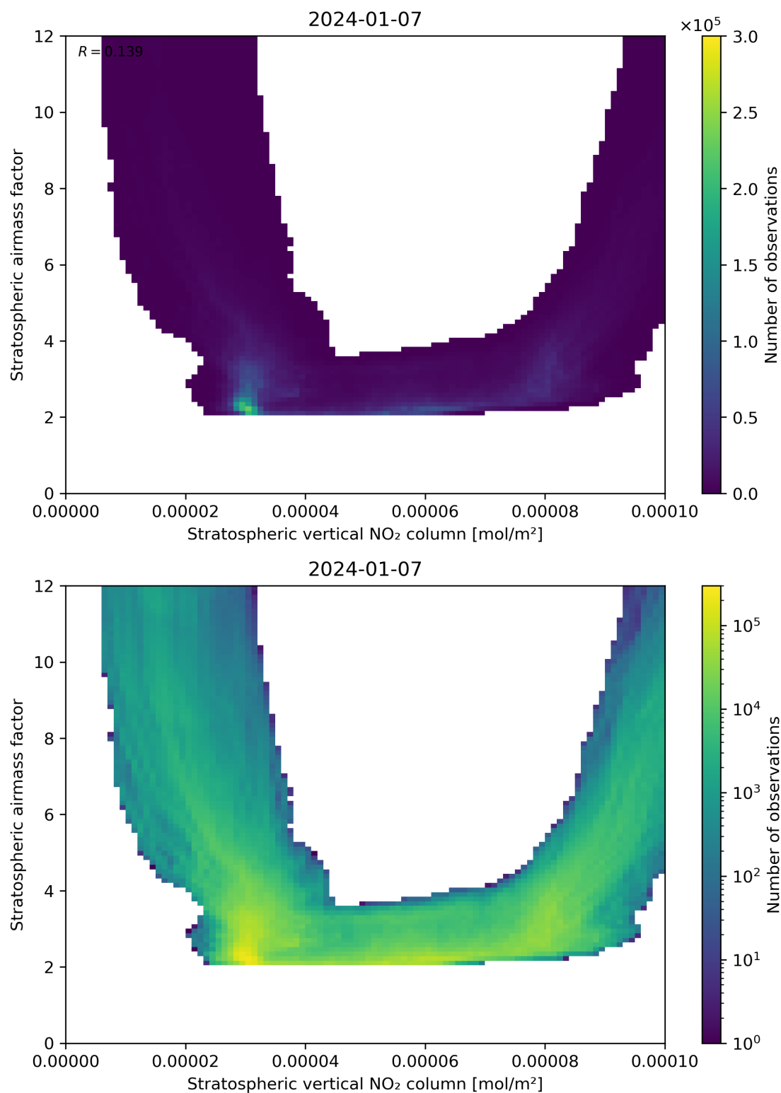
Figure 96: Scatter density plot of “Stratospheric vertical NO 2 column” against “Stratospheric airmass factor” for 2024-01-06 to 2024-01-08.
