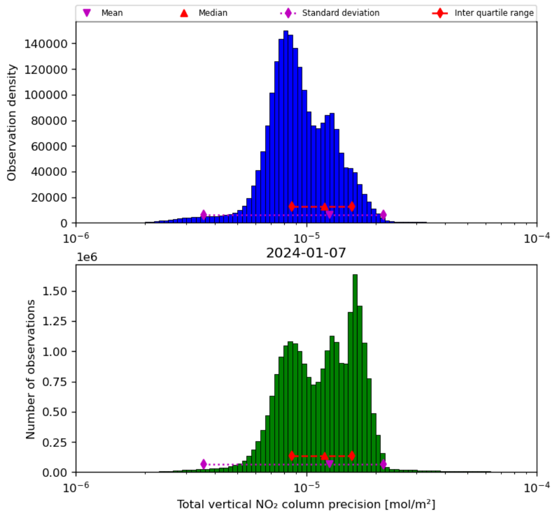
Figure 39: Histogram of “Total vertical NO 2 column precision” for 2024-01-06 to 2024-01-08
