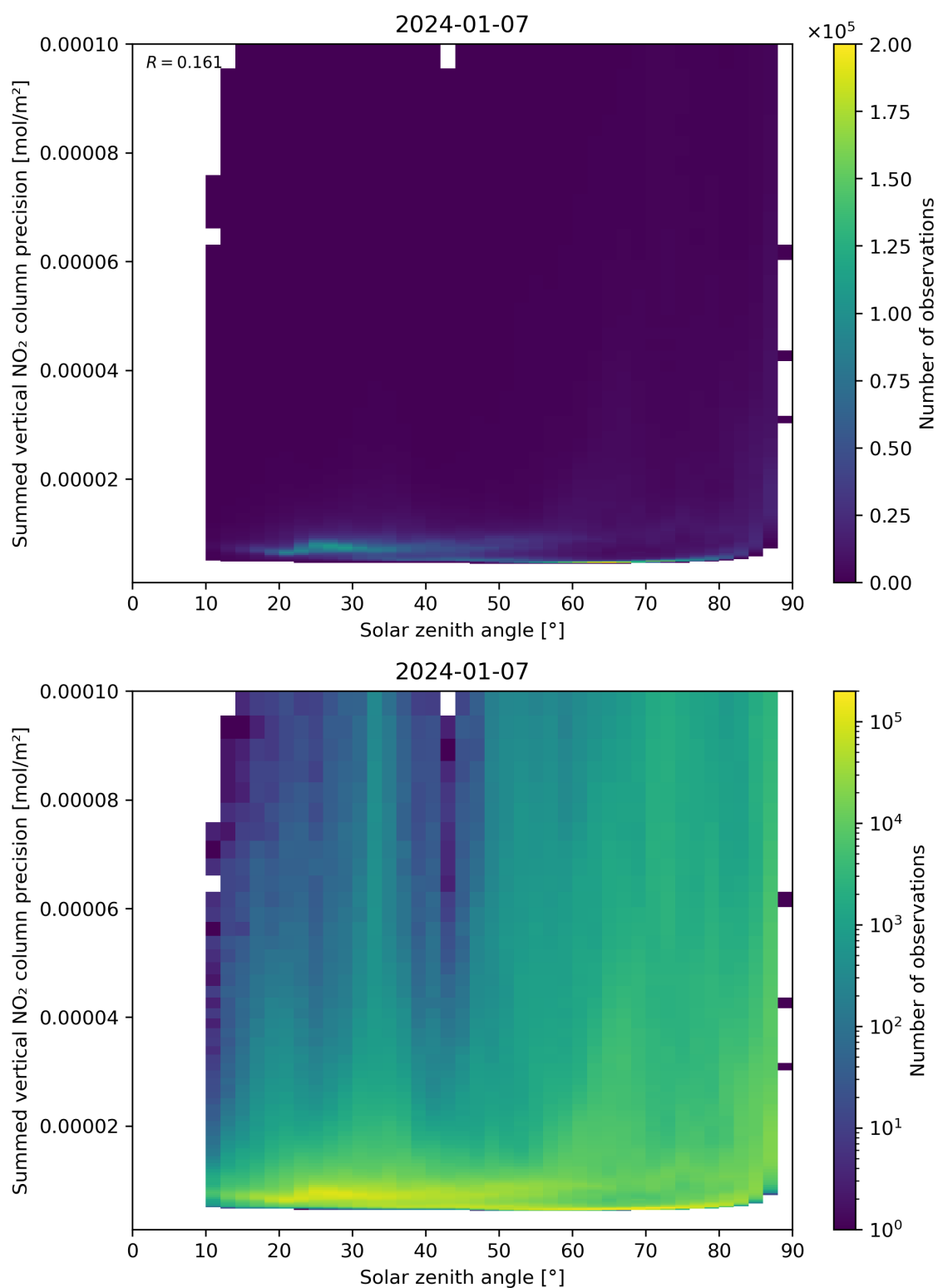
Figure 152: Scatter density plot of “Solar zenith angle” against “Summed vertical NO 2 column precision” for 2024-01-06 to 2024-01-08.
