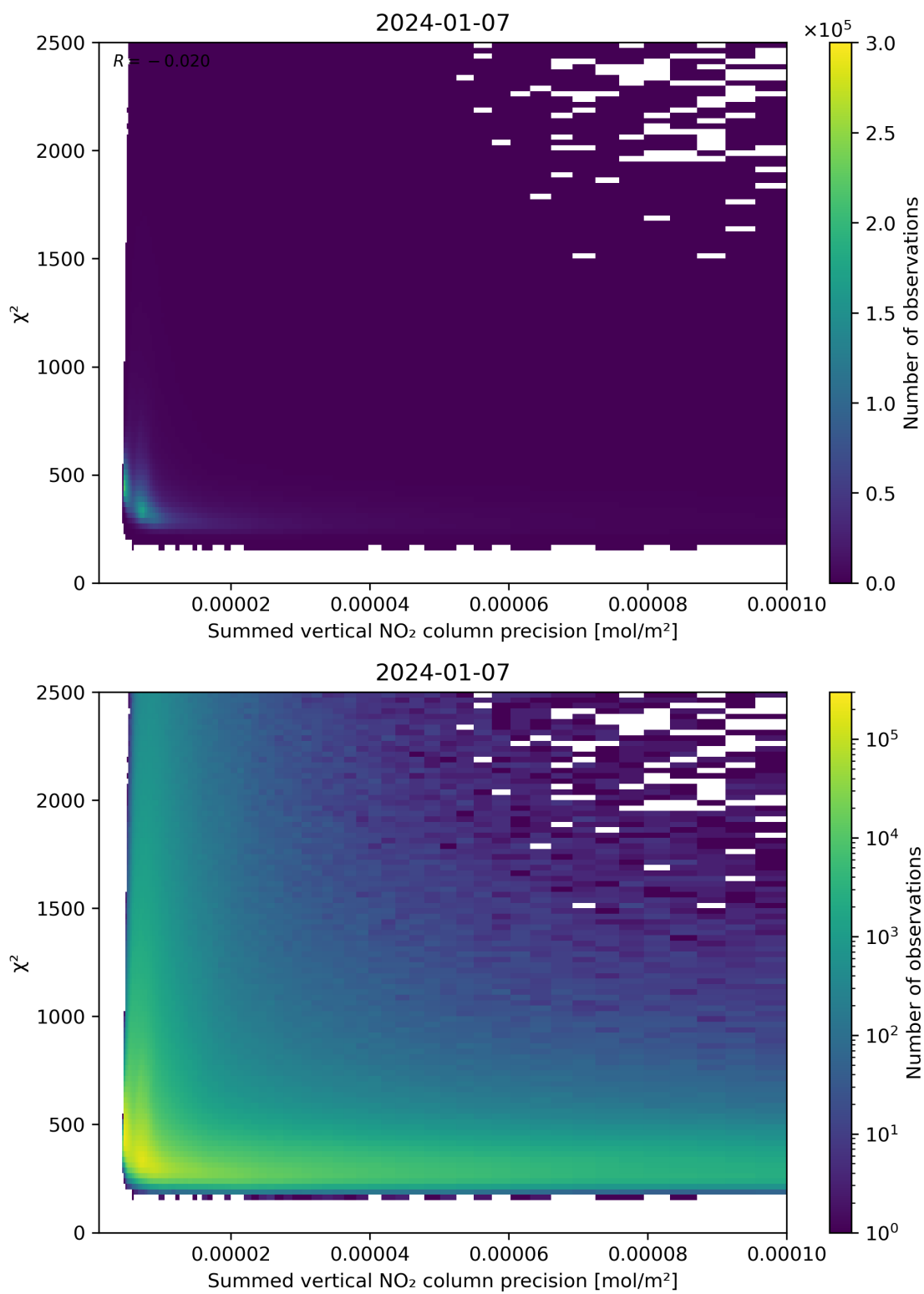
Figure 107: Scatter density plot of “Summed vertical NO 2 column precision” against “ \chi^2 ” for 2024-01-06 to 2024-01-08.
