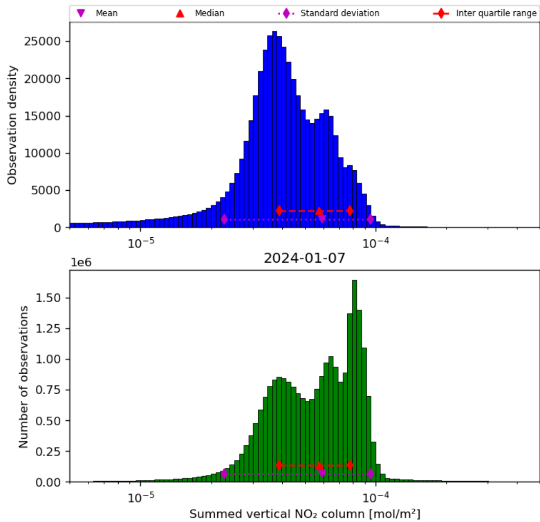
Figure 40: Histogram of “Summed vertical NO 2 column” for 2024-01-06 to 2024-01-08
