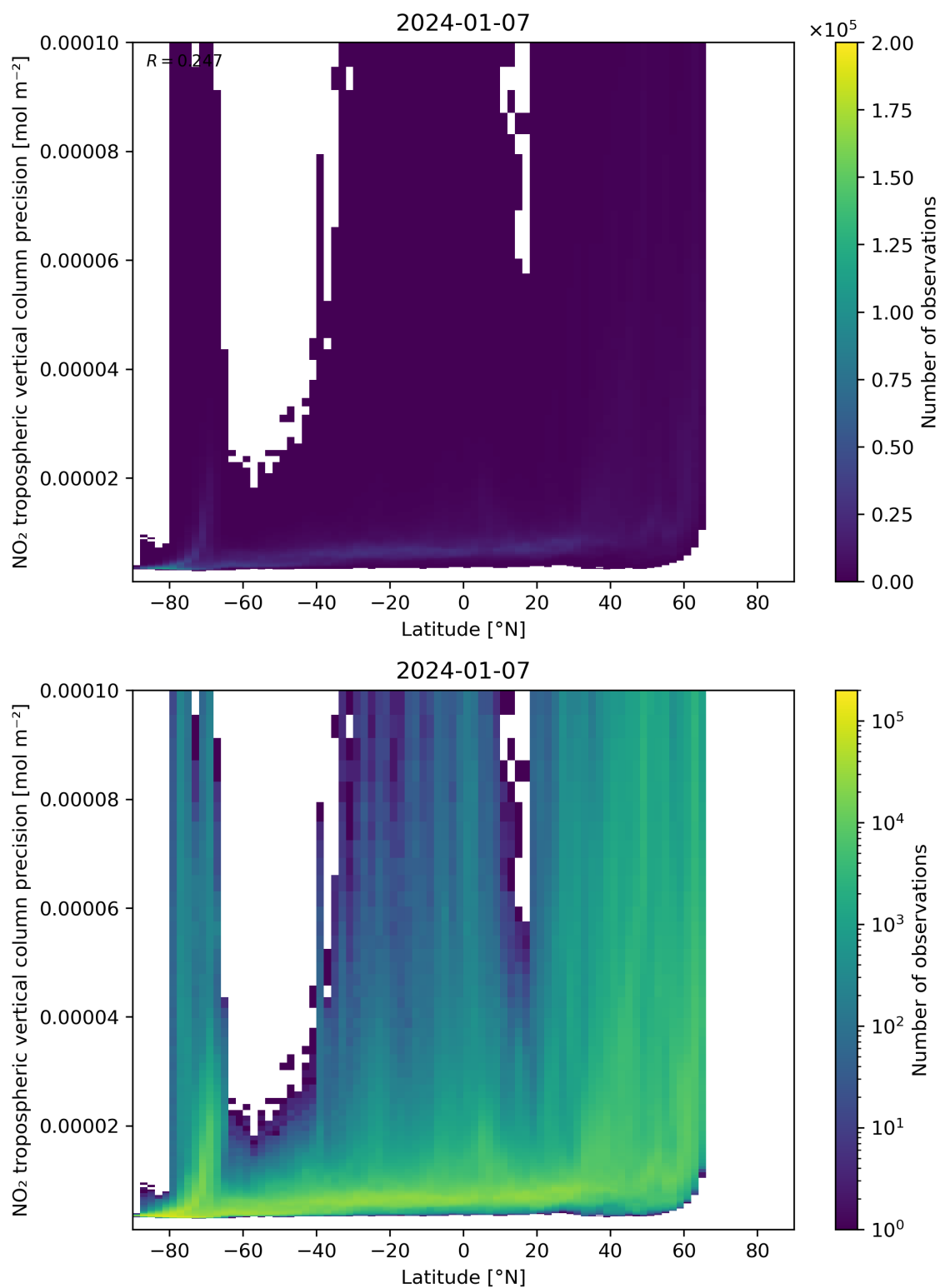
Figure 93: Scatter density plot of “Latitude” against “NO 2 tropospheric vertical column precision” for 2024-01-06 to 2024-01-08.
