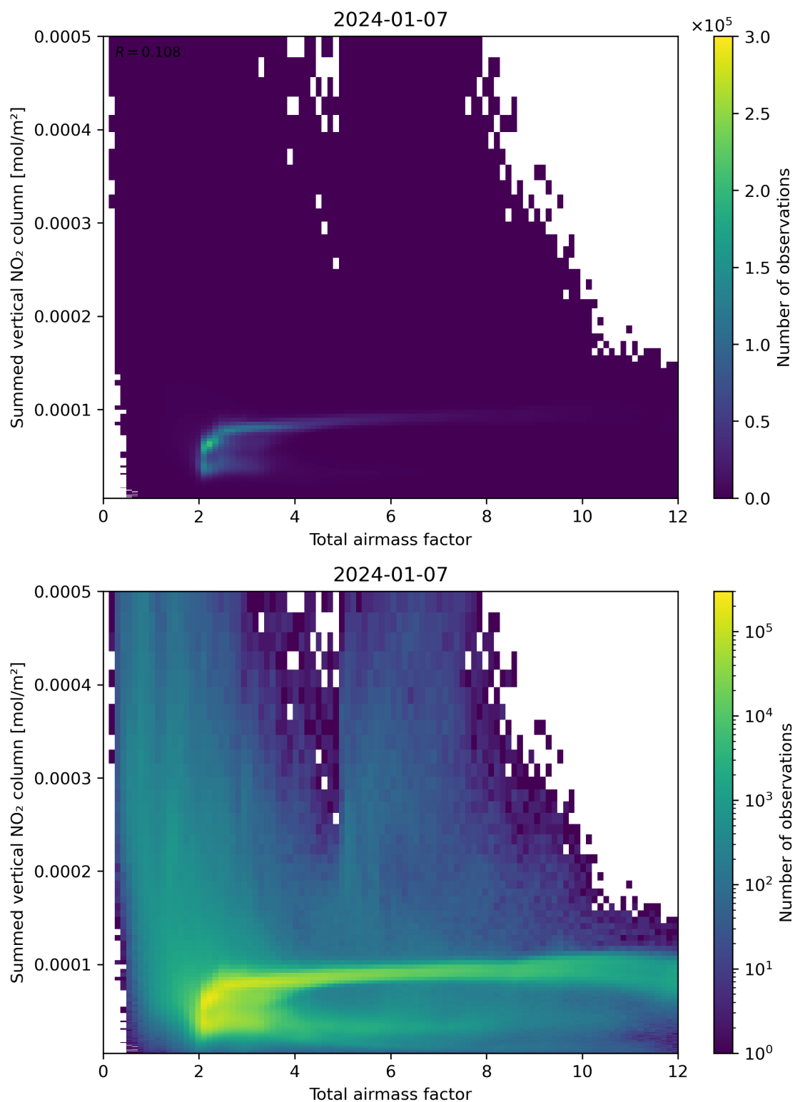
Figure 65: Scatter density plot of “Total airmass factor” against “Summed vertical NO 2 column” for 2024-01-06 to 2024-01-08.
