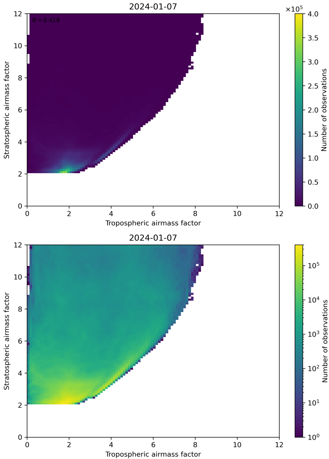
Figure 71: Scatter density plot of “Tropospheric airmass factor” against “Stratospheric airmass factor” for 2024-01-06 to 2024-01-08.
