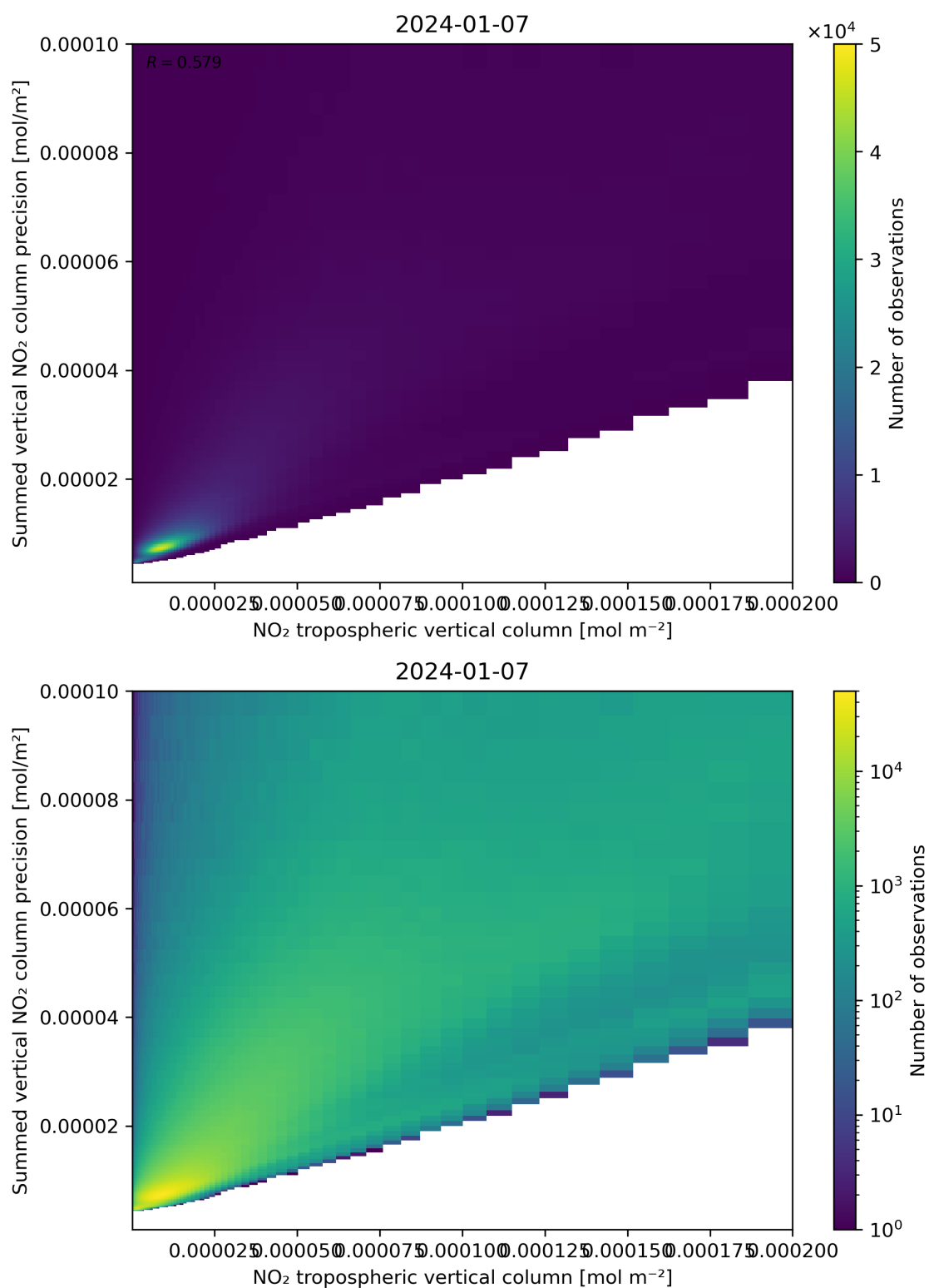
Figure 127: Scatter density plot of “NO 2 tropospheric vertical column” against “Summed vertical NO 2 column precision” for 2024-01-06 to 2024-01-08.
