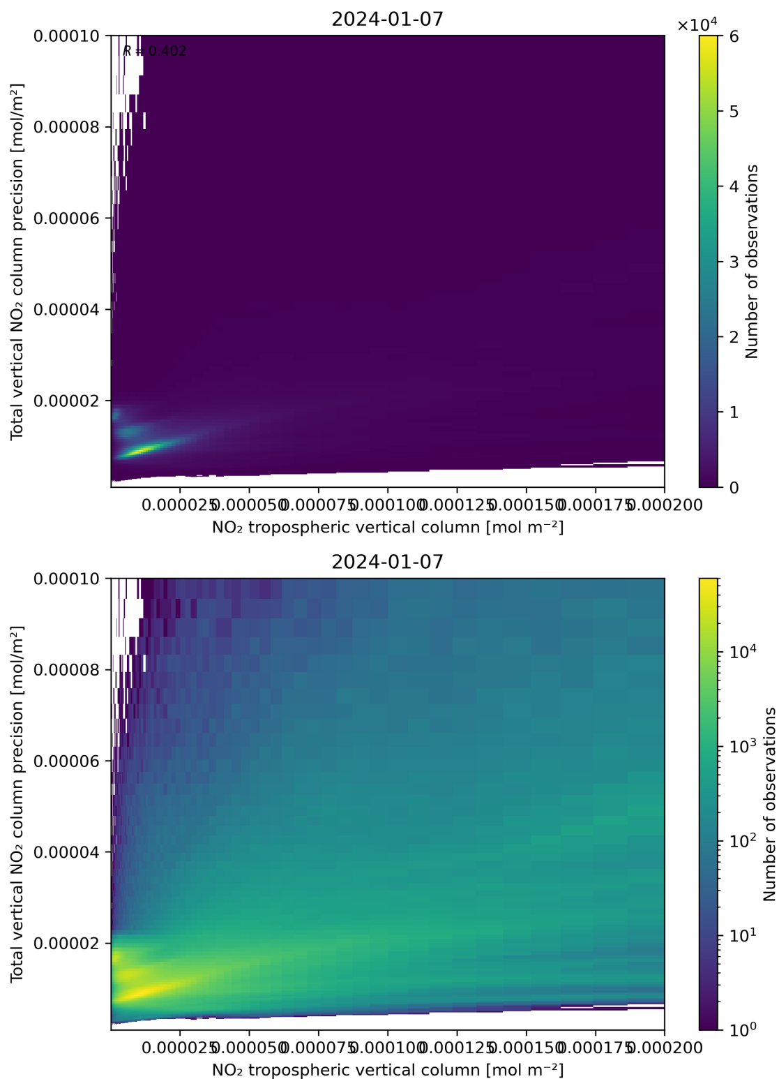
Figure 129: Scatter density plot of “NO 2 tropospheric vertical column” against “Total vertical NO 2 column precision” for 2024-01-06 to 2024-01-08.
