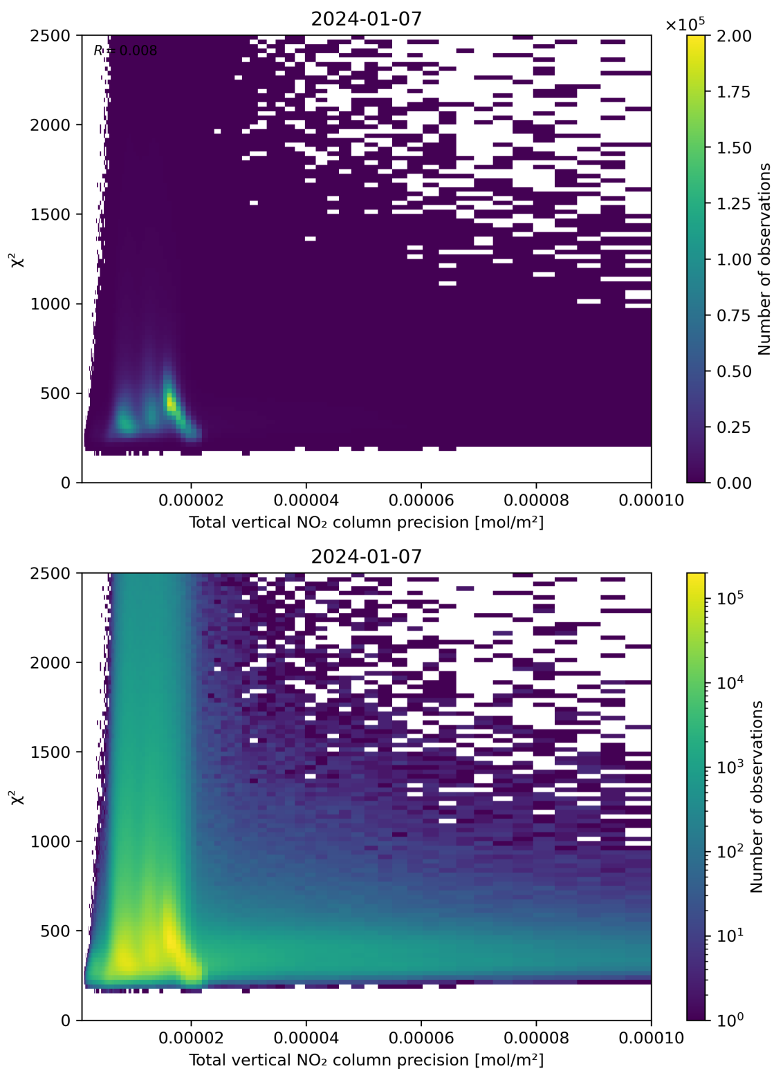
Figure 116: Scatter density plot of “Total vertical NO 2 column precision” against “ \chi^2 ” for 2024-01-06 to 2024-01-08.
