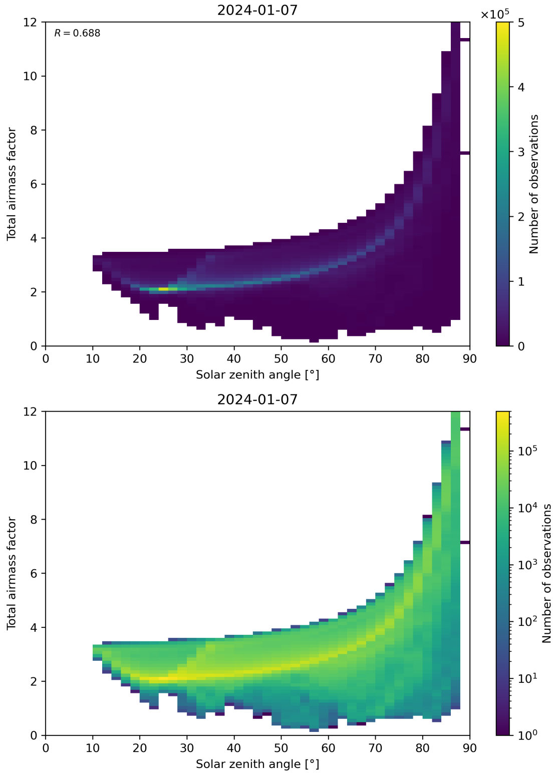
Figure 146: Scatter density plot of “Solar zenith angle” against “Total air mass factor” for 2024-01-06 to 2024-01-08.
