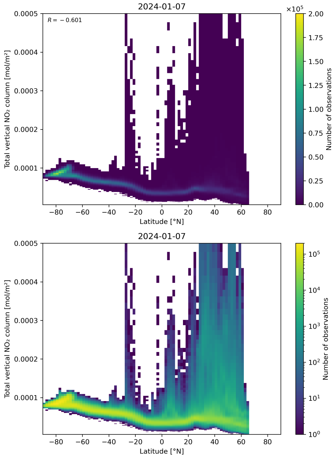
Figure 90: Scatter density plot of “Latitude” against “Total vertical NO 2 column” for 2024-01-06 to 2024-01-08.
