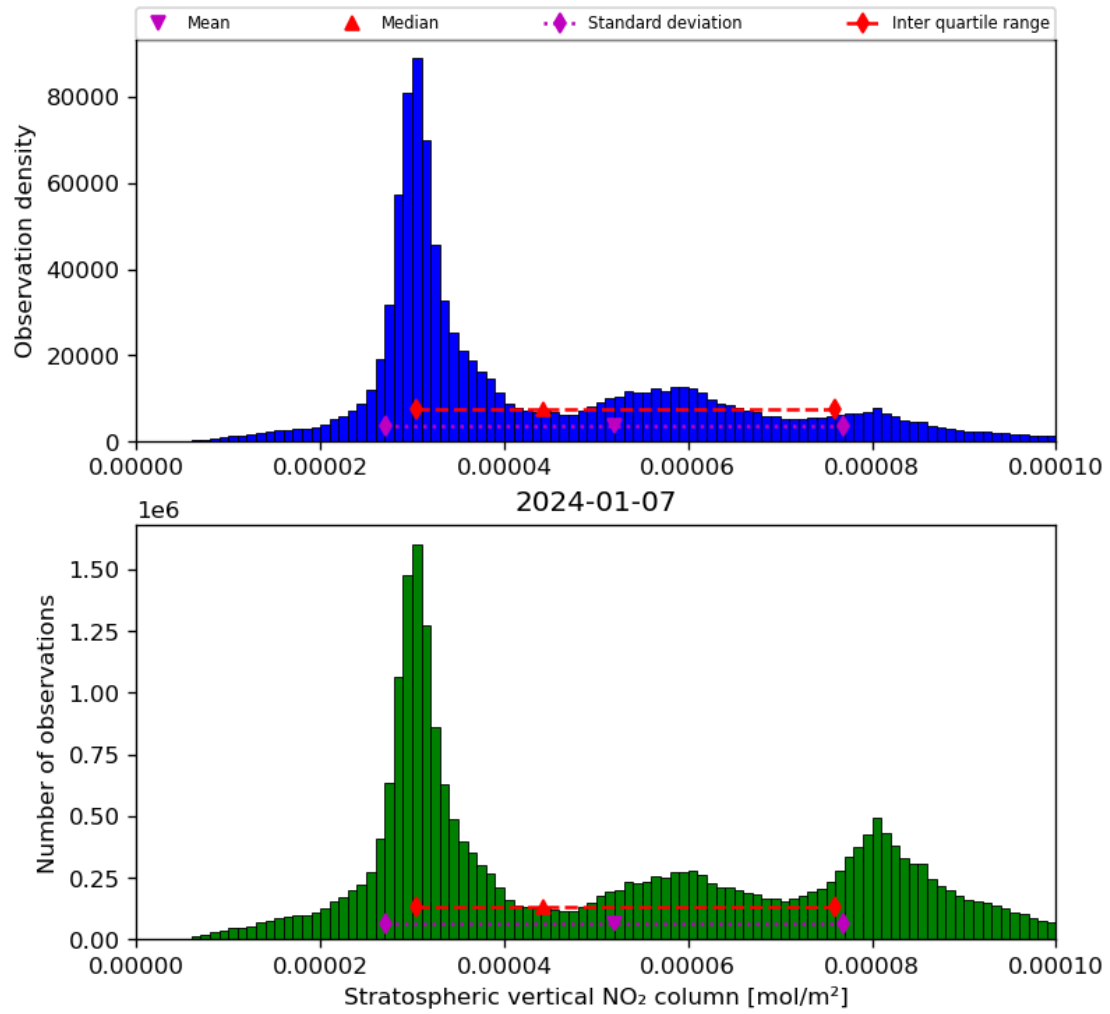
Figure 36: Histogram of “Stratospheric vertical NO 2 column” for 2024-01-06 to 2024-01-08
