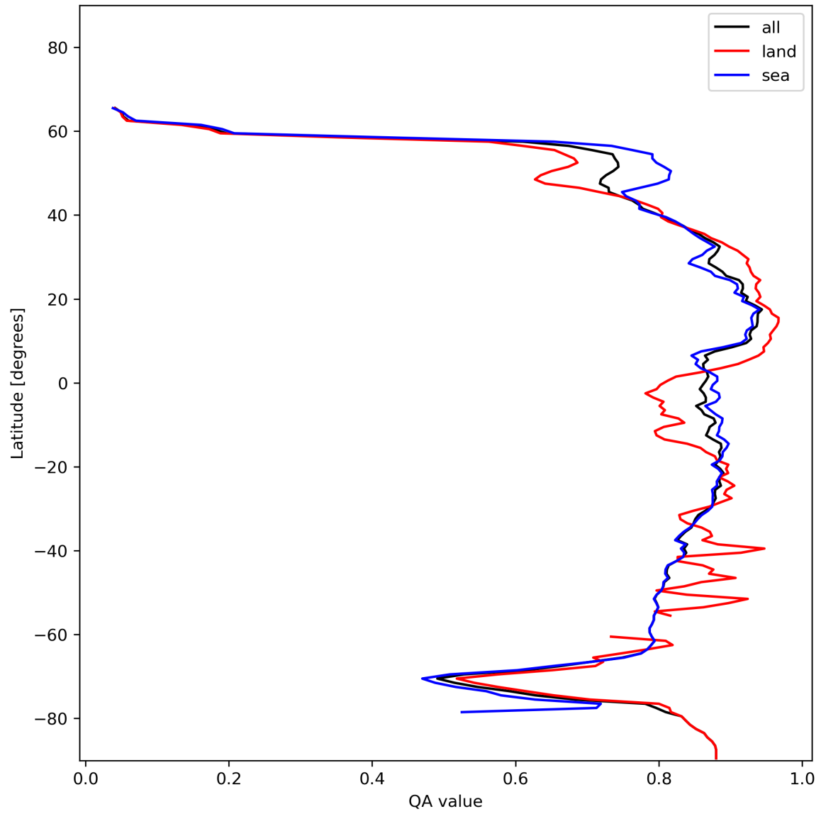
Figure 11: Zonal average of “QA value” for 2024-01-06 to 2024-01-08.
