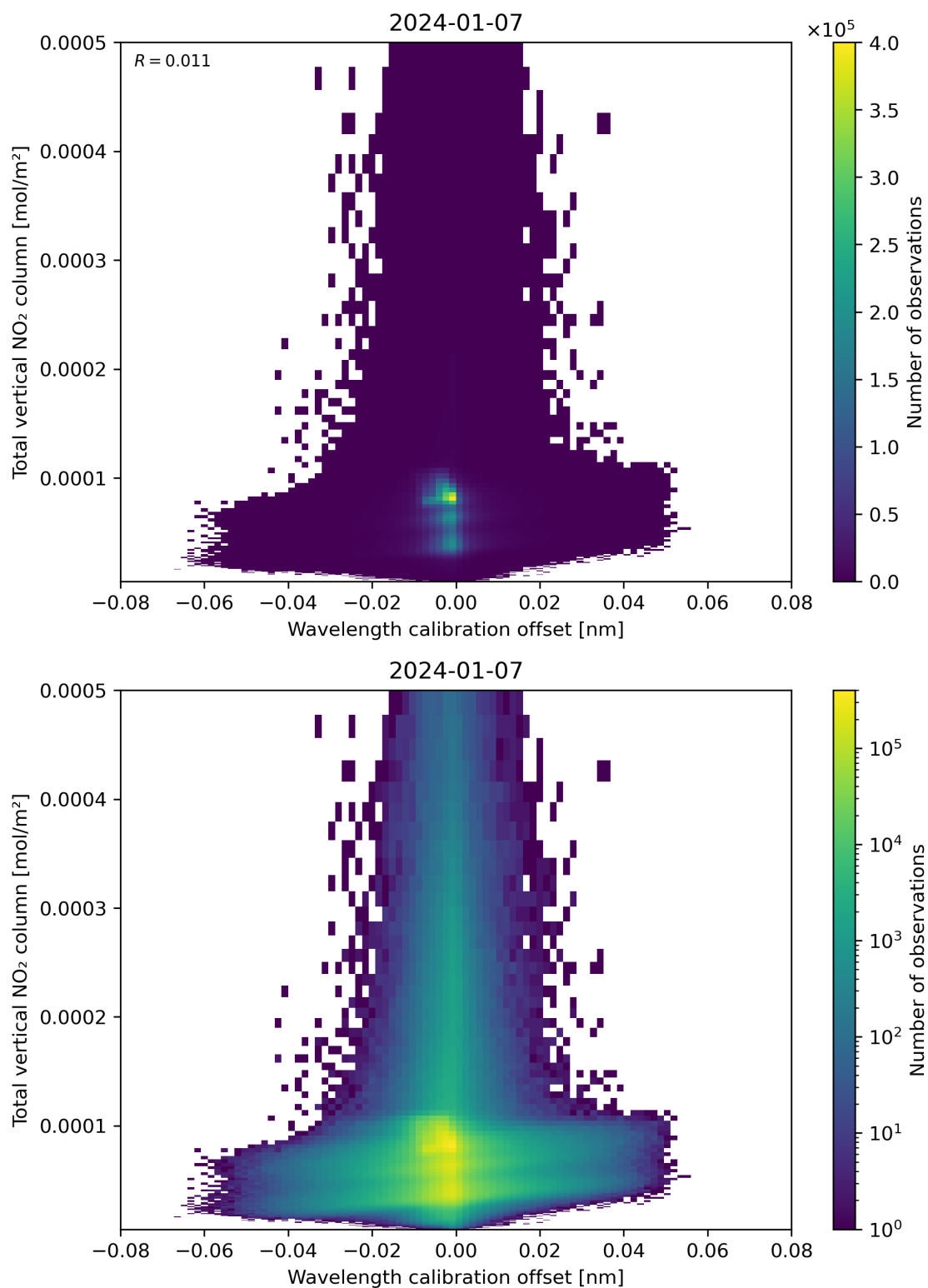
Figure 179: Scatter density plot of “Wavelength calibration offset” against “Total vertical NO 2 column” for 2024-01-06 to 2024-01-08.
