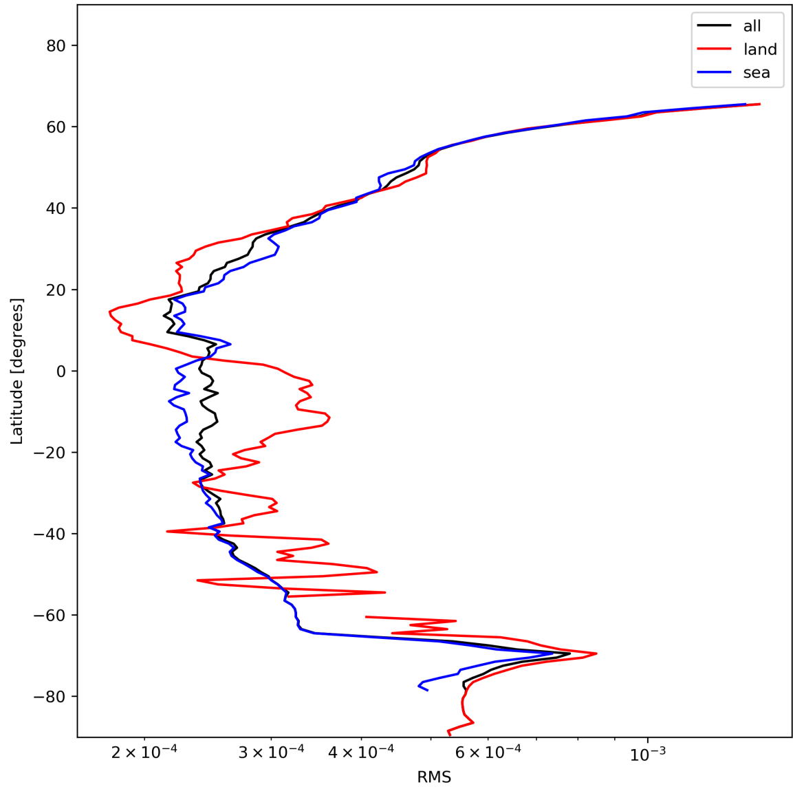
Figure 26: Zonal average of “RMS” for 2024-01-06 to 2024-01-08.
