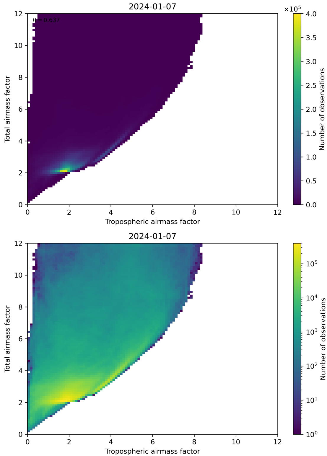
Figure 72: Scatter density plot of “Tropospheric airmass factor” against “Total airmass factor” for 2024-01-06 to 2024-01-08.
