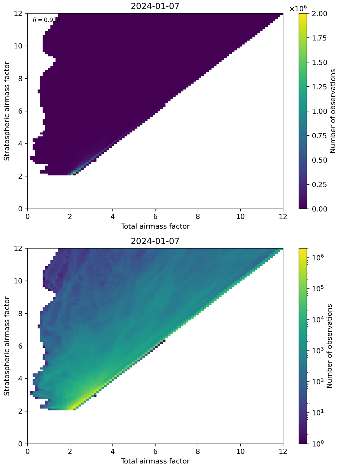
Figure 62: Scatter density plot of “Total airmass factor” against “Stratospheric airmass factor” for 2024-01-06 to 2024-01-08.
