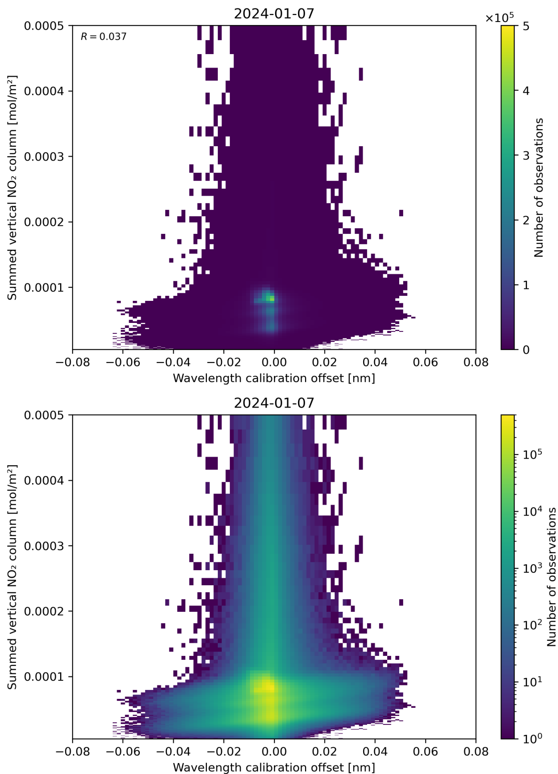
Figure 177: Scatter density plot of “Wavelength calibration offset” against “Summed vertical NO 2 column” for 2024-01-06 to 2024-01-08.
