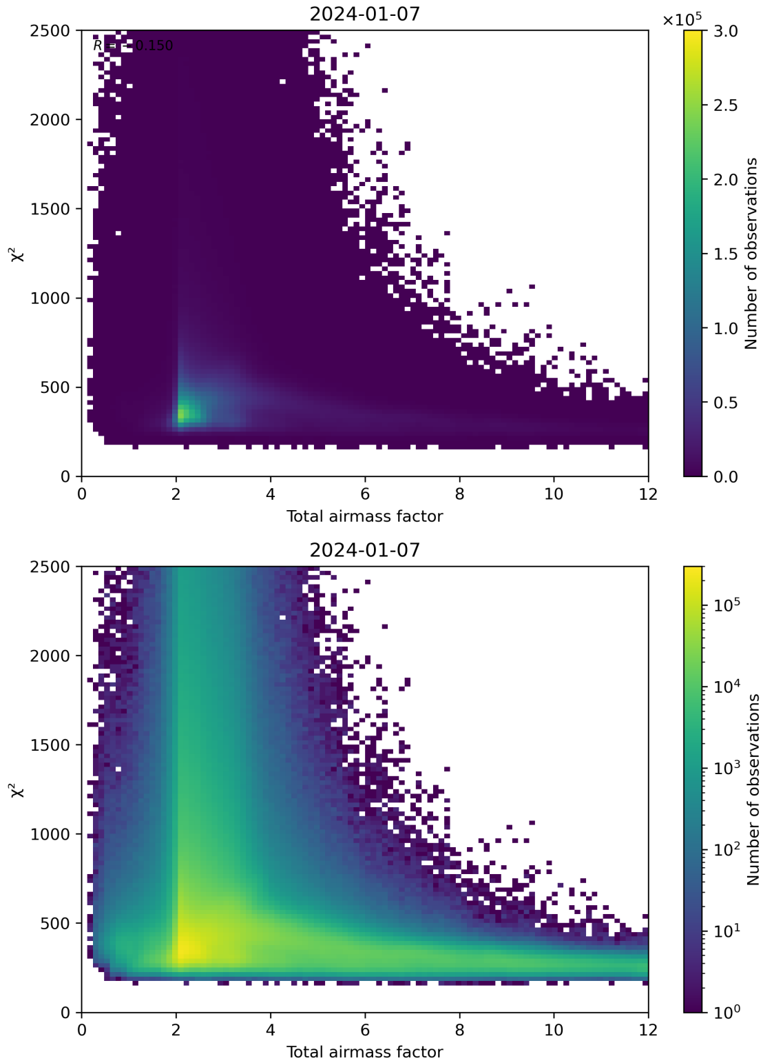
Figure 63: Scatter density plot of “Total airmass factor” against “ \chi^2 ” for 2024-01-06 to 2024-01-08.
