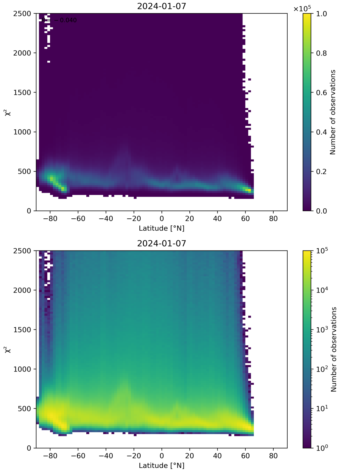
Figure 86: Scatter density plot of “Latitude” against “ \chi^2 ” for 2024-01-06 to 2024-01-08.
