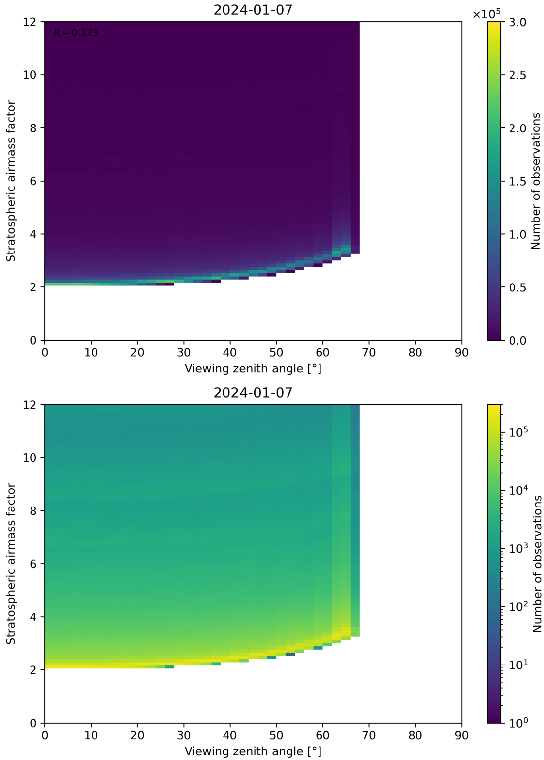
Figure 159: Scatter density plot of “Viewing zenith angle” against “Stratospheric airmass factor” for 2024-01-06 to 2024-01-08.
