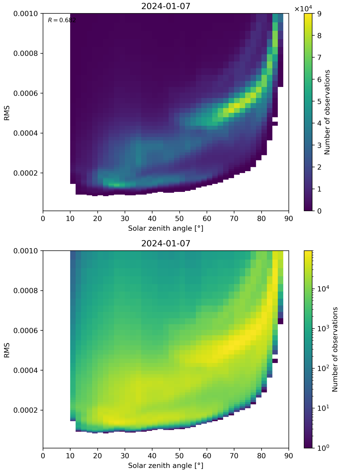
Figure 157: Scatter density plot of “Solar zenith angle” against “RMS” for 2024-01-06 to 2024-01-08.
