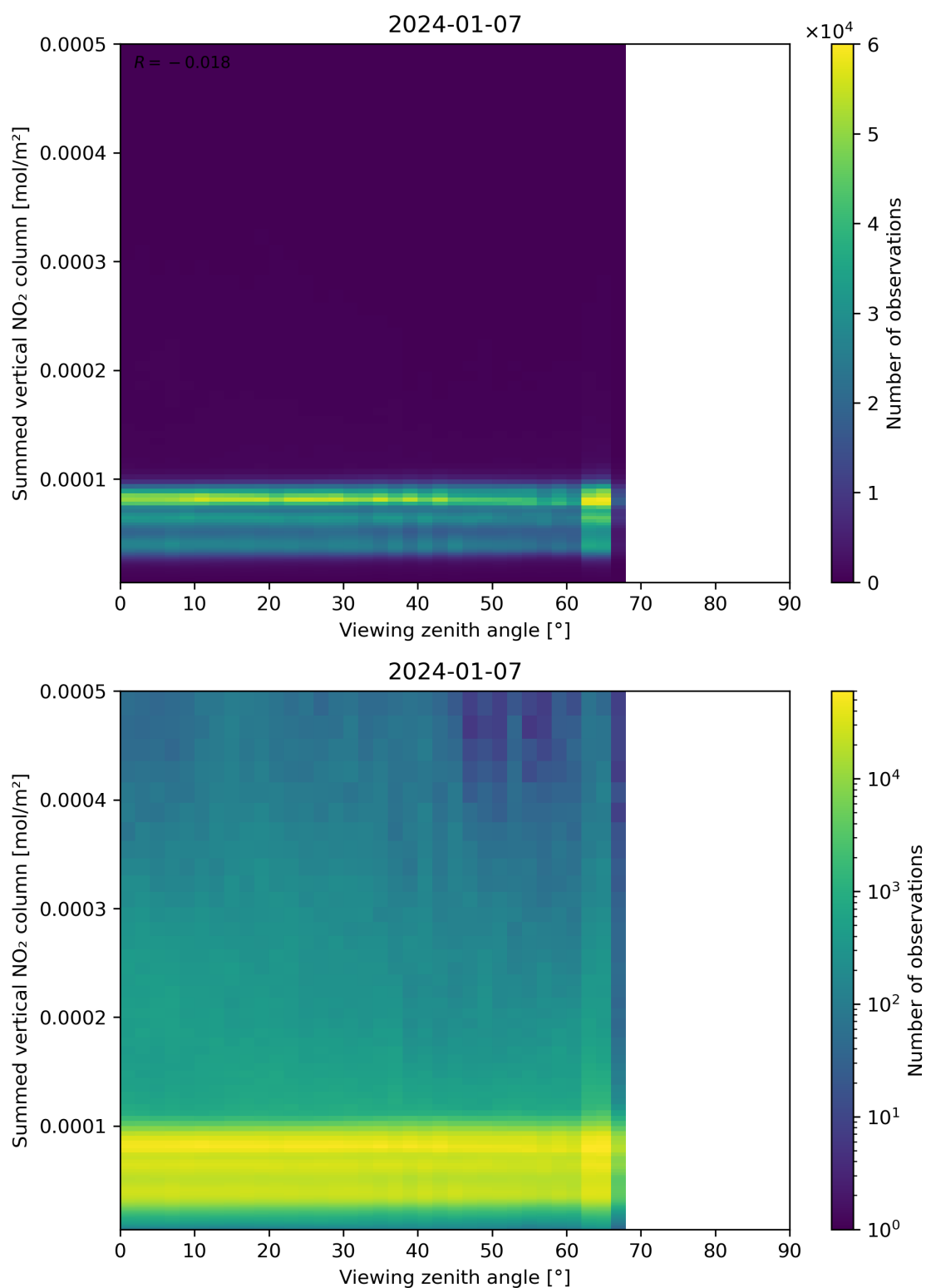
Figure 165: Scatter density plot of “Viewing zenith angle” against “Summed vertical NO 2 column” for 2024-01-06 to 2024-01-08.
