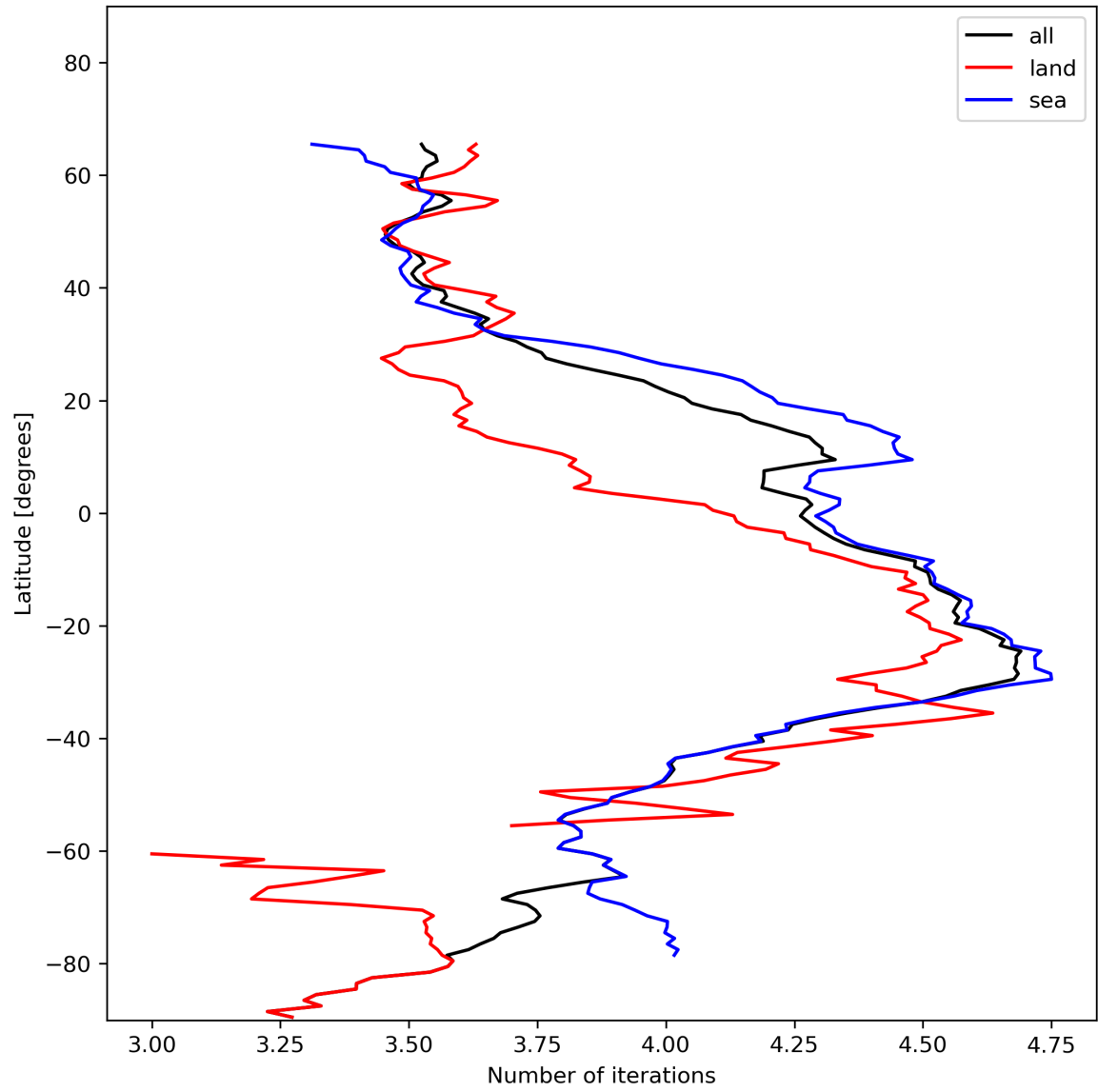
Figure 17: Zonal average of “Number of iterations” for 2024-01-06 to 2024-01-08.
