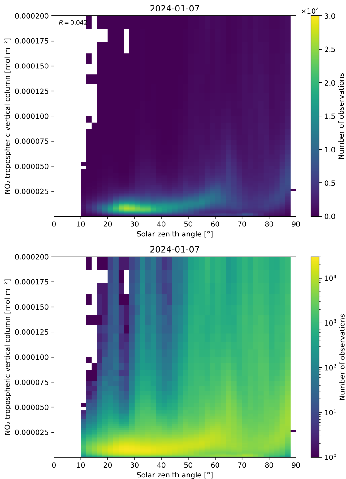
Figure 155: Scatter density plot of “Solar zenith angle” against “NO 2 tropospheric vertical column” for 2024-01-06 to 2024-01-08.
