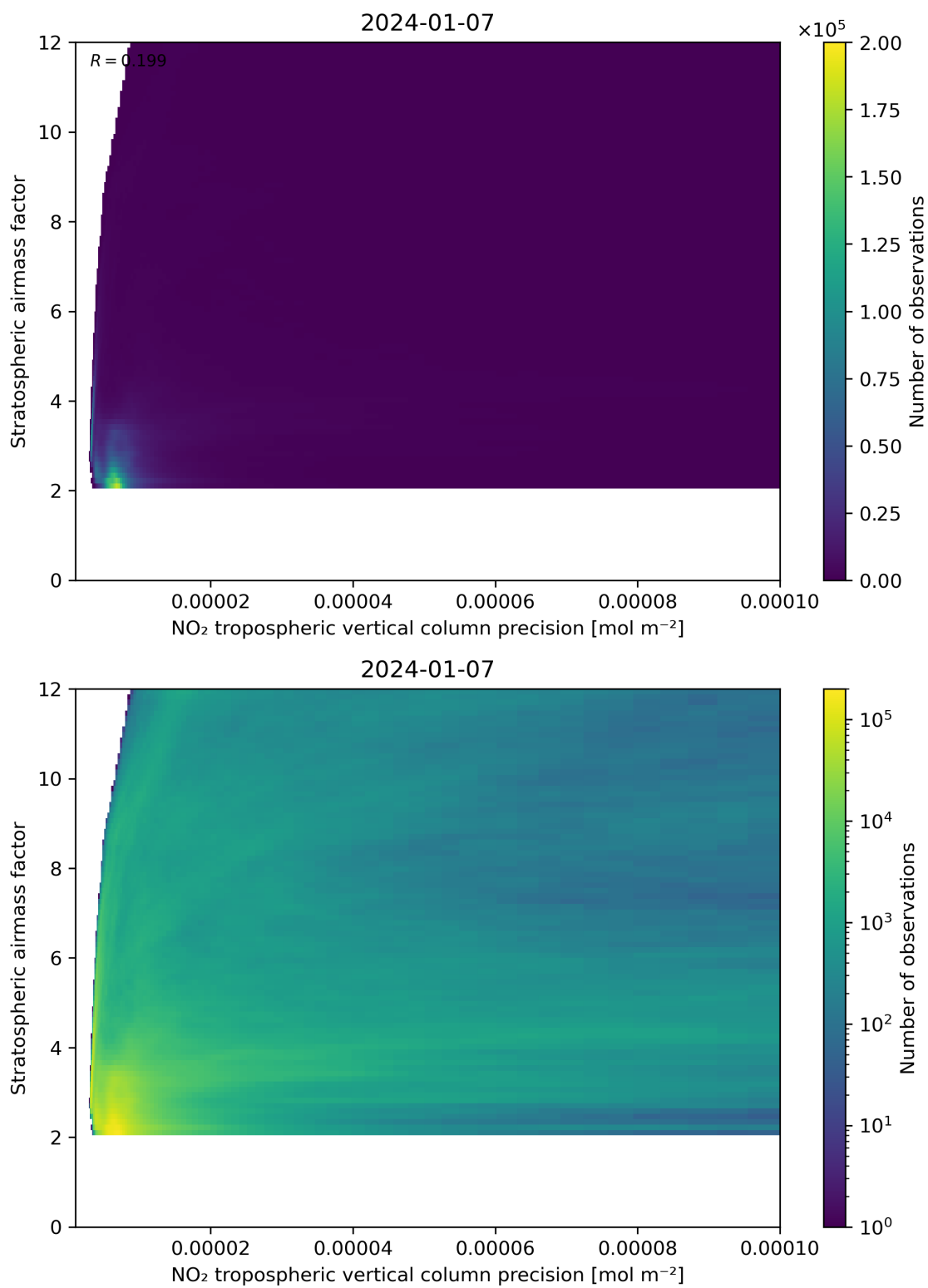
Figure 131: Scatter density plot of “NO 2 tropospheric vertical column precision” against “Stratospheric airmass factor” for 2024-01-06 to 2024-01-08.
