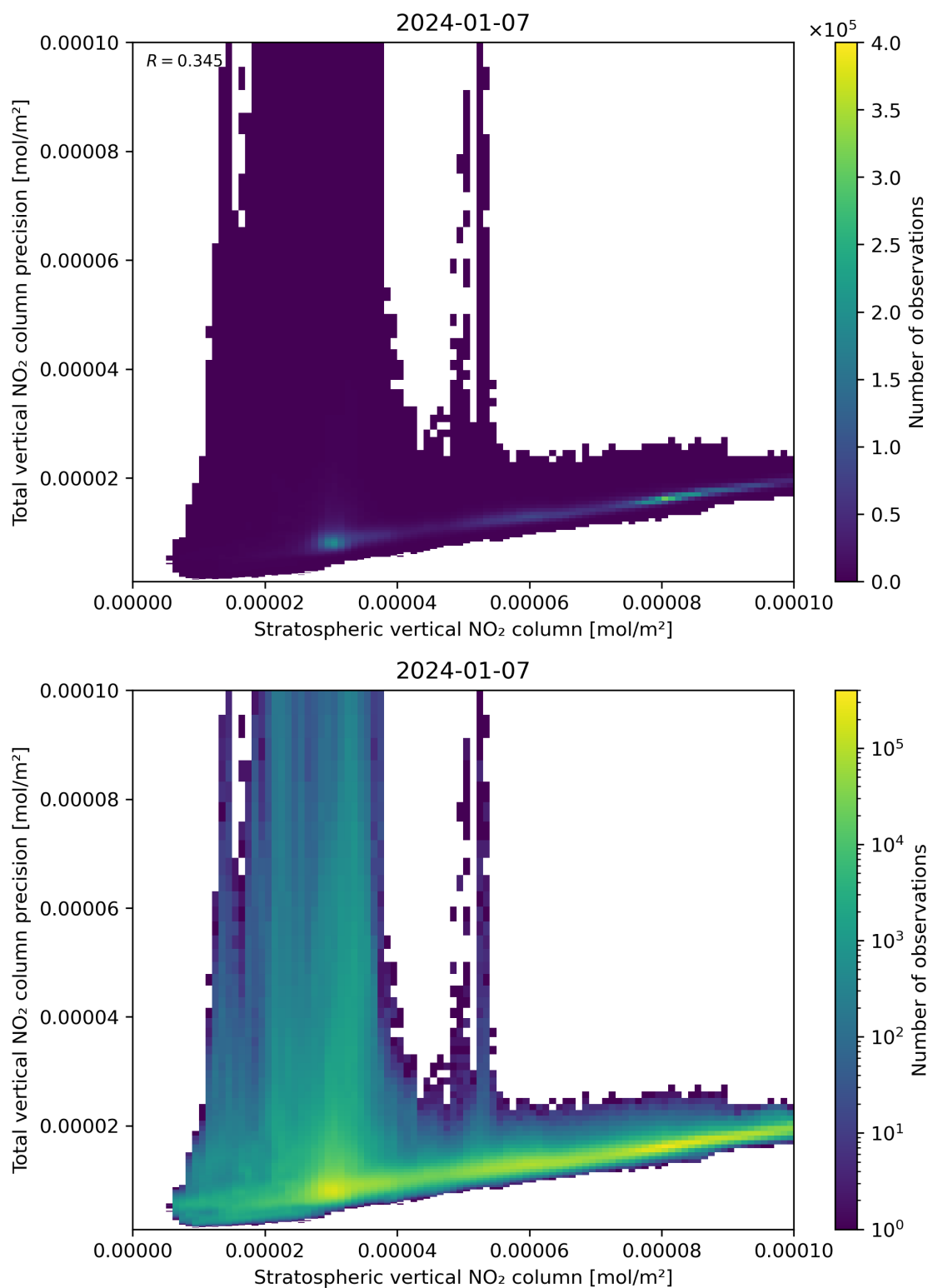
Figure 101: Scatter density plot of “Stratospheric vertical NO 2 column” against “Total vertical NO 2 column precision” for 2024-01-06 to 2024-01-08.
