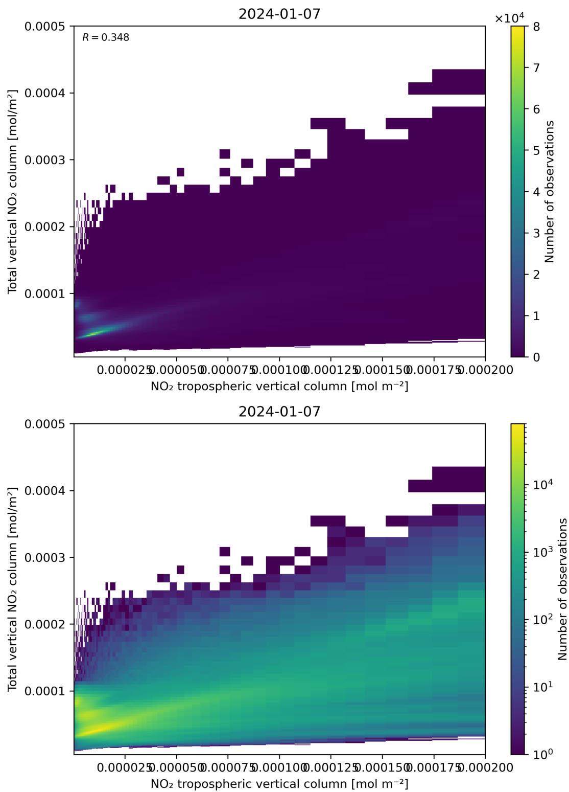
Figure 128: Scatter density plot of “NO 2 tropospheric vertical column” against “Total vertical NO 2 column” for 2024-01-06 to 2024-01-08.
