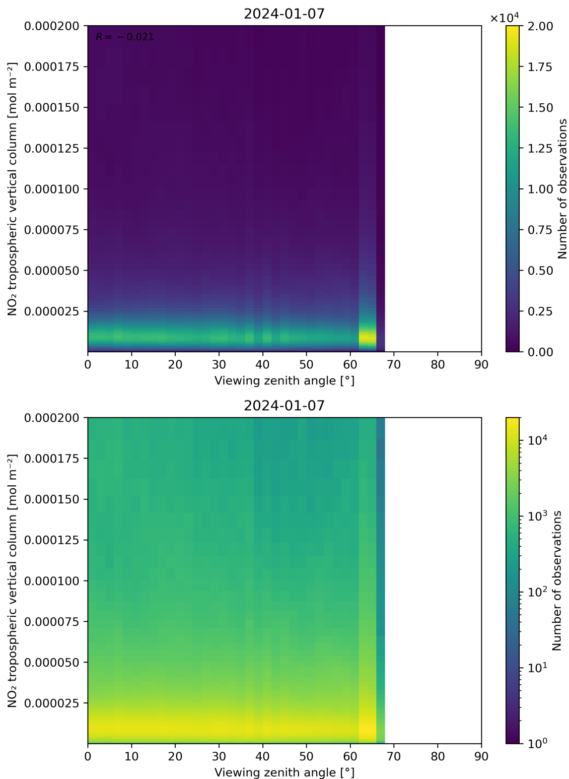
Figure 169: Scatter density plot of “Viewing zenith angle” against “NO 2 tropospheric vertical column” for 2024-01-06 to 2024-01-08.
