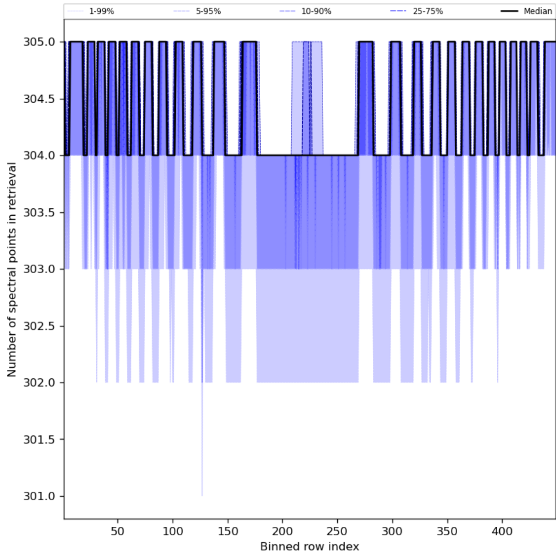
Figure 50: Along track statistics of “Number of spectral points in retrieval” for 2024-01-06 to 2024-01-08
