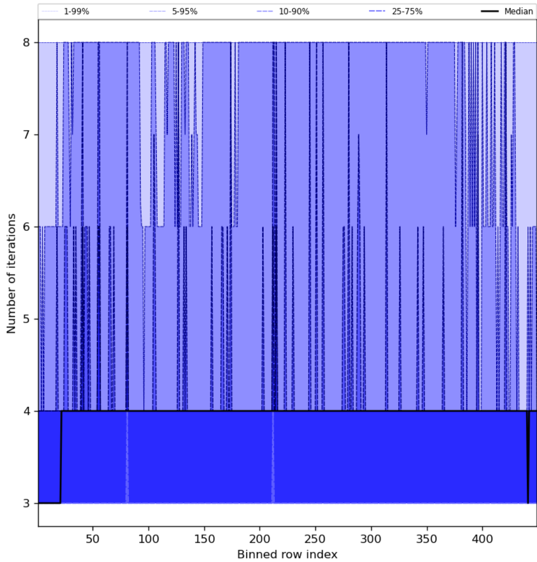
Figure 51: Along track statistics of “Number of iterations” for 2024-01-06 to 2024-01-08
