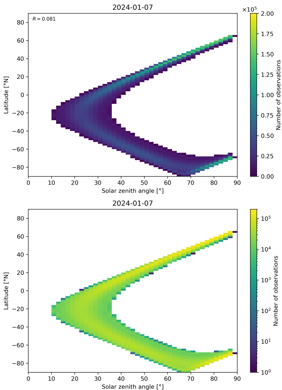
Figure 149: Scatter density plot of “Solar zenith angle” against “Latitude” for 2024-01-06 to 2024-01-08.
