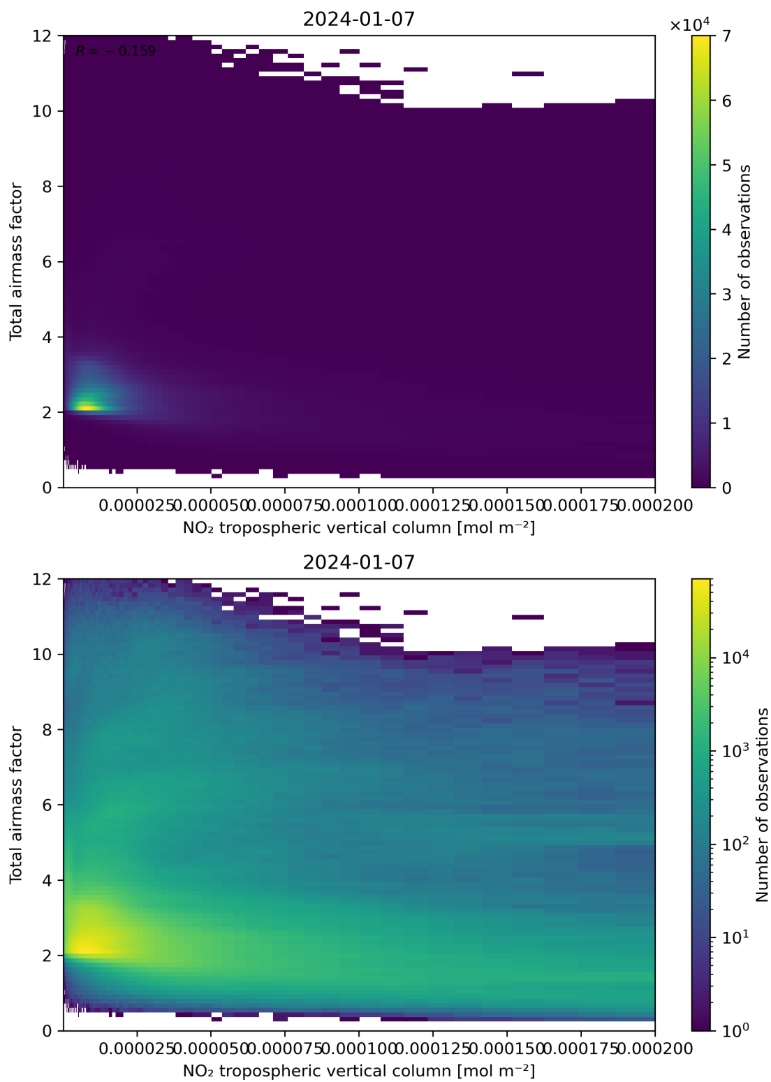
Figure 122: Scatter density plot of “NO 2 tropospheric vertical column” against “Total air mass factor” for 2024-01-06 to 2024-01-08.
