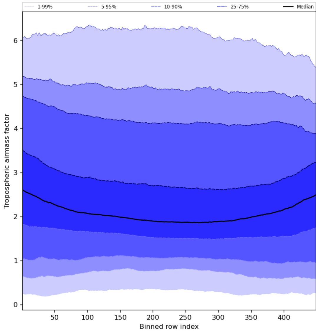
Figure 48: Along track statistics of “Tropospheric airmass factor” for 2024-01-06 to 2024-01-08
