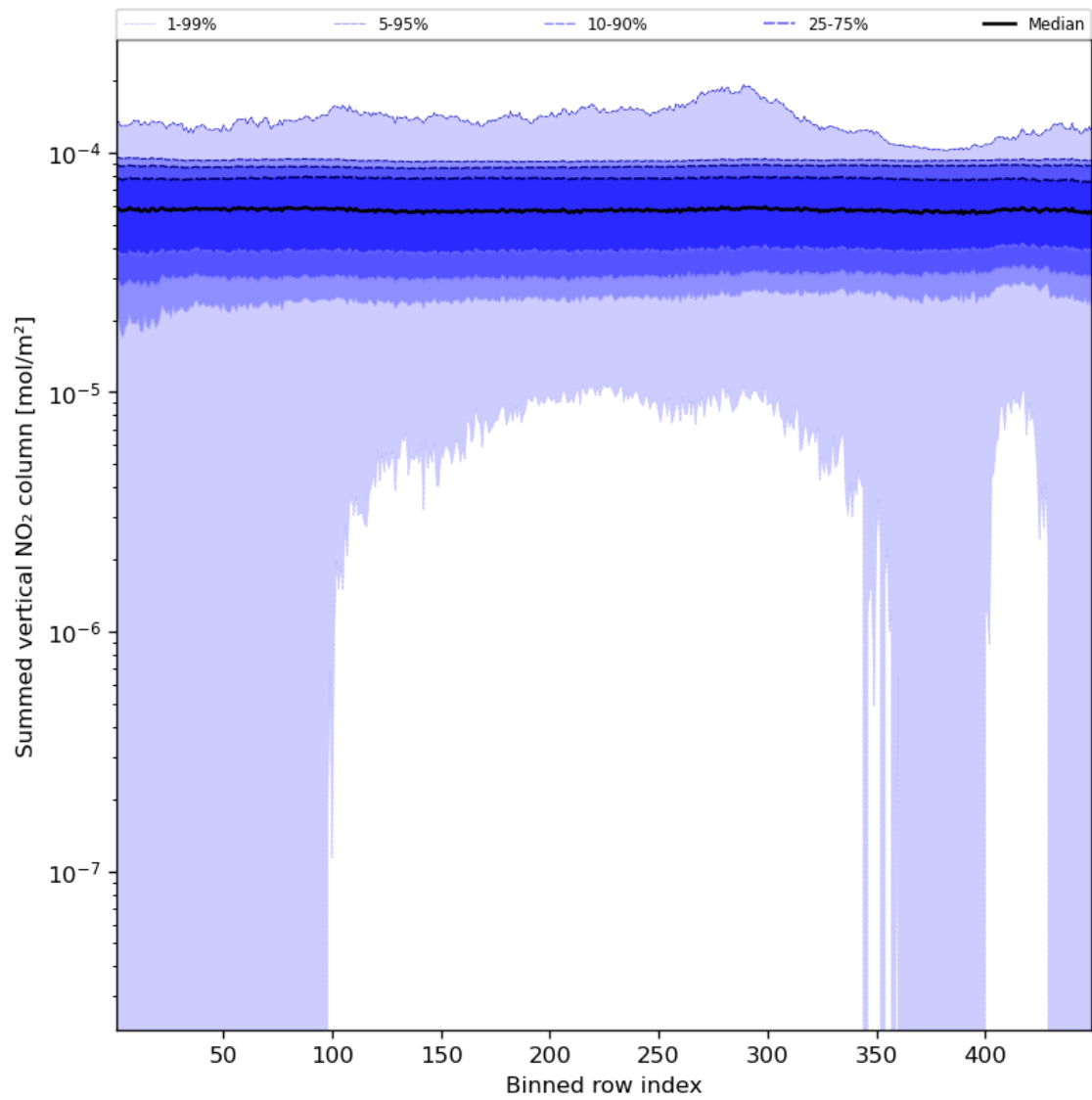
Figure 57: Along track statistics of “Summed vertical NO 2 column” for 2024-01-06 to 2024-01-08
