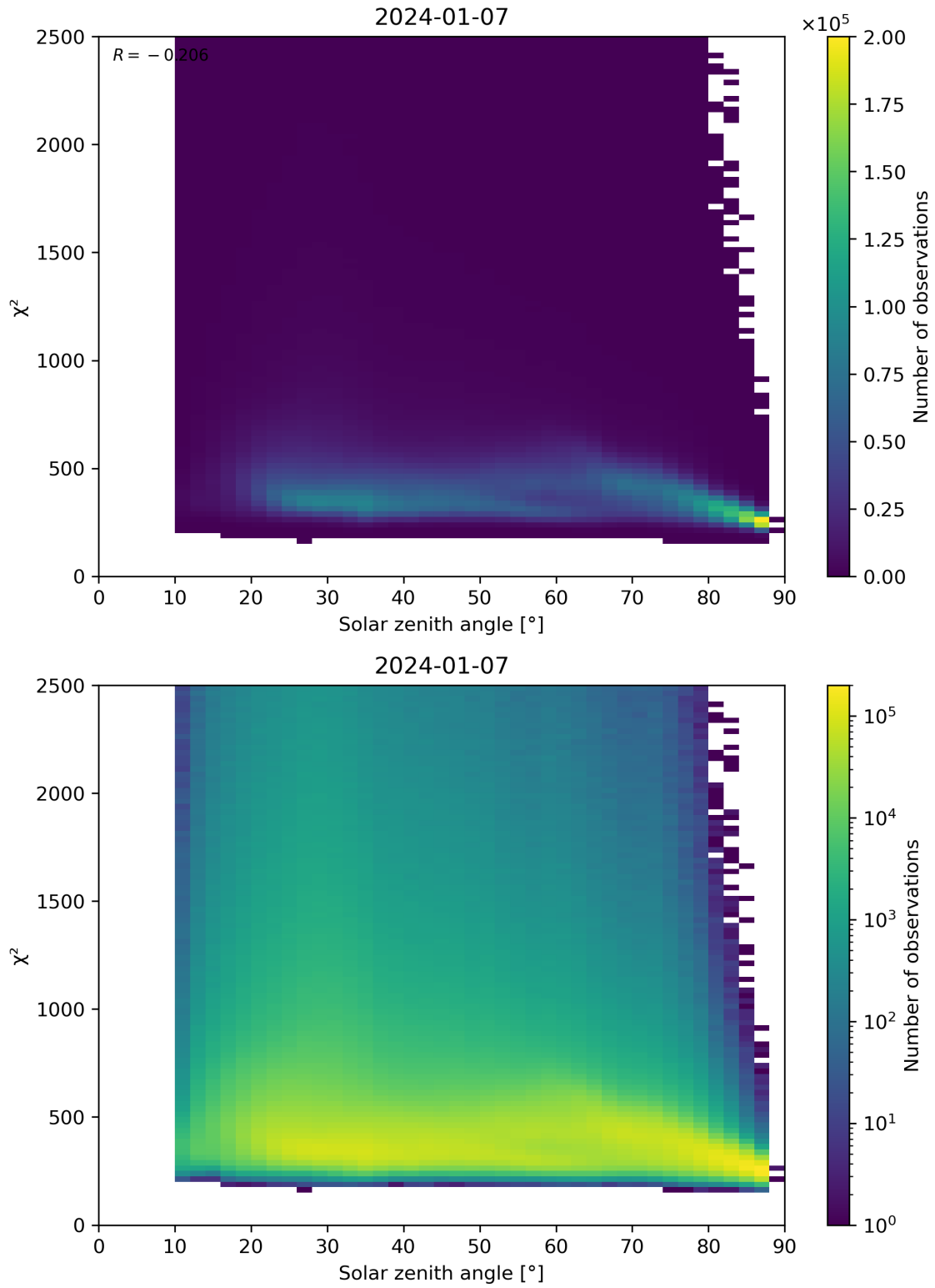
Figure 148: Scatter density plot of “Solar zenith angle” against “ \chi^2 ” for 2024-01-06 to 2024-01-08.
