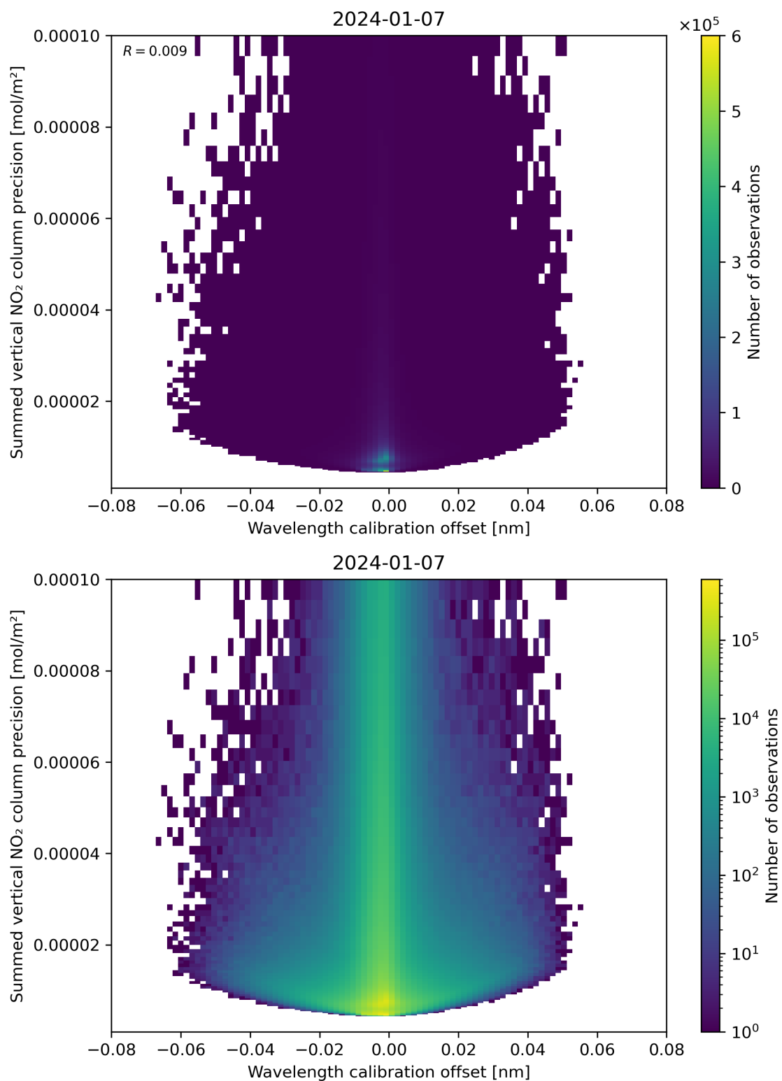
Figure 178: Scatter density plot of “Wavelength calibration offset” against “Summed vertical NO 2 column precision” for 2024-01-06 to 2024-01-08.
