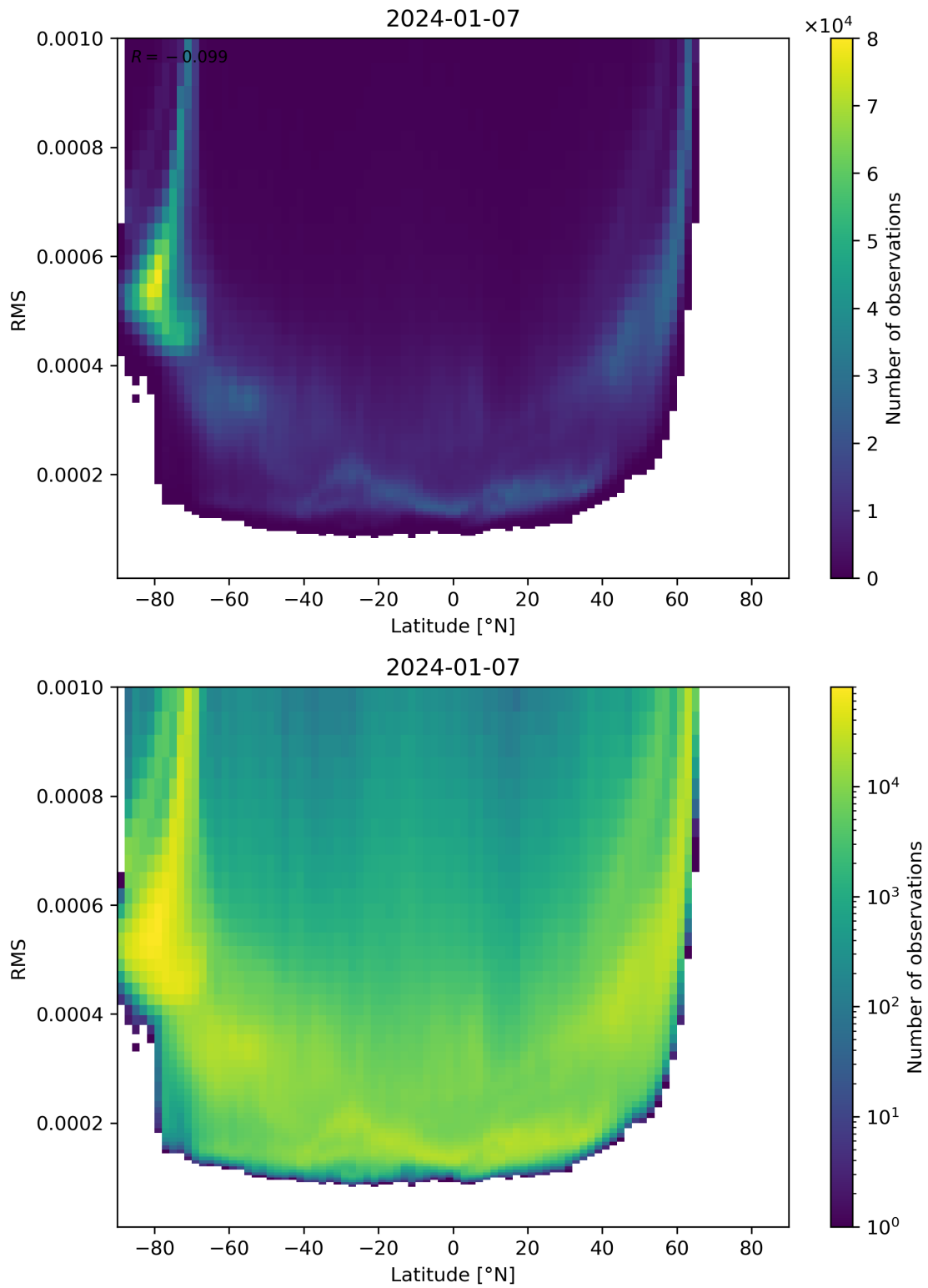
Figure 94: Scatter density plot of “Latitude” against “RMS” for 2024-01-06 to 2024-01-08.
