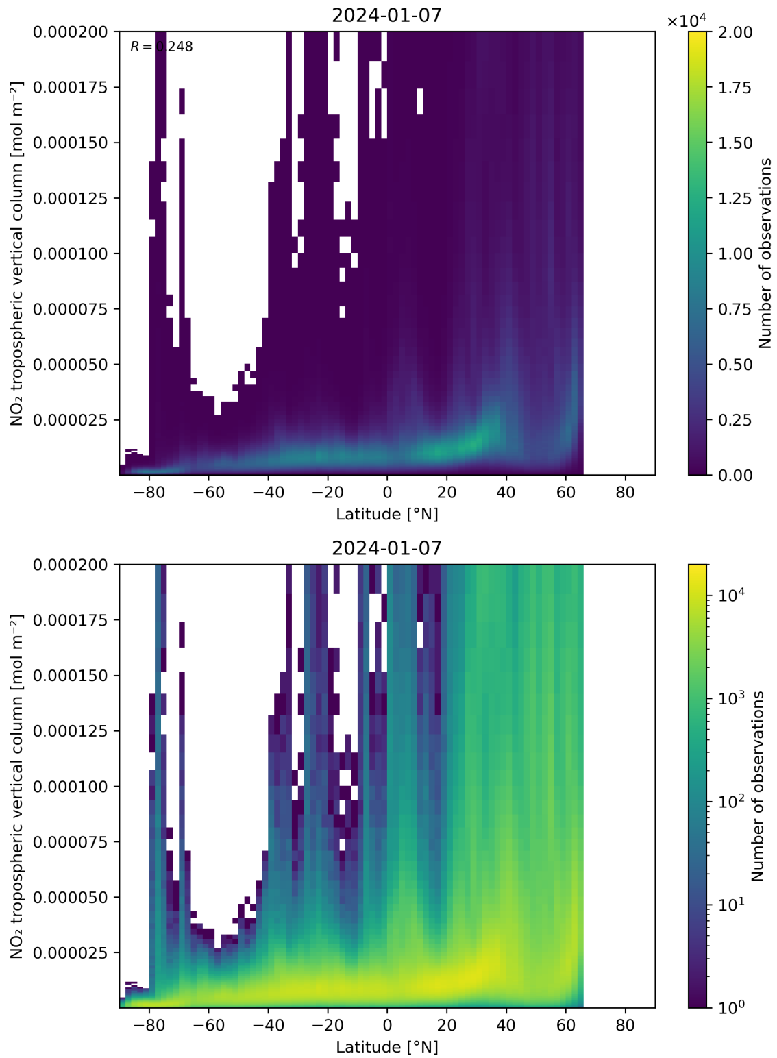
Figure 92: Scatter density plot of “Latitude” against “NO 2 tropospheric vertical column” for 2024-01-06 to 2024-01-08.
