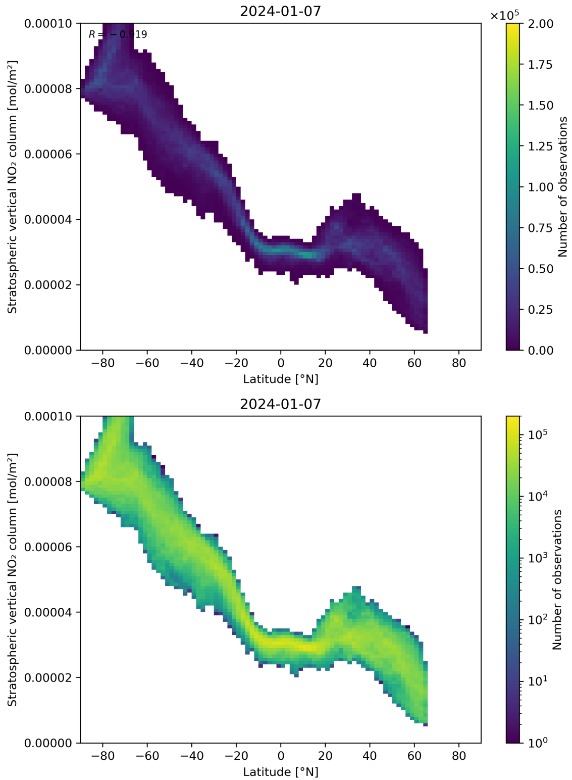
Figure 87: Scatter density plot of “Latitude” against “Stratospheric vertical NO 2 column” for 2024-01-06 to 2024-01-08.
