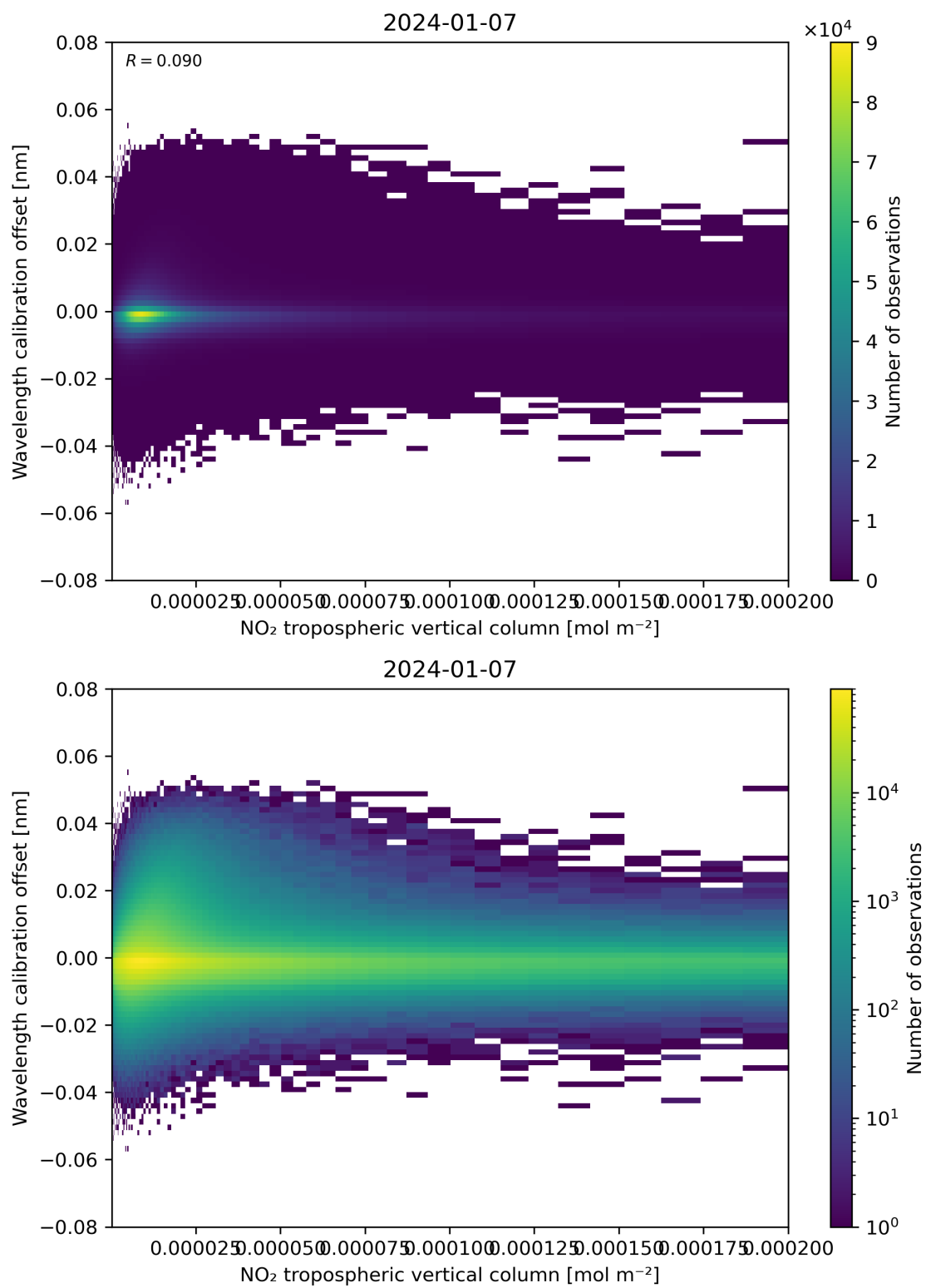
Figure 143: Scatter density plot of “NO 2 tropospheric vertical column” against “Wavelength calibration offset” for 2024-01-06 to 2024-01-08.
