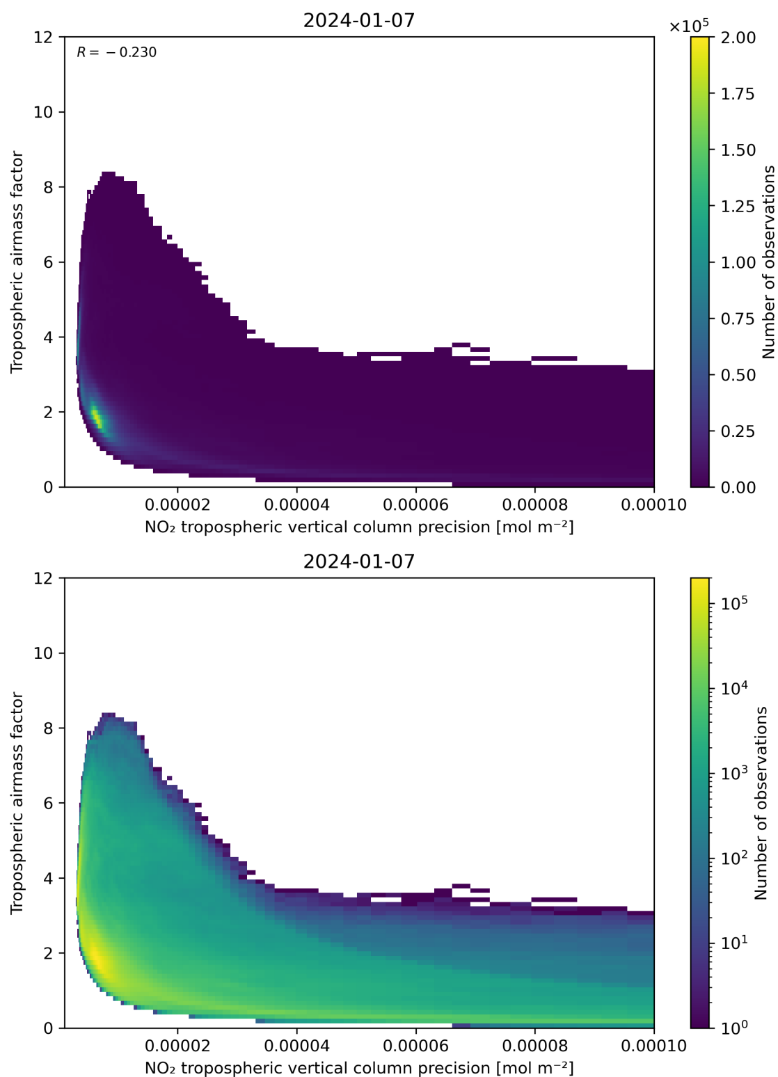
Figure 133: Scatter density plot of “NO 2 tropospheric vertical column precision” against “Tropospheric airmass factor” for 2024-01-06 to 2024-01-08.
