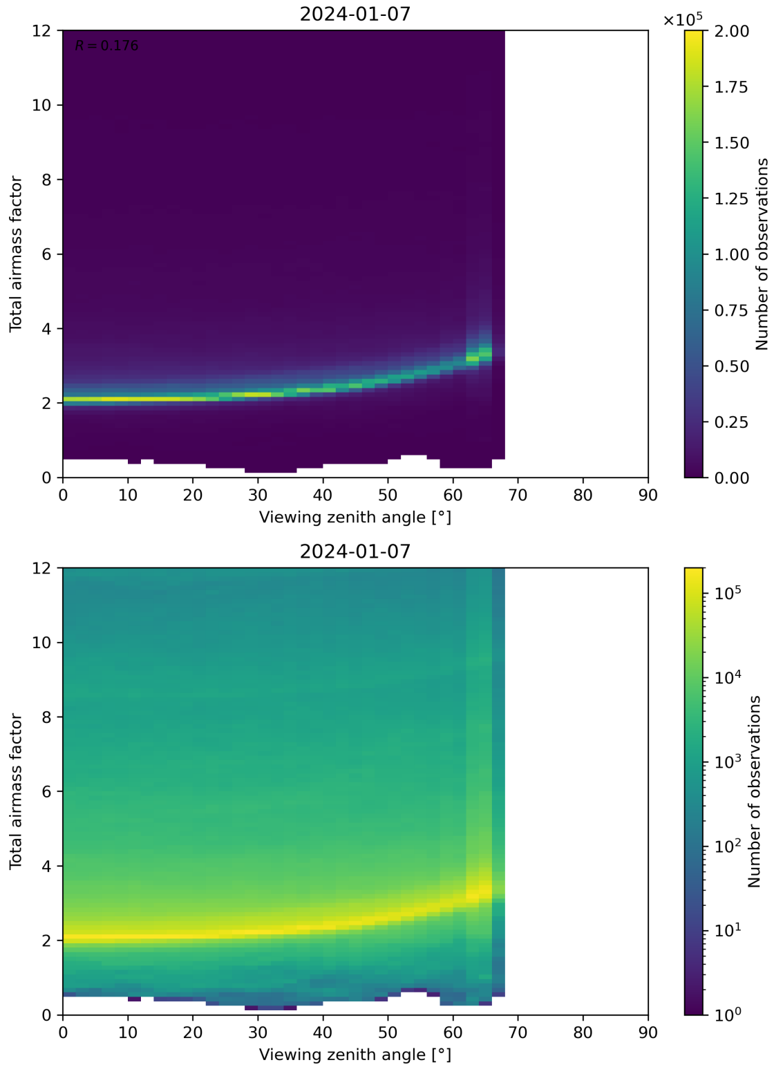
Figure 160: Scatter density plot of “Viewing zenith angle” against “Total airmass factor” for 2024-01-06 to 2024-01-08.
