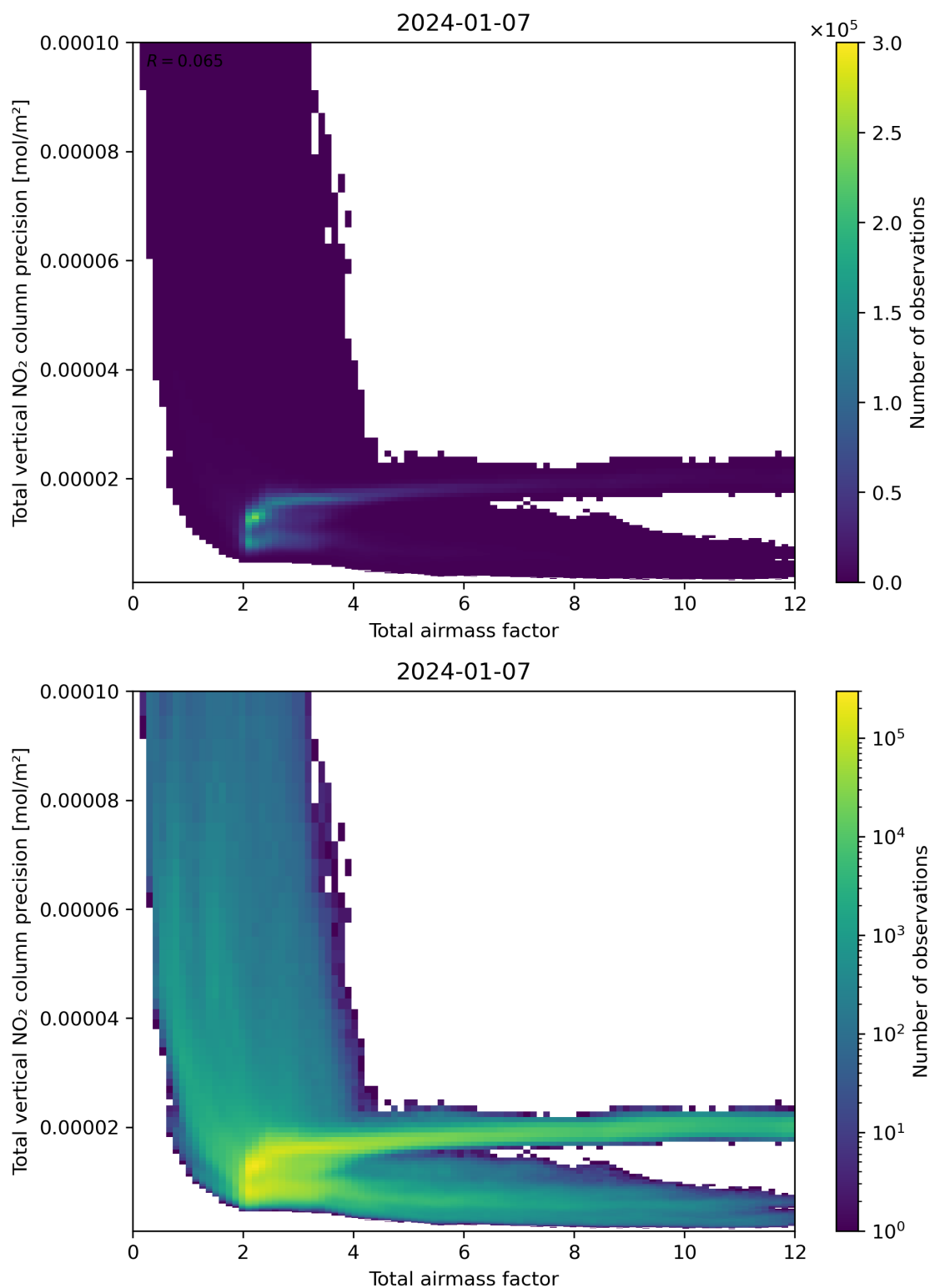
Figure 68: Scatter density plot of “Total airmass factor” against “Total vertical NO 2 column precision” for 2024-01-06 to 2024-01-08.
