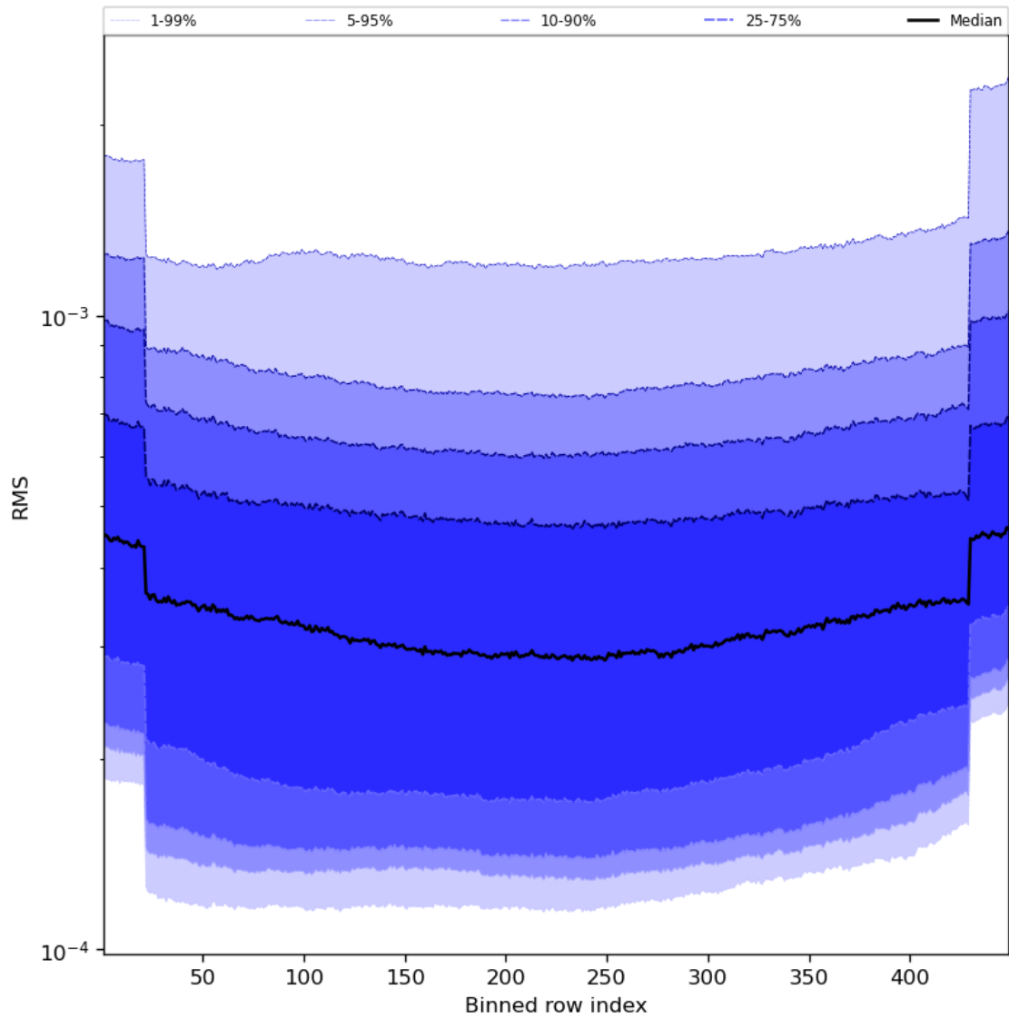
Figure 60: Along track statistics of “RMS” for 2024-01-06 to 2024-01-08
