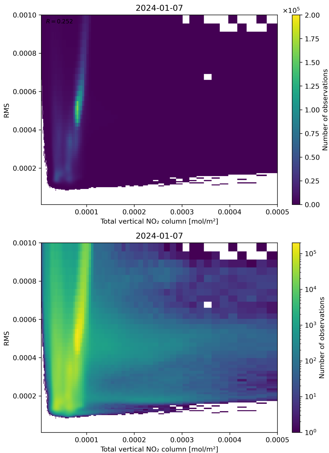
Figure 120: Scatter density plot of “Total vertical NO 2 column” against “RMS” for 2024-01-06 to 2024-01-08.
