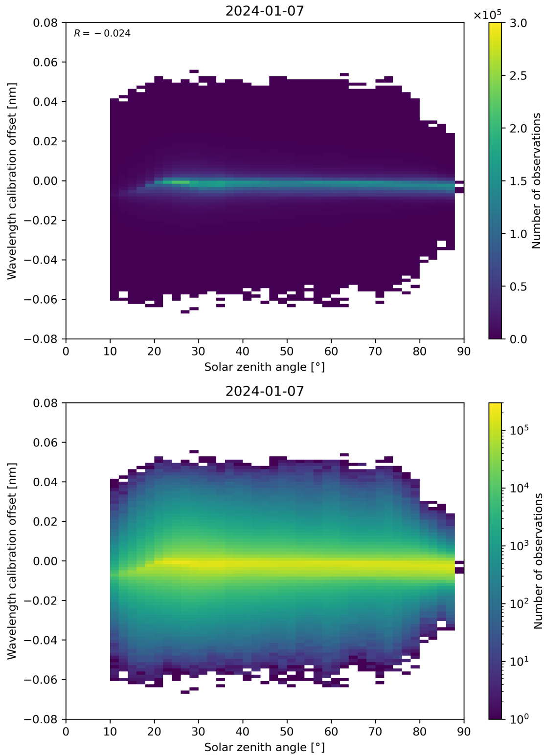
Figure 158: Scatter density plot of “Solar zenith angle” against “Wavelength calibration offset” for 2024-01-06 to 2024-01-08.
