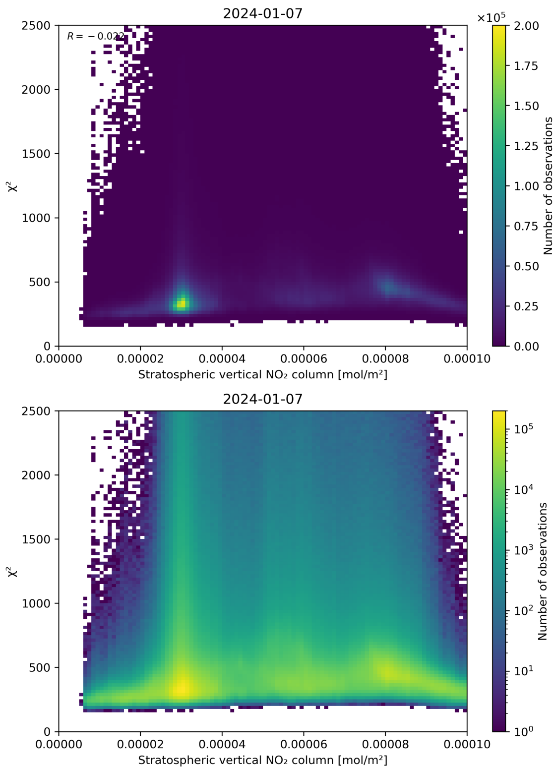
Figure 97: Scatter density plot of “Stratospheric vertical NO 2 column” against “ \chi^2 ” for 2024-01-06 to 2024-01-08.
