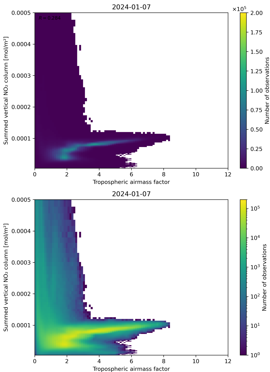
Figure 75: Scatter density plot of “Tropospheric airmass factor” against “Summed vertical NO 2 column” for 2024-01-06 to 2024-01-08.
