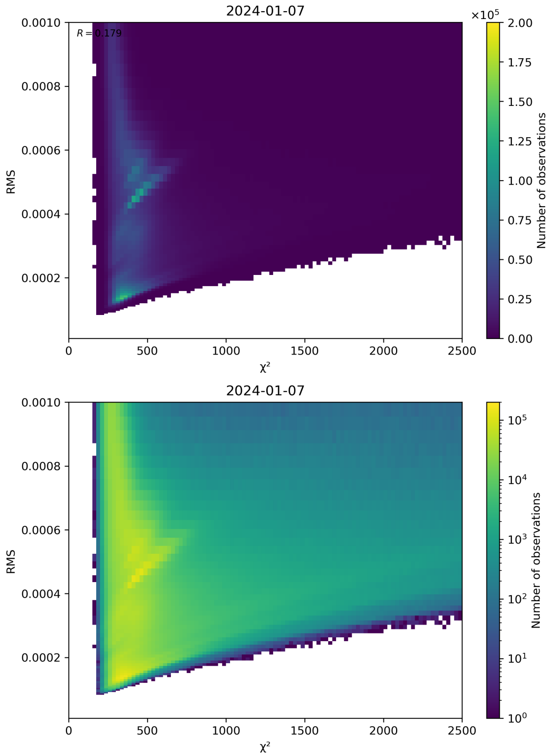
Figure 82: Scatter density plot of “ \chi^2 ” against “RMS” for 2024-01-06 to 2024-01-08.
