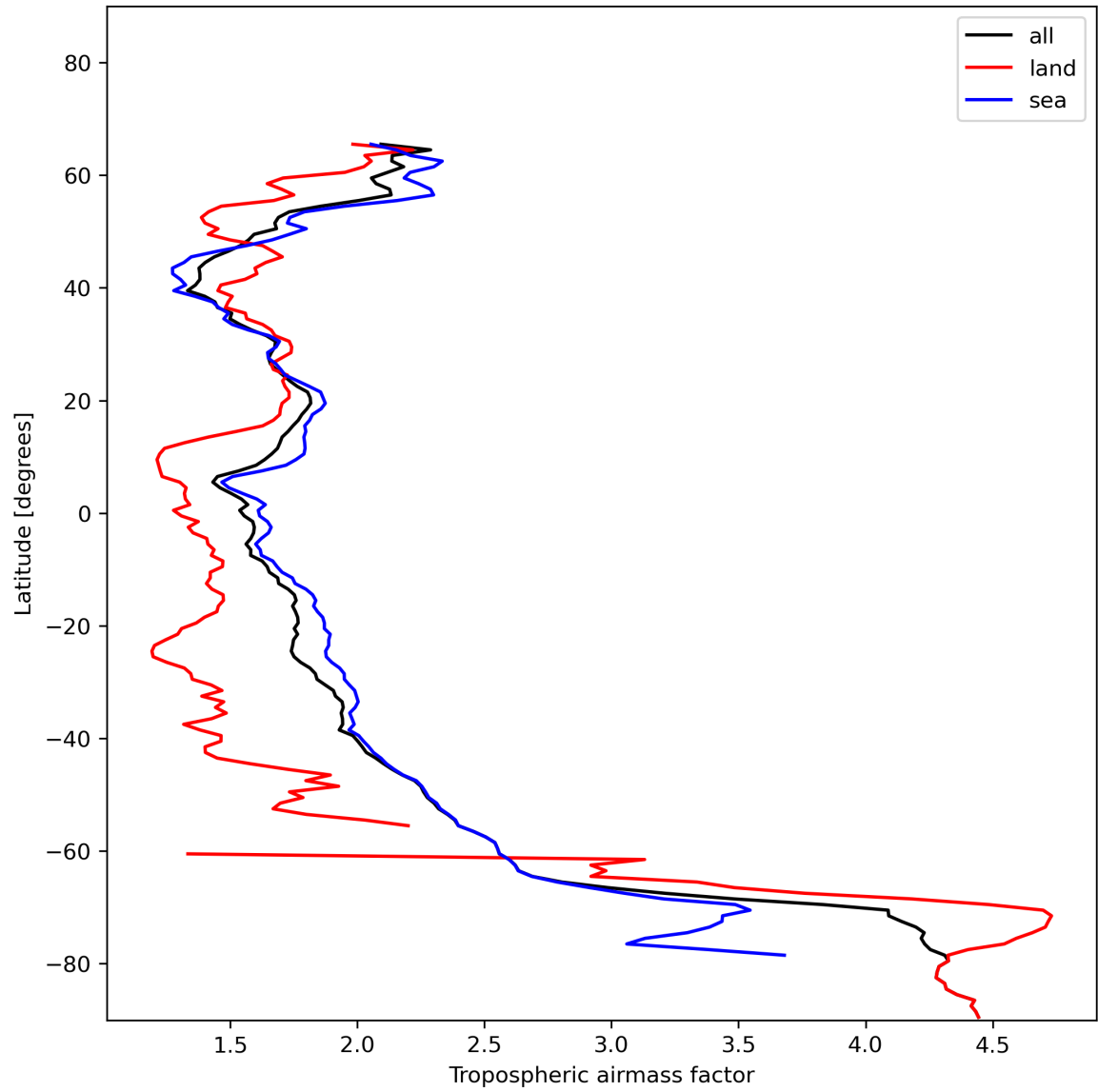
Figure 14: Zonal average of “Tropospheric airmass factor” for 2024-01-06 to 2024-01-08.
