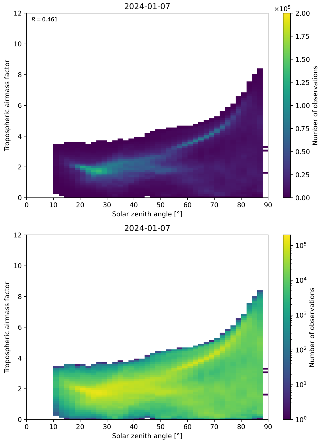
Figure 147: Scatter density plot of “Solar zenith angle” against “Tropospheric airmass factor” for 2024-01-06 to 2024-01-08.
