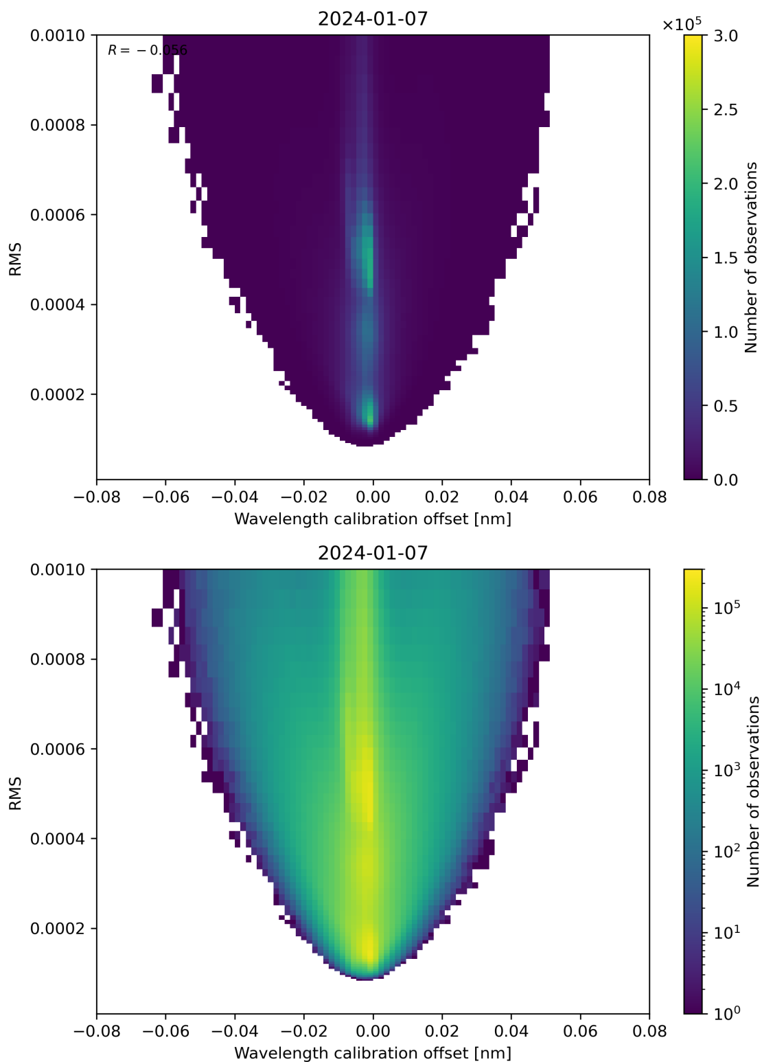
Figure 181: Scatter density plot of “Wavelength calibration offset” against “RMS” for 2024-01-06 to 2024-01-08.
