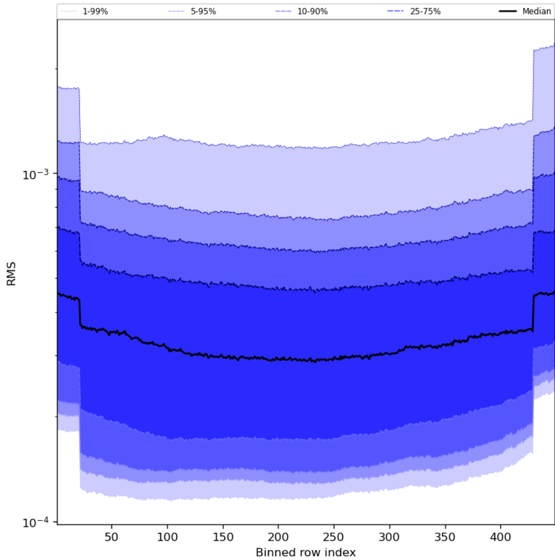
Figure 60: Along track statistics of “RMS” for 2024-01-12 to 2024-01-14
