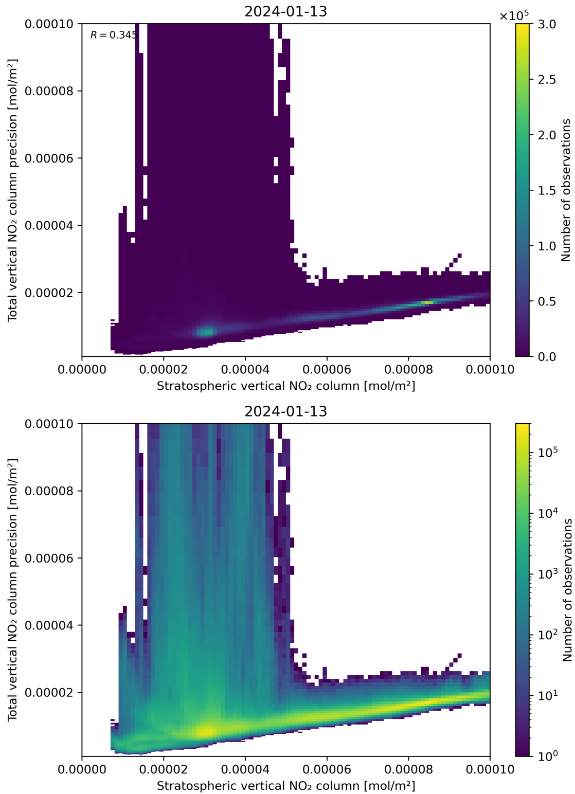
Figure 101: Scatter density plot of “Stratospheric vertical NO 2 column” against “Total vertical NO 2 column precision” for 2024-01-12 to 2024-01-14.
