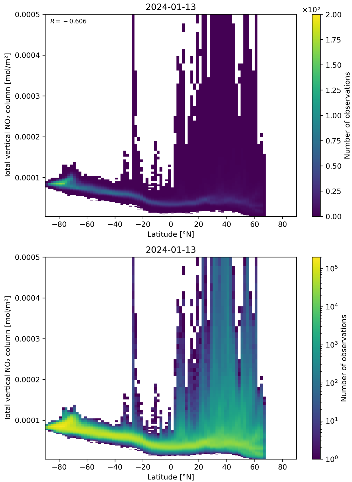
Figure 90: Scatter density plot of “Latitude” against “Total vertical NO 2 column” for 2024-01-12 to 2024-01-14.
