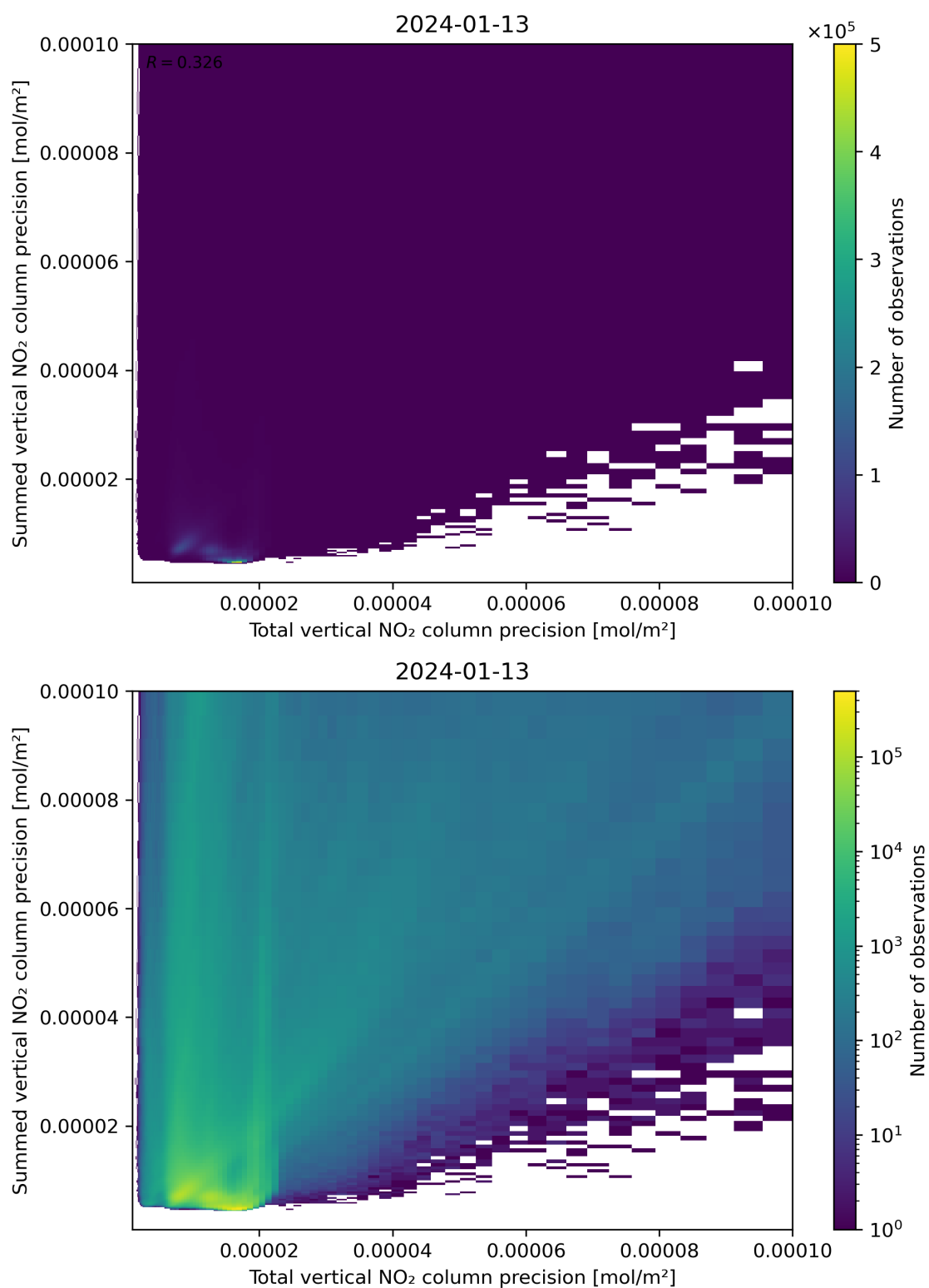
Figure 118: Scatter density plot of “Total vertical NO 2 column precision” against “Summed vertical NO 2 column precision” for 2024-01-12 to 2024-01-14.
