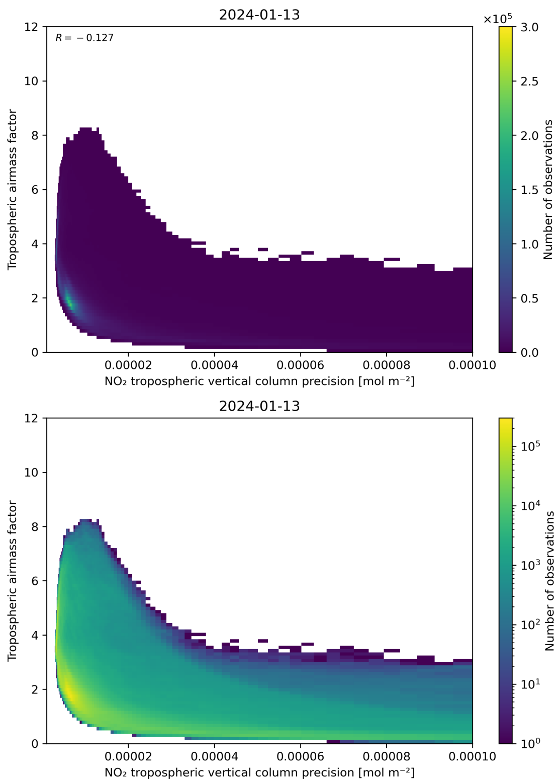
Figure 133: Scatter density plot of “NO 2 tropospheric vertical column precision” against “Tropospheric airmass factor” for 2024-01-12 to 2024-01-14.
