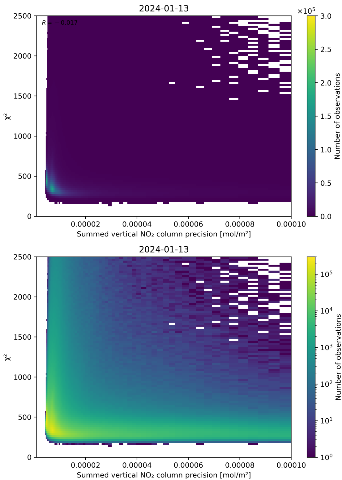
Figure 107: Scatter density plot of “Summed vertical NO 2 column precision” against “ \chi^2 ” for 2024-01-12 to 2024-01-14.
