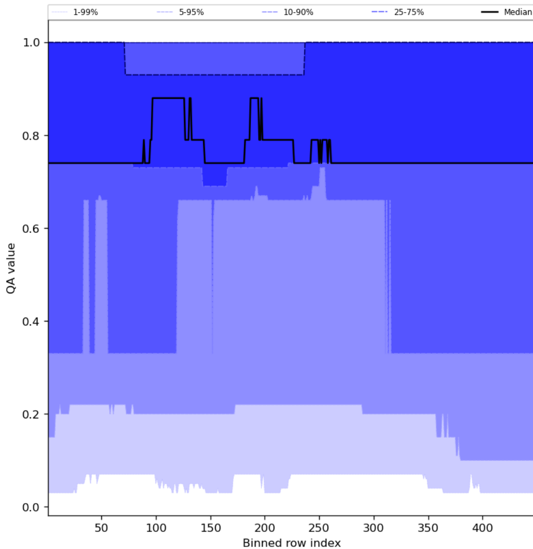
Figure 45: Along track statistics of “QA value” for 2024-01-12 to 2024-01-14
