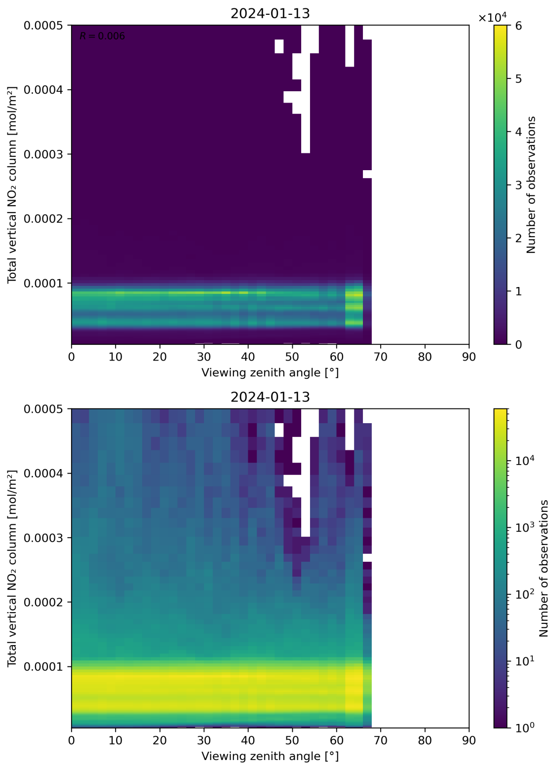
Figure 167: Scatter density plot of “Viewing zenith angle” against “Total vertical NO 2 column” for 2024-01-12 to 2024-01-14.
