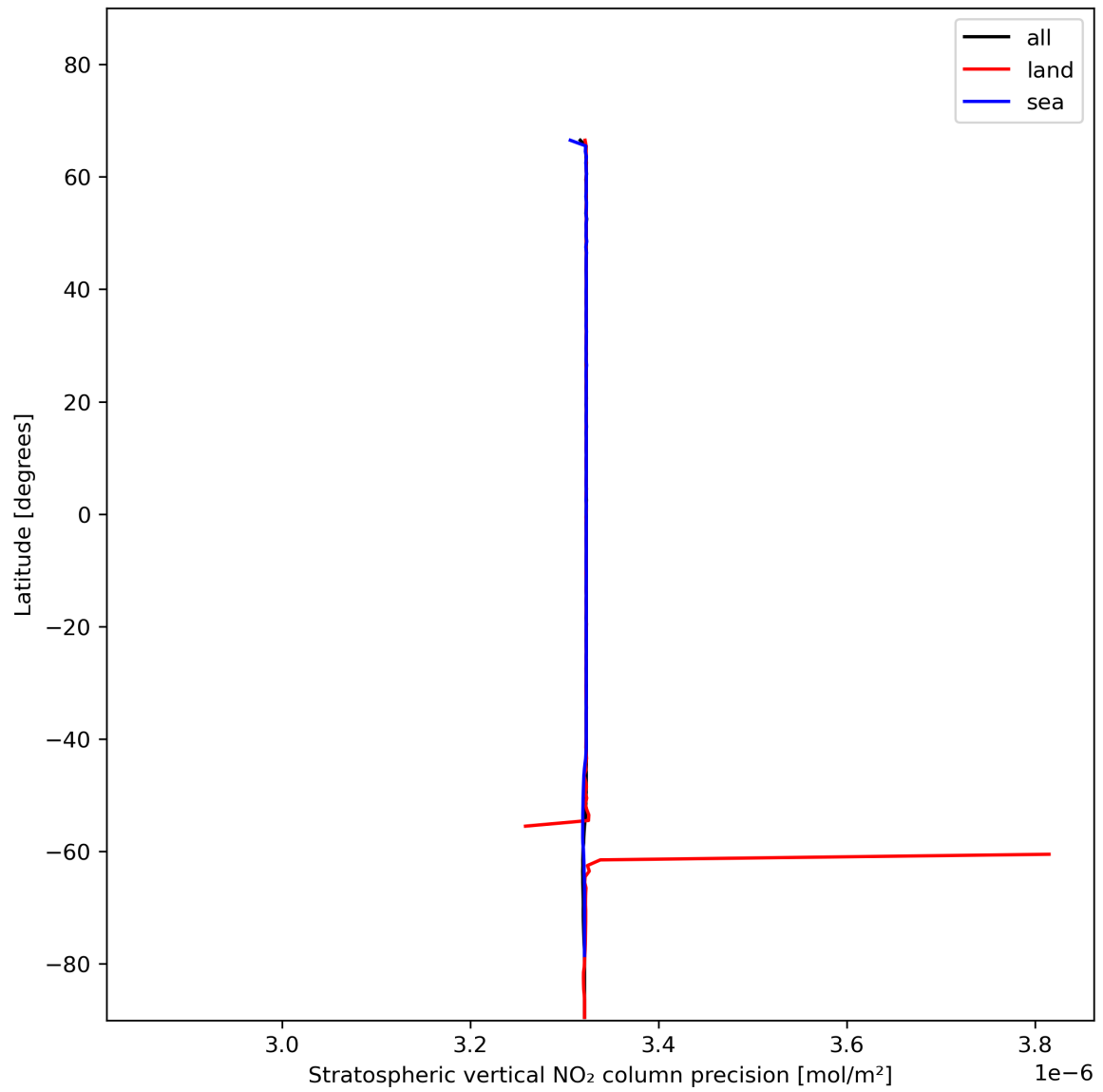
Figure 20: Zonal average of “Stratospheric vertical NO 2 column precision” for 2024-01-12 to 2024-01-14.
