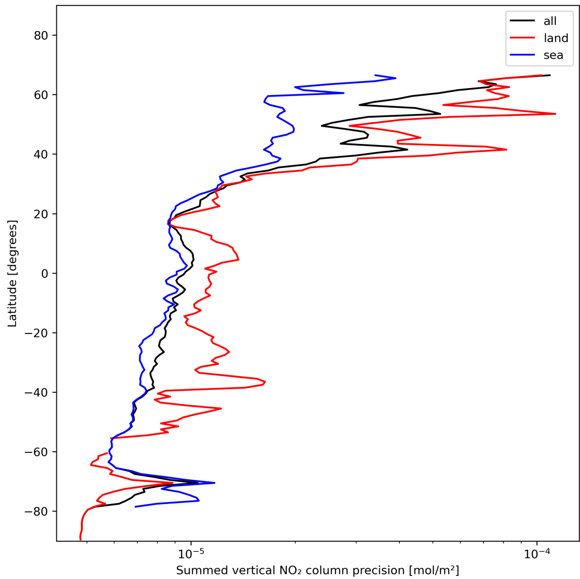
Figure 24: Zonal average of “Summed vertical NO 2 column precision” for 2024-01-12 to 2024-01-14.
