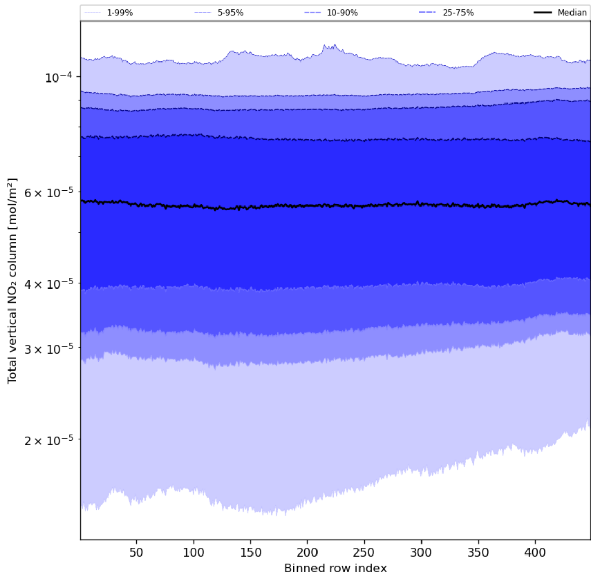
Figure 55: Along track statistics of “Total vertical NO 2 column” for 2024-01-12 to 2024-01-14
