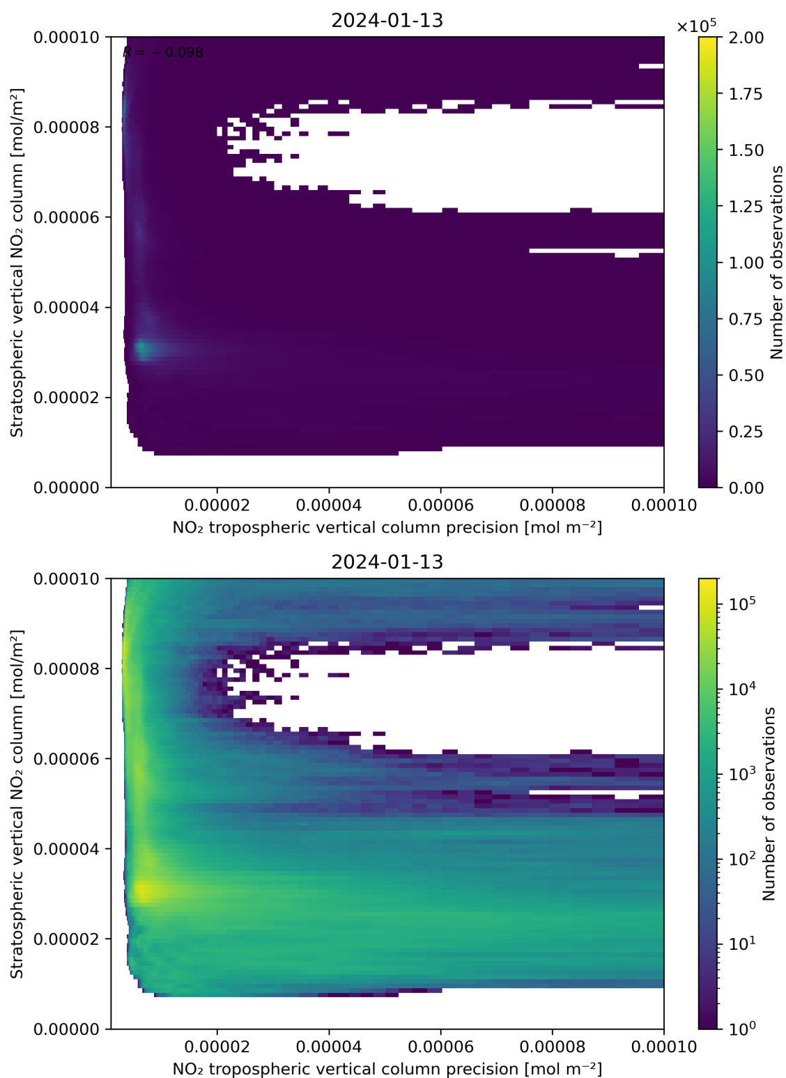
Figure 135: Scatter density plot of “NO 2 tropospheric vertical column precision” against “Stratospheric vertical NO 2 column” for 2024-01-12 to 2024-01-14.
