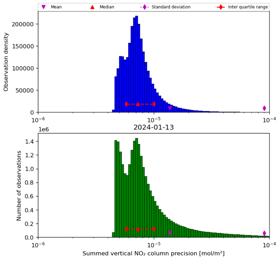
Figure 41: Histogram of “Summed vertical NO 2 column precision” for 2024-01-12 to 2024-01-14
