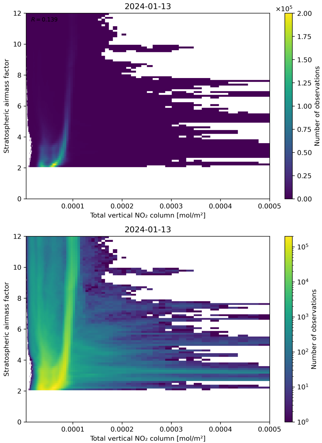
Figure 110: Scatter density plot of “Total vertical NO 2 column” against “Stratospheric airmass factor” for 2024-01-12 to 2024-01-14.
