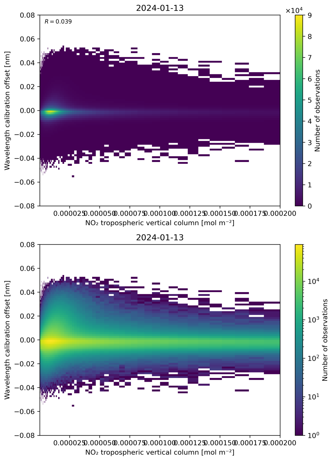
Figure 143: Scatter density plot of “NO 2 tropospheric vertical column” against “Wavelength calibration offset” for 2024-01-12 to 2024-01-14.
