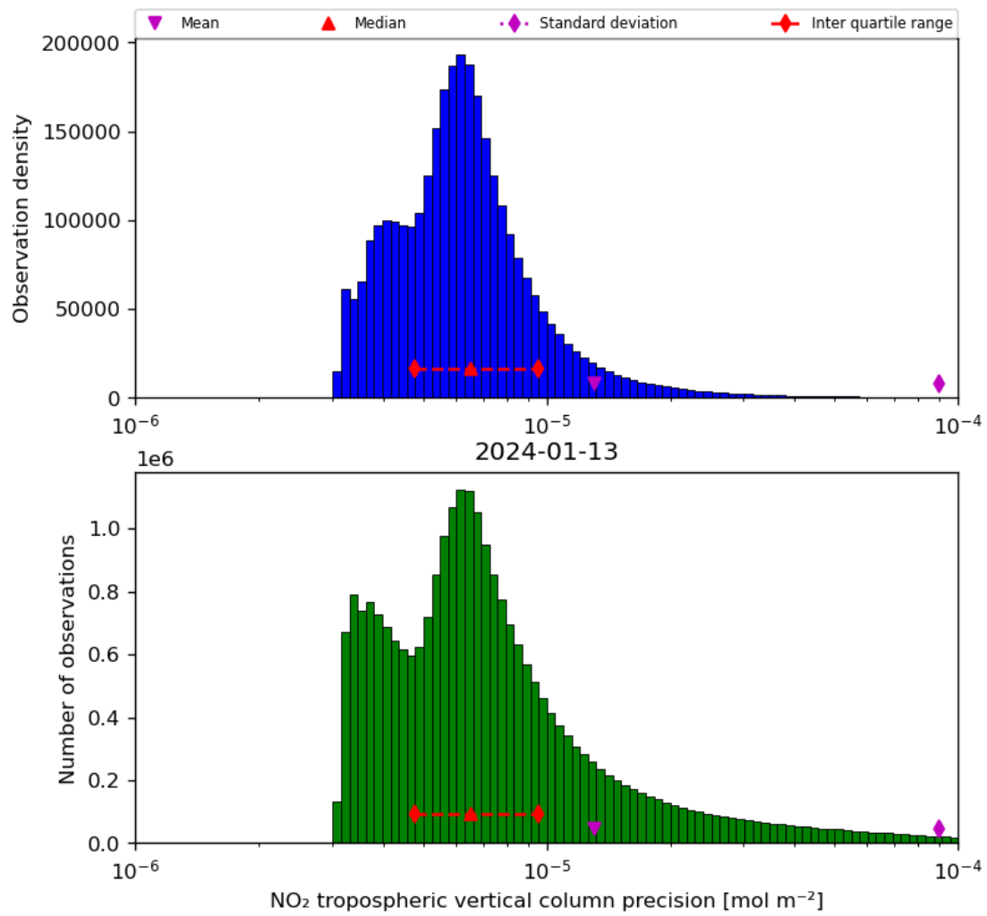
Figure 30: Histogram of “NO 2 tropospheric vertical column precision” for 2024-01-12 to 2024-01-14
