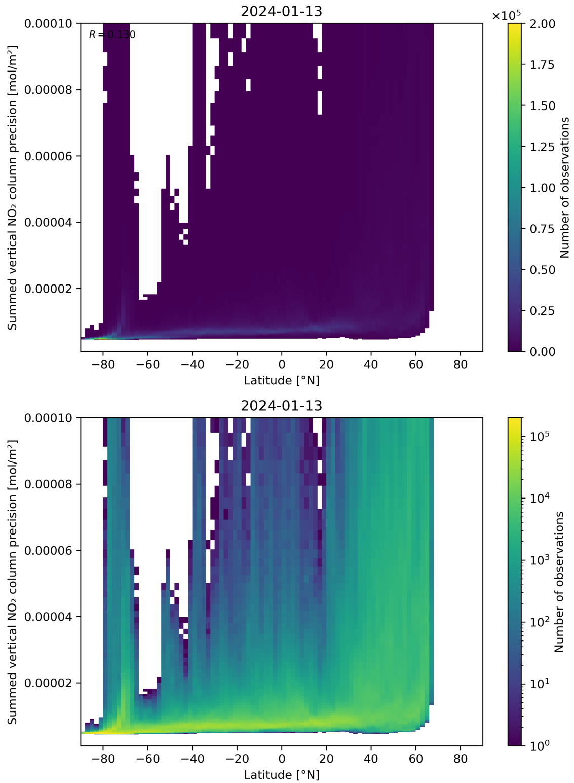
Figure 89: Scatter density plot of “Latitude” against “Summed vertical NO 2 column precision” for 2024-01-12 to 2024-01-14.
