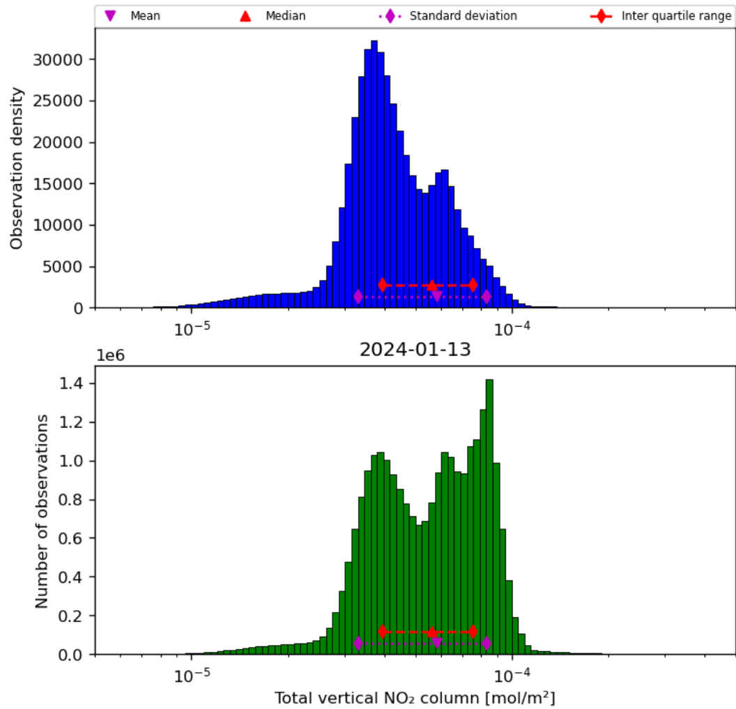
Figure 38: Histogram of “Total vertical NO 2 column” for 2024-01-12 to 2024-01-14
