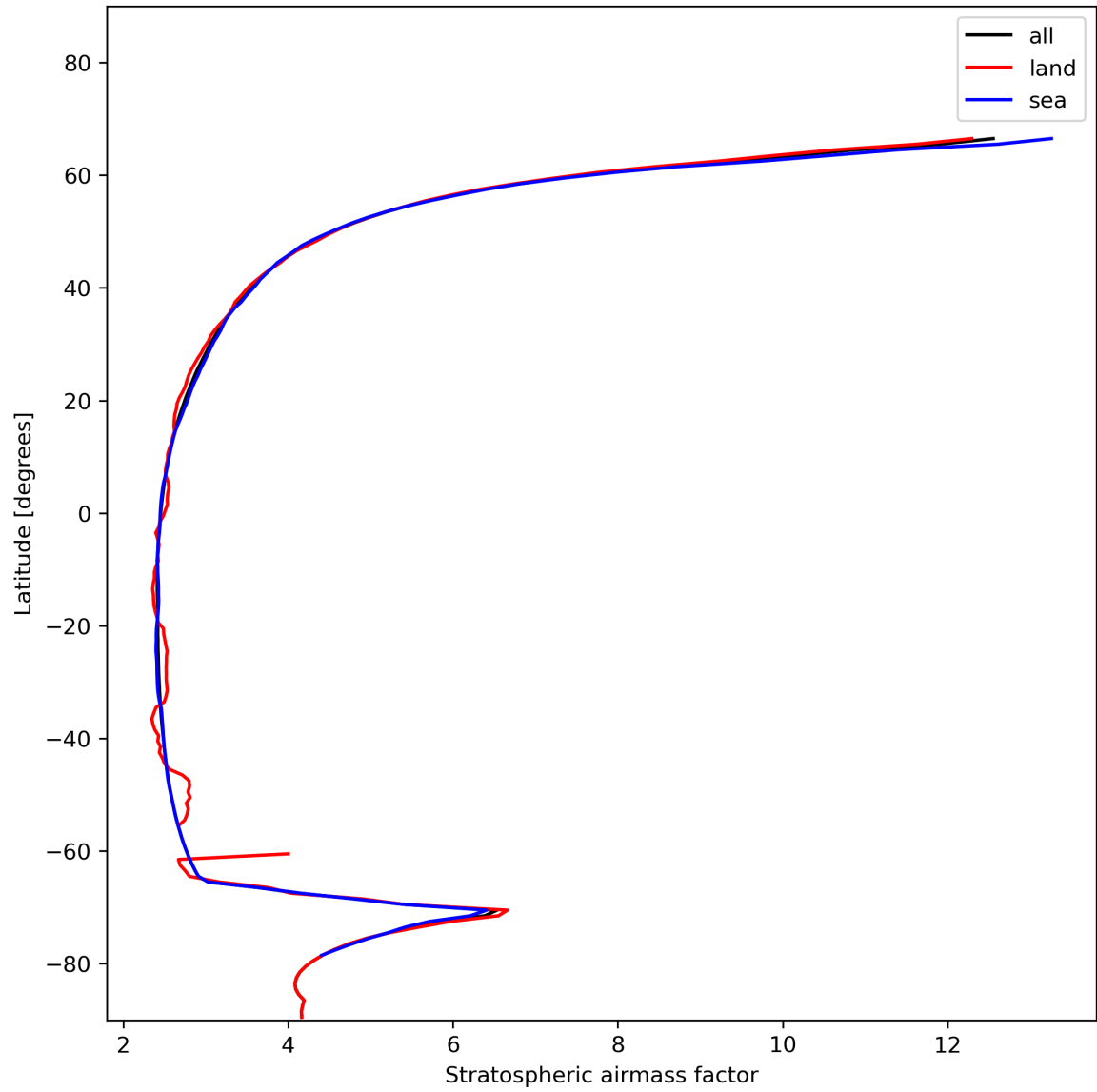
Figure 27: Zonal average of “Stratospheric airmass factor” for 2024-01-12 to 2024-01-14.
