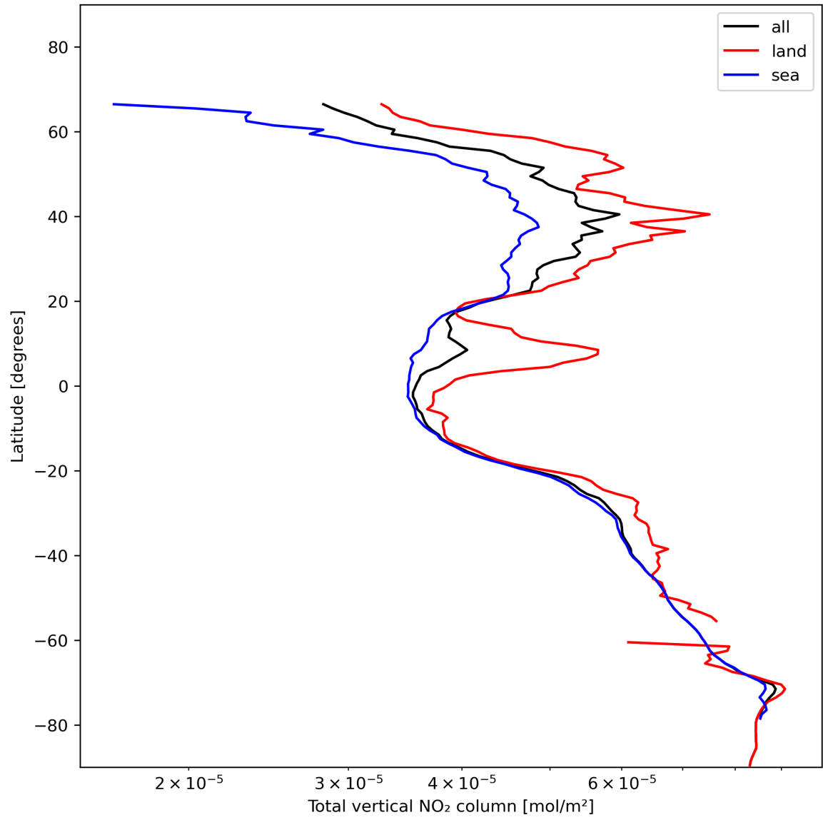
Figure 21: Zonal average of “Total vertical NO 2 column” for 2024-01-12 to 2024-01-14.
