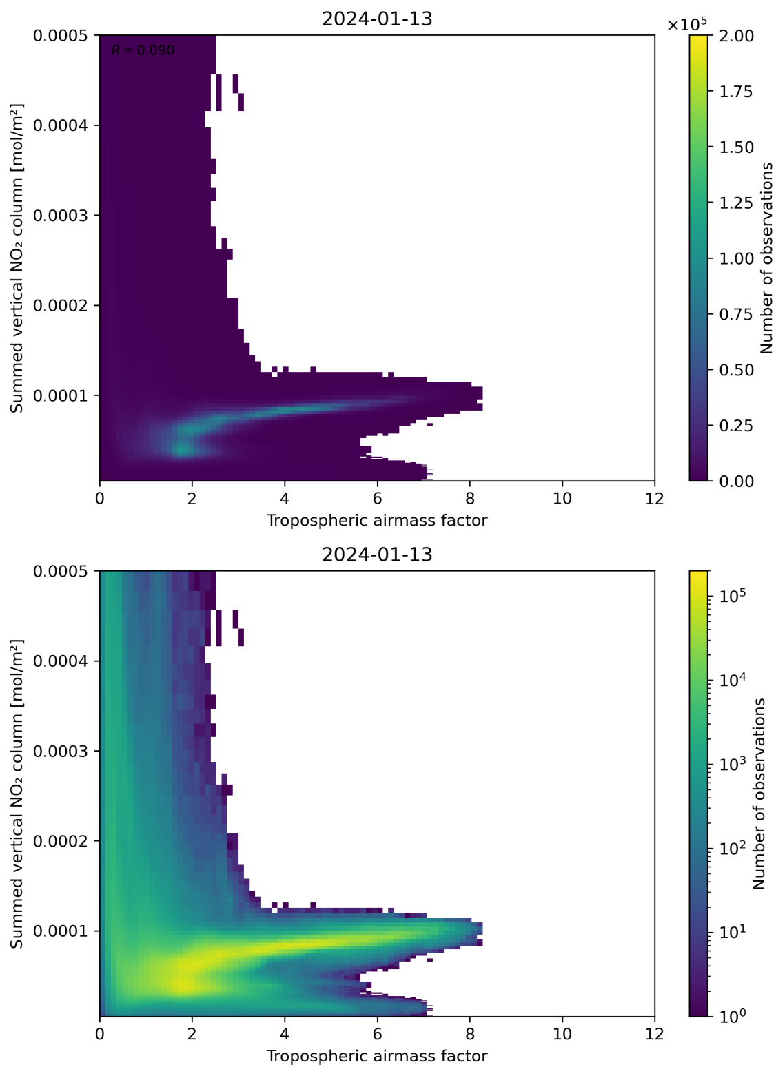
Figure 75: Scatter density plot of “Tropospheric airmass factor” against “Summed vertical NO 2 column” for 2024-01-12 to 2024-01-14.
