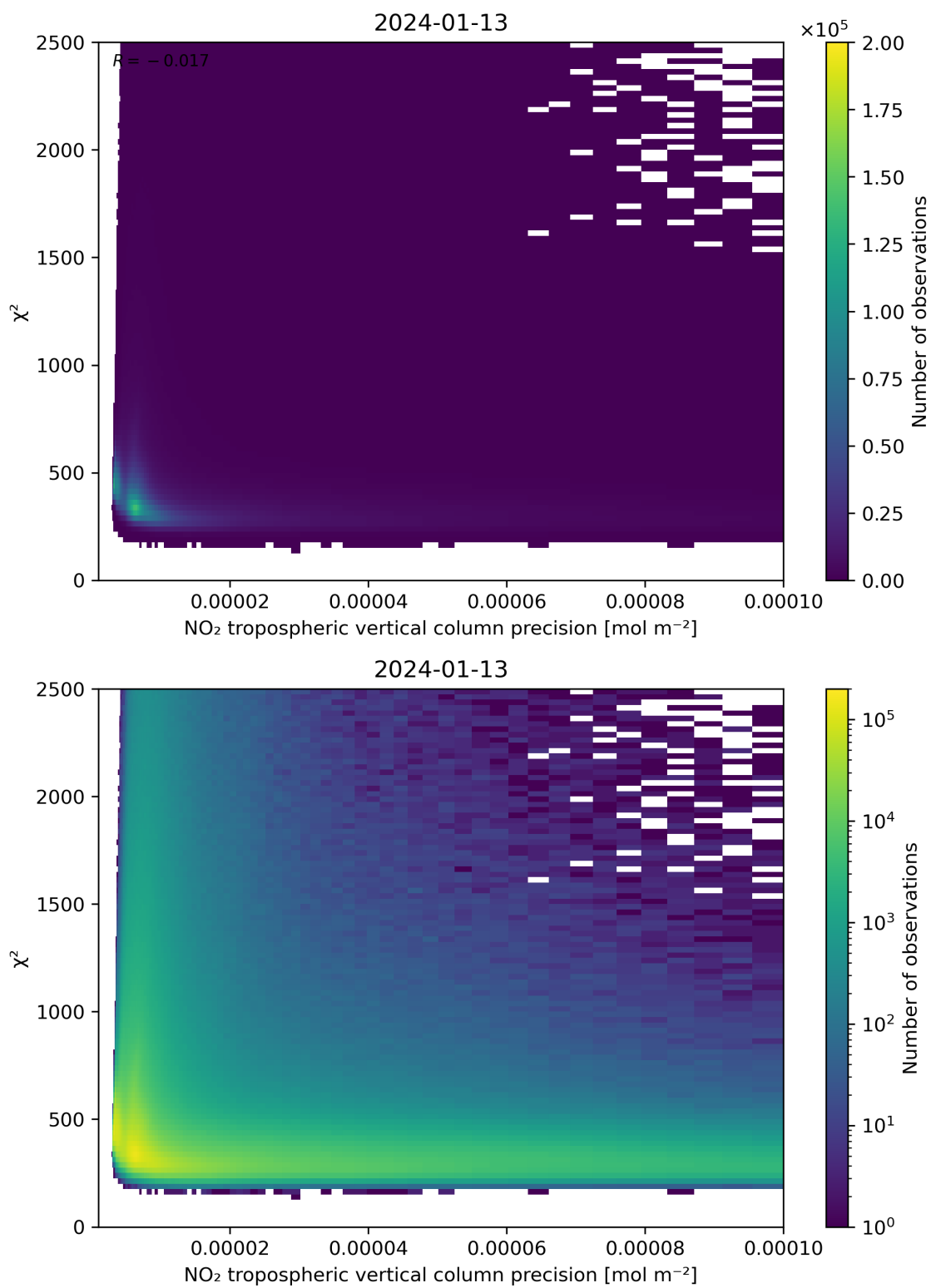
Figure 134: Scatter density plot of “NO 2 tropospheric vertical column precision” against “ \chi^2 ” for 2024-01-12 to 2024-01-14.
