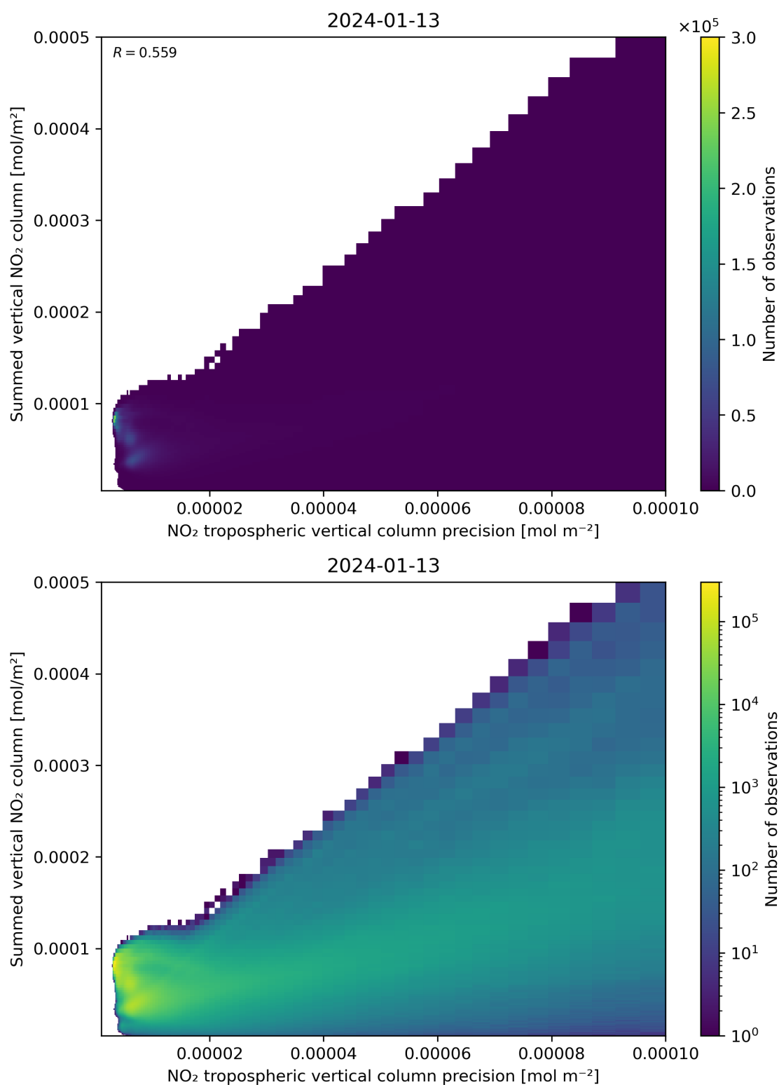
Figure 136: Scatter density plot of “NO 2 tropospheric vertical column precision” against “Summed vertical NO 2 column” for 2024-01-12 to 2024-01-14.
