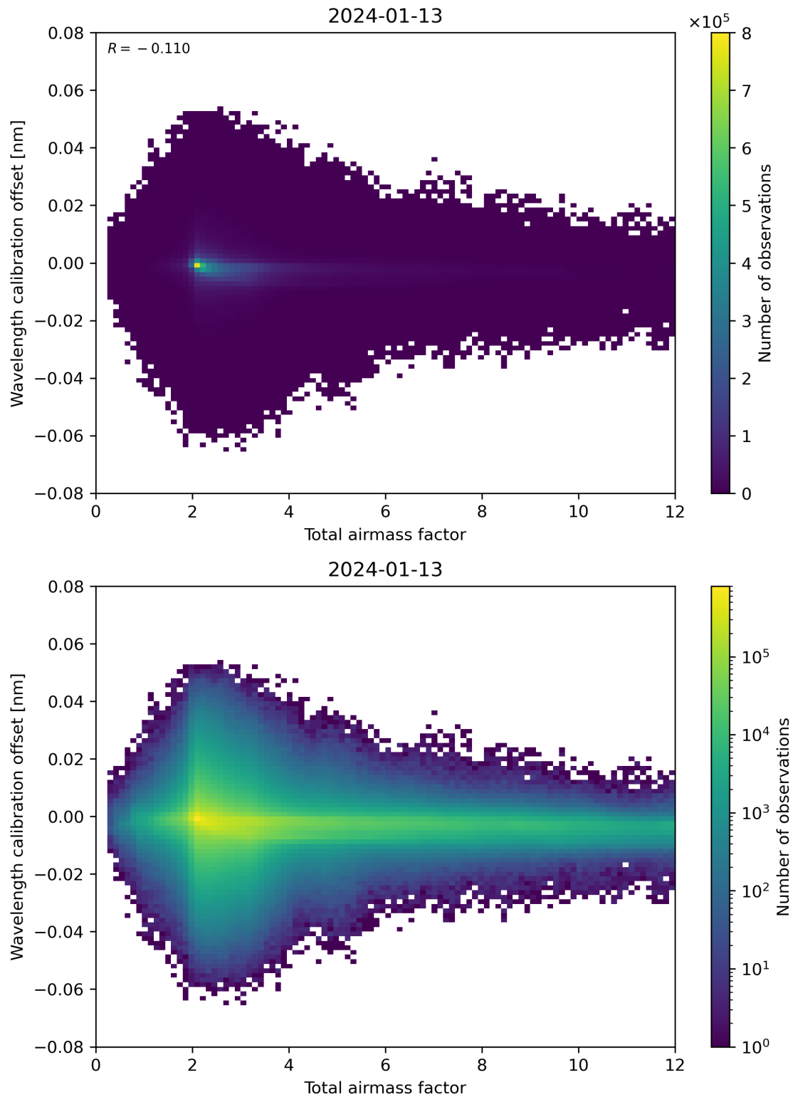
Figure 70: Scatter density plot of “Total airmass factor” against “Wavelength calibration offset” for 2024-01-12 to 2024-01-14.
