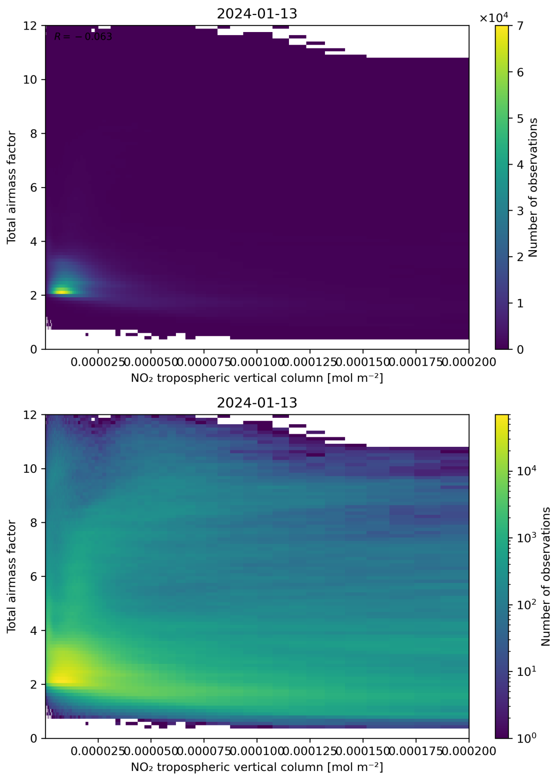
Figure 122: Scatter density plot of “NO 2 tropospheric vertical column” against “Total air mass factor” for 2024-01-12 to 2024-01-14.
