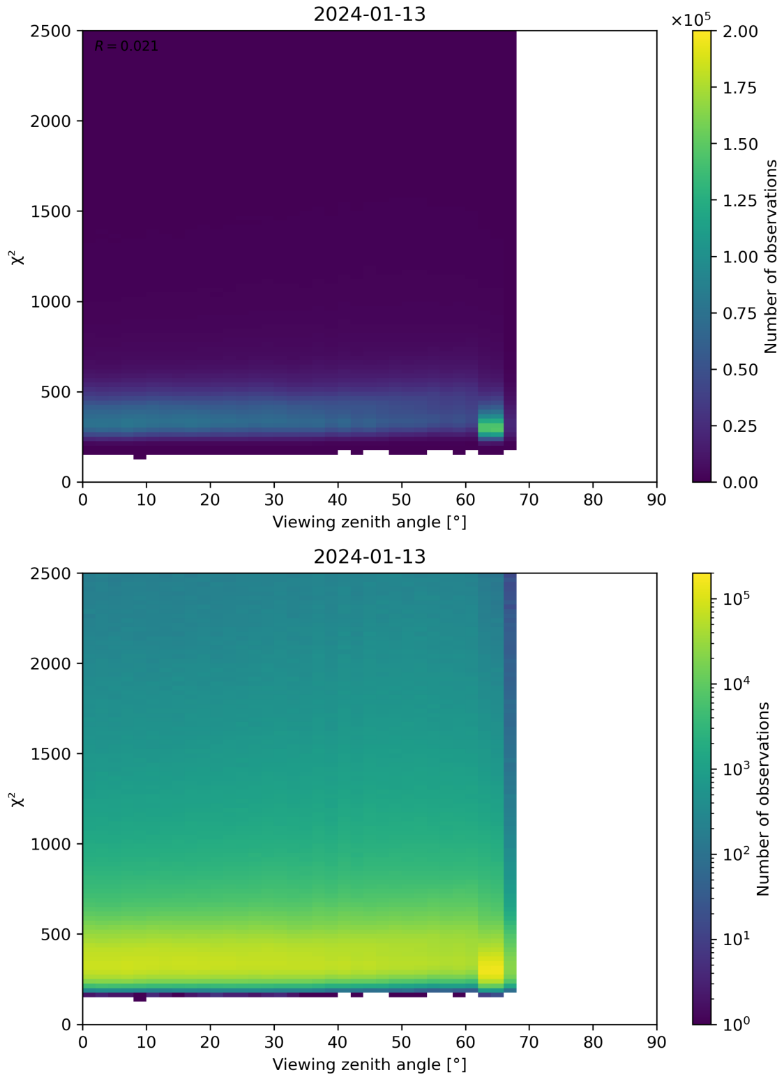
Figure 162: Scatter density plot of “Viewing zenith angle” against “ \chi^2 ” for 2024-01-12 to 2024-01-14.
