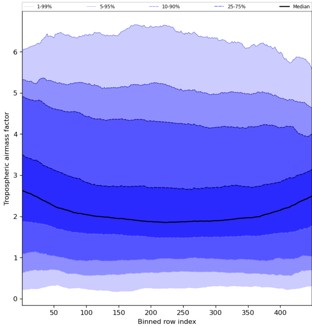
Figure 48: Along track statistics of “Tropospheric air mass factor” for 2024-01-12 to 2024-01-14
