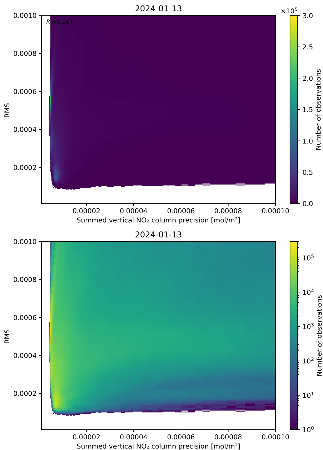
Figure 108: Scatter density plot of “Summed vertical NO 2 column precision” against “RMS” for 2024-01-12 to 2024-01-14.
