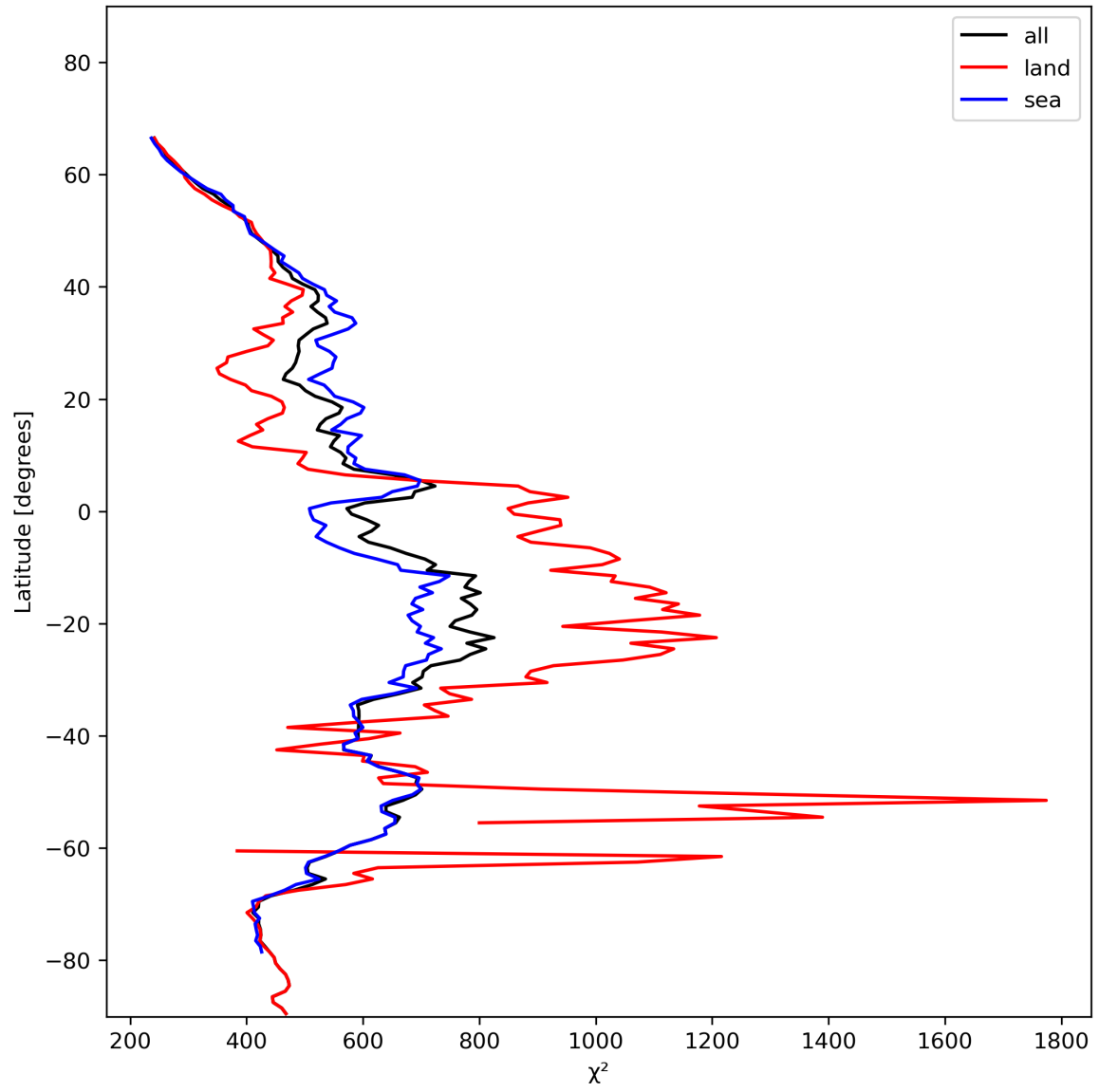
Figure 25: Zonal average of “ \chi^2 ” for 2024-01-12 to 2024-01-14.
