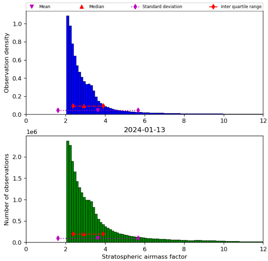
Figure 44: Histogram of “Stratospheric airmass factor” for 2024-01-12 to 2024-01-14
