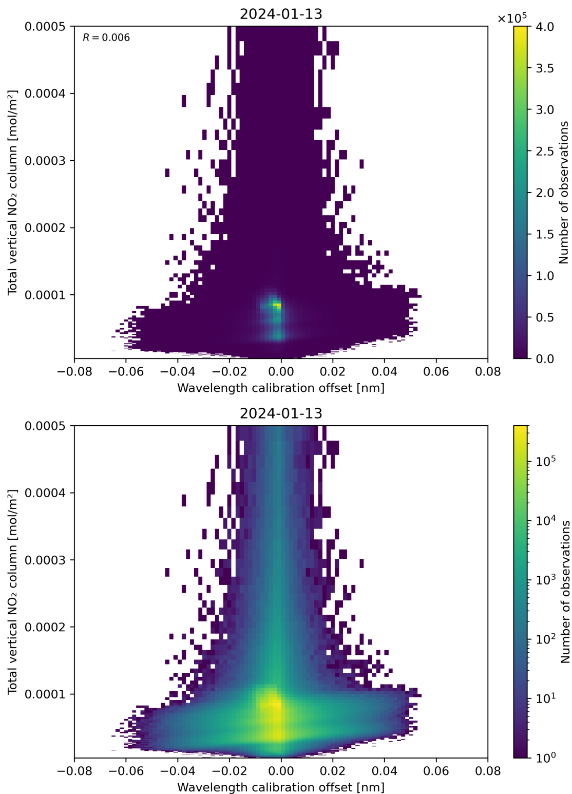
Figure 179: Scatter density plot of “Wavelength calibration offset” against “Total vertical NO 2 column” for 2024-01-12 to 2024-01-14.
