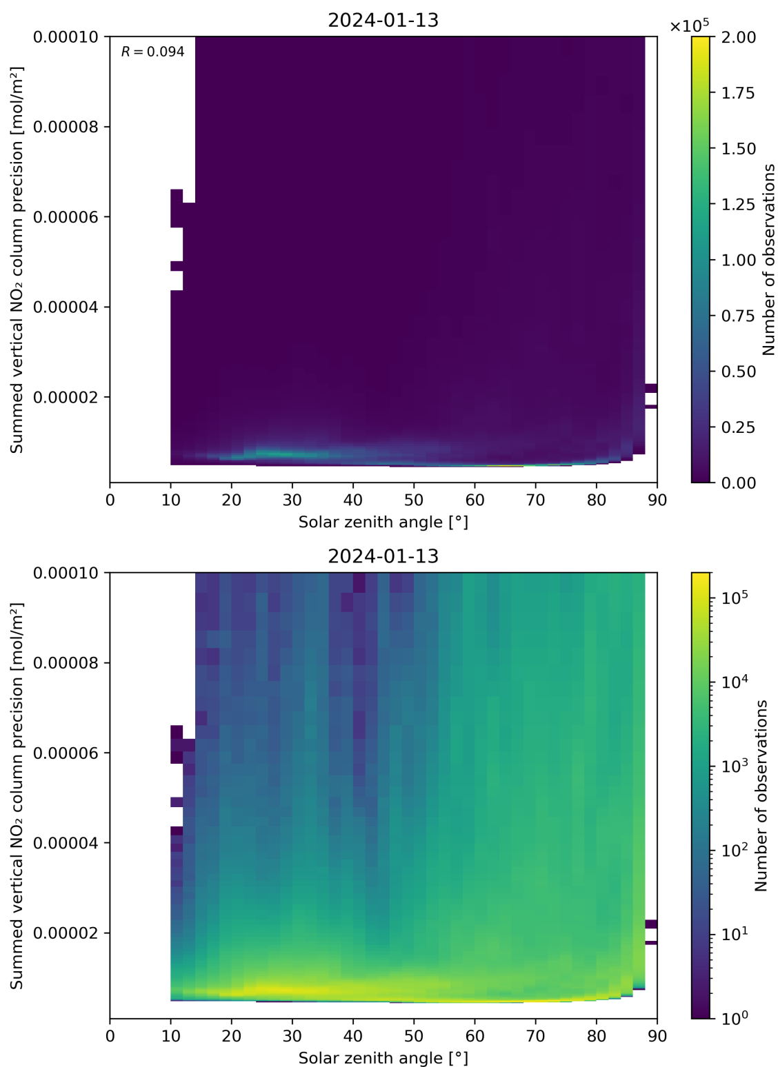
Figure 152: Scatter density plot of “Solar zenith angle” against “Summed vertical NO 2 column precision” for 2024-01-12 to 2024-01-14.
