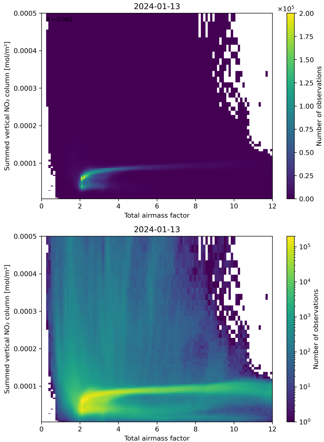
Figure 65: Scatter density plot of “Total airmass factor” against “Summed vertical NO 2 column” for 2024-01-12 to 2024-01-14.
