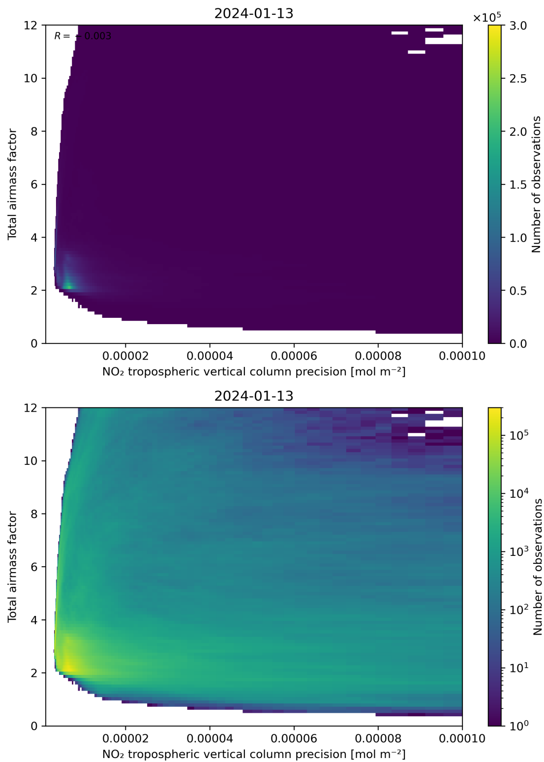
Figure 132: Scatter density plot of “NO 2 tropospheric vertical column precision” against “Total air mass factor” for 2024-01-12 to 2024-01-14.
