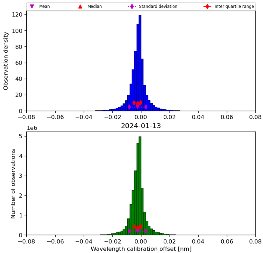
Figure 35: Histogram of “Wavelength calibration offset” for 2024-01-12 to 2024-01-14
