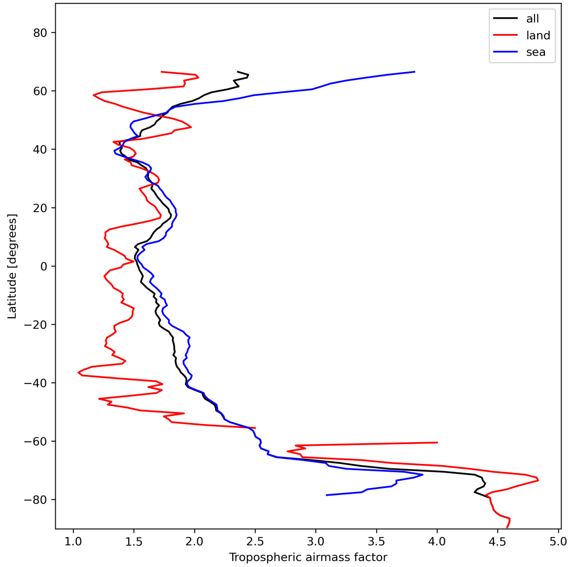
Figure 14: Zonal average of “Tropospheric airmass factor” for 2024-01-12 to 2024-01-14.
