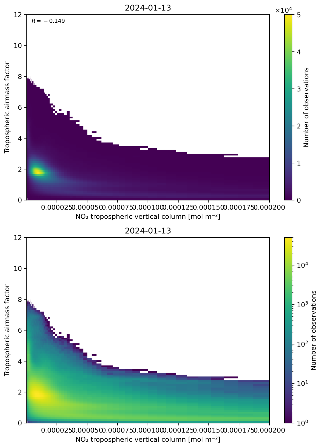
Figure 123: Scatter density plot of “NO 2 tropospheric vertical column” against “Tropospheric air mass factor” for 2024-01-12 to 2024-01-14.
