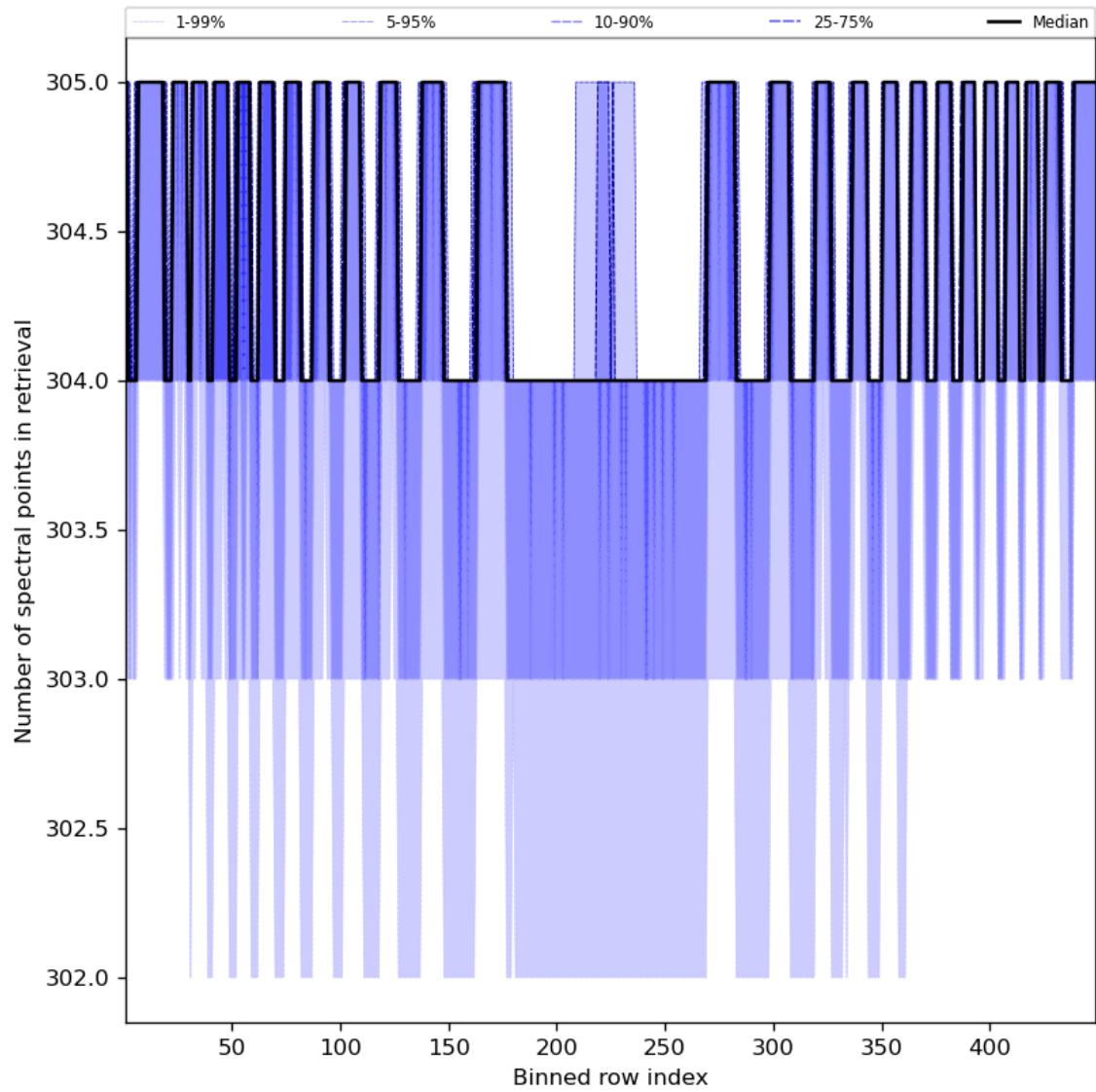
Figure 50: Along track statistics of “Number of spectral points in retrieval” for 2024-01-12 to 2024-01-14
