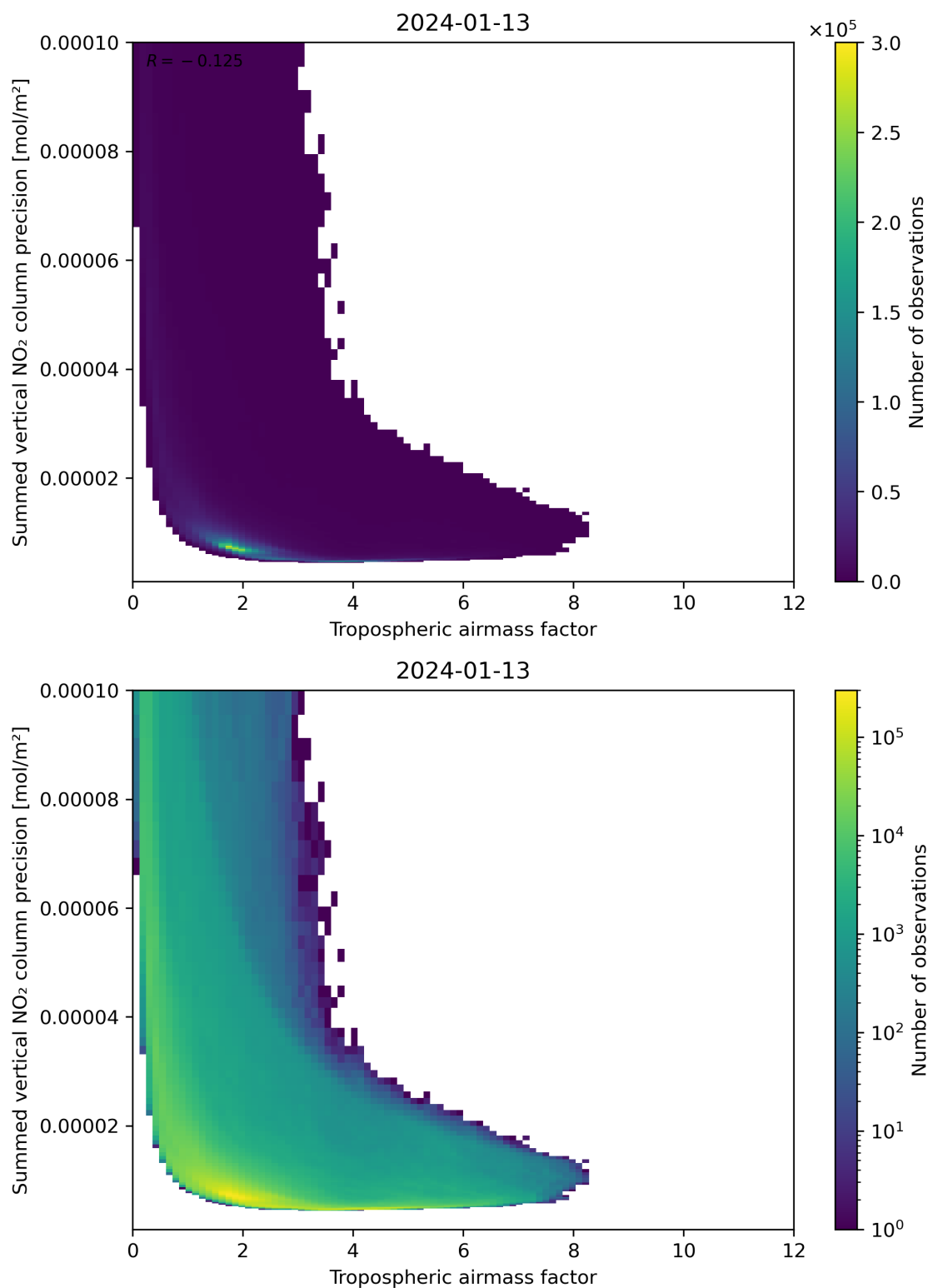
Figure 76: Scatter density plot of “Tropospheric air mass factor” against “Summed vertical NO 2 column precision” for 2024-01-12 to 2024-01-14.
