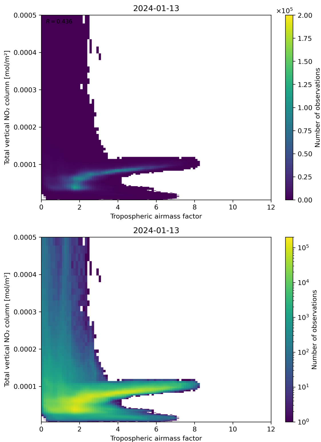
Figure 77: Scatter density plot of “Tropospheric airmass factor” against “Total vertical NO 2 column” for 2024-01-12 to 2024-01-14.
