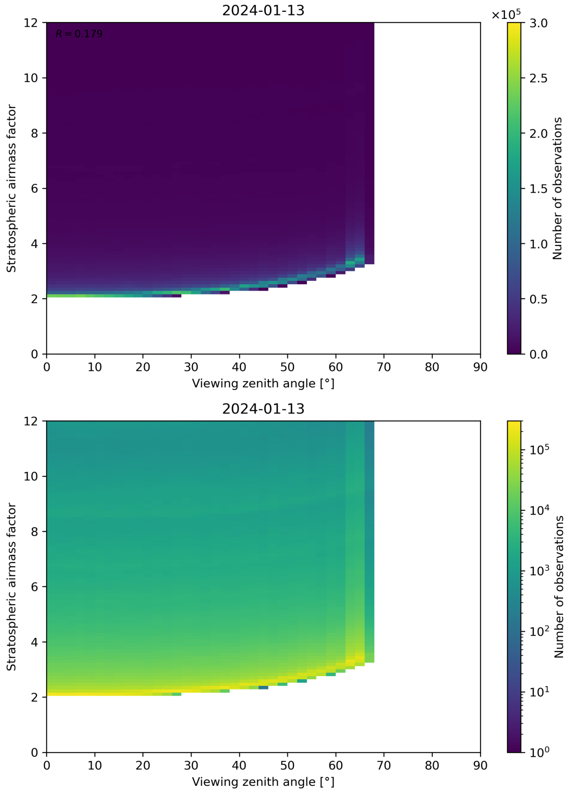
Figure 159: Scatter density plot of “Viewing zenith angle” against “Stratospheric airmass factor” for 2024-01-12 to 2024-01-14.
