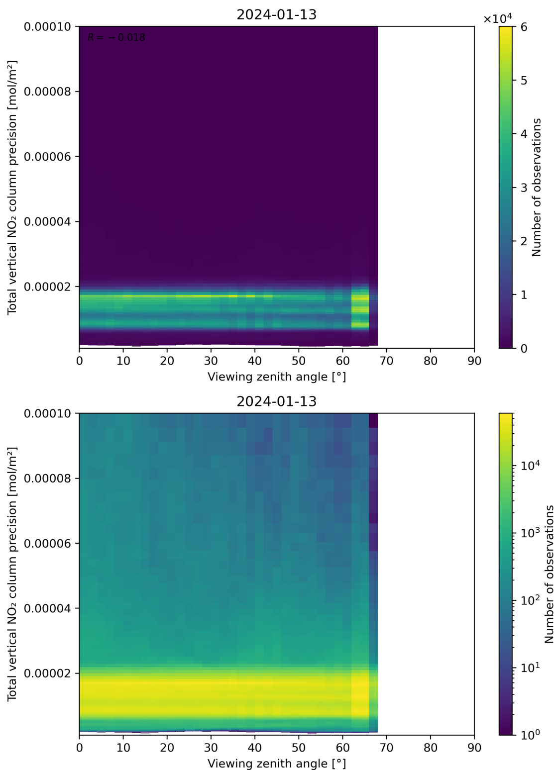
Figure 168: Scatter density plot of “Viewing zenith angle” against “Total vertical NO 2 column precision” for 2024-01-12 to 2024-01-14.
