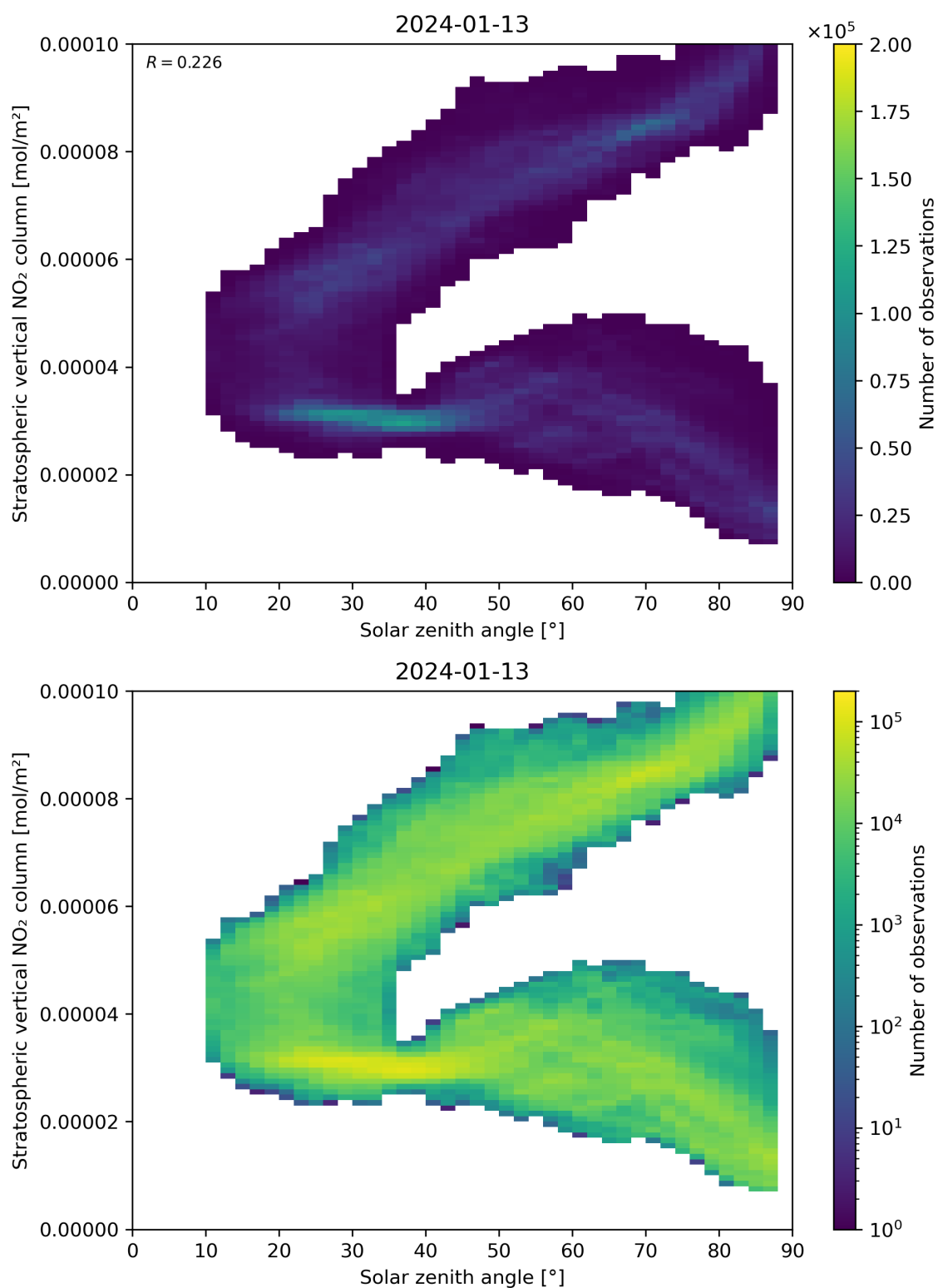
Figure 150: Scatter density plot of “Solar zenith angle” against “Stratospheric vertical NO 2 column” for 2024-01-12 to 2024-01-14.
