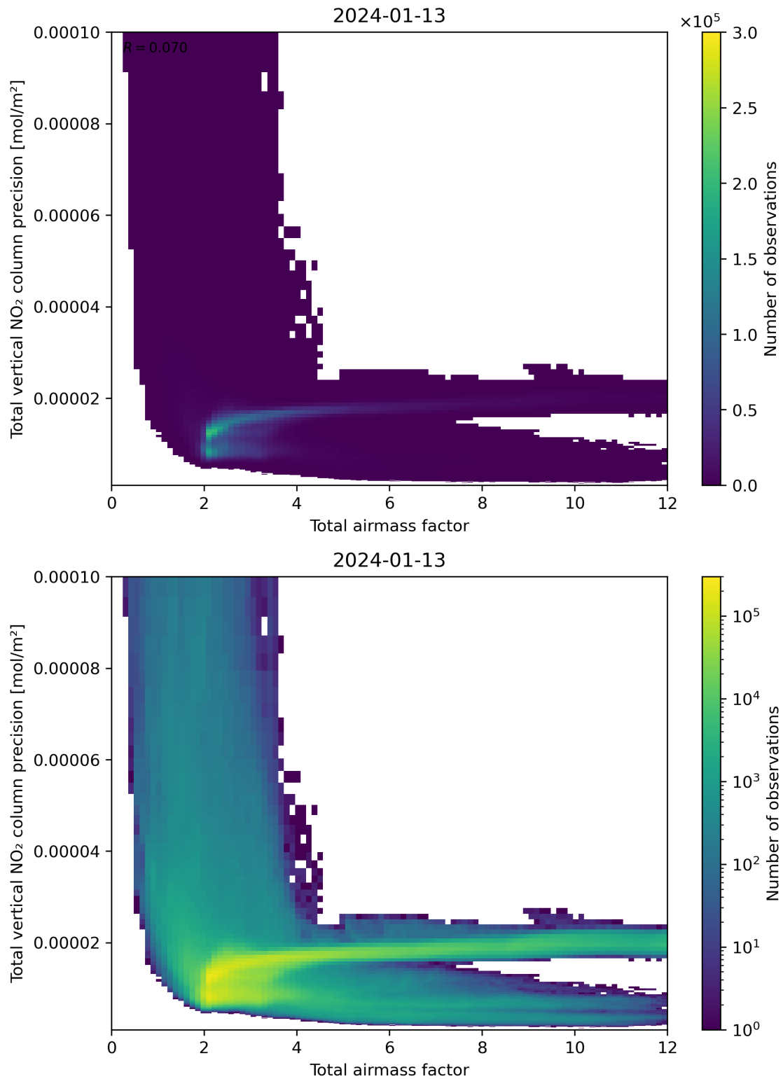
Figure 68: Scatter density plot of “Total airmass factor” against “Total vertical NO 2 column precision” for 2024-01-12 to 2024-01-14.
