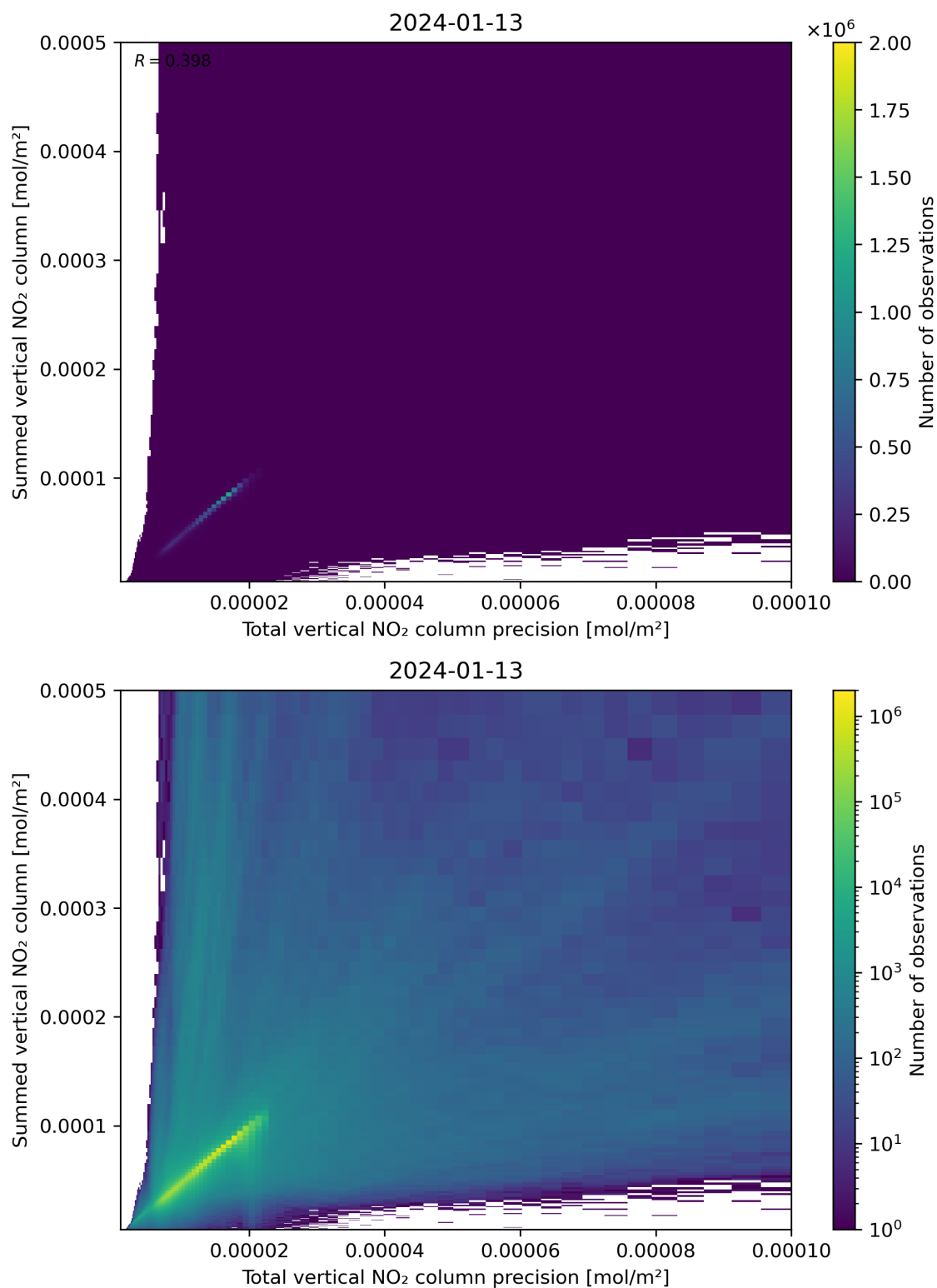
Figure 117: Scatter density plot of “Total vertical NO 2 column precision” against “Summed vertical NO 2 column” for 2024-01-12 to 2024-01-14.
