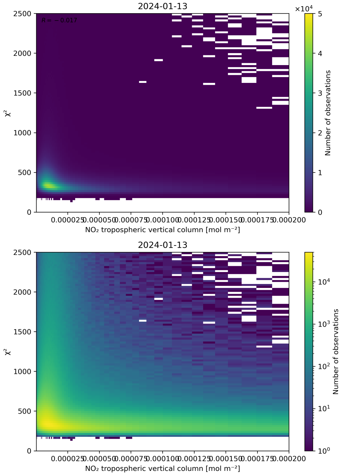
Figure 124: Scatter density plot of “NO 2 tropospheric vertical column” against “ \chi^2 ” for 2024-01-12 to 2024-01-14.
