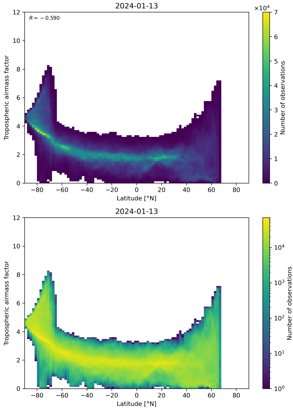
Figure 85: Scatter density plot of “Latitude” against “Tropospheric airmass factor” for 2024-01-12 to 2024-01-14.
