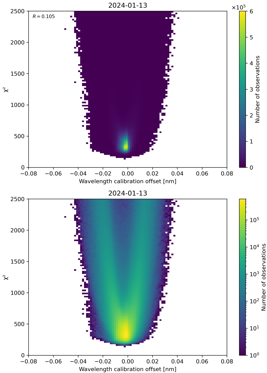
Figure 175: Scatter density plot of “Wavelength calibration offset” against “ \chi^2 ” for 2024-01-12 to 2024-01-14.
