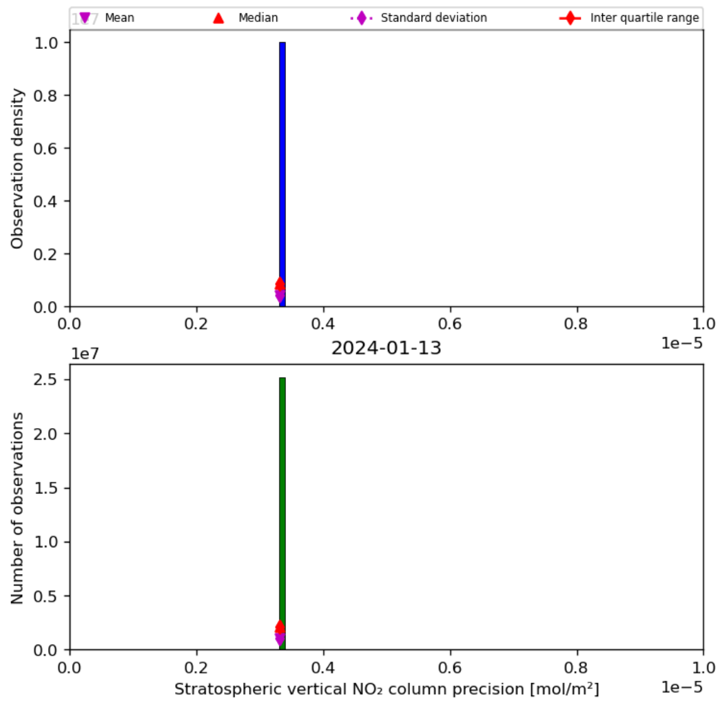
Figure 37: Histogram of “Stratospheric vertical NO 2 column precision” for 2024-01-12 to 2024-01-14
