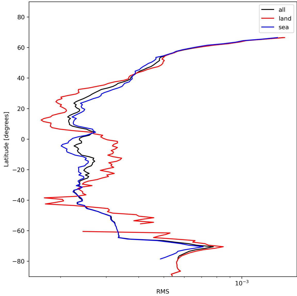
Figure 26: Zonal average of “RMS” for 2024-01-12 to 2024-01-14.
