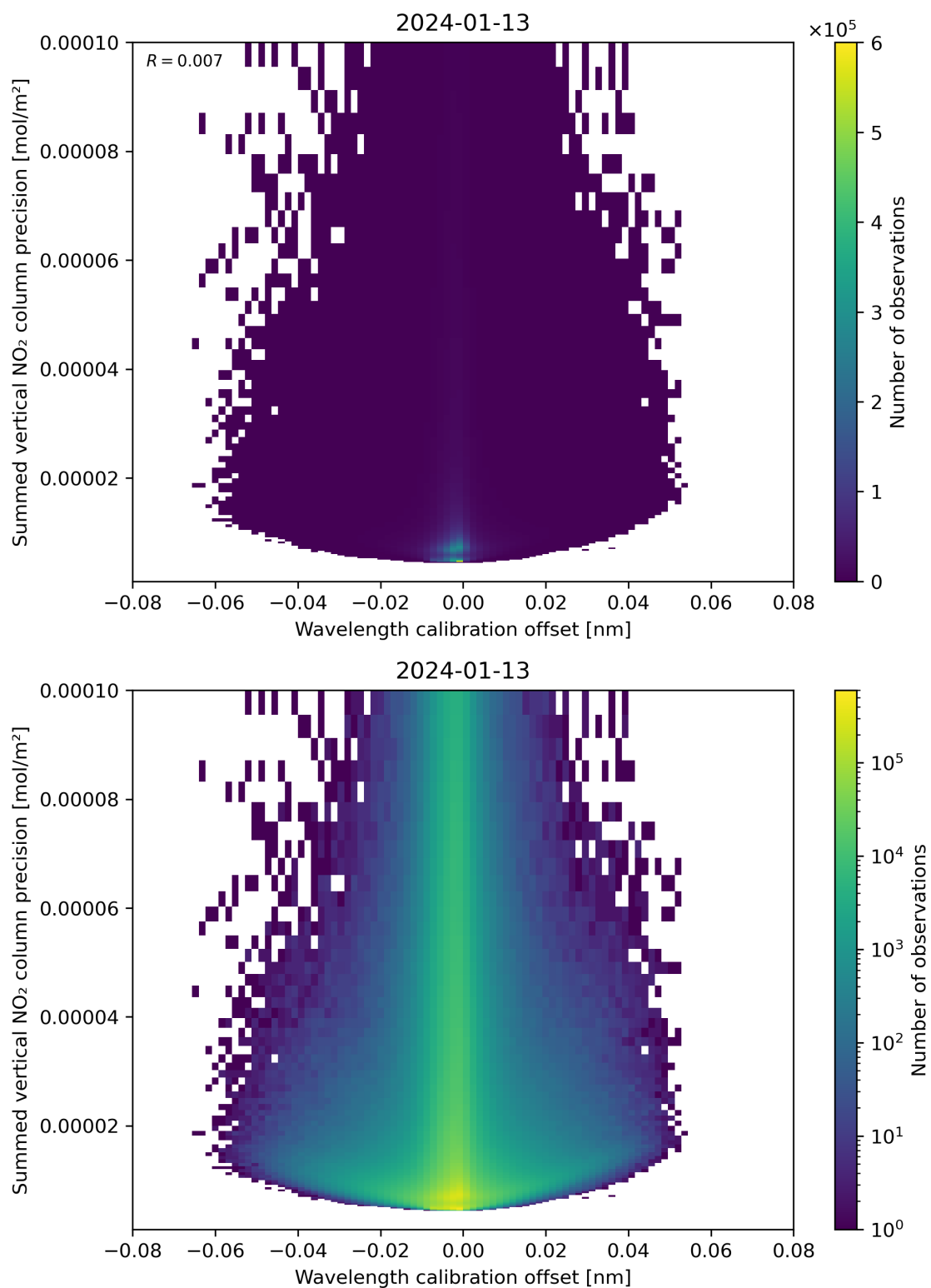
Figure 178: Scatter density plot of “Wavelength calibration offset” against “Summed vertical NO 2 column precision” for 2024-01-12 to 2024-01-14.
