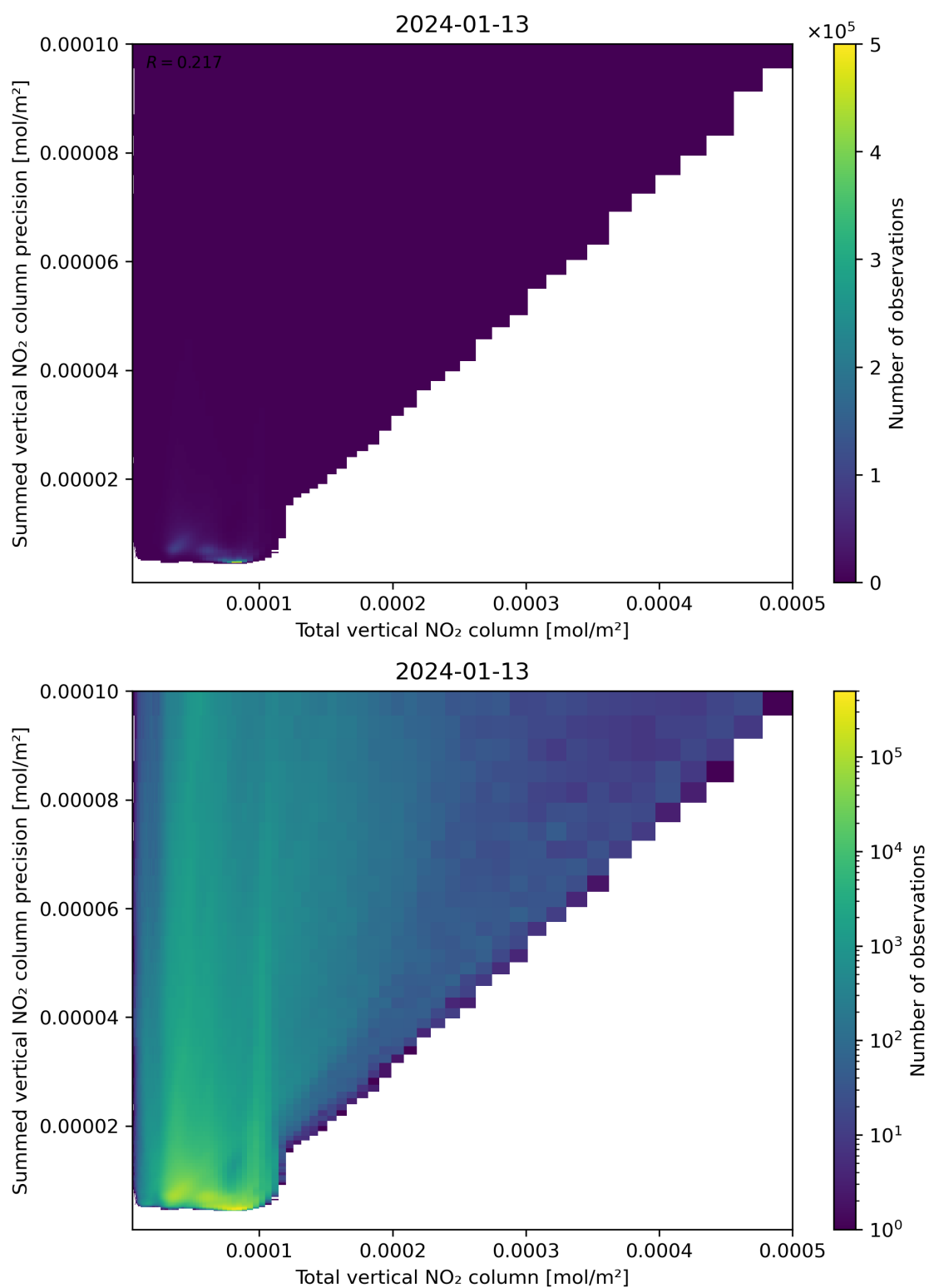
Figure 113: Scatter density plot of “Total vertical NO 2 column” against “Summed vertical NO 2 column precision” for 2024-01-12 to 2024-01-14.
