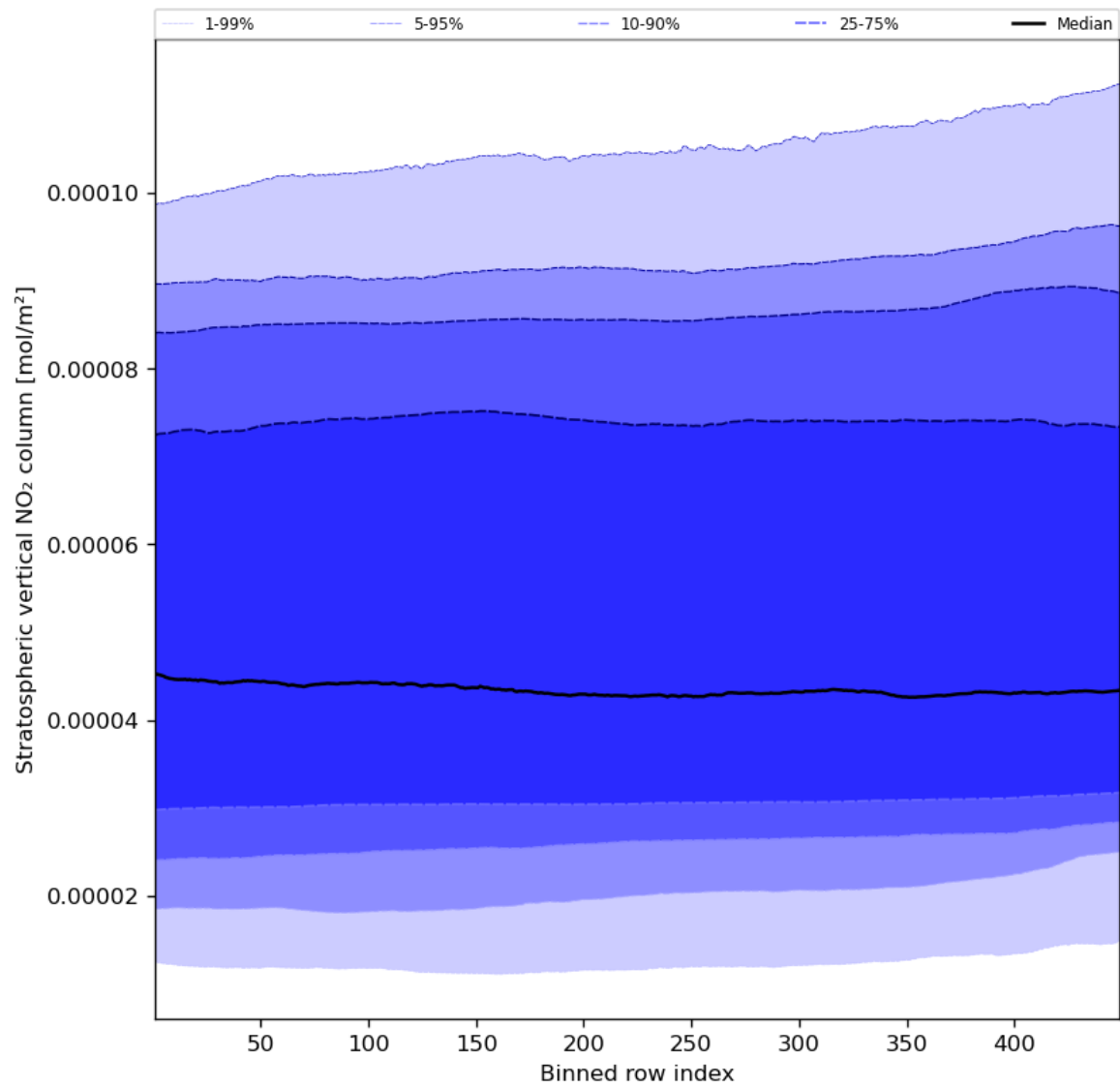
Figure 53: Along track statistics of “Stratospheric vertical NO 2 column” for 2024-01-12 to 2024-01-14
