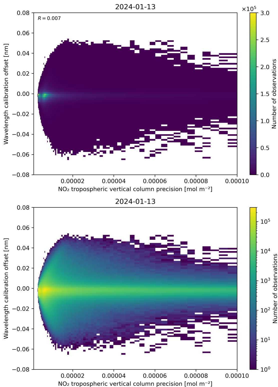
Figure 141: Scatter density plot of “NO 2 tropospheric vertical column precision” against “Wavelength calibration offset” for 2024-01-12 to 2024-01-14.
