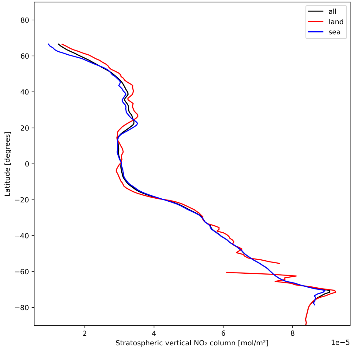
Figure 19: Zonal average of “Stratospheric vertical NO 2 column” for 2024-01-12 to 2024-01-14.
