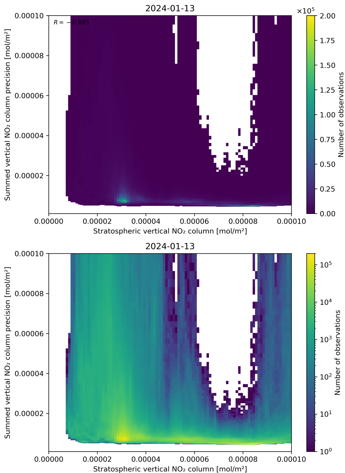
Figure 99: Scatter density plot of “Stratospheric vertical NO 2 column” against “Summed vertical NO 2 column precision” for 2024-01-12 to 2024-01-14.
