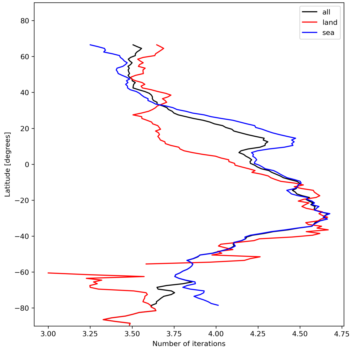
Figure 17: Zonal average of “Number of iterations” for 2024-01-12 to 2024-01-14.
