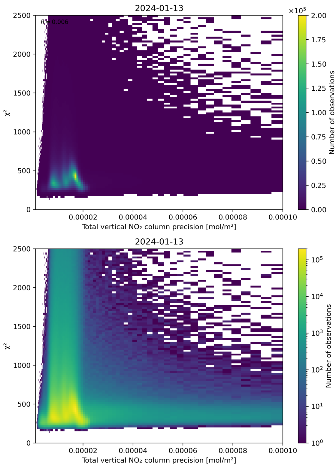
Figure 116: Scatter density plot of “Total vertical NO 2 column precision” against “ \chi^2 ” for 2024-01-12 to 2024-01-14.
