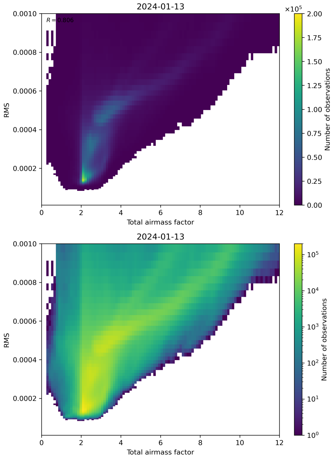
Figure 69: Scatter density plot of “Total airmass factor” against “RMS” for 2024-01-12 to 2024-01-14.
