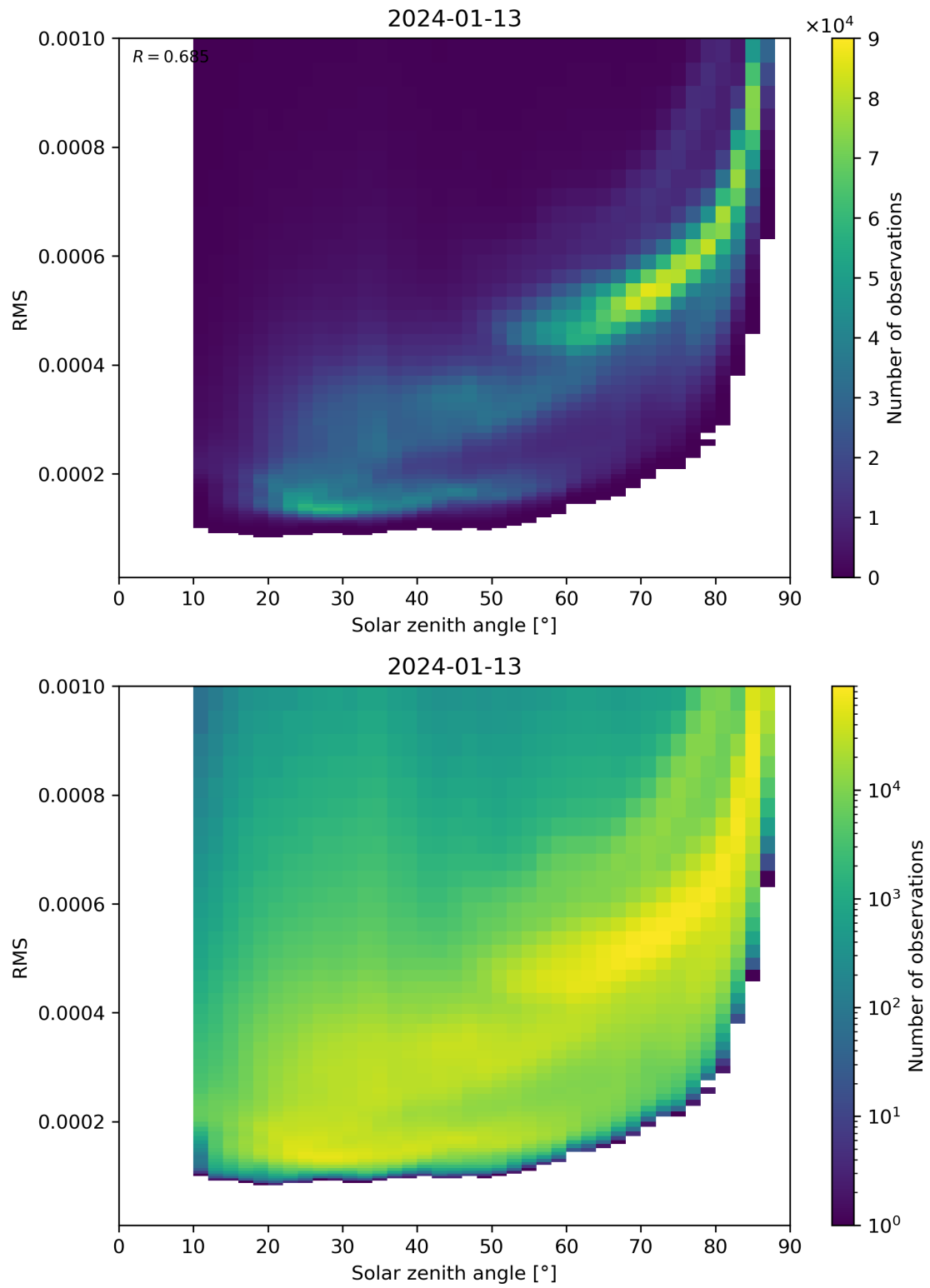
Figure 157: Scatter density plot of “Solar zenith angle” against “RMS” for 2024-01-12 to 2024-01-14.
