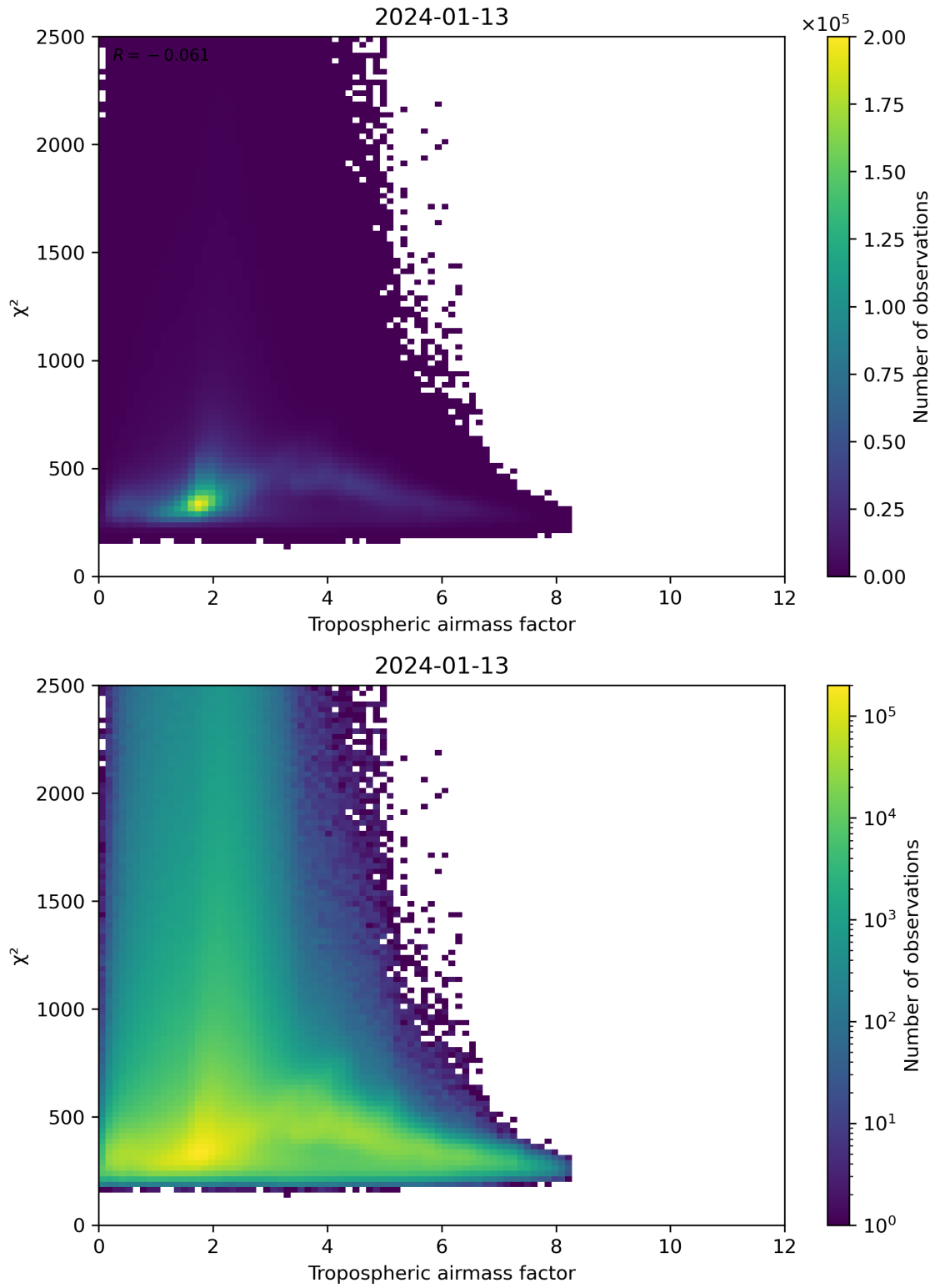
Figure 73: Scatter density plot of “Tropospheric airmass factor” against “ \chi^2 ” for 2024-01-12 to 2024-01-14.
