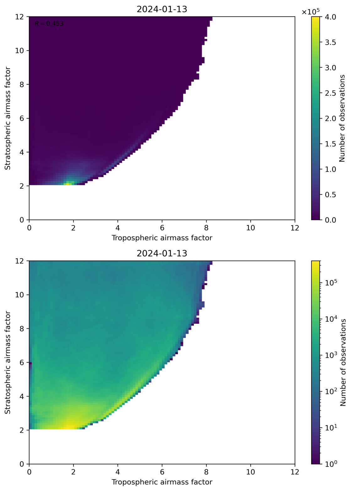
Figure 71: Scatter density plot of “Tropospheric airmass factor” against “Stratospheric airmass factor” for 2024-01-12 to 2024-01-14.
