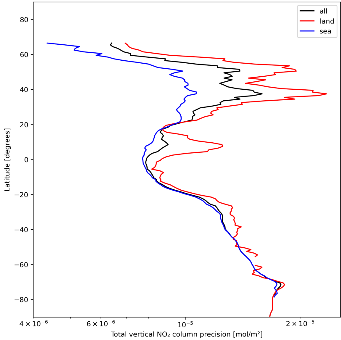
Figure 22: Zonal average of “Total vertical NO 2 column precision” for 2024-01-12 to 2024-01-14.
