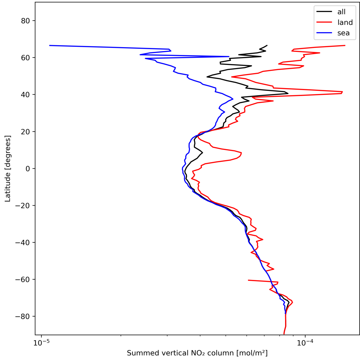
Figure 23: Zonal average of “Summed vertical NO 2 column” for 2024-01-12 to 2024-01-14.
