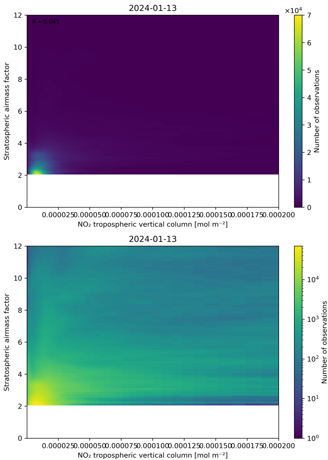
Figure 121: Scatter density plot of “NO 2 tropospheric vertical column” against “Stratospheric air mass factor” for 2024-01-12 to 2024-01-14.
