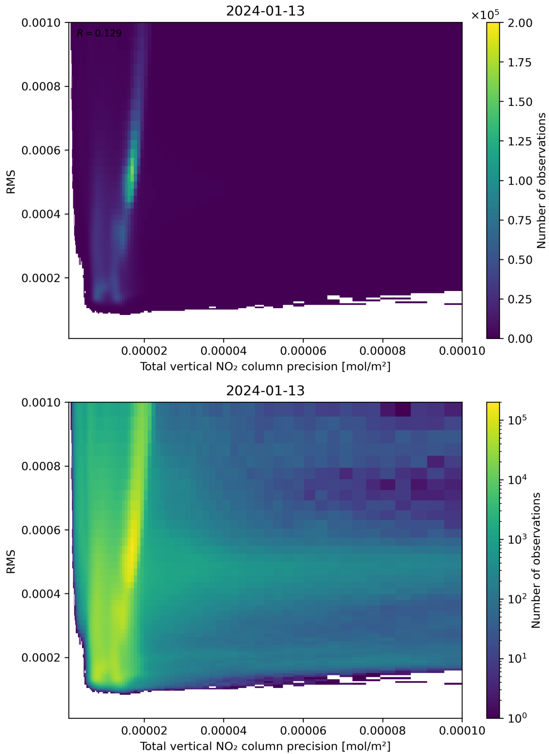
Figure 119: Scatter density plot of “Total vertical NO 2 column precision” against “RMS” for 2024-01-12 to 2024-01-14.
