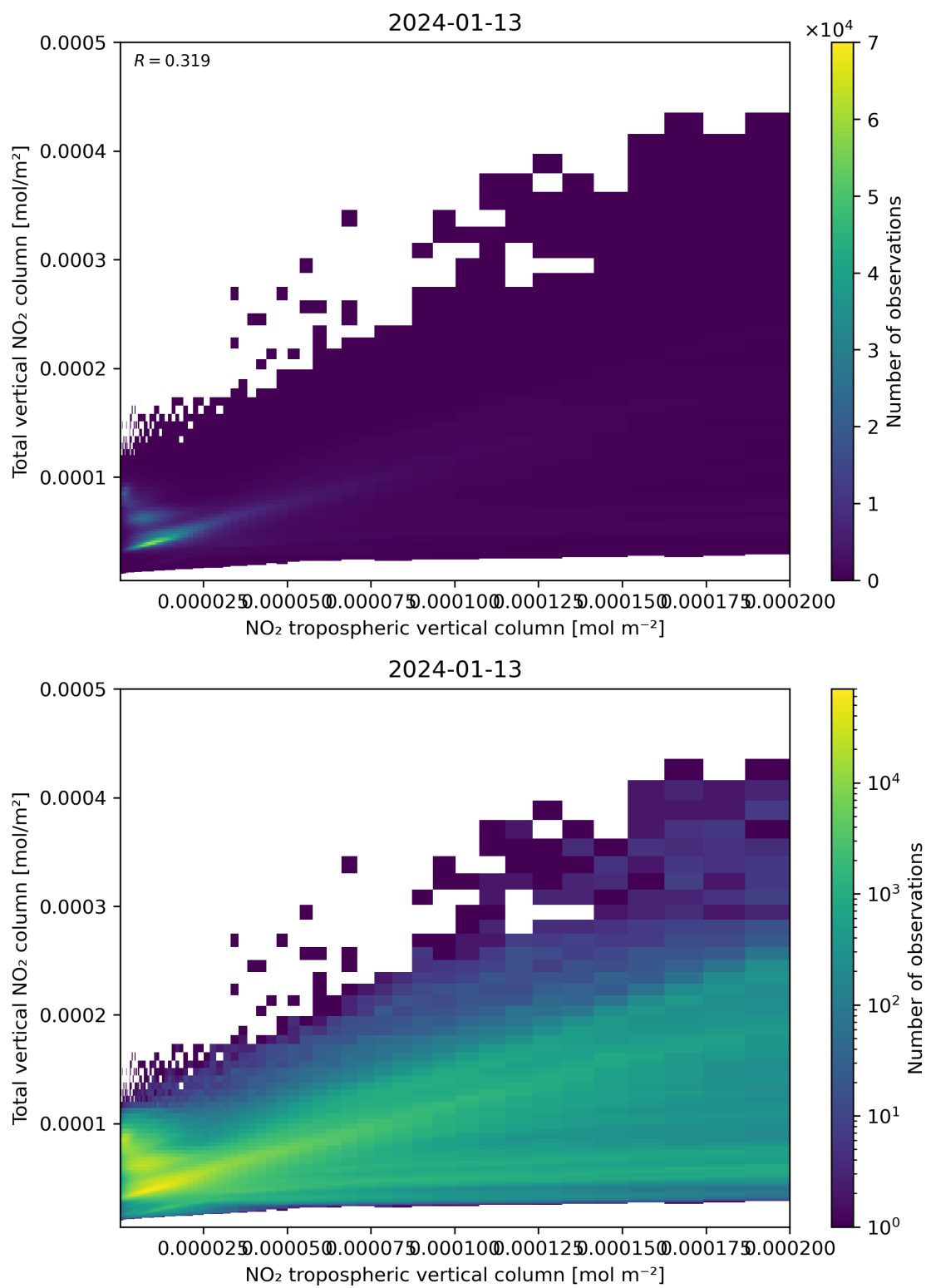
Figure 128: Scatter density plot of “NO 2 tropospheric vertical column” against “Total vertical NO 2 column” for 2024-01-12 to 2024-01-14.
