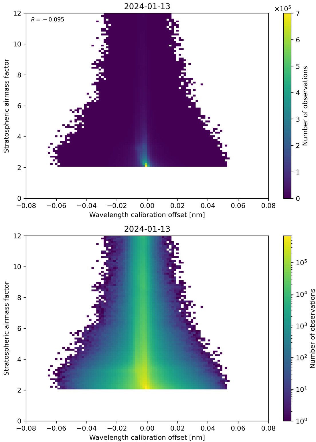
Figure 174: Scatter density plot of “Wavelength calibration offset” against “Stratospheric airmass factor” for 2024-01-12 to 2024-01-14.
