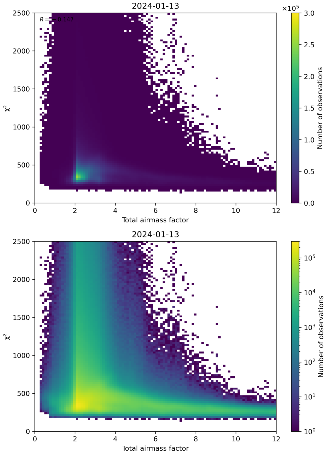
Figure 63: Scatter density plot of “Total airmass factor” against “ \chi^2 ” for 2024-01-12 to 2024-01-14.
