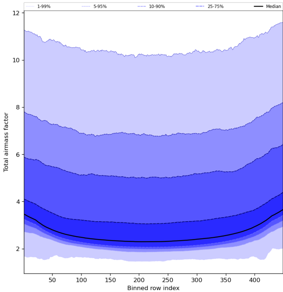
Figure 49: Along track statistics of “Total airmass factor” for 2024-01-12 to 2024-01-14
