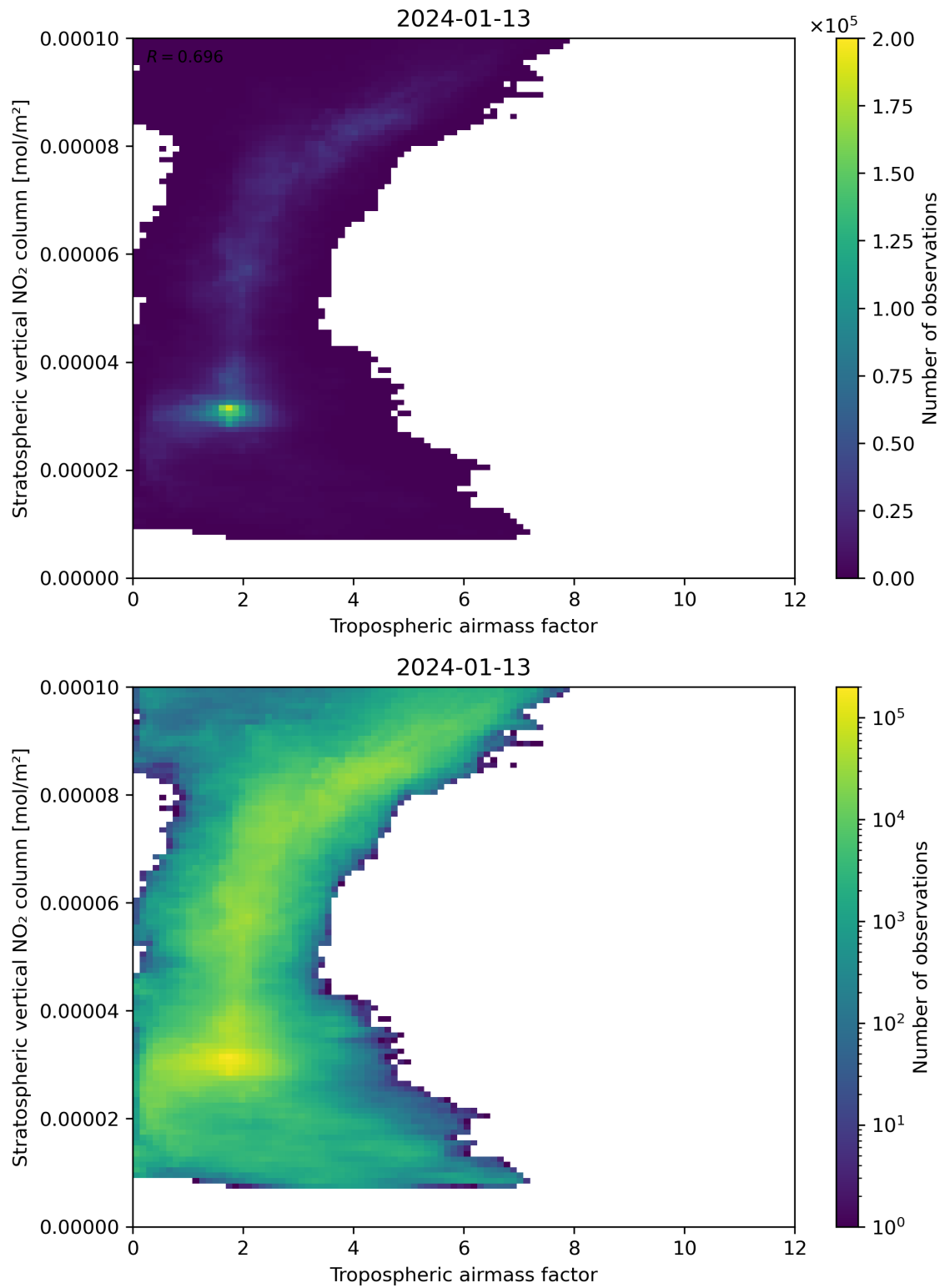
Figure 74: Scatter density plot of “Tropospheric air mass factor” against “Stratospheric vertical NO 2 column” for 2024-01-12 to 2024-01-14.
