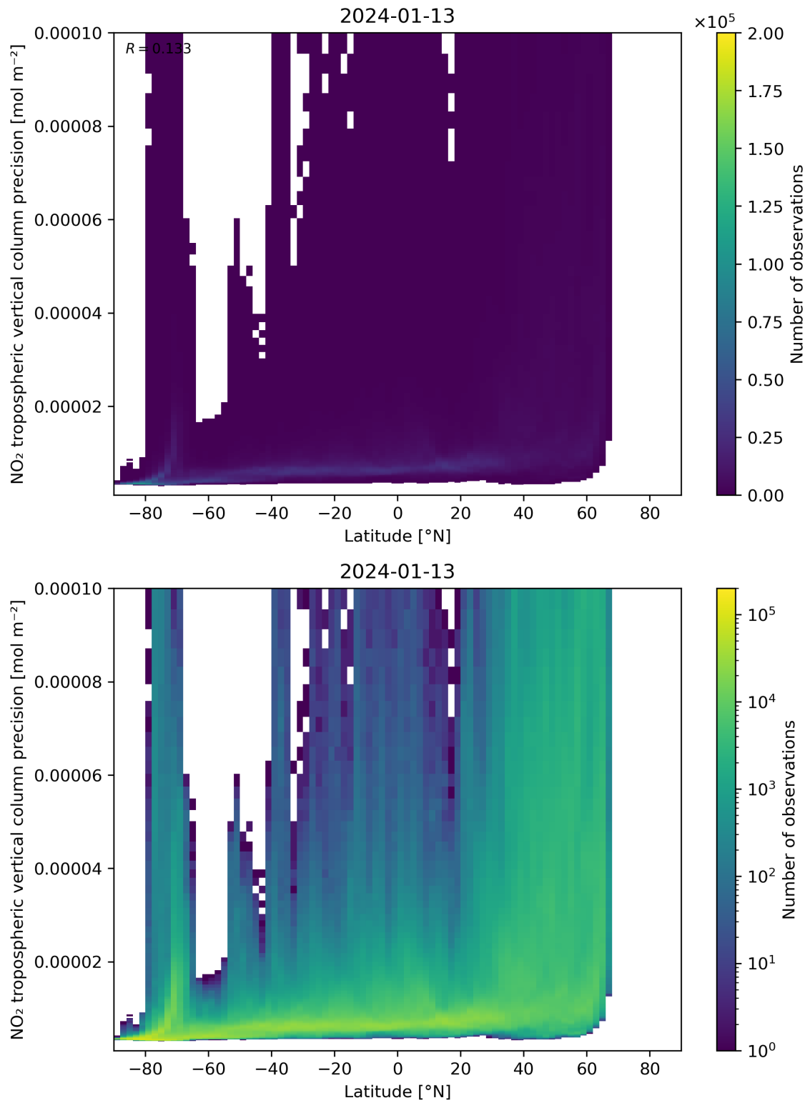
Figure 93: Scatter density plot of “Latitude” against “NO 2 tropospheric vertical column precision” for 2024-01-12 to 2024-01-14.
