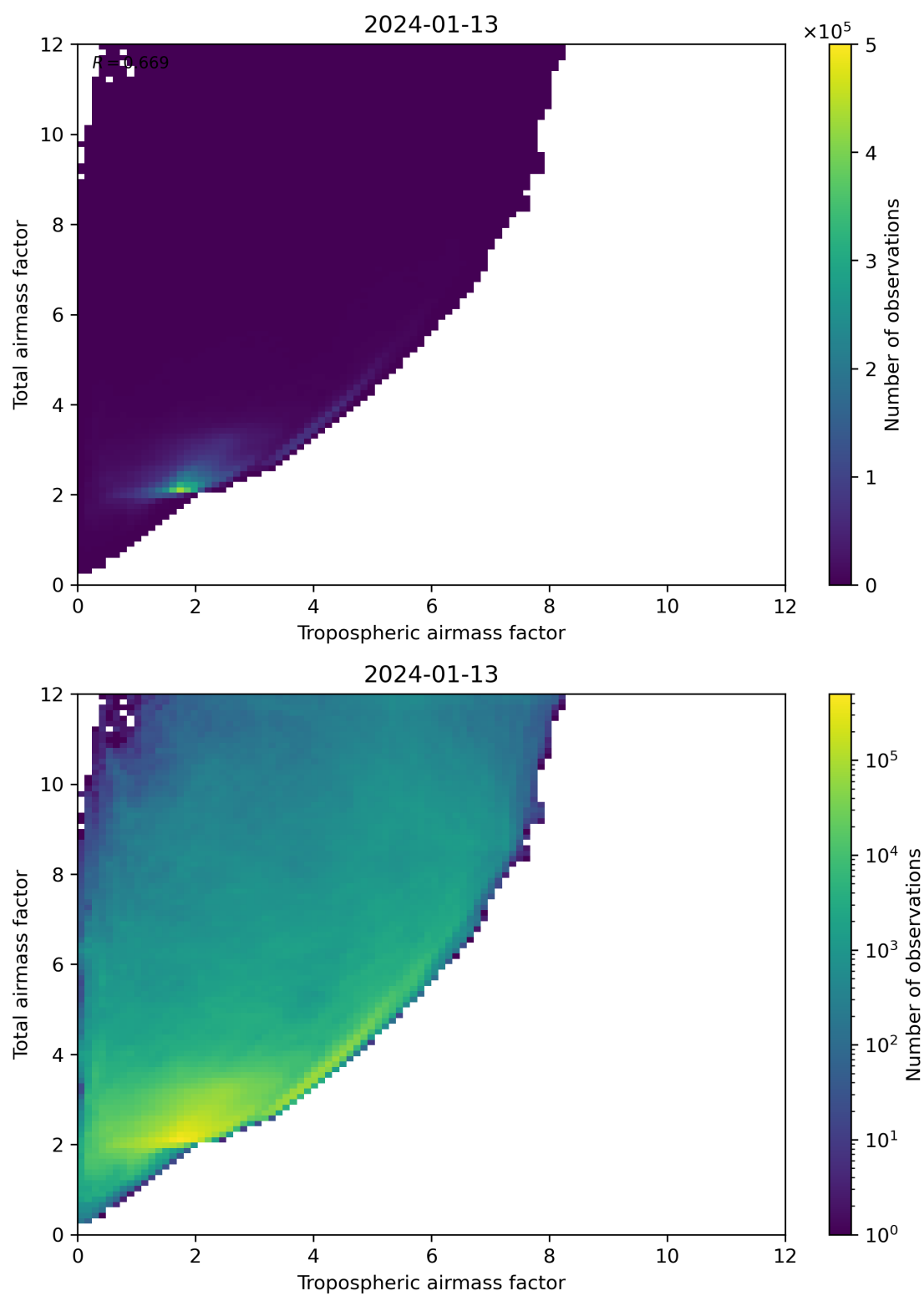
Figure 72: Scatter density plot of “Tropospheric airmass factor” against “Total airmass factor” for 2024-01-12 to 2024-01-14.
