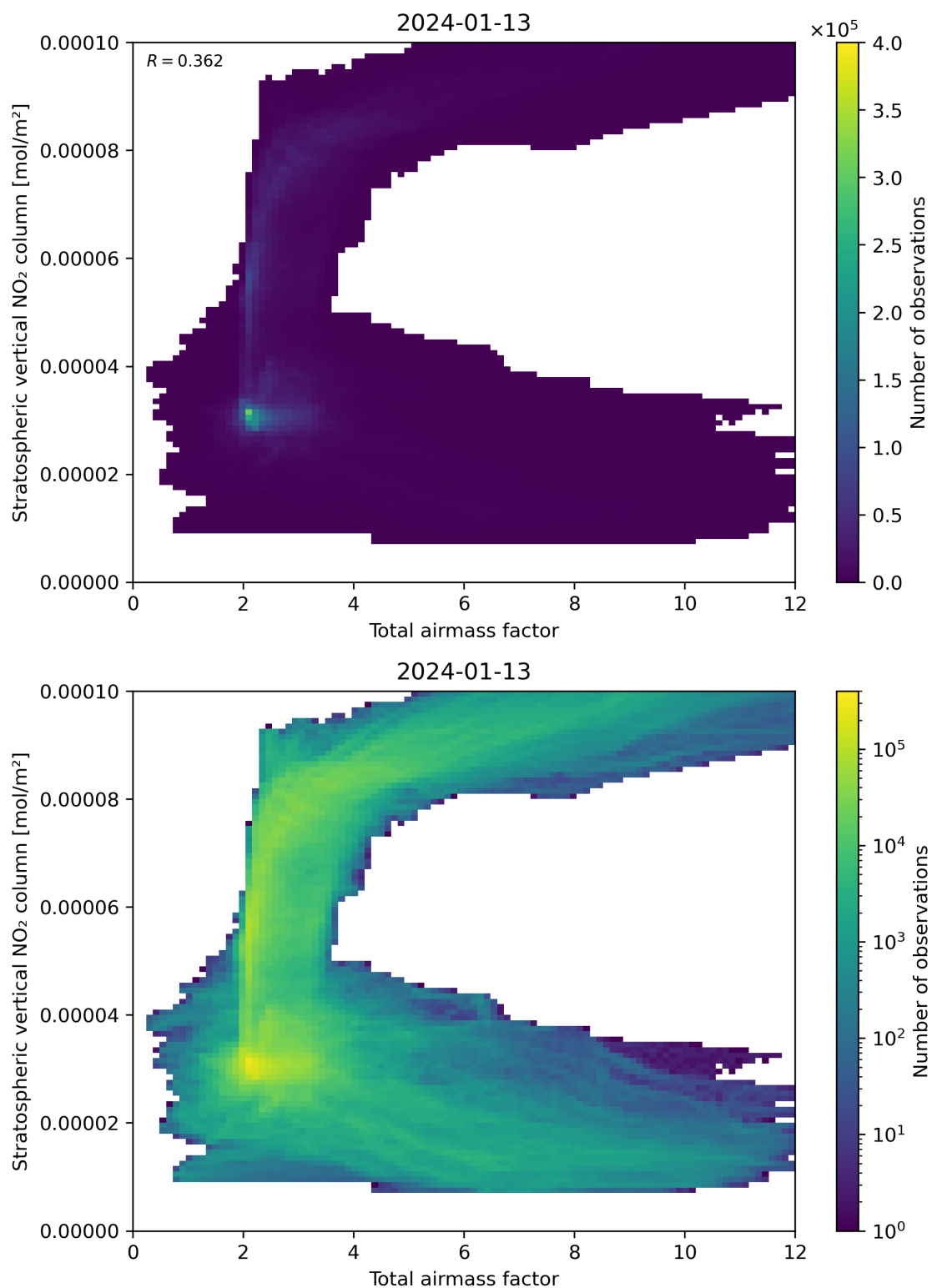
Figure 64: Scatter density plot of “Total airmass factor” against “Stratospheric vertical NO 2 column” for 2024-01-12 to 2024-01-14.
