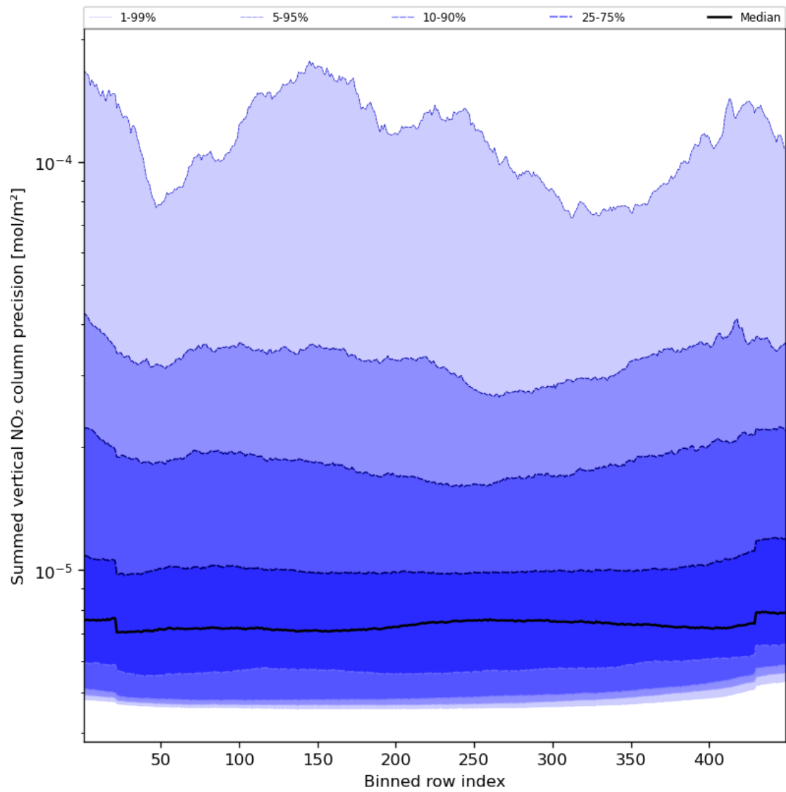
Figure 58: Along track statistics of “Summed vertical NO 2 column precision” for 2024-01-12 to 2024-01-14
