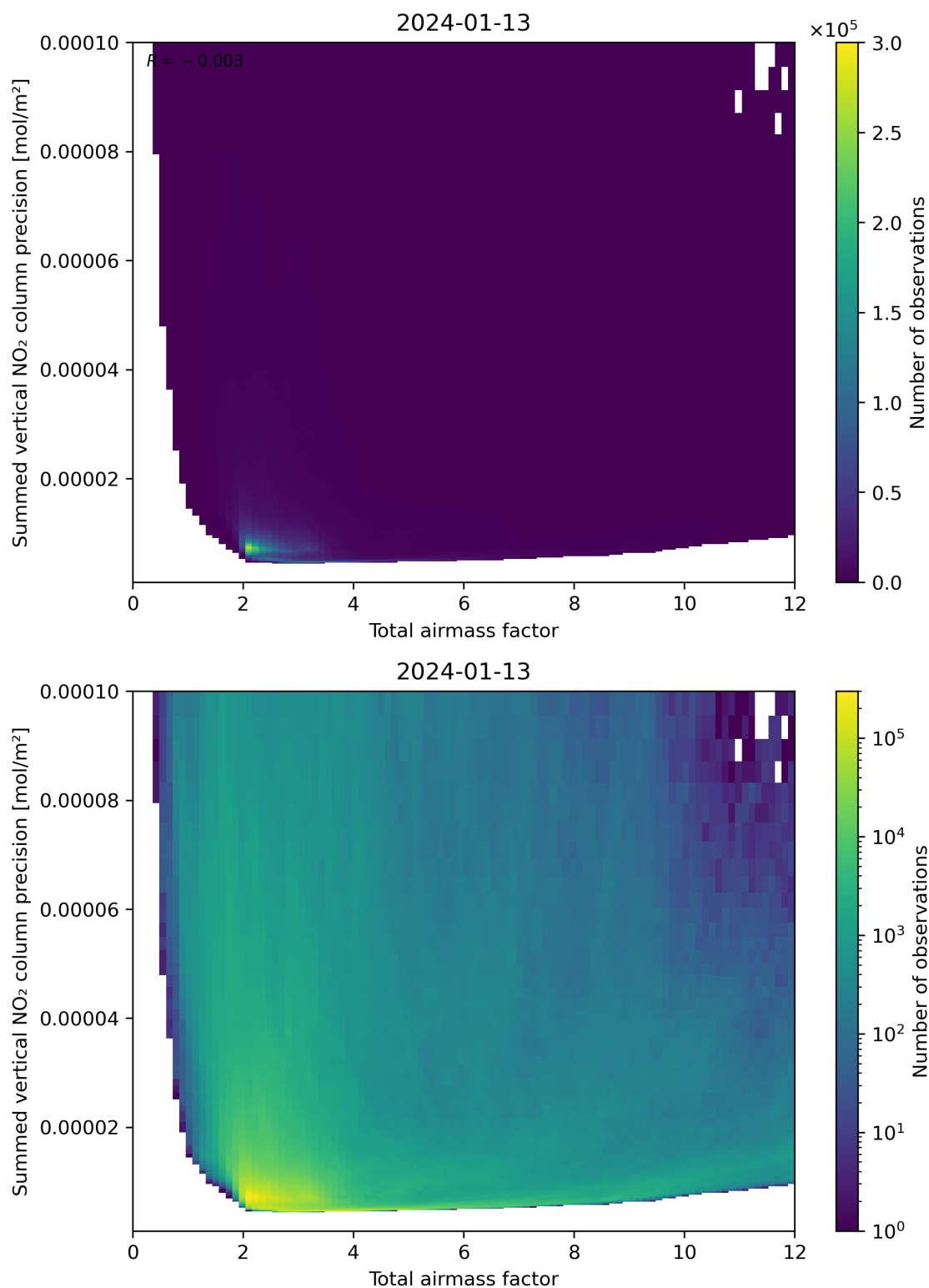
Figure 66: Scatter density plot of “Total airmass factor” against “Summed vertical NO 2 column precision” for 2024-01-12 to 2024-01-14.
