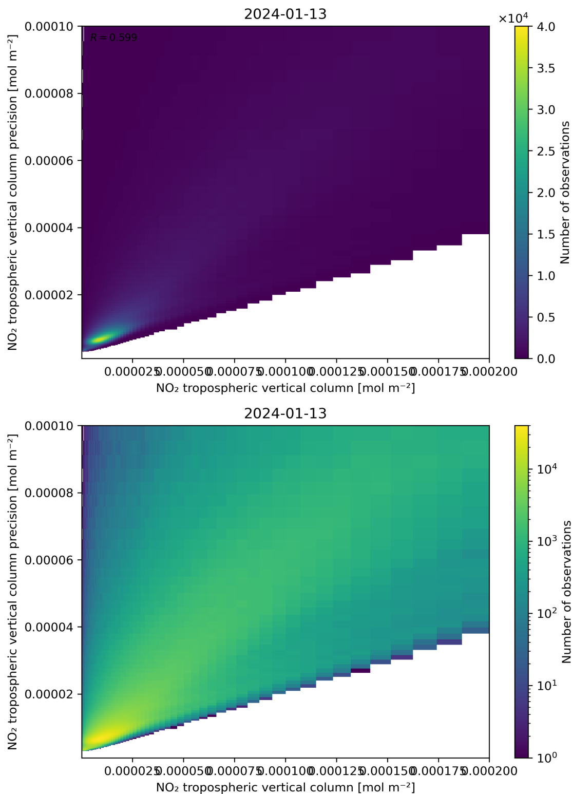
Figure 130: Scatter density plot of “NO 2 tropospheric vertical column” against “NO 2 tropospheric vertical column precision” for 2024-01-12 to 2024-01-14.
