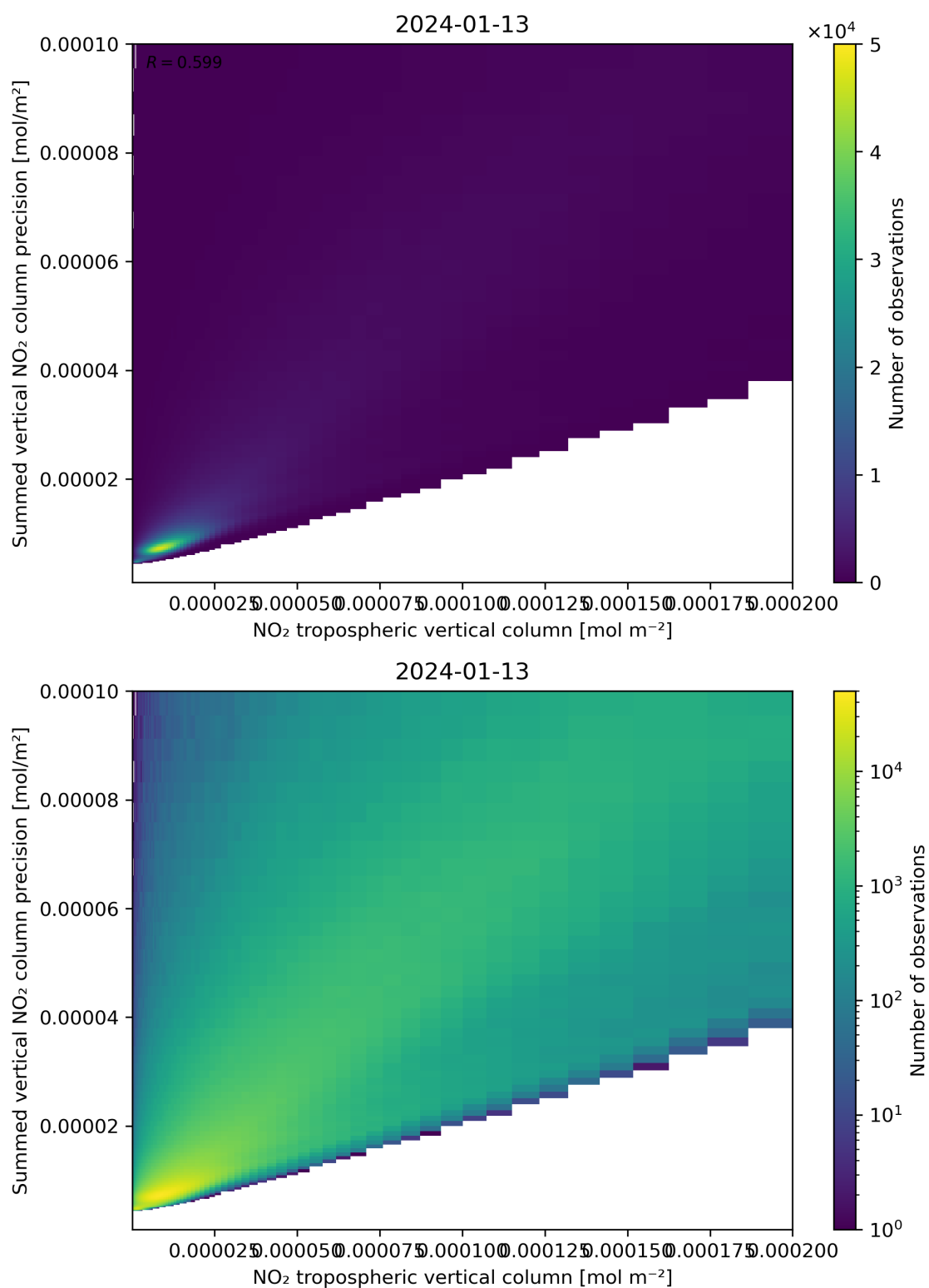
Figure 127: Scatter density plot of “NO 2 tropospheric vertical column” against “Summed vertical NO 2 column precision” for 2024-01-12 to 2024-01-14.
