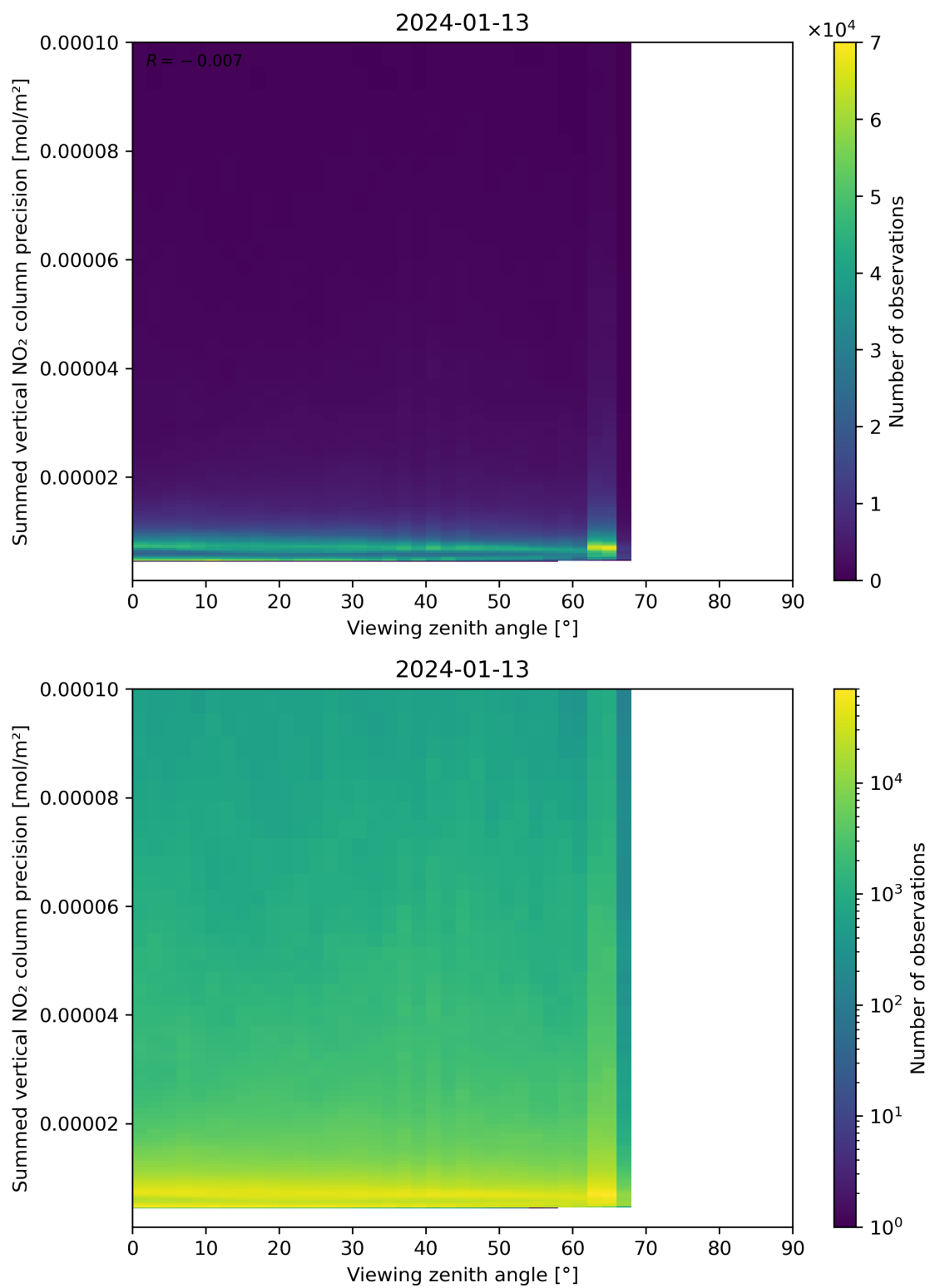
Figure 166: Scatter density plot of “Viewing zenith angle” against “Summed vertical NO 2 column precision” for 2024-01-12 to 2024-01-14.
