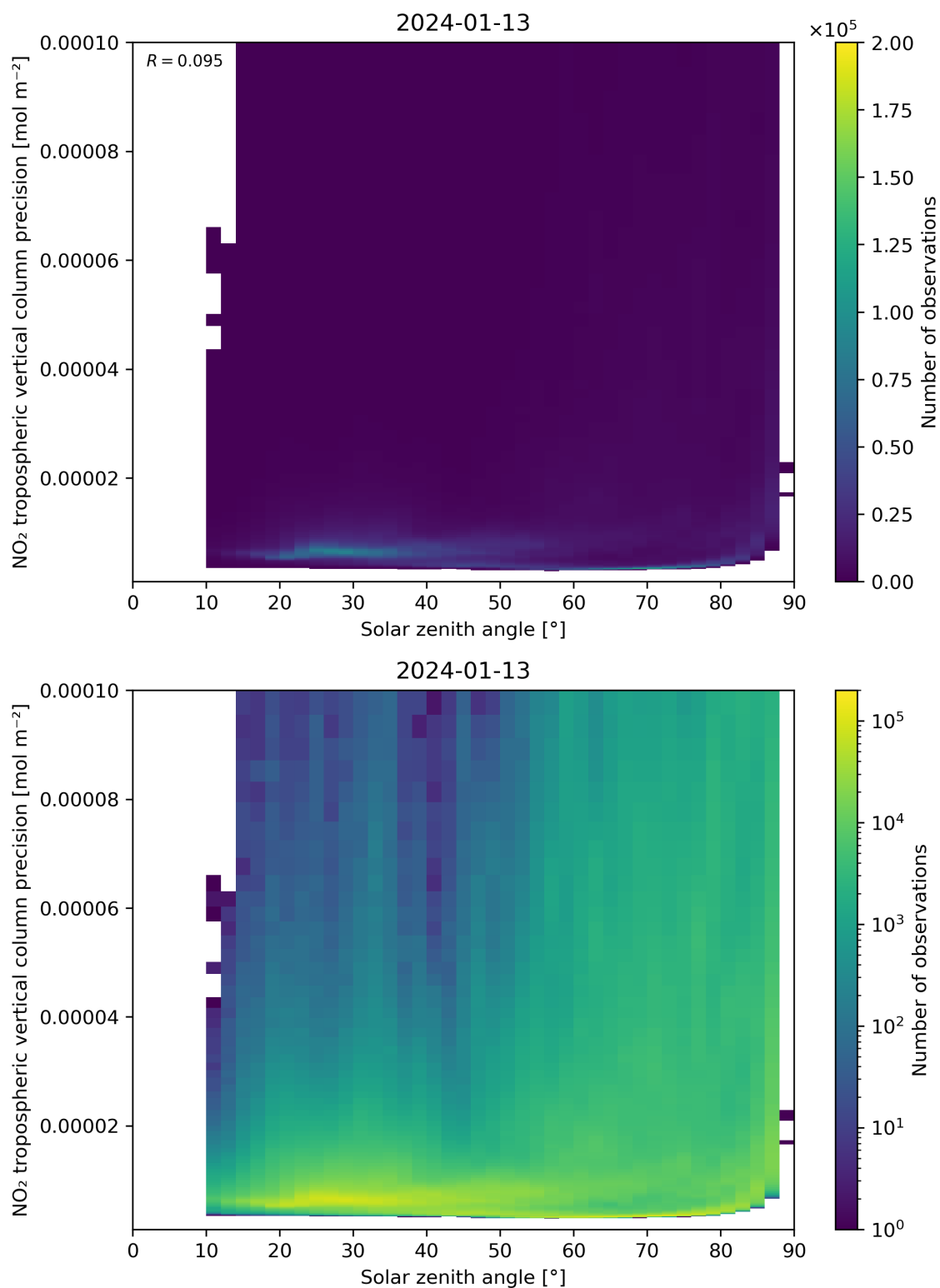
Figure 156: Scatter density plot of “Solar zenith angle” against “NO 2 tropospheric vertical column precision” for 2024-01-12 to 2024-01-14.
