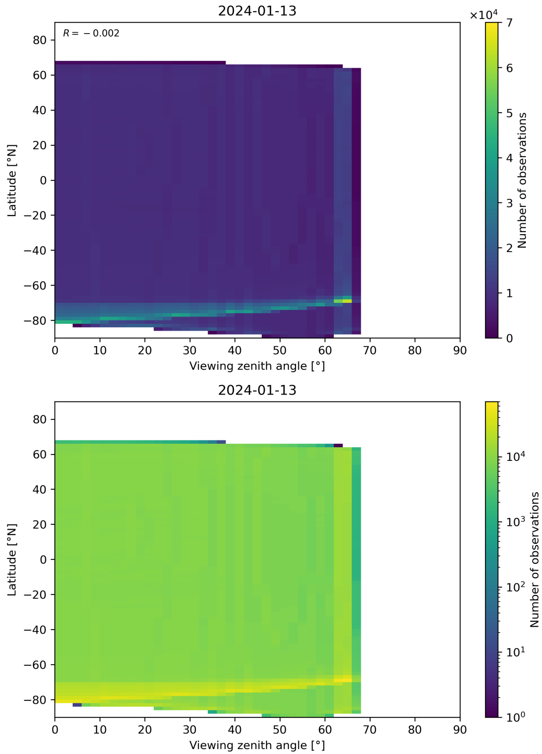
Figure 163: Scatter density plot of “Viewing zenith angle” against “Latitude” for 2024-01-12 to 2024-01-14.
