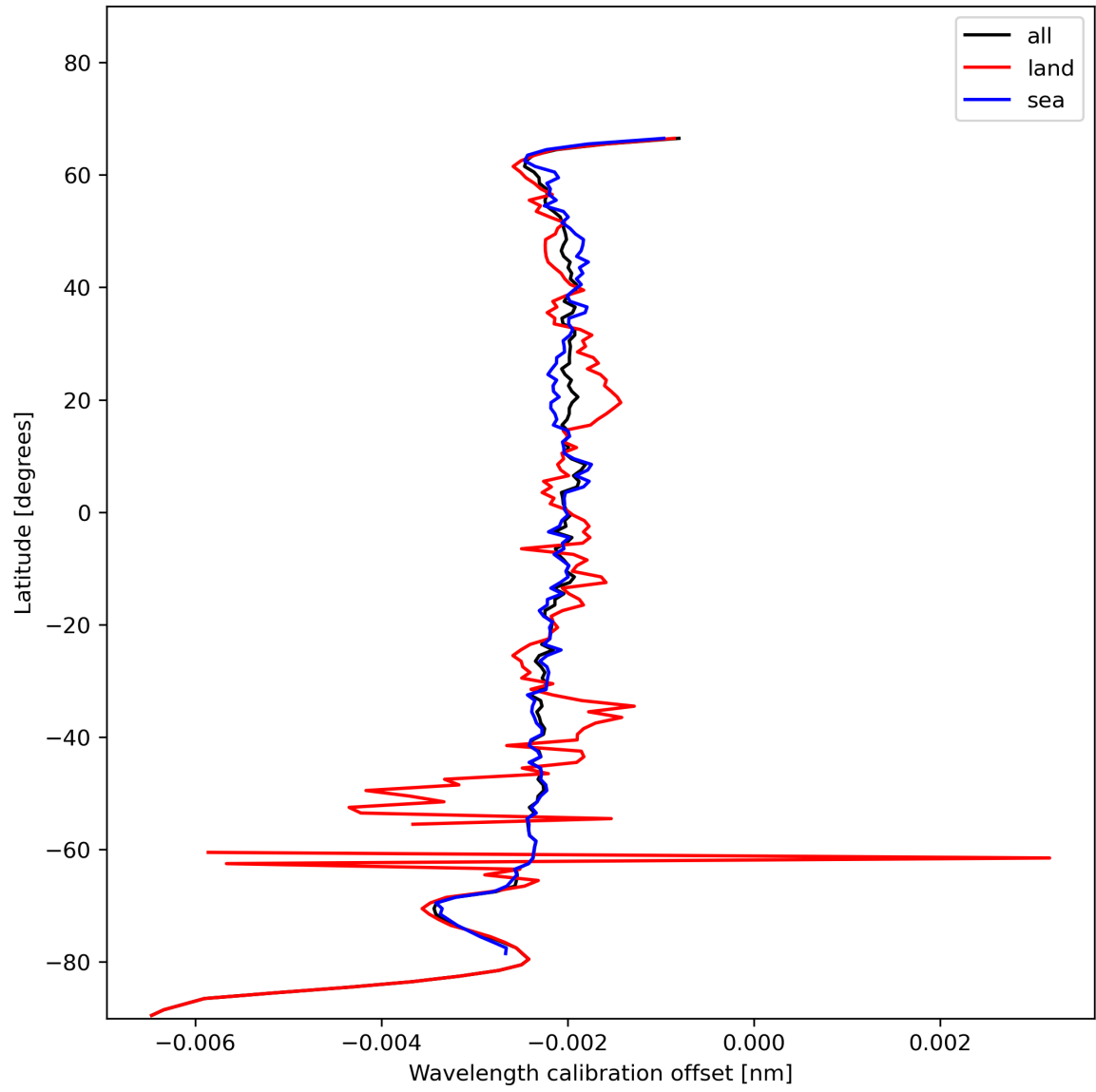
Figure 18: Zonal average of “Wavelength calibration offset” for 2024-01-12 to 2024-01-14.
