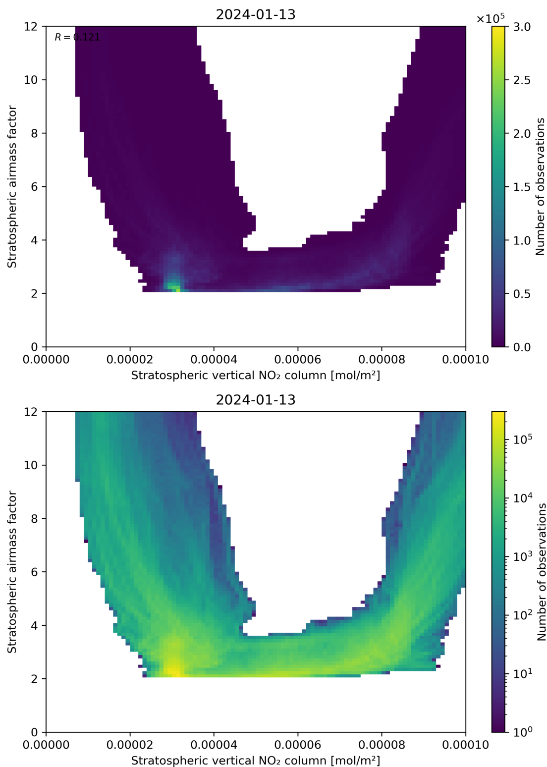
Figure 96: Scatter density plot of “Stratospheric vertical NO 2 column” against “Stratospheric airmass factor” for 2024-01-12 to 2024-01-14.
