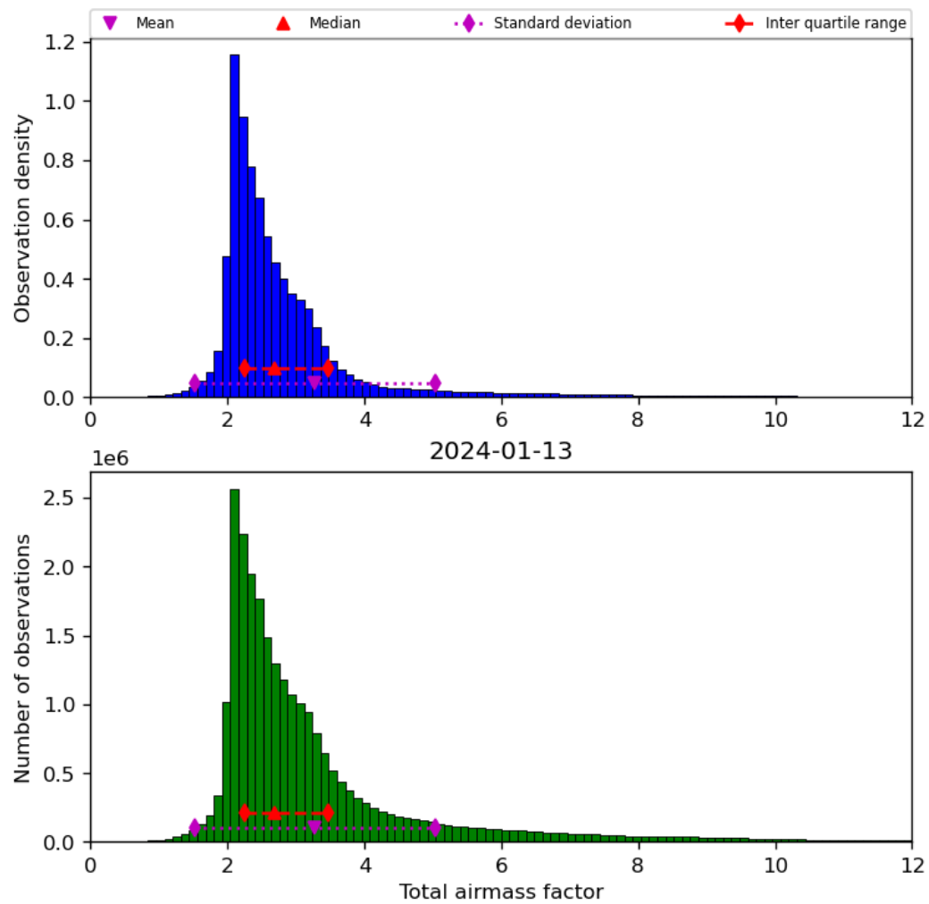
Figure 32: Histogram of “Total airmass factor” for 2024-01-12 to 2024-01-14
