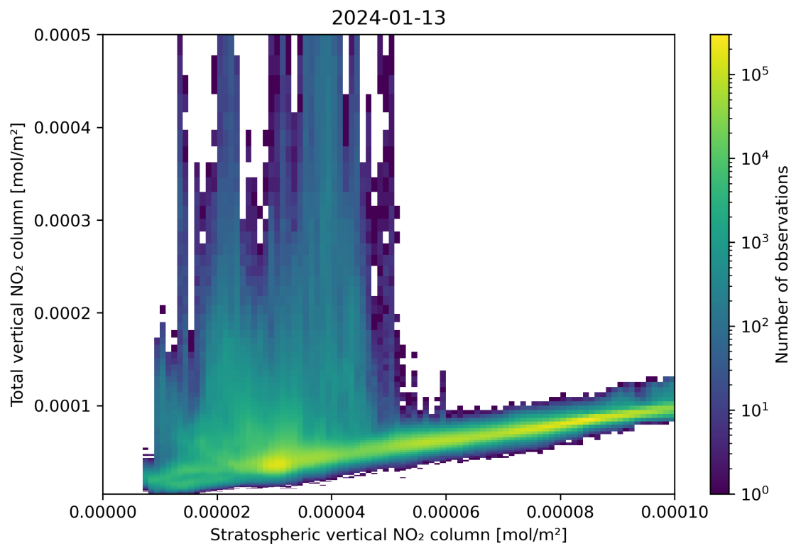
Figure 100: Scatter density plot of “Stratospheric vertical NO 2 column” against “Total vertical NO 2 column” for 2024-01-12 to 2024-01-14.
