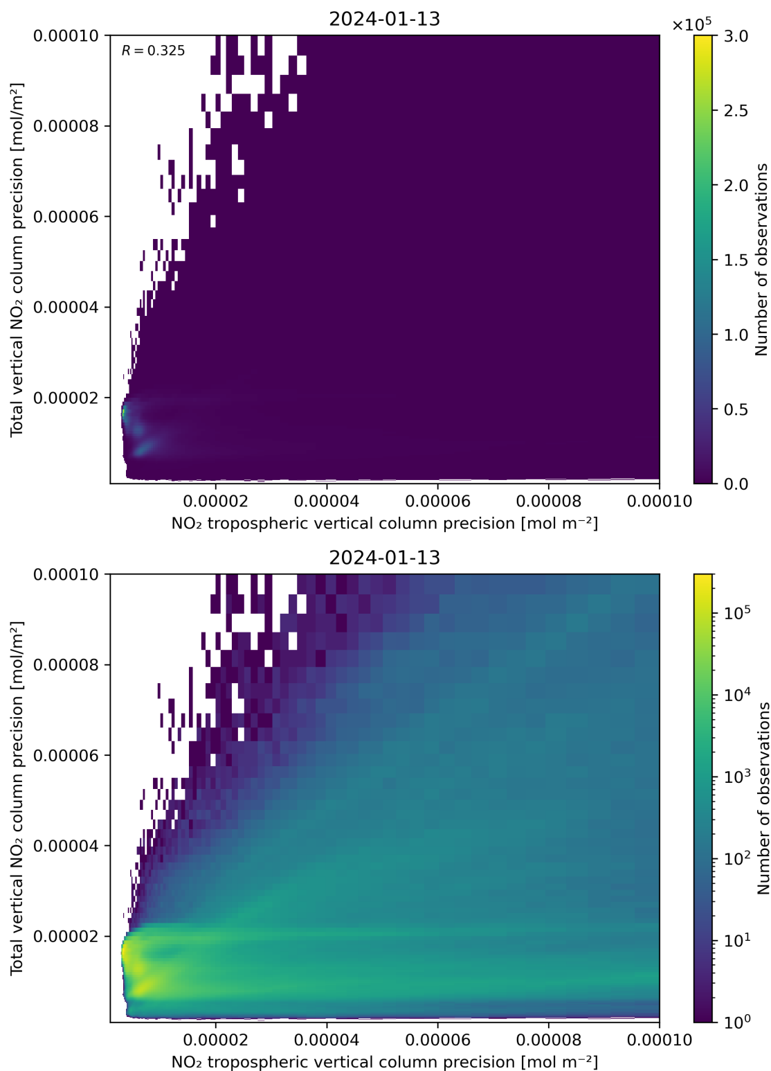
Figure 139: Scatter density plot of “NO 2 tropospheric vertical column precision” against “Total vertical NO 2 column precision” for 2024-01-12 to 2024-01-14.
