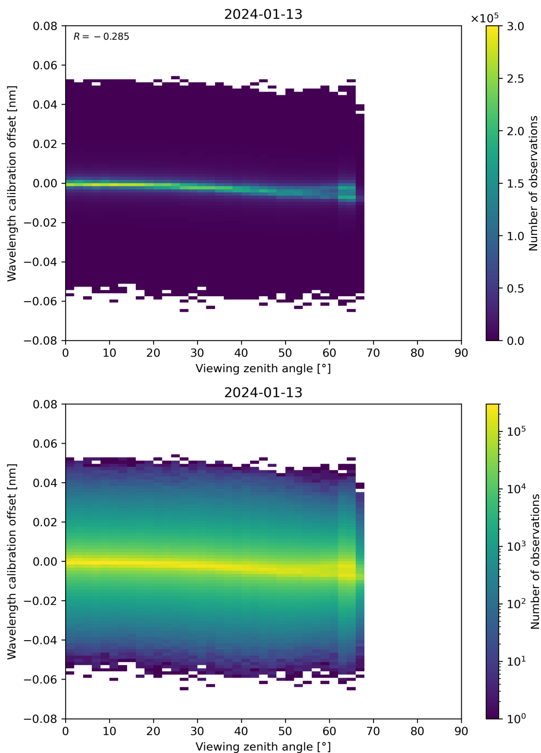
Figure 173: Scatter density plot of “Viewing zenith angle” against “Wavelength calibration offset” for 2024-01-12 to 2024-01-14.
