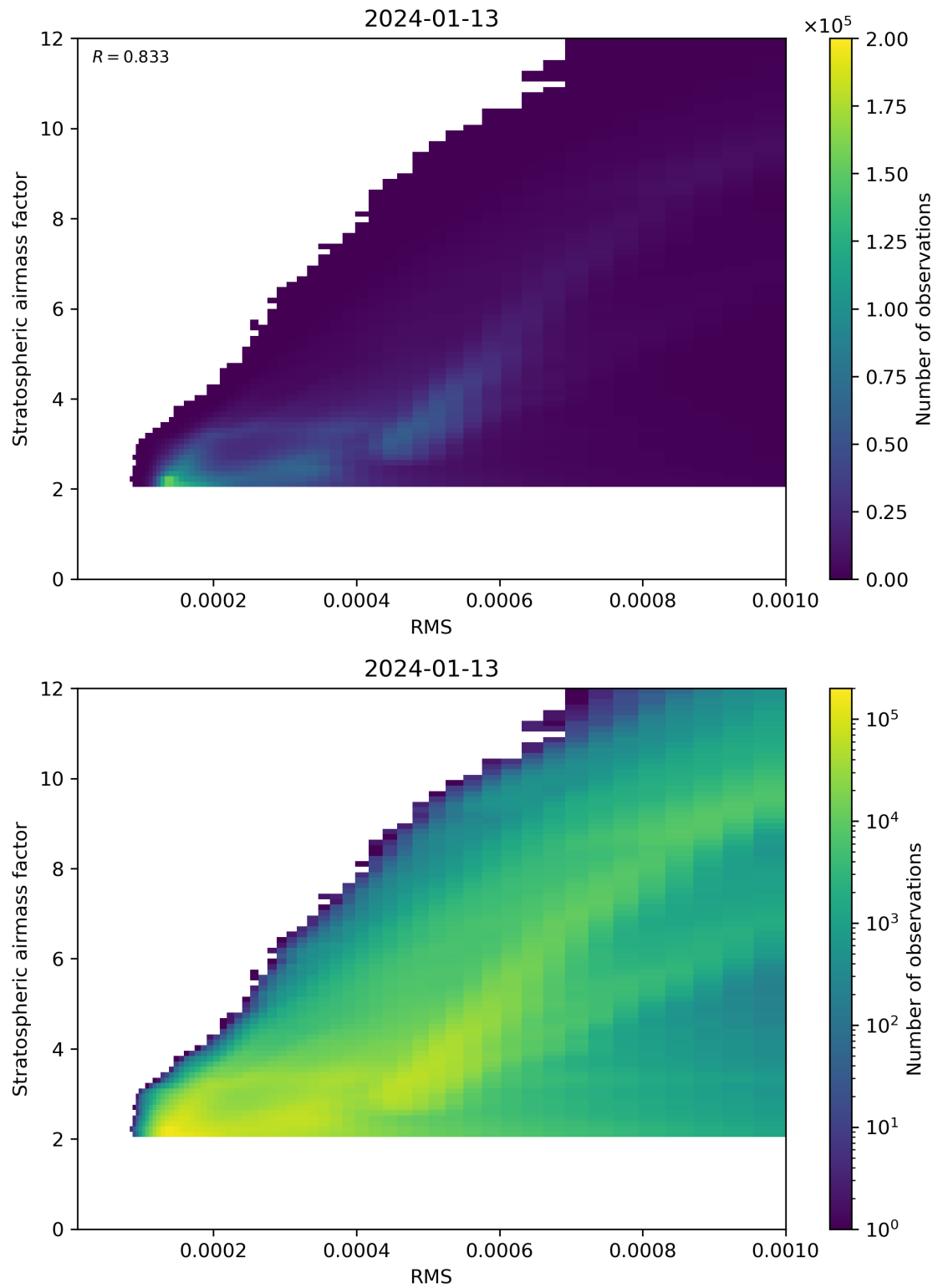
Figure 144: Scatter density plot of “RMS” against “Stratospheric airmass factor” for 2024-01-12 to 2024-01-14.
