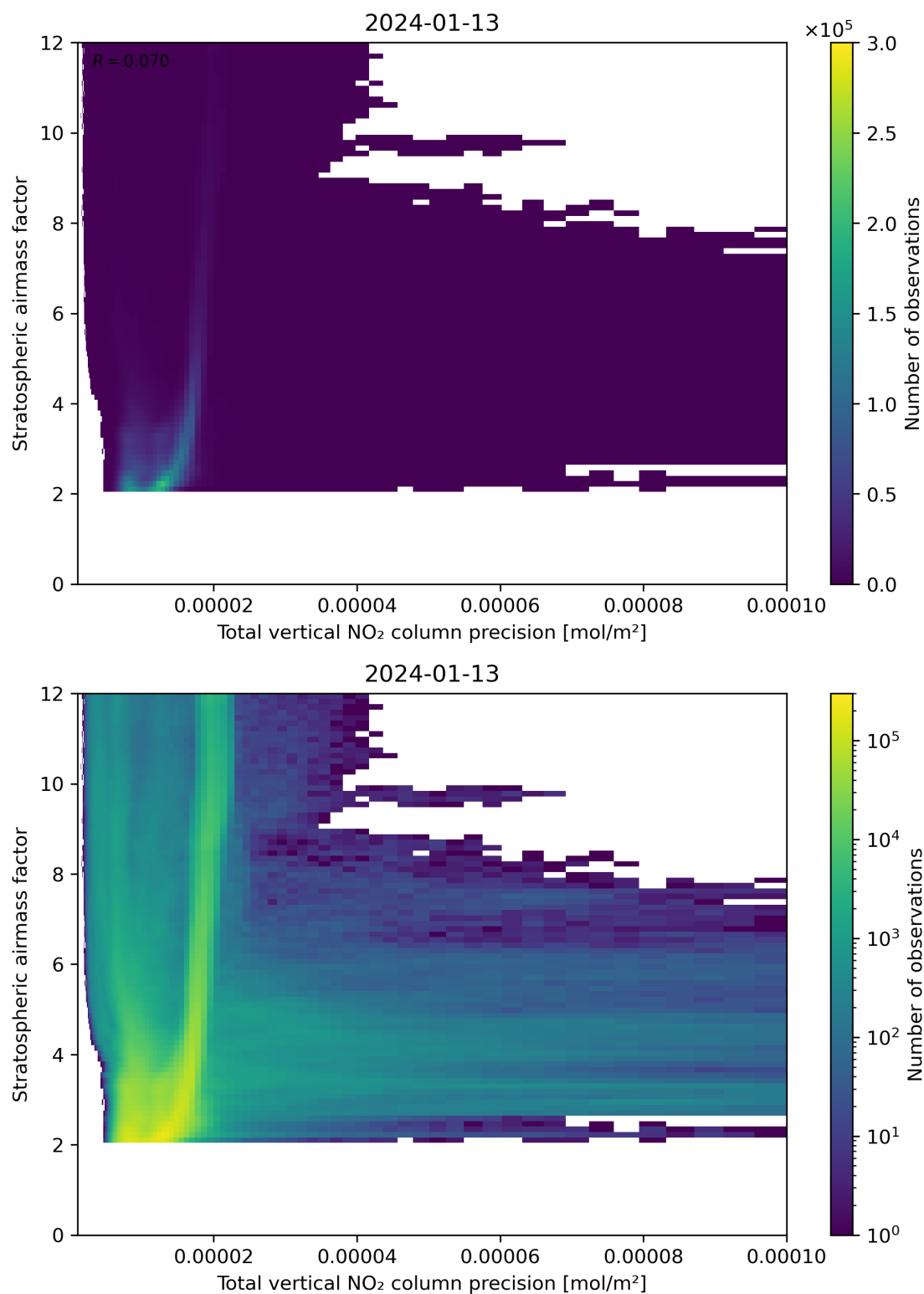
Figure 115: Scatter density plot of “Total vertical NO 2 column precision” against “Stratospheric air mass factor” for 2024-01-12 to 2024-01-14.
