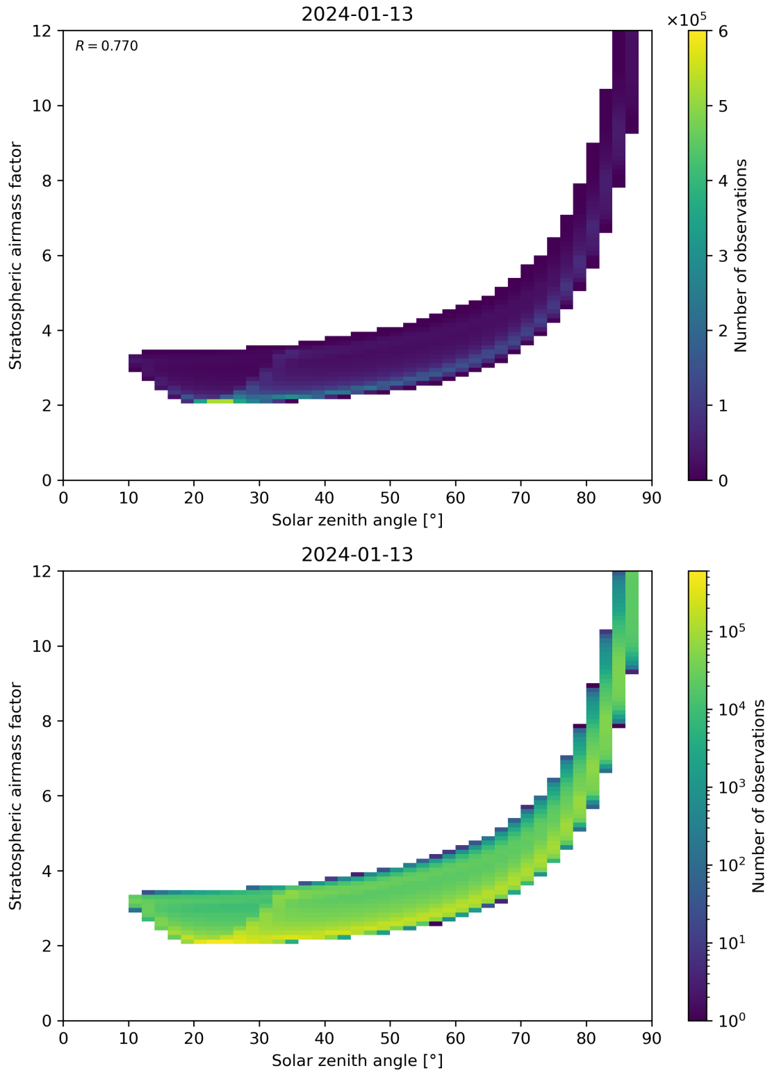
Figure 145: Scatter density plot of “Solar zenith angle” against “Stratospheric airmass factor” for 2024-01-12 to 2024-01-14.
